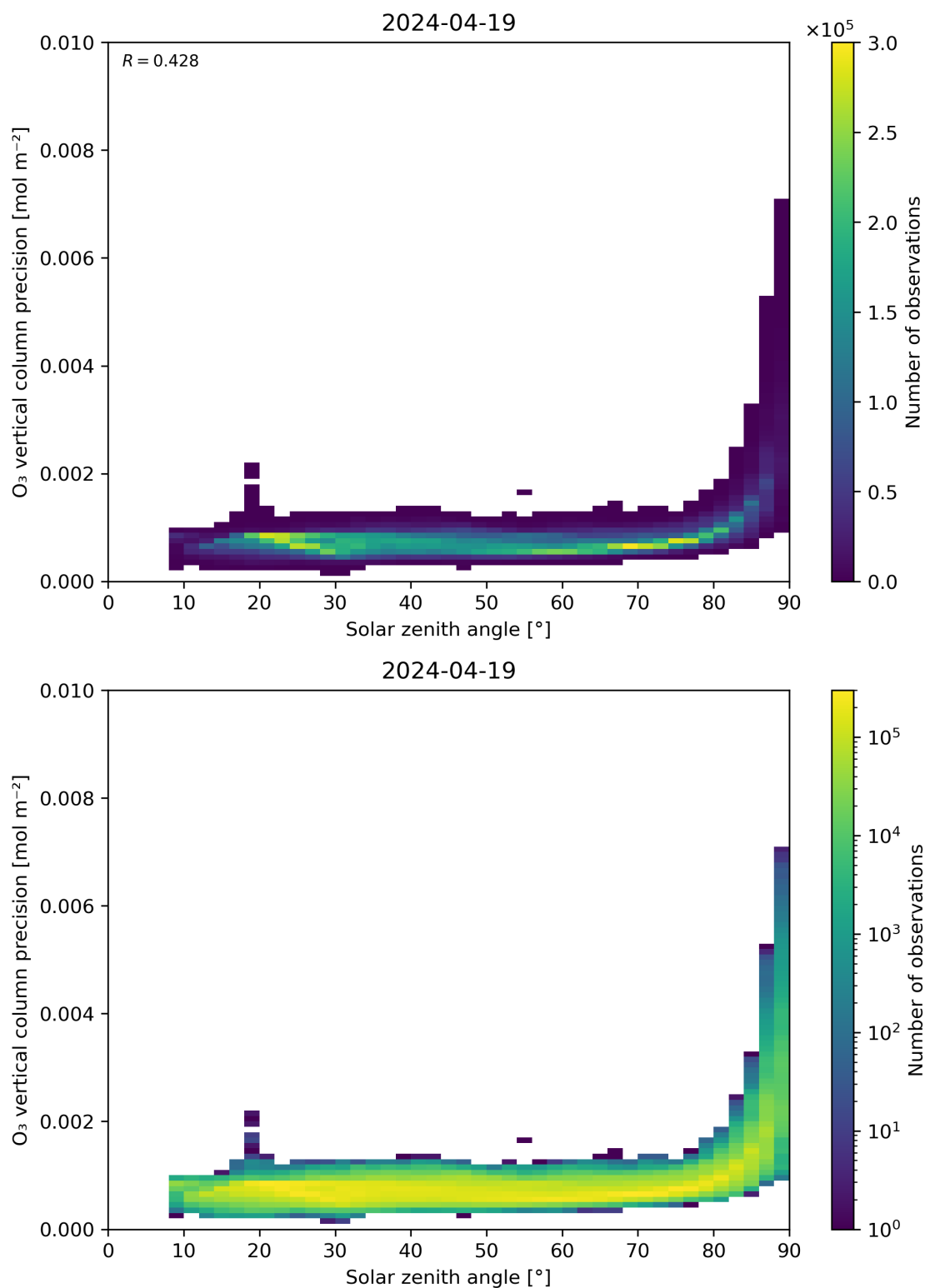
Figure 48: Scatter density plot of “Solar zenith angle” against “O 3 vertical column precision” for 2024-04-18 to 2024-04-20.
