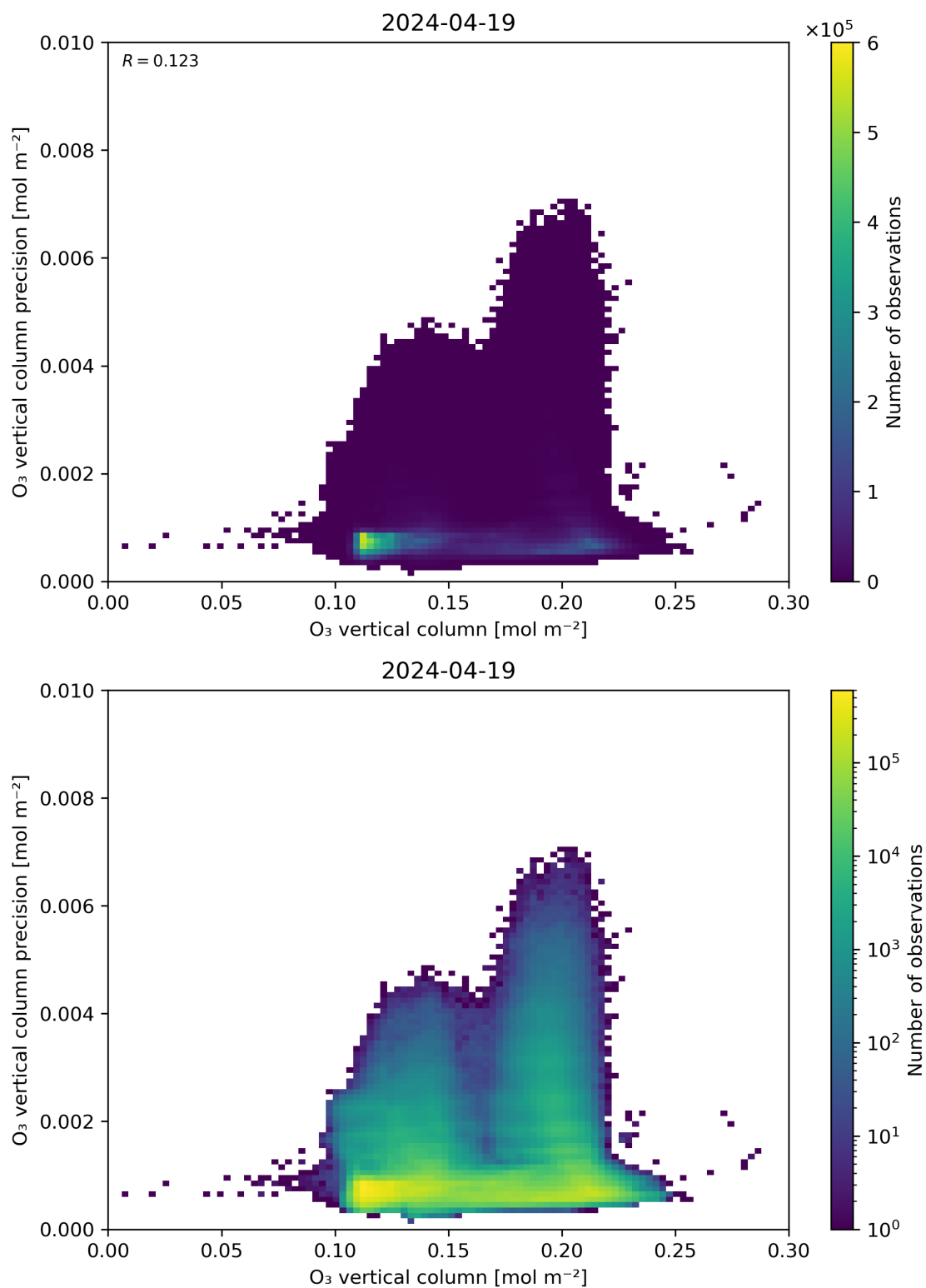
Figure 41: Scatter density plot of “O 3 vertical column” against “O 3 vertical column precision” for 2024-04-18 to 2024-04-20.
