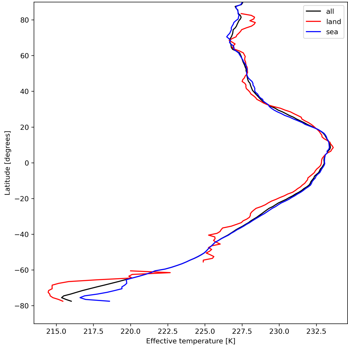
Figure 17: Zonal average of "Effective temperature" for 2024-04-18 to 2024-04-20.
