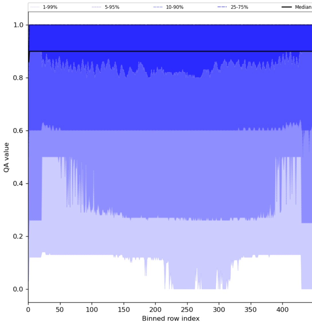
Figure 27: Along track statistics of “QA value” for 2024-04-18 to 2024-04-20
