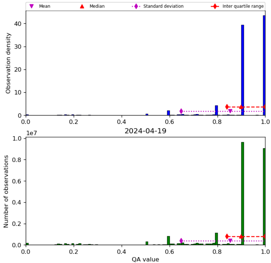
Figure 20: Histogram of “QA value” for 2024-04-18 to 2024-04-20
