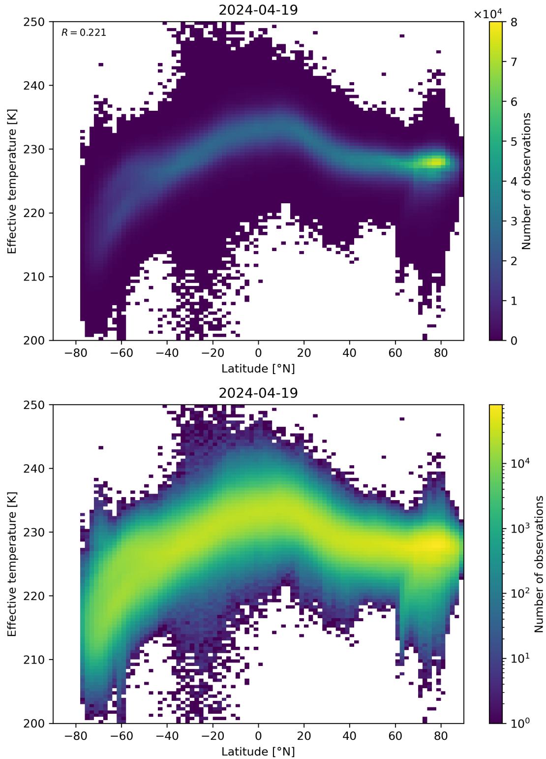
Figure 34: Scatter density plot of “Latitude” against “Effective temperature” for 2024-04-18 to 2024-04-20.
