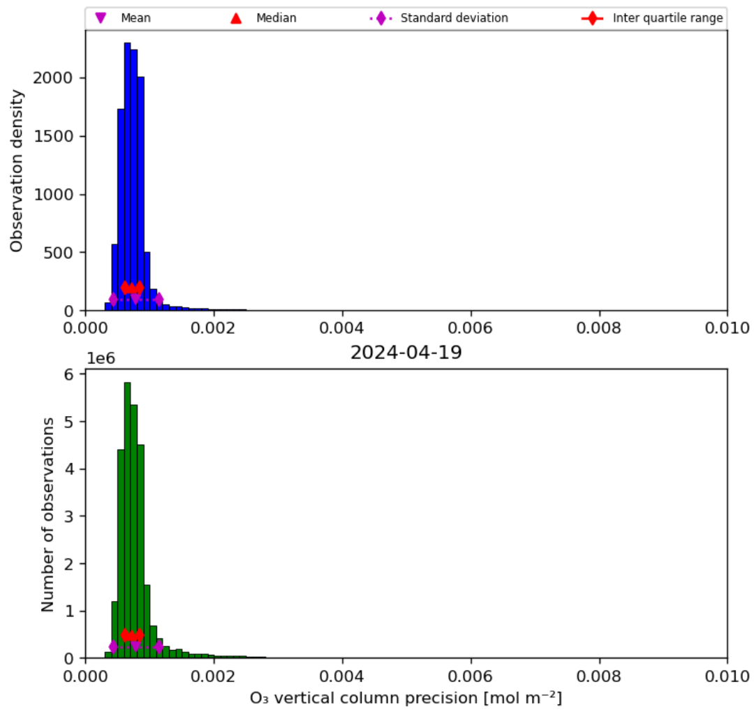
Figure 22: Histogram of “O 3 vertical column precision” for 2024-04-18 to 2024-04-20
