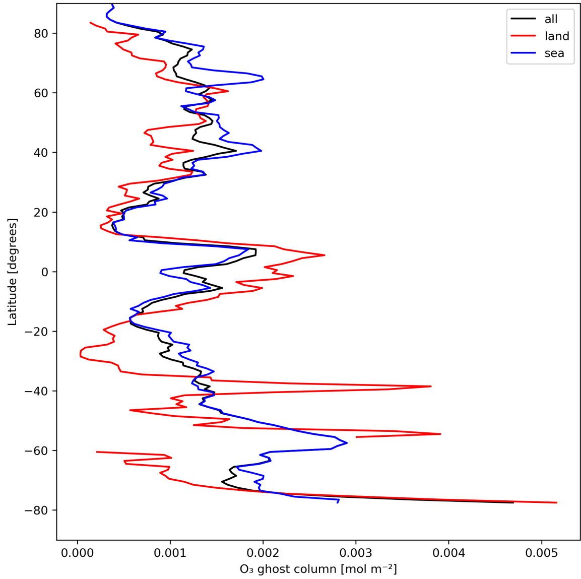
Figure 18: Zonal average of "O 3 ghost column" for 2024-04-18 to 2024-04-20.
