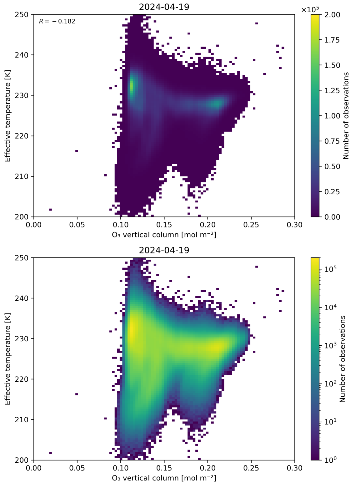
Figure 39: Scatter density plot of “O 3 vertical column” against “Effective temperature” for 2024-04-18 to 2024-04-20.
