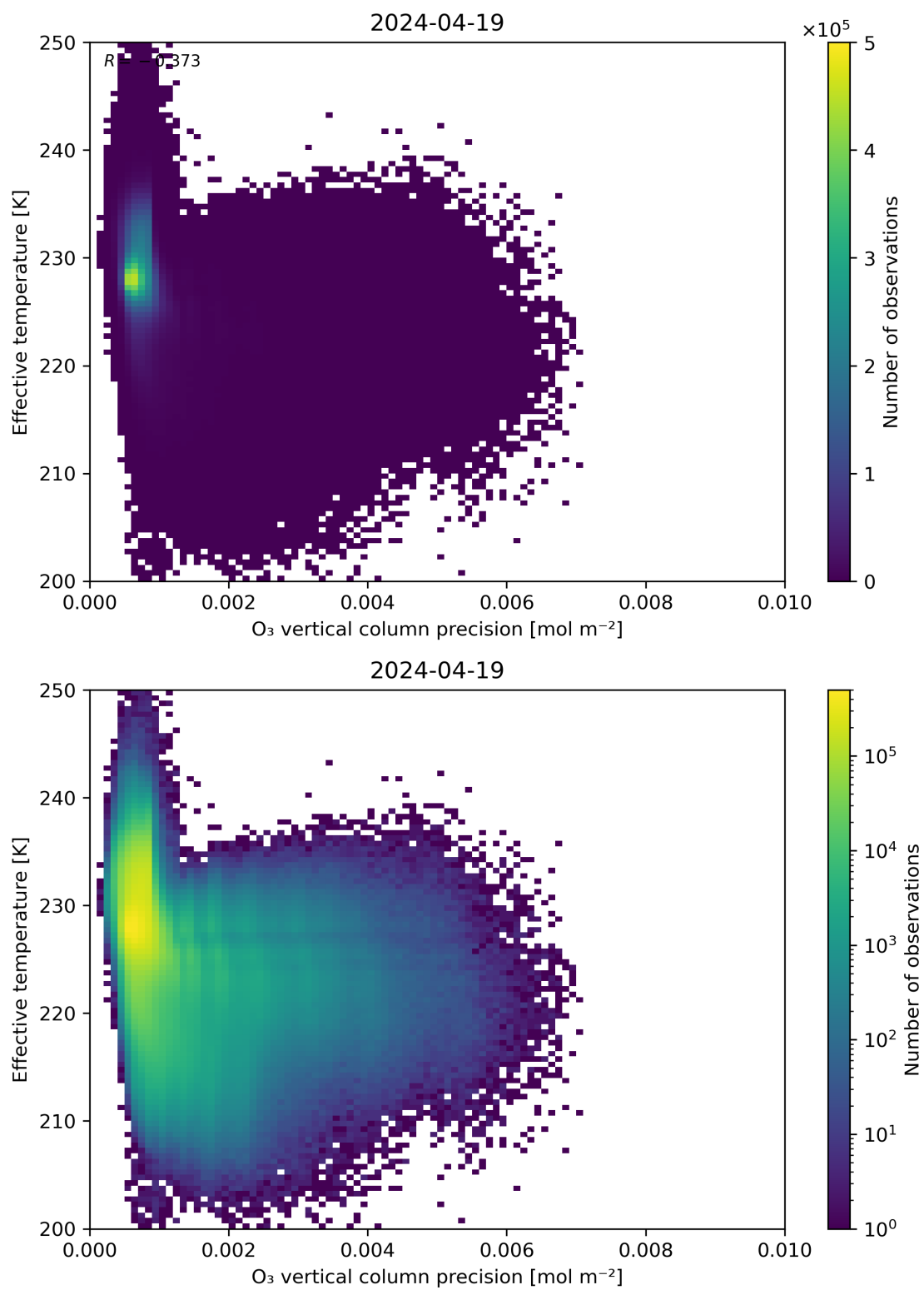
Figure 42: Scatter density plot of “O 3 vertical column precision” against “Effective temperature” for 2024-04-18 to 2024-04-20.
