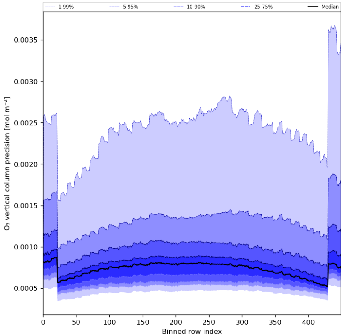
Figure 29: Along track statistics of “O 3 vertical column precision” for 2024-04-18 to 2024-04-20
