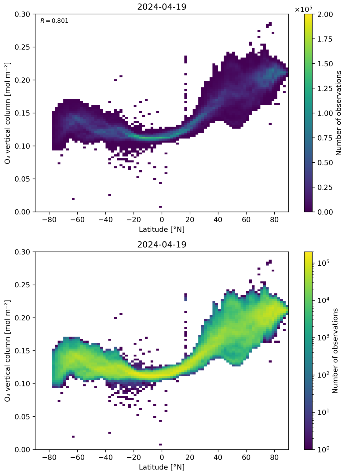
Figure 36: Scatter density plot of “Latitude” against “O 3 vertical column” for 2024-04-18 to 2024-04-20.
