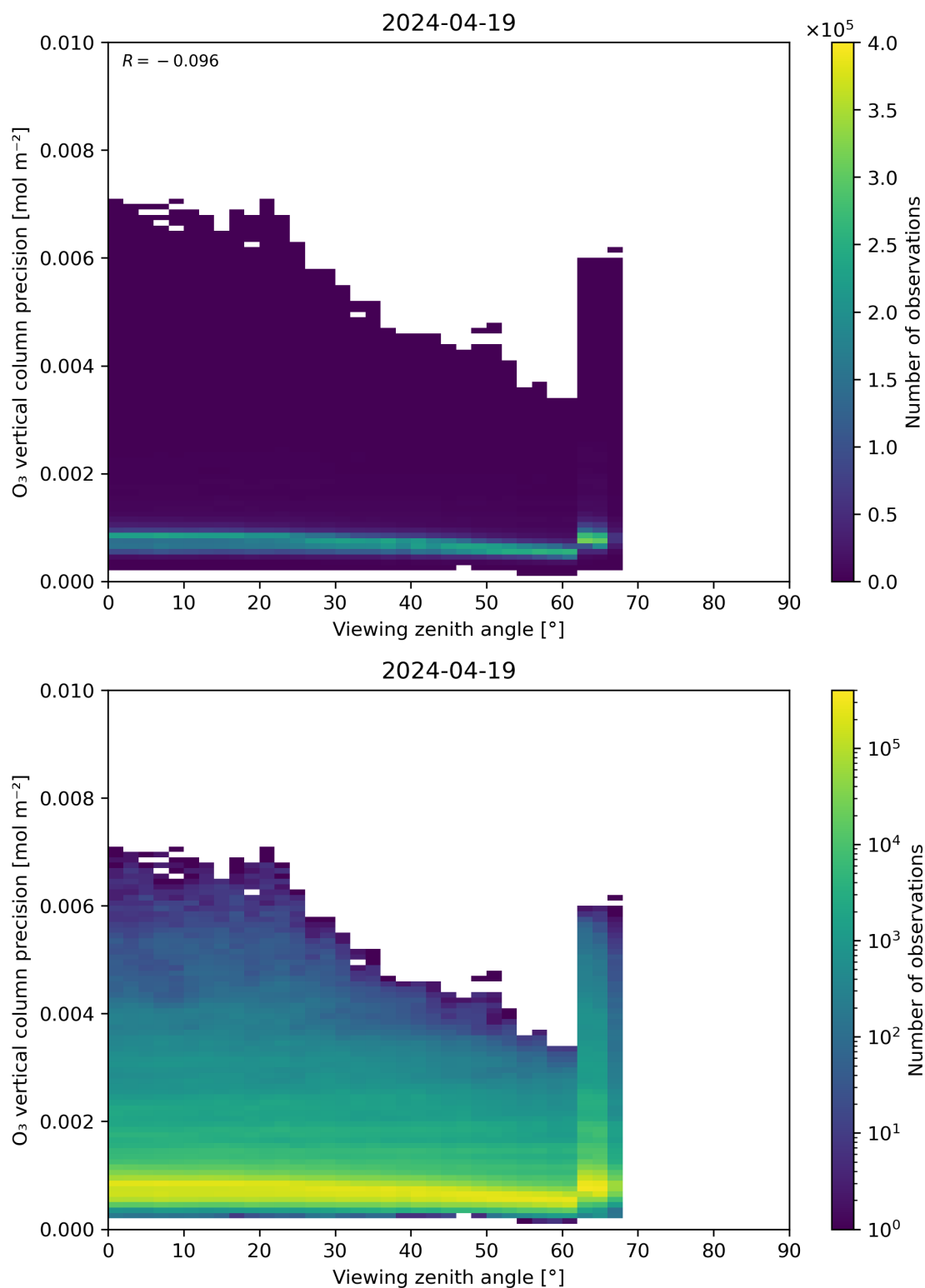
Figure 53: Scatter density plot of “Viewing zenith angle” against “O 3 vertical column precision” for 2024-04-18 to 2024-04-20.
