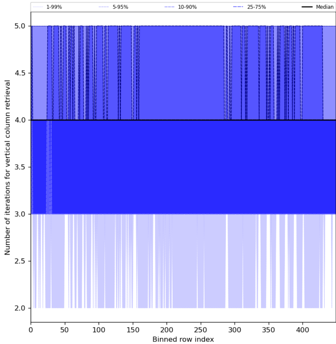
Figure 33: Along track statistics of “Number of iterations for vertical column retrieval” for 2024-04-18 to 2024-04-20
