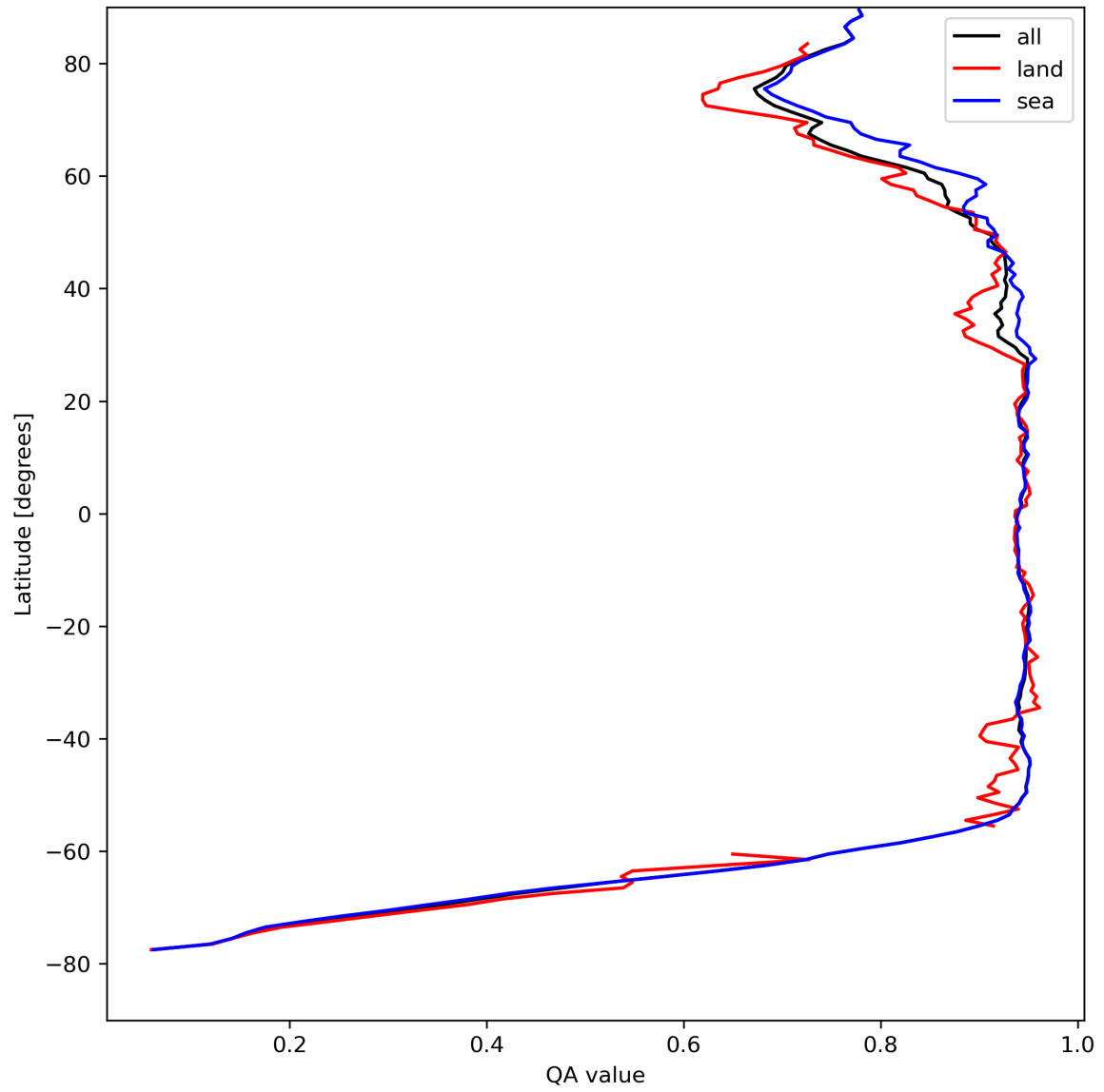
Figure 13: Zonal average of “QA value” for 2024-04-18 to 2024-04-20.
