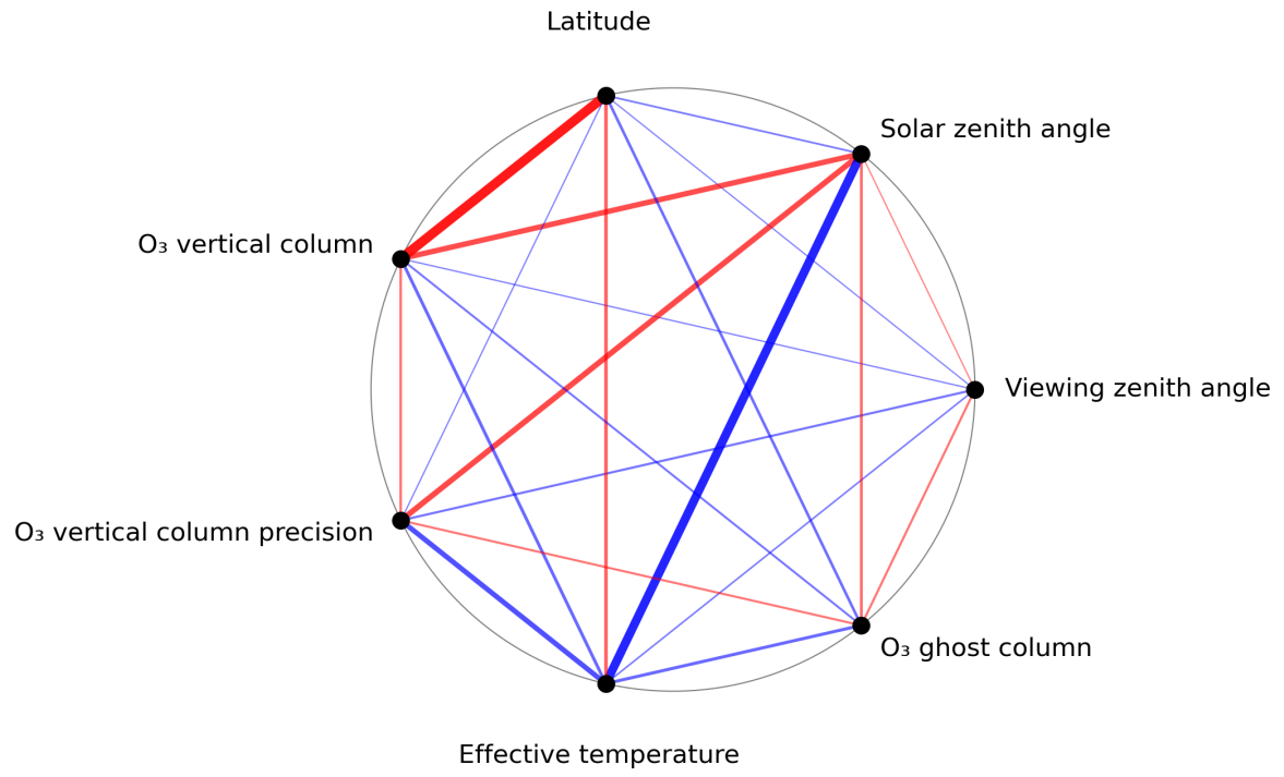
Figure 1: Map of correlation graph for 2024-04-18 to 2024-04-20.
