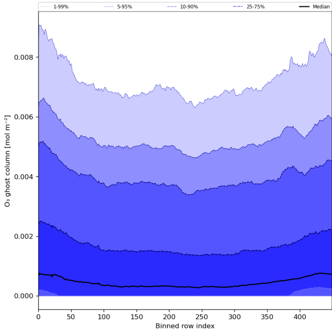
Figure 32: Along track statistics of “O 3 ghost column” for 2024-04-18 to 2024-04-20
