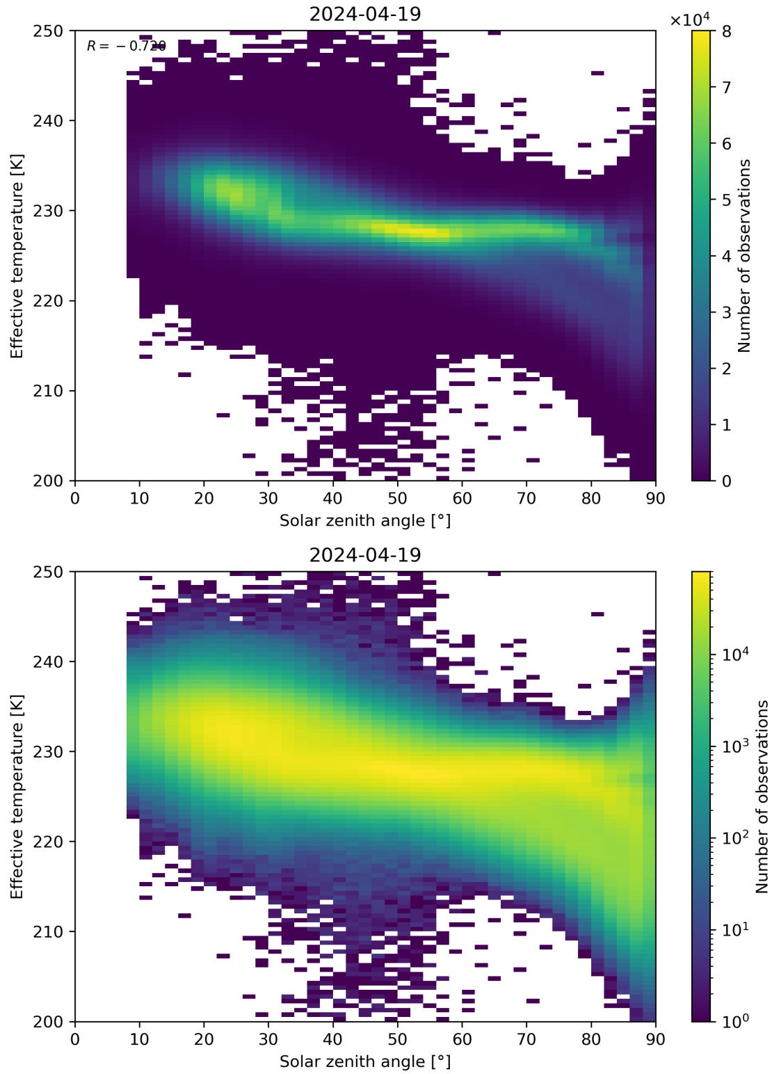
Figure 45: Scatter density plot of “Solar zenith angle” against “Effective temperature” for 2024-04-18 to 2024-04-20.
