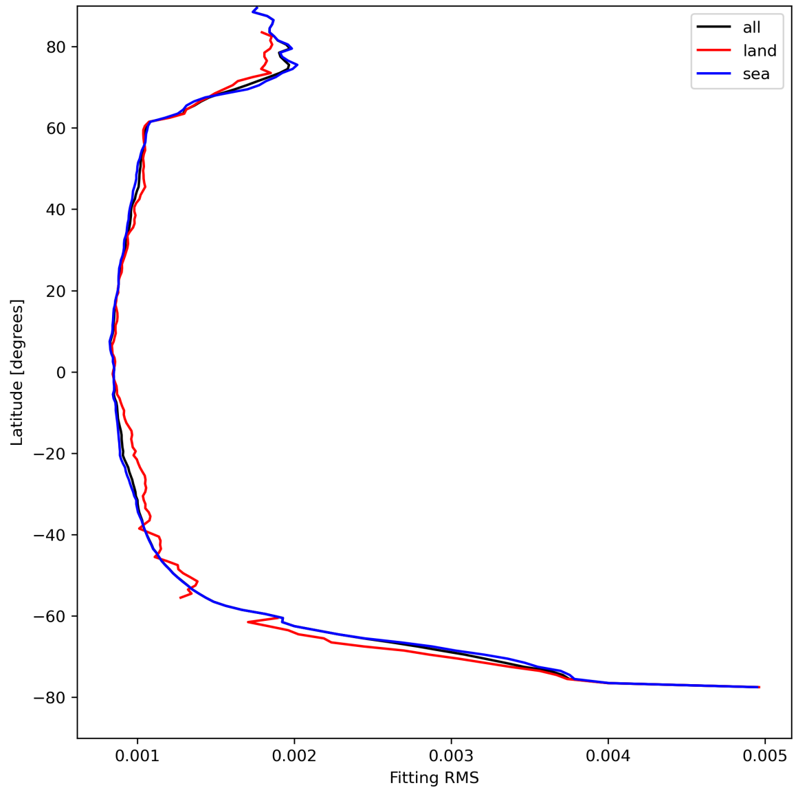
Figure 16: Zonal average of “Fitting RMS” for 2024-04-18 to 2024-04-20.
