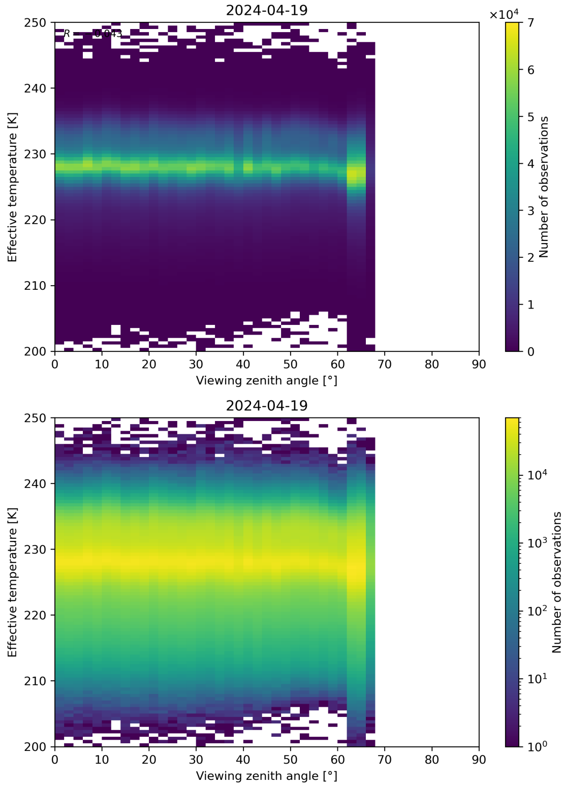
Figure 50: Scatter density plot of “Viewing zenith angle” against “Effective temperature” for 2024-04-18 to 2024-04-20.
