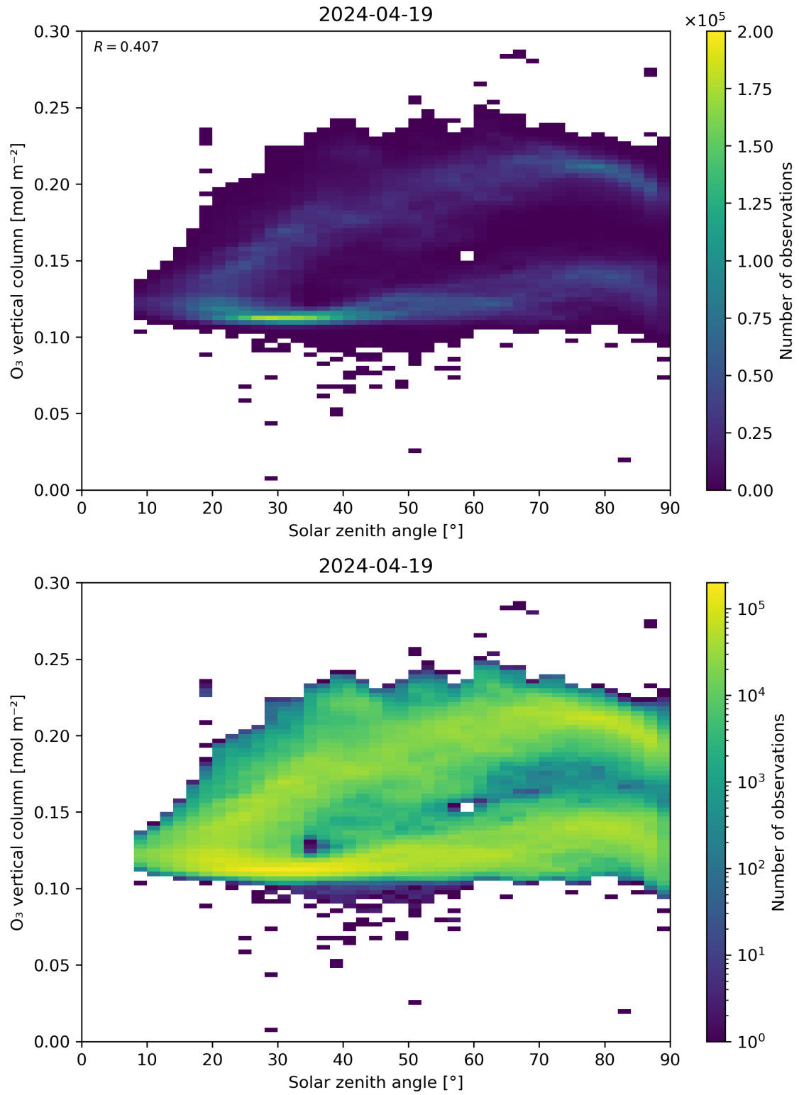
Figure 47: Scatter density plot of “Solar zenith angle” against “O 3 vertical column” for 2024-04-18 to 2024-04-20.
