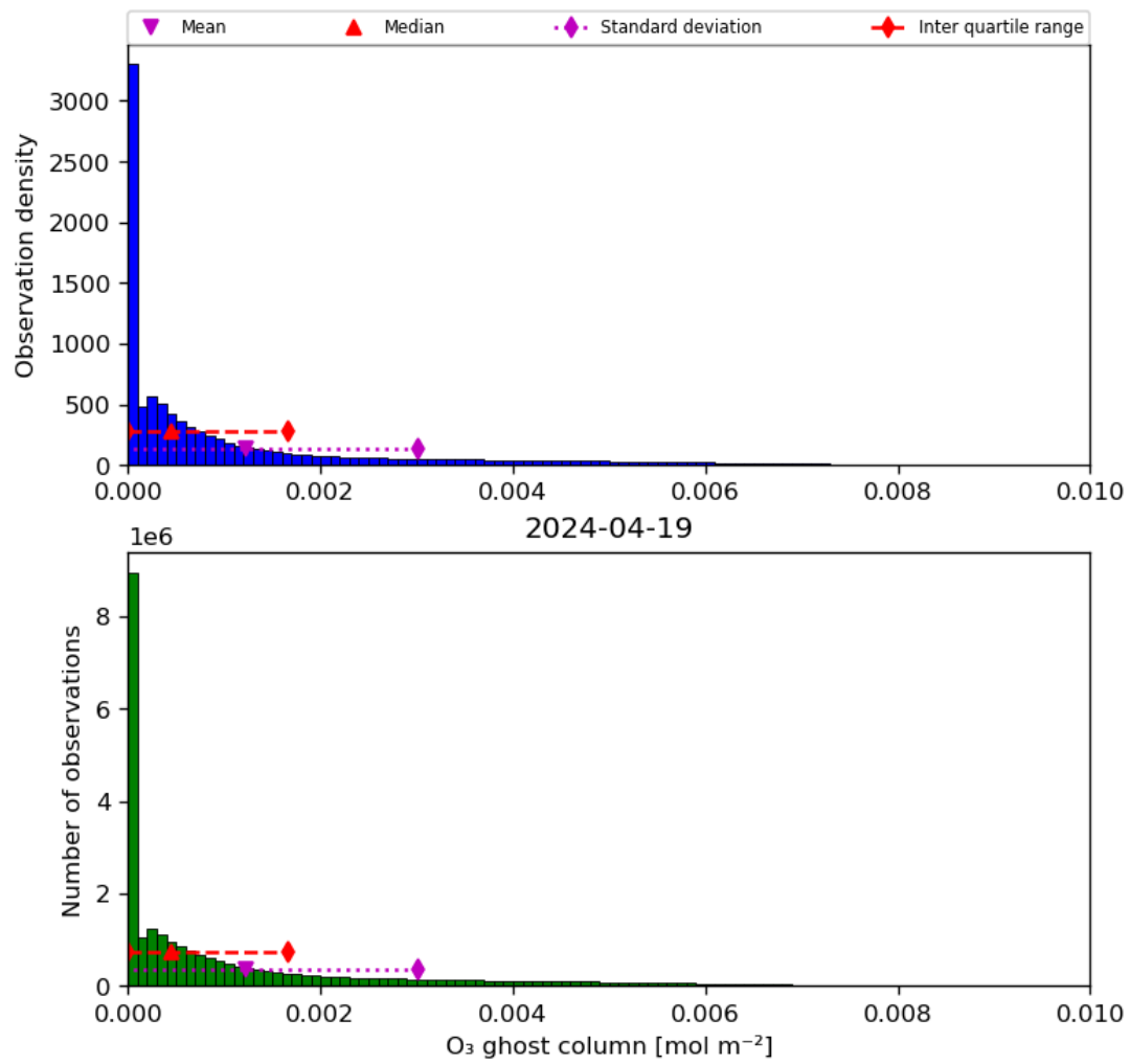
Figure 25: Histogram of "O 3 ghost column" for 2024-04-18 to 2024-04-20
