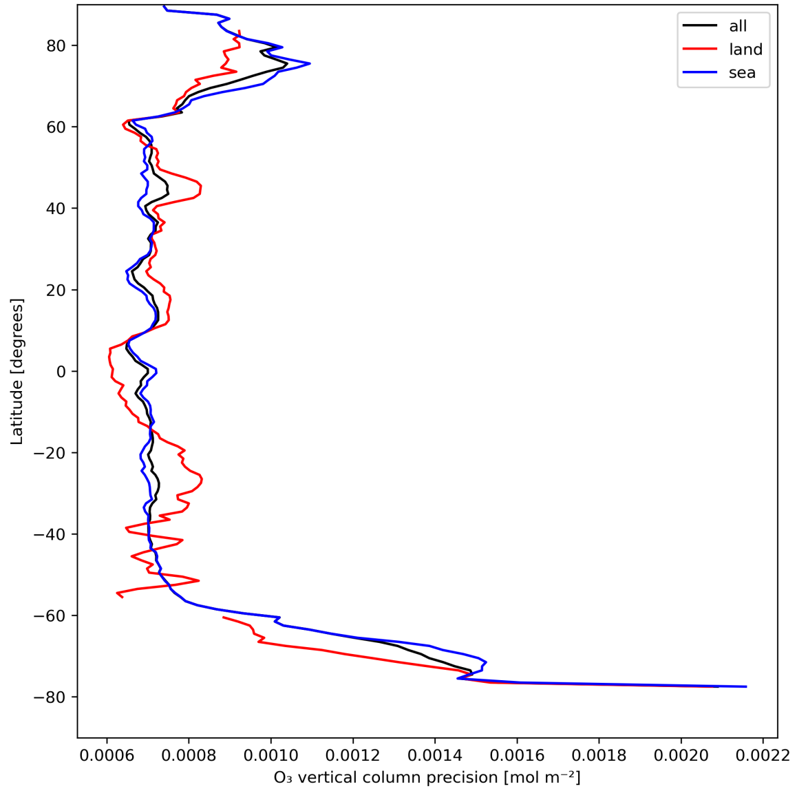
Figure 15: Zonal average of “O 3 vertical column precision” for 2024-04-18 to 2024-04-20.
