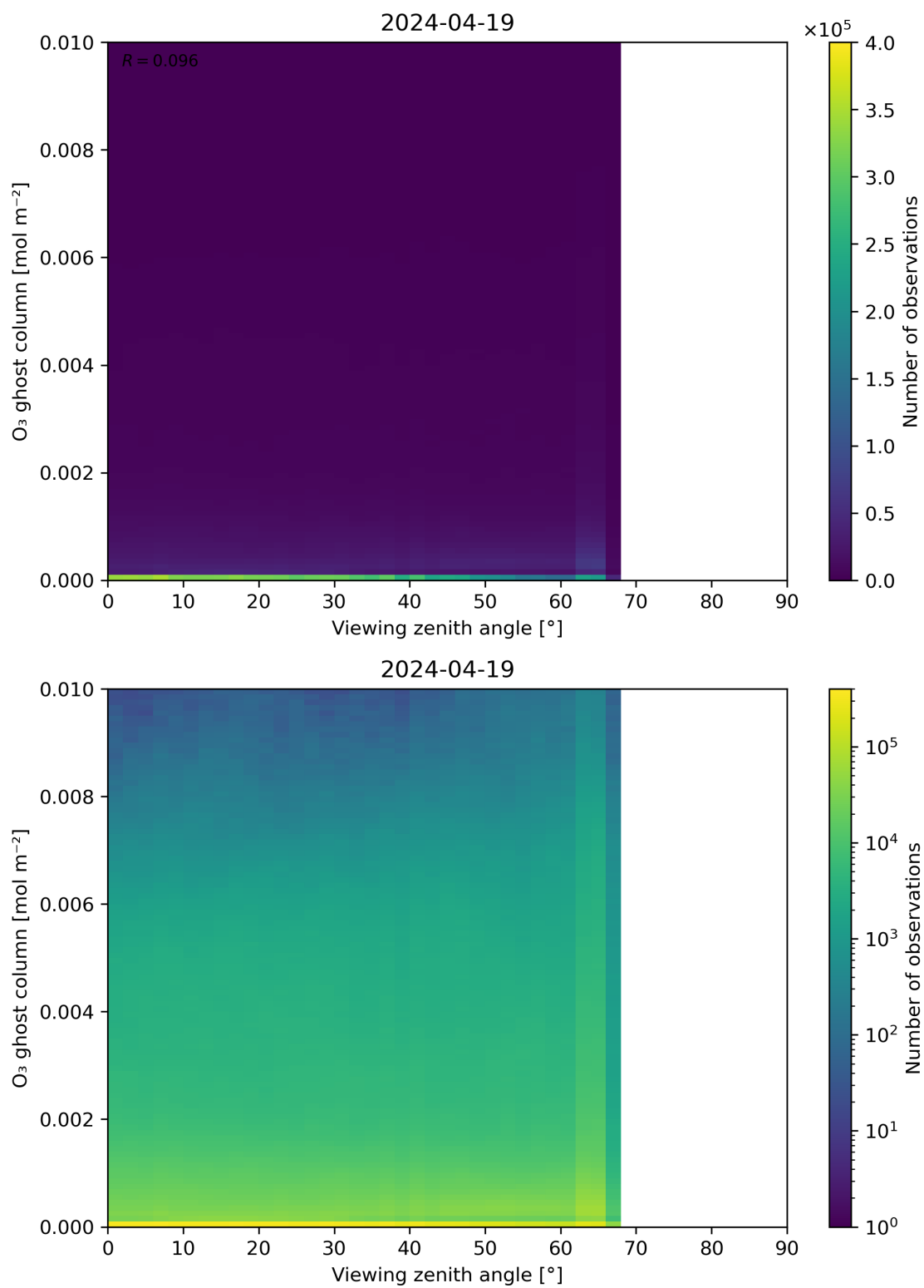
Figure 51: Scatter density plot of “Viewing zenith angle” against “O 3 ghost column” for 2024-04-18 to 2024-04-20.
