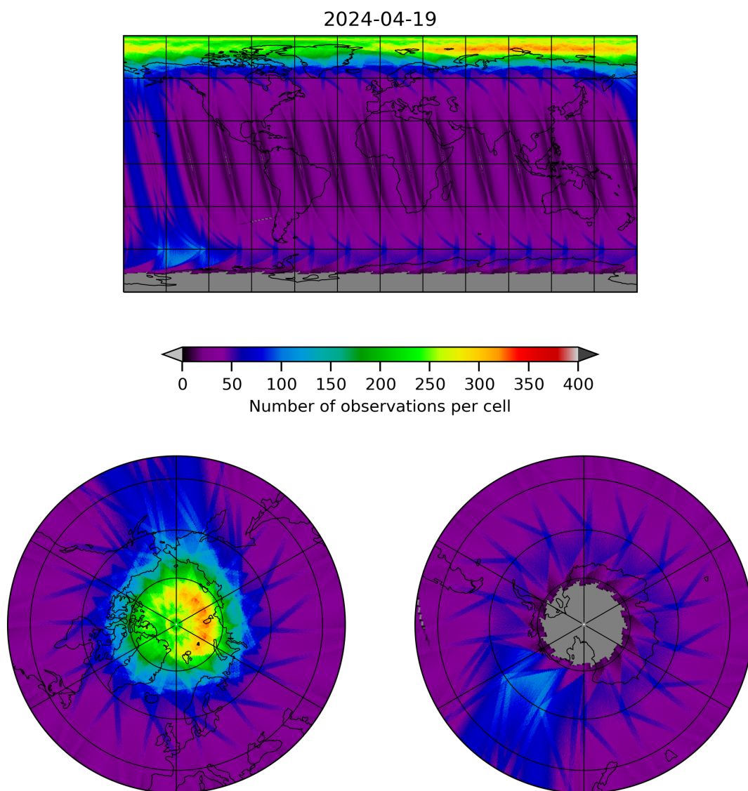
Figure 12: Map of the number of observations for 2024-04-18 to 2024-04-20
