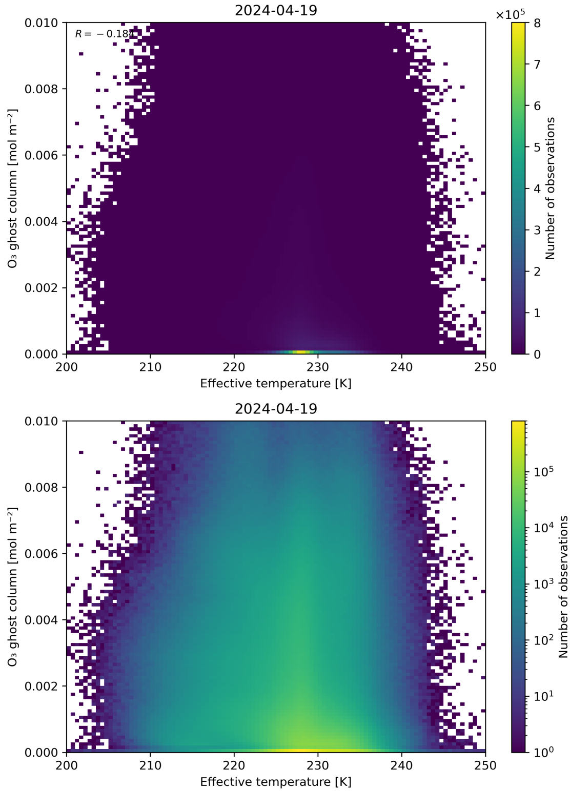
Figure 38: Scatter density plot of “Effective temperature” against “O 3 ghost column” for 2024-04-18 to 2024-04-20.
