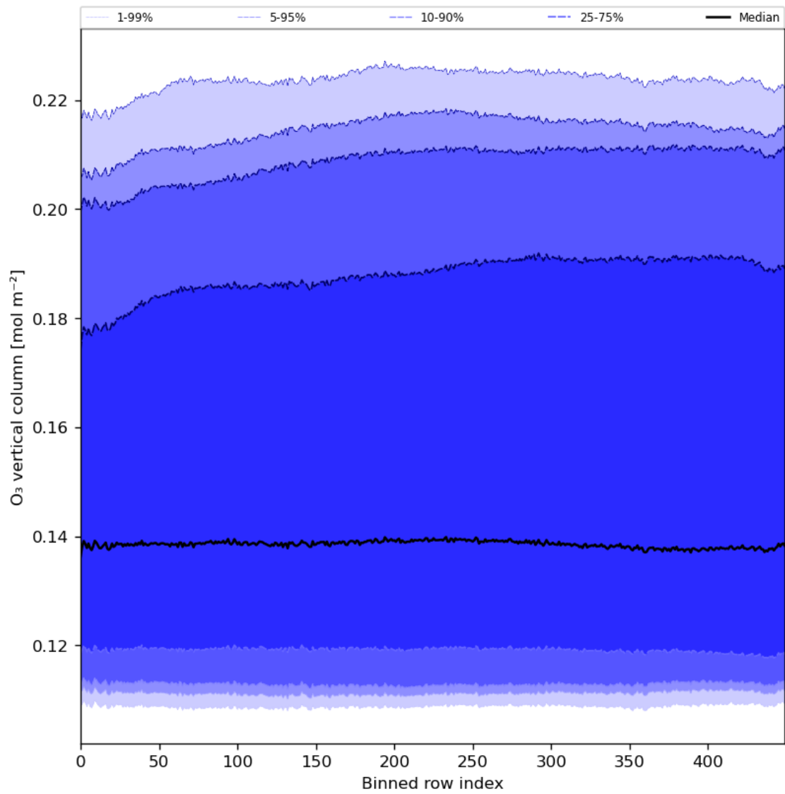
Figure 28: Along track statistics of “O 3 vertical column” for 2024-04-18 to 2024-04-20
