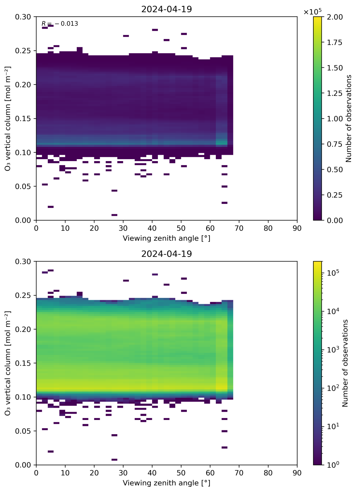
Figure 52: Scatter density plot of “Viewing zenith angle” against “O 3 vertical column” for 2024-04-18 to 2024-04-20.
