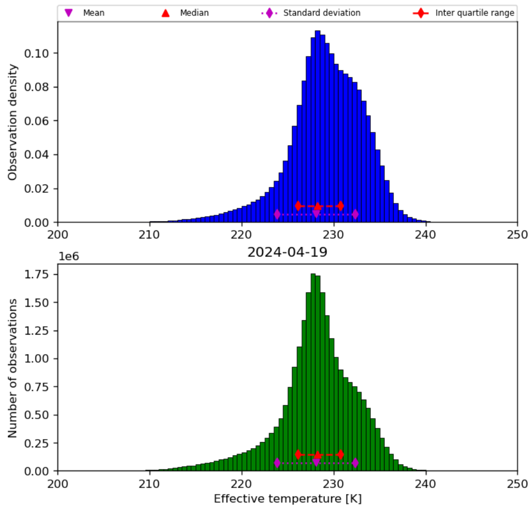
Figure 24: Histogram of “Effective temperature” for 2024-04-18 to 2024-04-20
