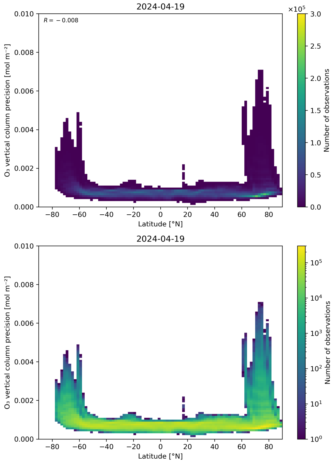
Figure 37: Scatter density plot of “Latitude” against “O 3 vertical column precision” for 2024-04-18 to 2024-04-20.
