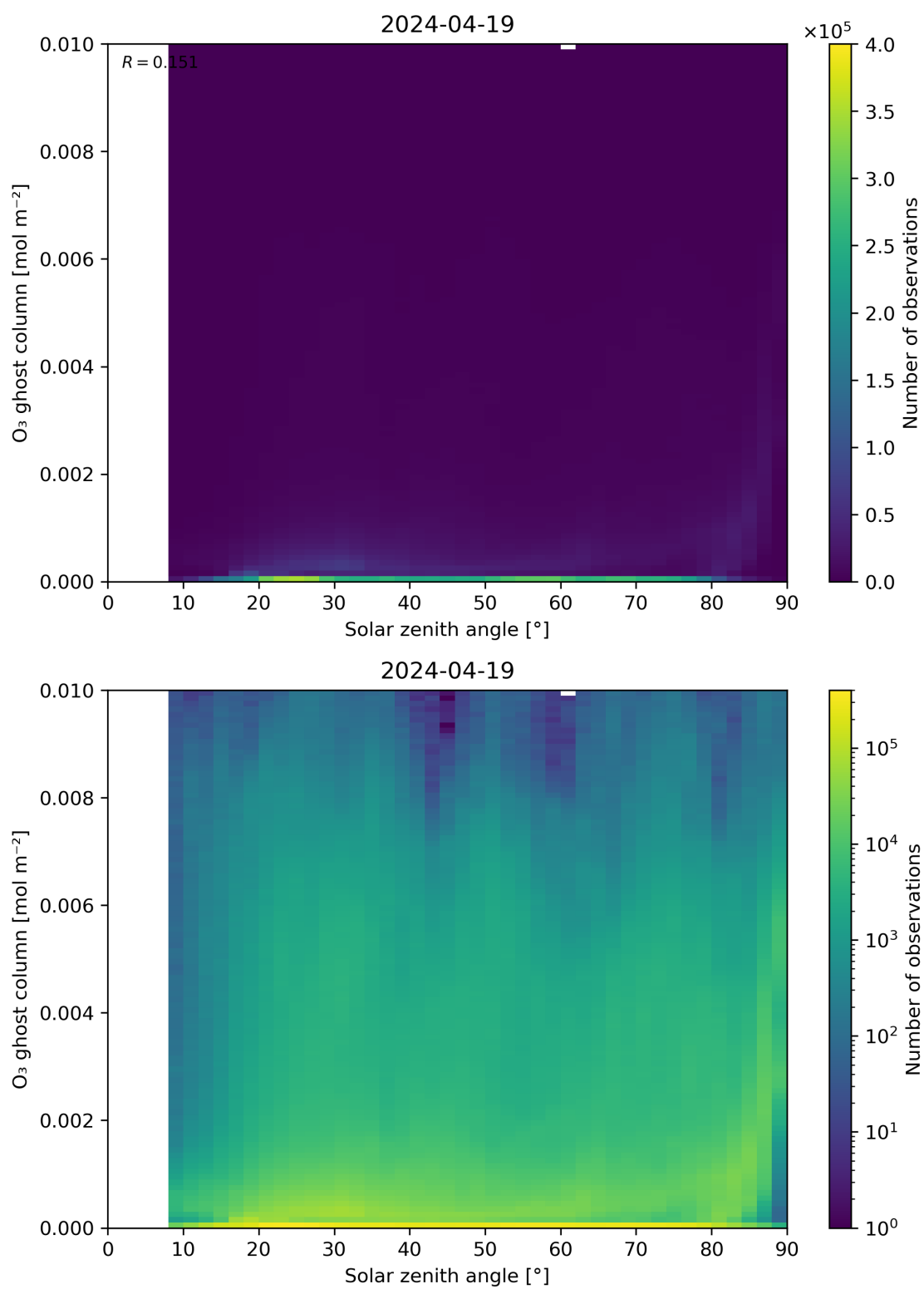
Figure 46: Scatter density plot of “Solar zenith angle” against “O 3 ghost column” for 2024-04-18 to 2024-04-20.
