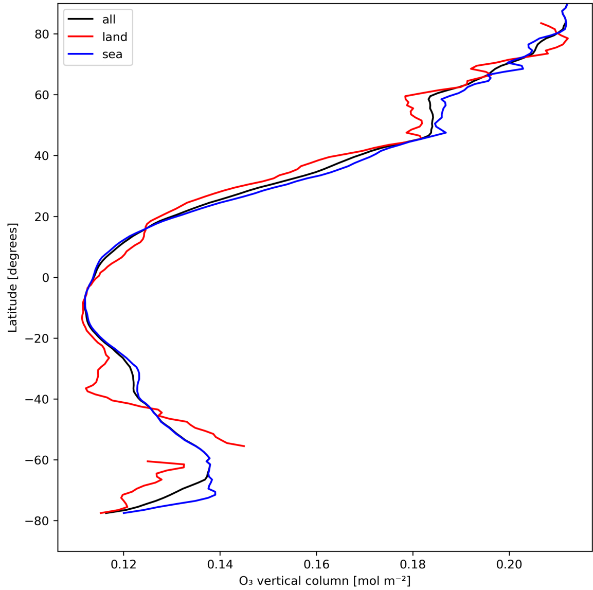
Figure 14: Zonal average of “O 3 vertical column” for 2024-04-18 to 2024-04-20.
