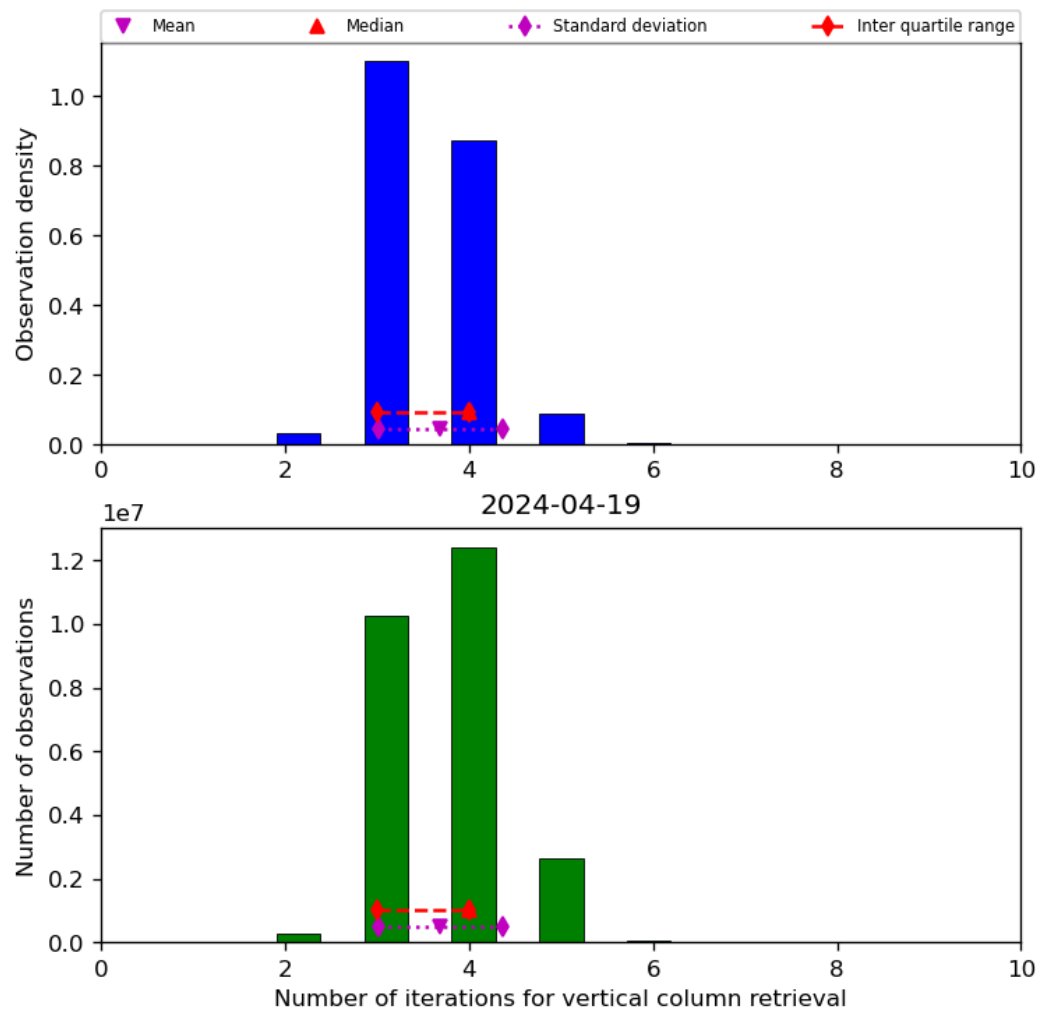
Figure 26: Histogram of “Number of iterations for vertical column retrieval” for 2024-04-18 to 2024-04-20
