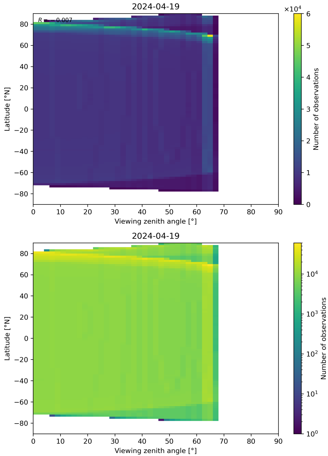
Figure 49: Scatter density plot of “Viewing zenith angle” against “Latitude” for 2024-04-18 to 2024-04-20.
