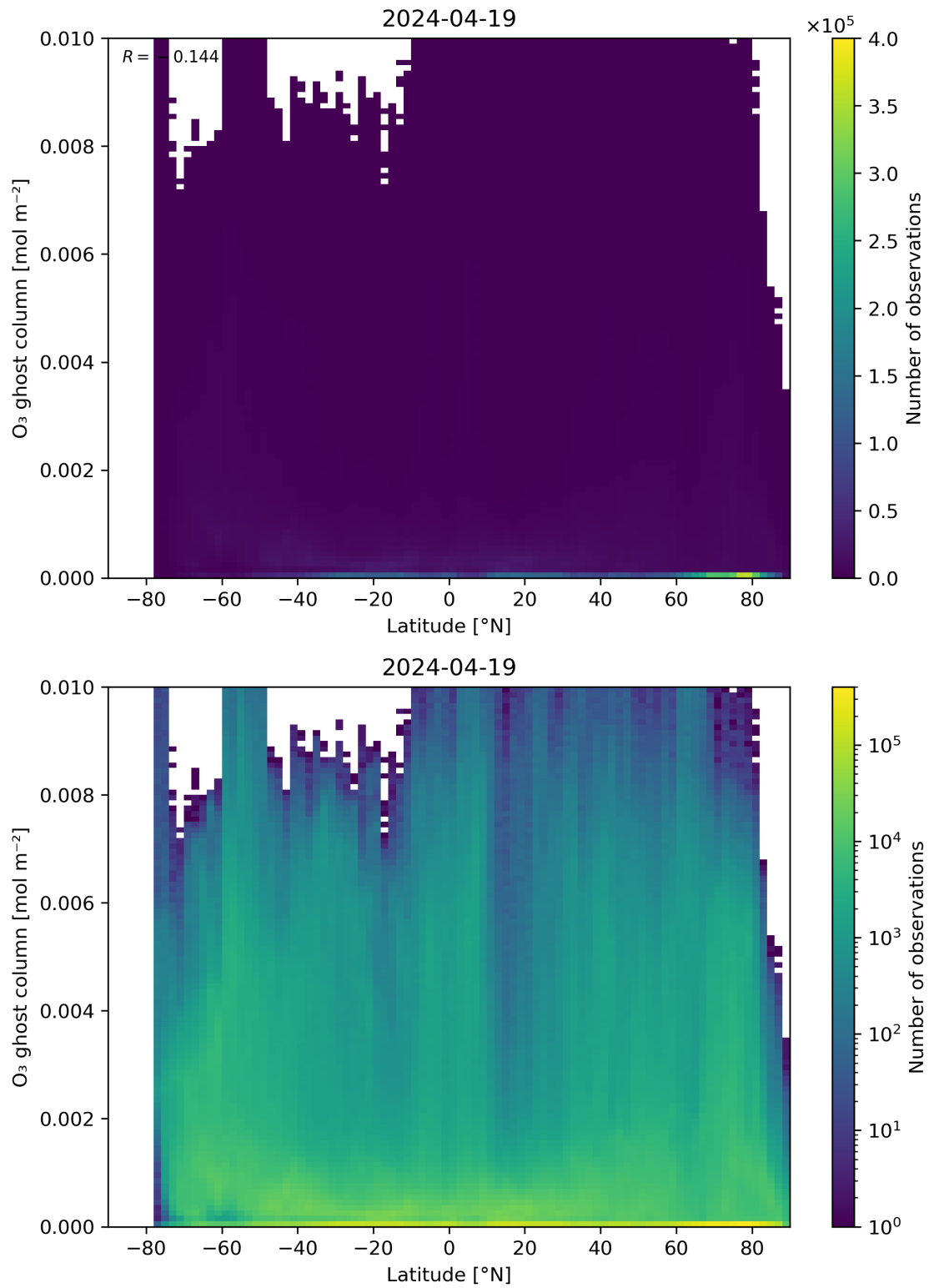
Figure 35: Scatter density plot of “Latitude” against “O 3 ghost column” for 2024-04-18 to 2024-04-20.
