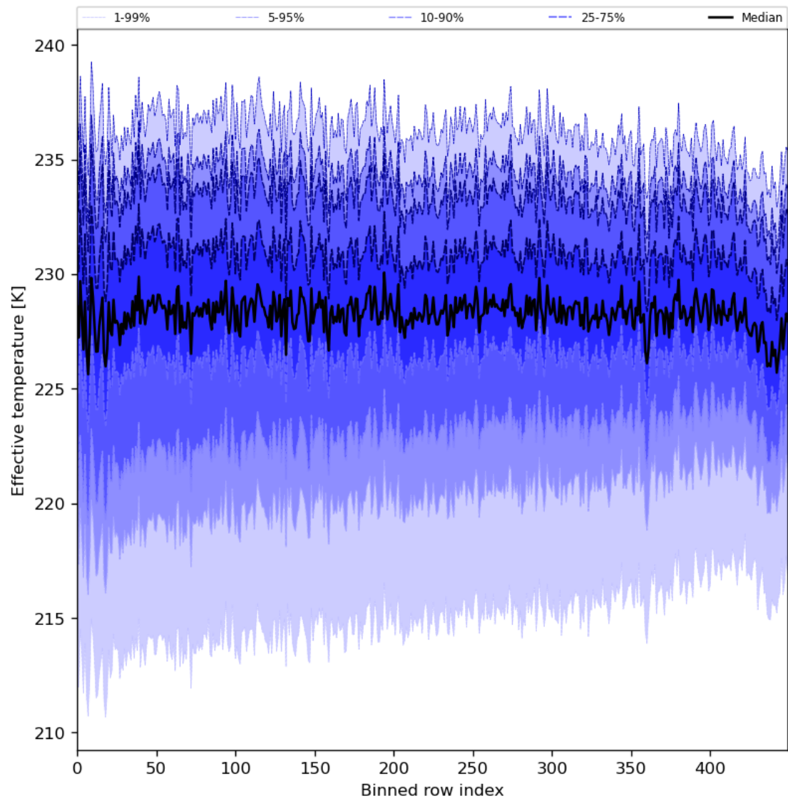
Figure 31: Along track statistics of “Effective temperature” for 2024-04-18 to 2024-04-20
