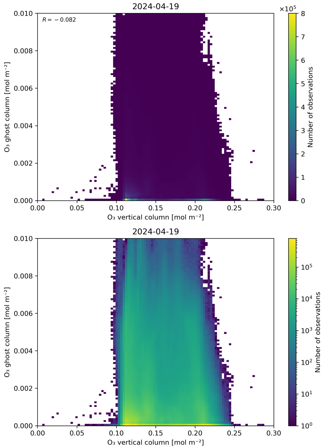
Figure 40: Scatter density plot of “O 3 vertical column” against “O 3 ghost column” for 2024-04-18 to 2024-04-20.
