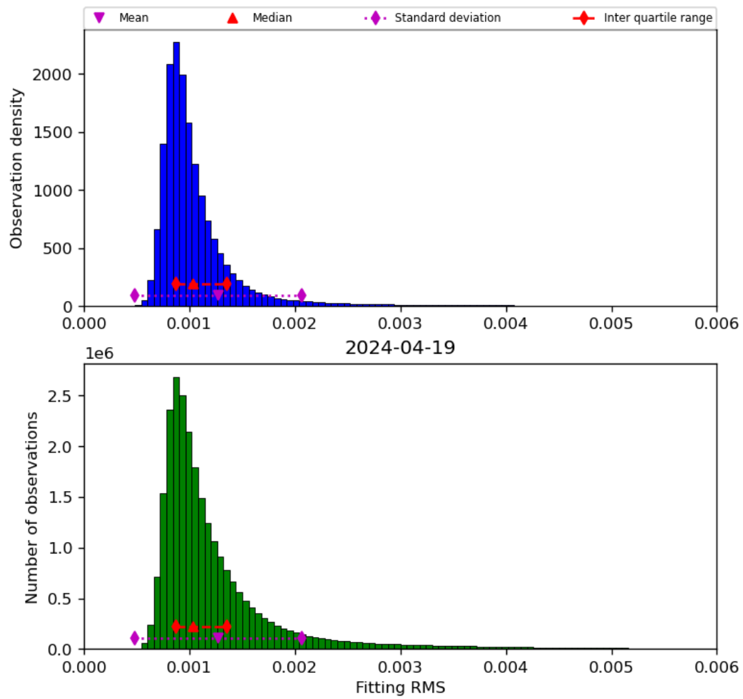
Figure 23: Histogram of “Fitting RMS” for 2024-04-18 to 2024-04-20
