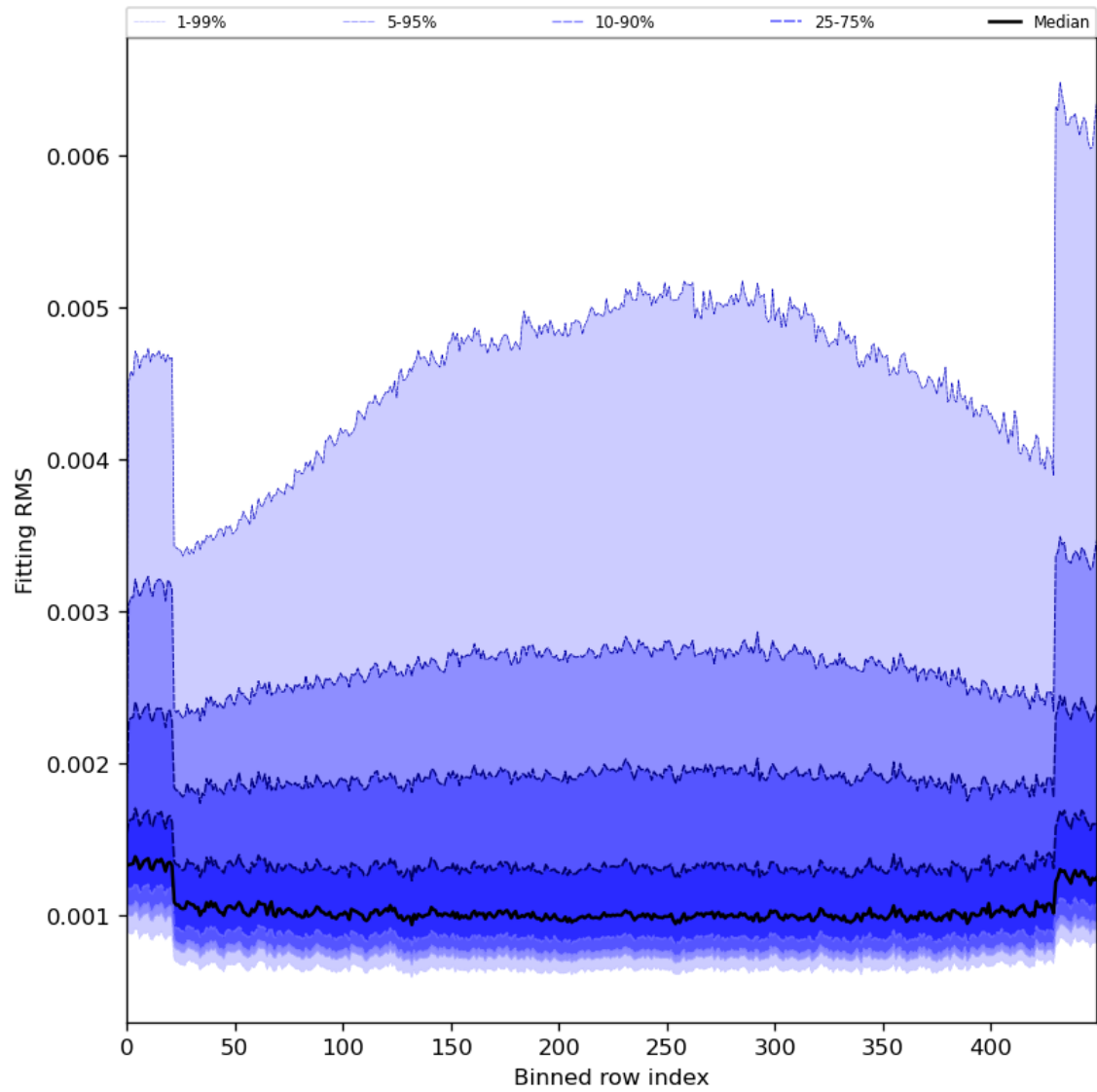
Figure 30: Along track statistics of “Fitting RMS” for 2024-04-18 to 2024-04-20
