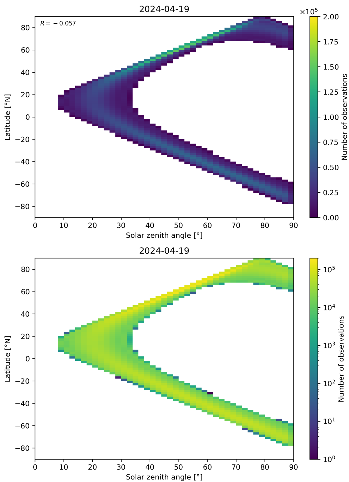
Figure 44: Scatter density plot of “Solar zenith angle” against “Latitude” for 2024-04-18 to 2024-04-20.
