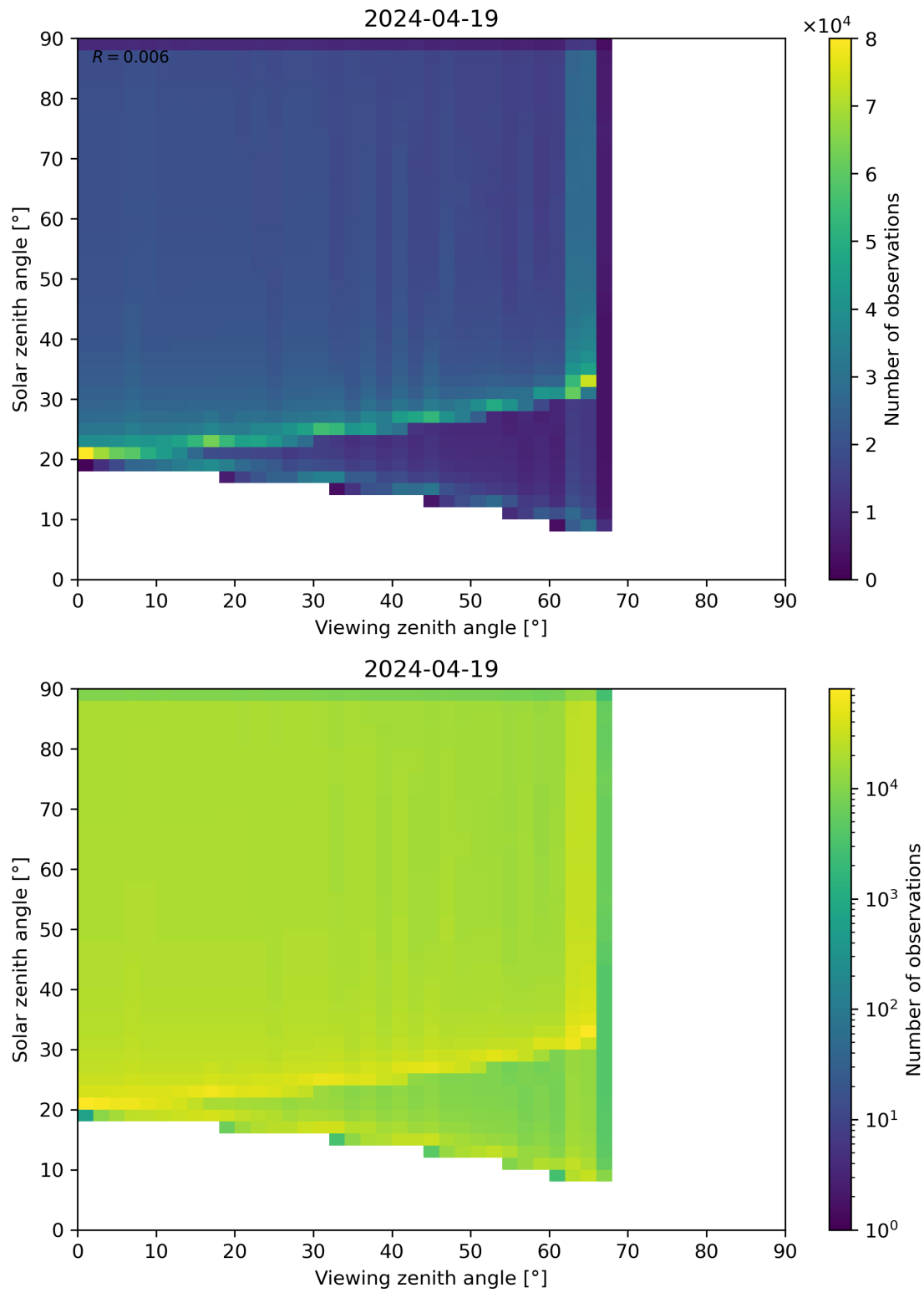
Figure 54: Scatter density plot of “Viewing zenith angle” against “Solar zenith angle” for 2024-04-18 to 2024-04-20.
