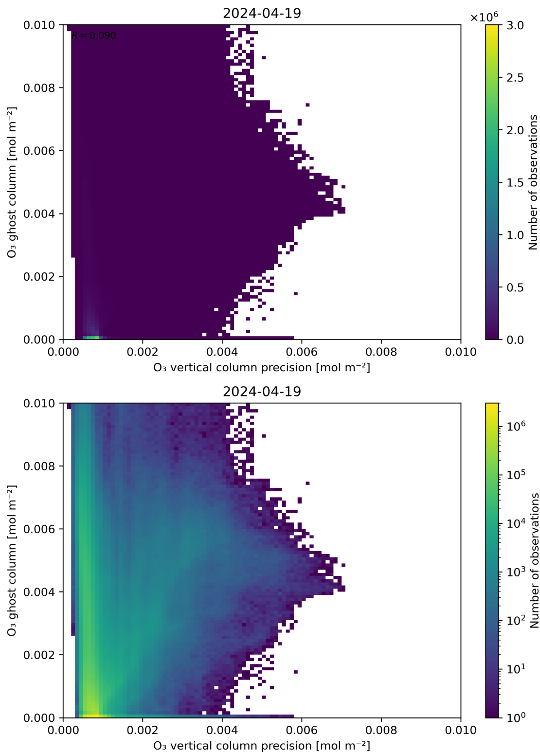
Figure 43: Scatter density plot of “ \text{O}_3 vertical column precision” against “ \text{O}_3 ghost column” for 2024-04-18 to 2024-04-20.
