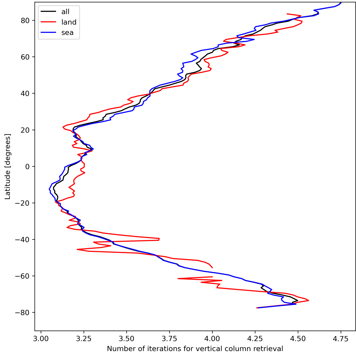
Figure 19: Zonal average of “Number of iterations for vertical column retrieval” for 2024-04-18 to 2024-04-20.
