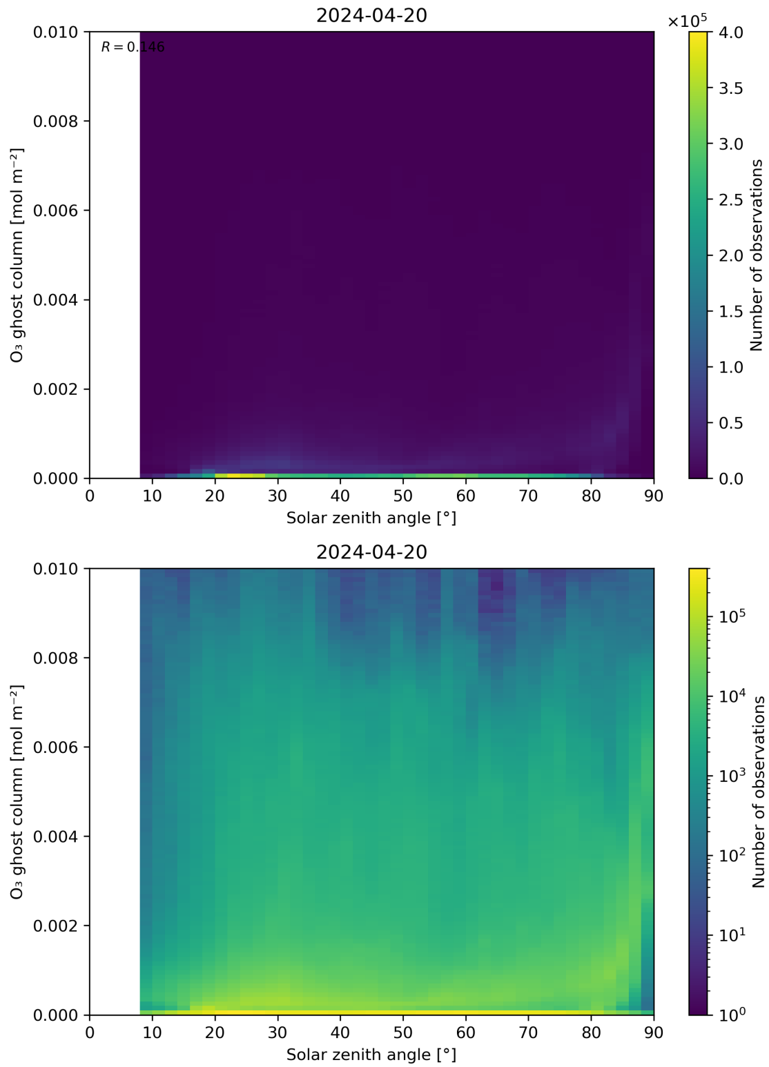
Figure 46: Scatter density plot of “Solar zenith angle” against “O 3 ghost column” for 2024-04-19 to 2024-04-21.
