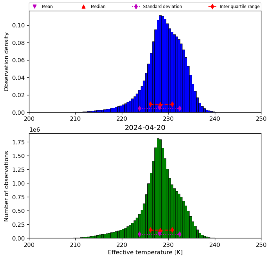
Figure 24: Histogram of “Effective temperature” for 2024-04-19 to 2024-04-21
