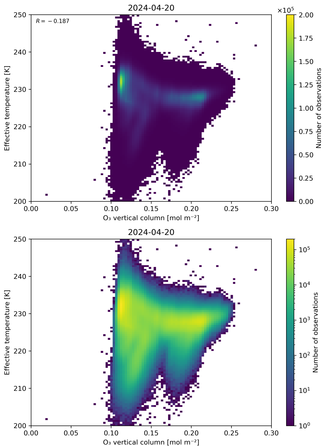
Figure 39: Scatter density plot of “O 3 vertical column” against “Effective temperature” for 2024-04-19 to 2024-04-21.
