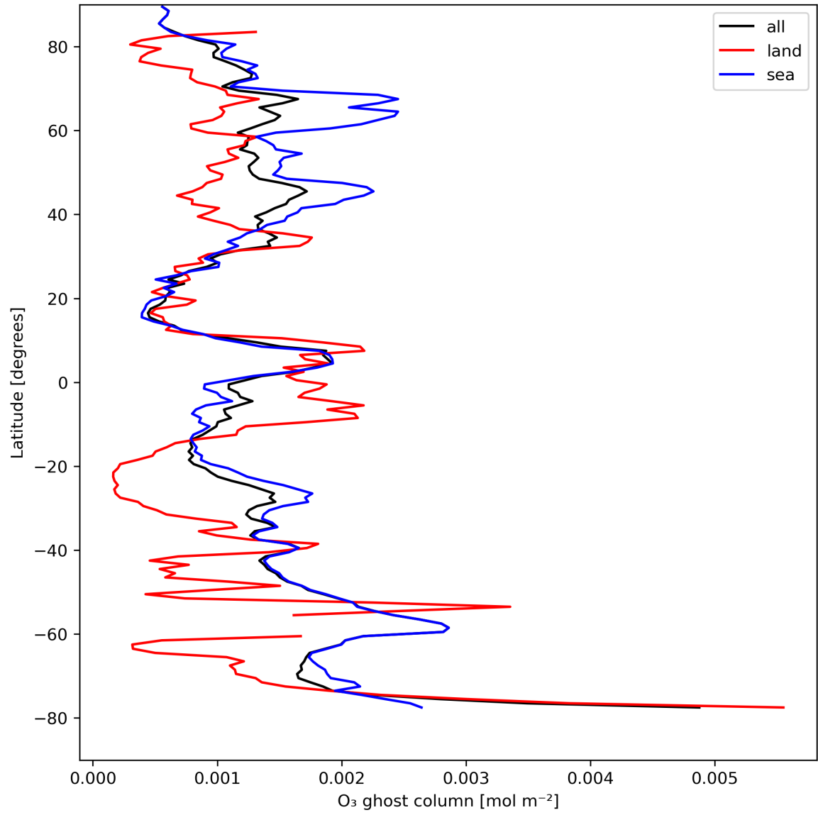
Figure 18: Zonal average of "O 3 ghost column" for 2024-04-19 to 2024-04-21.
