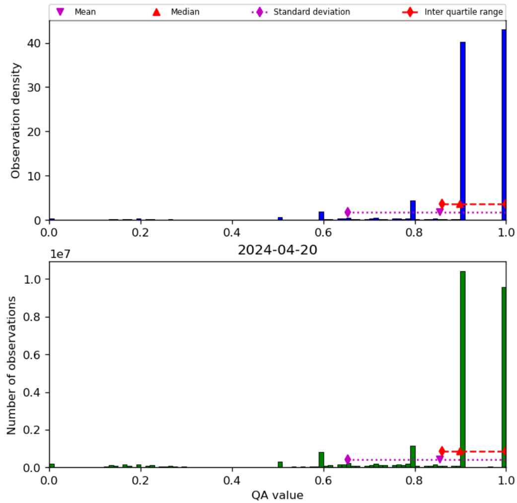
Figure 20: Histogram of “QA value” for 2024-04-19 to 2024-04-21
