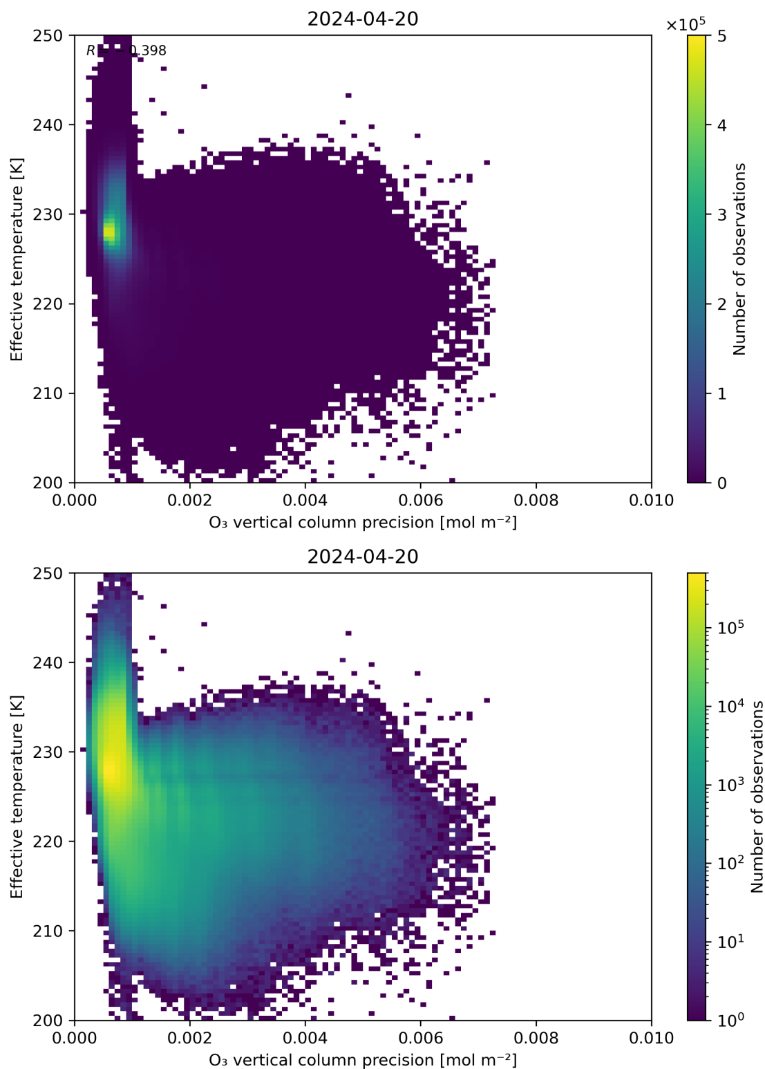
Figure 42: Scatter density plot of “O 3 vertical column precision” against “Effective temperature” for 2024-04-19 to 2024-04-21.
