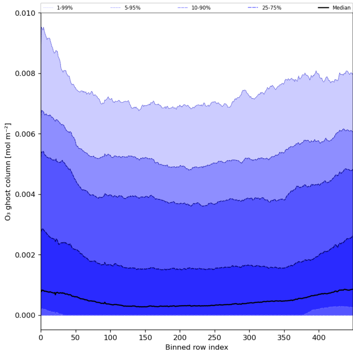
Figure 32: Along track statistics of "O 3 ghost column" for 2024-04-19 to 2024-04-21
