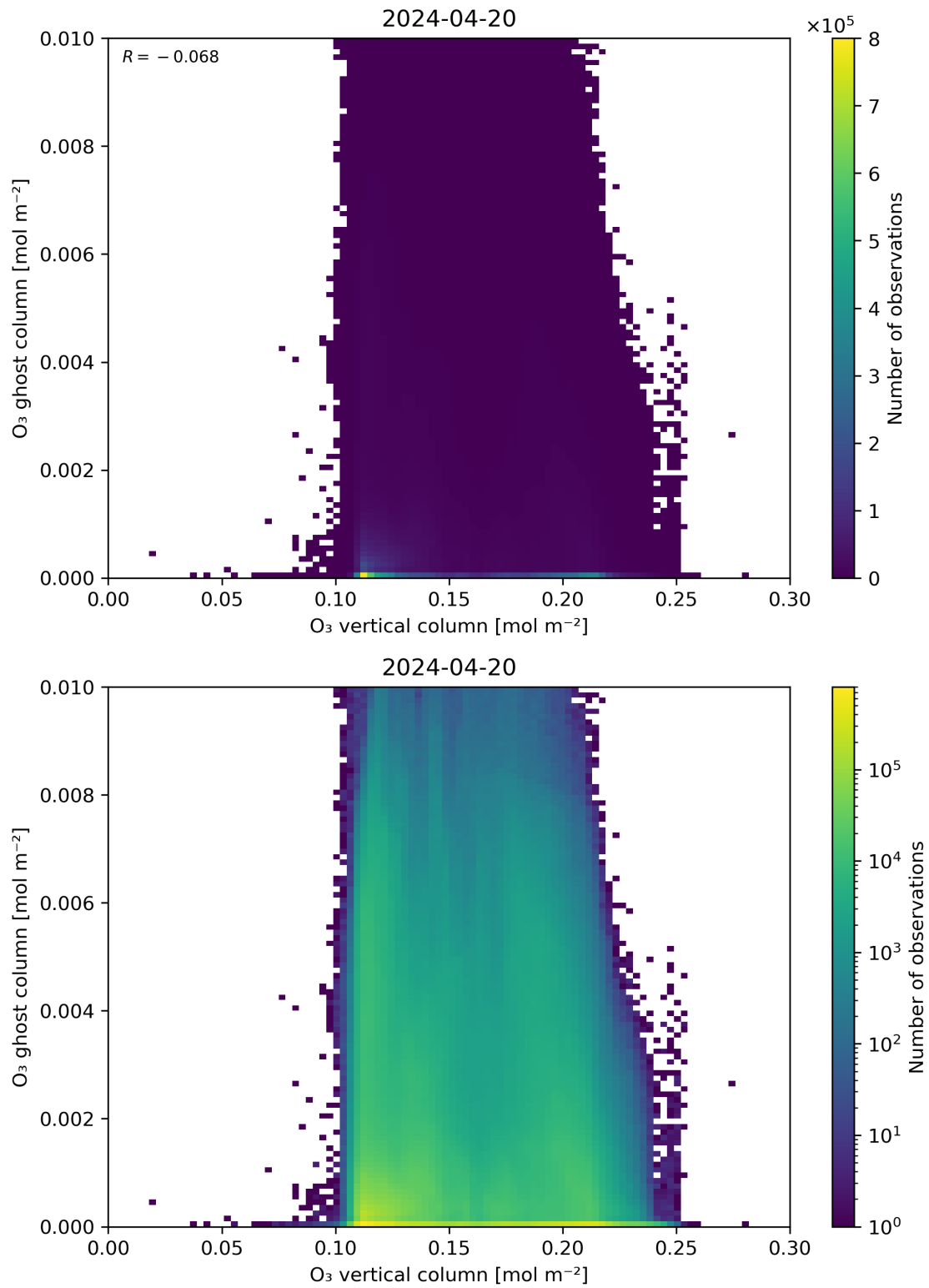
Figure 40: Scatter density plot of “O 3 vertical column” against “O 3 ghost column” for 2024-04-19 to 2024-04-21.
