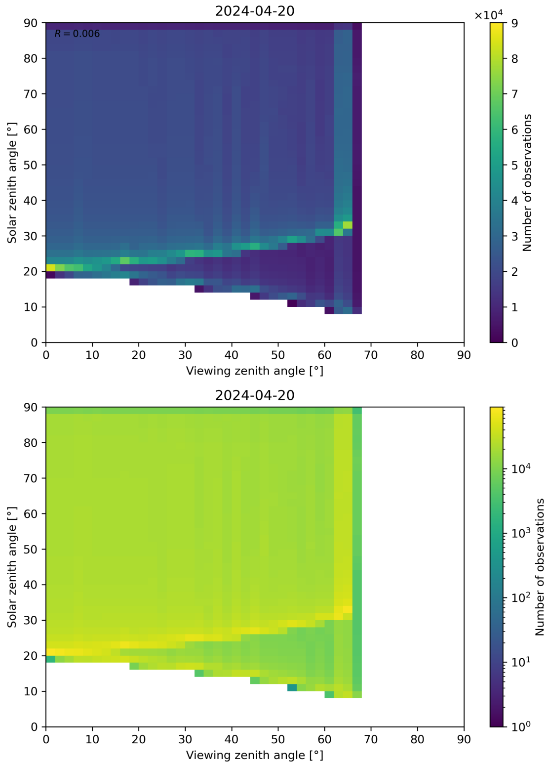
Figure 54: Scatter density plot of “Viewing zenith angle” against “Solar zenith angle” for 2024-04-19 to 2024-04-21.
