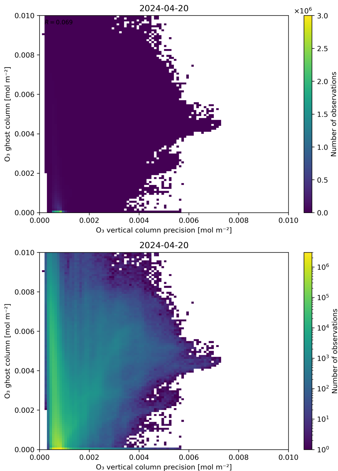
Figure 43: Scatter density plot of “O 3 vertical column precision” against “O 3 ghost column” for 2024-04-19 to 2024-04-21.
