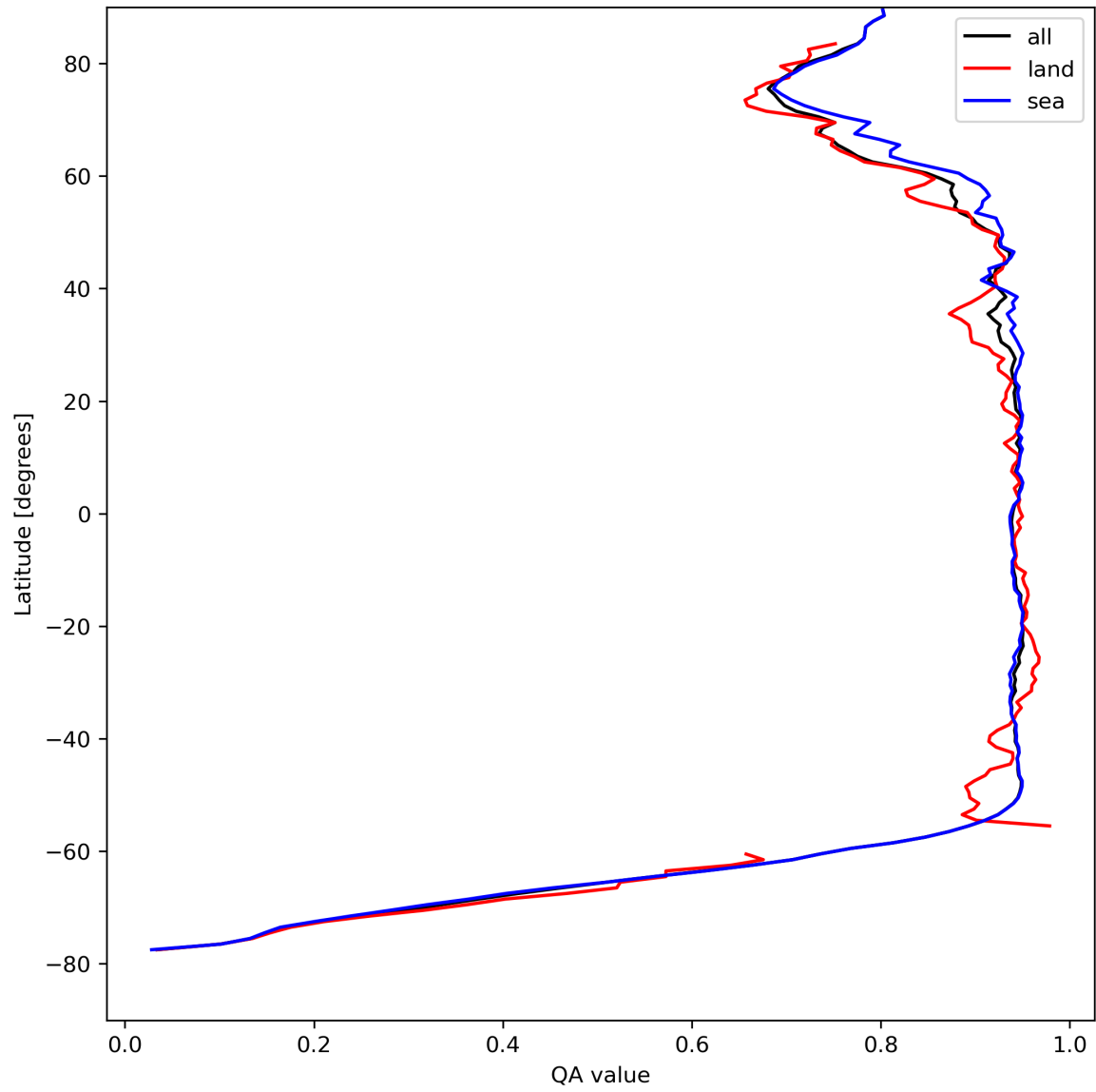
Figure 13: Zonal average of “QA value” for 2024-04-19 to 2024-04-21.
