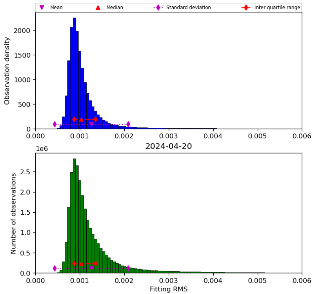
Figure 23: Histogram of “Fitting RMS” for 2024-04-19 to 2024-04-21
