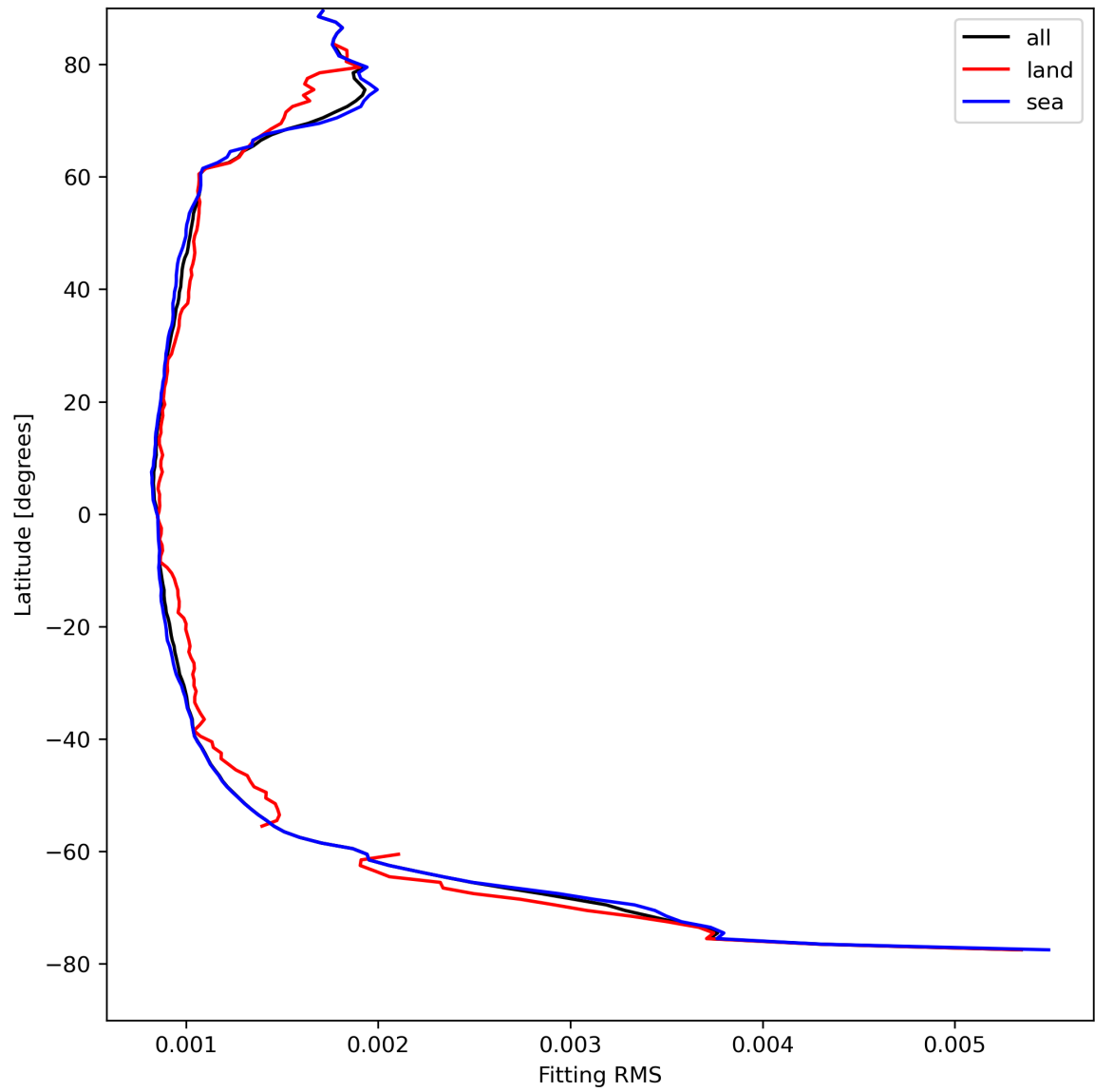
Figure 16: Zonal average of “Fitting RMS” for 2024-04-19 to 2024-04-21.
