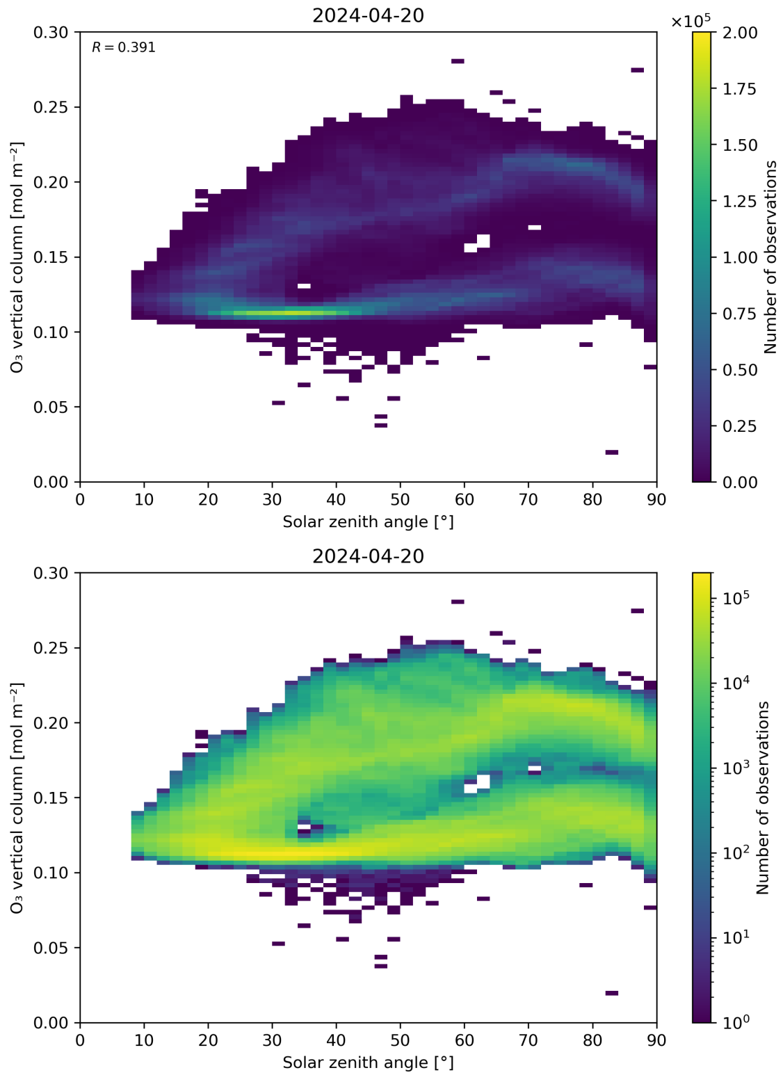
Figure 47: Scatter density plot of “Solar zenith angle” against “O 3 vertical column” for 2024-04-19 to 2024-04-21.
