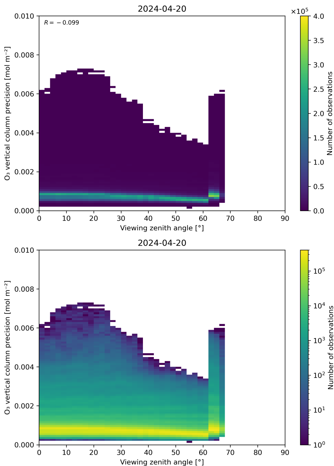
Figure 53: Scatter density plot of “Viewing zenith angle” against “O 3 vertical column precision” for 2024-04-19 to 2024-04-21.
