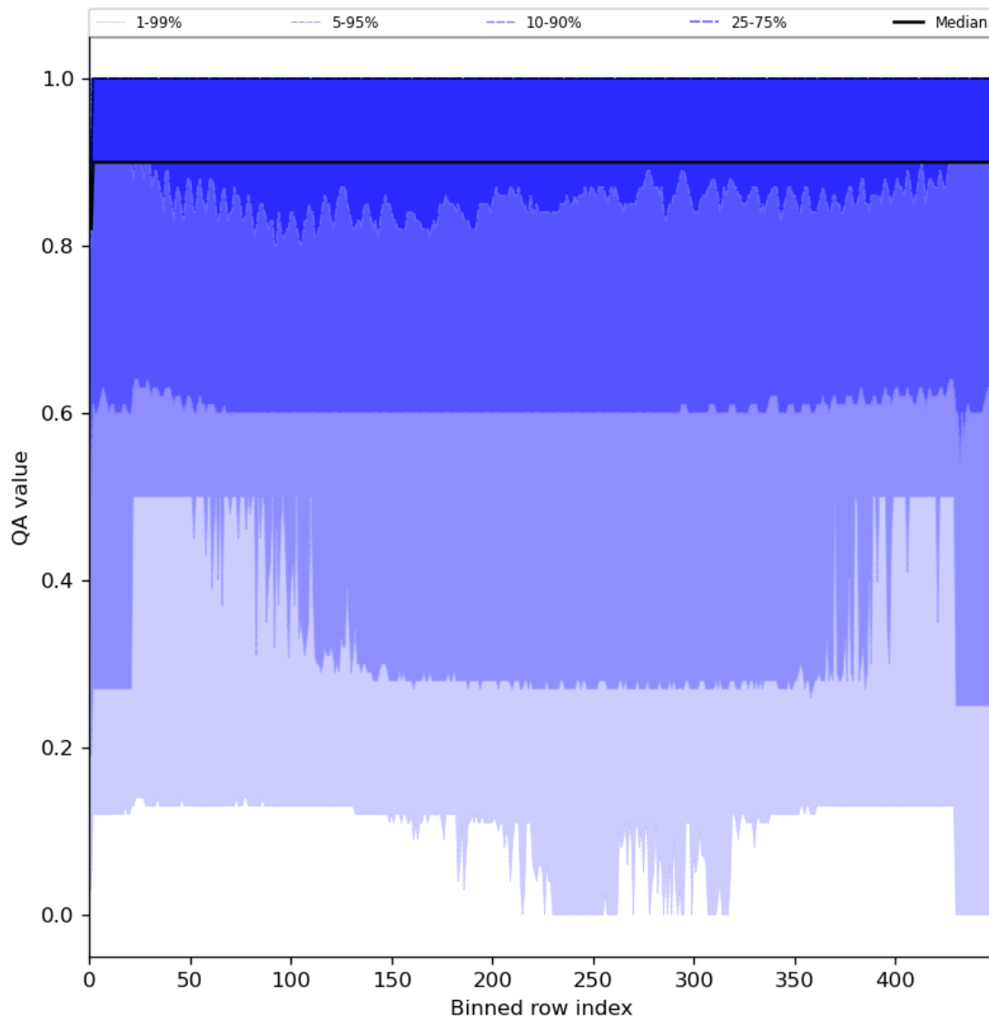
Figure 27: Along track statistics of “QA value” for 2024-04-19 to 2024-04-21
