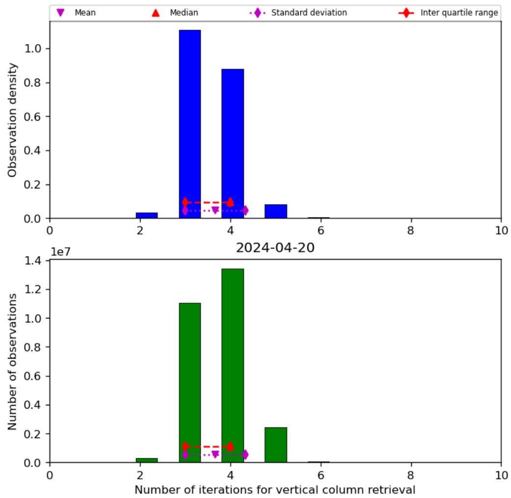
Figure 26: Histogram of “Number of iterations for vertical column retrieval” for 2024-04-19 to 2024-04-21
