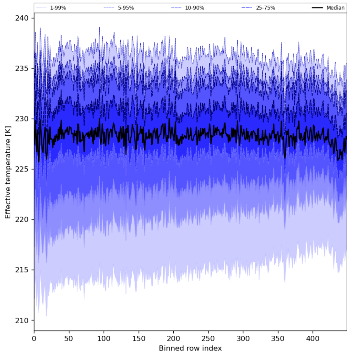
Figure 31: Along track statistics of “Effective temperature” for 2024-04-19 to 2024-04-21
