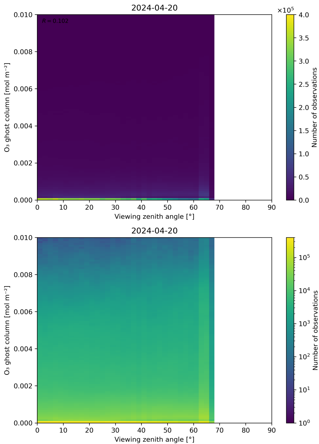
Figure 51: Scatter density plot of “Viewing zenith angle” against “O 3 ghost column” for 2024-04-19 to 2024-04-21.
