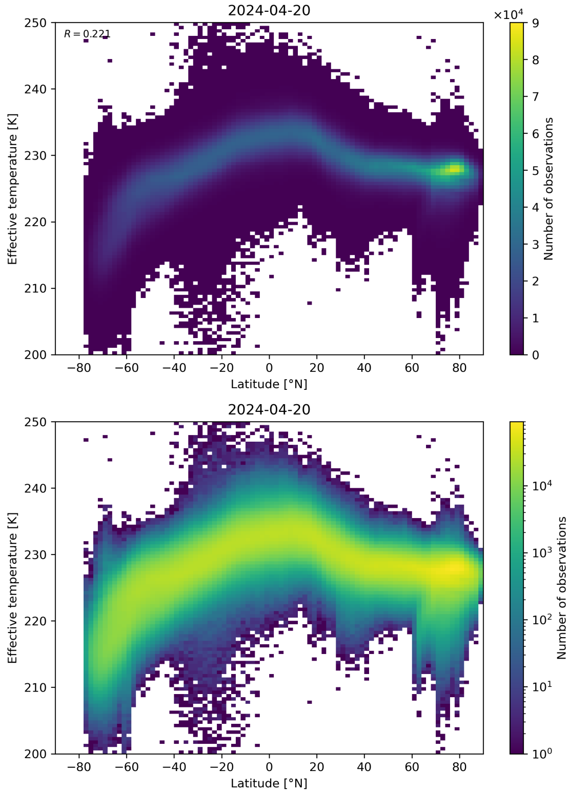
Figure 34: Scatter density plot of “Latitude” against “Effective temperature” for 2024-04-19 to 2024-04-21.
