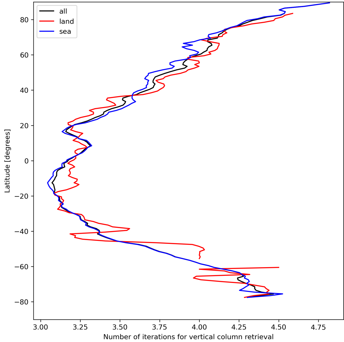
Figure 19: Zonal average of “Number of iterations for vertical column retrieval” for 2024-04-19 to 2024-04-21.
