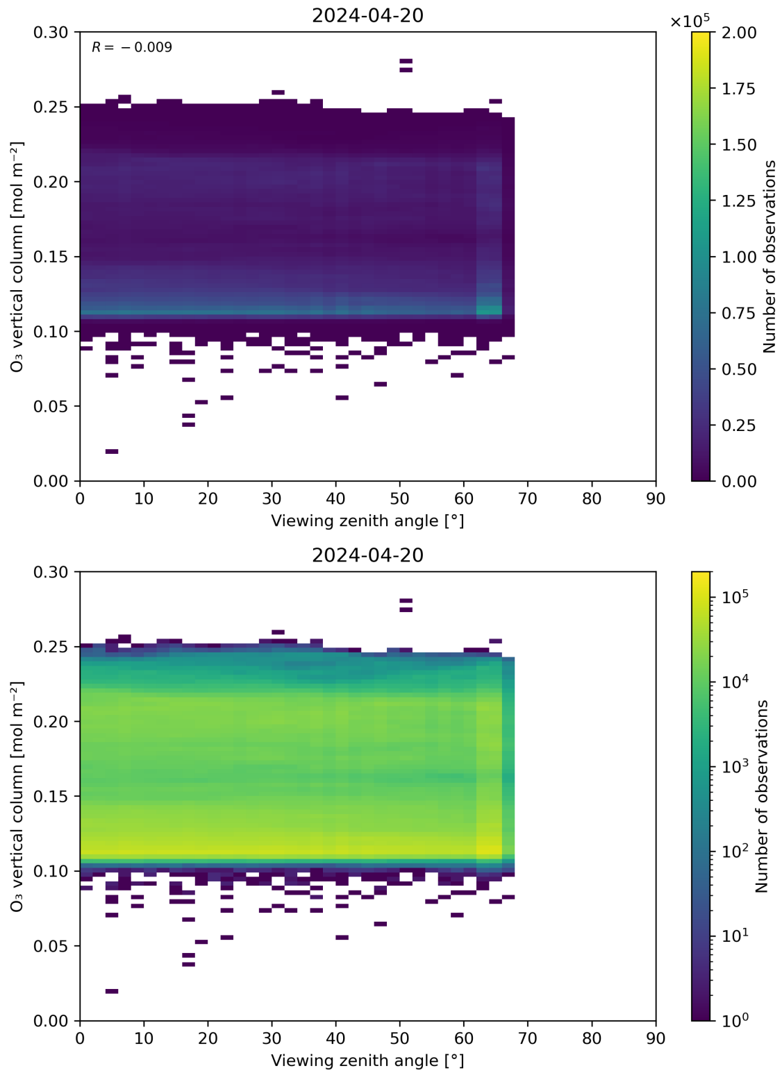
Figure 52: Scatter density plot of “Viewing zenith angle” against “O 3 vertical column” for 2024-04-19 to 2024-04-21.
