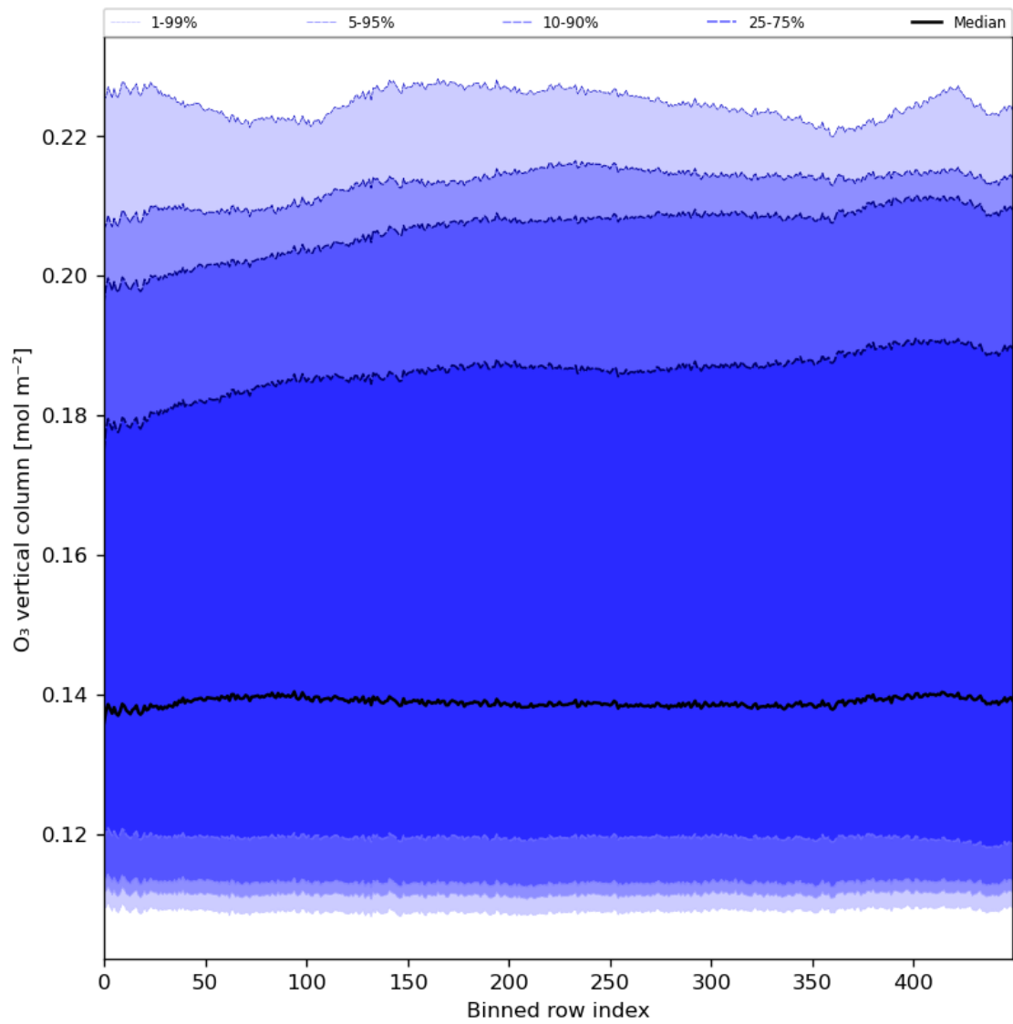
Figure 28: Along track statistics of “O 3 vertical column” for 2024-04-19 to 2024-04-21
