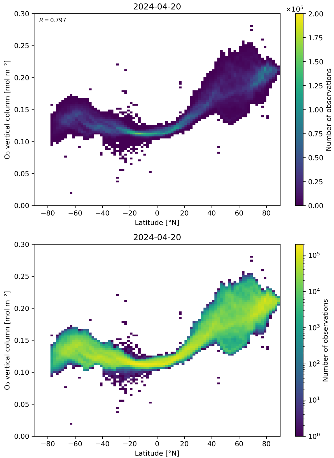
Figure 36: Scatter density plot of “Latitude” against “O 3 vertical column” for 2024-04-19 to 2024-04-21.
