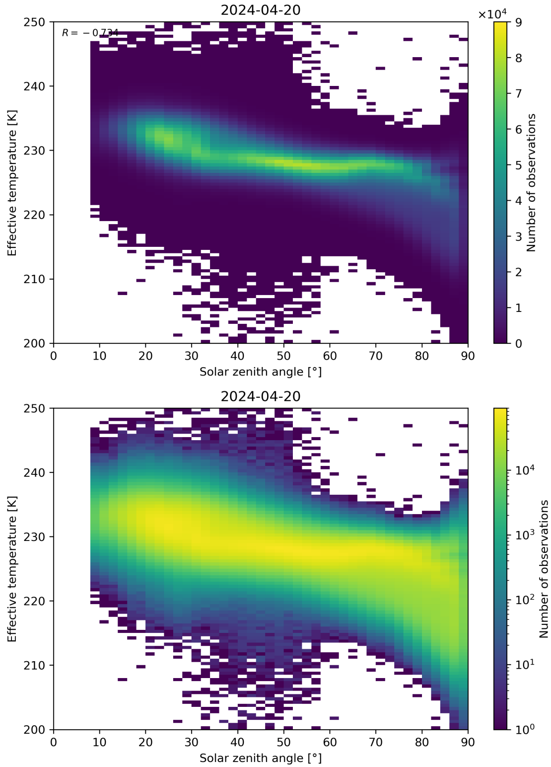
Figure 45: Scatter density plot of “Solar zenith angle” against “Effective temperature” for 2024-04-19 to 2024-04-21.
