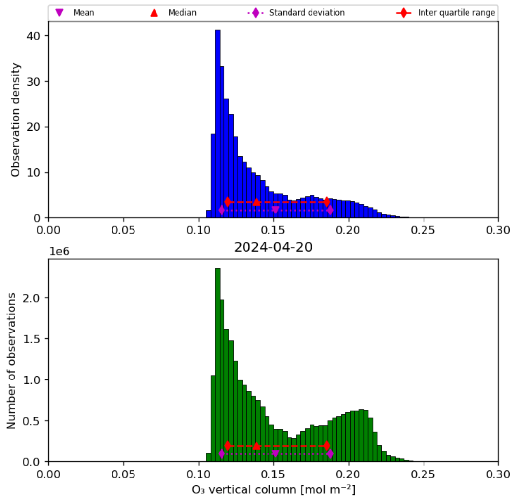
Figure 21: Histogram of “O 3 vertical column” for 2024-04-19 to 2024-04-21
