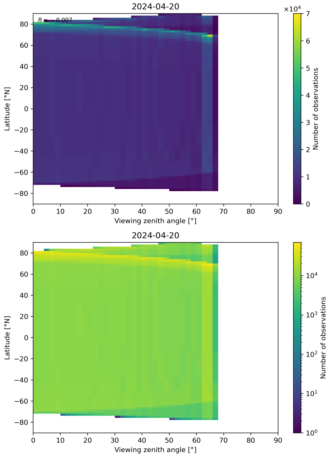
Figure 49: Scatter density plot of “Viewing zenith angle” against “Latitude” for 2024-04-19 to 2024-04-21.
