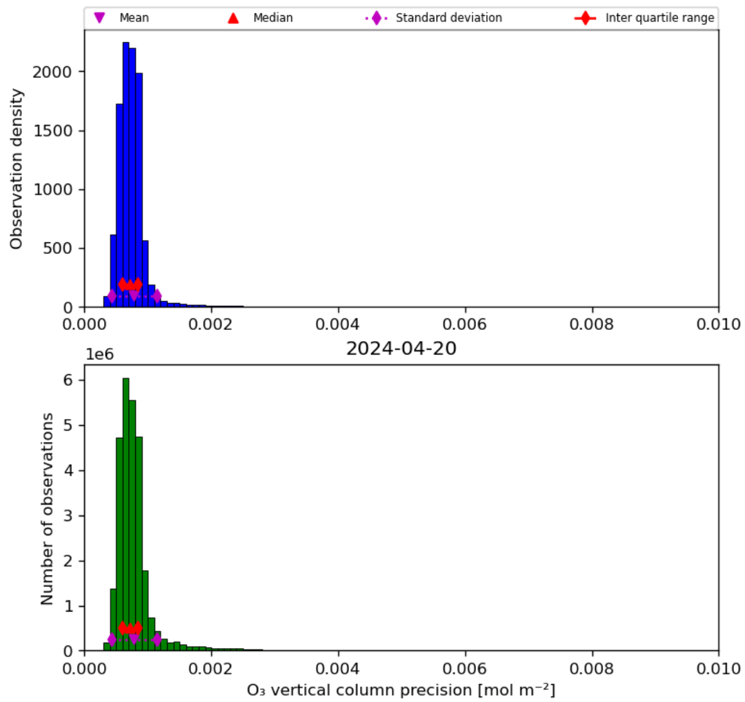
Figure 22: Histogram of “O 3 vertical column precision” for 2024-04-19 to 2024-04-21
