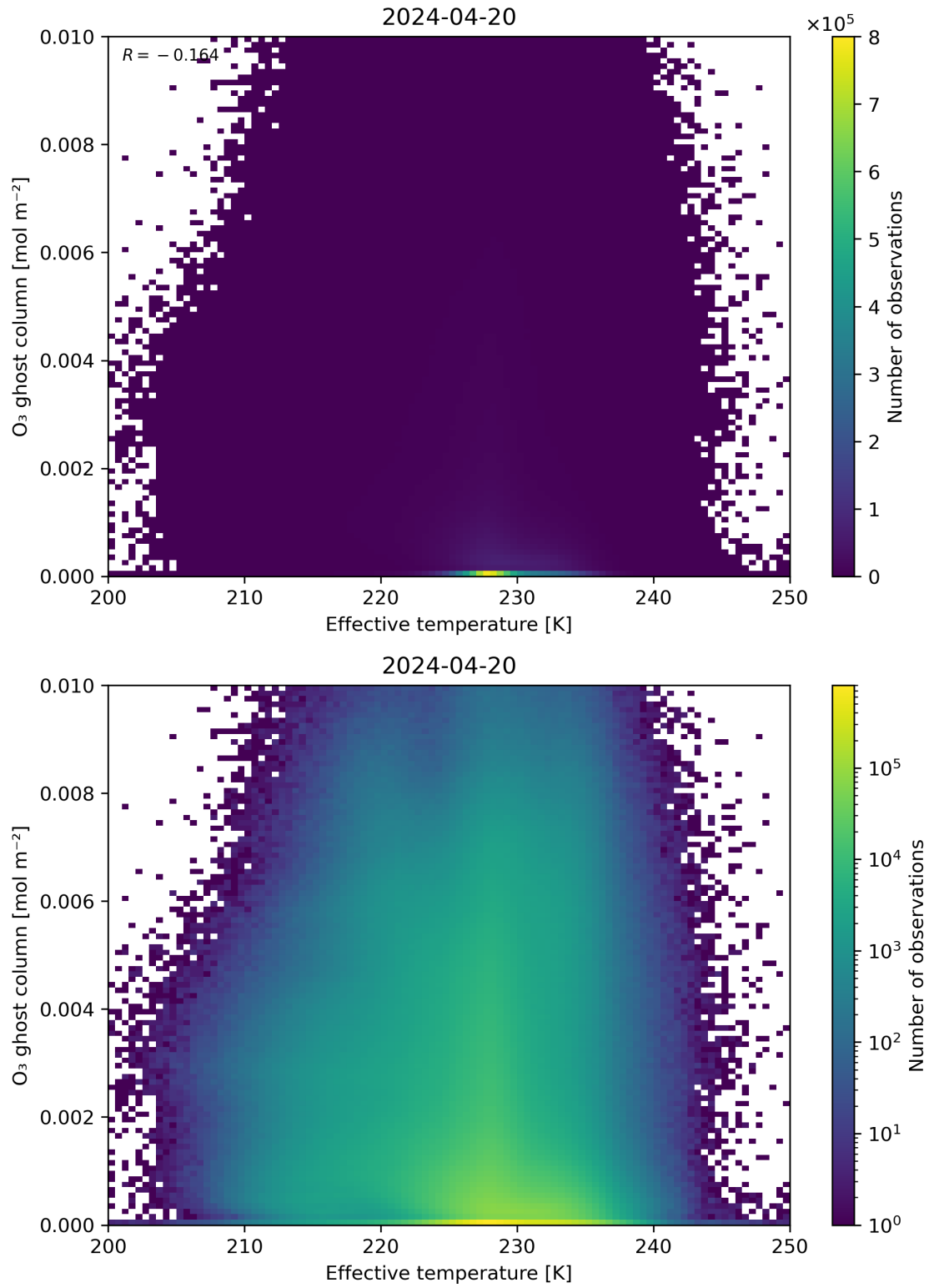
Figure 38: Scatter density plot of “Effective temperature” against “O 3 ghost column” for 2024-04-19 to 2024-04-21.
