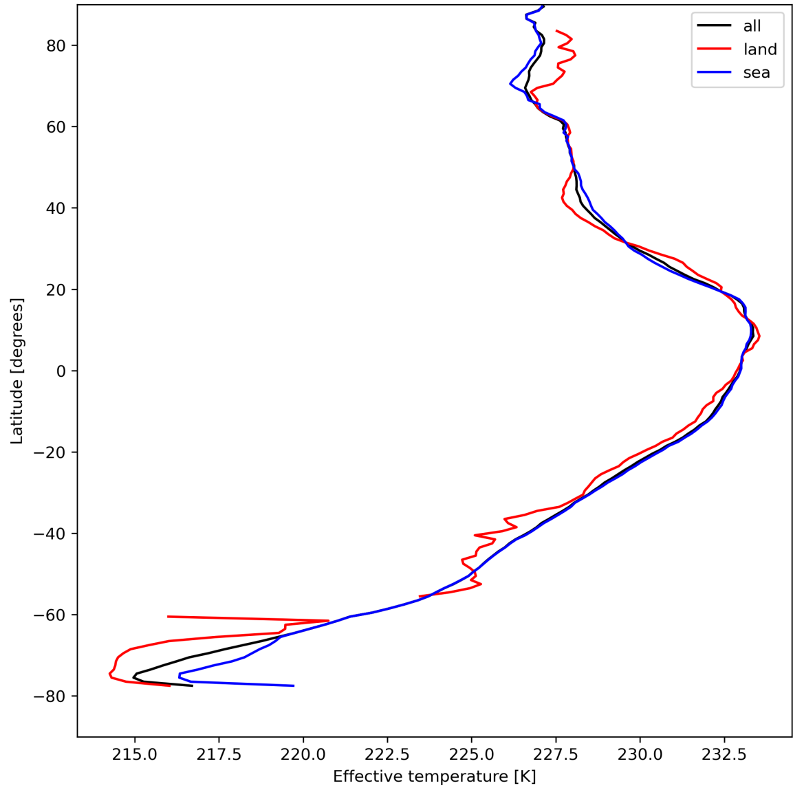
Figure 17: Zonal average of "Effective temperature" for 2024-04-19 to 2024-04-21.
