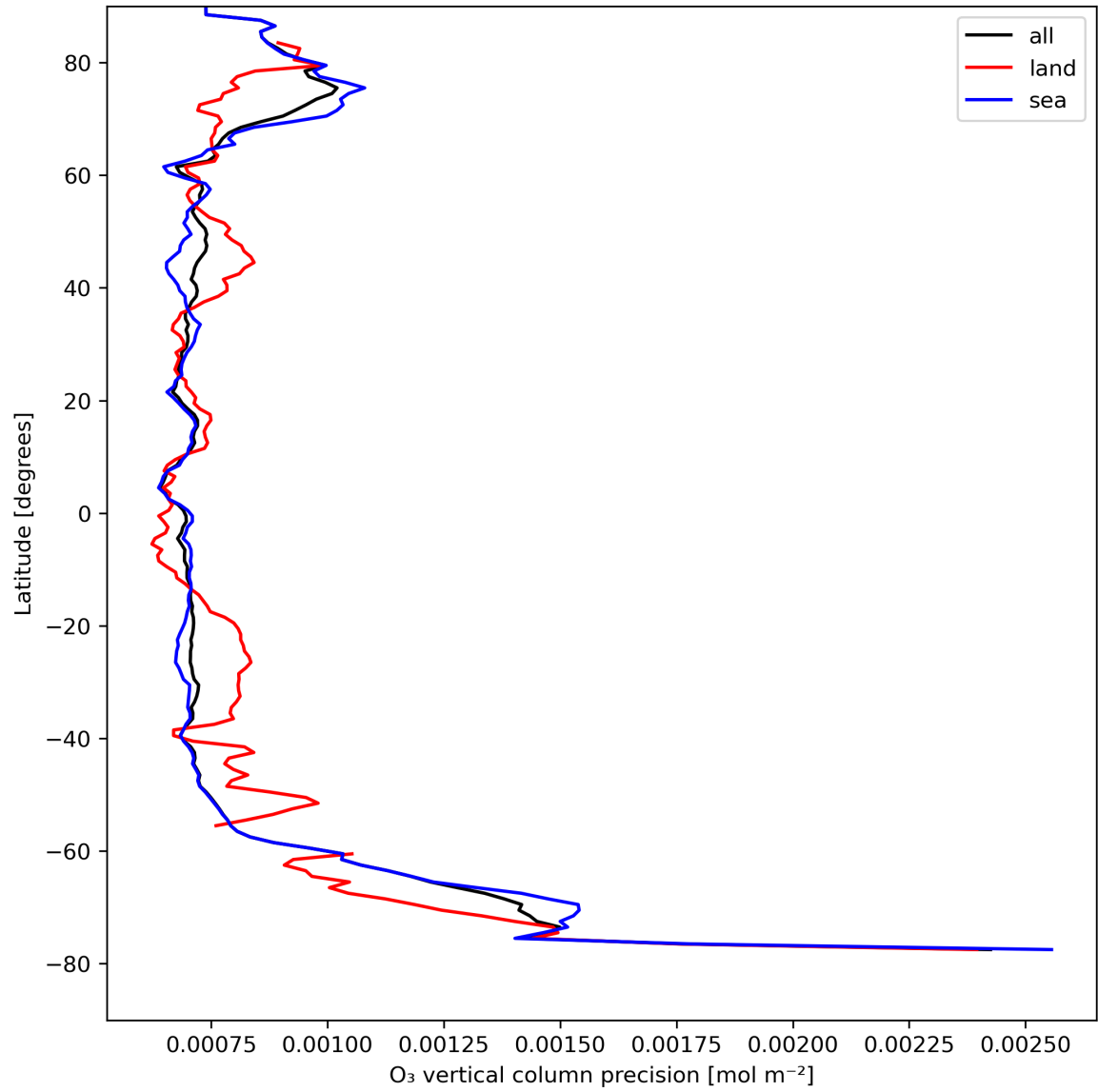
Figure 15: Zonal average of “O 3 vertical column precision” for 2024-04-19 to 2024-04-21.
