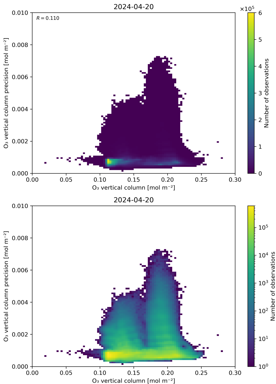
Figure 41: Scatter density plot of “O 3 vertical column” against “O 3 vertical column precision” for 2024-04-19 to 2024-04-21.
