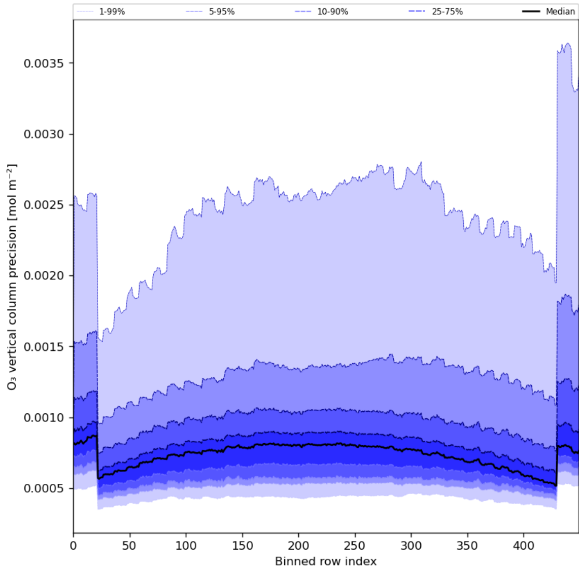
Figure 29: Along track statistics of “O 3 vertical column precision” for 2024-04-19 to 2024-04-21
