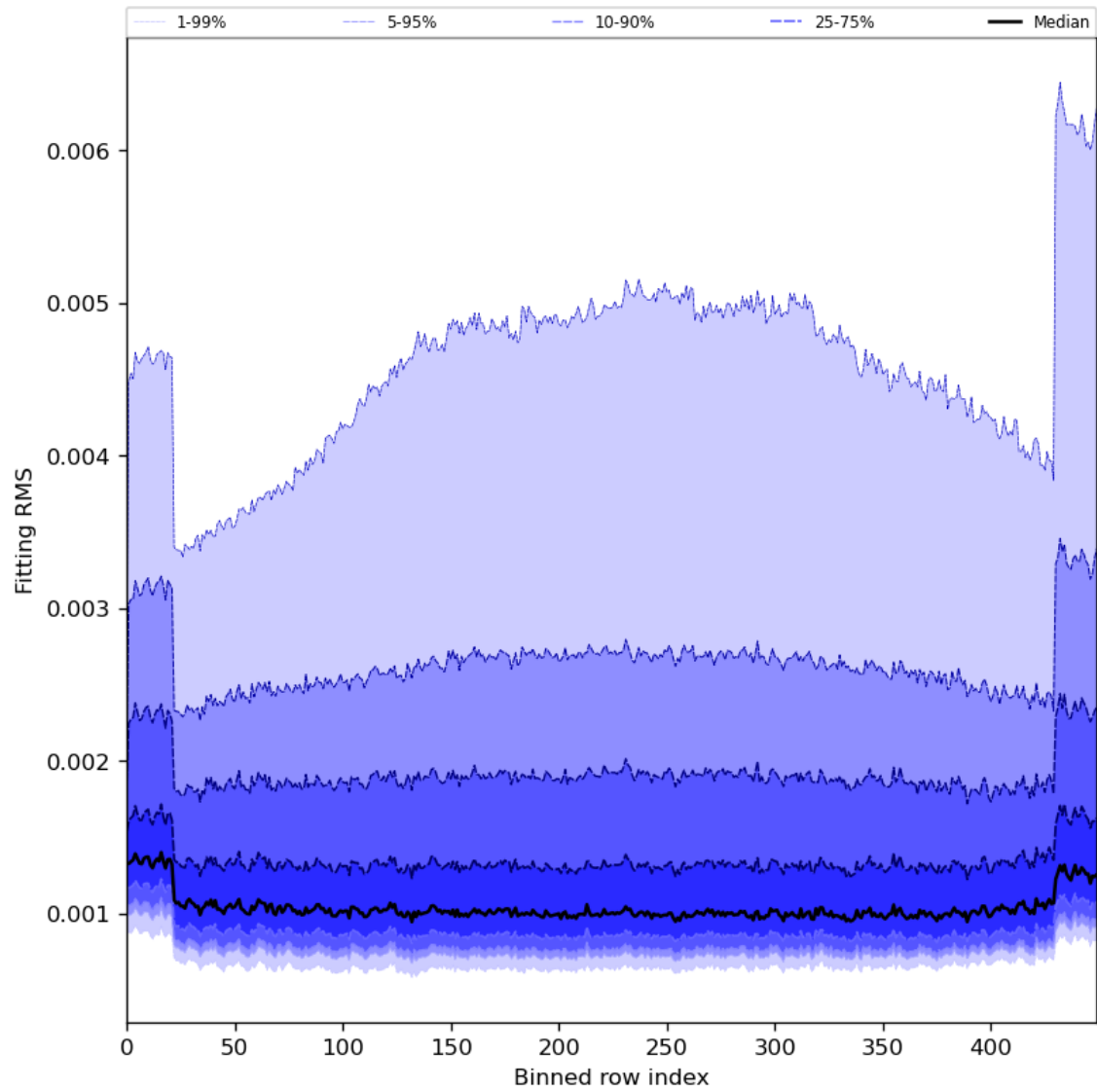
Figure 30: Along track statistics of “Fitting RMS” for 2024-04-19 to 2024-04-21
