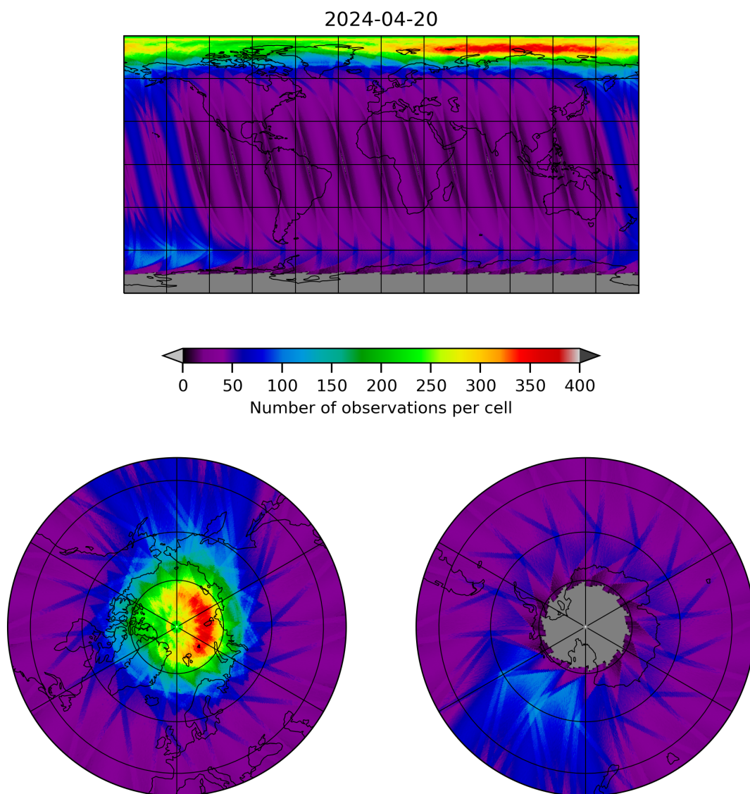
Figure 12: Map of the number of observations for 2024-04-19 to 2024-04-21
