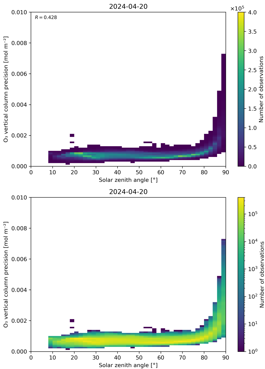
Figure 48: Scatter density plot of “Solar zenith angle” against “O 3 vertical column precision” for 2024-04-19 to 2024-04-21.
