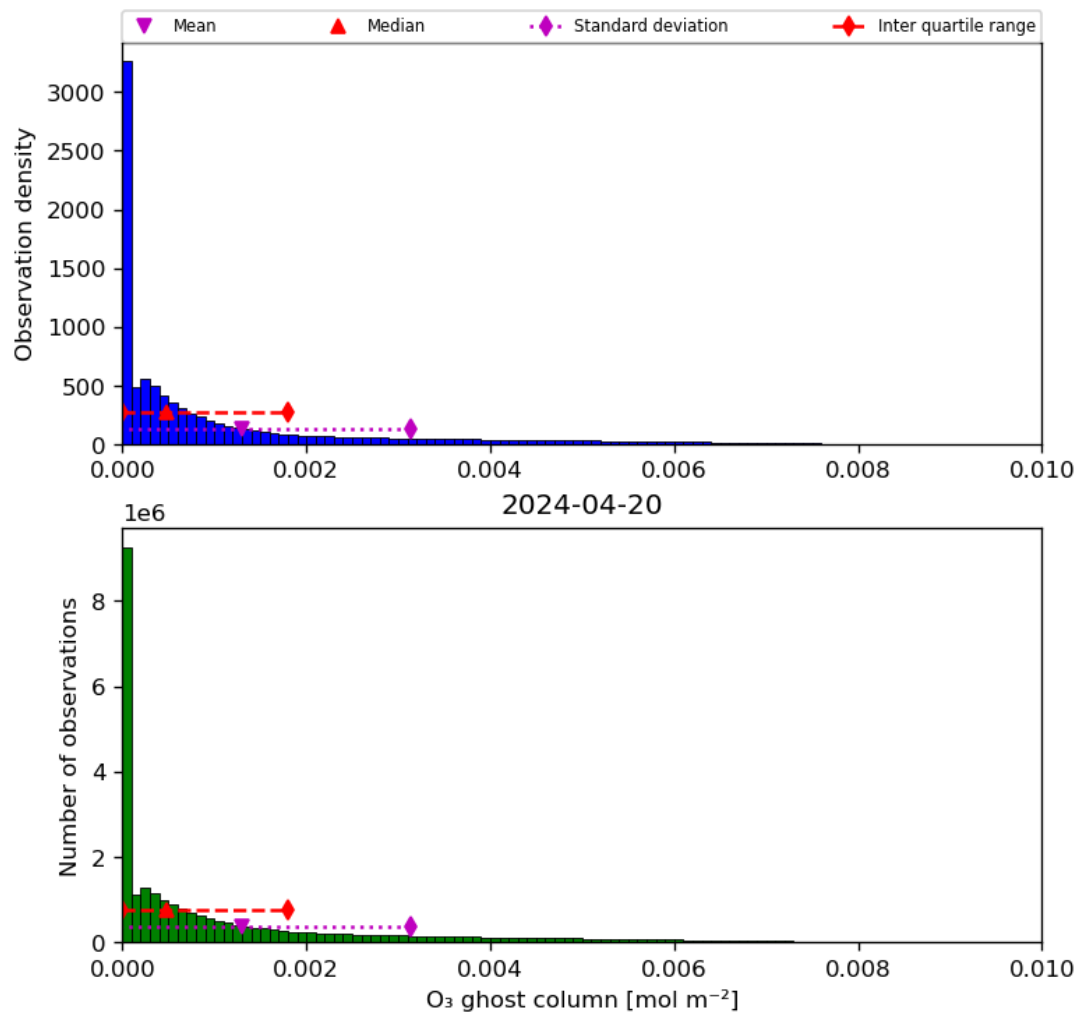
Figure 25: Histogram of “O 3 ghost column” for 2024-04-19 to 2024-04-21
