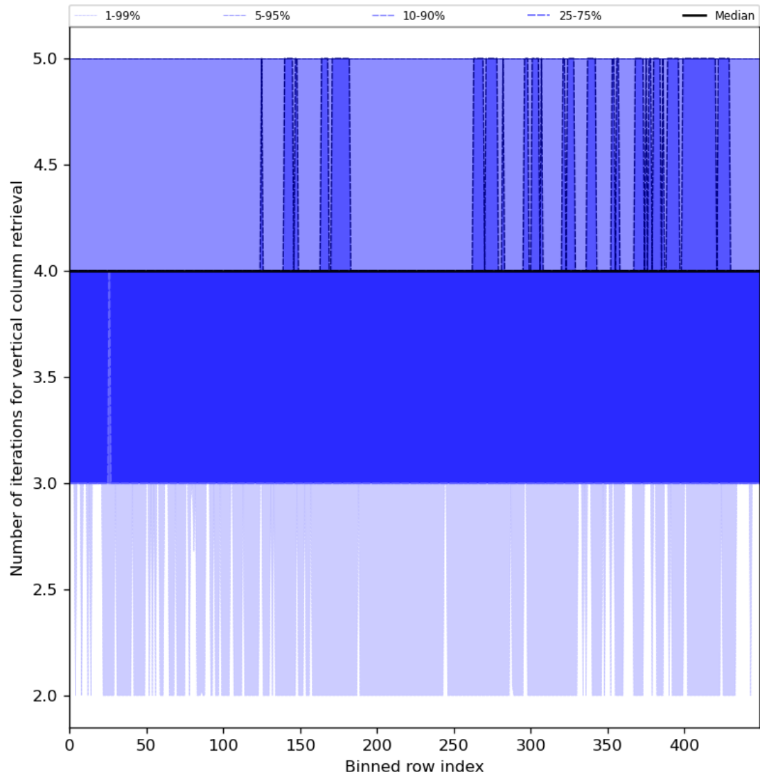
Figure 33: Along track statistics of “Number of iterations for vertical column retrieval” for 2024-04-19 to 2024-04-21
