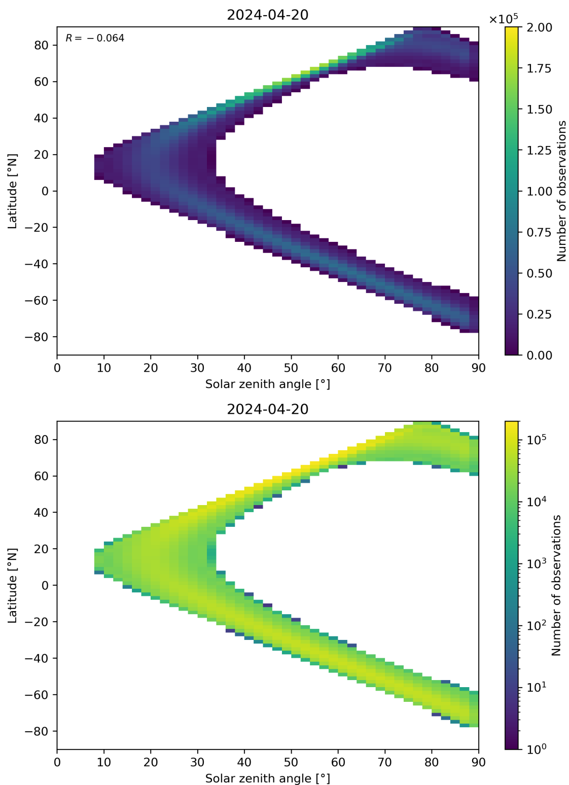
Figure 44: Scatter density plot of “Solar zenith angle” against “Latitude” for 2024-04-19 to 2024-04-21.
