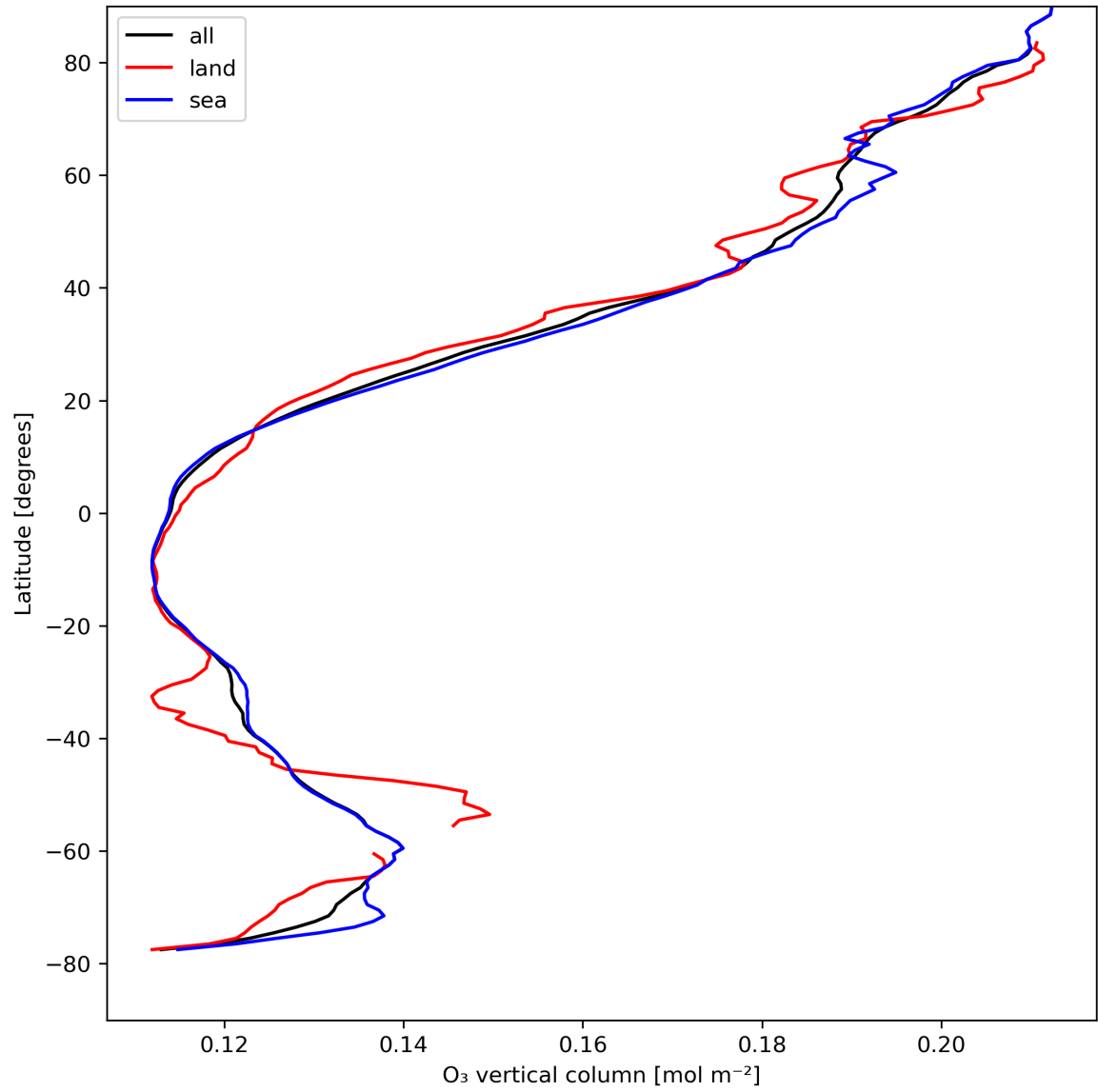
Figure 14: Zonal average of “O 3 vertical column” for 2024-04-19 to 2024-04-21.
