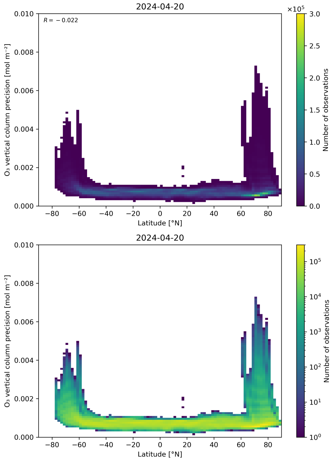
Figure 37: Scatter density plot of “Latitude” against “O 3 vertical column precision” for 2024-04-19 to 2024-04-21.
