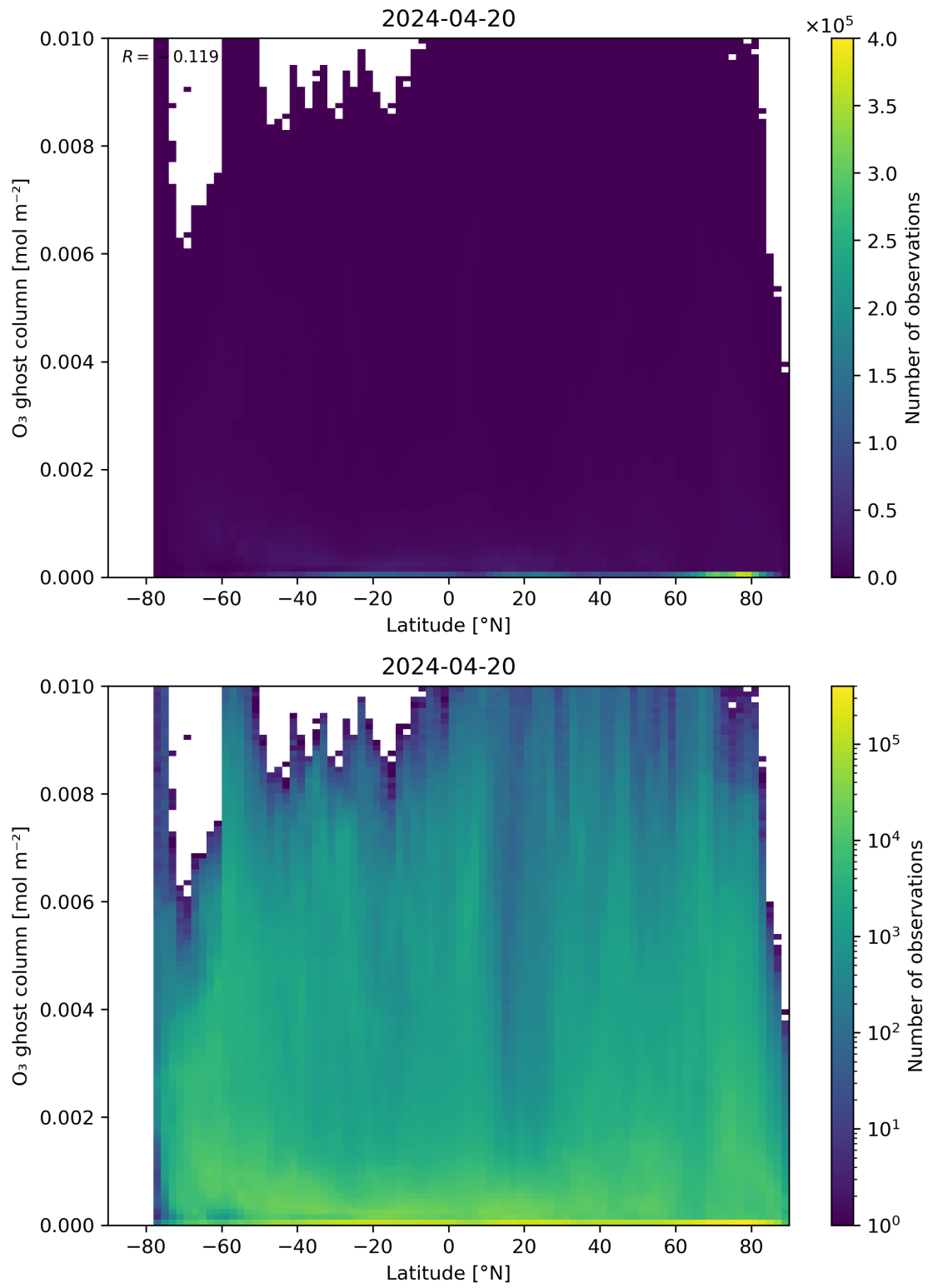
Figure 35: Scatter density plot of “Latitude” against “O 3 ghost column” for 2024-04-19 to 2024-04-21.
