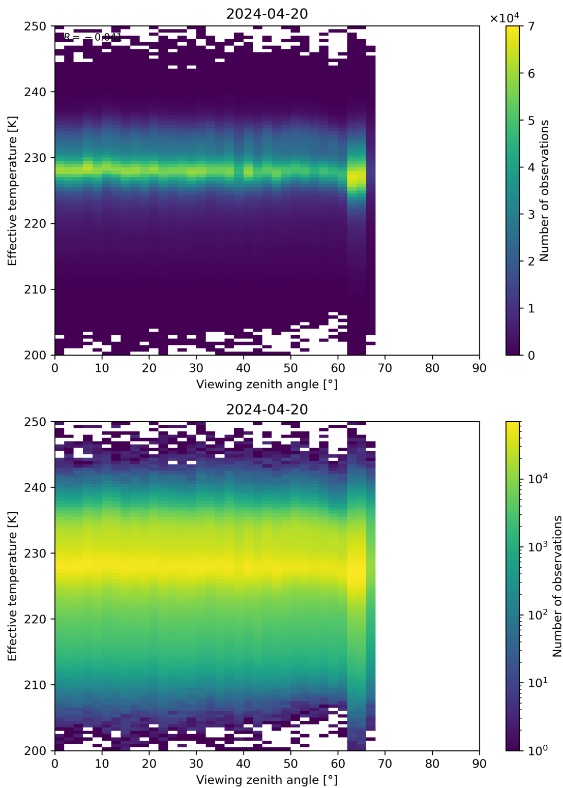
Figure 50: Scatter density plot of “Viewing zenith angle” against “Effective temperature” for 2024-04-19 to 2024-04-21.
