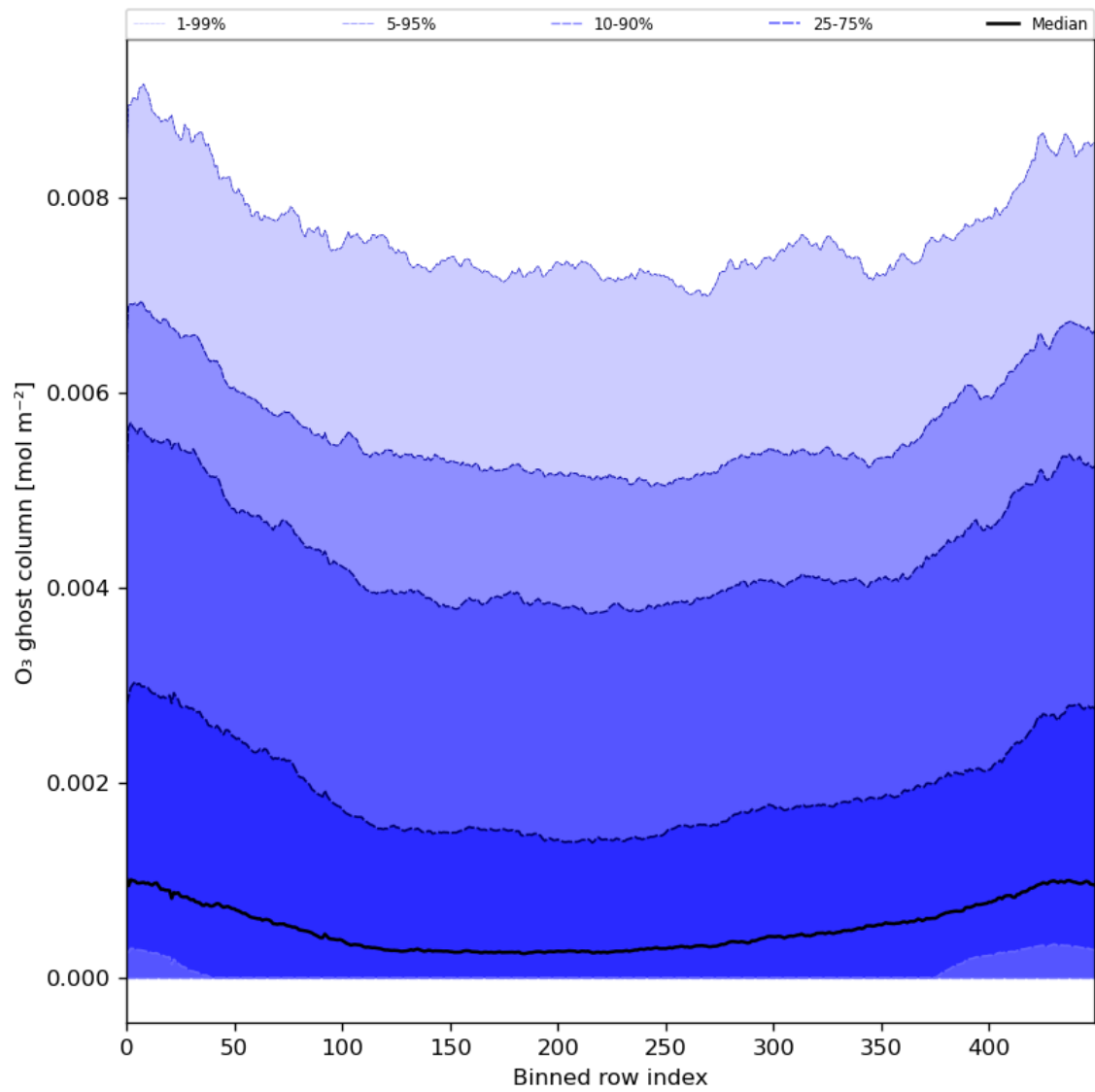
Figure 32: Along track statistics of “O 3 ghost column” for 2024-04-21 to 2024-04-22
