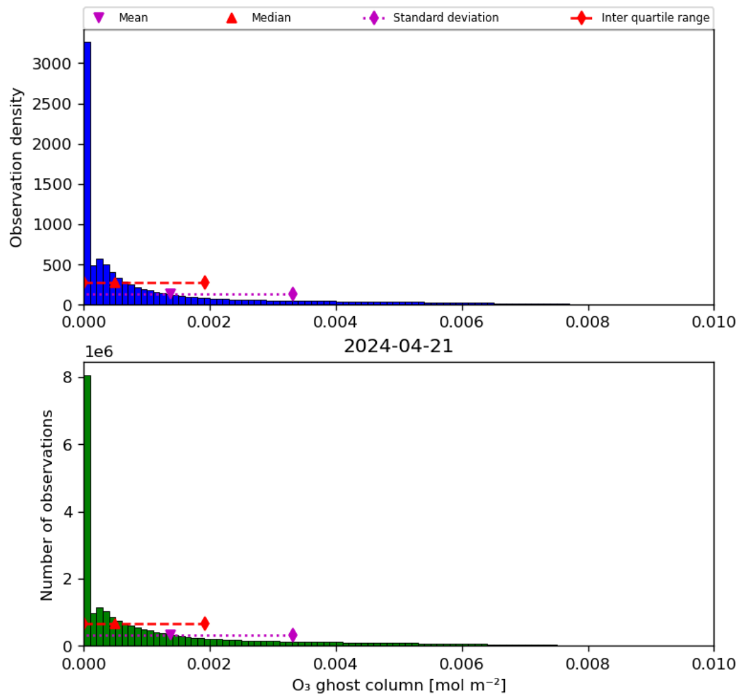
Figure 25: Histogram of “O 3 ghost column” for 2024-04-21 to 2024-04-22
