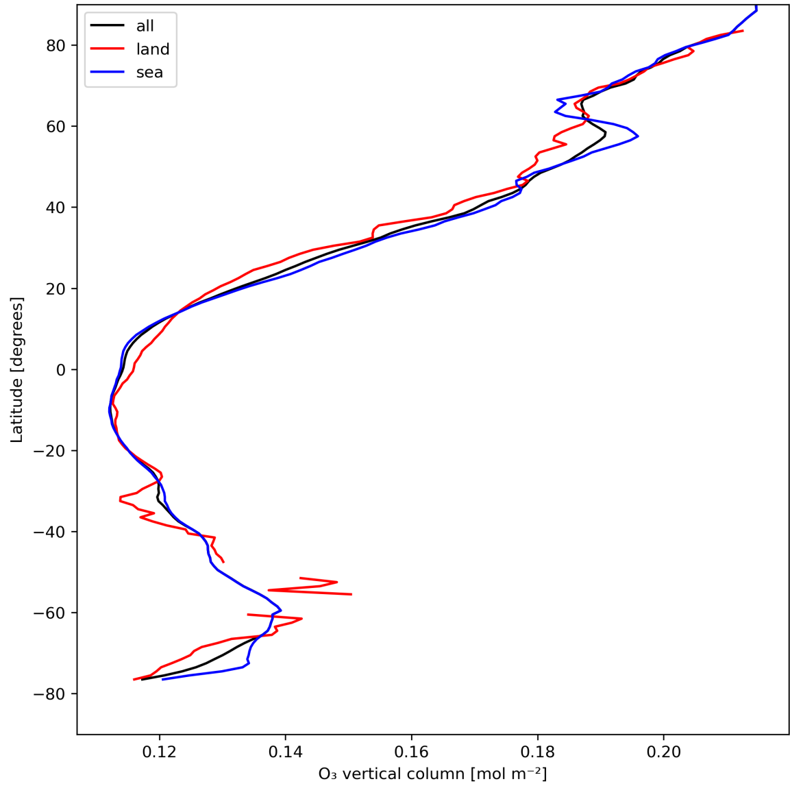
Figure 14: Zonal average of “O 3 vertical column” for 2024-04-21 to 2024-04-22.
