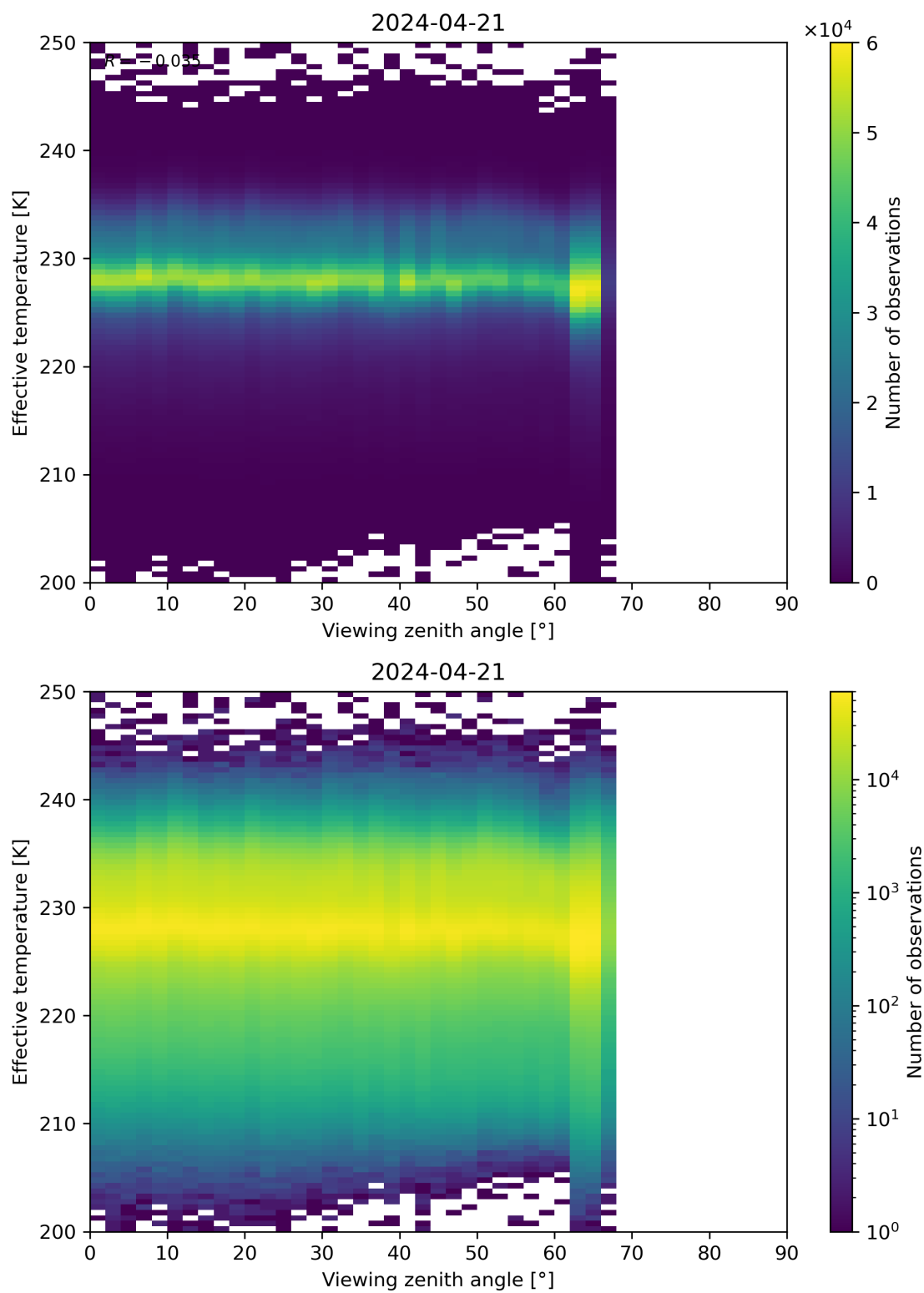
Figure 50: Scatter density plot of “Viewing zenith angle” against “Effective temperature” for 2024-04-21 to 2024-04-22.
