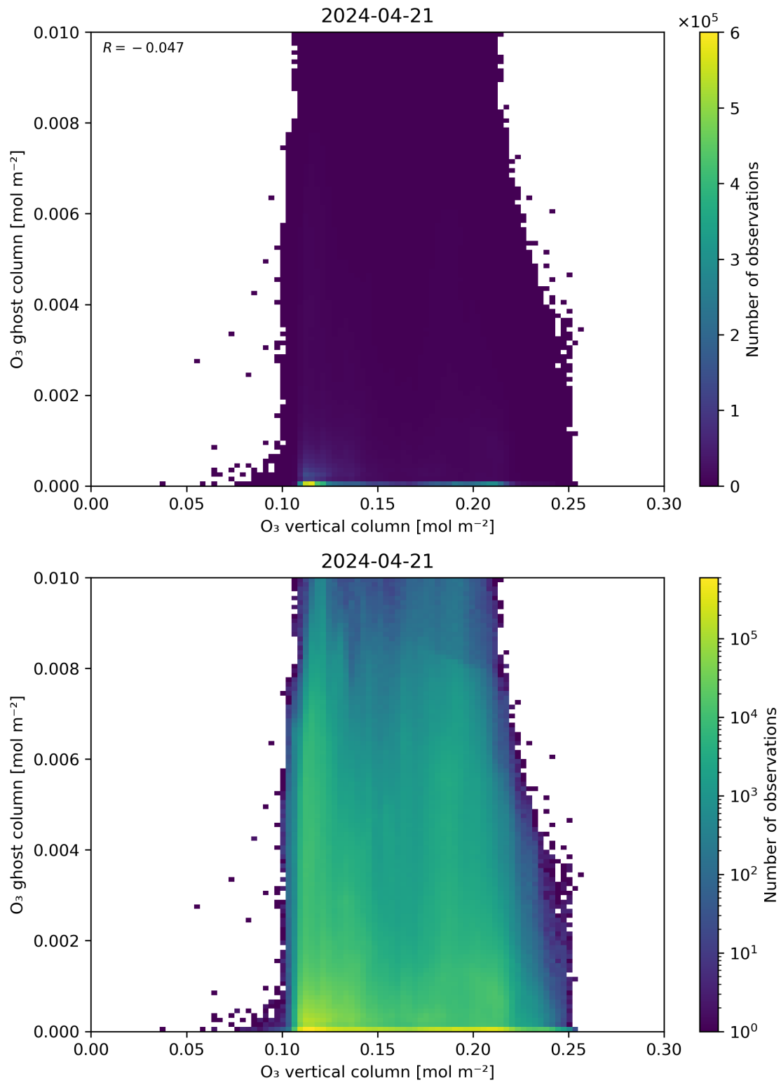
Figure 40: Scatter density plot of “O 3 vertical column” against “O 3 ghost column” for 2024-04-21 to 2024-04-22.
