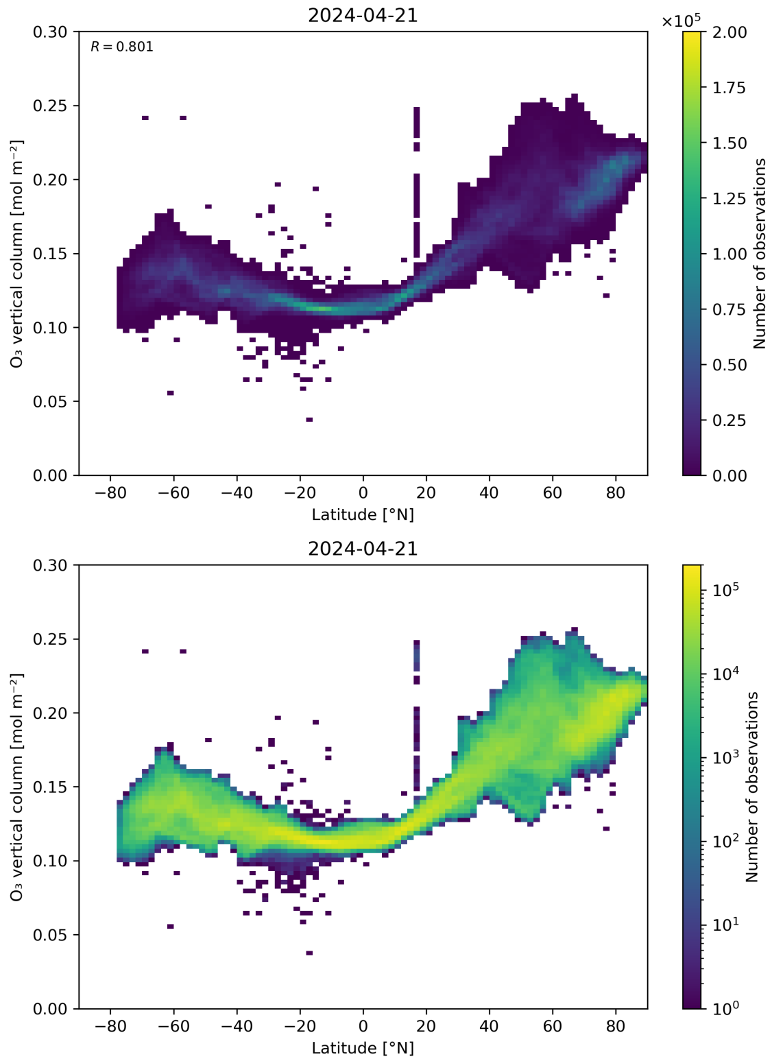
Figure 36: Scatter density plot of “Latitude” against “O 3 vertical column” for 2024-04-21 to 2024-04-22.
