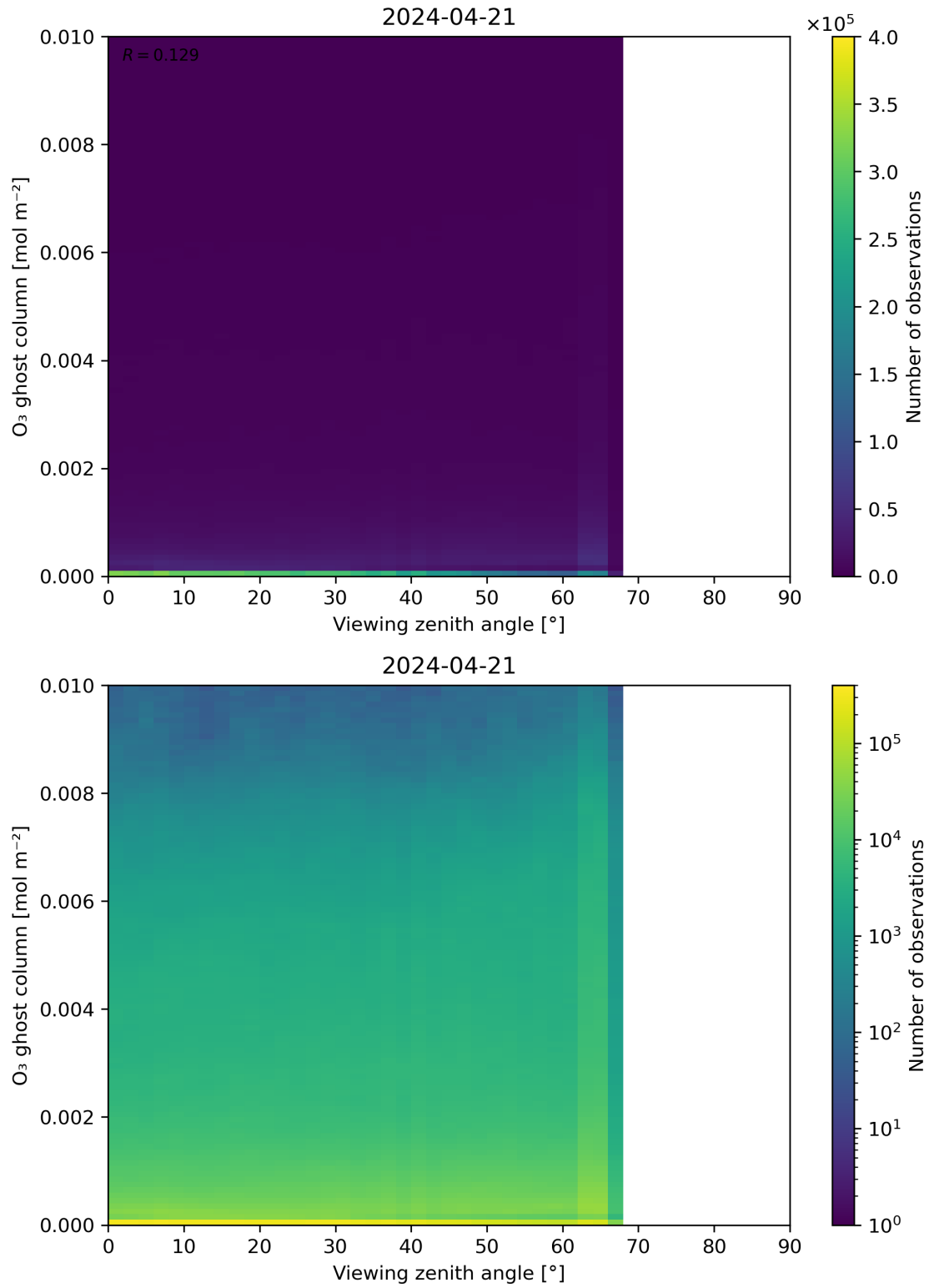
Figure 51: Scatter density plot of “Viewing zenith angle” against “O 3 ghost column” for 2024-04-21 to 2024-04-22.
