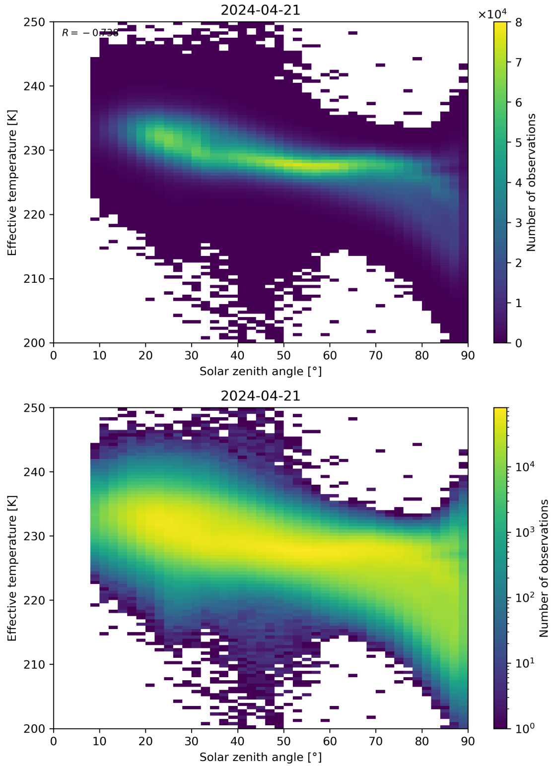
Figure 45: Scatter density plot of “Solar zenith angle” against “Effective temperature” for 2024-04-21 to 2024-04-22.
