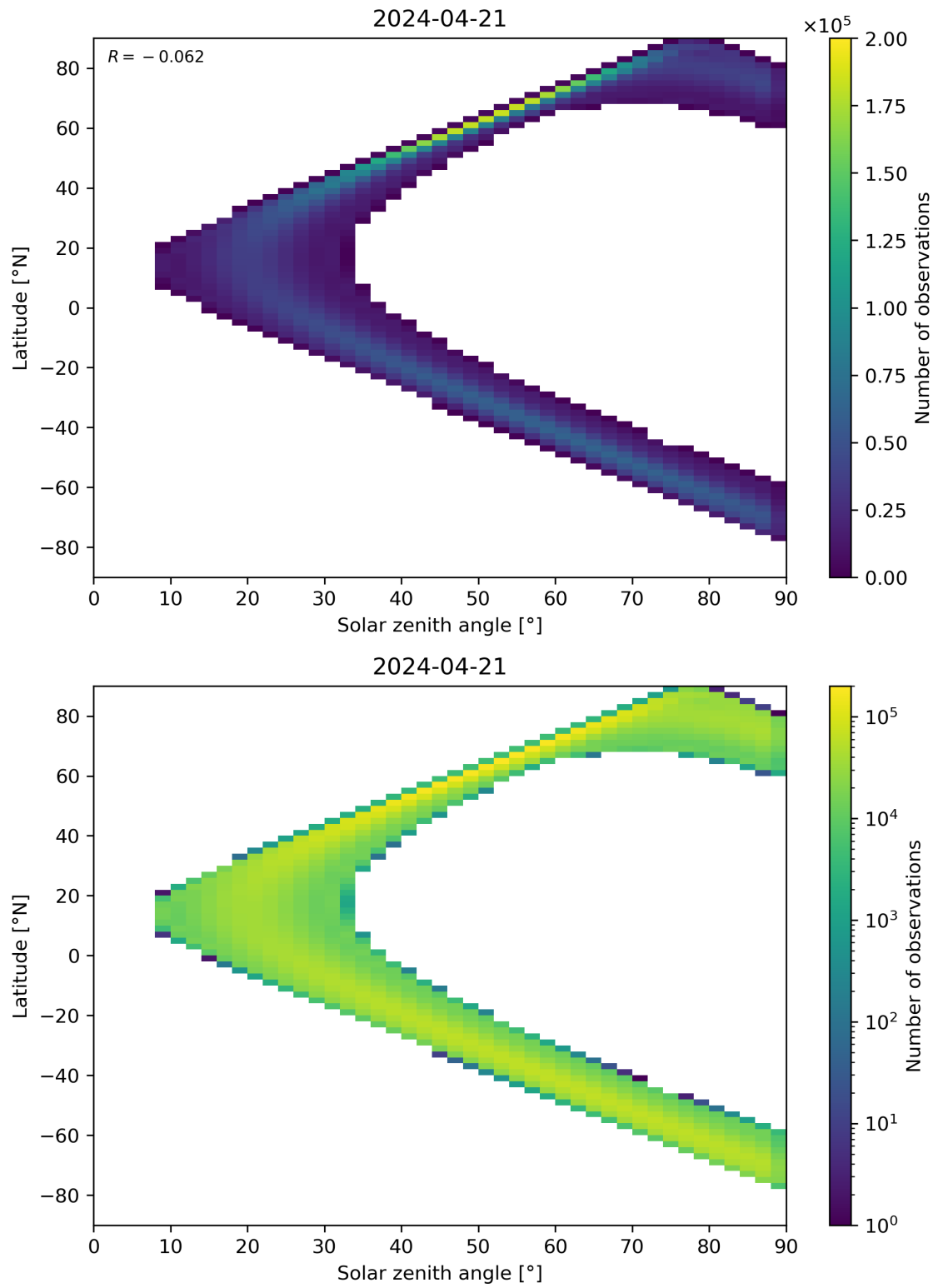
Figure 44: Scatter density plot of “Solar zenith angle” against “Latitude” for 2024-04-21 to 2024-04-22.
