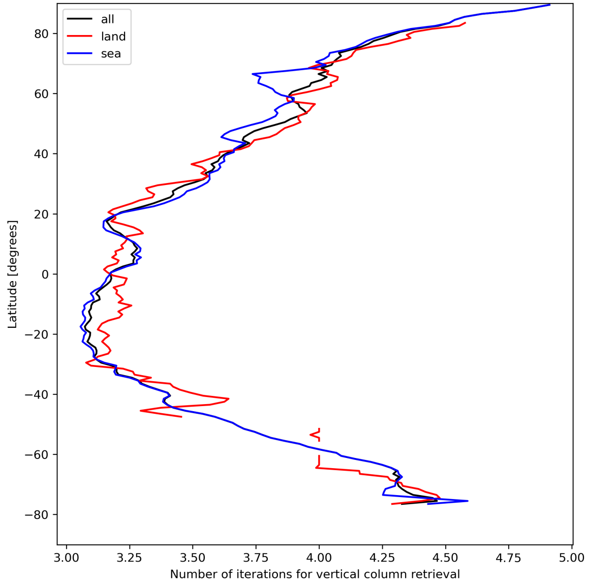
Figure 19: Zonal average of “Number of iterations for vertical column retrieval” for 2024-04-21 to 2024-04-22.
