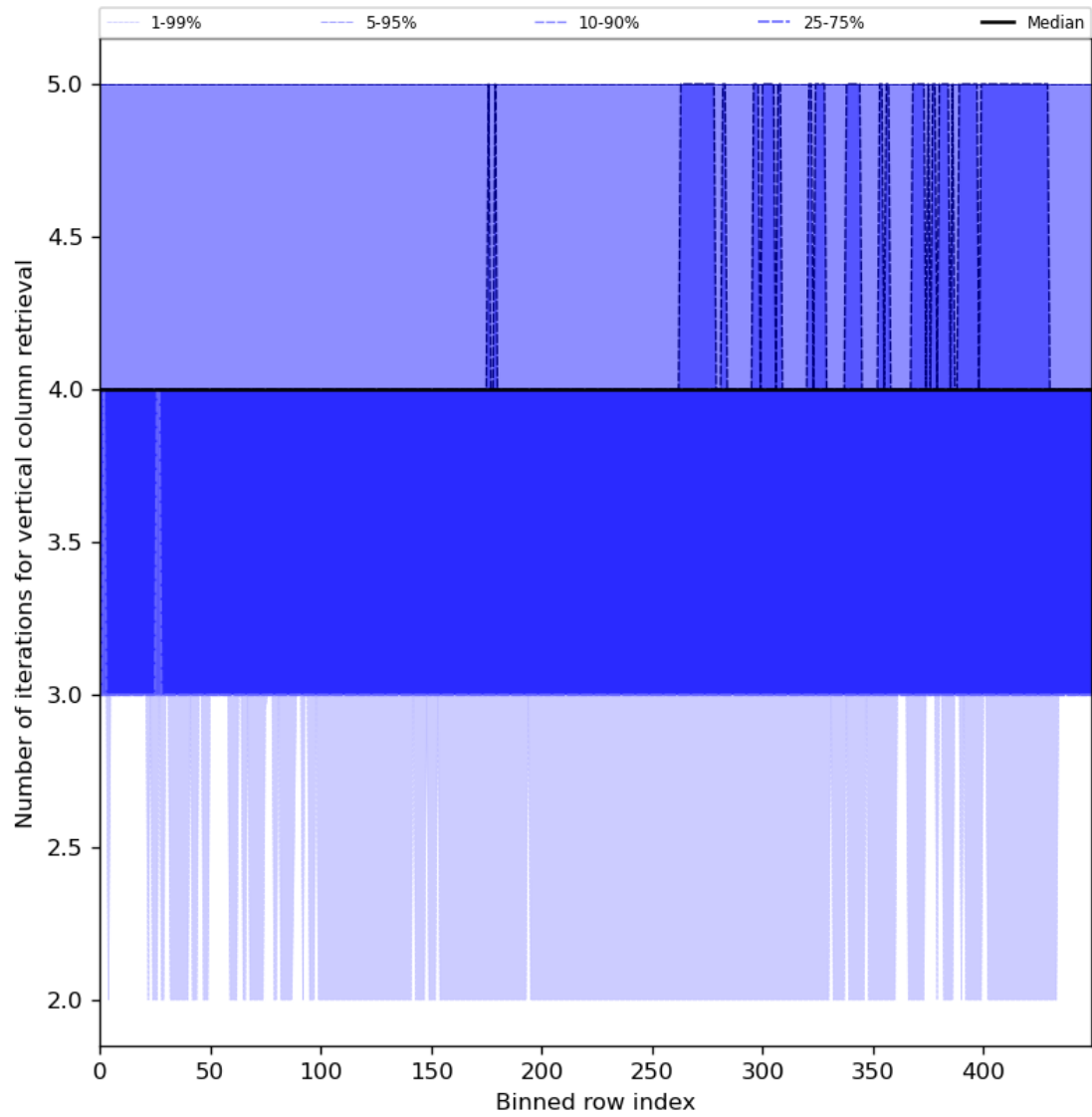
Figure 33: Along track statistics of “Number of iterations for vertical column retrieval” for 2024-04-21 to 2024-04-22
