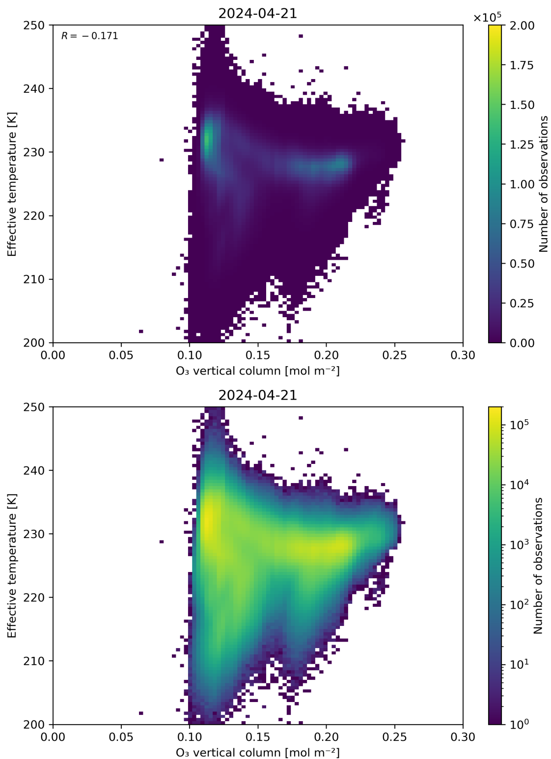
Figure 39: Scatter density plot of “O 3 vertical column” against “Effective temperature” for 2024-04-21 to 2024-04-22.
