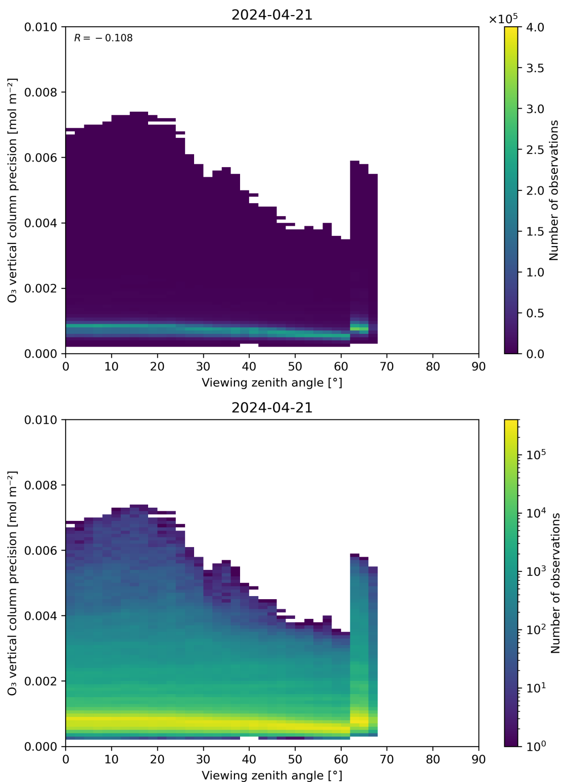
Figure 53: Scatter density plot of “Viewing zenith angle” against “O 3 vertical column precision” for 2024-04-21 to 2024-04-22.
