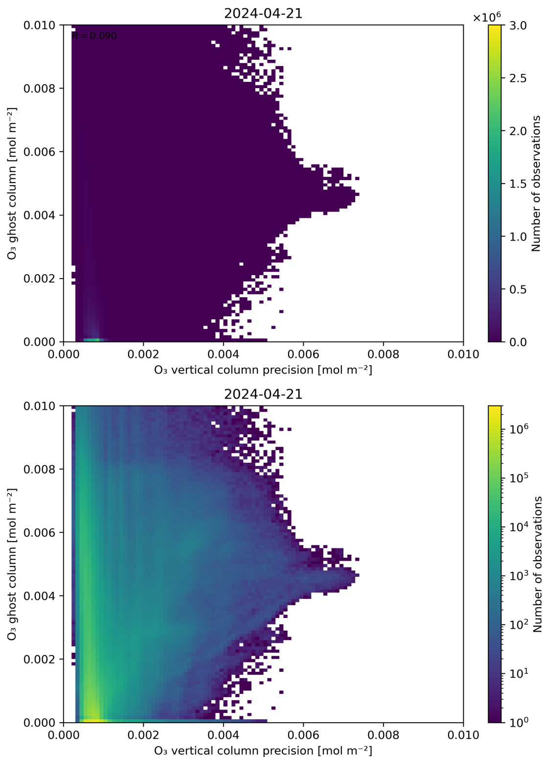
Figure 43: Scatter density plot of “O 3 vertical column precision” against “O 3 ghost column” for 2024-04-21 to 2024-04-22.
