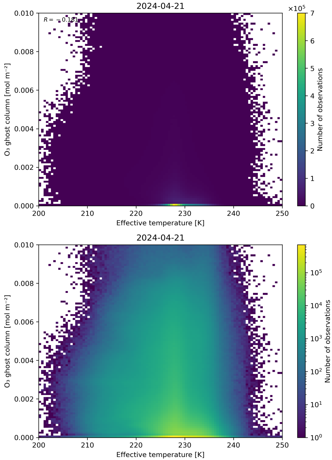
Figure 38: Scatter density plot of “Effective temperature” against “O 3 ghost column” for 2024-04-21 to 2024-04-22.
