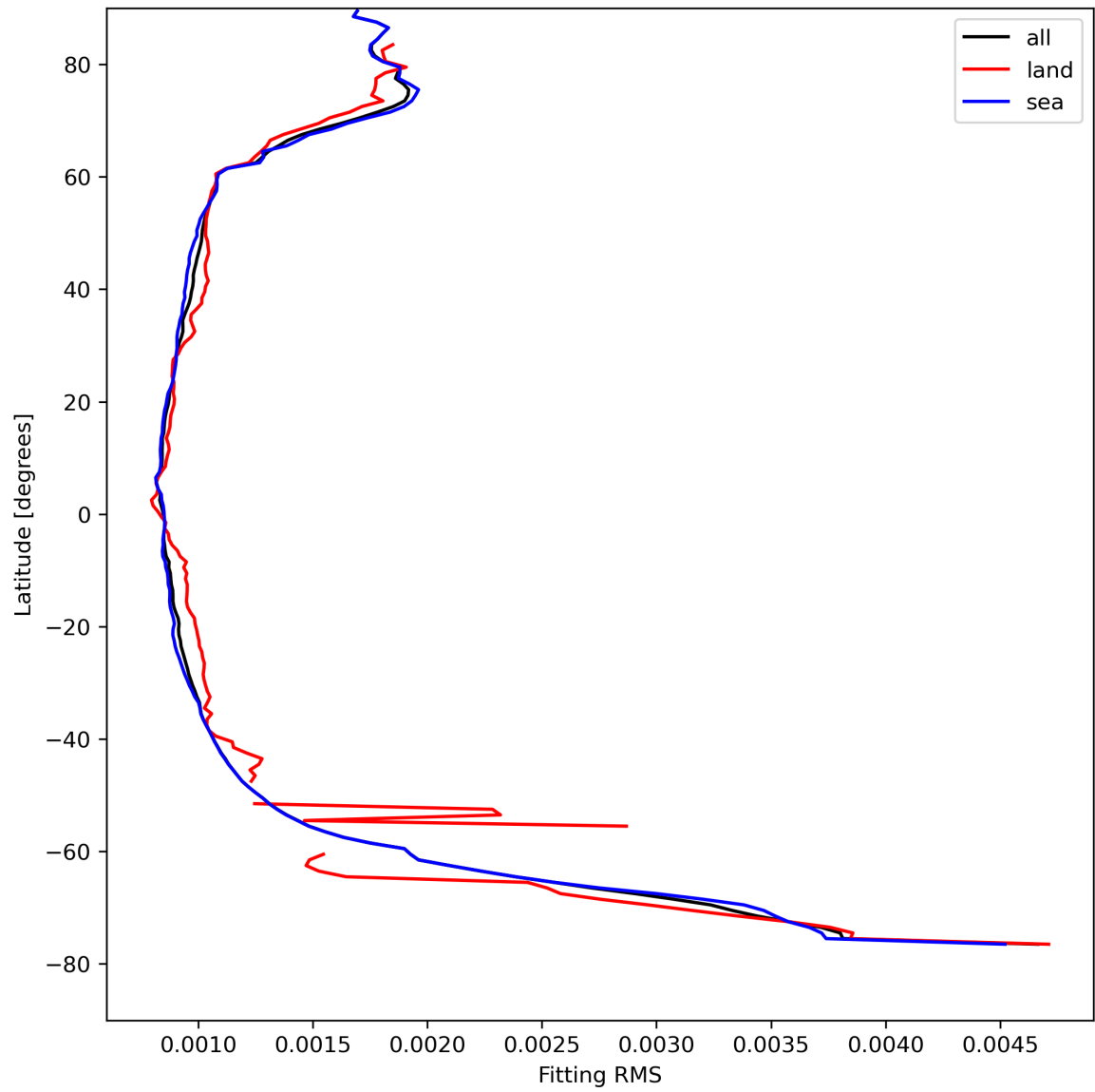
Figure 16: Zonal average of “Fitting RMS” for 2024-04-21 to 2024-04-22.
