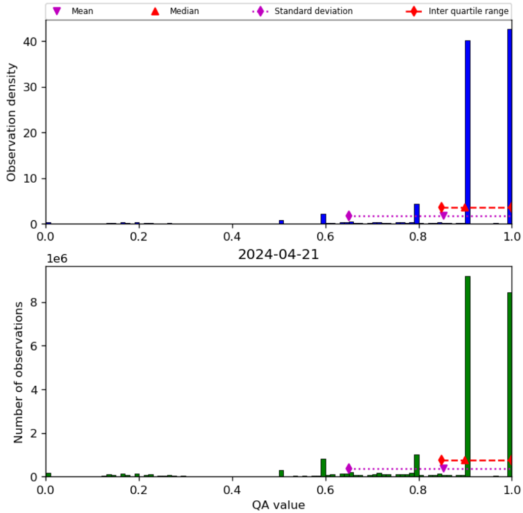
Figure 20: Histogram of “QA value” for 2024-04-21 to 2024-04-22
