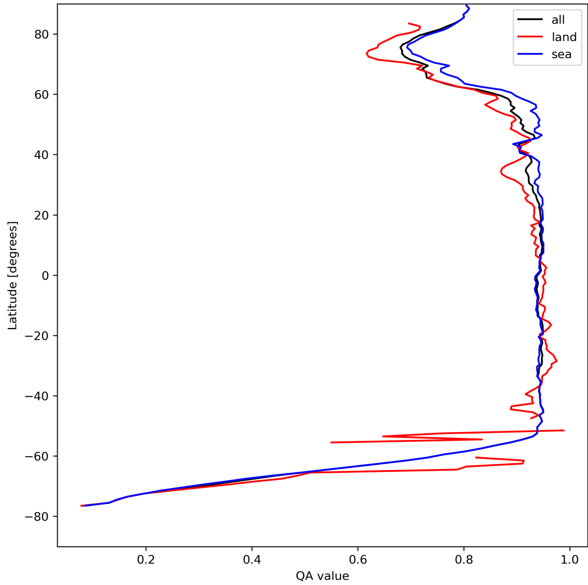
Figure 13: Zonal average of “QA value” for 2024-04-21 to 2024-04-22.
