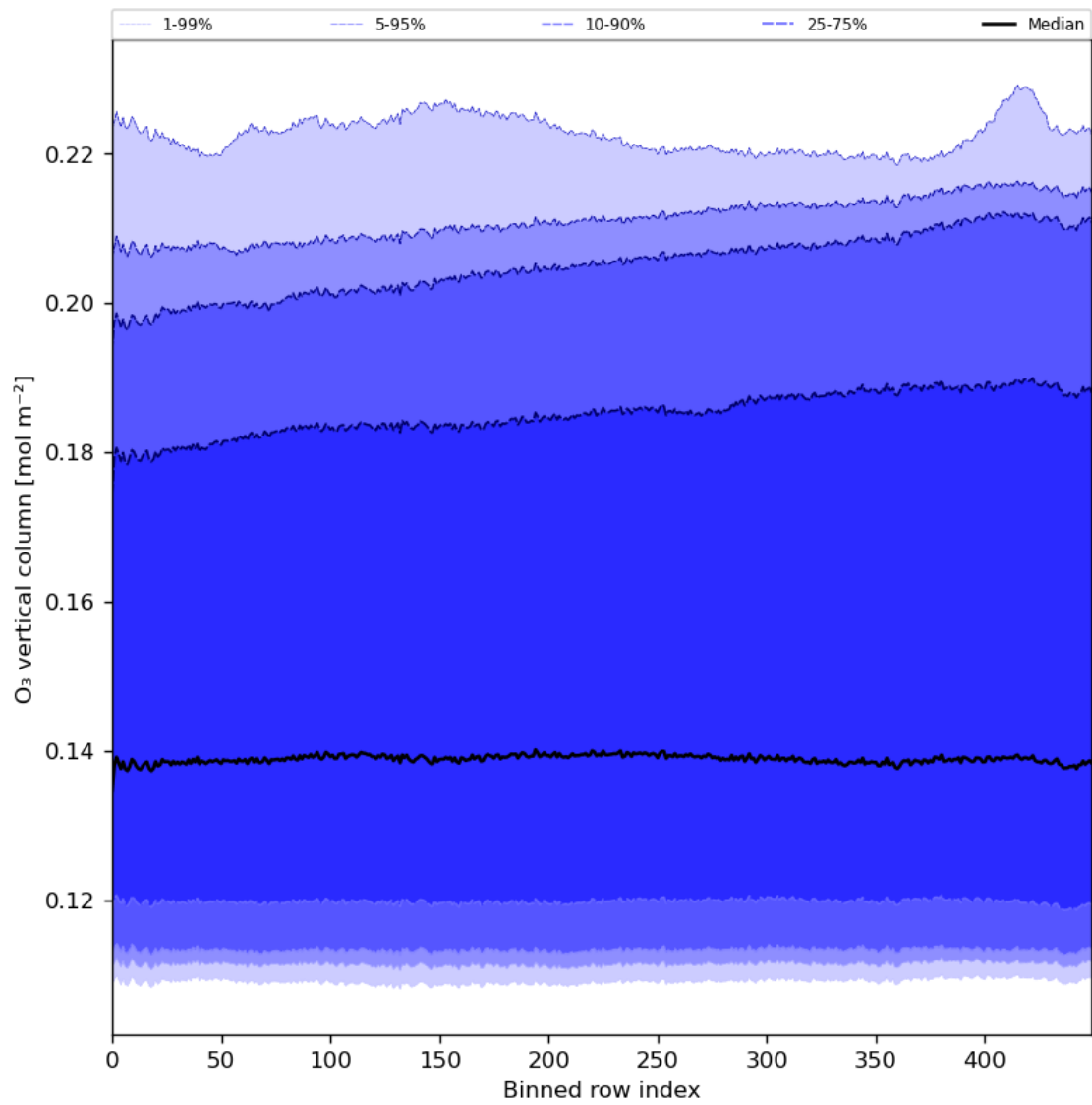
Figure 28: Along track statistics of “O 3 vertical column” for 2024-04-21 to 2024-04-22
