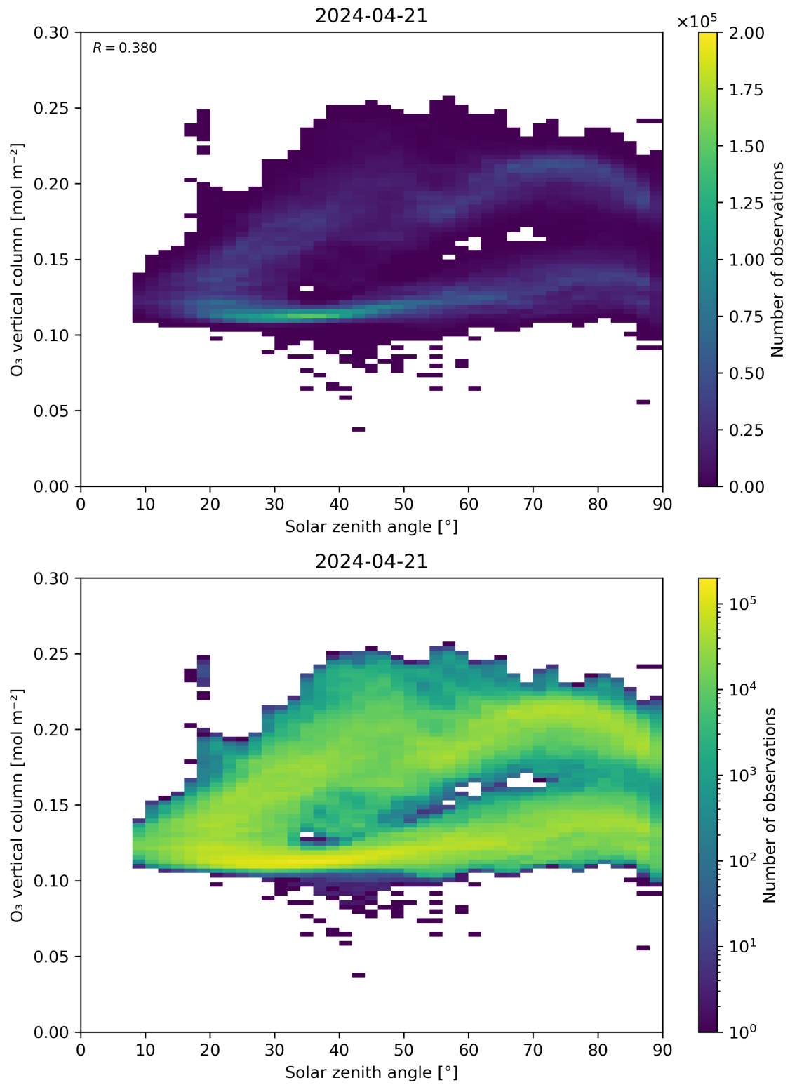
Figure 47: Scatter density plot of “Solar zenith angle” against “O 3 vertical column” for 2024-04-21 to 2024-04-22.
