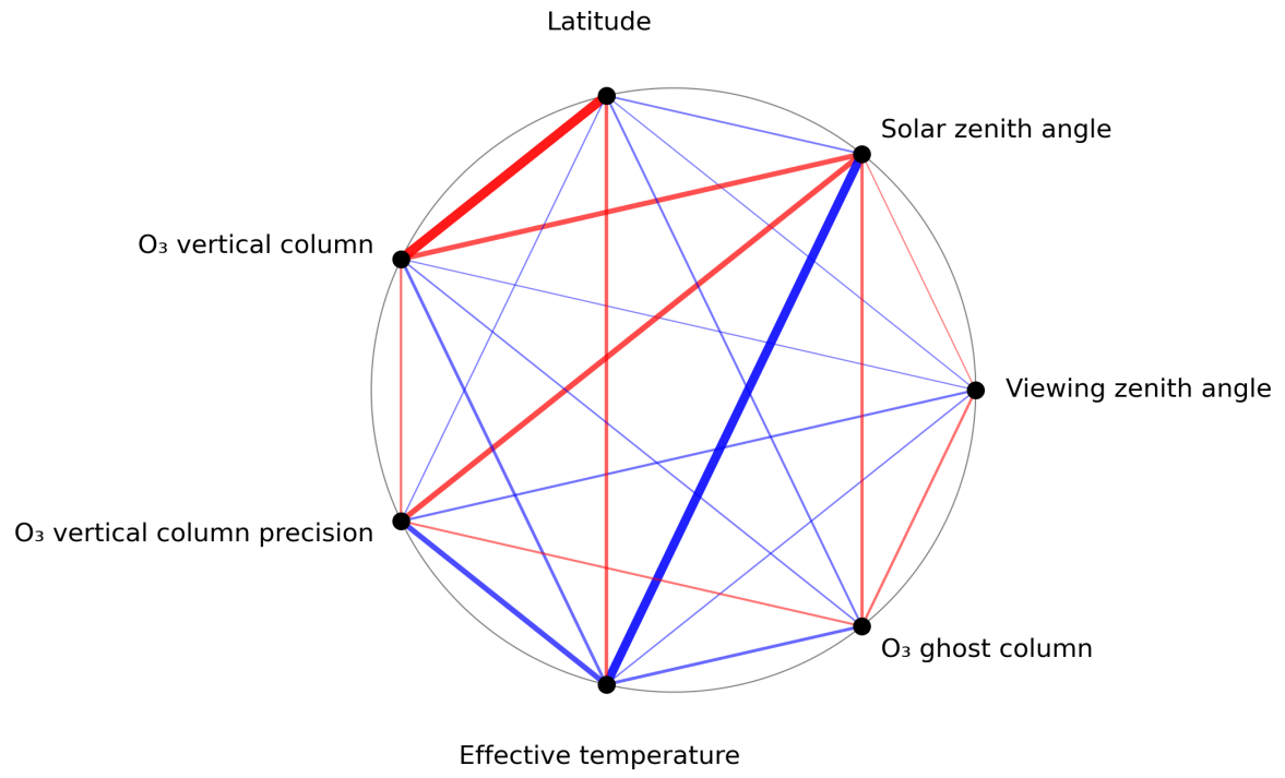
Figure 1: Map of correlation graph for 2024-04-21 to 2024-04-22.
