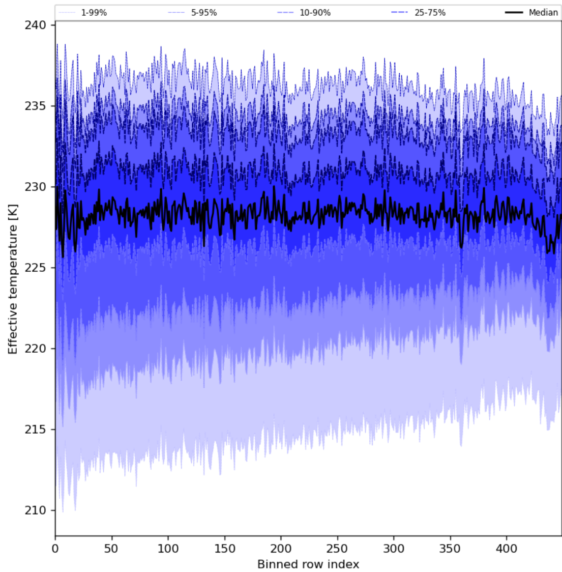
Figure 31: Along track statistics of “Effective temperature” for 2024-04-21 to 2024-04-22
