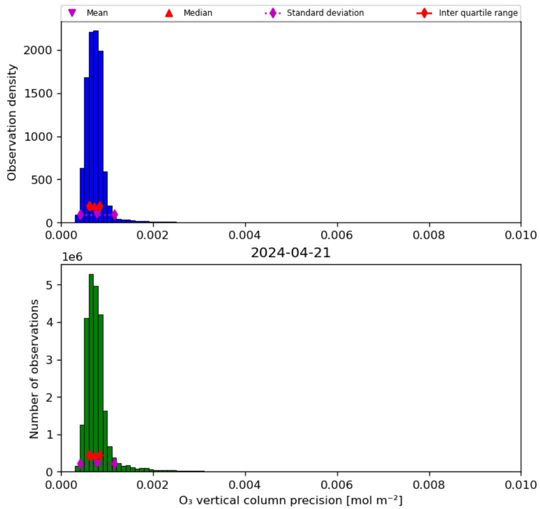
Figure 22: Histogram of “O 3 vertical column precision” for 2024-04-21 to 2024-04-22
