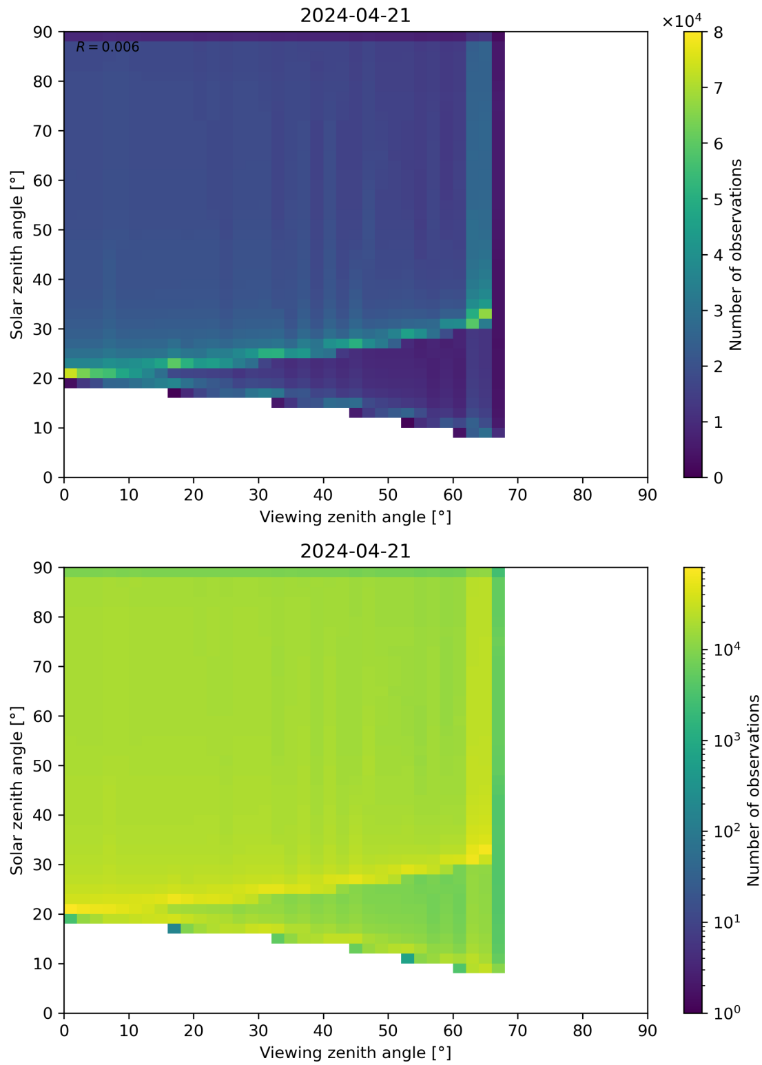
Figure 54: Scatter density plot of “Viewing zenith angle” against “Solar zenith angle” for 2024-04-21 to 2024-04-22.
