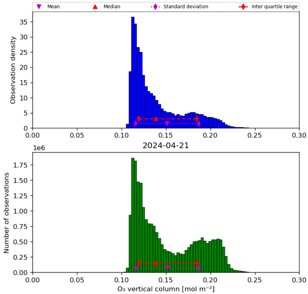
Figure 21: Histogram of “O 3 vertical column” for 2024-04-21 to 2024-04-22
