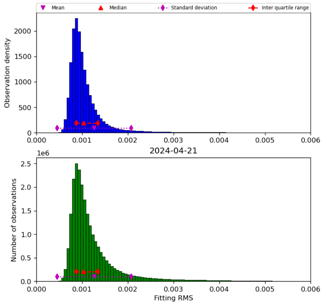
Figure 23: Histogram of “Fitting RMS” for 2024-04-21 to 2024-04-22
