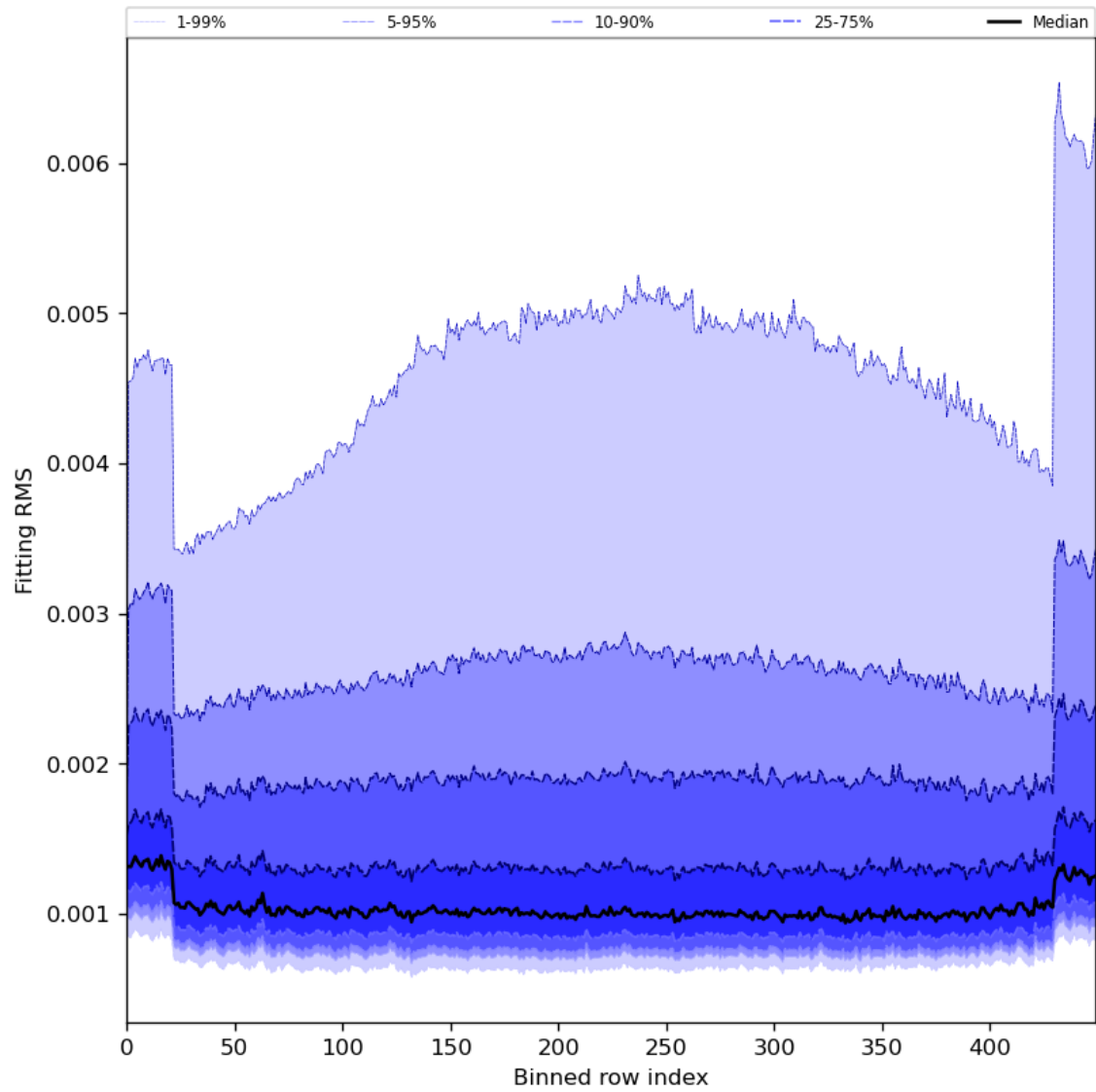
Figure 30: Along track statistics of “Fitting RMS” for 2024-04-21 to 2024-04-22
