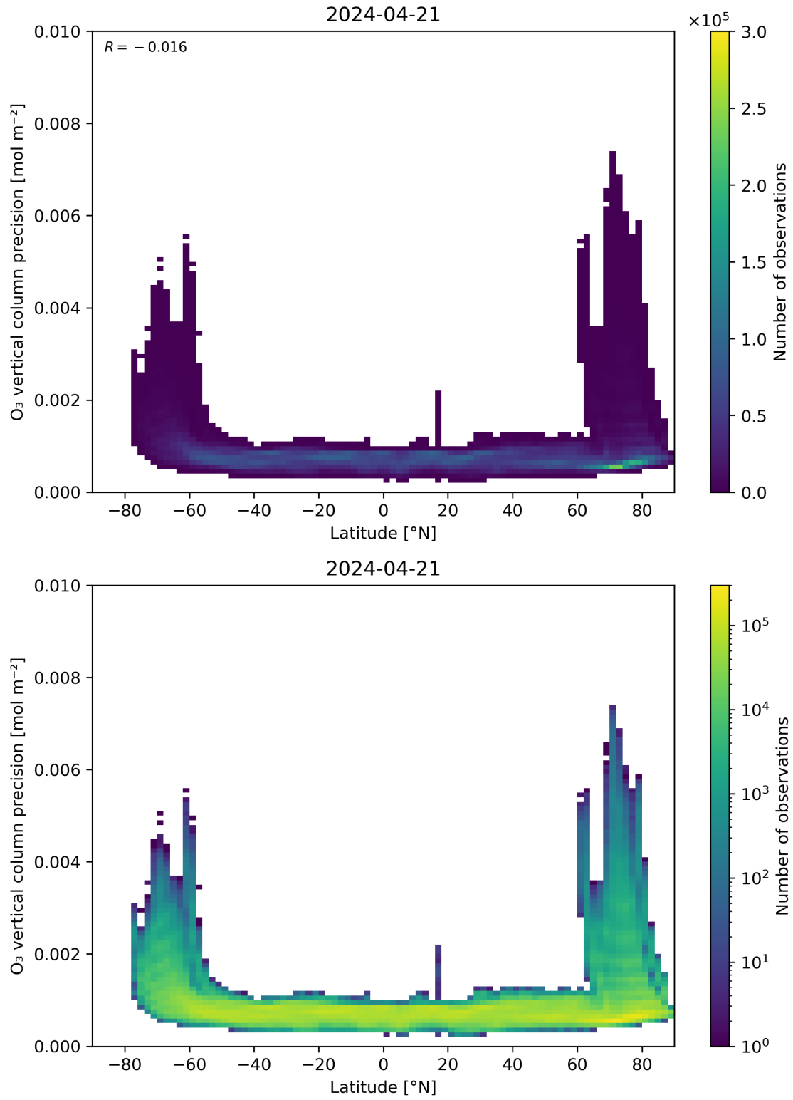
Figure 37: Scatter density plot of “Latitude” against “O 3 vertical column precision” for 2024-04-21 to 2024-04-22.
