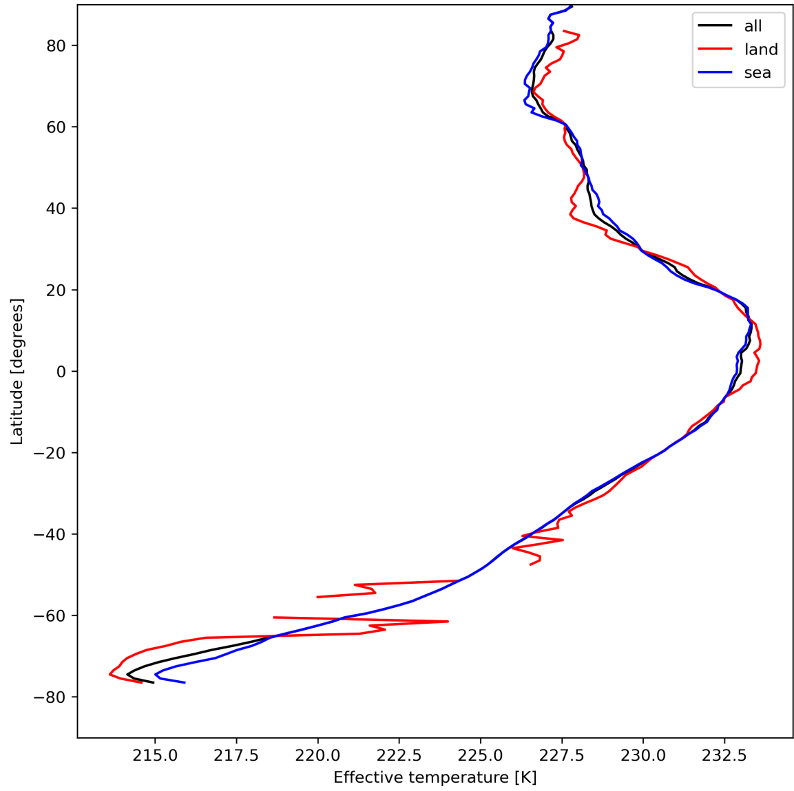
Figure 17: Zonal average of "Effective temperature" for 2024-04-21 to 2024-04-22.
