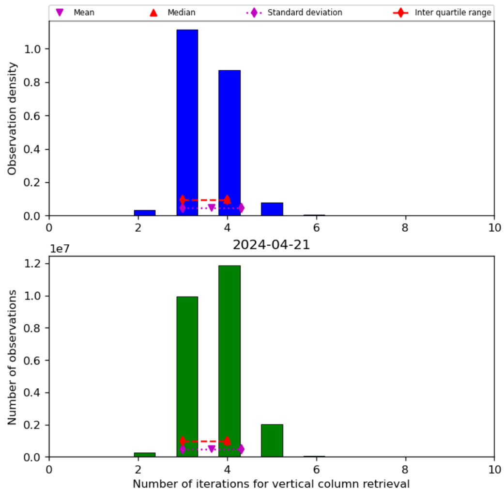
Figure 26: Histogram of “Number of iterations for vertical column retrieval” for 2024-04-21 to 2024-04-22
