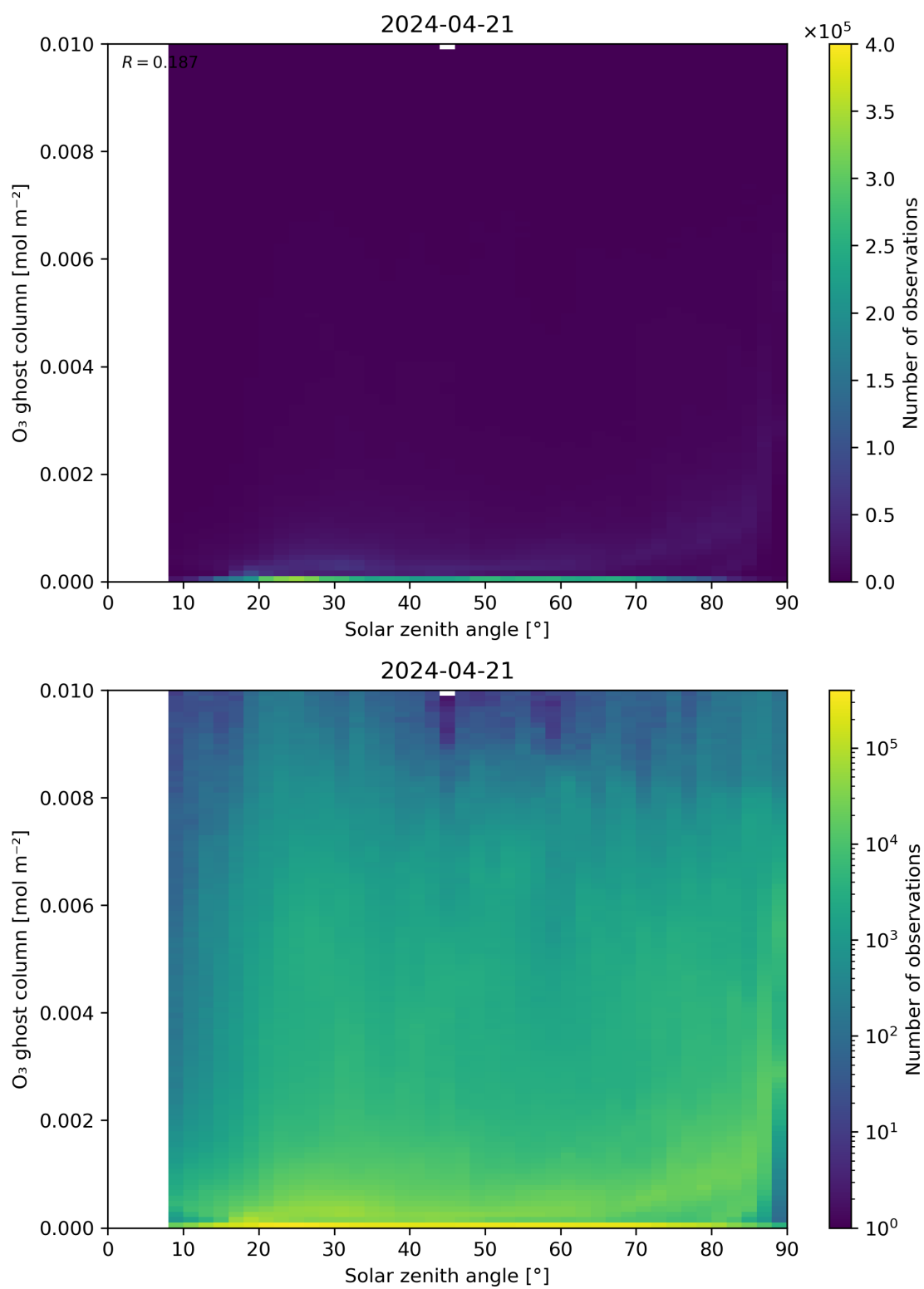
Figure 46: Scatter density plot of “Solar zenith angle” against “O 3 ghost column” for 2024-04-21 to 2024-04-22.
