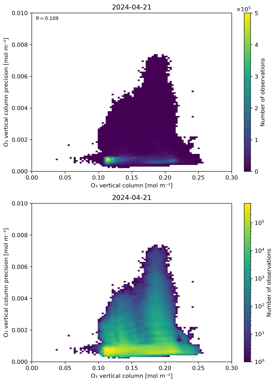
Figure 41: Scatter density plot of “O 3 vertical column” against “O 3 vertical column precision” for 2024-04-21 to 2024-04-22.
