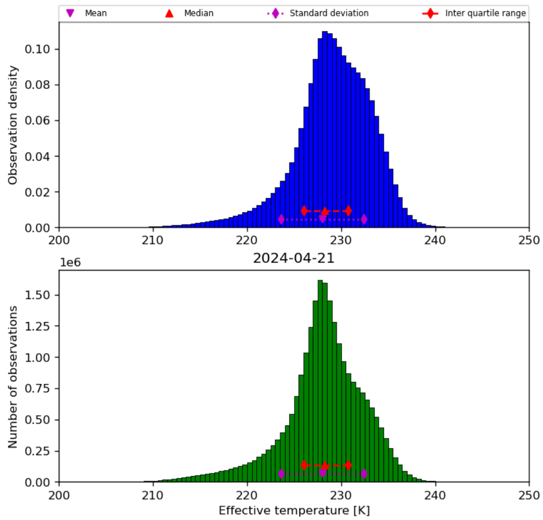
Figure 24: Histogram of “Effective temperature” for 2024-04-21 to 2024-04-22
