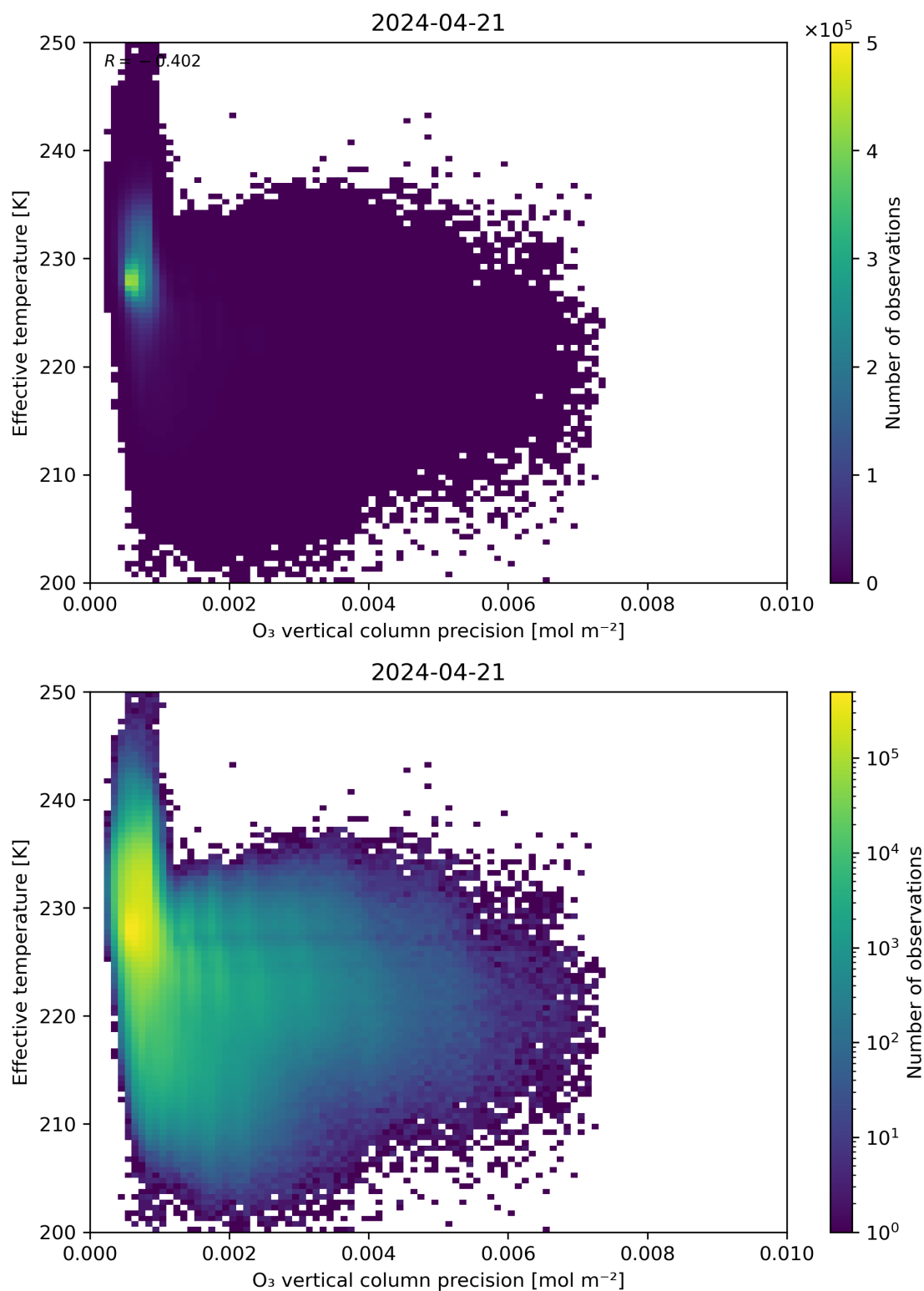
Figure 42: Scatter density plot of “O 3 vertical column precision” against “Effective temperature” for 2024-04-21 to 2024-04-22.
