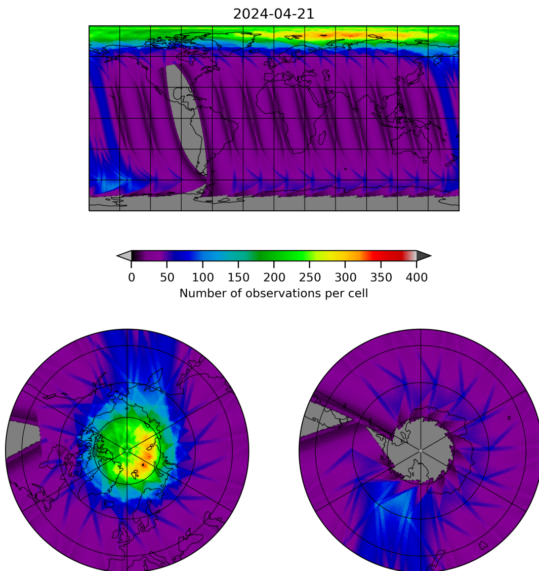
Figure 12: Map of the number of observations for 2024-04-21 to 2024-04-22
