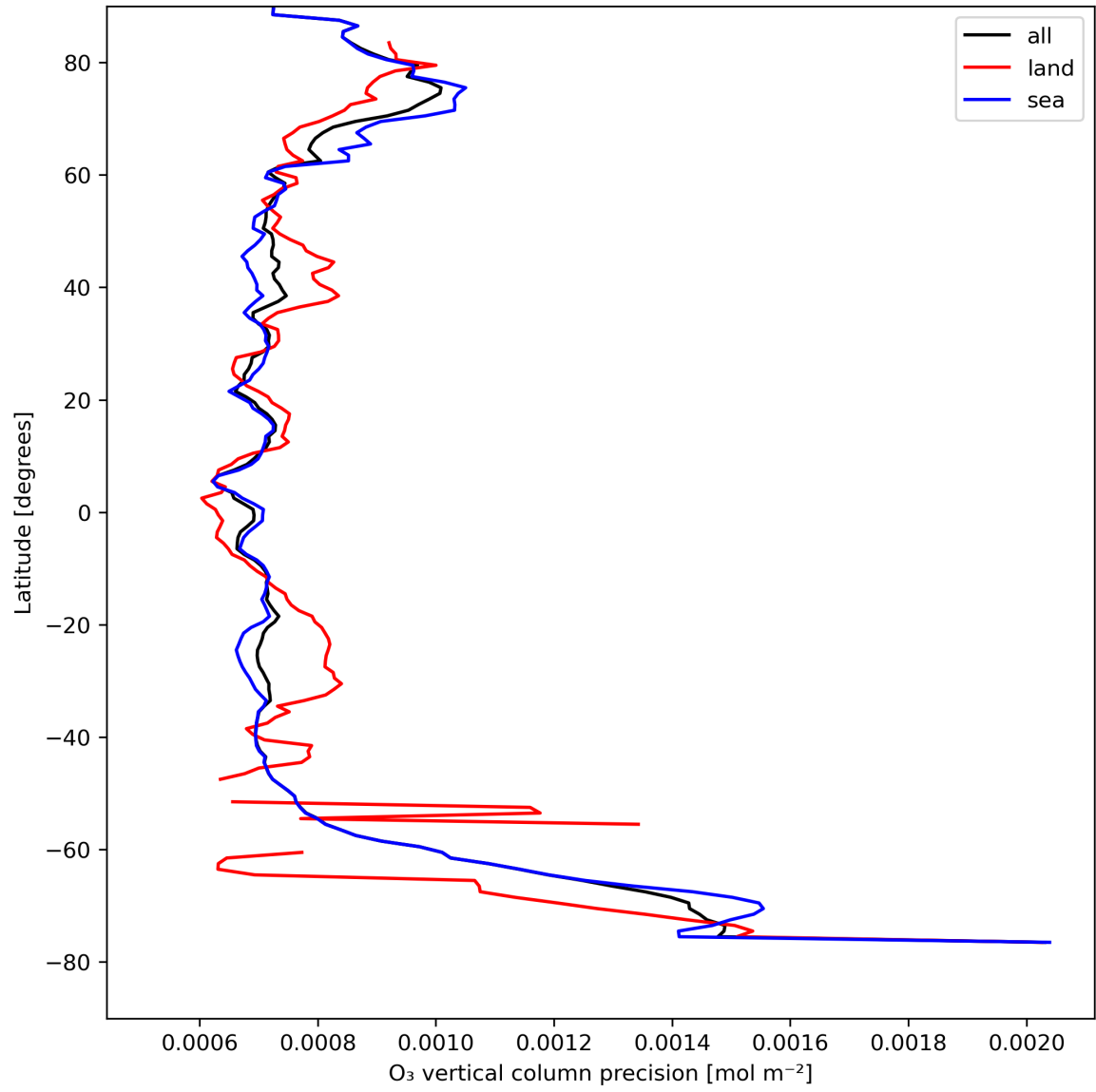
Figure 15: Zonal average of "O 3 vertical column precision" for 2024-04-21 to 2024-04-22.
