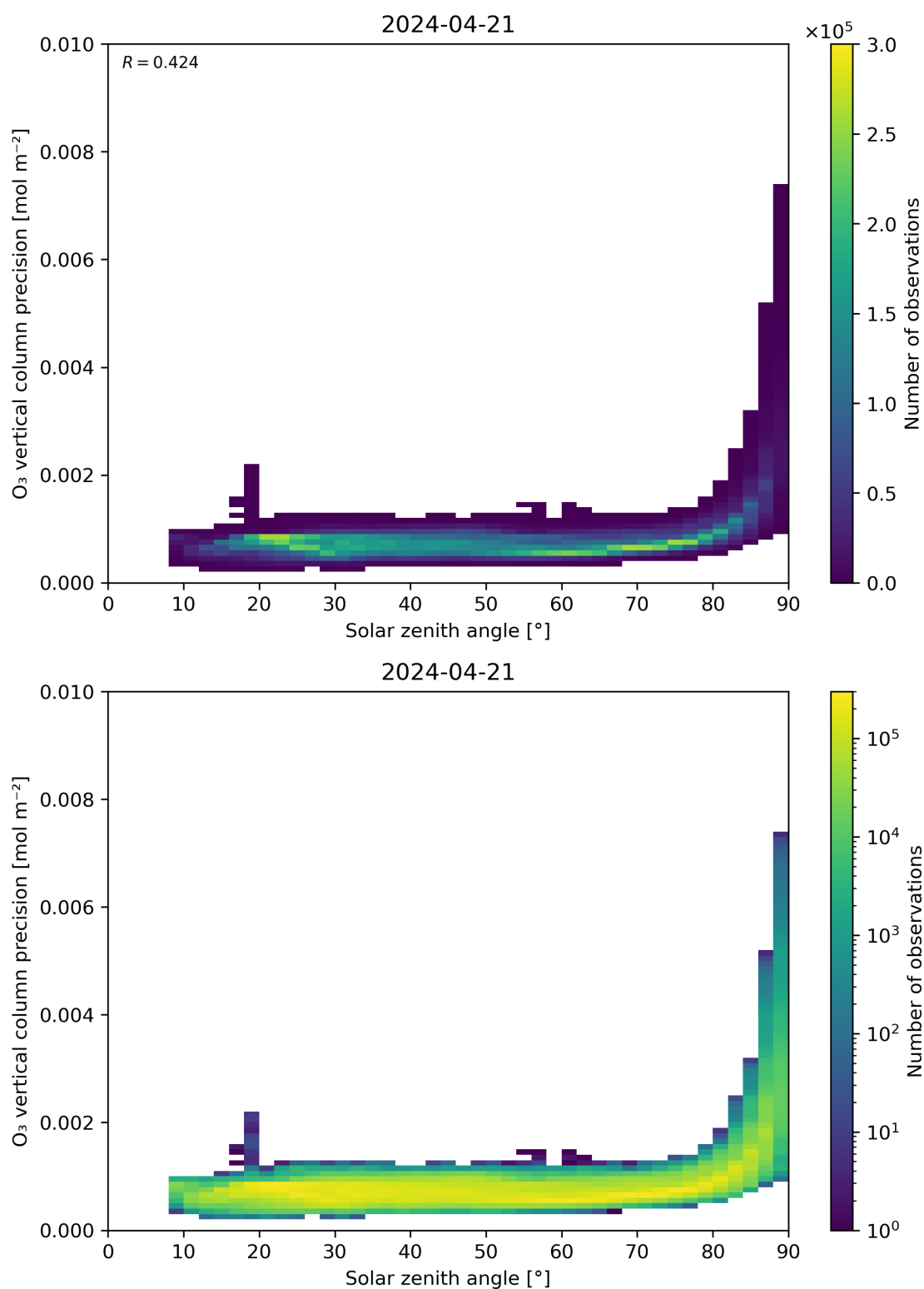
Figure 48: Scatter density plot of “Solar zenith angle” against “O 3 vertical column precision” for 2024-04-21 to 2024-04-22.
