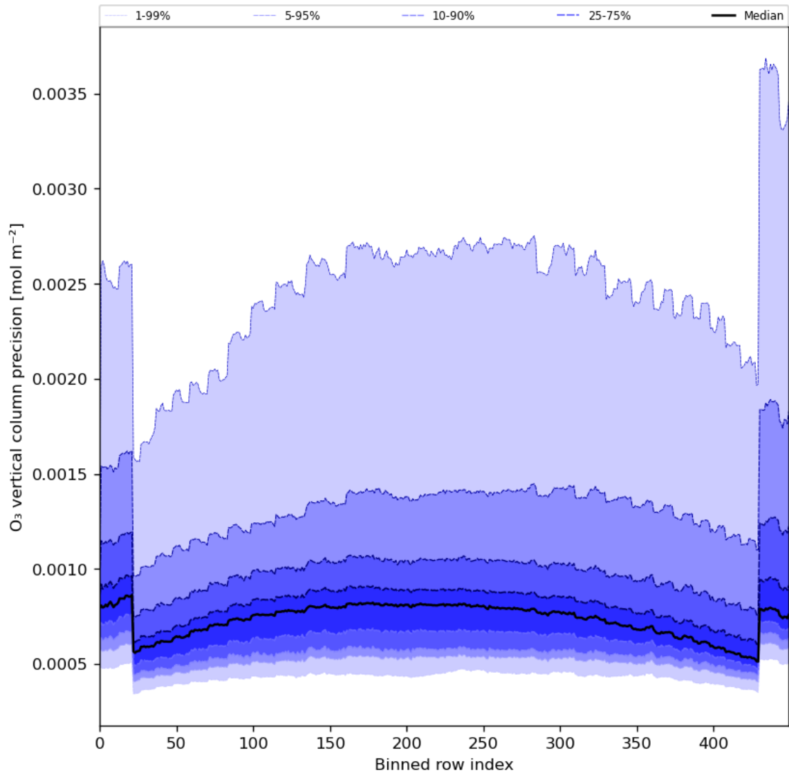
Figure 29: Along track statistics of “O 3 vertical column precision” for 2024-04-21 to 2024-04-22
