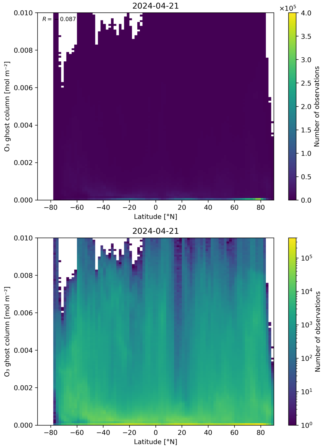
Figure 35: Scatter density plot of “Latitude” against “O 3 ghost column” for 2024-04-21 to 2024-04-22.
