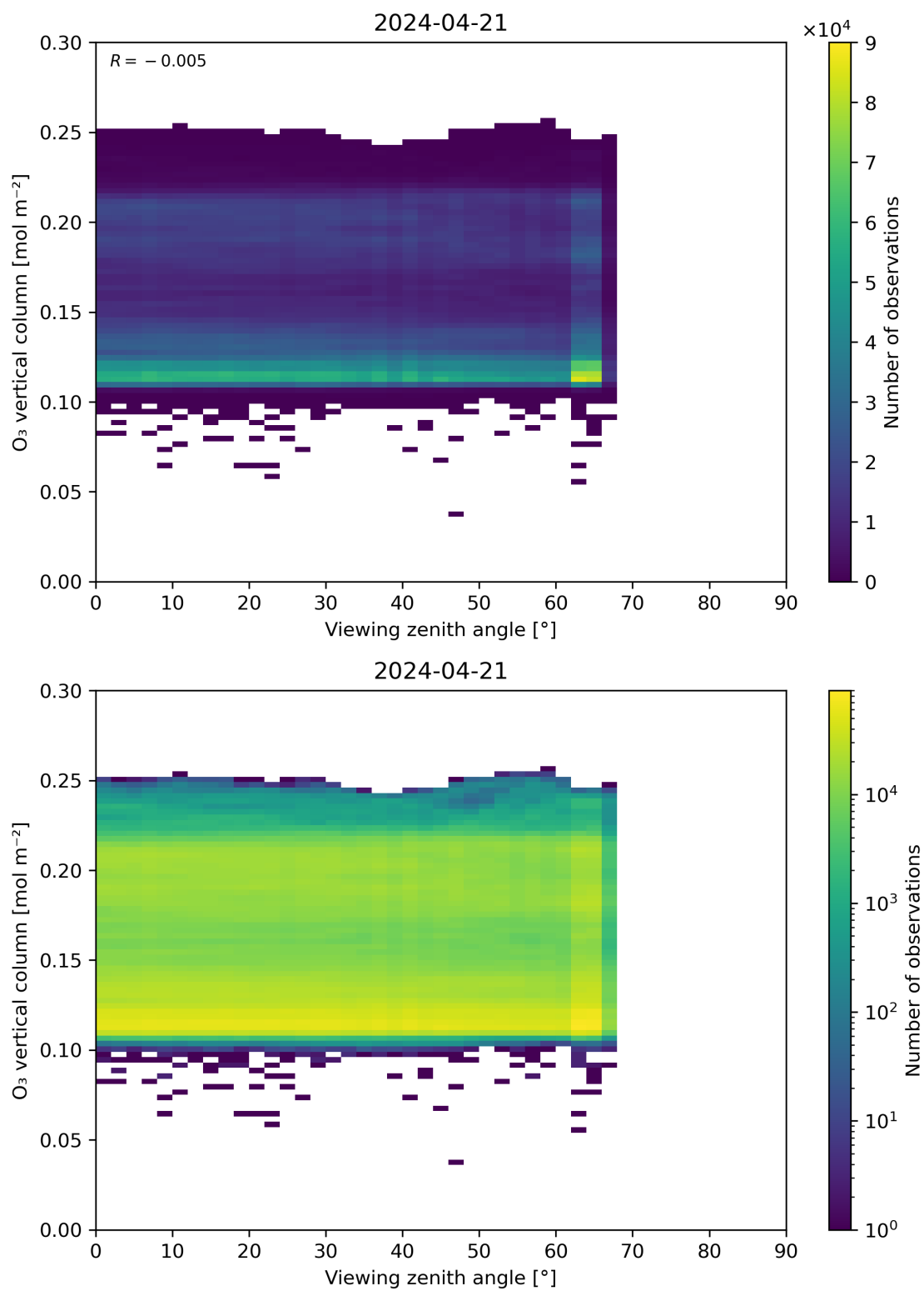
Figure 52: Scatter density plot of “Viewing zenith angle” against “O 3 vertical column” for 2024-04-21 to 2024-04-22.
