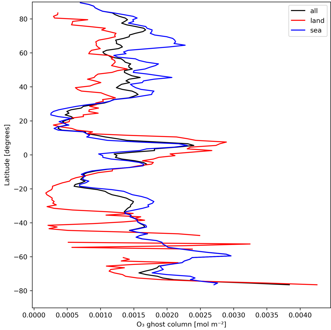
Figure 18: Zonal average of “O 3 ghost column” for 2024-04-21 to 2024-04-22.
