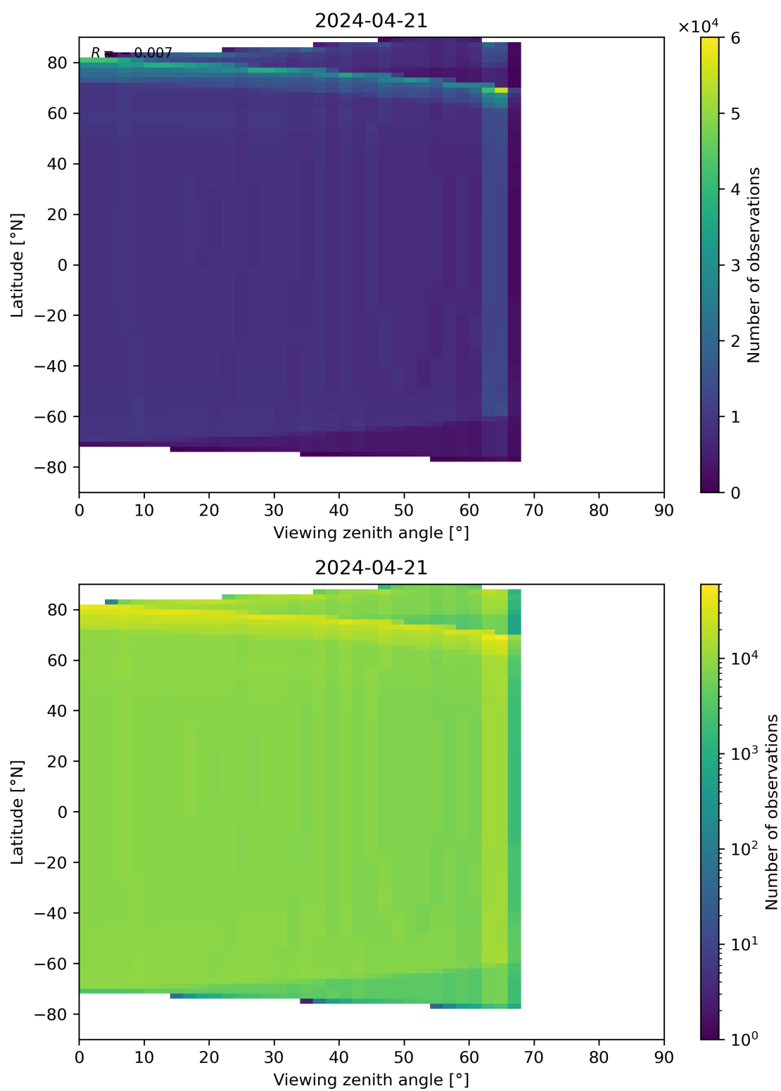
Figure 49: Scatter density plot of “Viewing zenith angle” against “Latitude” for 2024-04-21 to 2024-04-22.
