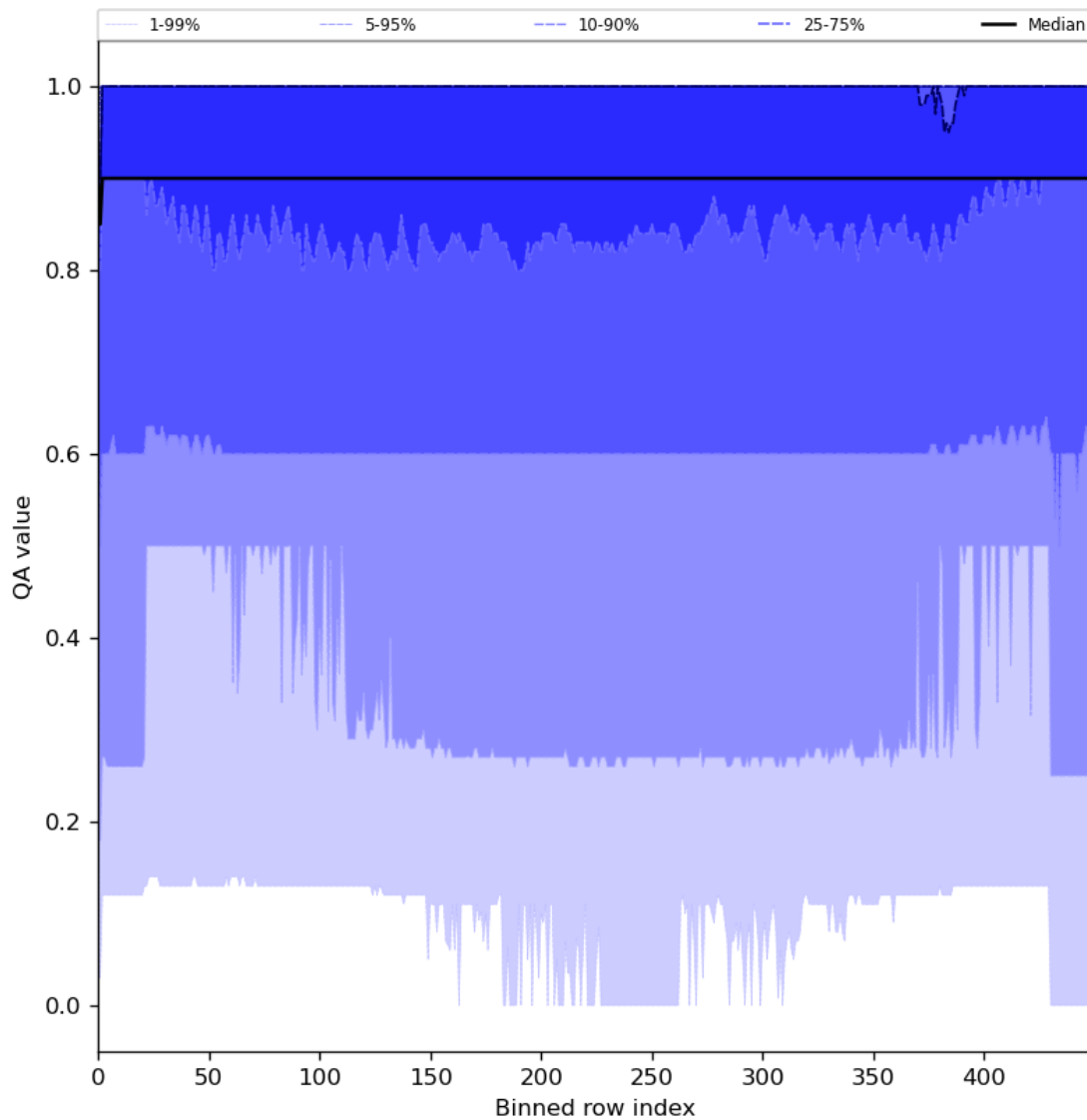
Figure 27: Along track statistics of “QA value” for 2024-04-21 to 2024-04-22
