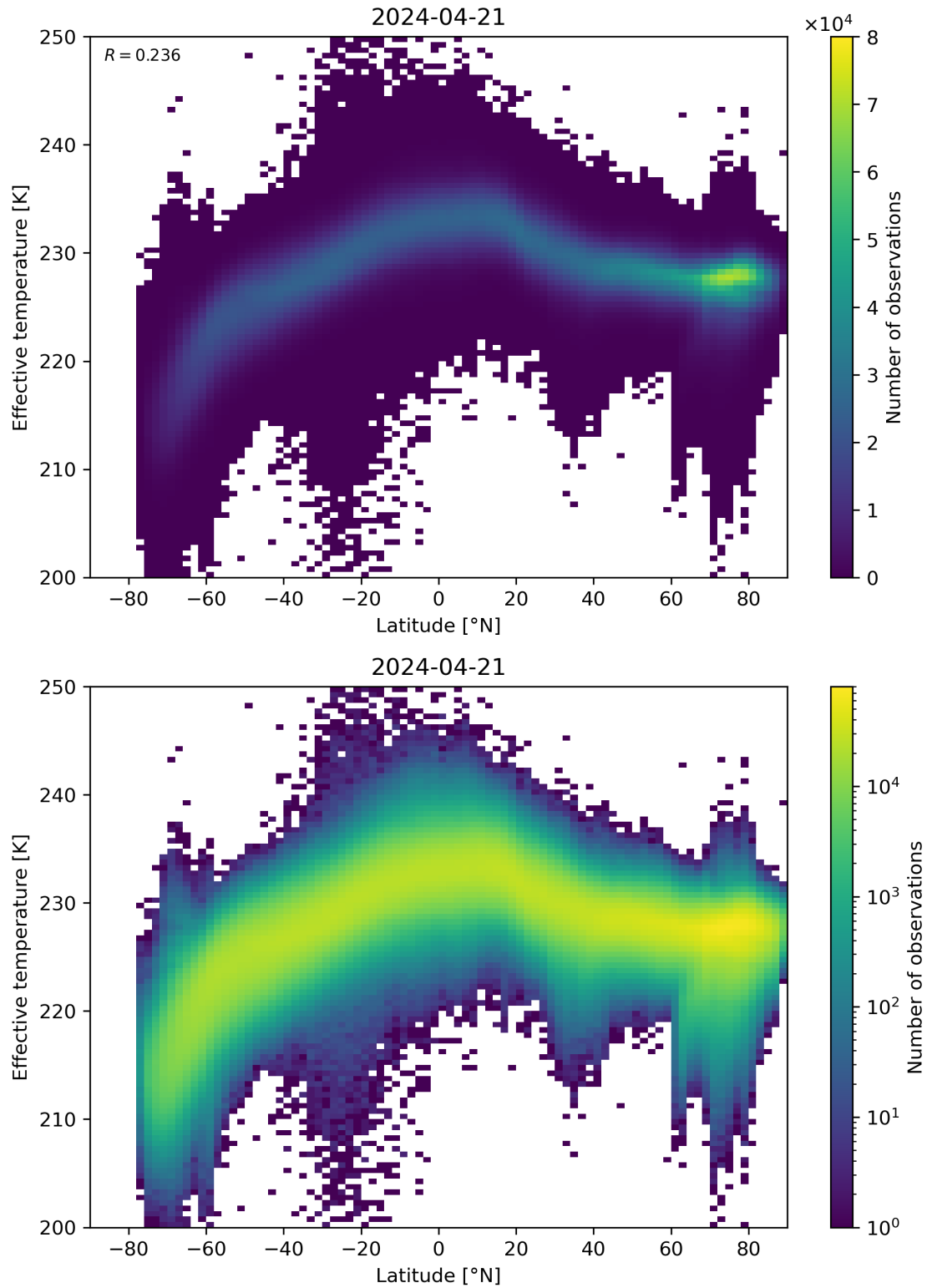
Figure 34: Scatter density plot of “Latitude” against “Effective temperature” for 2024-04-21 to 2024-04-22.
