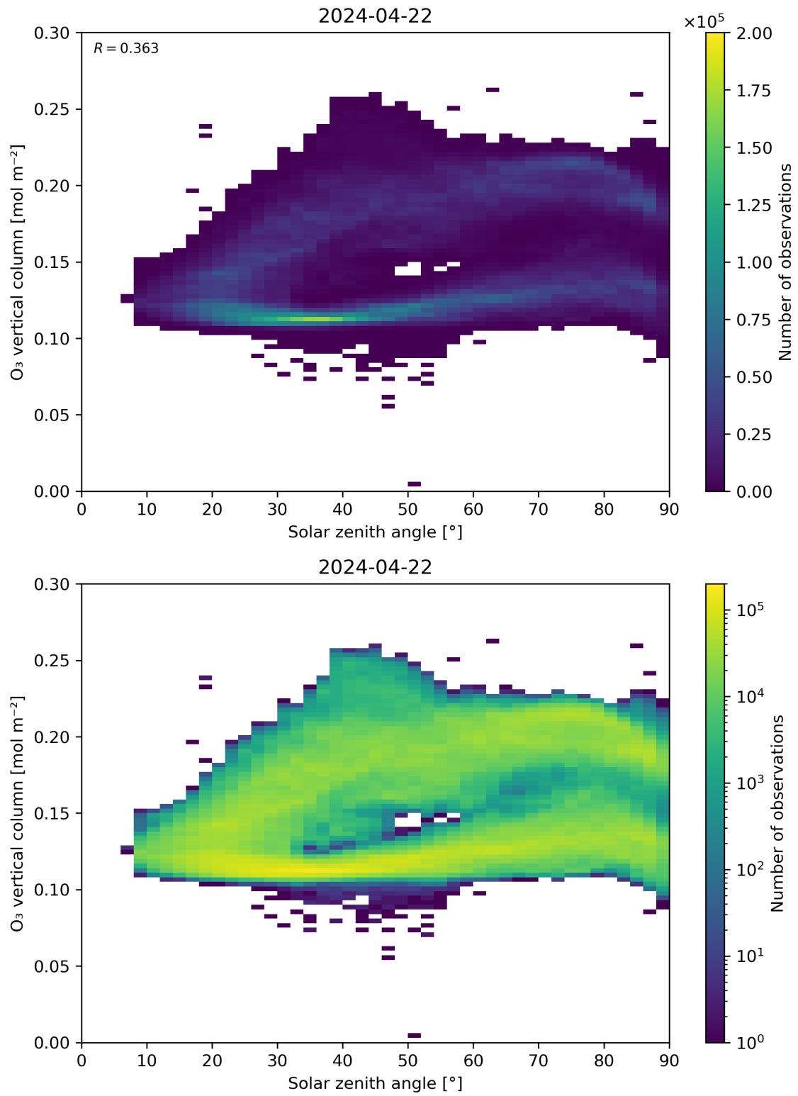
Figure 47: Scatter density plot of “Solar zenith angle” against “O 3 vertical column” for 2024-04-21 to 2024-04-23.
