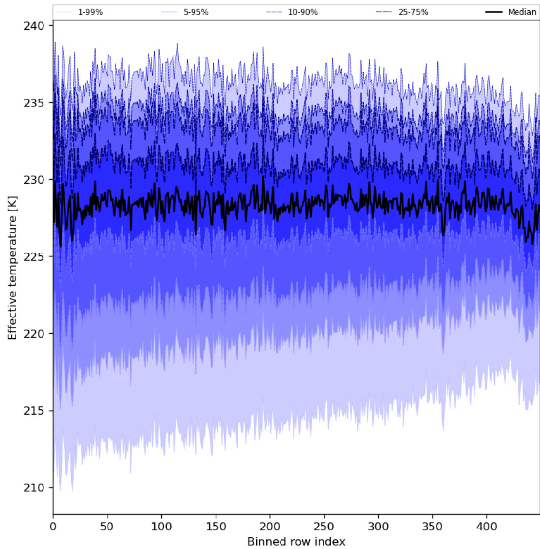
Figure 31: Along track statistics of “Effective temperature” for 2024-04-21 to 2024-04-23
