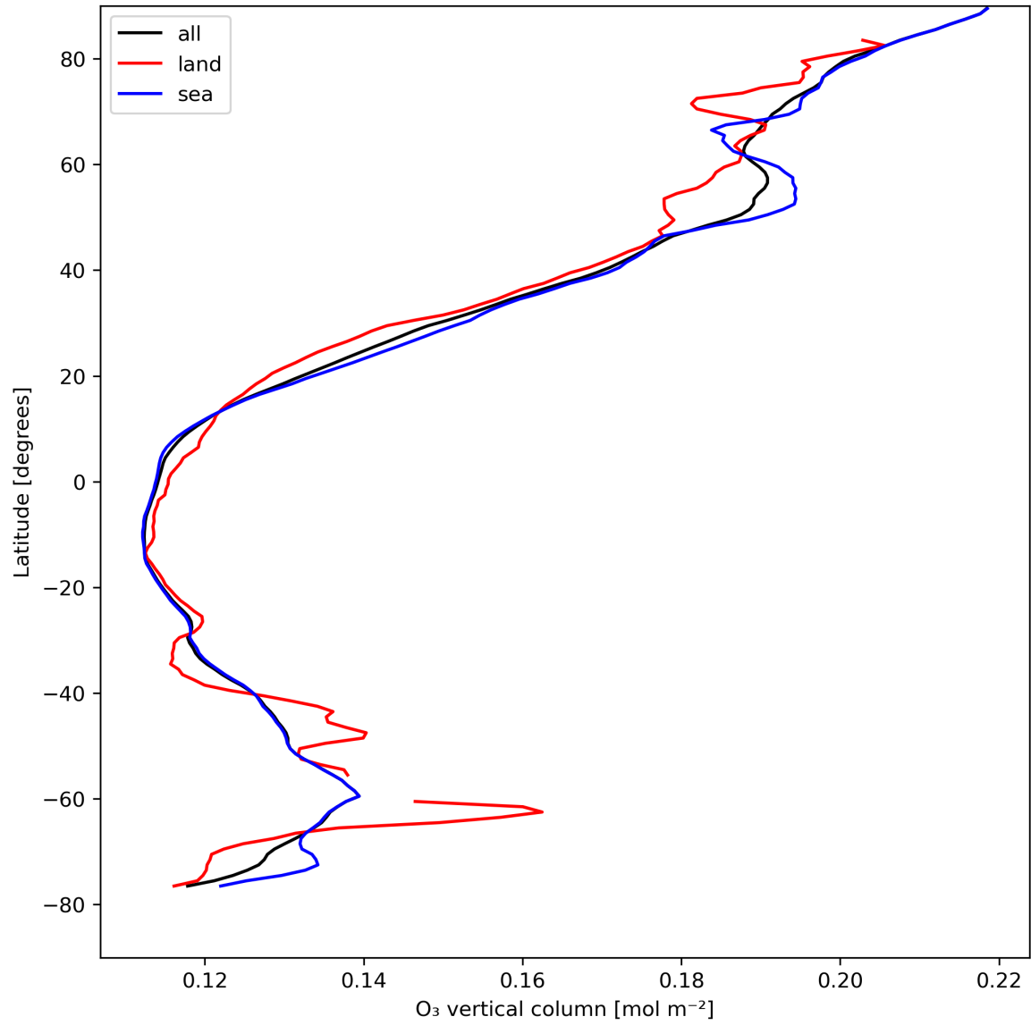
Figure 14: Zonal average of “O 3 vertical column” for 2024-04-21 to 2024-04-23.
