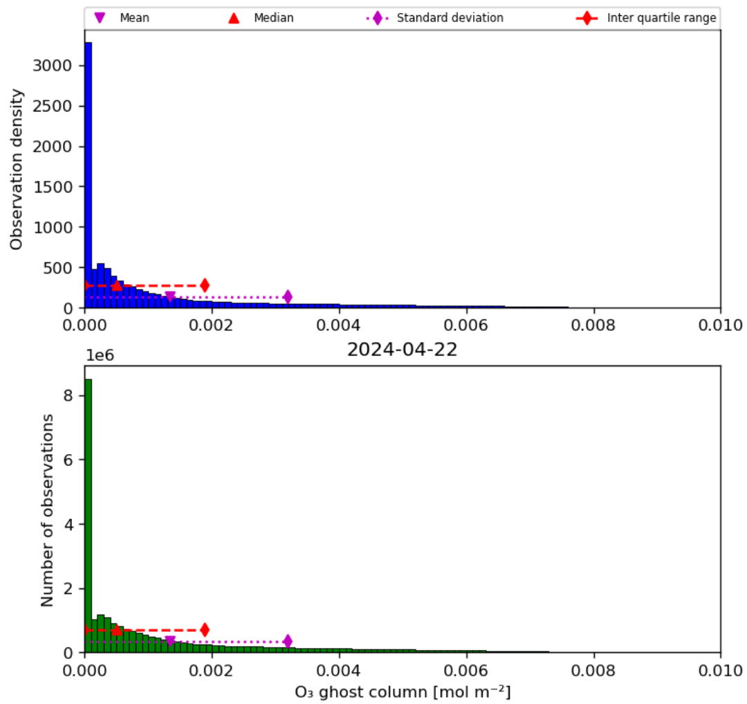
Figure 25: Histogram of “O 3 ghost column” for 2024-04-21 to 2024-04-23
