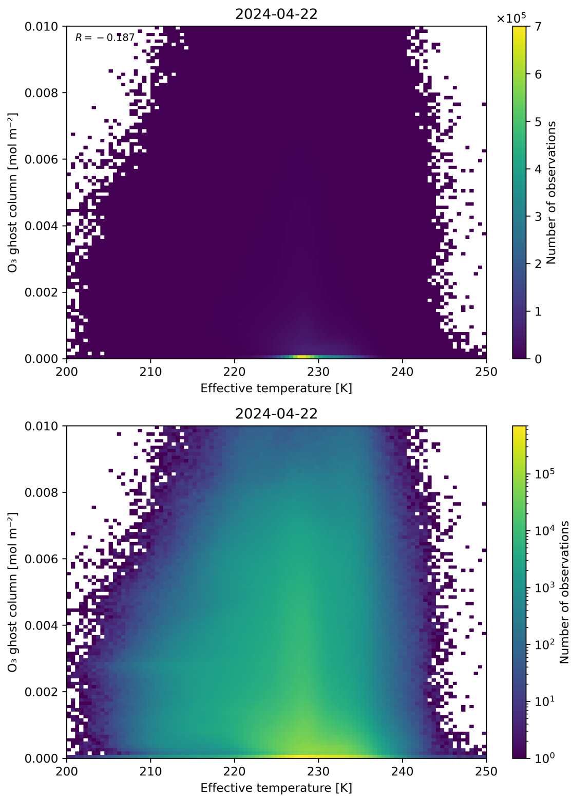
Figure 38: Scatter density plot of “Effective temperature” against “O 3 ghost column” for 2024-04-21 to 2024-04-23.
