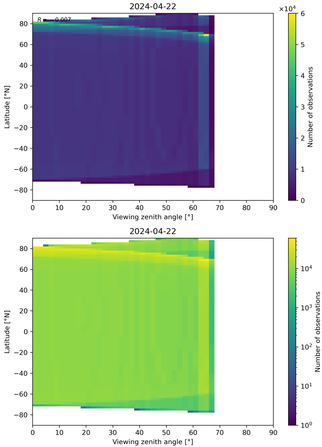
Figure 49: Scatter density plot of “Viewing zenith angle” against “Latitude” for 2024-04-21 to 2024-04-23.
