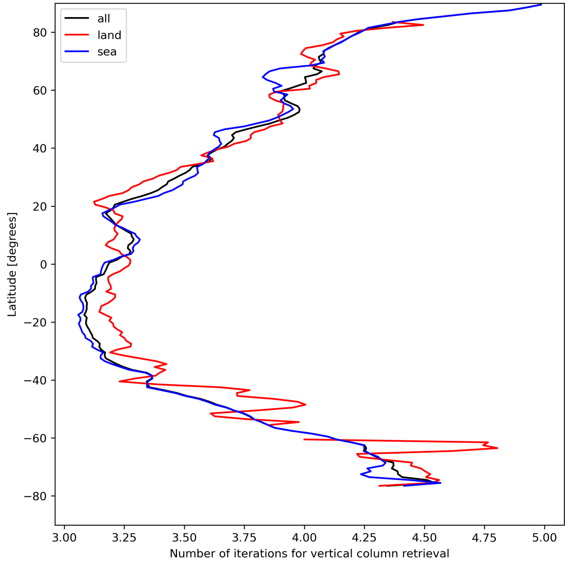
Figure 19: Zonal average of “Number of iterations for vertical column retrieval” for 2024-04-21 to 2024-04-23.
