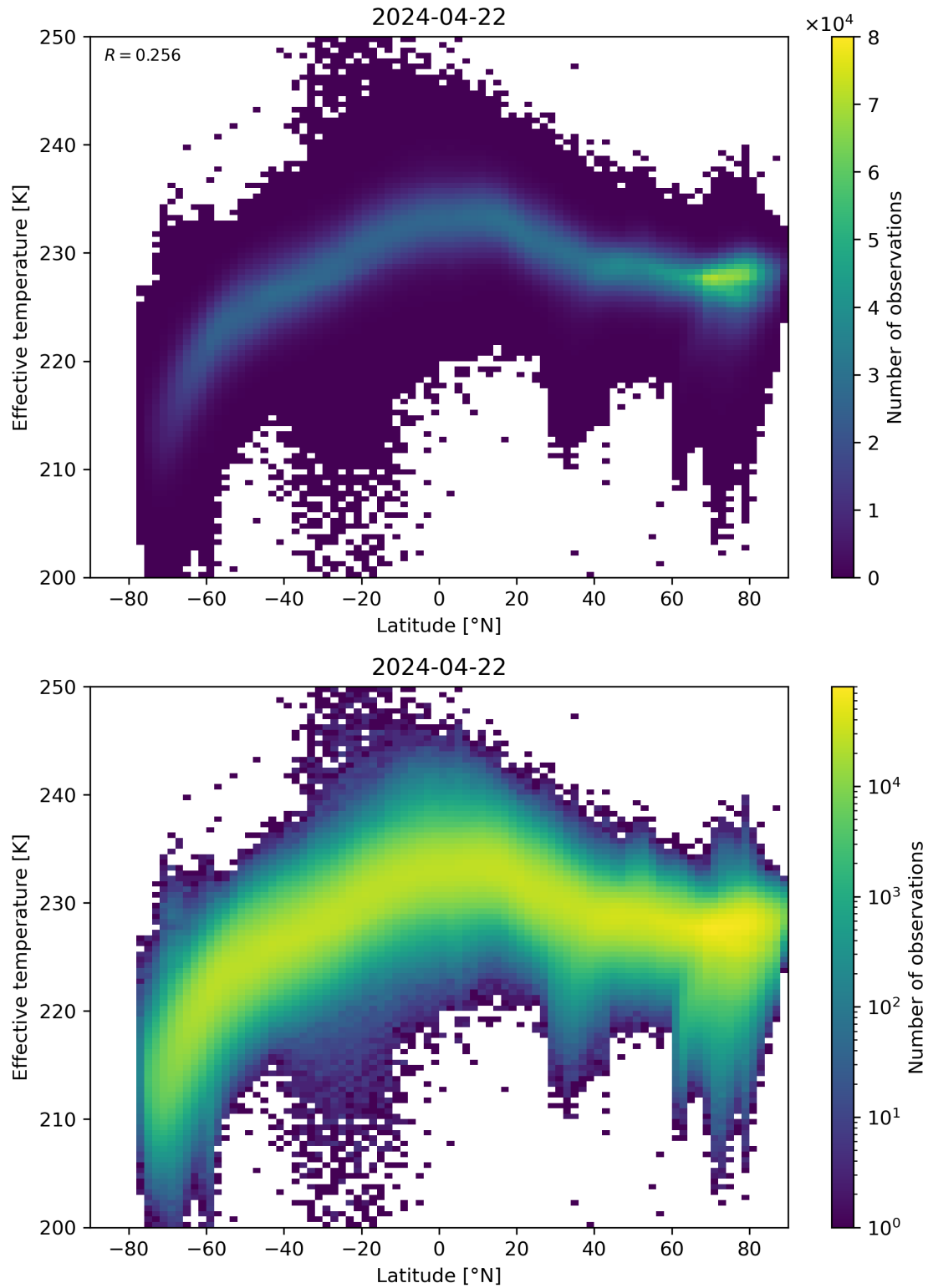
Figure 34: Scatter density plot of “Latitude” against “Effective temperature” for 2024-04-21 to 2024-04-23.
