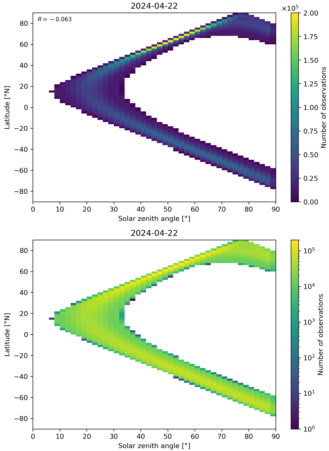
Figure 44: Scatter density plot of “Solar zenith angle” against “Latitude” for 2024-04-21 to 2024-04-23.
