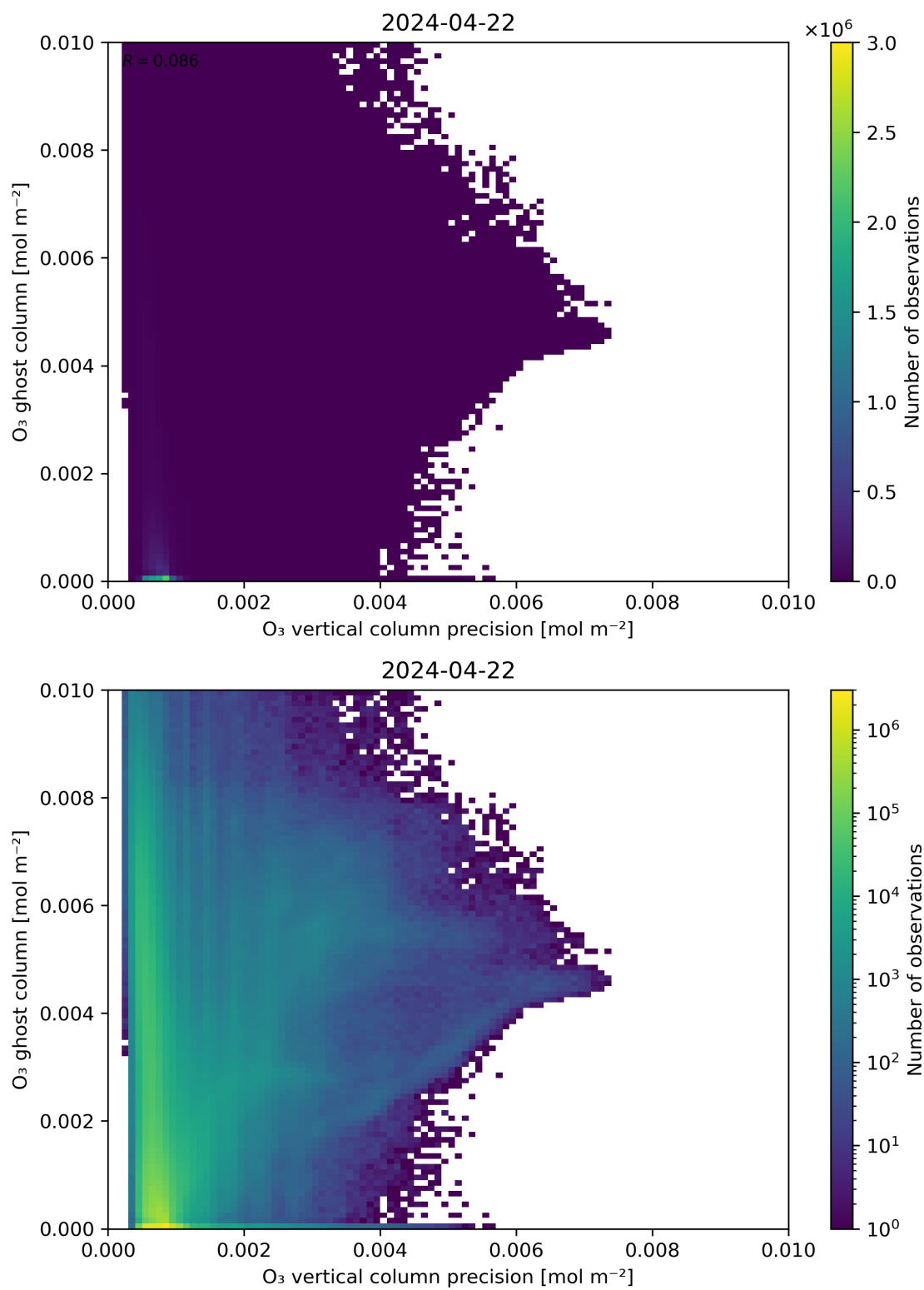
Figure 43: Scatter density plot of “ O_3 vertical column precision” against “ O_3 ghost column” for 2024-04-21 to 2024-04-23.
