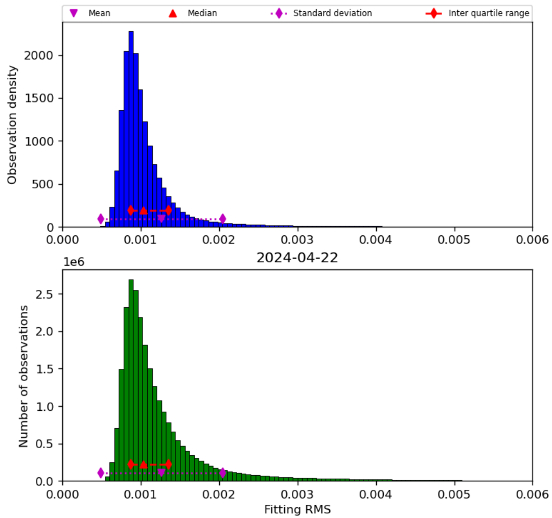
Figure 23: Histogram of “Fitting RMS” for 2024-04-21 to 2024-04-23
