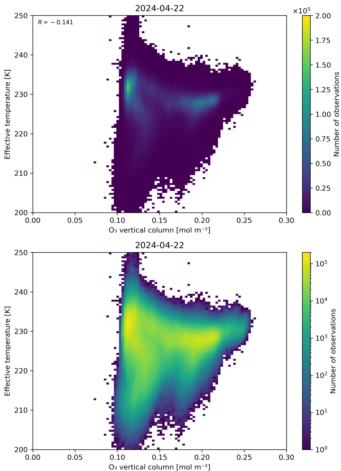
Figure 39: Scatter density plot of “O 3 vertical column” against “Effective temperature” for 2024-04-21 to 2024-04-23.
