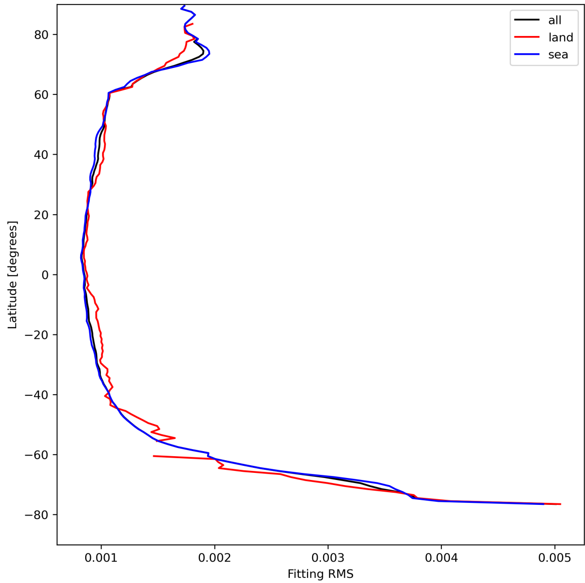
Figure 16: Zonal average of “Fitting RMS” for 2024-04-21 to 2024-04-23.
