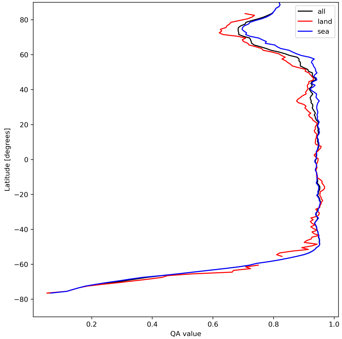
Figure 13: Zonal average of “QA value” for 2024-04-21 to 2024-04-23.
