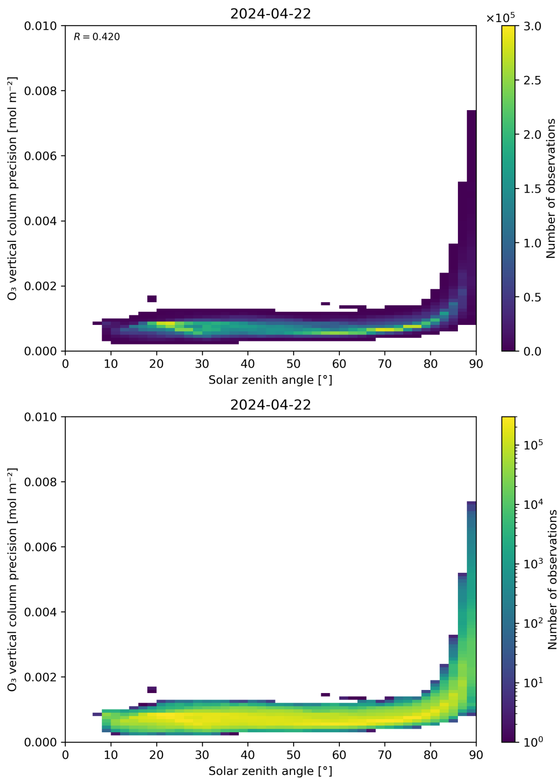
Figure 48: Scatter density plot of “Solar zenith angle” against “O 3 vertical column precision” for 2024-04-21 to 2024-04-23.
