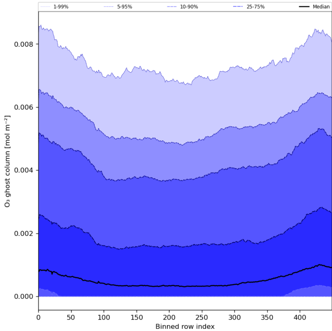
Figure 32: Along track statistics of “O 3 ghost column” for 2024-04-21 to 2024-04-23
