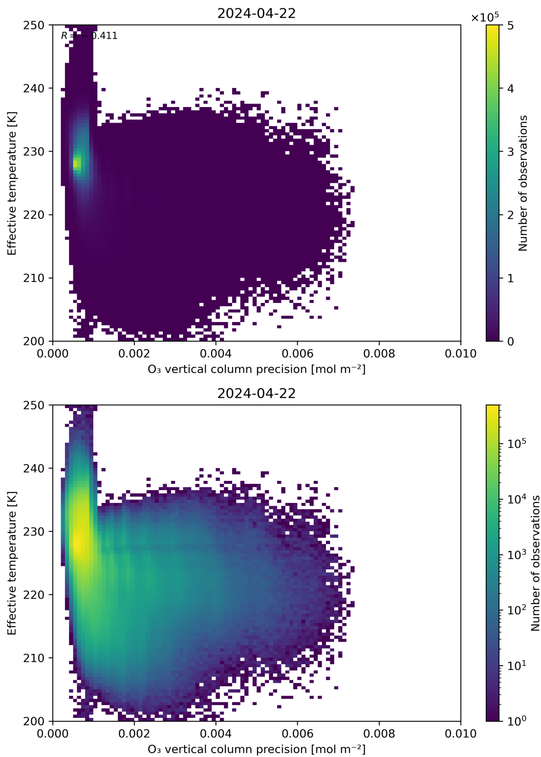
Figure 42: Scatter density plot of “O 3 vertical column precision” against “Effective temperature” for 2024-04-21 to 2024-04-23.
