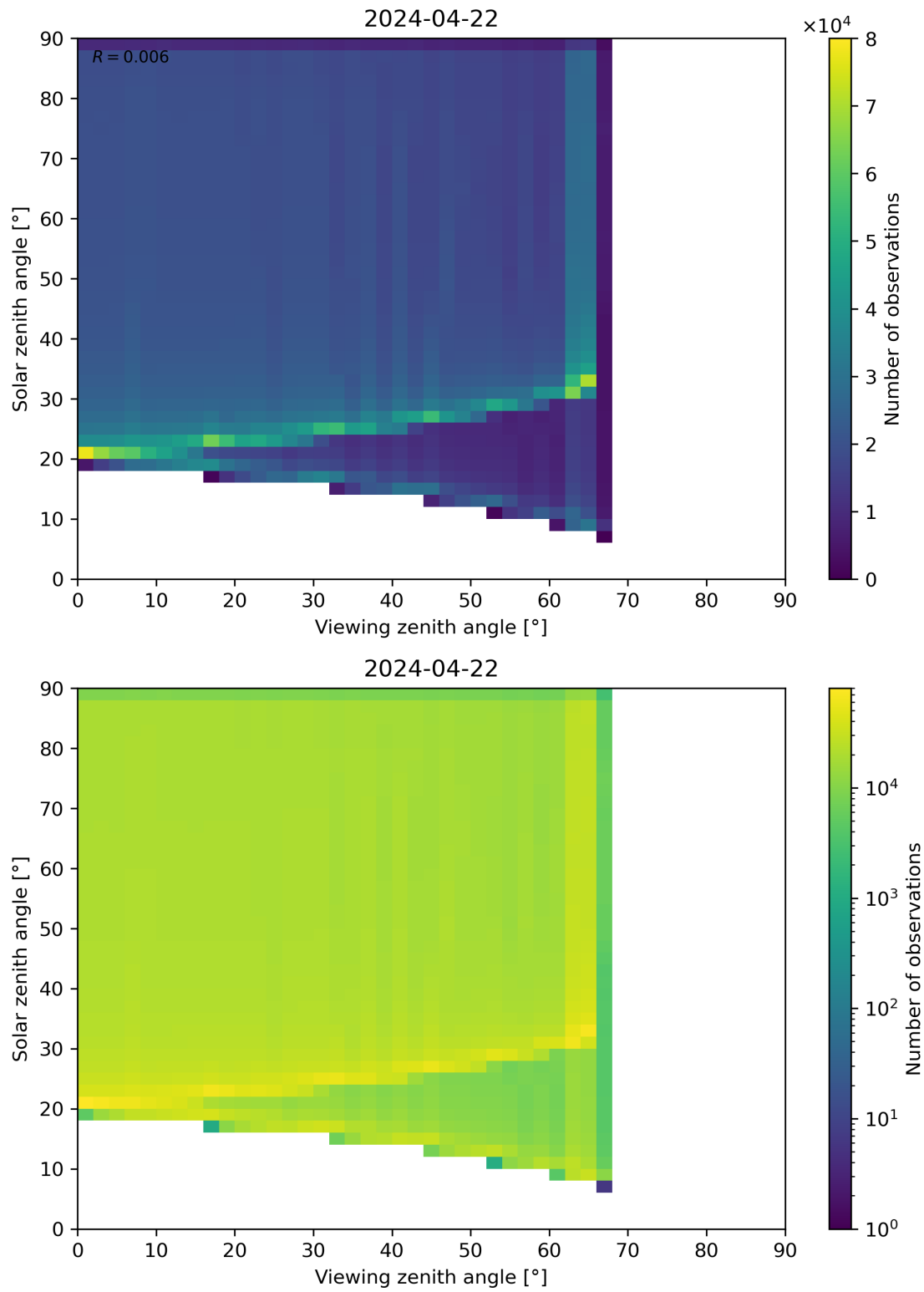
Figure 54: Scatter density plot of “Viewing zenith angle” against “Solar zenith angle” for 2024-04-21 to 2024-04-23.
