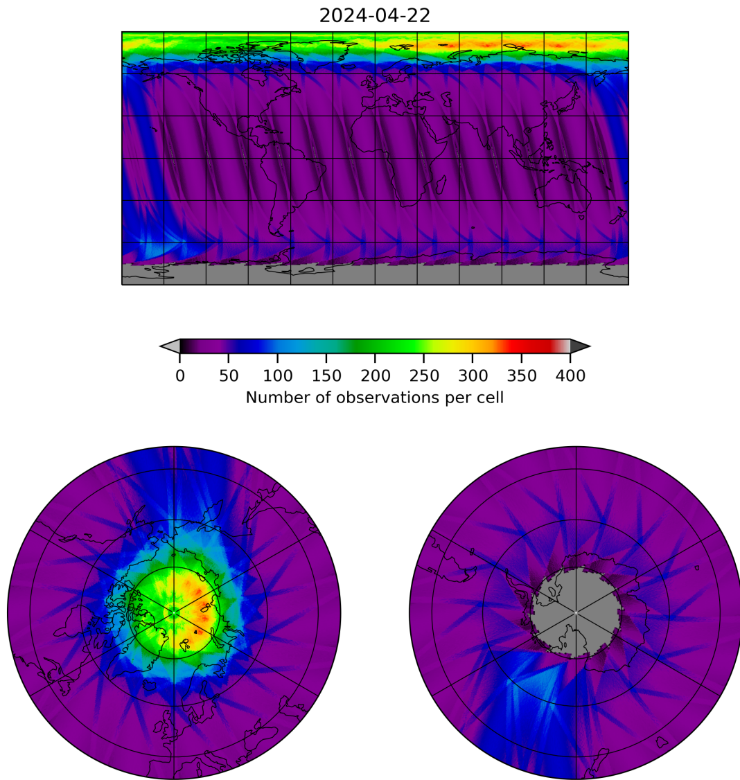
Figure 12: Map of the number of observations for 2024-04-21 to 2024-04-23
