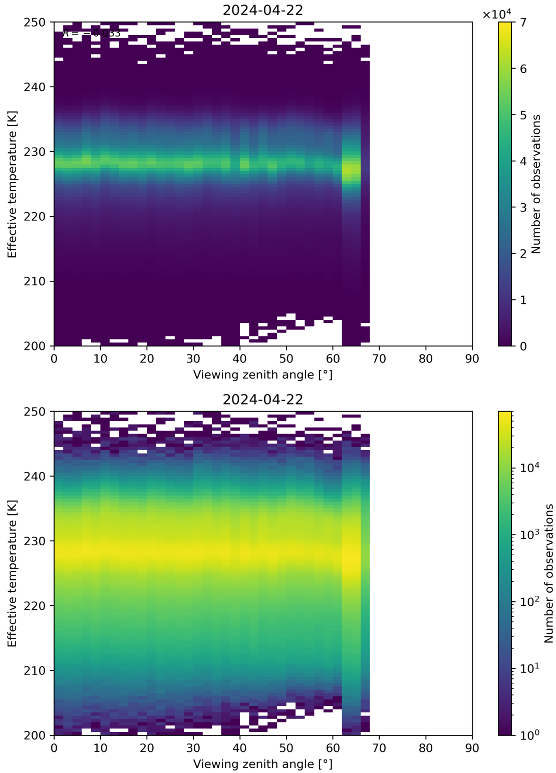
Figure 50: Scatter density plot of “Viewing zenith angle” against “Effective temperature” for 2024-04-21 to 2024-04-23.
