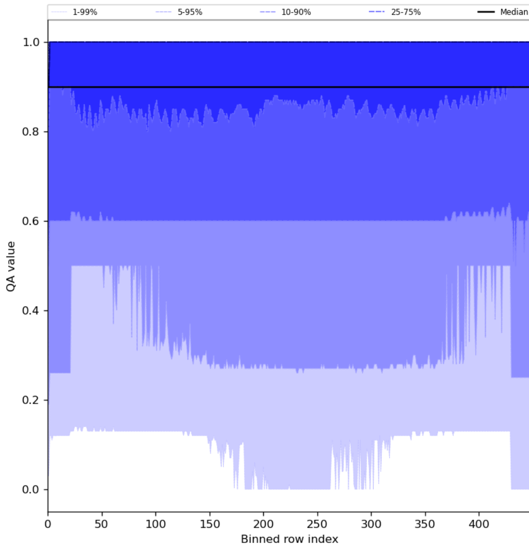
Figure 27: Along track statistics of “QA value” for 2024-04-21 to 2024-04-23
