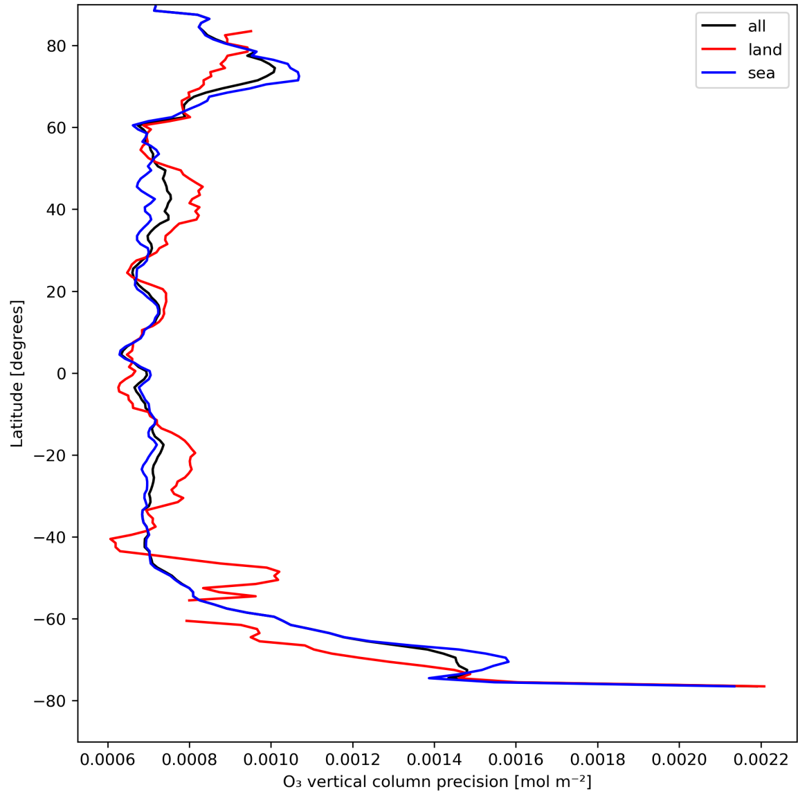
Figure 15: Zonal average of “O 3 vertical column precision” for 2024-04-21 to 2024-04-23.
