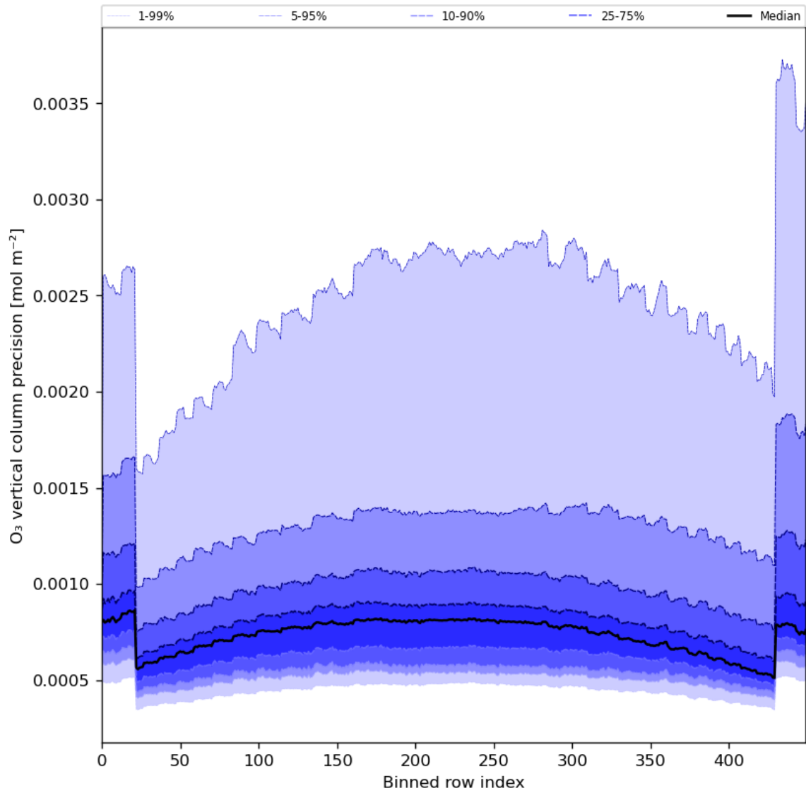
Figure 29: Along track statistics of “O 3 vertical column precision” for 2024-04-21 to 2024-04-23
