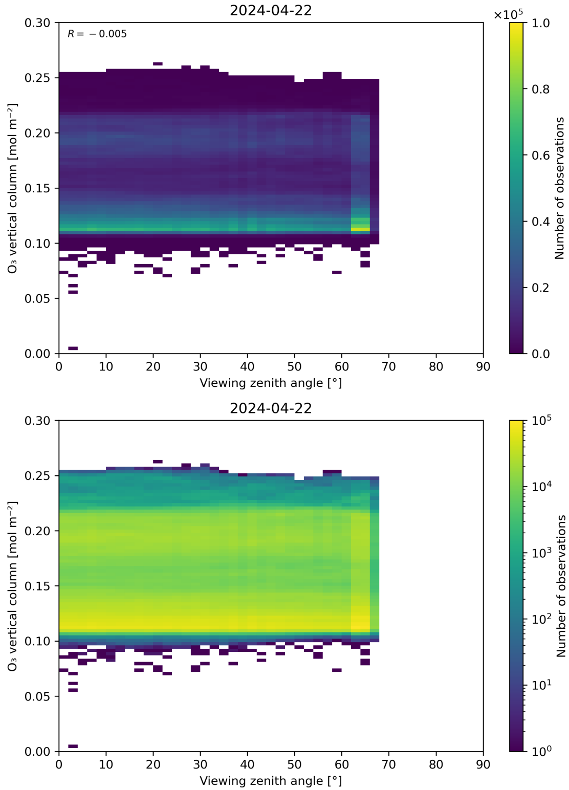
Figure 52: Scatter density plot of “Viewing zenith angle” against “O 3 vertical column” for 2024-04-21 to 2024-04-23.
