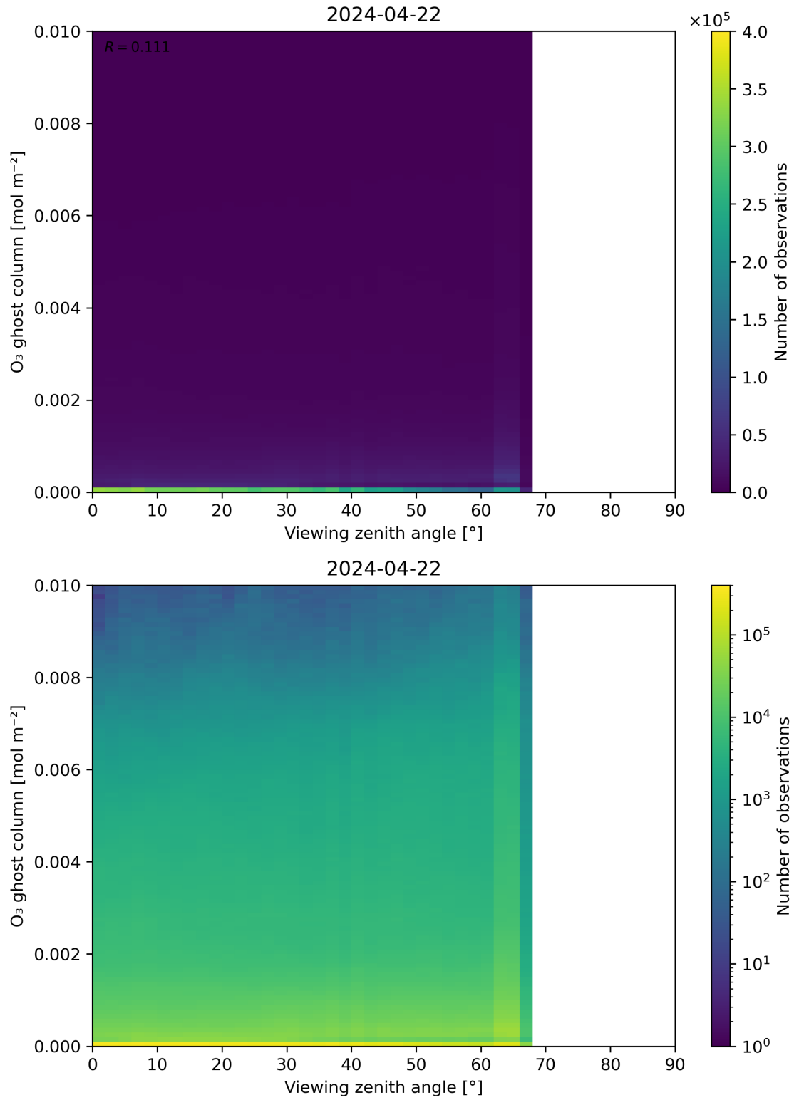
Figure 51: Scatter density plot of “Viewing zenith angle” against “O 3 ghost column” for 2024-04-21 to 2024-04-23.
