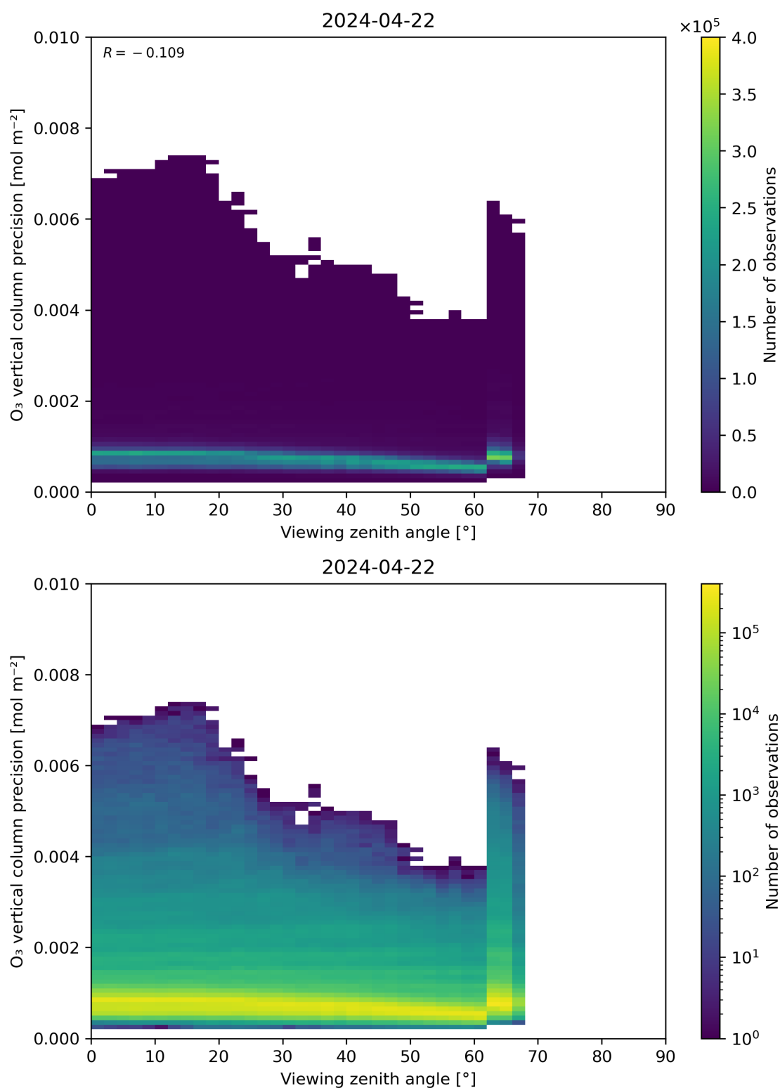
Figure 53: Scatter density plot of “Viewing zenith angle” against “O 3 vertical column precision” for 2024-04-21 to 2024-04-23.
