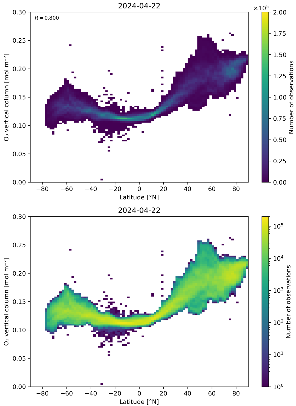
Figure 36: Scatter density plot of “Latitude” against “O 3 vertical column” for 2024-04-21 to 2024-04-23.
