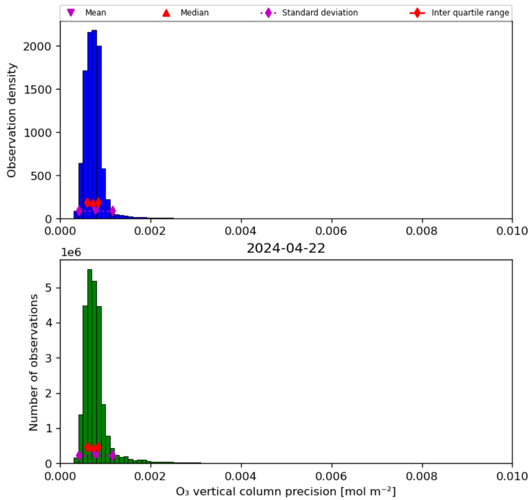
Figure 22: Histogram of “O 3 vertical column precision” for 2024-04-21 to 2024-04-23
