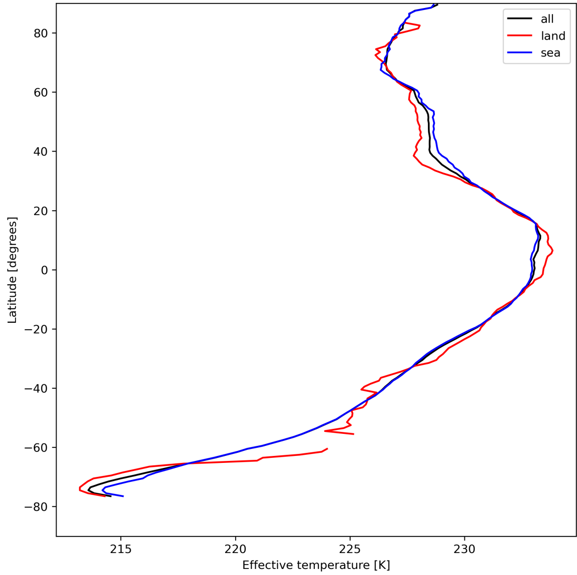
Figure 17: Zonal average of “Effective temperature” for 2024-04-21 to 2024-04-23.
