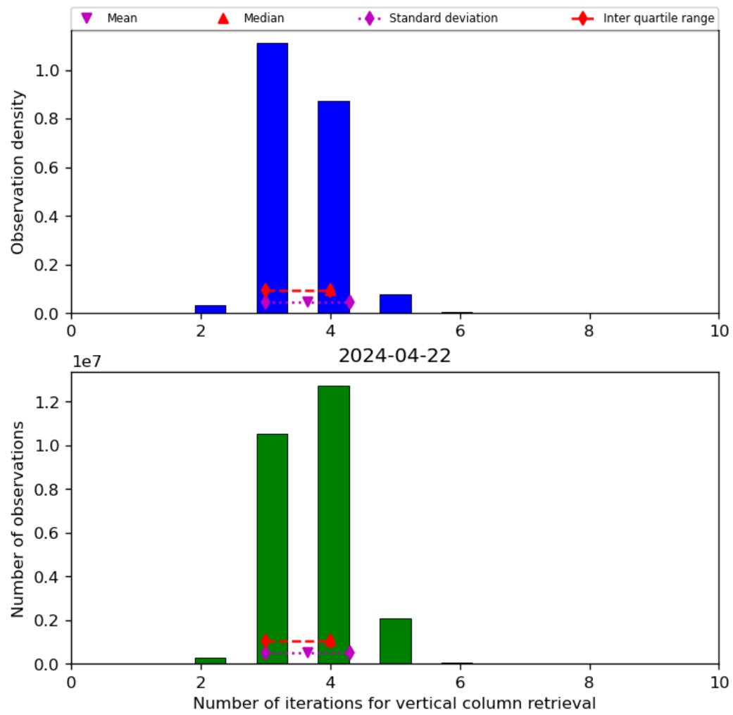
Figure 26: Histogram of “Number of iterations for vertical column retrieval” for 2024-04-21 to 2024-04-23
