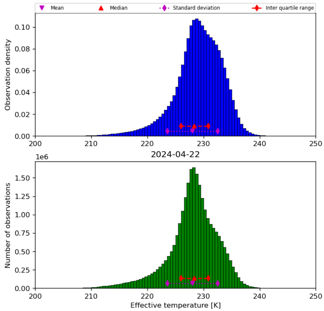
Figure 24: Histogram of “Effective temperature” for 2024-04-21 to 2024-04-23
