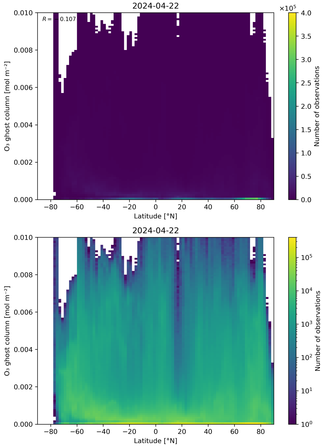
Figure 35: Scatter density plot of “Latitude” against “O 3 ghost column” for 2024-04-21 to 2024-04-23.
