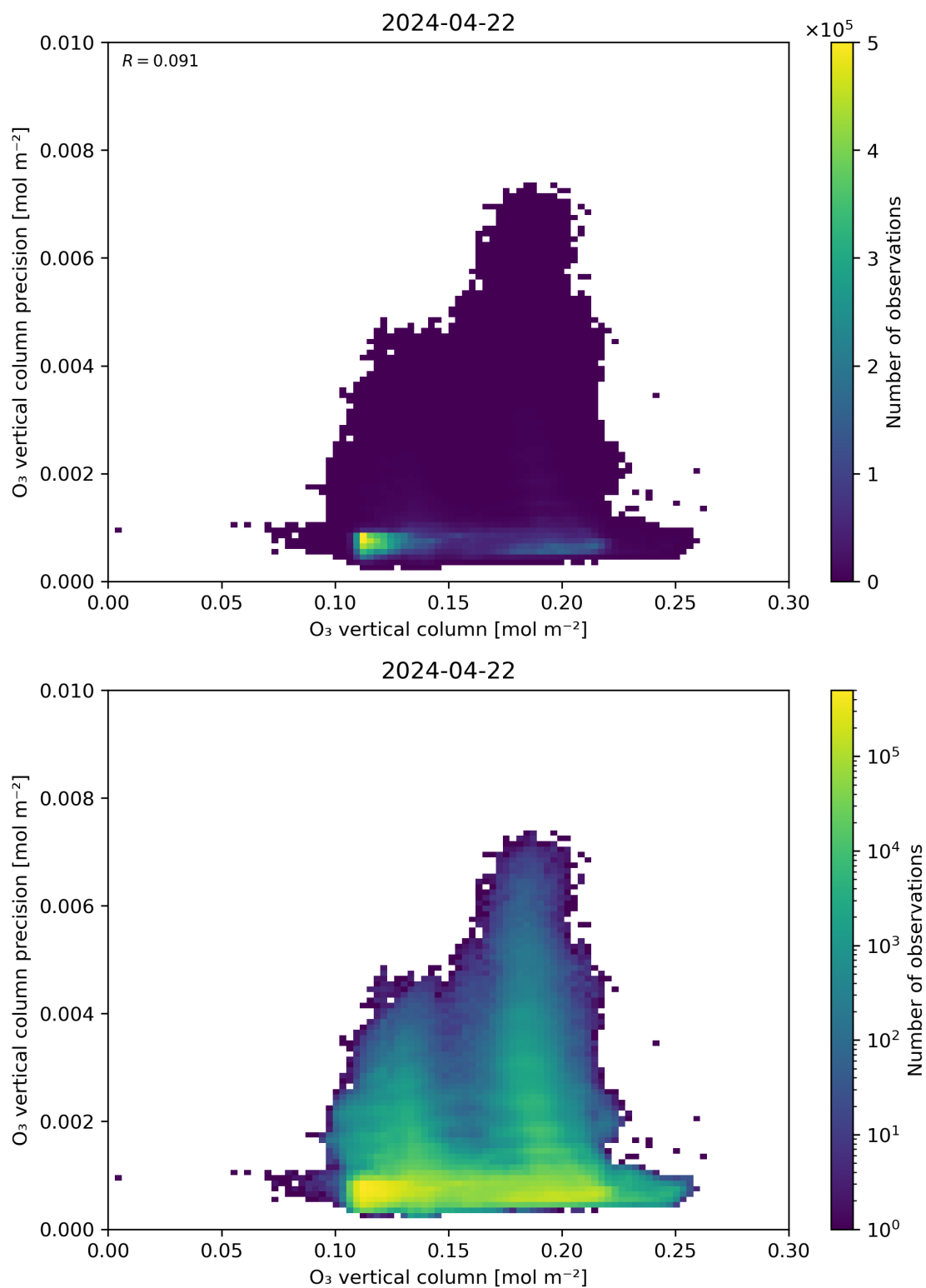
Figure 41: Scatter density plot of “O 3 vertical column” against “O 3 vertical column precision” for 2024-04-21 to 2024-04-23.
