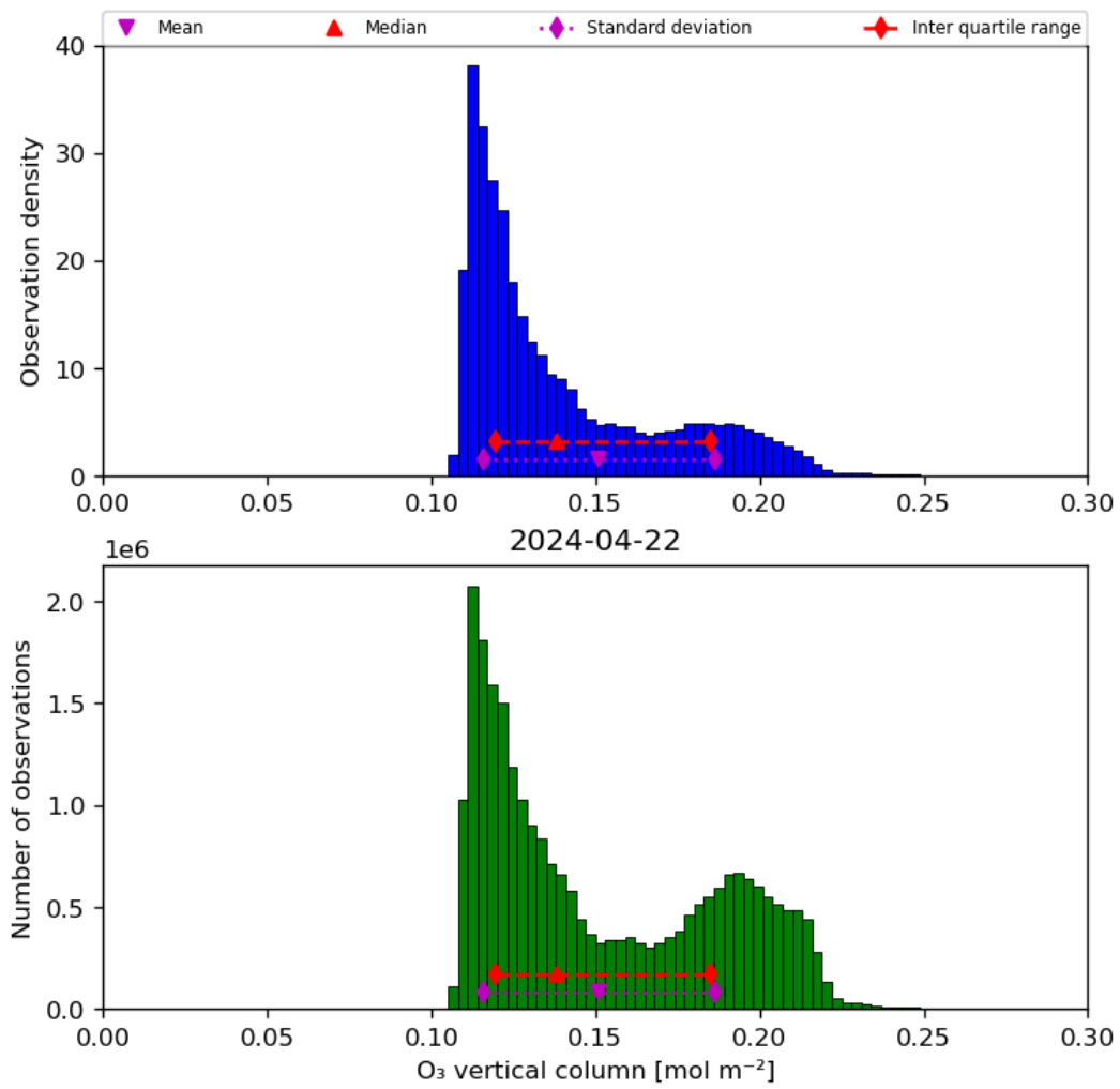
Figure 21: Histogram of “O 3 vertical column” for 2024-04-21 to 2024-04-23
