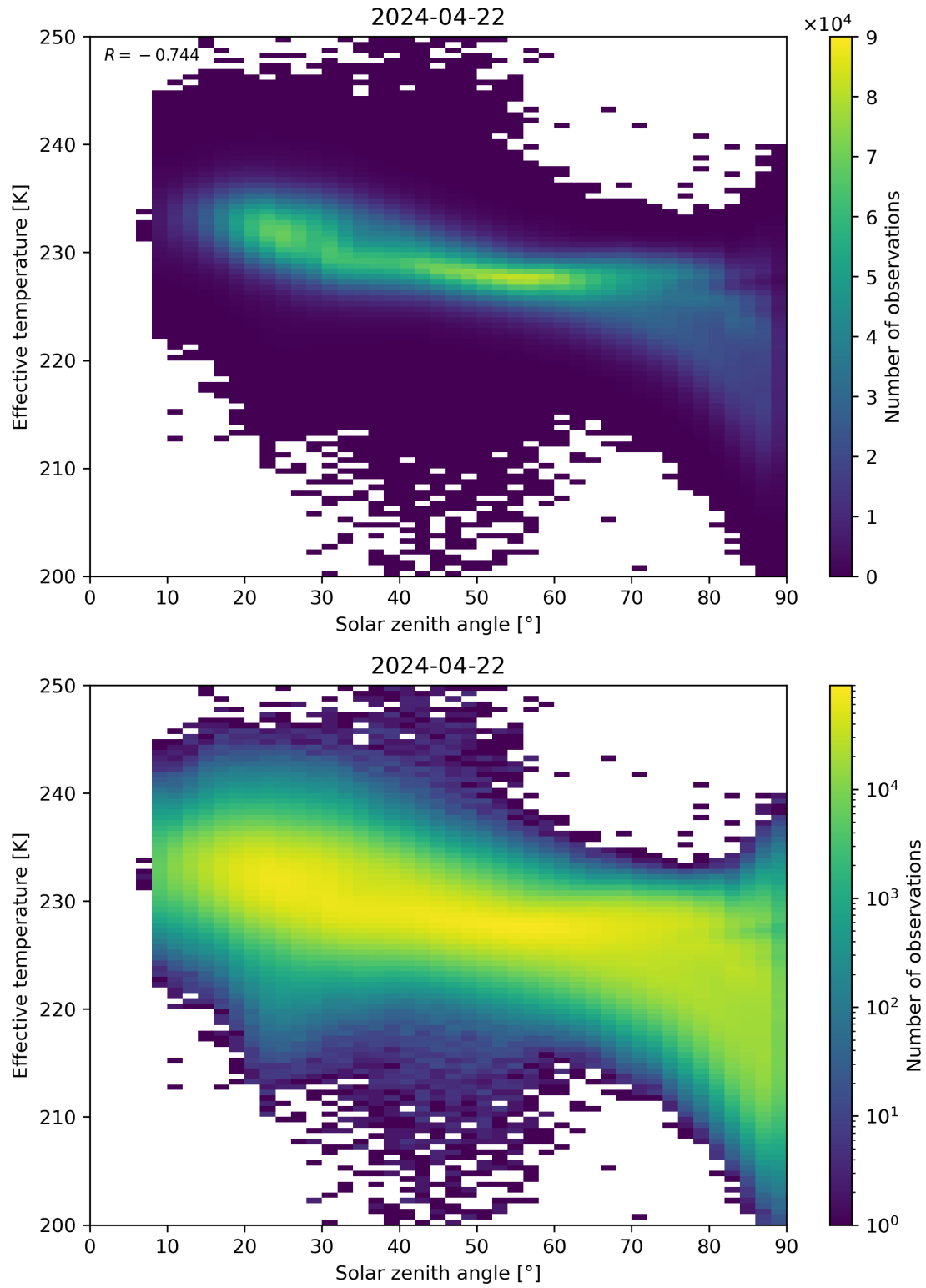
Figure 45: Scatter density plot of “Solar zenith angle” against “Effective temperature” for 2024-04-21 to 2024-04-23.
