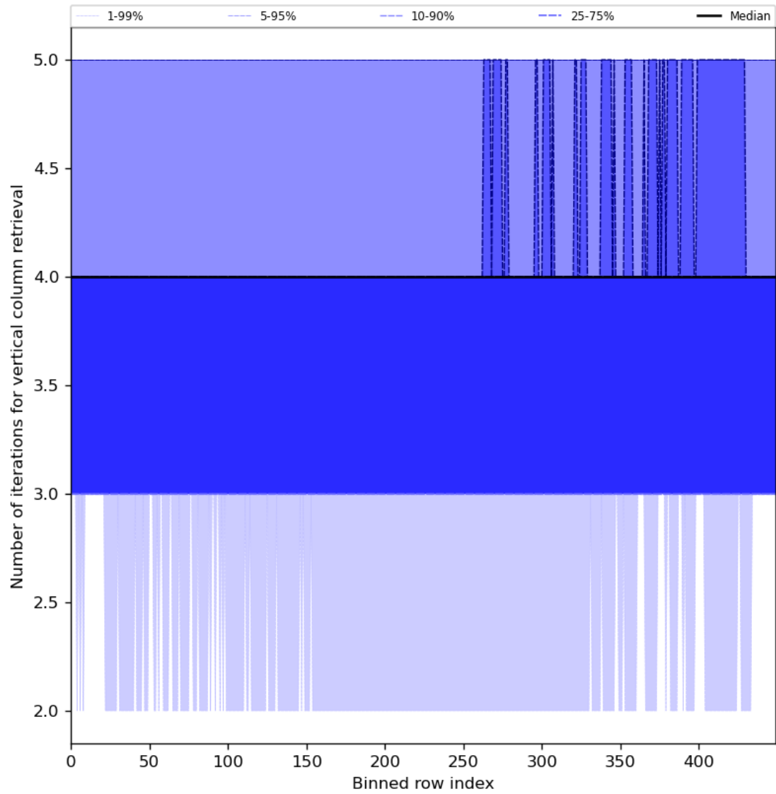
Figure 33: Along track statistics of “Number of iterations for vertical column retrieval” for 2024-04-21 to 2024-04-23
