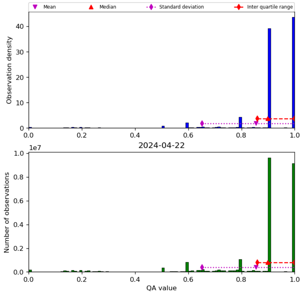
Figure 20: Histogram of “QA value” for 2024-04-21 to 2024-04-23
