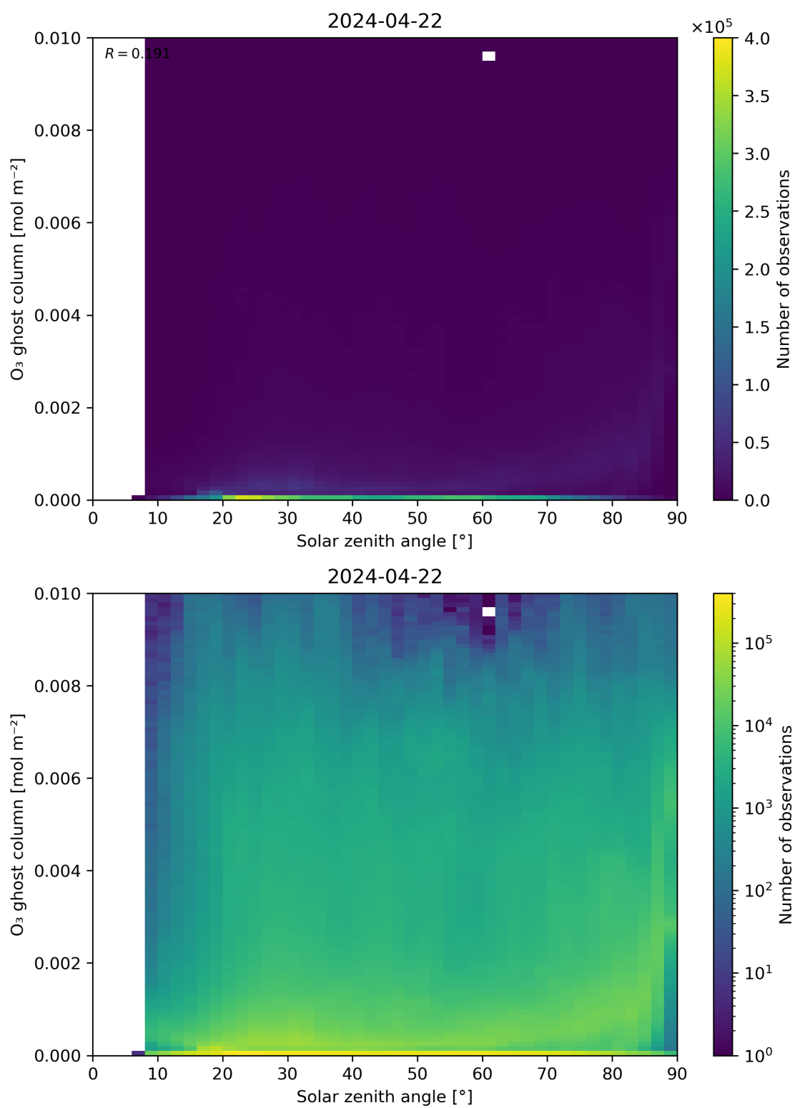
Figure 46: Scatter density plot of “Solar zenith angle” against “O 3 ghost column” for 2024-04-21 to 2024-04-23.
