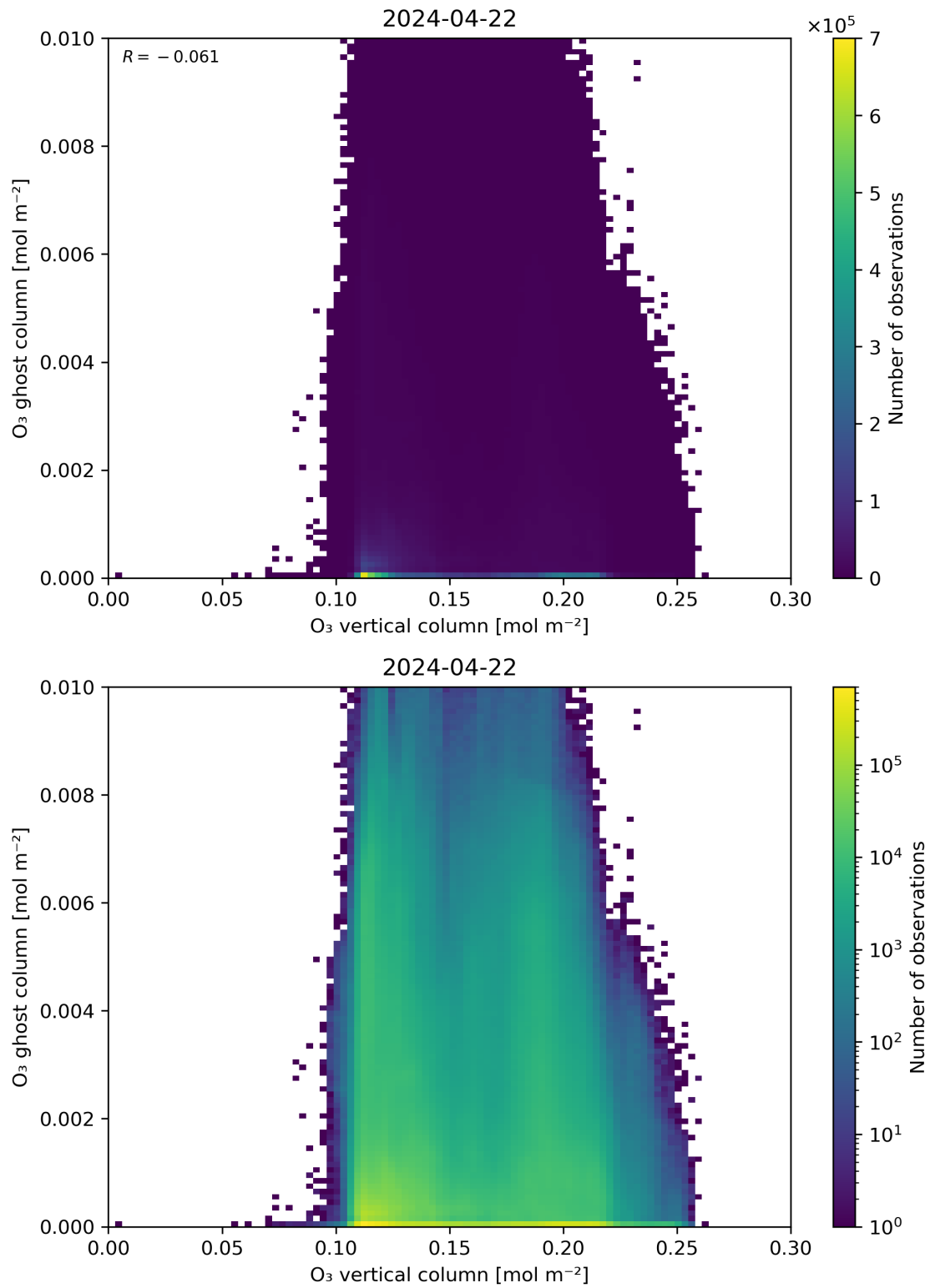
Figure 40: Scatter density plot of “O 3 vertical column” against “O 3 ghost column” for 2024-04-21 to 2024-04-23.
