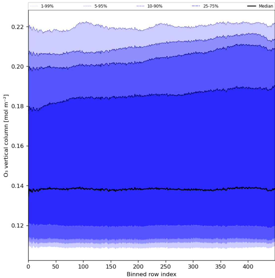
Figure 28: Along track statistics of “O 3 vertical column” for 2024-04-21 to 2024-04-23
