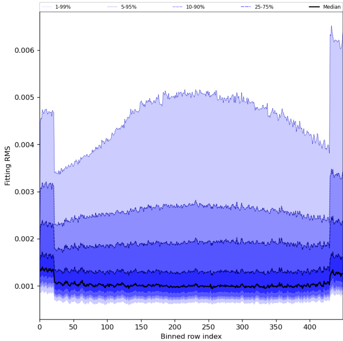
Figure 30: Along track statistics of “Fitting RMS” for 2024-04-21 to 2024-04-23
