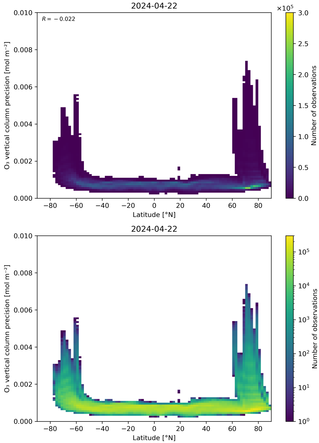
Figure 37: Scatter density plot of “Latitude” against “O 3 vertical column precision” for 2024-04-21 to 2024-04-23.
