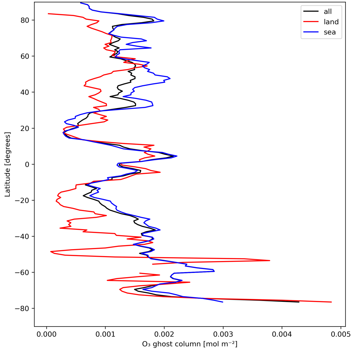
Figure 18: Zonal average of "O 3 ghost column" for 2024-04-21 to 2024-04-23.
