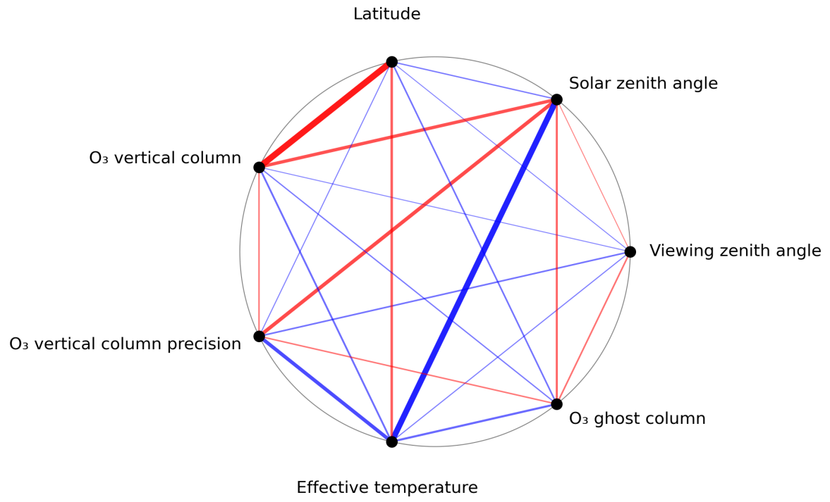
Figure 1: Map of correlation graph for 2024-04-21 to 2024-04-23.
