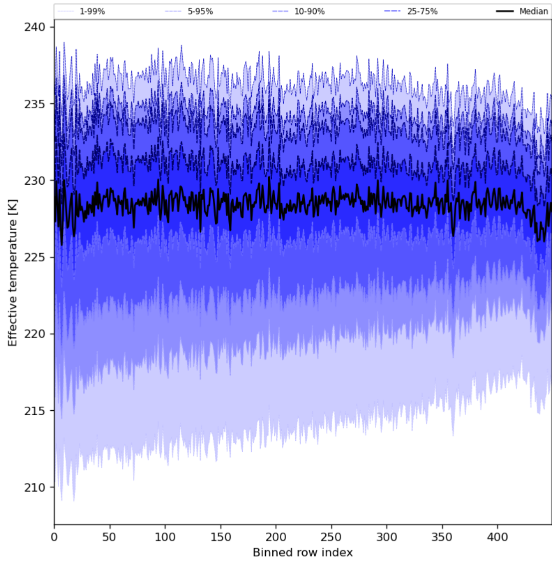
Figure 31: Along track statistics of “Effective temperature” for 2024-04-22 to 2024-04-24
