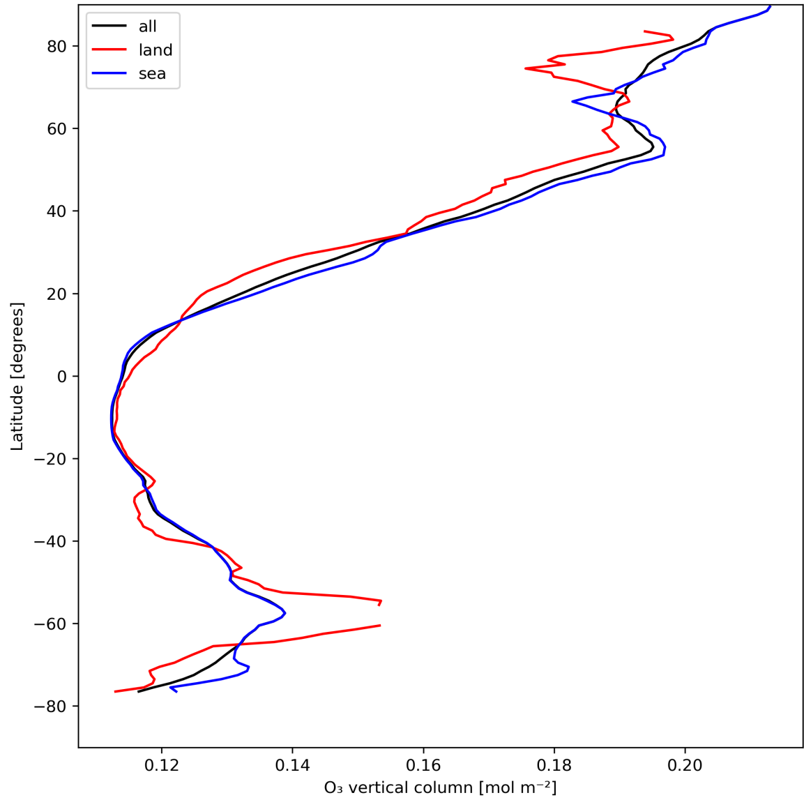
Figure 14: Zonal average of “O 3 vertical column” for 2024-04-22 to 2024-04-24.
