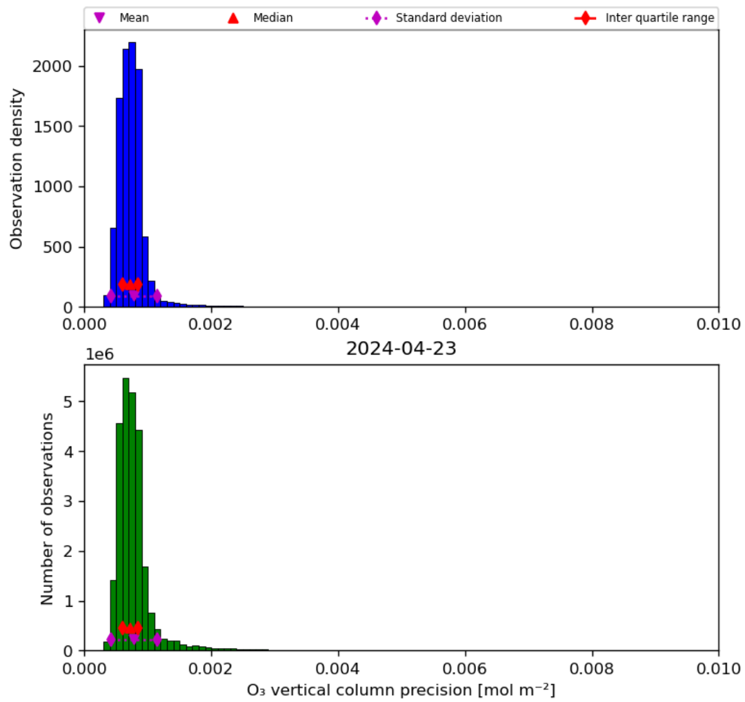
Figure 22: Histogram of “O 3 vertical column precision” for 2024-04-22 to 2024-04-24
