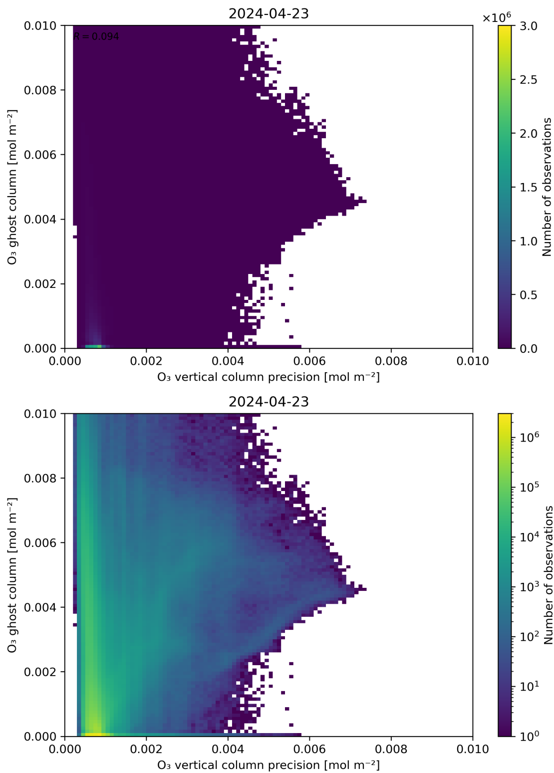
Figure 43: Scatter density plot of “ \text{O}_3 vertical column precision” against “ \text{O}_3 ghost column” for 2024-04-22 to 2024-04-24.
