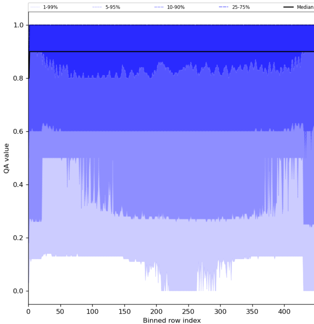
Figure 27: Along track statistics of “QA value” for 2024-04-22 to 2024-04-24
