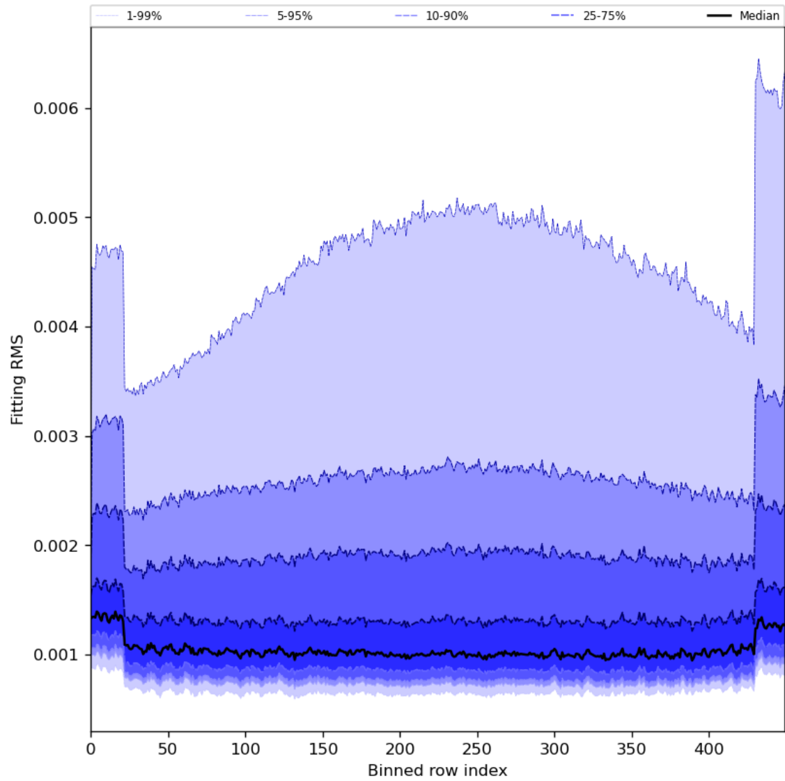
Figure 30: Along track statistics of “Fitting RMS” for 2024-04-22 to 2024-04-24
