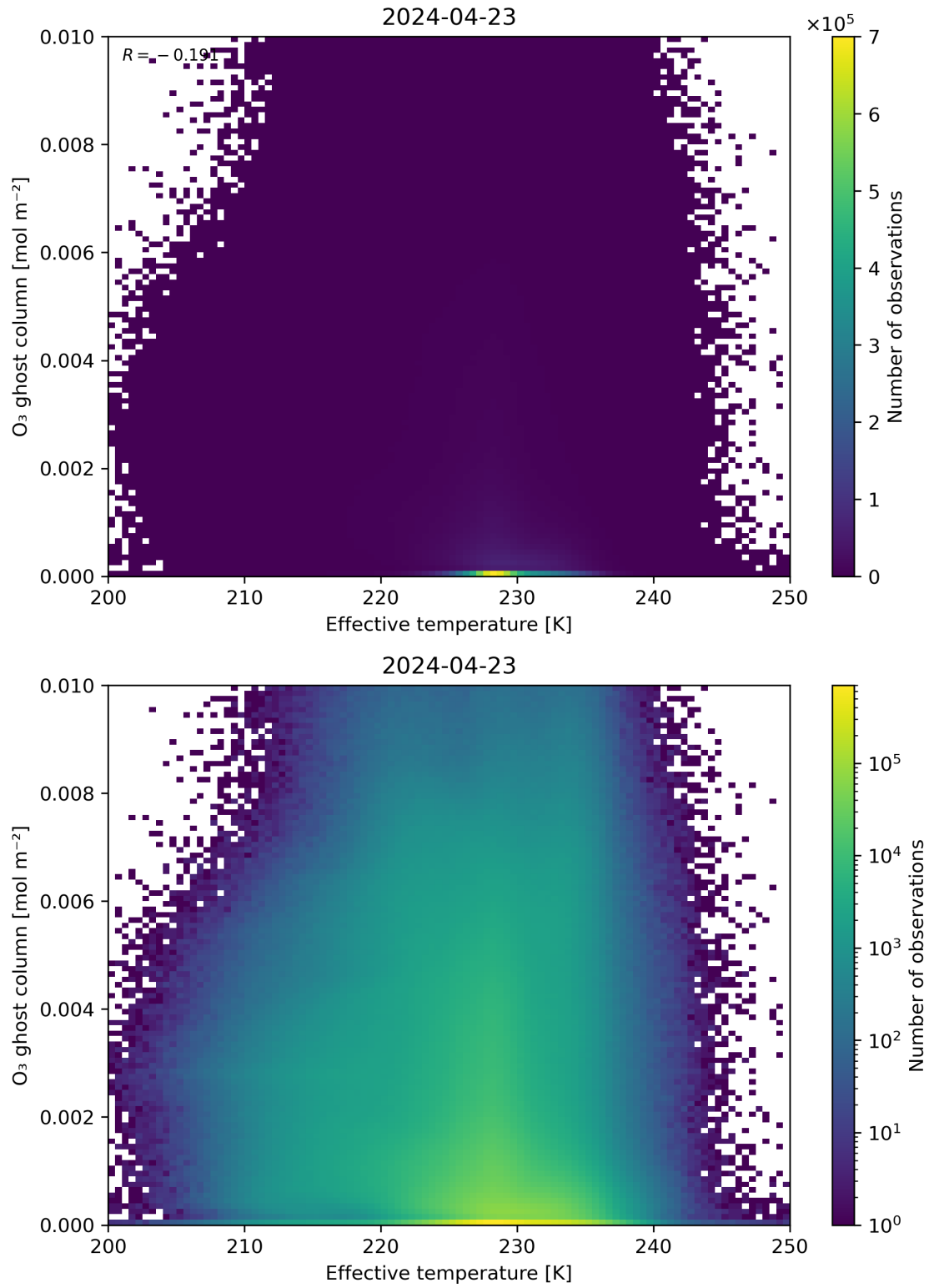
Figure 38: Scatter density plot of “Effective temperature” against “O 3 ghost column” for 2024-04-22 to 2024-04-24.
