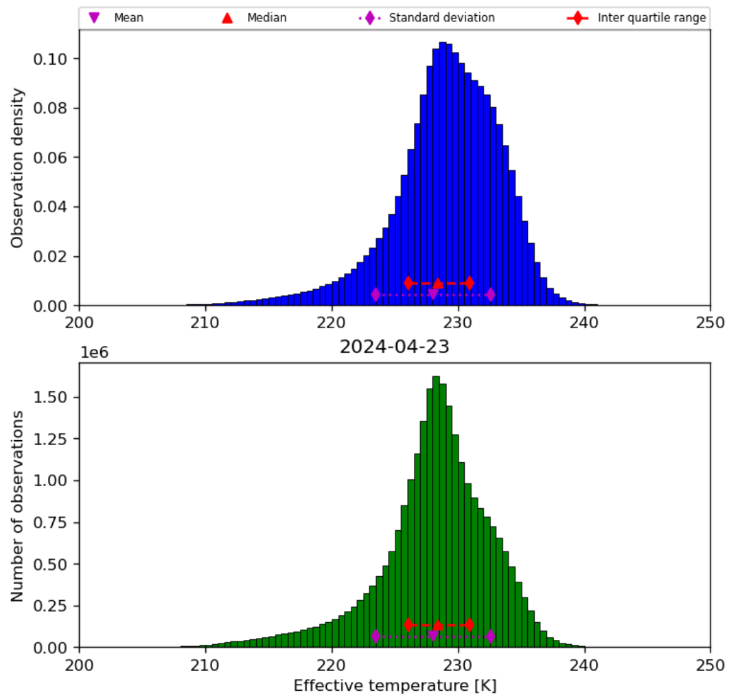
Figure 24: Histogram of “Effective temperature” for 2024-04-22 to 2024-04-24
