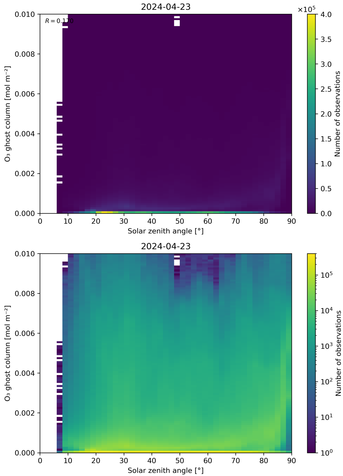
Figure 46: Scatter density plot of “Solar zenith angle” against “O 3 ghost column” for 2024-04-22 to 2024-04-24.
