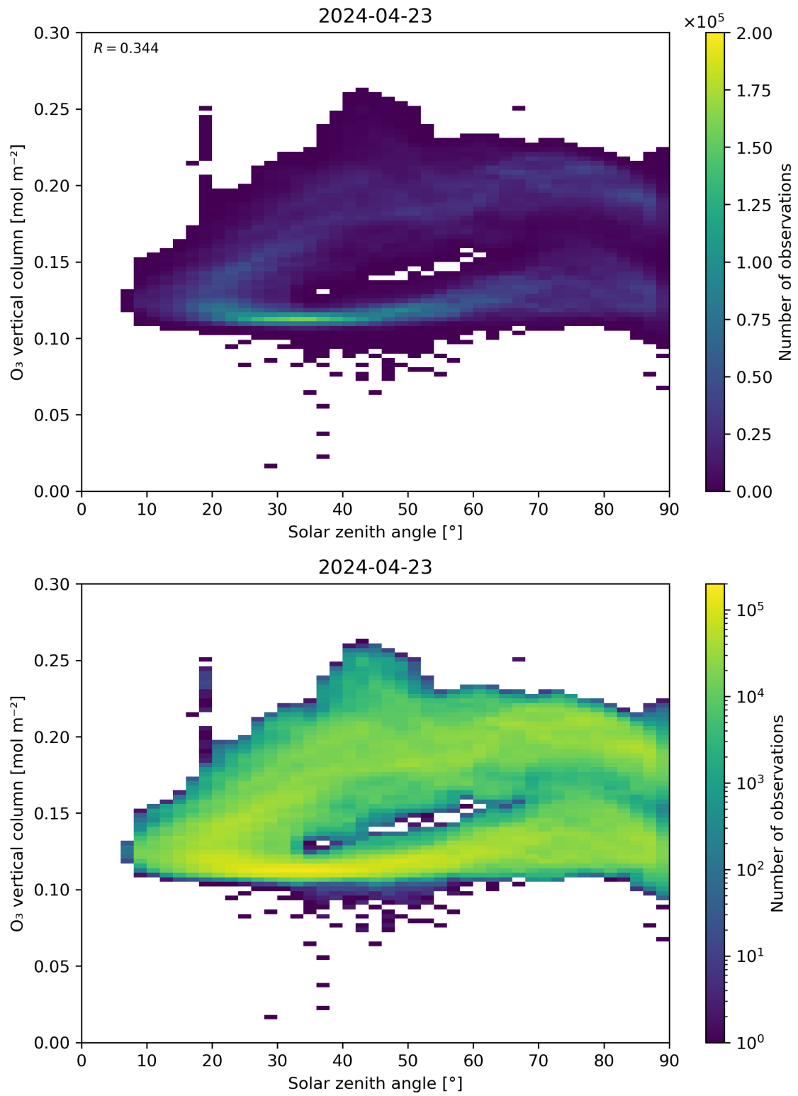
Figure 47: Scatter density plot of “Solar zenith angle” against “O 3 vertical column” for 2024-04-22 to 2024-04-24.
