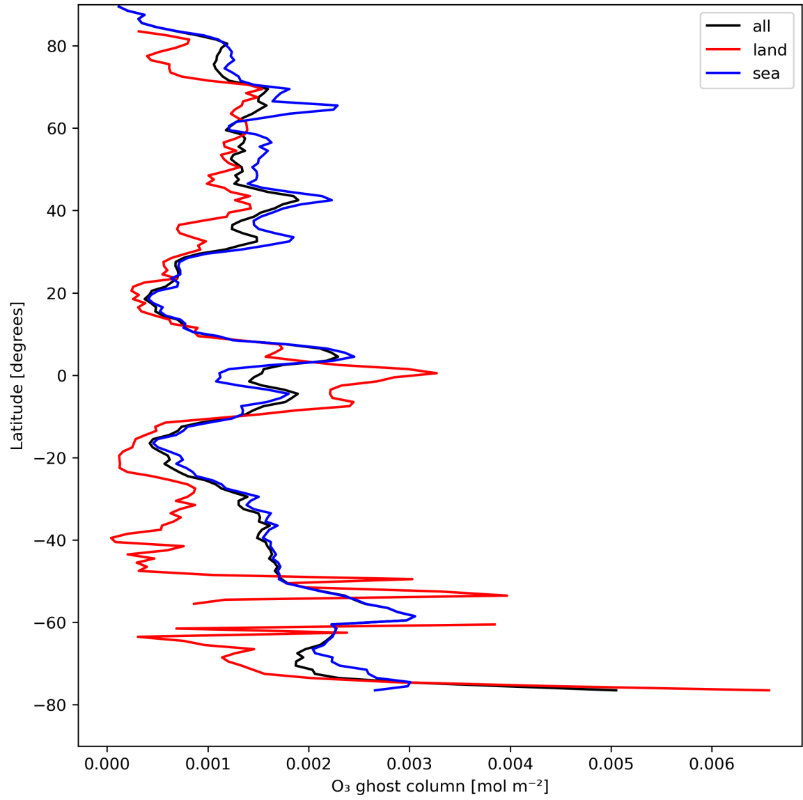
Figure 18: Zonal average of “O 3 ghost column” for 2024-04-22 to 2024-04-24.
