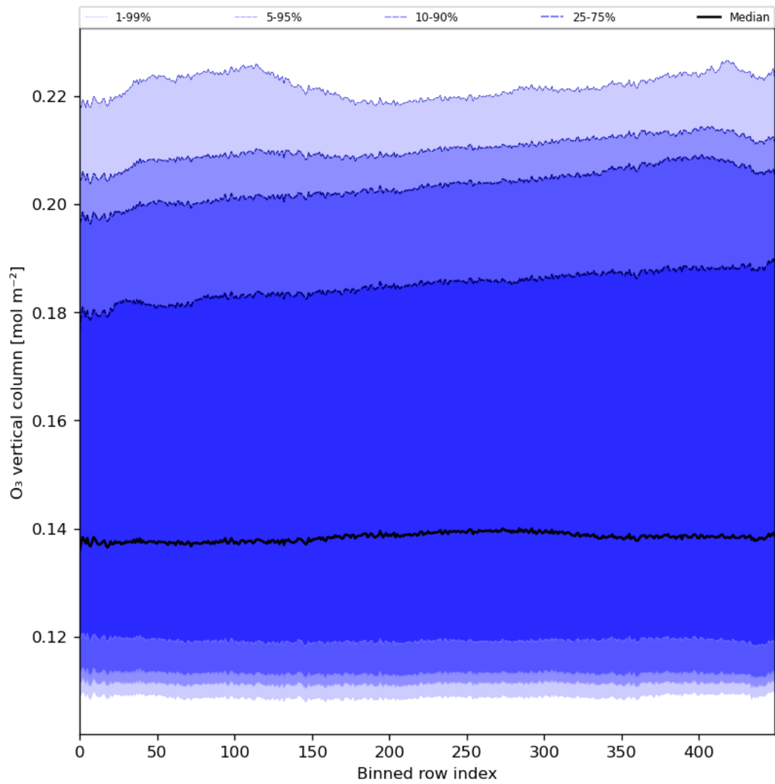
Figure 28: Along track statistics of “O 3 vertical column” for 2024-04-22 to 2024-04-24
