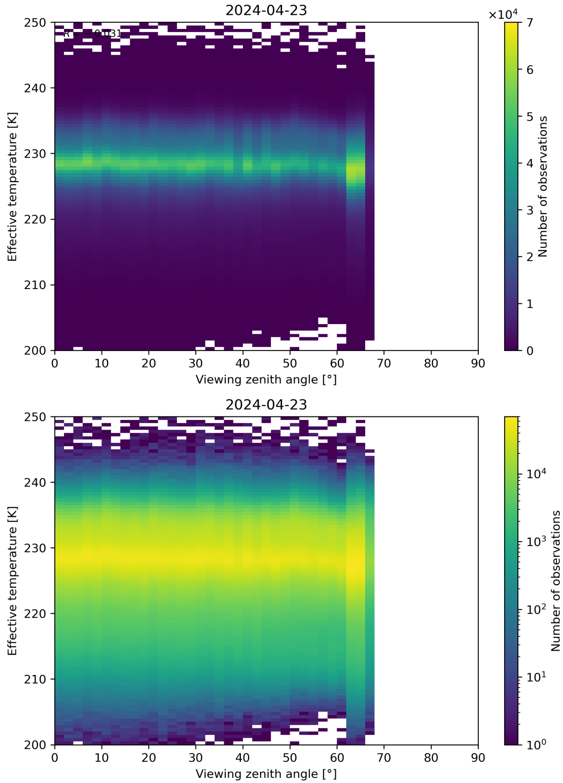
Figure 50: Scatter density plot of “Viewing zenith angle” against “Effective temperature” for 2024-04-22 to 2024-04-24.
