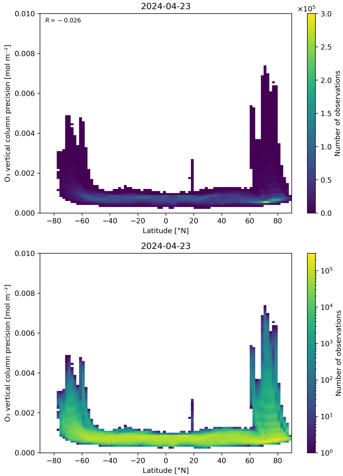
Figure 37: Scatter density plot of “Latitude” against “O 3 vertical column precision” for 2024-04-22 to 2024-04-24.
