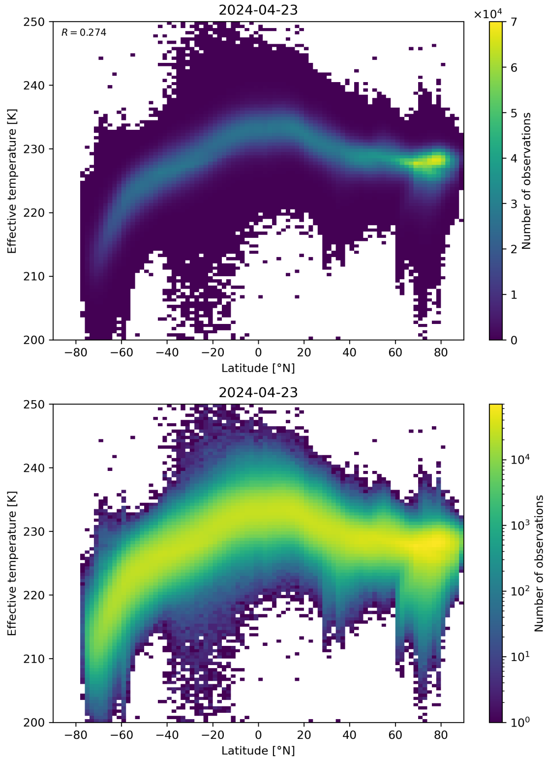
Figure 34: Scatter density plot of “Latitude” against “Effective temperature” for 2024-04-22 to 2024-04-24.
