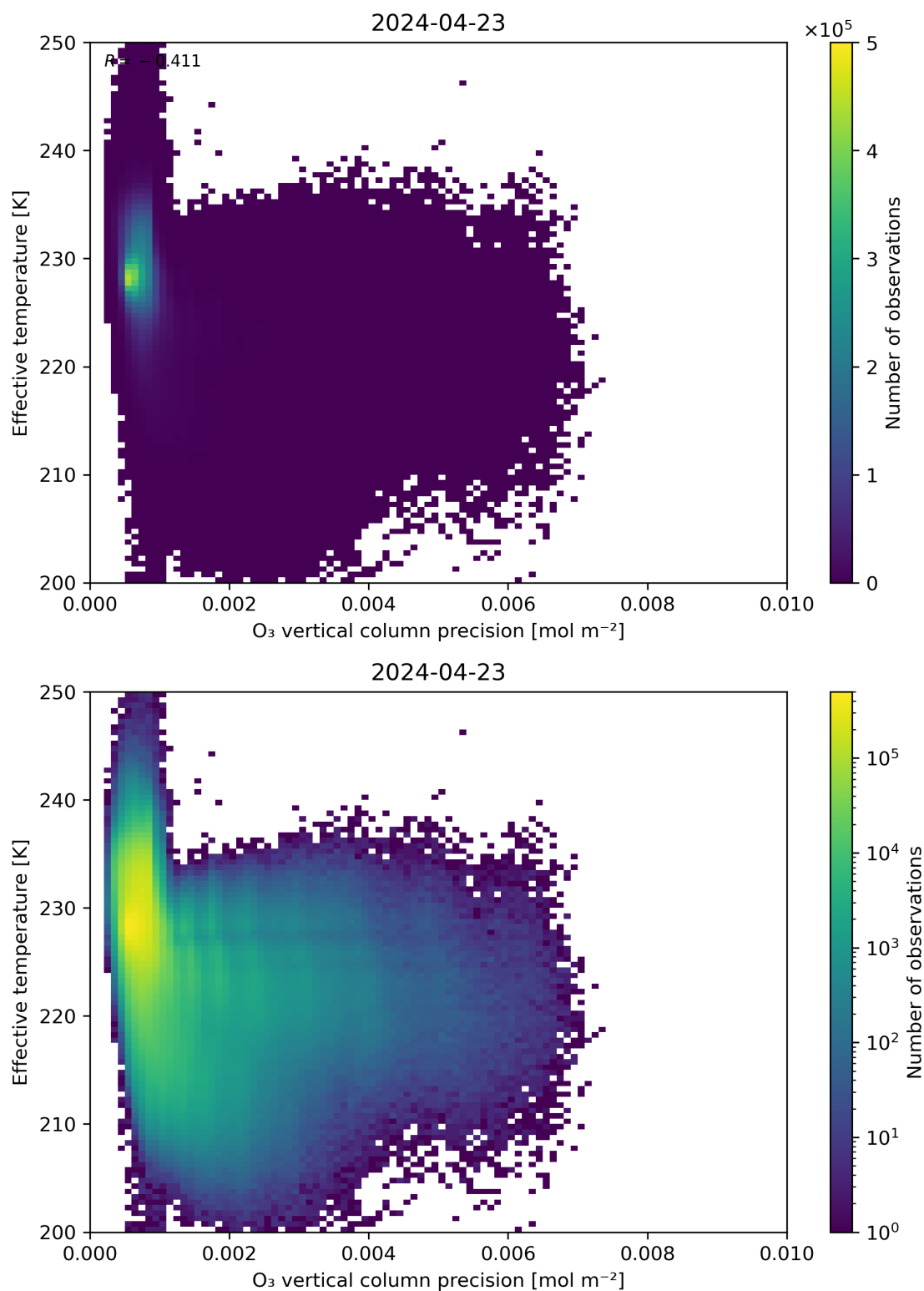
Figure 42: Scatter density plot of “O 3 vertical column precision” against “Effective temperature” for 2024-04-22 to 2024-04-24.
