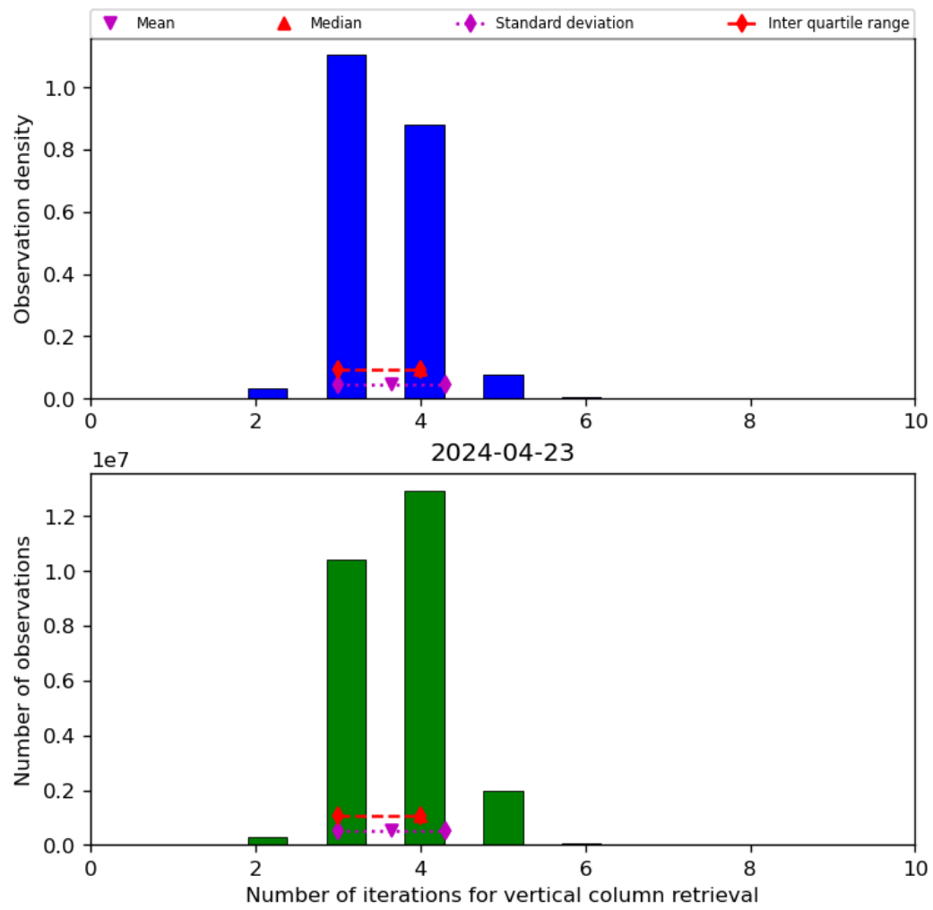
Figure 26: Histogram of “Number of iterations for vertical column retrieval” for 2024-04-22 to 2024-04-24
