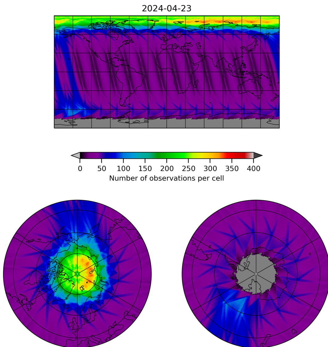
Figure 12: Map of the number of observations for 2024-04-22 to 2024-04-24
