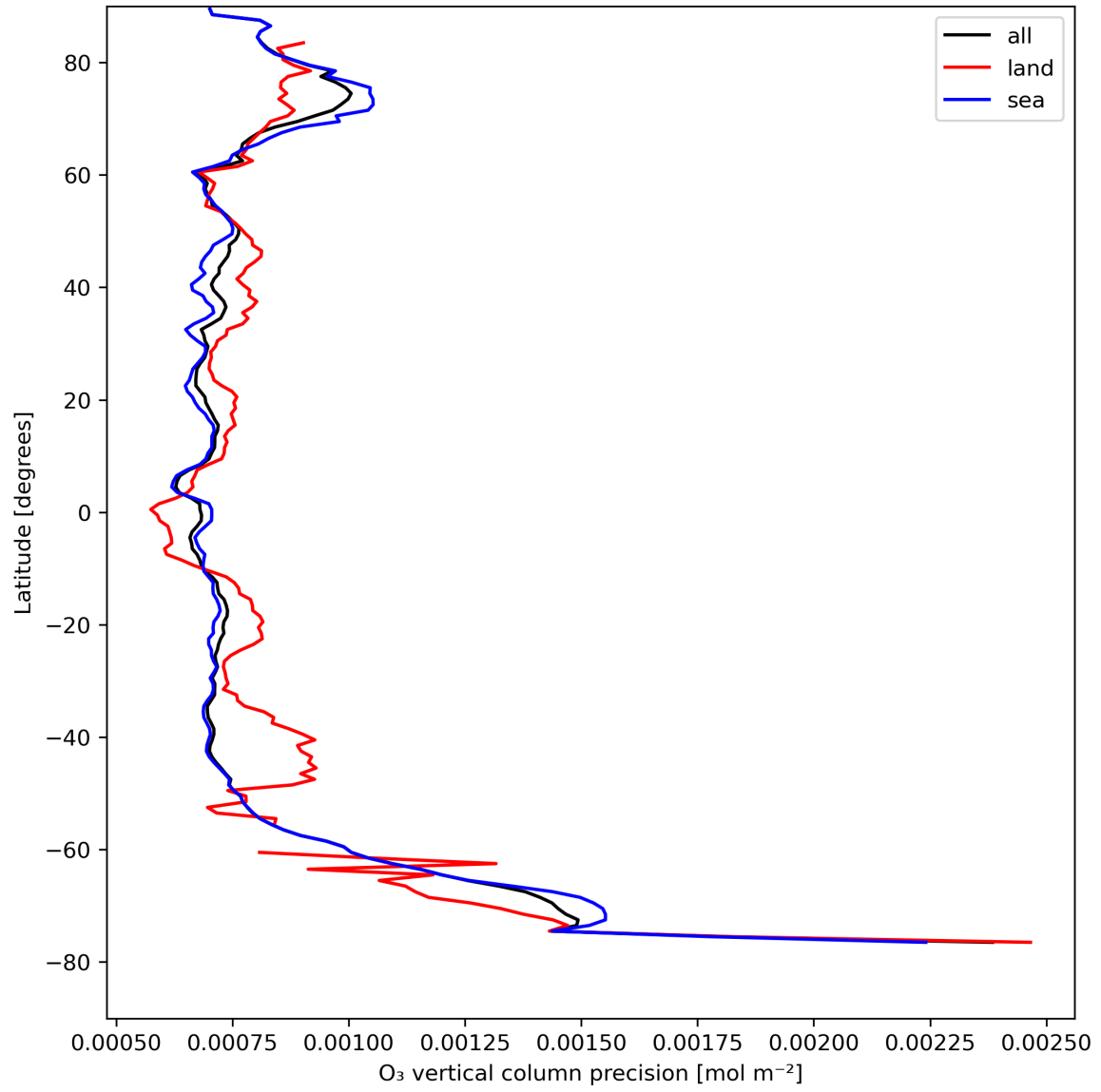
Figure 15: Zonal average of “O 3 vertical column precision” for 2024-04-22 to 2024-04-24.
