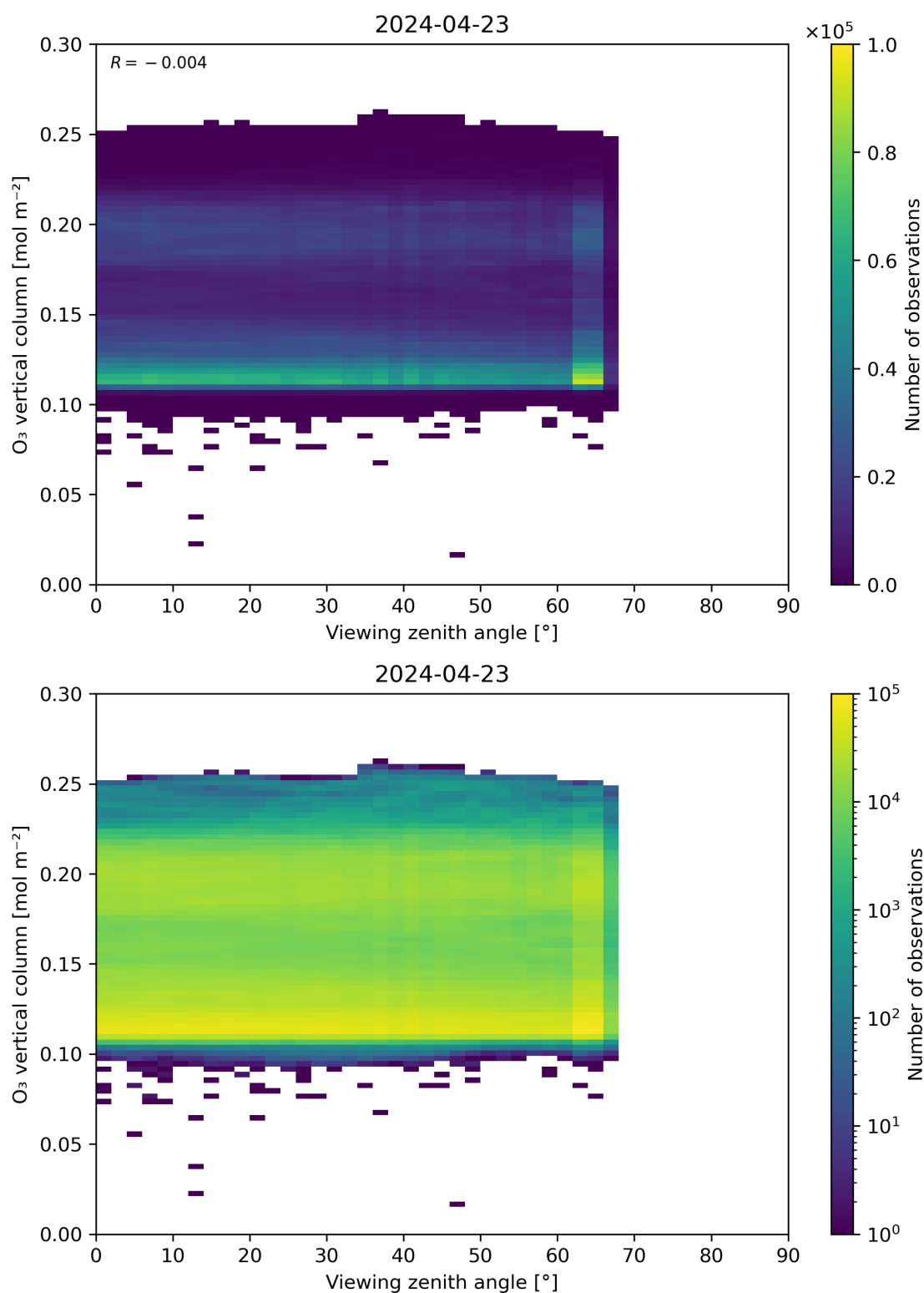
Figure 52: Scatter density plot of “Viewing zenith angle” against “O 3 vertical column” for 2024-04-22 to 2024-04-24.
