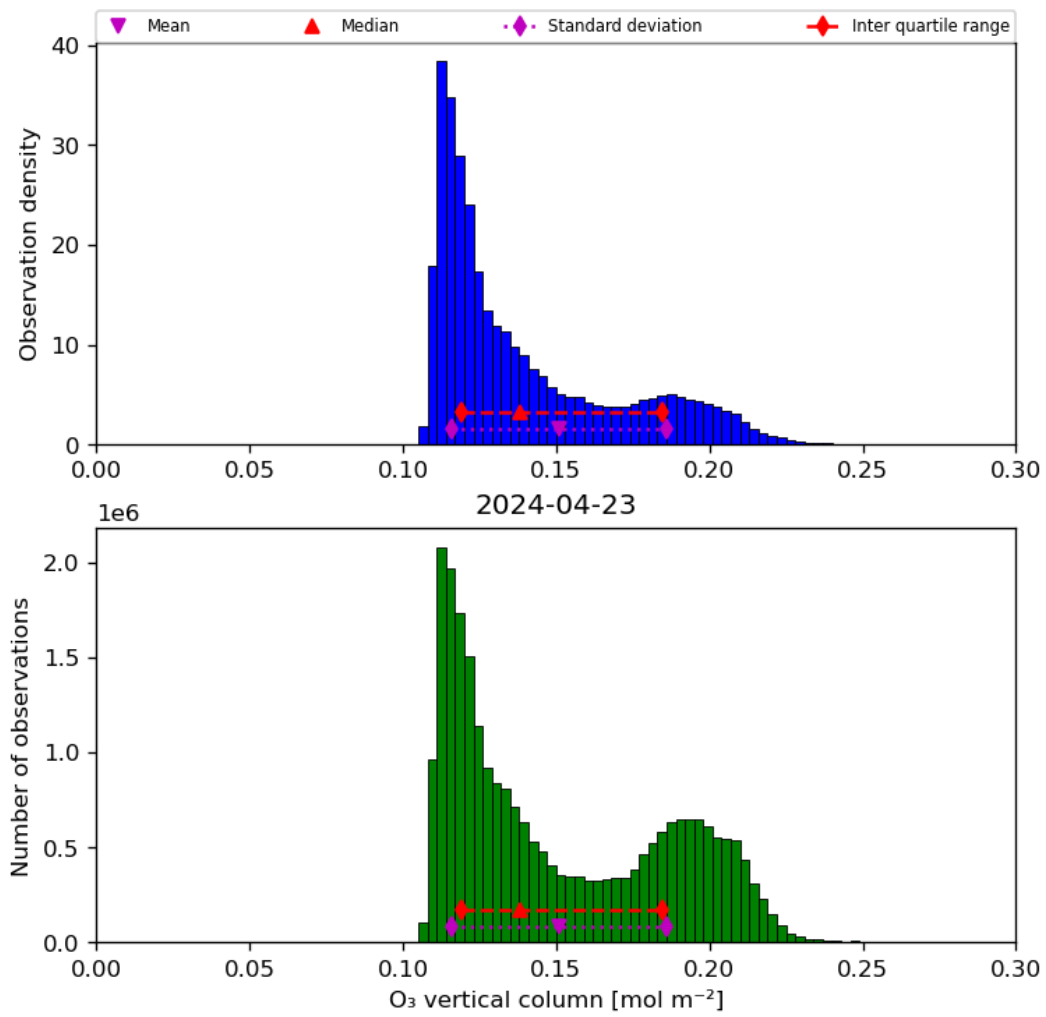
Figure 21: Histogram of “O 3 vertical column” for 2024-04-22 to 2024-04-24
