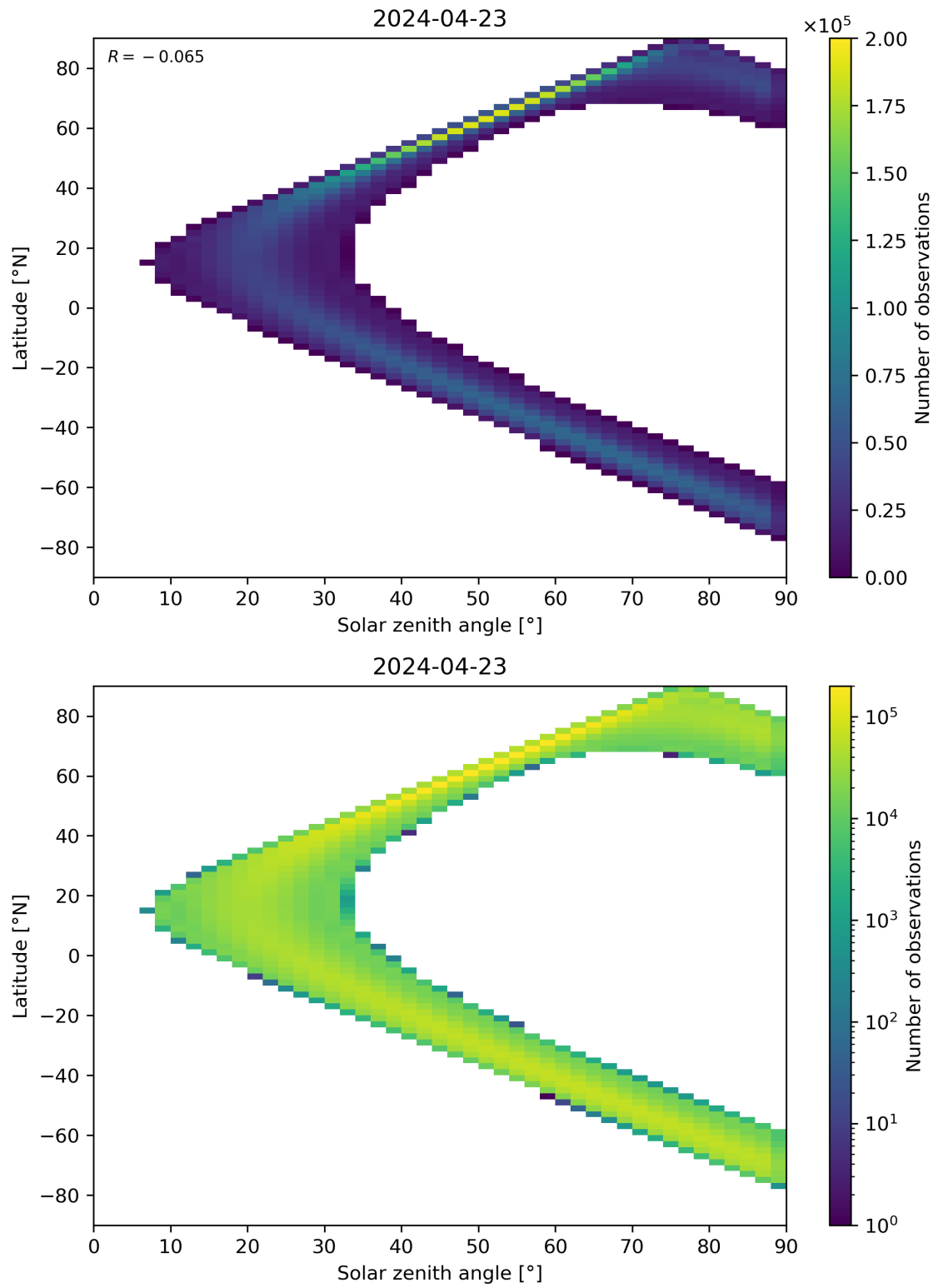
Figure 44: Scatter density plot of “Solar zenith angle” against “Latitude” for 2024-04-22 to 2024-04-24.
