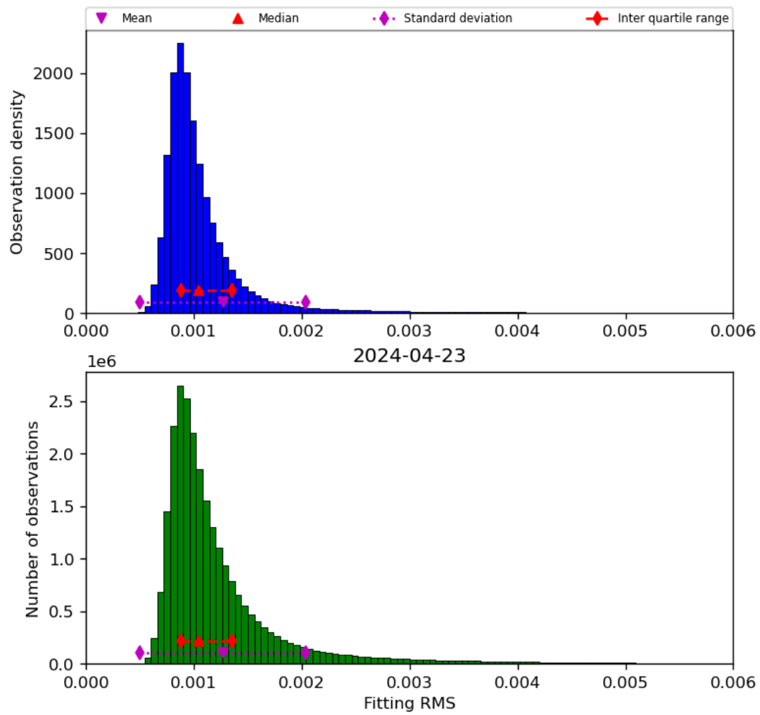
Figure 23: Histogram of “Fitting RMS” for 2024-04-22 to 2024-04-24
