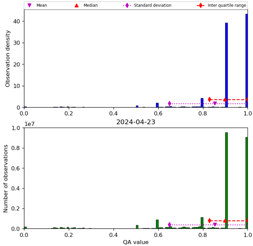
Figure 20: Histogram of “QA value” for 2024-04-22 to 2024-04-24
