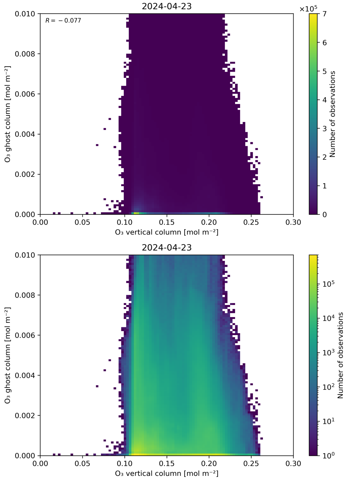
Figure 40: Scatter density plot of “O 3 vertical column” against “O 3 ghost column” for 2024-04-22 to 2024-04-24.
