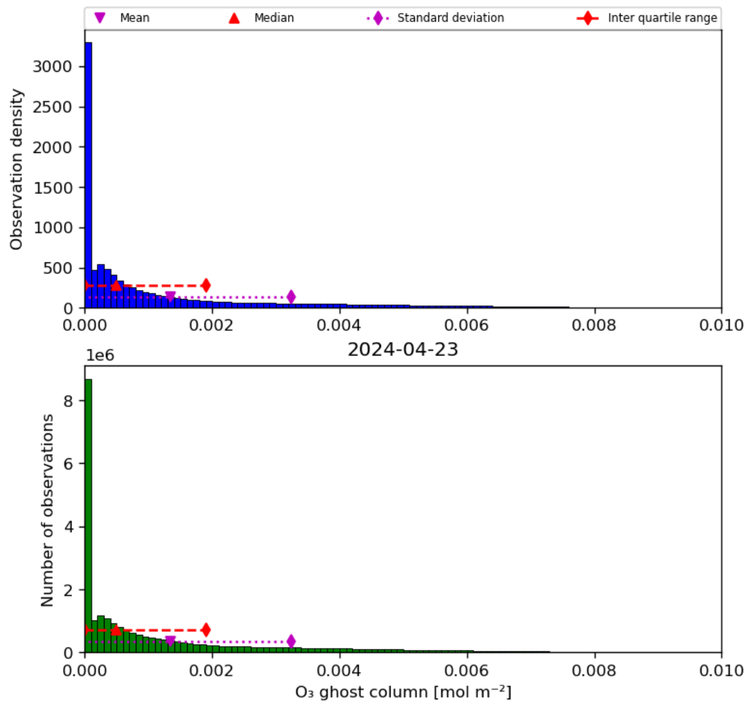
Figure 25: Histogram of “O 3 ghost column” for 2024-04-22 to 2024-04-24
