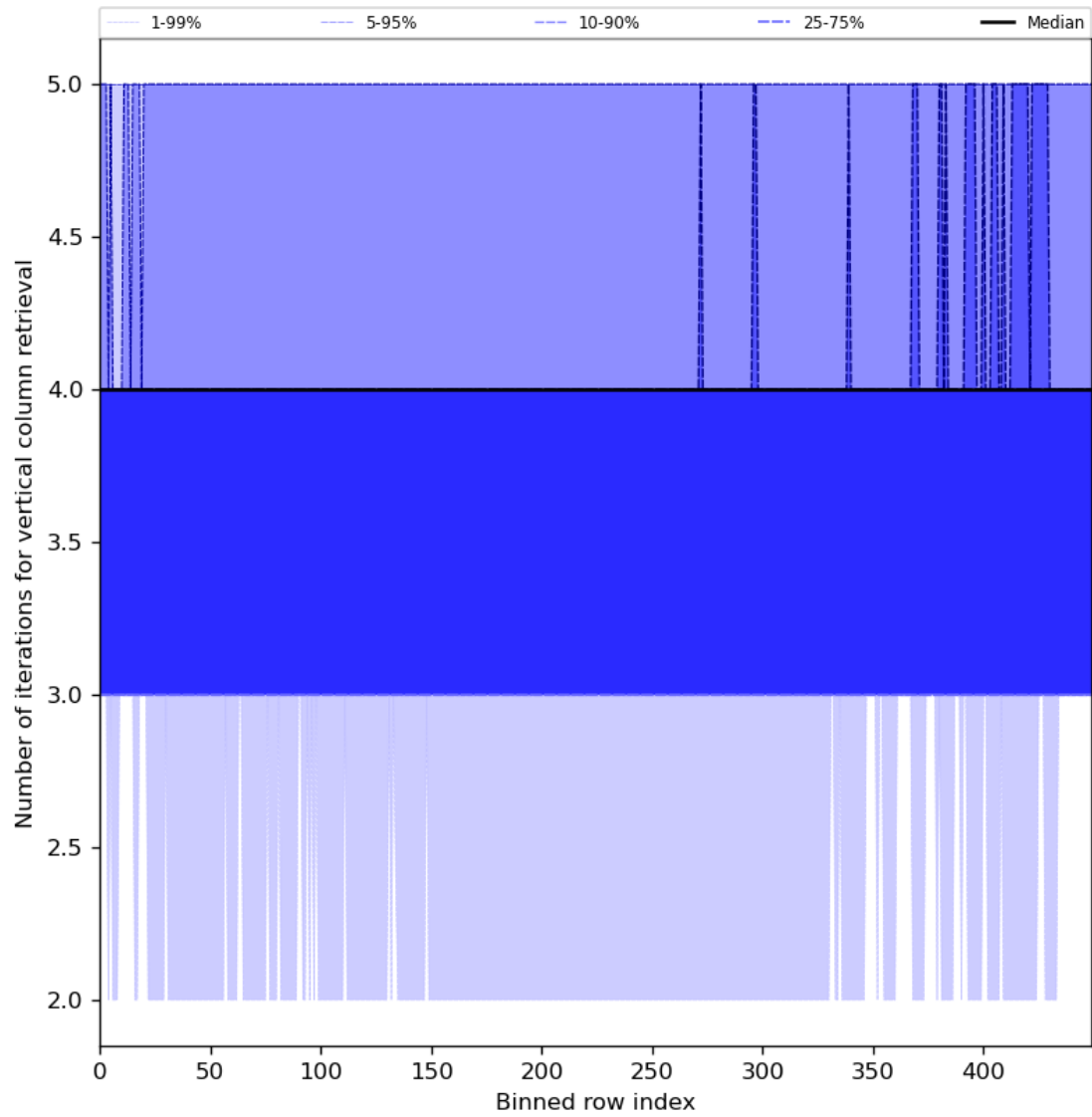
Figure 33: Along track statistics of “Number of iterations for vertical column retrieval” for 2024-04-22 to 2024-04-24
