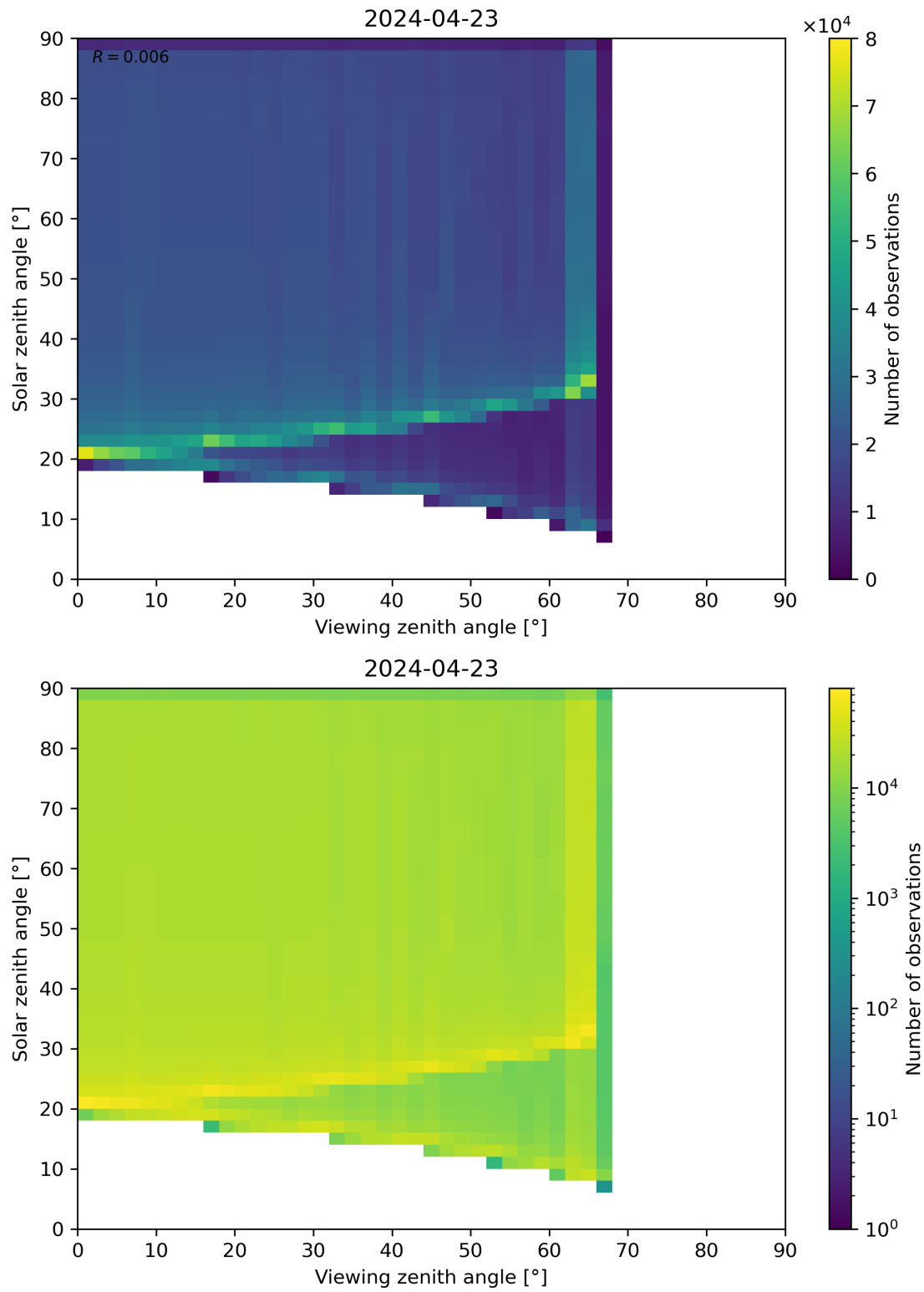
Figure 54: Scatter density plot of “Viewing zenith angle” against “Solar zenith angle” for 2024-04-22 to 2024-04-24.
