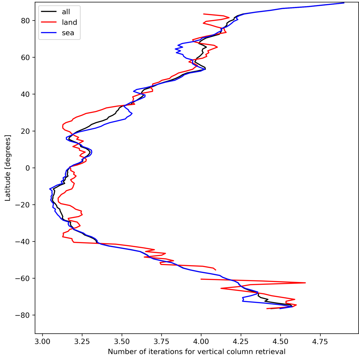
Figure 19: Zonal average of “Number of iterations for vertical column retrieval” for 2024-04-22 to 2024-04-24.
