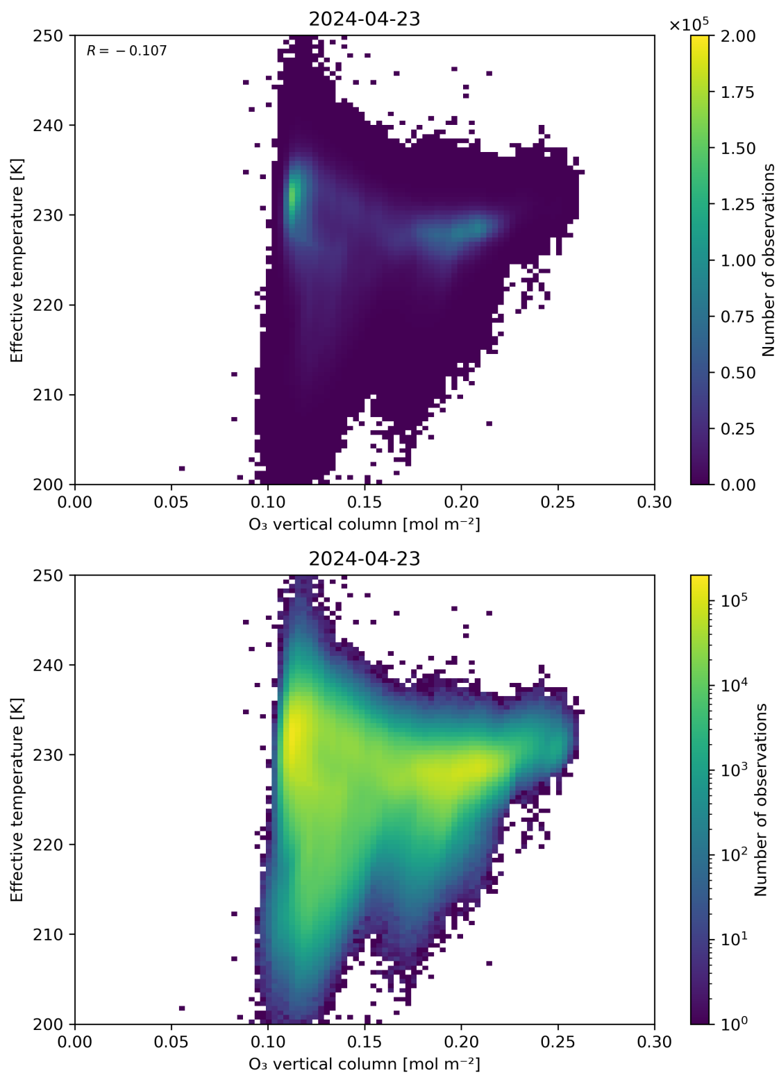
Figure 39: Scatter density plot of “O 3 vertical column” against “Effective temperature” for 2024-04-22 to 2024-04-24.
