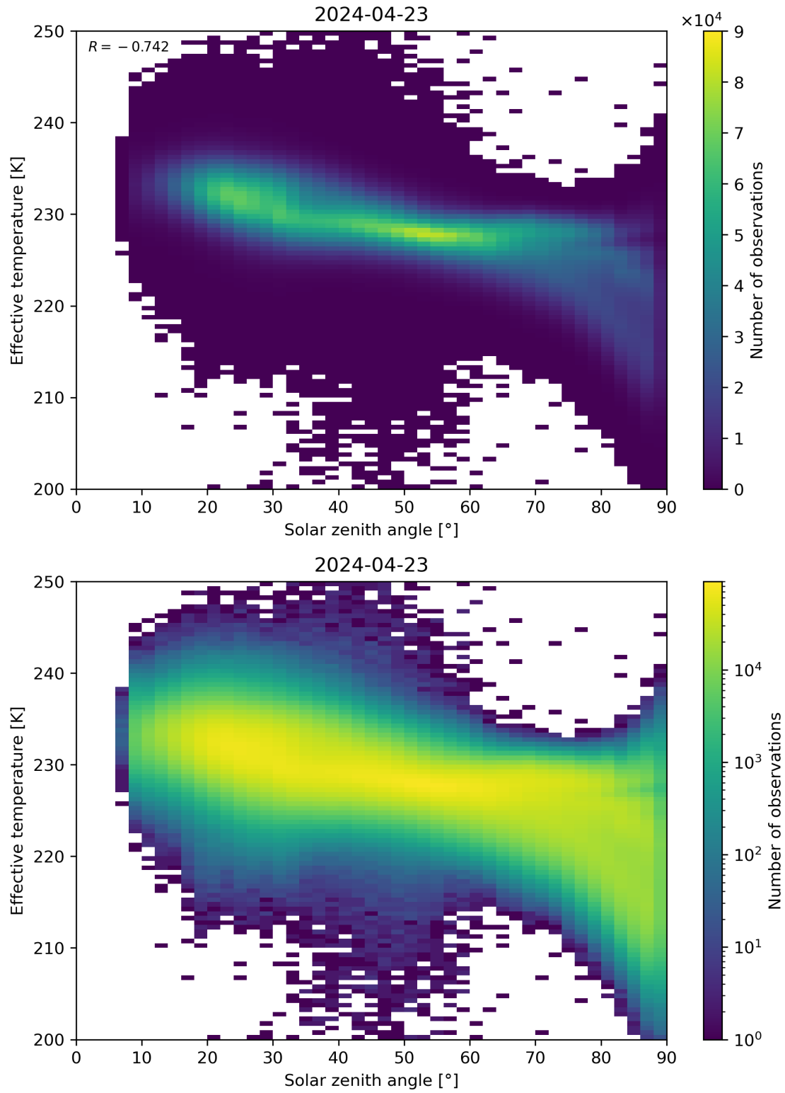
Figure 45: Scatter density plot of “Solar zenith angle” against “Effective temperature” for 2024-04-22 to 2024-04-24.
