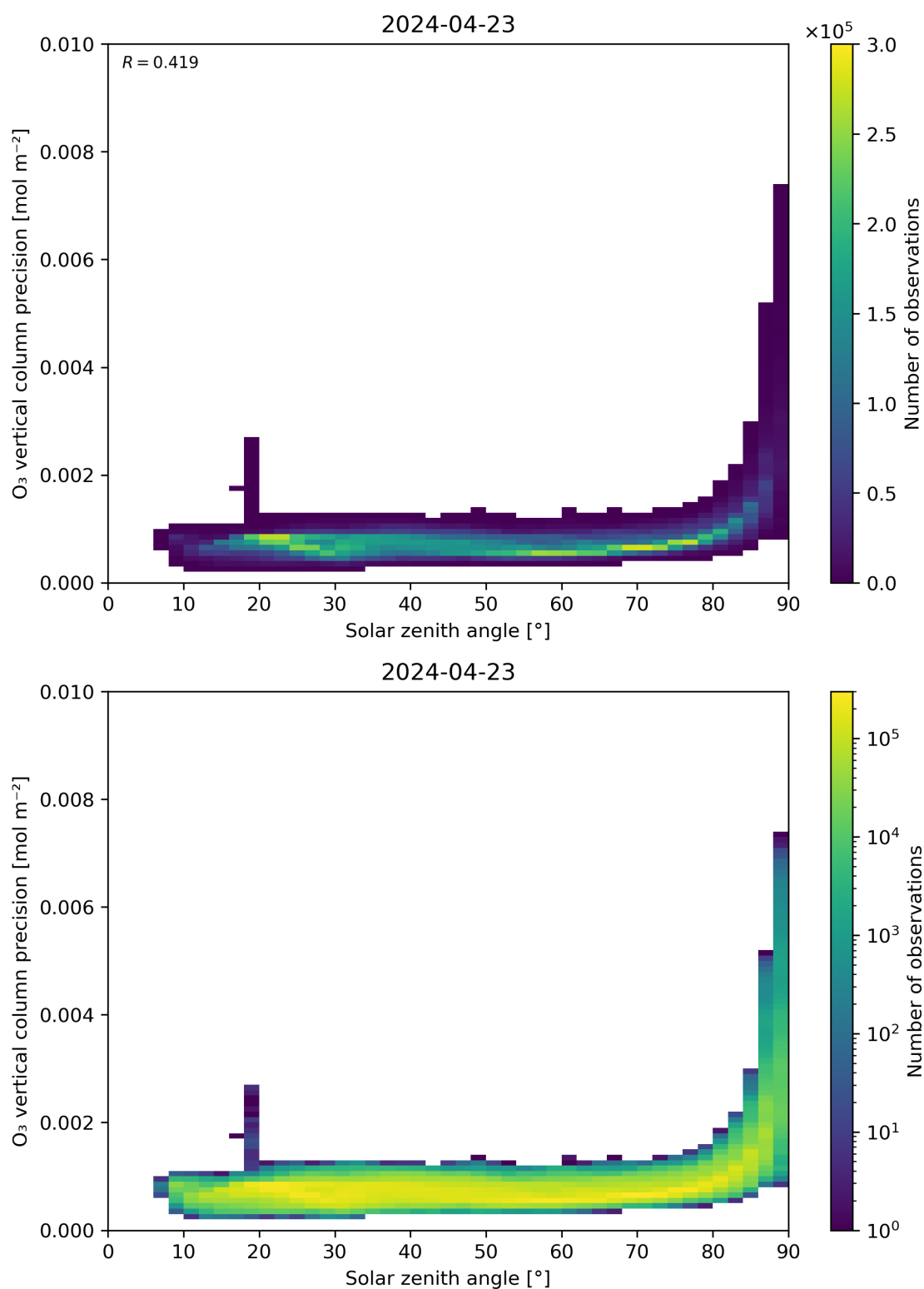
Figure 48: Scatter density plot of “Solar zenith angle” against “O 3 vertical column precision” for 2024-04-22 to 2024-04-24.
