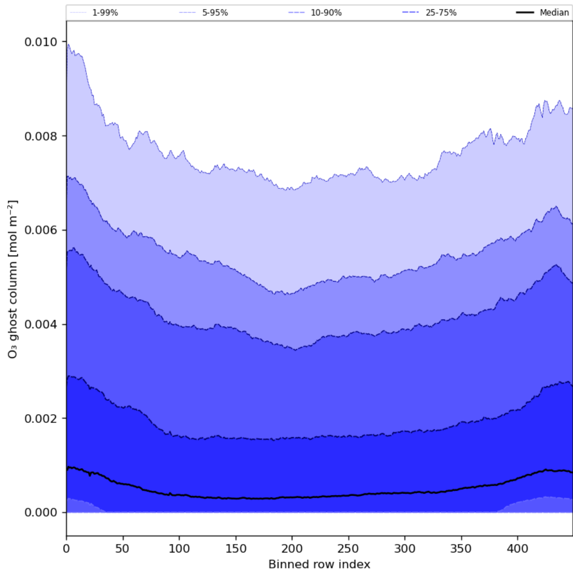
Figure 32: Along track statistics of “O 3 ghost column” for 2024-04-22 to 2024-04-24
