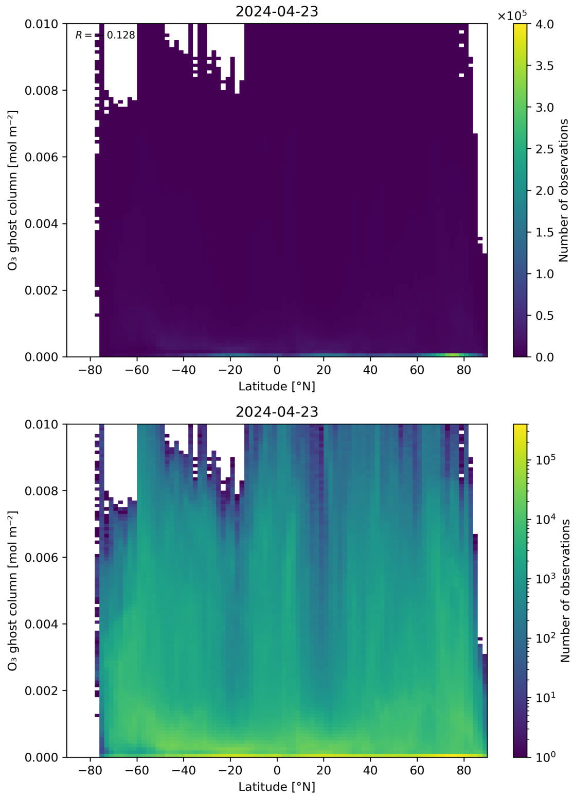
Figure 35: Scatter density plot of “Latitude” against “O 3 ghost column” for 2024-04-22 to 2024-04-24.
