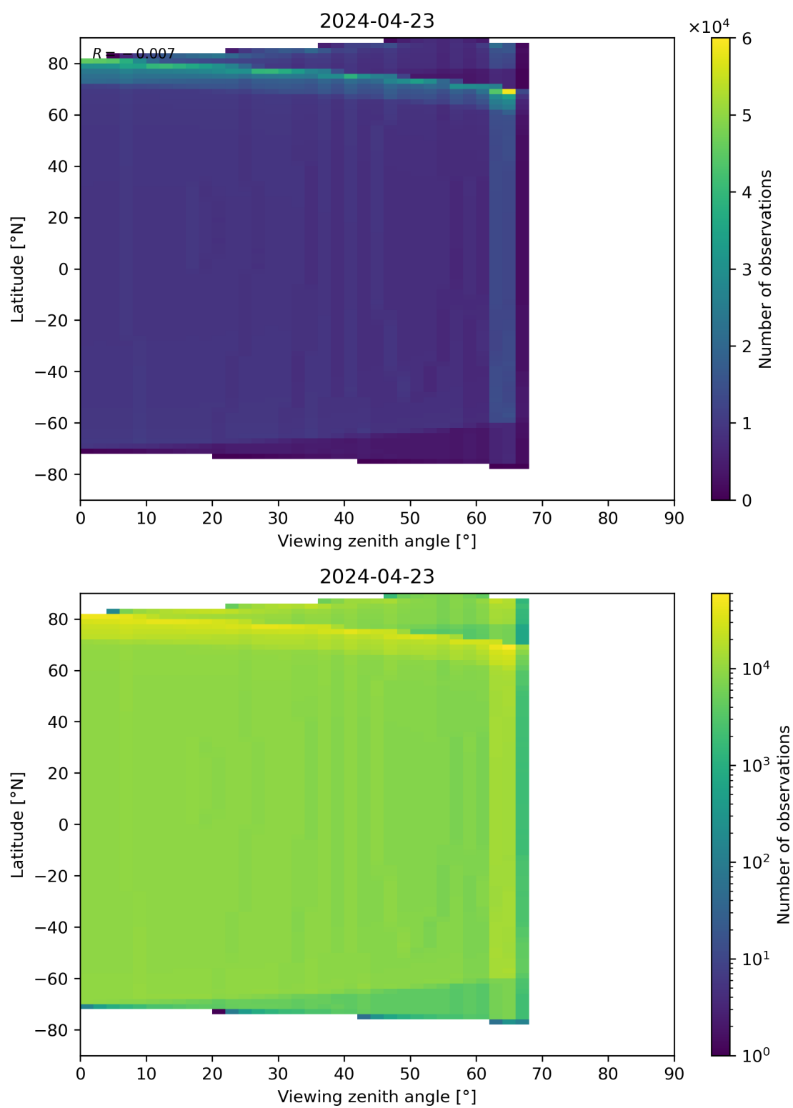
Figure 49: Scatter density plot of “Viewing zenith angle” against “Latitude” for 2024-04-22 to 2024-04-24.
