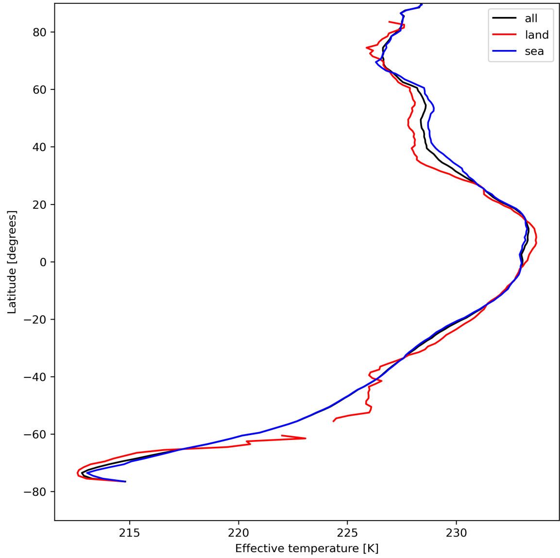
Figure 17: Zonal average of “Effective temperature” for 2024-04-22 to 2024-04-24.
