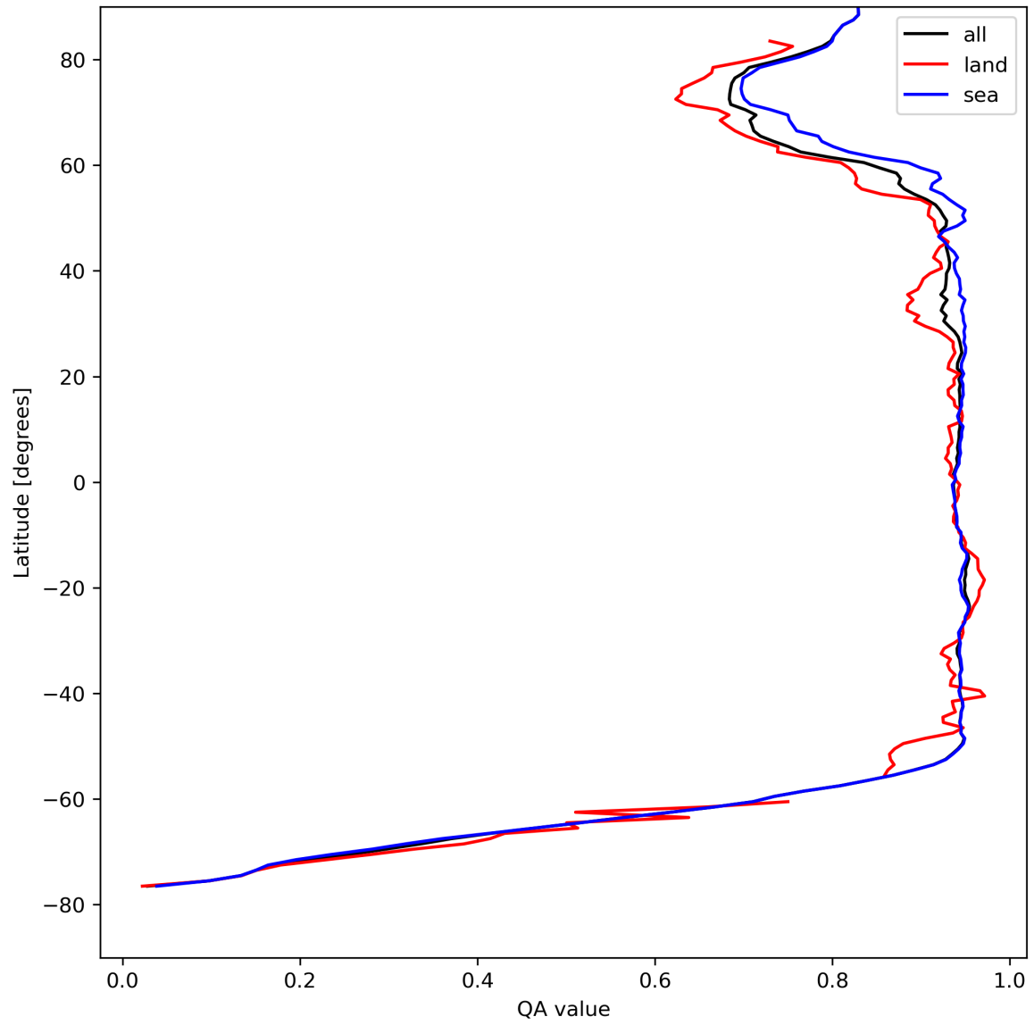
Figure 13: Zonal average of “QA value” for 2024-04-22 to 2024-04-24.
