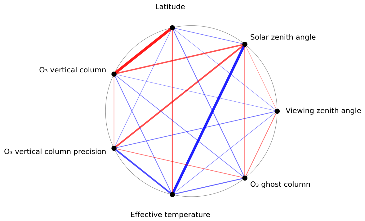
Figure 1: Map of correlation graph for 2024-04-22 to 2024-04-24.
