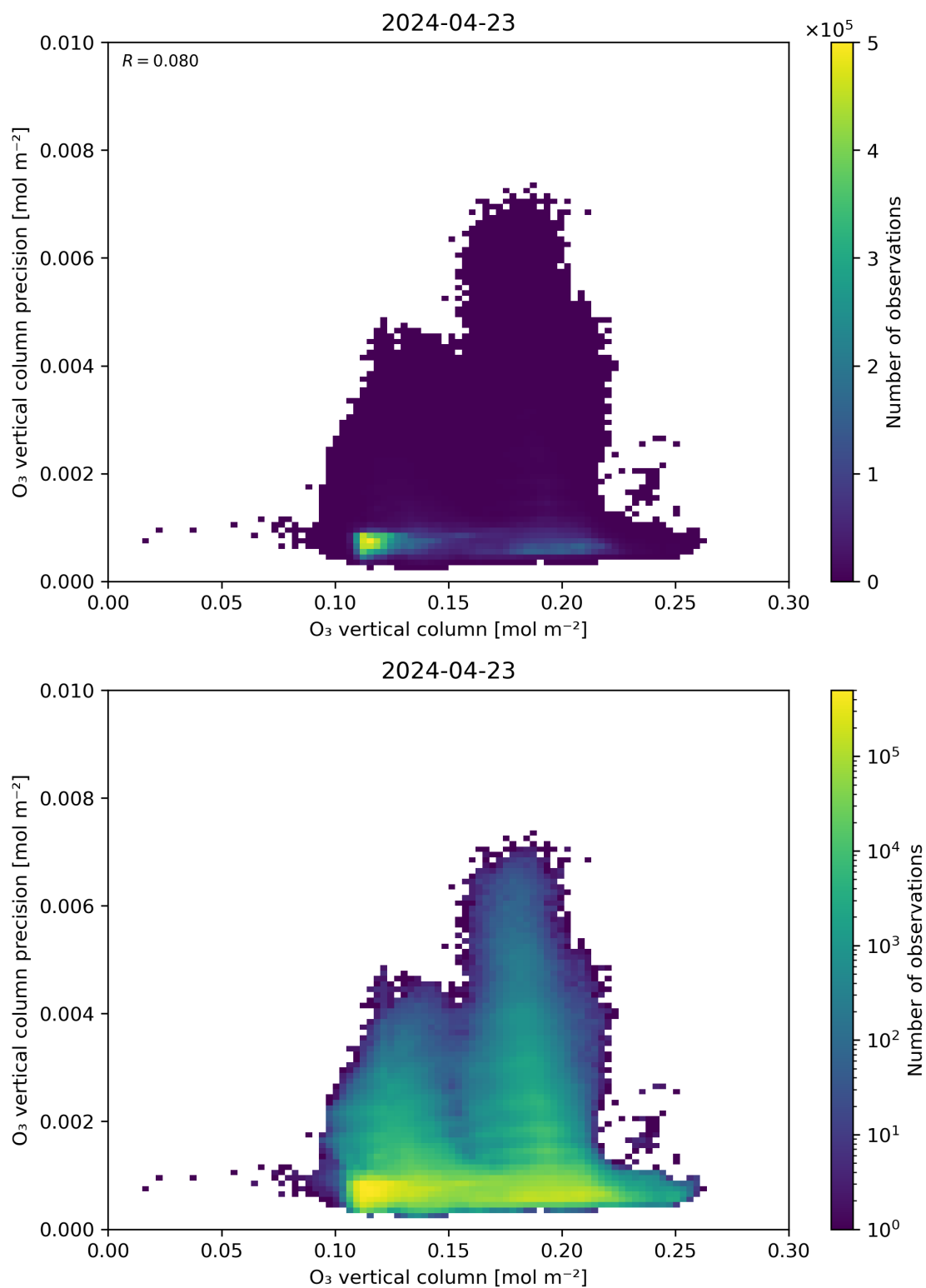
Figure 41: Scatter density plot of “O 3 vertical column” against “O 3 vertical column precision” for 2024-04-22 to 2024-04-24.
