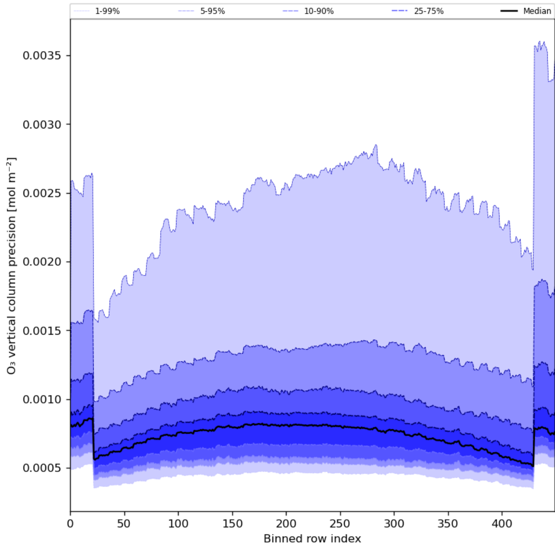
Figure 29: Along track statistics of “O 3 vertical column precision” for 2024-04-22 to 2024-04-24
