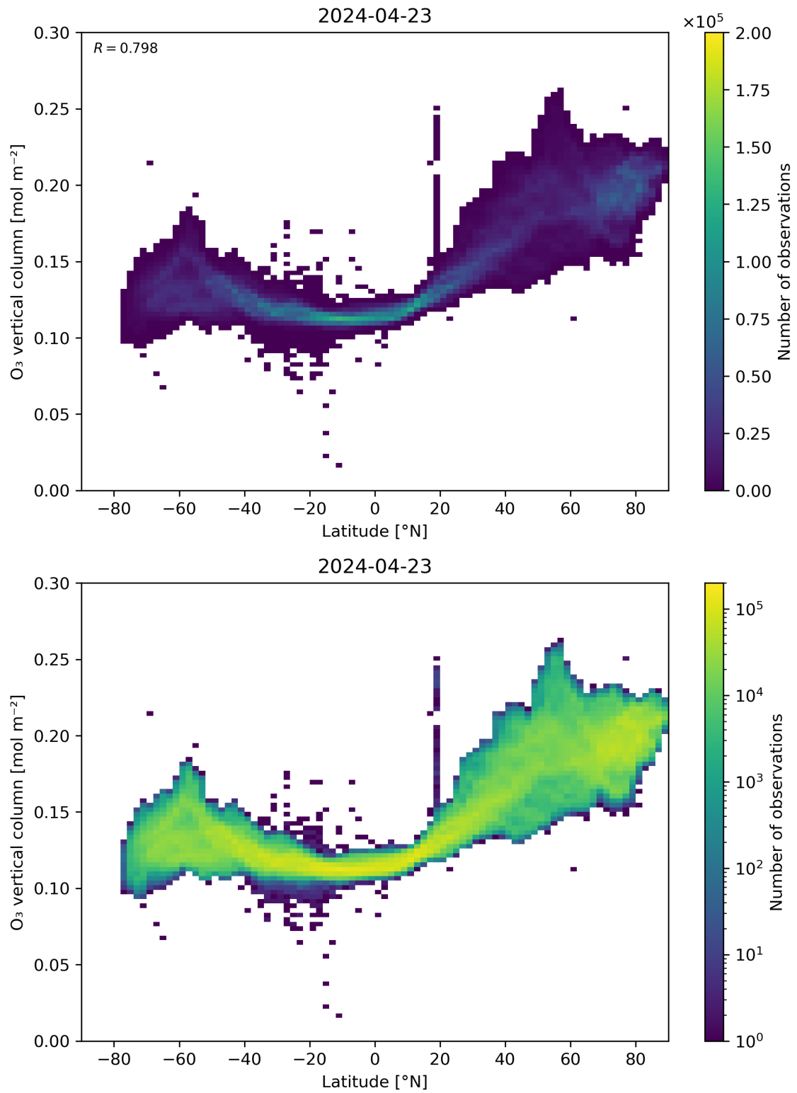
Figure 36: Scatter density plot of “Latitude” against “O 3 vertical column” for 2024-04-22 to 2024-04-24.
