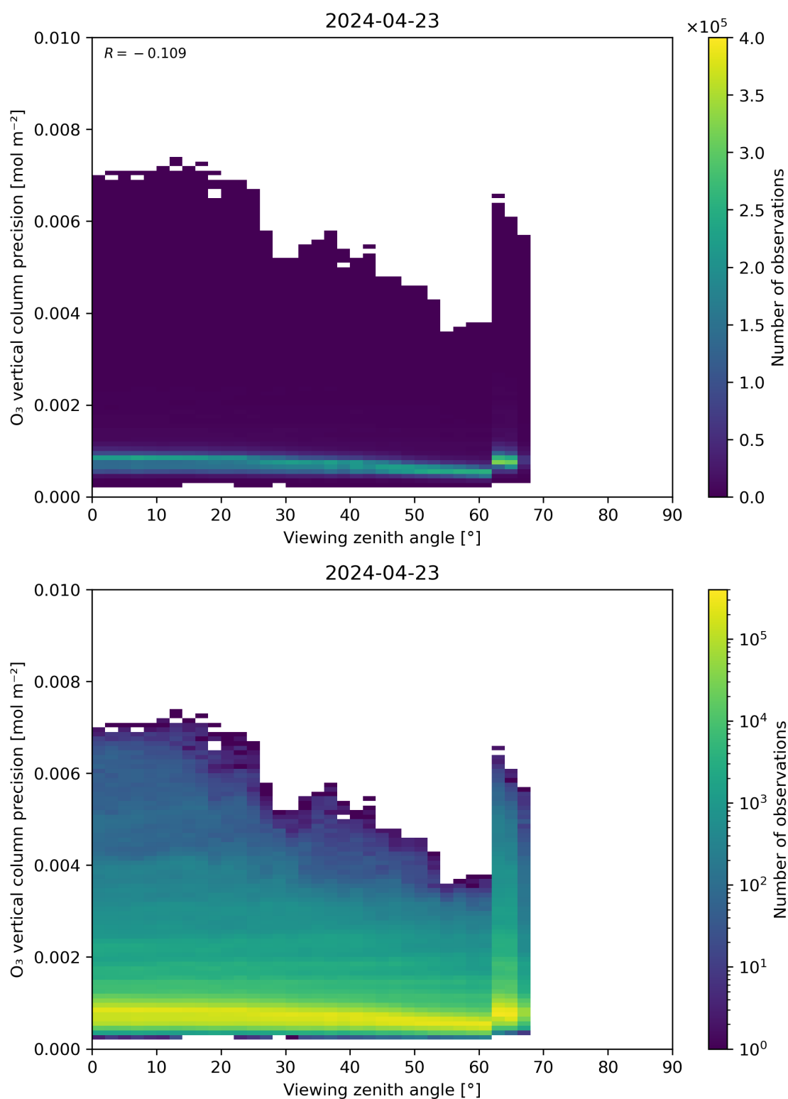
Figure 53: Scatter density plot of “Viewing zenith angle” against “O 3 vertical column precision” for 2024-04-22 to 2024-04-24.
