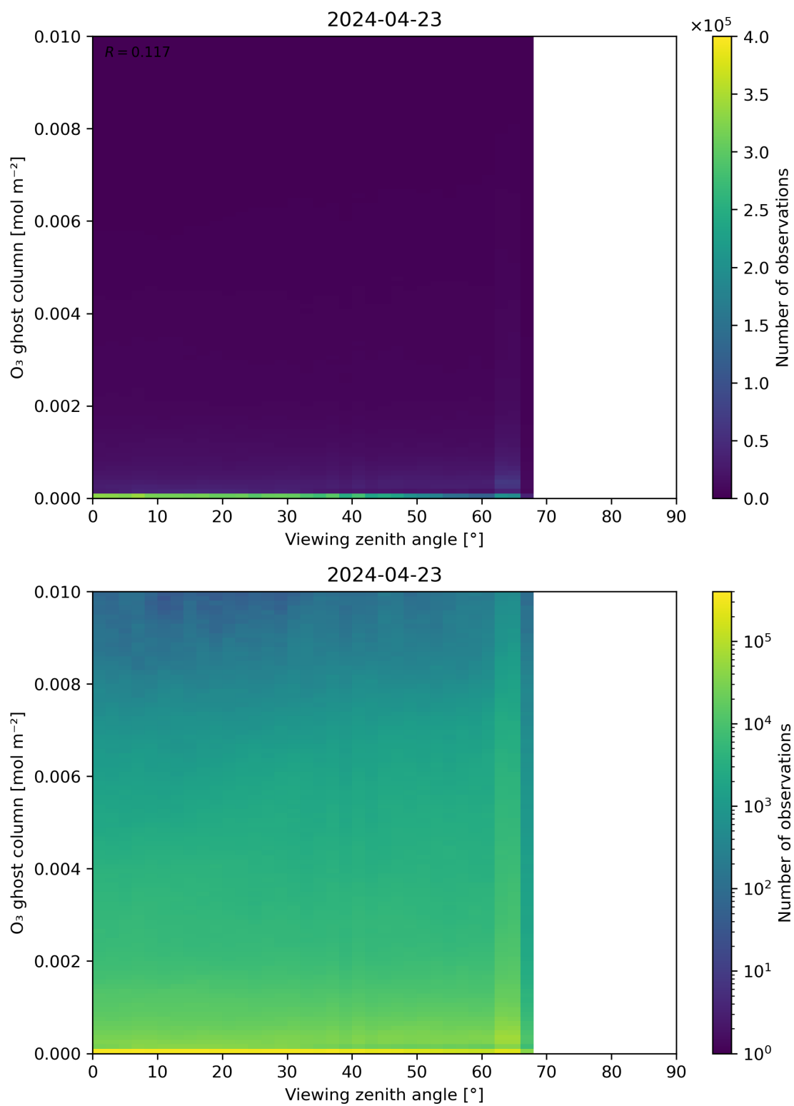
Figure 51: Scatter density plot of “Viewing zenith angle” against “O 3 ghost column” for 2024-04-22 to 2024-04-24.
