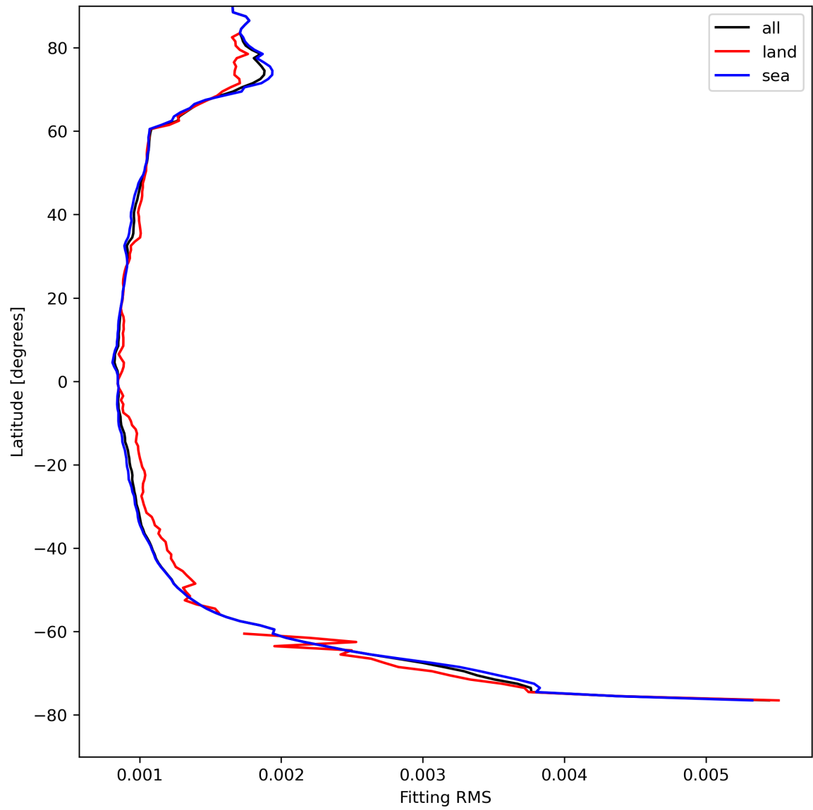
Figure 16: Zonal average of “Fitting RMS” for 2024-04-22 to 2024-04-24.
