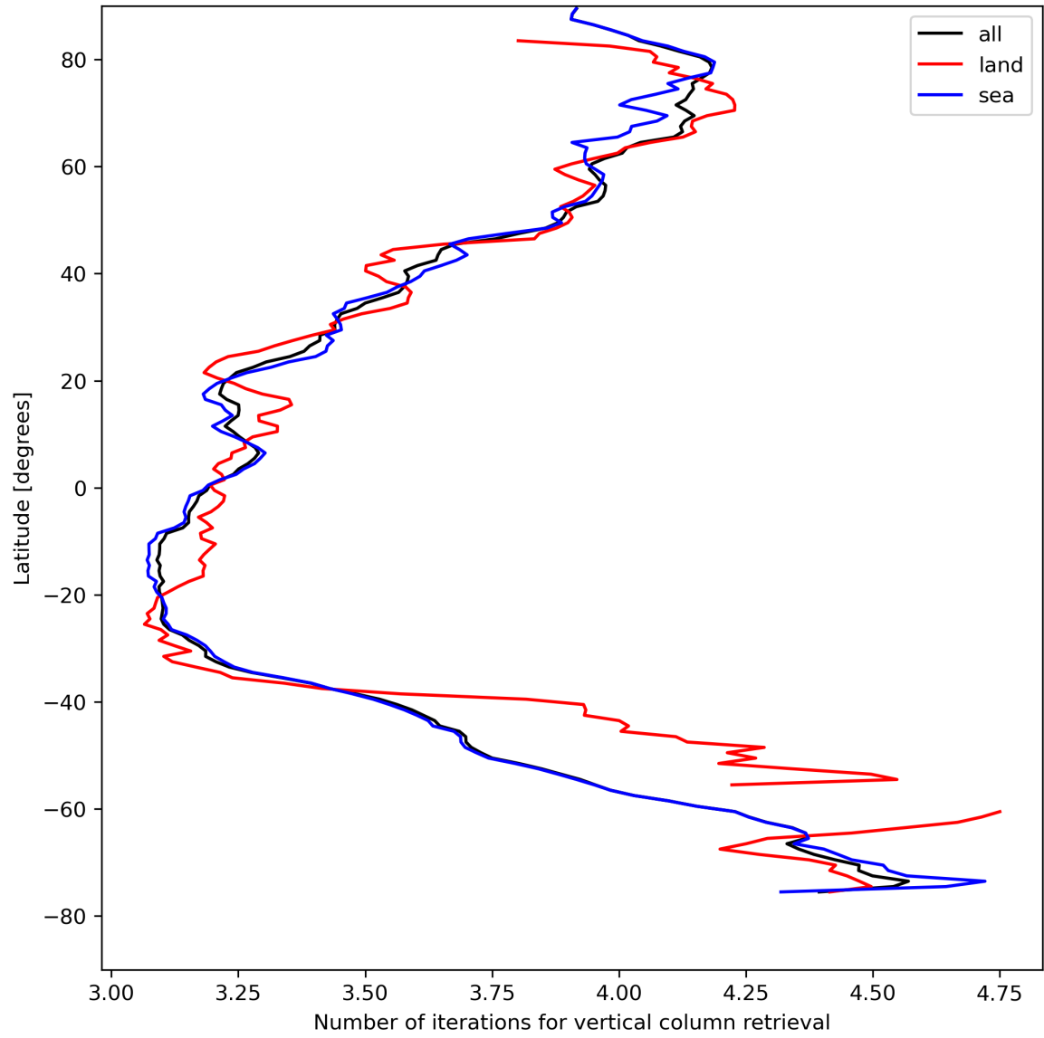
Figure 19: Zonal average of “Number of iterations for vertical column retrieval” for 2024-04-26 to 2024-04-27.
