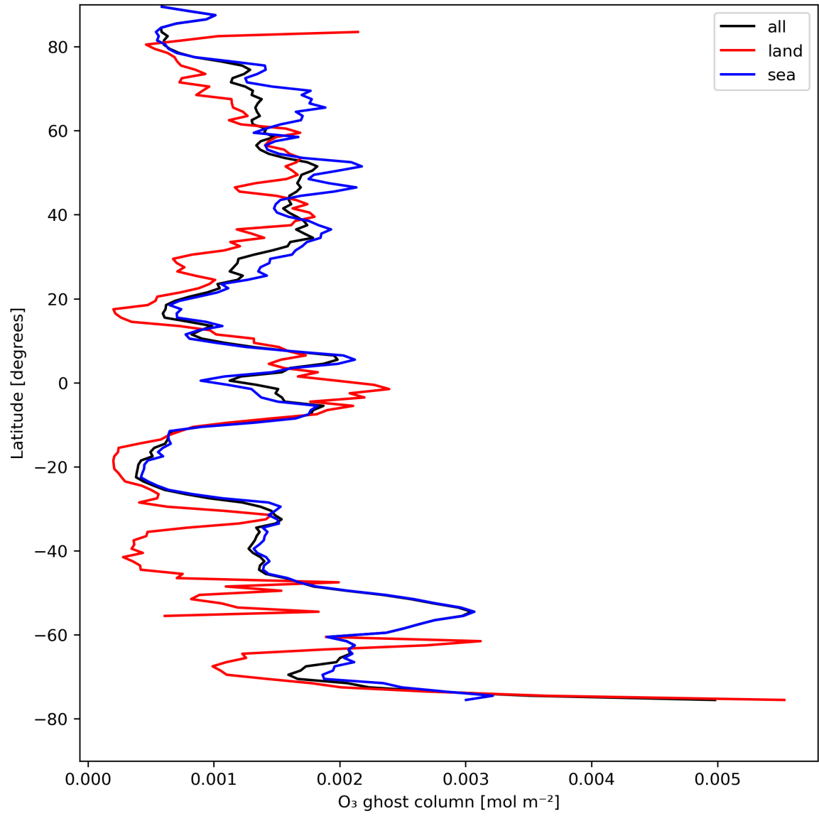
Figure 18: Zonal average of “O 3 ghost column” for 2024-04-26 to 2024-04-27.
