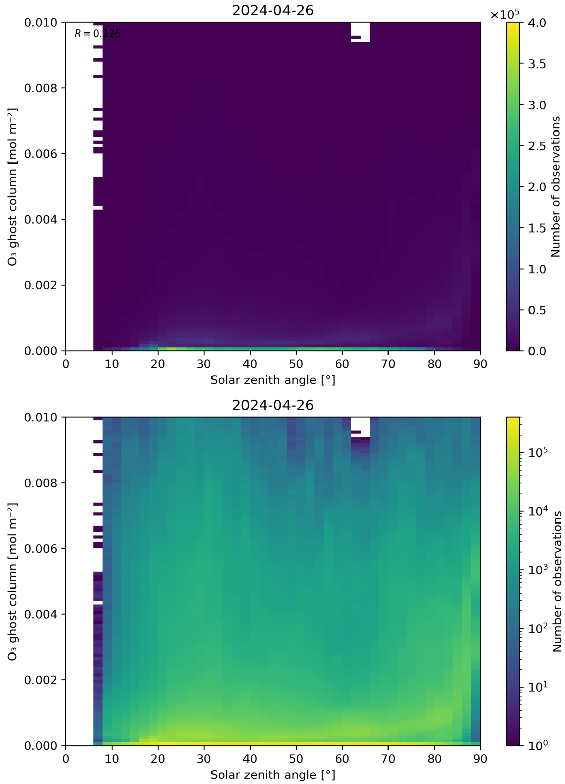
Figure 46: Scatter density plot of “Solar zenith angle” against “O 3 ghost column” for 2024-04-26 to 2024-04-27.
