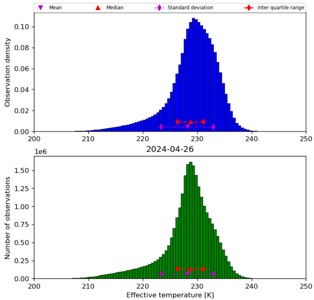
Figure 24: Histogram of “Effective temperature” for 2024-04-26 to 2024-04-27
