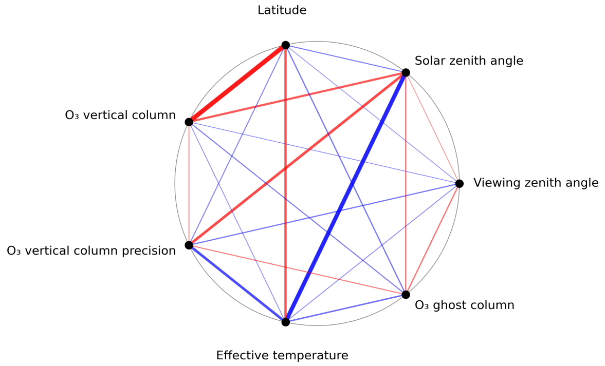
Figure 1: Map of correlation graph for 2024-04-26 to 2024-04-27.
