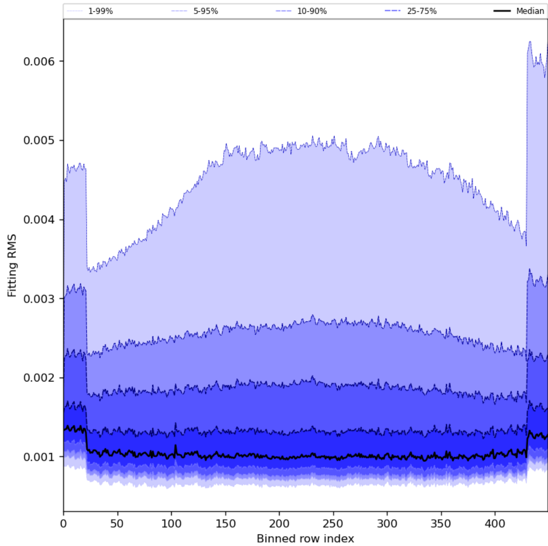
Figure 30: Along track statistics of “Fitting RMS” for 2024-04-26 to 2024-04-27
