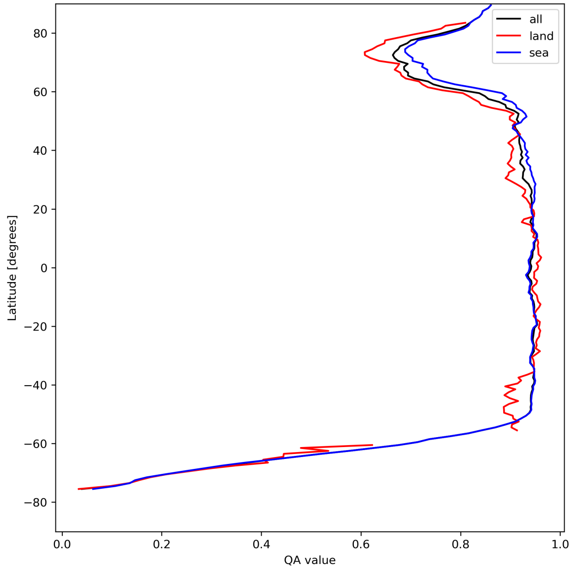
Figure 13: Zonal average of “QA value” for 2024-04-26 to 2024-04-27.
