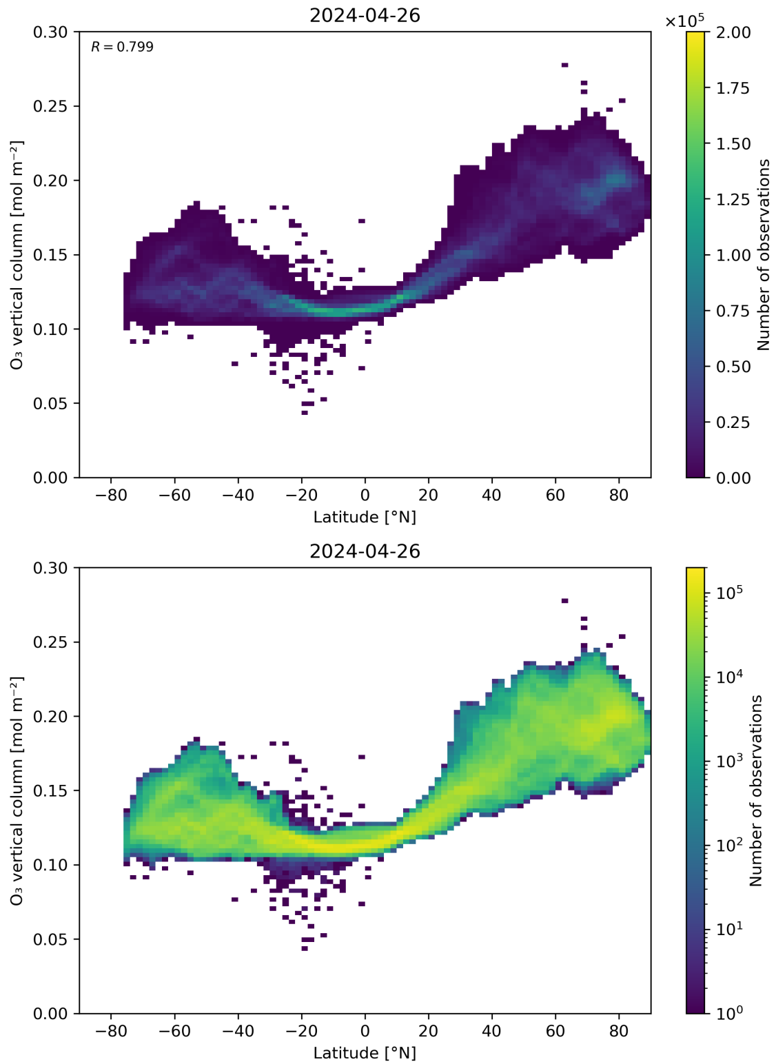
Figure 36: Scatter density plot of “Latitude” against “O 3 vertical column” for 2024-04-26 to 2024-04-27.
