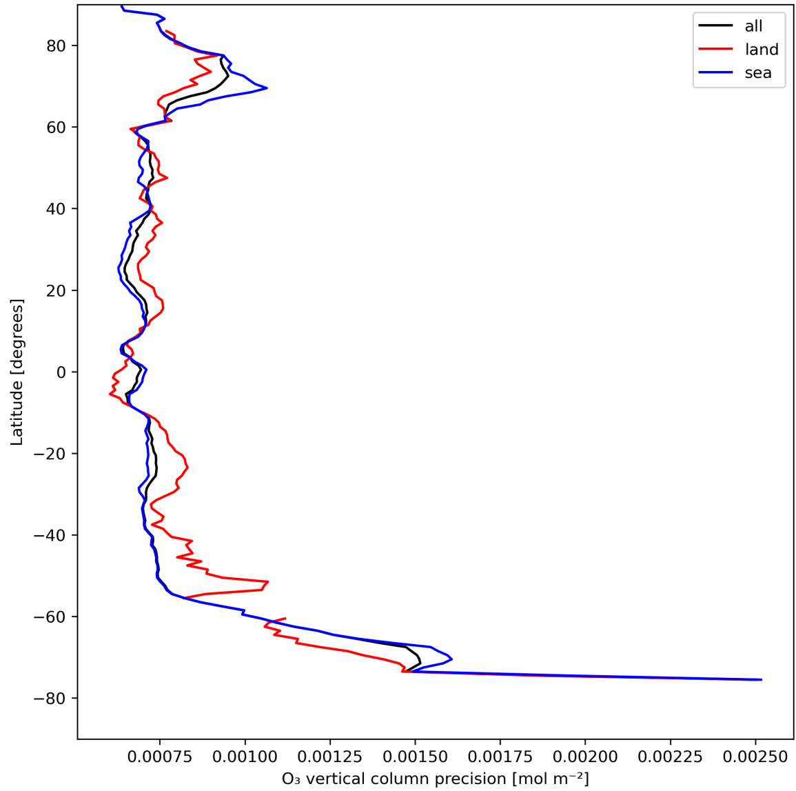
Figure 15: Zonal average of “O 3 vertical column precision” for 2024-04-26 to 2024-04-27.
