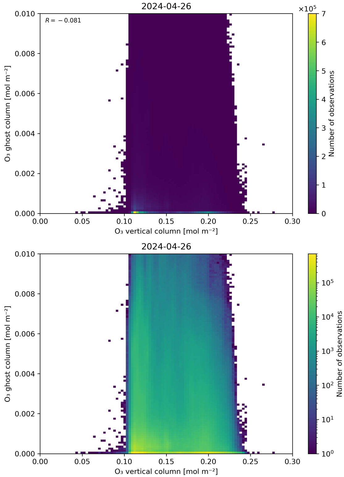
Figure 40: Scatter density plot of “O 3 vertical column” against “O 3 ghost column” for 2024-04-26 to 2024-04-27.
