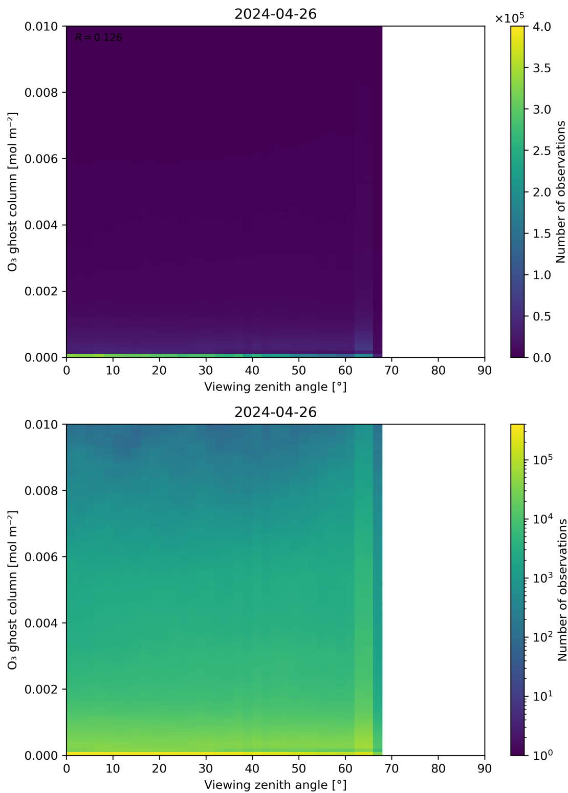
Figure 51: Scatter density plot of “Viewing zenith angle” against “O 3 ghost column” for 2024-04-26 to 2024-04-27.
