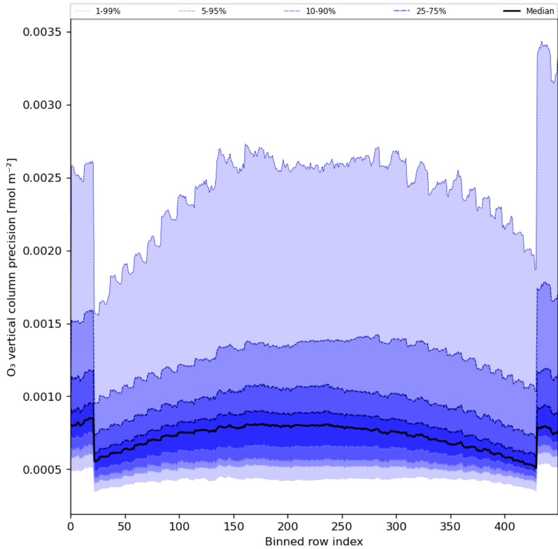
Figure 29: Along track statistics of “O 3 vertical column precision” for 2024-04-26 to 2024-04-27
