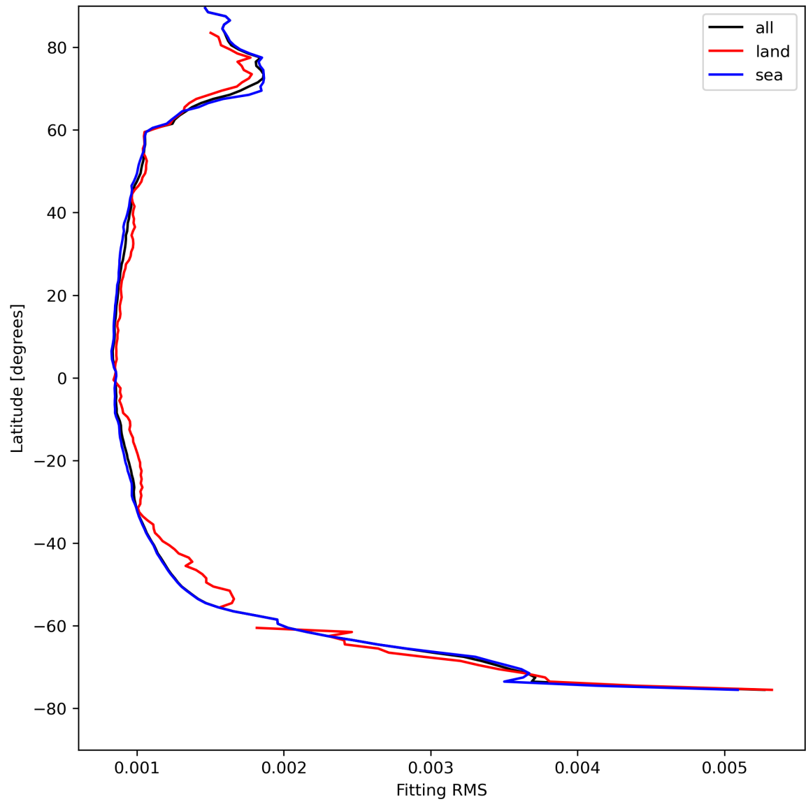
Figure 16: Zonal average of “Fitting RMS” for 2024-04-26 to 2024-04-27.
