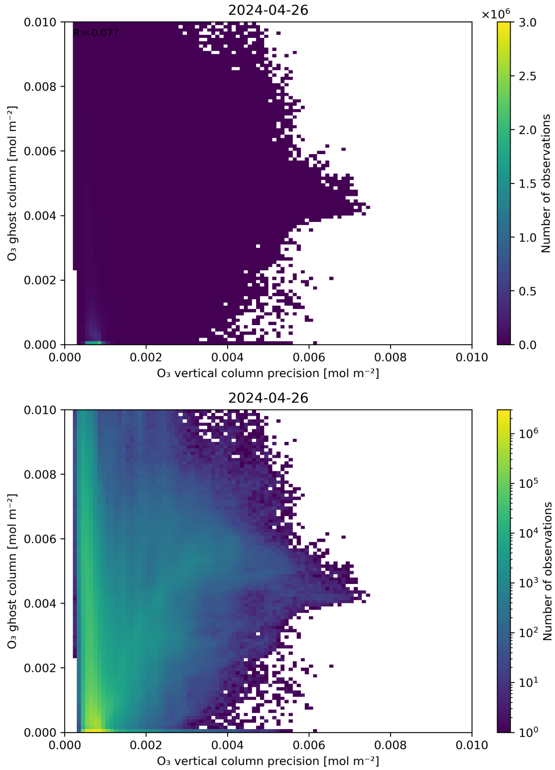
Figure 43: Scatter density plot of “O 3 vertical column precision” against “O 3 ghost column” for 2024-04-26 to 2024-04-27.
