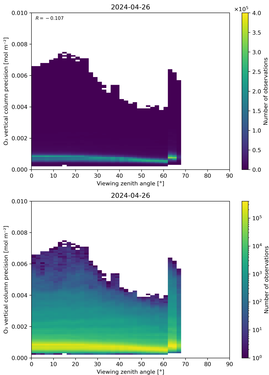
Figure 53: Scatter density plot of “Viewing zenith angle” against “O 3 vertical column precision” for 2024-04-26 to 2024-04-27.
