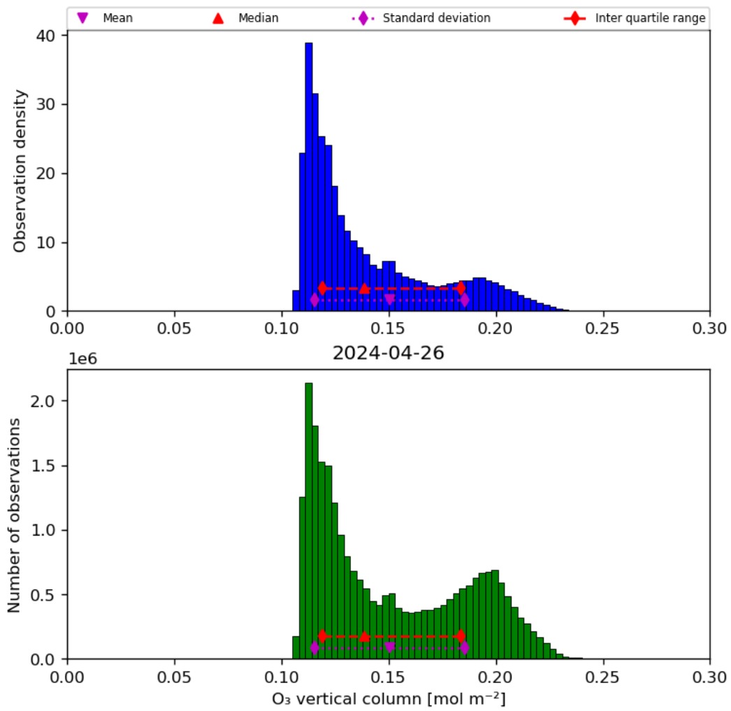
Figure 21: Histogram of “O 3 vertical column” for 2024-04-26 to 2024-04-27
