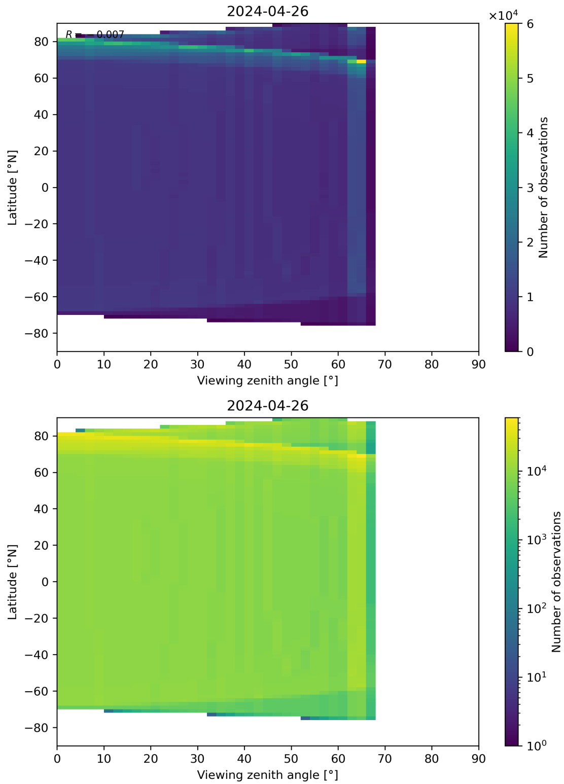
Figure 49: Scatter density plot of “Viewing zenith angle” against “Latitude” for 2024-04-26 to 2024-04-27.
