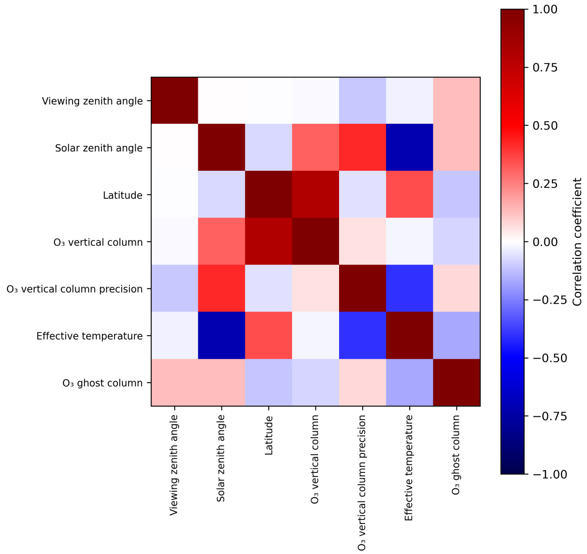
Figure 2: Map of correlation matrix for 2024-04-26 to 2024-04-27.
