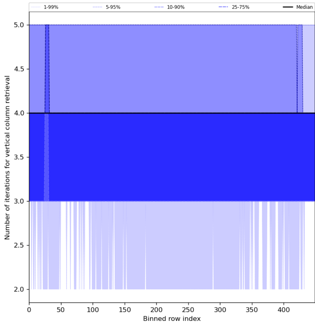
Figure 33: Along track statistics of “Number of iterations for vertical column retrieval” for 2024-04-26 to 2024-04-27
