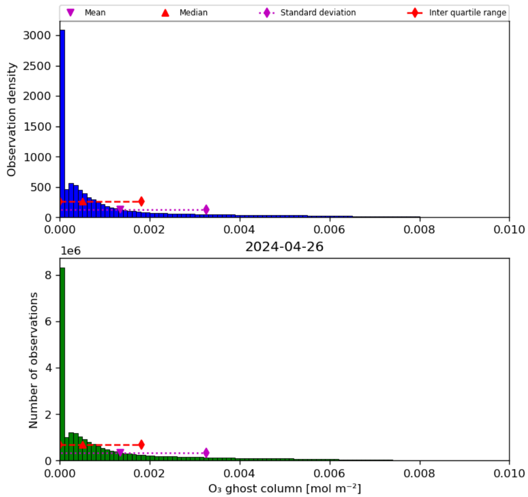
Figure 25: Histogram of “O 3 ghost column” for 2024-04-26 to 2024-04-27
