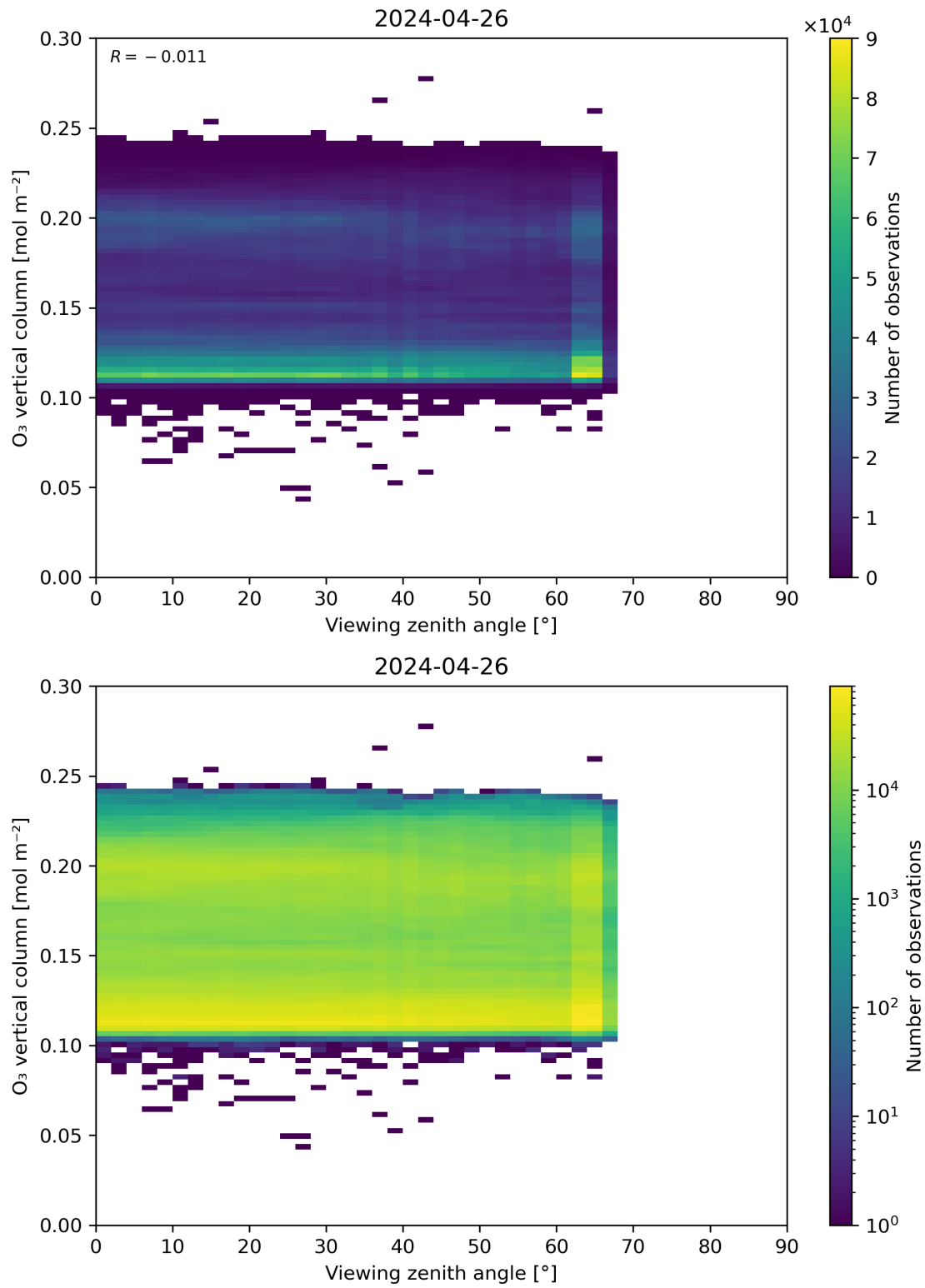
Figure 52: Scatter density plot of “Viewing zenith angle” against “O 3 vertical column” for 2024-04-26 to 2024-04-27.
