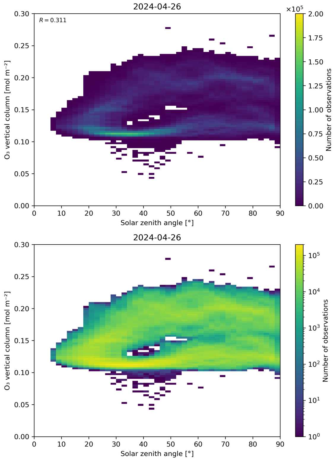
Figure 47: Scatter density plot of “Solar zenith angle” against “O 3 vertical column” for 2024-04-26 to 2024-04-27.
