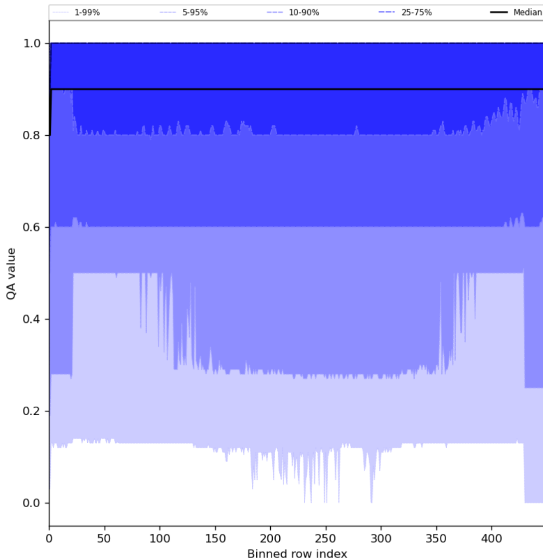
Figure 27: Along track statistics of “QA value” for 2024-04-26 to 2024-04-27
