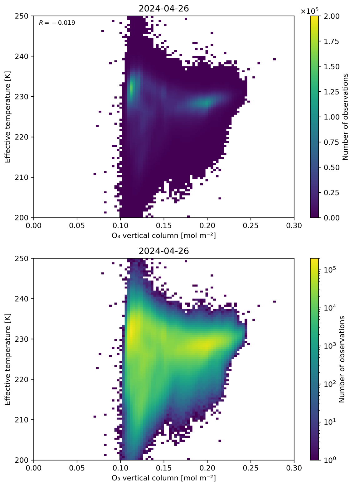
Figure 39: Scatter density plot of “O 3 vertical column” against “Effective temperature” for 2024-04-26 to 2024-04-27.
