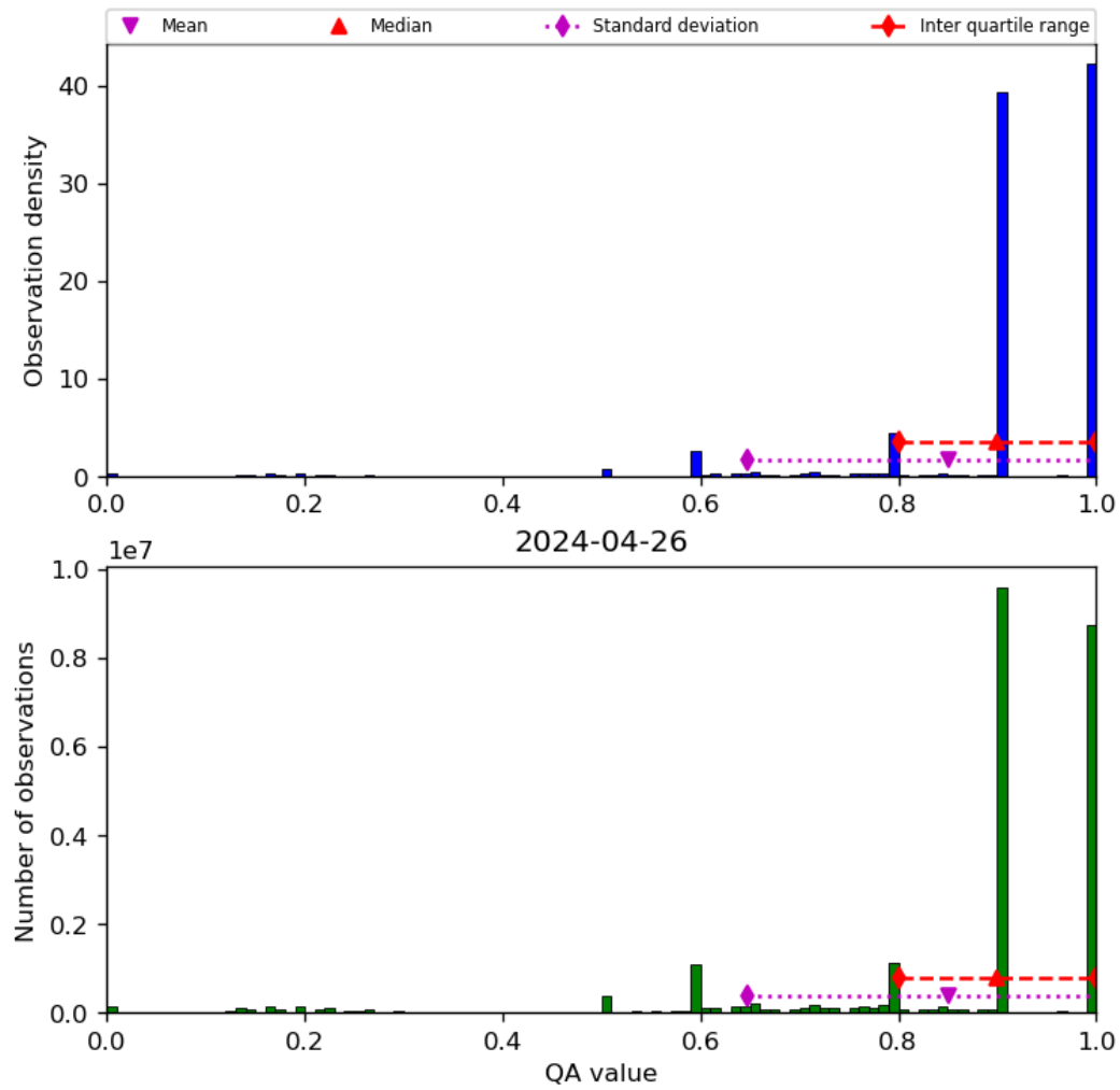
Figure 20: Histogram of “QA value” for 2024-04-26 to 2024-04-27
