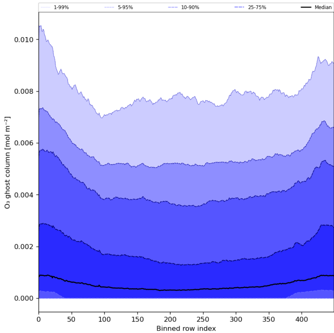
Figure 32: Along track statistics of “O 3 ghost column” for 2024-04-26 to 2024-04-27
