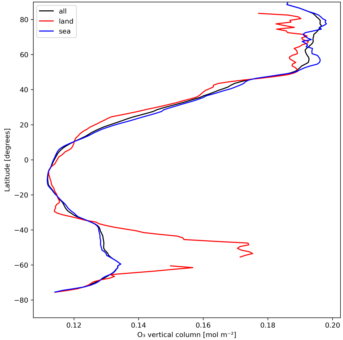
Figure 14: Zonal average of “O 3 vertical column” for 2024-04-26 to 2024-04-27.
