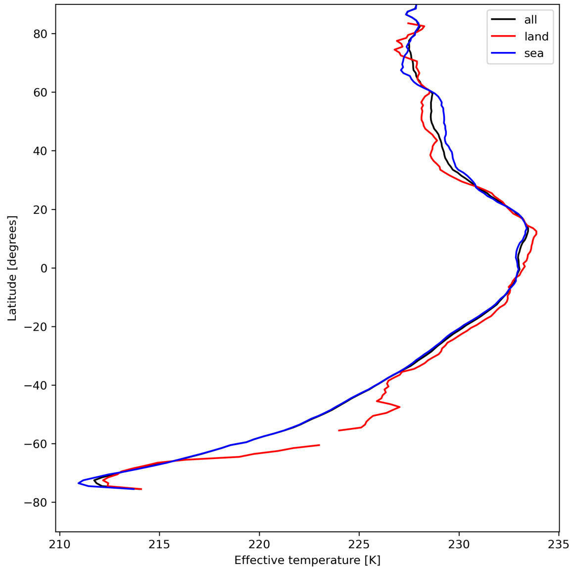
Figure 17: Zonal average of “Effective temperature” for 2024-04-26 to 2024-04-27.
