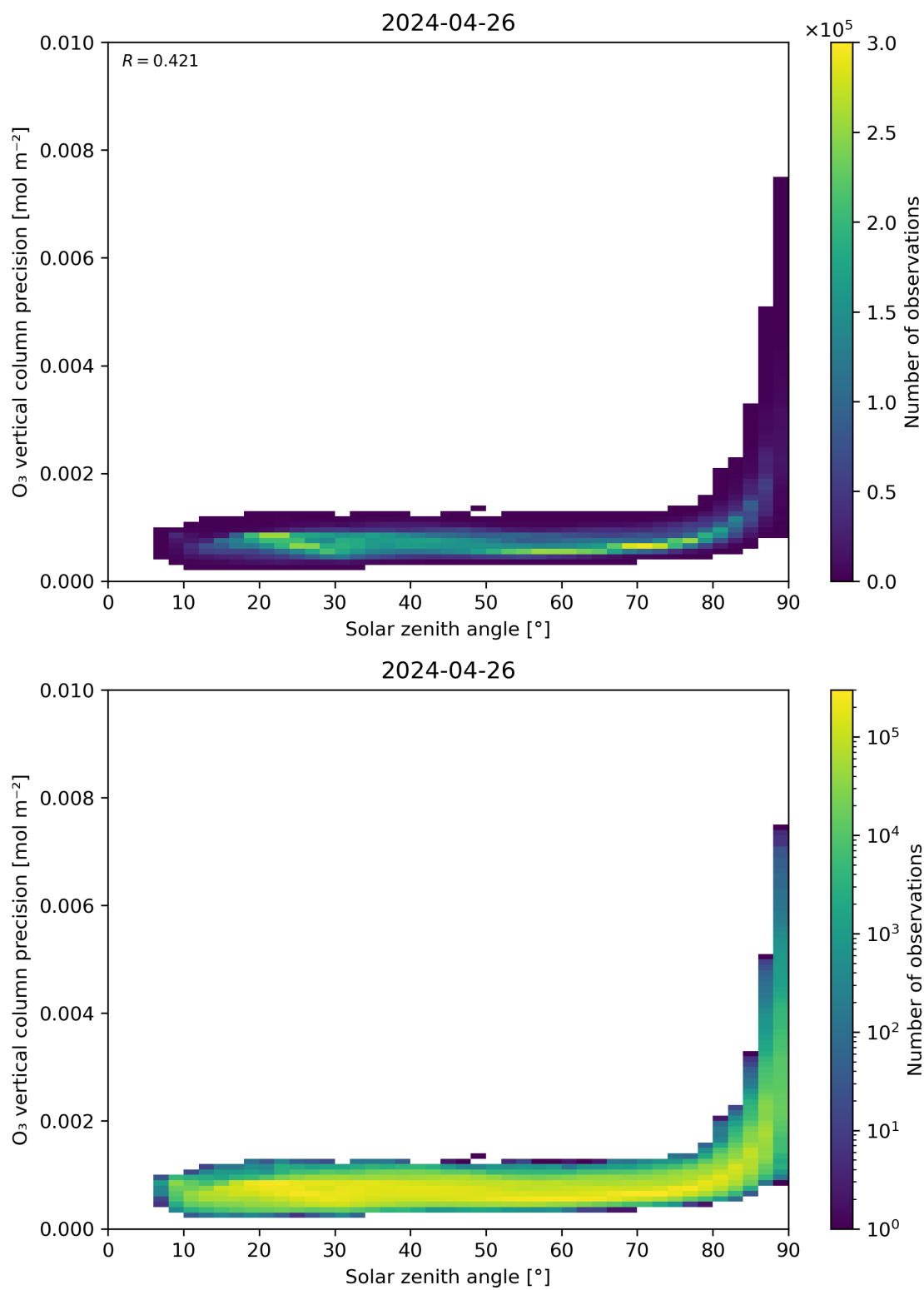
Figure 48: Scatter density plot of “Solar zenith angle” against “O 3 vertical column precision” for 2024-04-26 to 2024-04-27.
