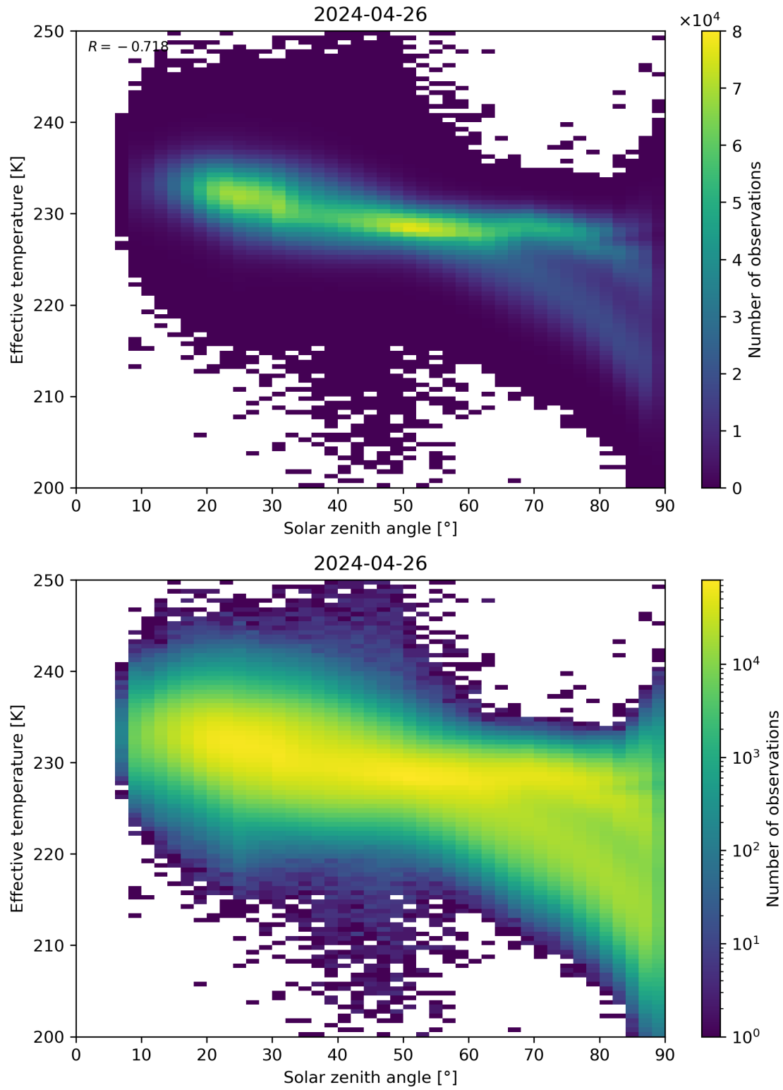
Figure 45: Scatter density plot of “Solar zenith angle” against “Effective temperature” for 2024-04-26 to 2024-04-27.
