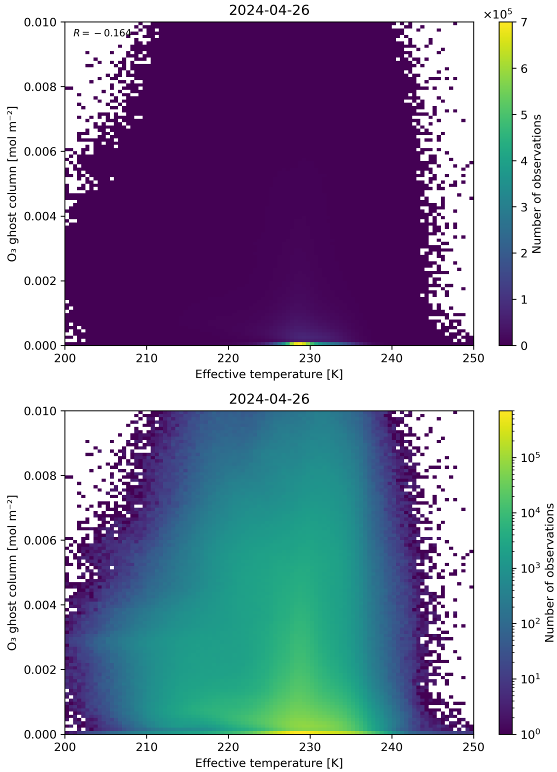
Figure 38: Scatter density plot of “Effective temperature” against “O 3 ghost column” for 2024-04-26 to 2024-04-27.
