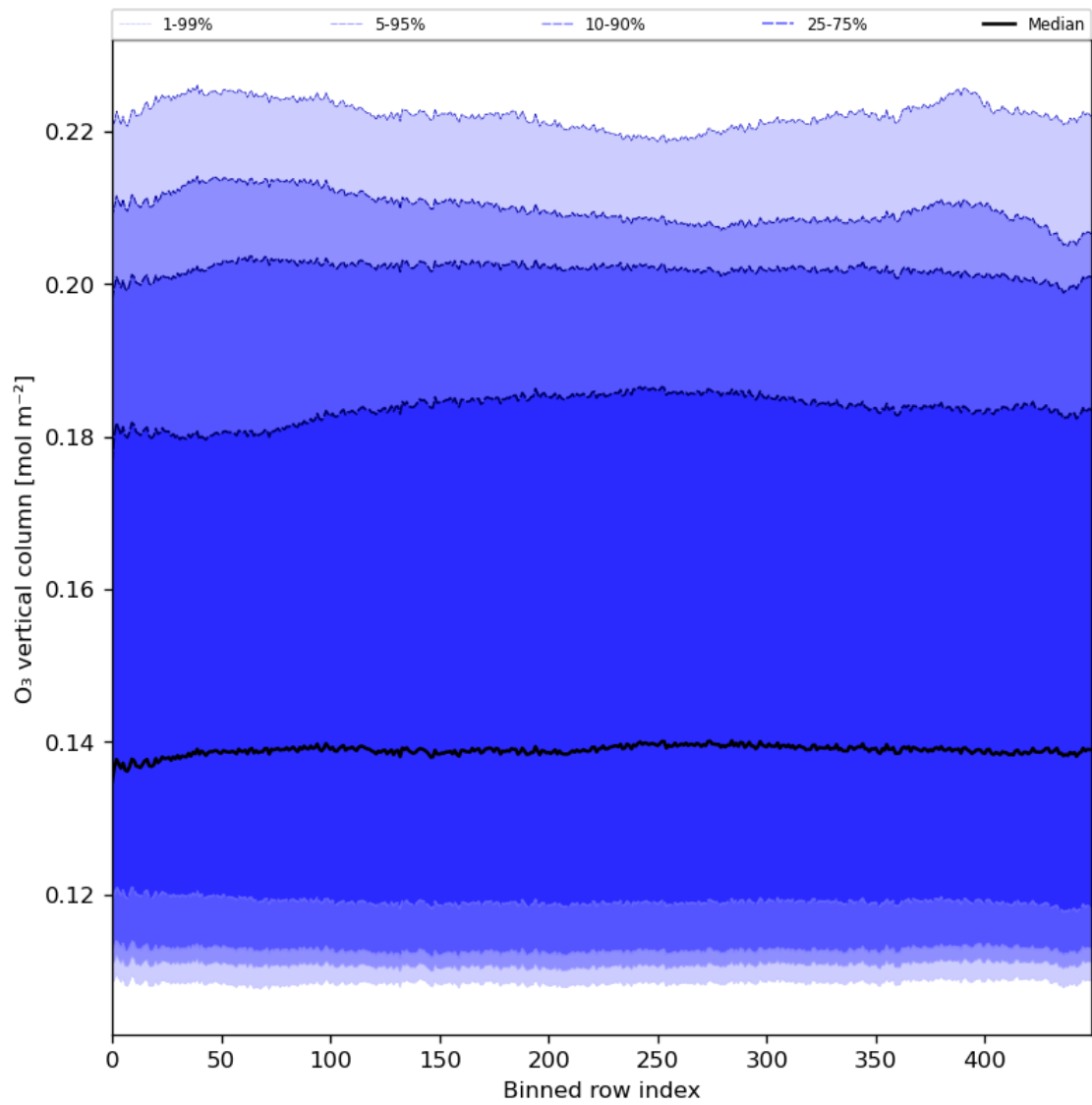
Figure 28: Along track statistics of “ O_3 vertical column” for 2024-04-26 to 2024-04-27
