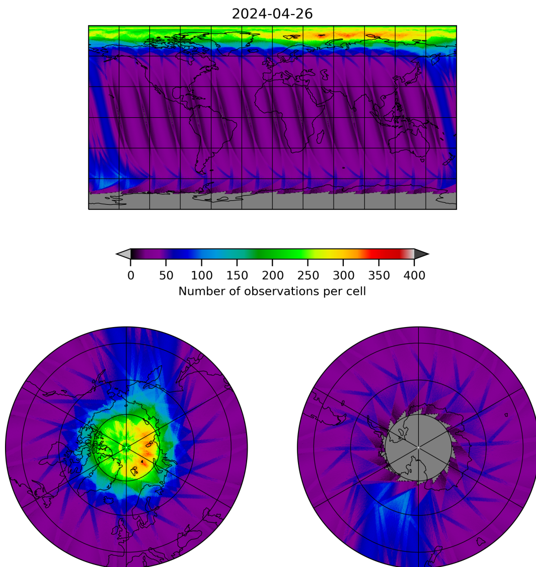
Figure 12: Map of the number of observations for 2024-04-26 to 2024-04-27
