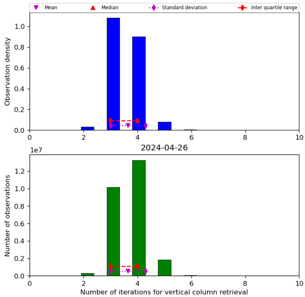
Figure 26: Histogram of “Number of iterations for vertical column retrieval” for 2024-04-26 to 2024-04-27
