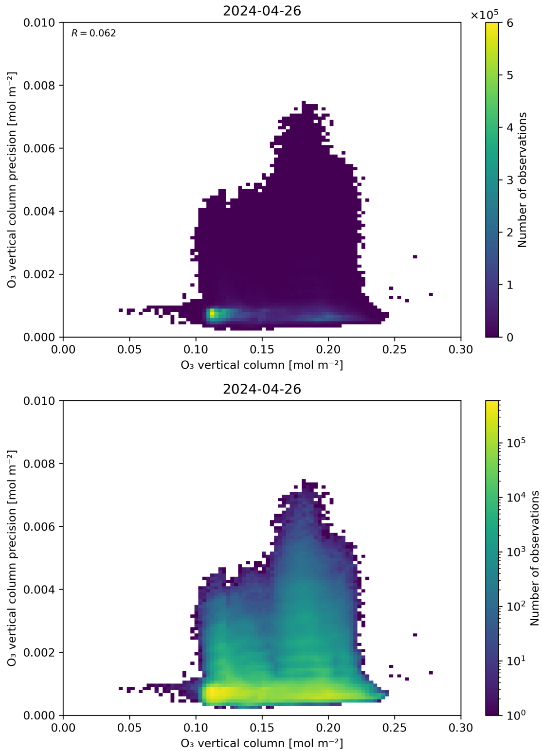
Figure 41: Scatter density plot of “O 3 vertical column” against “O 3 vertical column precision” for 2024-04-26 to 2024-04-27.
