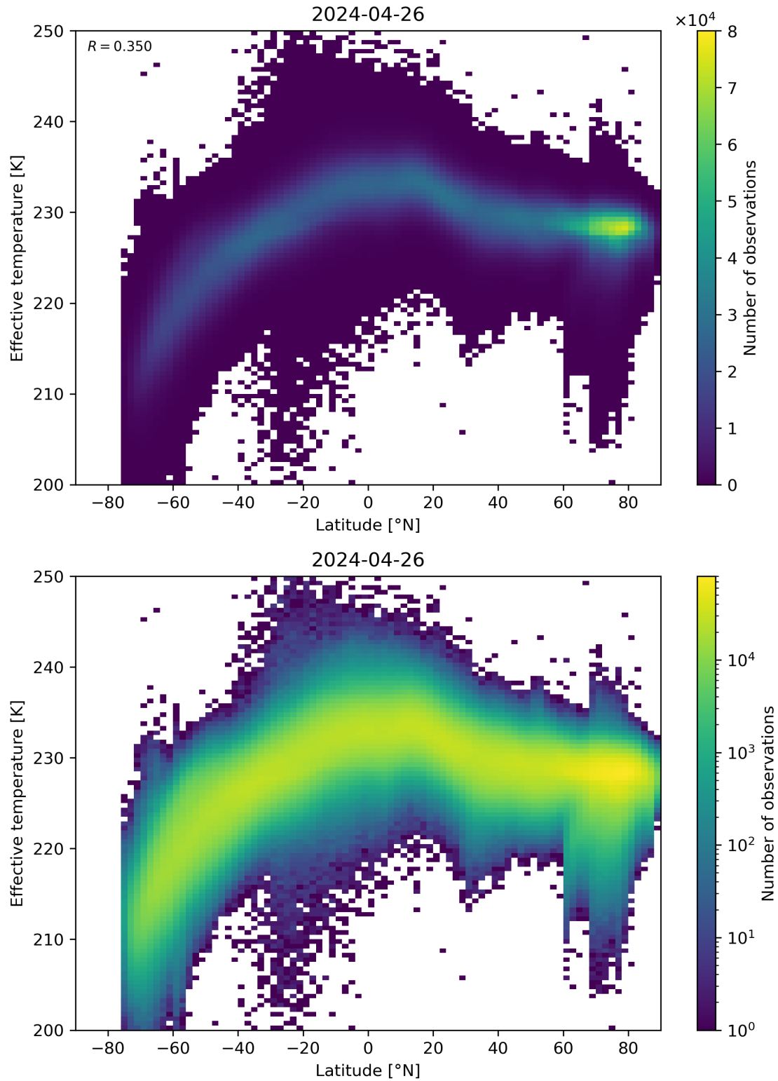
Figure 34: Scatter density plot of “Latitude” against “Effective temperature” for 2024-04-26 to 2024-04-27.
