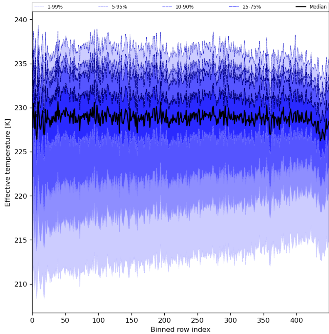
Figure 31: Along track statistics of “Effective temperature” for 2024-04-26 to 2024-04-27
