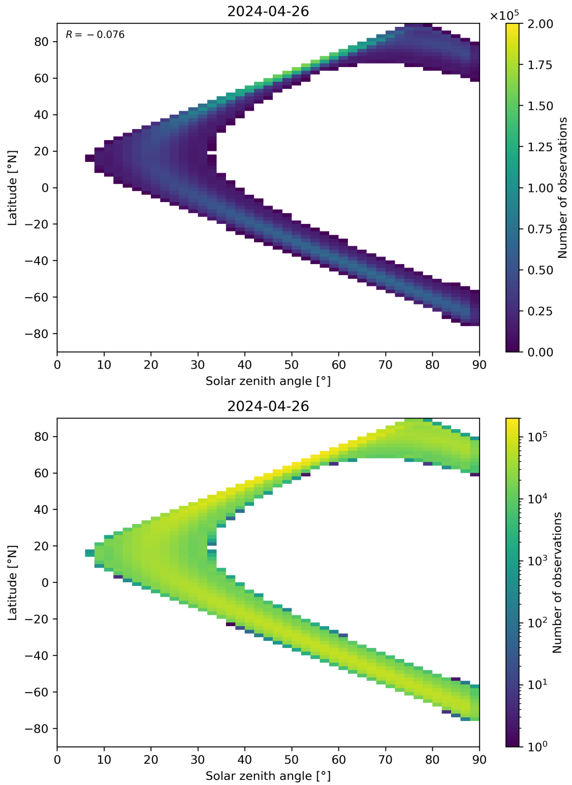
Figure 44: Scatter density plot of “Solar zenith angle” against “Latitude” for 2024-04-26 to 2024-04-27.
