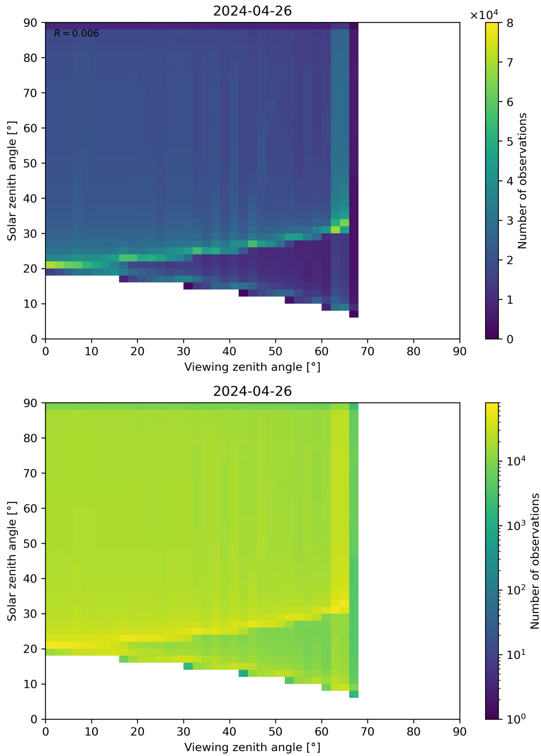
Figure 54: Scatter density plot of “Viewing zenith angle” against “Solar zenith angle” for 2024-04-26 to 2024-04-27.
