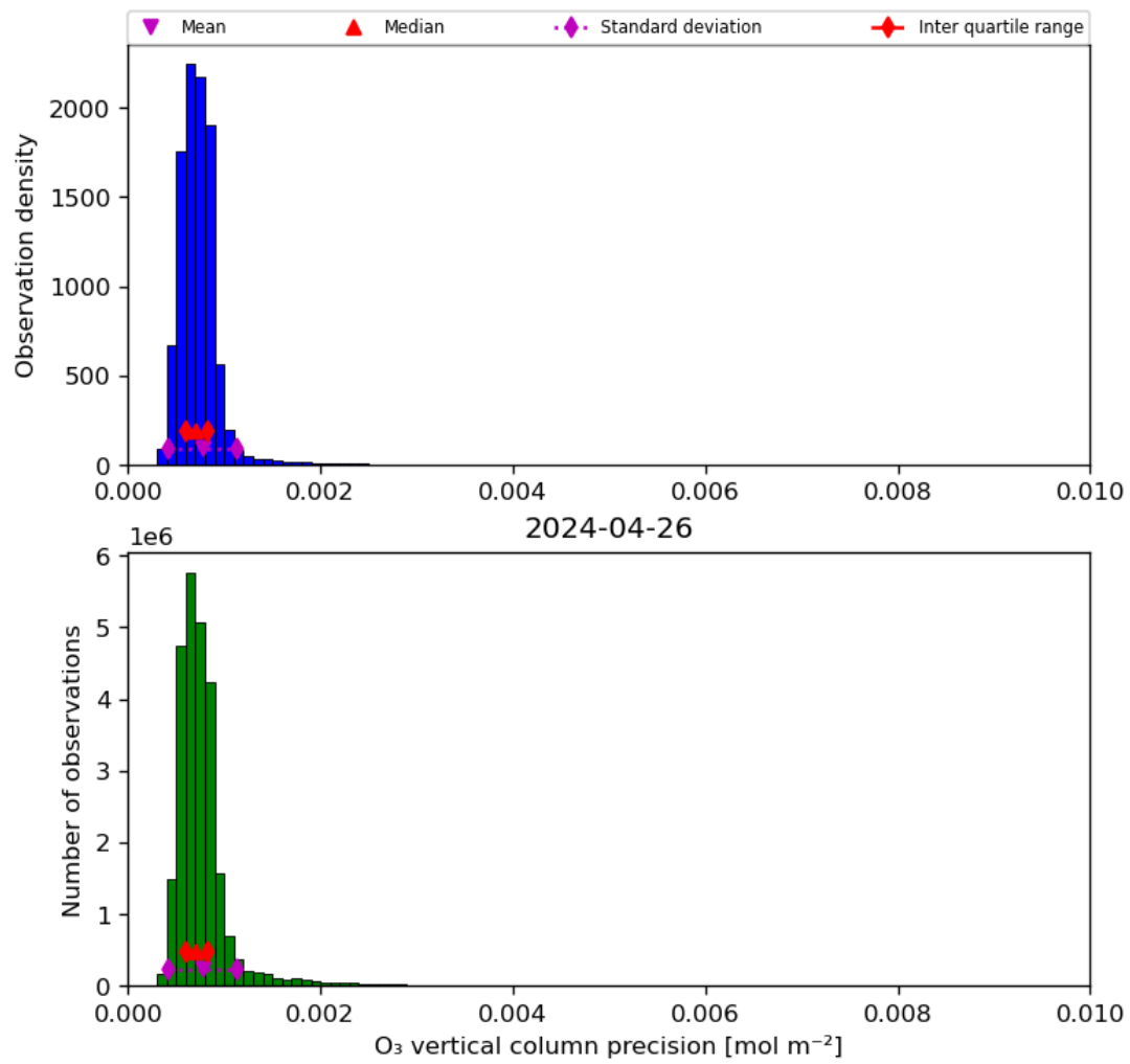
Figure 22: Histogram of “O 3 vertical column precision” for 2024-04-26 to 2024-04-27
