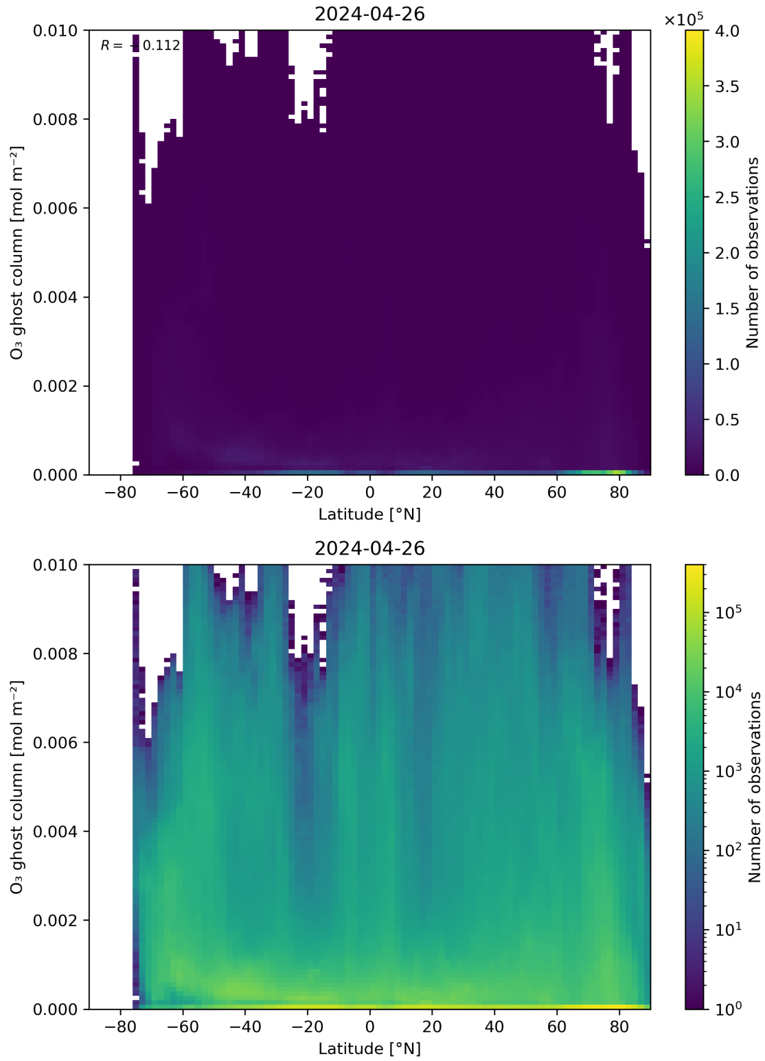
Figure 35: Scatter density plot of “Latitude” against “O 3 ghost column” for 2024-04-26 to 2024-04-27.
