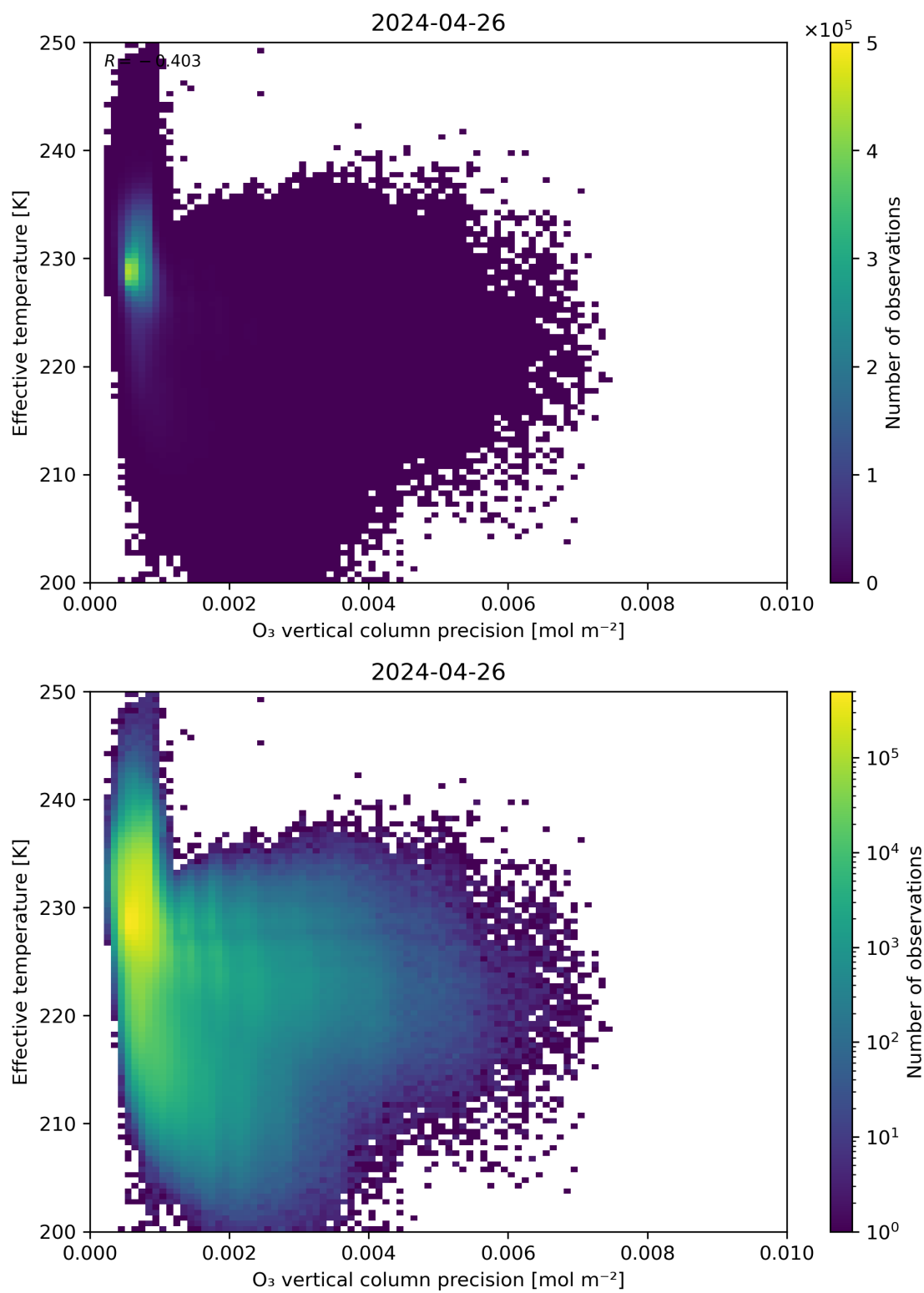
Figure 42: Scatter density plot of “O 3 vertical column precision” against “Effective temperature” for 2024-04-26 to 2024-04-27.
