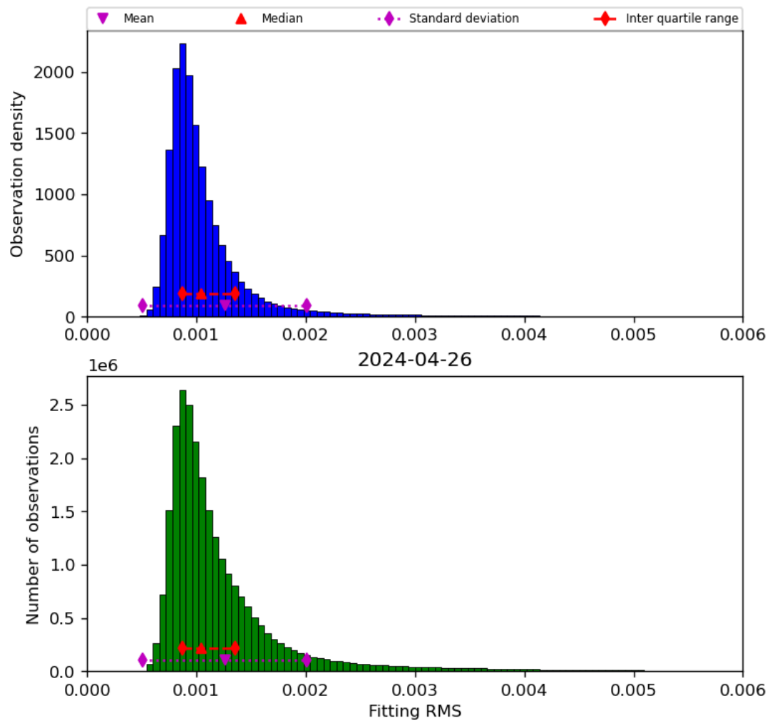
Figure 23: Histogram of “Fitting RMS” for 2024-04-26 to 2024-04-27
