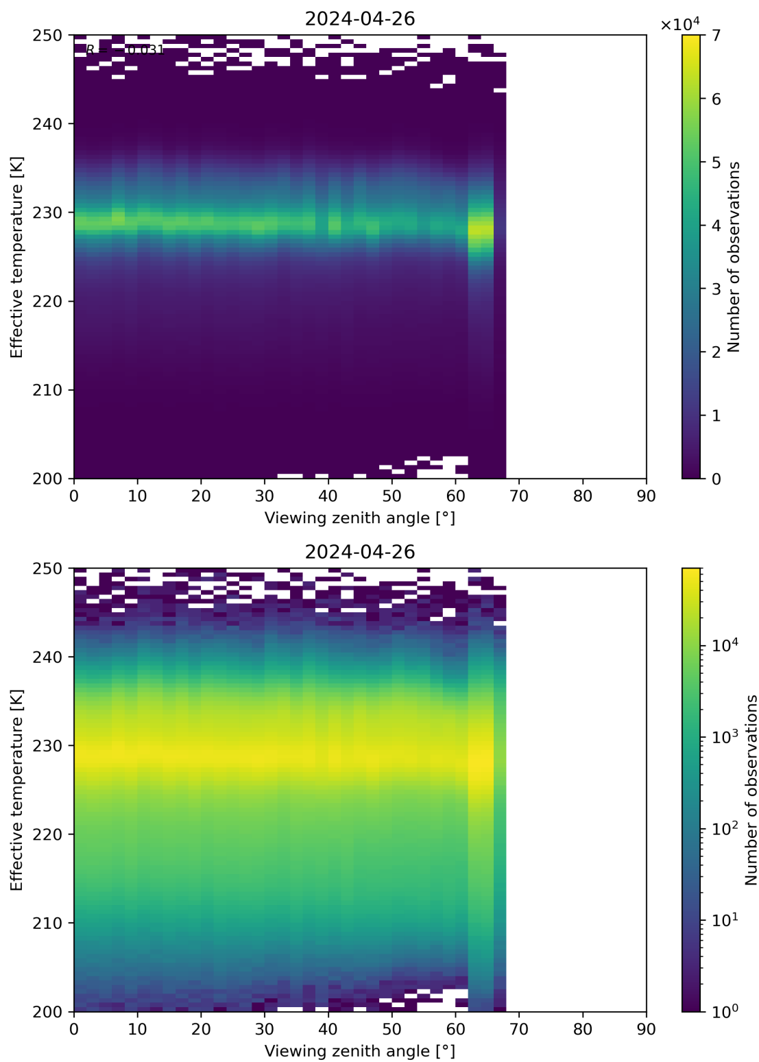
Figure 50: Scatter density plot of “Viewing zenith angle” against “Effective temperature” for 2024-04-26 to 2024-04-27.
