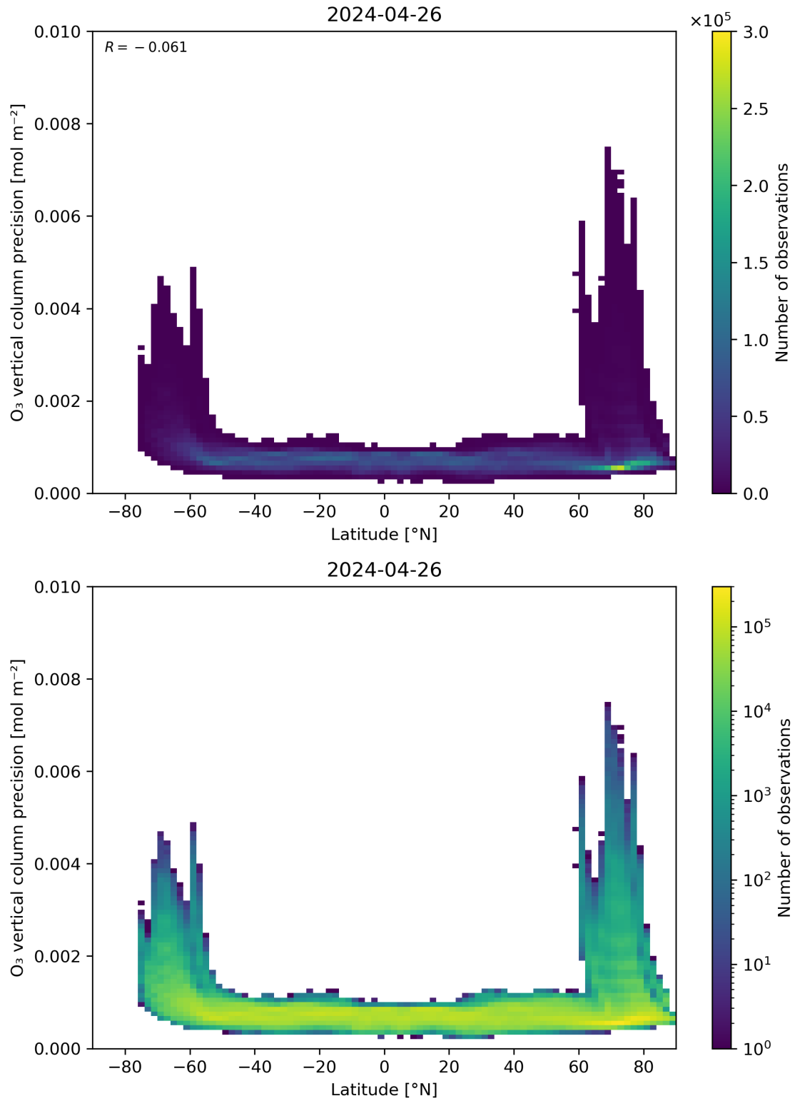
Figure 37: Scatter density plot of “Latitude” against “O 3 vertical column precision” for 2024-04-26 to 2024-04-27.
