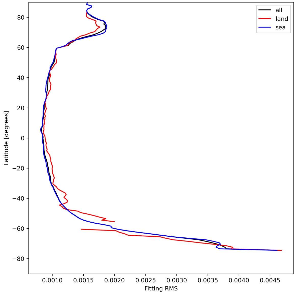
Figure 16: Zonal average of “Fitting RMS” for 2024-04-26 to 2024-04-28.
