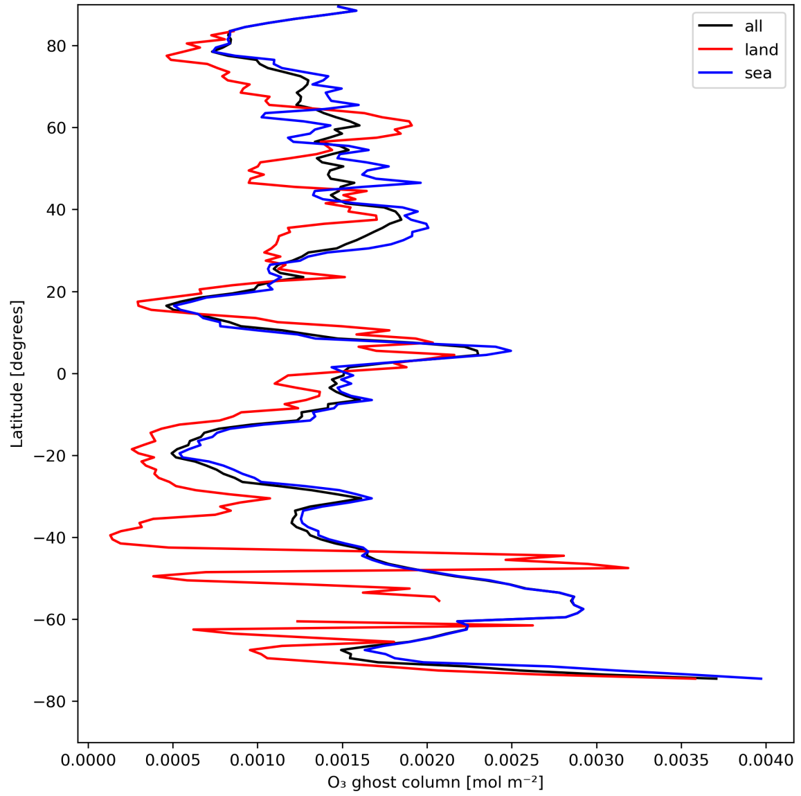
Figure 18: Zonal average of “O 3 ghost column” for 2024-04-26 to 2024-04-28.
