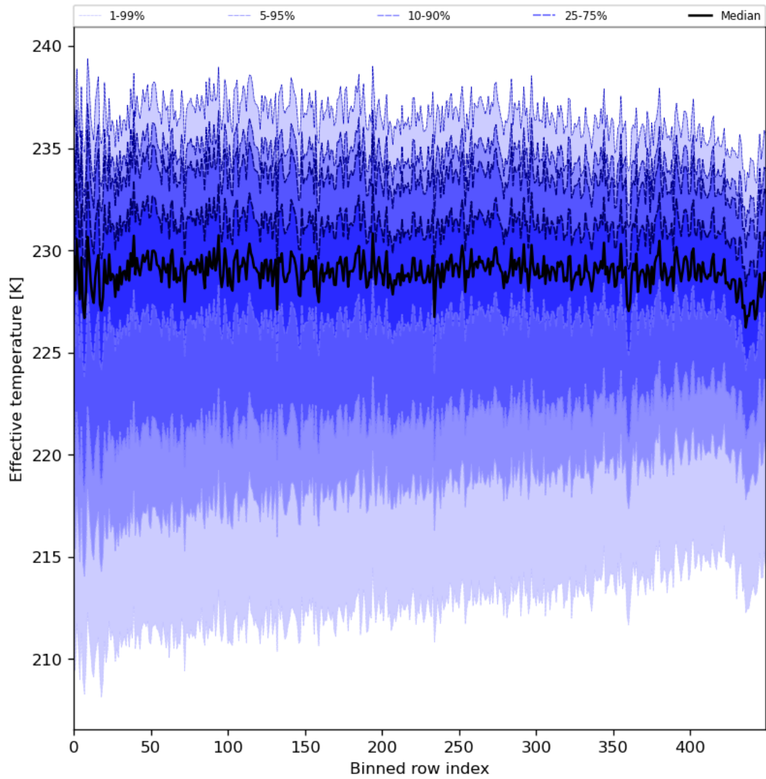
Figure 31: Along track statistics of “Effective temperature” for 2024-04-26 to 2024-04-28
