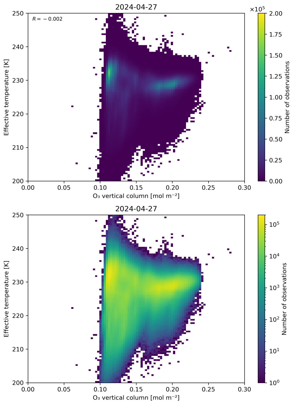
Figure 39: Scatter density plot of “O 3 vertical column” against “Effective temperature” for 2024-04-26 to 2024-04-28.
