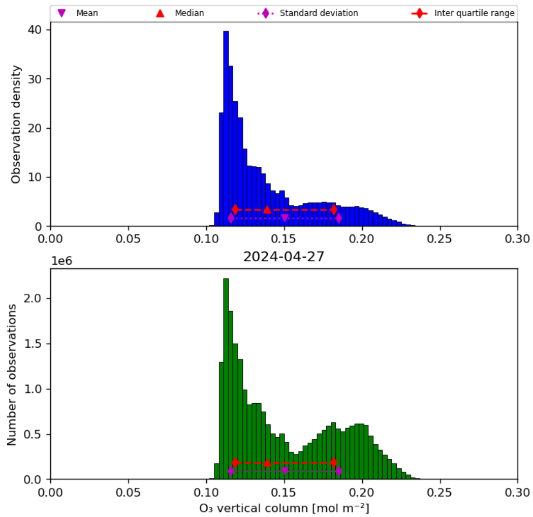
Figure 21: Histogram of “O 3 vertical column” for 2024-04-26 to 2024-04-28
