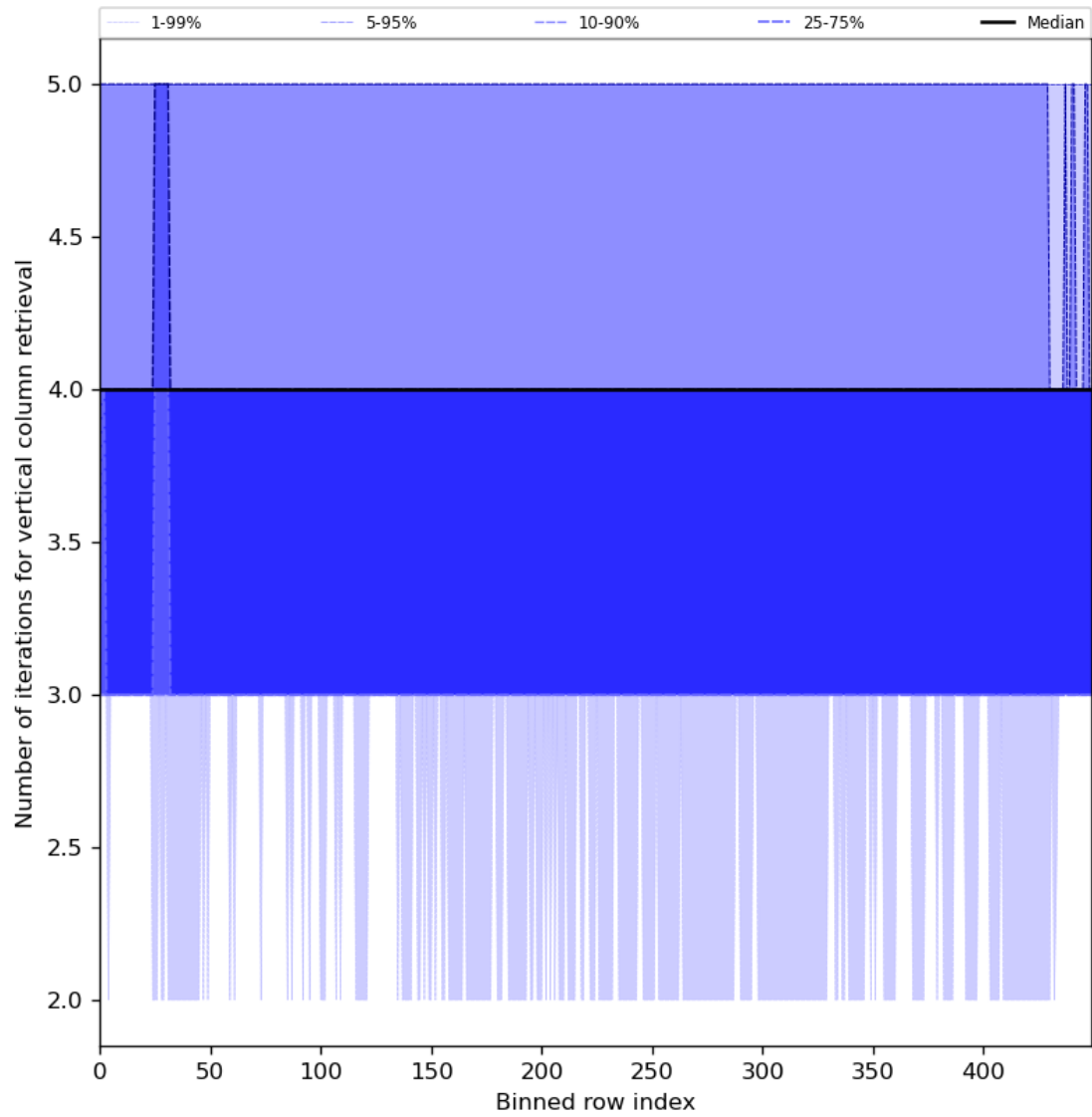
Figure 33: Along track statistics of “Number of iterations for vertical column retrieval” for 2024-04-26 to 2024-04-28
