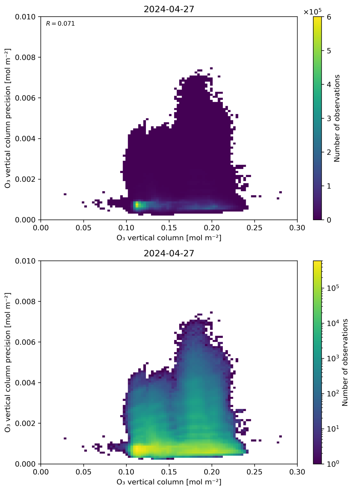
Figure 41: Scatter density plot of “O 3 vertical column” against “O 3 vertical column precision” for 2024-04-26 to 2024-04-28.
