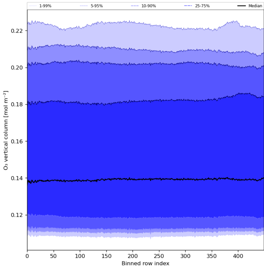
Figure 28: Along track statistics of “O 3 vertical column” for 2024-04-26 to 2024-04-28
