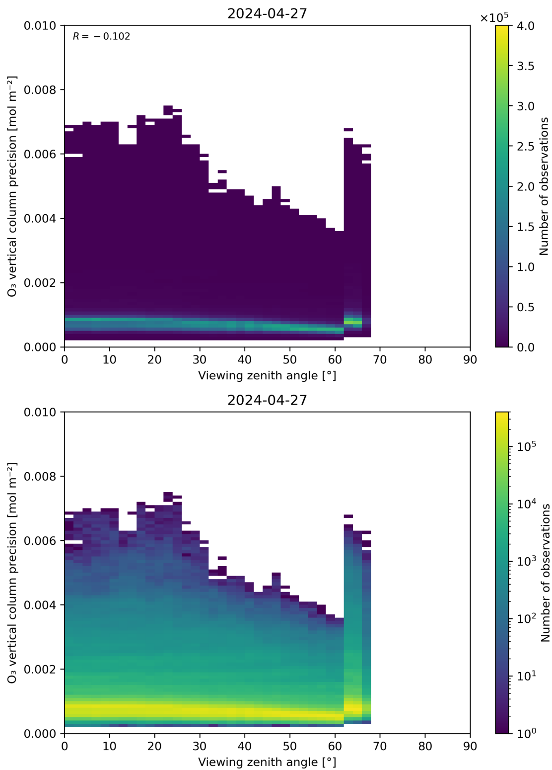
Figure 53: Scatter density plot of “Viewing zenith angle” against “O 3 vertical column precision” for 2024-04-26 to 2024-04-28.
