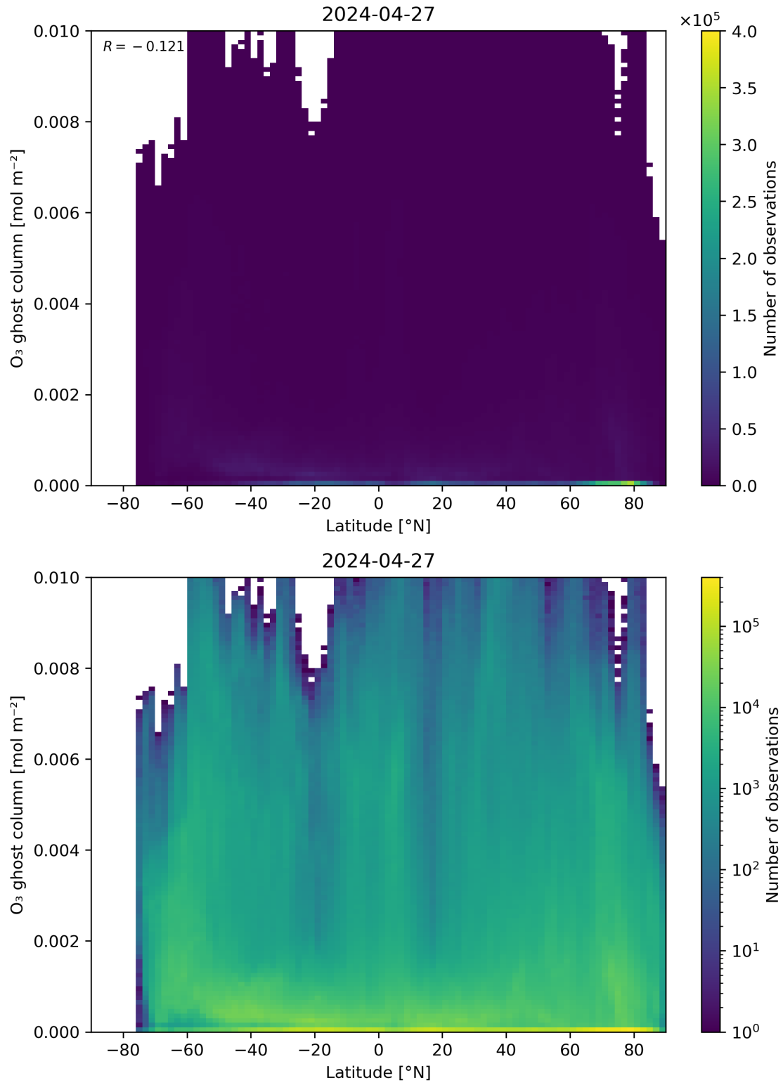
Figure 35: Scatter density plot of “Latitude” against “O 3 ghost column” for 2024-04-26 to 2024-04-28.
