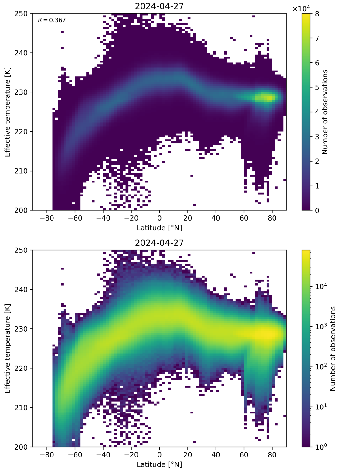
Figure 34: Scatter density plot of “Latitude” against “Effective temperature” for 2024-04-26 to 2024-04-28.
