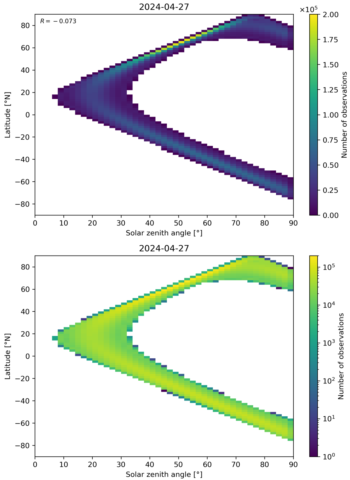
Figure 44: Scatter density plot of “Solar zenith angle” against “Latitude” for 2024-04-26 to 2024-04-28.
