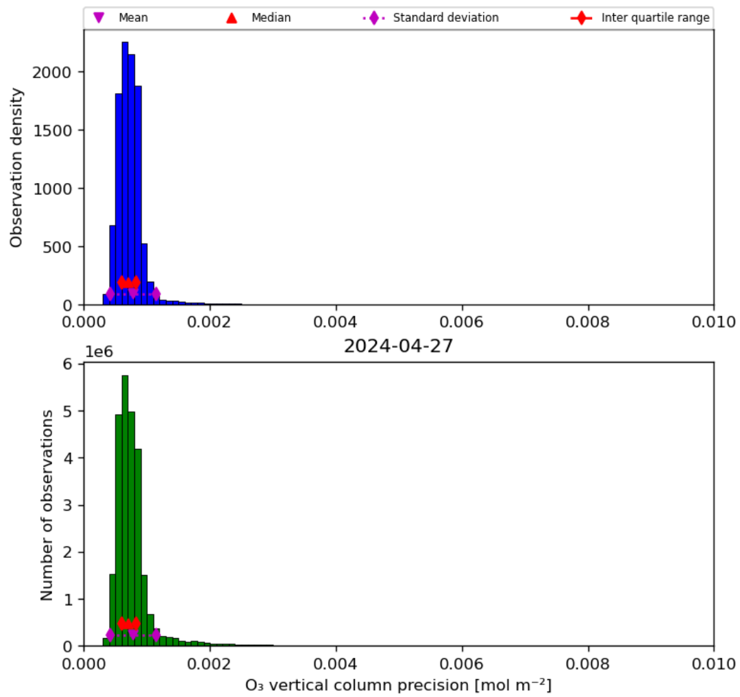
Figure 22: Histogram of “O 3 vertical column precision” for 2024-04-26 to 2024-04-28
