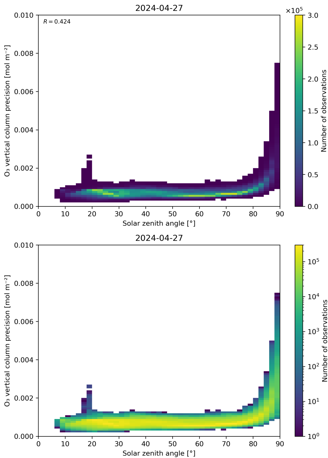
Figure 48: Scatter density plot of “Solar zenith angle” against “O 3 vertical column precision” for 2024-04-26 to 2024-04-28.
