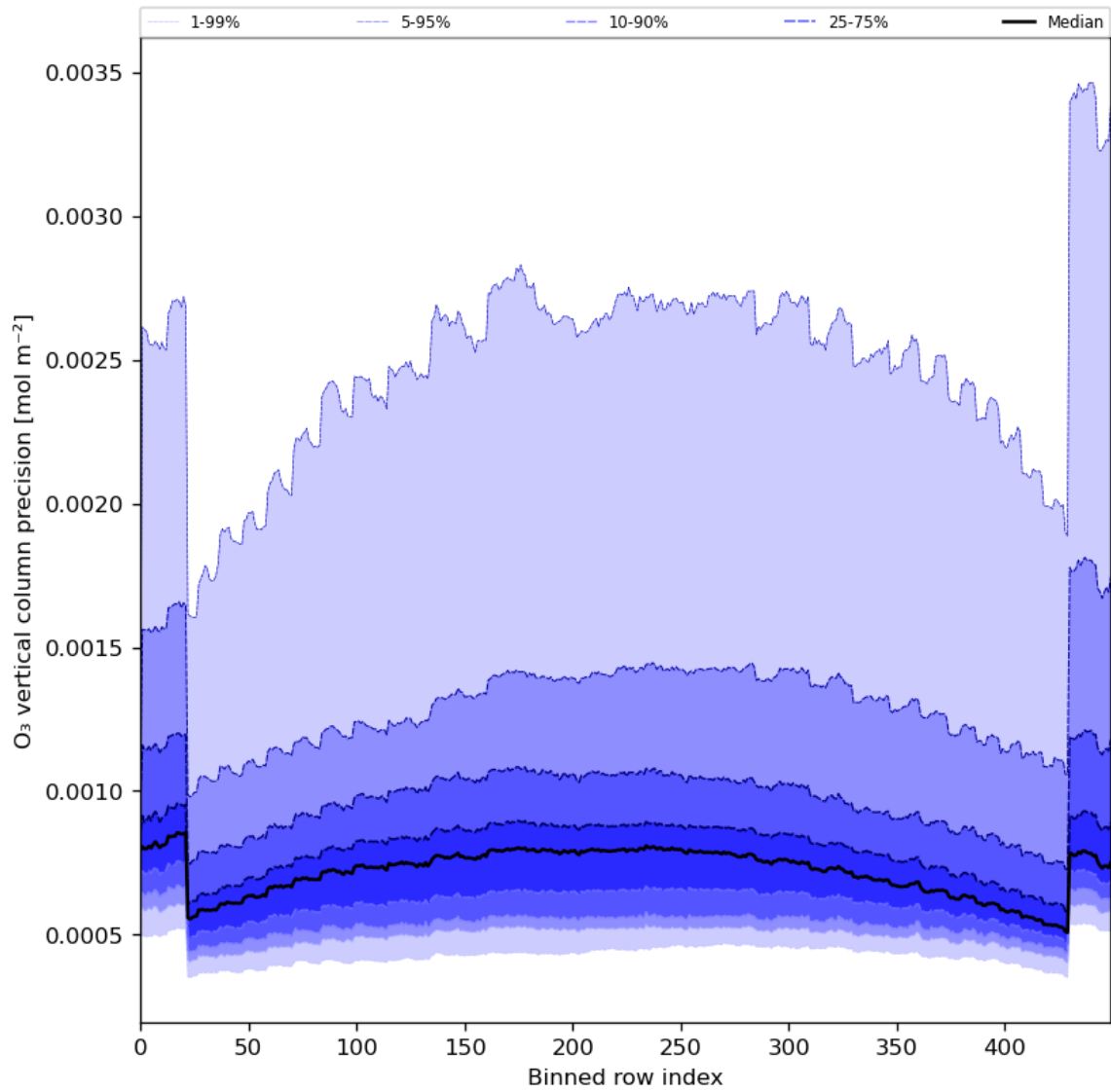
Figure 29: Along track statistics of “O 3 vertical column precision” for 2024-04-26 to 2024-04-28
