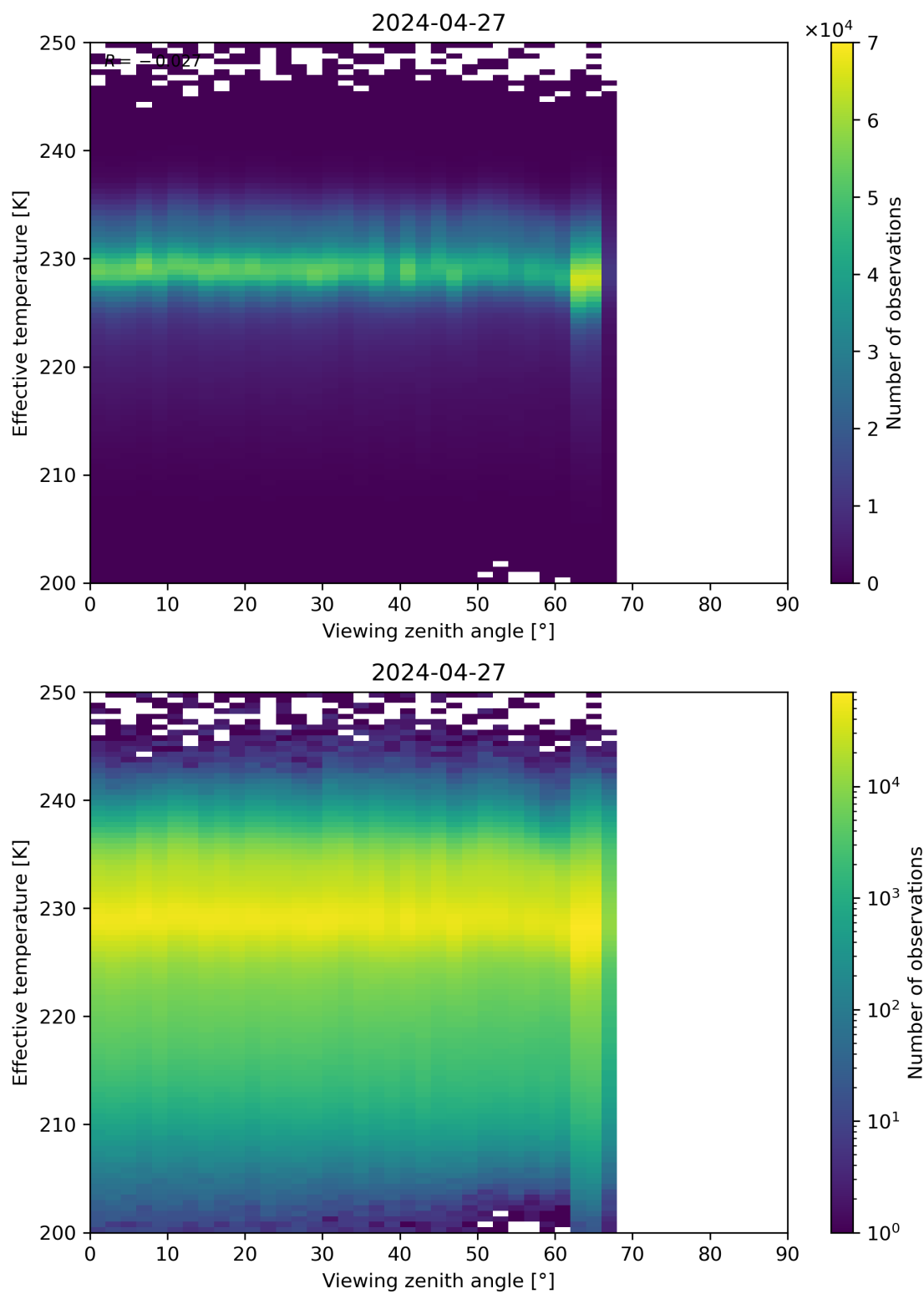
Figure 50: Scatter density plot of “Viewing zenith angle” against “Effective temperature” for 2024-04-26 to 2024-04-28.
