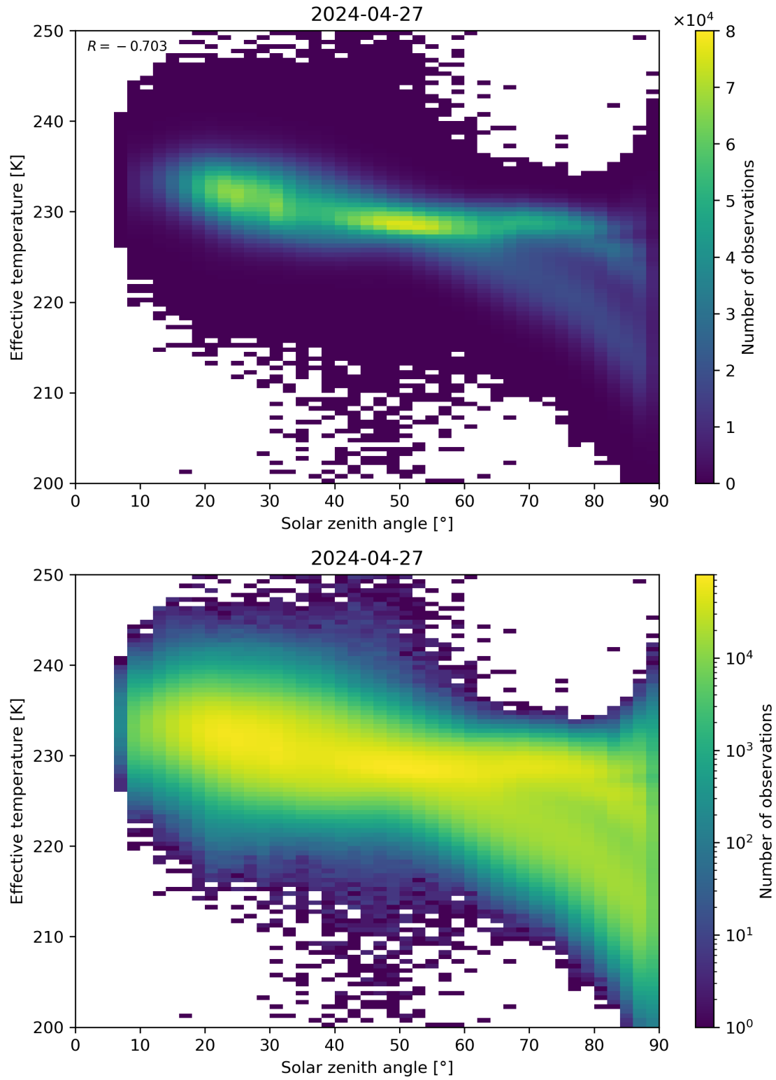
Figure 45: Scatter density plot of “Solar zenith angle” against “Effective temperature” for 2024-04-26 to 2024-04-28.
