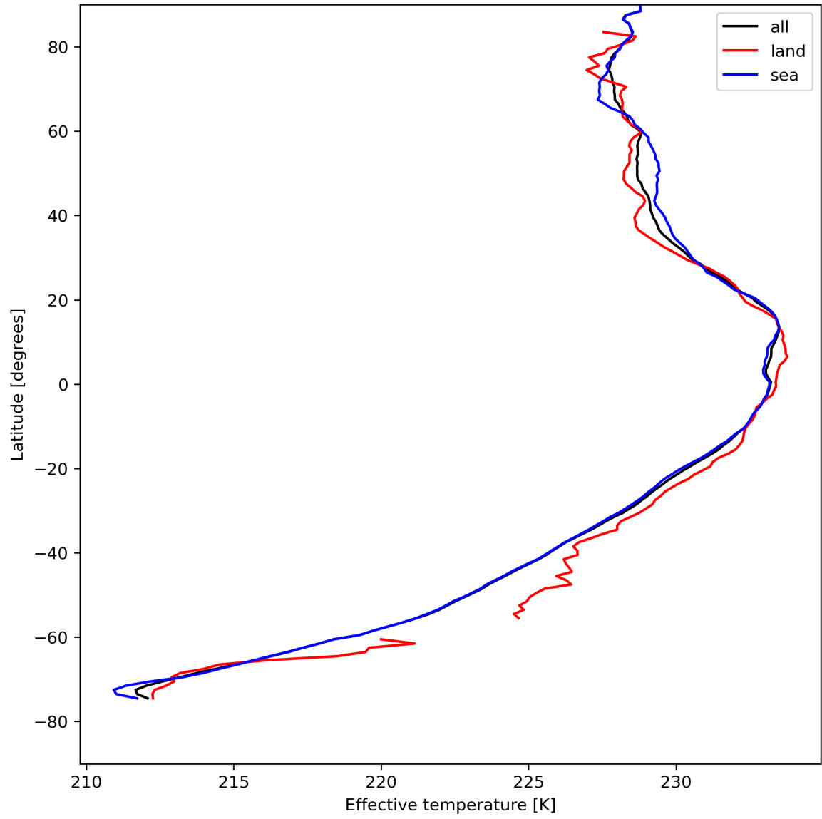
Figure 17: Zonal average of “Effective temperature” for 2024-04-26 to 2024-04-28.
