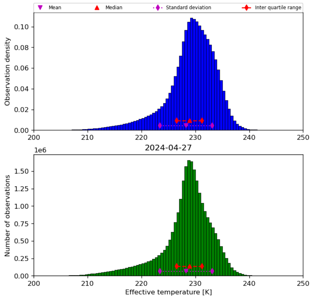
Figure 24: Histogram of “Effective temperature” for 2024-04-26 to 2024-04-28
