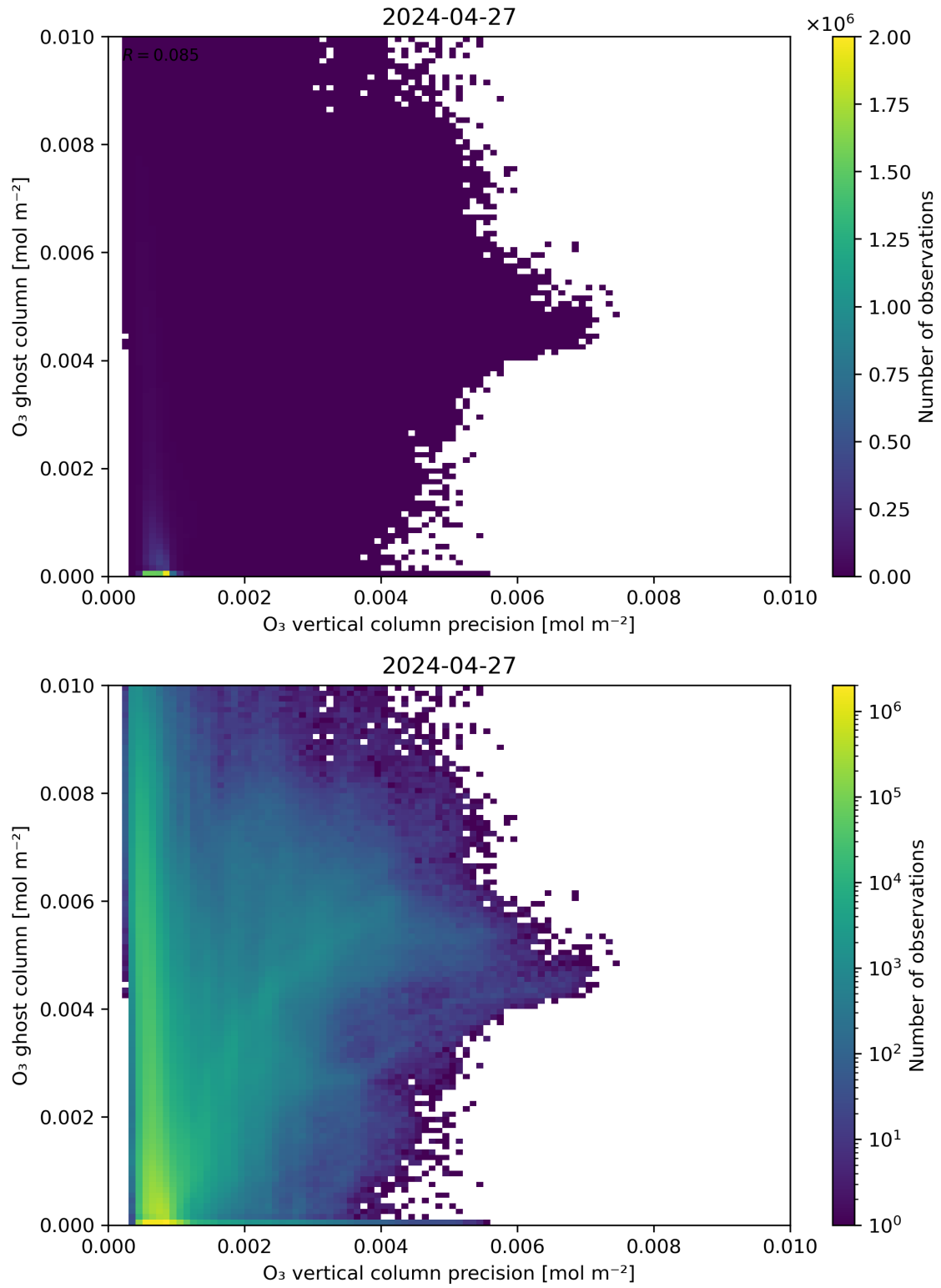
Figure 43: Scatter density plot of “ \text{O}_3 vertical column precision” against “ \text{O}_3 ghost column” for 2024-04-26 to 2024-04-28.
