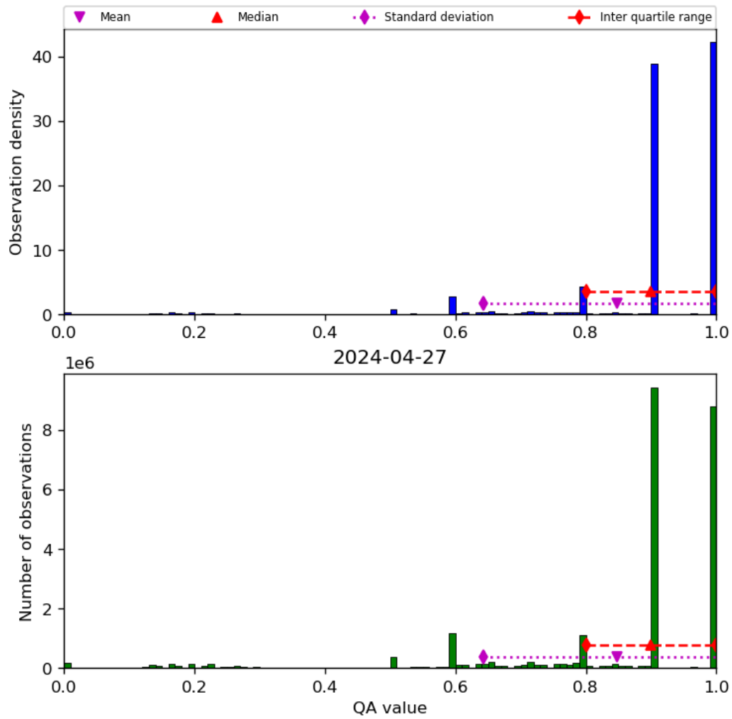
Figure 20: Histogram of “QA value” for 2024-04-26 to 2024-04-28
