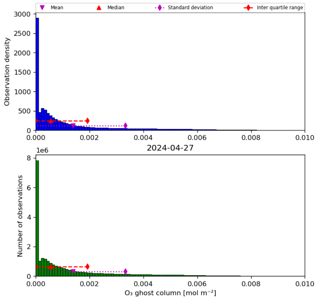
Figure 25: Histogram of “O 3 ghost column” for 2024-04-26 to 2024-04-28
