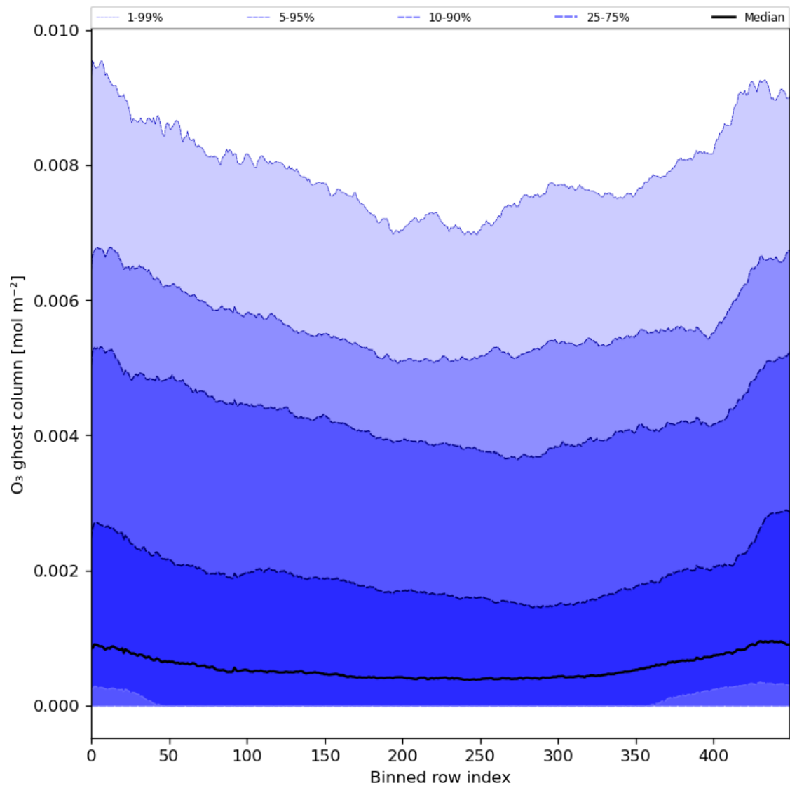
Figure 32: Along track statistics of “O 3 ghost column” for 2024-04-26 to 2024-04-28
