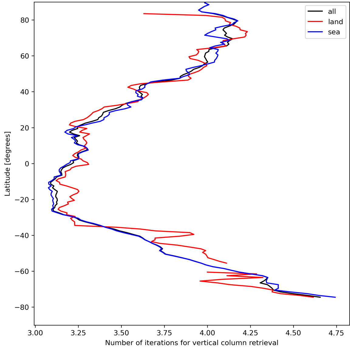
Figure 19: Zonal average of “Number of iterations for vertical column retrieval” for 2024-04-26 to 2024-04-28.
