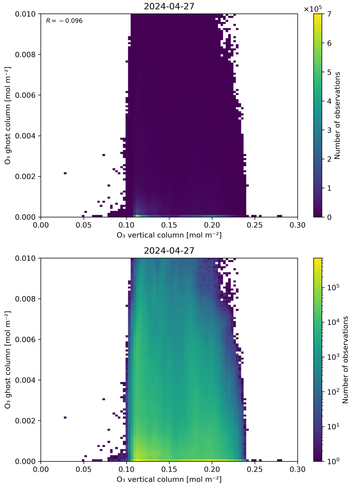
Figure 40: Scatter density plot of “O 3 vertical column” against “O 3 ghost column” for 2024-04-26 to 2024-04-28.
