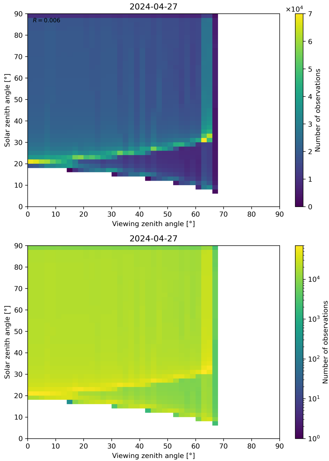
Figure 54: Scatter density plot of “Viewing zenith angle” against “Solar zenith angle” for 2024-04-26 to 2024-04-28.
