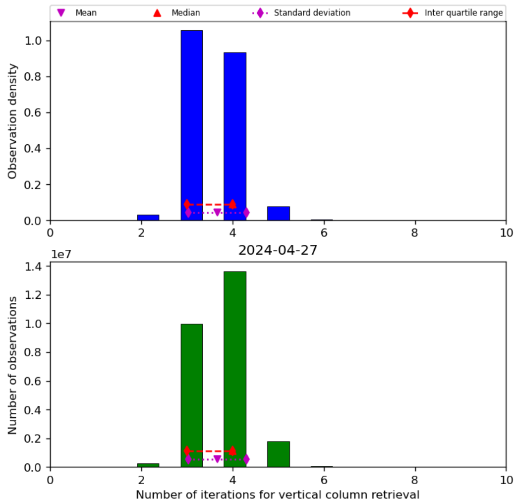
Figure 26: Histogram of “Number of iterations for vertical column retrieval” for 2024-04-26 to 2024-04-28
