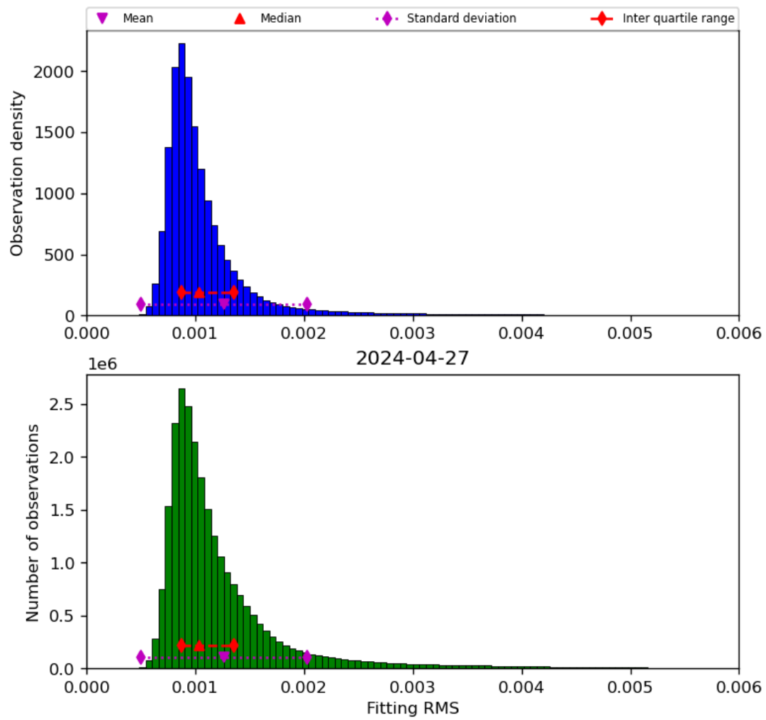
Figure 23: Histogram of “Fitting RMS” for 2024-04-26 to 2024-04-28
