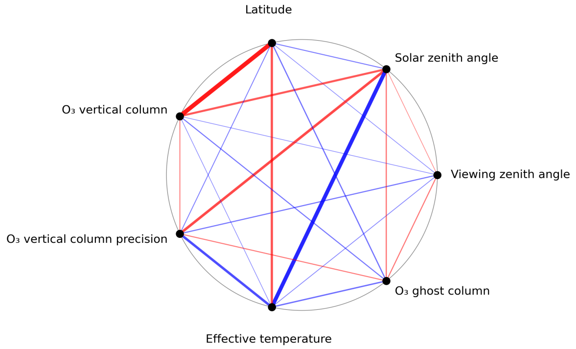
Figure 1: Map of correlation graph for 2024-04-26 to 2024-04-28.
