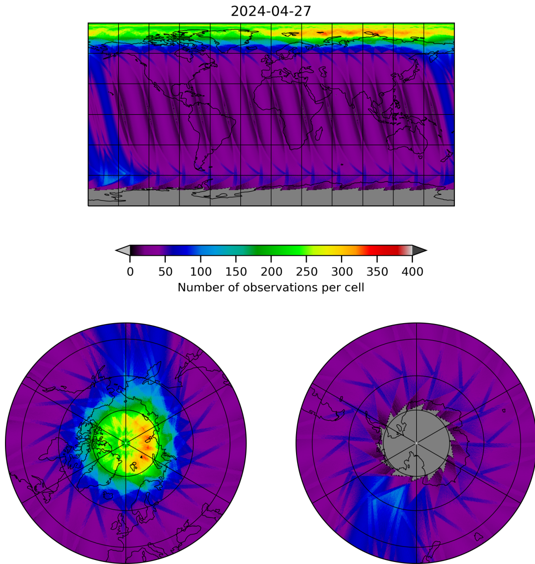
Figure 12: Map of the number of observations for 2024-04-26 to 2024-04-28
