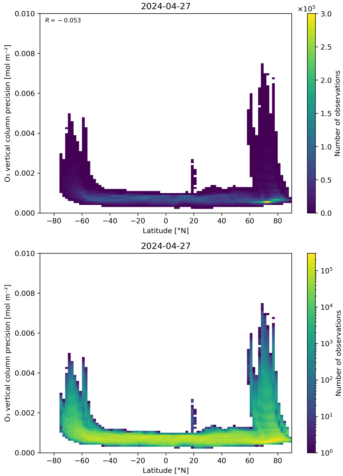
Figure 37: Scatter density plot of “Latitude” against “O 3 vertical column precision” for 2024-04-26 to 2024-04-28.
