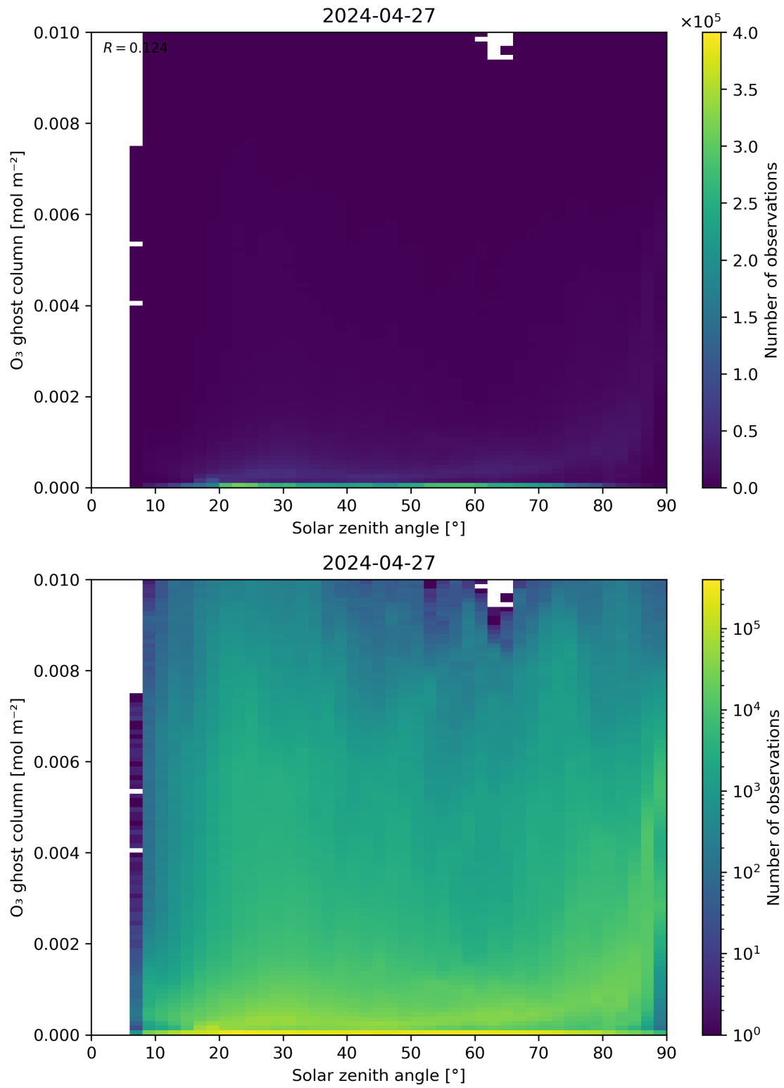
Figure 46: Scatter density plot of “Solar zenith angle” against “O 3 ghost column” for 2024-04-26 to 2024-04-28.
