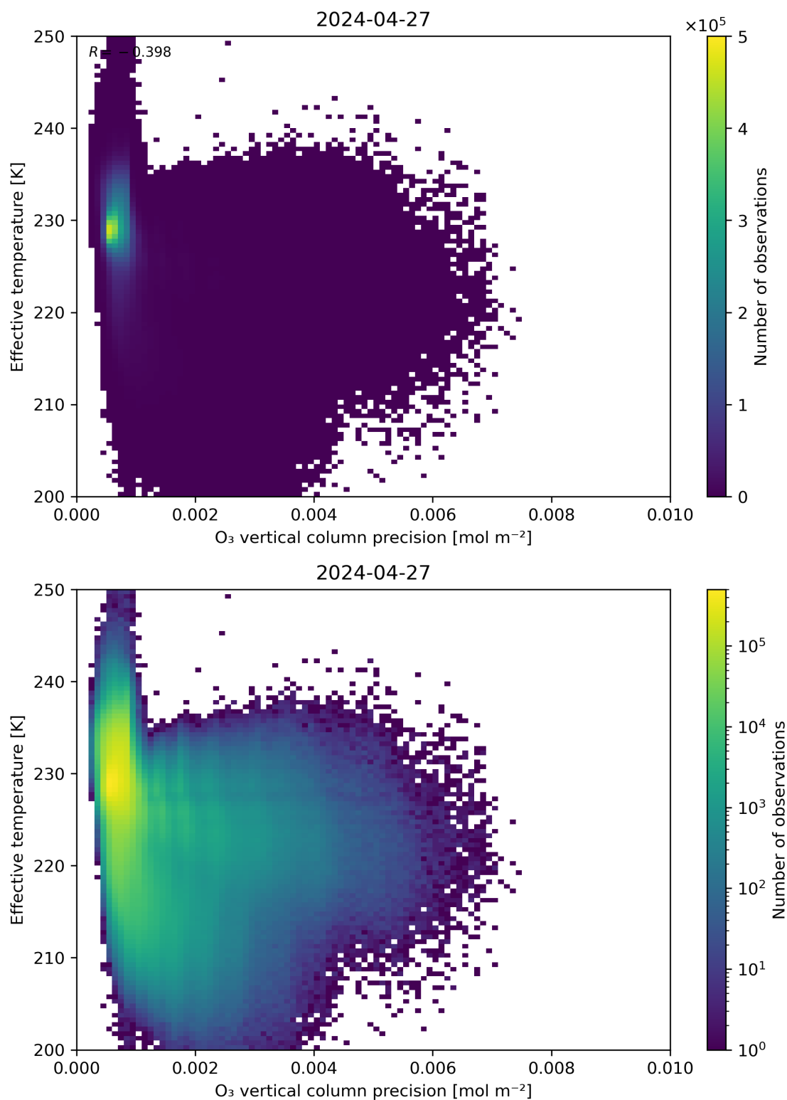
Figure 42: Scatter density plot of “O 3 vertical column precision” against “Effective temperature” for 2024-04-26 to 2024-04-28.
