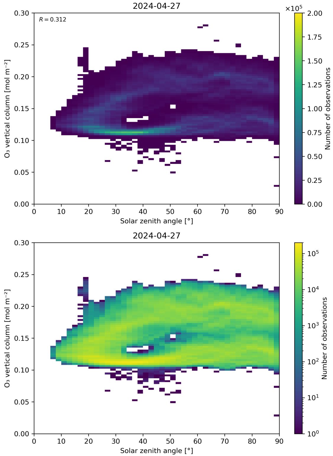
Figure 47: Scatter density plot of “Solar zenith angle” against “O 3 vertical column” for 2024-04-26 to 2024-04-28.
