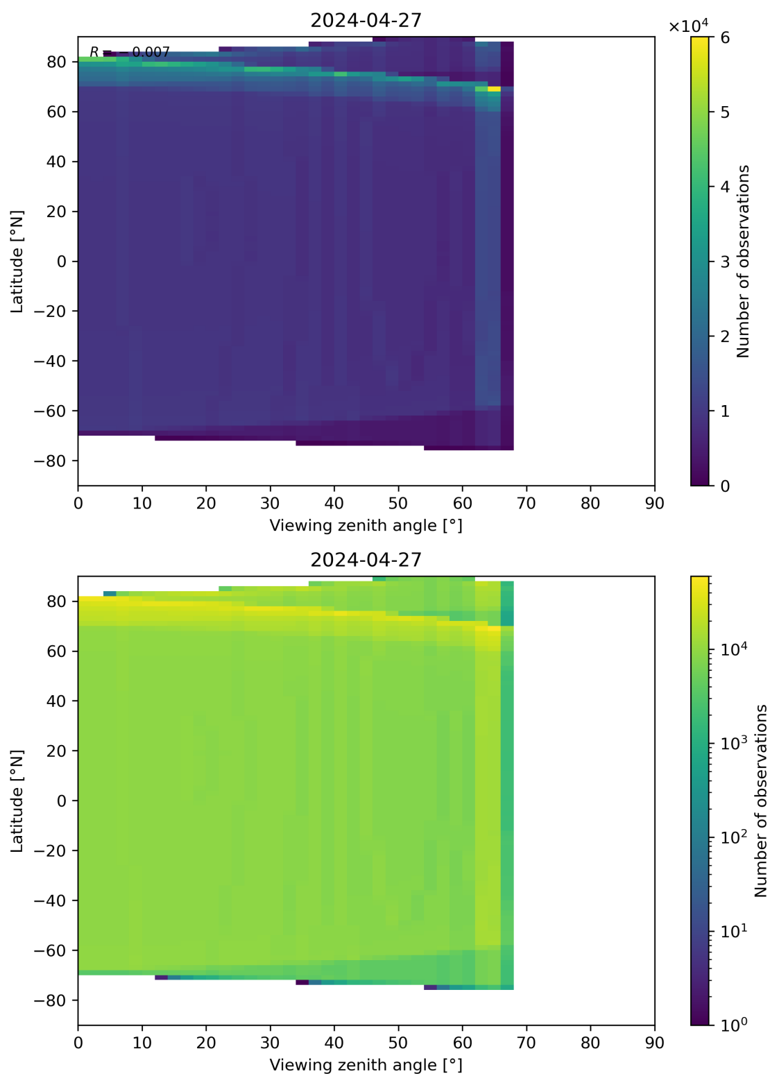
Figure 49: Scatter density plot of “Viewing zenith angle” against “Latitude” for 2024-04-26 to 2024-04-28.
