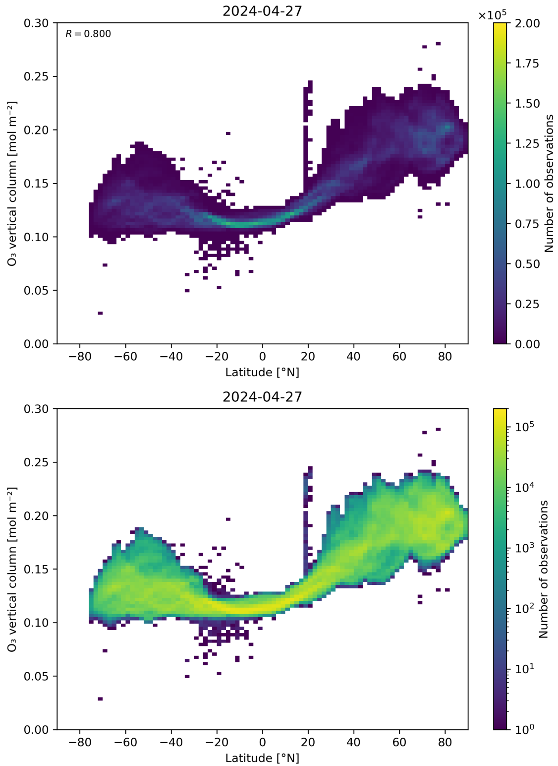
Figure 36: Scatter density plot of “Latitude” against “O 3 vertical column” for 2024-04-26 to 2024-04-28.
