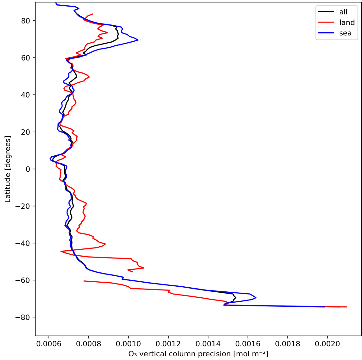
Figure 15: Zonal average of "O 3 vertical column precision" for 2024-04-26 to 2024-04-28.
