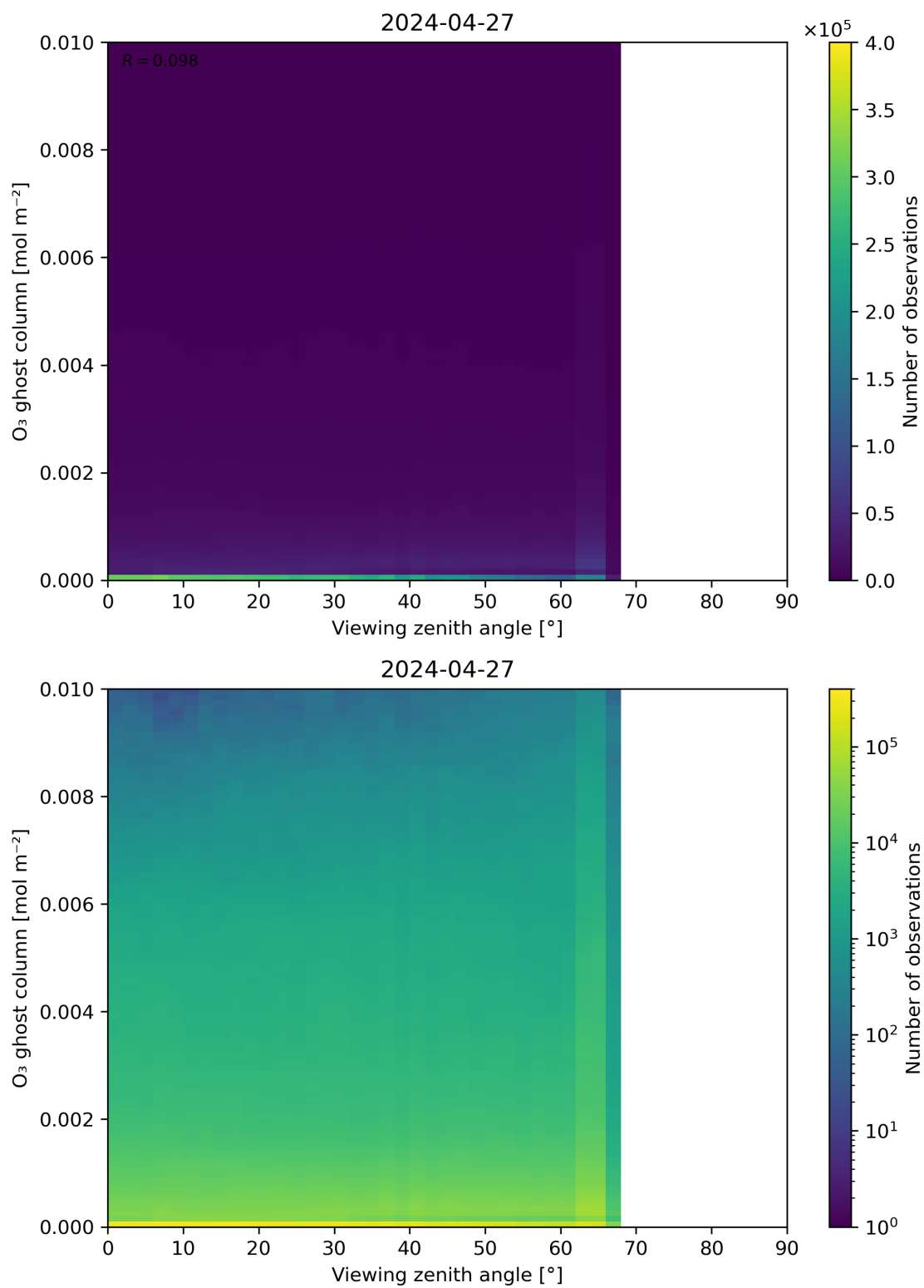
Figure 51: Scatter density plot of “Viewing zenith angle” against “O 3 ghost column” for 2024-04-26 to 2024-04-28.
