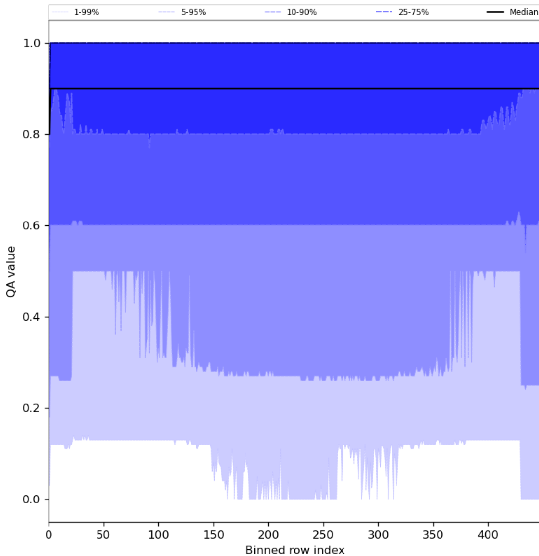
Figure 27: Along track statistics of “QA value” for 2024-04-26 to 2024-04-28
