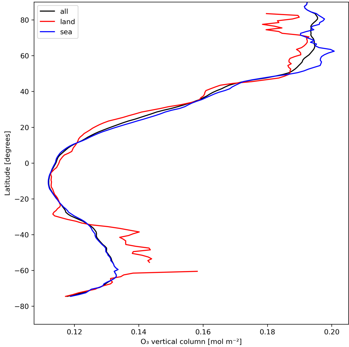
Figure 14: Zonal average of “O 3 vertical column” for 2024-04-26 to 2024-04-28.
