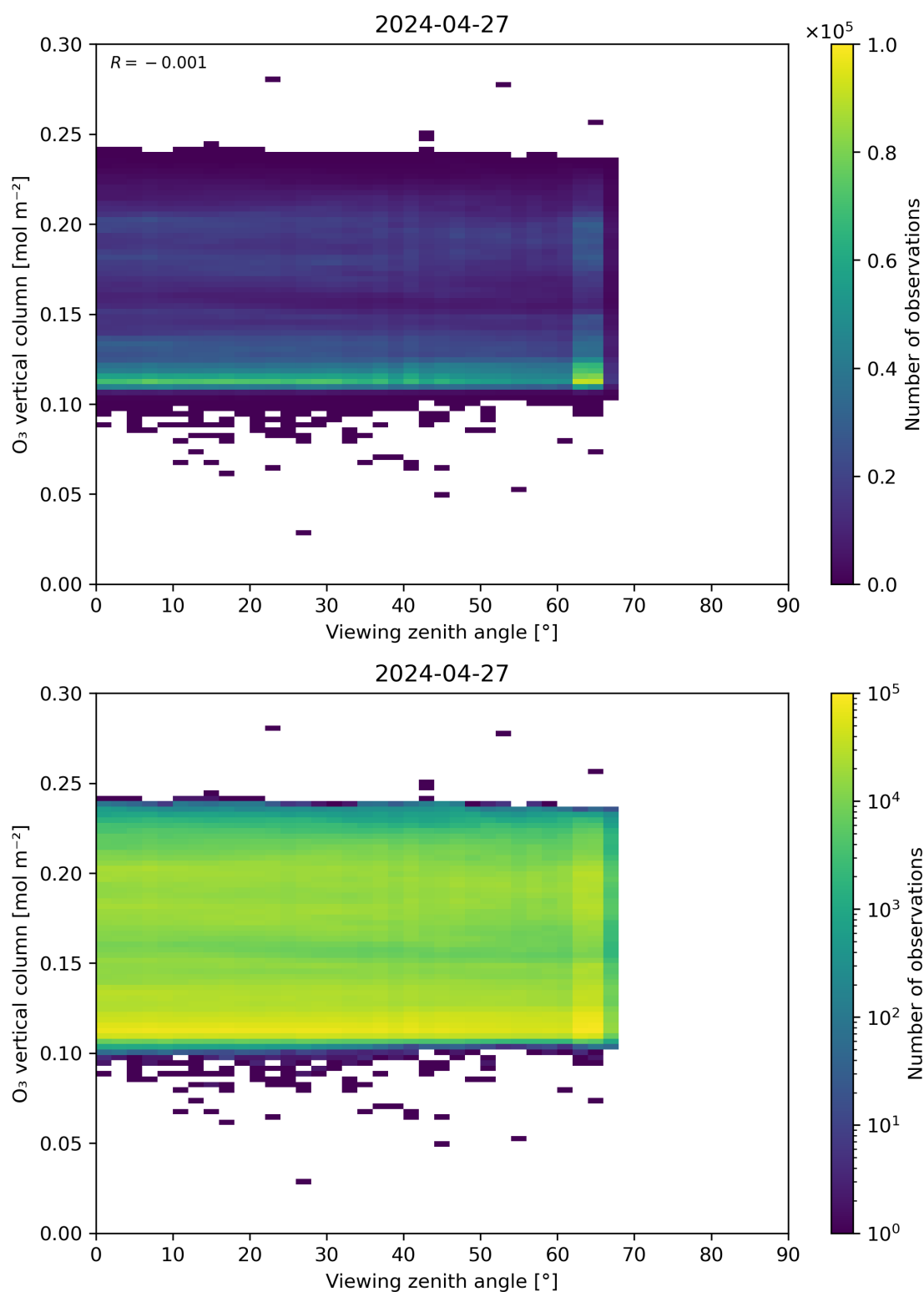
Figure 52: Scatter density plot of “Viewing zenith angle” against “O 3 vertical column” for 2024-04-26 to 2024-04-28.
