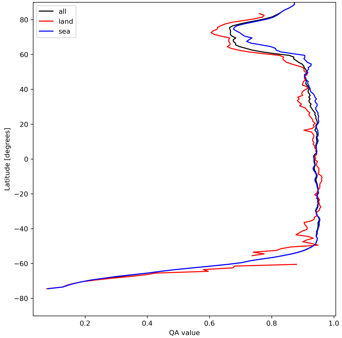
Figure 13: Zonal average of “QA value” for 2024-04-26 to 2024-04-28.
