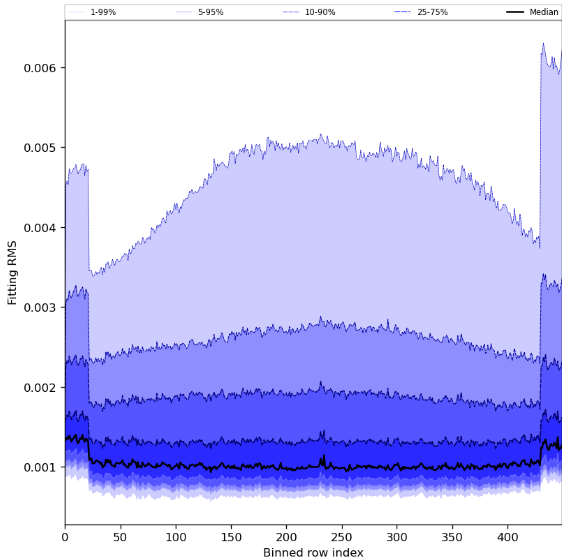
Figure 30: Along track statistics of “Fitting RMS” for 2024-04-26 to 2024-04-28
