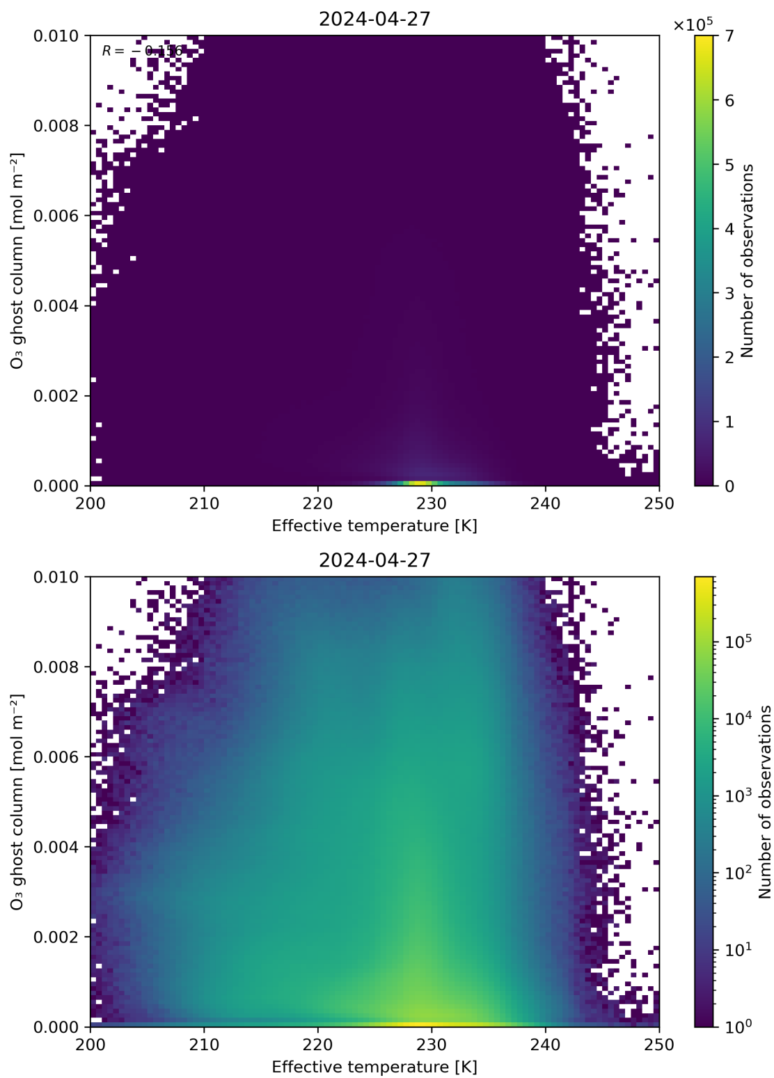
Figure 38: Scatter density plot of “Effective temperature” against “O 3 ghost column” for 2024-04-26 to 2024-04-28.
