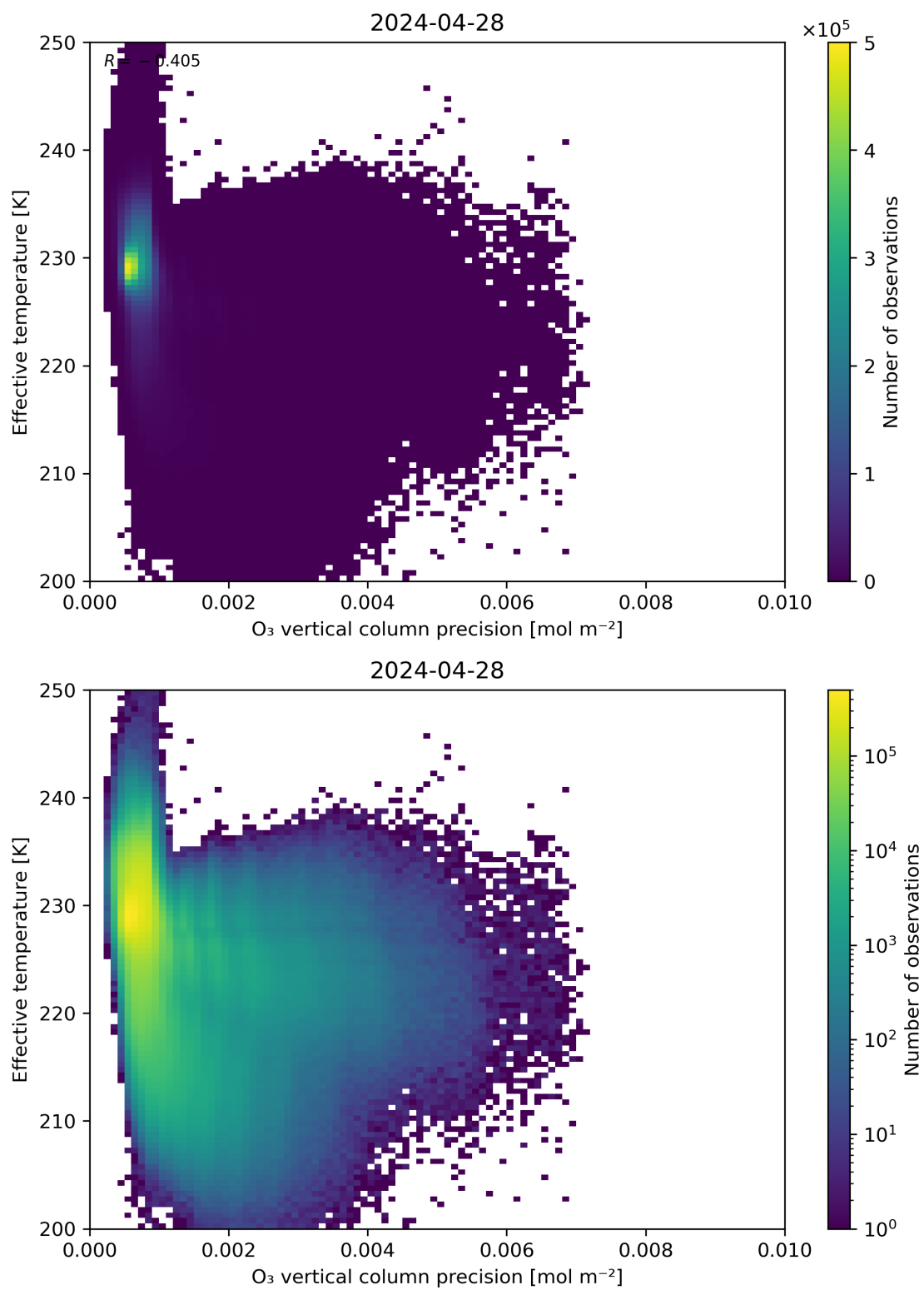
Figure 42: Scatter density plot of “O 3 vertical column precision” against “Effective temperature” for 2024-04-27 to 2024-04-29.
