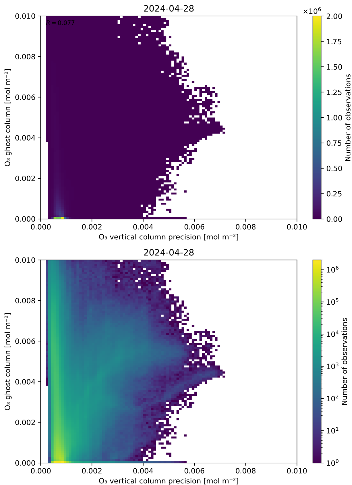
Figure 43: Scatter density plot of “ \text{O}_3 vertical column precision” against “ \text{O}_3 ghost column” for 2024-04-27 to 2024-04-29.
