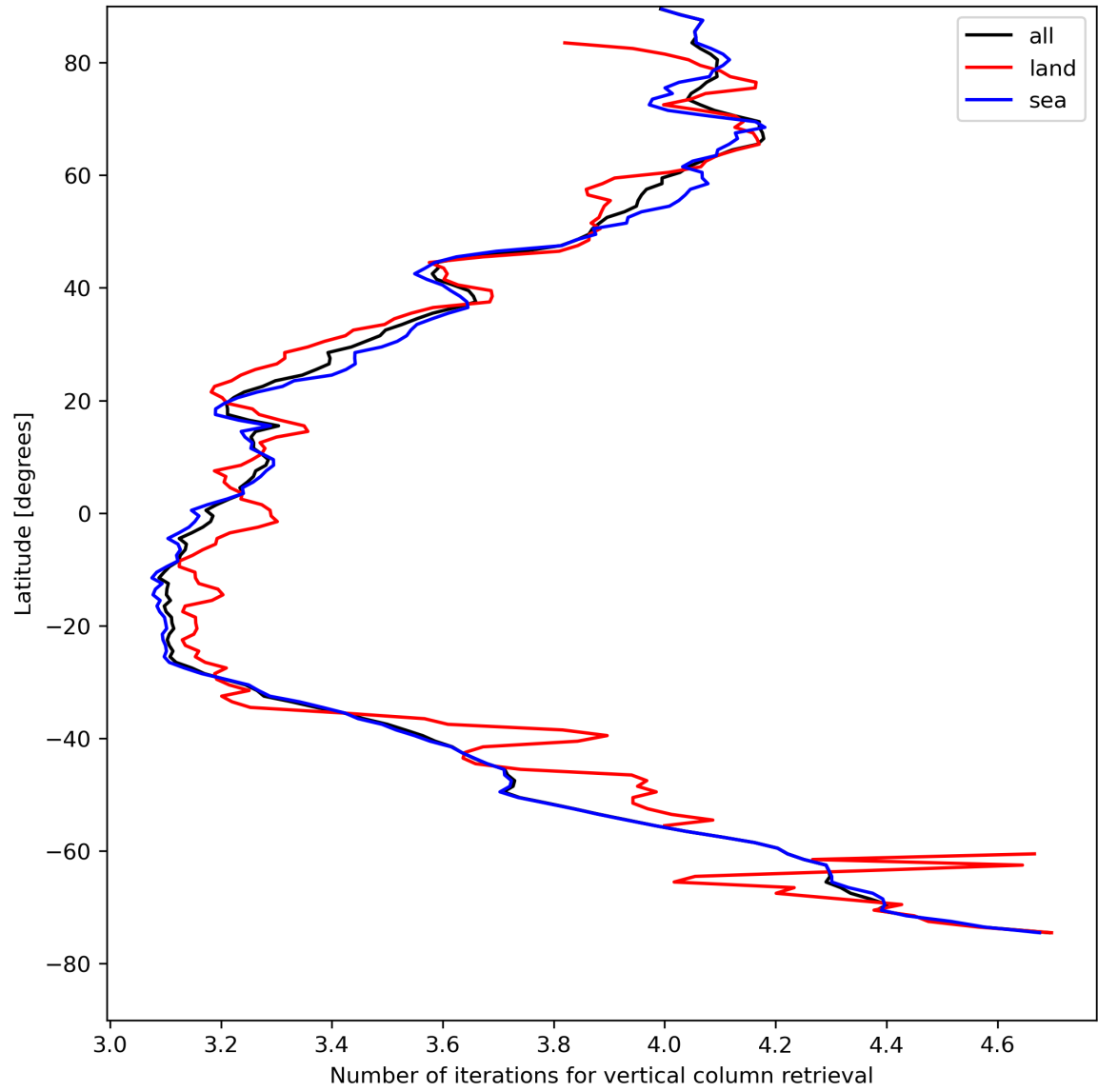
Figure 19: Zonal average of “Number of iterations for vertical column retrieval” for 2024-04-27 to 2024-04-29.
