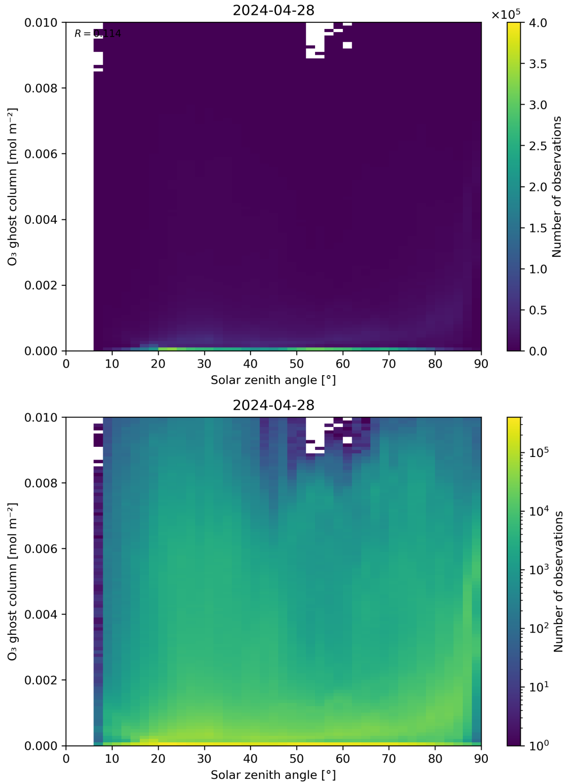
Figure 46: Scatter density plot of “Solar zenith angle” against “O 3 ghost column” for 2024-04-27 to 2024-04-29.
