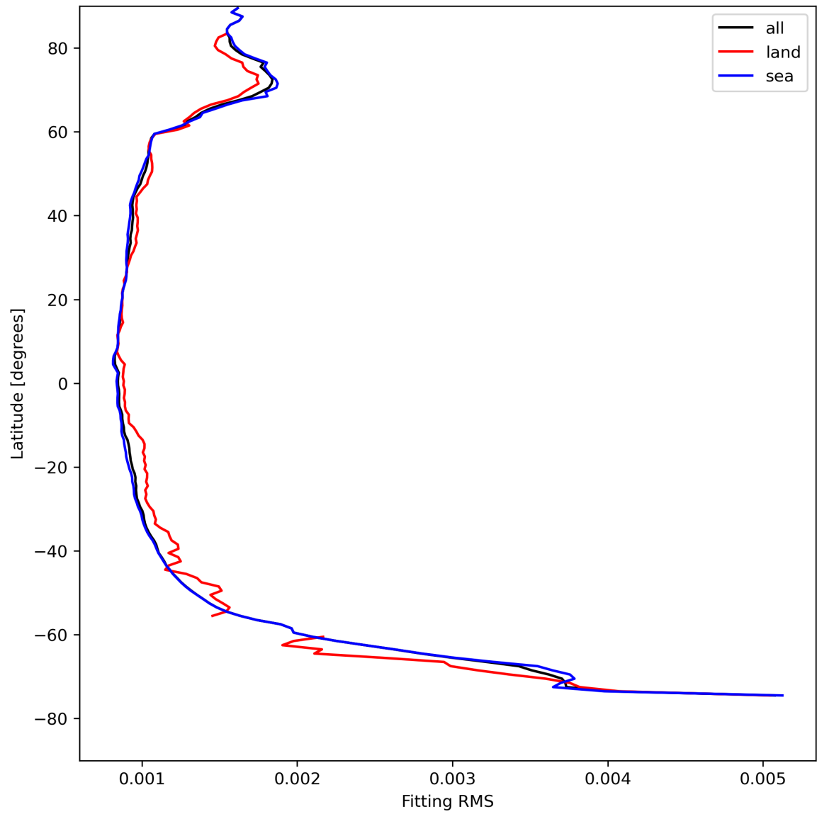
Figure 16: Zonal average of “Fitting RMS” for 2024-04-27 to 2024-04-29.
