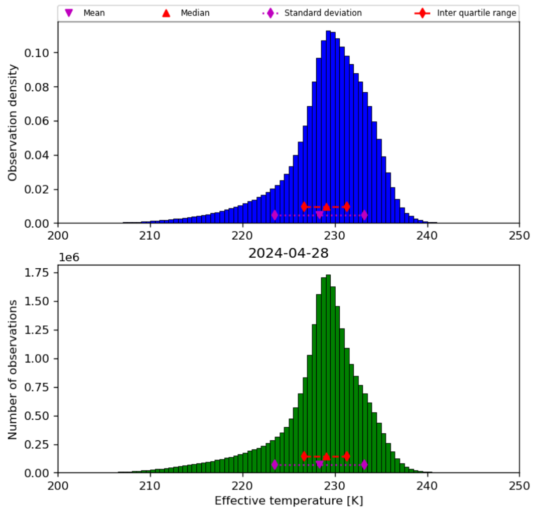
Figure 24: Histogram of “Effective temperature” for 2024-04-27 to 2024-04-29
