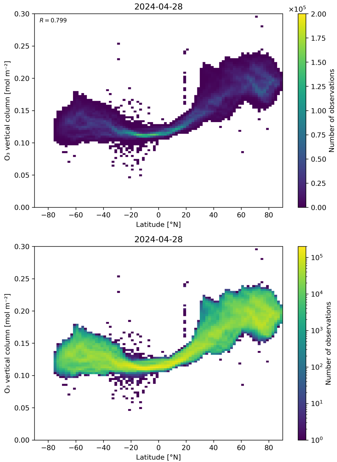
Figure 36: Scatter density plot of “Latitude” against “O 3 vertical column” for 2024-04-27 to 2024-04-29.
