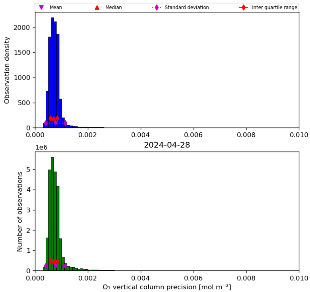
Figure 22: Histogram of “O 3 vertical column precision” for 2024-04-27 to 2024-04-29
