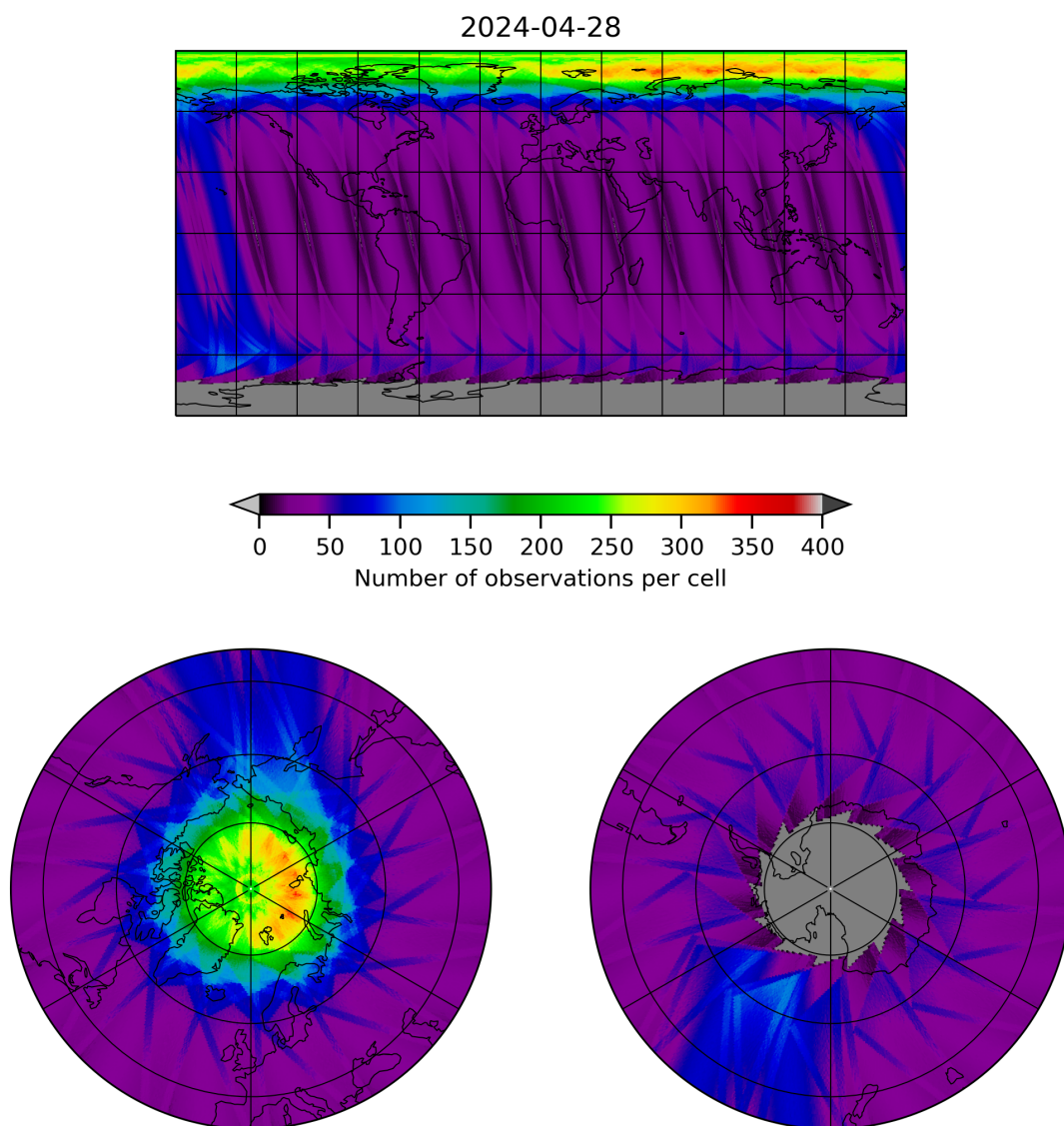
Figure 12: Map of the number of observations for 2024-04-27 to 2024-04-29
