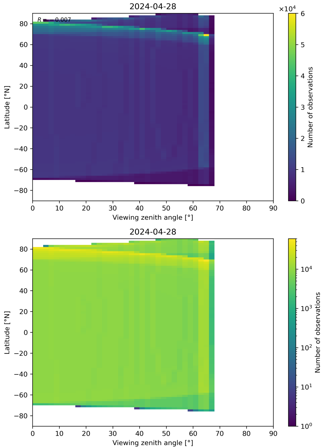
Figure 49: Scatter density plot of “Viewing zenith angle” against “Latitude” for 2024-04-27 to 2024-04-29.
