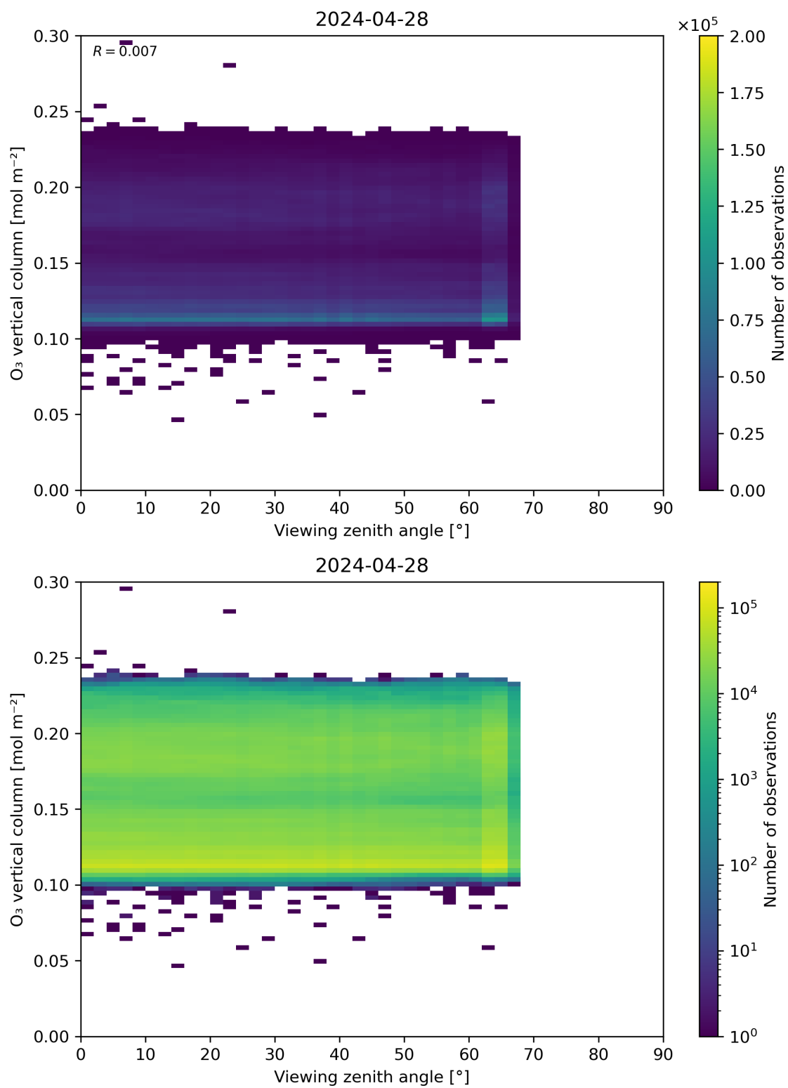
Figure 52: Scatter density plot of “Viewing zenith angle” against “O 3 vertical column” for 2024-04-27 to 2024-04-29.
