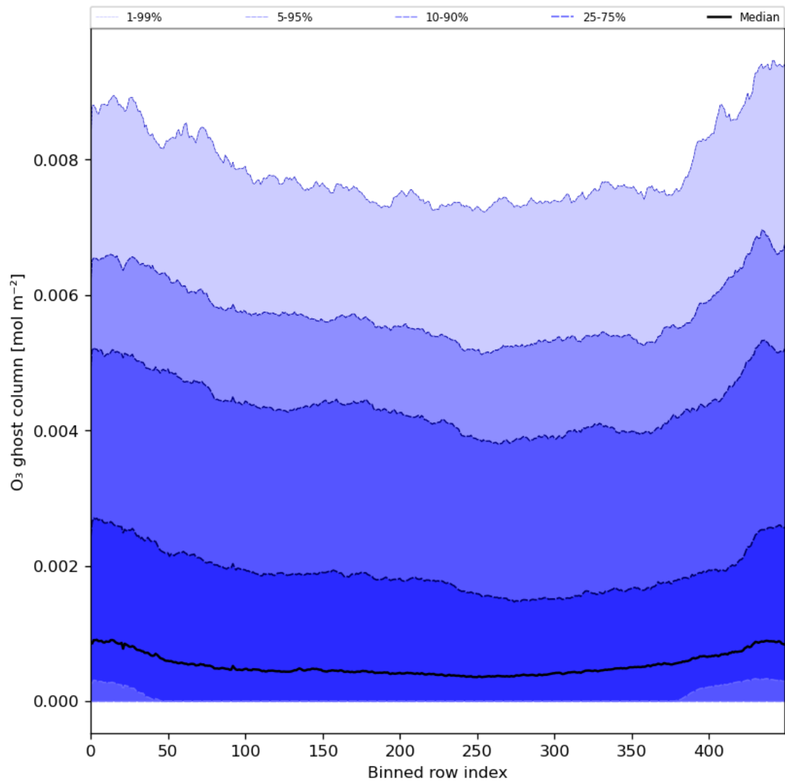
Figure 32: Along track statistics of “O 3 ghost column” for 2024-04-27 to 2024-04-29
