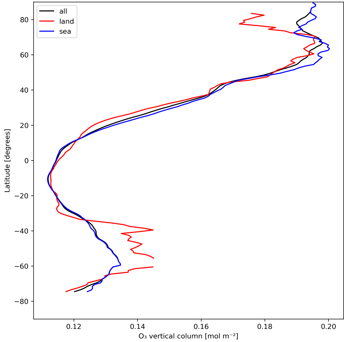
Figure 14: Zonal average of “O 3 vertical column” for 2024-04-27 to 2024-04-29.
