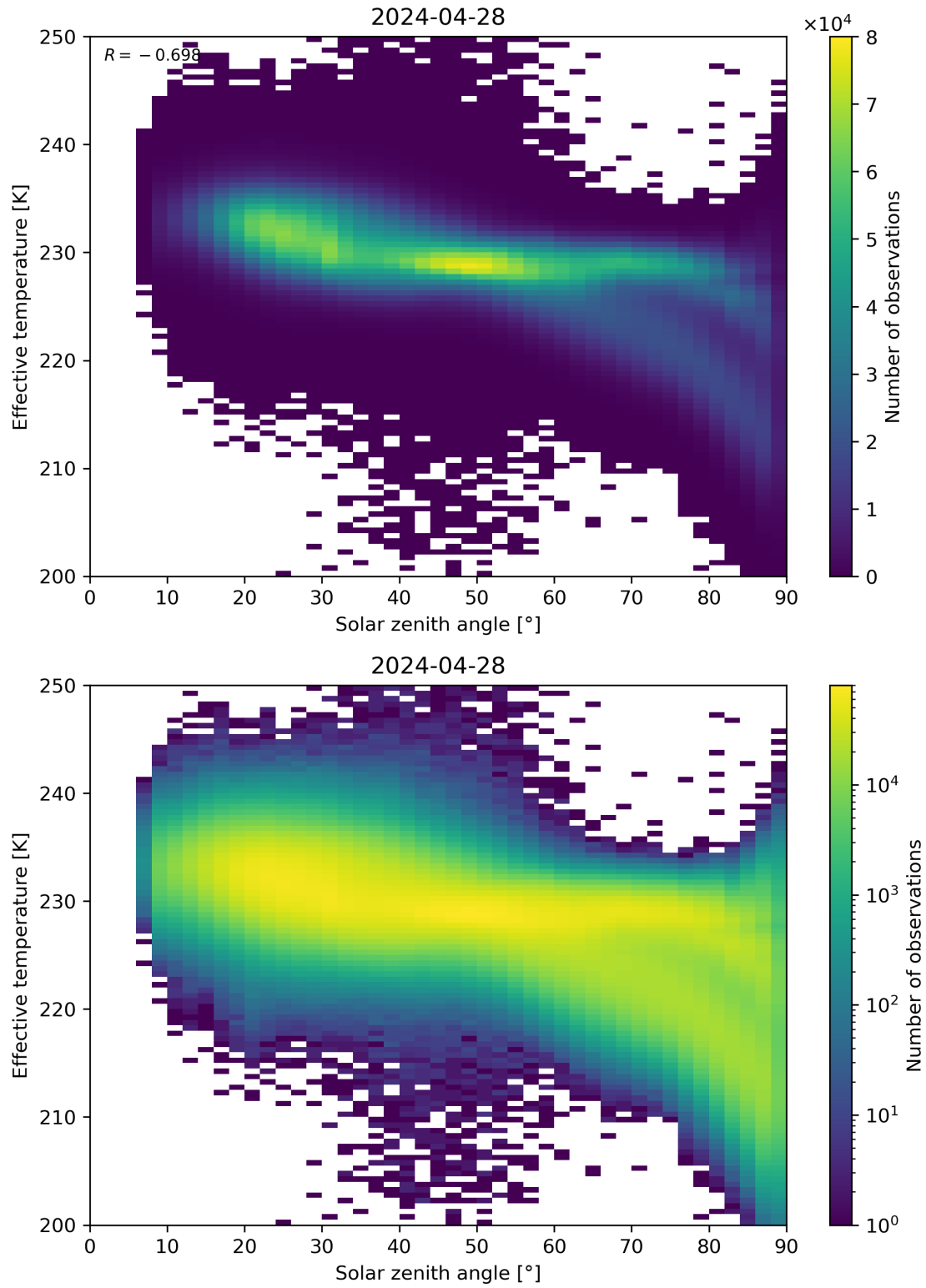
Figure 45: Scatter density plot of “Solar zenith angle” against “Effective temperature” for 2024-04-27 to 2024-04-29.
