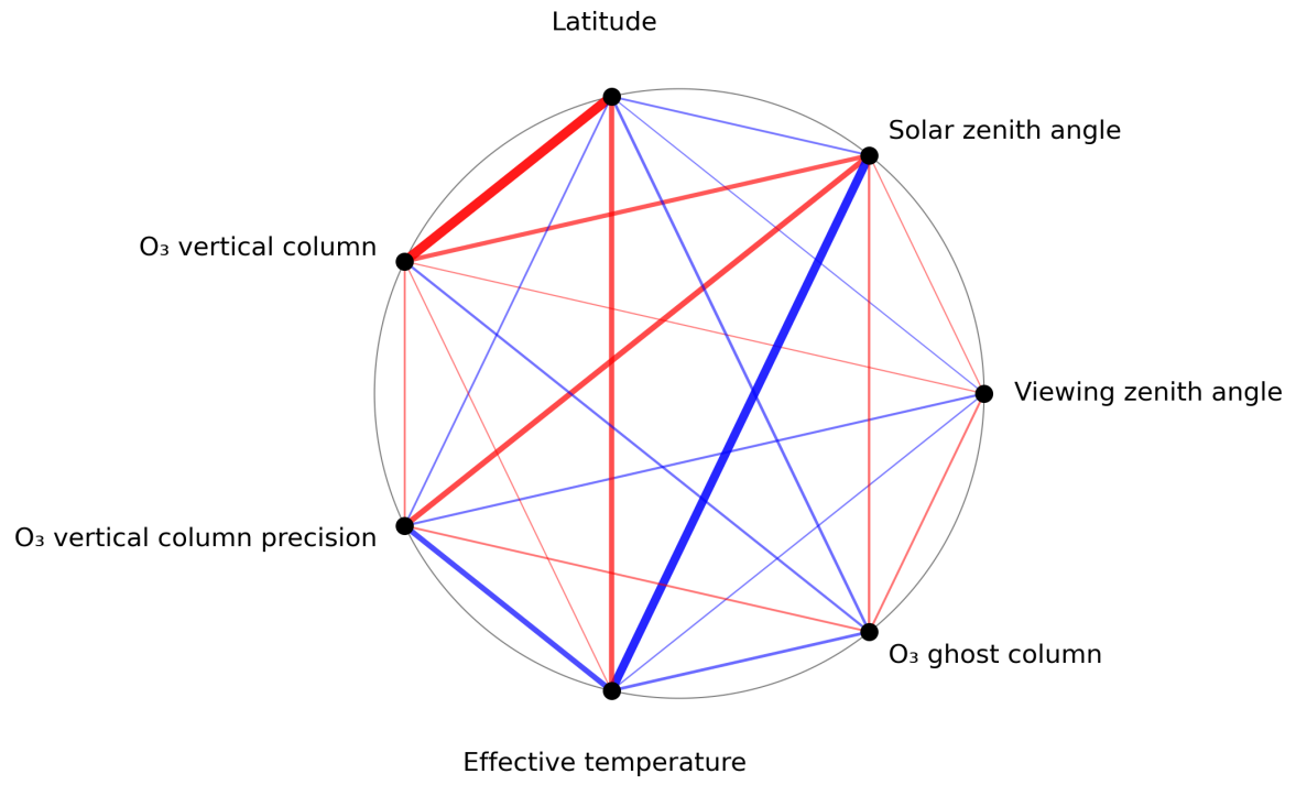
Figure 1: Map of correlation graph for 2024-04-27 to 2024-04-29.
