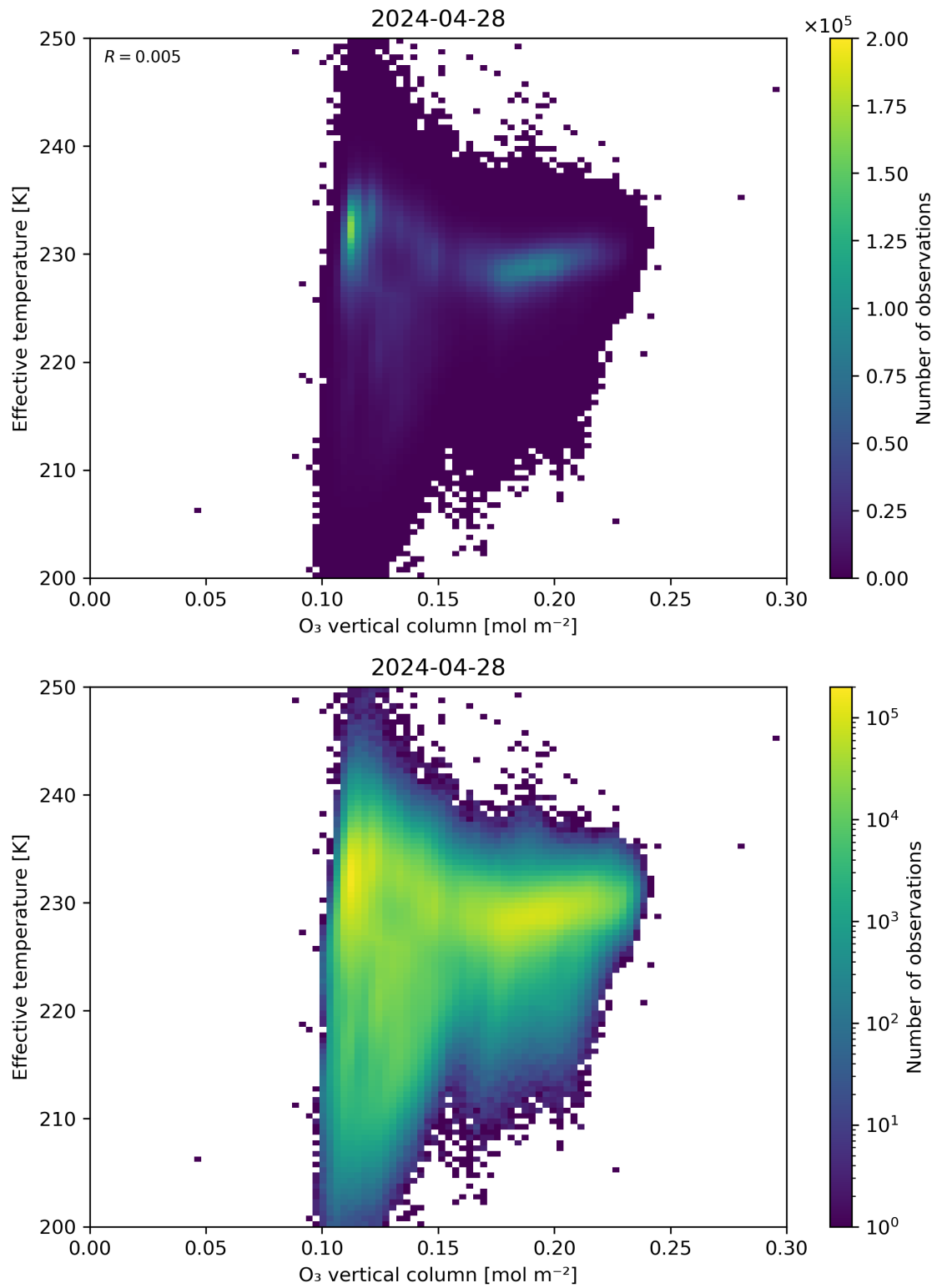
Figure 39: Scatter density plot of “O 3 vertical column” against “Effective temperature” for 2024-04-27 to 2024-04-29.
