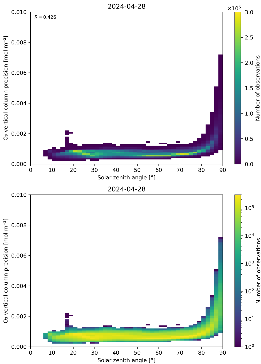
Figure 48: Scatter density plot of “Solar zenith angle” against “O 3 vertical column precision” for 2024-04-27 to 2024-04-29.
