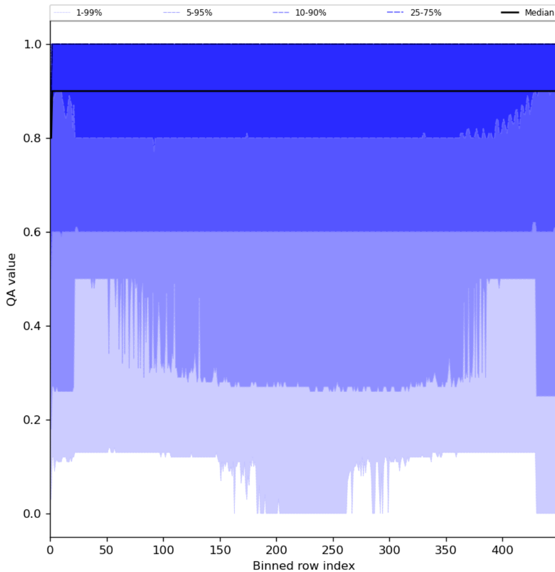
Figure 27: Along track statistics of “QA value” for 2024-04-27 to 2024-04-29
