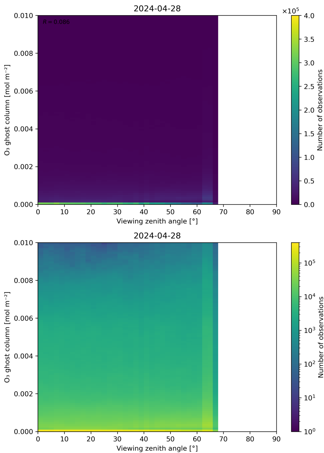
Figure 51: Scatter density plot of “Viewing zenith angle” against “O 3 ghost column” for 2024-04-27 to 2024-04-29.
