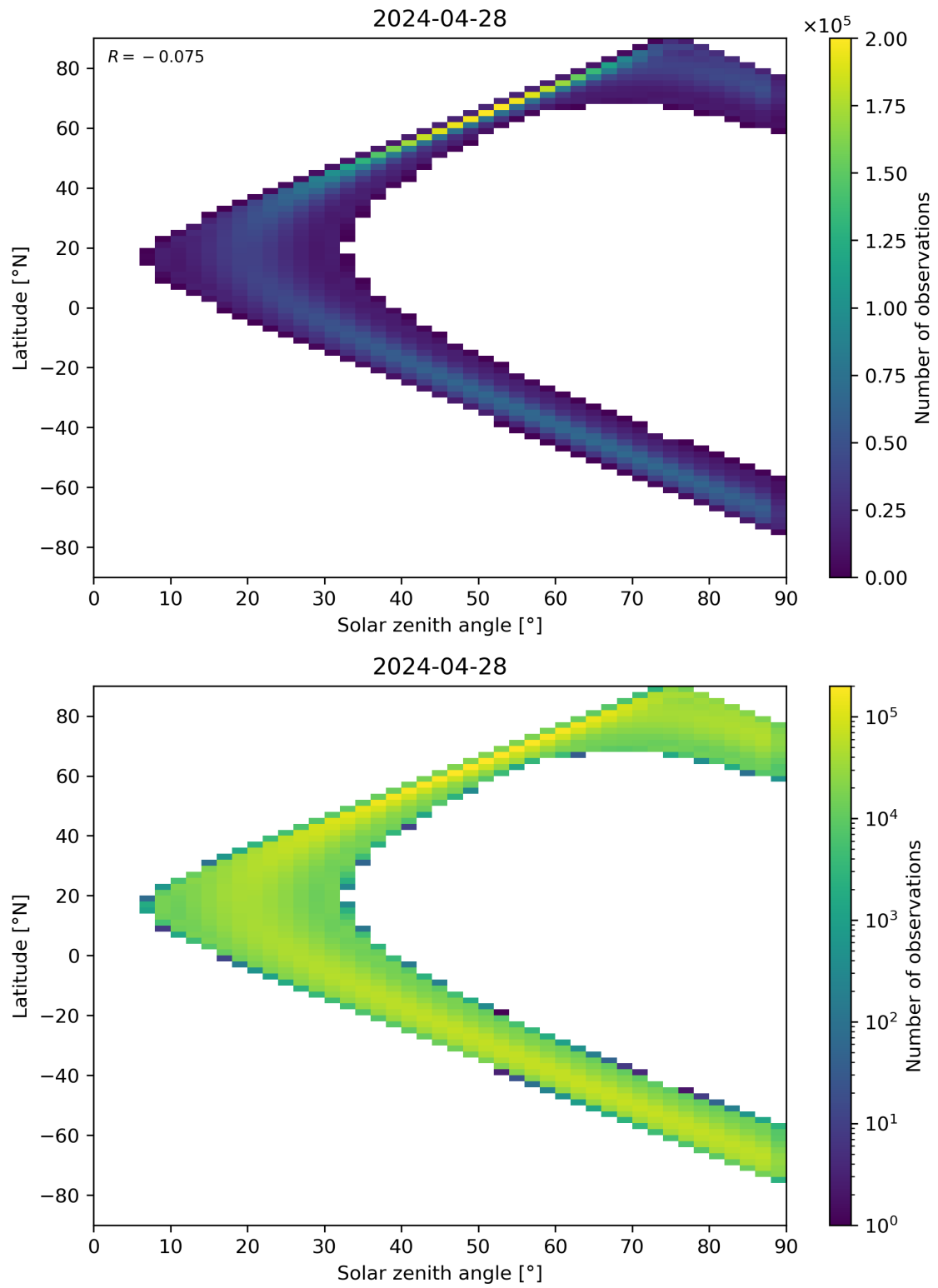
Figure 44: Scatter density plot of “Solar zenith angle” against “Latitude” for 2024-04-27 to 2024-04-29.
