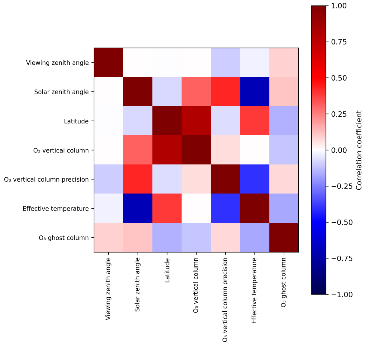
Figure 2: Map of correlation matrix for 2024-04-27 to 2024-04-29.
