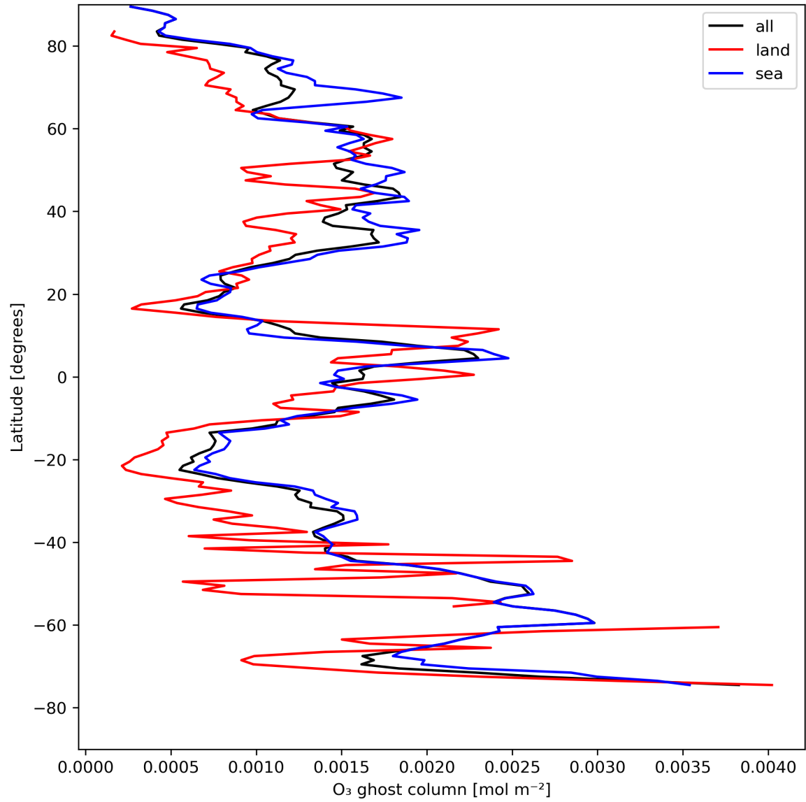
Figure 18: Zonal average of “O 3 ghost column” for 2024-04-27 to 2024-04-29.
