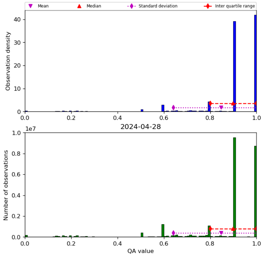
Figure 20: Histogram of “QA value” for 2024-04-27 to 2024-04-29
