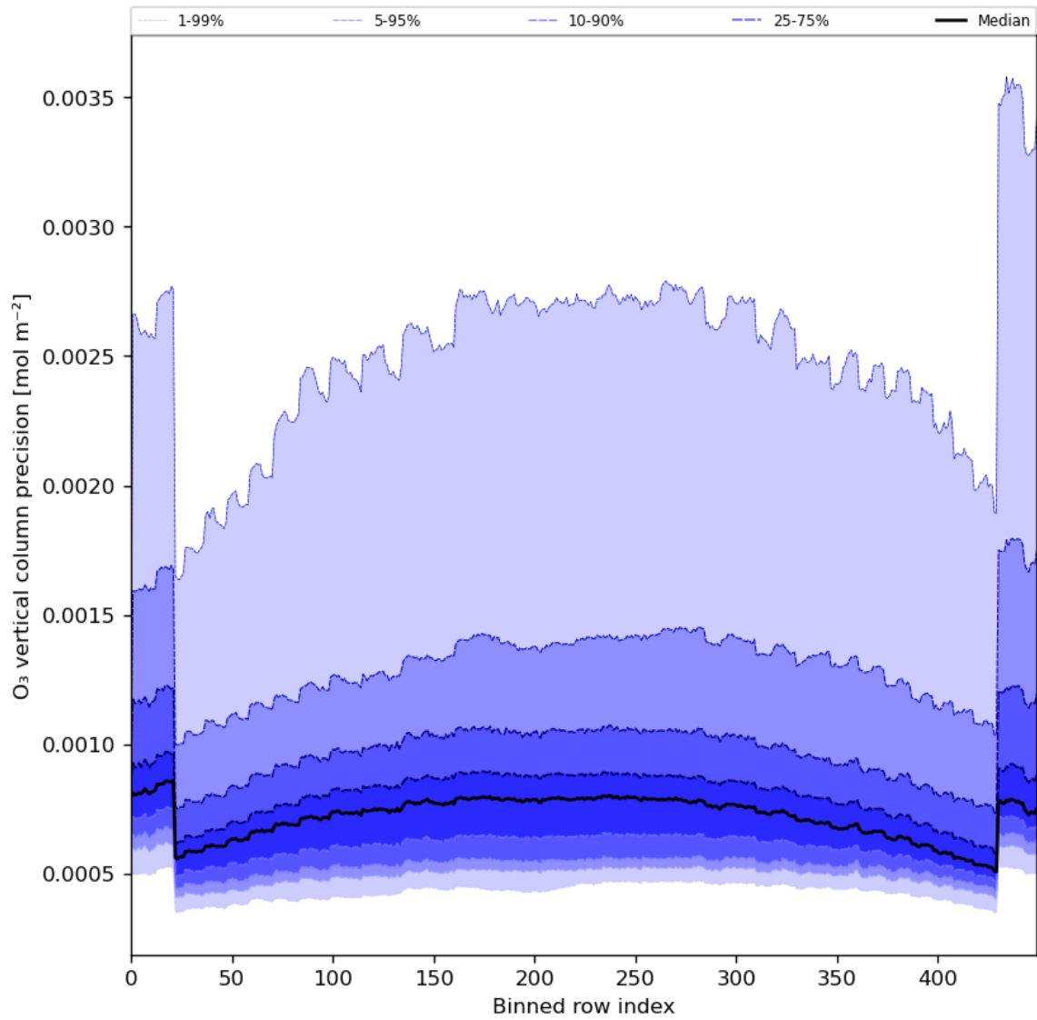
Figure 29: Along track statistics of “O 3 vertical column precision” for 2024-04-27 to 2024-04-29
