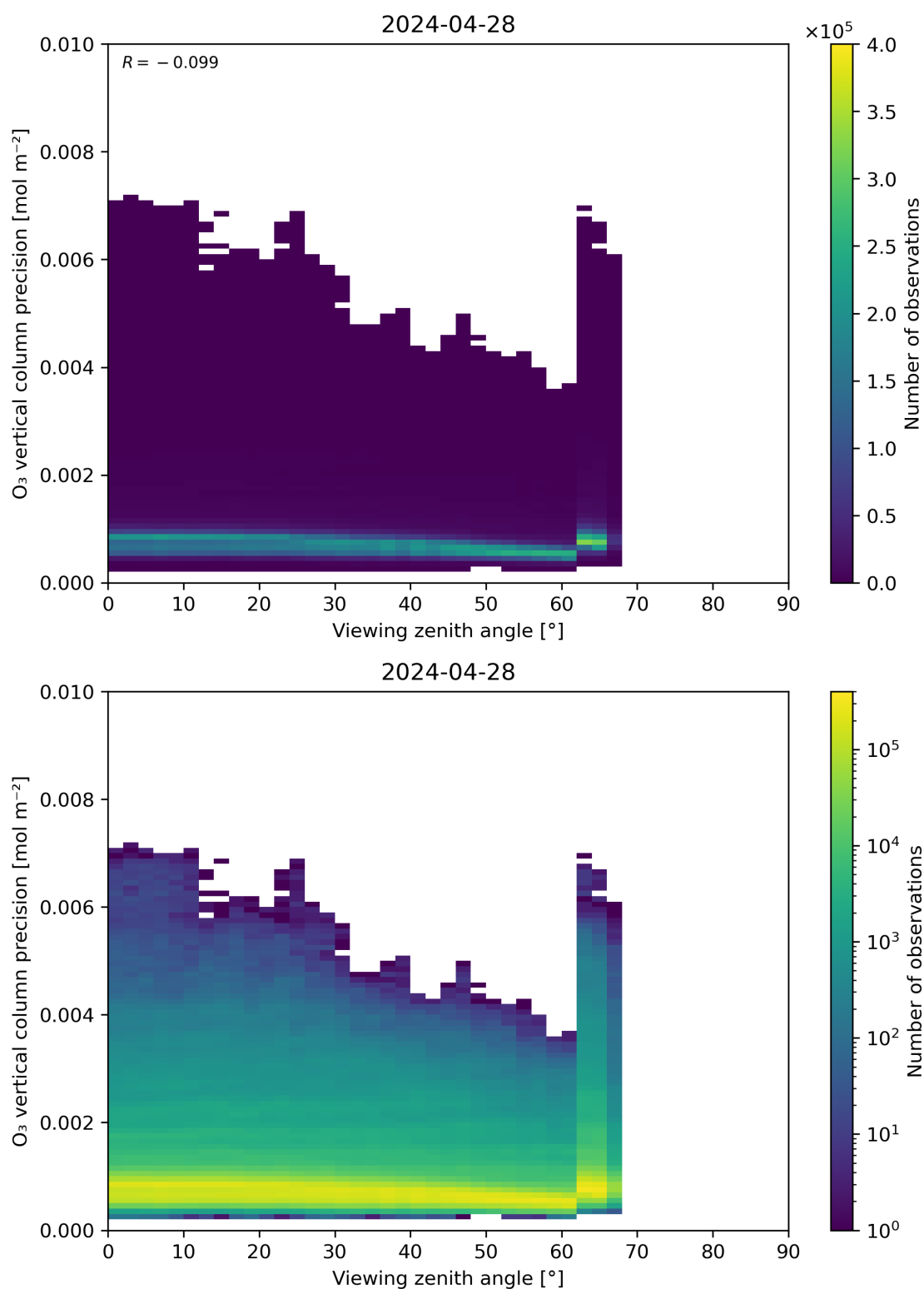
Figure 53: Scatter density plot of “Viewing zenith angle” against “O 3 vertical column precision” for 2024-04-27 to 2024-04-29.
