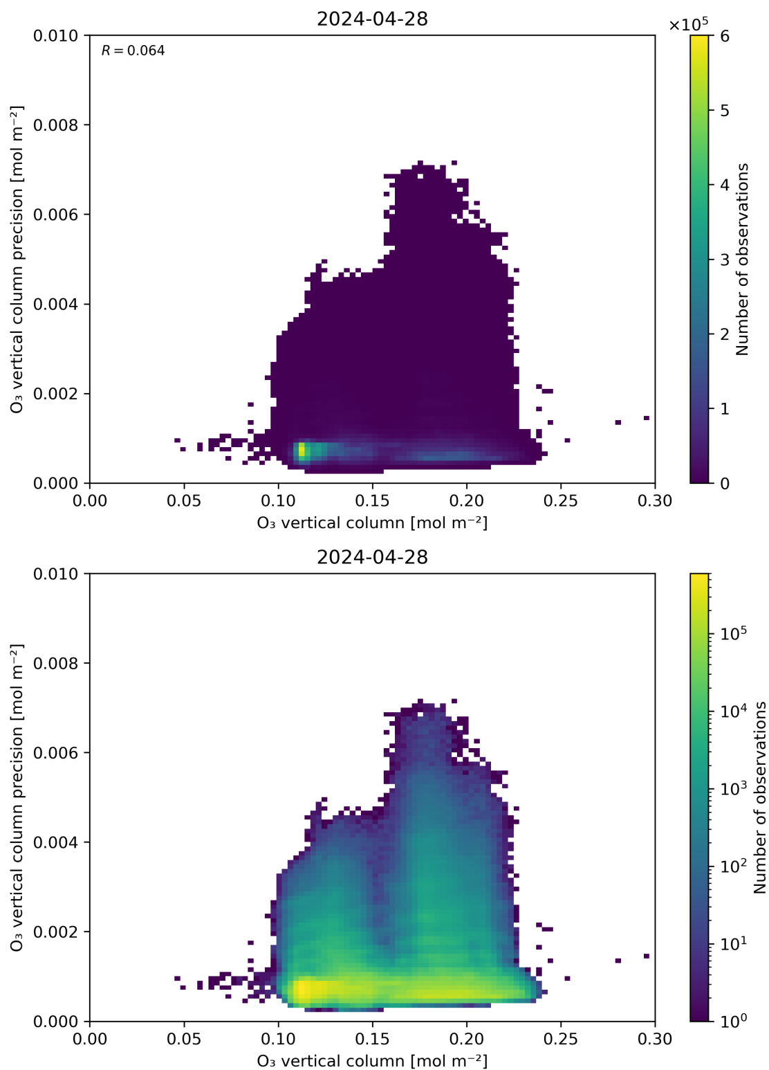
Figure 41: Scatter density plot of “O 3 vertical column” against “O 3 vertical column precision” for 2024-04-27 to 2024-04-29.
