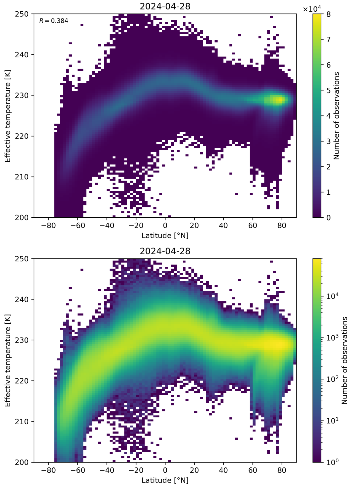
Figure 34: Scatter density plot of “Latitude” against “Effective temperature” for 2024-04-27 to 2024-04-29.
