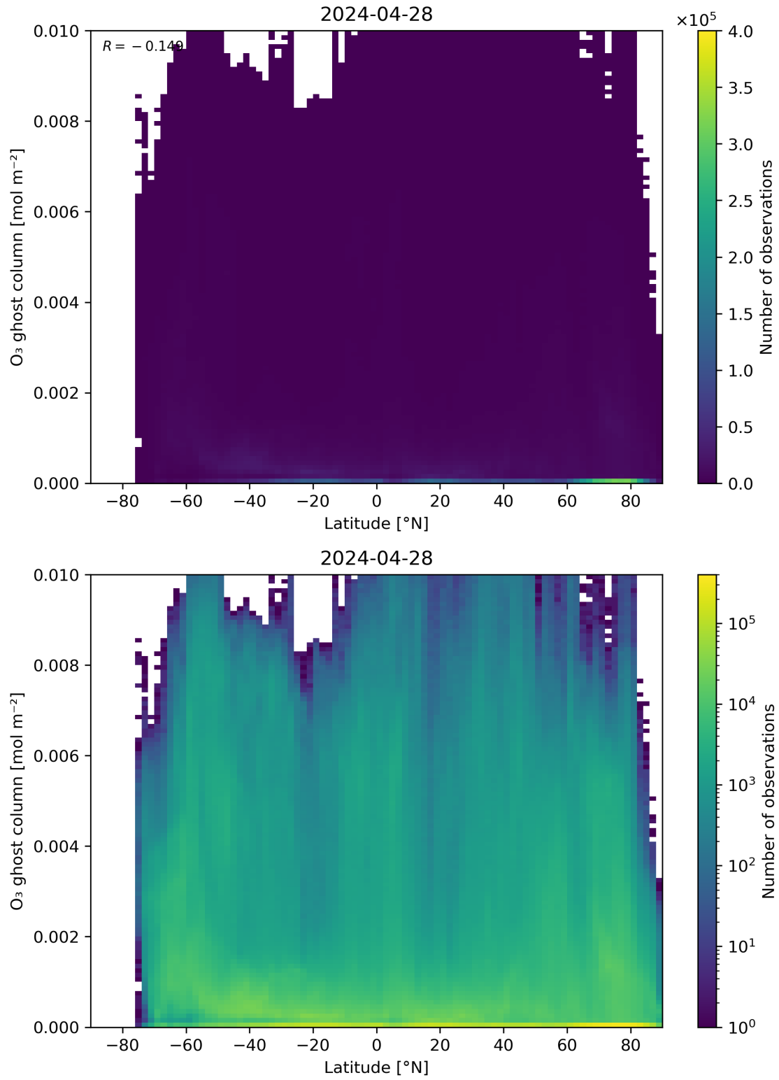
Figure 35: Scatter density plot of “Latitude” against “O 3 ghost column” for 2024-04-27 to 2024-04-29.
