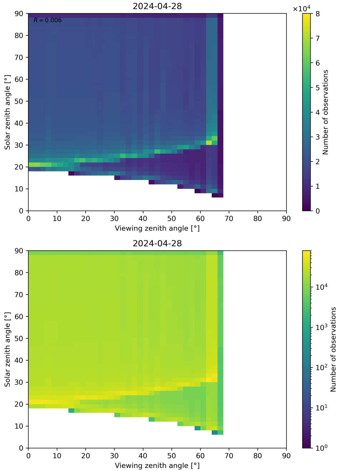
Figure 54: Scatter density plot of “Viewing zenith angle” against “Solar zenith angle” for 2024-04-27 to 2024-04-29.
