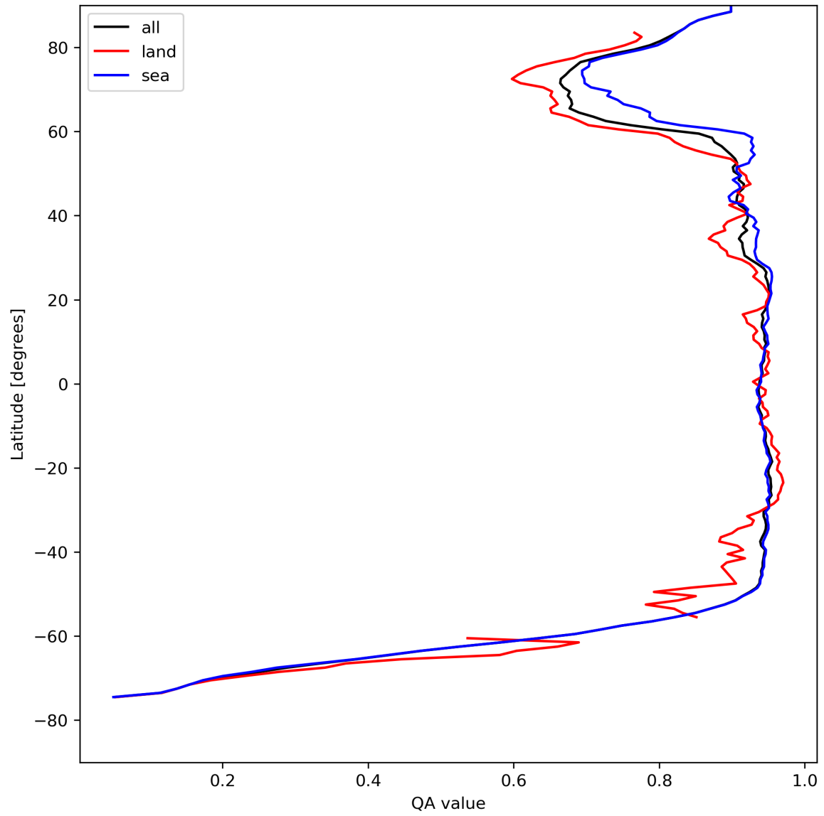
Figure 13: Zonal average of “QA value” for 2024-04-27 to 2024-04-29.
