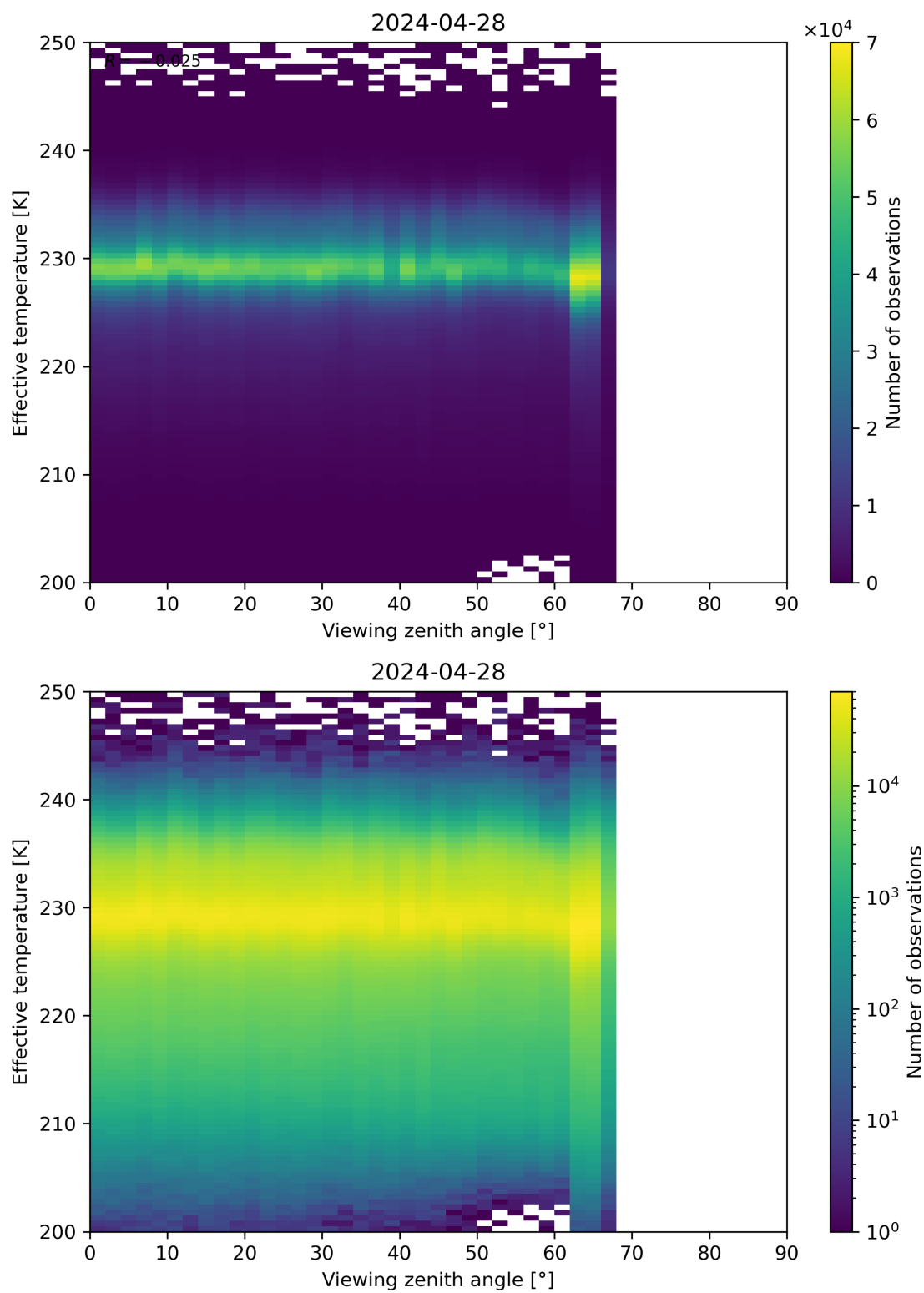
Figure 50: Scatter density plot of “Viewing zenith angle” against “Effective temperature” for 2024-04-27 to 2024-04-29.
