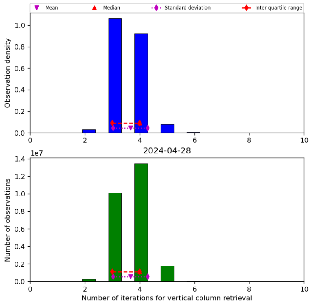
Figure 26: Histogram of “Number of iterations for vertical column retrieval” for 2024-04-27 to 2024-04-29
