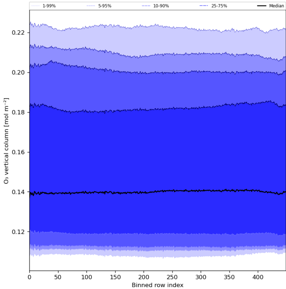
Figure 28: Along track statistics of “O 3 vertical column” for 2024-04-27 to 2024-04-29
