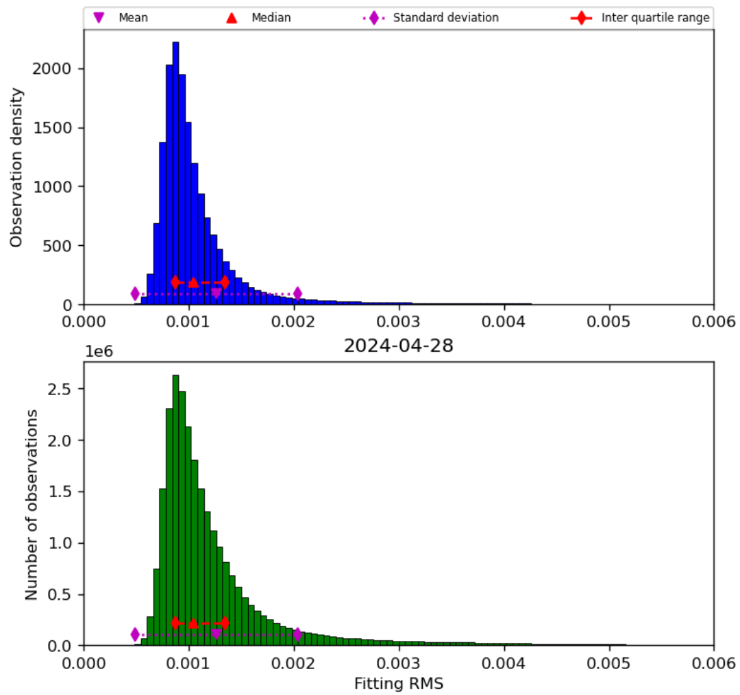
Figure 23: Histogram of “Fitting RMS” for 2024-04-27 to 2024-04-29
