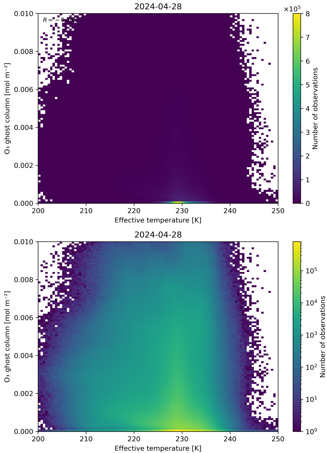
Figure 38: Scatter density plot of “Effective temperature” against “O 3 ghost column” for 2024-04-27 to 2024-04-29.
