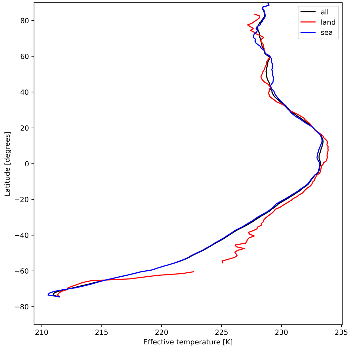
Figure 17: Zonal average of "Effective temperature" for 2024-04-27 to 2024-04-29.
