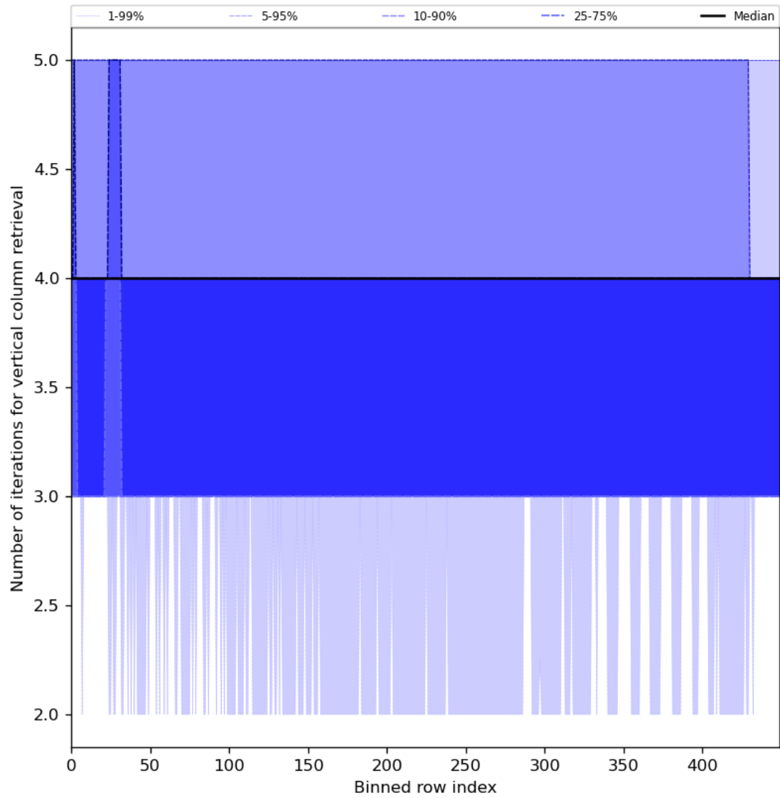
Figure 33: Along track statistics of “Number of iterations for vertical column retrieval” for 2024-04-27 to 2024-04-29
