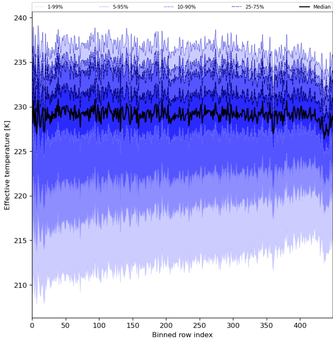
Figure 31: Along track statistics of “Effective temperature” for 2024-04-27 to 2024-04-29
