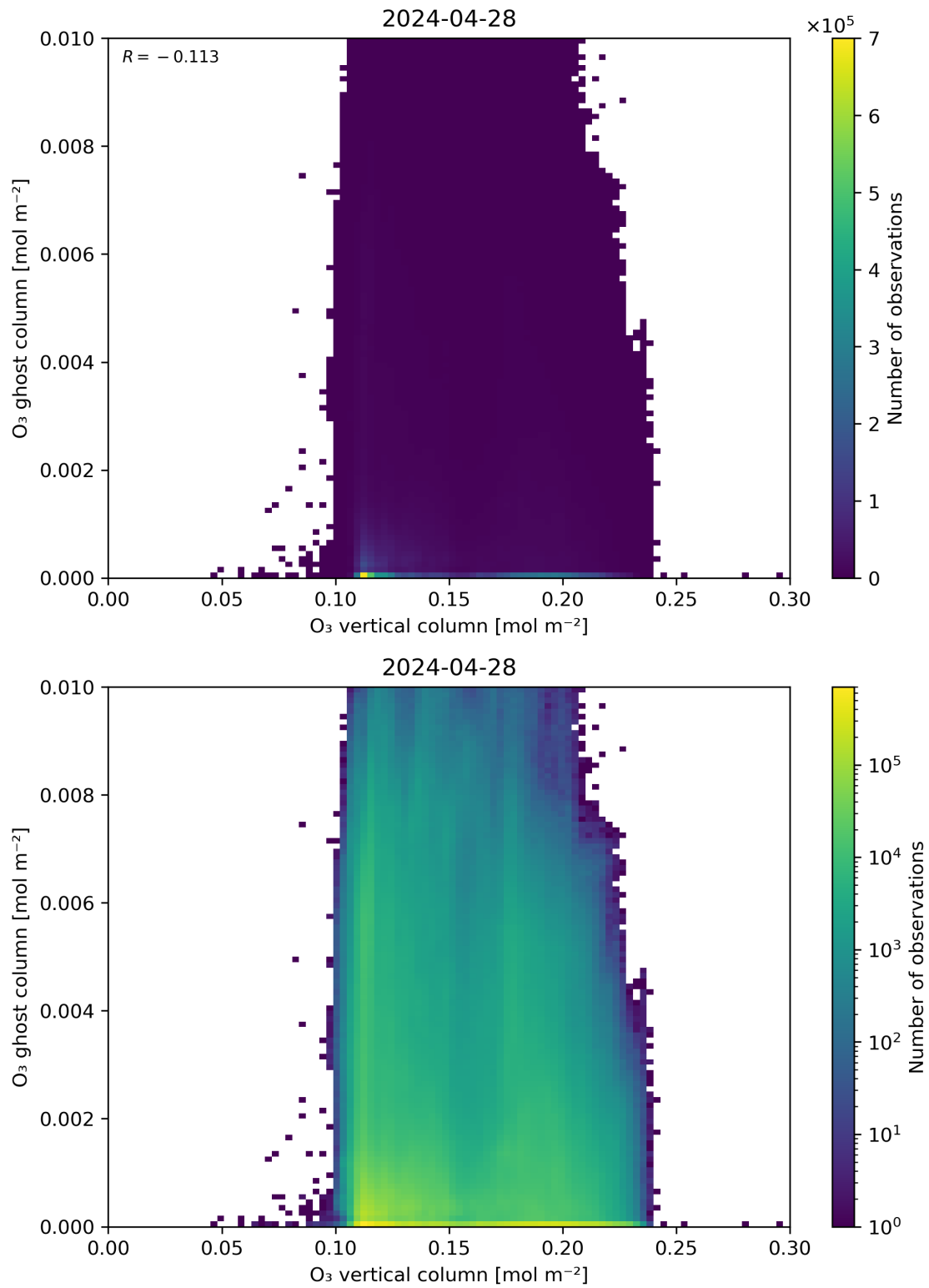
Figure 40: Scatter density plot of “O 3 vertical column” against “O 3 ghost column” for 2024-04-27 to 2024-04-29.
