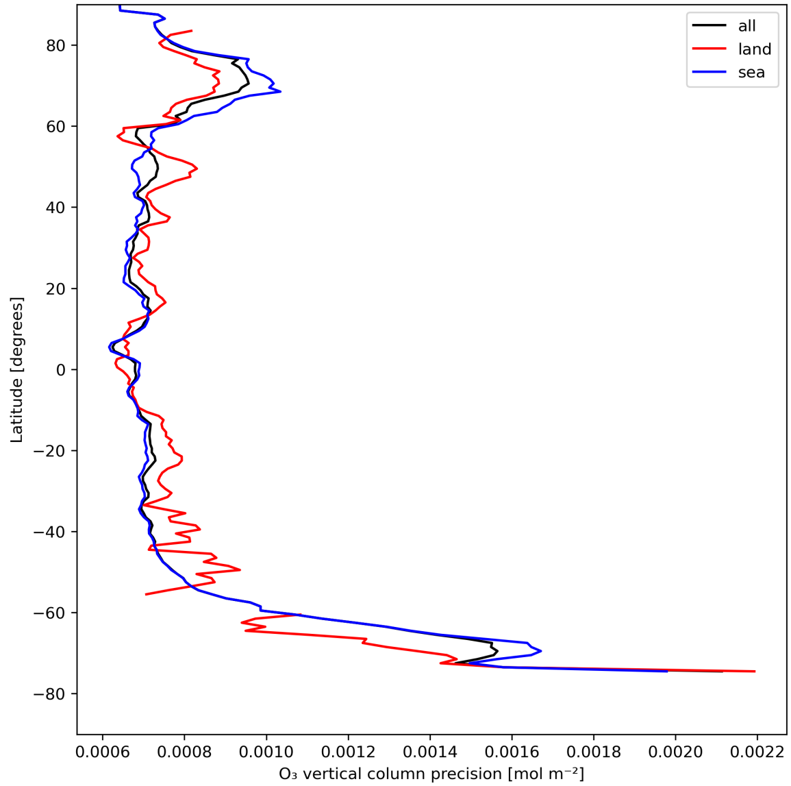
Figure 15: Zonal average of "O 3 vertical column precision" for 2024-04-27 to 2024-04-29.
