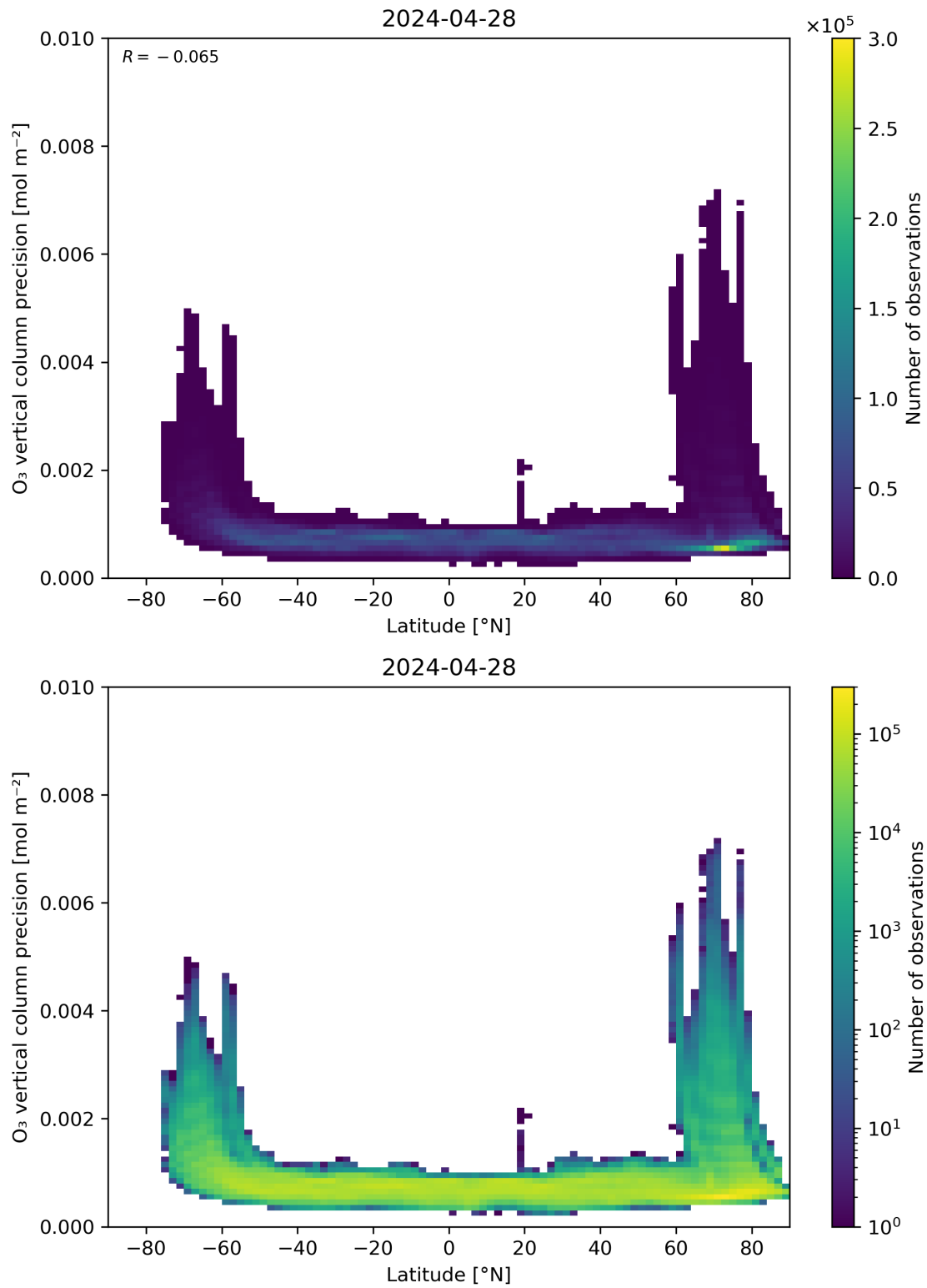
Figure 37: Scatter density plot of “Latitude” against “O 3 vertical column precision” for 2024-04-27 to 2024-04-29.
