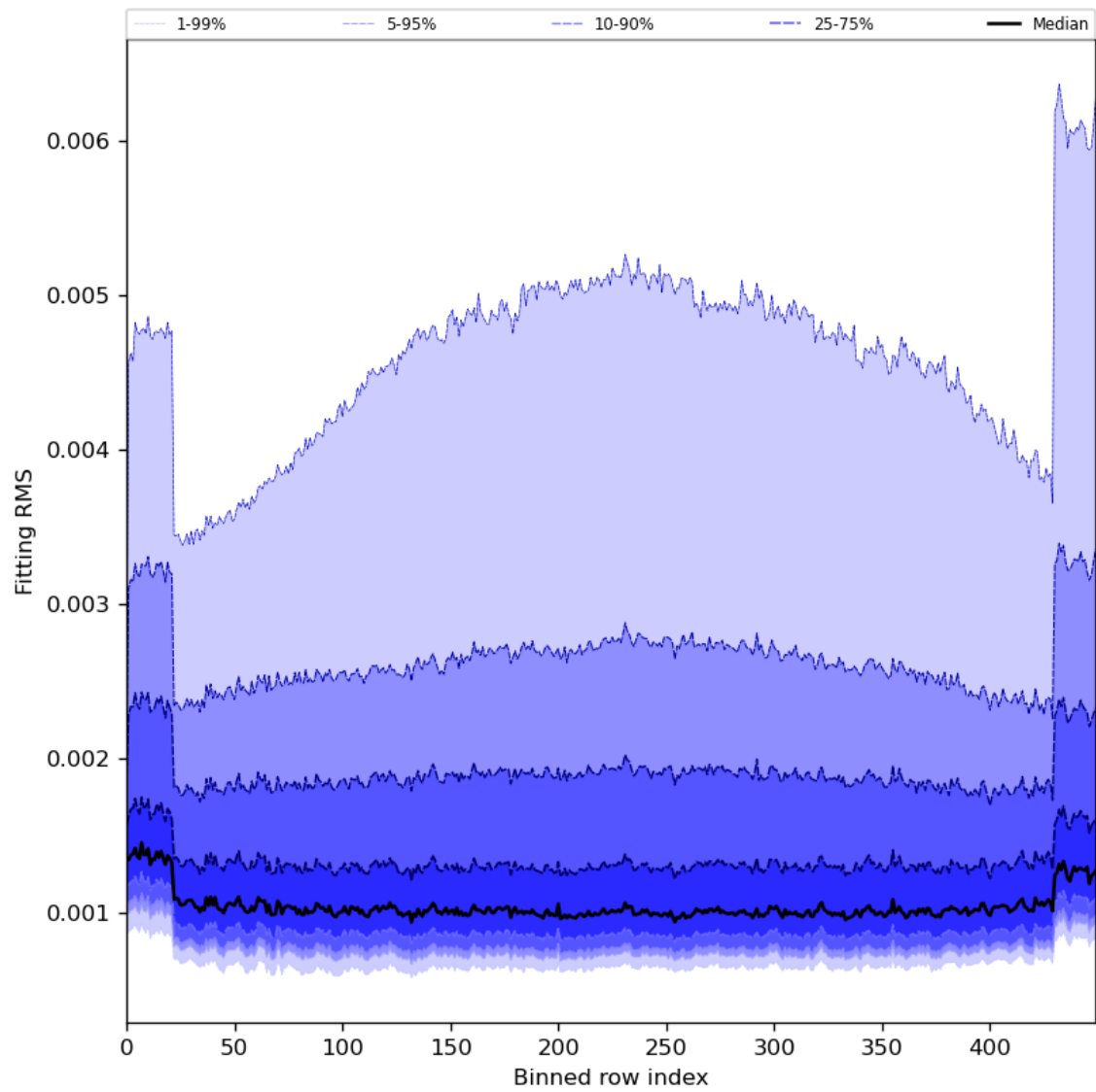
Figure 30: Along track statistics of “Fitting RMS” for 2024-04-27 to 2024-04-29
