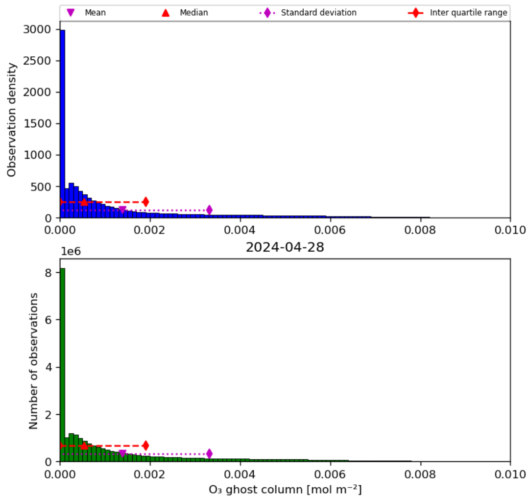
Figure 25: Histogram of “O 3 ghost column” for 2024-04-27 to 2024-04-29
