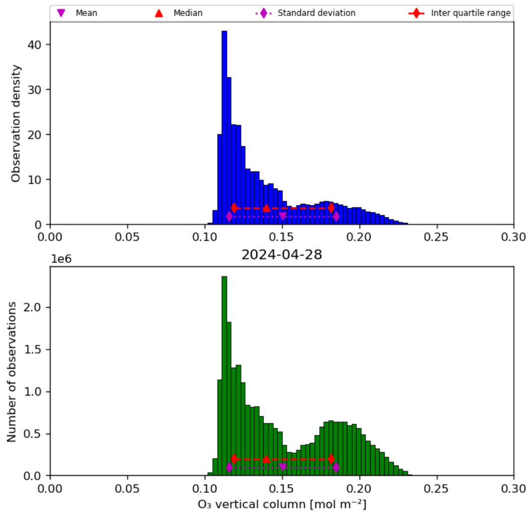
Figure 21: Histogram of “O 3 vertical column” for 2024-04-27 to 2024-04-29
