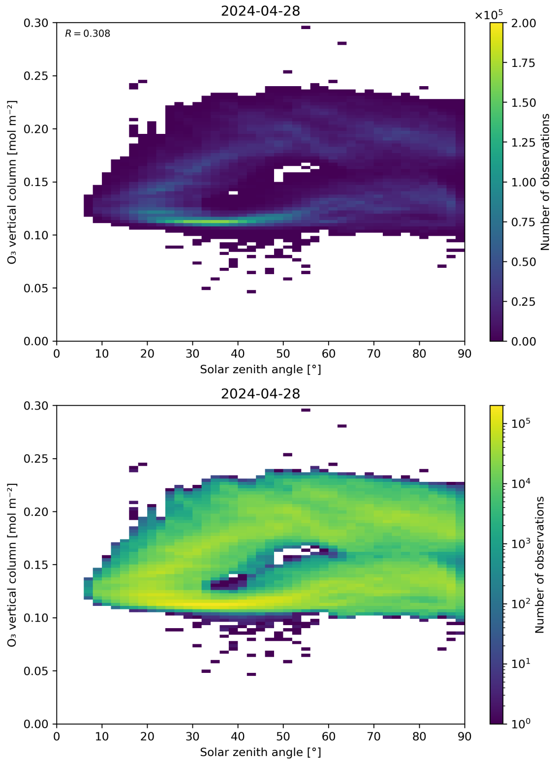
Figure 47: Scatter density plot of “Solar zenith angle” against “O 3 vertical column” for 2024-04-27 to 2024-04-29.
