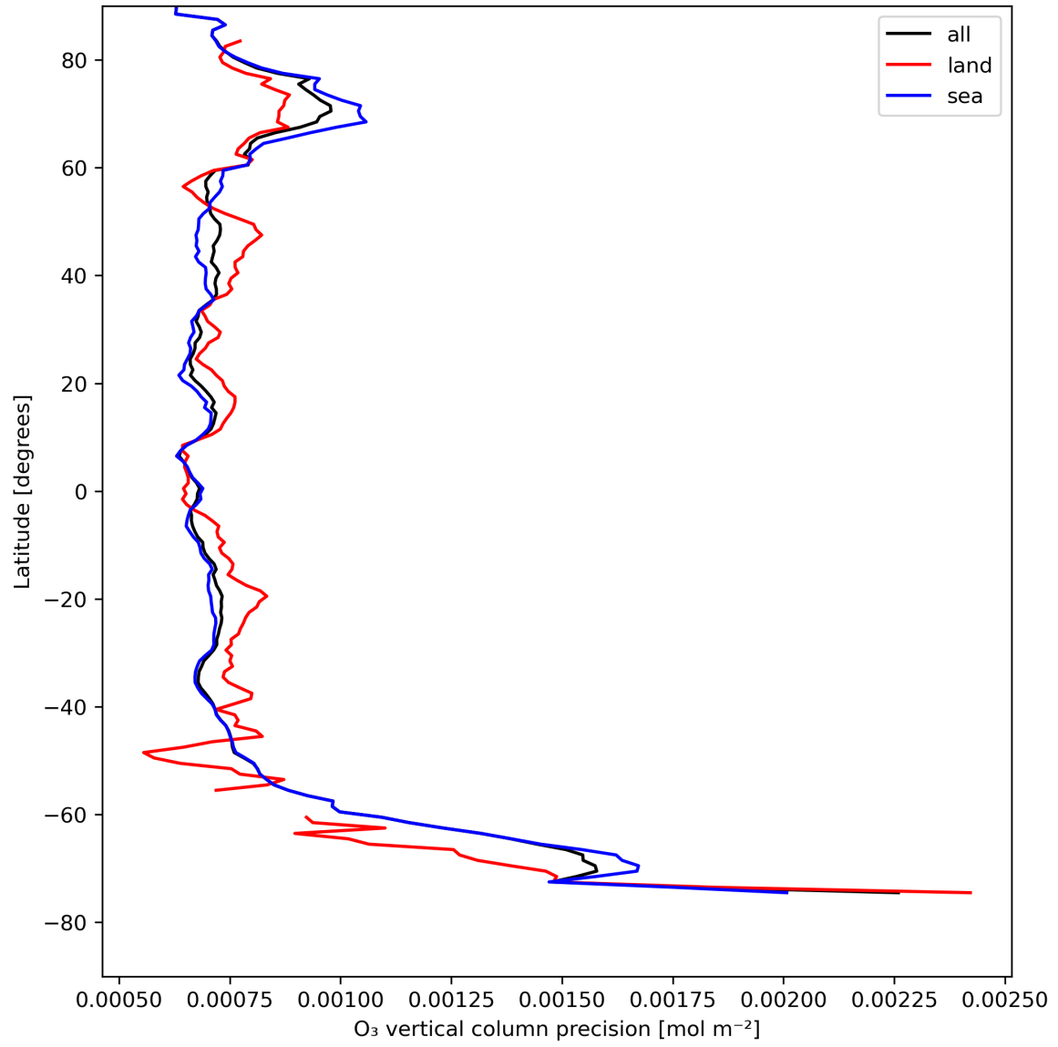
Figure 15: Zonal average of “O 3 vertical column precision” for 2024-04-28 to 2024-04-30.
