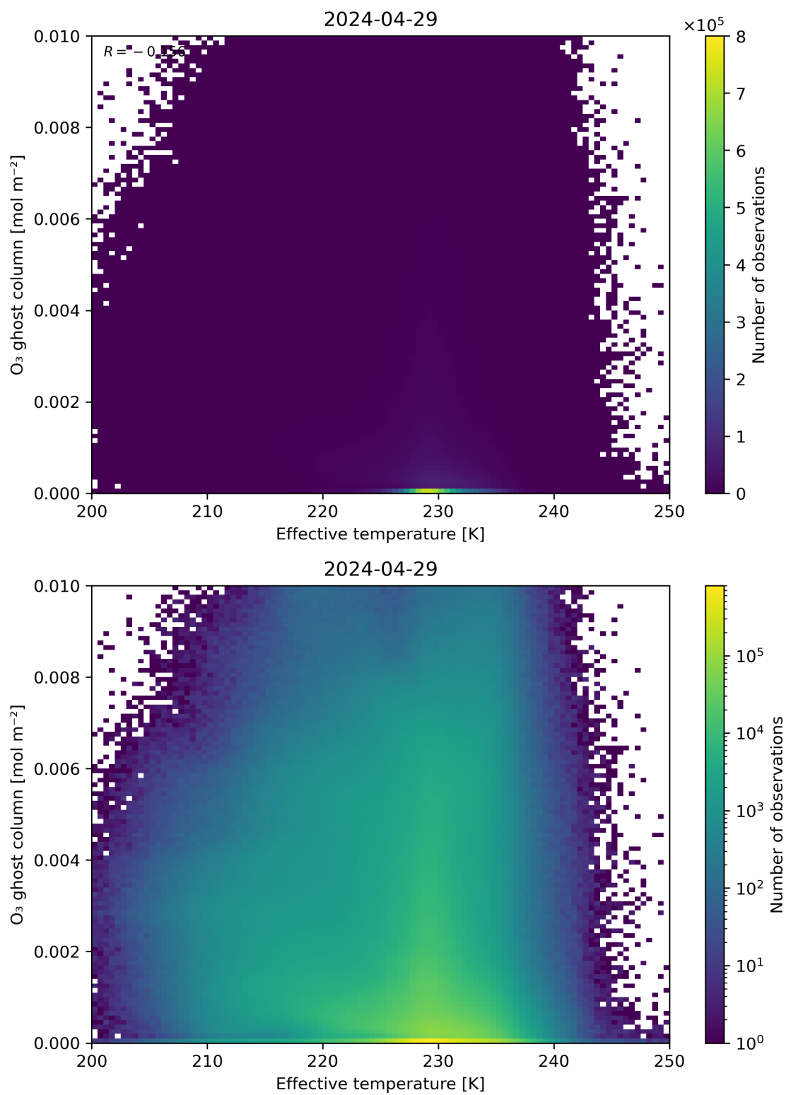
Figure 38: Scatter density plot of “Effective temperature” against “O 3 ghost column” for 2024-04-28 to 2024-04-30.
