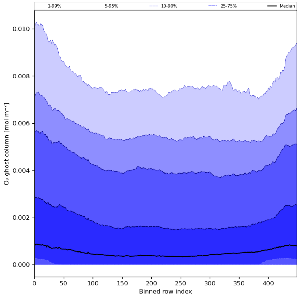
Figure 32: Along track statistics of “O 3 ghost column” for 2024-04-28 to 2024-04-30
