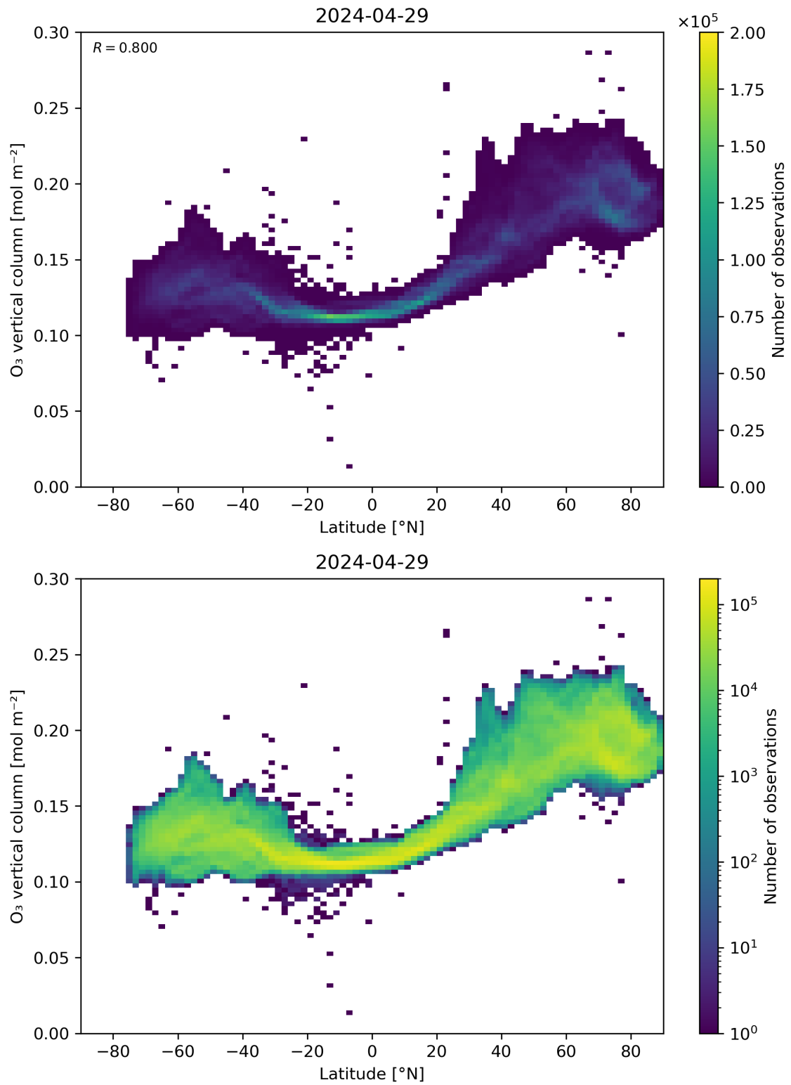
Figure 36: Scatter density plot of “Latitude” against “O 3 vertical column” for 2024-04-28 to 2024-04-30.
