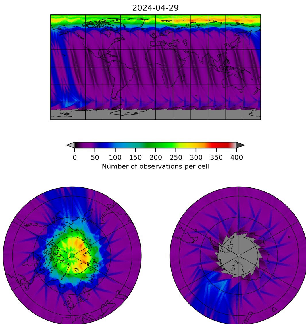
Figure 12: Map of the number of observations for 2024-04-28 to 2024-04-30
