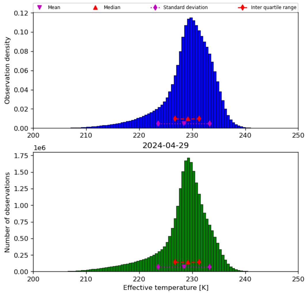
Figure 24: Histogram of “Effective temperature” for 2024-04-28 to 2024-04-30
