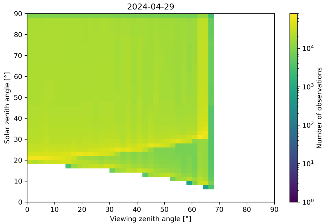
Figure 54: Scatter density plot of “Viewing zenith angle” against “Solar zenith angle” for 2024-04-28 to 2024-04-30.
