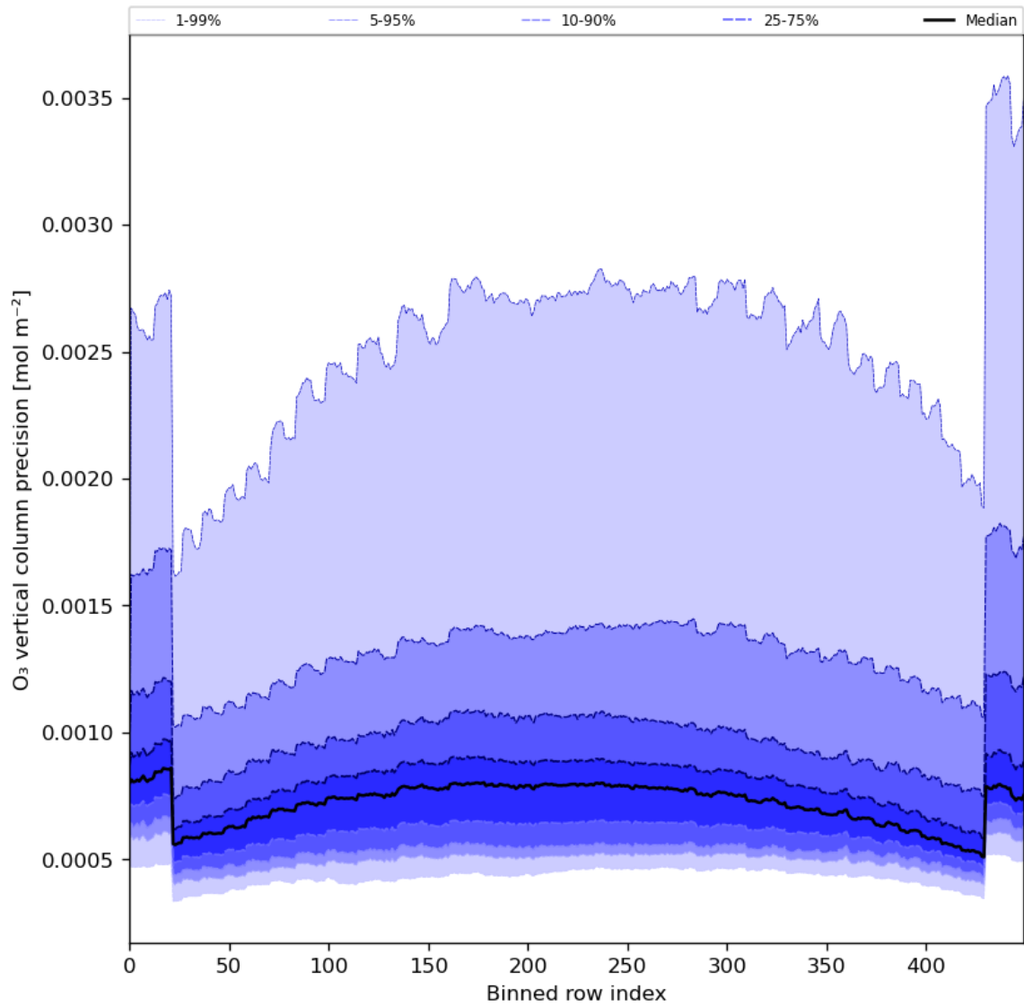
Figure 29: Along track statistics of “O 3 vertical column precision” for 2024-04-28 to 2024-04-30
