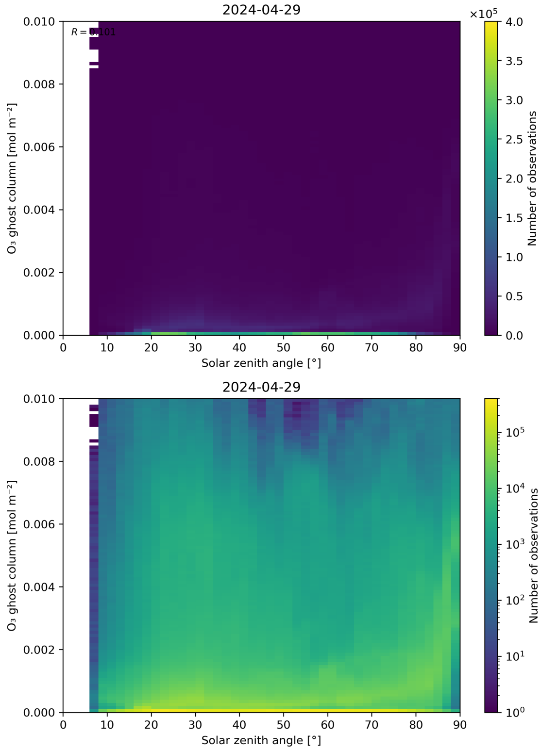
Figure 46: Scatter density plot of “Solar zenith angle” against “O 3 ghost column” for 2024-04-28 to 2024-04-30.
