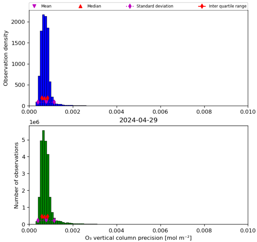
Figure 22: Histogram of “O 3 vertical column precision” for 2024-04-28 to 2024-04-30
