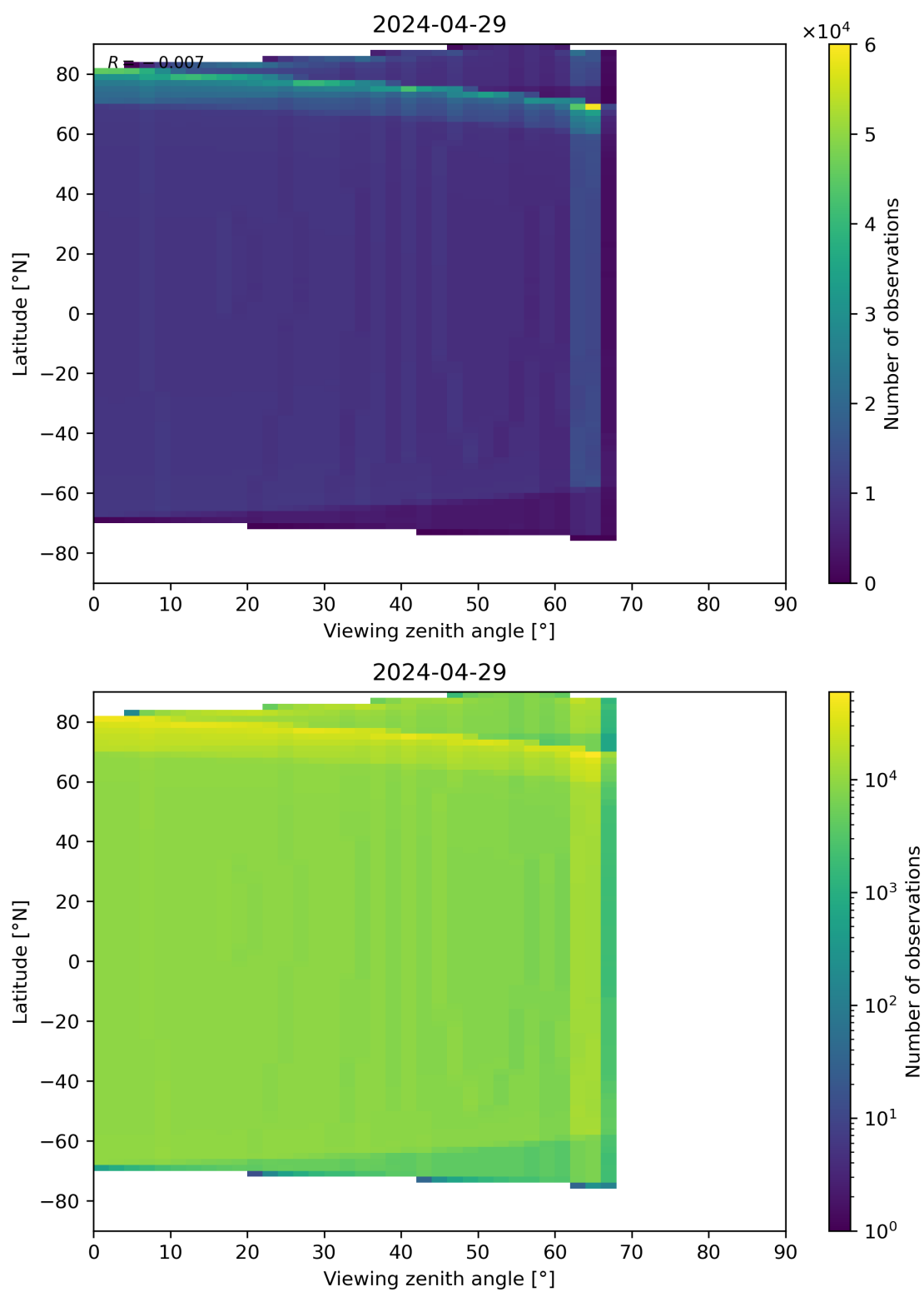
Figure 49: Scatter density plot of “Viewing zenith angle” against “Latitude” for 2024-04-28 to 2024-04-30.
