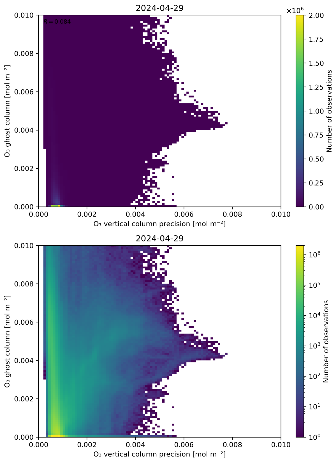
Figure 43: Scatter density plot of “ \text{O}_3 vertical column precision” against “ \text{O}_3 ghost column” for 2024-04-28 to 2024-04-30.
