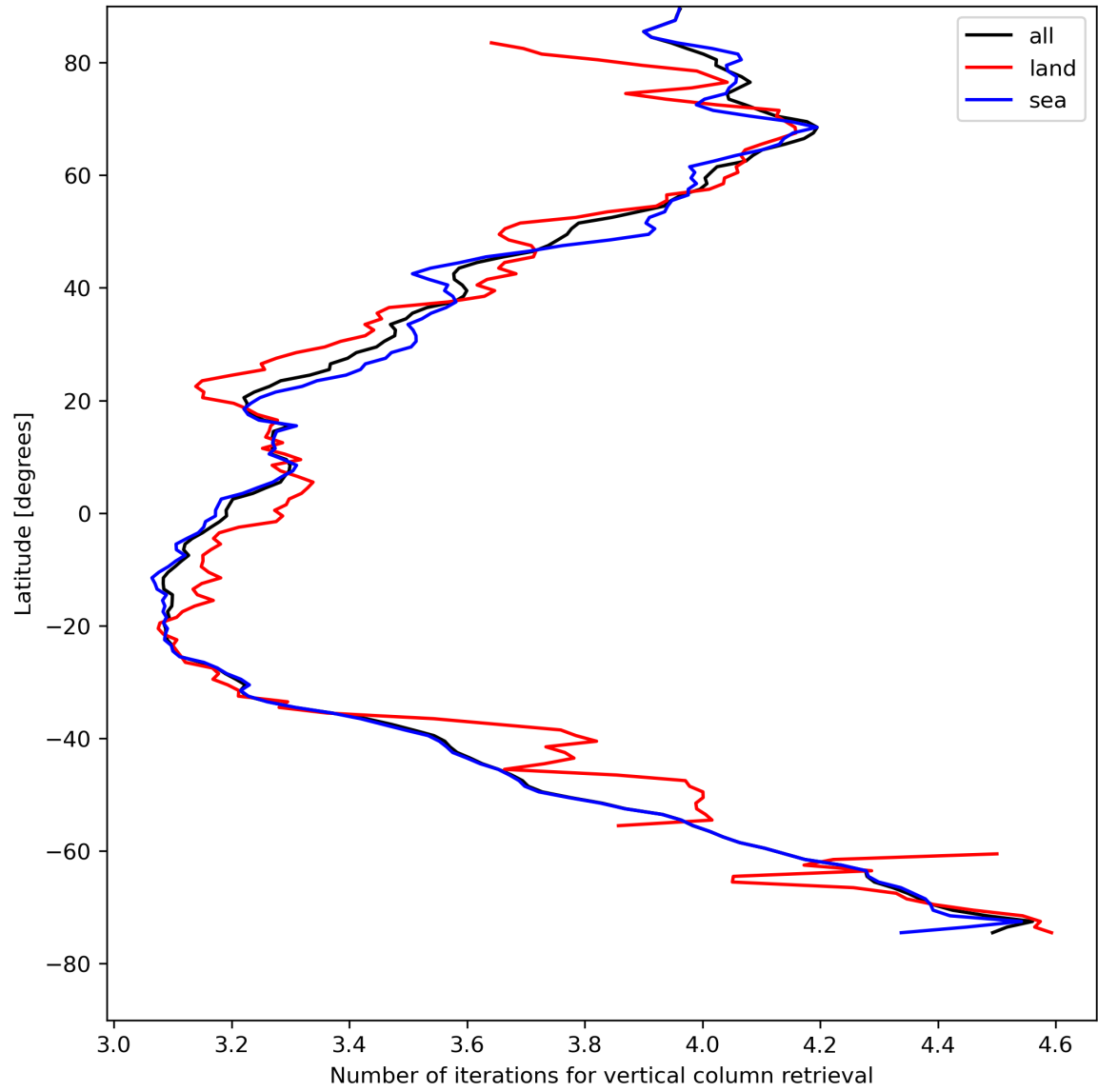
Figure 19: Zonal average of “Number of iterations for vertical column retrieval” for 2024-04-28 to 2024-04-30.
