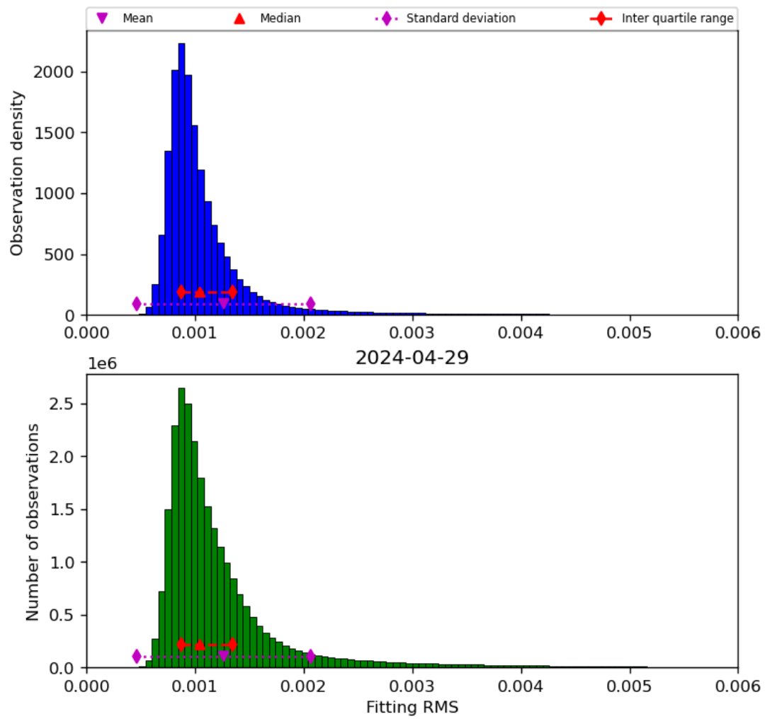
Figure 23: Histogram of “Fitting RMS” for 2024-04-28 to 2024-04-30
