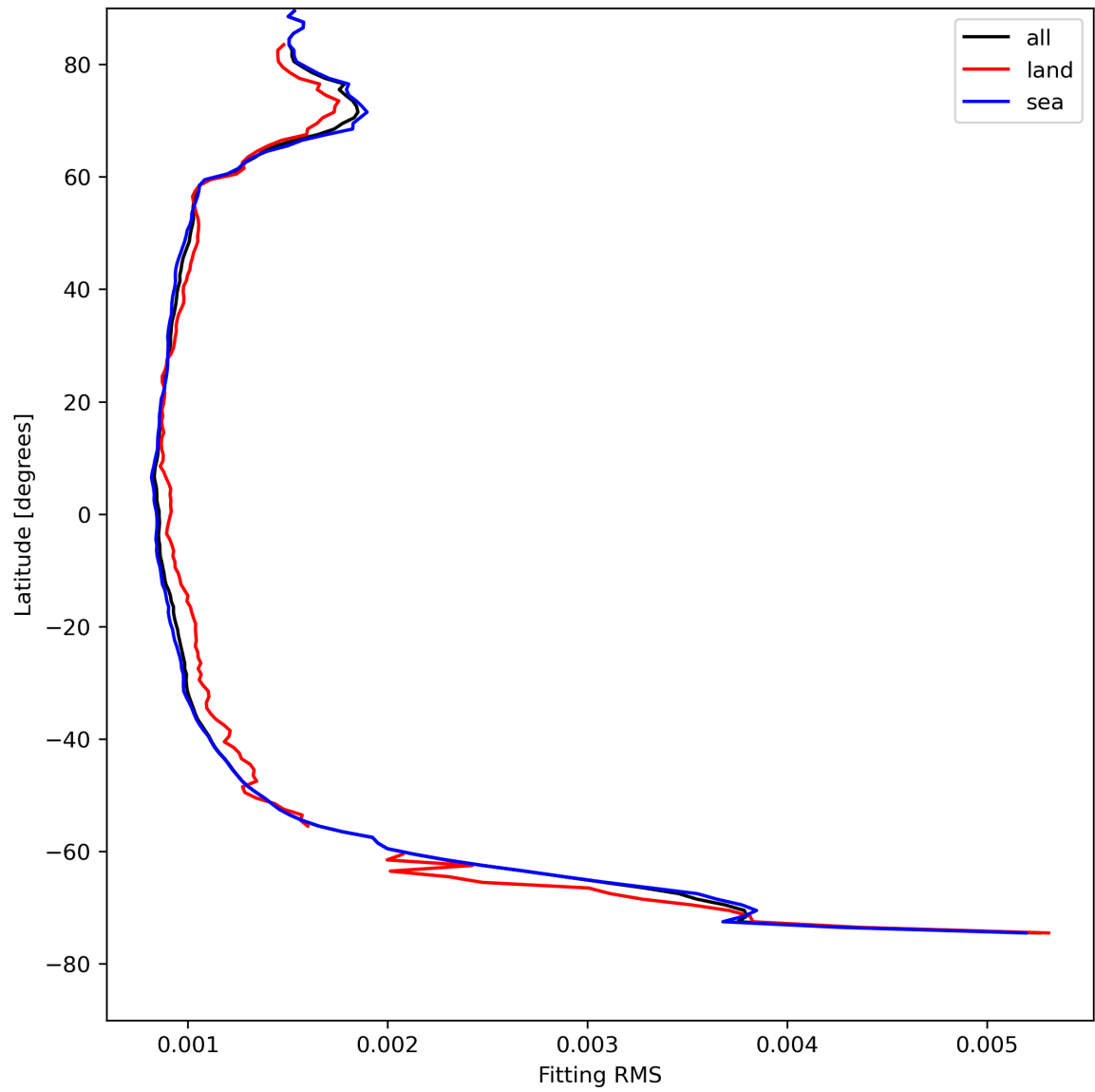
Figure 16: Zonal average of “Fitting RMS” for 2024-04-28 to 2024-04-30.
