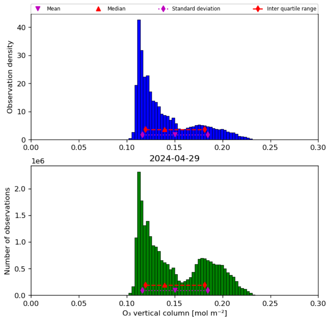
Figure 21: Histogram of “O 3 vertical column” for 2024-04-28 to 2024-04-30
