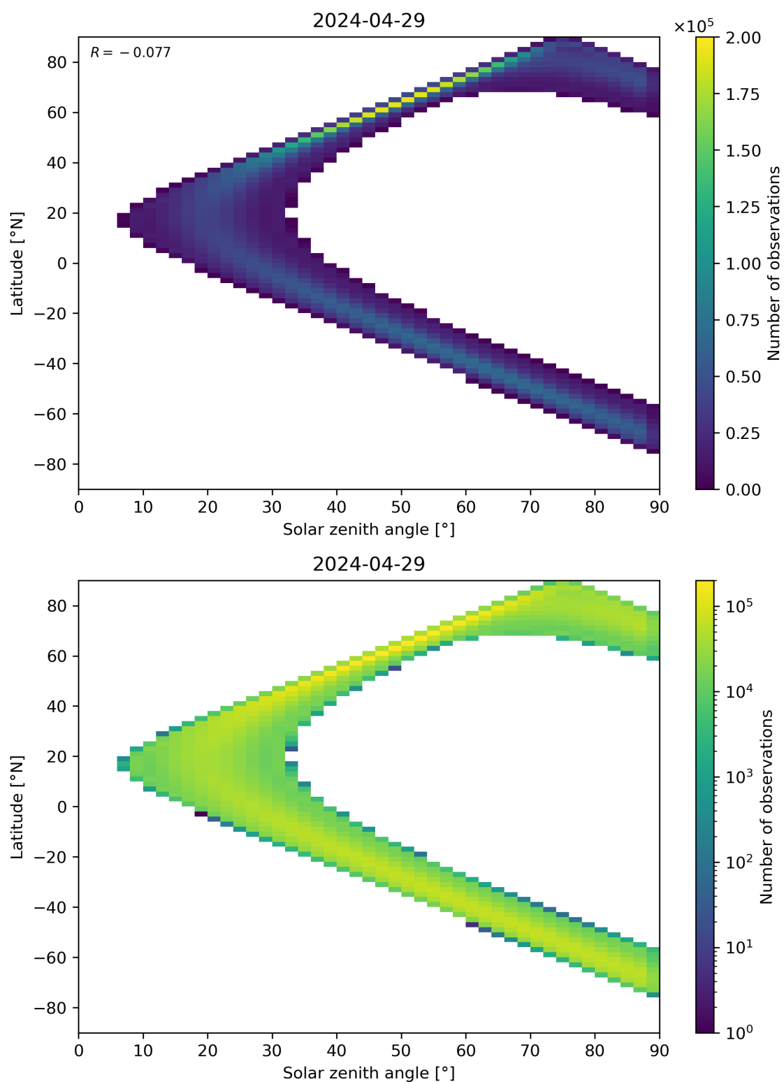
Figure 44: Scatter density plot of “Solar zenith angle” against “Latitude” for 2024-04-28 to 2024-04-30.
