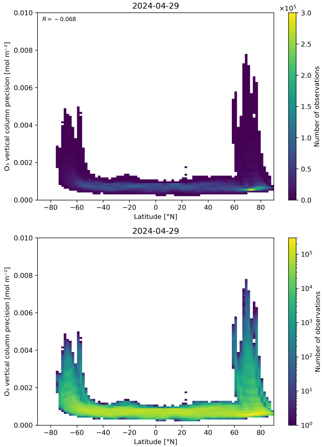
Figure 37: Scatter density plot of “Latitude” against “O 3 vertical column precision” for 2024-04-28 to 2024-04-30.
