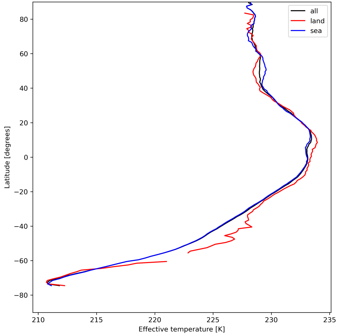
Figure 17: Zonal average of “Effective temperature” for 2024-04-28 to 2024-04-30.
