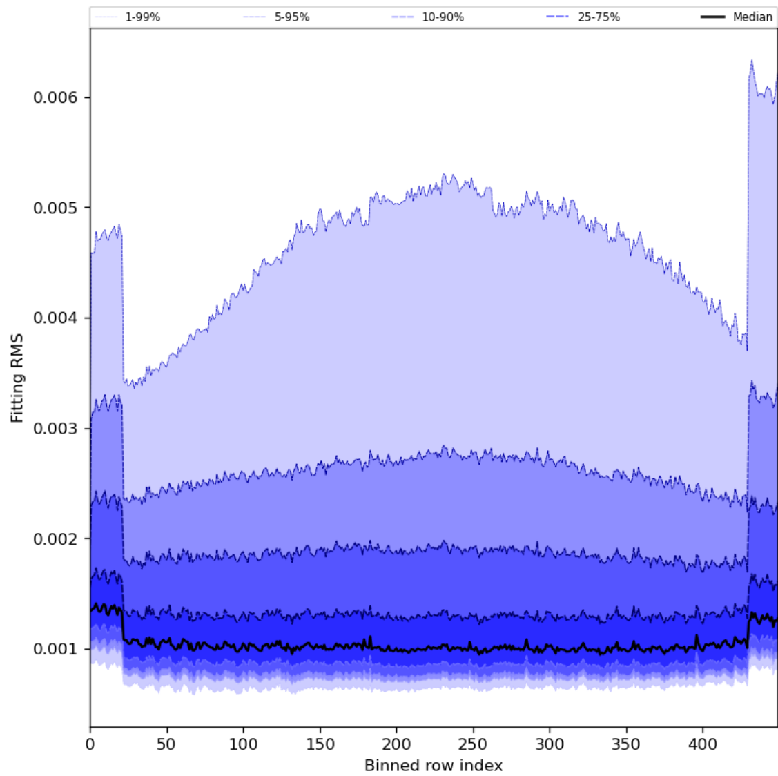
Figure 30: Along track statistics of “Fitting RMS” for 2024-04-28 to 2024-04-30
