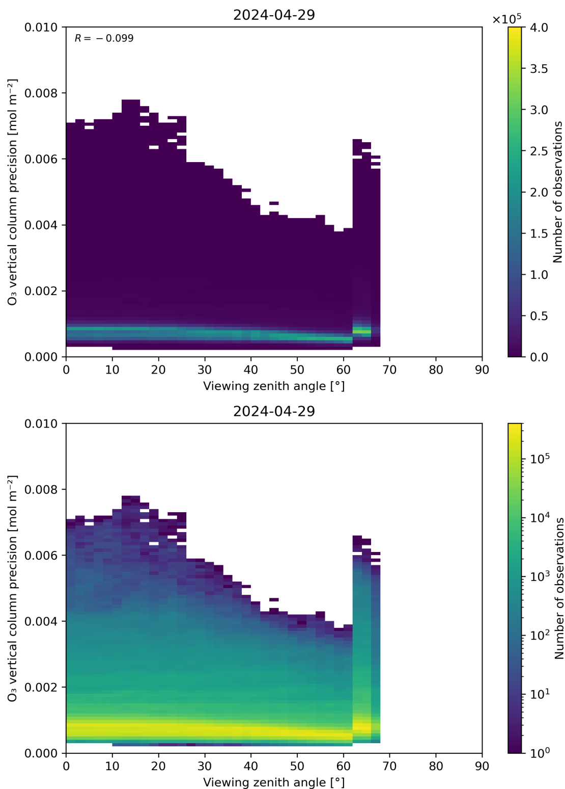
Figure 53: Scatter density plot of “Viewing zenith angle” against “O 3 vertical column precision” for 2024-04-28 to 2024-04-30.
