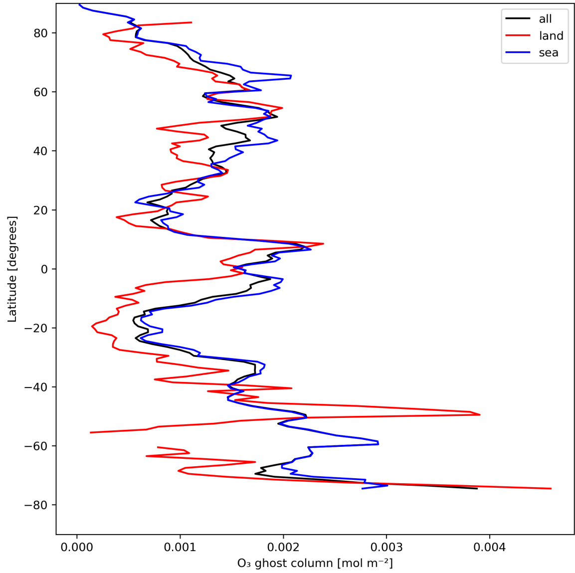
Figure 18: Zonal average of "O 3 ghost column" for 2024-04-28 to 2024-04-30.
