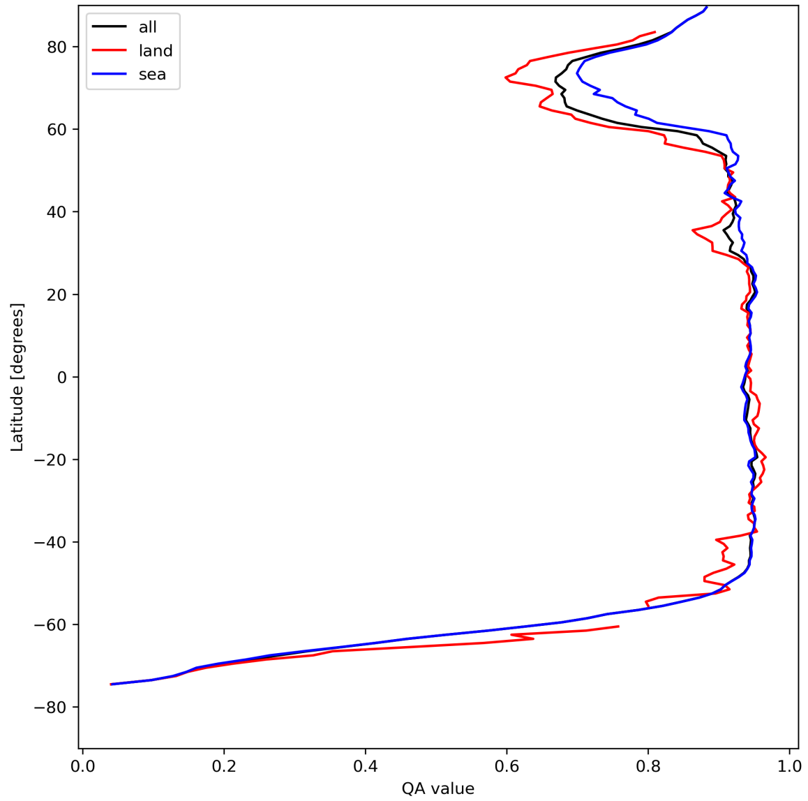
Figure 13: Zonal average of “QA value” for 2024-04-28 to 2024-04-30.
