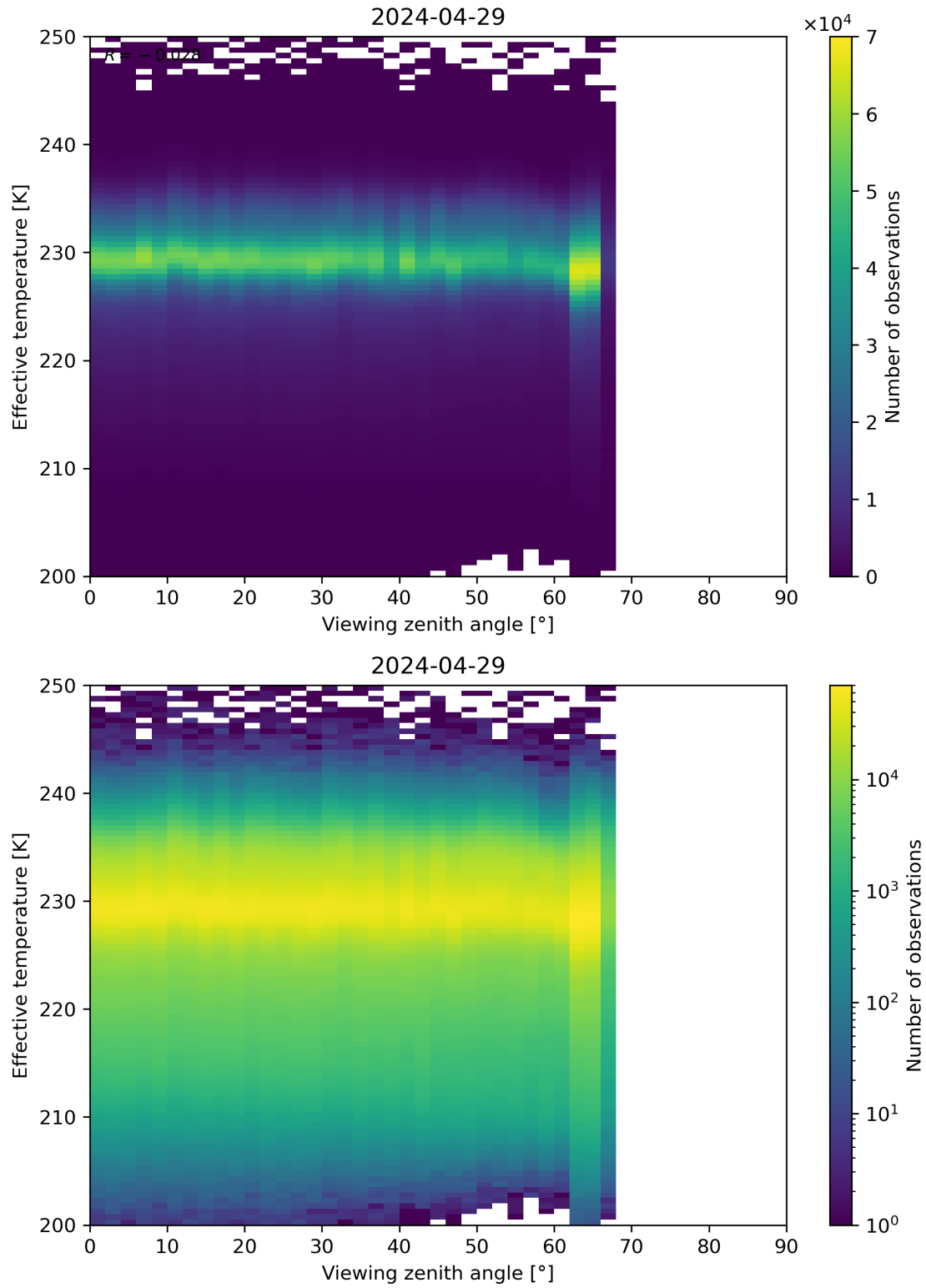
Figure 50: Scatter density plot of “Viewing zenith angle” against “Effective temperature” for 2024-04-28 to 2024-04-30.
