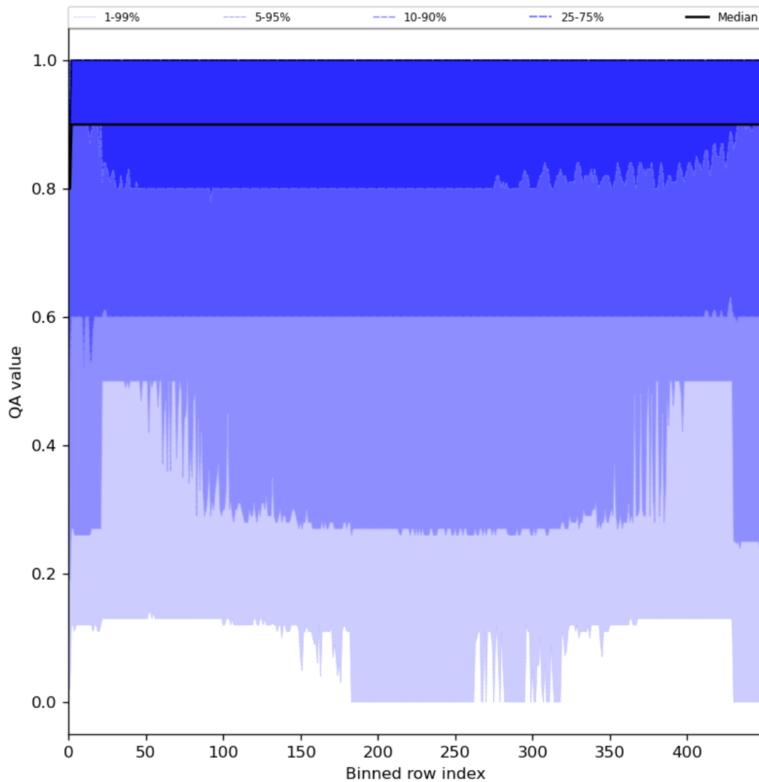
Figure 27: Along track statistics of “QA value” for 2024-04-28 to 2024-04-30
