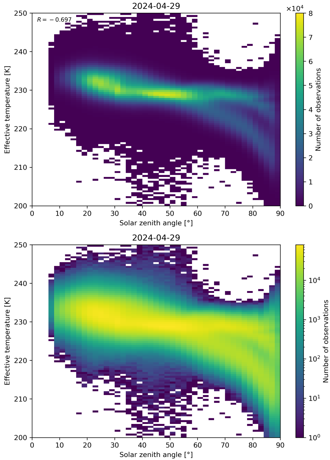
Figure 45: Scatter density plot of “Solar zenith angle” against “Effective temperature” for 2024-04-28 to 2024-04-30.
