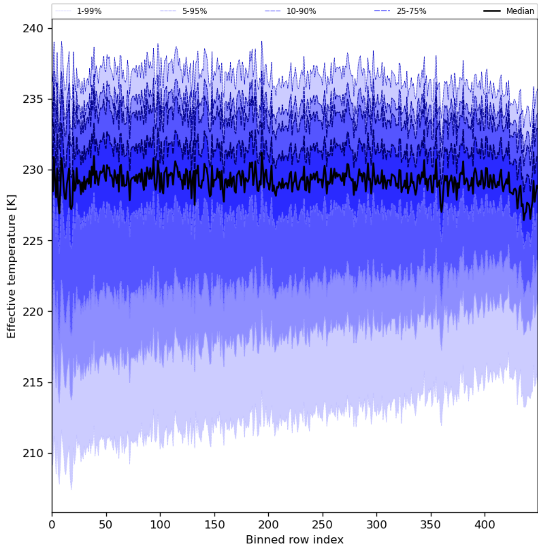
Figure 31: Along track statistics of “Effective temperature” for 2024-04-28 to 2024-04-30
