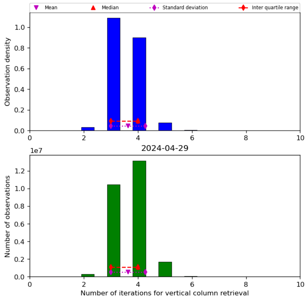
Figure 26: Histogram of “Number of iterations for vertical column retrieval” for 2024-04-28 to 2024-04-30
