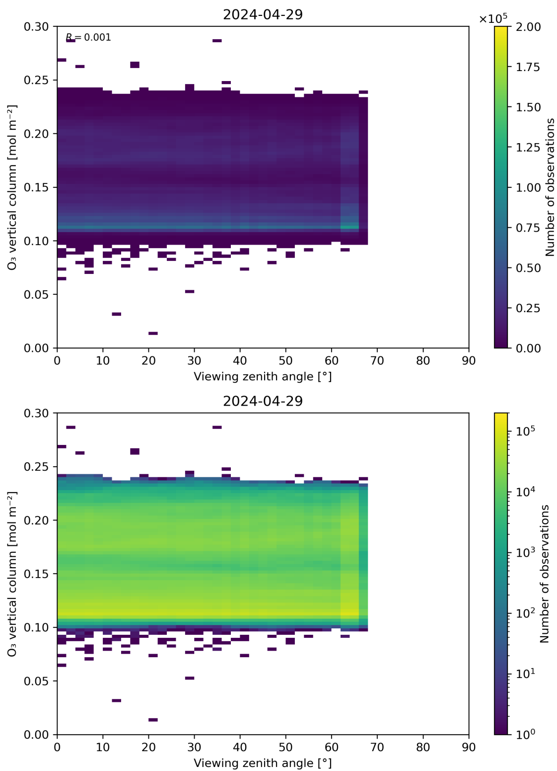
Figure 52: Scatter density plot of “Viewing zenith angle” against “O 3 vertical column” for 2024-04-28 to 2024-04-30.
