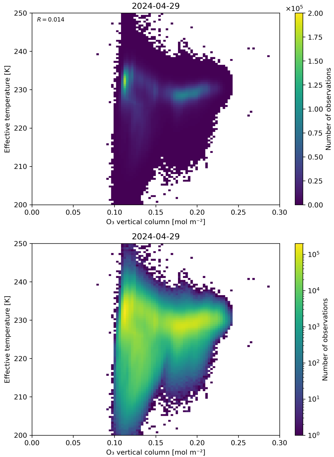
Figure 39: Scatter density plot of “O 3 vertical column” against “Effective temperature” for 2024-04-28 to 2024-04-30.
