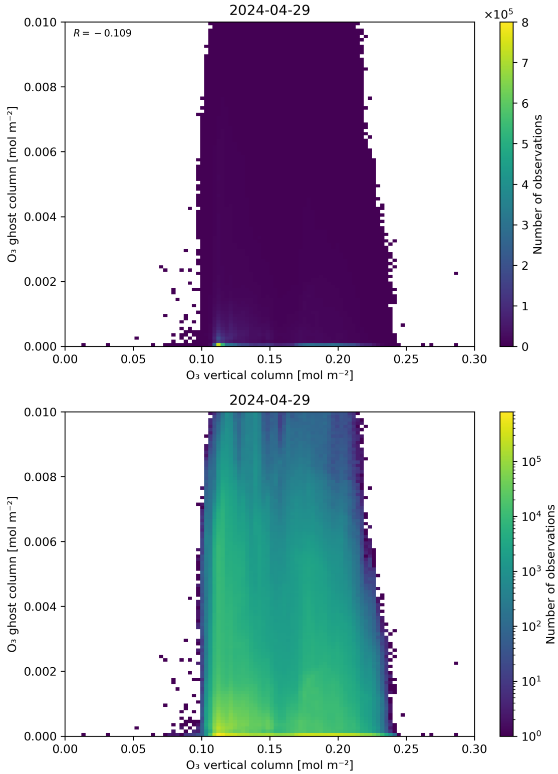
Figure 40: Scatter density plot of “O 3 vertical column” against “O 3 ghost column” for 2024-04-28 to 2024-04-30.
