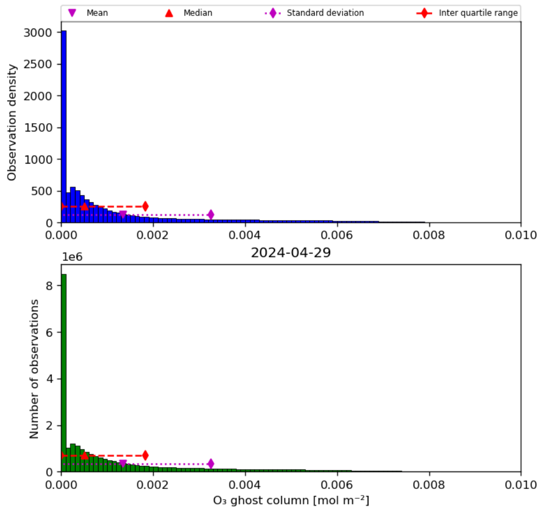
Figure 25: Histogram of “O 3 ghost column” for 2024-04-28 to 2024-04-30
