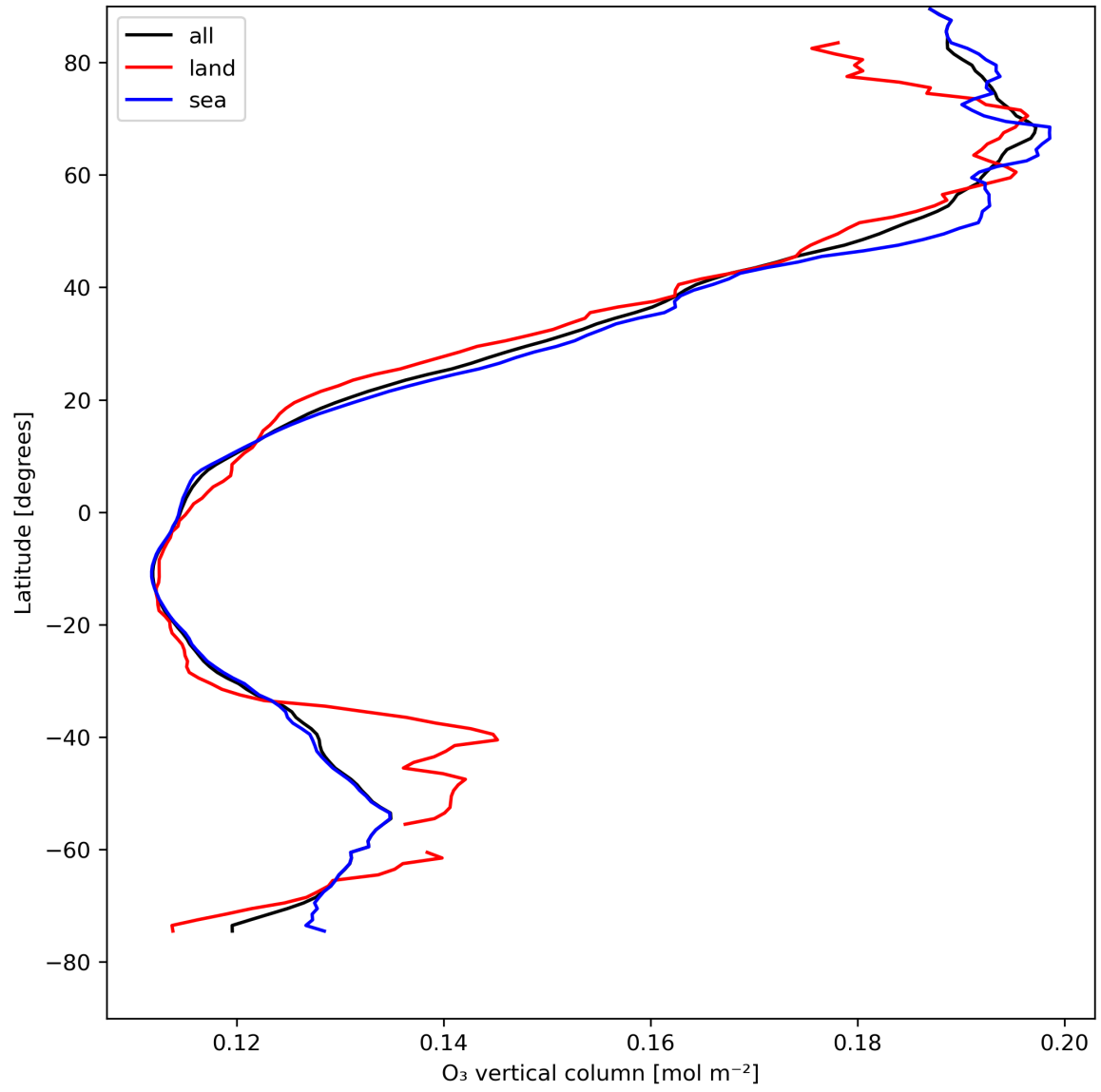
Figure 14: Zonal average of “O 3 vertical column” for 2024-04-28 to 2024-04-30.
