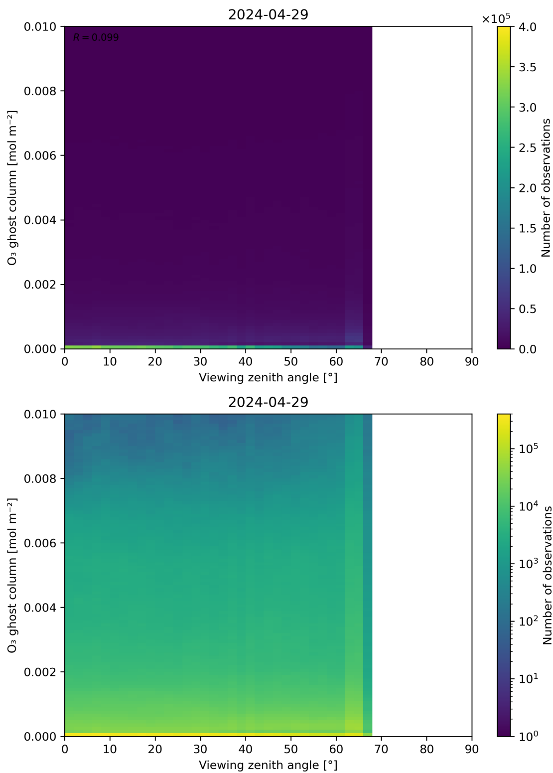
Figure 51: Scatter density plot of “Viewing zenith angle” against “O 3 ghost column” for 2024-04-28 to 2024-04-30.
