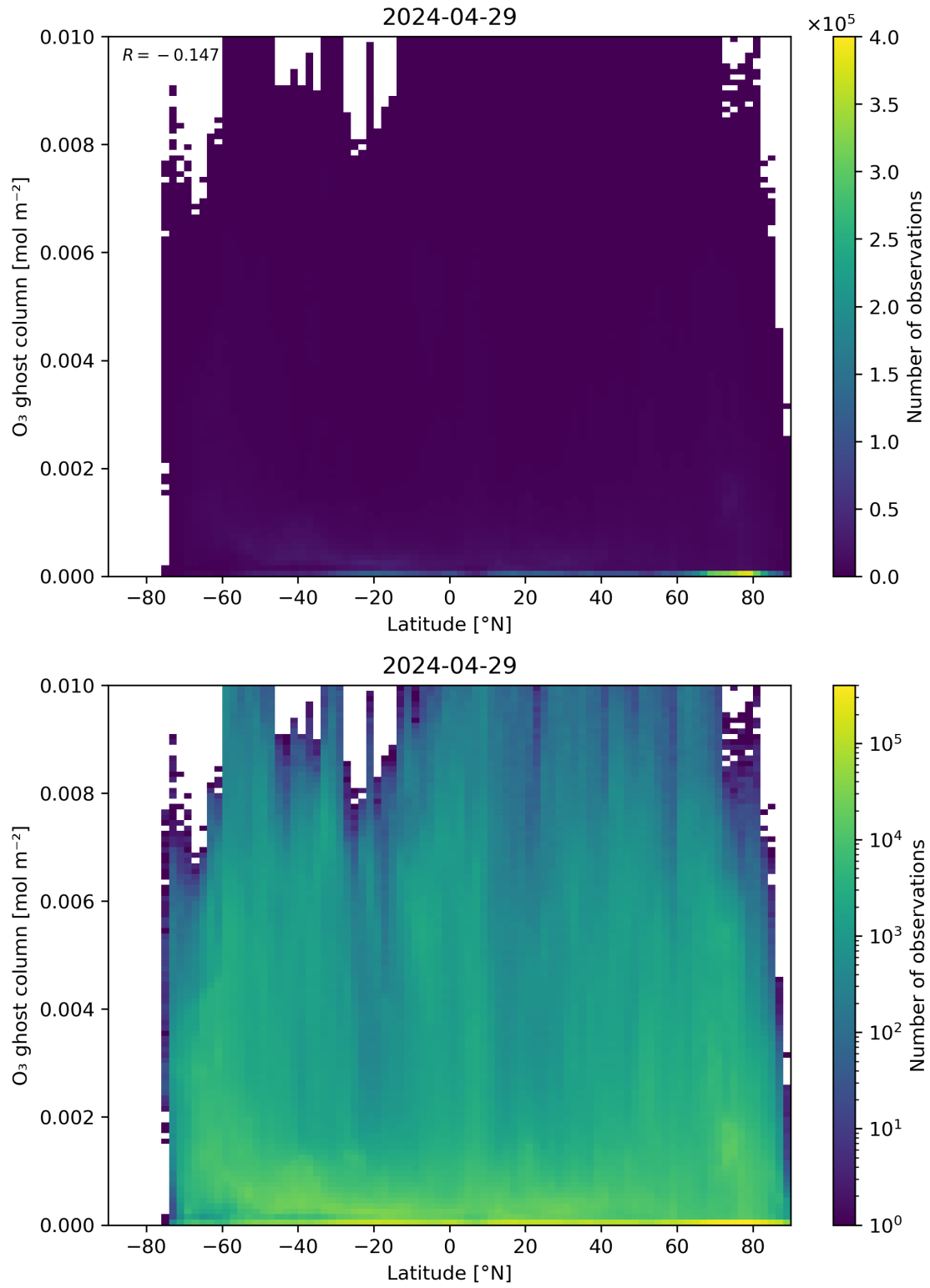
Figure 35: Scatter density plot of “Latitude” against “O 3 ghost column” for 2024-04-28 to 2024-04-30.
