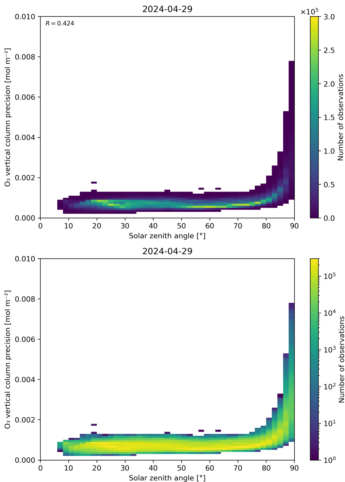
Figure 48: Scatter density plot of “Solar zenith angle” against “O 3 vertical column precision” for 2024-04-28 to 2024-04-30.
