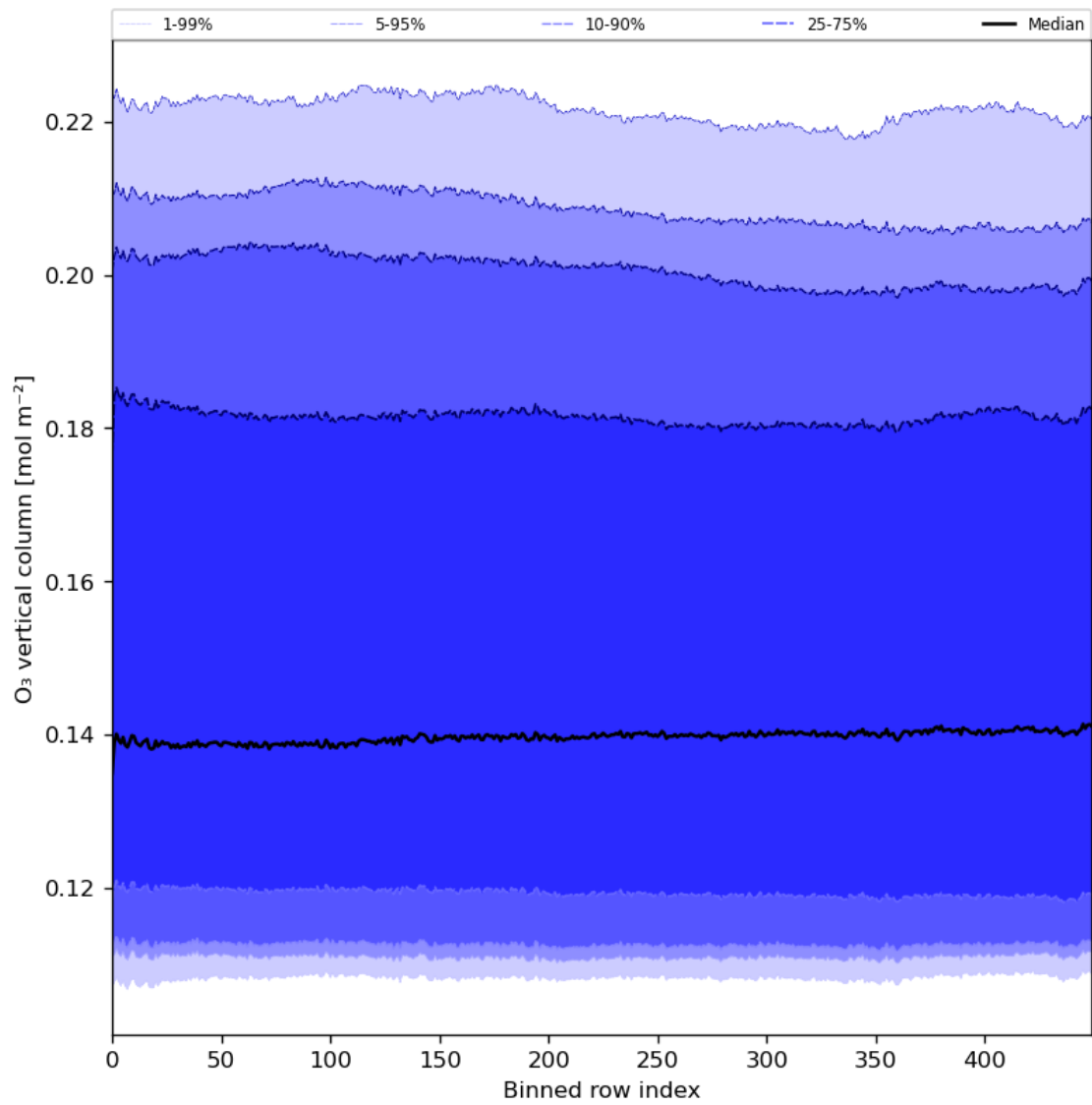
Figure 28: Along track statistics of “O 3 vertical column” for 2024-04-28 to 2024-04-30
