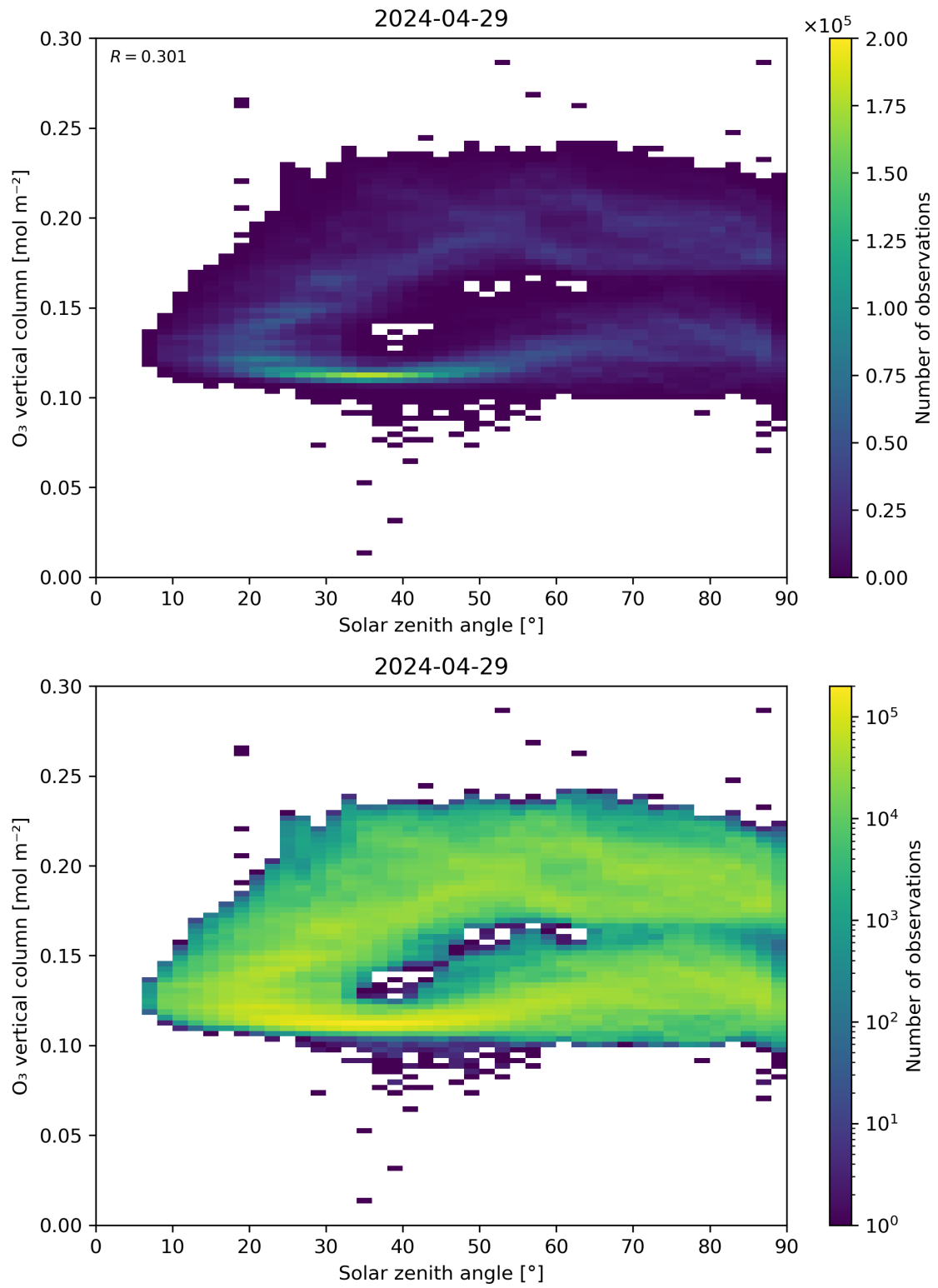
Figure 47: Scatter density plot of “Solar zenith angle” against “O 3 vertical column” for 2024-04-28 to 2024-04-30.
