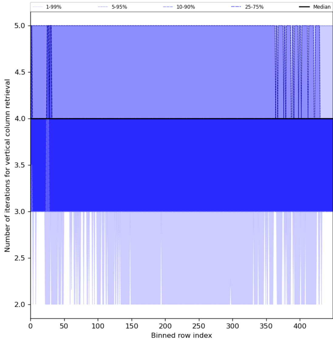
Figure 33: Along track statistics of “Number of iterations for vertical column retrieval” for 2024-04-28 to 2024-04-30
