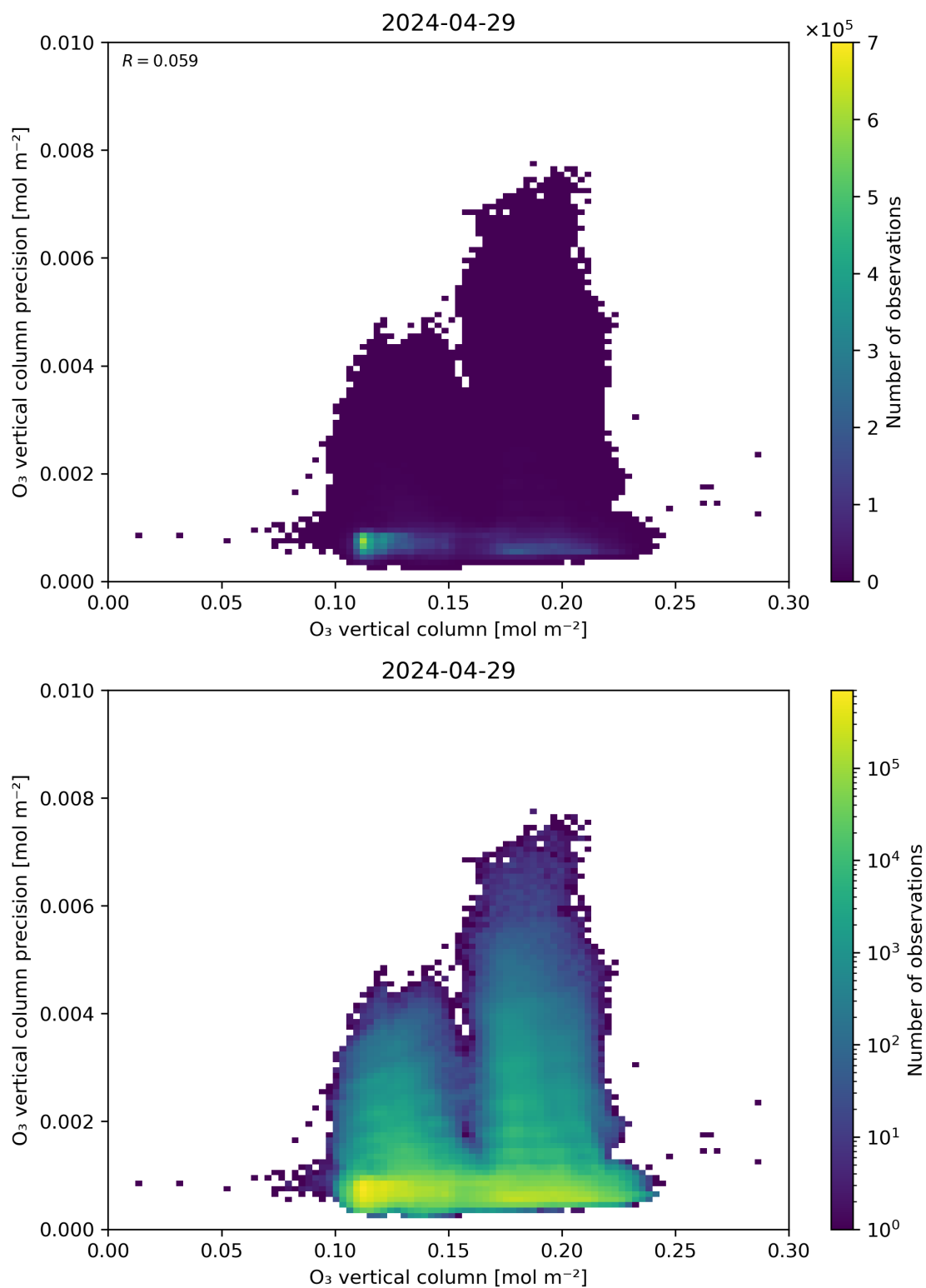
Figure 41: Scatter density plot of “O 3 vertical column” against “O 3 vertical column precision” for 2024-04-28 to 2024-04-30.
