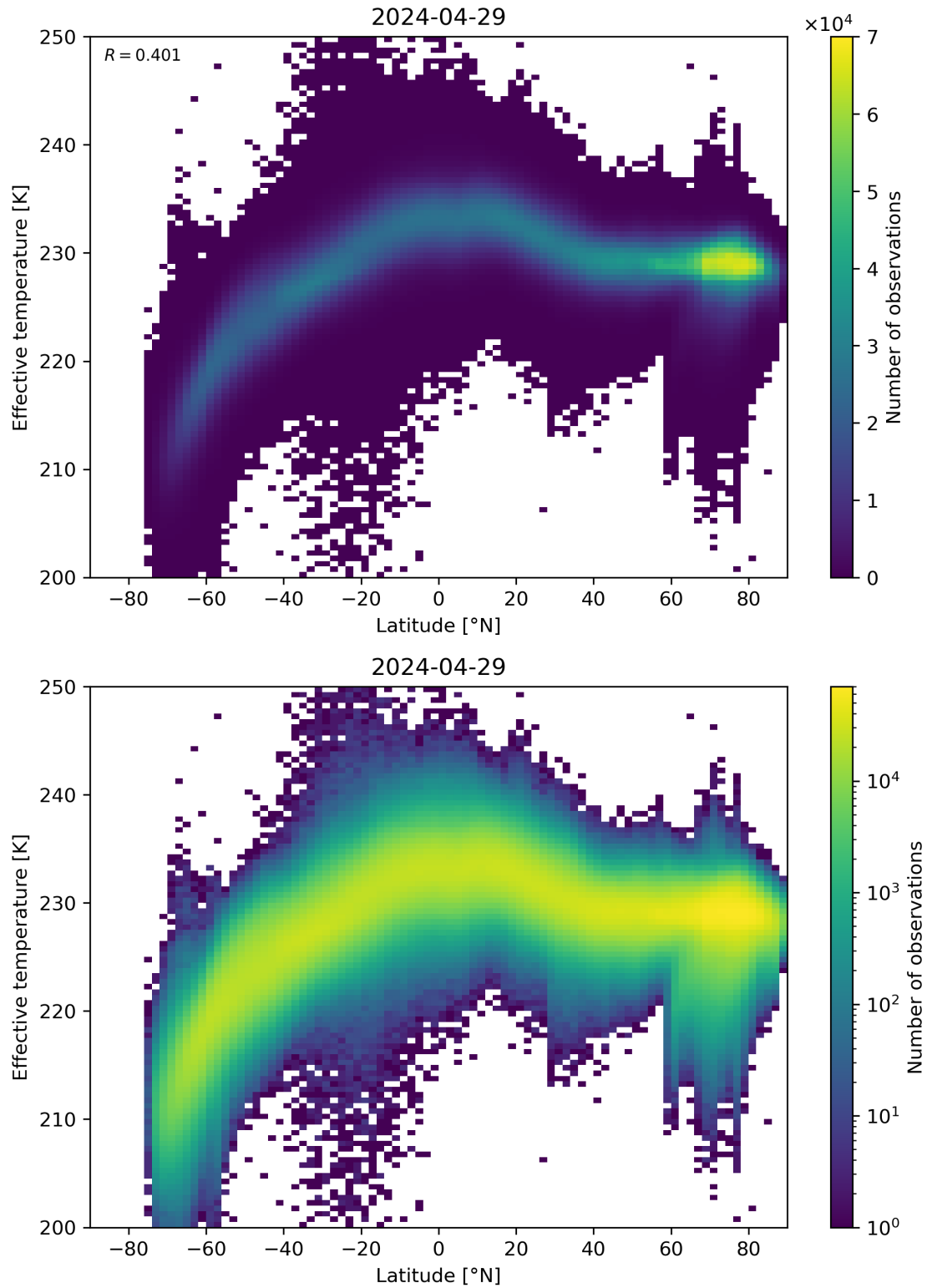
Figure 34: Scatter density plot of “Latitude” against “Effective temperature” for 2024-04-28 to 2024-04-30.
