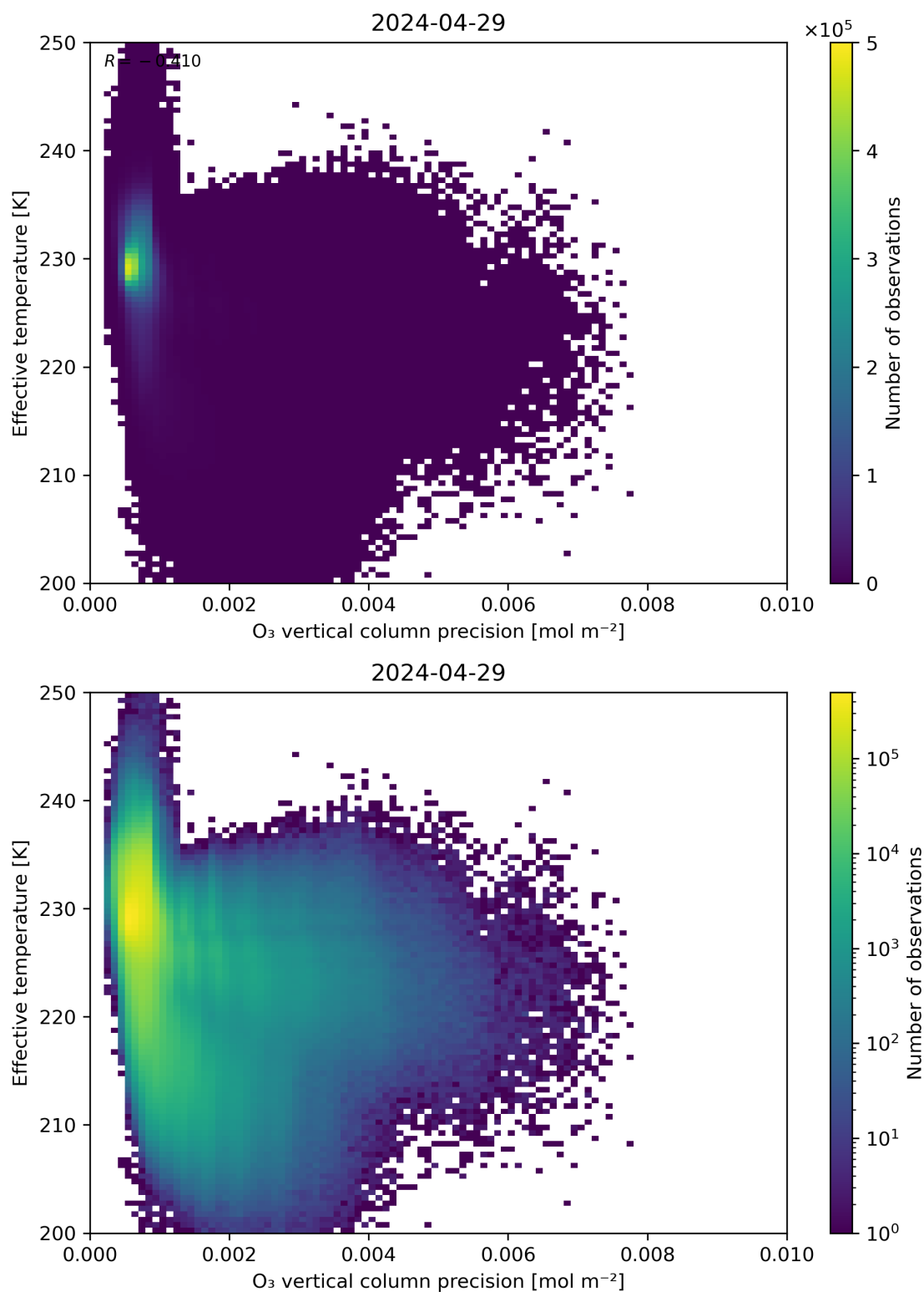
Figure 42: Scatter density plot of “O 3 vertical column precision” against “Effective temperature” for 2024-04-28 to 2024-04-30.
