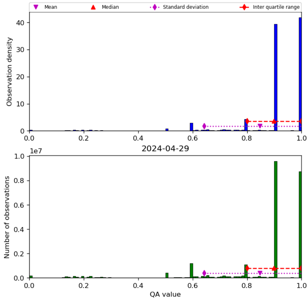
Figure 20: Histogram of “QA value” for 2024-04-28 to 2024-04-30
