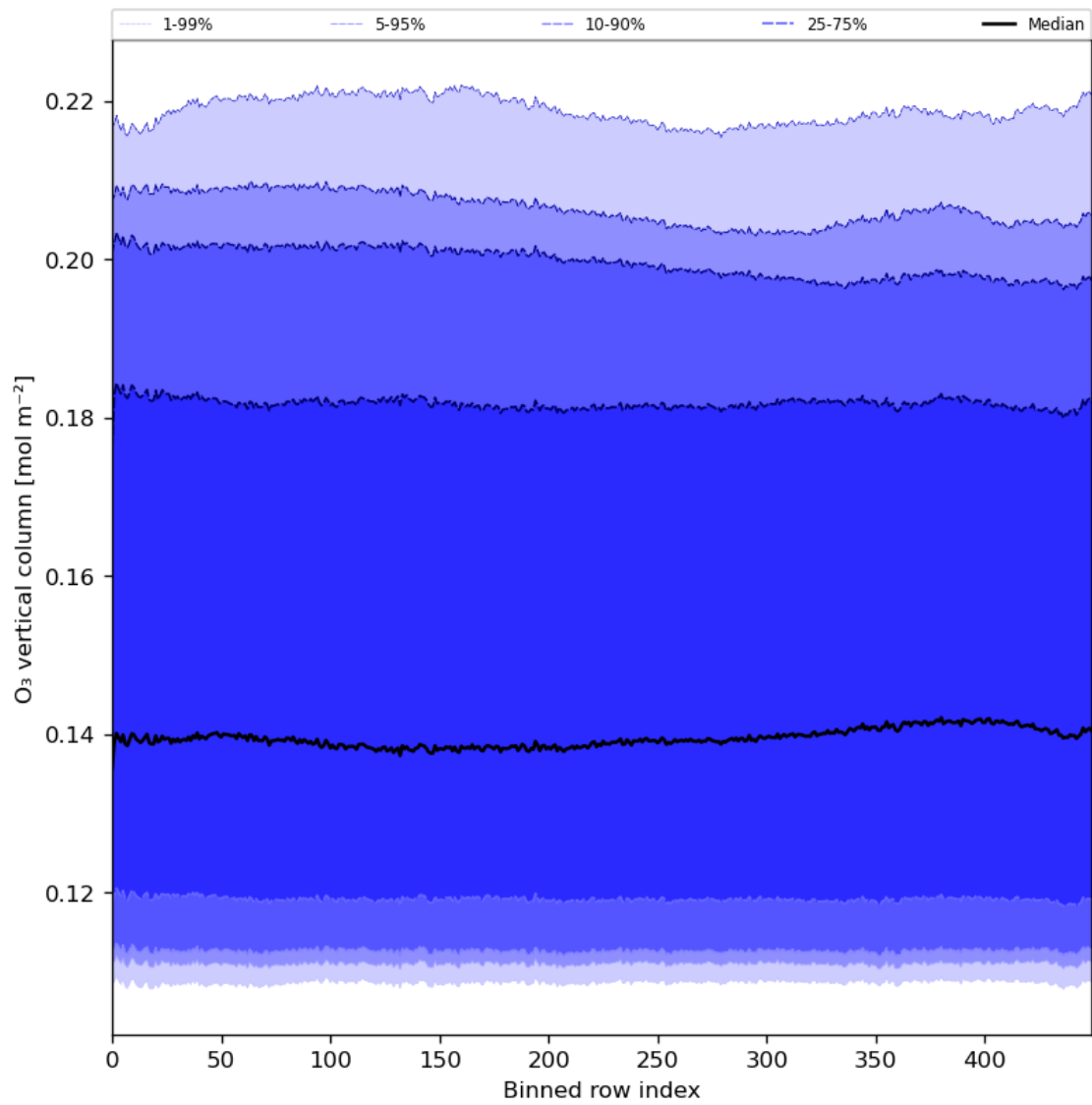
Figure 28: Along track statistics of “O 3 vertical column” for 2024-04-29 to 2024-05-01
