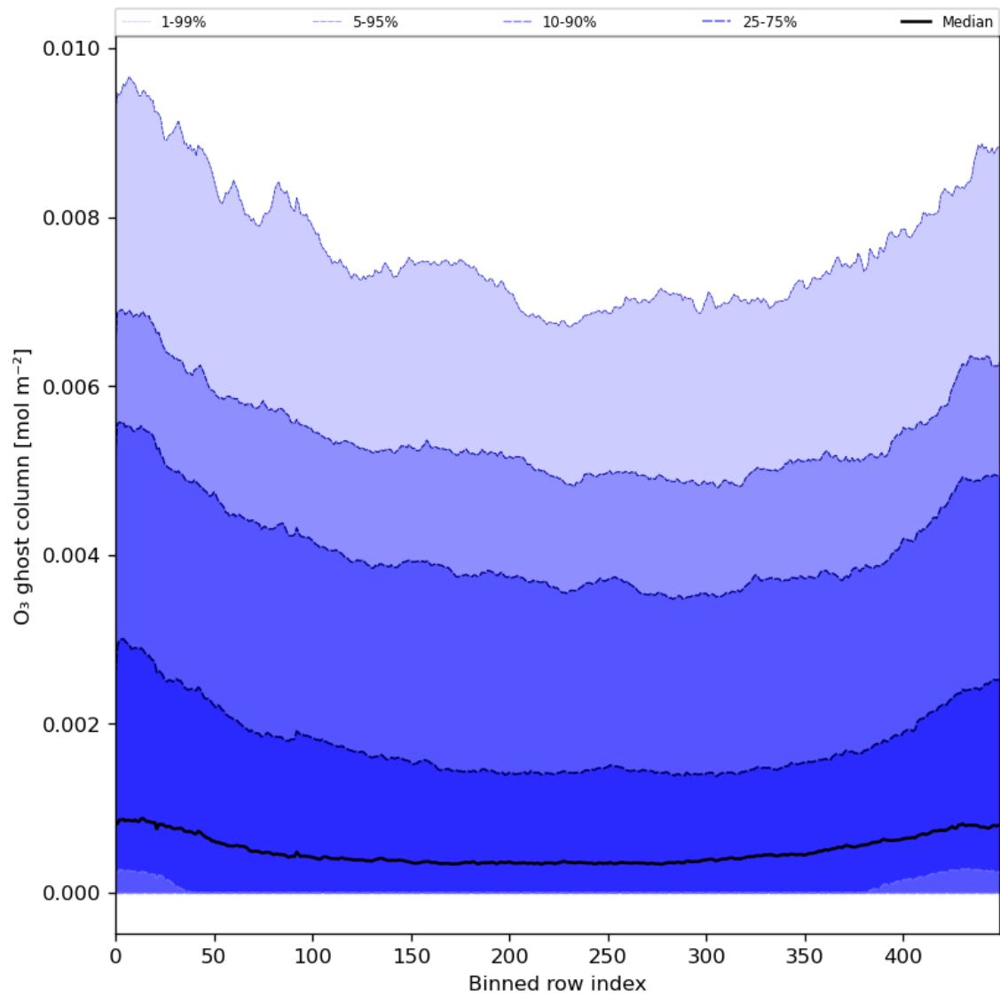
Figure 32: Along track statistics of “O 3 ghost column” for 2024-04-29 to 2024-05-01
