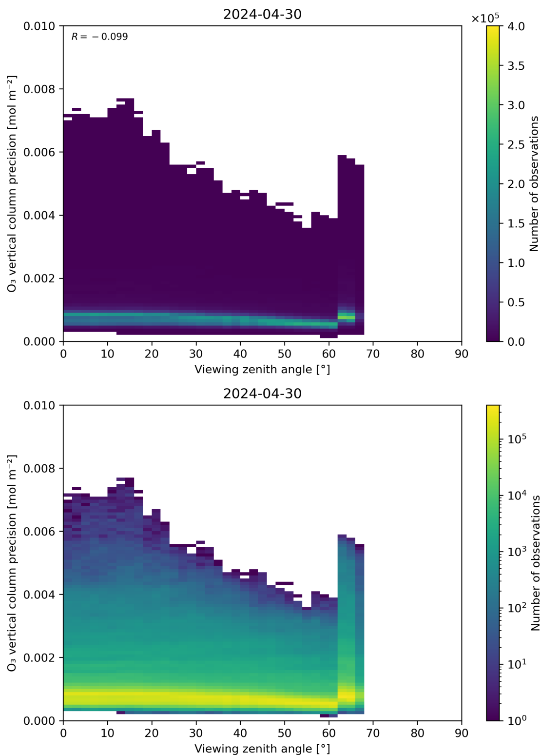
Figure 53: Scatter density plot of “Viewing zenith angle” against “O 3 vertical column precision” for 2024-04-29 to 2024-05-01.
