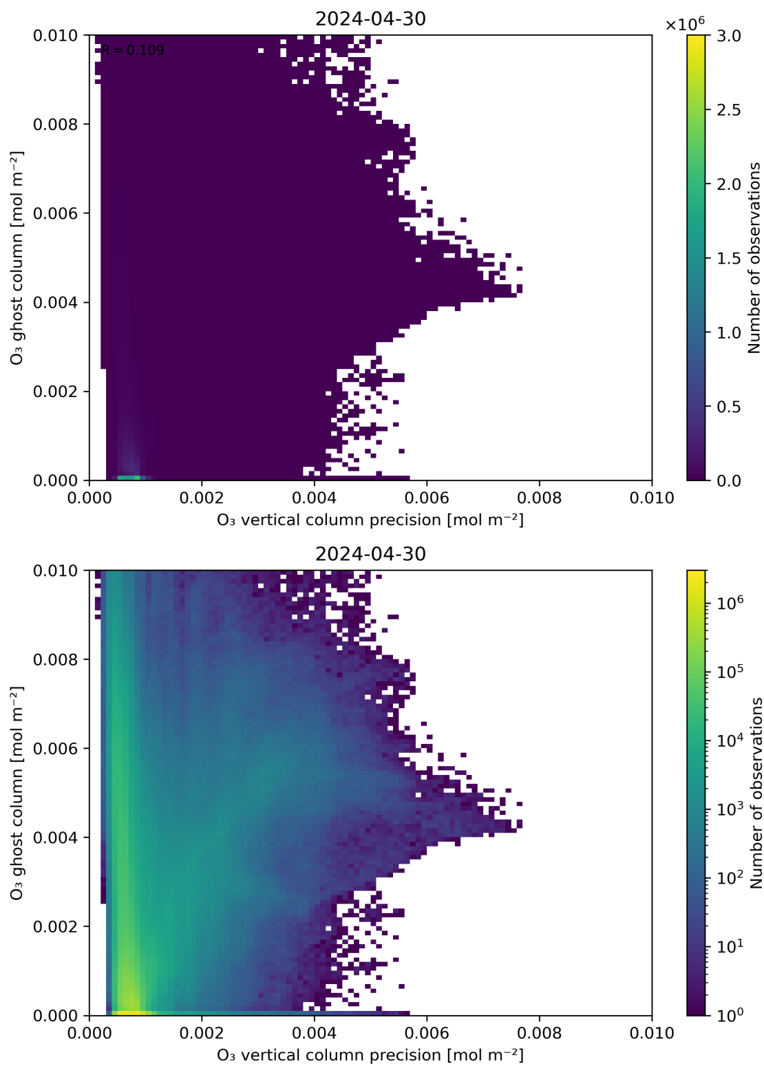
Figure 43: Scatter density plot of “ O_3 vertical column precision” against “ O_3 ghost column” for 2024-04-29 to 2024-05-01.
