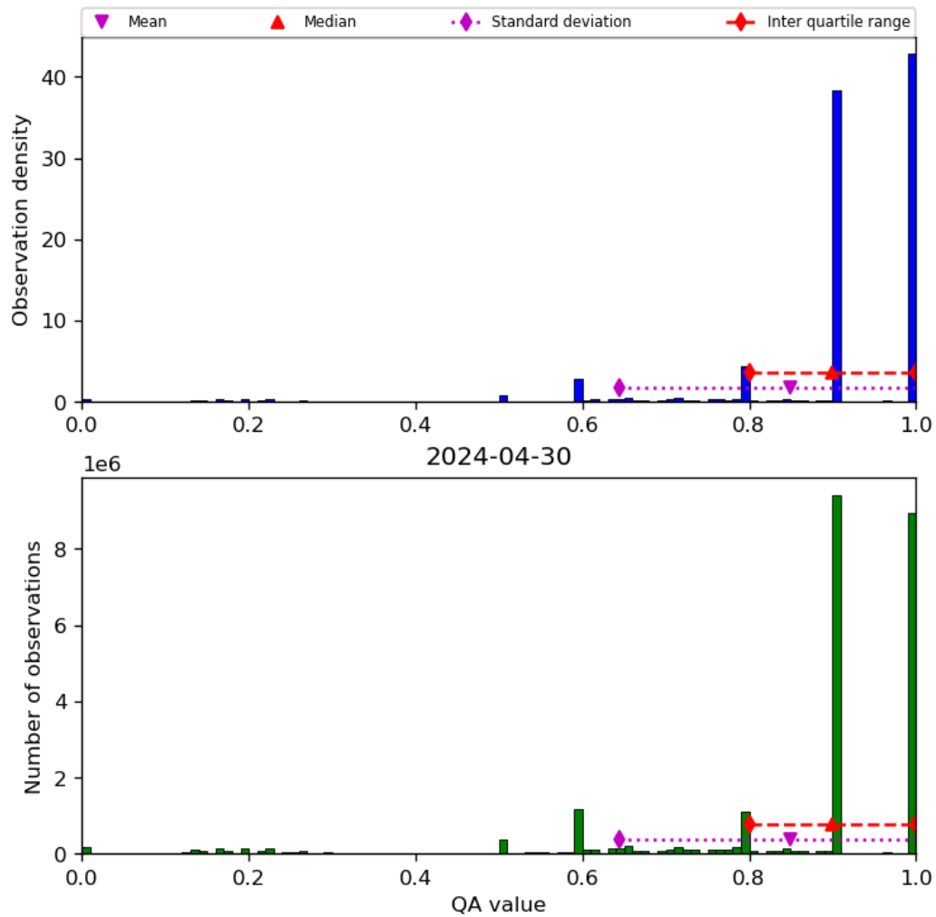
Figure 20: Histogram of “QA value” for 2024-04-29 to 2024-05-01
