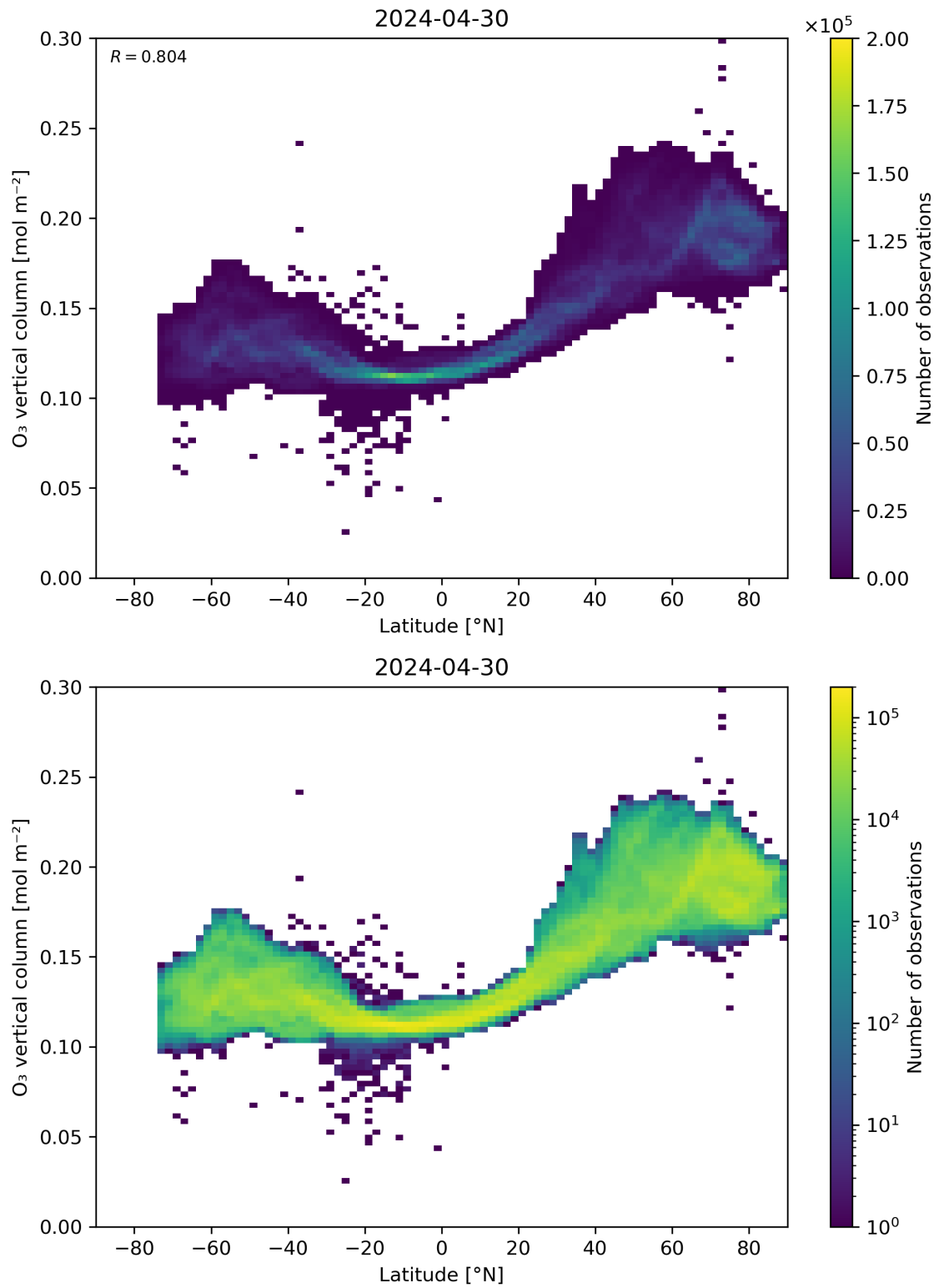
Figure 36: Scatter density plot of “Latitude” against “O 3 vertical column” for 2024-04-29 to 2024-05-01.
