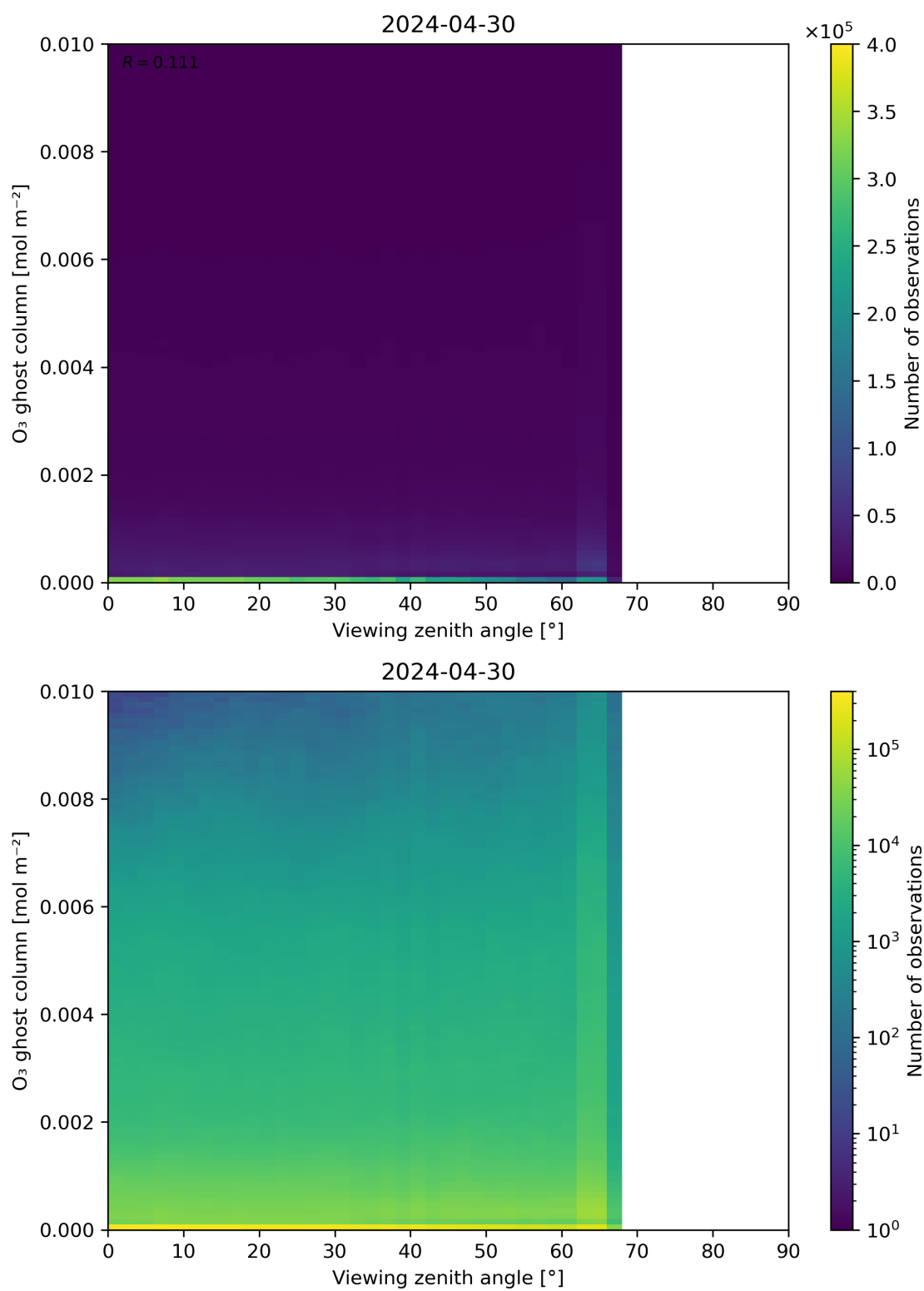
Figure 51: Scatter density plot of “Viewing zenith angle” against “O 3 ghost column” for 2024-04-29 to 2024-05-01.
