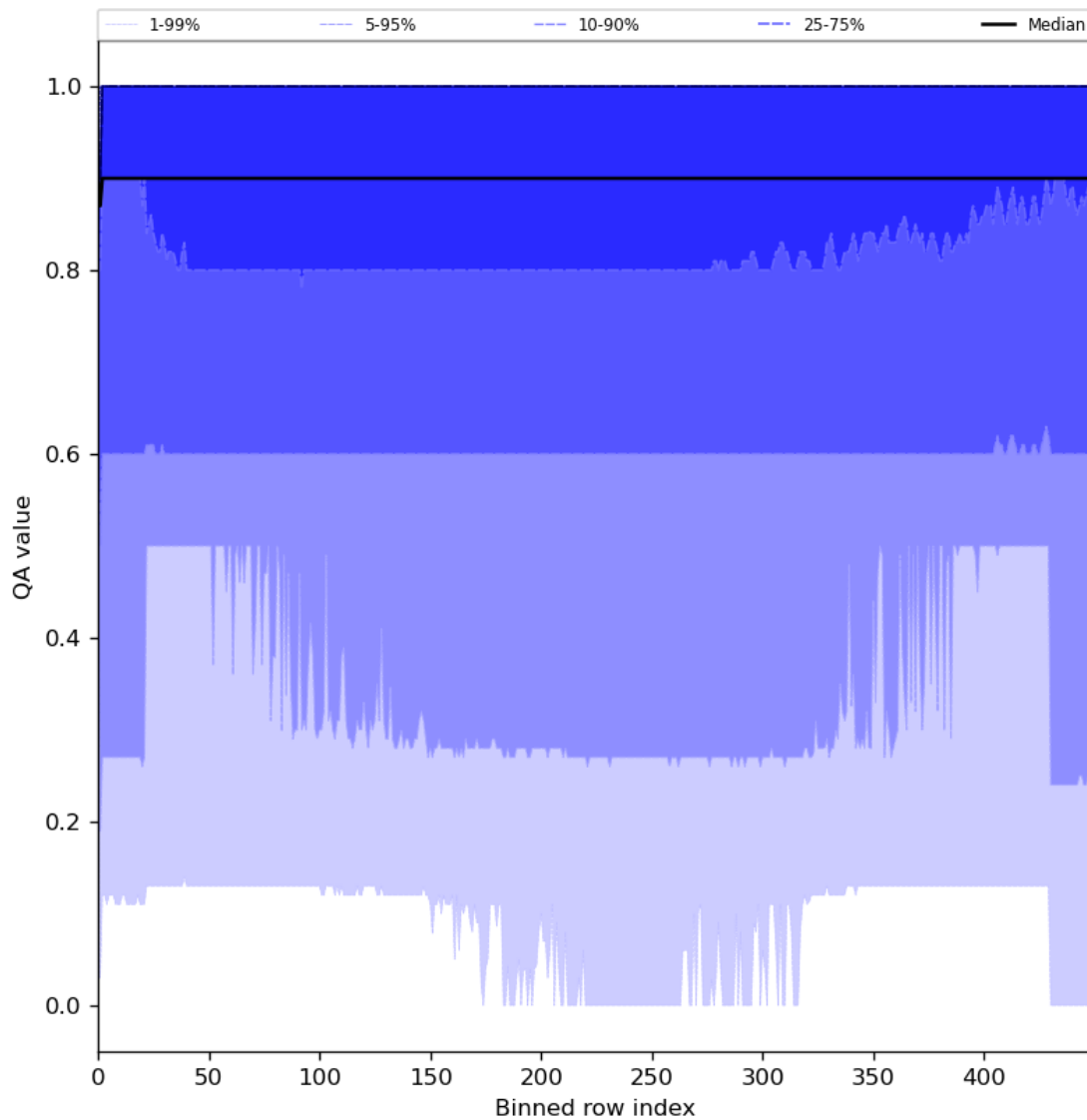
Figure 27: Along track statistics of “QA value” for 2024-04-29 to 2024-05-01
