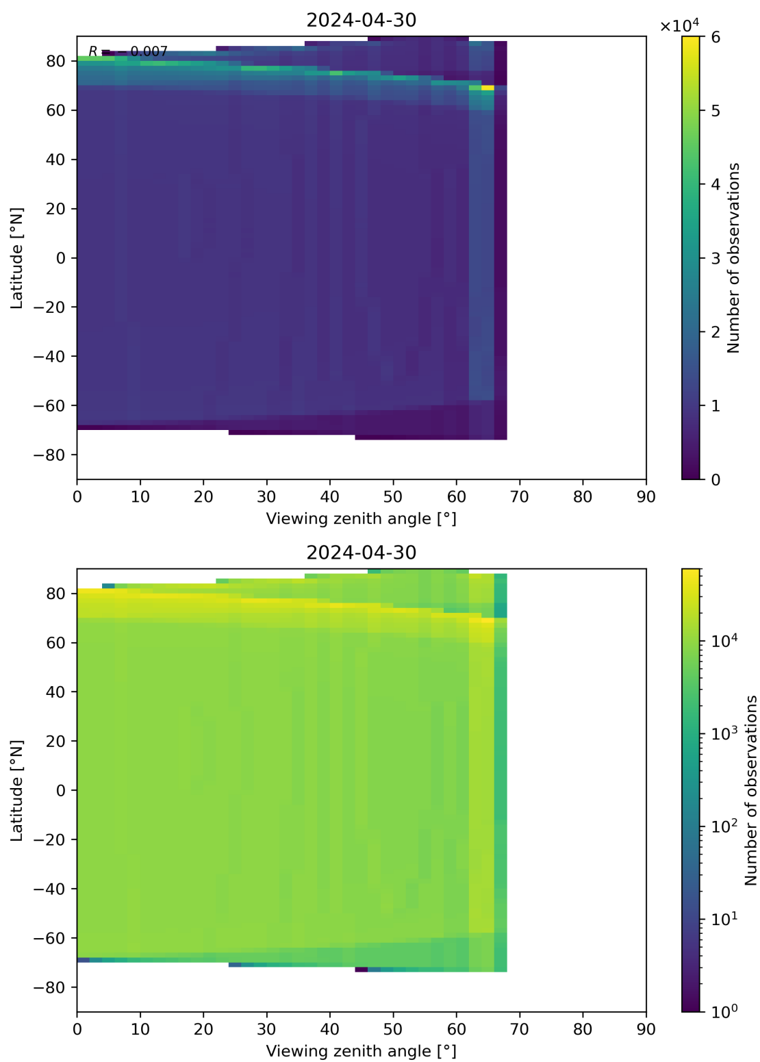
Figure 49: Scatter density plot of “Viewing zenith angle” against “Latitude” for 2024-04-29 to 2024-05-01.
