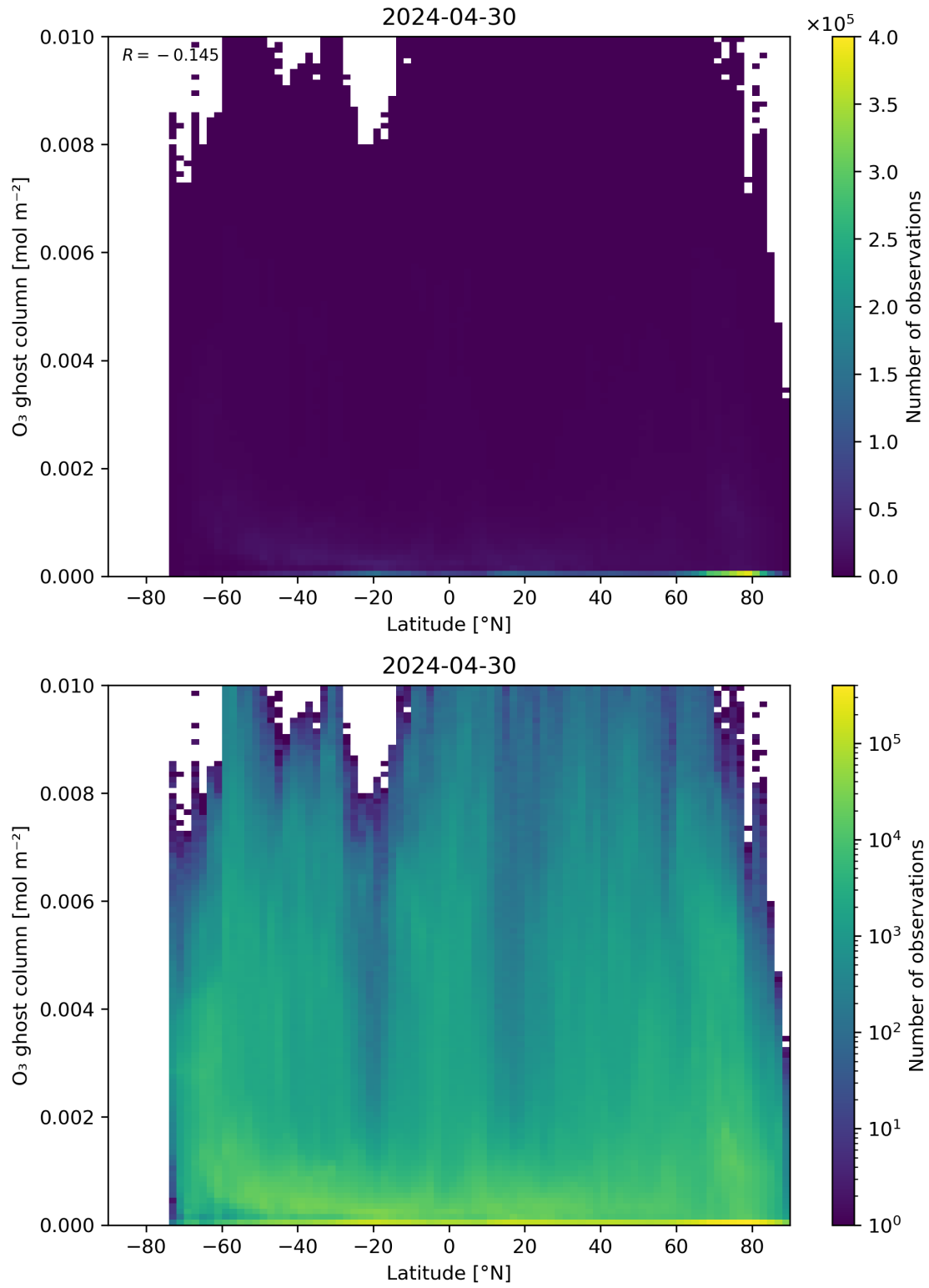
Figure 35: Scatter density plot of “Latitude” against “O 3 ghost column” for 2024-04-29 to 2024-05-01.
