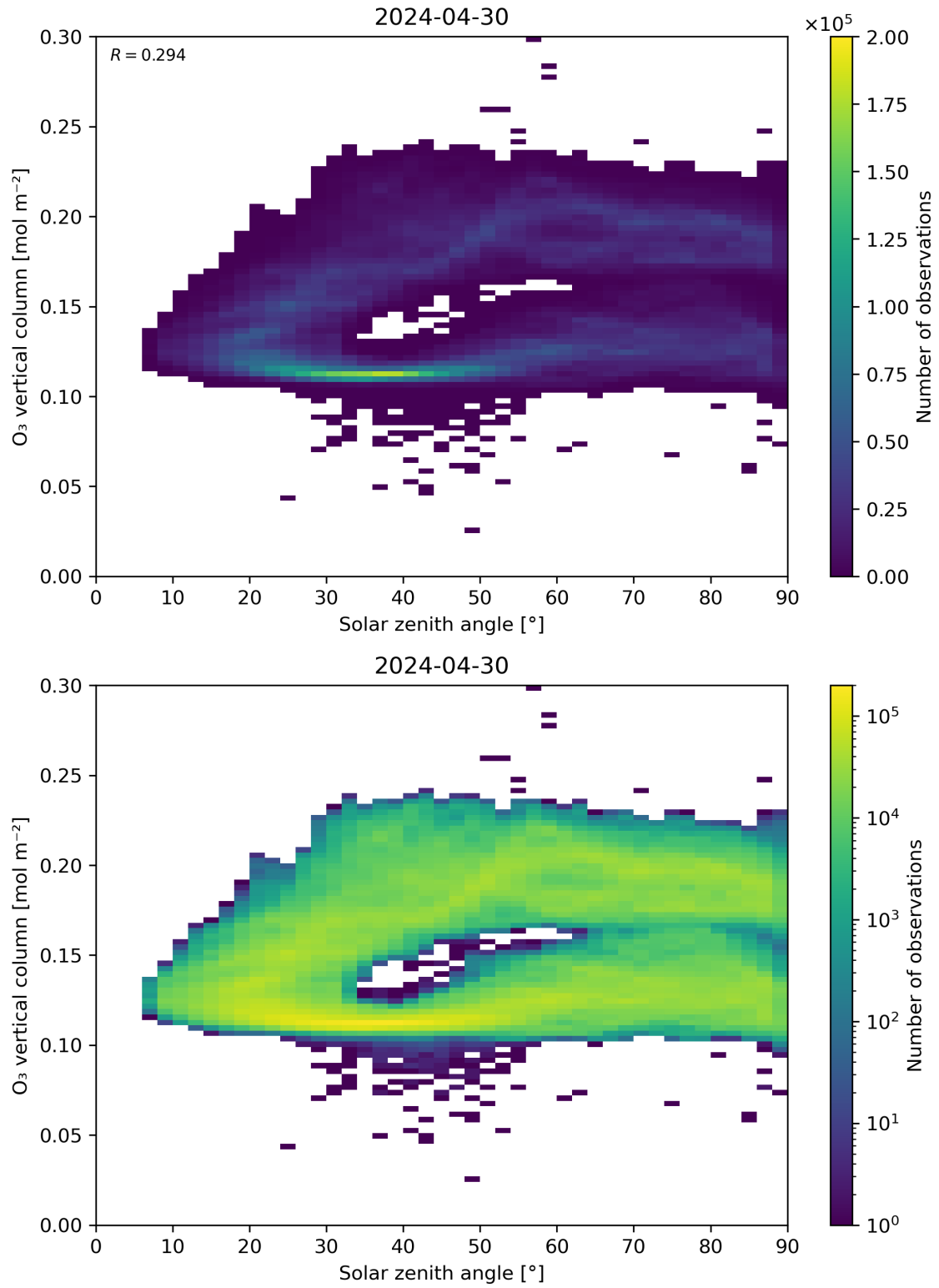
Figure 47: Scatter density plot of “Solar zenith angle” against “O 3 vertical column” for 2024-04-29 to 2024-05-01.
