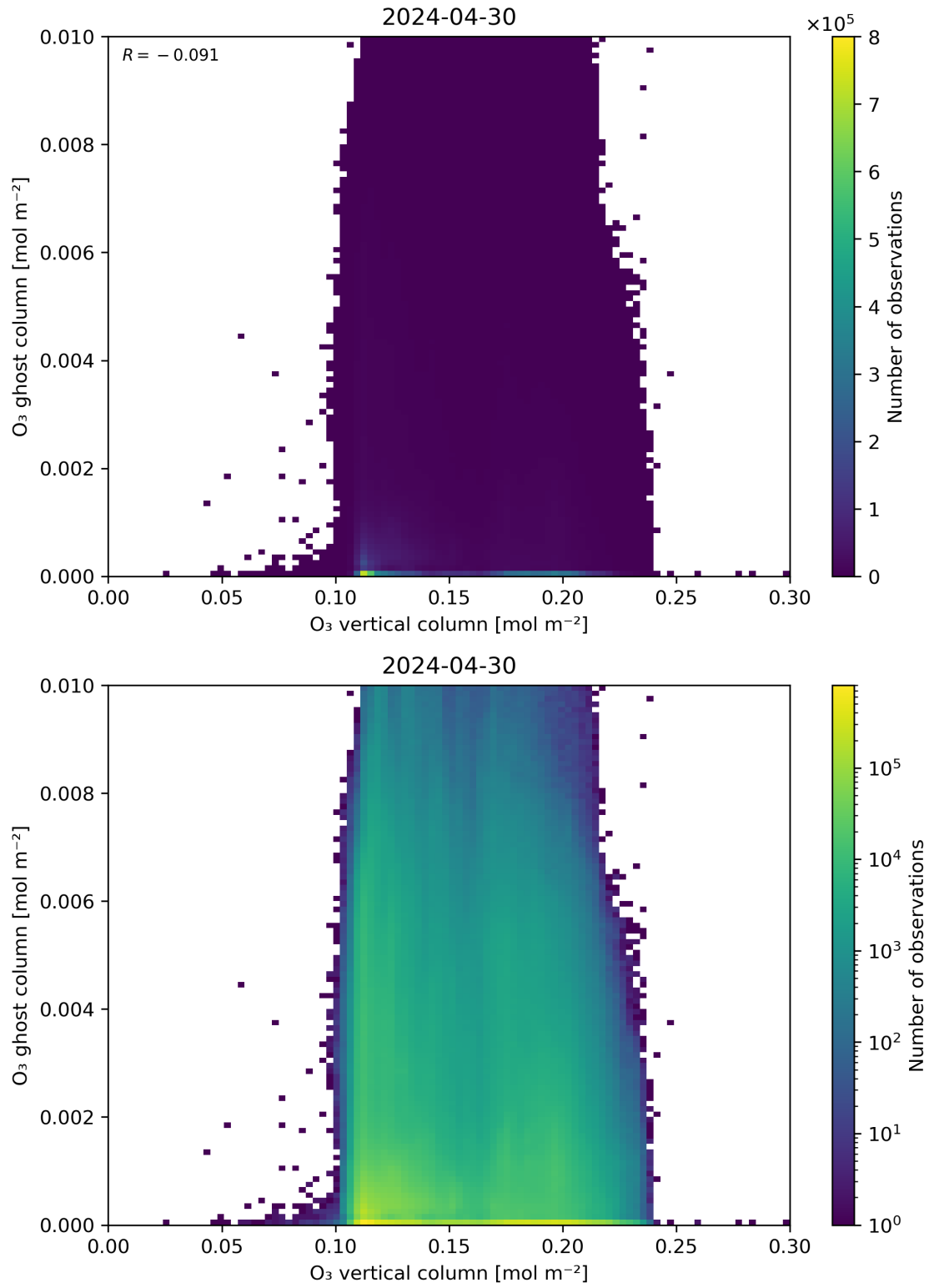
Figure 40: Scatter density plot of “O 3 vertical column” against “O 3 ghost column” for 2024-04-29 to 2024-05-01.
