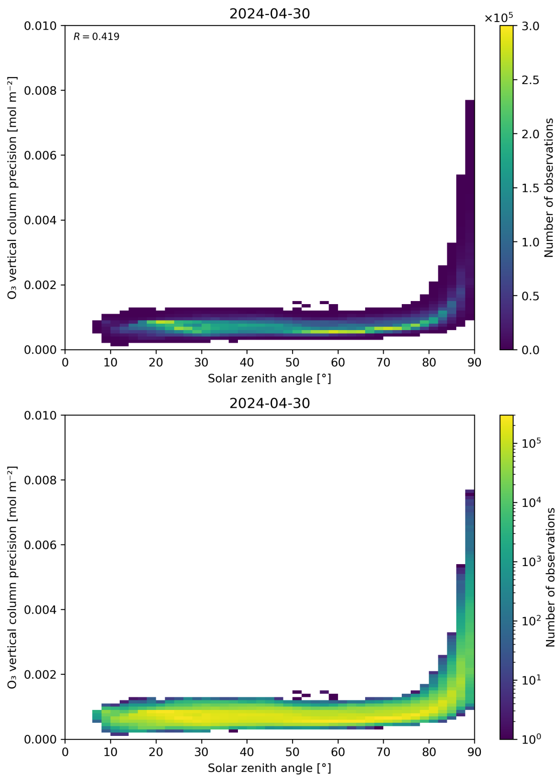
Figure 48: Scatter density plot of “Solar zenith angle” against “O 3 vertical column precision” for 2024-04-29 to 2024-05-01.
