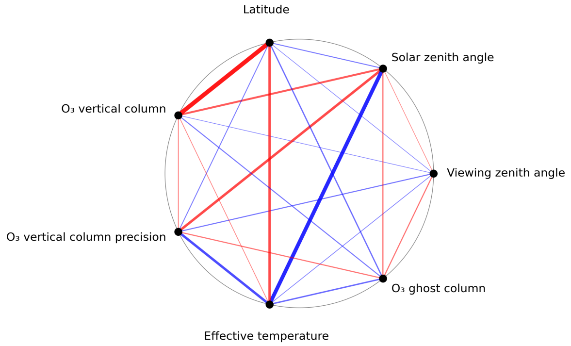
Figure 1: Map of correlation graph for 2024-04-29 to 2024-05-01.
