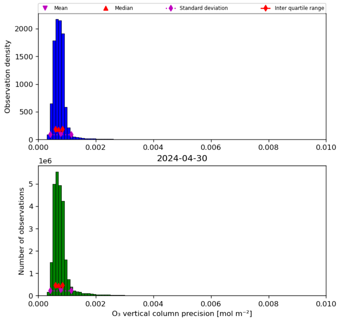
Figure 22: Histogram of “O 3 vertical column precision” for 2024-04-29 to 2024-05-01
