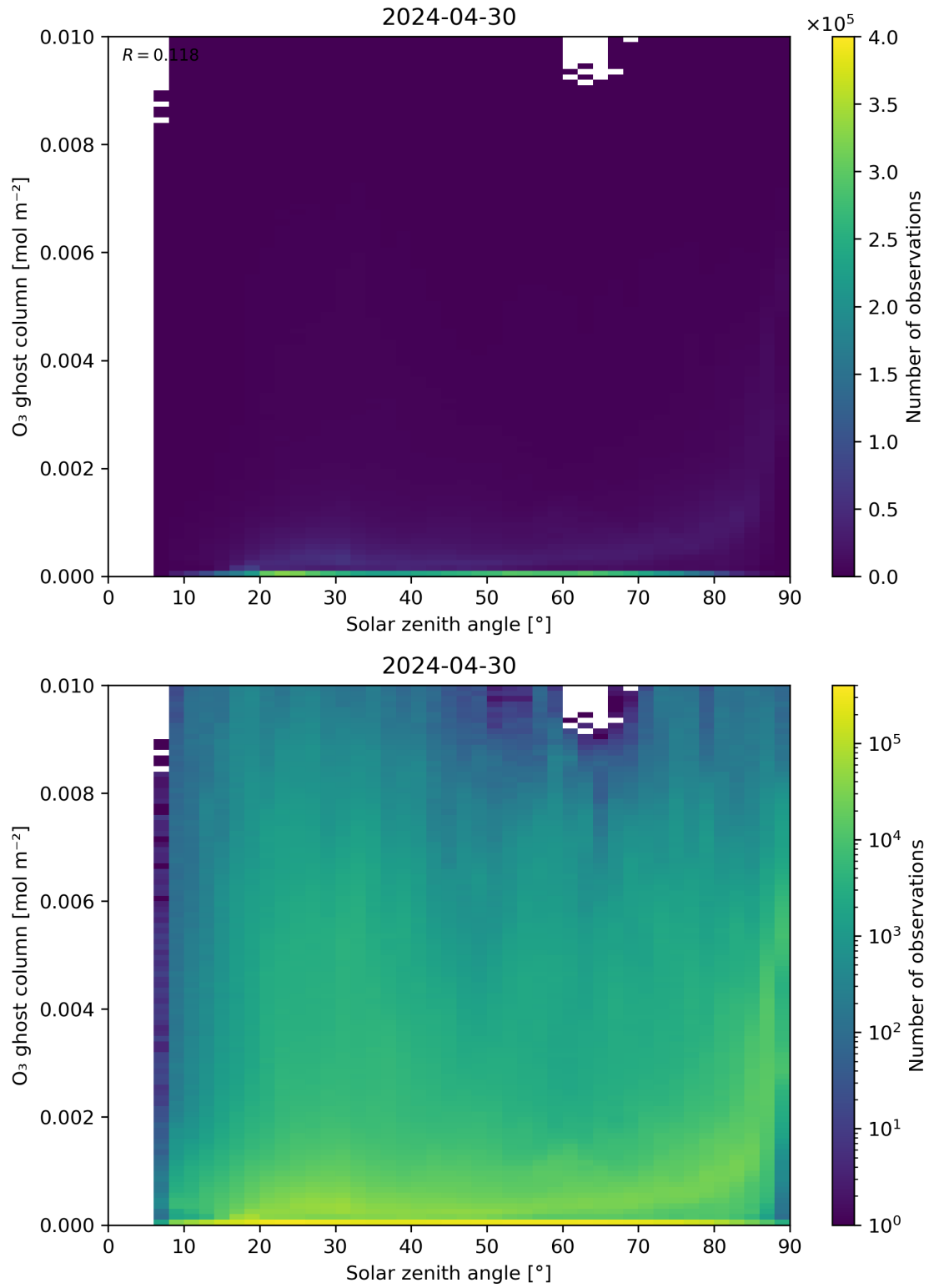
Figure 46: Scatter density plot of “Solar zenith angle” against “O 3 ghost column” for 2024-04-29 to 2024-05-01.
