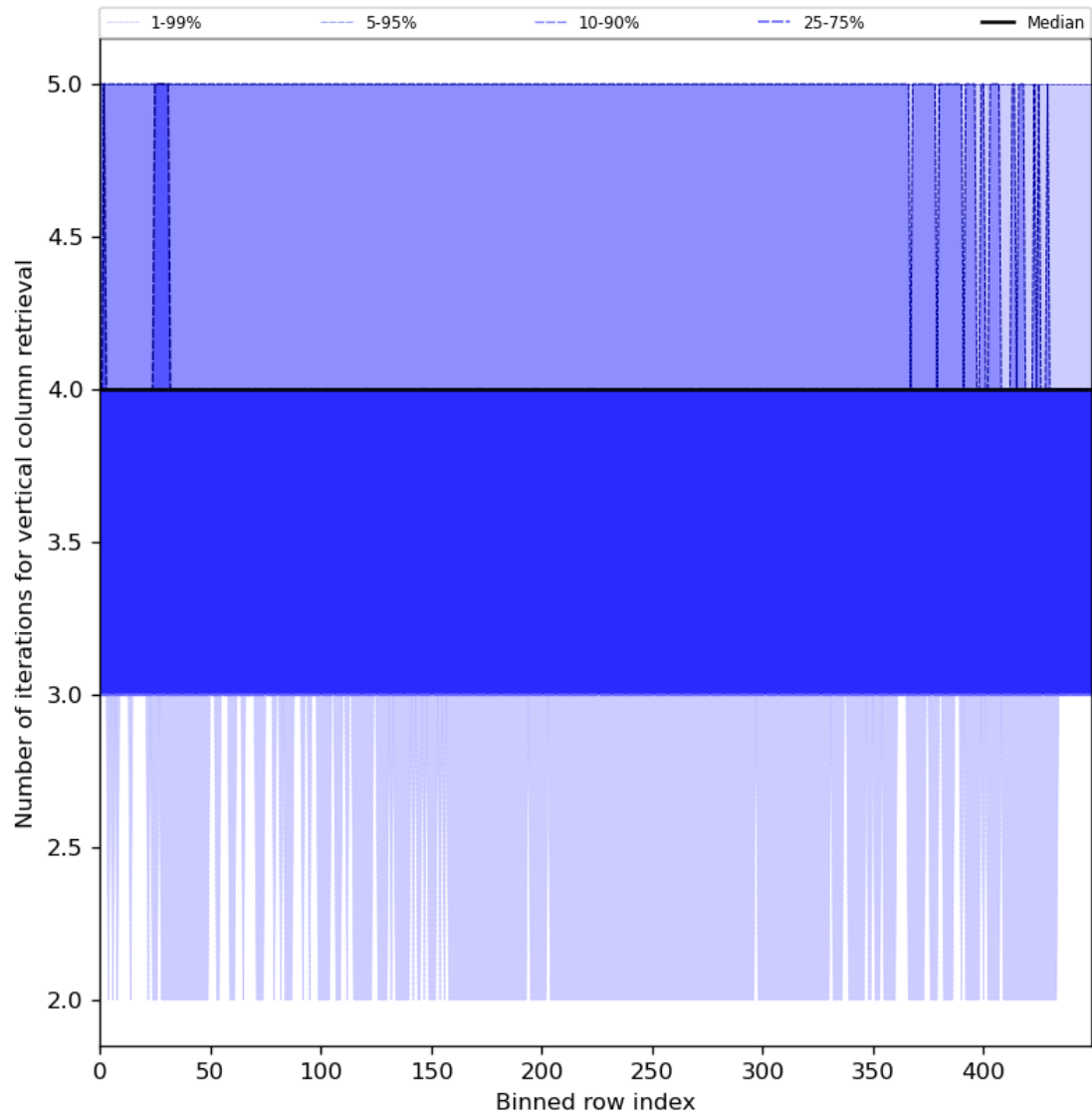
Figure 33: Along track statistics of “Number of iterations for vertical column retrieval” for 2024-04-29 to 2024-05-01
