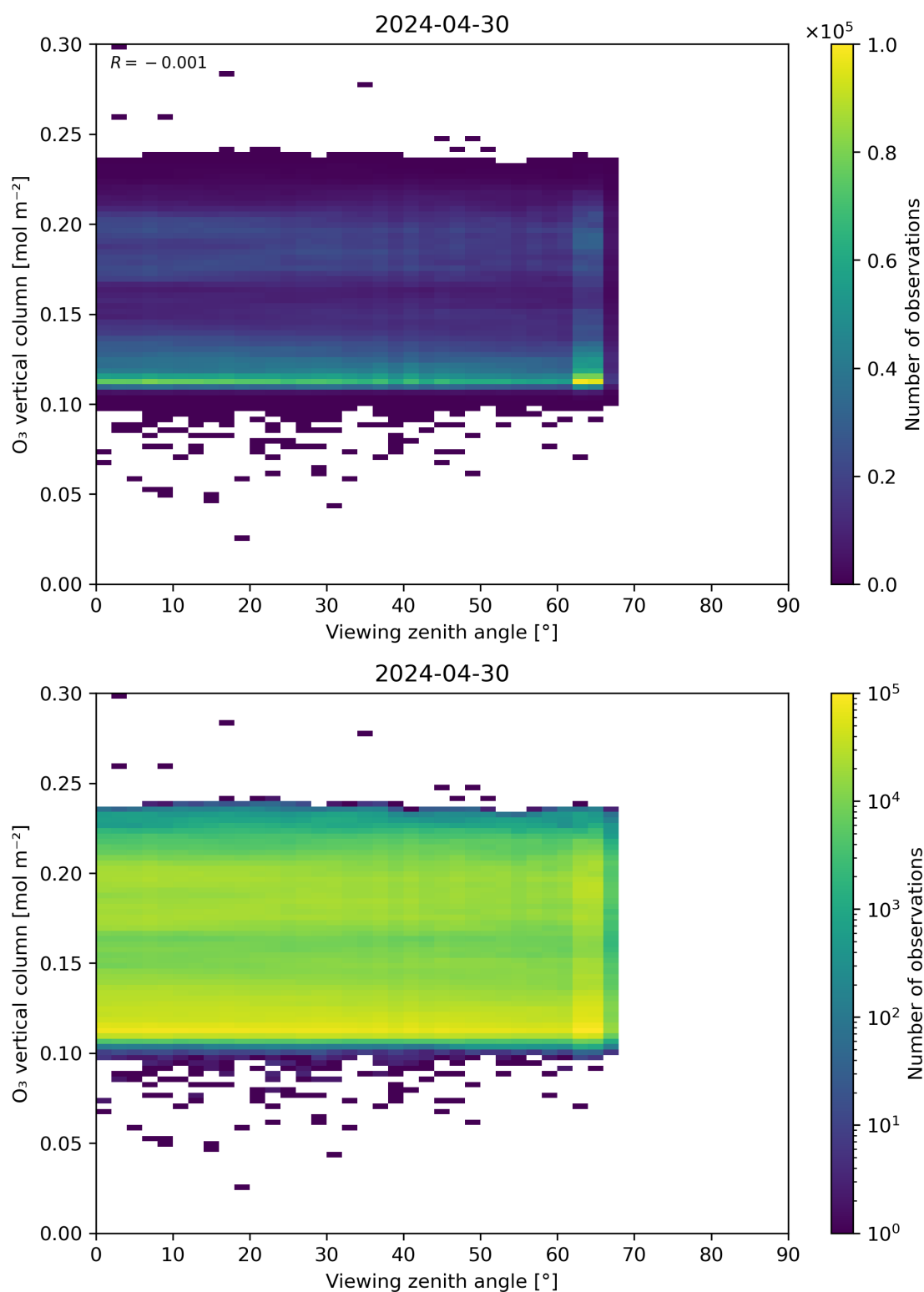
Figure 52: Scatter density plot of “Viewing zenith angle” against “O 3 vertical column” for 2024-04-29 to 2024-05-01.
