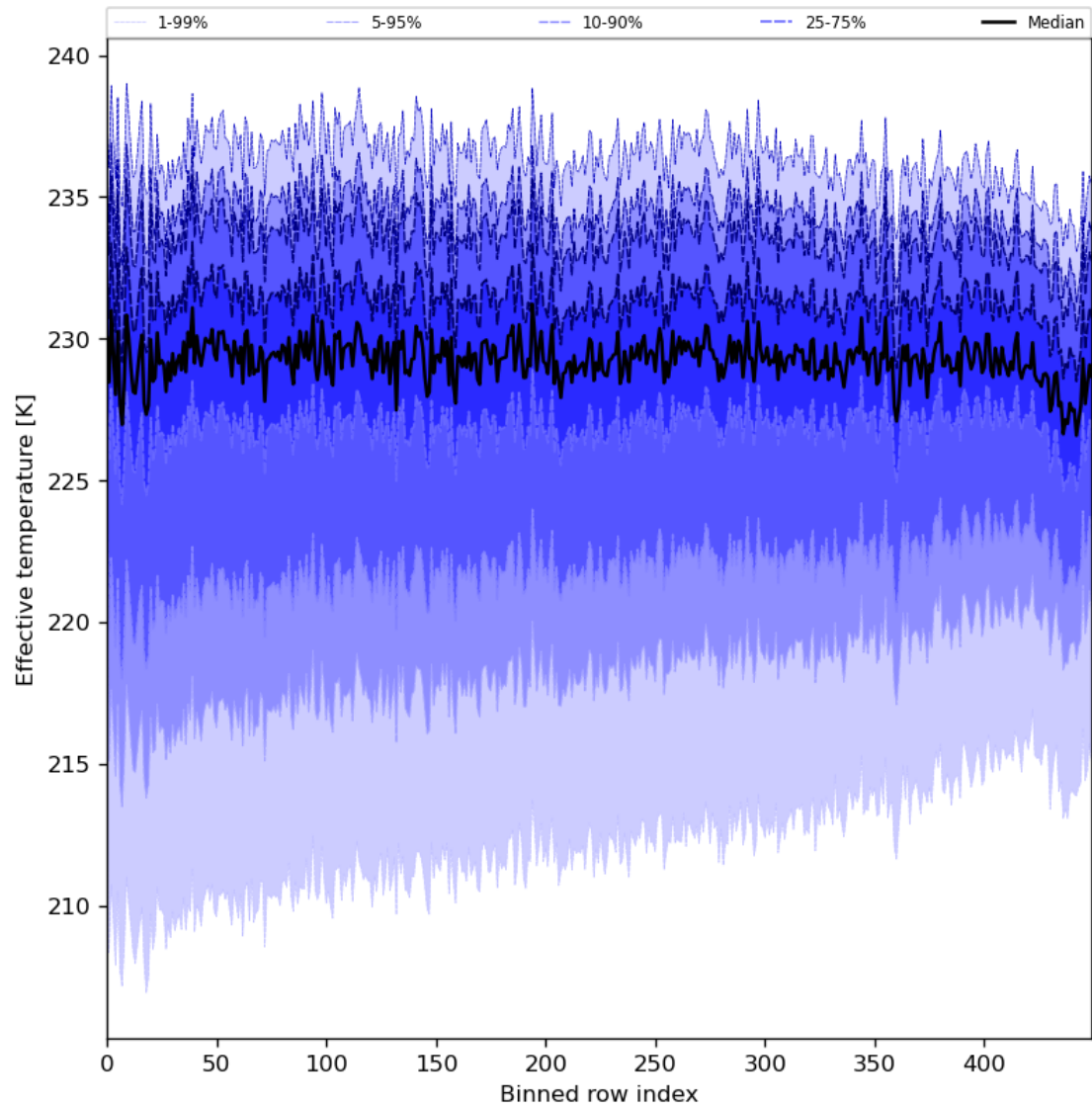
Figure 31: Along track statistics of “Effective temperature” for 2024-04-29 to 2024-05-01
