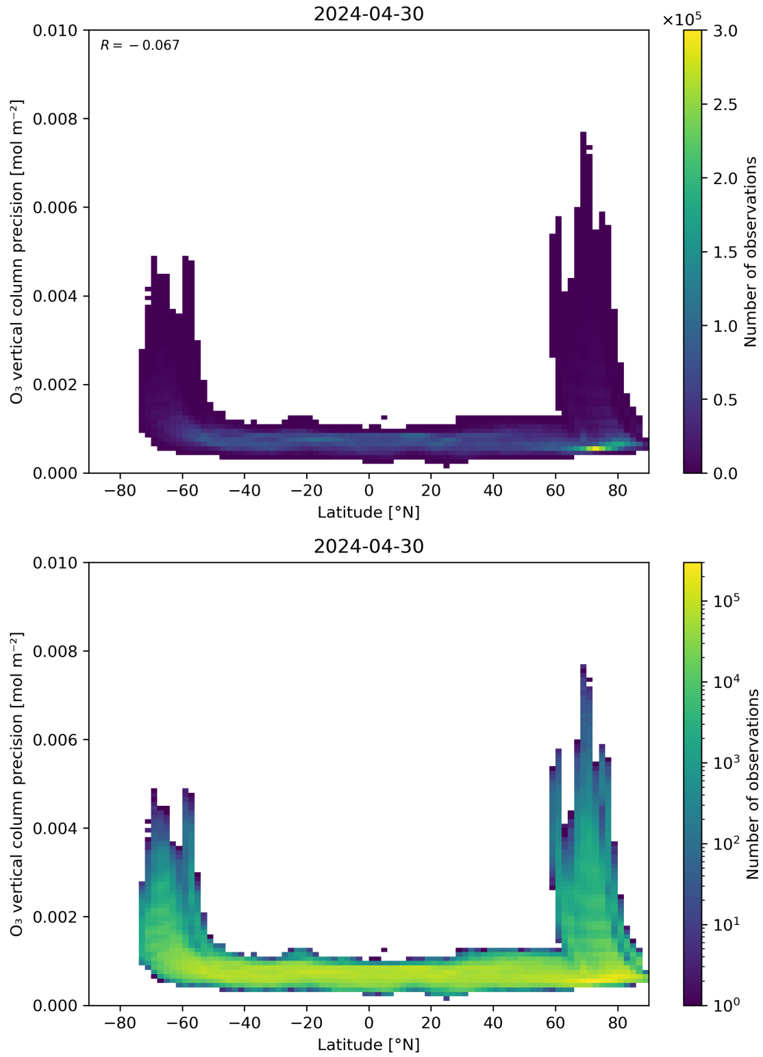
Figure 37: Scatter density plot of “Latitude” against “O 3 vertical column precision” for 2024-04-29 to 2024-05-01.
