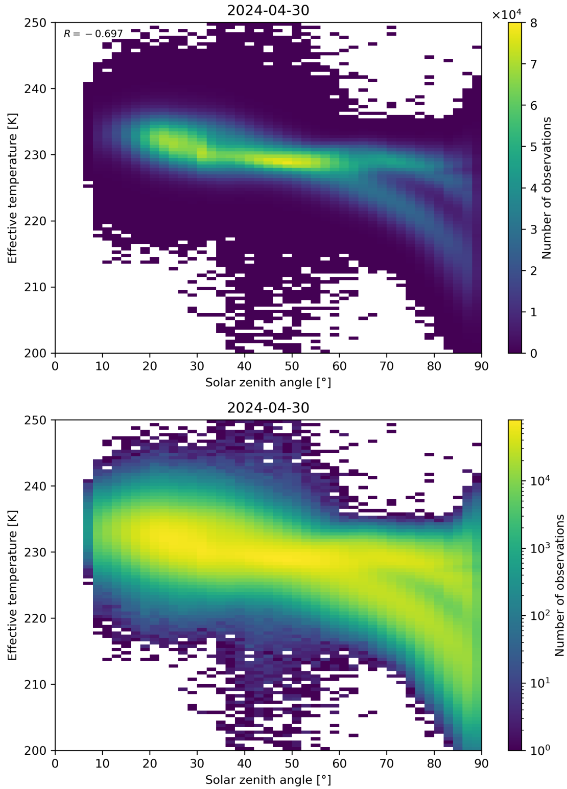
Figure 45: Scatter density plot of “Solar zenith angle” against “Effective temperature” for 2024-04-29 to 2024-05-01.
