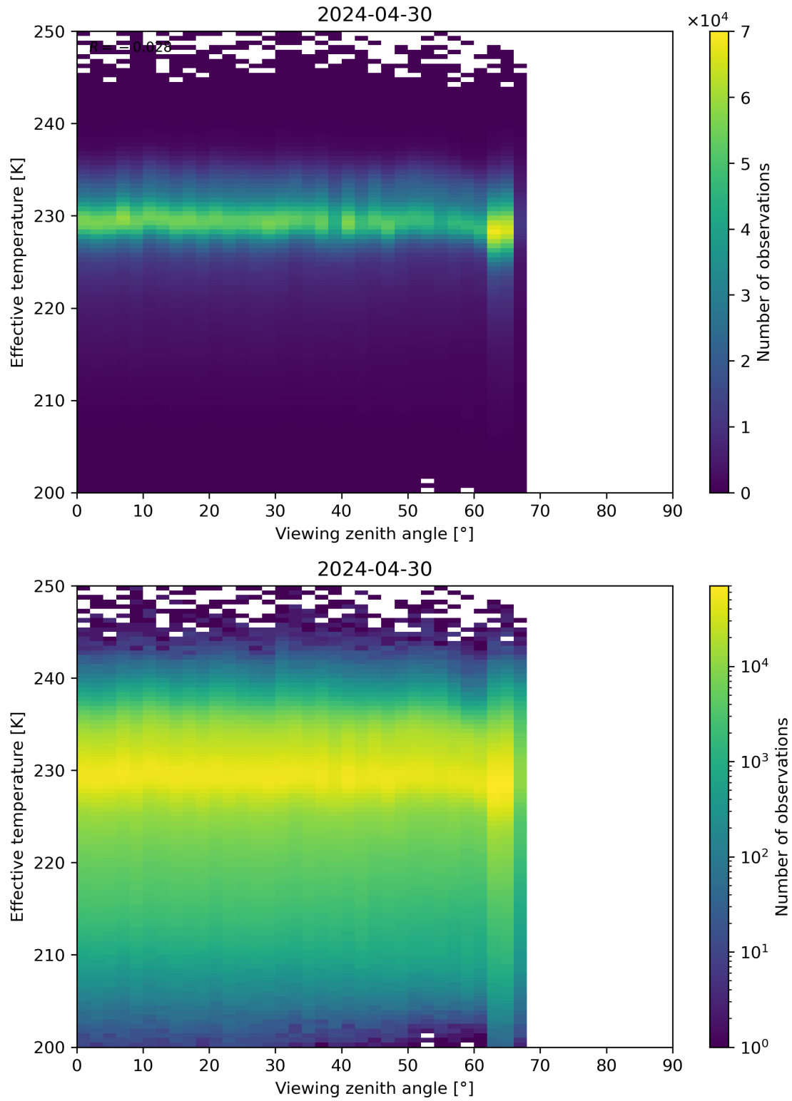
Figure 50: Scatter density plot of “Viewing zenith angle” against “Effective temperature” for 2024-04-29 to 2024-05-01.
