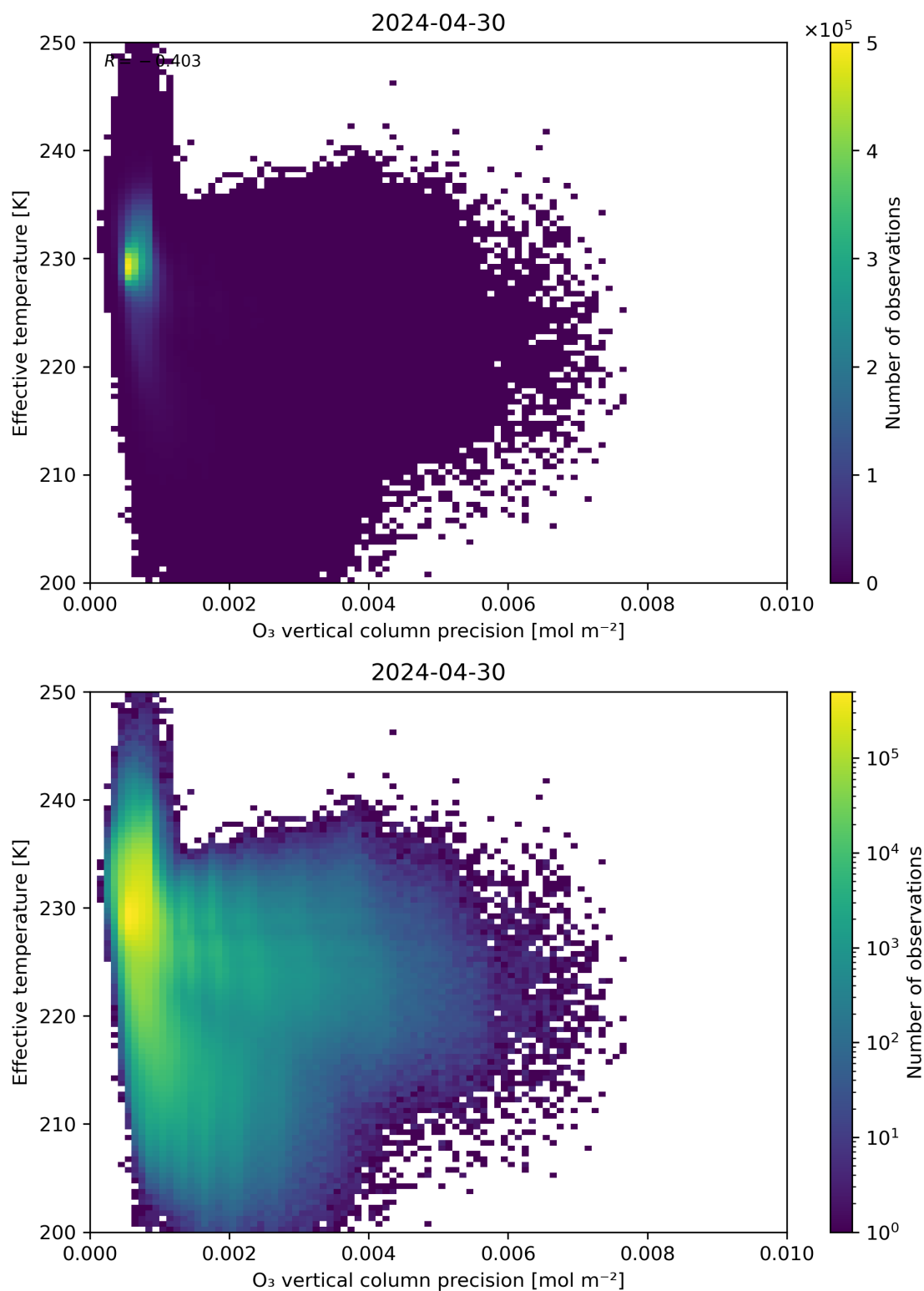
Figure 42: Scatter density plot of “O 3 vertical column precision” against “Effective temperature” for 2024-04-29 to 2024-05-01.
