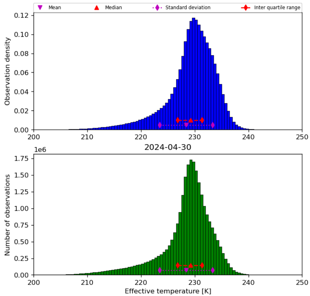
Figure 24: Histogram of “Effective temperature” for 2024-04-29 to 2024-05-01
