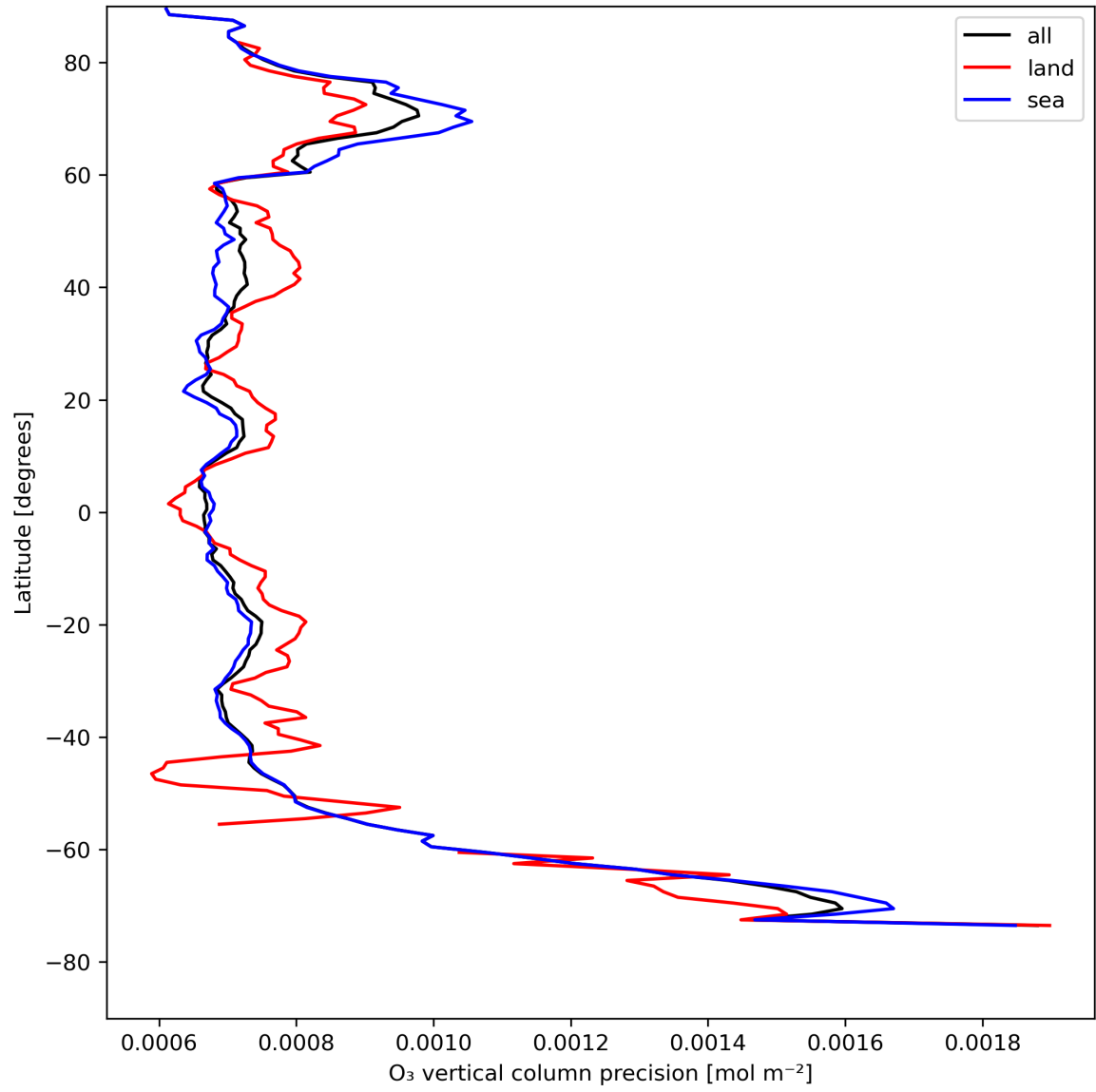
Figure 15: Zonal average of “O 3 vertical column precision” for 2024-04-29 to 2024-05-01.
