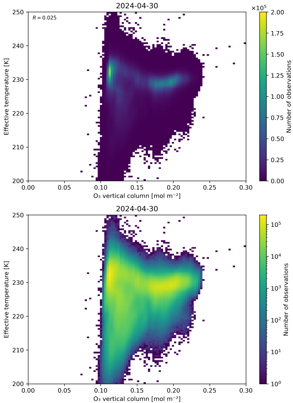
Figure 39: Scatter density plot of “O 3 vertical column” against “Effective temperature” for 2024-04-29 to 2024-05-01.
