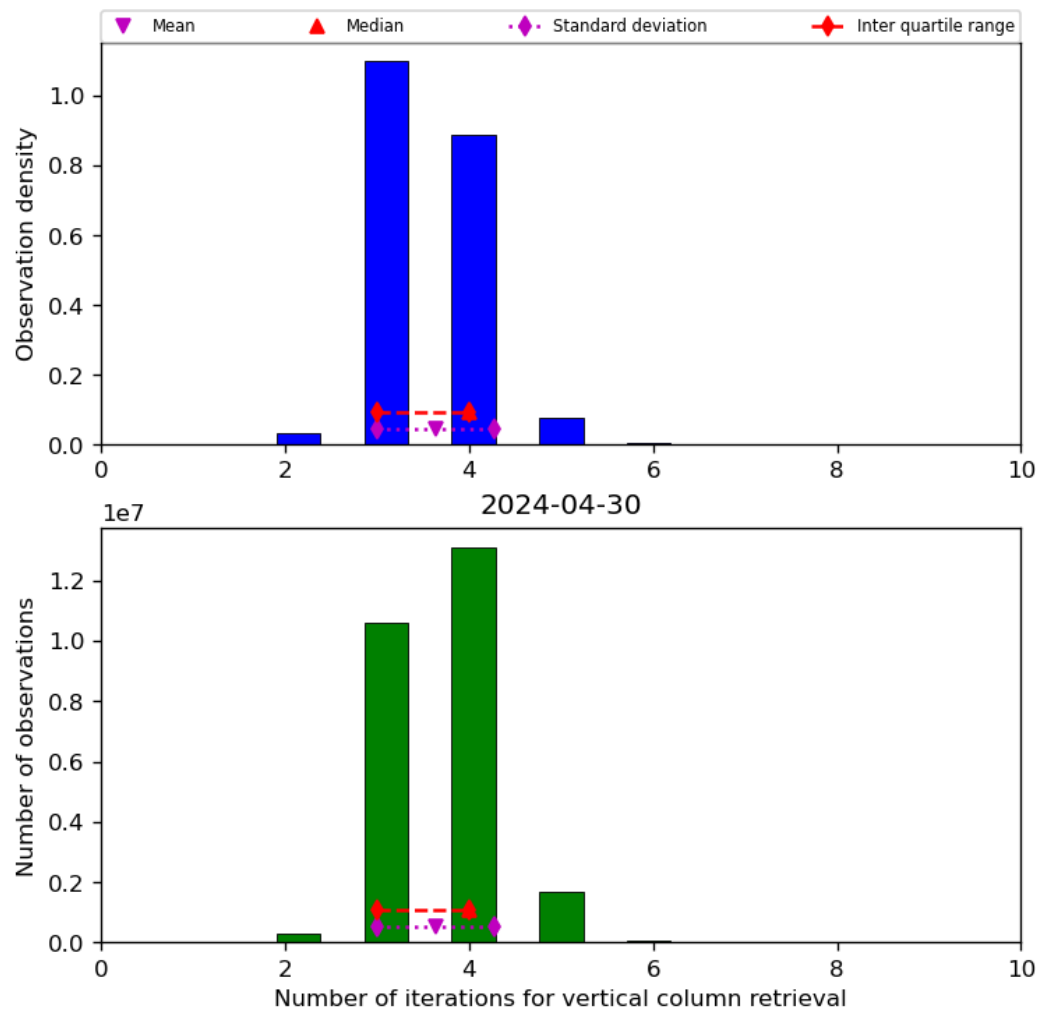
Figure 26: Histogram of “Number of iterations for vertical column retrieval” for 2024-04-29 to 2024-05-01
