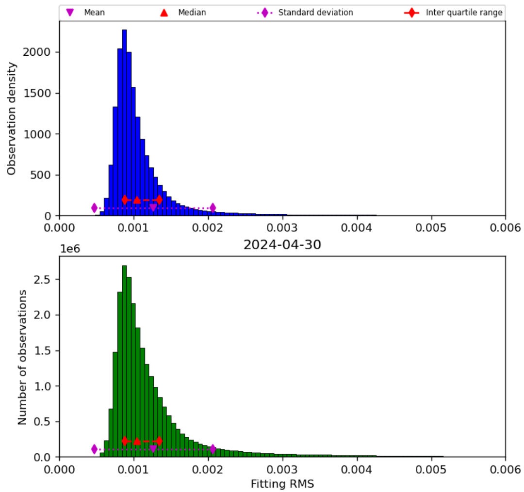
Figure 23: Histogram of “Fitting RMS” for 2024-04-29 to 2024-05-01
