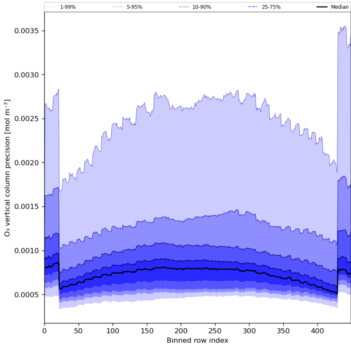
Figure 29: Along track statistics of “O 3 vertical column precision” for 2024-04-29 to 2024-05-01
