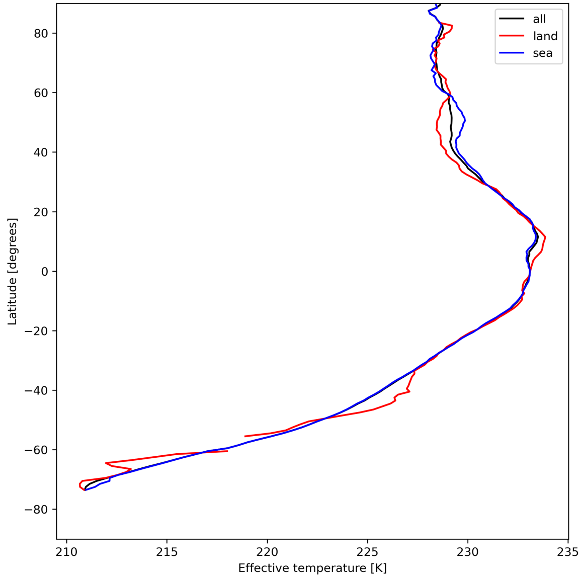
Figure 17: Zonal average of “Effective temperature” for 2024-04-29 to 2024-05-01.
