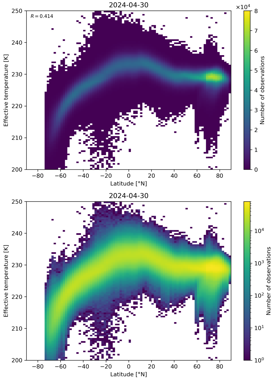
Figure 34: Scatter density plot of “Latitude” against “Effective temperature” for 2024-04-29 to 2024-05-01.
