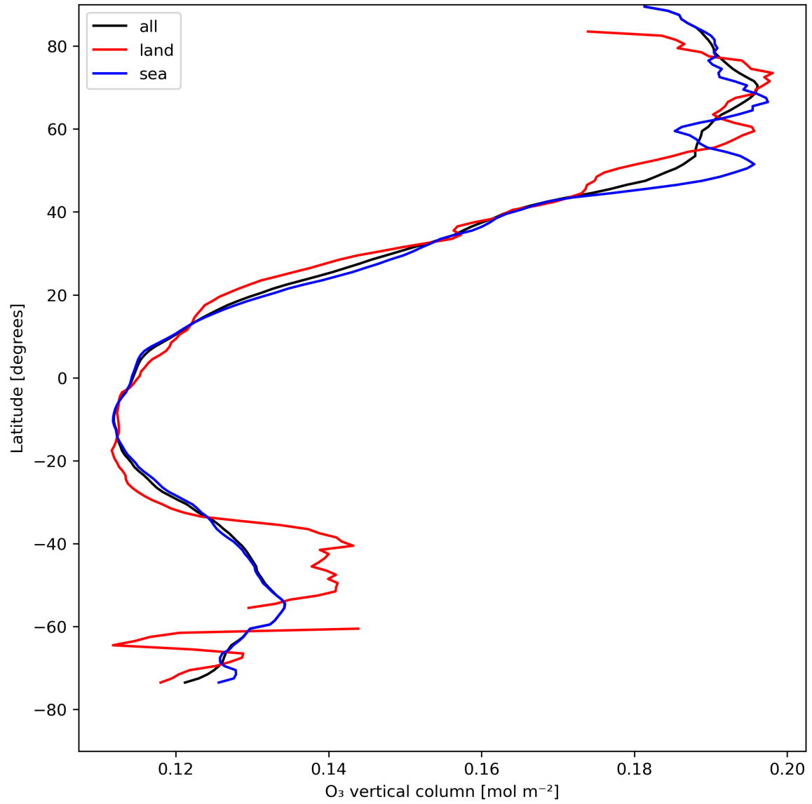
Figure 14: Zonal average of “O 3 vertical column” for 2024-04-29 to 2024-05-01.
