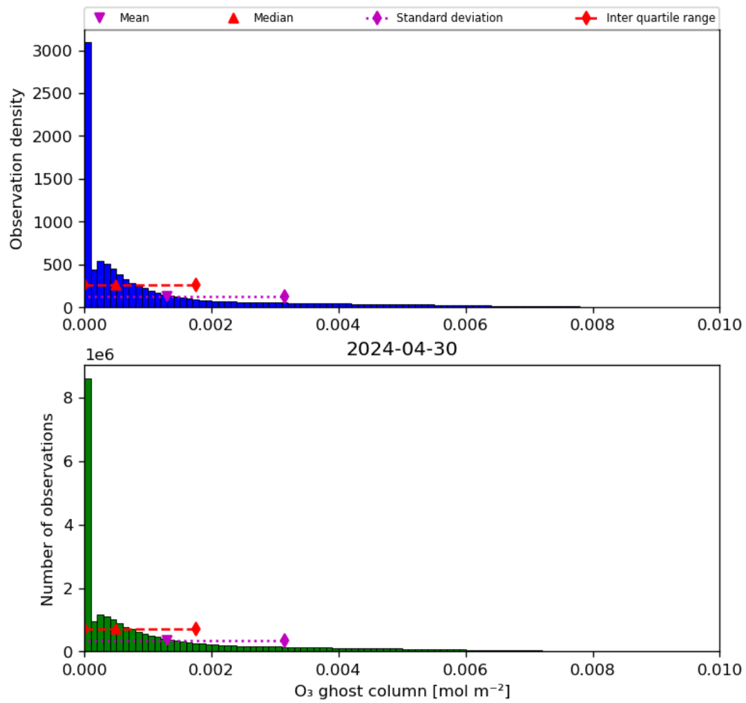
Figure 25: Histogram of “O 3 ghost column” for 2024-04-29 to 2024-05-01
