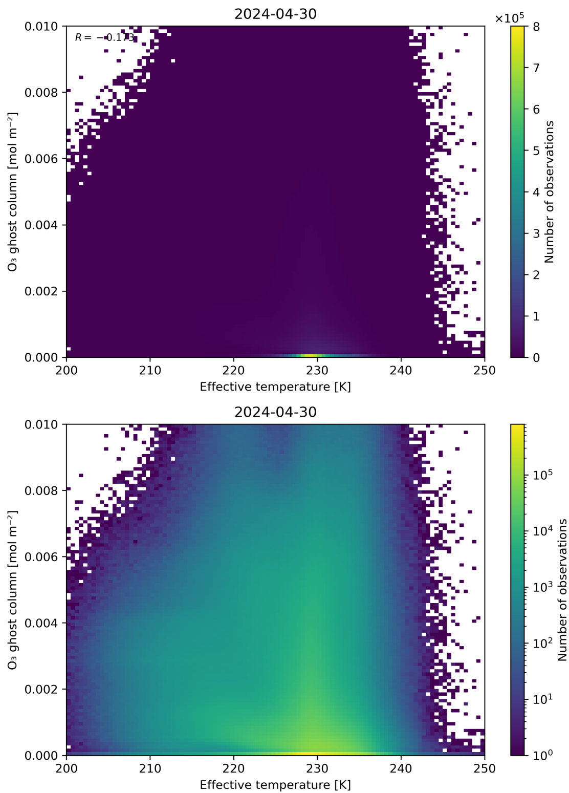
Figure 38: Scatter density plot of “Effective temperature” against “O 3 ghost column” for 2024-04-29 to 2024-05-01.
