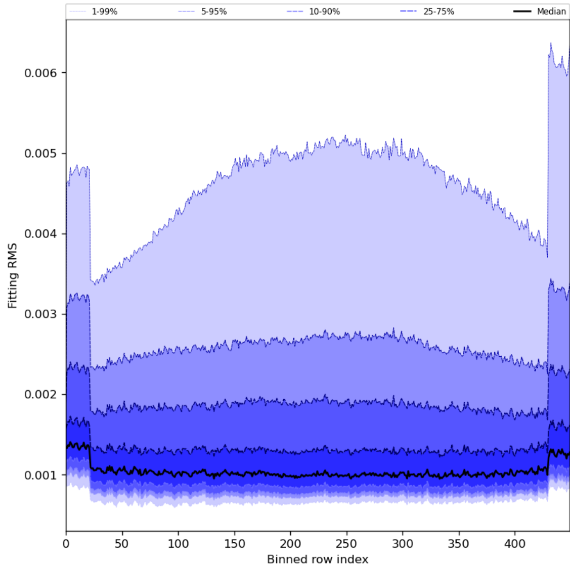
Figure 30: Along track statistics of “Fitting RMS” for 2024-04-29 to 2024-05-01
