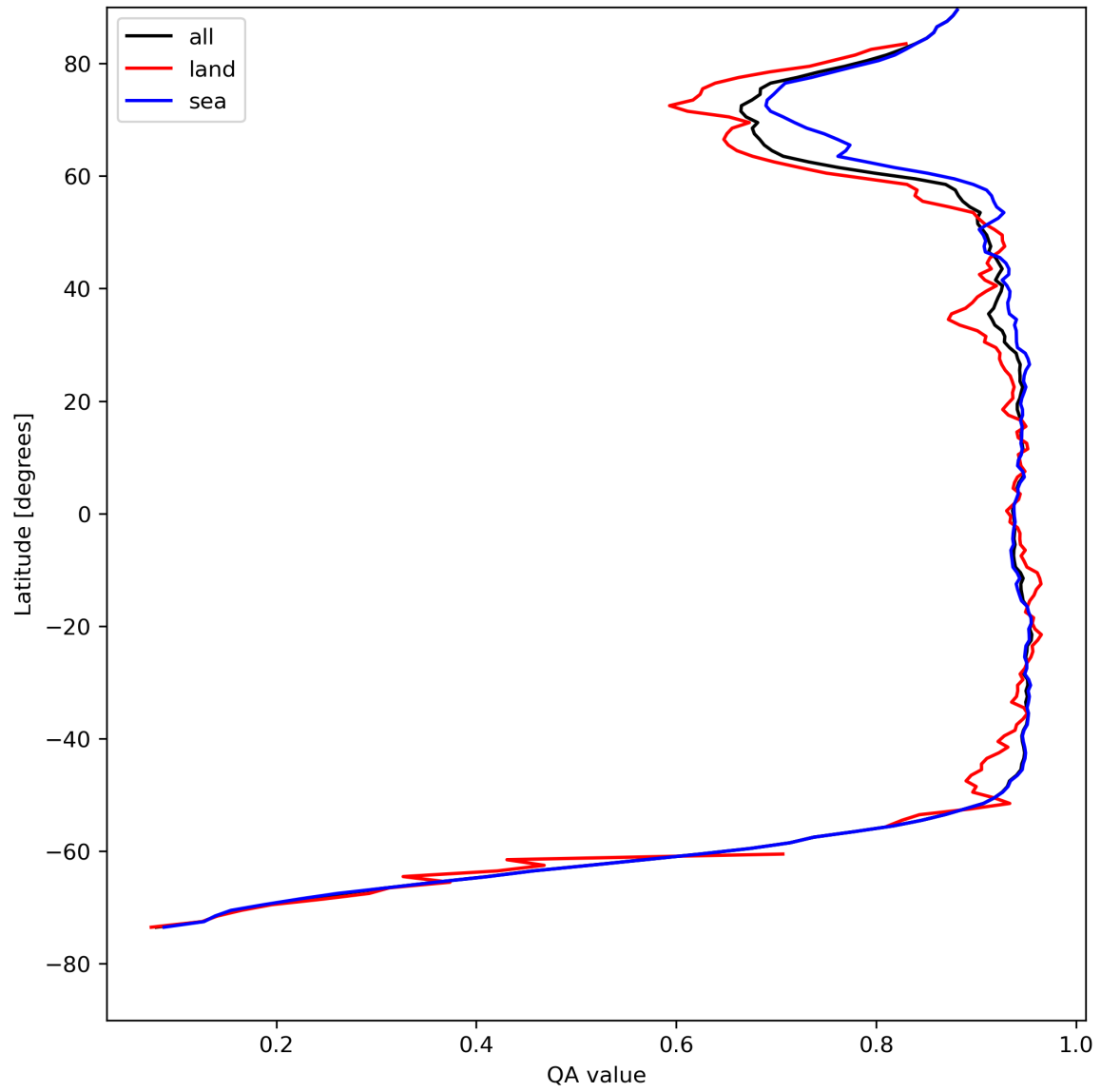
Figure 13: Zonal average of “QA value” for 2024-04-29 to 2024-05-01.
