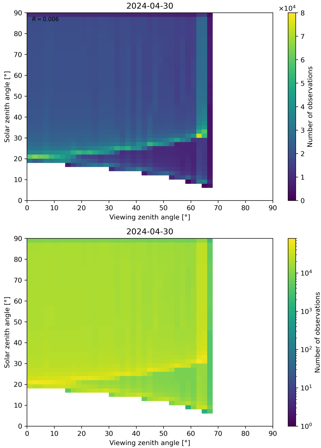
Figure 54: Scatter density plot of “Viewing zenith angle” against “Solar zenith angle” for 2024-04-29 to 2024-05-01.
