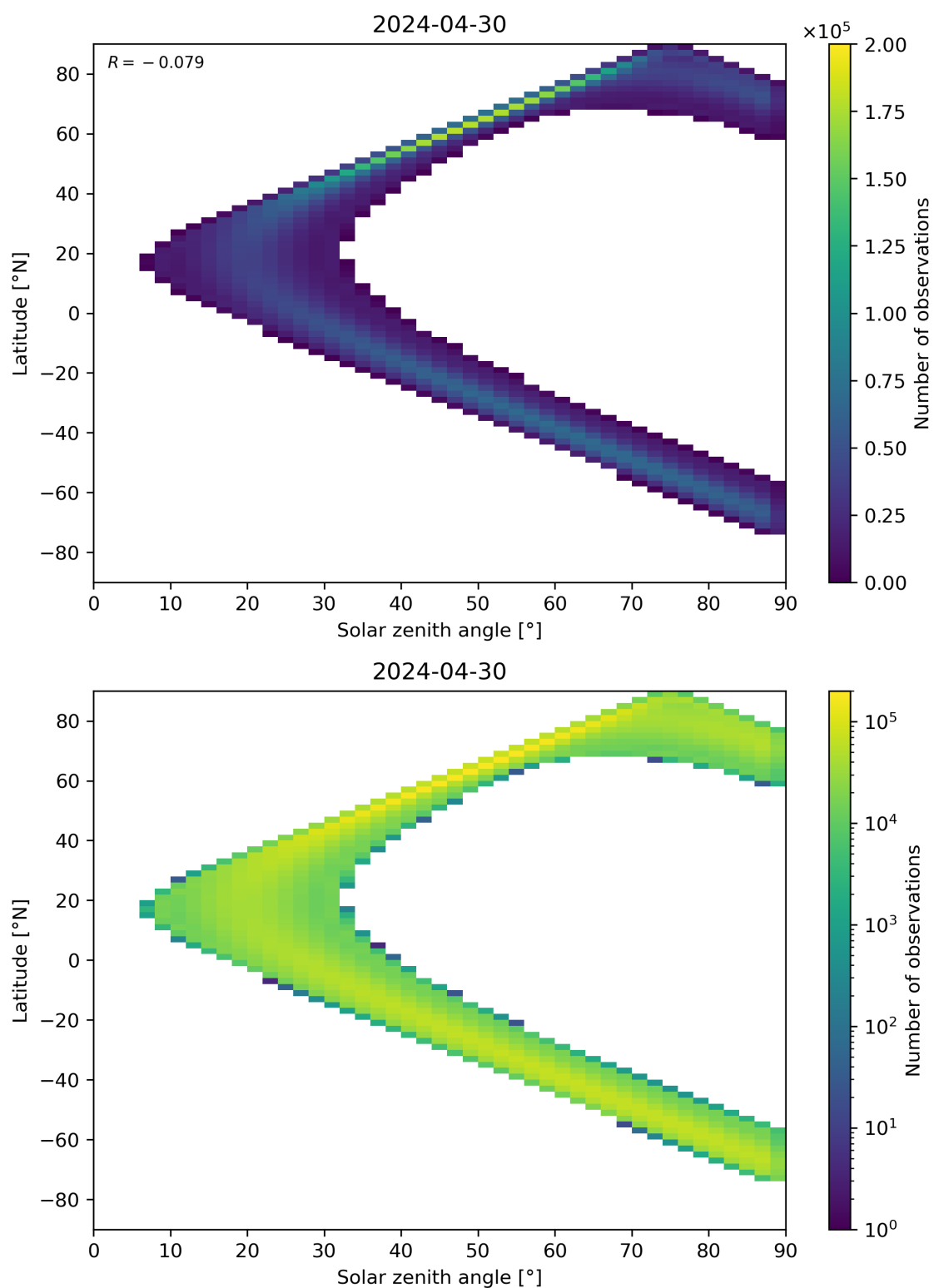
Figure 44: Scatter density plot of “Solar zenith angle” against “Latitude” for 2024-04-29 to 2024-05-01.
