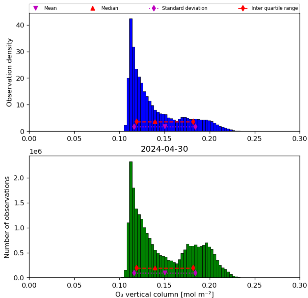
Figure 21: Histogram of “O 3 vertical column” for 2024-04-29 to 2024-05-01
