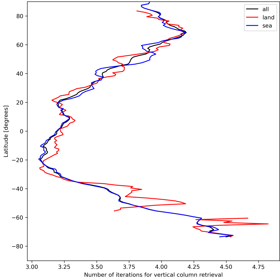
Figure 19: Zonal average of “Number of iterations for vertical column retrieval” for 2024-04-29 to 2024-05-01.
