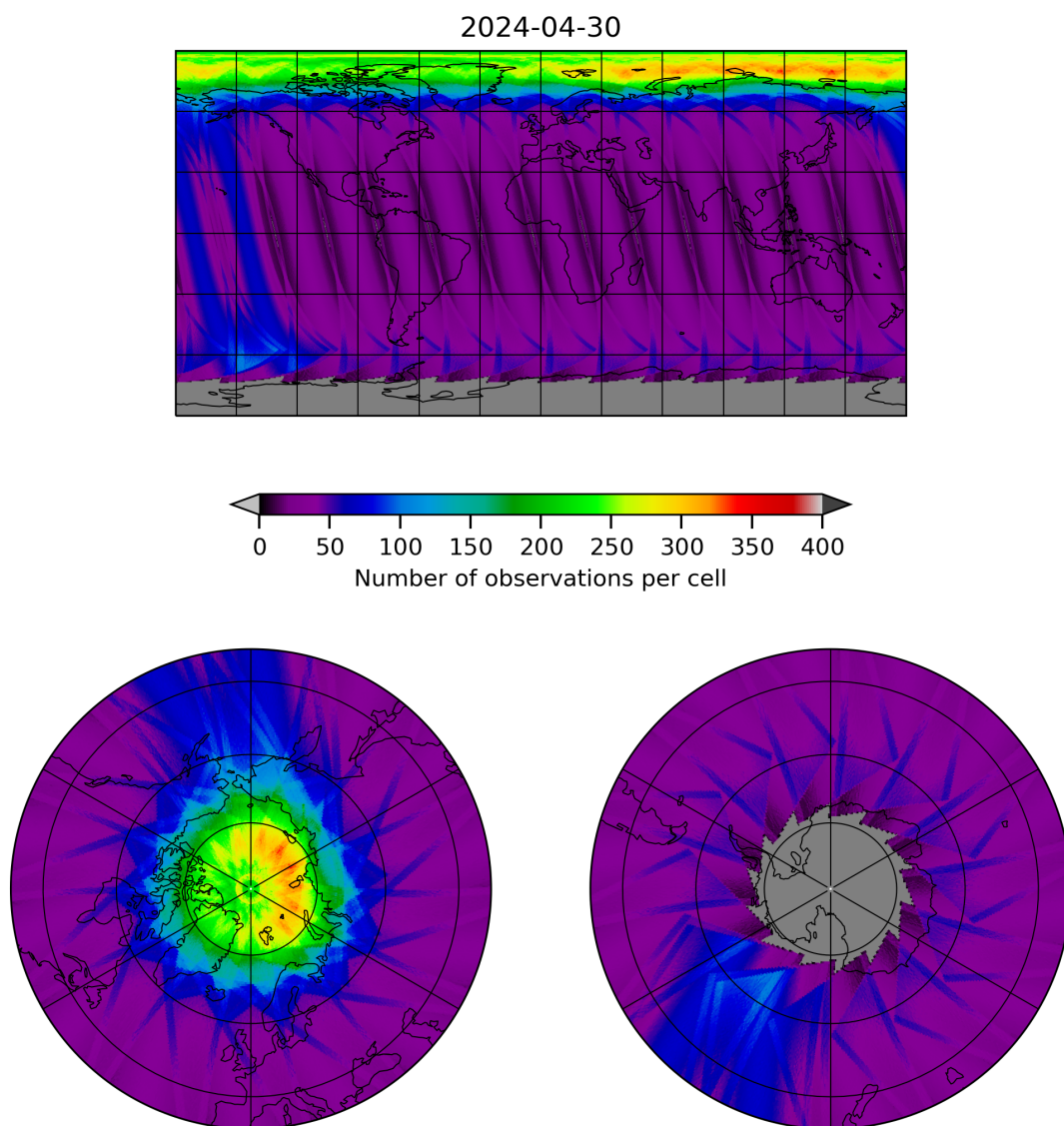
Figure 12: Map of the number of observations for 2024-04-29 to 2024-05-01
