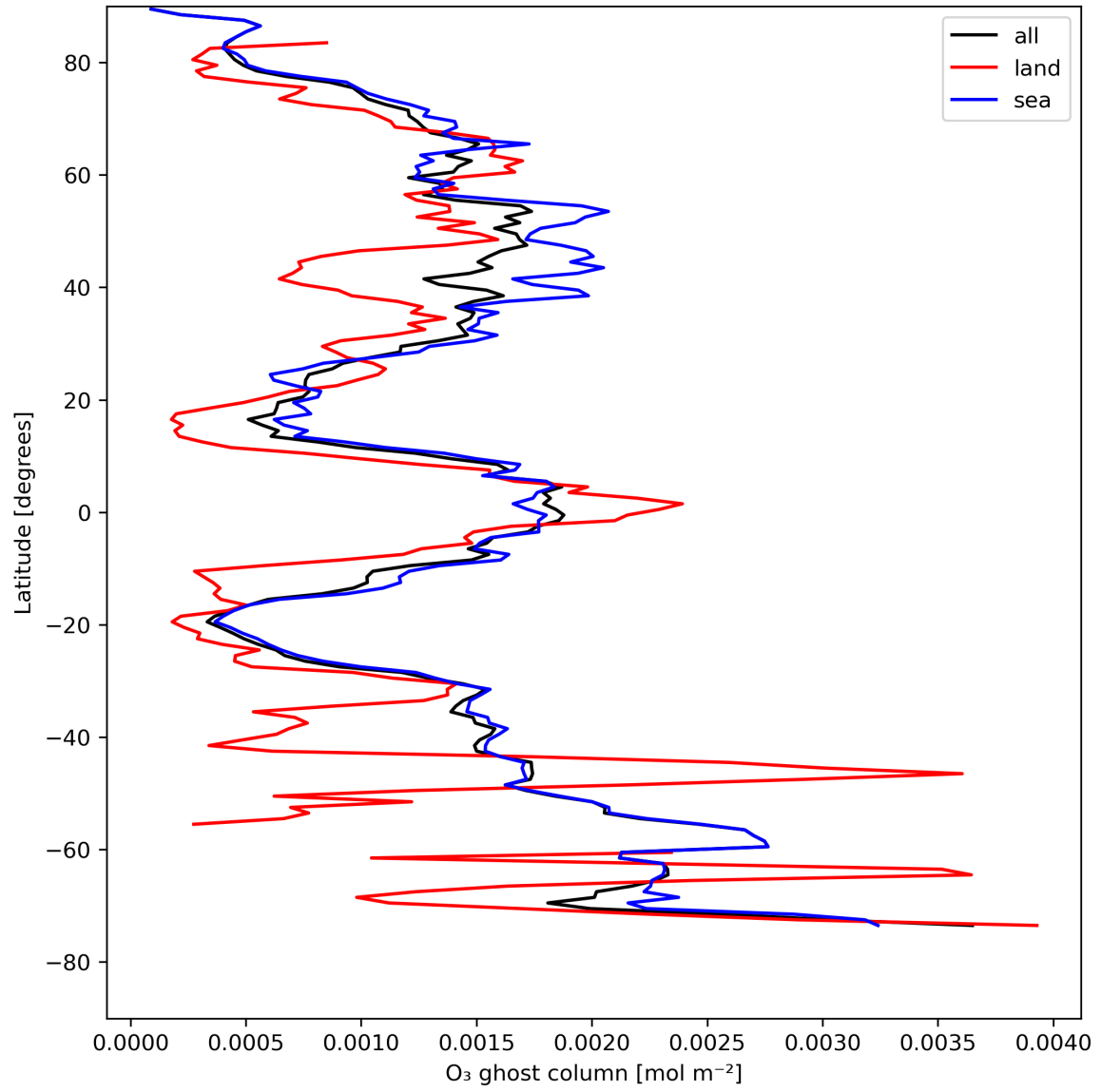
Figure 18: Zonal average of "O 3 ghost column" for 2024-04-29 to 2024-05-01.
