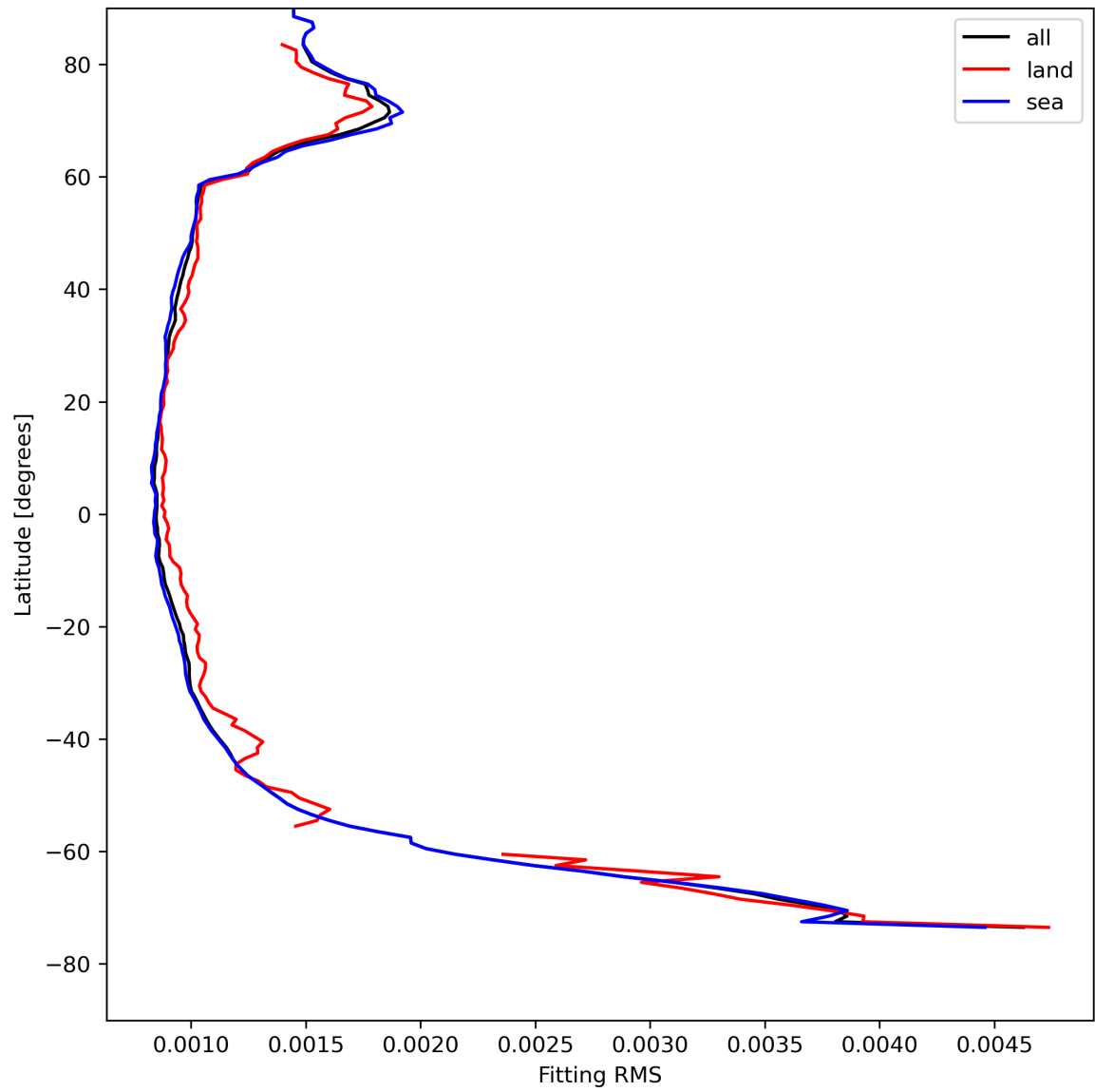
Figure 16: Zonal average of “Fitting RMS” for 2024-04-29 to 2024-05-01.
