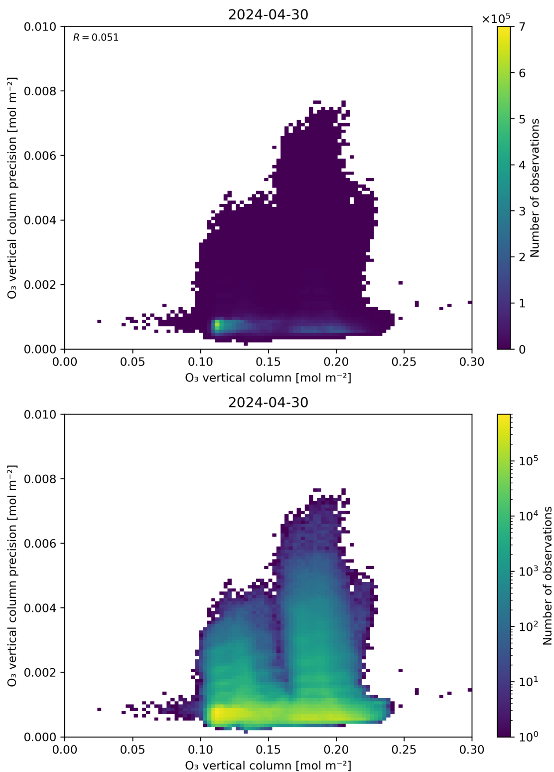
Figure 41: Scatter density plot of “O 3 vertical column” against “O 3 vertical column precision” for 2024-04-29 to 2024-05-01.
