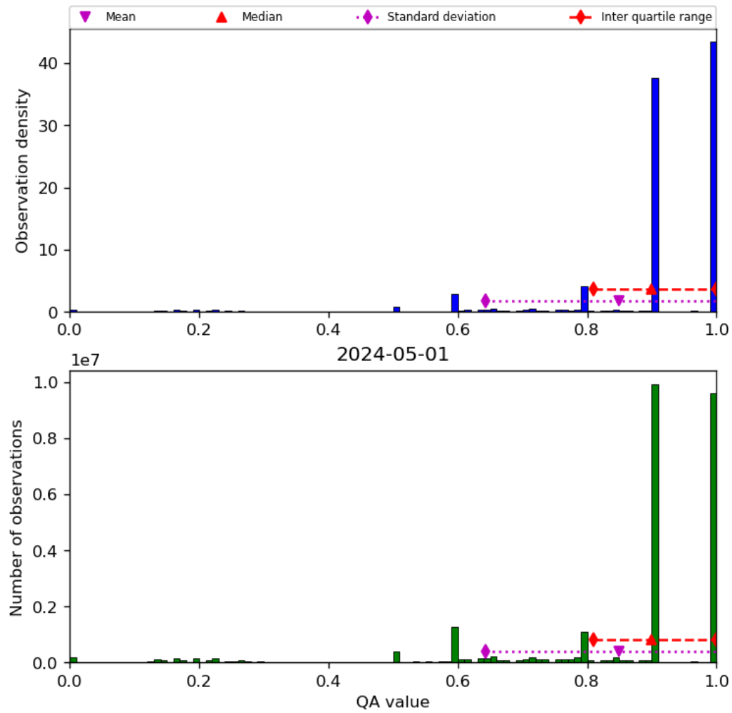
Figure 20: Histogram of “QA value” for 2024-04-30 to 2024-05-02
