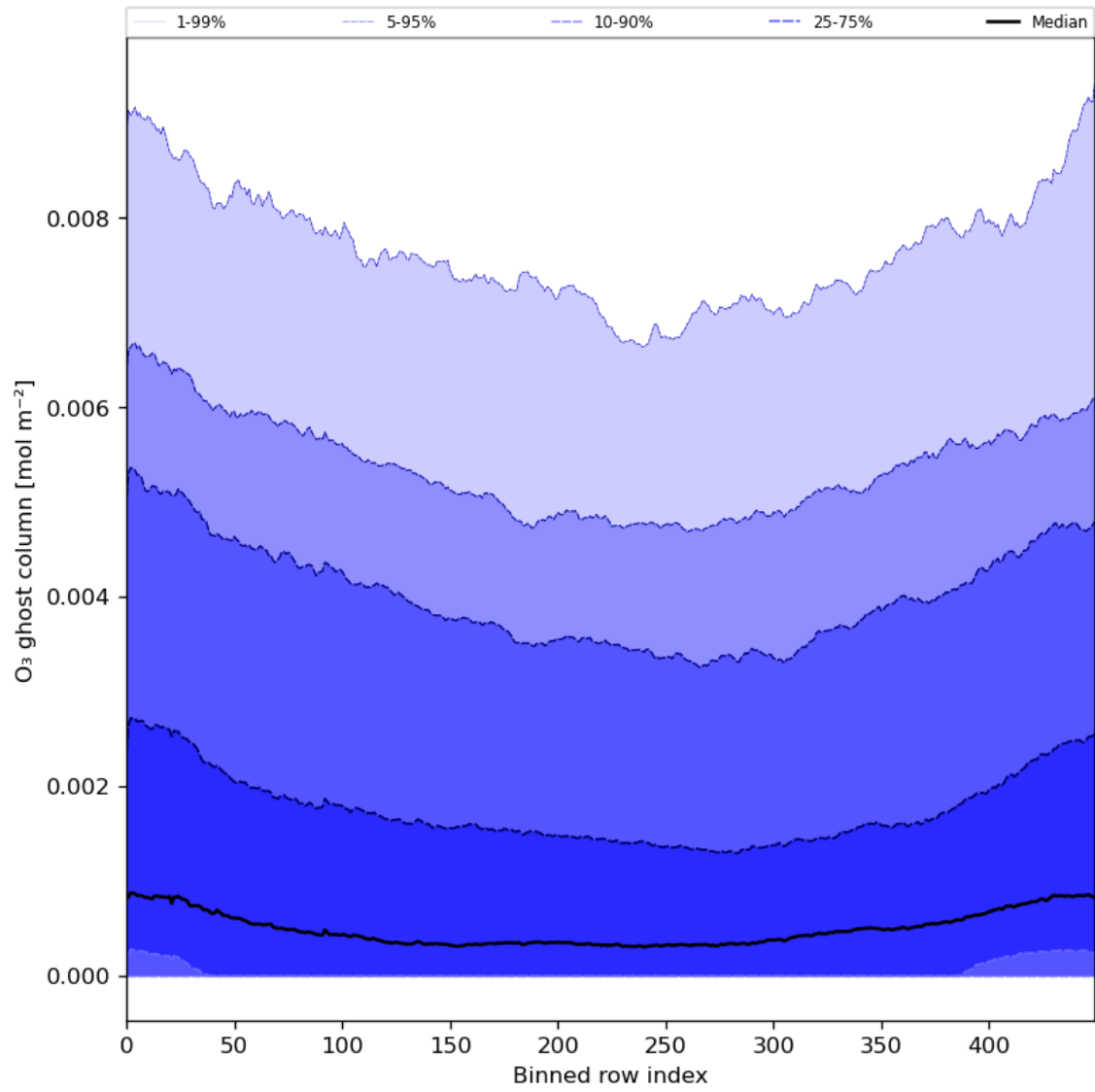
Figure 32: Along track statistics of “O 3 ghost column” for 2024-04-30 to 2024-05-02
