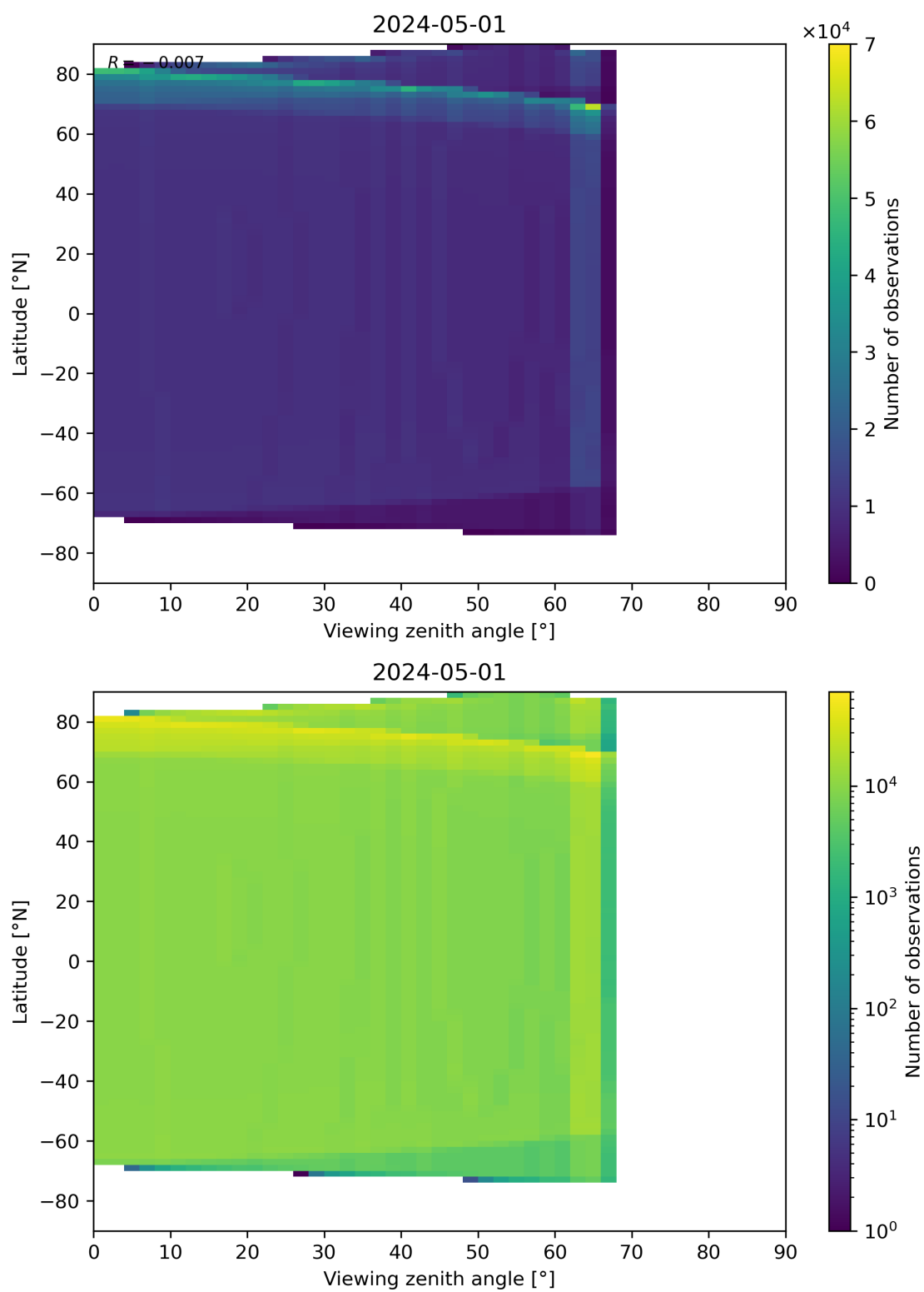
Figure 49: Scatter density plot of “Viewing zenith angle” against “Latitude” for 2024-04-30 to 2024-05-02.
