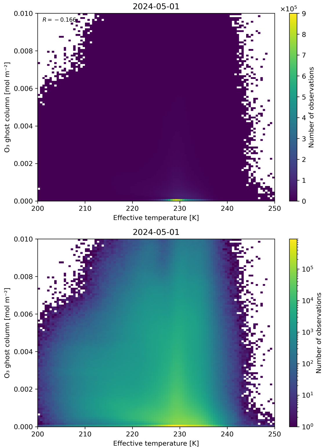
Figure 38: Scatter density plot of “Effective temperature” against “O 3 ghost column” for 2024-04-30 to 2024-05-02.
