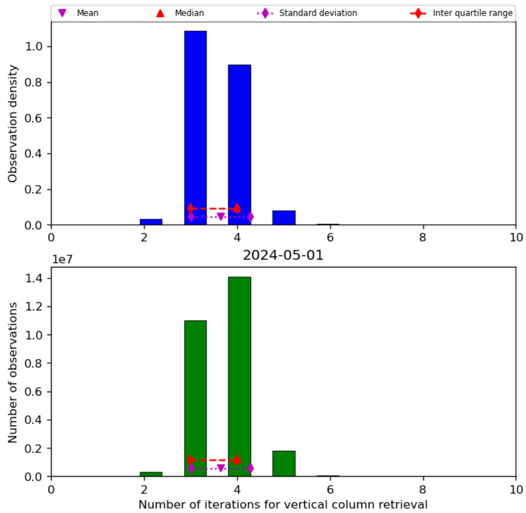
Figure 26: Histogram of “Number of iterations for vertical column retrieval” for 2024-04-30 to 2024-05-02
