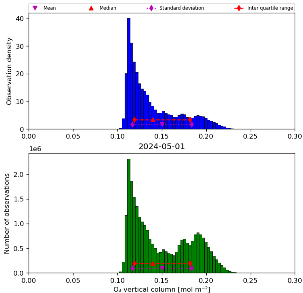
Figure 21: Histogram of “O 3 vertical column” for 2024-04-30 to 2024-05-02
