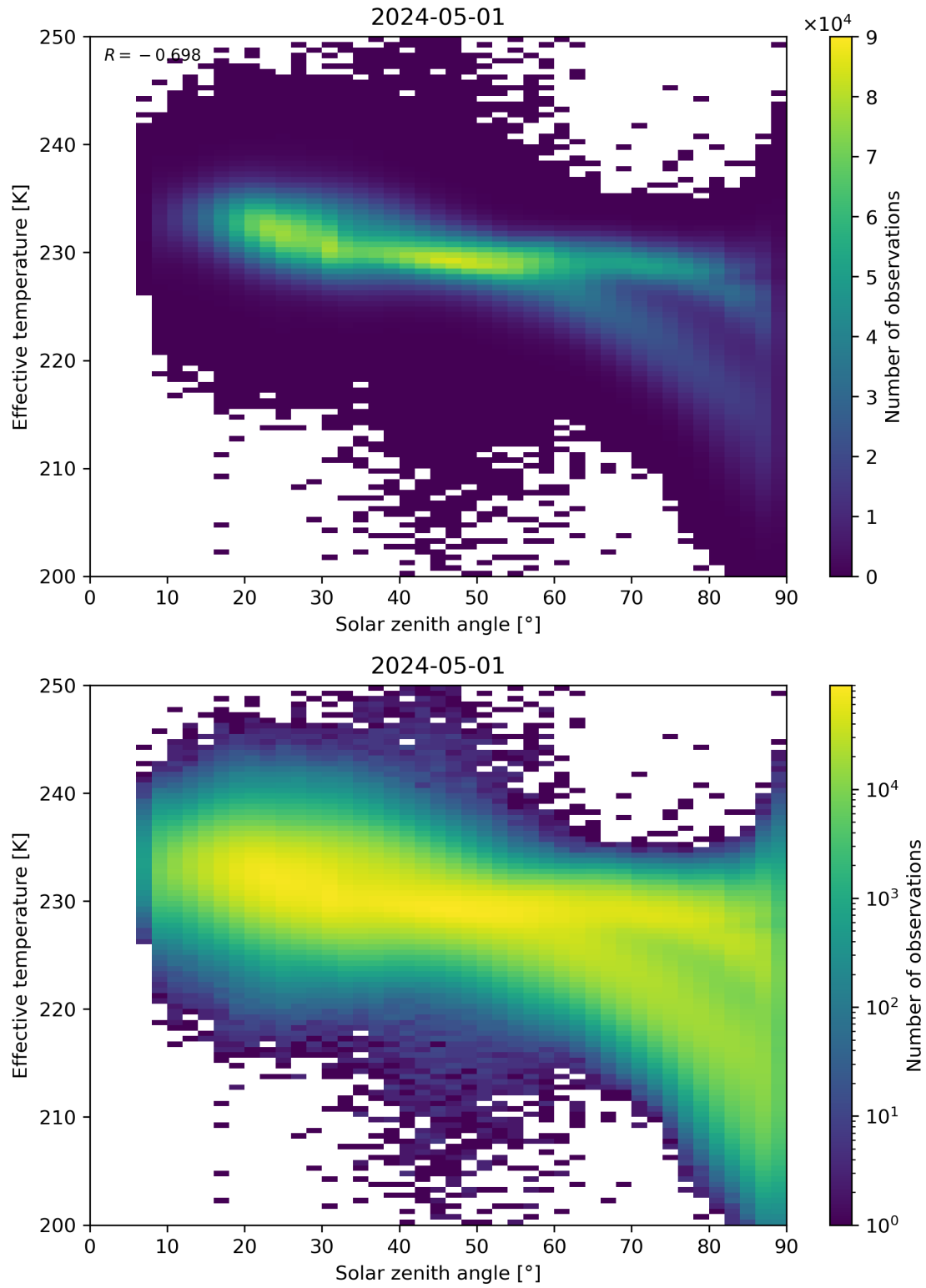
Figure 45: Scatter density plot of “Solar zenith angle” against “Effective temperature” for 2024-04-30 to 2024-05-02.
