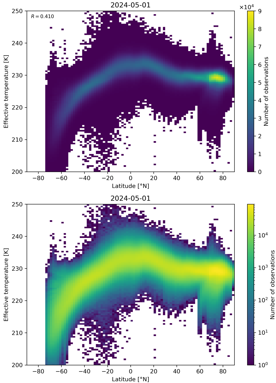
Figure 34: Scatter density plot of “Latitude” against “Effective temperature” for 2024-04-30 to 2024-05-02.
