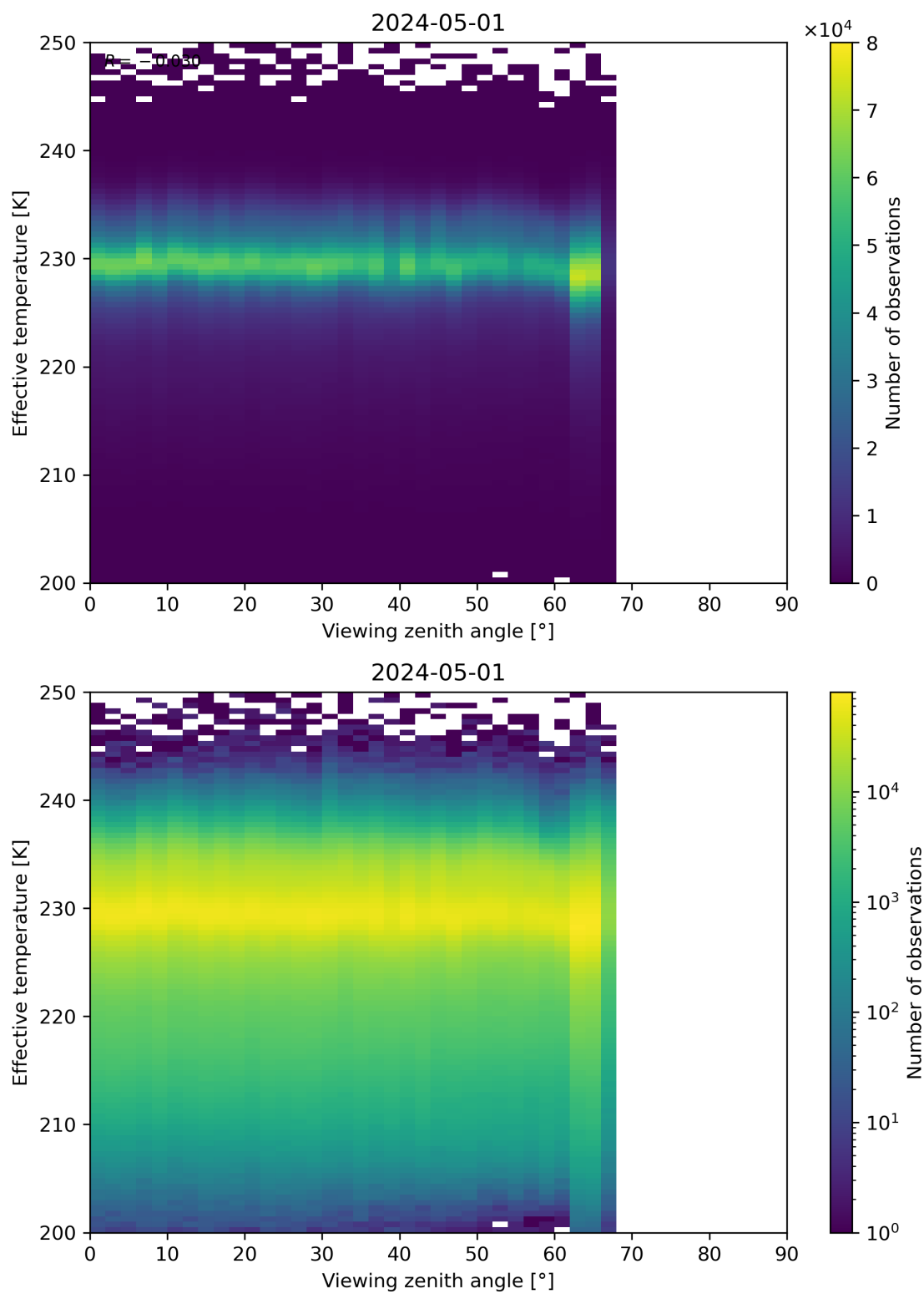
Figure 50: Scatter density plot of “Viewing zenith angle” against “Effective temperature” for 2024-04-30 to 2024-05-02.
