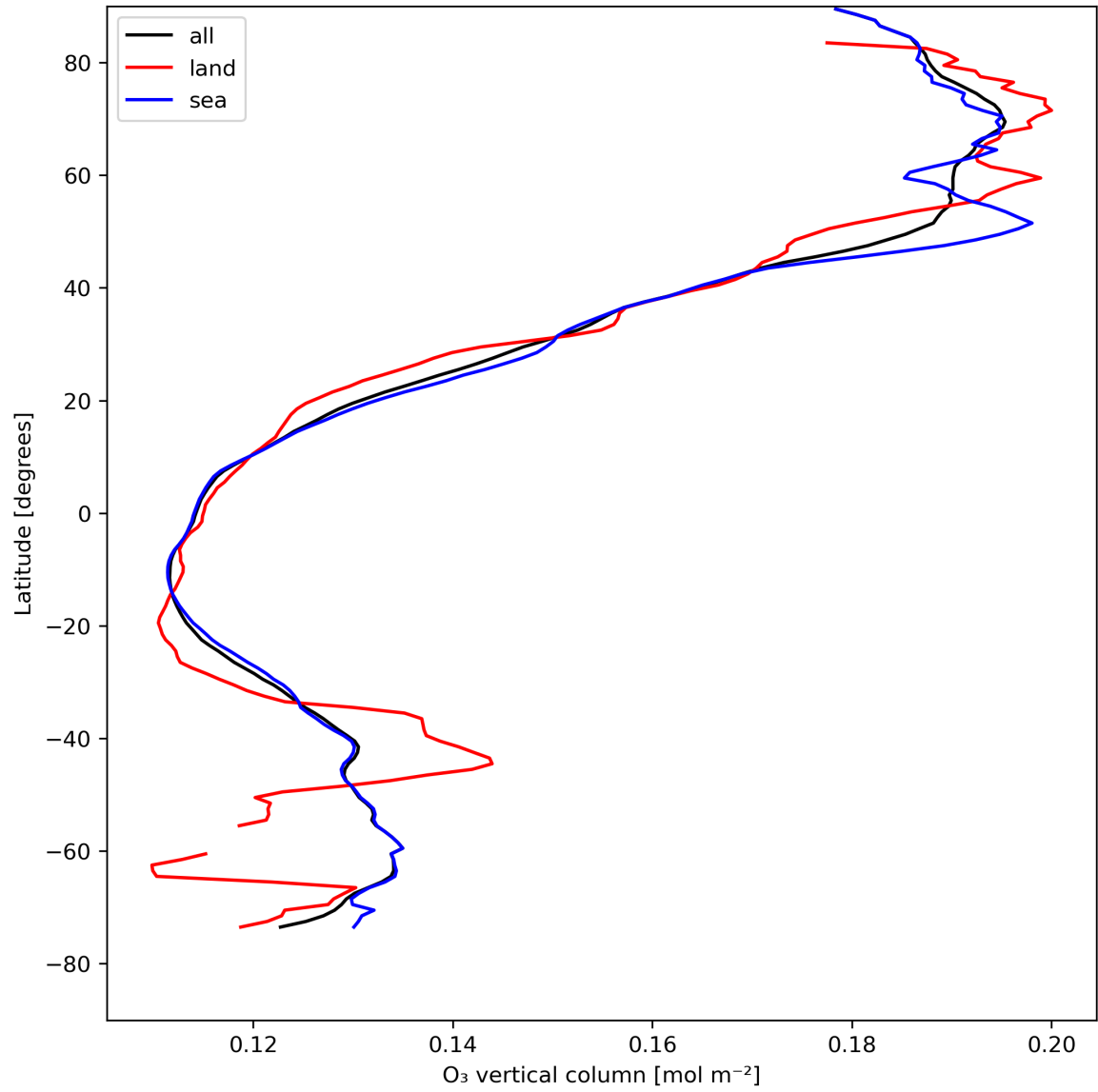
Figure 14: Zonal average of “O 3 vertical column” for 2024-04-30 to 2024-05-02.
