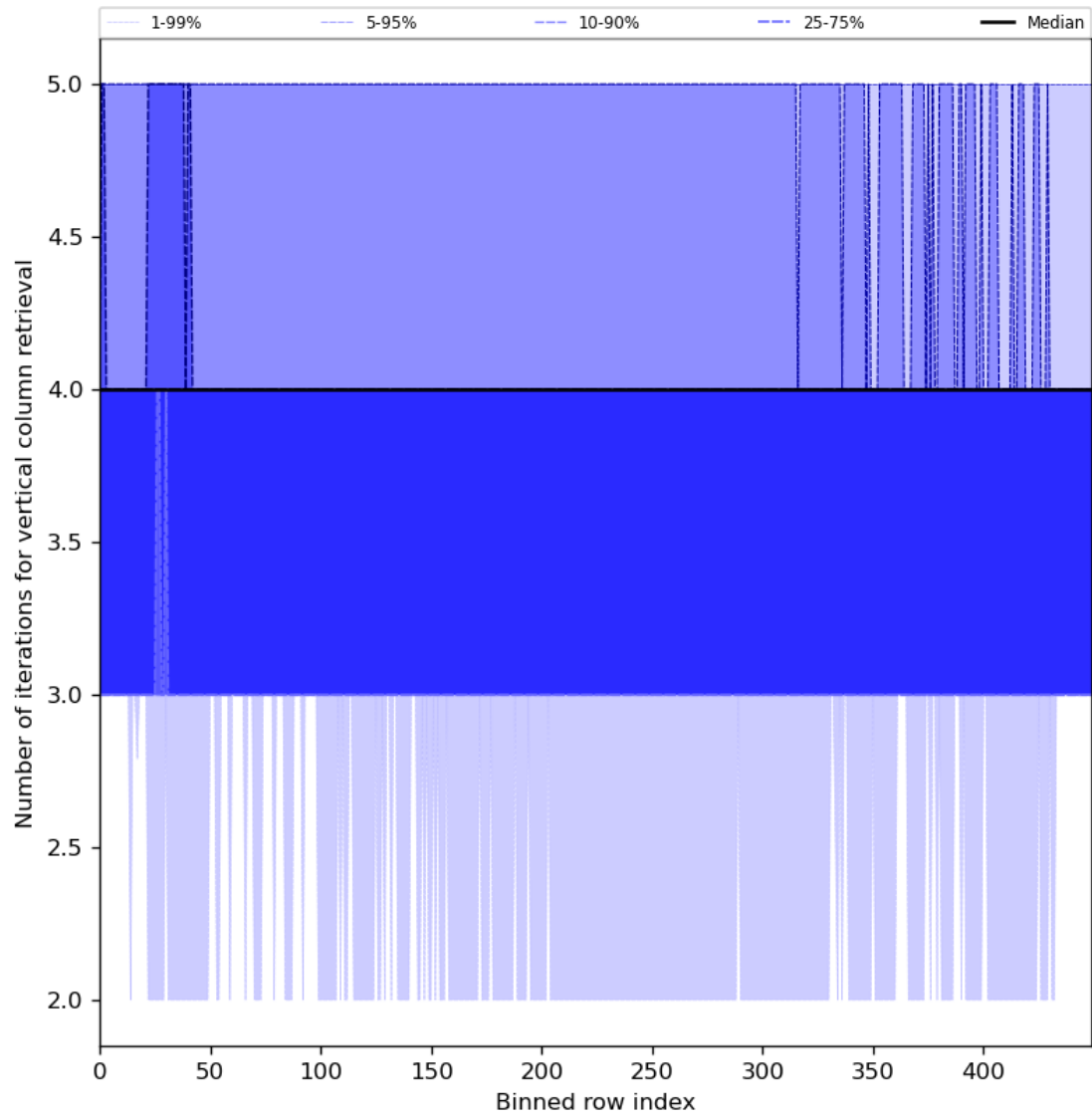
Figure 33: Along track statistics of “Number of iterations for vertical column retrieval” for 2024-04-30 to 2024-05-02
