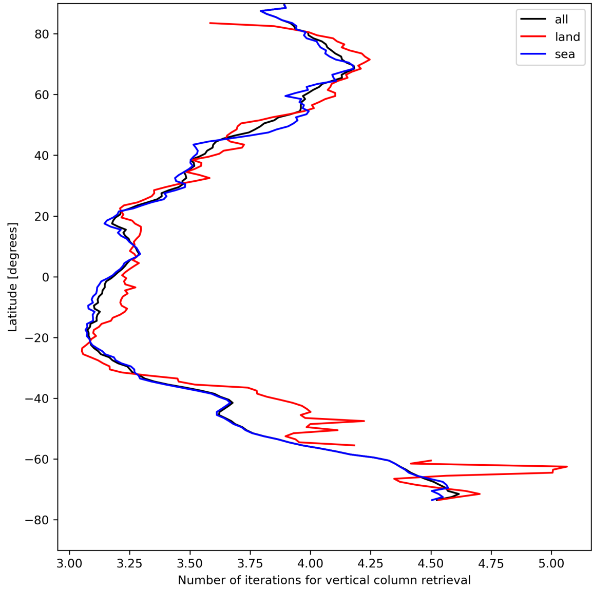
Figure 19: Zonal average of “Number of iterations for vertical column retrieval” for 2024-04-30 to 2024-05-02.
