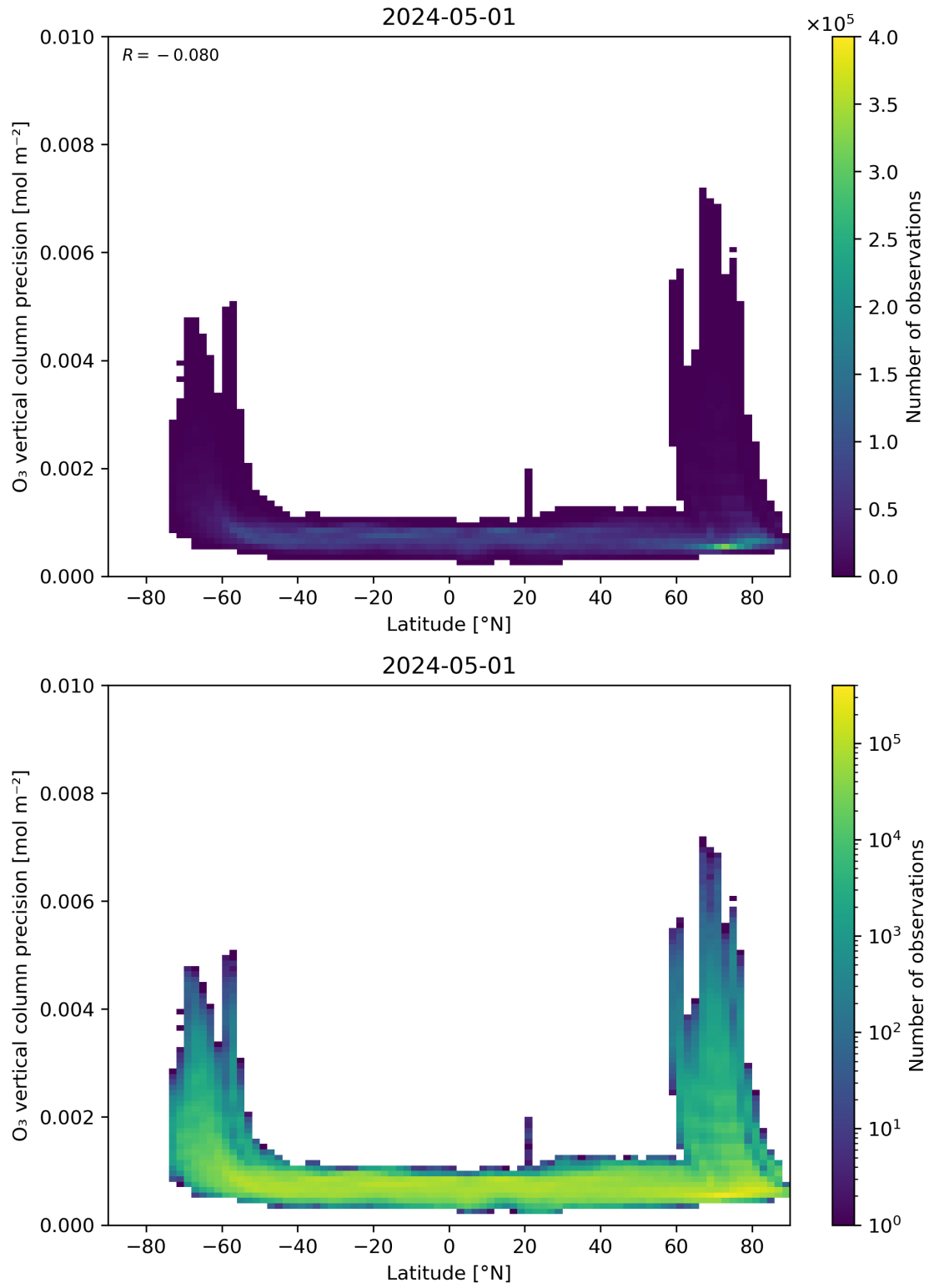
Figure 37: Scatter density plot of “Latitude” against “O 3 vertical column precision” for 2024-04-30 to 2024-05-02.
