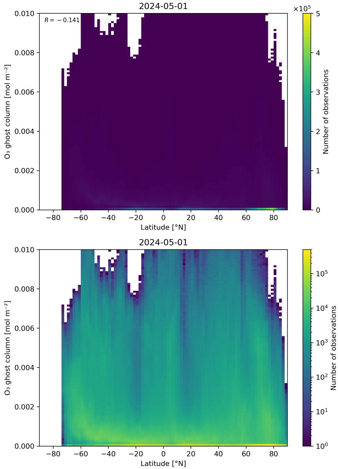
Figure 35: Scatter density plot of “Latitude” against “O 3 ghost column” for 2024-04-30 to 2024-05-02.
