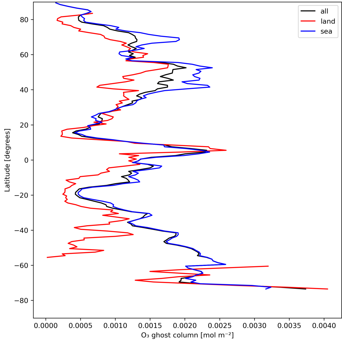
Figure 18: Zonal average of "O 3 ghost column" for 2024-04-30 to 2024-05-02.
