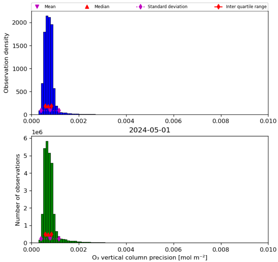
Figure 22: Histogram of “O 3 vertical column precision” for 2024-04-30 to 2024-05-02
