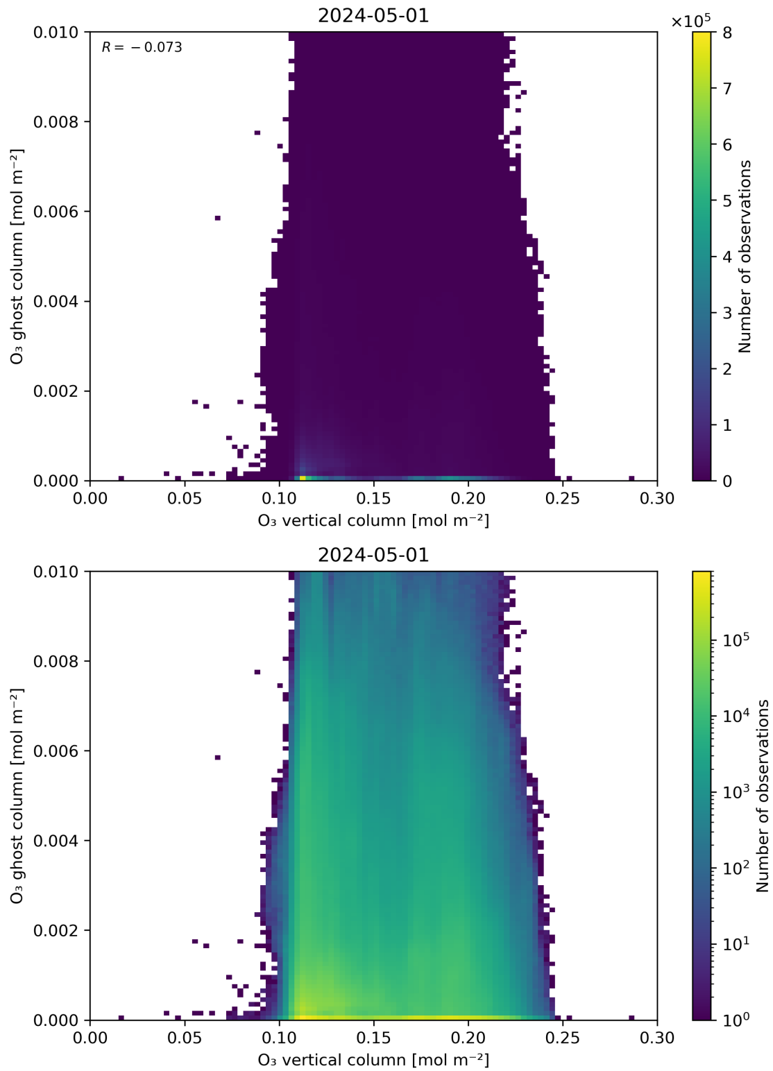
Figure 40: Scatter density plot of “O 3 vertical column” against “O 3 ghost column” for 2024-04-30 to 2024-05-02.
