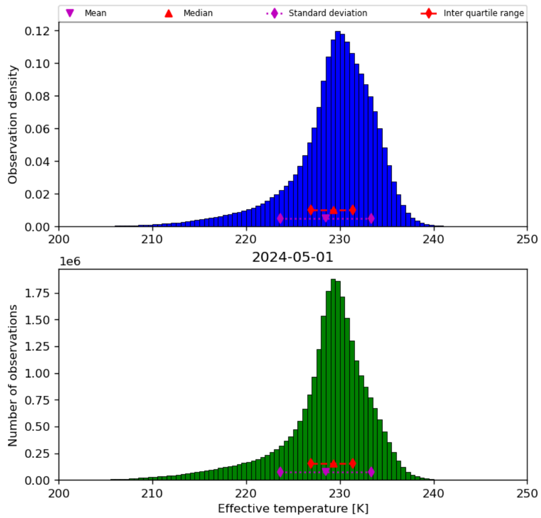
Figure 24: Histogram of “Effective temperature” for 2024-04-30 to 2024-05-02
