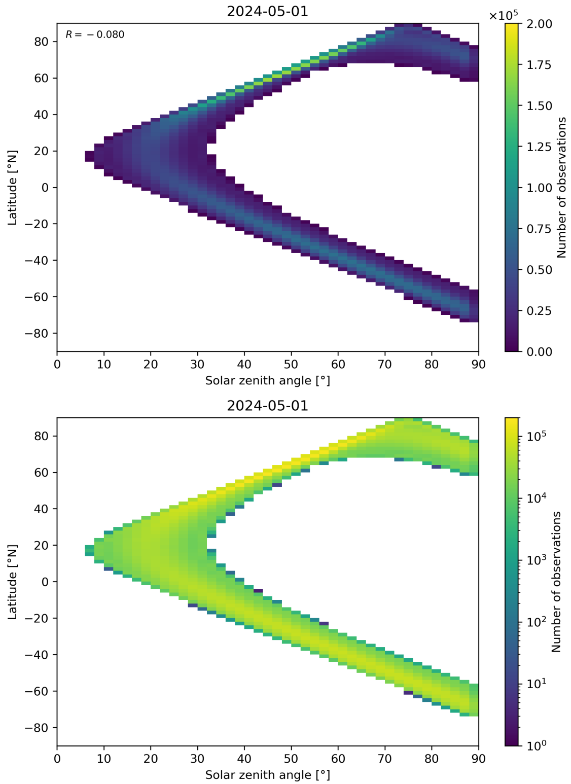
Figure 44: Scatter density plot of “Solar zenith angle” against “Latitude” for 2024-04-30 to 2024-05-02.
