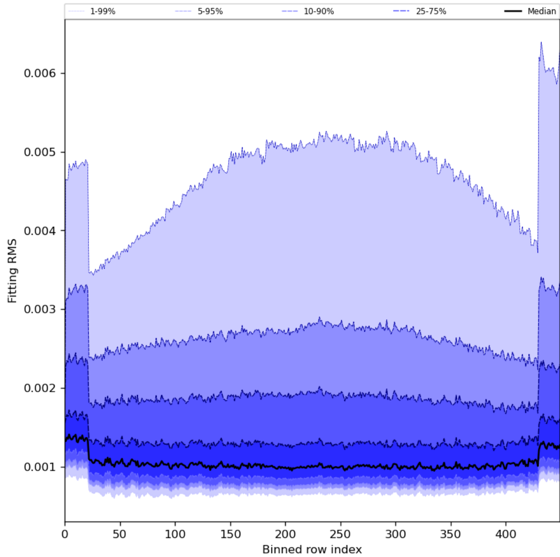
Figure 30: Along track statistics of “Fitting RMS” for 2024-04-30 to 2024-05-02
