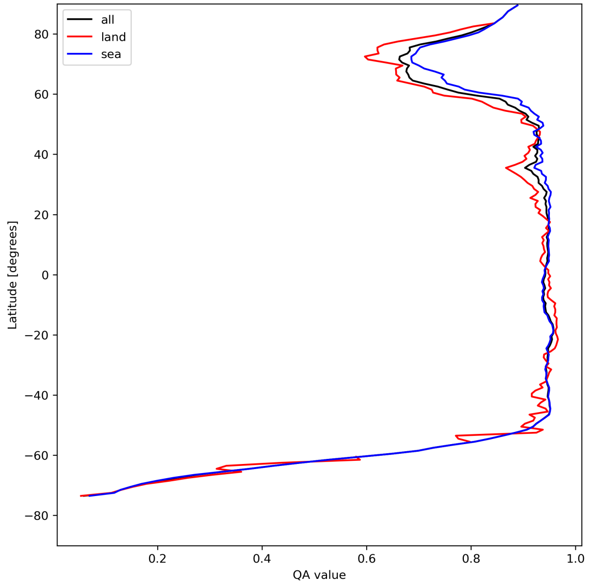
Figure 13: Zonal average of “QA value” for 2024-04-30 to 2024-05-02.
