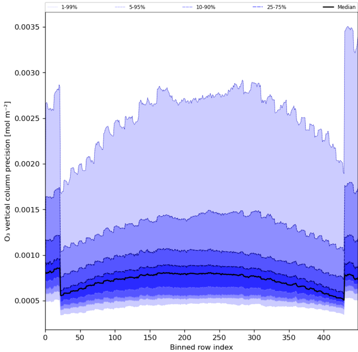
Figure 29: Along track statistics of “O 3 vertical column precision” for 2024-04-30 to 2024-05-02
