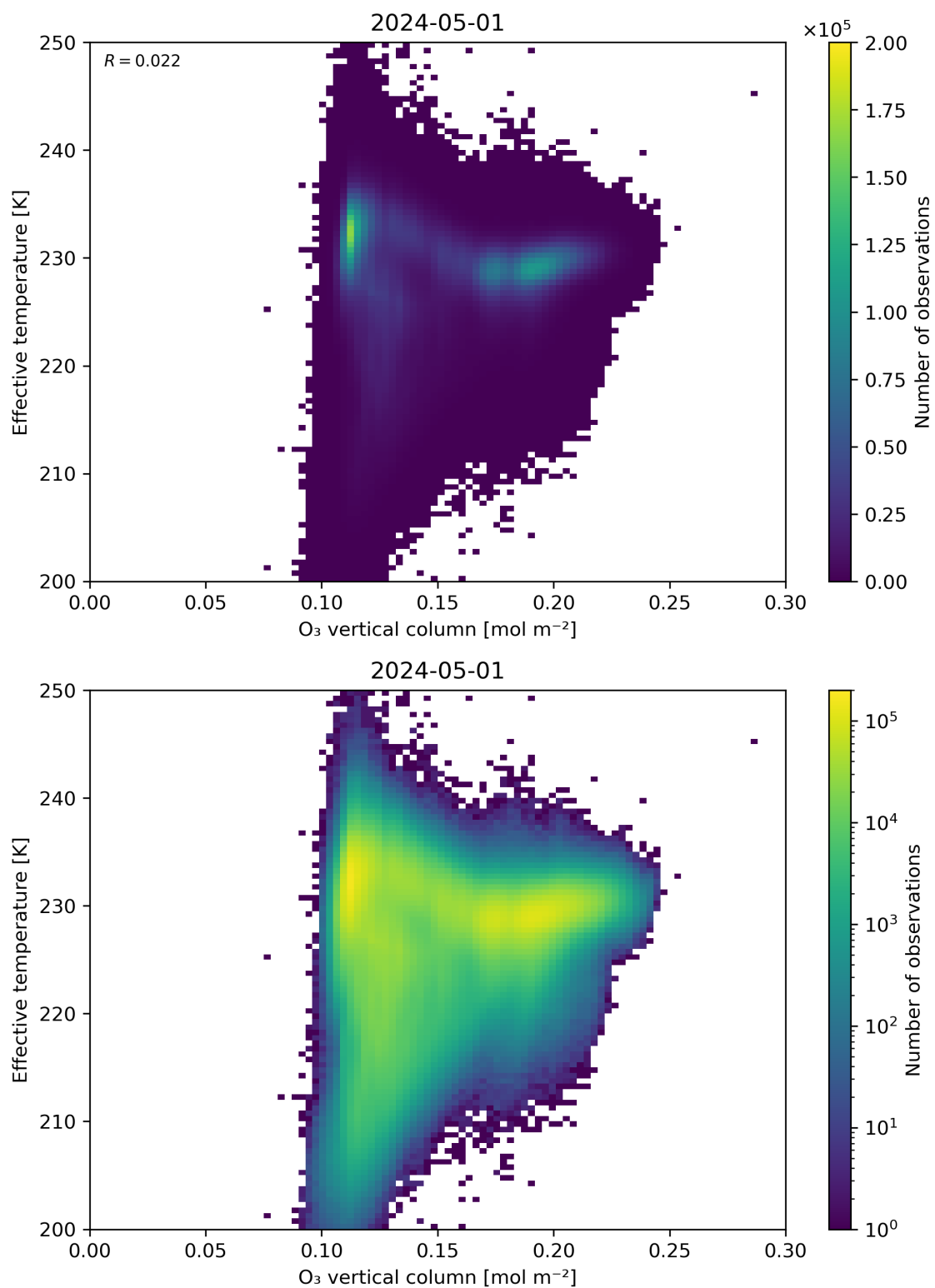
Figure 39: Scatter density plot of “O 3 vertical column” against “Effective temperature” for 2024-04-30 to 2024-05-02.
