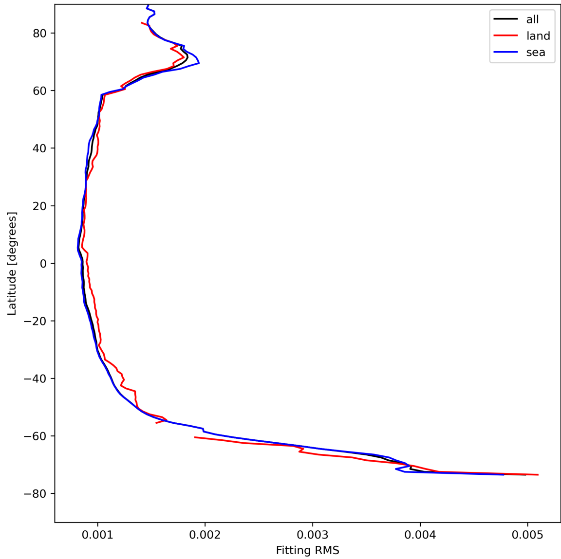
Figure 16: Zonal average of “Fitting RMS” for 2024-04-30 to 2024-05-02.
