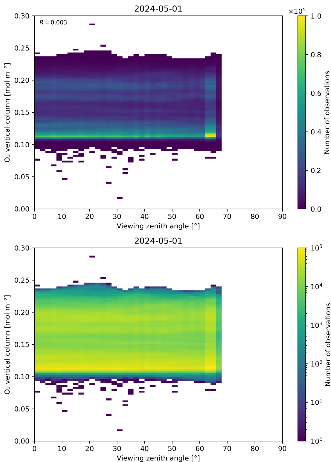
Figure 52: Scatter density plot of “Viewing zenith angle” against “O 3 vertical column” for 2024-04-30 to 2024-05-02.
