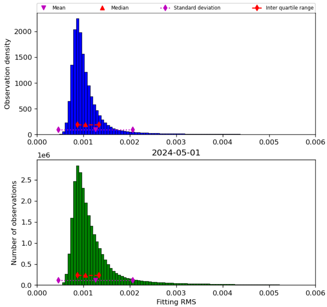
Figure 23: Histogram of “Fitting RMS” for 2024-04-30 to 2024-05-02
