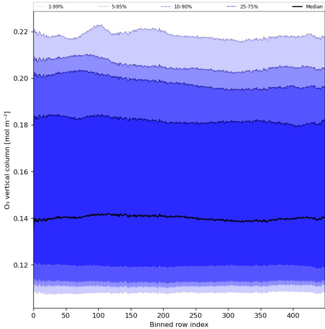
Figure 28: Along track statistics of “ \text{O}_3 vertical column” for 2024-04-30 to 2024-05-02
