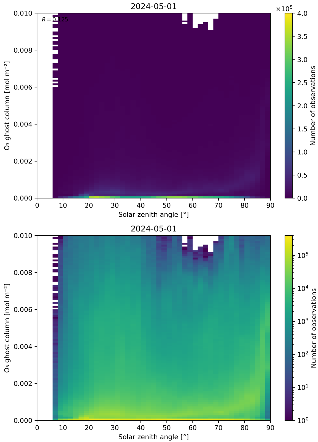
Figure 46: Scatter density plot of “Solar zenith angle” against “O 3 ghost column” for 2024-04-30 to 2024-05-02.
