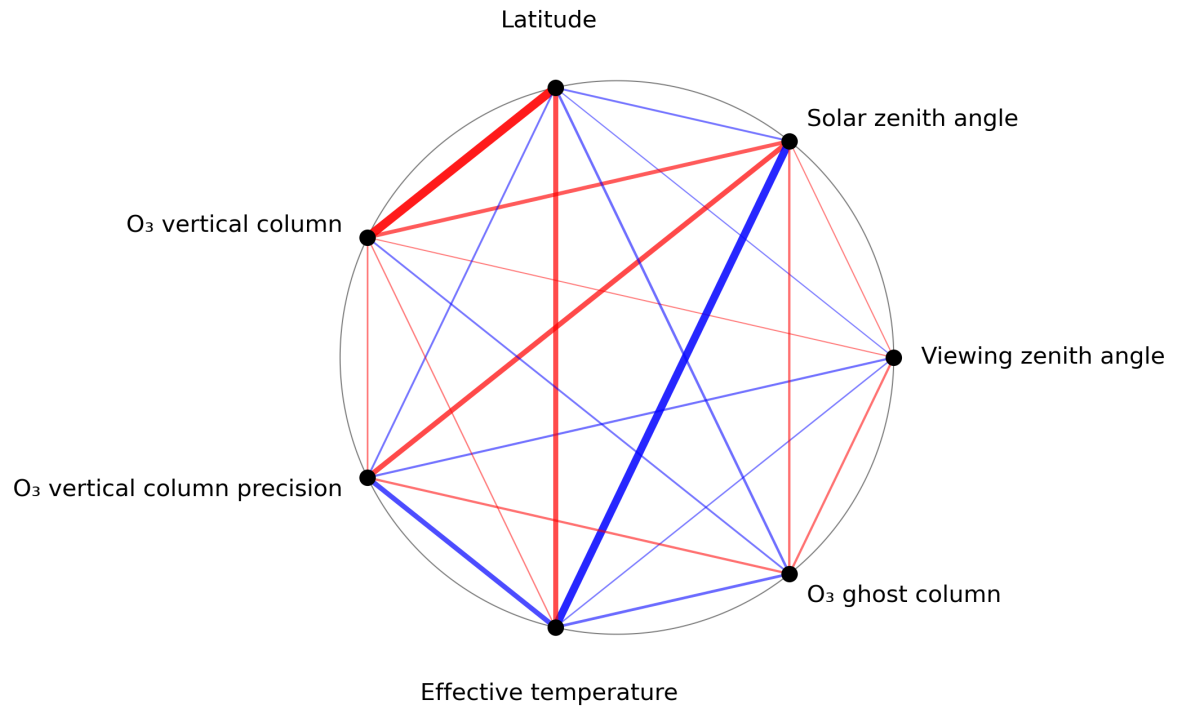
Figure 1: Map of correlation graph for 2024-04-30 to 2024-05-02.
