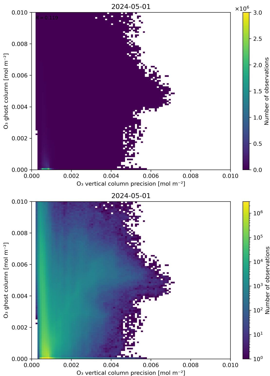
Figure 43: Scatter density plot of “O 3 vertical column precision” against “O 3 ghost column” for 2024-04-30 to 2024-05-02.
