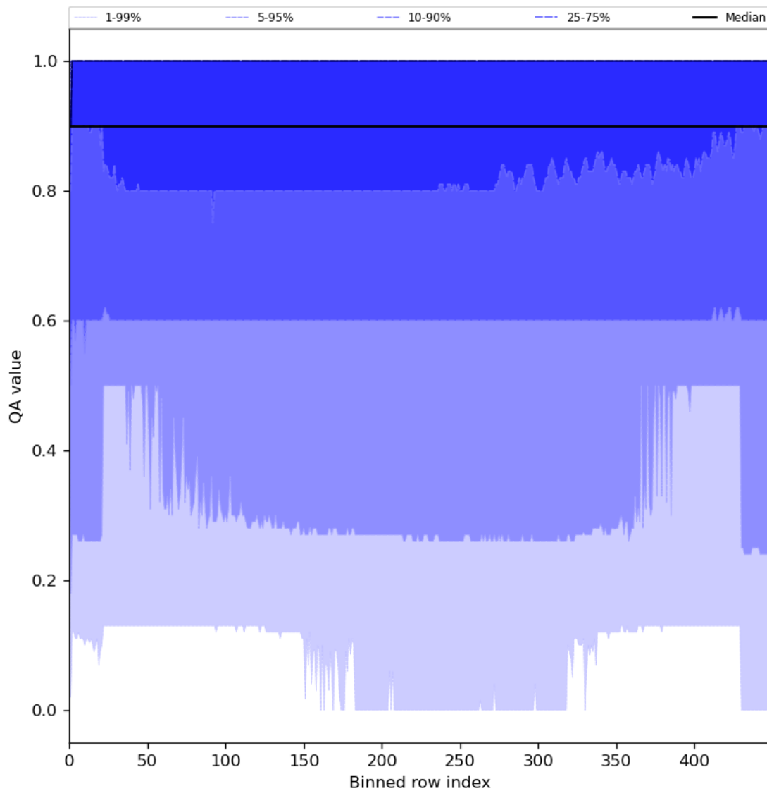
Figure 27: Along track statistics of “QA value” for 2024-04-30 to 2024-05-02
