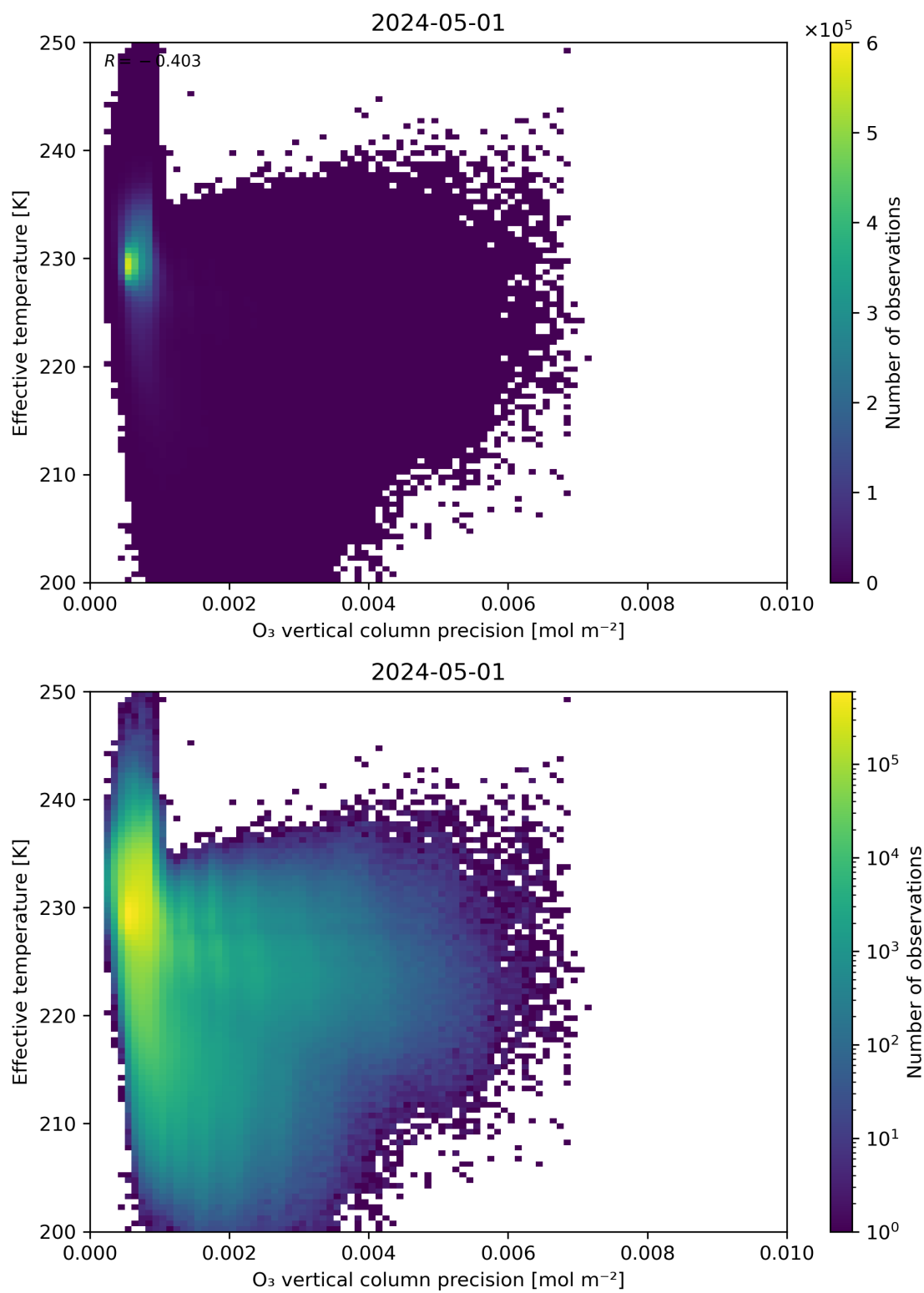
Figure 42: Scatter density plot of “O 3 vertical column precision” against “Effective temperature” for 2024-04-30 to 2024-05-02.
