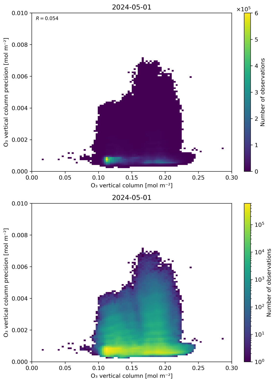
Figure 41: Scatter density plot of “O 3 vertical column” against “O 3 vertical column precision” for 2024-04-30 to 2024-05-02.
