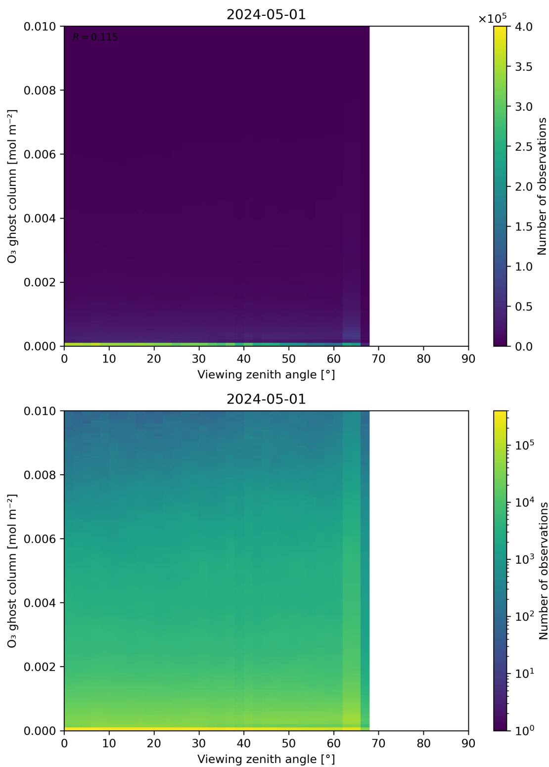
Figure 51: Scatter density plot of “Viewing zenith angle” against “O 3 ghost column” for 2024-04-30 to 2024-05-02.
