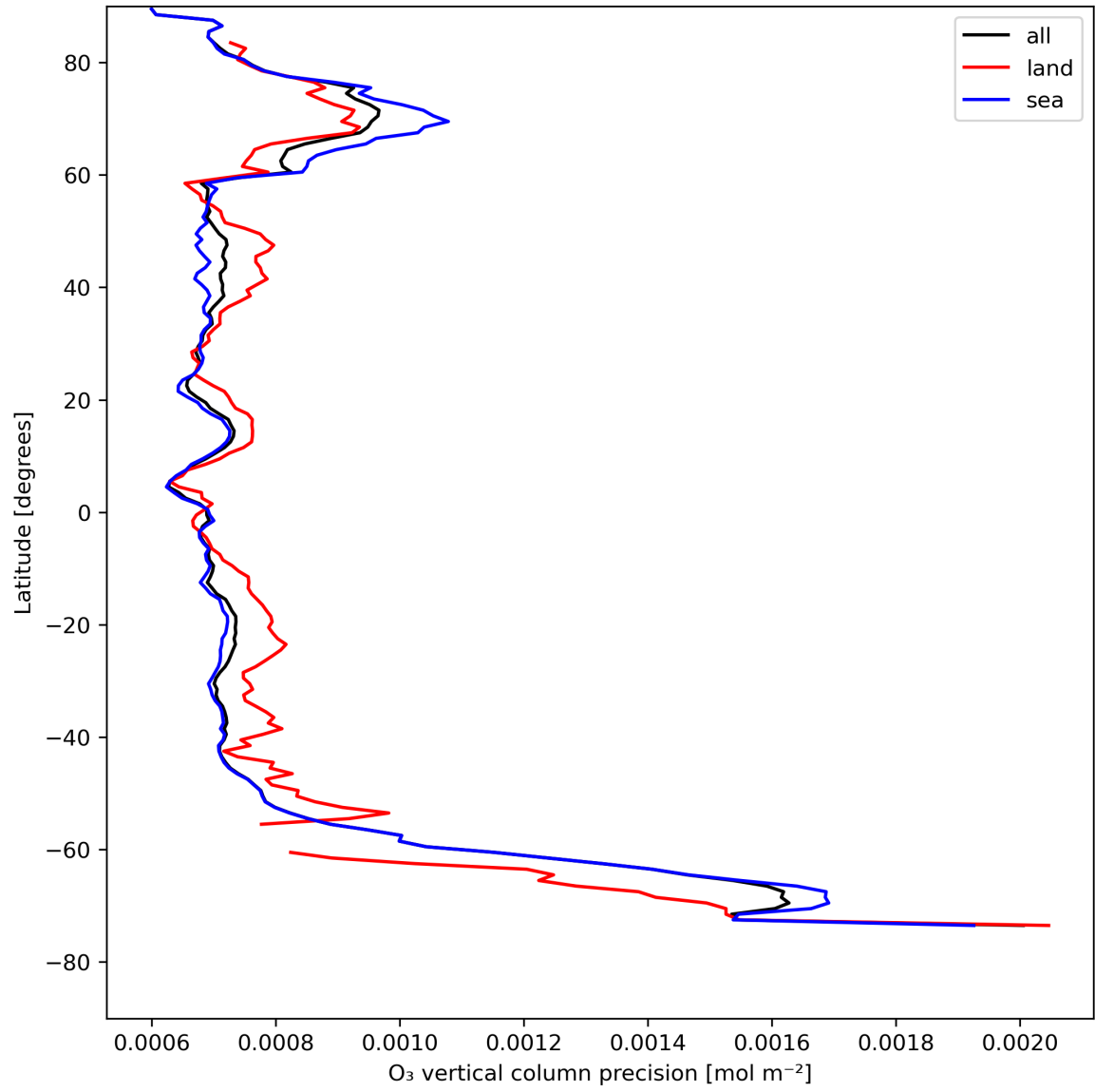
Figure 15: Zonal average of "O 3 vertical column precision" for 2024-04-30 to 2024-05-02.
