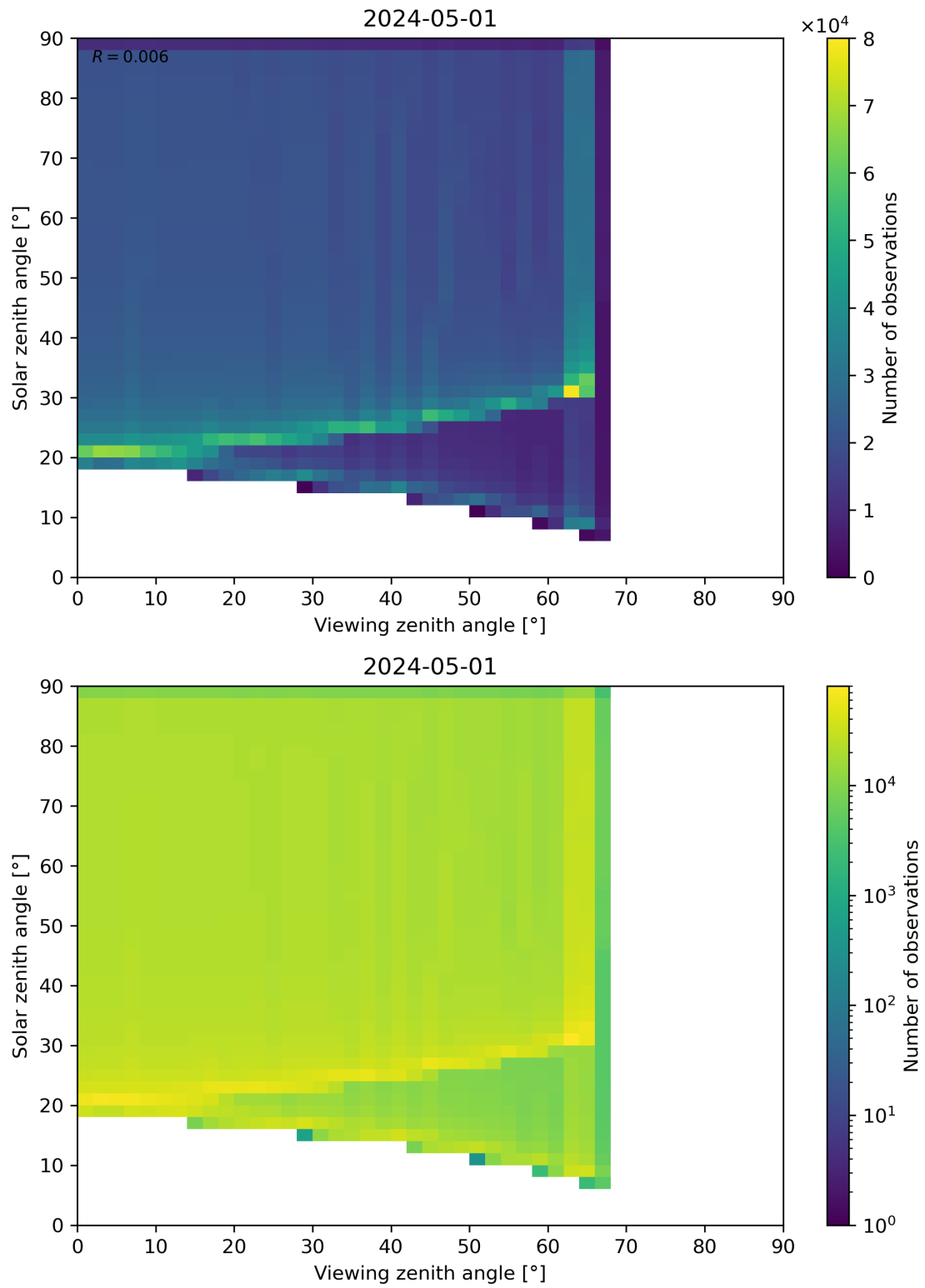
Figure 54: Scatter density plot of “Viewing zenith angle” against “Solar zenith angle” for 2024-04-30 to 2024-05-02.
