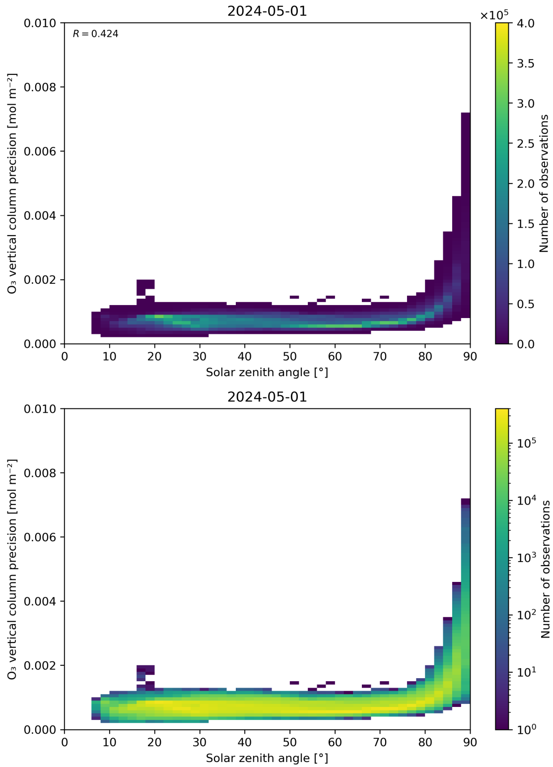
Figure 48: Scatter density plot of “Solar zenith angle” against “O 3 vertical column precision” for 2024-04-30 to 2024-05-02.
