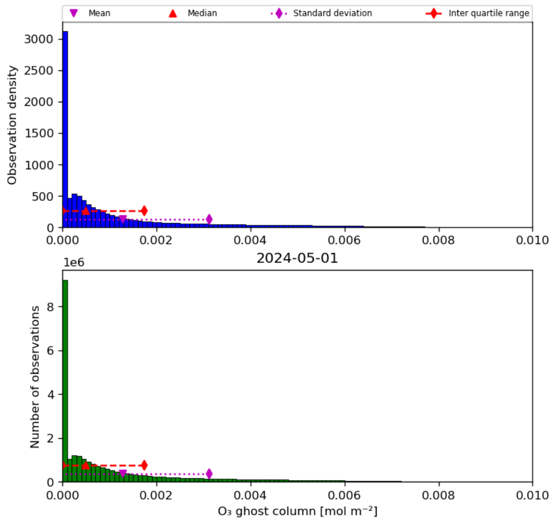
Figure 25: Histogram of "O 3 ghost column" for 2024-04-30 to 2024-05-02
