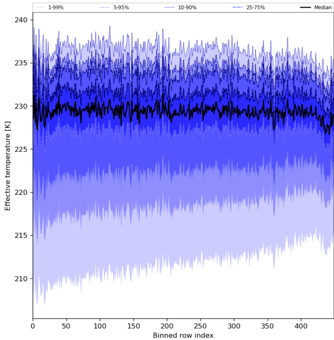
Figure 31: Along track statistics of “Effective temperature” for 2024-04-30 to 2024-05-02
