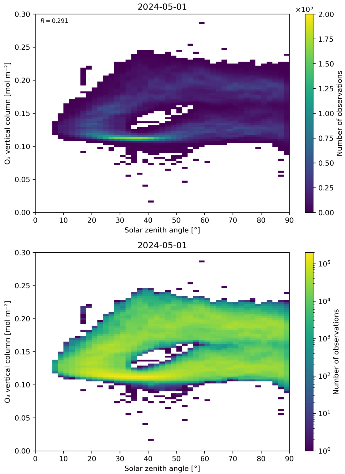
Figure 47: Scatter density plot of “Solar zenith angle” against “O 3 vertical column” for 2024-04-30 to 2024-05-02.
