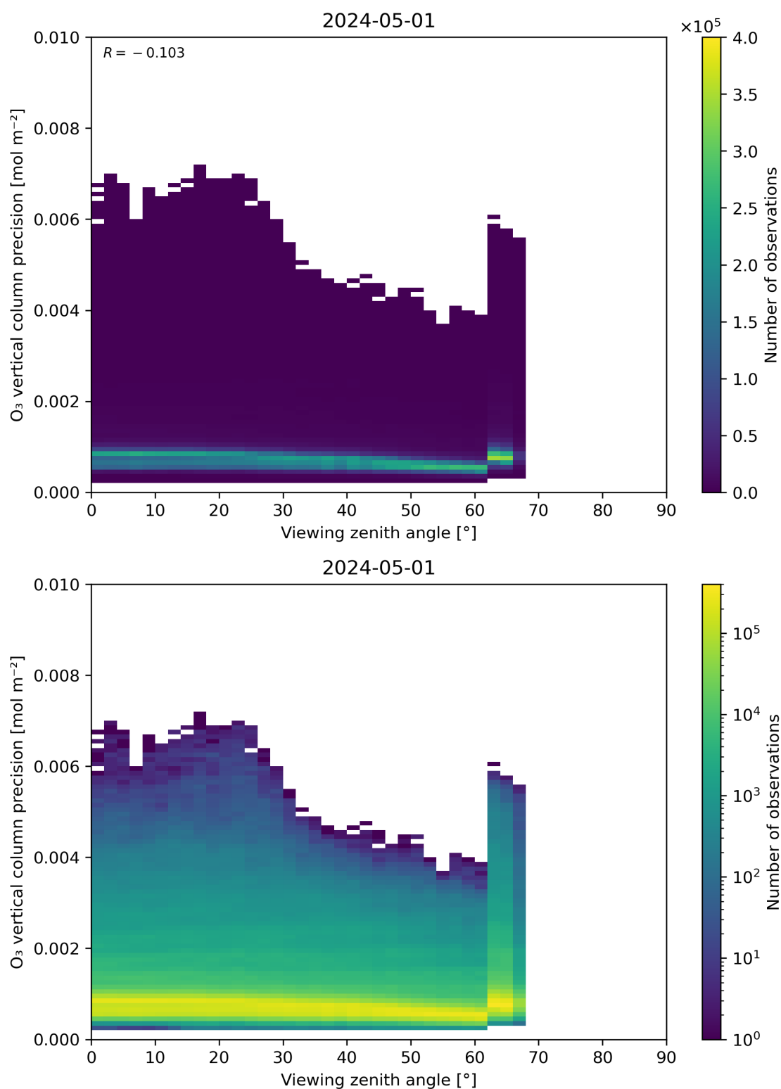
Figure 53: Scatter density plot of “Viewing zenith angle” against “O 3 vertical column precision” for 2024-04-30 to 2024-05-02.
