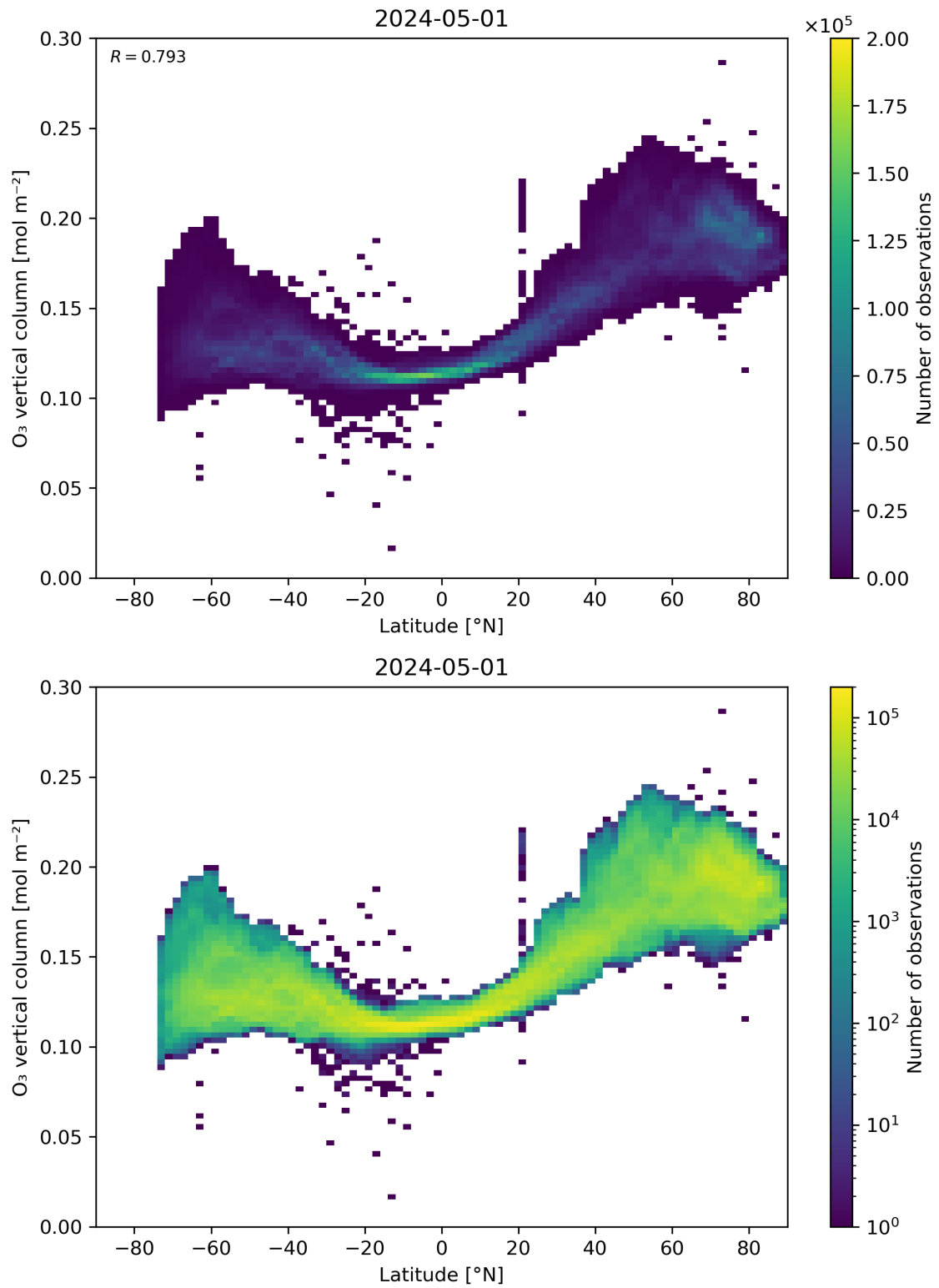
Figure 36: Scatter density plot of “Latitude” against “O 3 vertical column” for 2024-04-30 to 2024-05-02.
