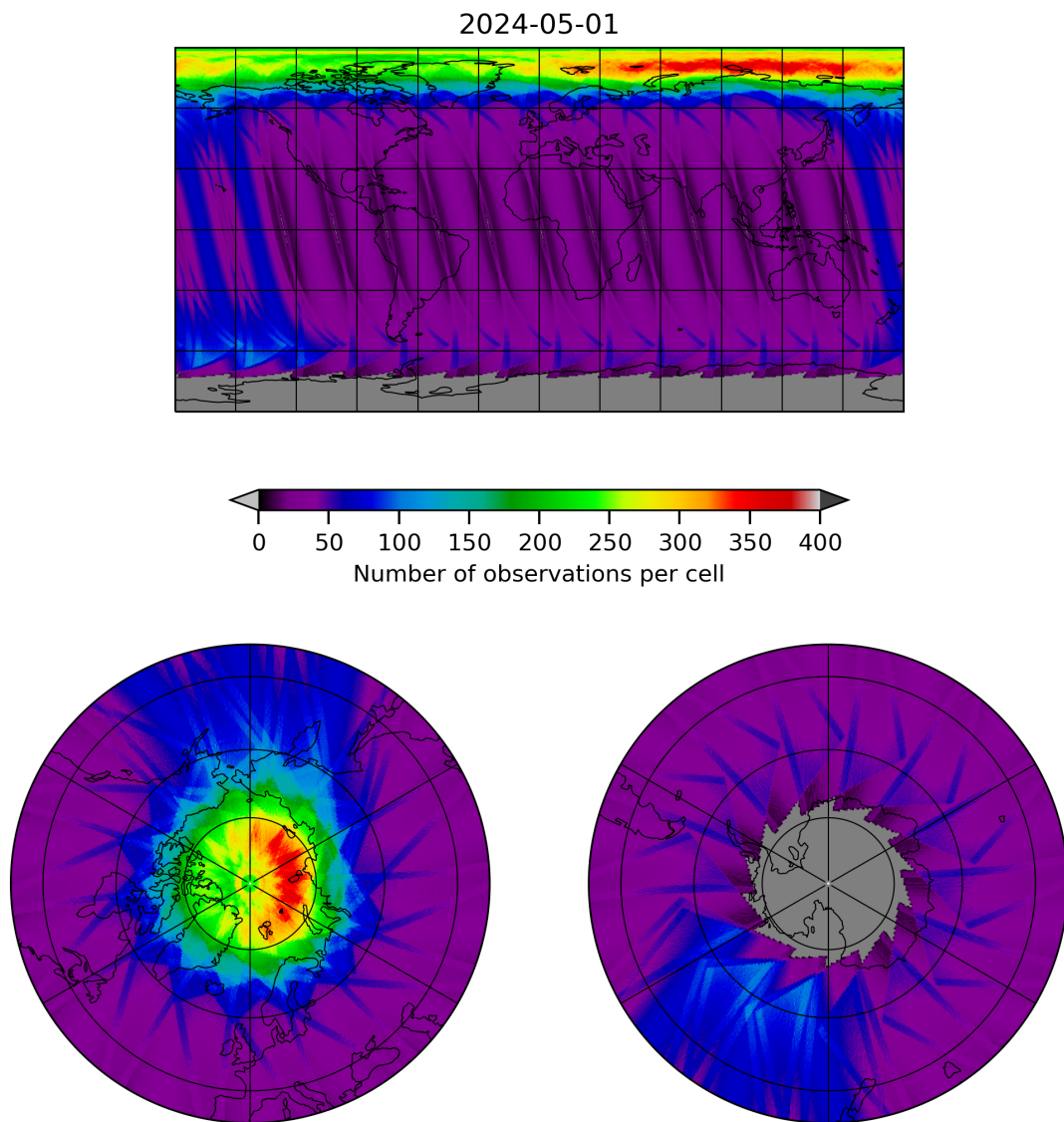
Figure 12: Map of the number of observations for 2024-04-30 to 2024-05-02
