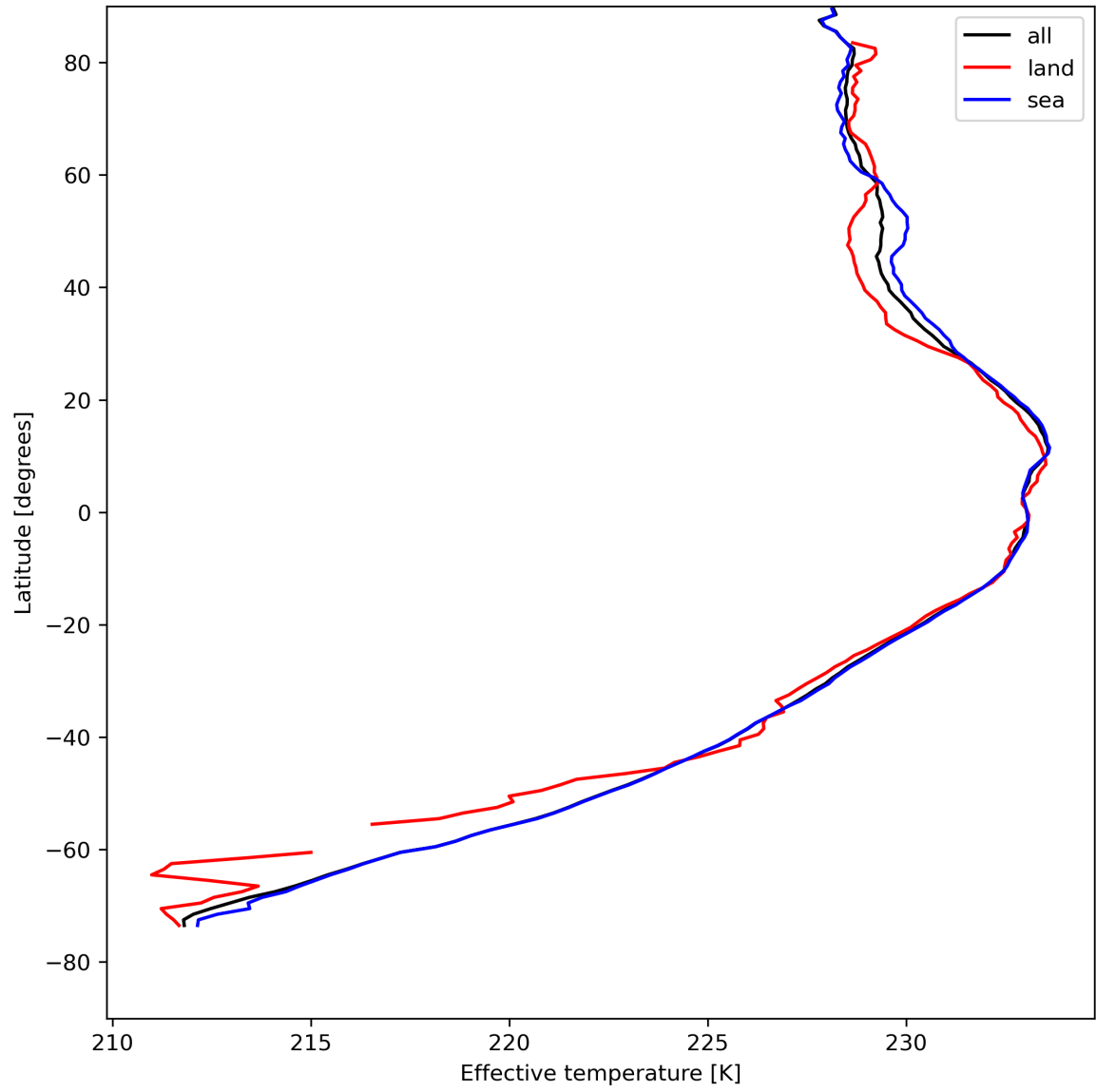
Figure 17: Zonal average of “Effective temperature” for 2024-04-30 to 2024-05-02.
