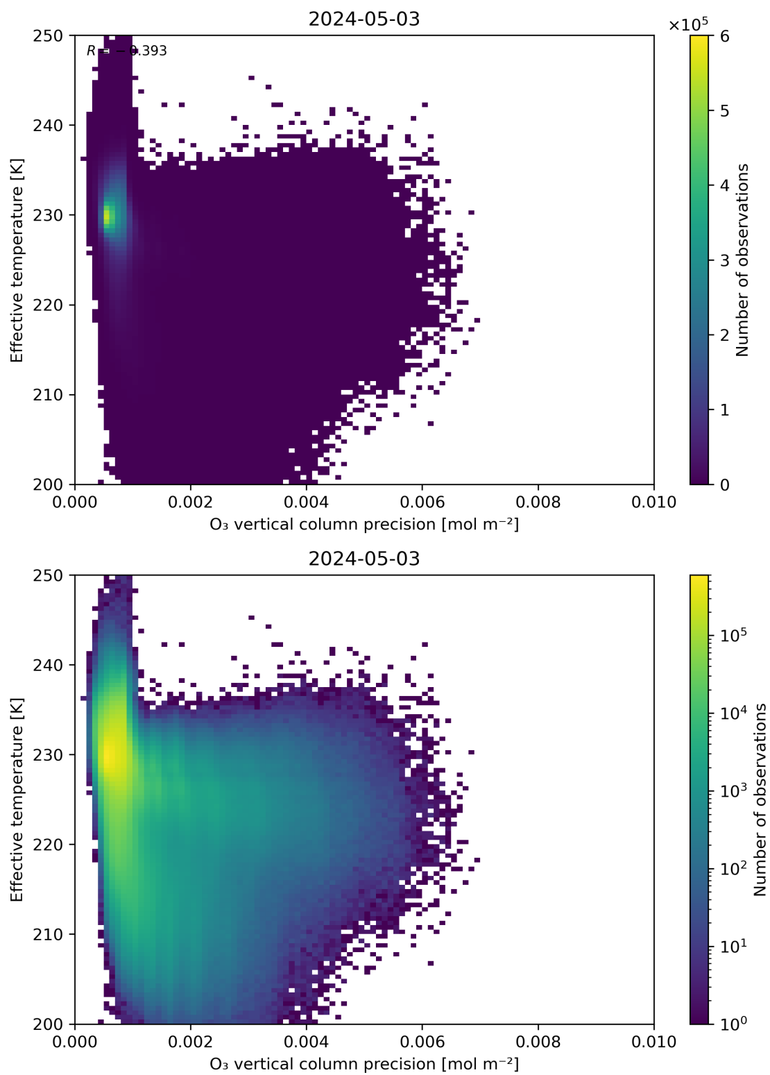
Figure 42: Scatter density plot of “O 3 vertical column precision” against “Effective temperature” for 2024-05-02 to 2024-05-04.
