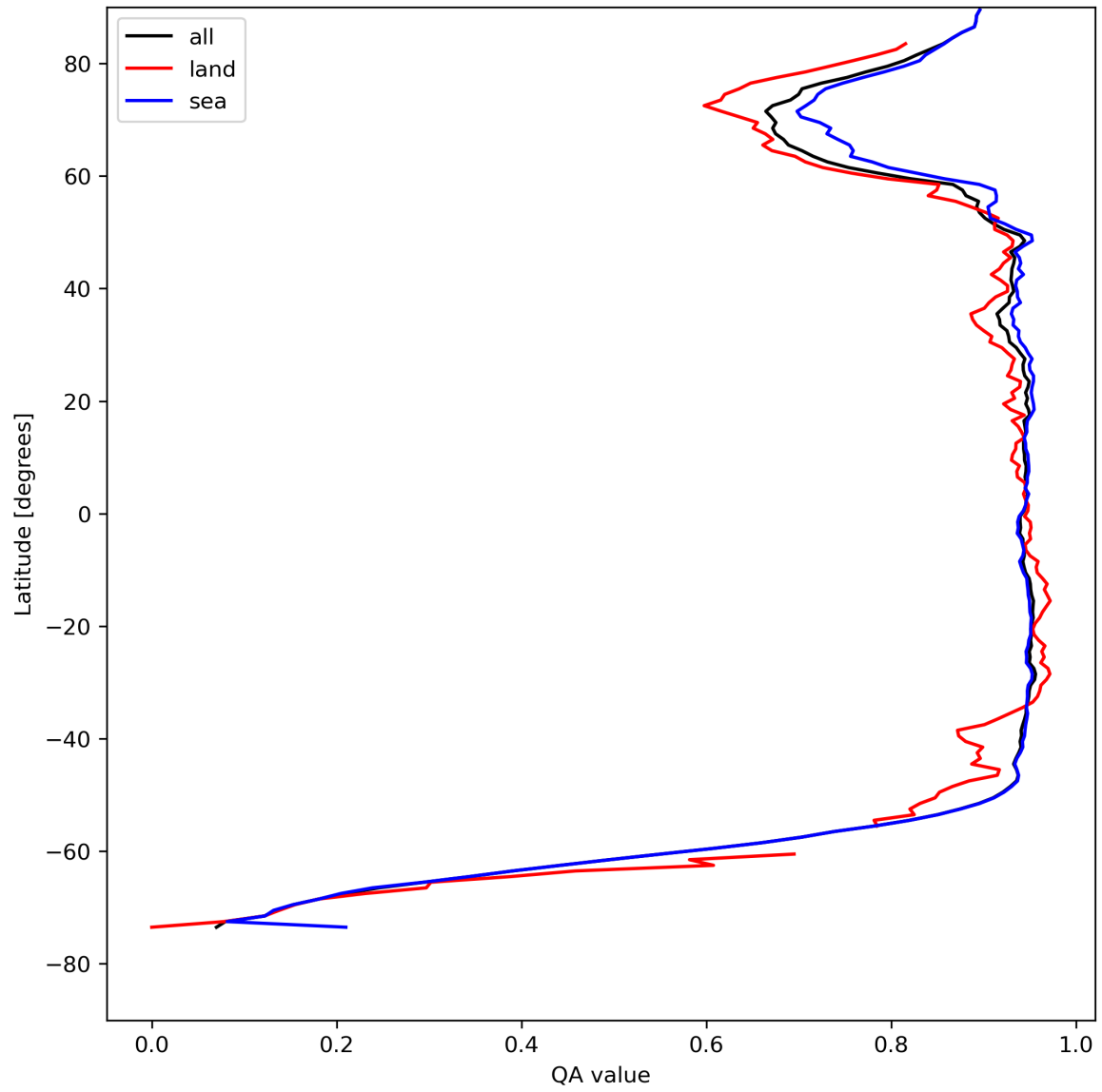
Figure 13: Zonal average of “QA value” for 2024-05-02 to 2024-05-04.
