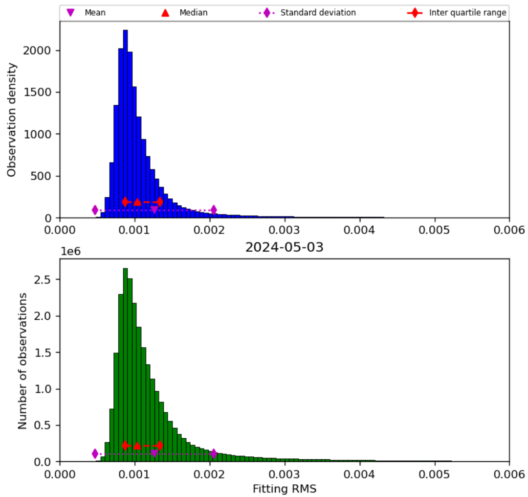
Figure 23: Histogram of “Fitting RMS” for 2024-05-02 to 2024-05-04
