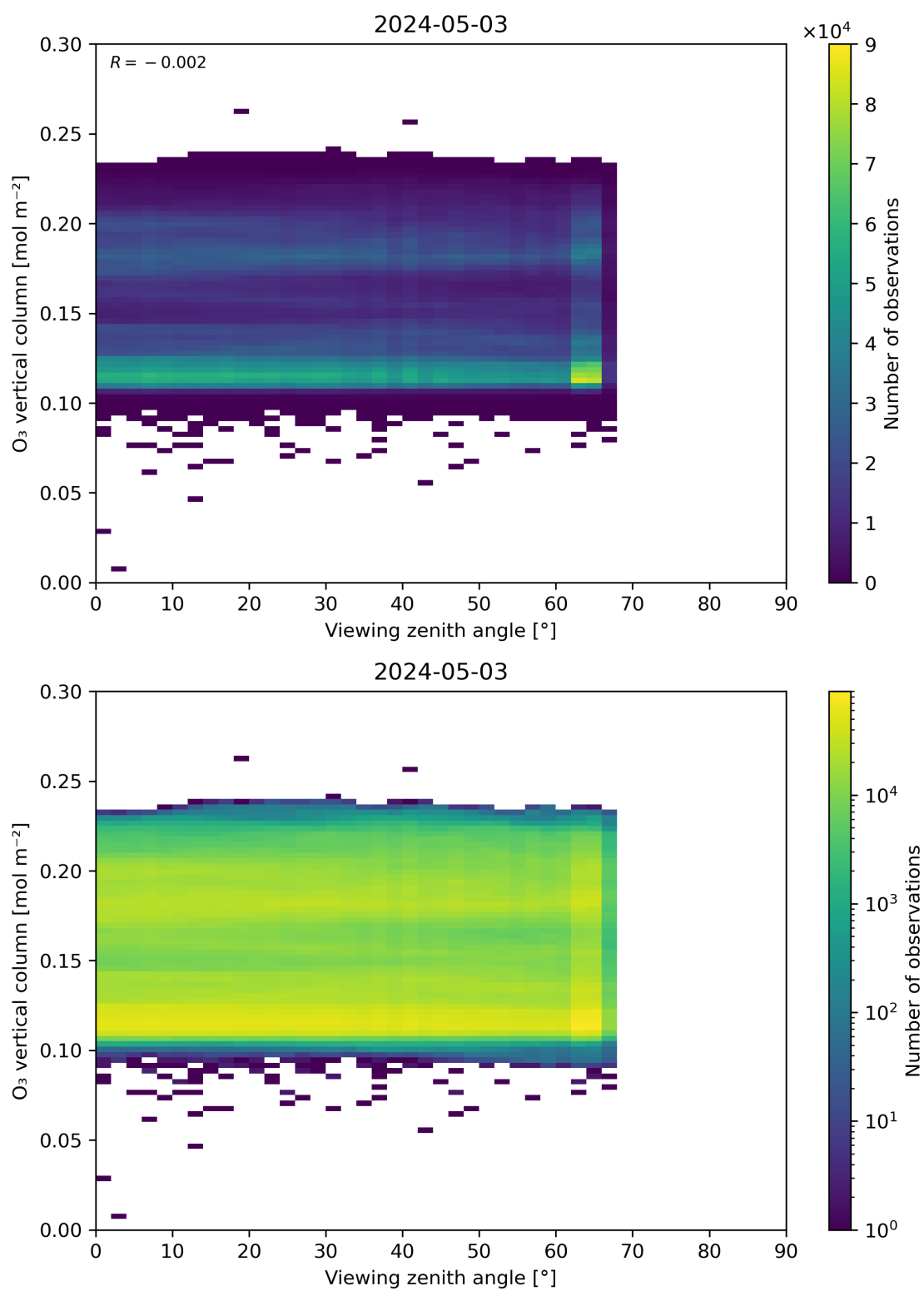
Figure 52: Scatter density plot of “Viewing zenith angle” against “O 3 vertical column” for 2024-05-02 to 2024-05-04.
