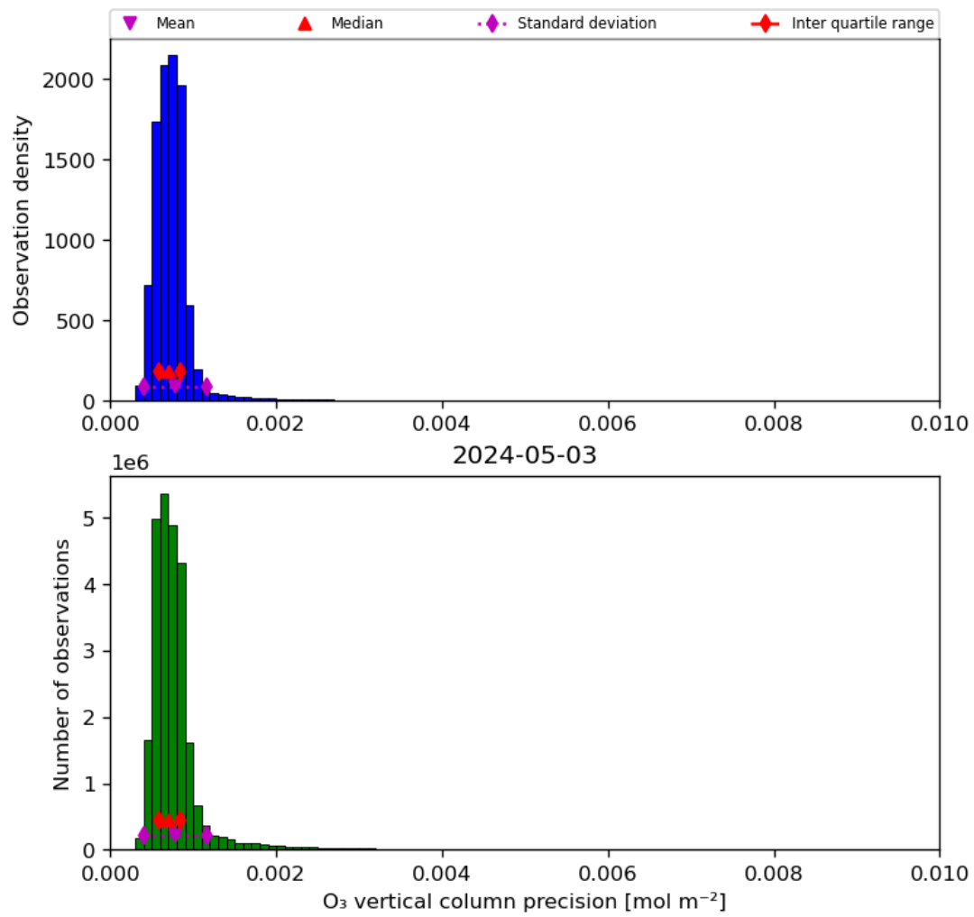
Figure 22: Histogram of “O 3 vertical column precision” for 2024-05-02 to 2024-05-04
