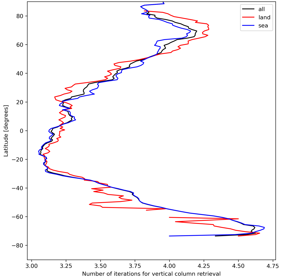
Figure 19: Zonal average of “Number of iterations for vertical column retrieval” for 2024-05-02 to 2024-05-04.
