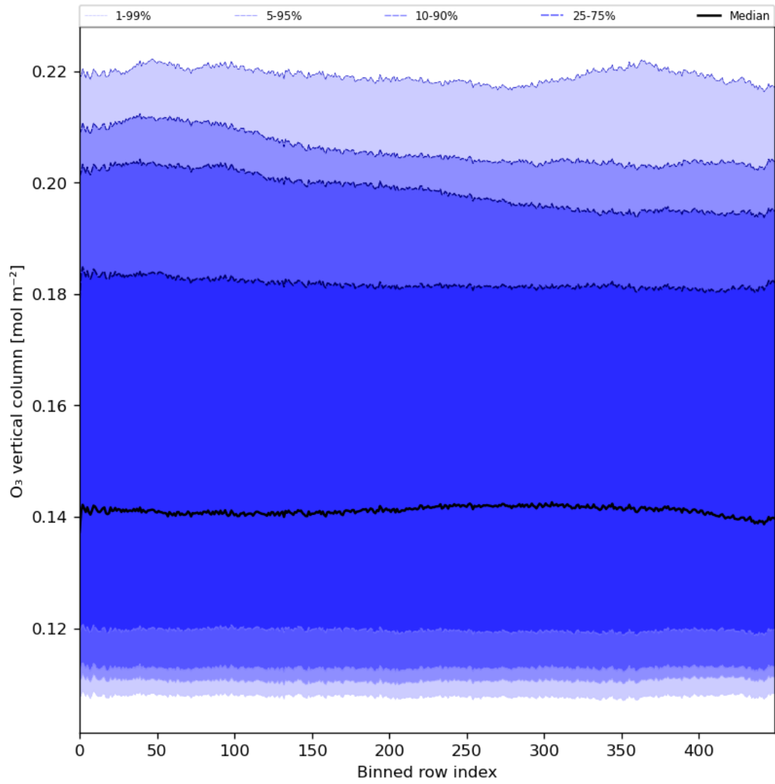
Figure 28: Along track statistics of “O 3 vertical column” for 2024-05-02 to 2024-05-04
