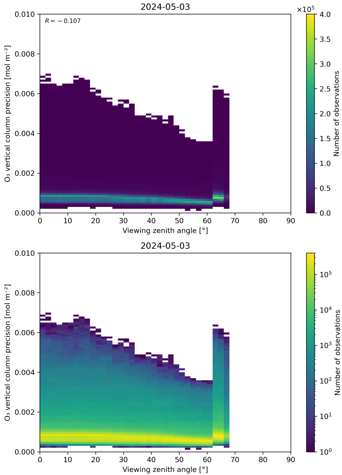
Figure 53: Scatter density plot of “Viewing zenith angle” against “O 3 vertical column precision” for 2024-05-02 to 2024-05-04.
