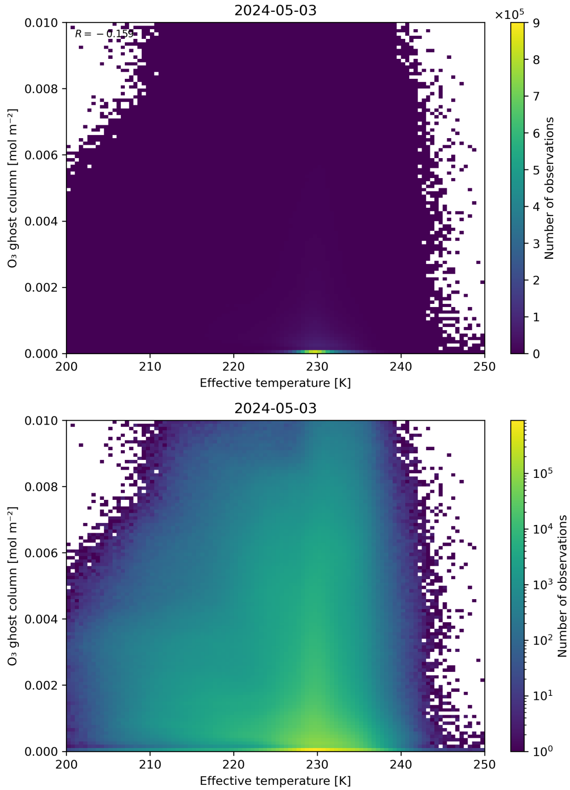
Figure 38: Scatter density plot of “Effective temperature” against “O 3 ghost column” for 2024-05-02 to 2024-05-04.
