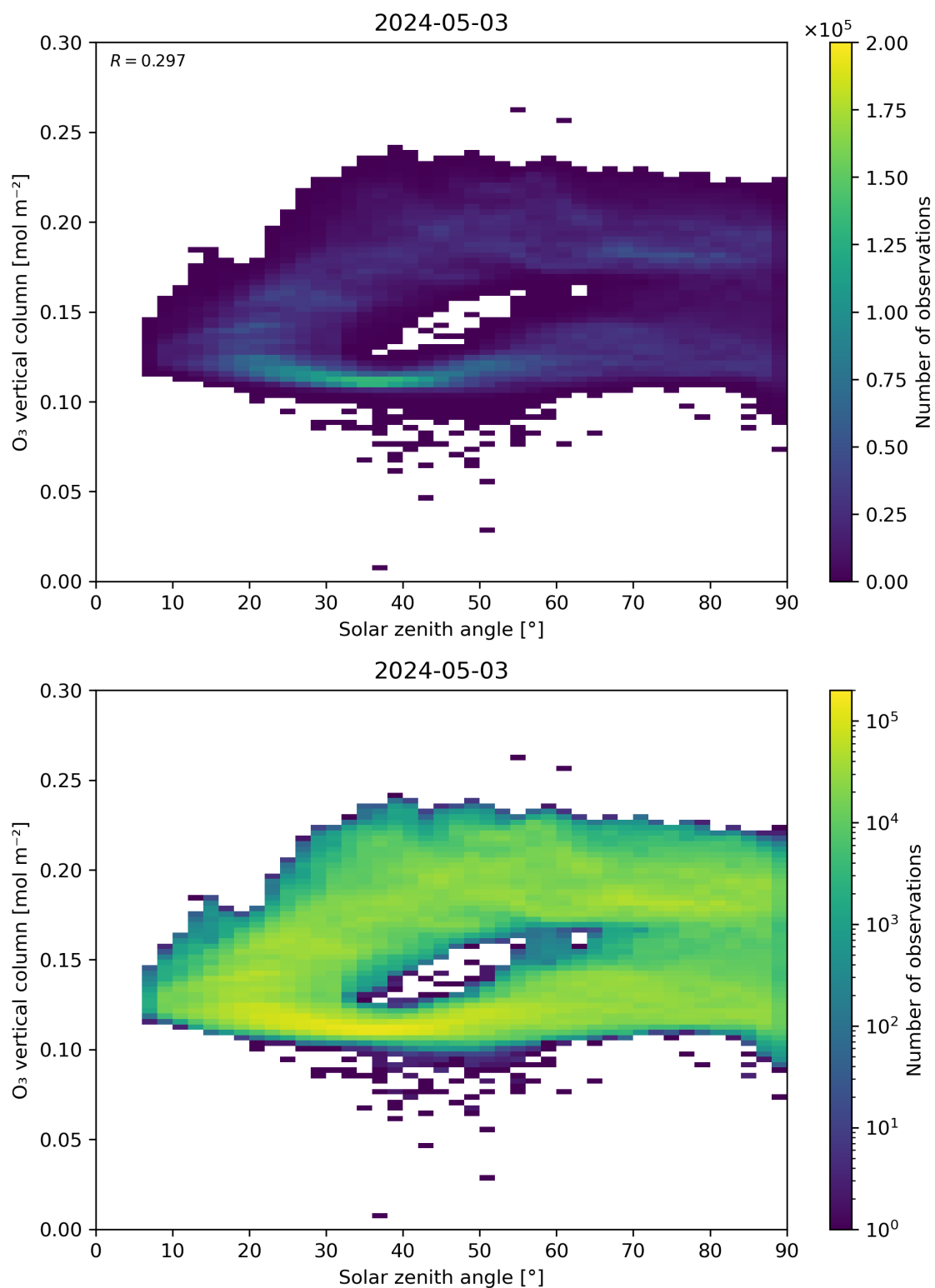
Figure 47: Scatter density plot of “Solar zenith angle” against “O 3 vertical column” for 2024-05-02 to 2024-05-04.
