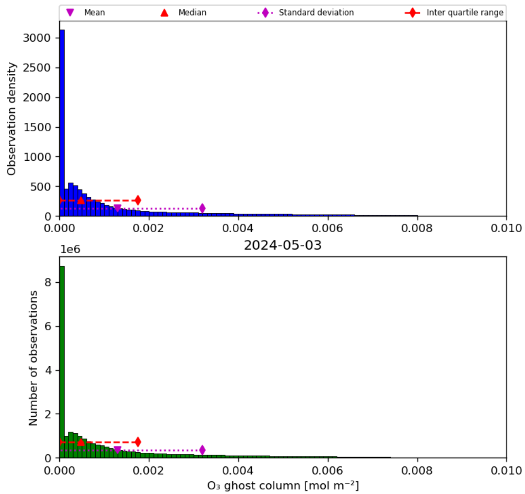
Figure 25: Histogram of “O 3 ghost column” for 2024-05-02 to 2024-05-04
