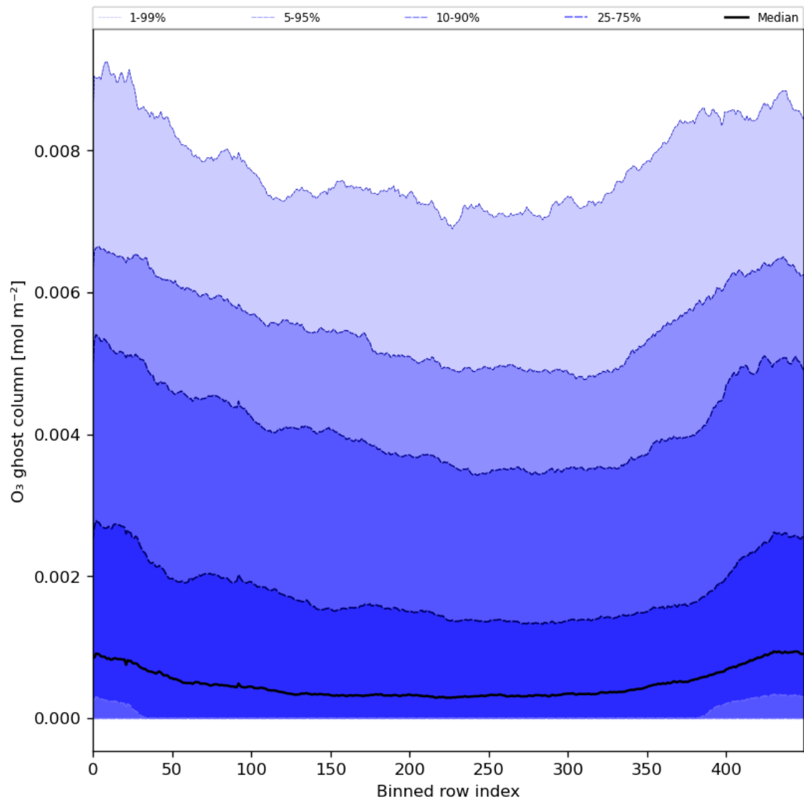
Figure 32: Along track statistics of “O 3 ghost column” for 2024-05-02 to 2024-05-04
