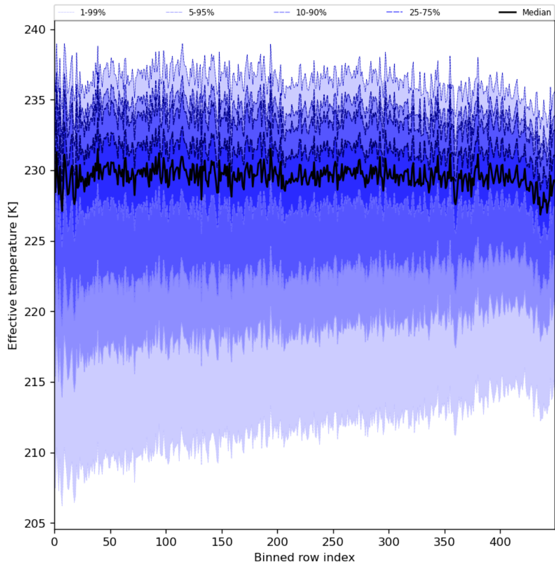
Figure 31: Along track statistics of “Effective temperature” for 2024-05-02 to 2024-05-04
