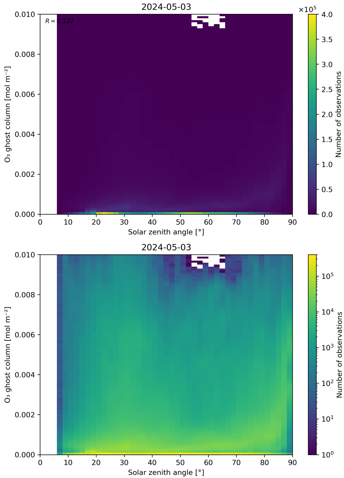
Figure 46: Scatter density plot of “Solar zenith angle” against “O 3 ghost column” for 2024-05-02 to 2024-05-04.
