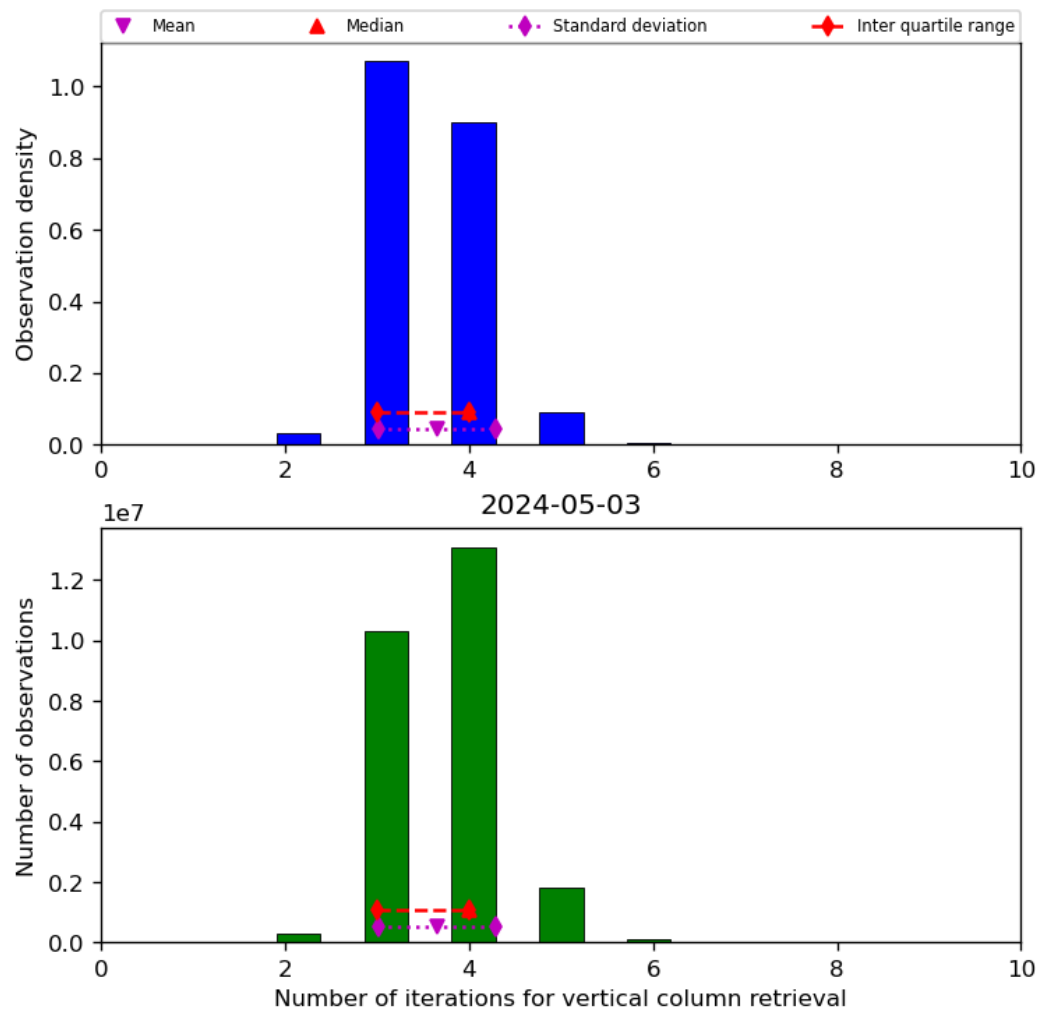
Figure 26: Histogram of “Number of iterations for vertical column retrieval” for 2024-05-02 to 2024-05-04
