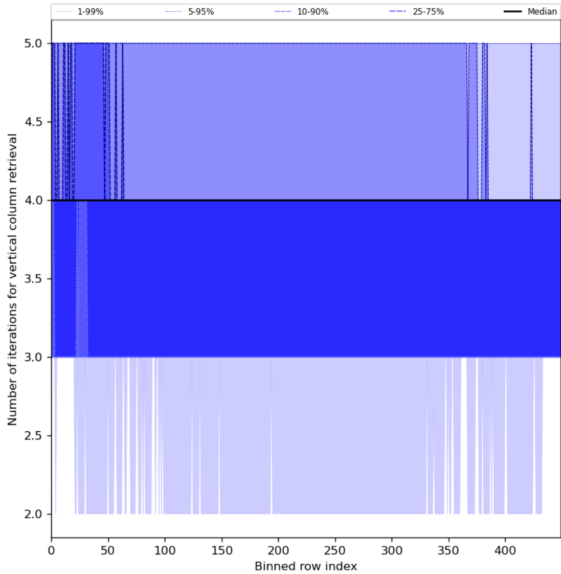
Figure 33: Along track statistics of “Number of iterations for vertical column retrieval” for 2024-05-02 to 2024-05-04
