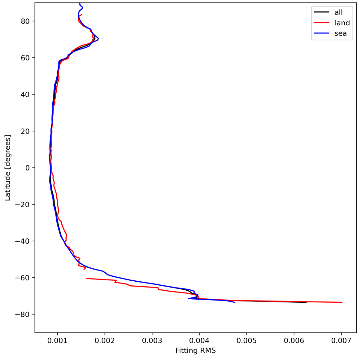
Figure 16: Zonal average of “Fitting RMS” for 2024-05-02 to 2024-05-04.
