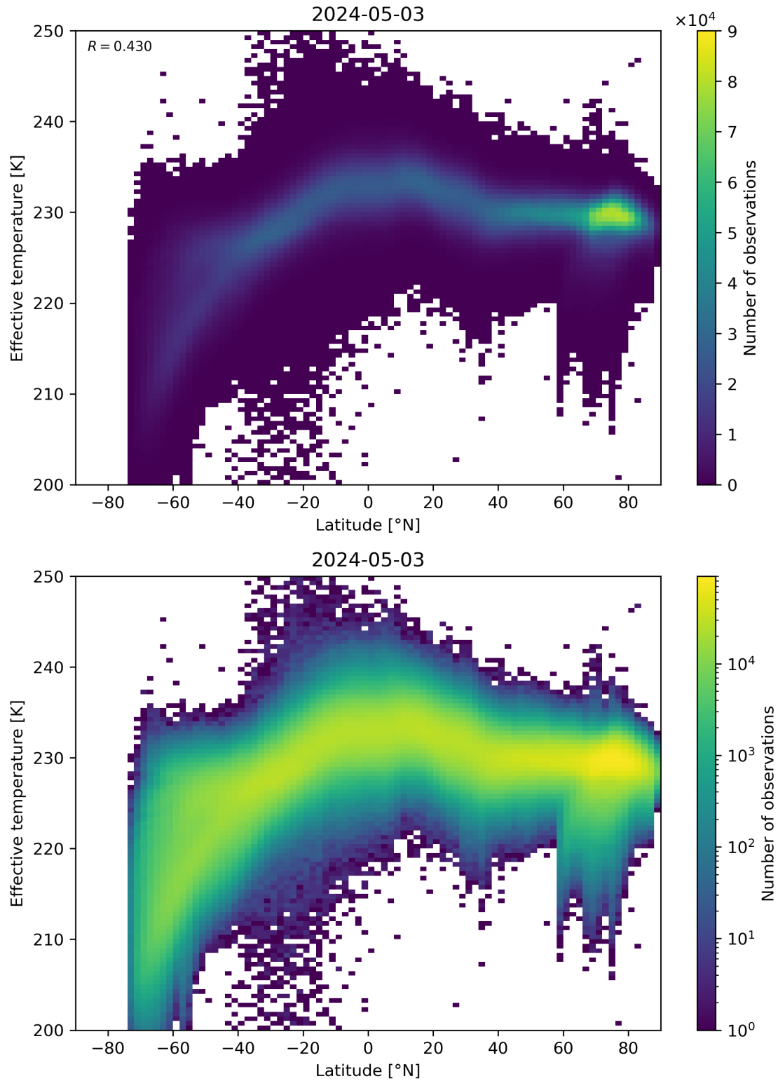
Figure 34: Scatter density plot of “Latitude” against “Effective temperature” for 2024-05-02 to 2024-05-04.
