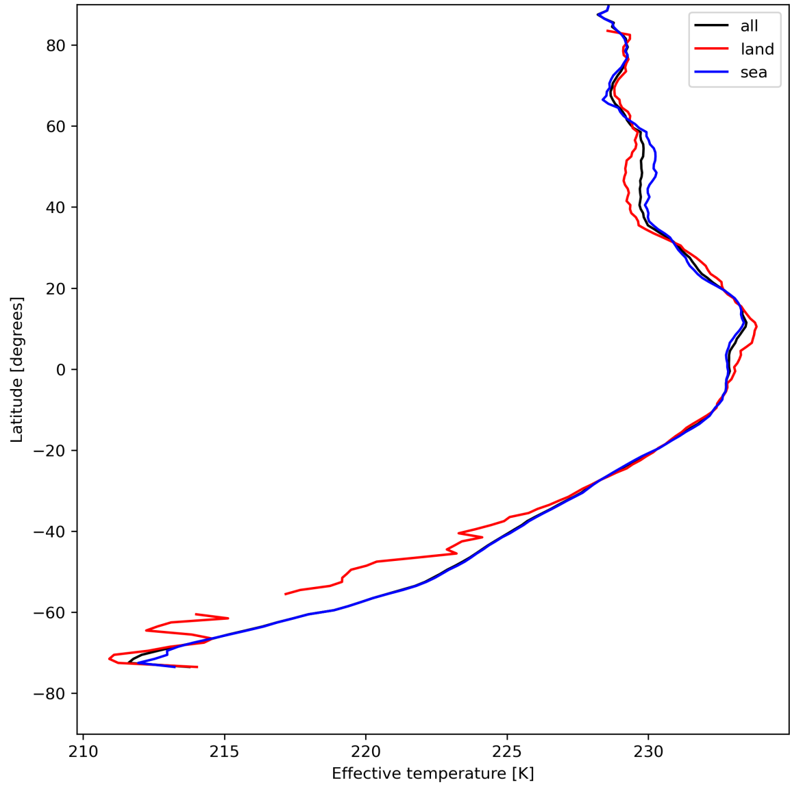
Figure 17: Zonal average of "Effective temperature" for 2024-05-02 to 2024-05-04.
