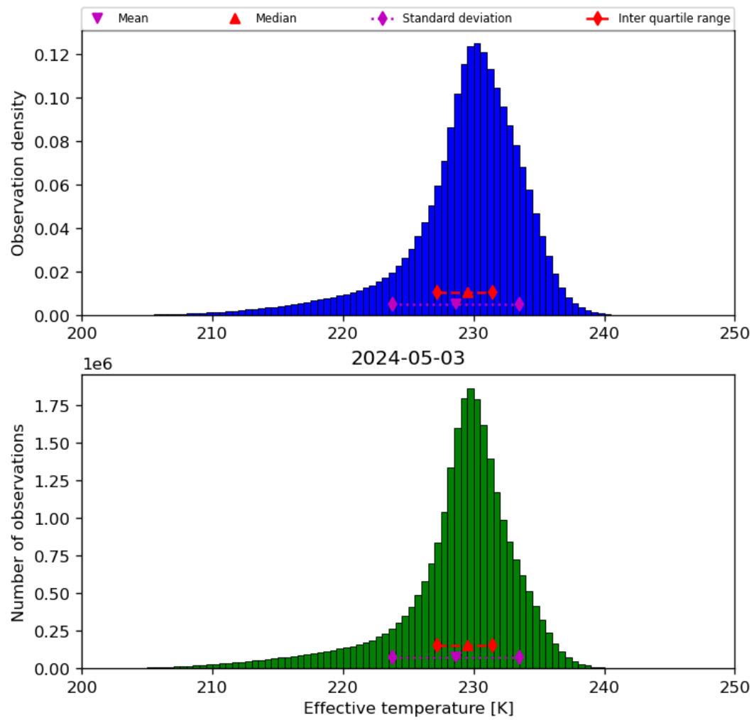
Figure 24: Histogram of “Effective temperature” for 2024-05-02 to 2024-05-04
