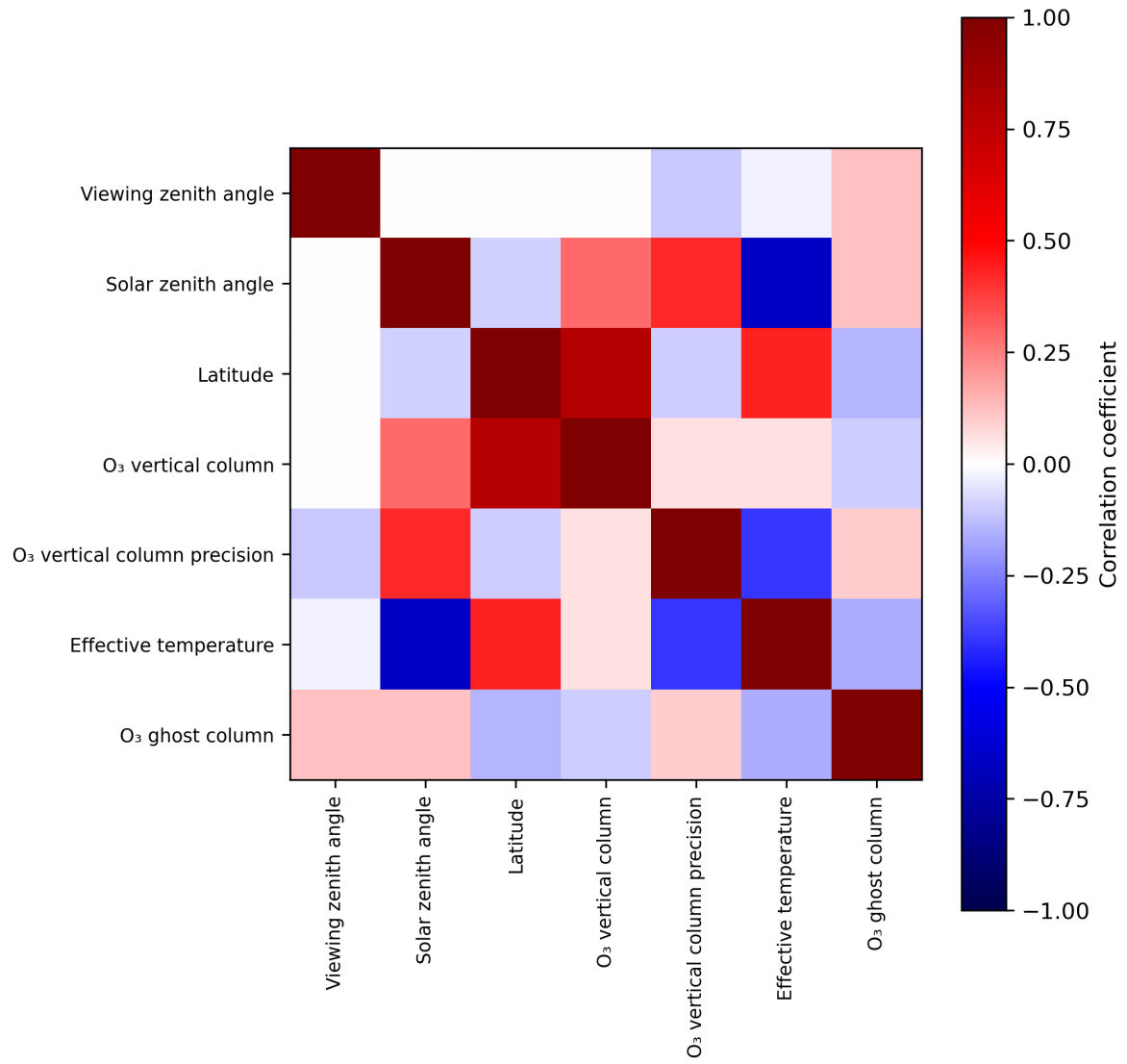
Figure 2: Map of correlation matrix for 2024-05-02 to 2024-05-04.
