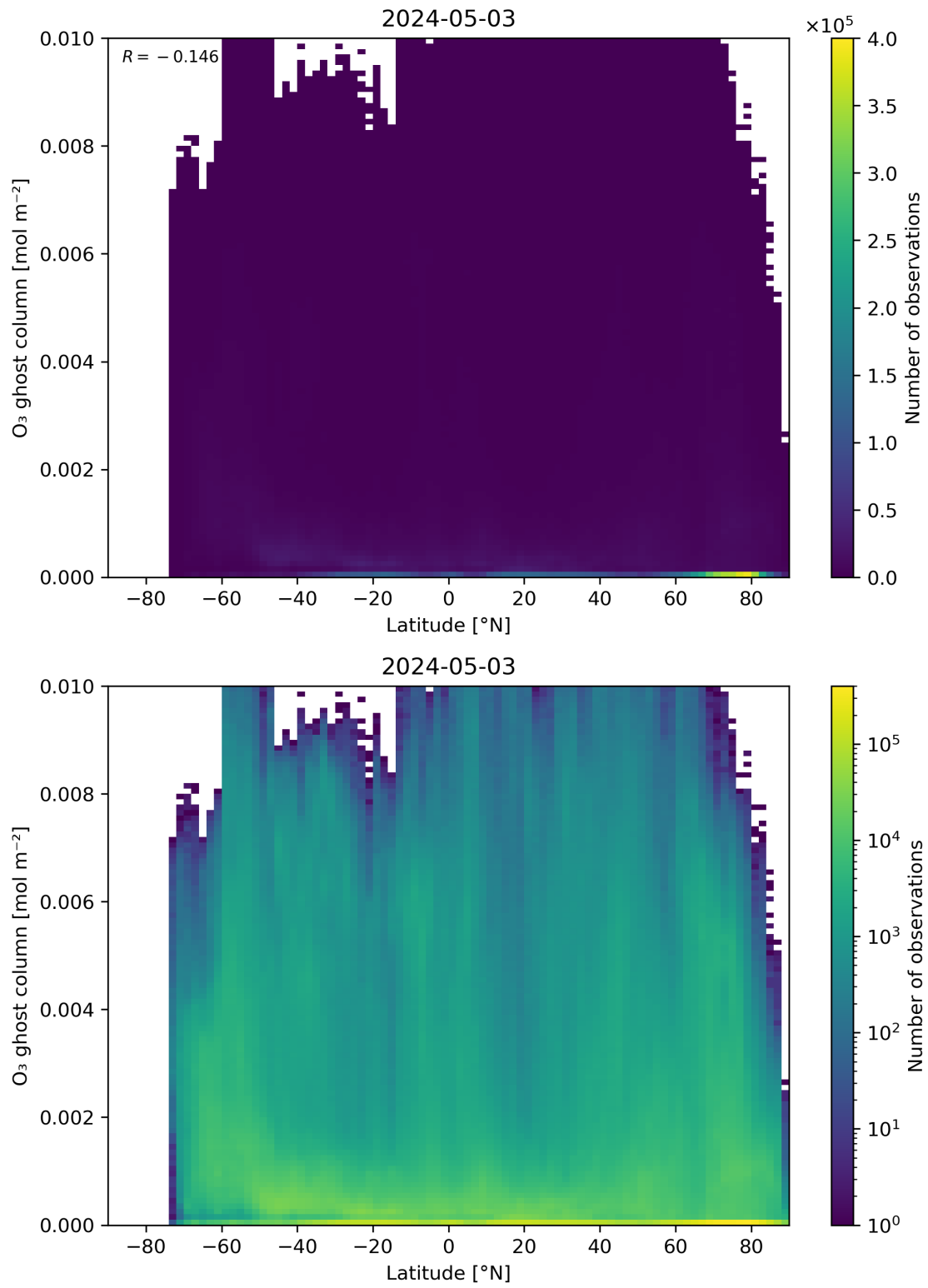
Figure 35: Scatter density plot of “Latitude” against “O 3 ghost column” for 2024-05-02 to 2024-05-04.
