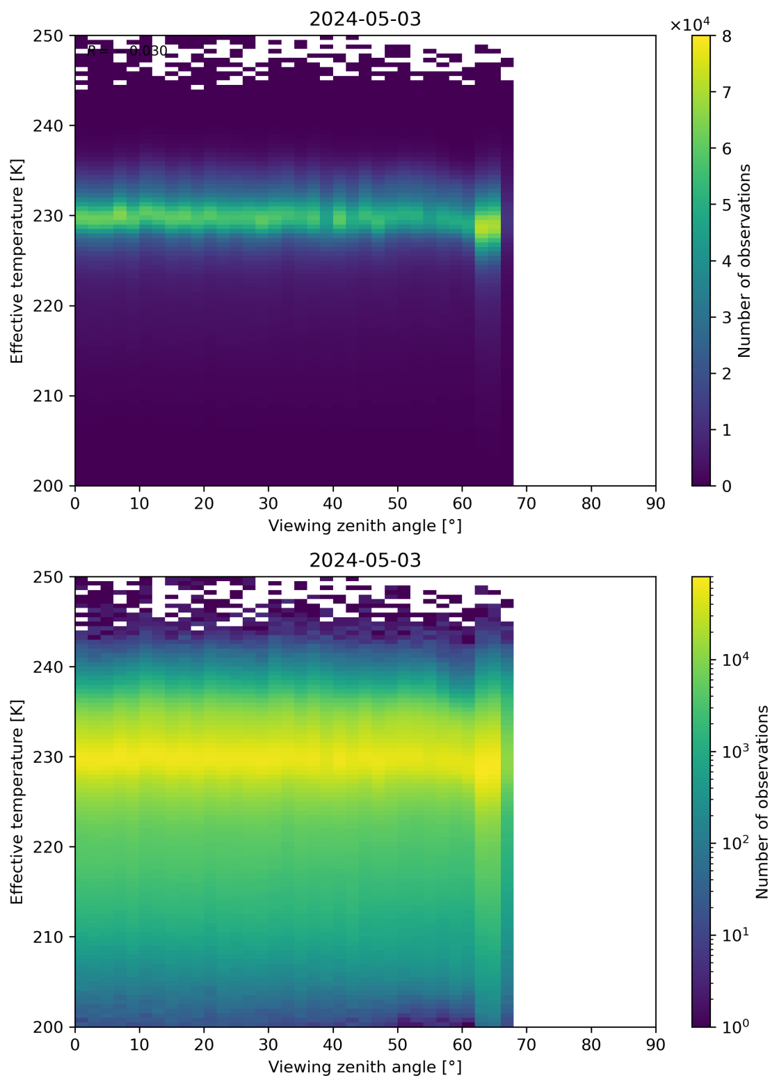
Figure 50: Scatter density plot of “Viewing zenith angle” against “Effective temperature” for 2024-05-02 to 2024-05-04.
