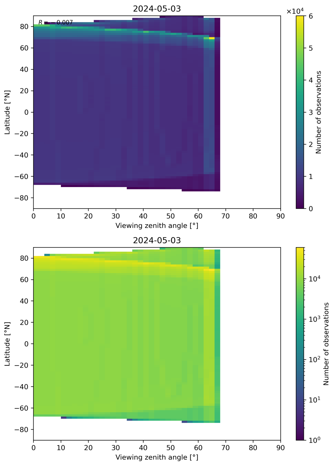
Figure 49: Scatter density plot of “Viewing zenith angle” against “Latitude” for 2024-05-02 to 2024-05-04.
