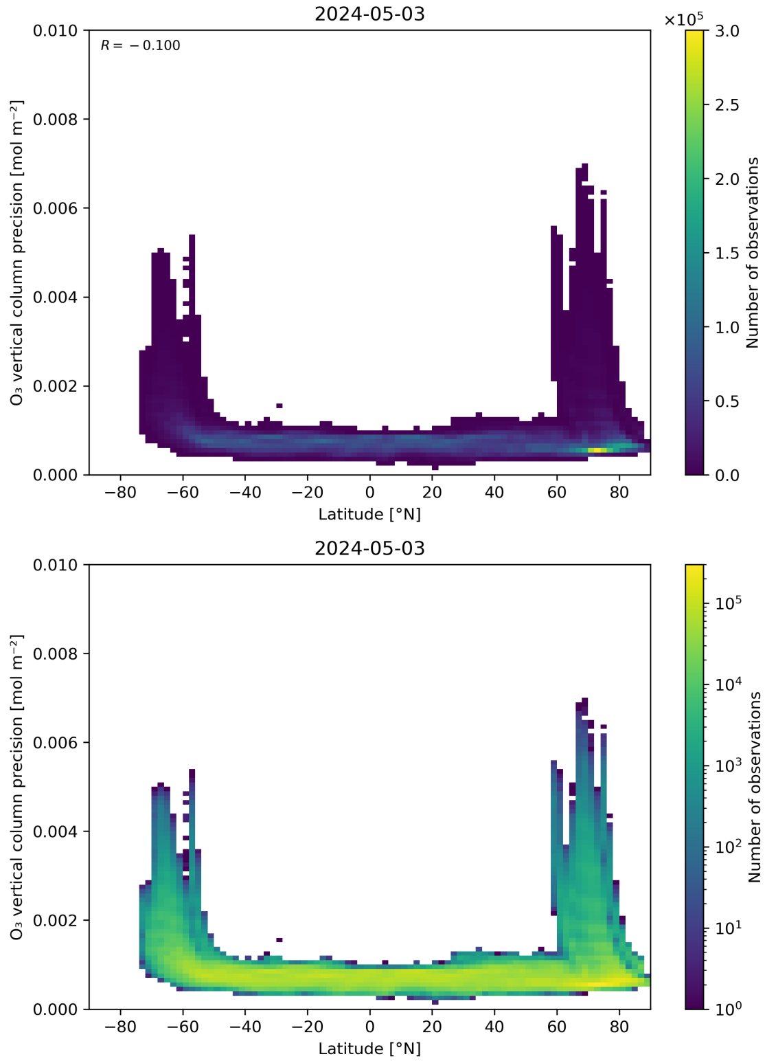
Figure 37: Scatter density plot of “Latitude” against “O 3 vertical column precision” for 2024-05-02 to 2024-05-04.
