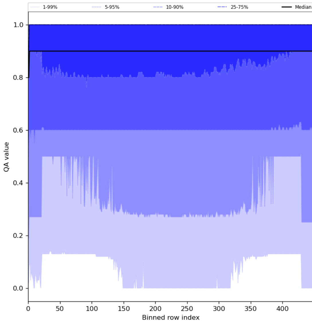
Figure 27: Along track statistics of “QA value” for 2024-05-02 to 2024-05-04
