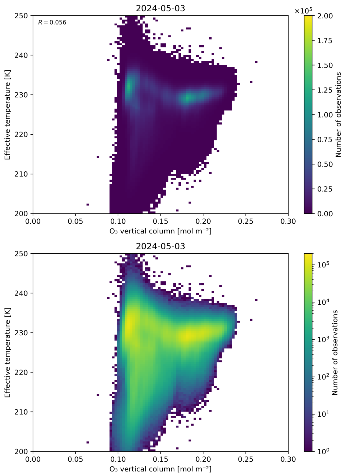
Figure 39: Scatter density plot of “O 3 vertical column” against “Effective temperature” for 2024-05-02 to 2024-05-04.
