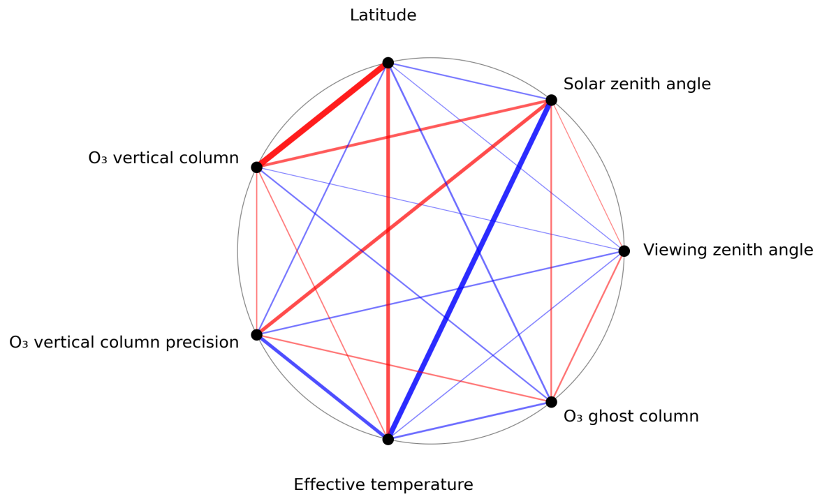
Figure 1: Map of correlation graph for 2024-05-02 to 2024-05-04.
