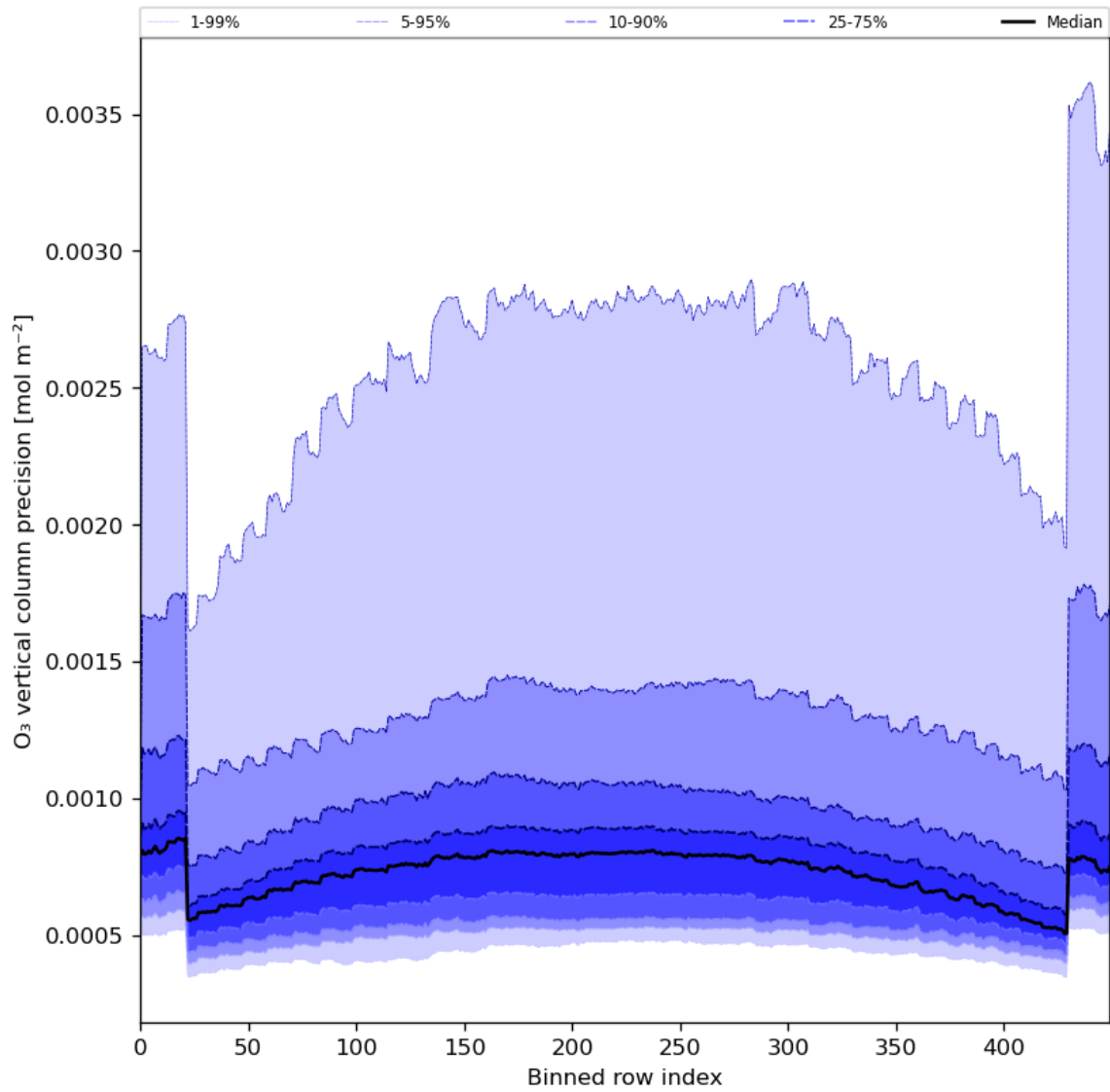
Figure 29: Along track statistics of “O 3 vertical column precision” for 2024-05-02 to 2024-05-04
