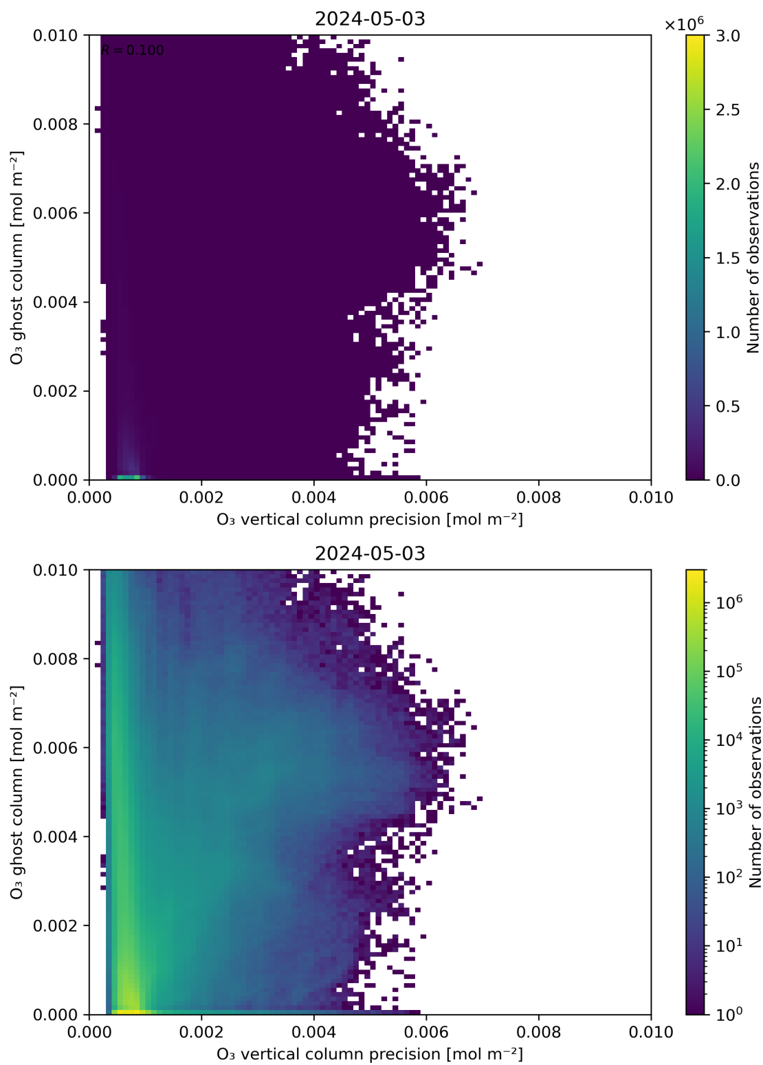
Figure 43: Scatter density plot of “ \text{O}_3 vertical column precision” against “ \text{O}_3 ghost column” for 2024-05-02 to 2024-05-04.
