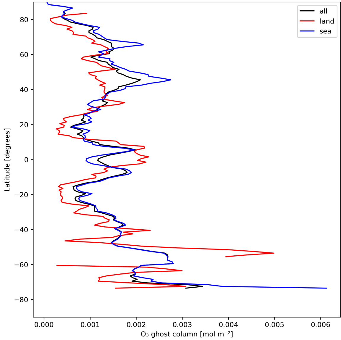
Figure 18: Zonal average of “O 3 ghost column” for 2024-05-02 to 2024-05-04.
