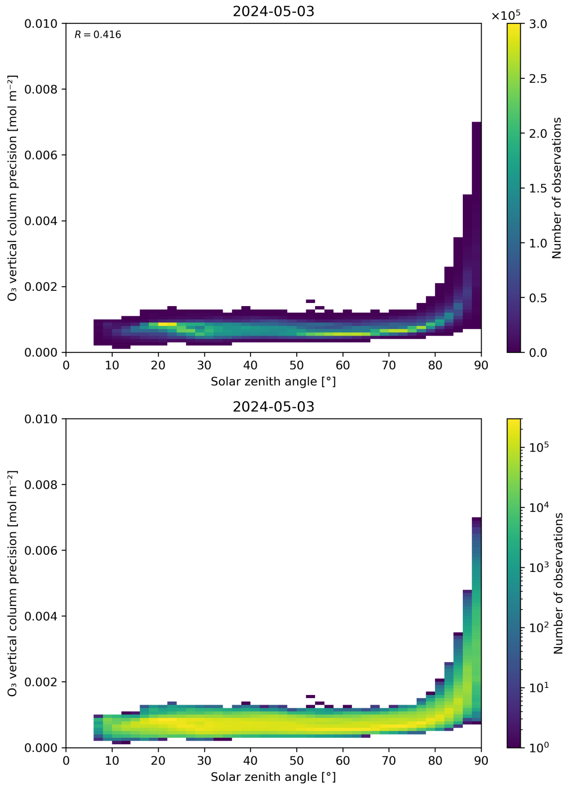
Figure 48: Scatter density plot of “Solar zenith angle” against “O 3 vertical column precision” for 2024-05-02 to 2024-05-04.
