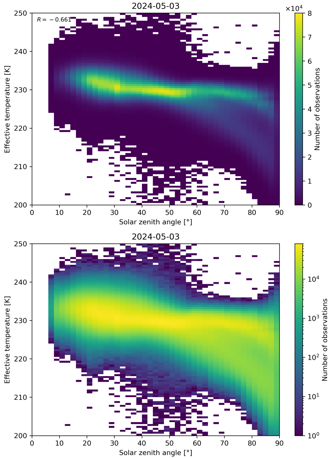
Figure 45: Scatter density plot of “Solar zenith angle” against “Effective temperature” for 2024-05-02 to 2024-05-04.
