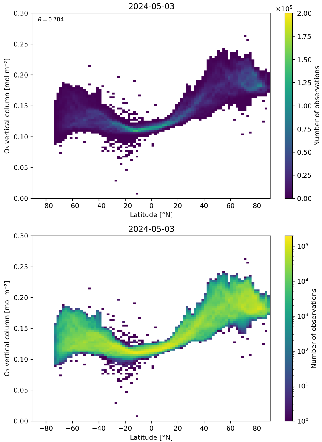
Figure 36: Scatter density plot of “Latitude” against “O 3 vertical column” for 2024-05-02 to 2024-05-04.
