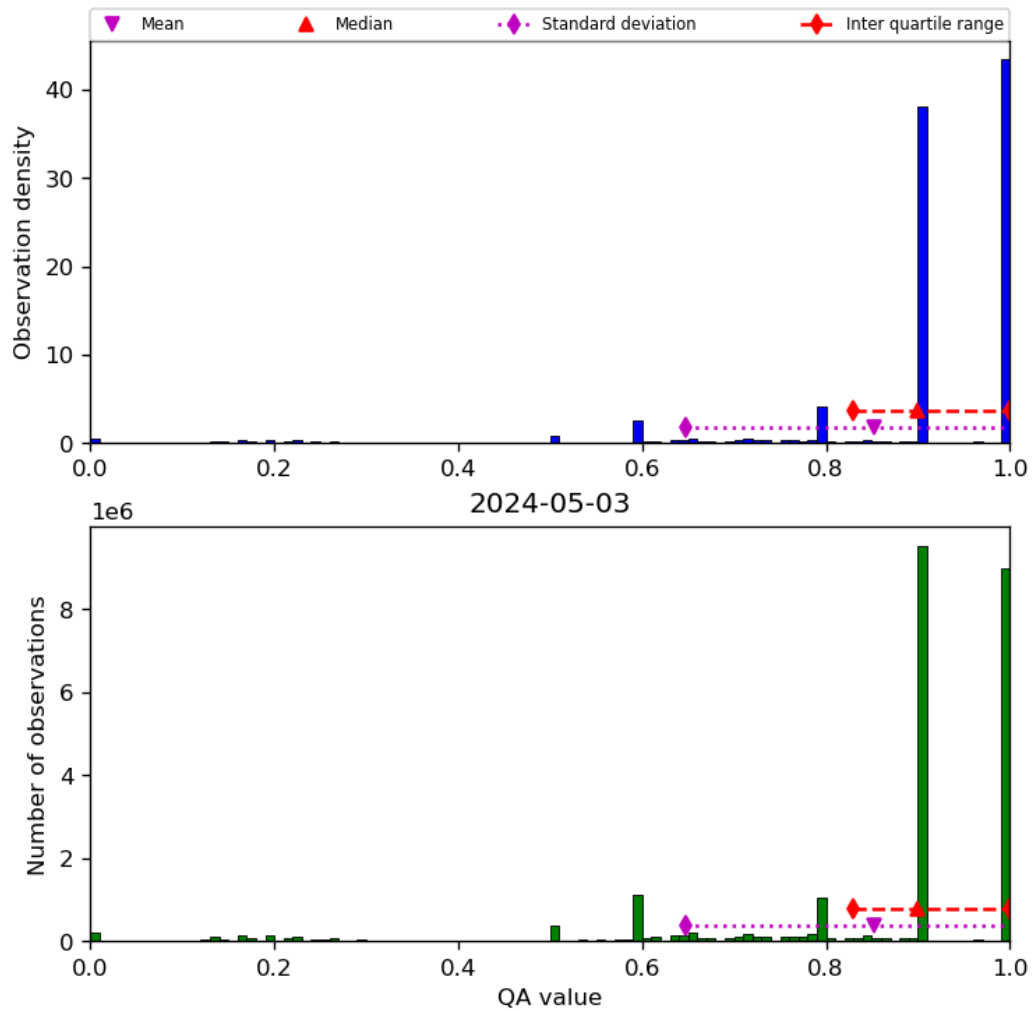
Figure 20: Histogram of “QA value” for 2024-05-02 to 2024-05-04
