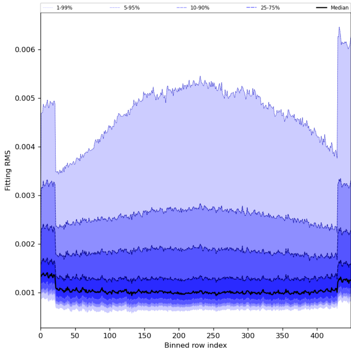
Figure 30: Along track statistics of “Fitting RMS” for 2024-05-02 to 2024-05-04
