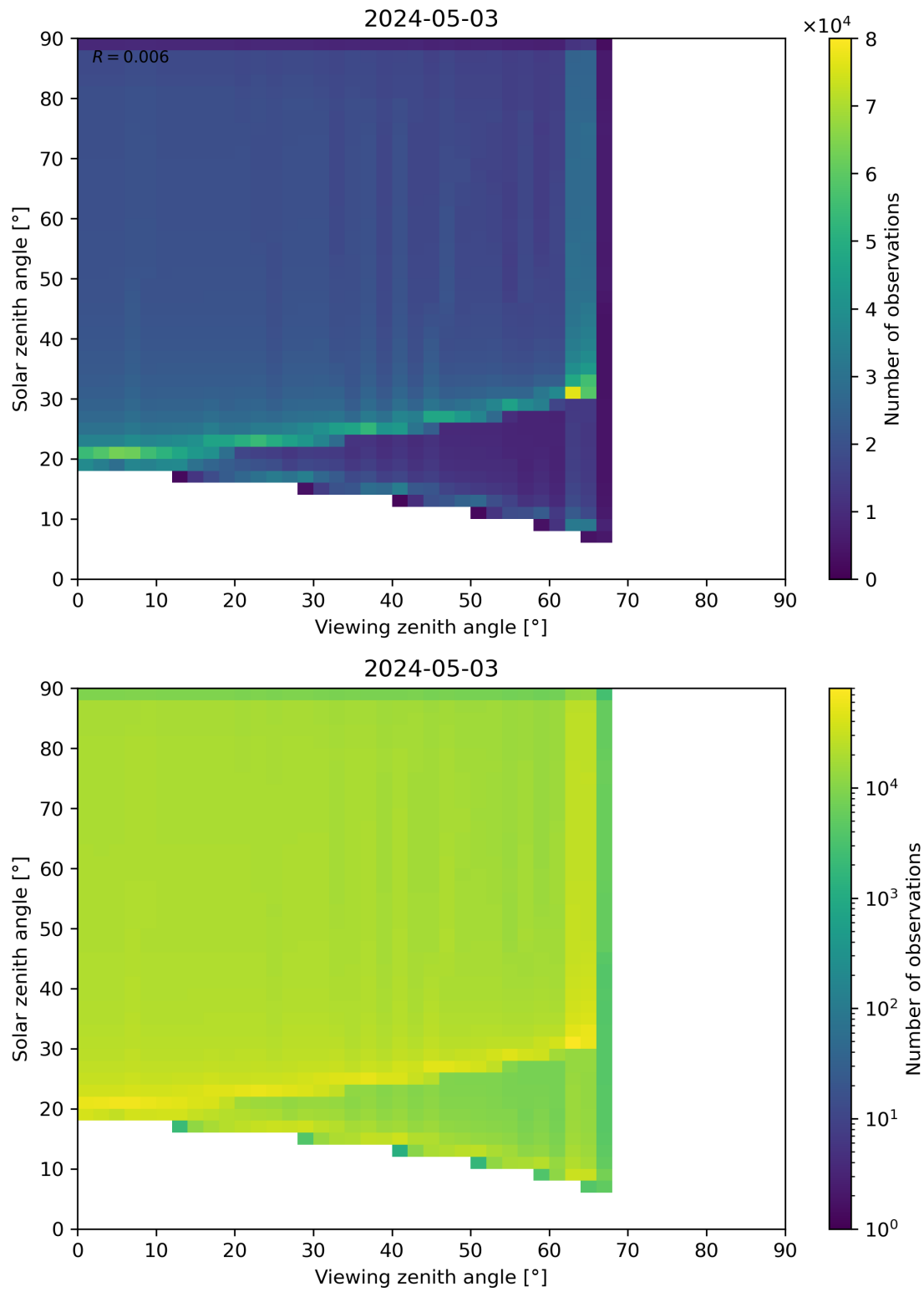
Figure 54: Scatter density plot of “Viewing zenith angle” against “Solar zenith angle” for 2024-05-02 to 2024-05-04.
