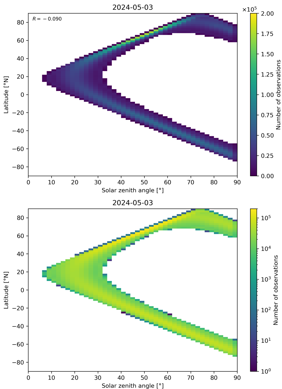
Figure 44: Scatter density plot of “Solar zenith angle” against “Latitude” for 2024-05-02 to 2024-05-04.
