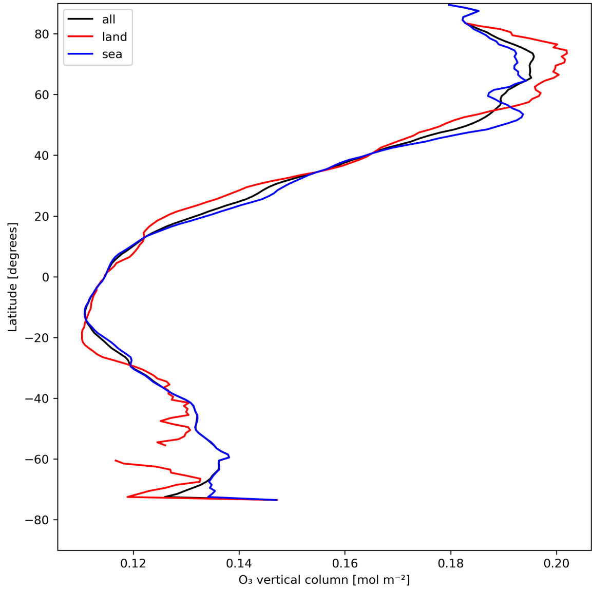
Figure 14: Zonal average of “O 3 vertical column” for 2024-05-02 to 2024-05-04.
