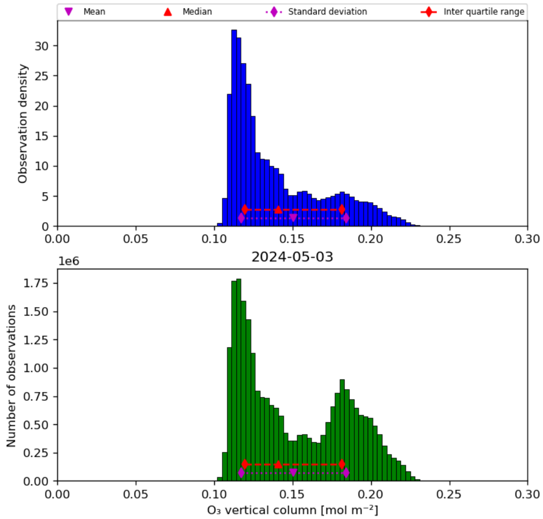
Figure 21: Histogram of “O 3 vertical column” for 2024-05-02 to 2024-05-04
