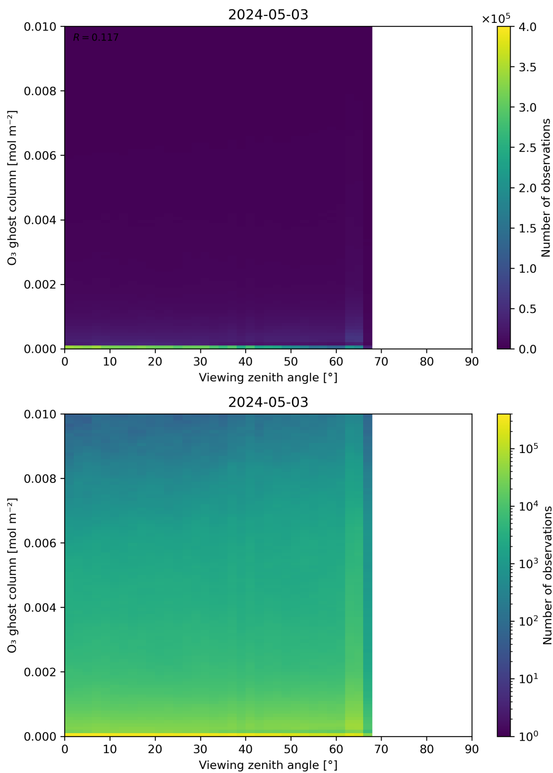
Figure 51: Scatter density plot of “Viewing zenith angle” against “O 3 ghost column” for 2024-05-02 to 2024-05-04.
