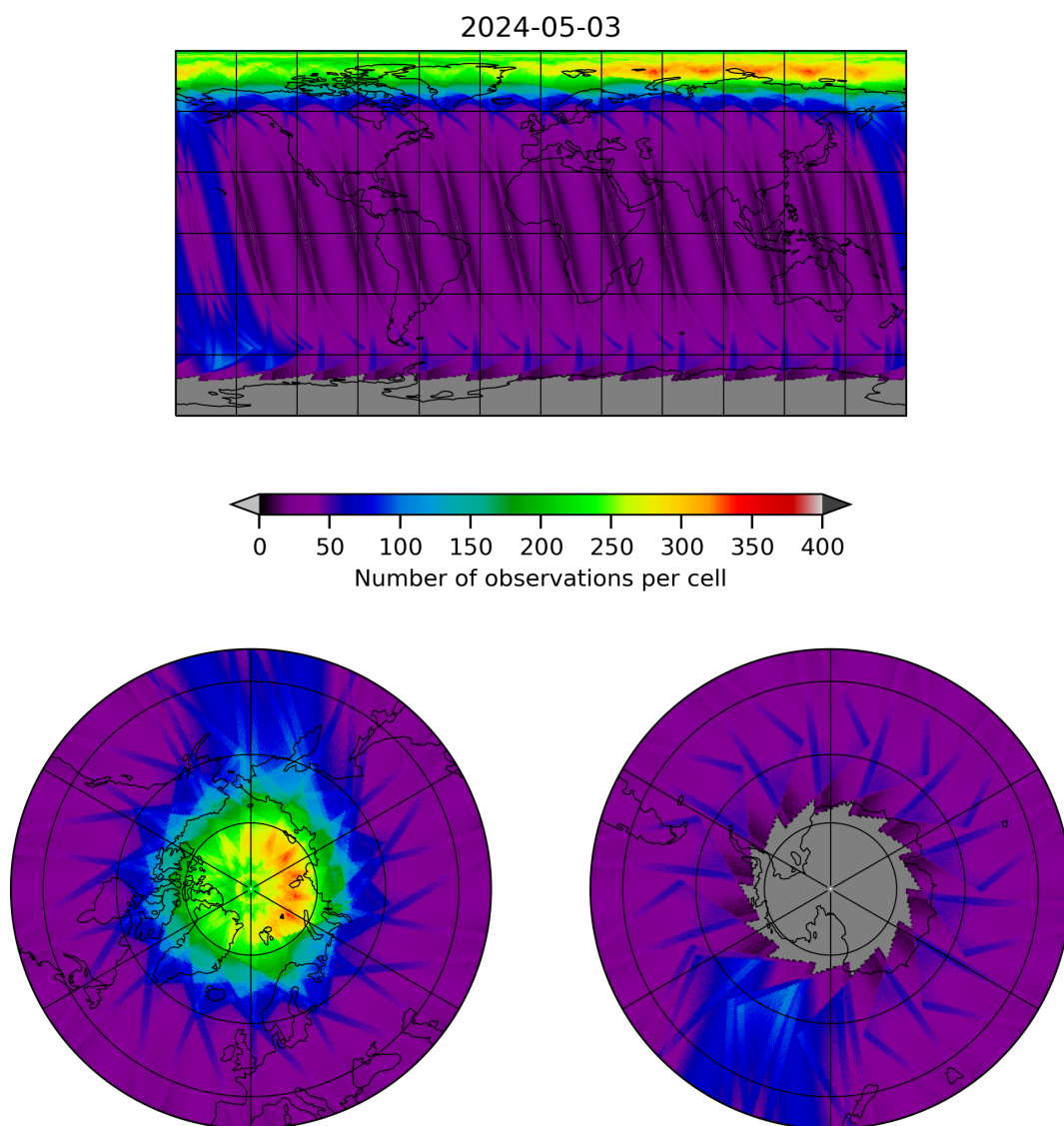
Figure 12: Map of the number of observations for 2024-05-02 to 2024-05-04
