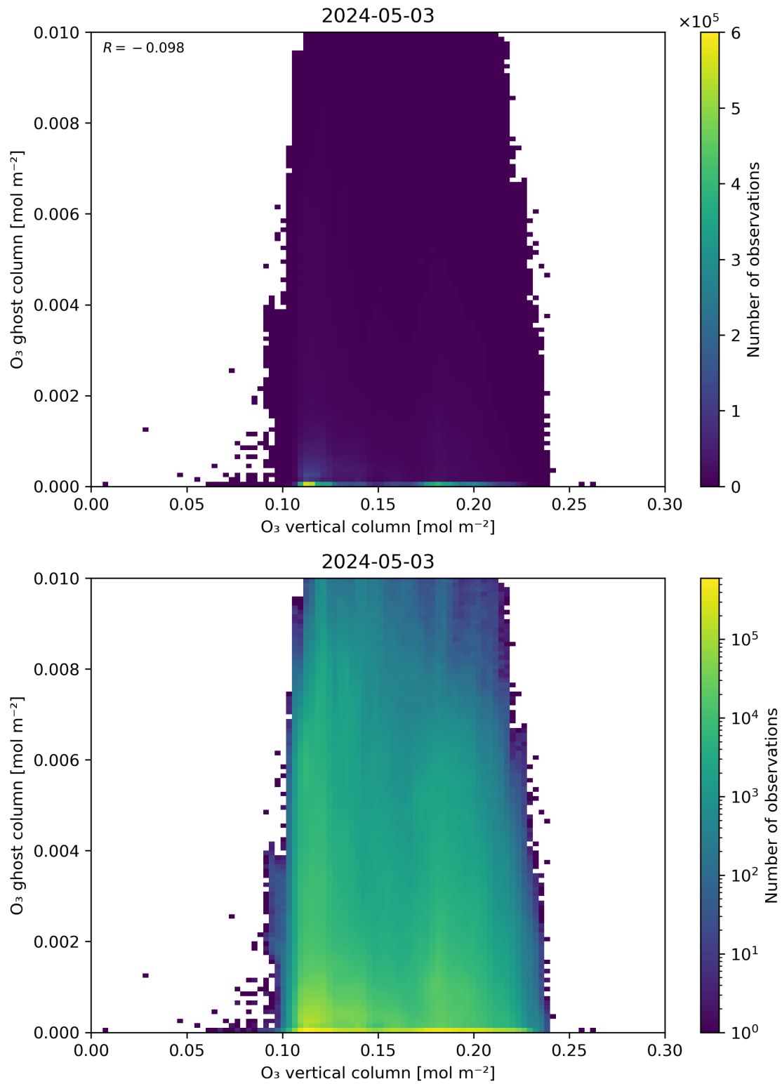
Figure 40: Scatter density plot of “O 3 vertical column” against “O 3 ghost column” for 2024-05-02 to 2024-05-04.
