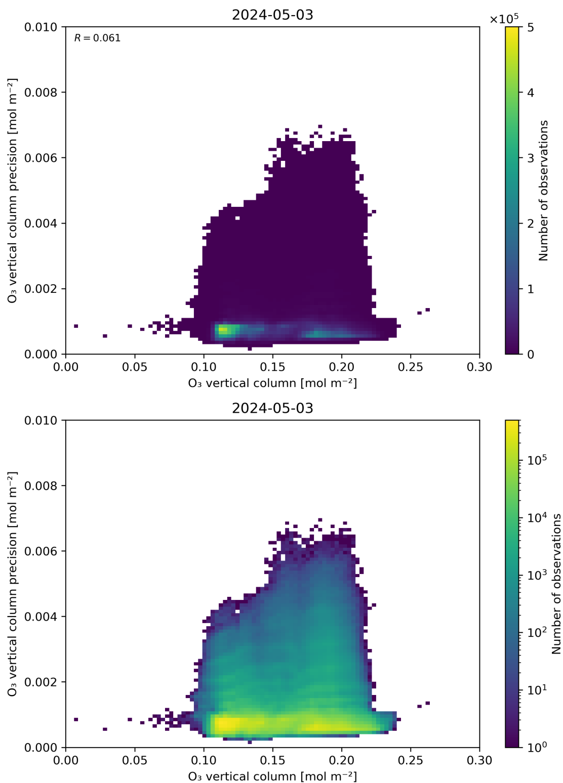
Figure 41: Scatter density plot of “O 3 vertical column” against “O 3 vertical column precision” for 2024-05-02 to 2024-05-04.
