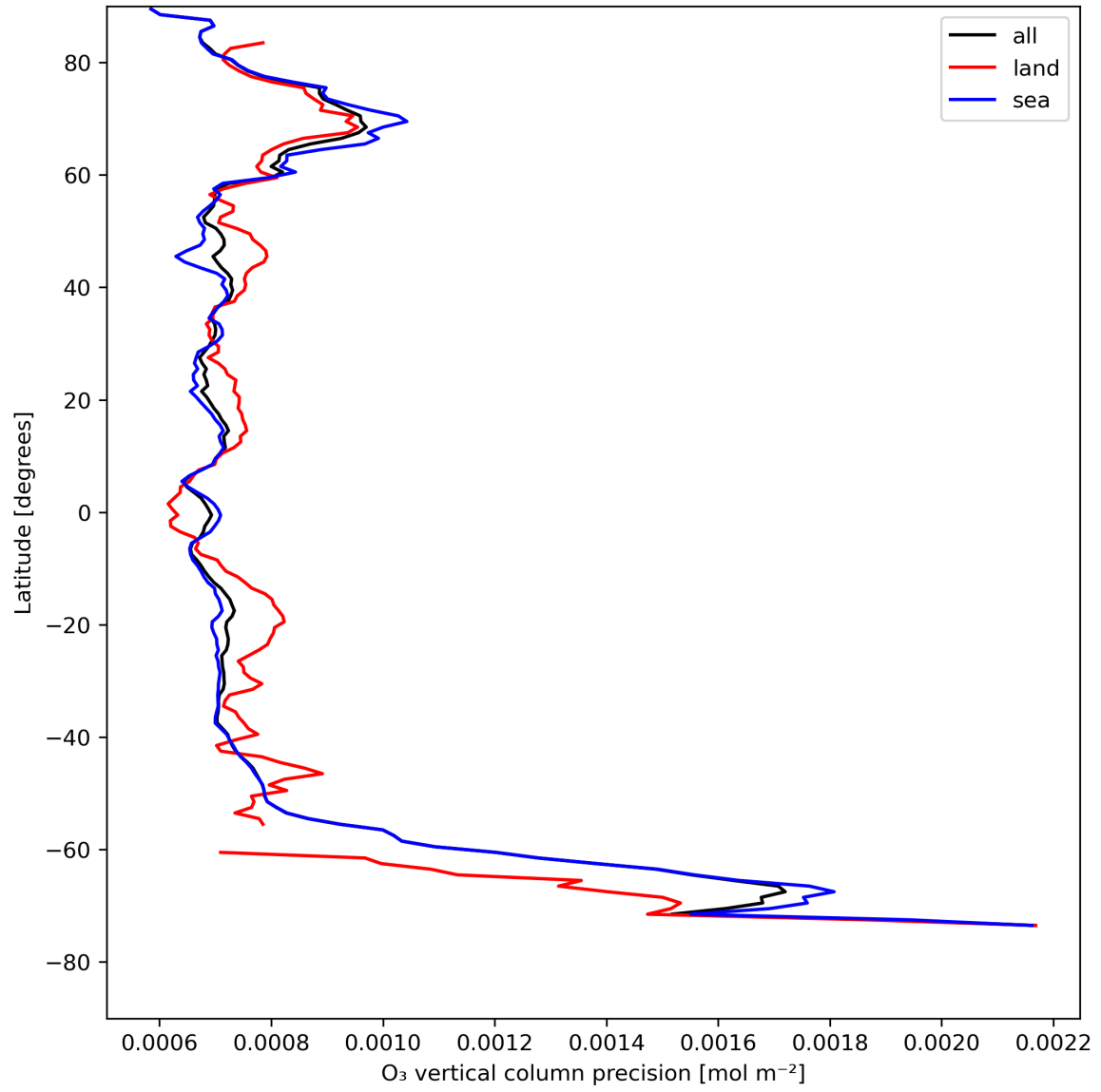
Figure 15: Zonal average of “O 3 vertical column precision” for 2024-05-02 to 2024-05-04.
