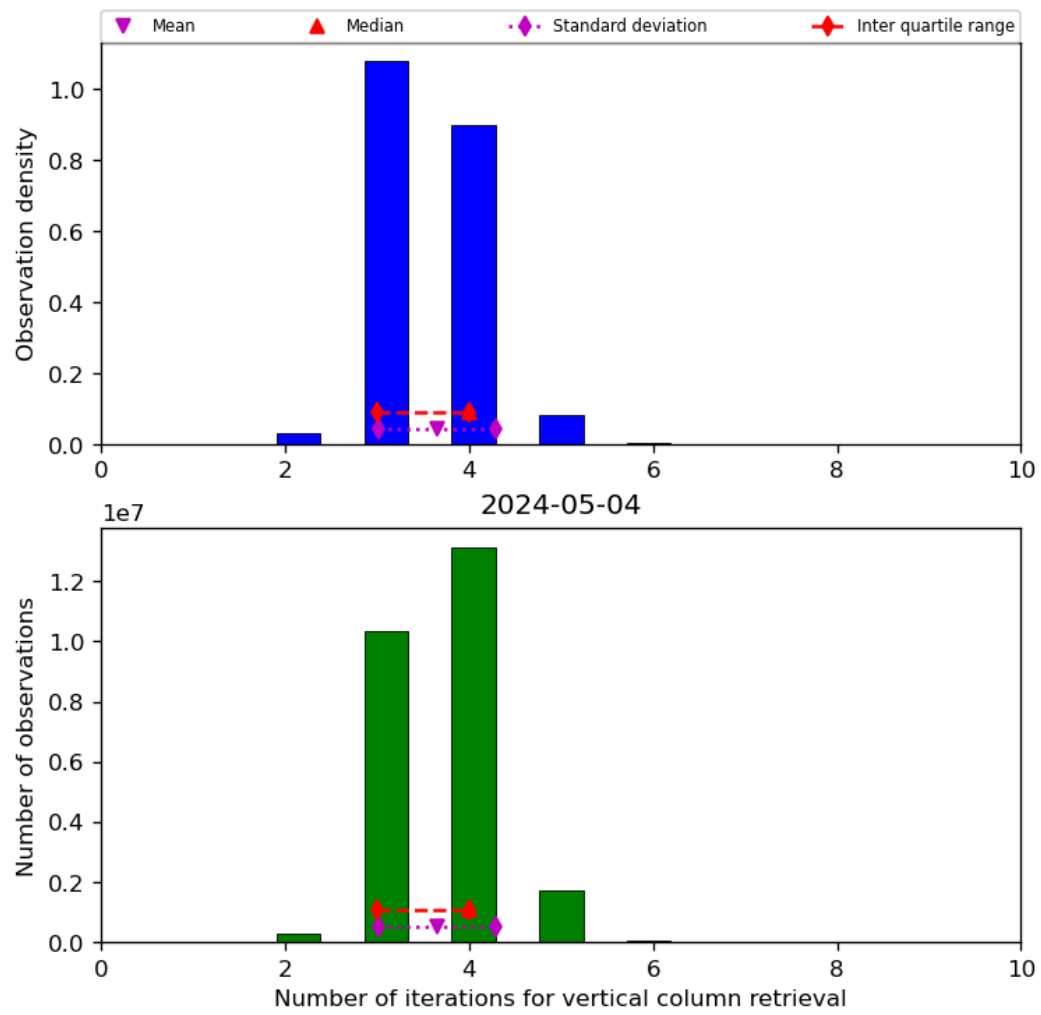
Figure 26: Histogram of “Number of iterations for vertical column retrieval” for 2024-05-03 to 2024-05-05
