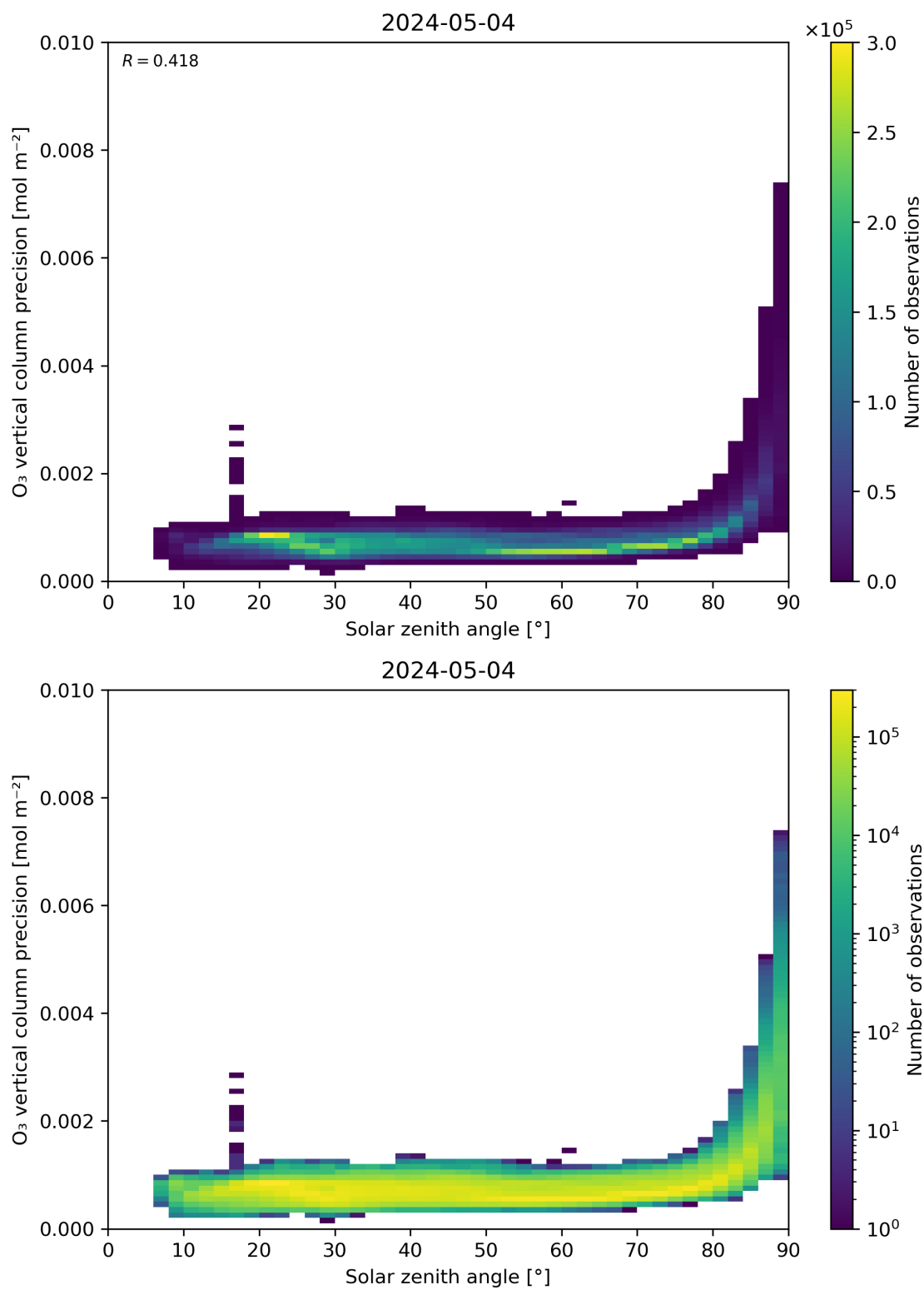
Figure 48: Scatter density plot of “Solar zenith angle” against “O 3 vertical column precision” for 2024-05-03 to 2024-05-05.
