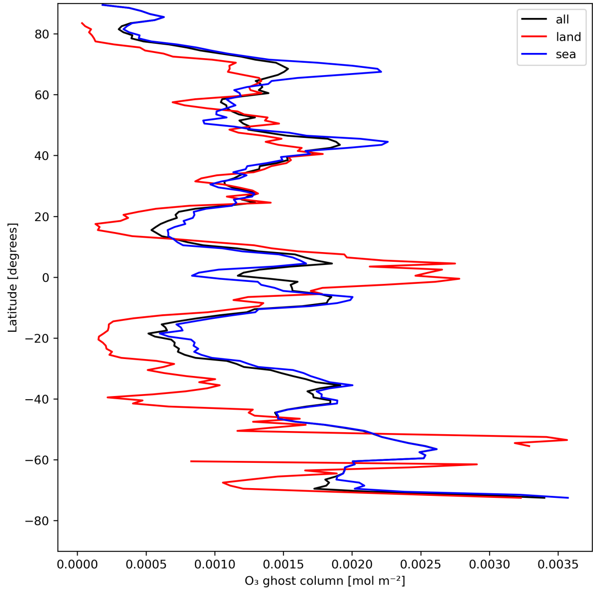
Figure 18: Zonal average of "O 3 ghost column" for 2024-05-03 to 2024-05-05.
