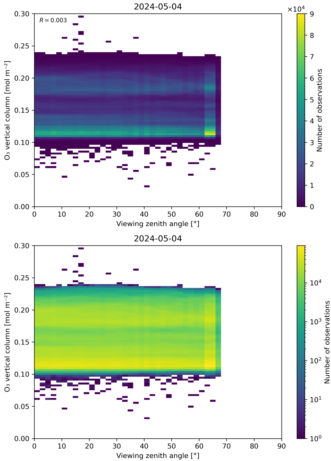
Figure 52: Scatter density plot of “Viewing zenith angle” against “O 3 vertical column” for 2024-05-03 to 2024-05-05.
