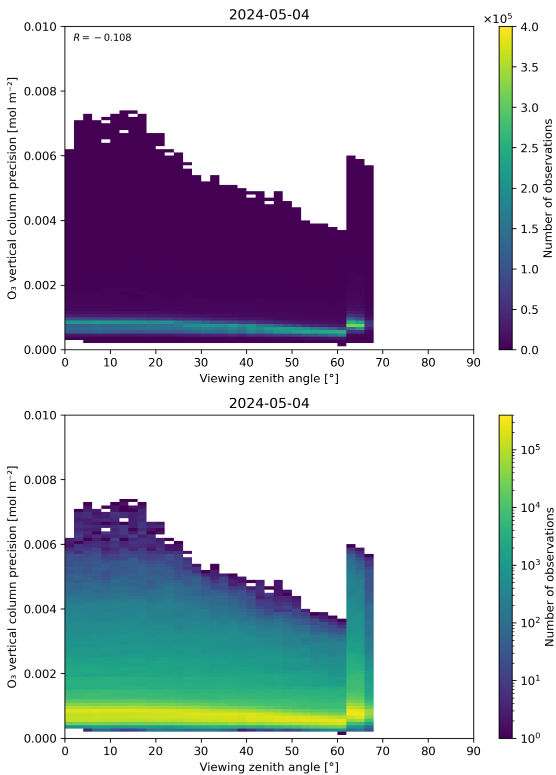
Figure 53: Scatter density plot of “Viewing zenith angle” against “O 3 vertical column precision” for 2024-05-03 to 2024-05-05.
