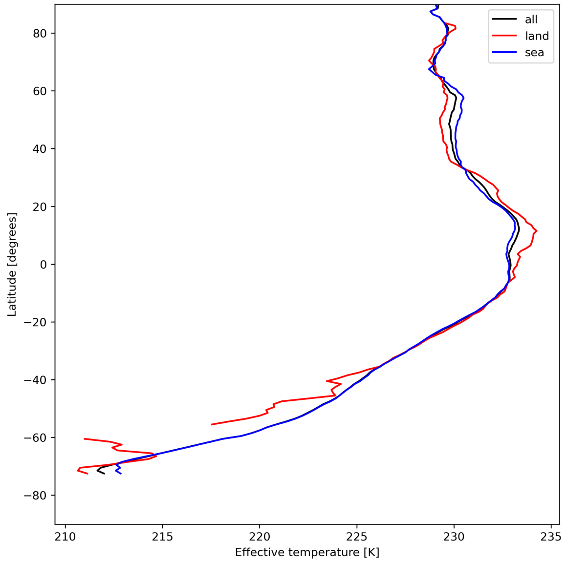
Figure 17: Zonal average of “Effective temperature” for 2024-05-03 to 2024-05-05.
