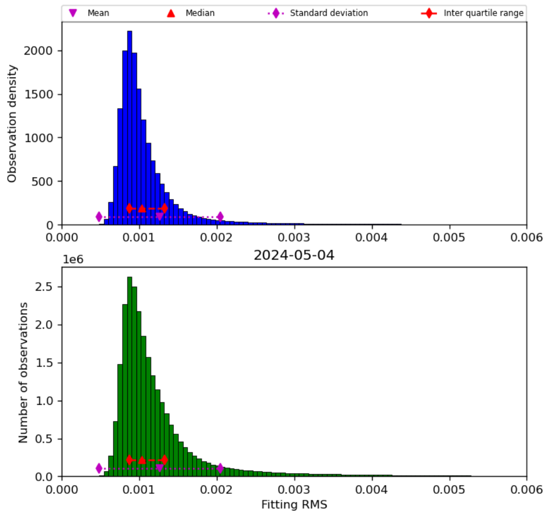
Figure 23: Histogram of “Fitting RMS” for 2024-05-03 to 2024-05-05
