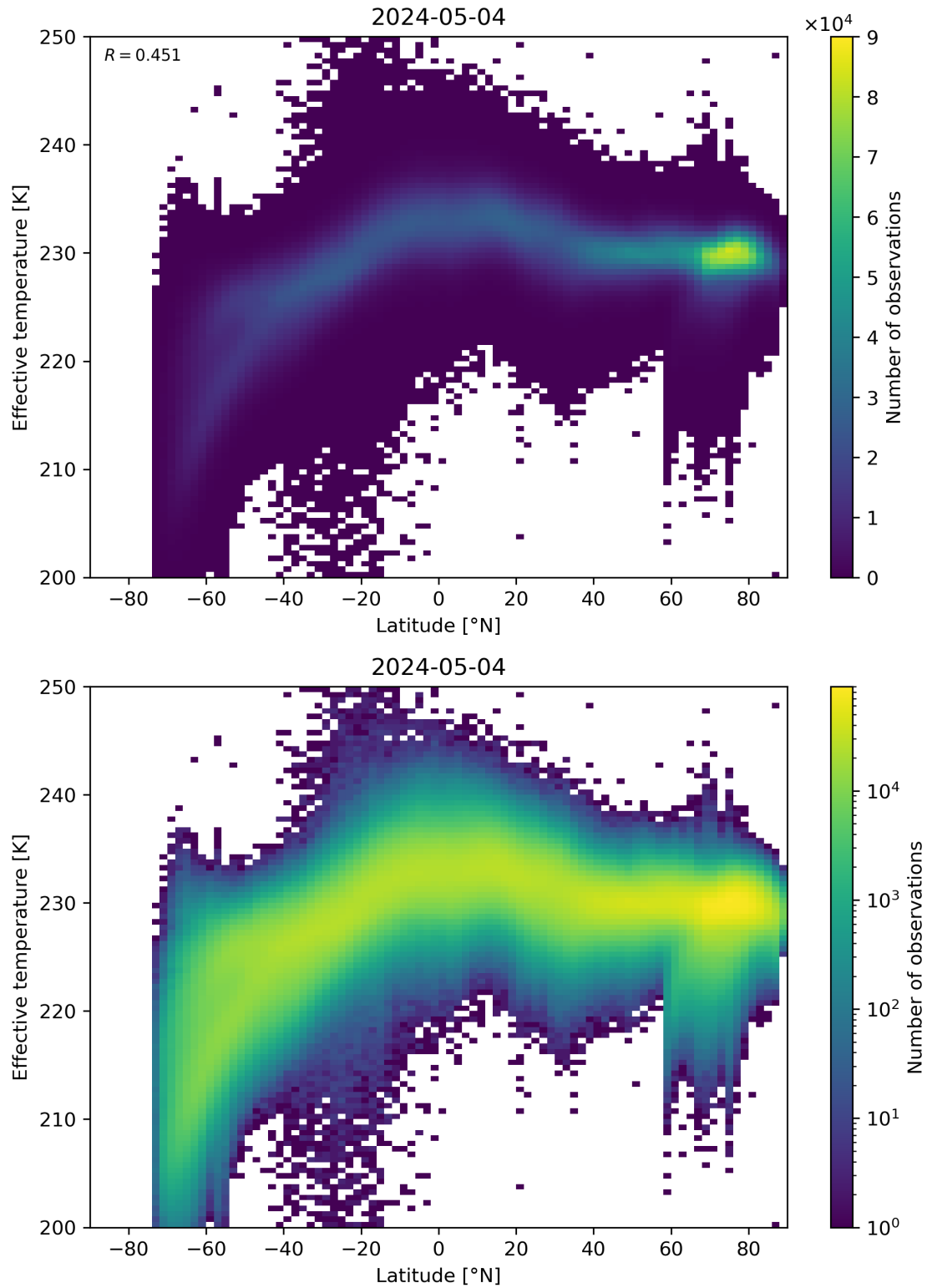
Figure 34: Scatter density plot of “Latitude” against “Effective temperature” for 2024-05-03 to 2024-05-05.
