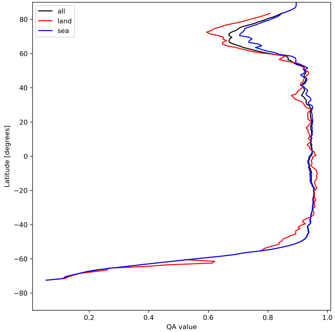
Figure 13: Zonal average of “QA value” for 2024-05-03 to 2024-05-05.
