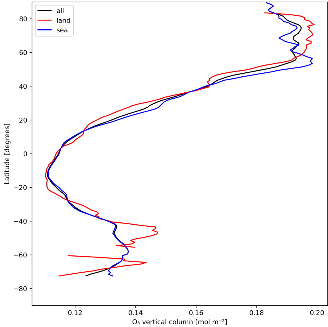
Figure 14: Zonal average of “O 3 vertical column” for 2024-05-03 to 2024-05-05.
