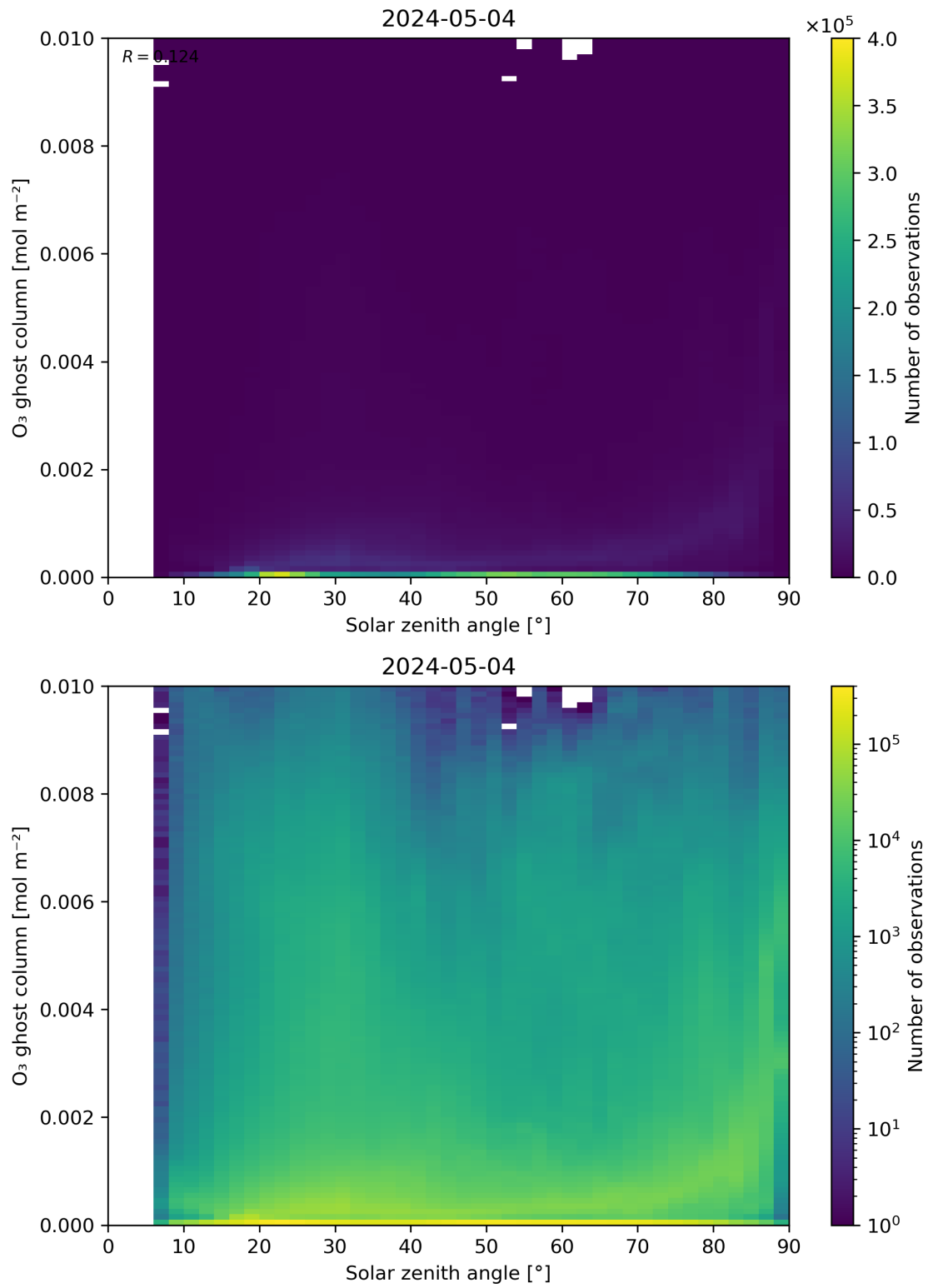
Figure 46: Scatter density plot of “Solar zenith angle” against “O 3 ghost column” for 2024-05-03 to 2024-05-05.
