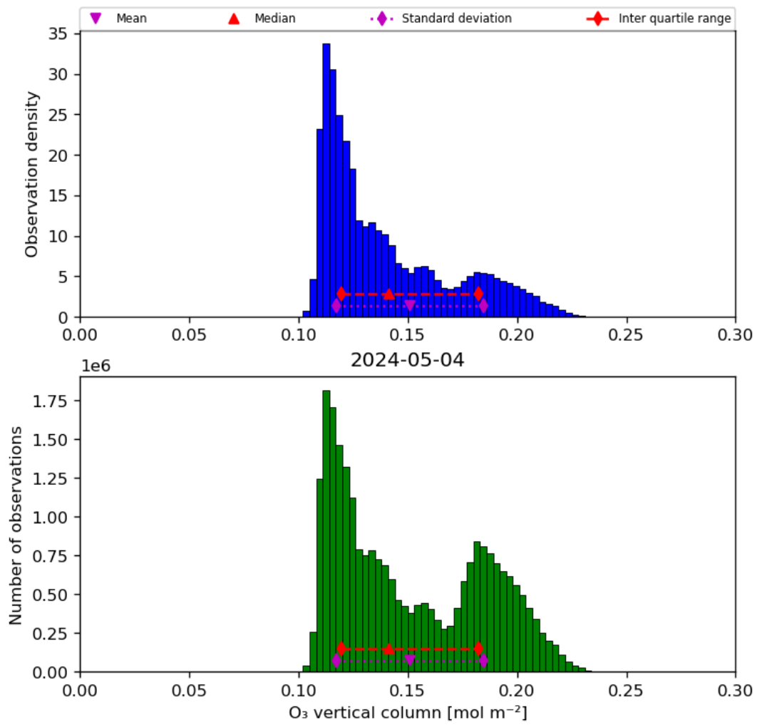
Figure 21: Histogram of “O 3 vertical column” for 2024-05-03 to 2024-05-05
