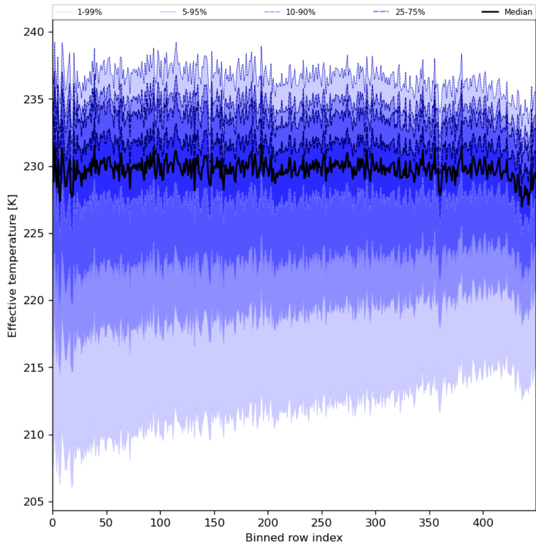
Figure 31: Along track statistics of “Effective temperature” for 2024-05-03 to 2024-05-05
