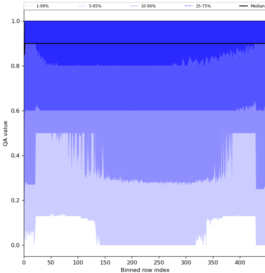
Figure 27: Along track statistics of “QA value” for 2024-05-03 to 2024-05-05
