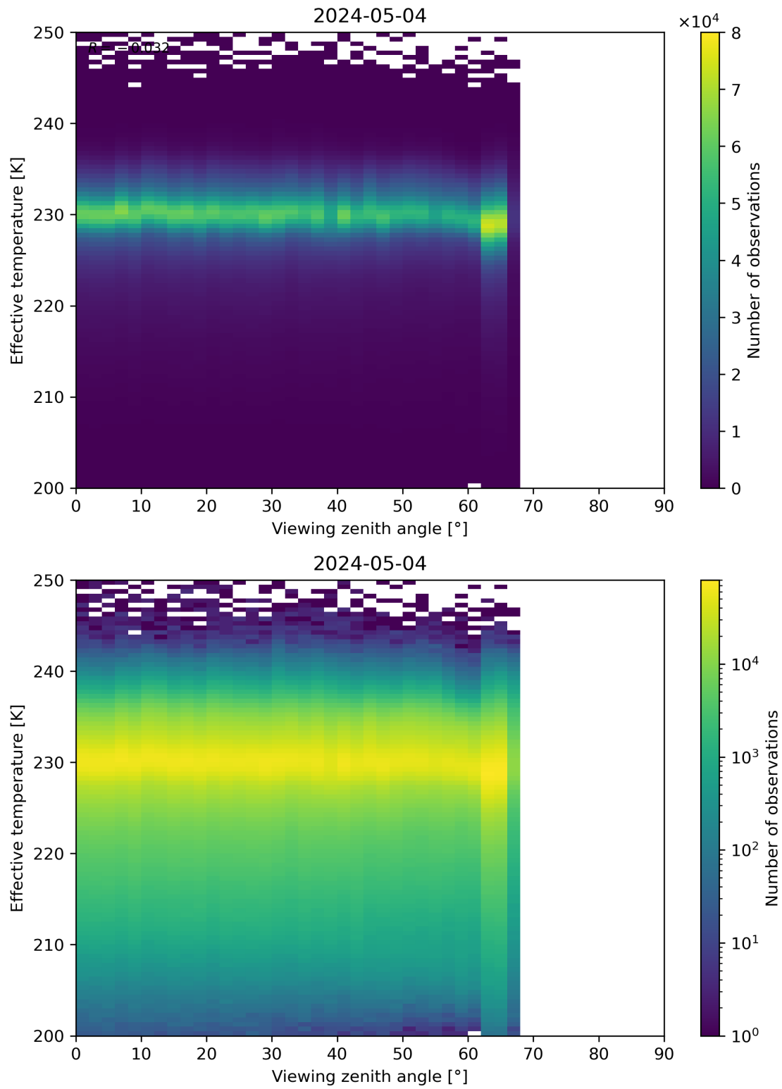
Figure 50: Scatter density plot of “Viewing zenith angle” against “Effective temperature” for 2024-05-03 to 2024-05-05.
