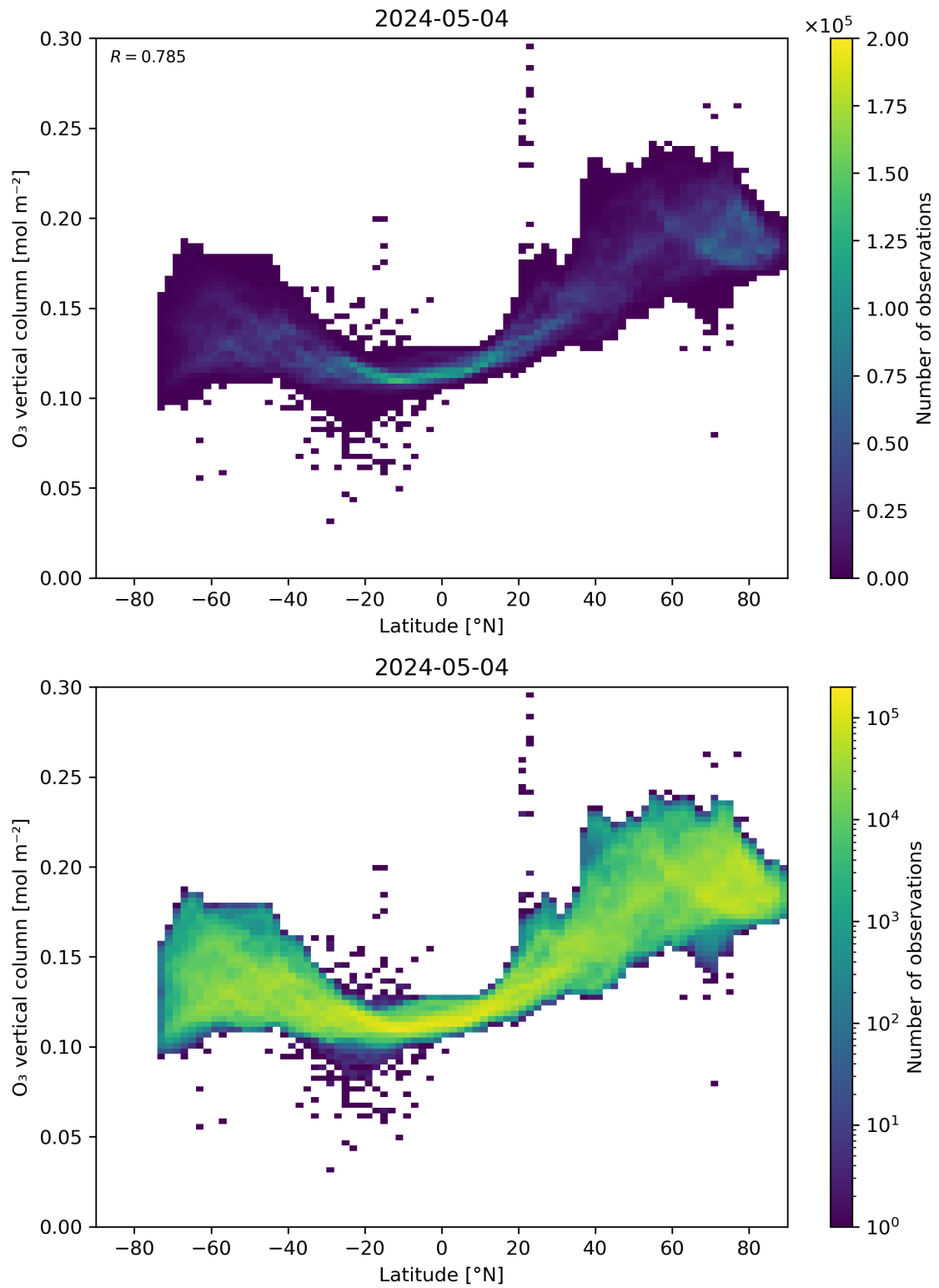
Figure 36: Scatter density plot of “Latitude” against “O 3 vertical column” for 2024-05-03 to 2024-05-05.
