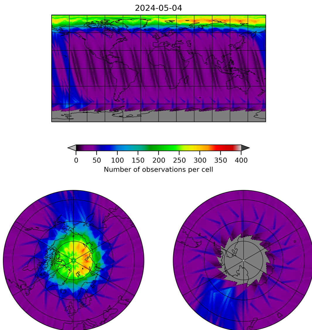
Figure 12: Map of the number of observations for 2024-05-03 to 2024-05-05
