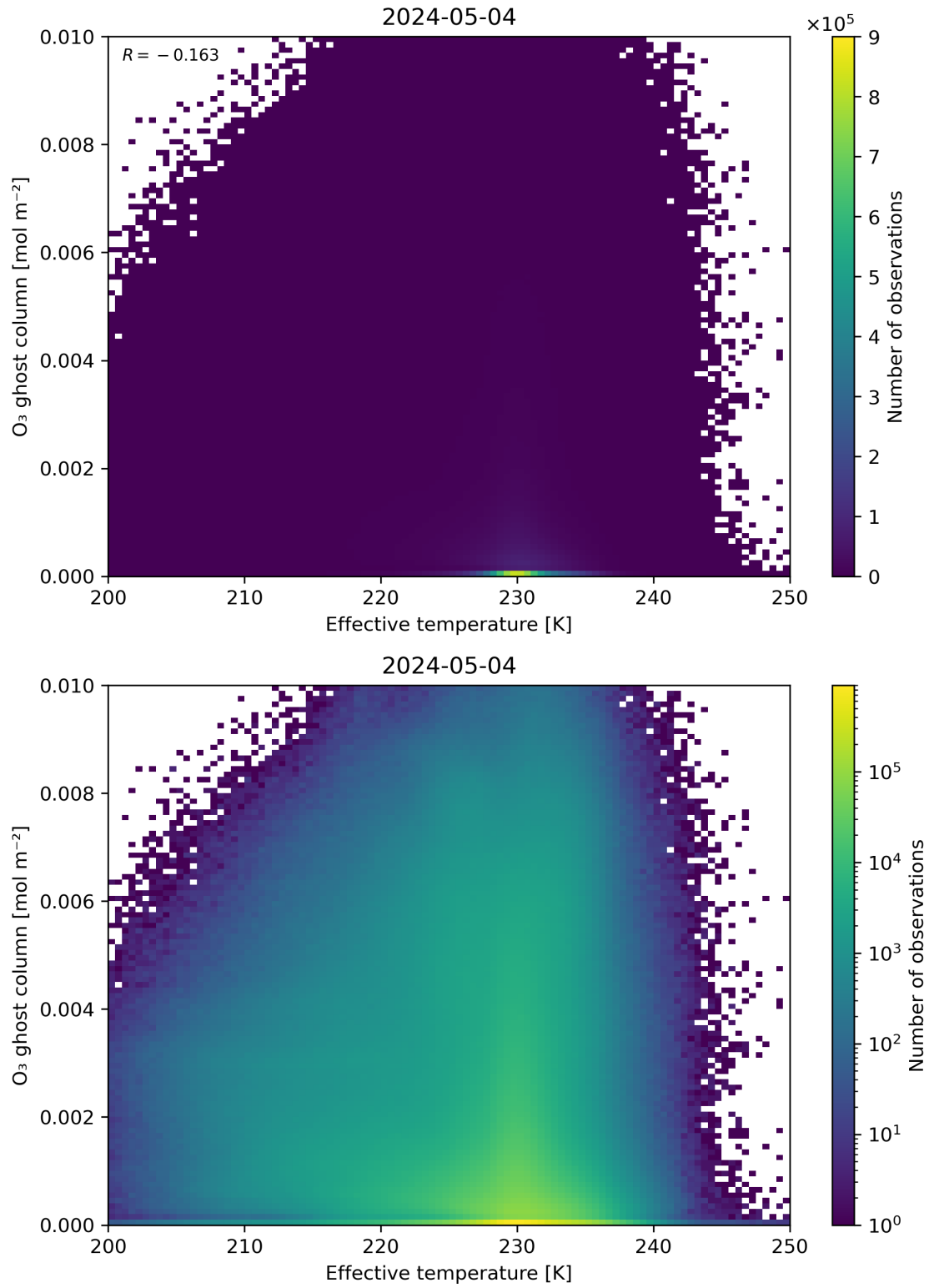
Figure 38: Scatter density plot of “Effective temperature” against “O 3 ghost column” for 2024-05-03 to 2024-05-05.
