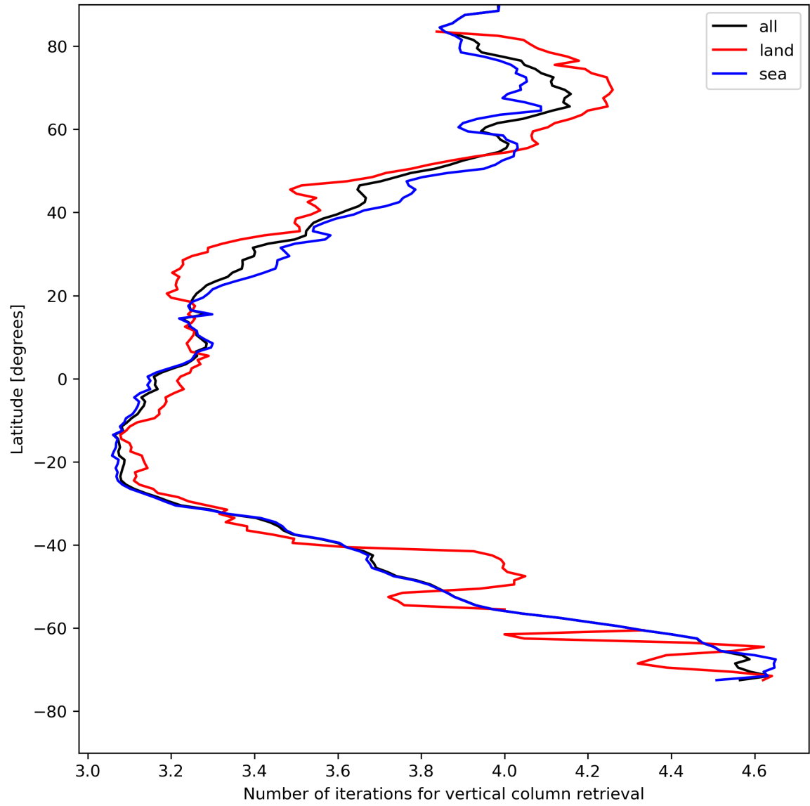
Figure 19: Zonal average of “Number of iterations for vertical column retrieval” for 2024-05-03 to 2024-05-05.
