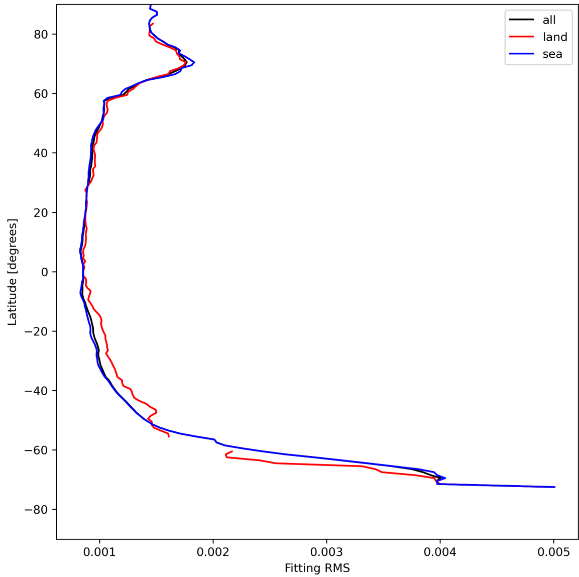
Figure 16: Zonal average of “Fitting RMS” for 2024-05-03 to 2024-05-05.
