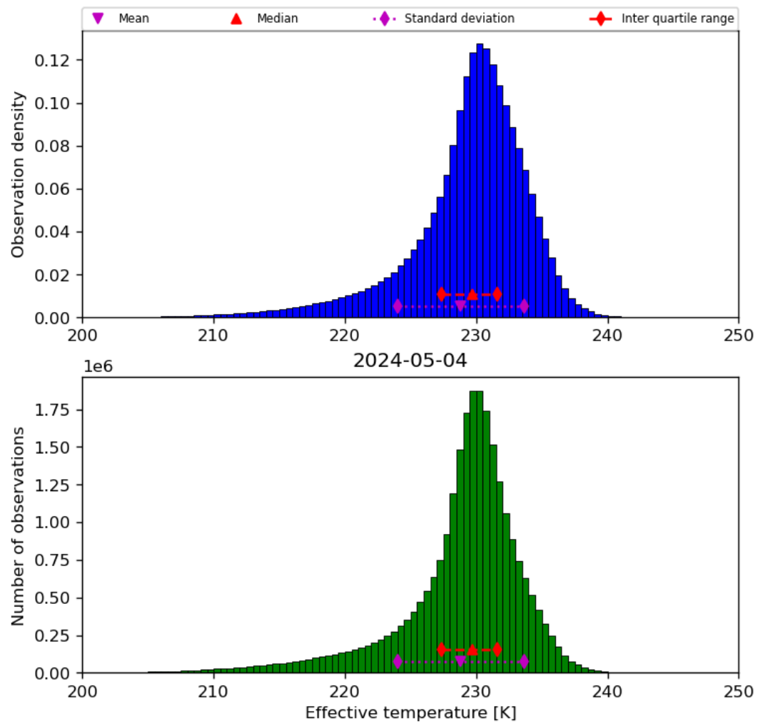
Figure 24: Histogram of “Effective temperature” for 2024-05-03 to 2024-05-05
