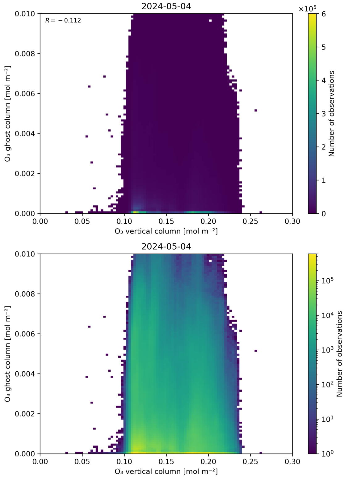
Figure 40: Scatter density plot of “O 3 vertical column” against “O 3 ghost column” for 2024-05-03 to 2024-05-05.
