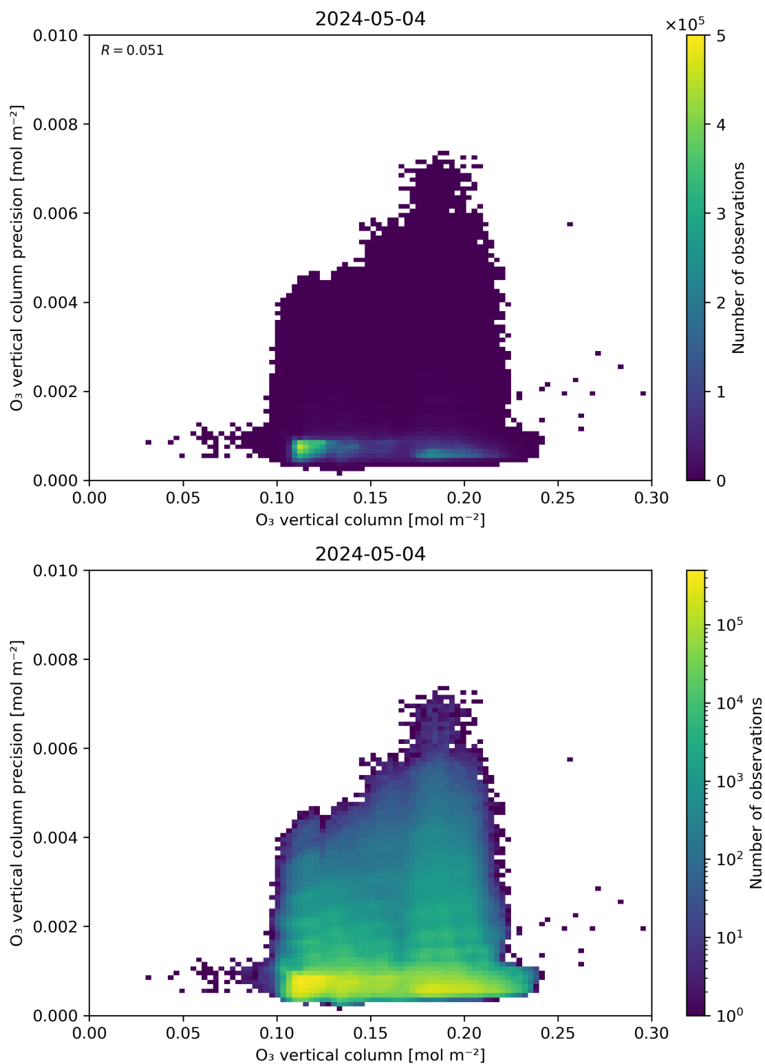
Figure 41: Scatter density plot of “O 3 vertical column” against “O 3 vertical column precision” for 2024-05-03 to 2024-05-05.
