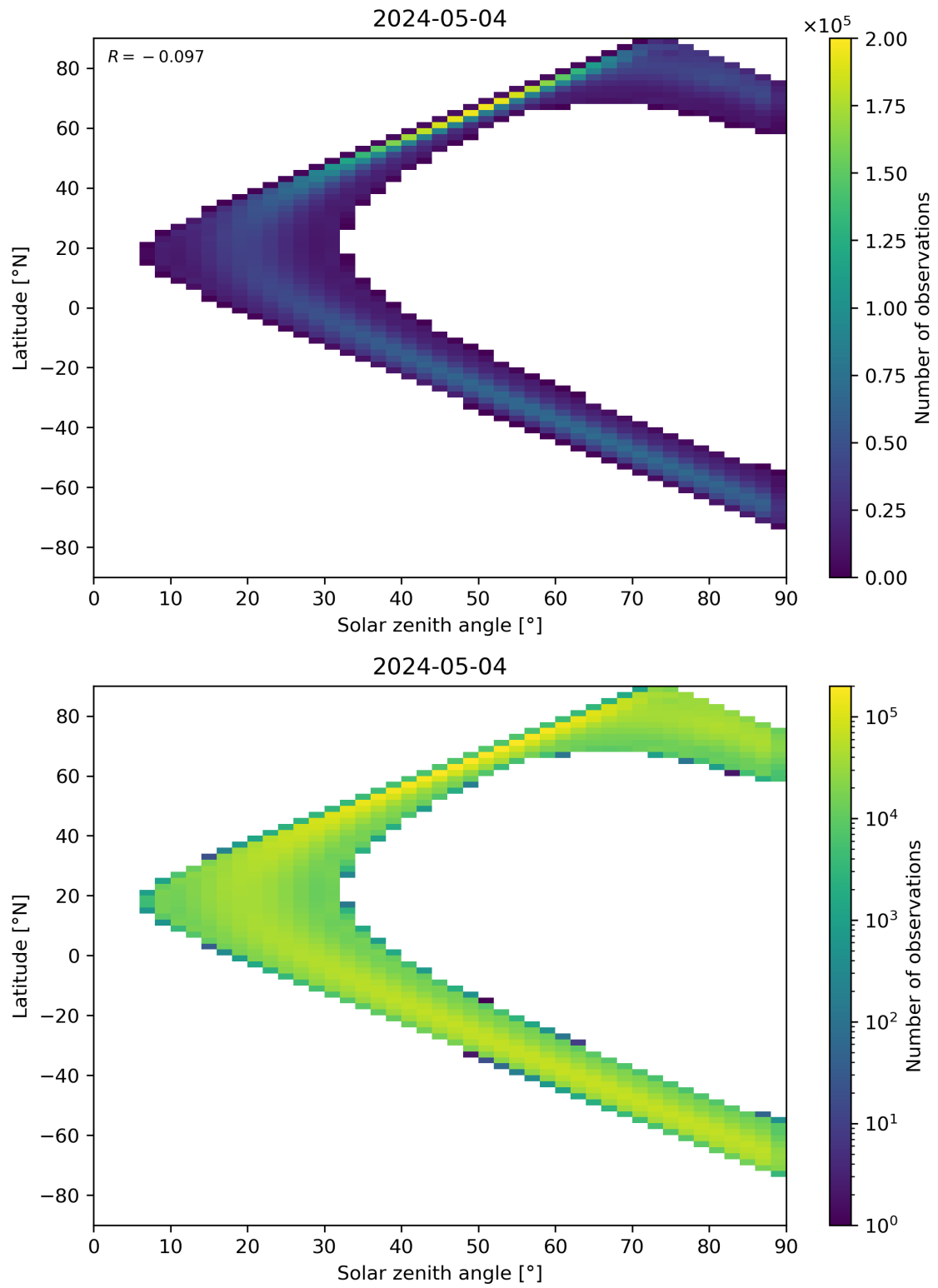
Figure 44: Scatter density plot of “Solar zenith angle” against “Latitude” for 2024-05-03 to 2024-05-05.
