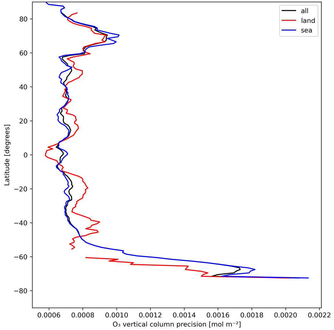
Figure 15: Zonal average of “O 3 vertical column precision” for 2024-05-03 to 2024-05-05.
