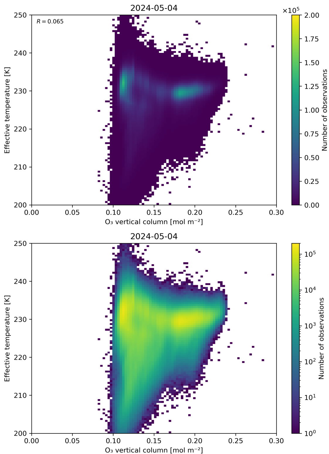
Figure 39: Scatter density plot of “O 3 vertical column” against “Effective temperature” for 2024-05-03 to 2024-05-05.
