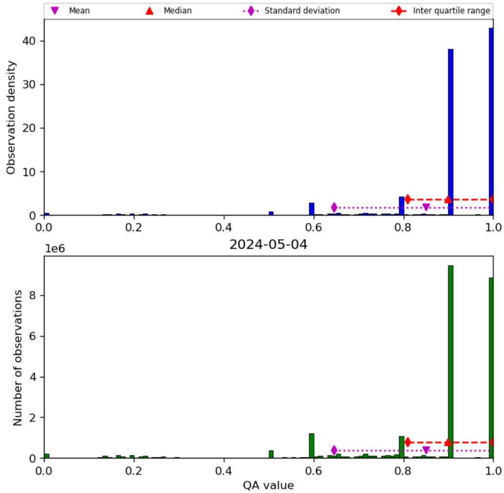
Figure 20: Histogram of “QA value” for 2024-05-03 to 2024-05-05
