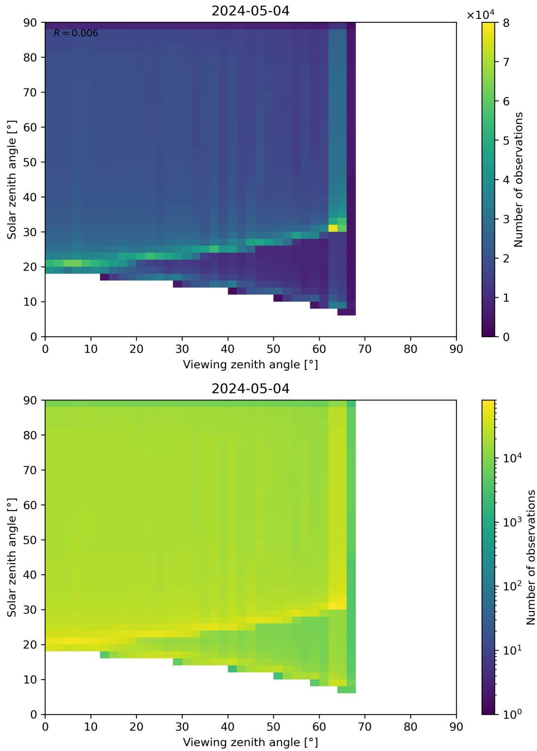
Figure 54: Scatter density plot of “Viewing zenith angle” against “Solar zenith angle” for 2024-05-03 to 2024-05-05.
