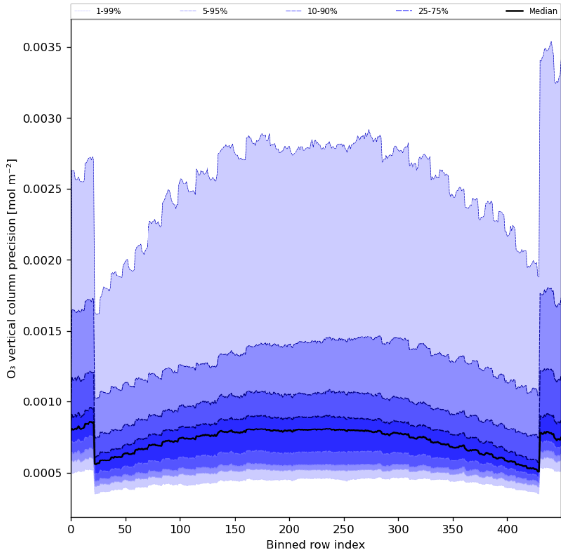
Figure 29: Along track statistics of “O 3 vertical column precision” for 2024-05-03 to 2024-05-05
