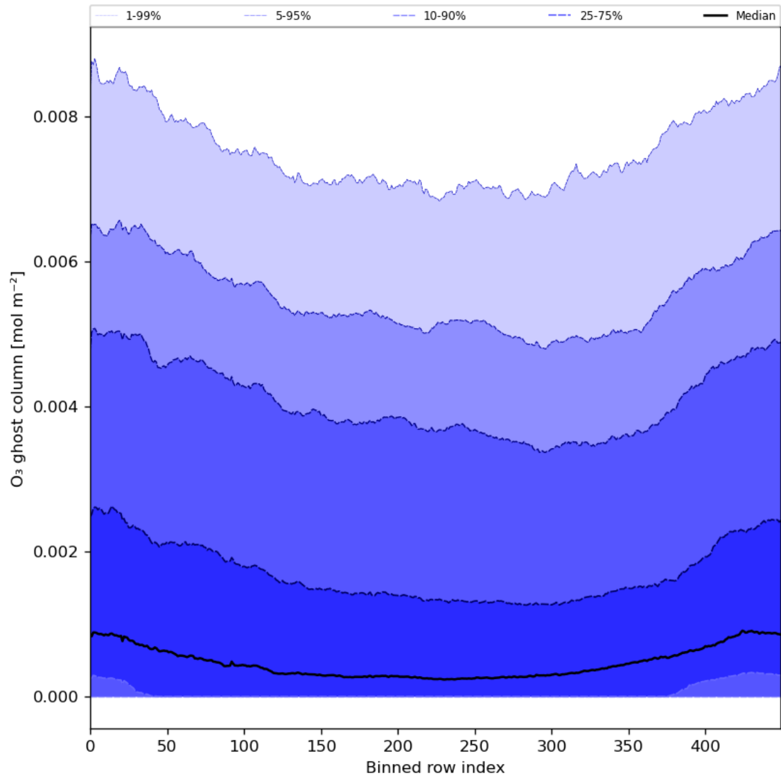
Figure 32: Along track statistics of “O 3 ghost column” for 2024-05-03 to 2024-05-05
