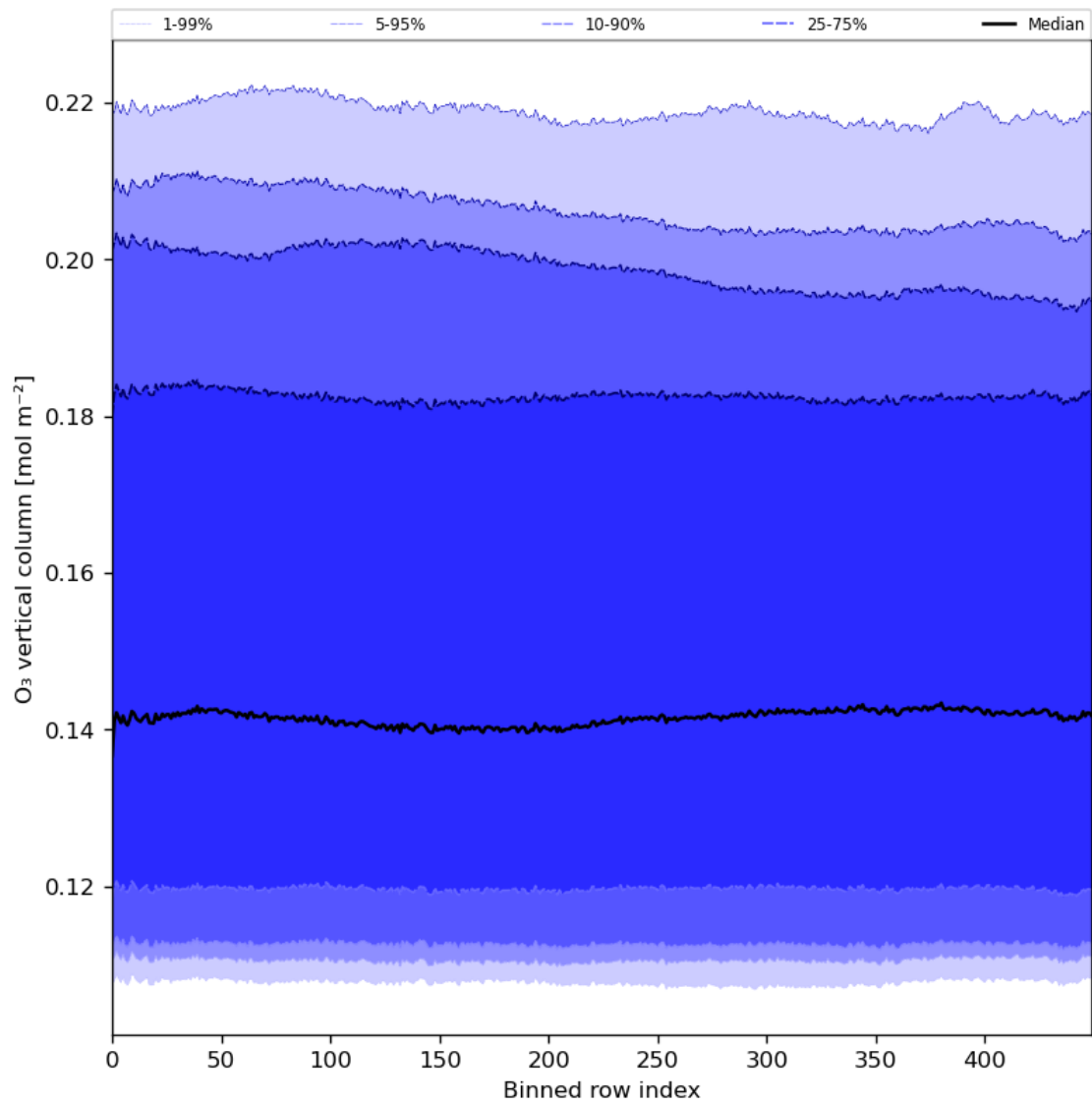
Figure 28: Along track statistics of “O 3 vertical column” for 2024-05-03 to 2024-05-05
