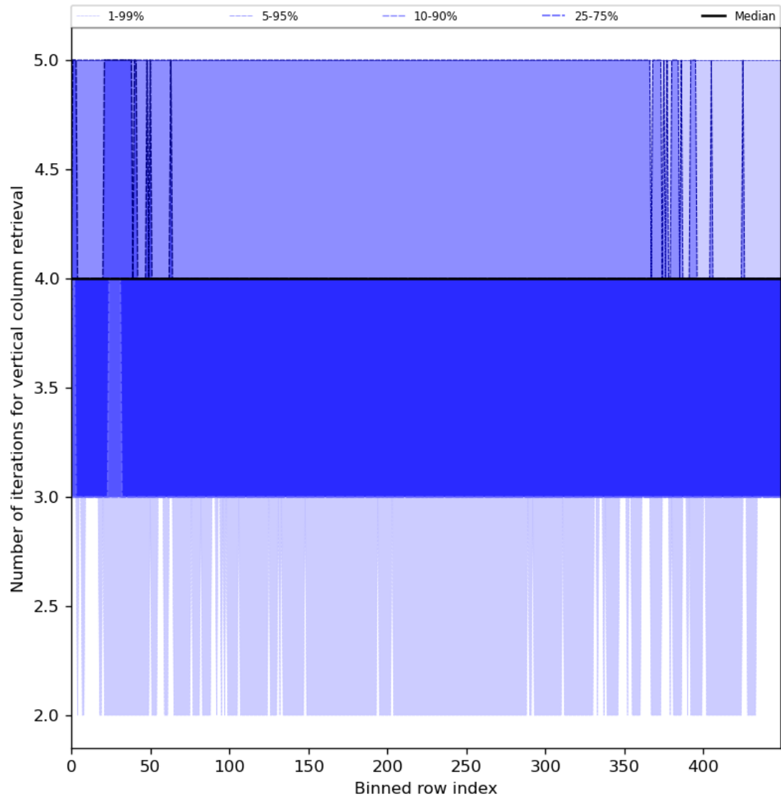
Figure 33: Along track statistics of “Number of iterations for vertical column retrieval” for 2024-05-03 to 2024-05-05
