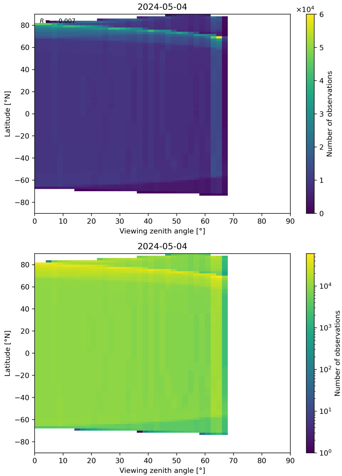
Figure 49: Scatter density plot of “Viewing zenith angle” against “Latitude” for 2024-05-03 to 2024-05-05.
