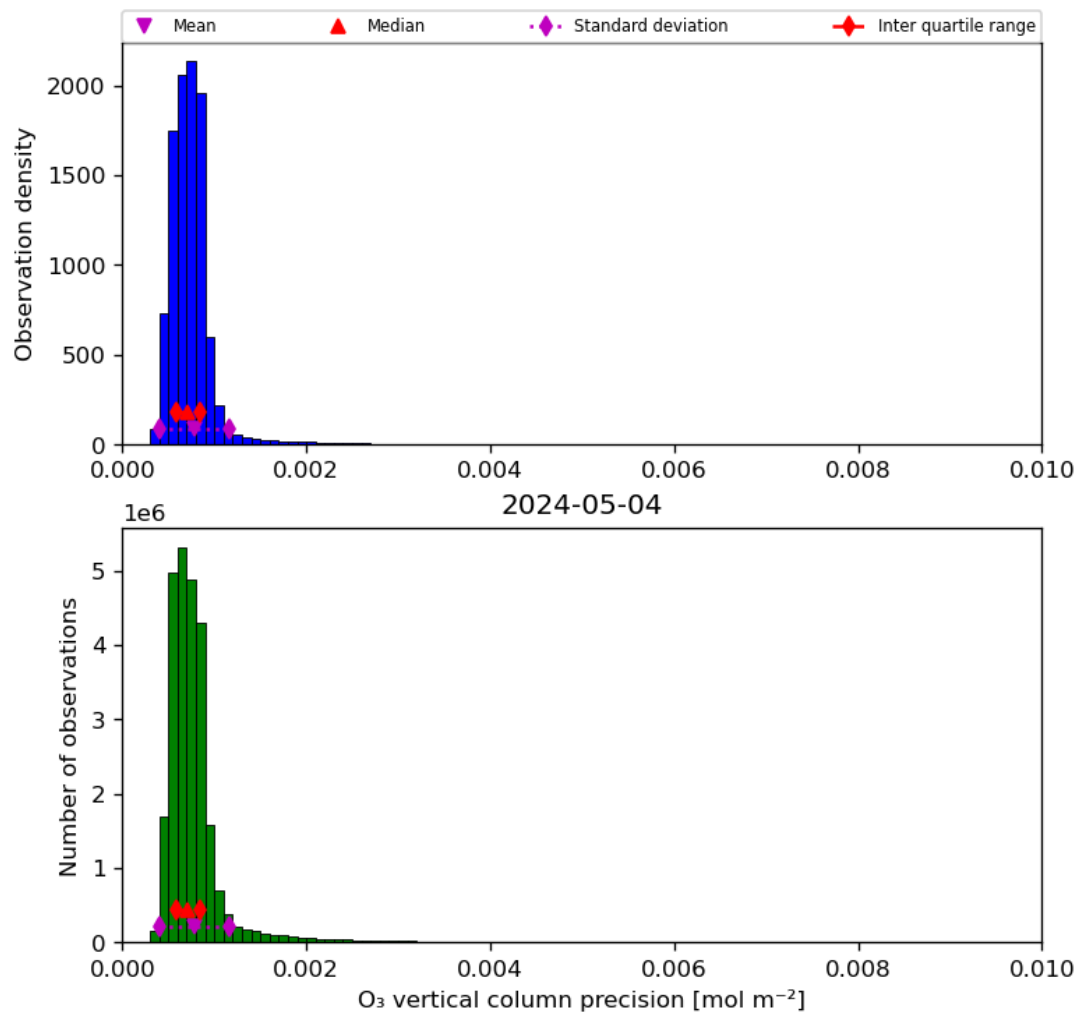
Figure 22: Histogram of “O 3 vertical column precision” for 2024-05-03 to 2024-05-05
