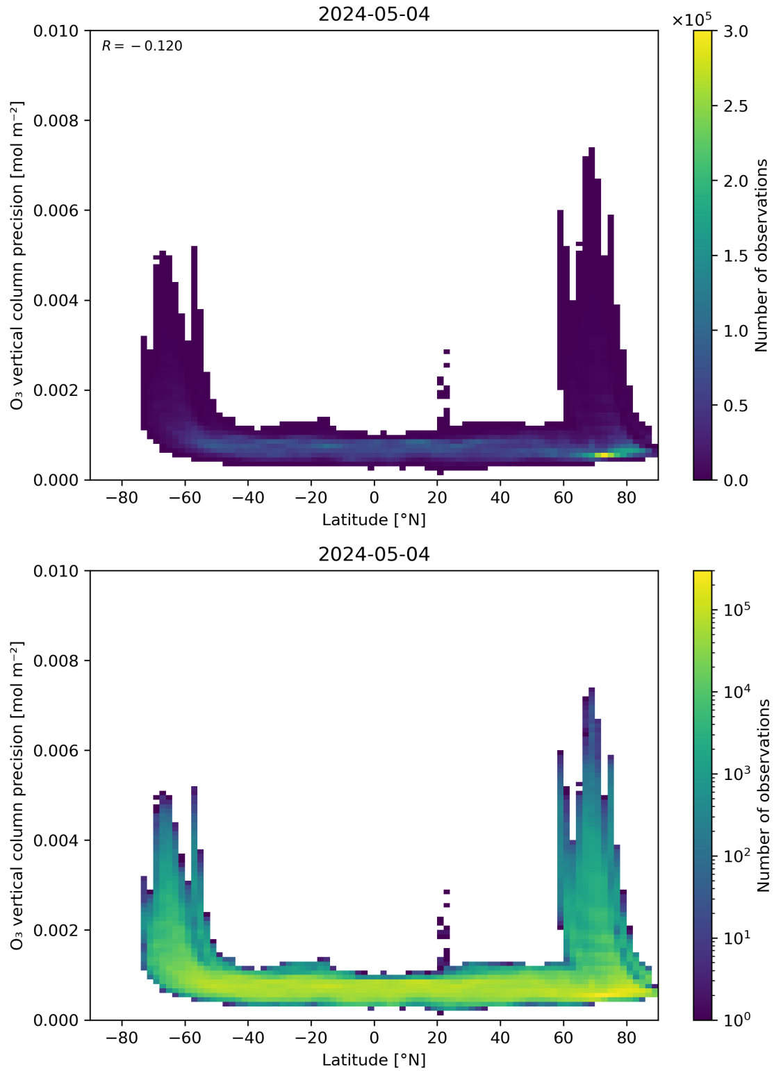
Figure 37: Scatter density plot of “Latitude” against “O 3 vertical column precision” for 2024-05-03 to 2024-05-05.
