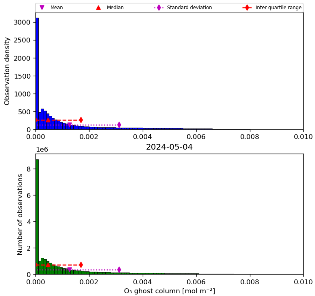
Figure 25: Histogram of "O 3 ghost column" for 2024-05-03 to 2024-05-05
