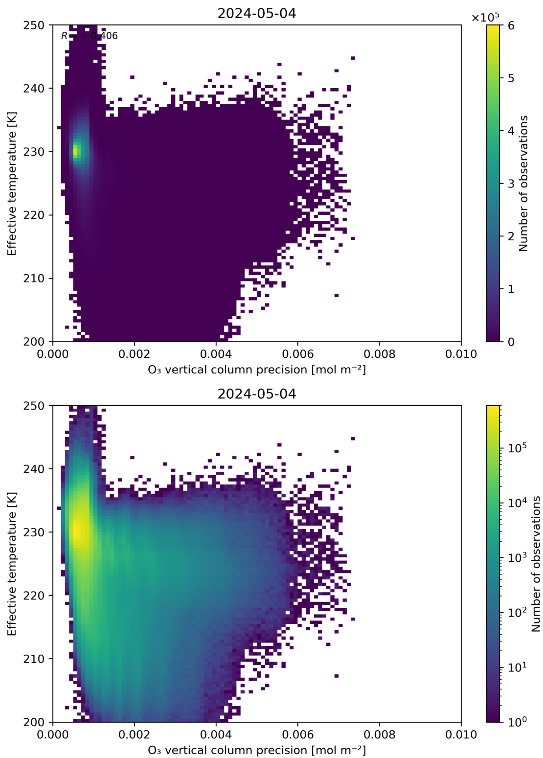
Figure 42: Scatter density plot of “O 3 vertical column precision” against “Effective temperature” for 2024-05-03 to 2024-05-05.
