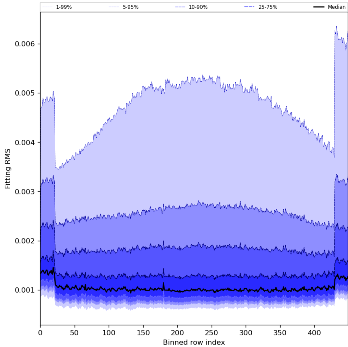
Figure 30: Along track statistics of “Fitting RMS” for 2024-05-03 to 2024-05-05
