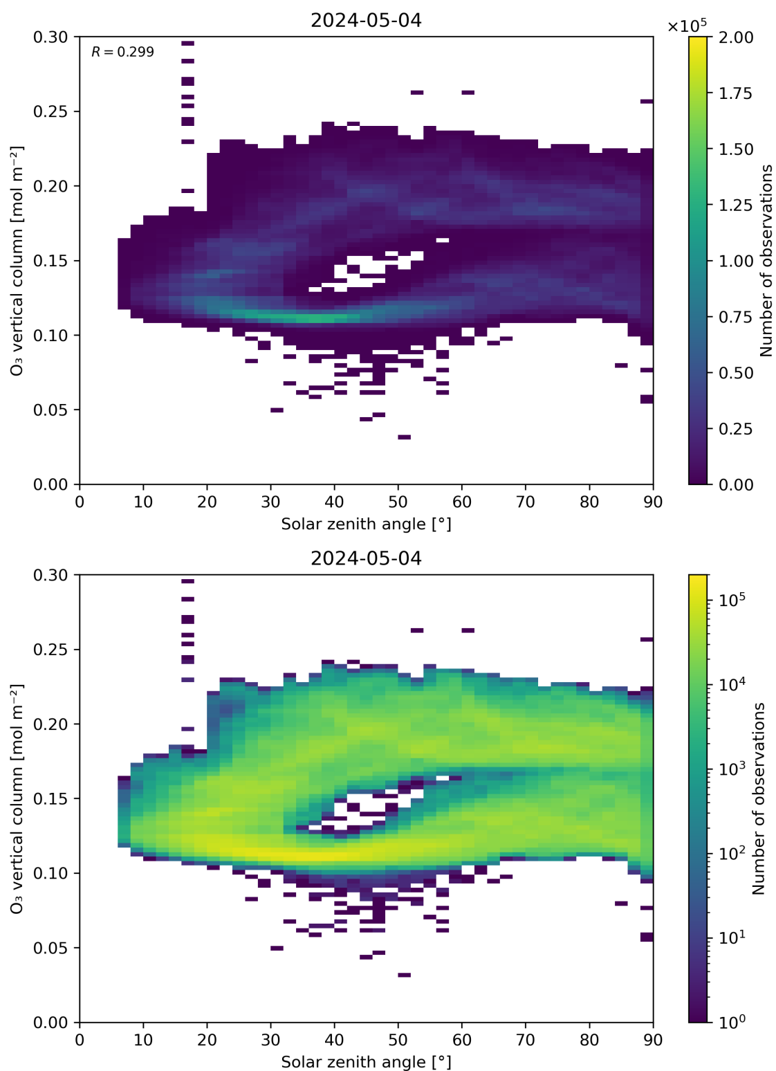
Figure 47: Scatter density plot of “Solar zenith angle” against “O 3 vertical column” for 2024-05-03 to 2024-05-05.
