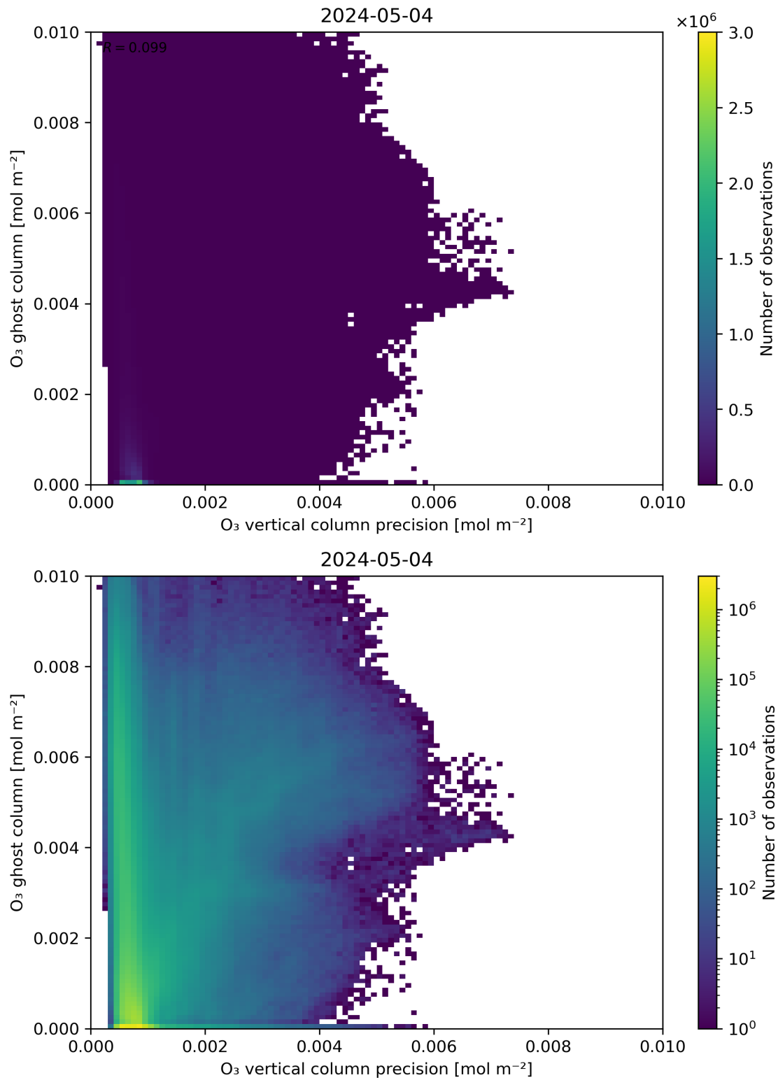
Figure 43: Scatter density plot of “O 3 vertical column precision” against “O 3 ghost column” for 2024-05-03 to 2024-05-05.
