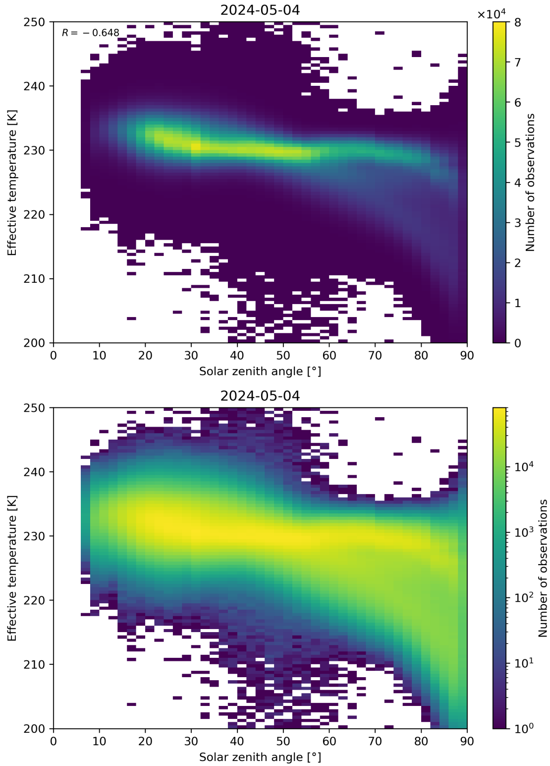
Figure 45: Scatter density plot of “Solar zenith angle” against “Effective temperature” for 2024-05-03 to 2024-05-05.
