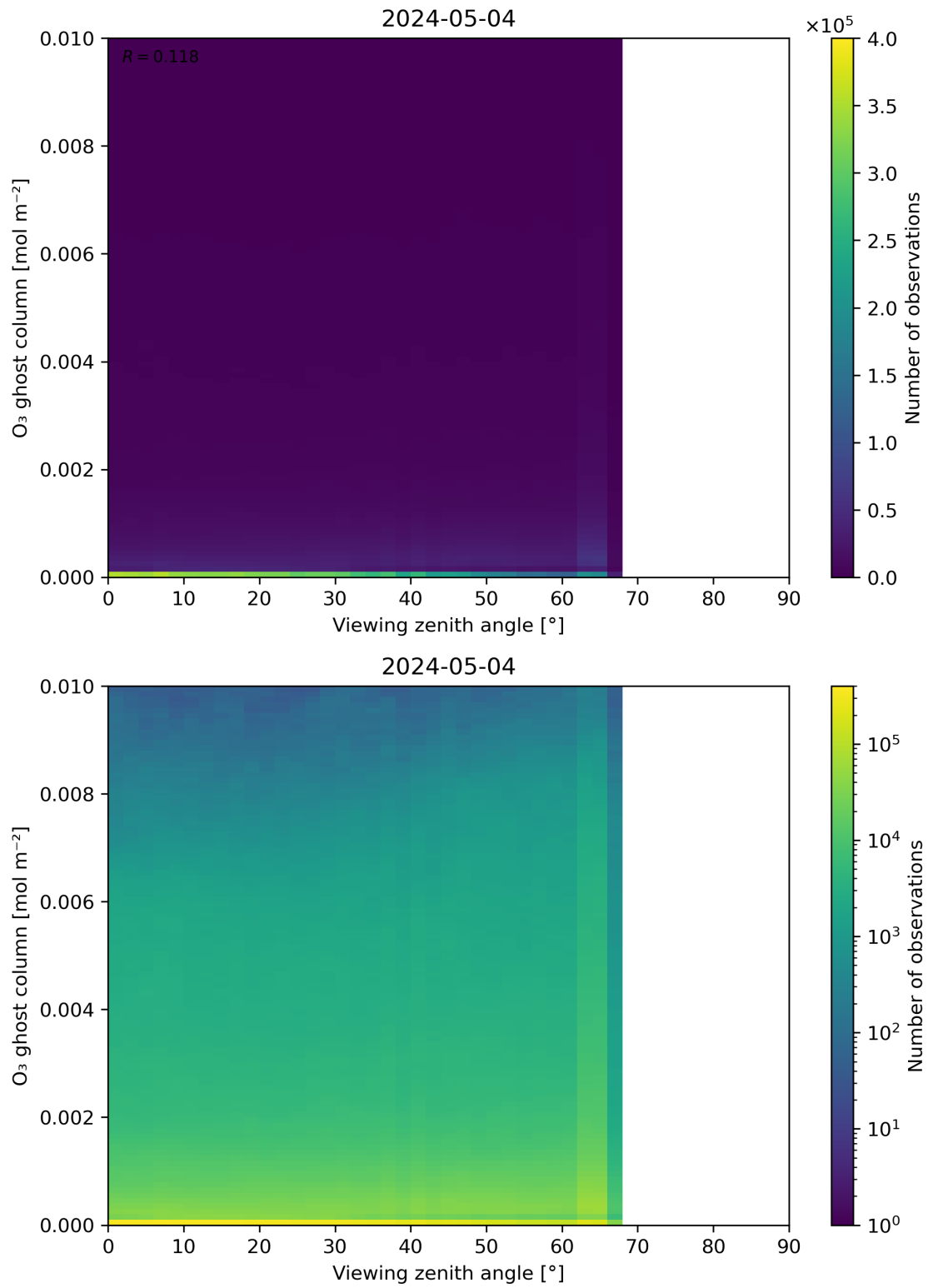
Figure 51: Scatter density plot of “Viewing zenith angle” against “O 3 ghost column” for 2024-05-03 to 2024-05-05.
