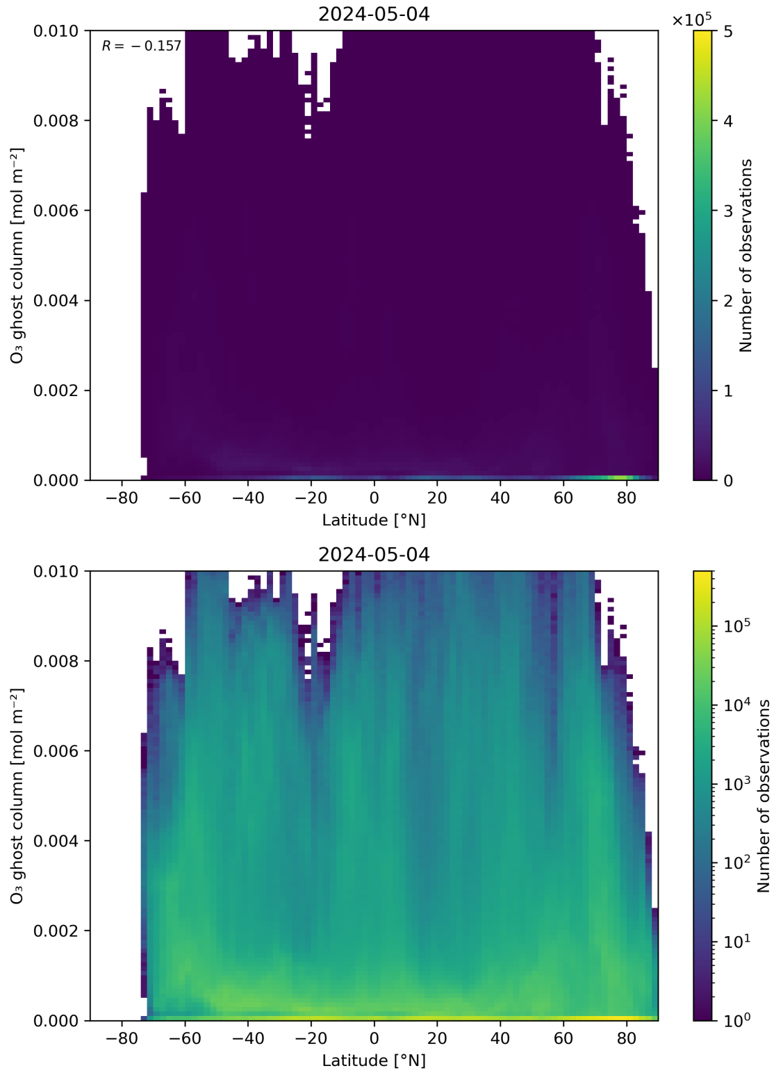
Figure 35: Scatter density plot of “Latitude” against “O 3 ghost column” for 2024-05-03 to 2024-05-05.
