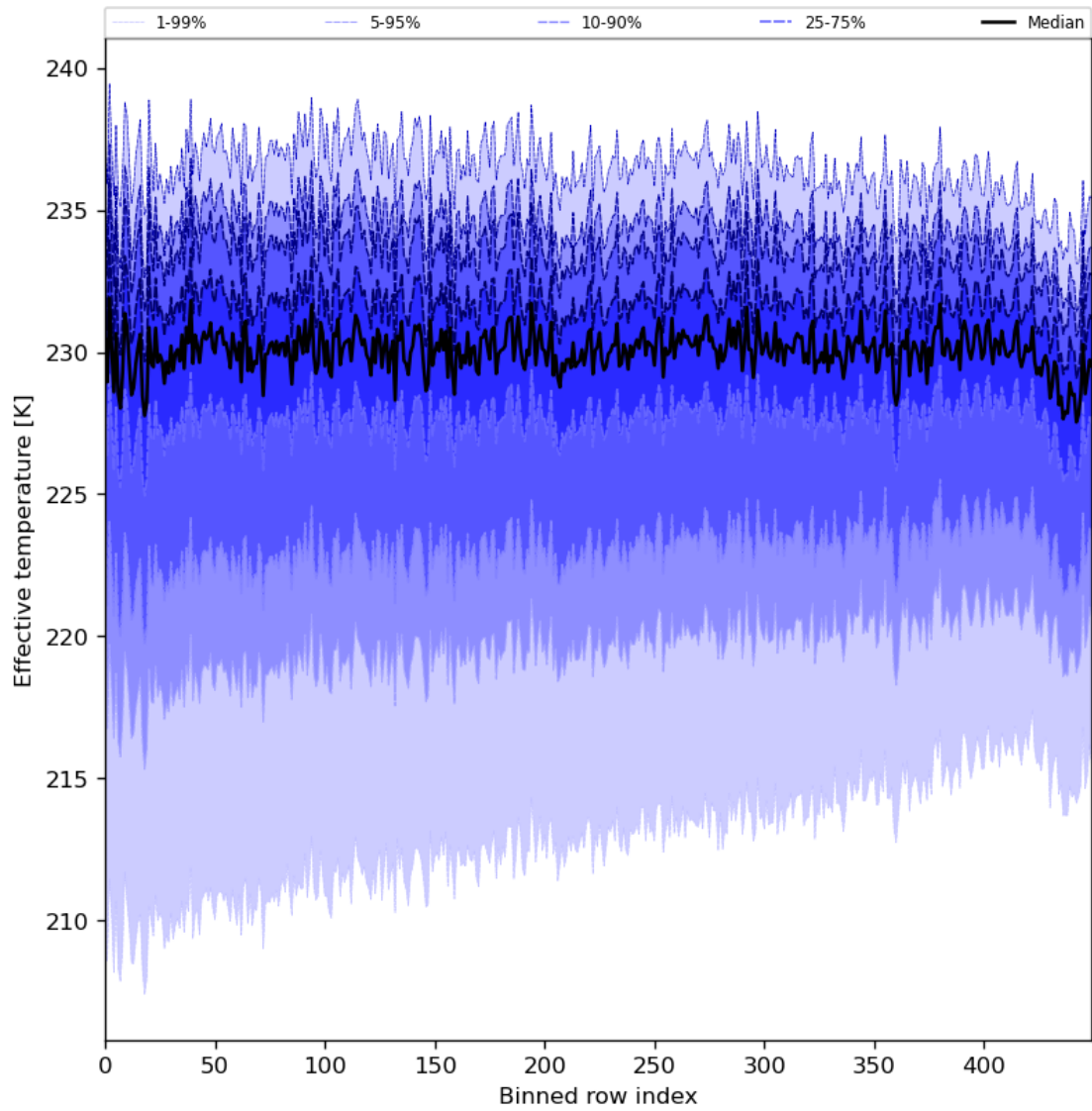
Figure 31: Along track statistics of “Effective temperature” for 2024-05-05 to 2024-05-07
