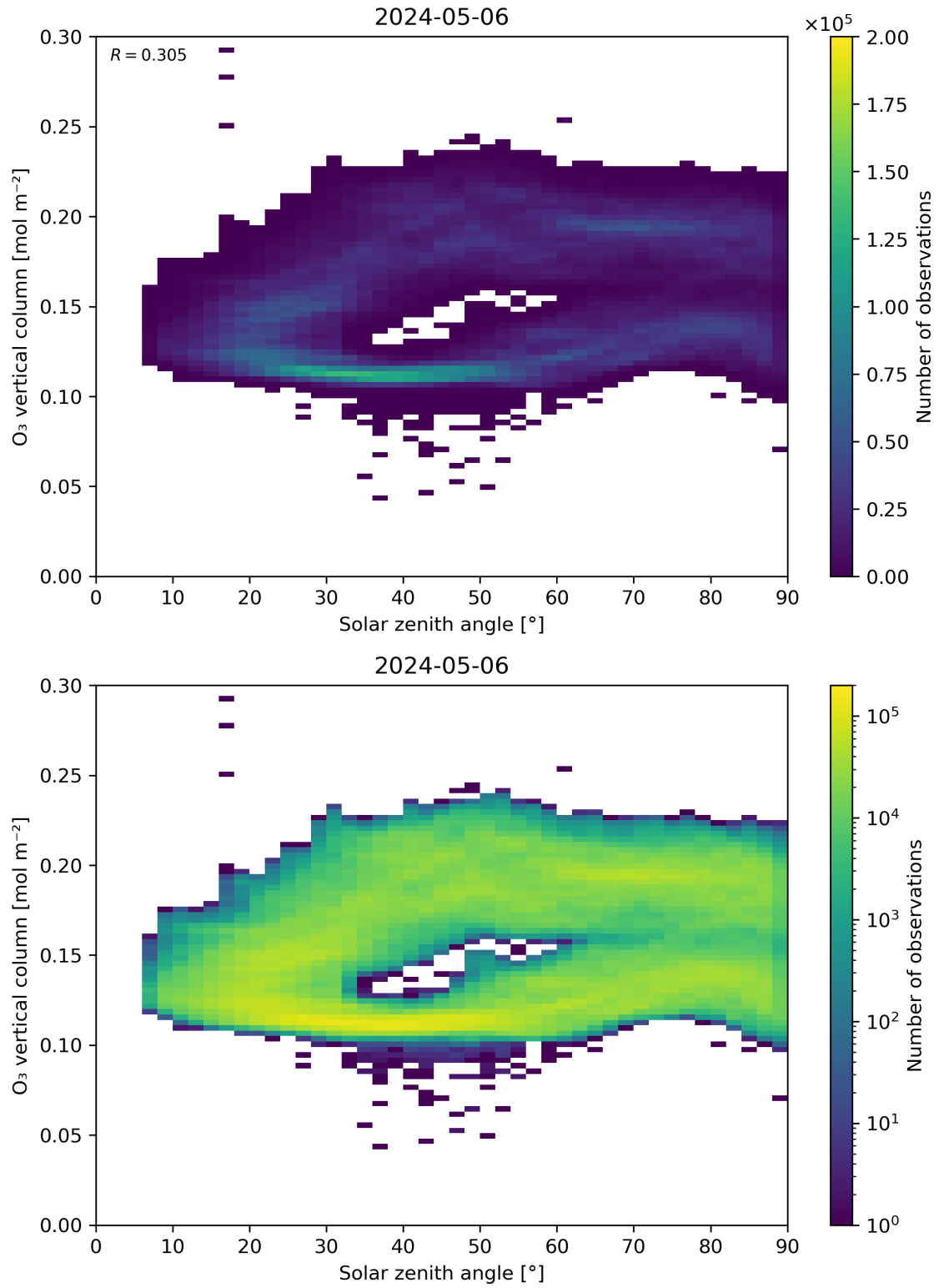
Figure 47: Scatter density plot of “Solar zenith angle” against “O 3 vertical column” for 2024-05-05 to 2024-05-07.
