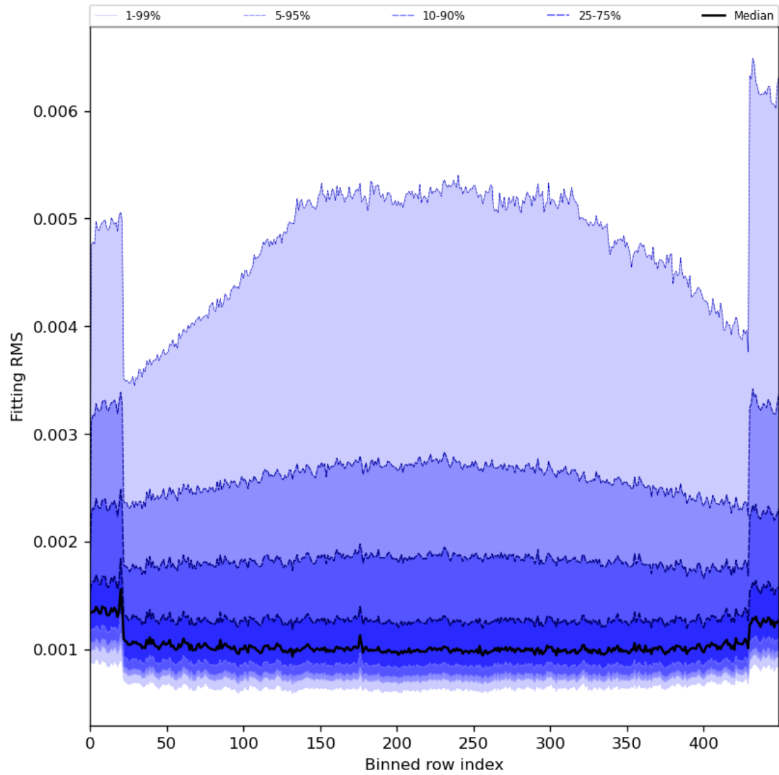
Figure 30: Along track statistics of “Fitting RMS” for 2024-05-05 to 2024-05-07
