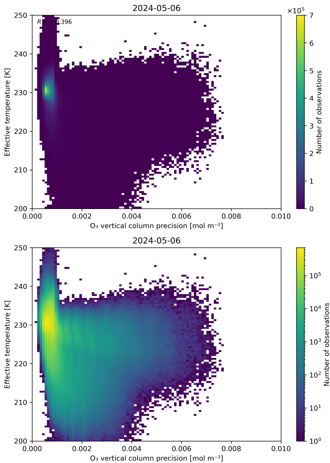
Figure 42: Scatter density plot of “O 3 vertical column precision” against “Effective temperature” for 2024-05-05 to 2024-05-07.
