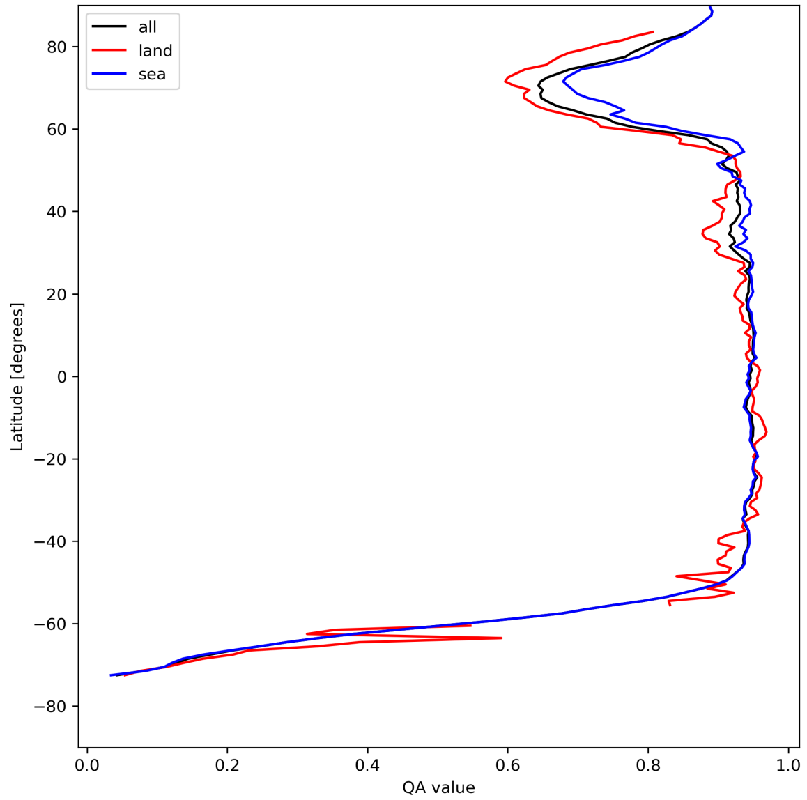
Figure 13: Zonal average of “QA value” for 2024-05-05 to 2024-05-07.
