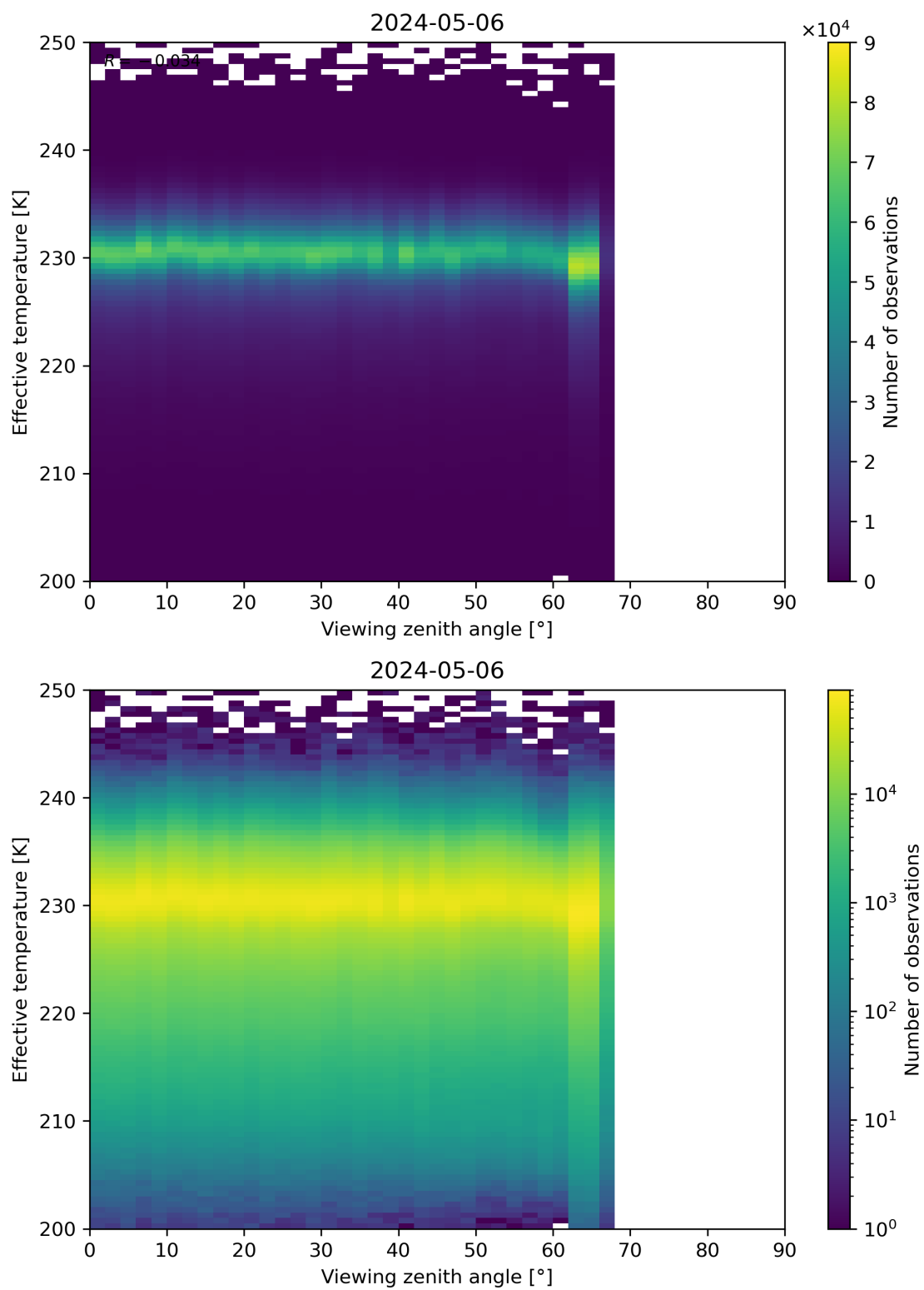
Figure 50: Scatter density plot of “Viewing zenith angle” against “Effective temperature” for 2024-05-05 to 2024-05-07.
