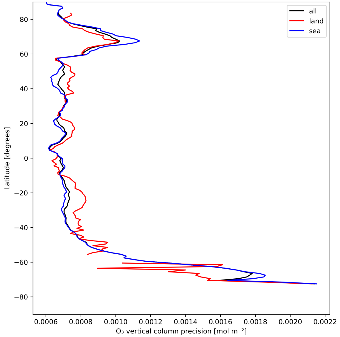
Figure 15: Zonal average of "O 3 vertical column precision" for 2024-05-05 to 2024-05-07.
