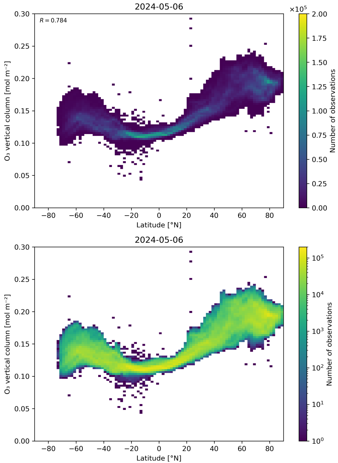
Figure 36: Scatter density plot of “Latitude” against “O 3 vertical column” for 2024-05-05 to 2024-05-07.
