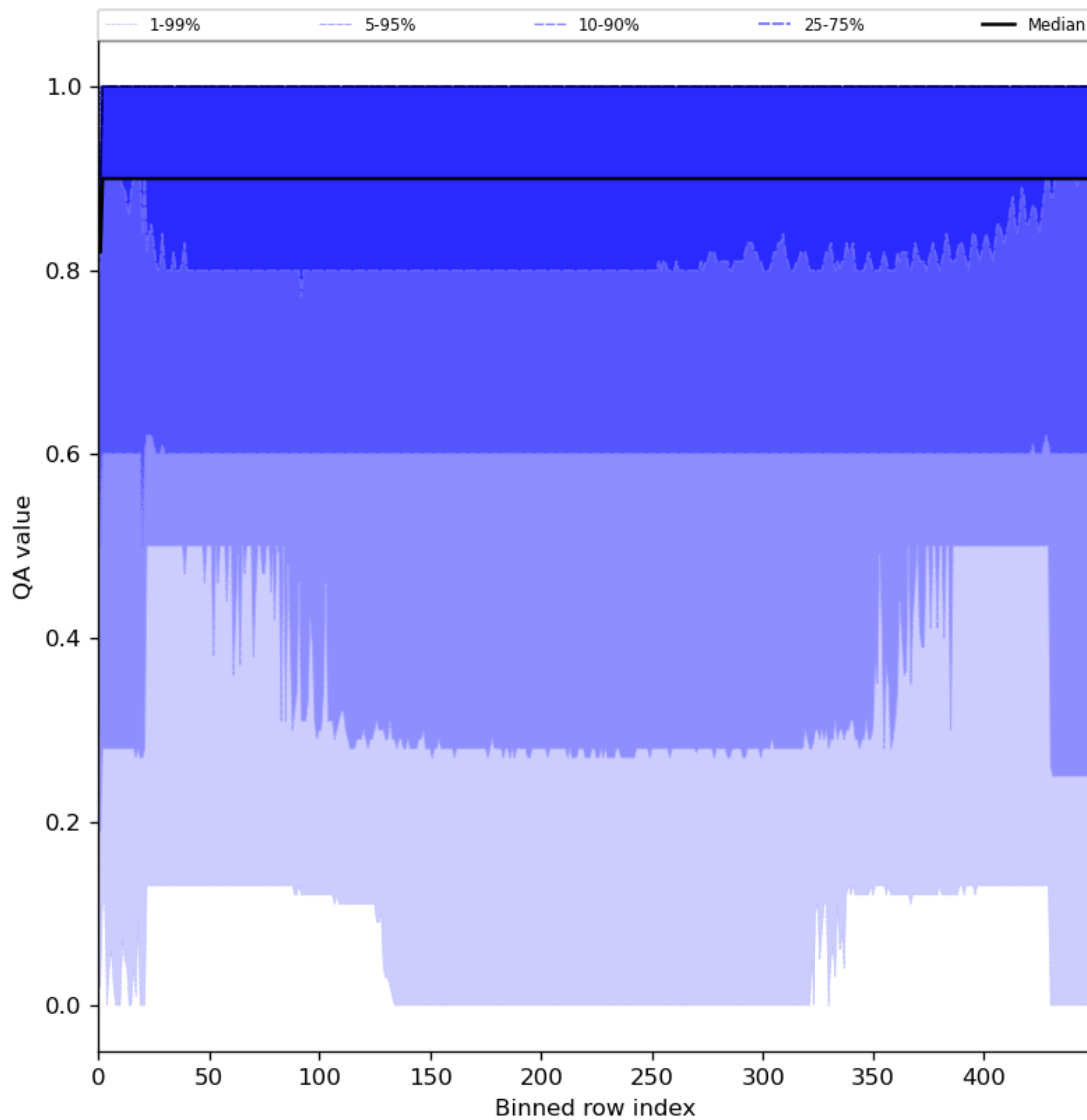
Figure 27: Along track statistics of “QA value” for 2024-05-05 to 2024-05-07
