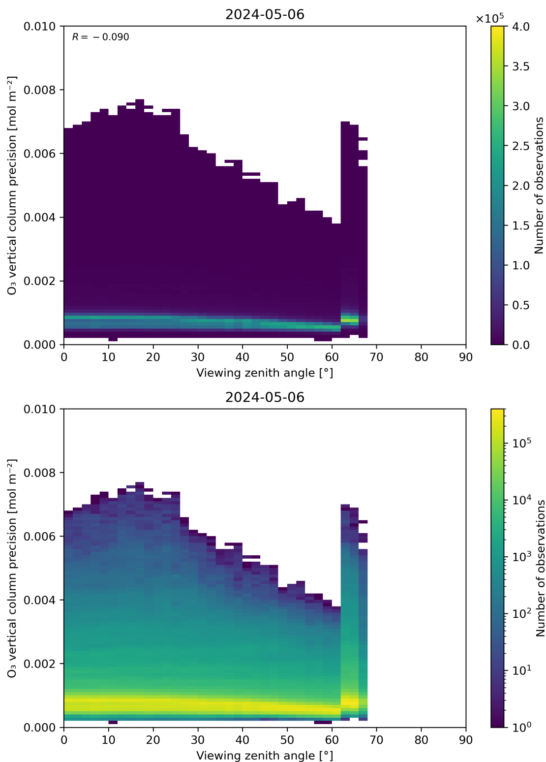
Figure 53: Scatter density plot of “Viewing zenith angle” against “O 3 vertical column precision” for 2024-05-05 to 2024-05-07.
