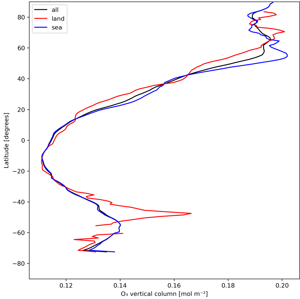
Figure 14: Zonal average of “O 3 vertical column” for 2024-05-05 to 2024-05-07.
