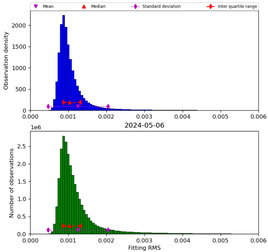
Figure 23: Histogram of “Fitting RMS” for 2024-05-05 to 2024-05-07
