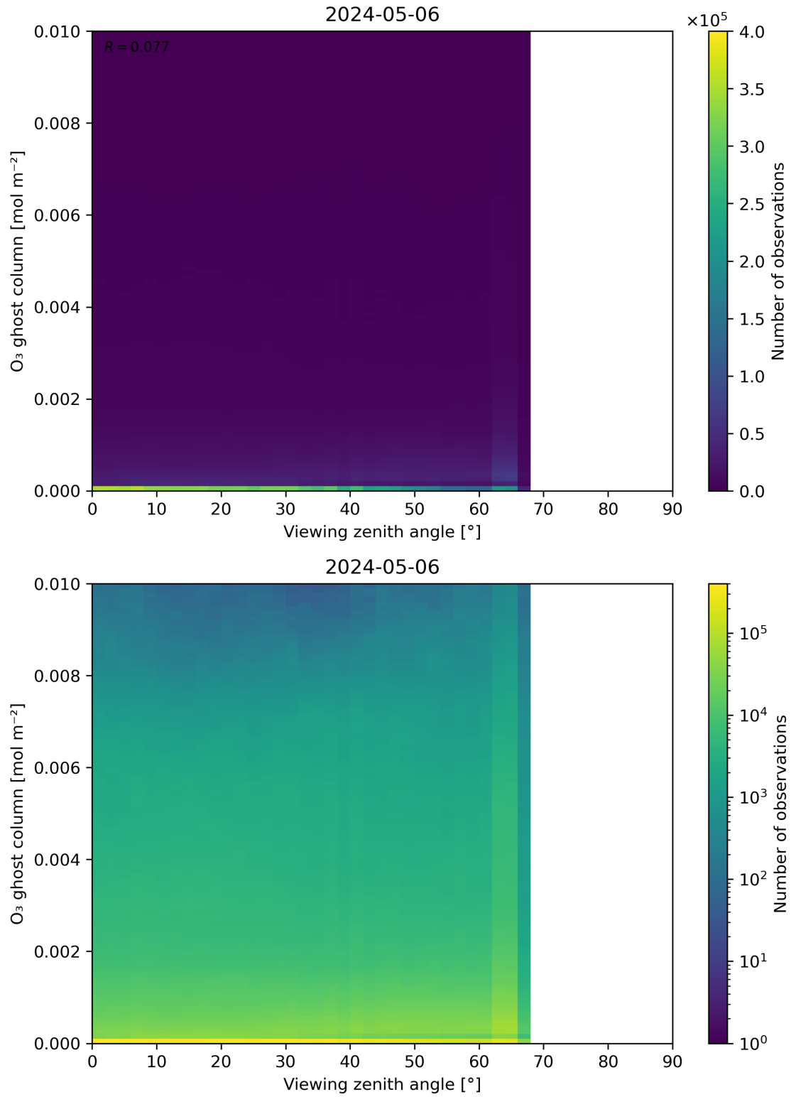
Figure 51: Scatter density plot of “Viewing zenith angle” against “O 3 ghost column” for 2024-05-05 to 2024-05-07.
