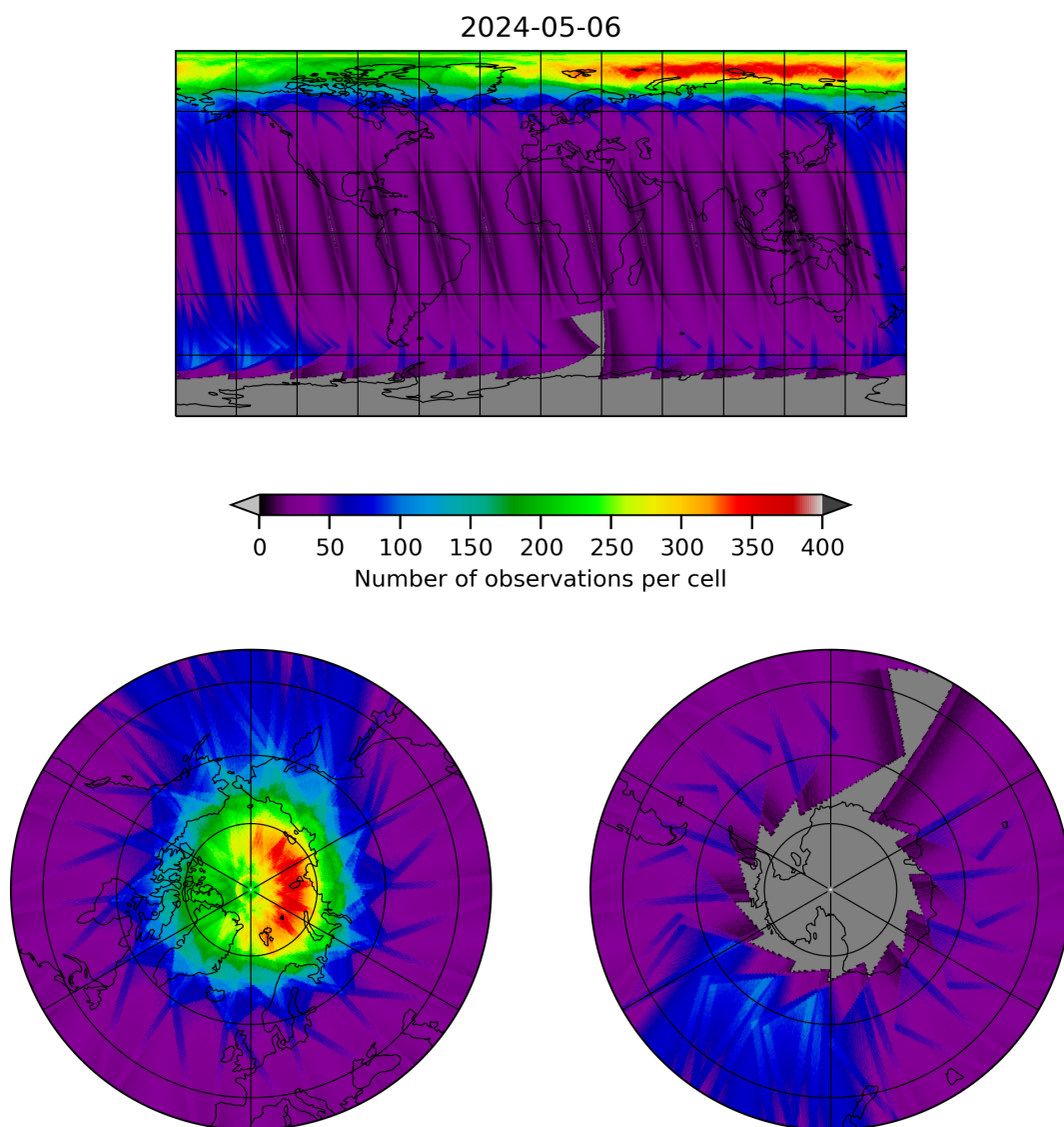
Figure 12: Map of the number of observations for 2024-05-05 to 2024-05-07
