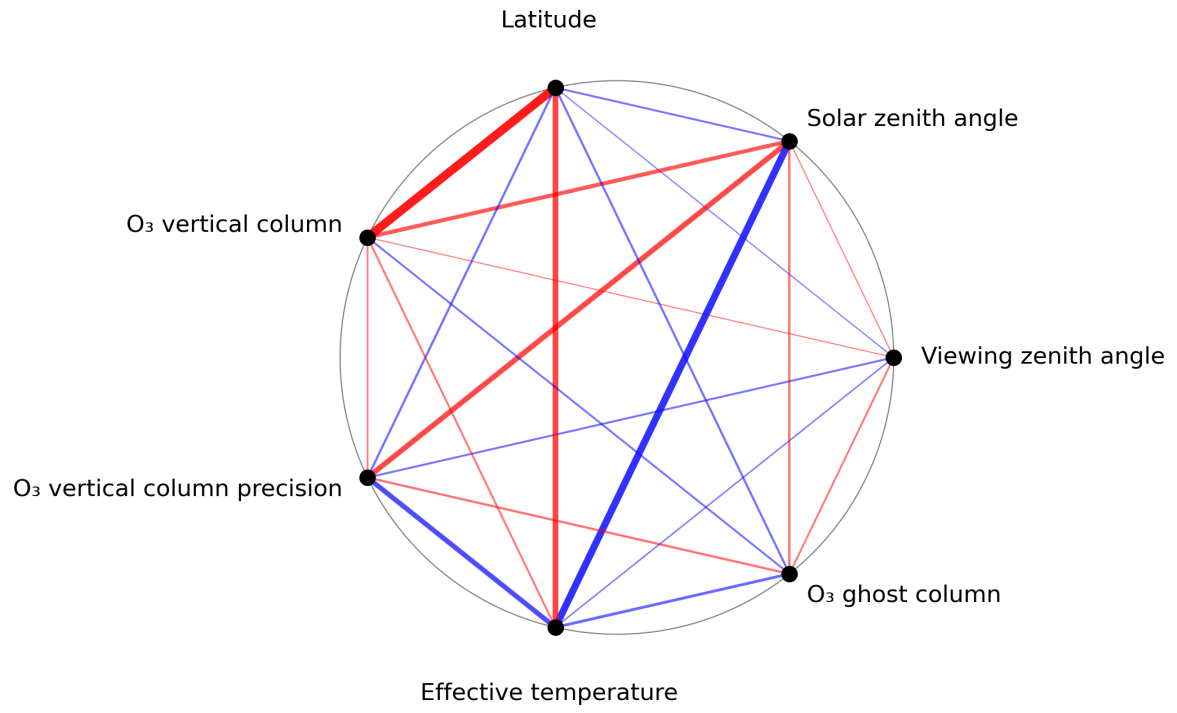
Figure 1: Map of correlation graph for 2024-05-05 to 2024-05-07.
