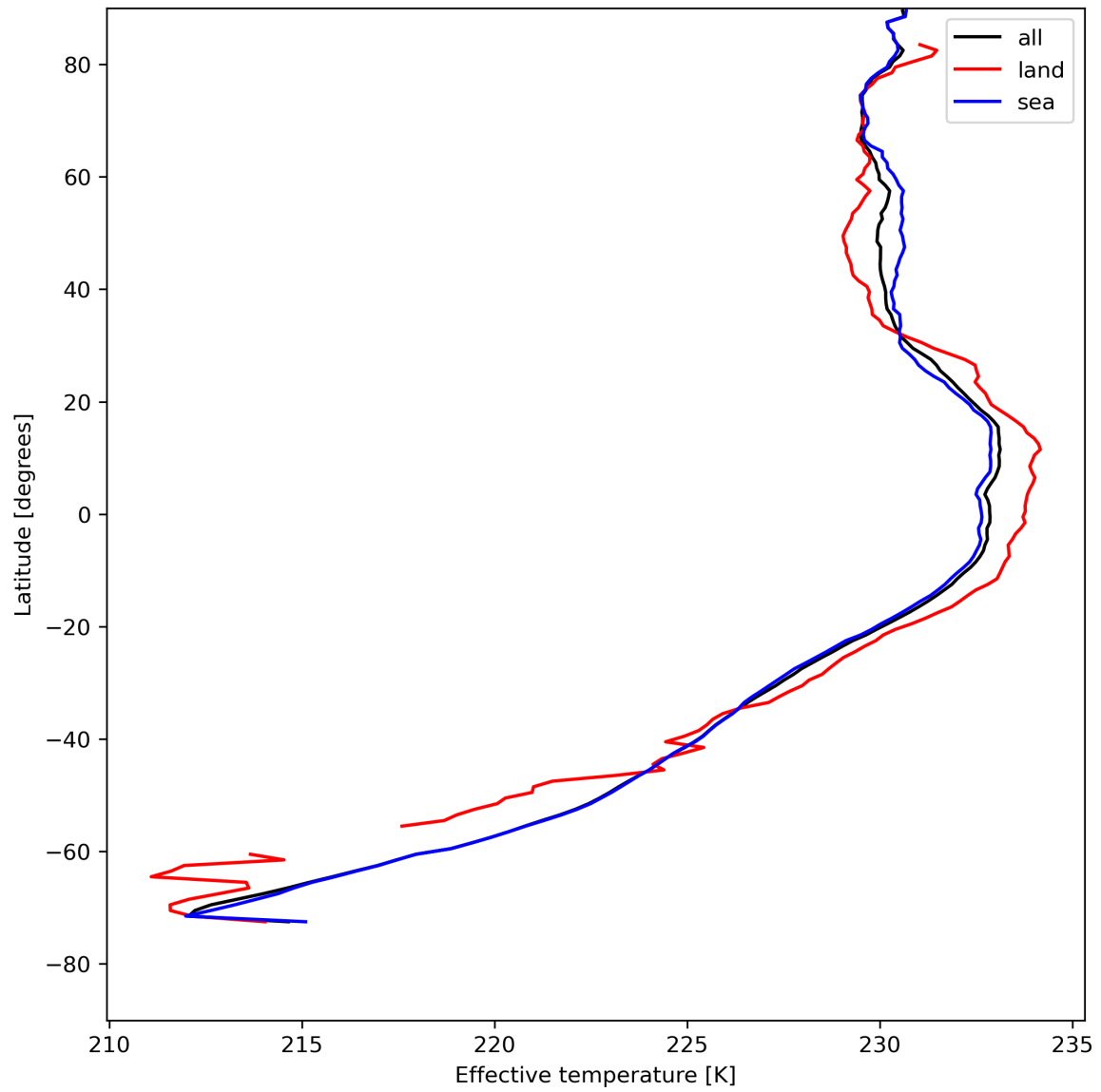
Figure 17: Zonal average of “Effective temperature” for 2024-05-05 to 2024-05-07.
