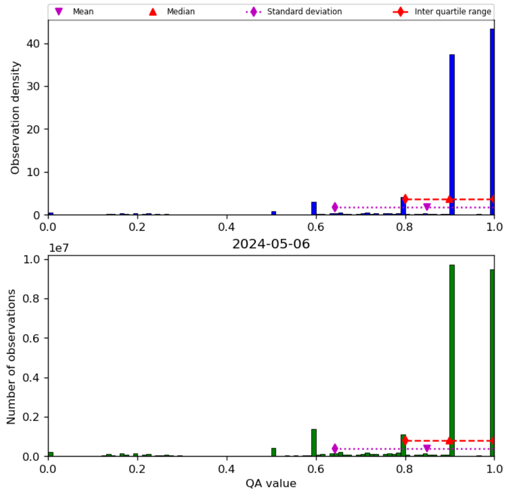
Figure 20: Histogram of “QA value” for 2024-05-05 to 2024-05-07
