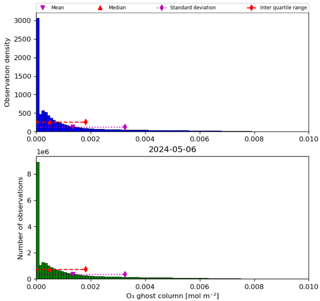
Figure 25: Histogram of “O 3 ghost column” for 2024-05-05 to 2024-05-07
