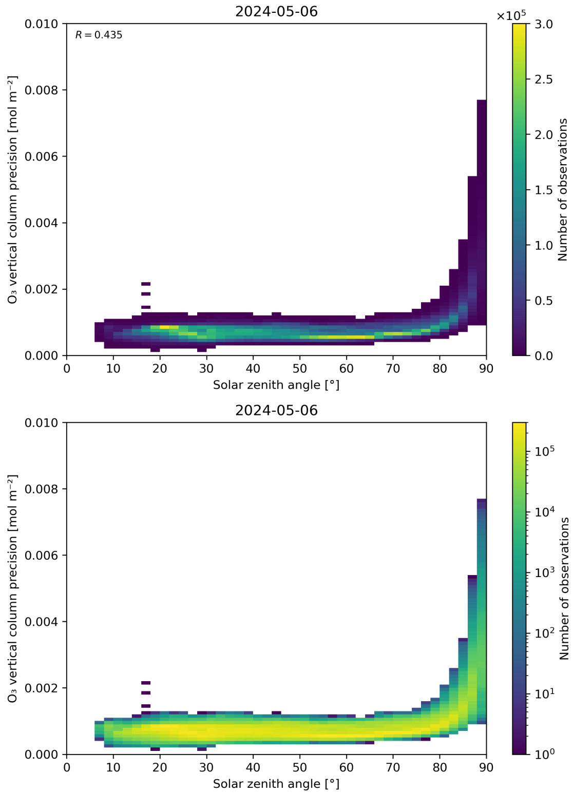
Figure 48: Scatter density plot of “Solar zenith angle” against “O 3 vertical column precision” for 2024-05-05 to 2024-05-07.
