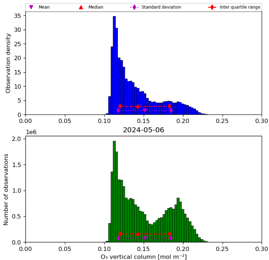
Figure 21: Histogram of “O 3 vertical column” for 2024-05-05 to 2024-05-07
