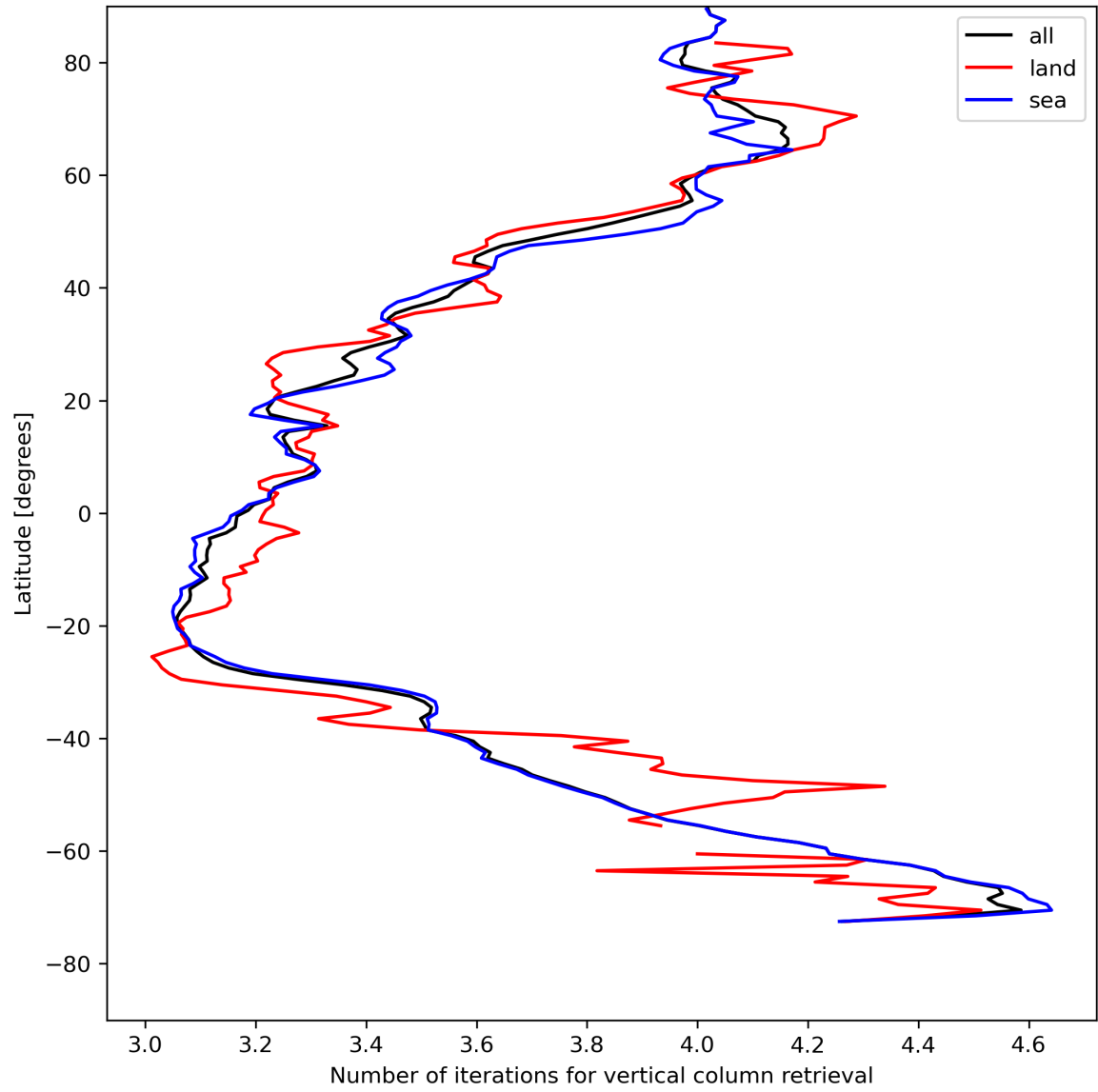
Figure 19: Zonal average of “Number of iterations for vertical column retrieval” for 2024-05-05 to 2024-05-07.
