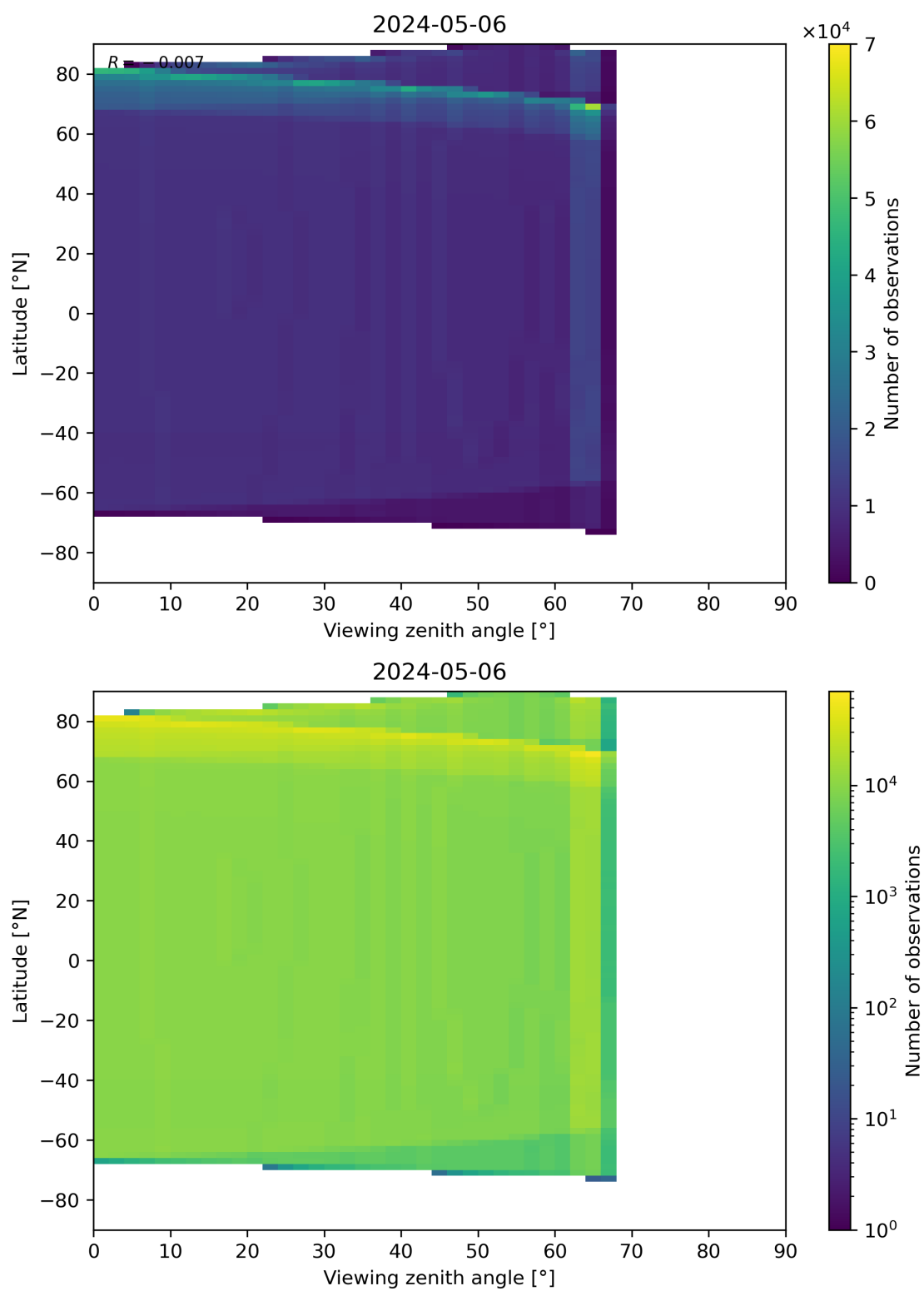
Figure 49: Scatter density plot of “Viewing zenith angle” against “Latitude” for 2024-05-05 to 2024-05-07.
