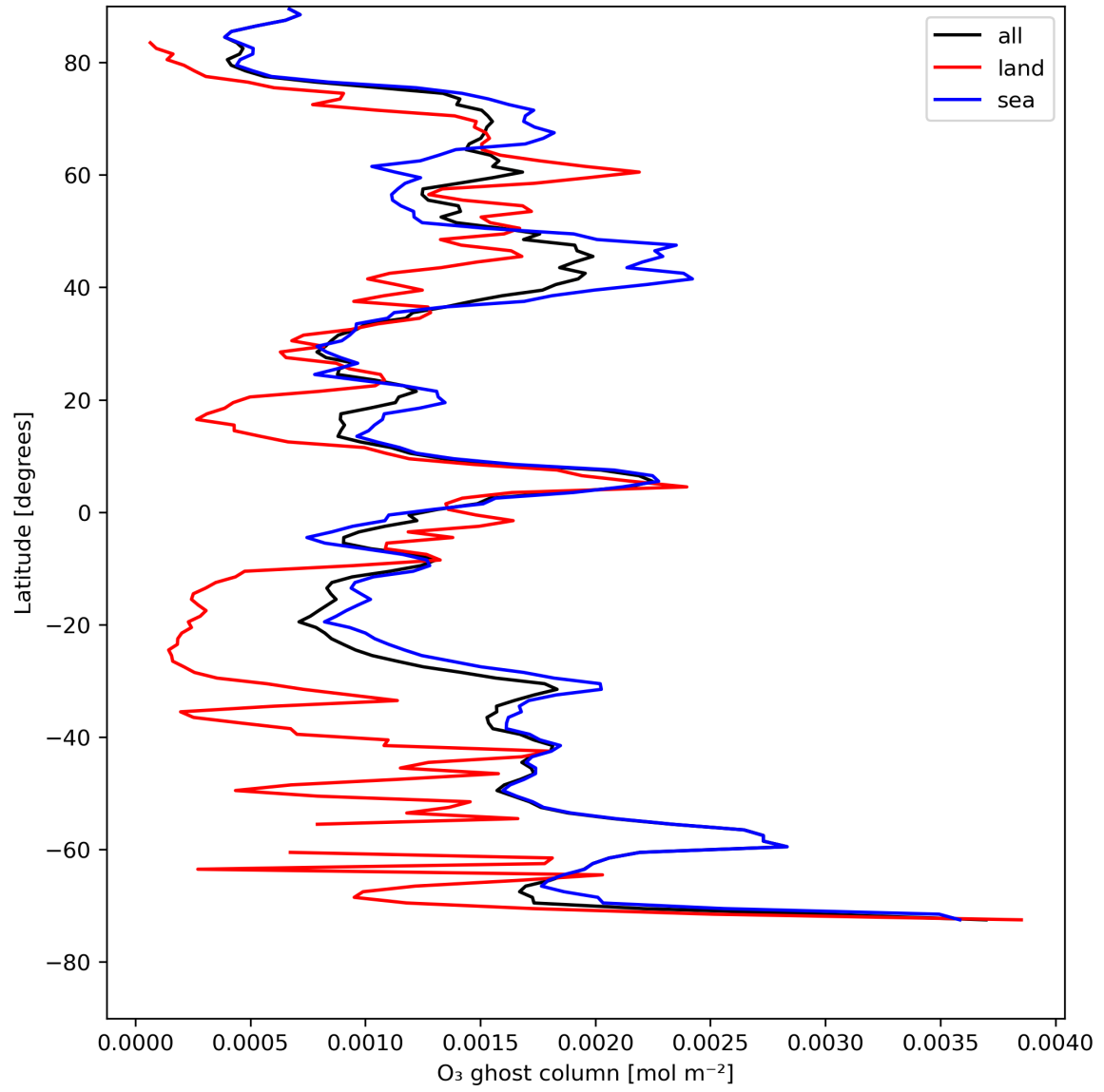
Figure 18: Zonal average of “O 3 ghost column” for 2024-05-05 to 2024-05-07.
