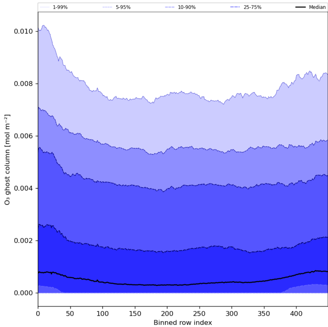
Figure 32: Along track statistics of “O 3 ghost column” for 2024-05-05 to 2024-05-07
