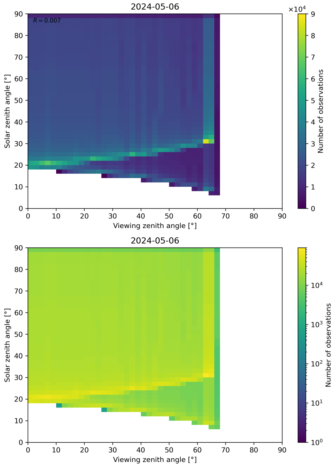
Figure 54: Scatter density plot of “Viewing zenith angle” against “Solar zenith angle” for 2024-05-05 to 2024-05-07.
