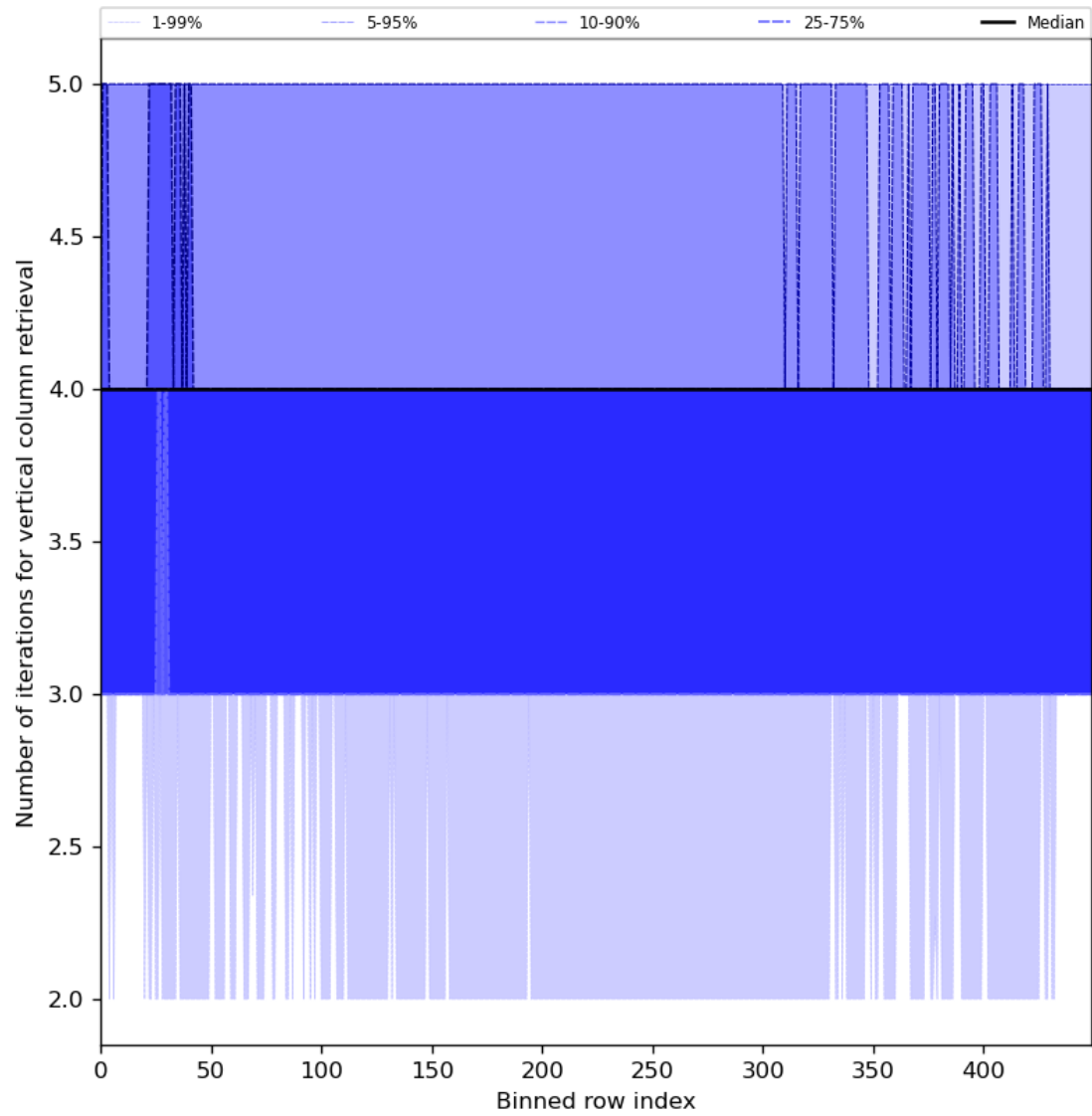
Figure 33: Along track statistics of “Number of iterations for vertical column retrieval” for 2024-05-05 to 2024-05-07
