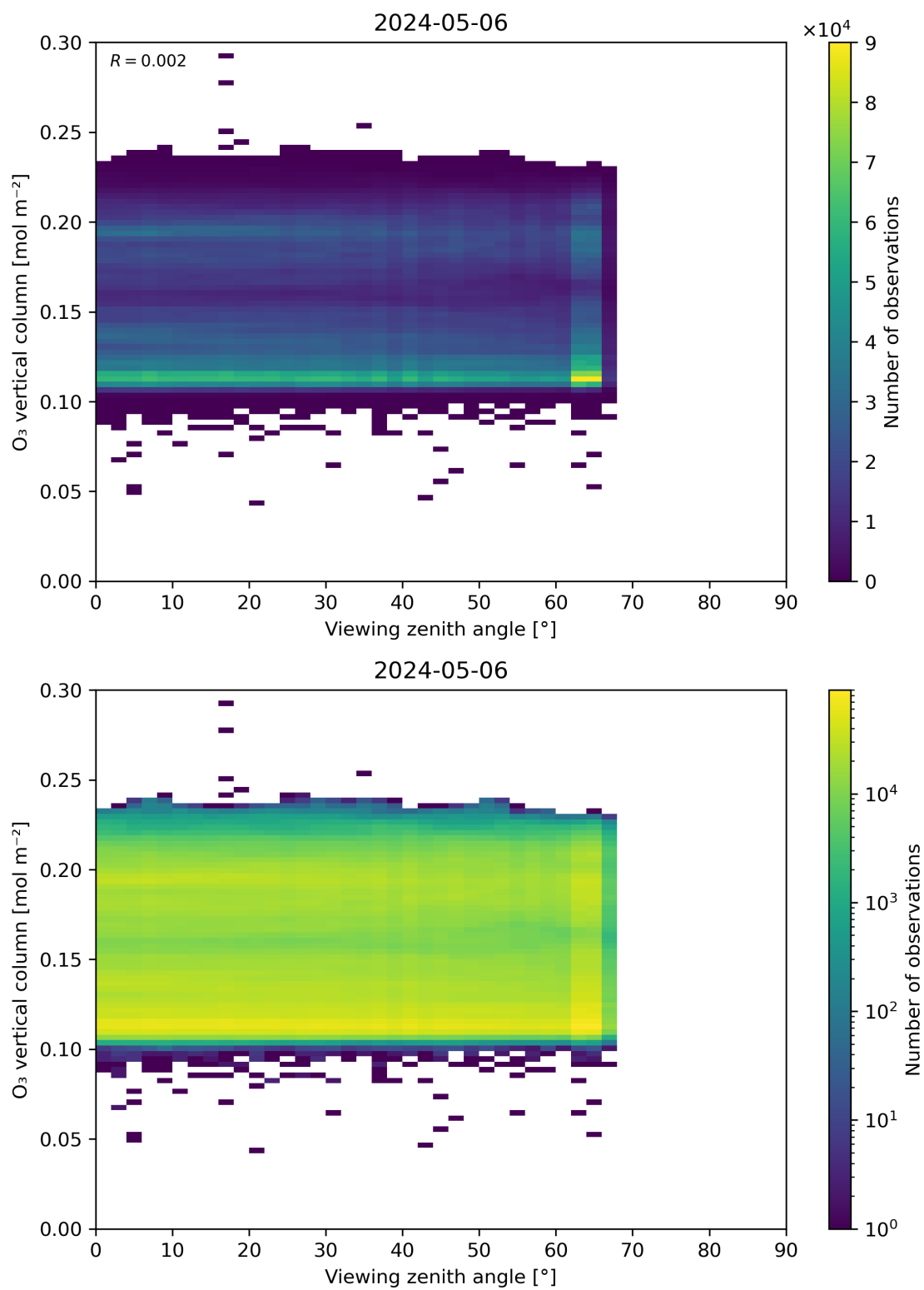
Figure 52: Scatter density plot of “Viewing zenith angle” against “O 3 vertical column” for 2024-05-05 to 2024-05-07.
