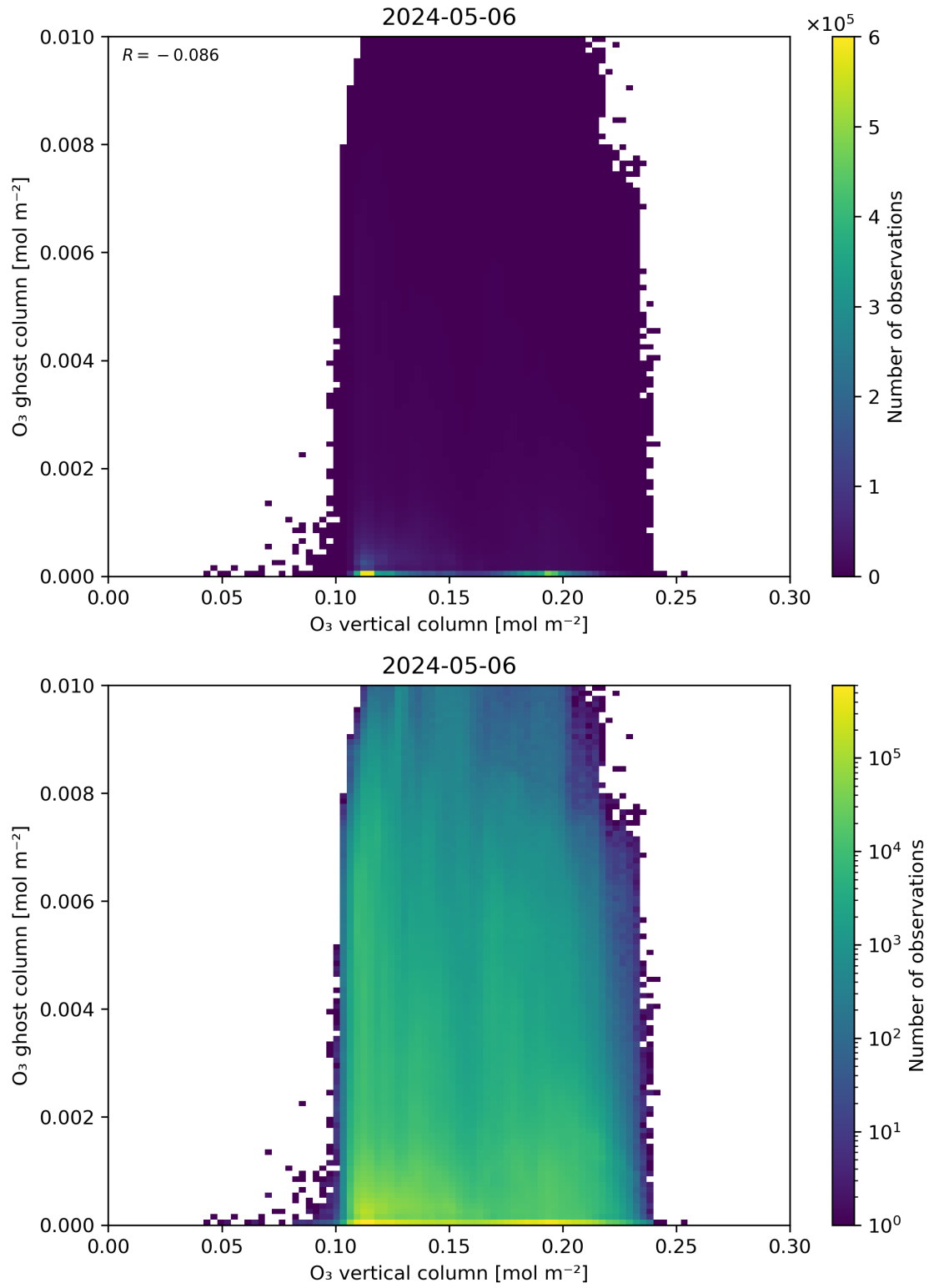
Figure 40: Scatter density plot of “O 3 vertical column” against “O 3 ghost column” for 2024-05-05 to 2024-05-07.
