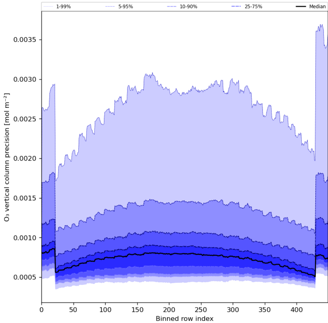
Figure 29: Along track statistics of “O 3 vertical column precision” for 2024-05-05 to 2024-05-07
