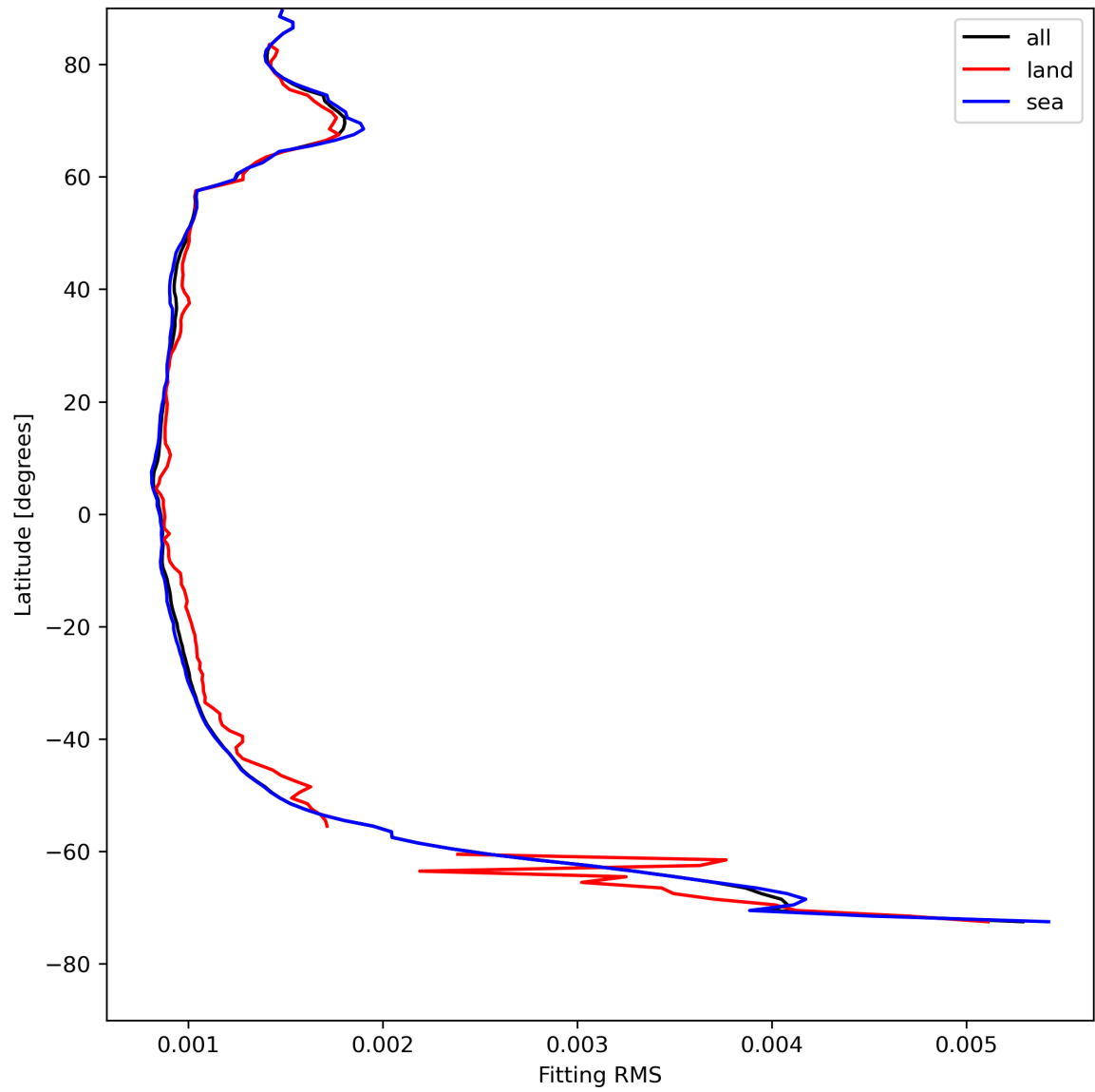
Figure 16: Zonal average of “Fitting RMS” for 2024-05-05 to 2024-05-07.
