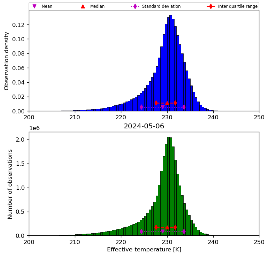
Figure 24: Histogram of “Effective temperature” for 2024-05-05 to 2024-05-07
