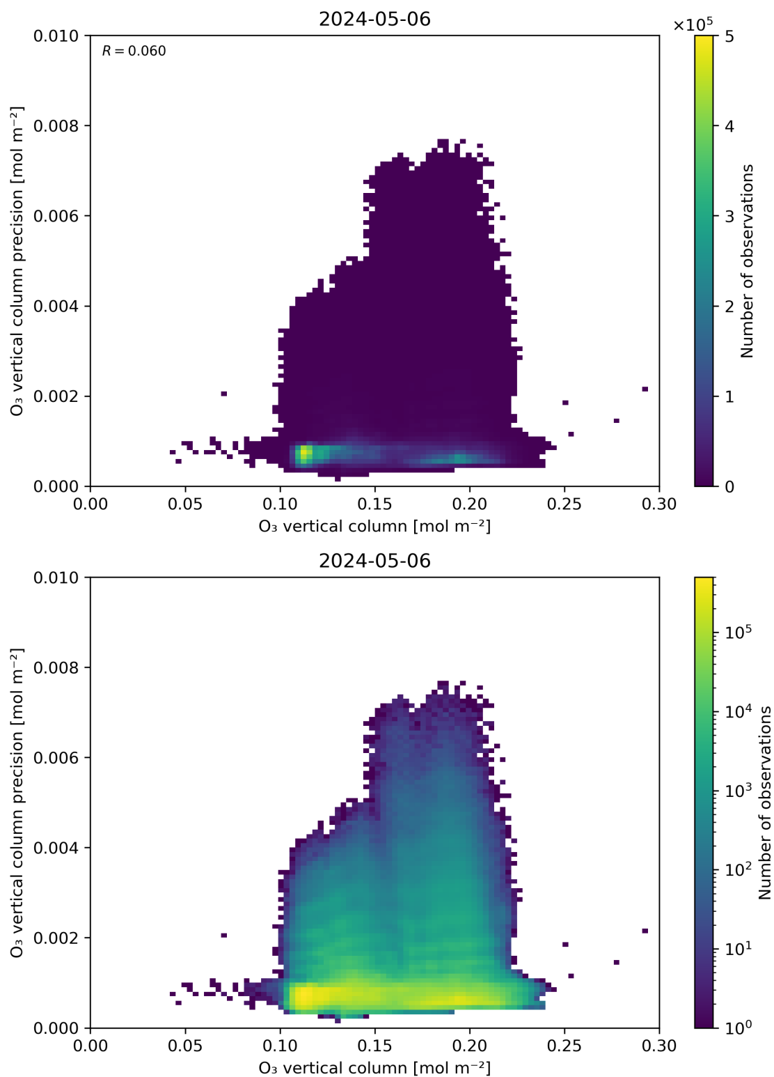
Figure 41: Scatter density plot of “O 3 vertical column” against “O 3 vertical column precision” for 2024-05-05 to 2024-05-07.
