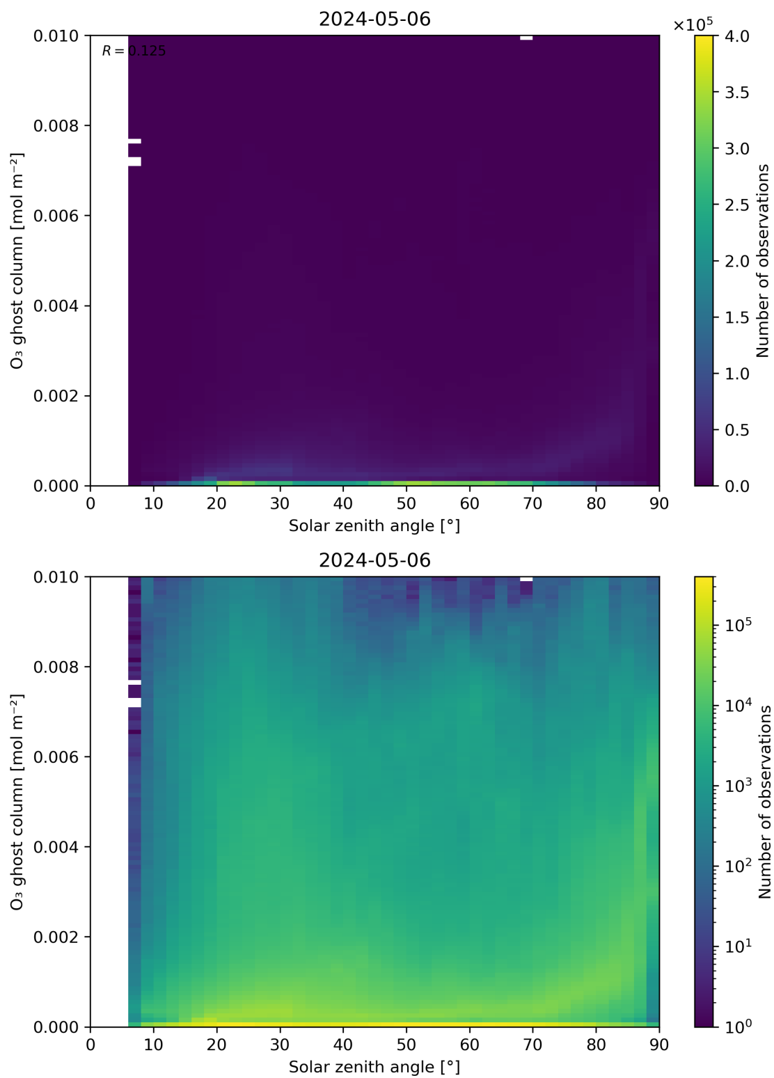
Figure 46: Scatter density plot of “Solar zenith angle” against “O 3 ghost column” for 2024-05-05 to 2024-05-07.
