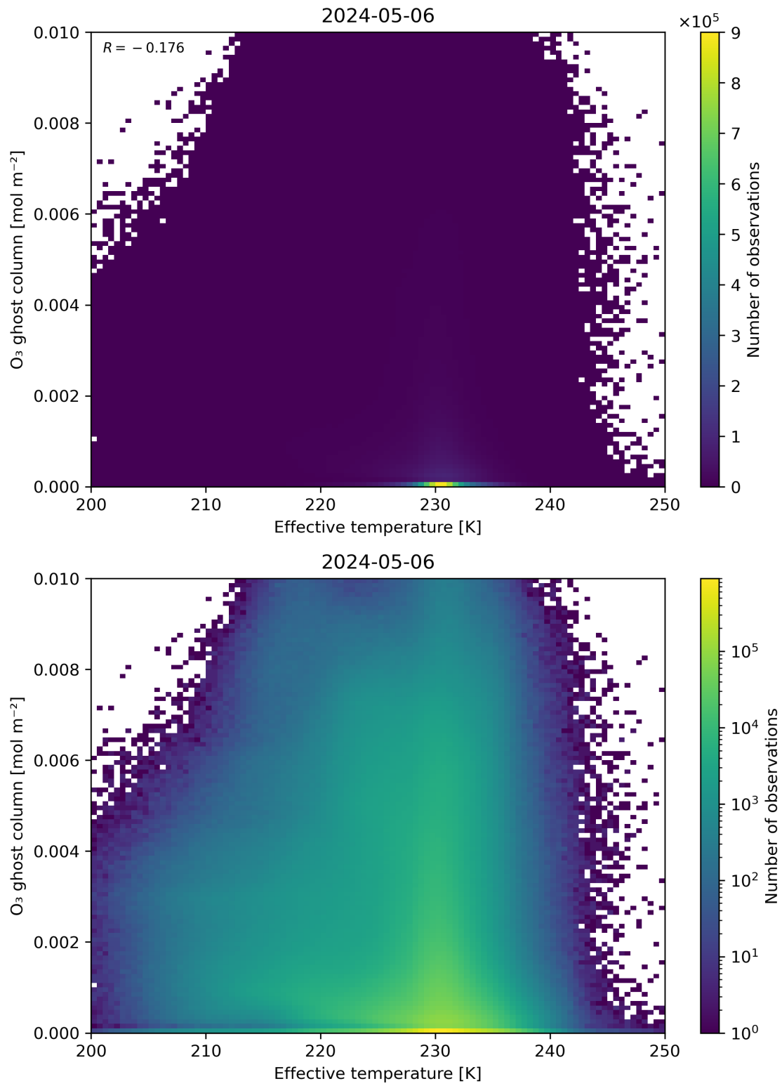
Figure 38: Scatter density plot of “Effective temperature” against “O 3 ghost column” for 2024-05-05 to 2024-05-07.
