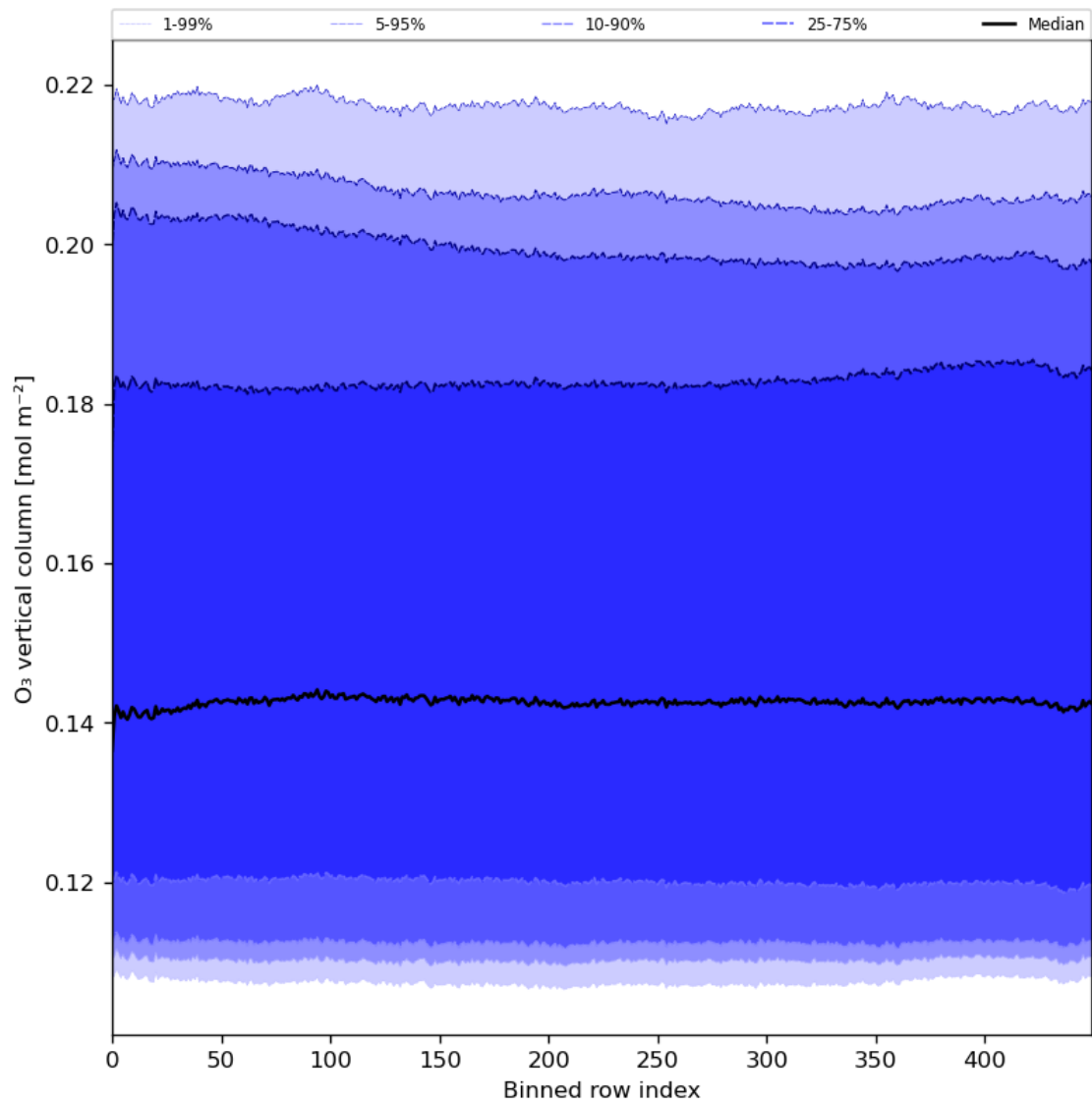
Figure 28: Along track statistics of “O 3 vertical column” for 2024-05-05 to 2024-05-07
