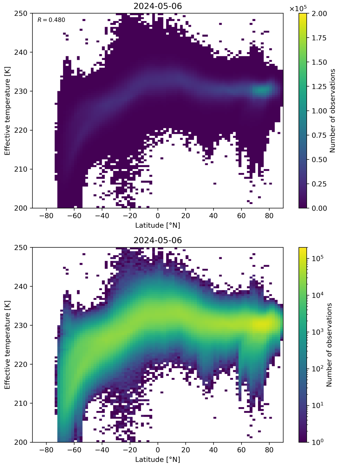
Figure 34: Scatter density plot of “Latitude” against “Effective temperature” for 2024-05-05 to 2024-05-07.
