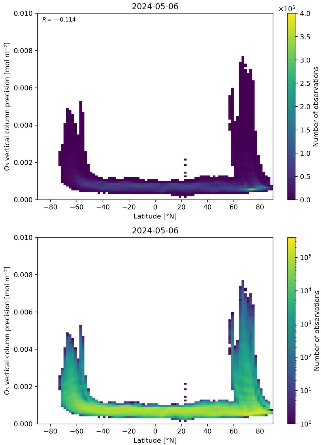
Figure 37: Scatter density plot of “Latitude” against “O 3 vertical column precision” for 2024-05-05 to 2024-05-07.
