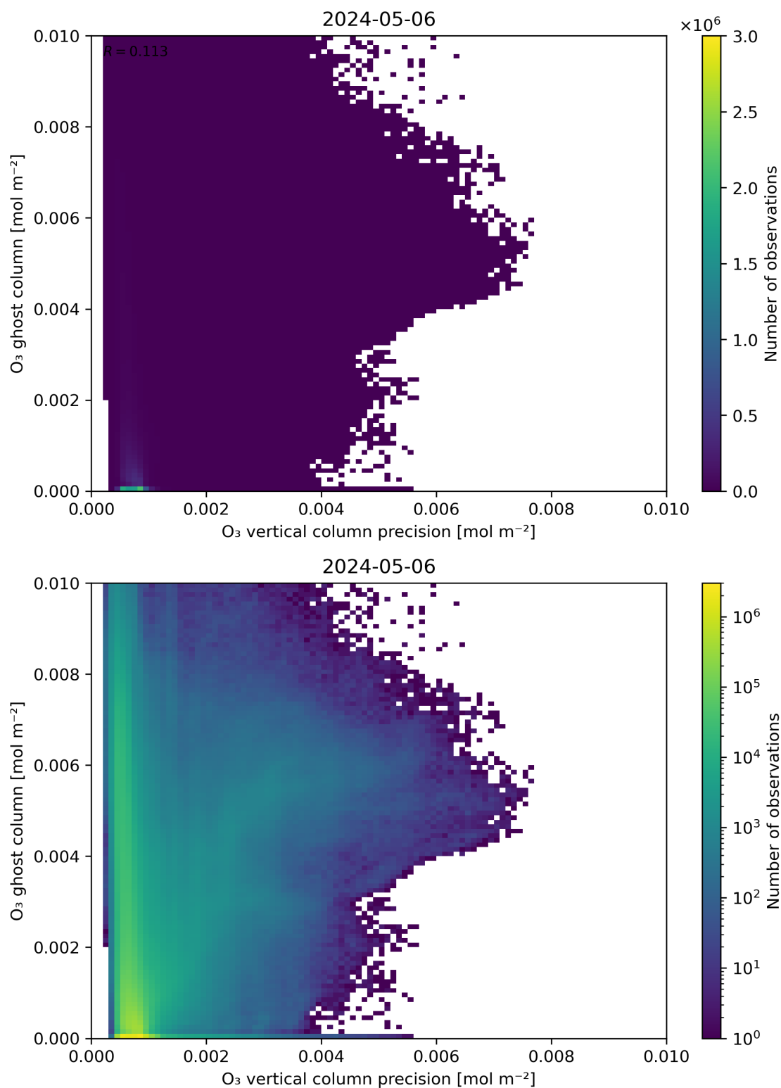
Figure 43: Scatter density plot of “O 3 vertical column precision” against “O 3 ghost column” for 2024-05-05 to 2024-05-07.
