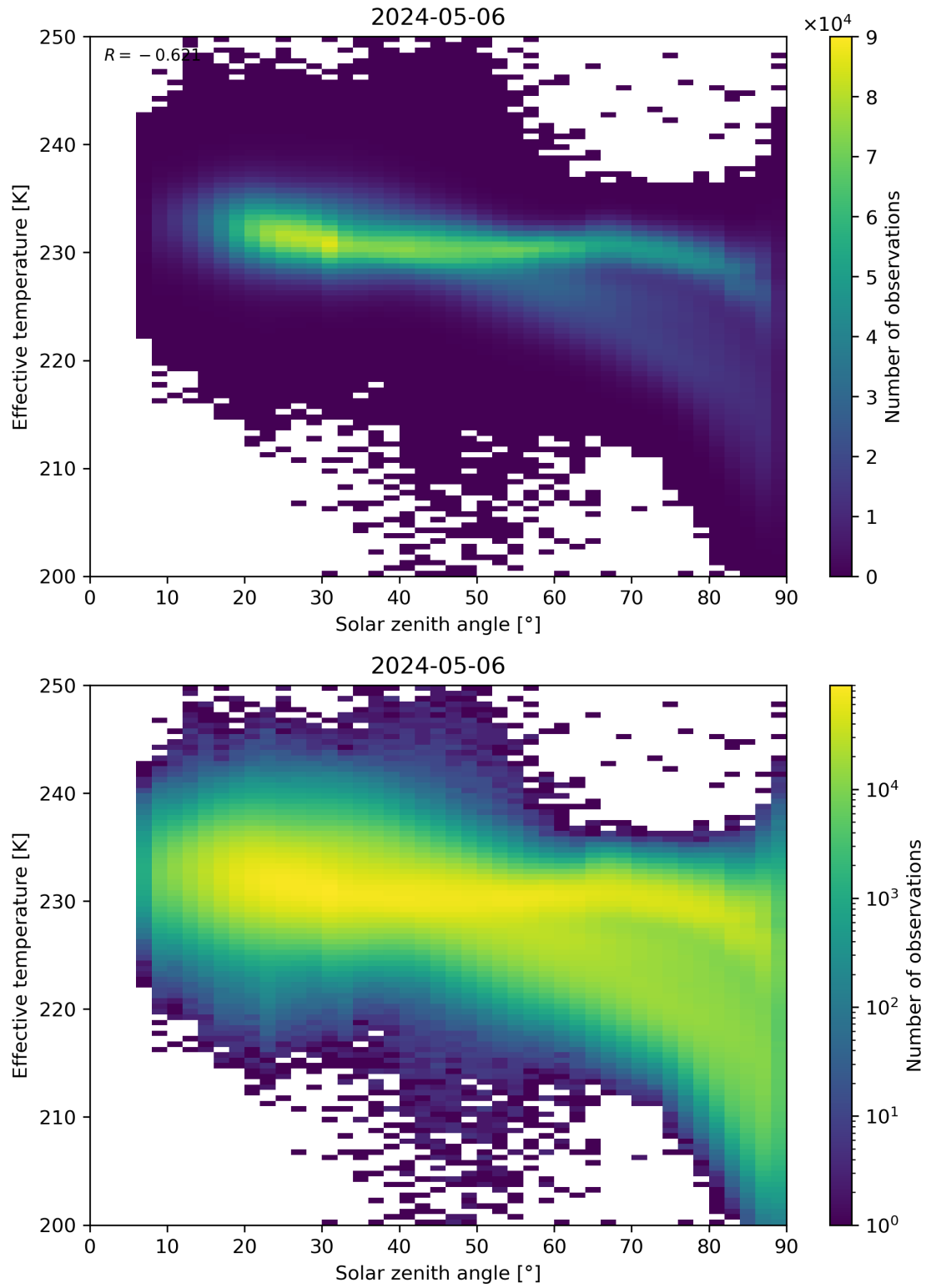
Figure 45: Scatter density plot of “Solar zenith angle” against “Effective temperature” for 2024-05-05 to 2024-05-07.
