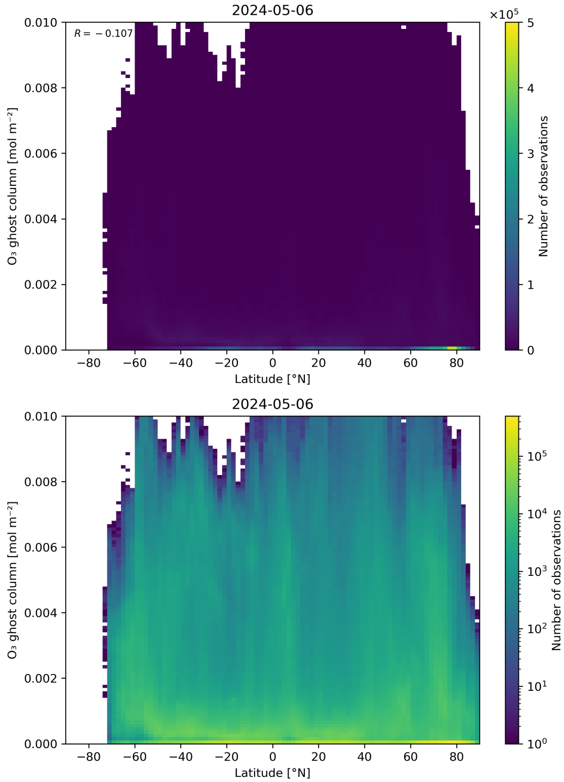
Figure 35: Scatter density plot of “Latitude” against “O 3 ghost column” for 2024-05-05 to 2024-05-07.
