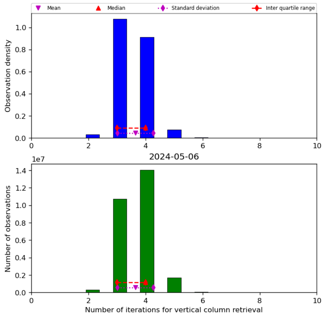
Figure 26: Histogram of “Number of iterations for vertical column retrieval” for 2024-05-05 to 2024-05-07
