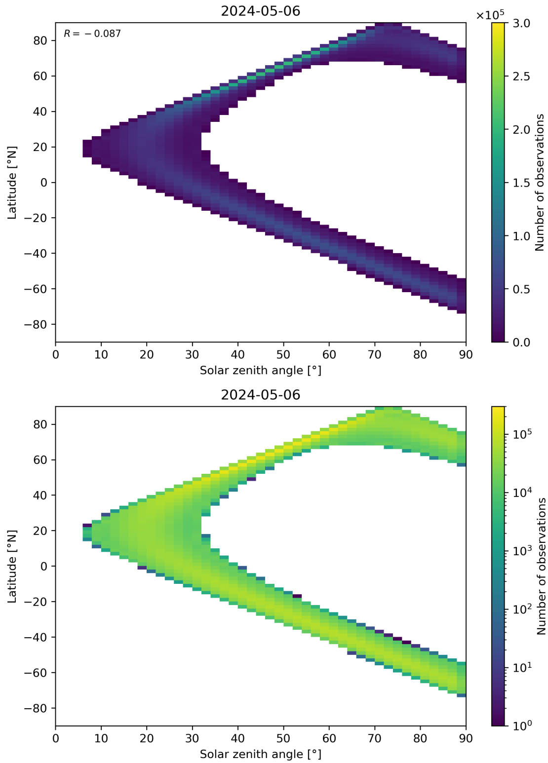
Figure 44: Scatter density plot of “Solar zenith angle” against “Latitude” for 2024-05-05 to 2024-05-07.
