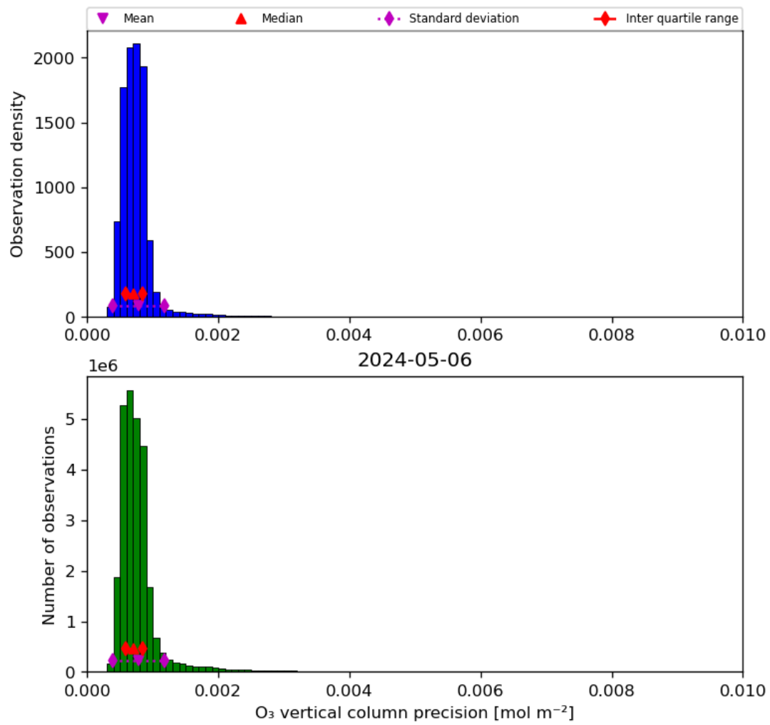
Figure 22: Histogram of “O 3 vertical column precision” for 2024-05-05 to 2024-05-07
