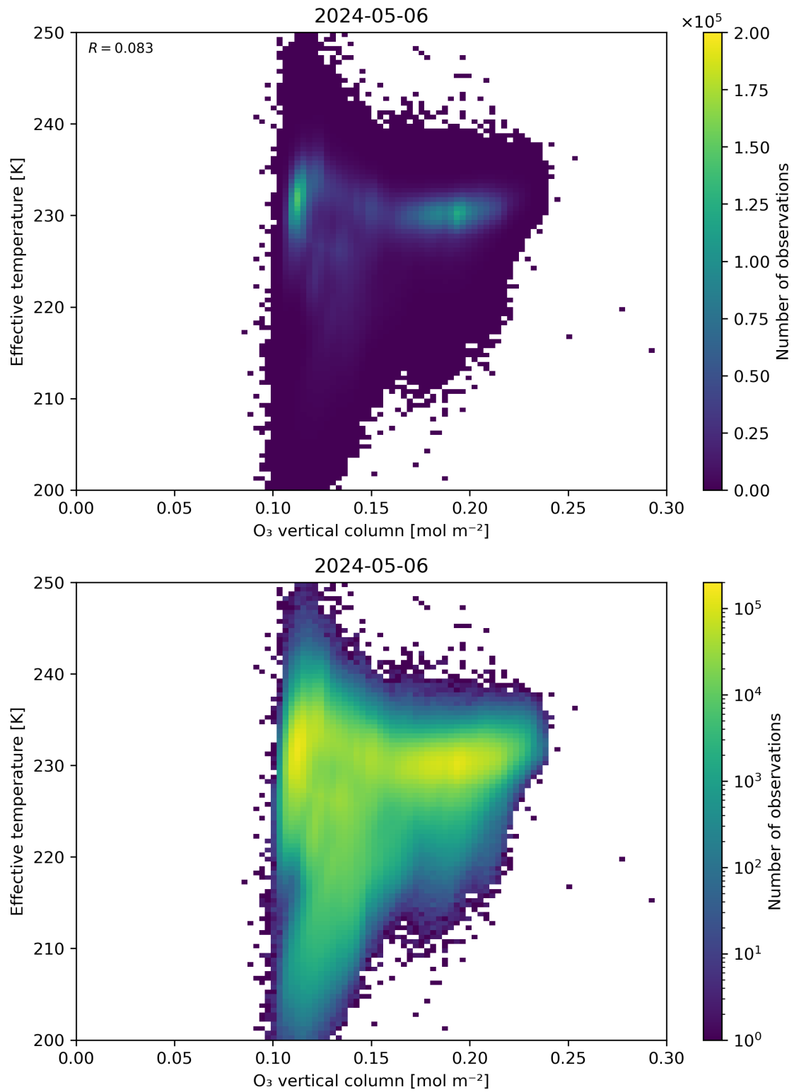
Figure 39: Scatter density plot of “O 3 vertical column” against “Effective temperature” for 2024-05-05 to 2024-05-07.
