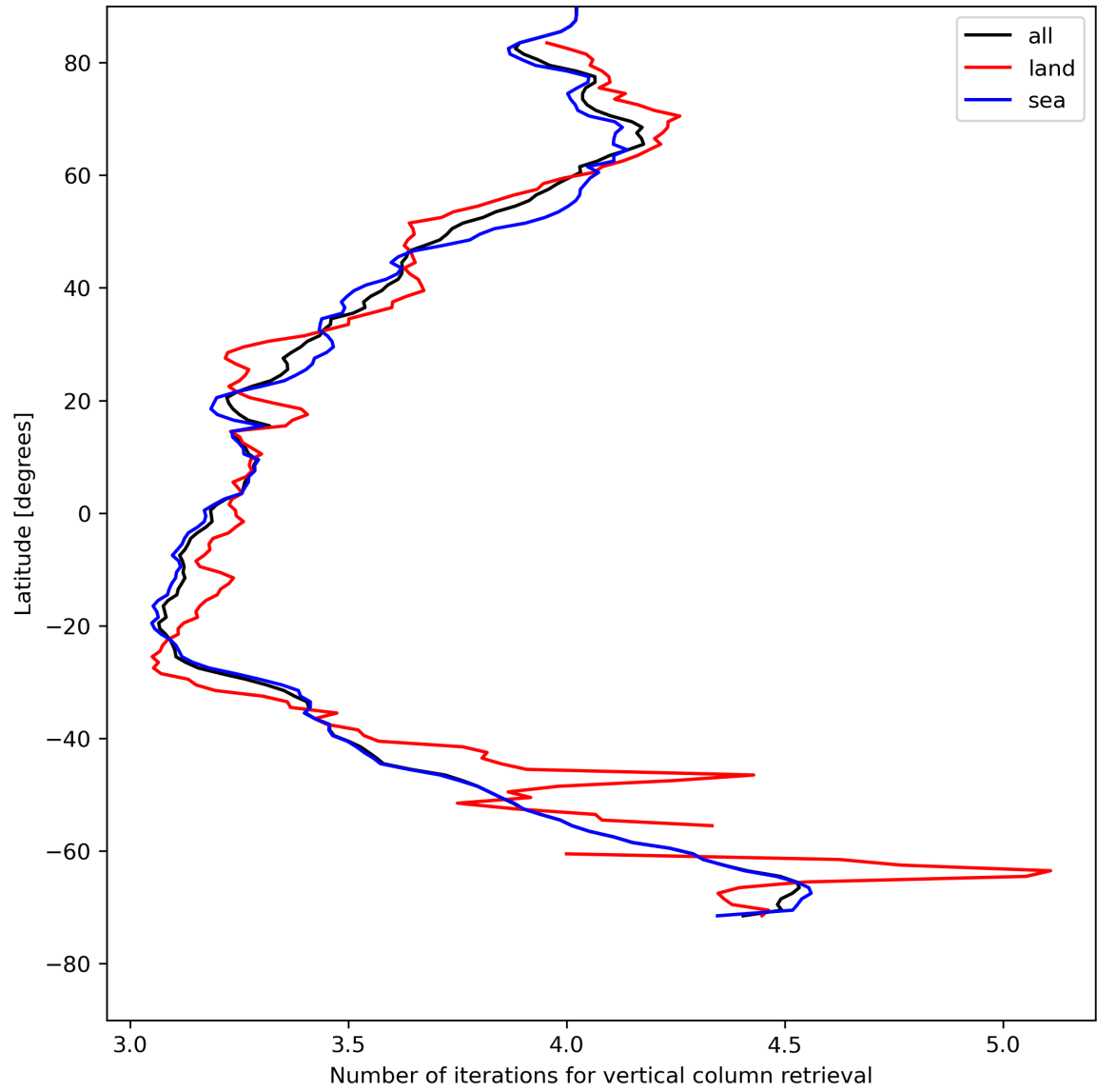
Figure 19: Zonal average of “Number of iterations for vertical column retrieval” for 2024-05-07 to 2024-05-08.
