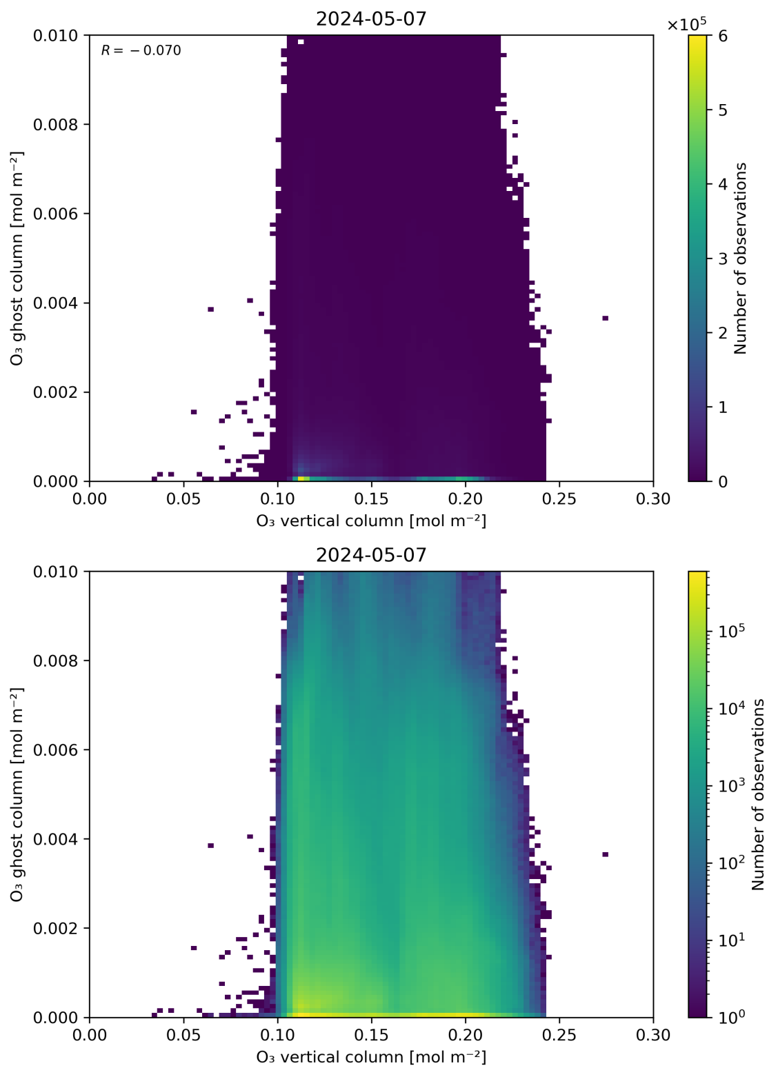
Figure 40: Scatter density plot of “O 3 vertical column” against “O 3 ghost column” for 2024-05-07 to 2024-05-08.
