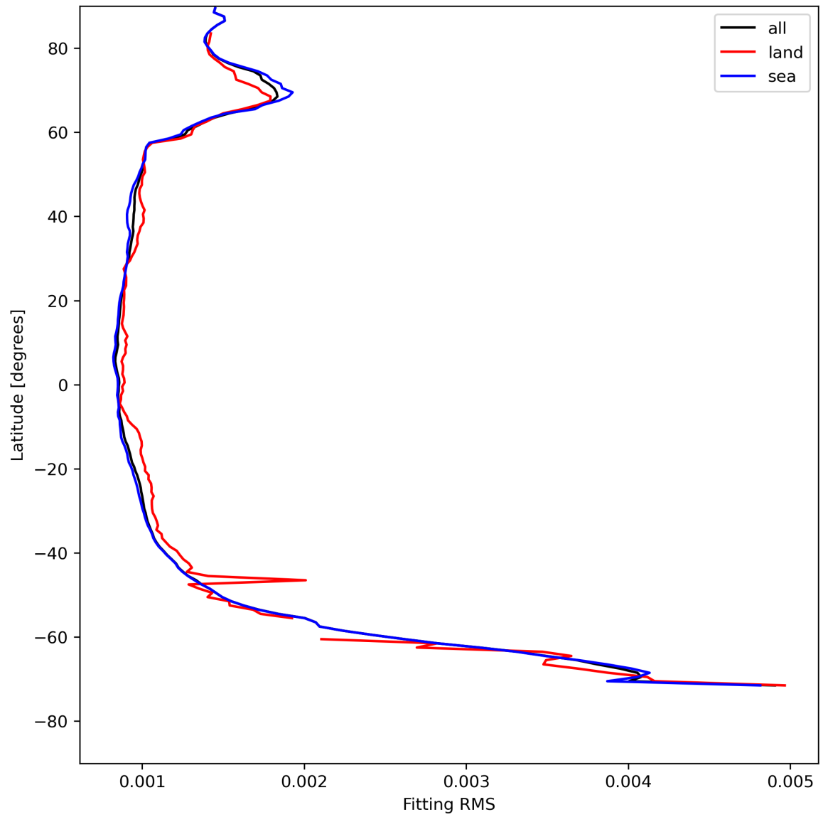
Figure 16: Zonal average of “Fitting RMS” for 2024-05-07 to 2024-05-08.
