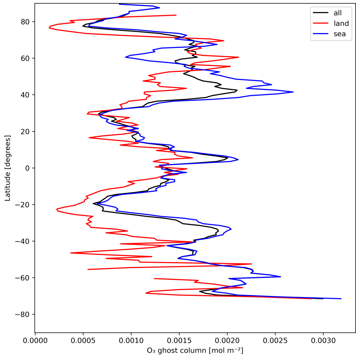
Figure 18: Zonal average of "O 3 ghost column" for 2024-05-07 to 2024-05-08.
