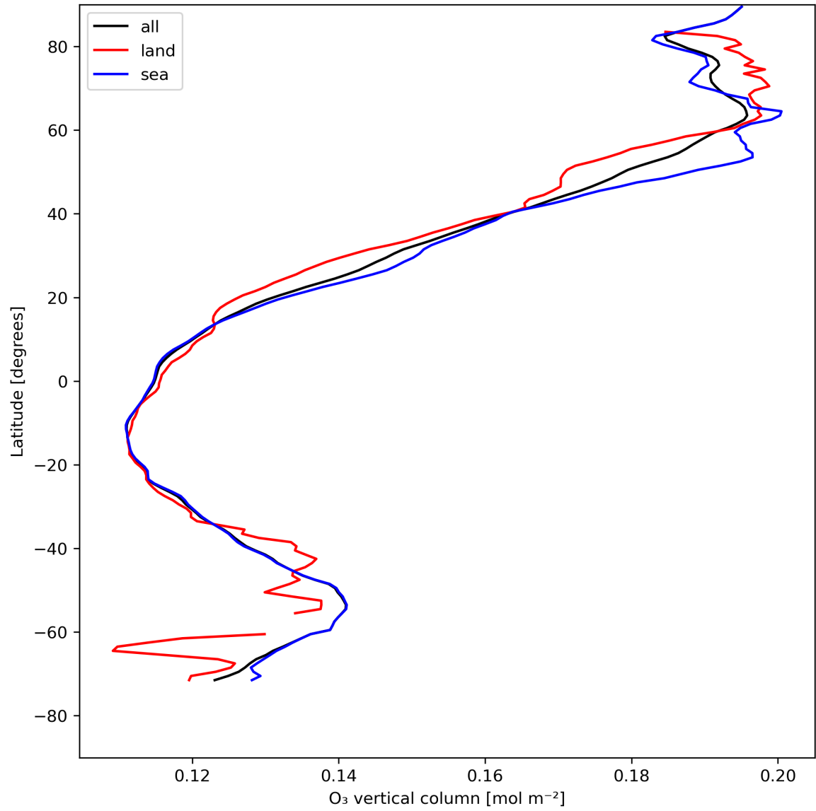
Figure 14: Zonal average of “O 3 vertical column” for 2024-05-07 to 2024-05-08.
