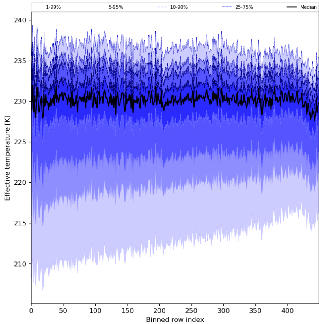
Figure 31: Along track statistics of “Effective temperature” for 2024-05-07 to 2024-05-08
