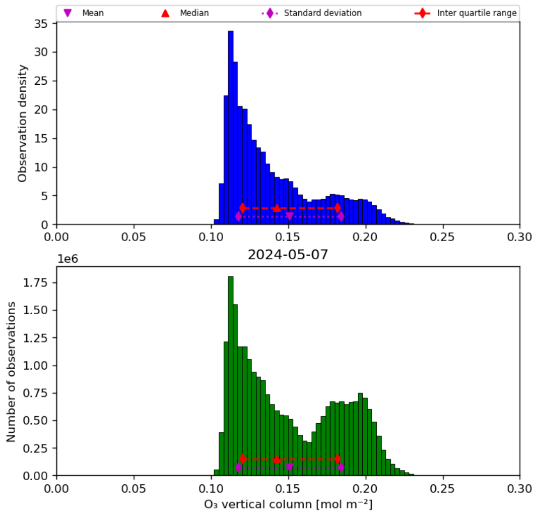
Figure 21: Histogram of “O 3 vertical column” for 2024-05-07 to 2024-05-08
