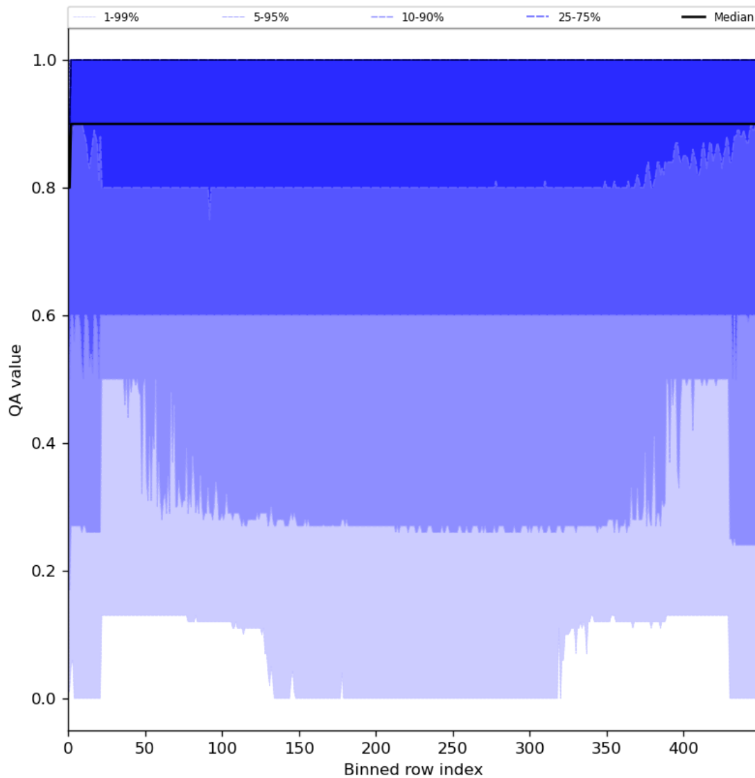
Figure 27: Along track statistics of “QA value” for 2024-05-07 to 2024-05-08
