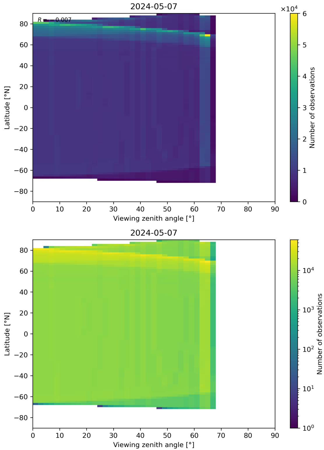
Figure 49: Scatter density plot of “Viewing zenith angle” against “Latitude” for 2024-05-07 to 2024-05-08.
