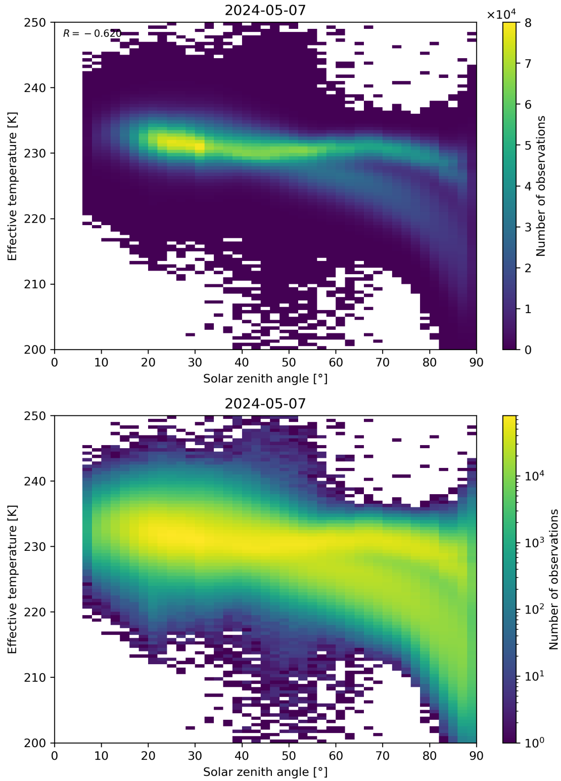
Figure 45: Scatter density plot of “Solar zenith angle” against “Effective temperature” for 2024-05-07 to 2024-05-08.
