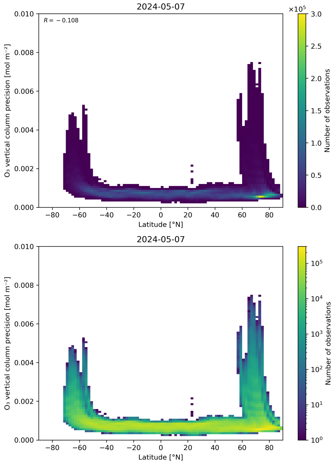
Figure 37: Scatter density plot of “Latitude” against “O 3 vertical column precision” for 2024-05-07 to 2024-05-08.
