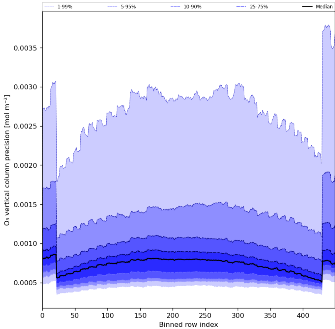
Figure 29: Along track statistics of “O 3 vertical column precision” for 2024-05-07 to 2024-05-08
