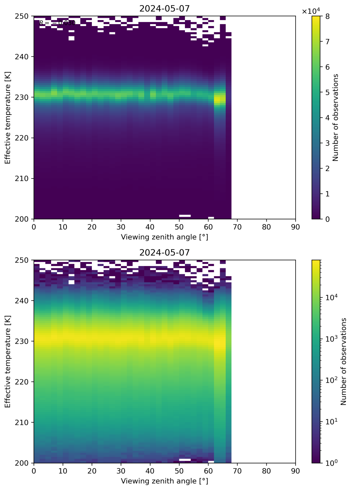
Figure 50: Scatter density plot of “Viewing zenith angle” against “Effective temperature” for 2024-05-07 to 2024-05-08.
