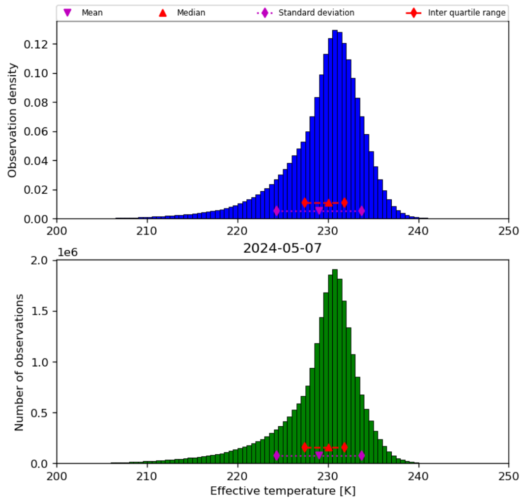
Figure 24: Histogram of “Effective temperature” for 2024-05-07 to 2024-05-08
