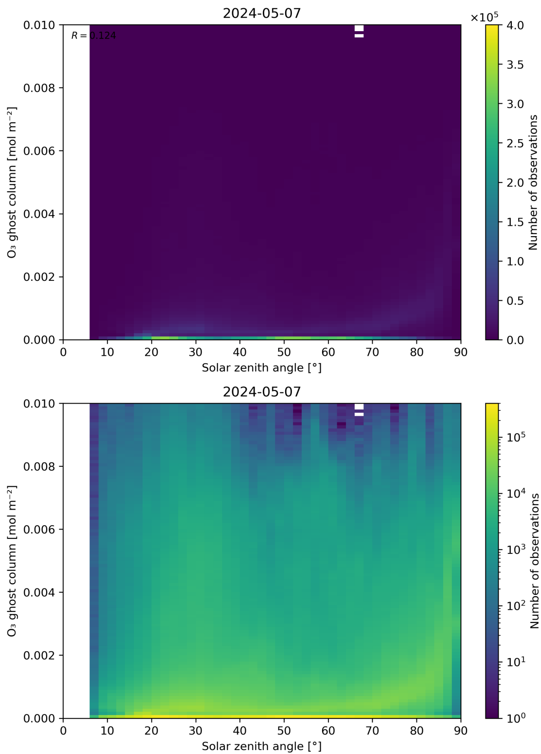
Figure 46: Scatter density plot of “Solar zenith angle” against “O 3 ghost column” for 2024-05-07 to 2024-05-08.
