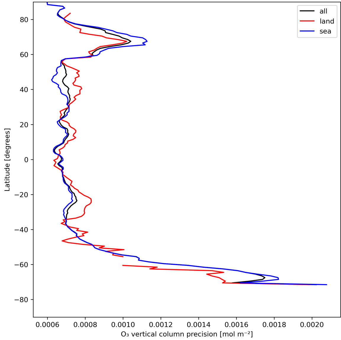
Figure 15: Zonal average of “O 3 vertical column precision” for 2024-05-07 to 2024-05-08.
