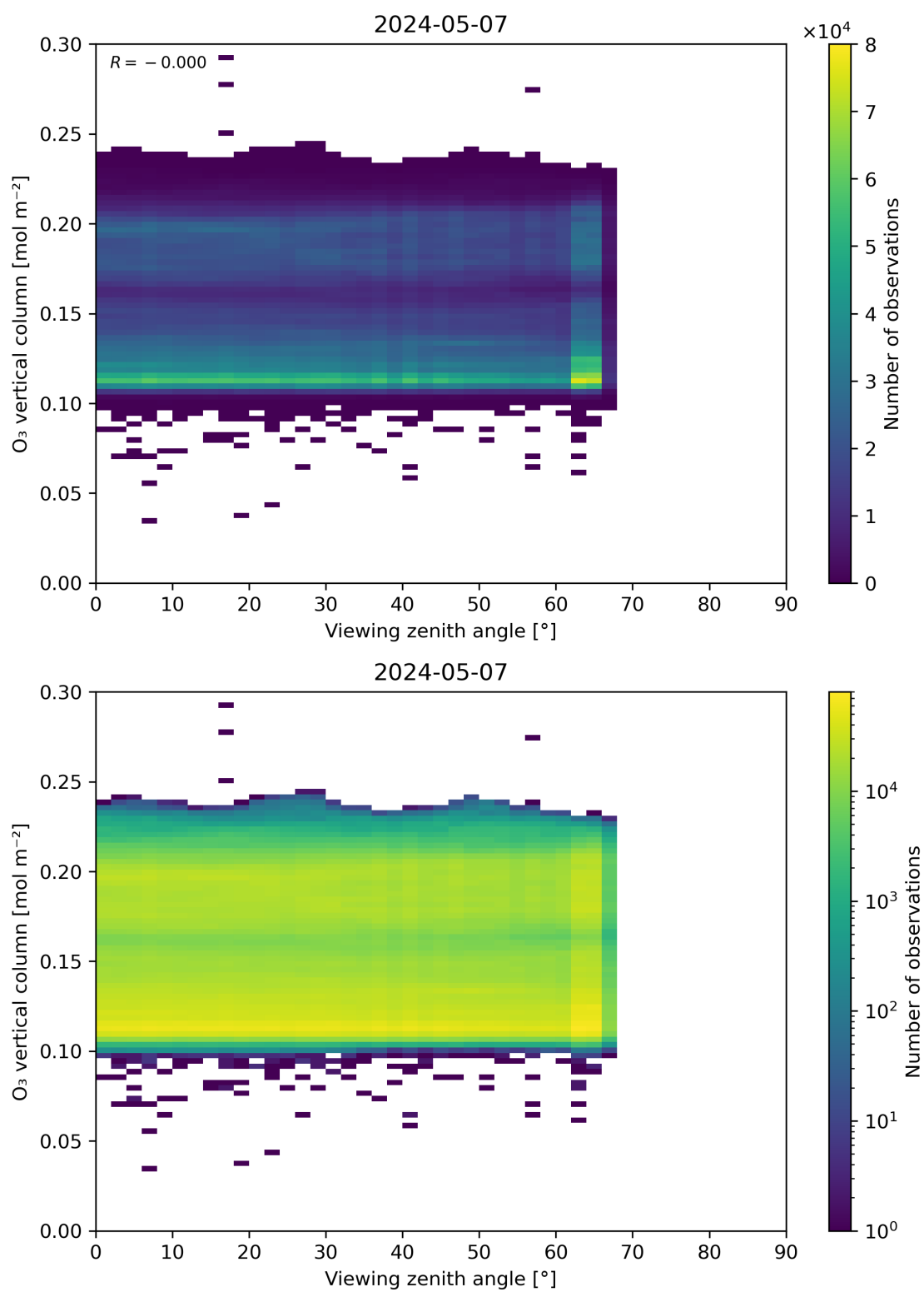
Figure 52: Scatter density plot of “Viewing zenith angle” against “O 3 vertical column” for 2024-05-07 to 2024-05-08.
