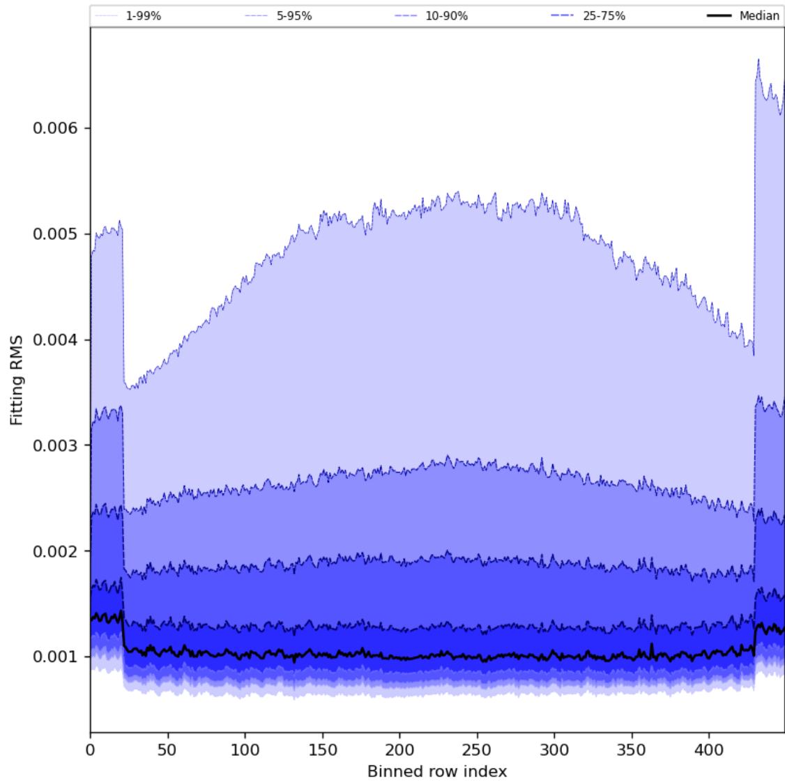
Figure 30: Along track statistics of “Fitting RMS” for 2024-05-07 to 2024-05-08
