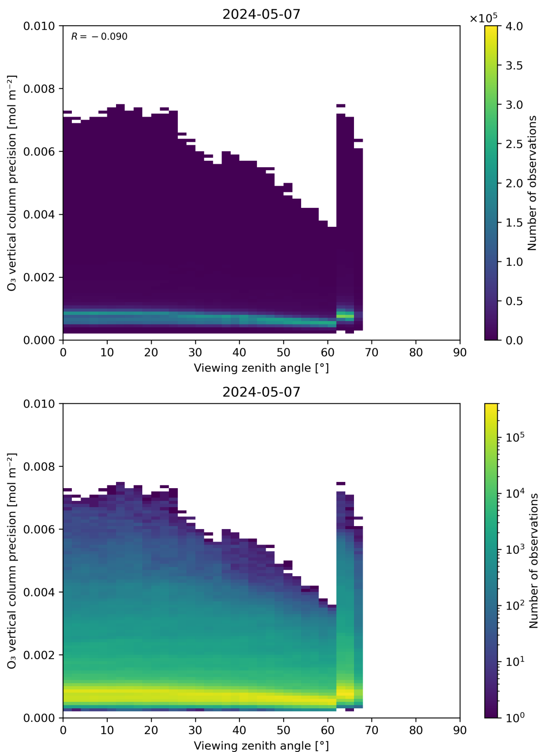
Figure 53: Scatter density plot of “Viewing zenith angle” against “O 3 vertical column precision” for 2024-05-07 to 2024-05-08.
