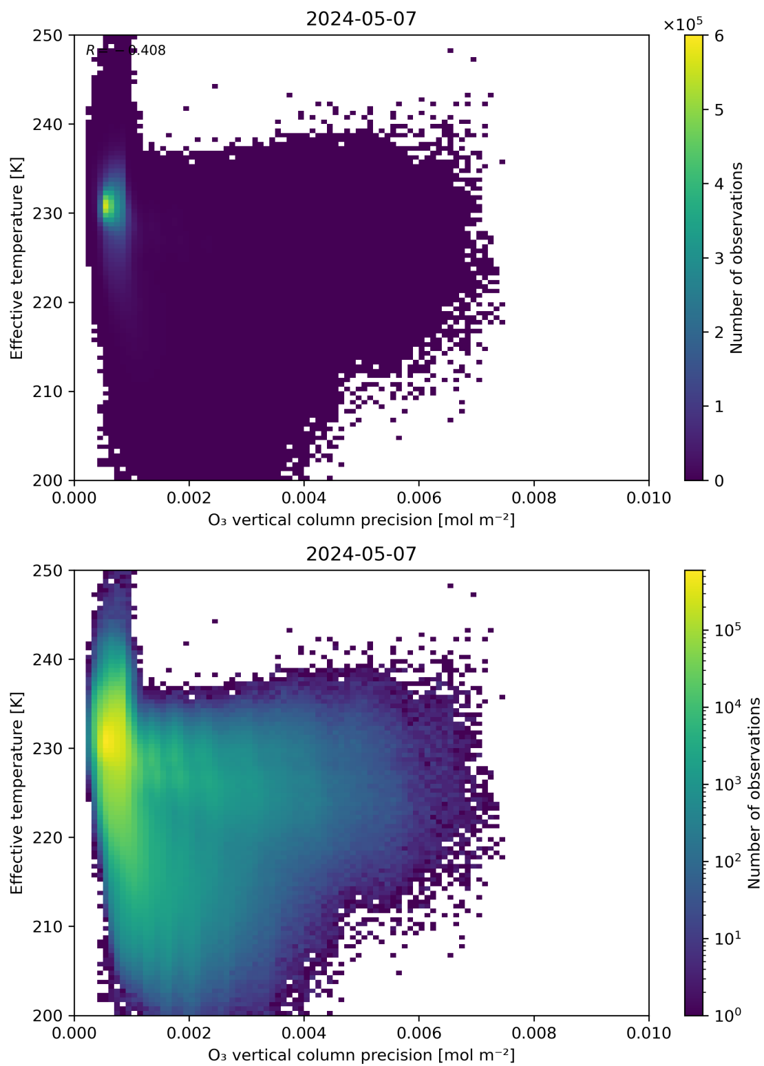
Figure 42: Scatter density plot of “O 3 vertical column precision” against “Effective temperature” for 2024-05-07 to 2024-05-08.
