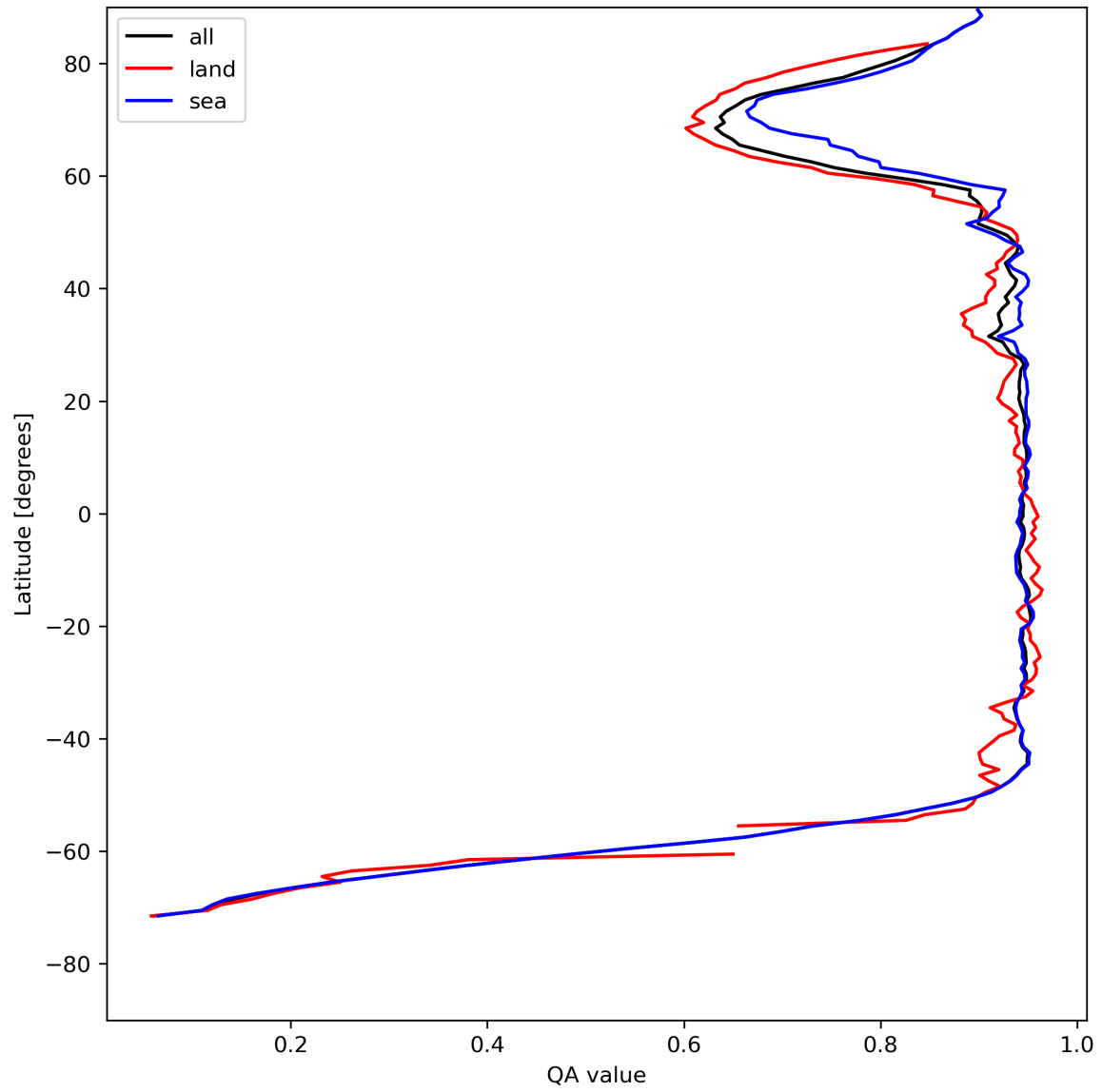
Figure 13: Zonal average of “QA value” for 2024-05-07 to 2024-05-08.
