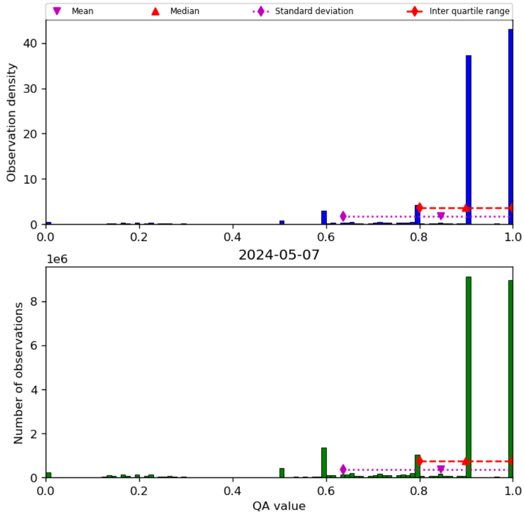
Figure 20: Histogram of “QA value” for 2024-05-07 to 2024-05-08
