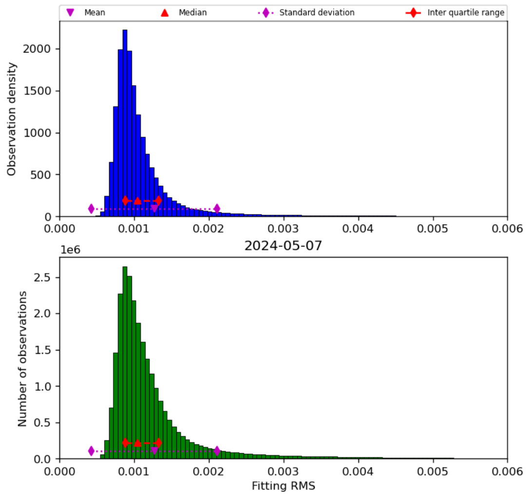
Figure 23: Histogram of “Fitting RMS” for 2024-05-07 to 2024-05-08
