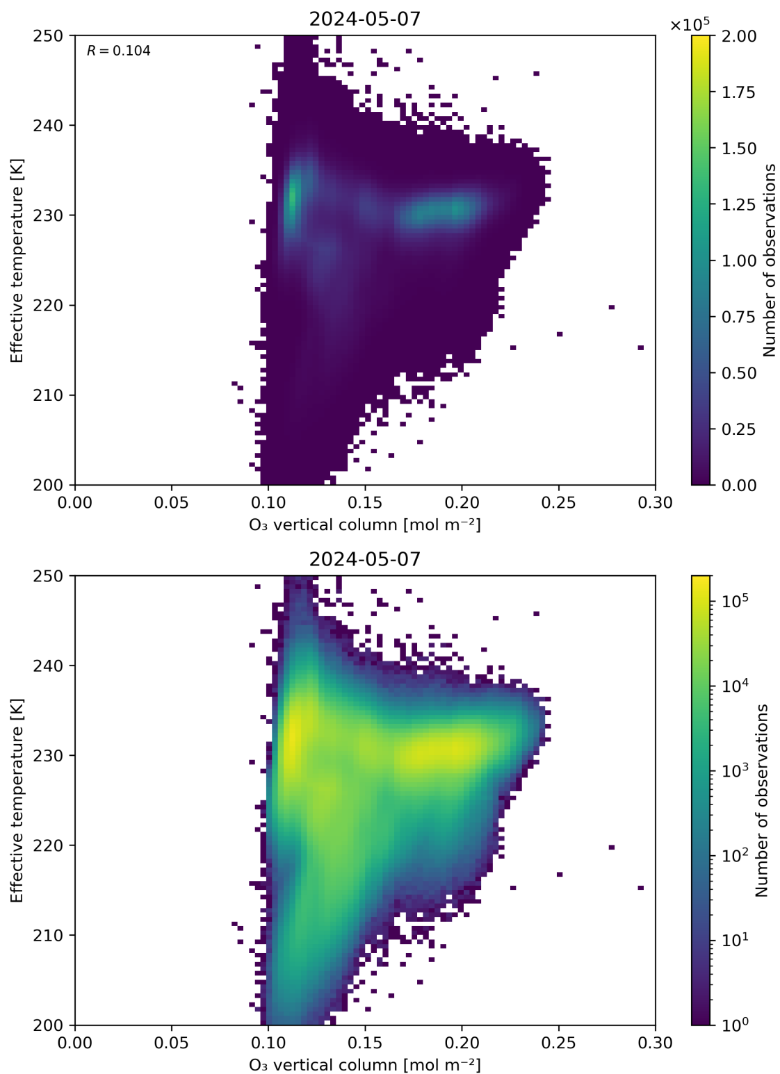
Figure 39: Scatter density plot of “O 3 vertical column” against “Effective temperature” for 2024-05-07 to 2024-05-08.
