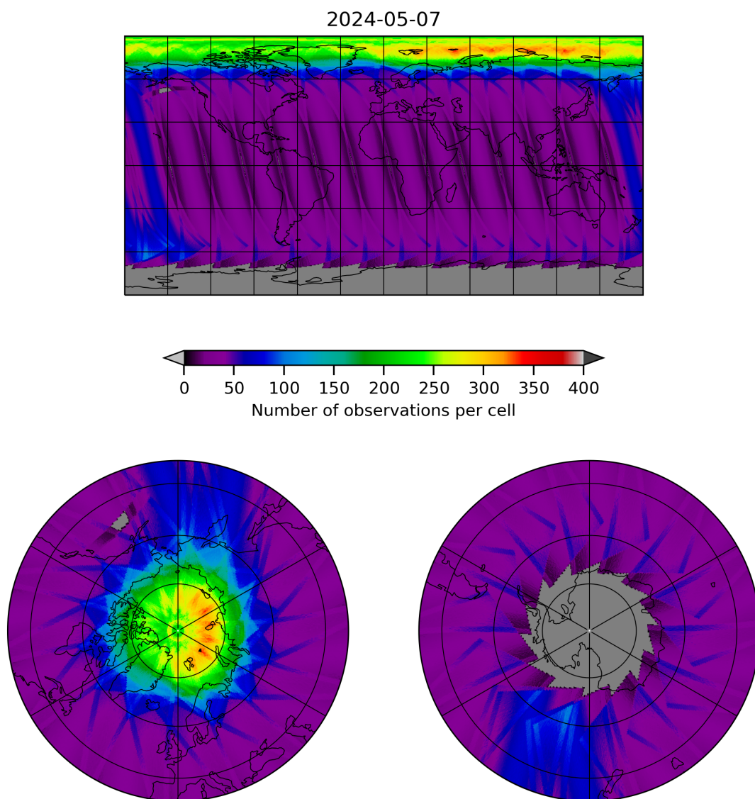
Figure 12: Map of the number of observations for 2024-05-07 to 2024-05-08
