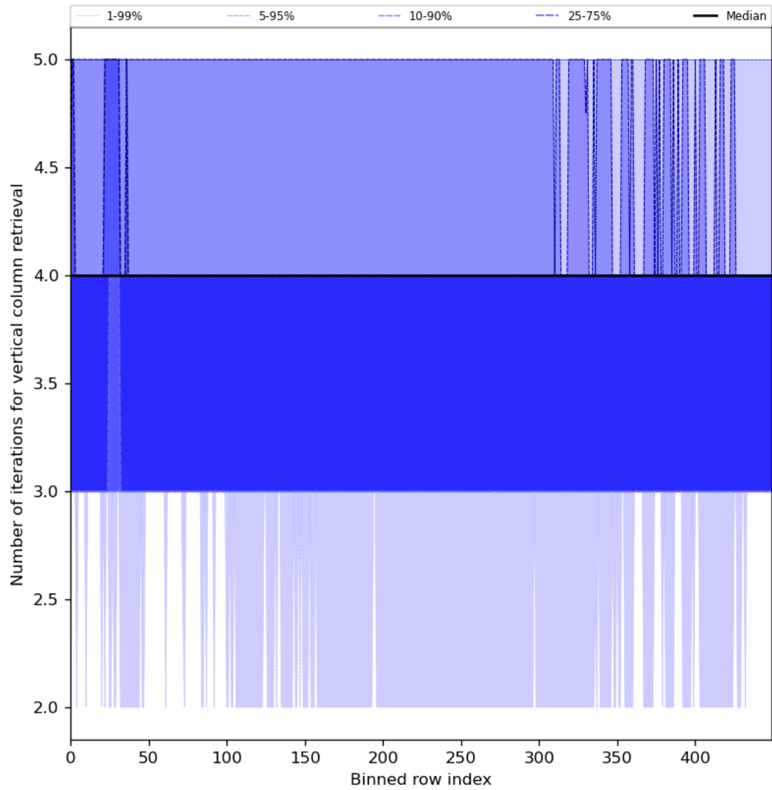
Figure 33: Along track statistics of “Number of iterations for vertical column retrieval” for 2024-05-07 to 2024-05-08
