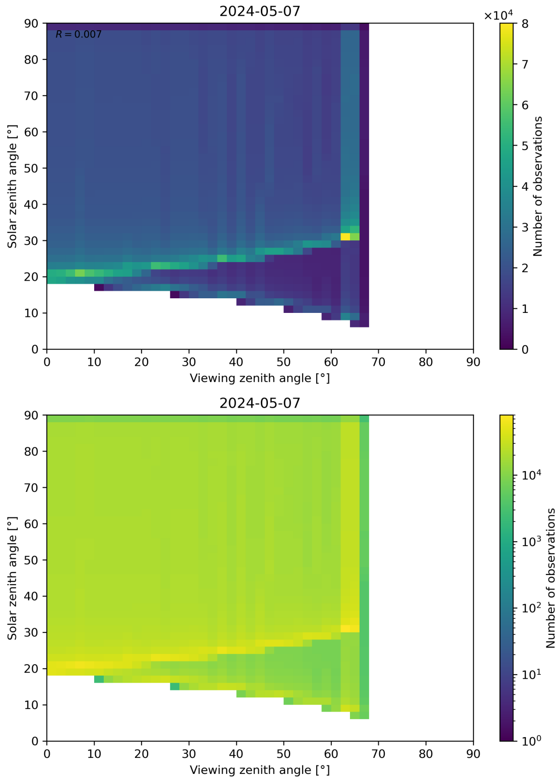
Figure 54: Scatter density plot of “Viewing zenith angle” against “Solar zenith angle” for 2024-05-07 to 2024-05-08.
