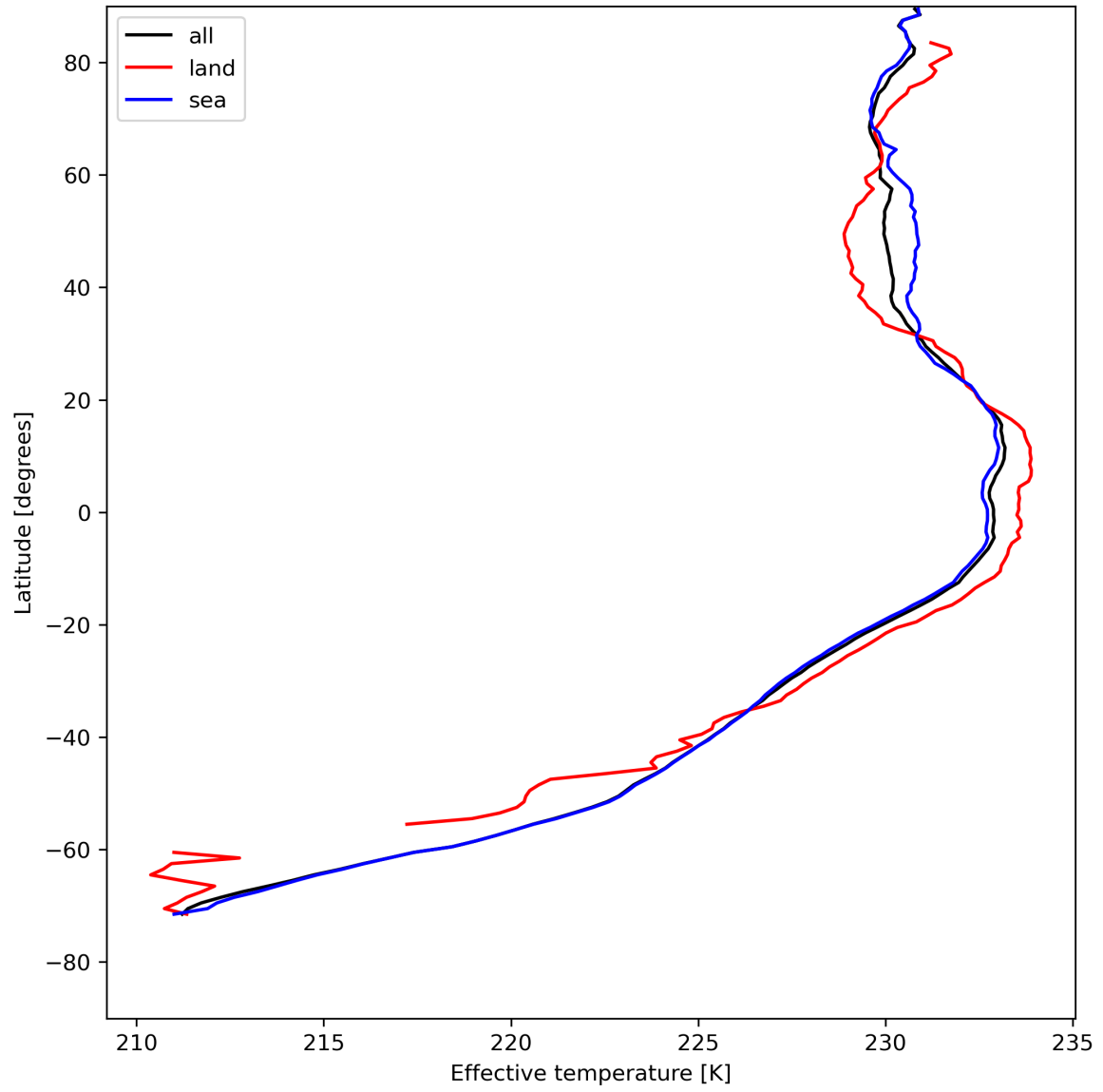
Figure 17: Zonal average of "Effective temperature" for 2024-05-07 to 2024-05-08.
