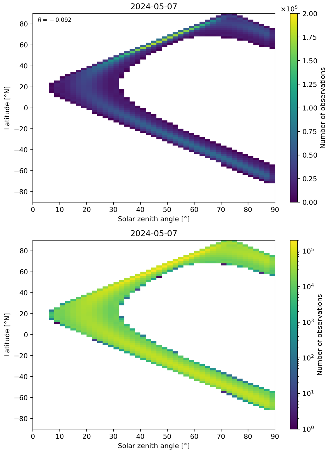
Figure 44: Scatter density plot of “Solar zenith angle” against “Latitude” for 2024-05-07 to 2024-05-08.
