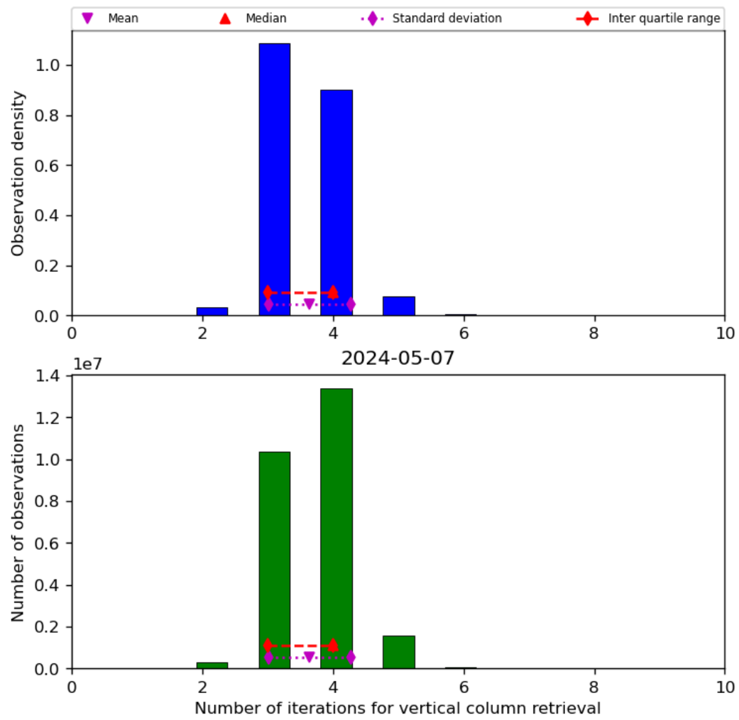
Figure 26: Histogram of “Number of iterations for vertical column retrieval” for 2024-05-07 to 2024-05-08
