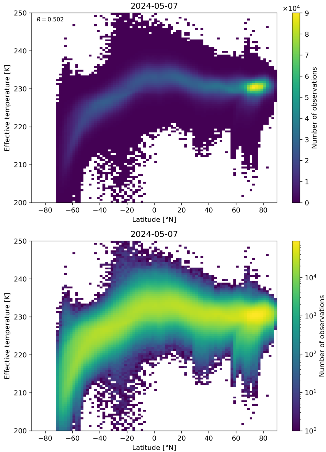
Figure 34: Scatter density plot of “Latitude” against “Effective temperature” for 2024-05-07 to 2024-05-08.
