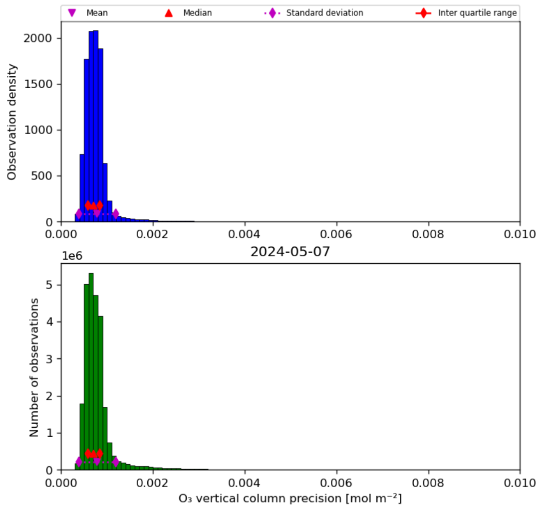
Figure 22: Histogram of “O 3 vertical column precision” for 2024-05-07 to 2024-05-08
