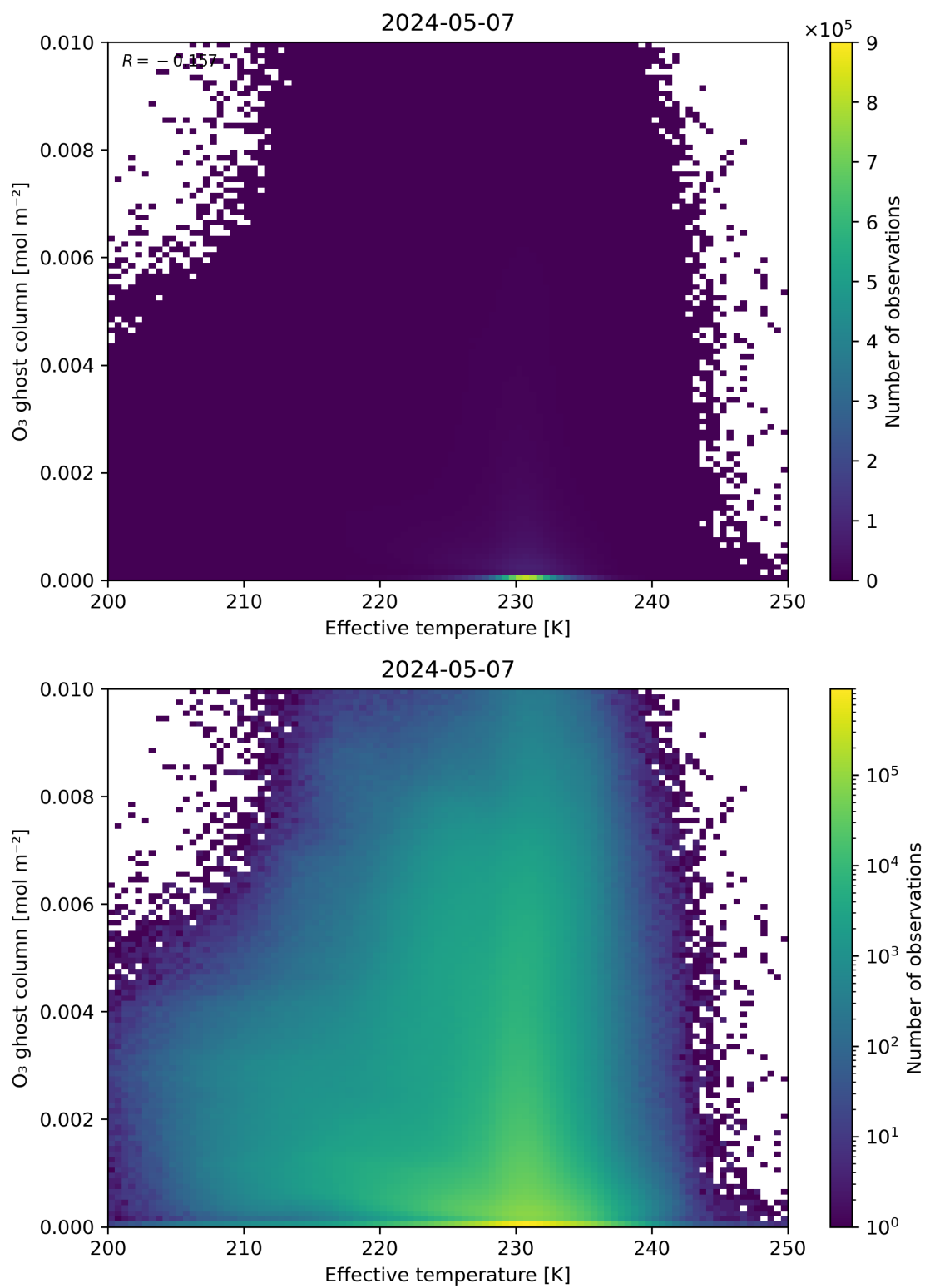
Figure 38: Scatter density plot of “Effective temperature” against “O 3 ghost column” for 2024-05-07 to 2024-05-08.
