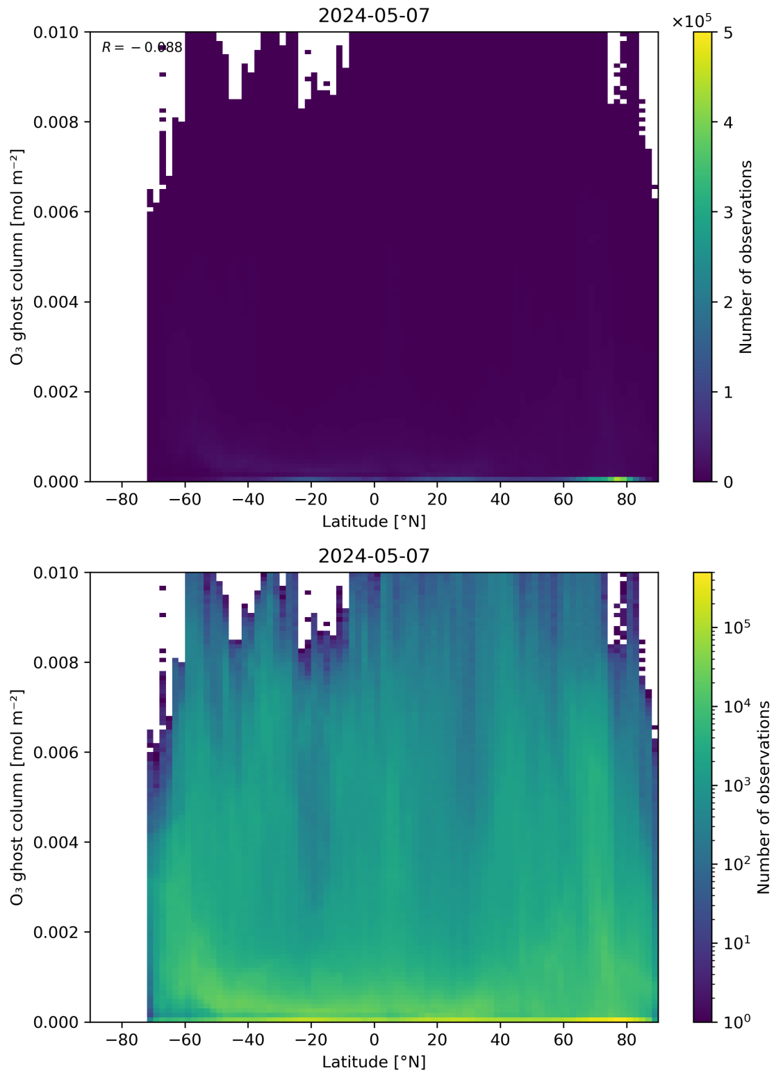
Figure 35: Scatter density plot of “Latitude” against “O 3 ghost column” for 2024-05-07 to 2024-05-08.
