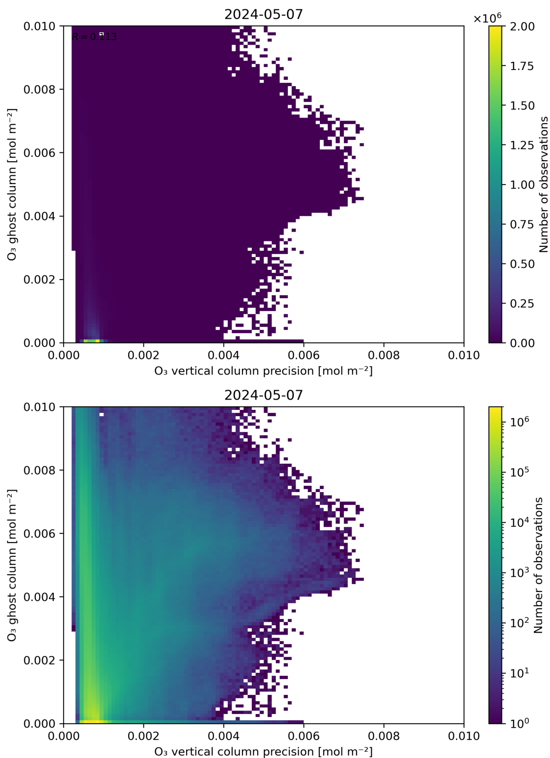
Figure 43: Scatter density plot of “O 3 vertical column precision” against “O 3 ghost column” for 2024-05-07 to 2024-05-08.
