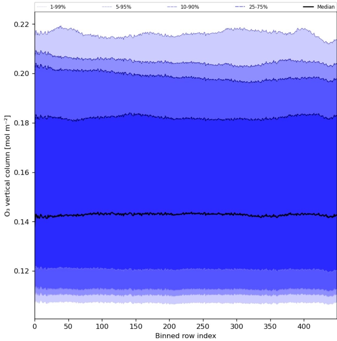
Figure 28: Along track statistics of “ \text{O}_3 vertical column” for 2024-05-07 to 2024-05-08
