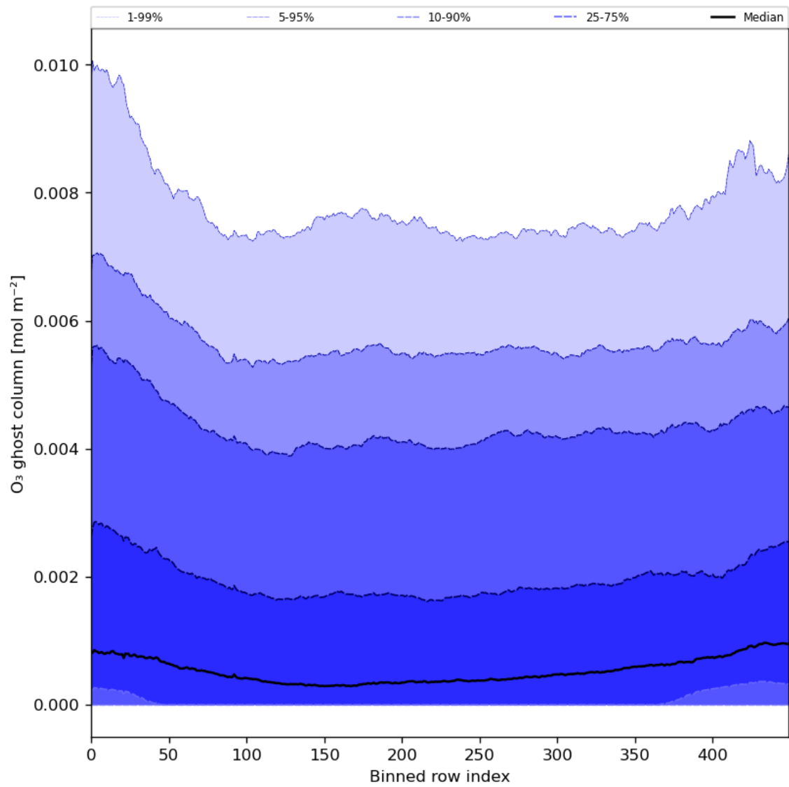
Figure 32: Along track statistics of “O 3 ghost column” for 2024-05-07 to 2024-05-08
