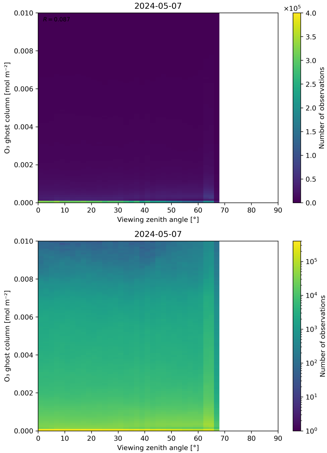
Figure 51: Scatter density plot of “Viewing zenith angle” against “O 3 ghost column” for 2024-05-07 to 2024-05-08.
