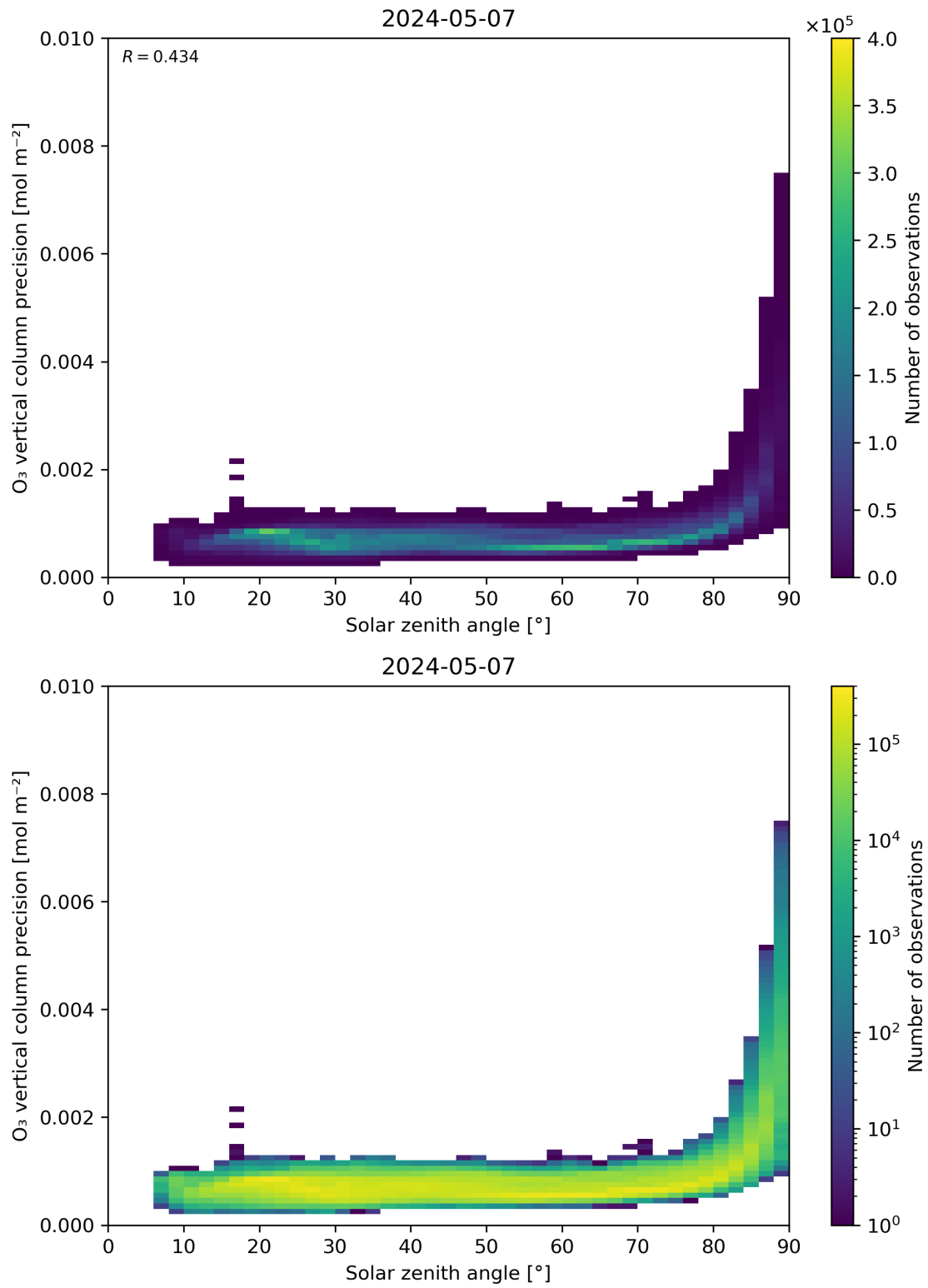
Figure 48: Scatter density plot of “Solar zenith angle” against “O 3 vertical column precision” for 2024-05-07 to 2024-05-08.
