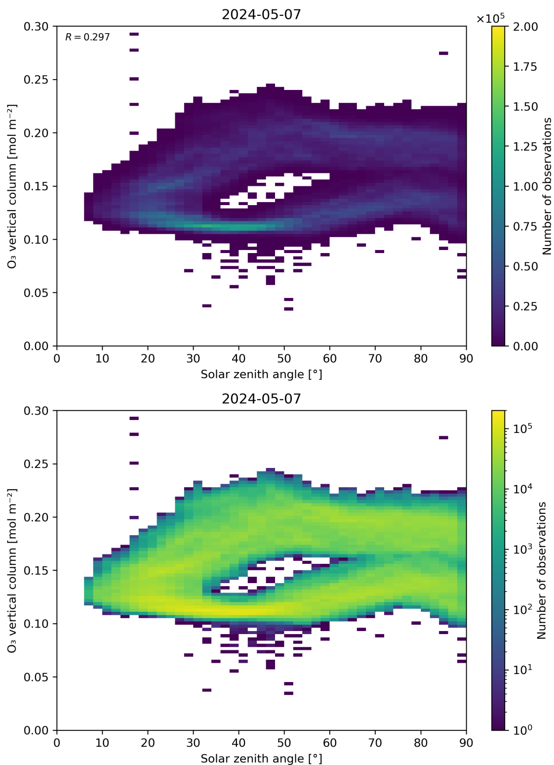
Figure 47: Scatter density plot of “Solar zenith angle” against “O 3 vertical column” for 2024-05-07 to 2024-05-08.
