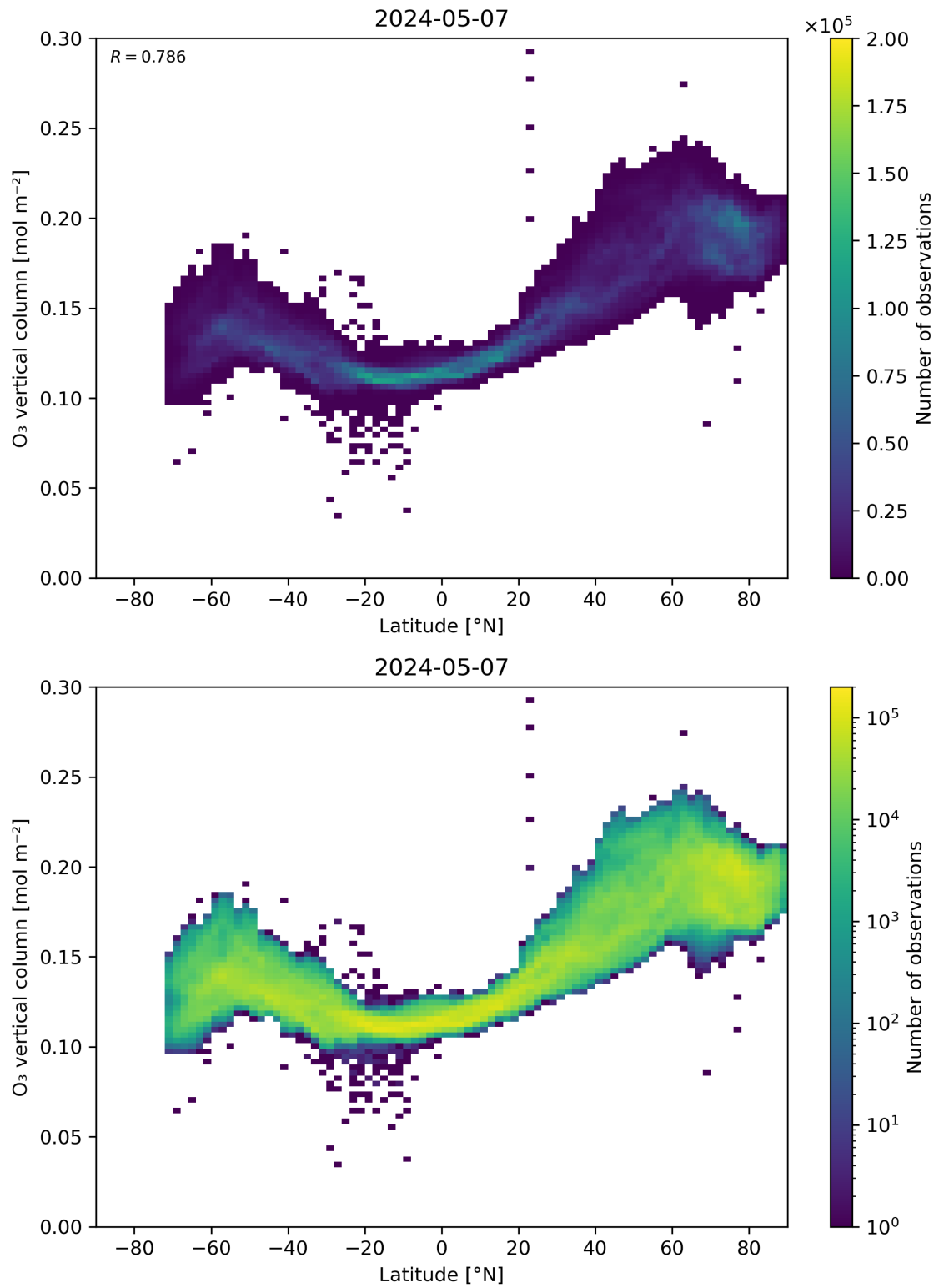
Figure 36: Scatter density plot of “Latitude” against “O 3 vertical column” for 2024-05-07 to 2024-05-08.
