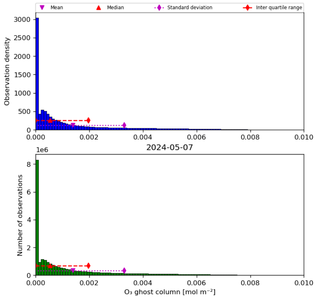
Figure 25: Histogram of “O 3 ghost column” for 2024-05-07 to 2024-05-08
