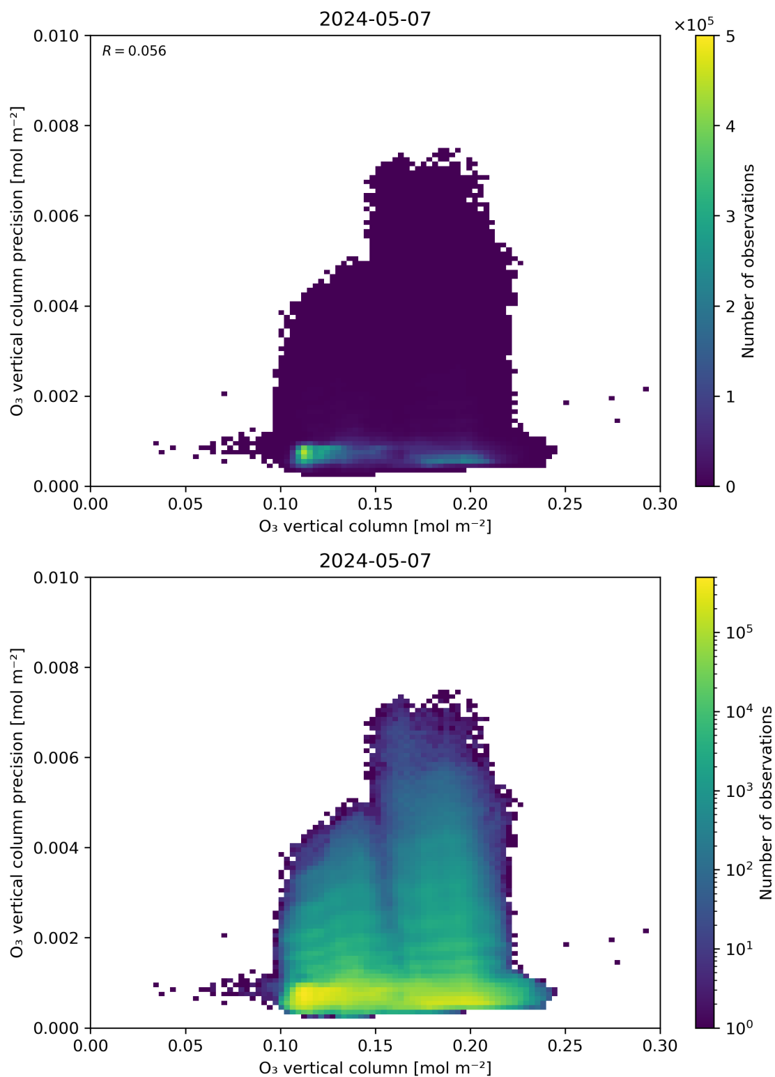
Figure 41: Scatter density plot of “O 3 vertical column” against “O 3 vertical column precision” for 2024-05-07 to 2024-05-08.
