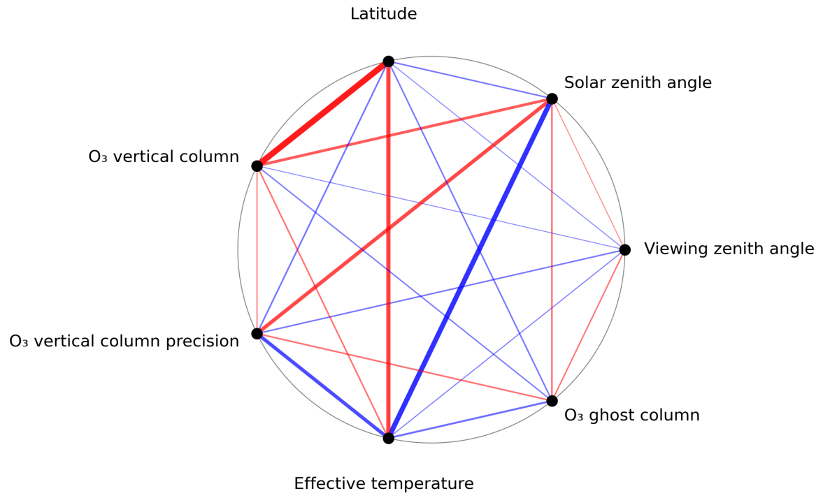
Figure 1: Map of correlation graph for 2024-05-07 to 2024-05-08.
