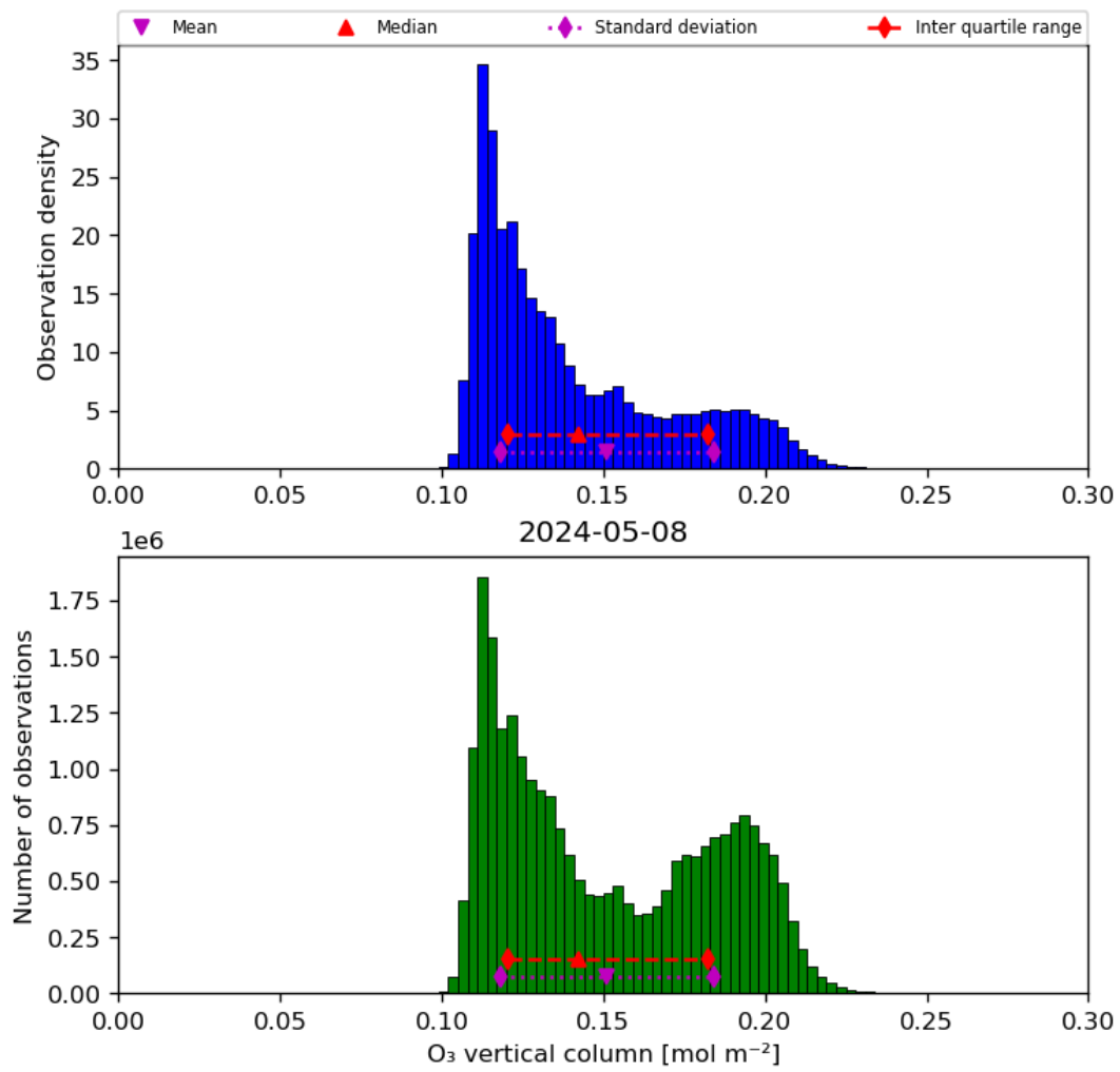
Figure 21: Histogram of “O 3 vertical column” for 2024-05-07 to 2024-05-09
