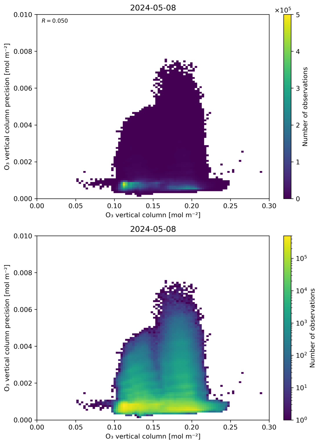
Figure 41: Scatter density plot of “O 3 vertical column” against “O 3 vertical column precision” for 2024-05-07 to 2024-05-09.
