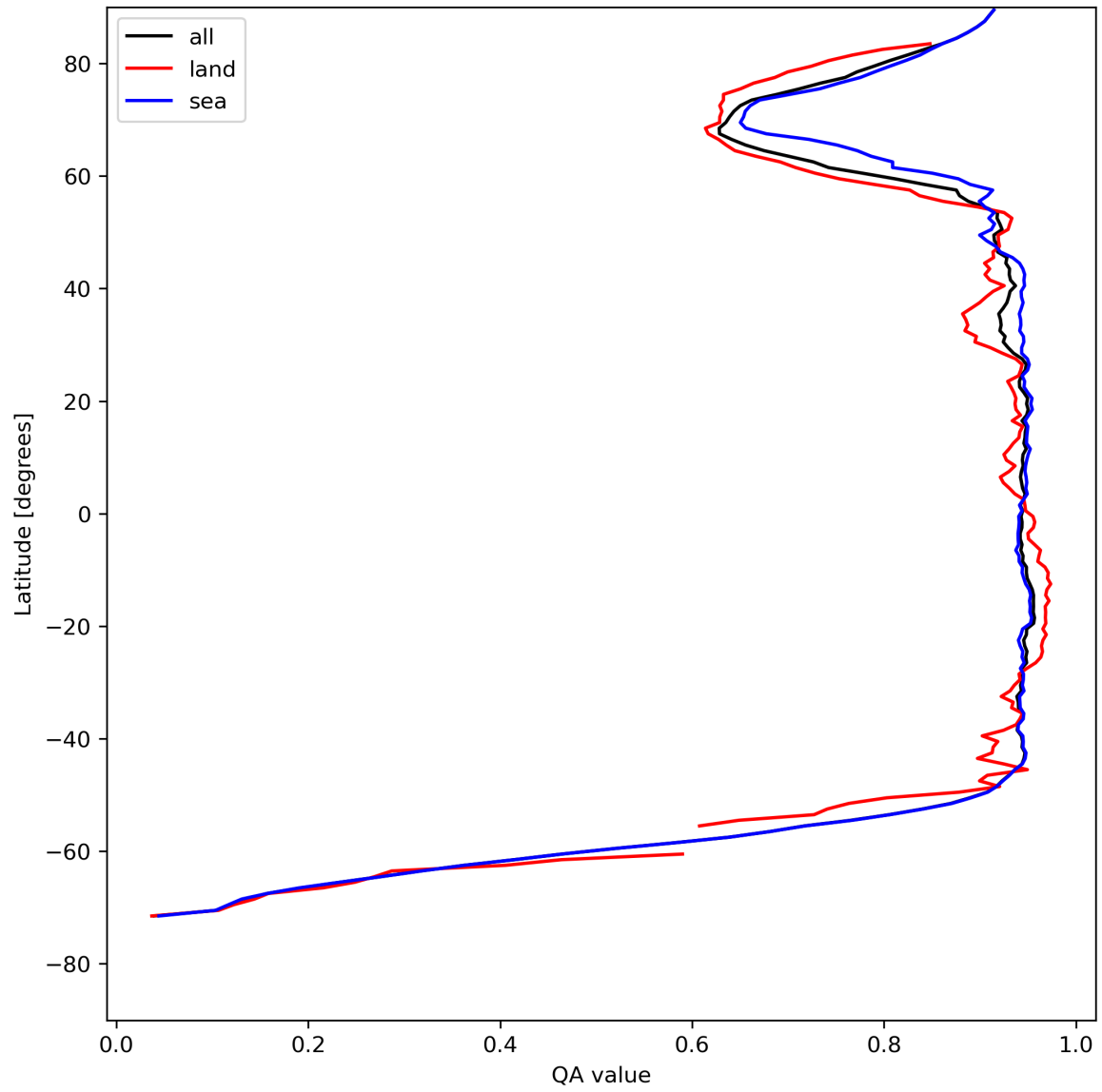
Figure 13: Zonal average of “QA value” for 2024-05-07 to 2024-05-09.
