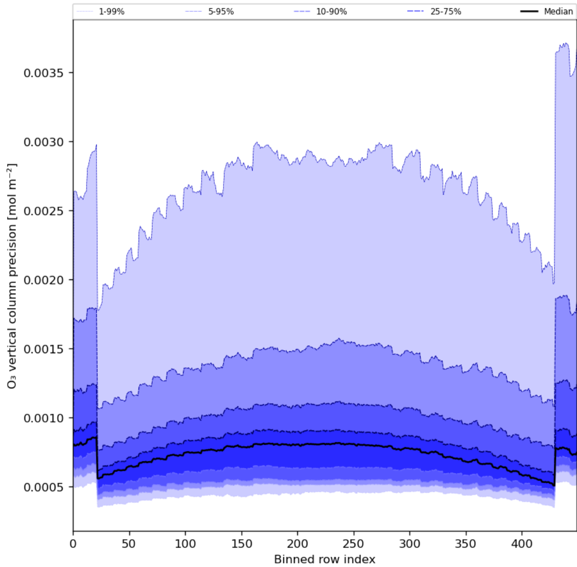
Figure 29: Along track statistics of “O 3 vertical column precision” for 2024-05-07 to 2024-05-09
