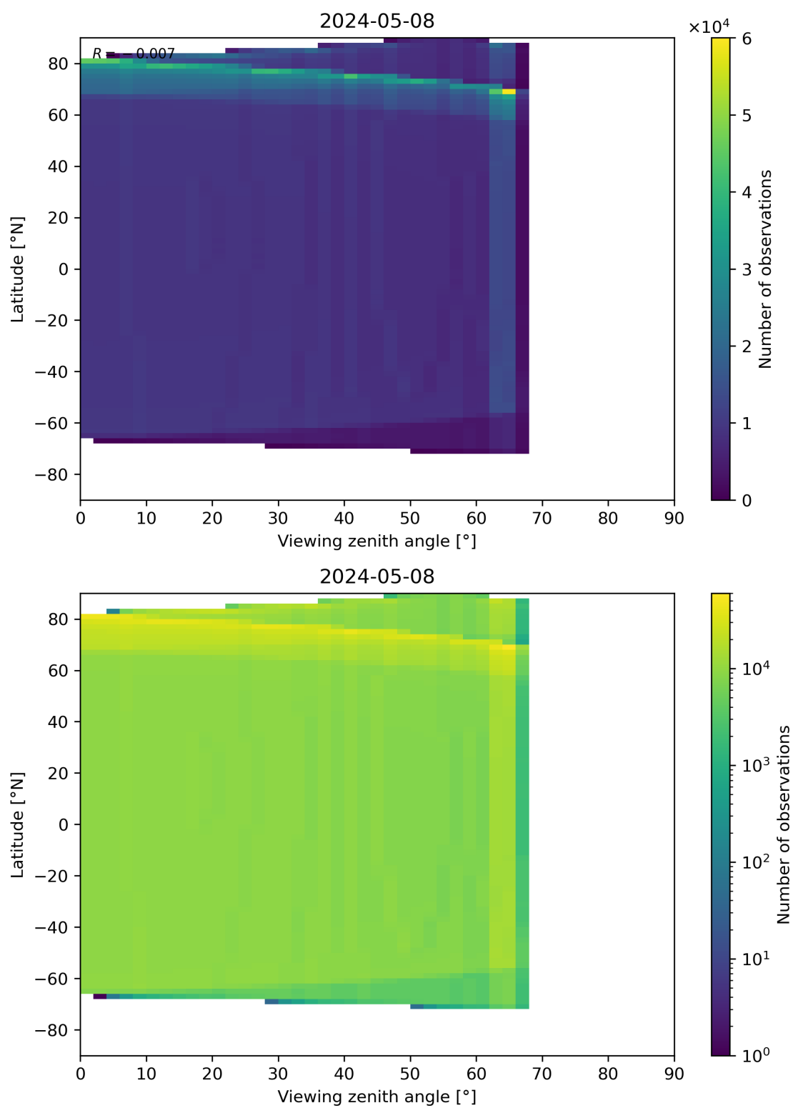
Figure 49: Scatter density plot of “Viewing zenith angle” against “Latitude” for 2024-05-07 to 2024-05-09.
