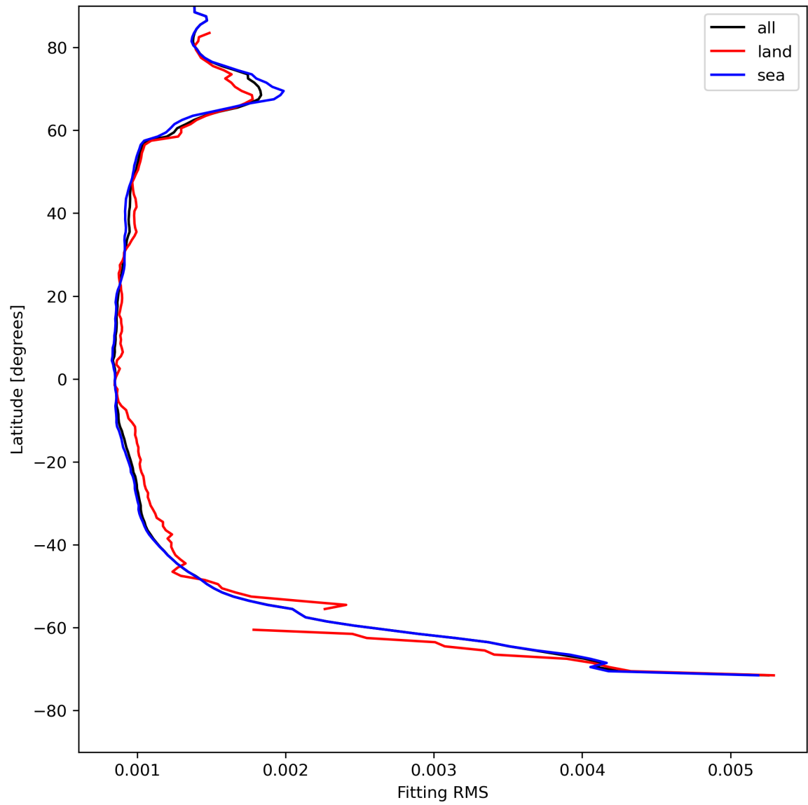
Figure 16: Zonal average of “Fitting RMS” for 2024-05-07 to 2024-05-09.
