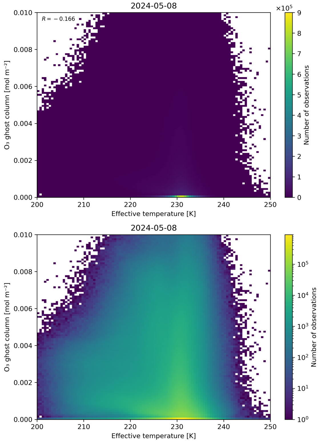
Figure 38: Scatter density plot of “Effective temperature” against “O 3 ghost column” for 2024-05-07 to 2024-05-09.
