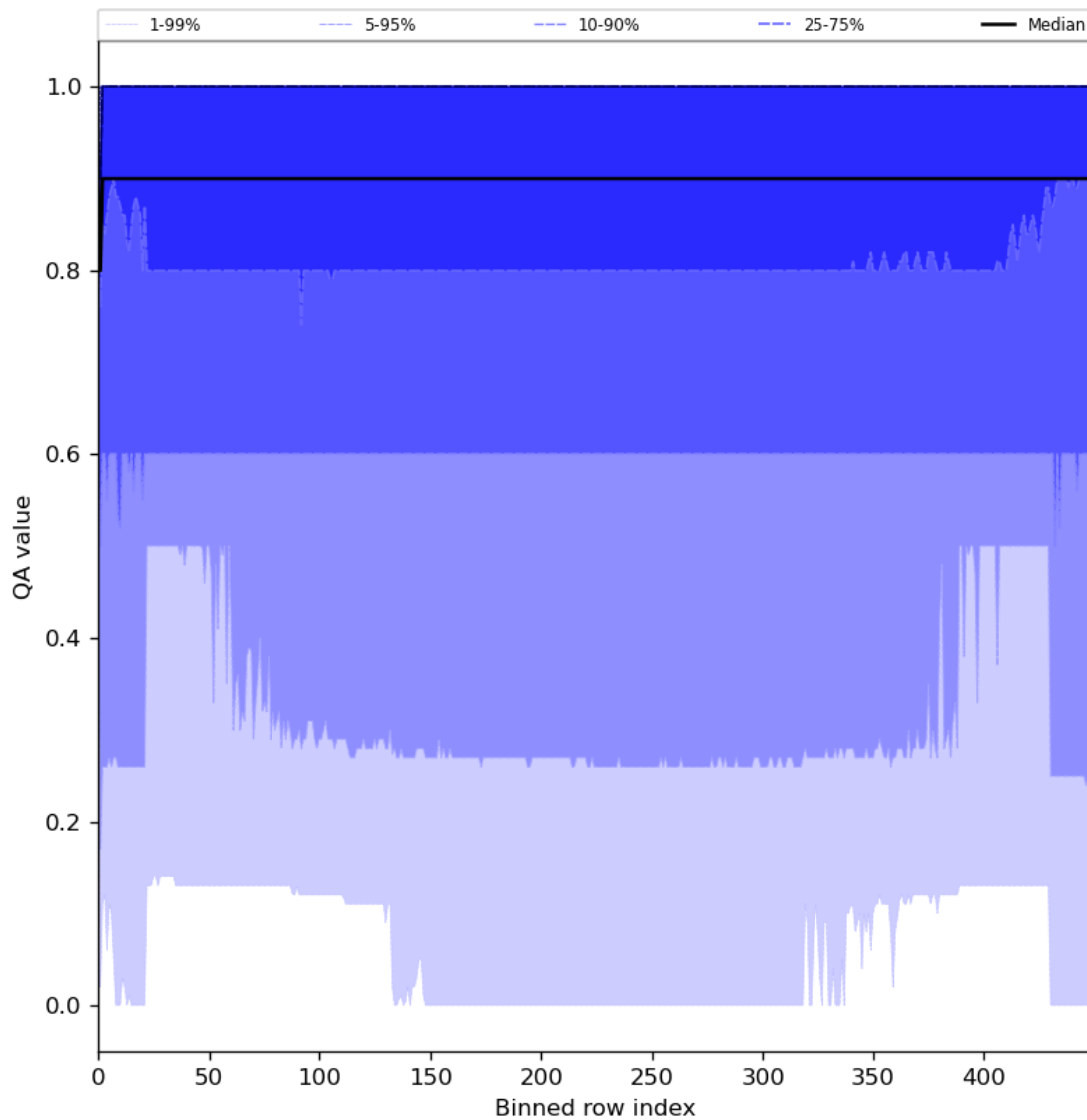
Figure 27: Along track statistics of “QA value” for 2024-05-07 to 2024-05-09
