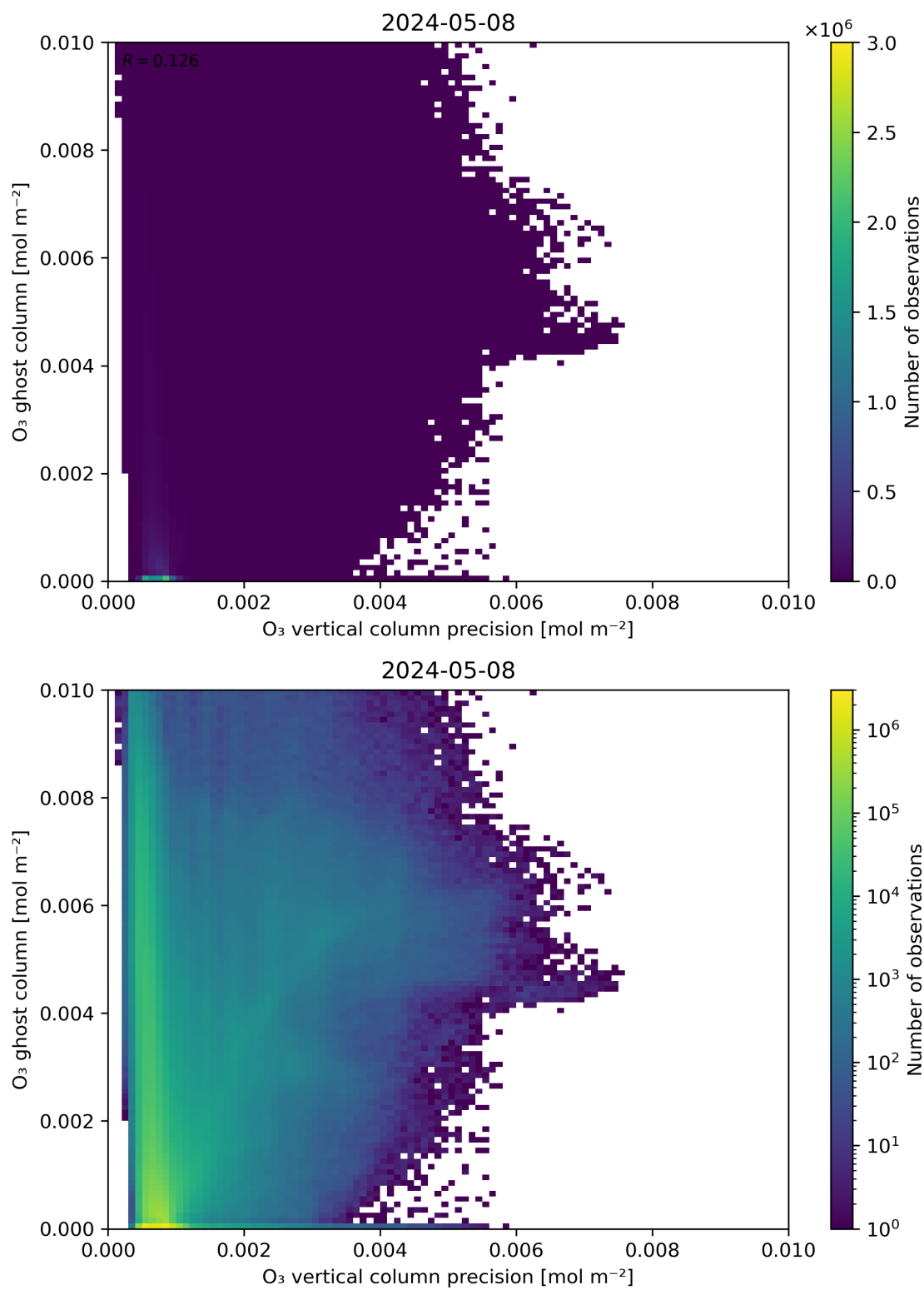
Figure 43: Scatter density plot of “O 3 vertical column precision” against “O 3 ghost column” for 2024-05-07 to 2024-05-09.
