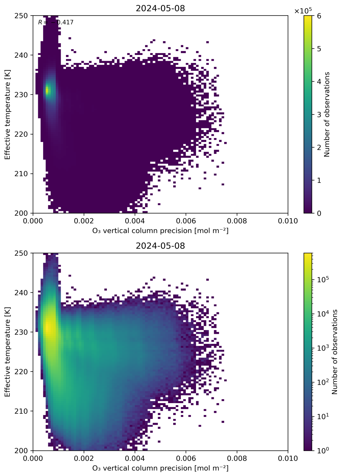
Figure 42: Scatter density plot of “O 3 vertical column precision” against “Effective temperature” for 2024-05-07 to 2024-05-09.
