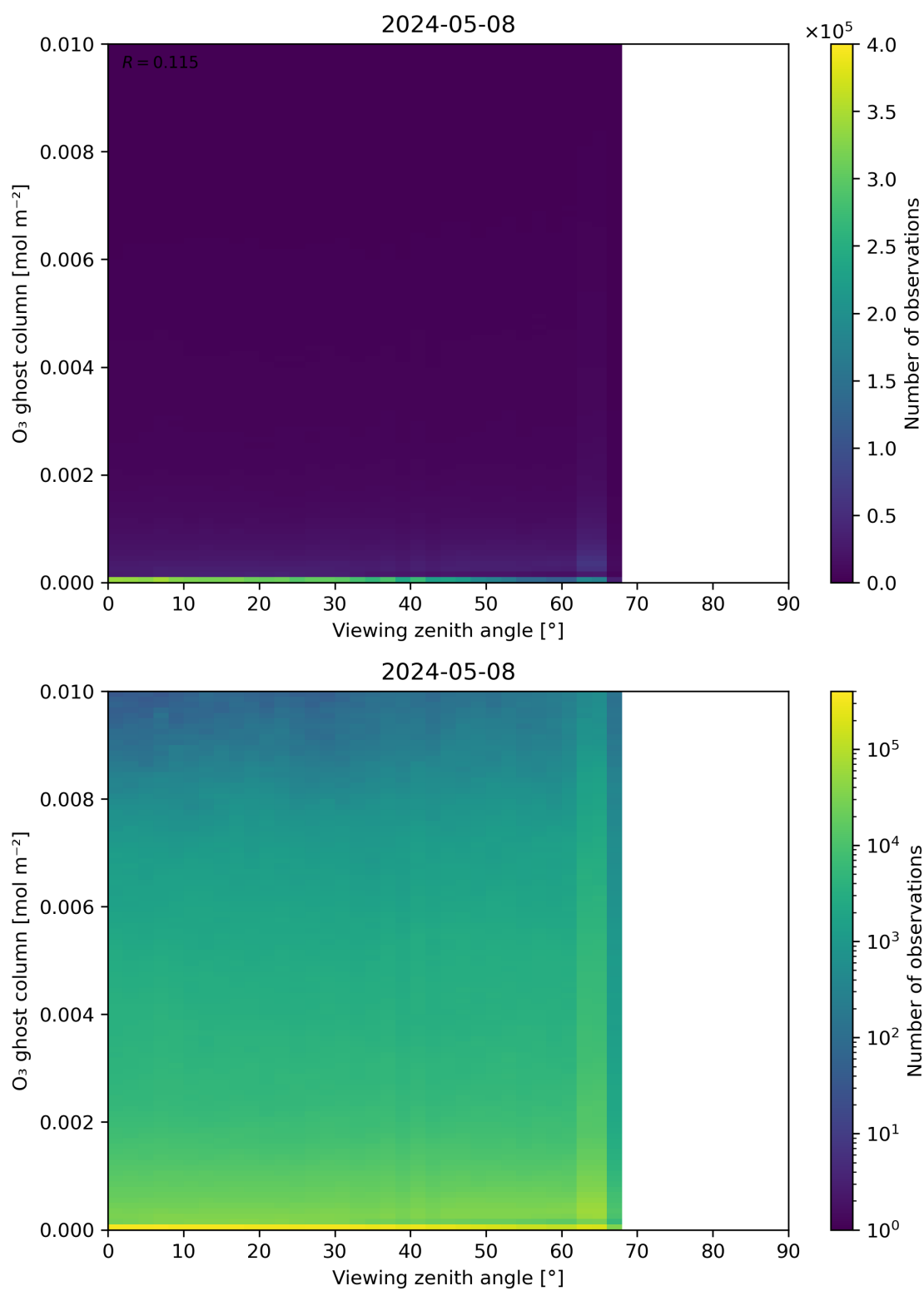
Figure 51: Scatter density plot of “Viewing zenith angle” against “O 3 ghost column” for 2024-05-07 to 2024-05-09.
