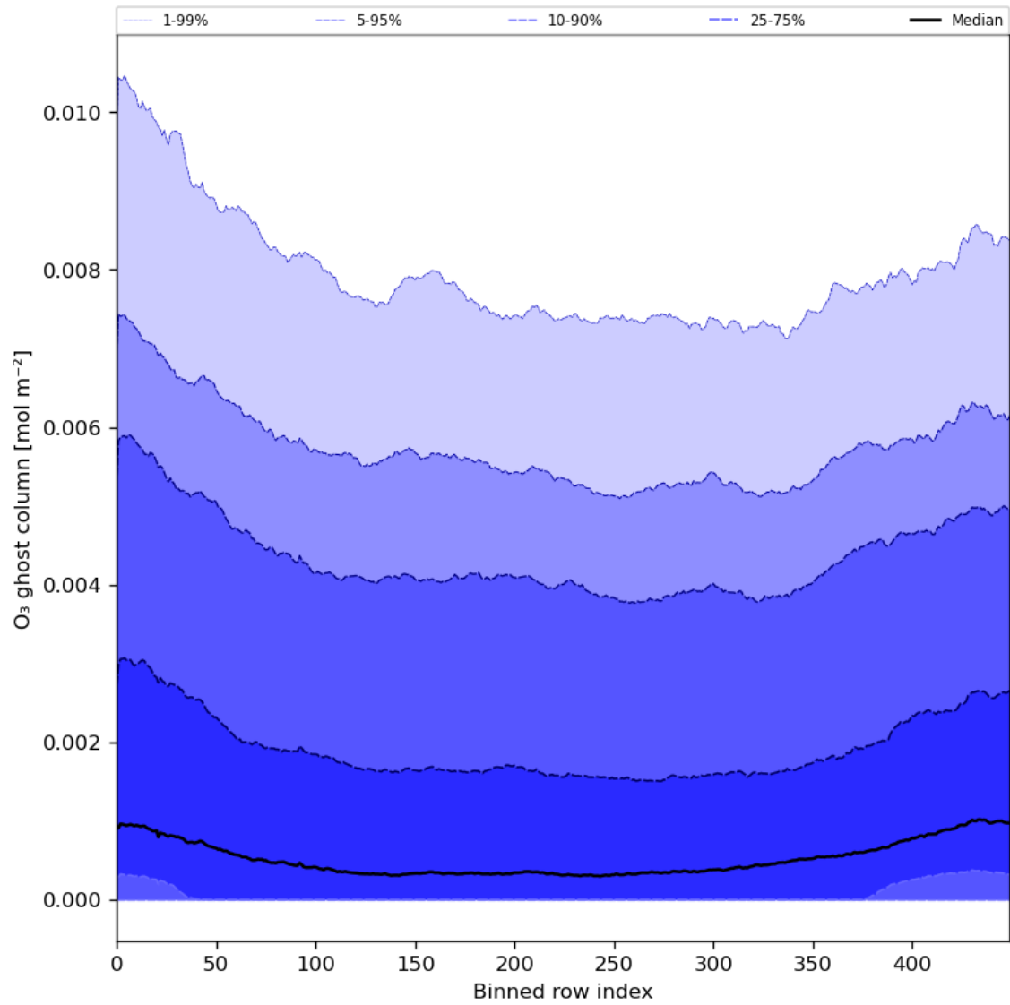
Figure 32: Along track statistics of “O 3 ghost column” for 2024-05-07 to 2024-05-09
