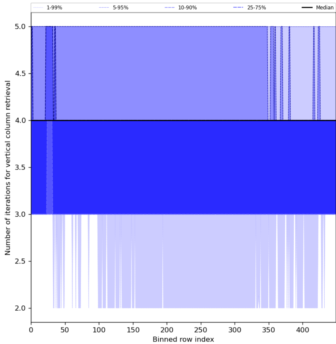
Figure 33: Along track statistics of “Number of iterations for vertical column retrieval” for 2024-05-07 to 2024-05-09
