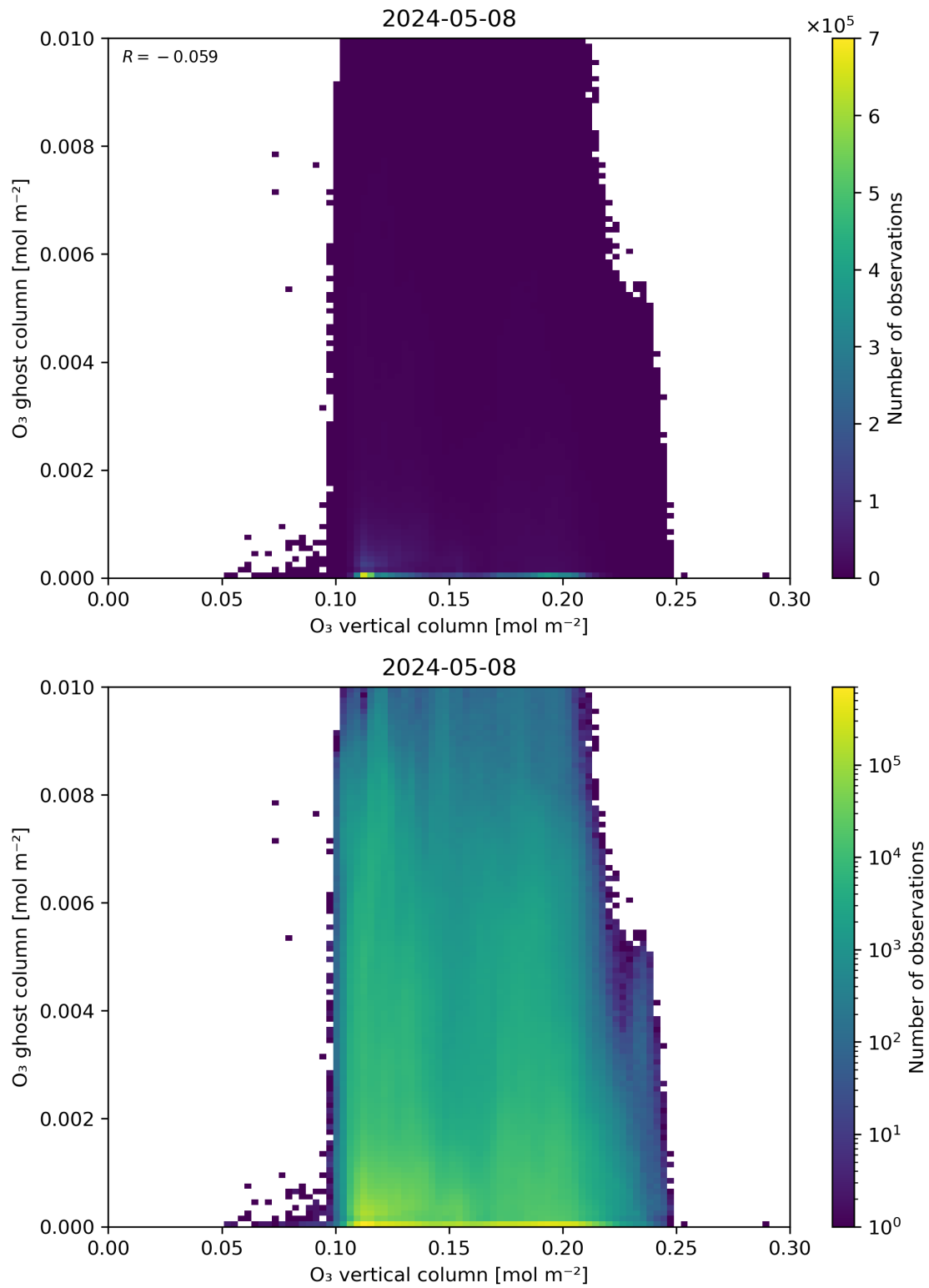
Figure 40: Scatter density plot of “O 3 vertical column” against “O 3 ghost column” for 2024-05-07 to 2024-05-09.
