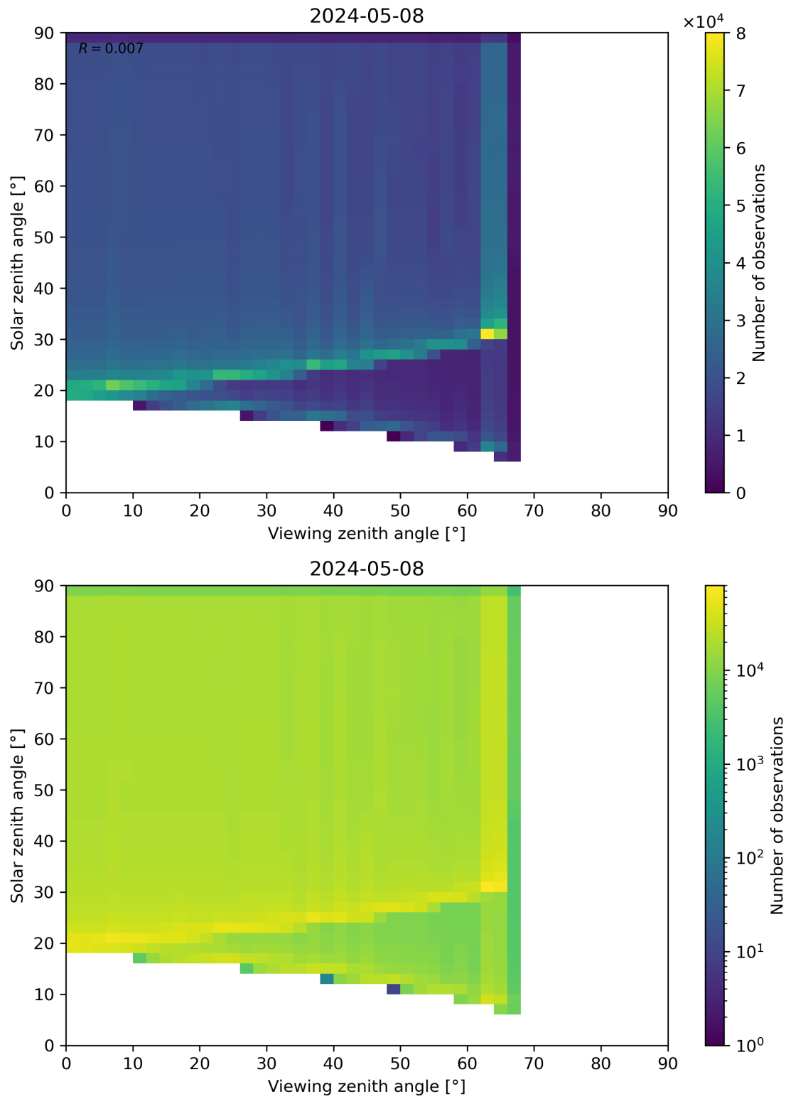
Figure 54: Scatter density plot of “Viewing zenith angle” against “Solar zenith angle” for 2024-05-07 to 2024-05-09.
