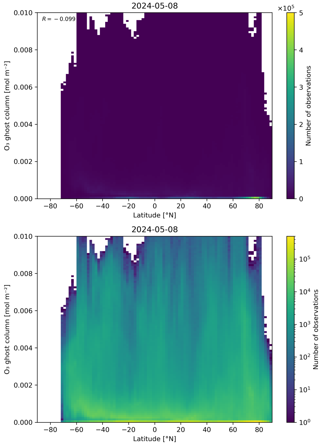
Figure 35: Scatter density plot of “Latitude” against “O 3 ghost column” for 2024-05-07 to 2024-05-09.
