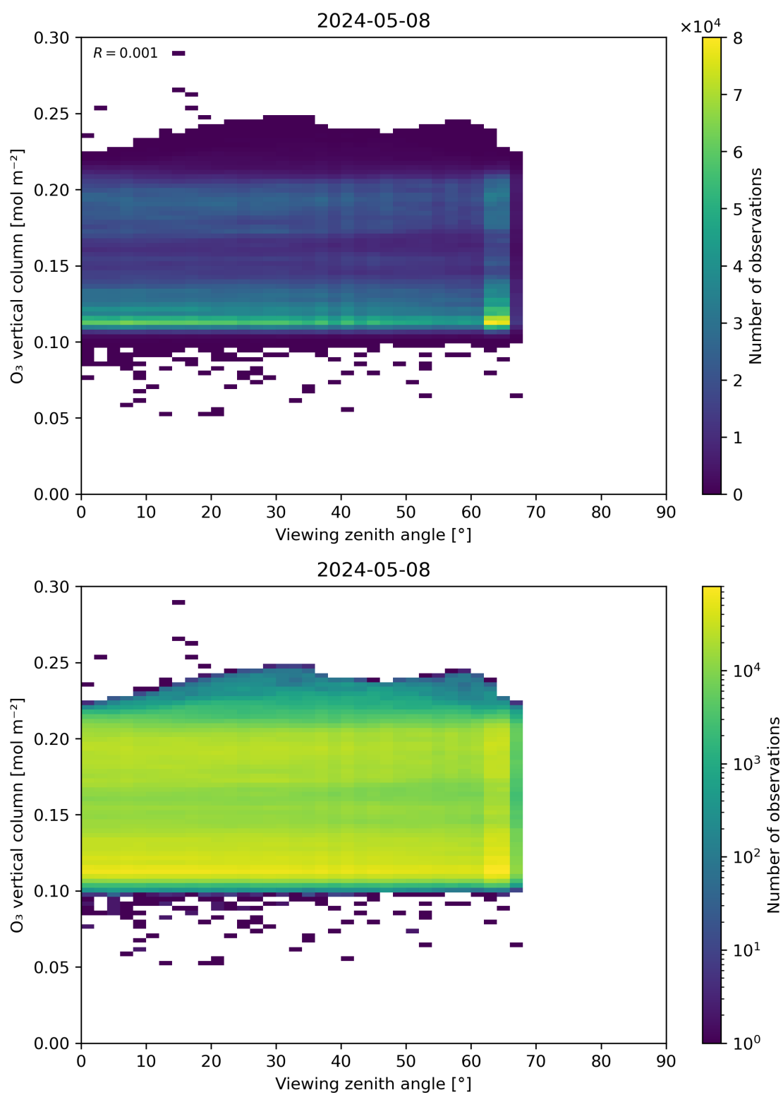
Figure 52: Scatter density plot of “Viewing zenith angle” against “O 3 vertical column” for 2024-05-07 to 2024-05-09.
