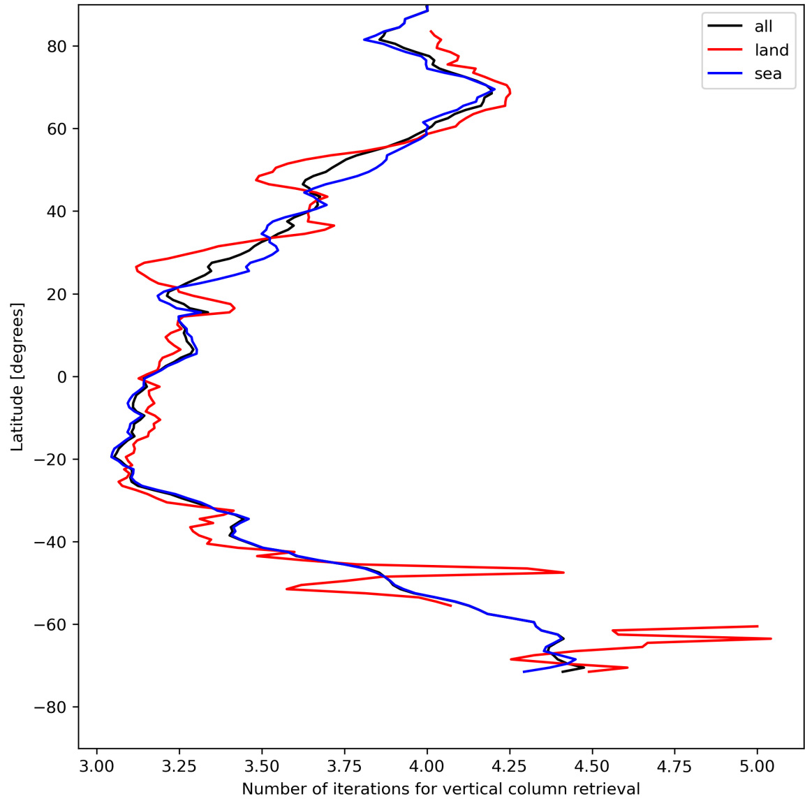
Figure 19: Zonal average of “Number of iterations for vertical column retrieval” for 2024-05-07 to 2024-05-09.
