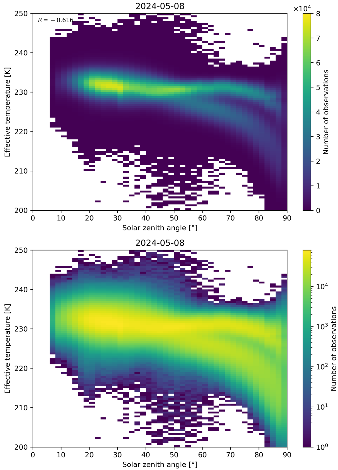
Figure 45: Scatter density plot of “Solar zenith angle” against “Effective temperature” for 2024-05-07 to 2024-05-09.
