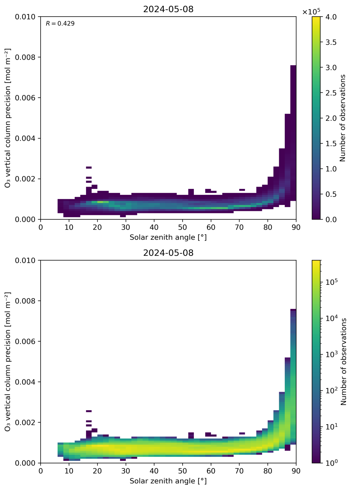
Figure 48: Scatter density plot of “Solar zenith angle” against “O 3 vertical column precision” for 2024-05-07 to 2024-05-09.
