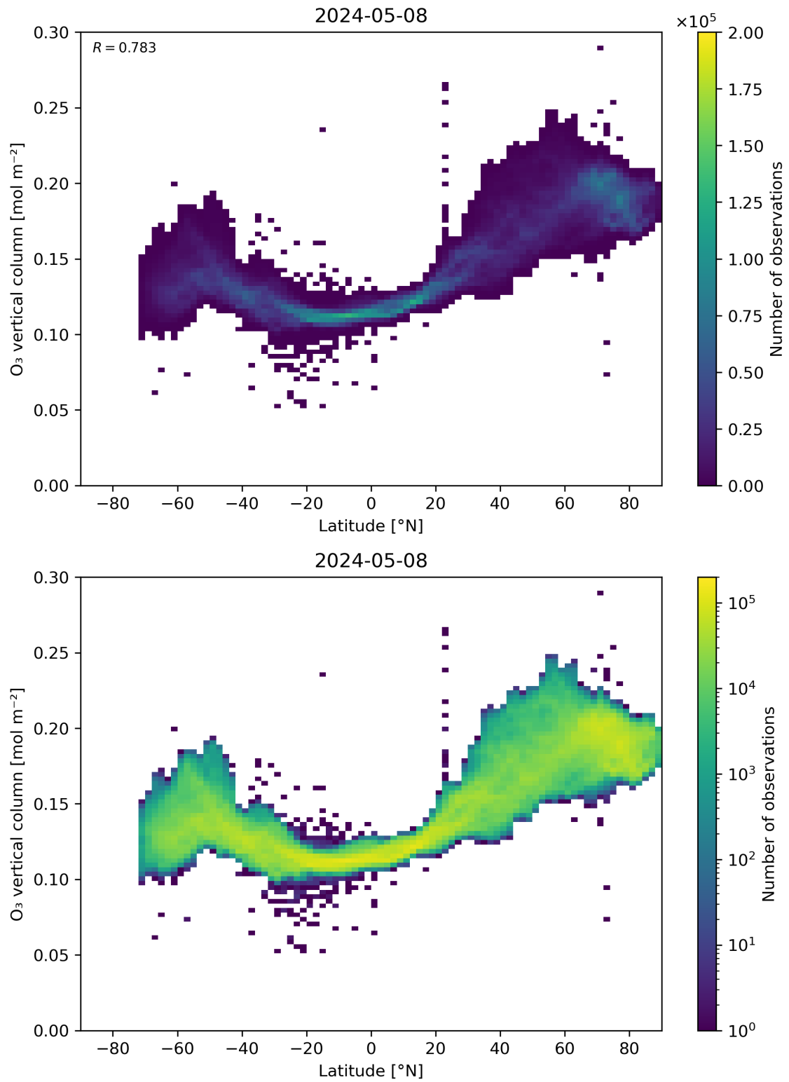
Figure 36: Scatter density plot of “Latitude” against “O 3 vertical column” for 2024-05-07 to 2024-05-09.
