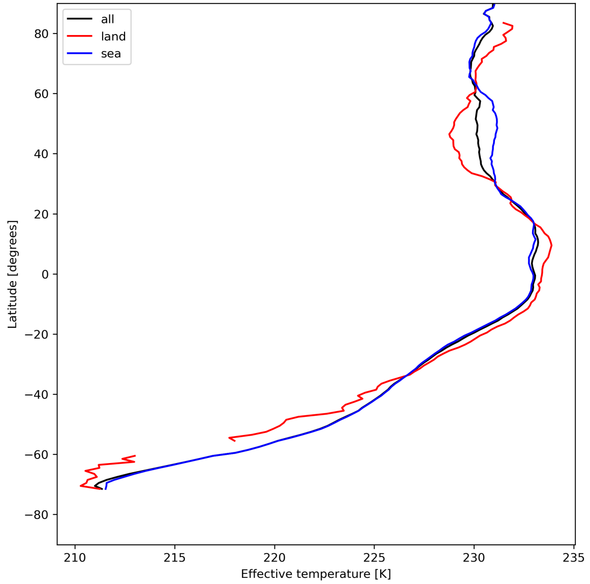
Figure 17: Zonal average of "Effective temperature" for 2024-05-07 to 2024-05-09.
