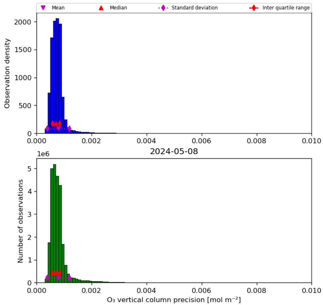
Figure 22: Histogram of “O 3 vertical column precision” for 2024-05-07 to 2024-05-09
