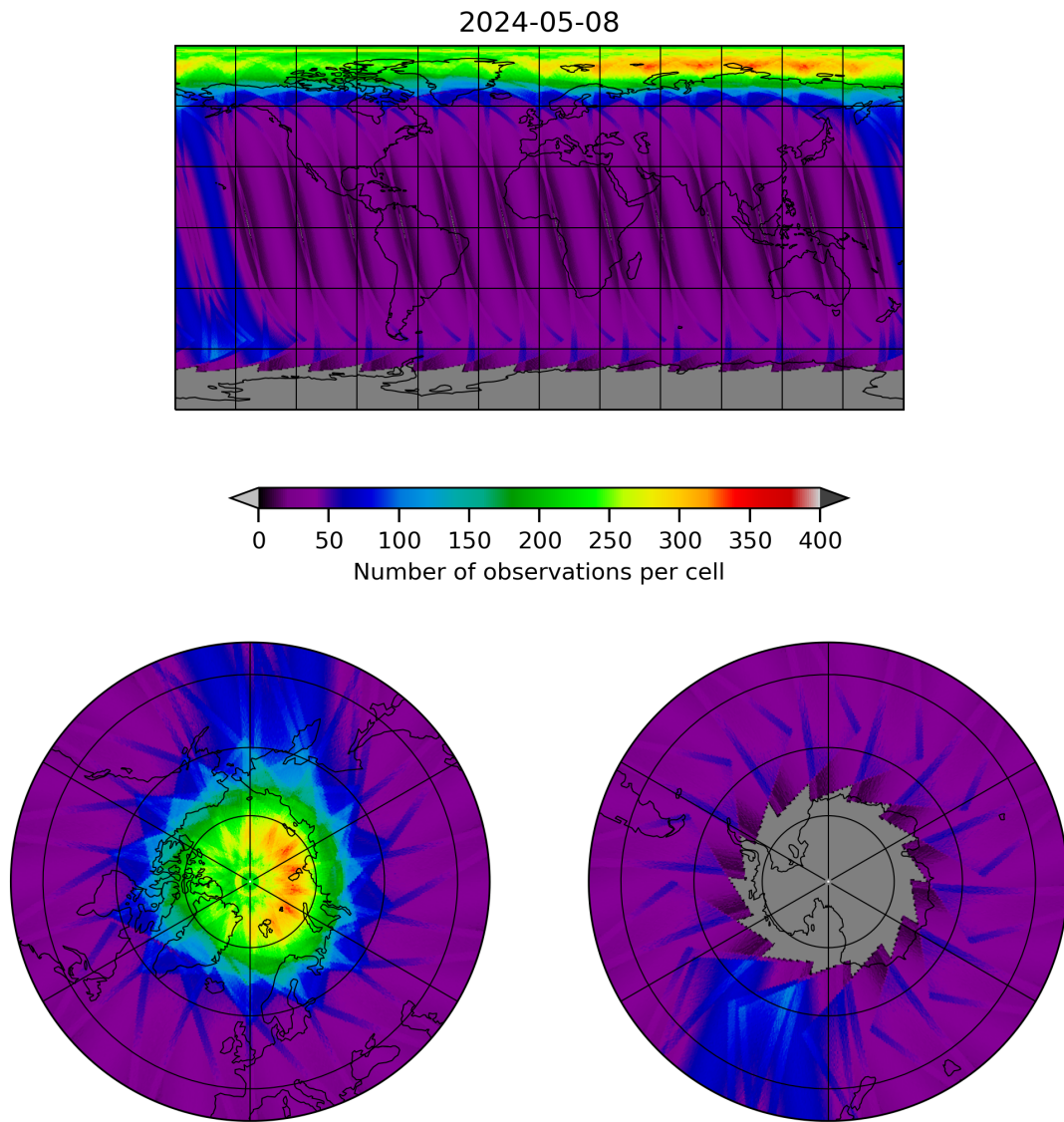
Figure 12: Map of the number of observations for 2024-05-07 to 2024-05-09
