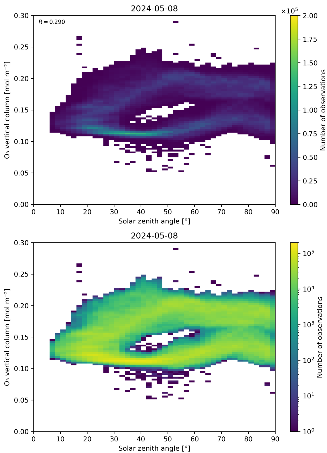
Figure 47: Scatter density plot of “Solar zenith angle” against “O 3 vertical column” for 2024-05-07 to 2024-05-09.
