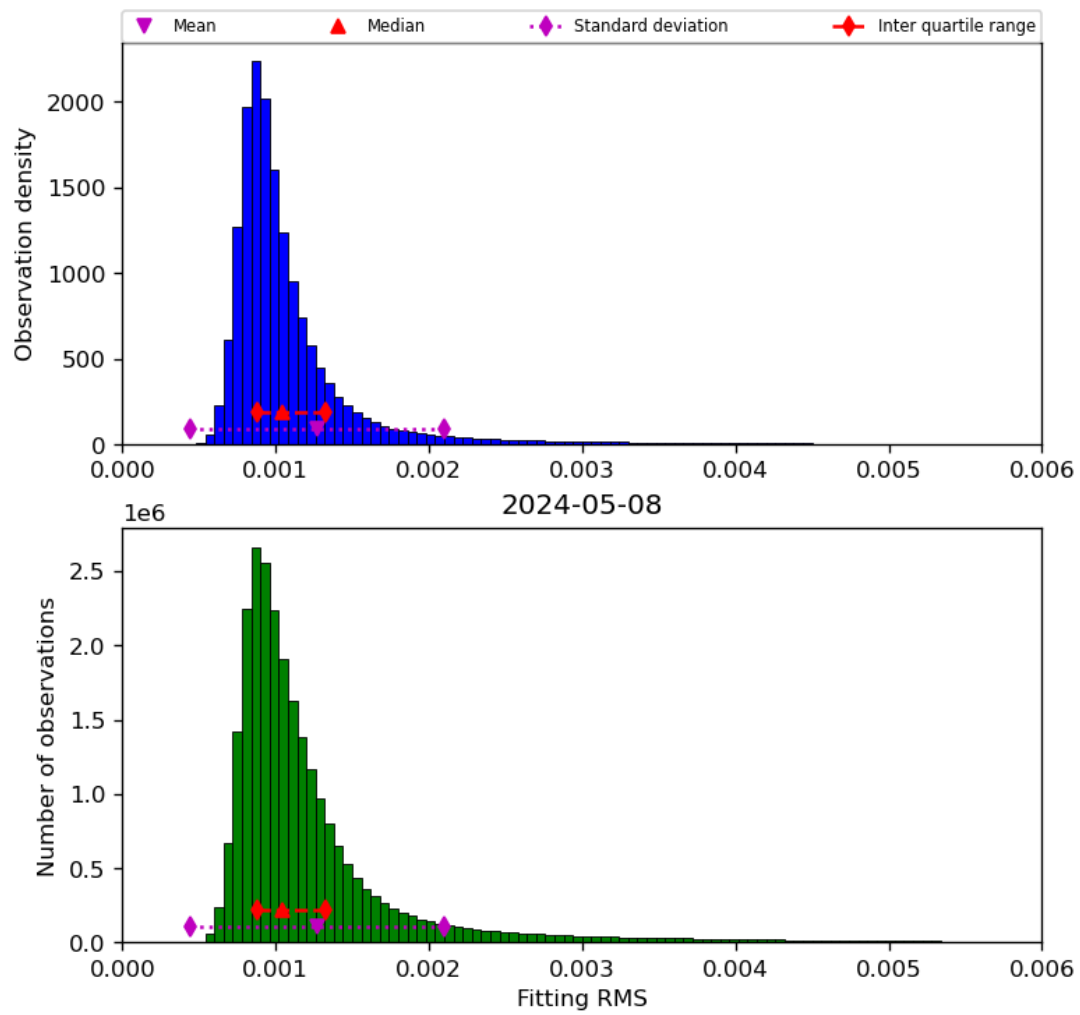
Figure 23: Histogram of “Fitting RMS” for 2024-05-07 to 2024-05-09
