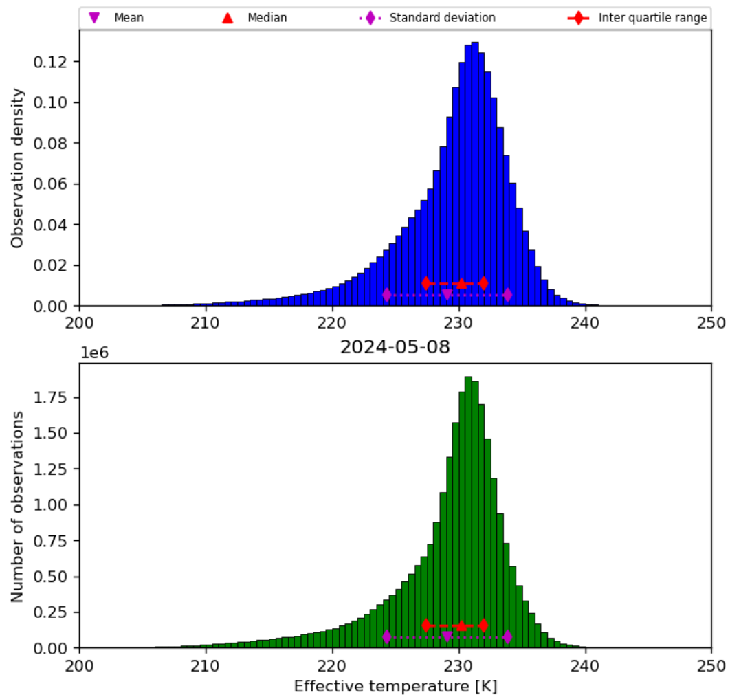
Figure 24: Histogram of “Effective temperature” for 2024-05-07 to 2024-05-09
