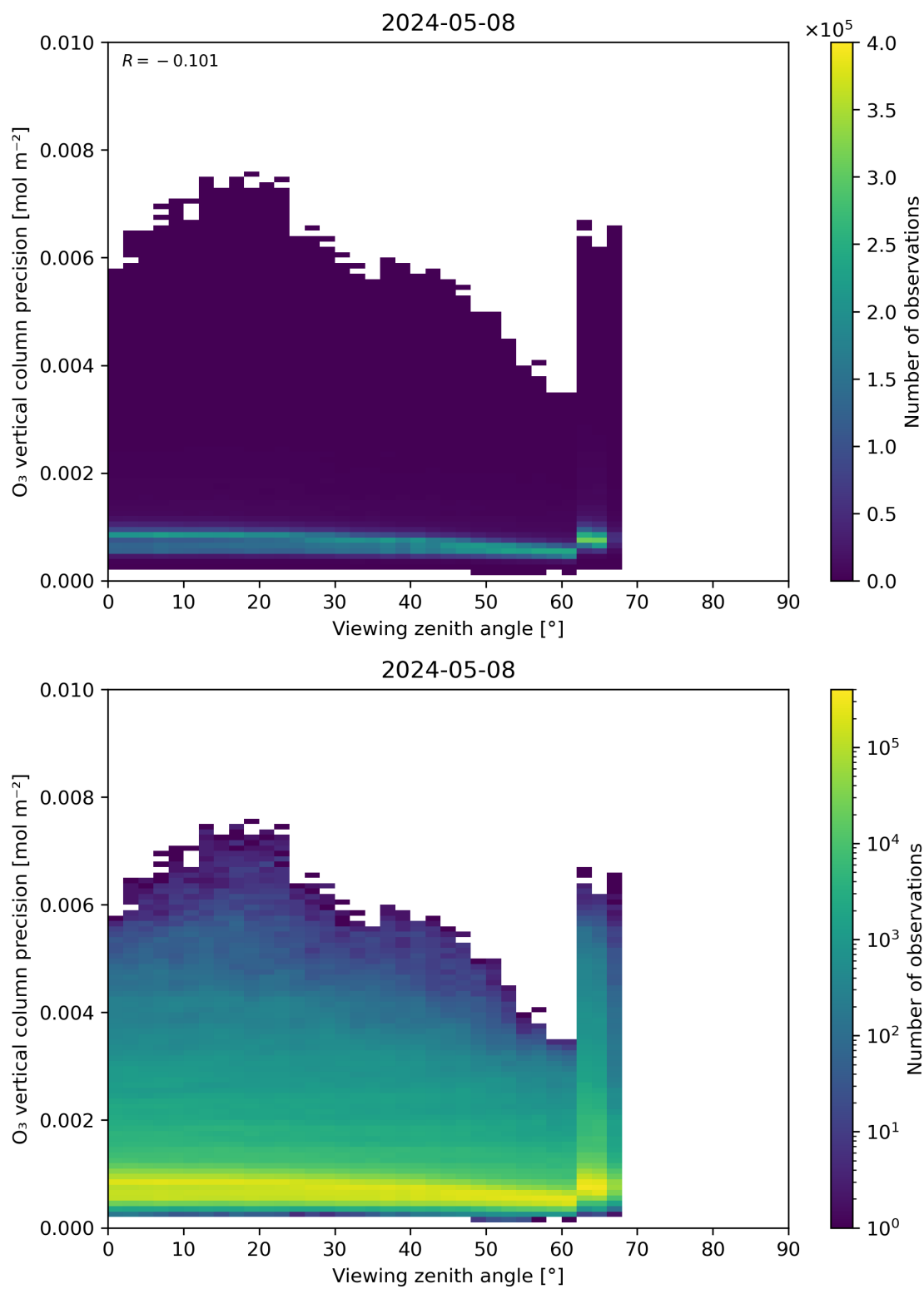
Figure 53: Scatter density plot of “Viewing zenith angle” against “O 3 vertical column precision” for 2024-05-07 to 2024-05-09.
