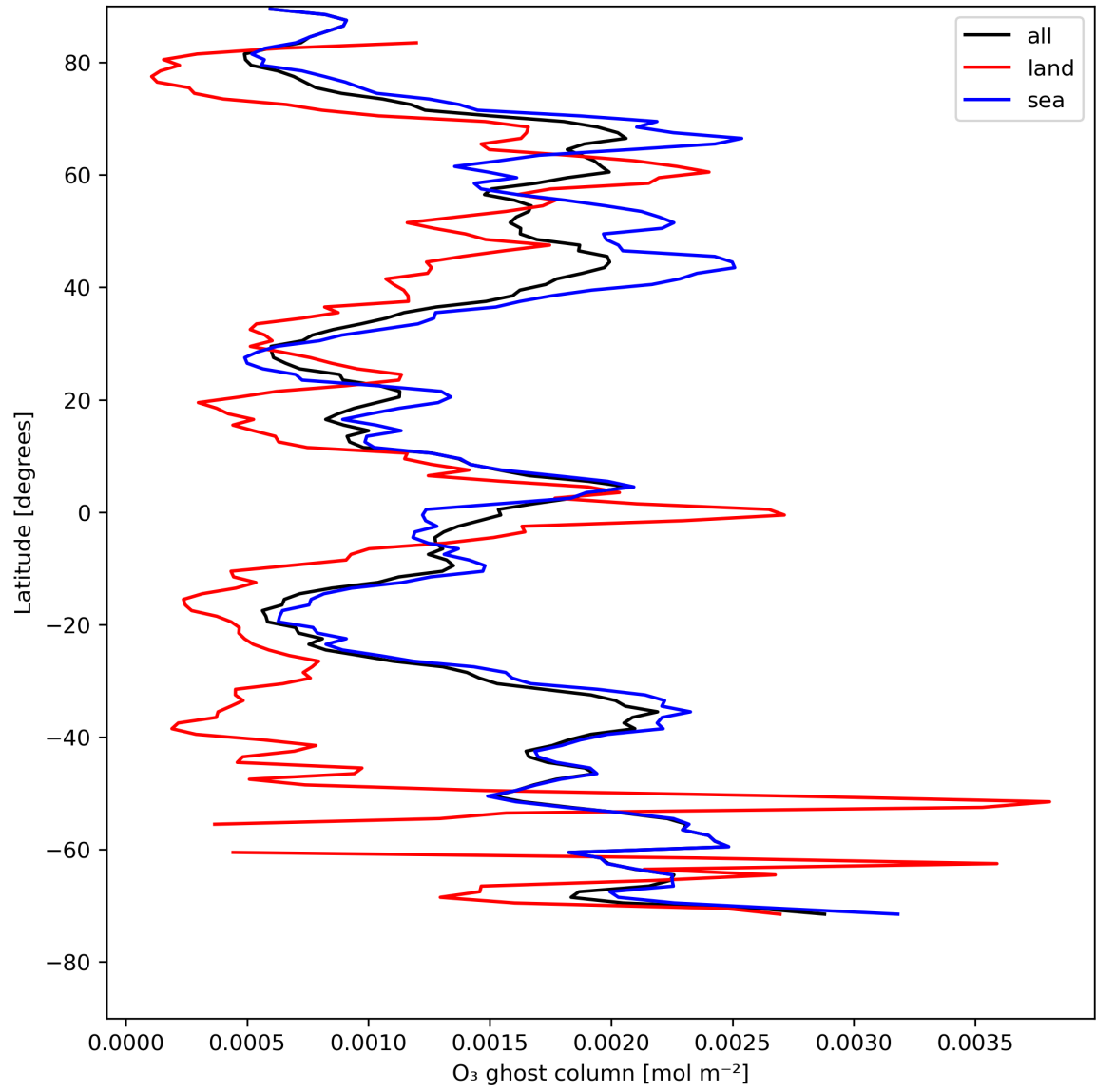
Figure 18: Zonal average of “O 3 ghost column” for 2024-05-07 to 2024-05-09.
