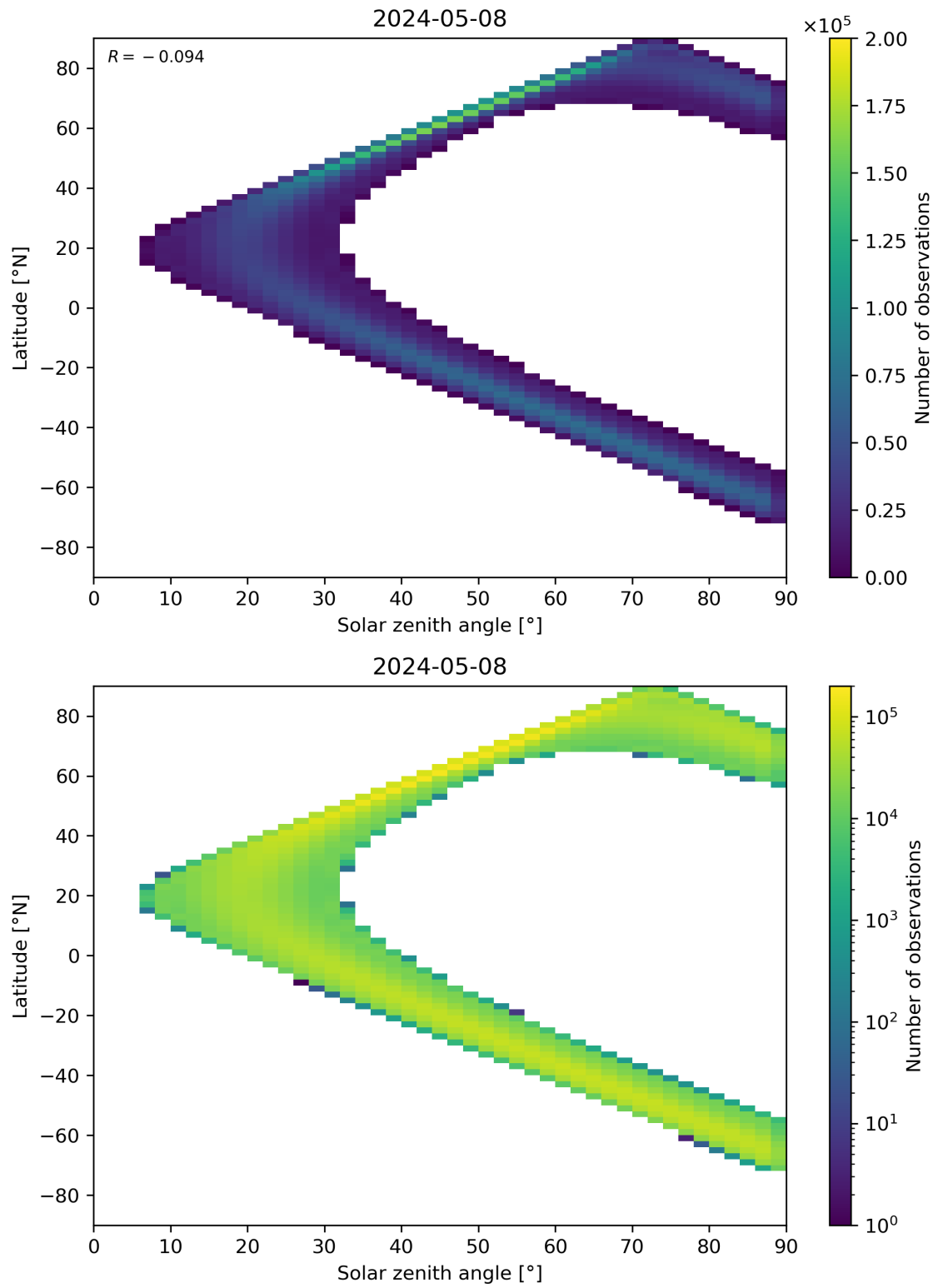
Figure 44: Scatter density plot of “Solar zenith angle” against “Latitude” for 2024-05-07 to 2024-05-09.
