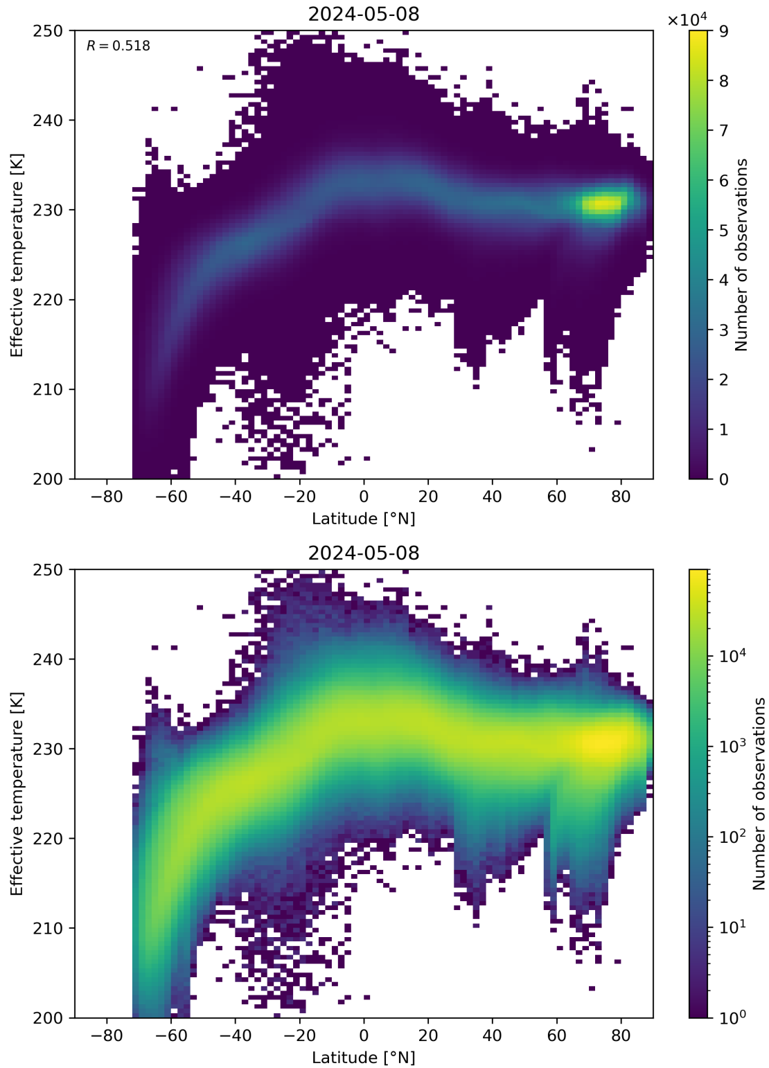
Figure 34: Scatter density plot of “Latitude” against “Effective temperature” for 2024-05-07 to 2024-05-09.
