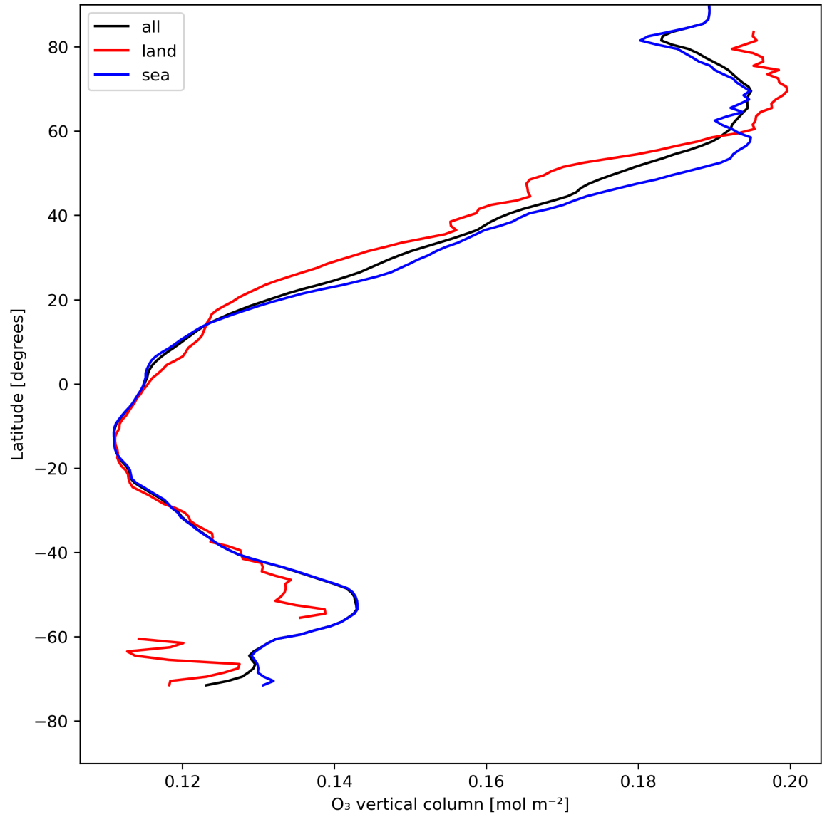
Figure 14: Zonal average of “O 3 vertical column” for 2024-05-07 to 2024-05-09.
