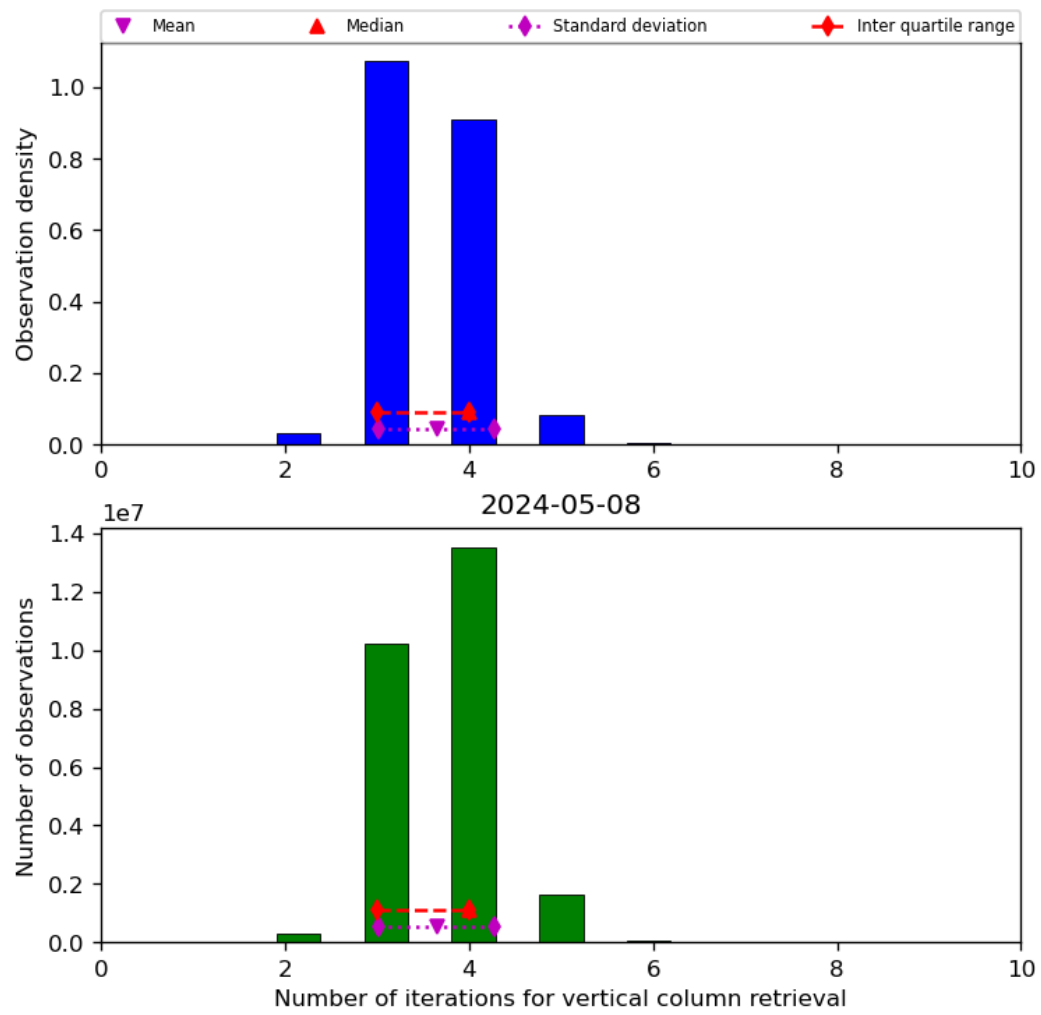
Figure 26: Histogram of “Number of iterations for vertical column retrieval” for 2024-05-07 to 2024-05-09
