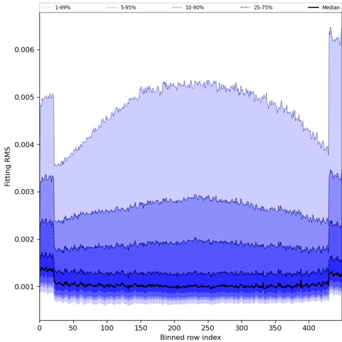
Figure 30: Along track statistics of “Fitting RMS” for 2024-05-07 to 2024-05-09
