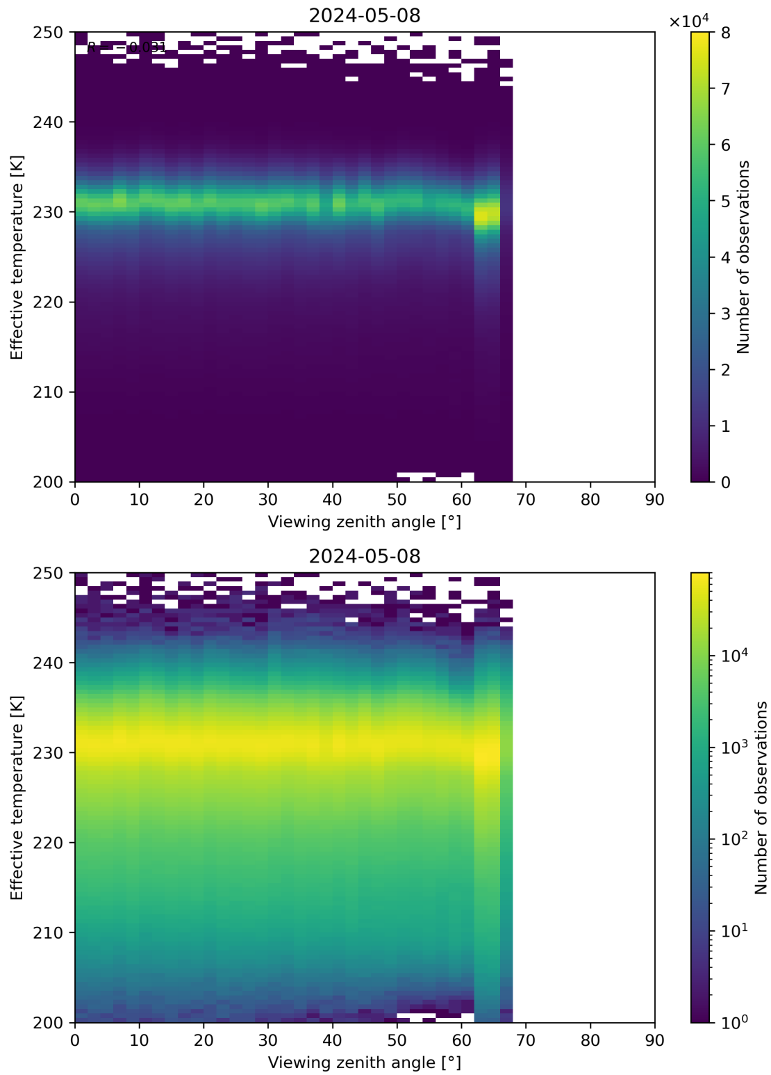
Figure 50: Scatter density plot of “Viewing zenith angle” against “Effective temperature” for 2024-05-07 to 2024-05-09.
