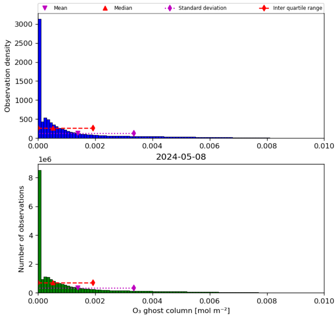
Figure 25: Histogram of “O 3 ghost column” for 2024-05-07 to 2024-05-09
