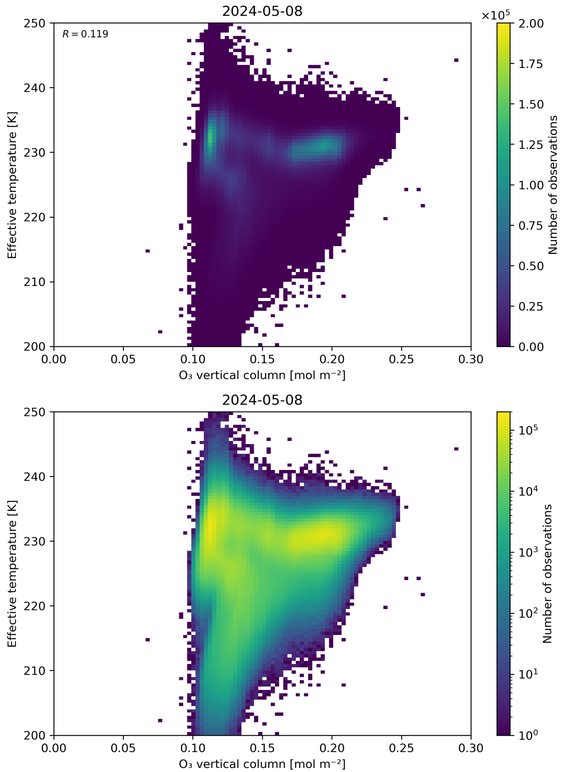
Figure 39: Scatter density plot of “O 3 vertical column” against “Effective temperature” for 2024-05-07 to 2024-05-09.
