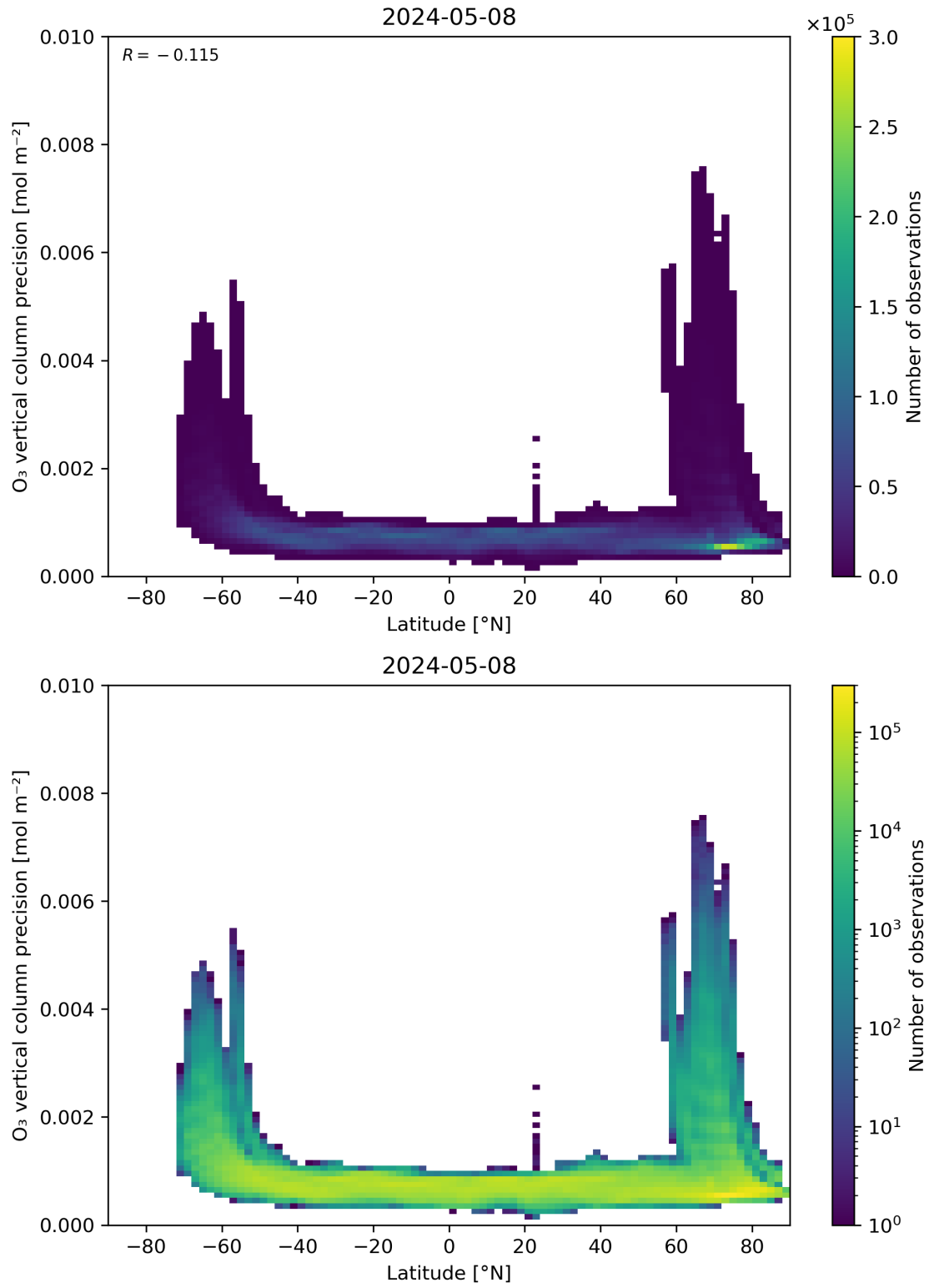
Figure 37: Scatter density plot of “Latitude” against “O 3 vertical column precision” for 2024-05-07 to 2024-05-09.
