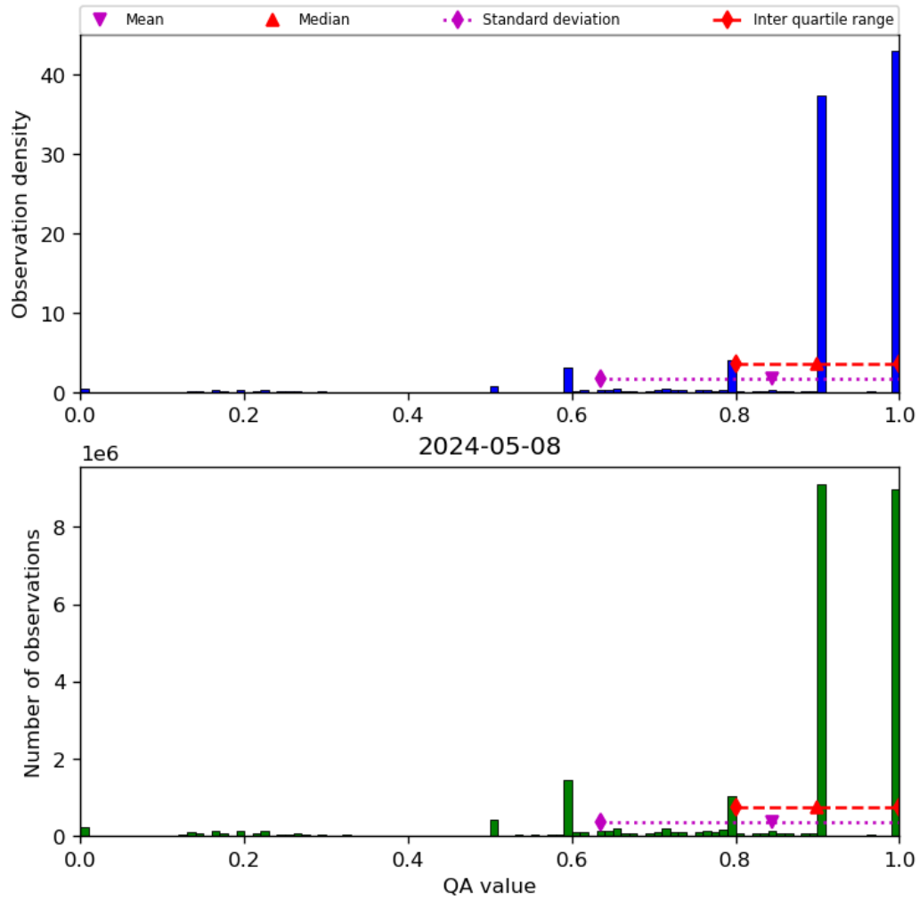
Figure 20: Histogram of “QA value” for 2024-05-07 to 2024-05-09
