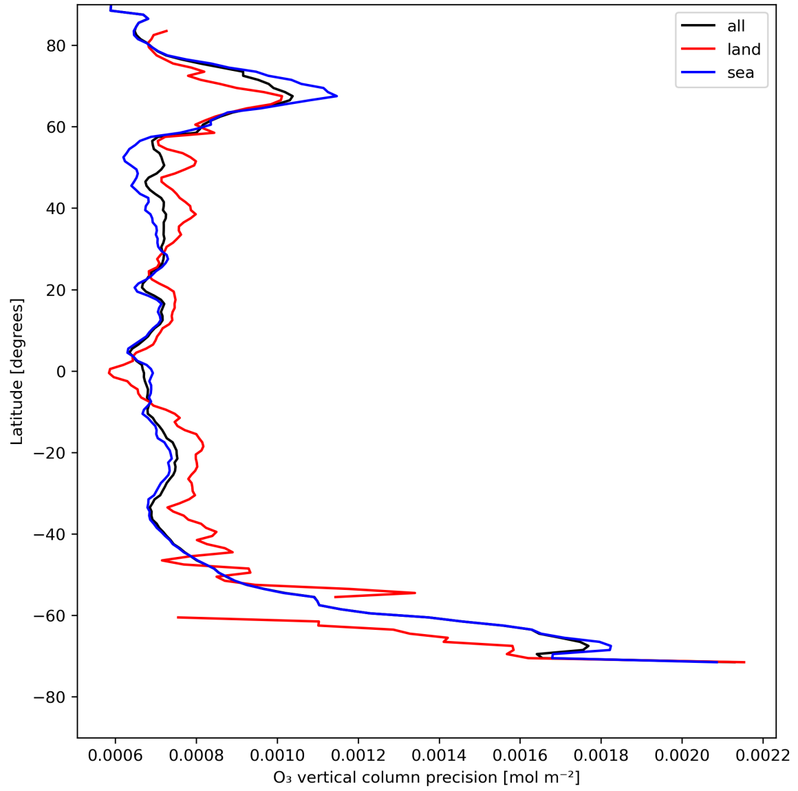
Figure 15: Zonal average of “O 3 vertical column precision” for 2024-05-07 to 2024-05-09.
