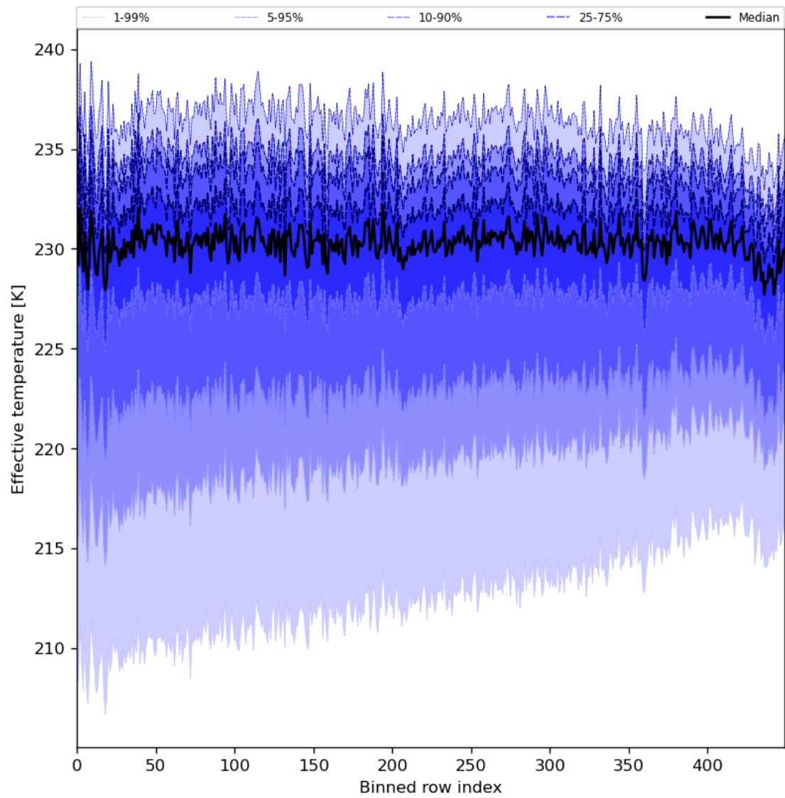
Figure 31: Along track statistics of “Effective temperature” for 2024-05-07 to 2024-05-09
