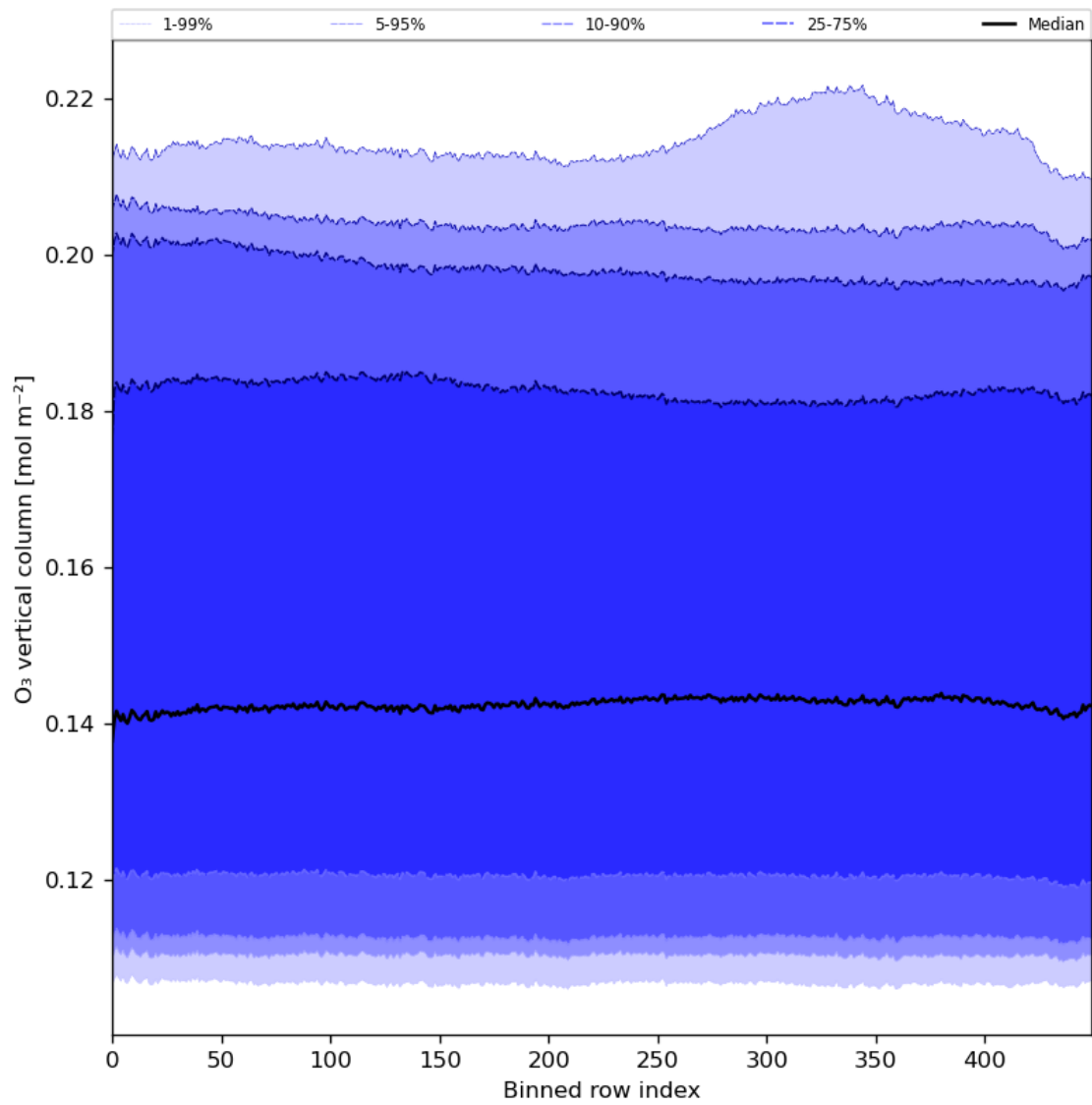
Figure 28: Along track statistics of “O 3 vertical column” for 2024-05-07 to 2024-05-09
