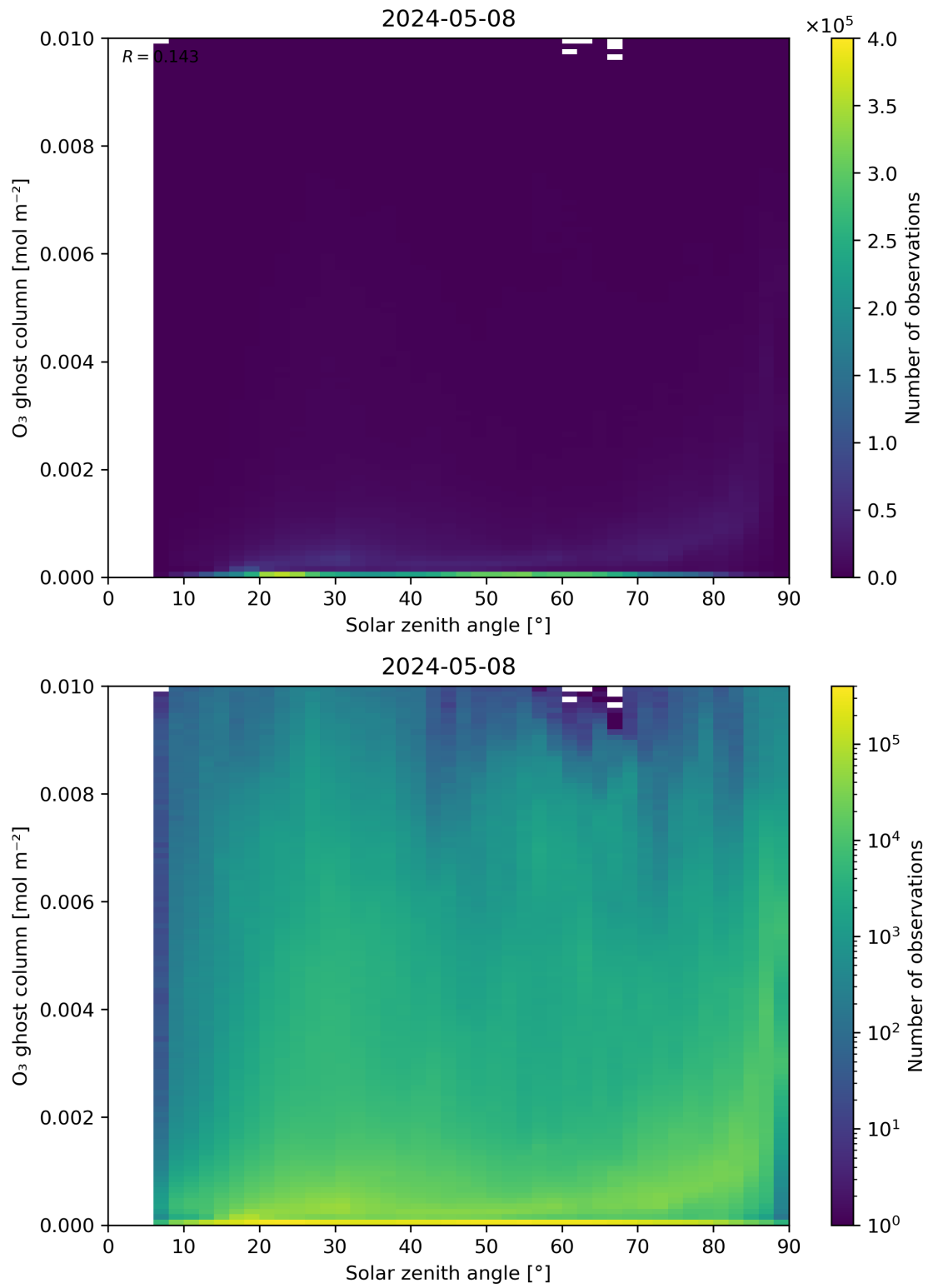
Figure 46: Scatter density plot of “Solar zenith angle” against “O 3 ghost column” for 2024-05-07 to 2024-05-09.
