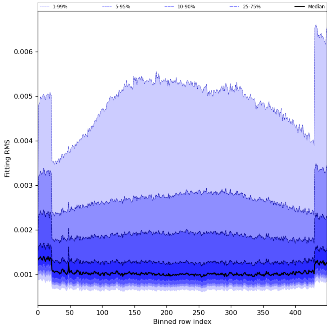
Figure 30: Along track statistics of “Fitting RMS” for 2024-05-09 to 2024-05-11
