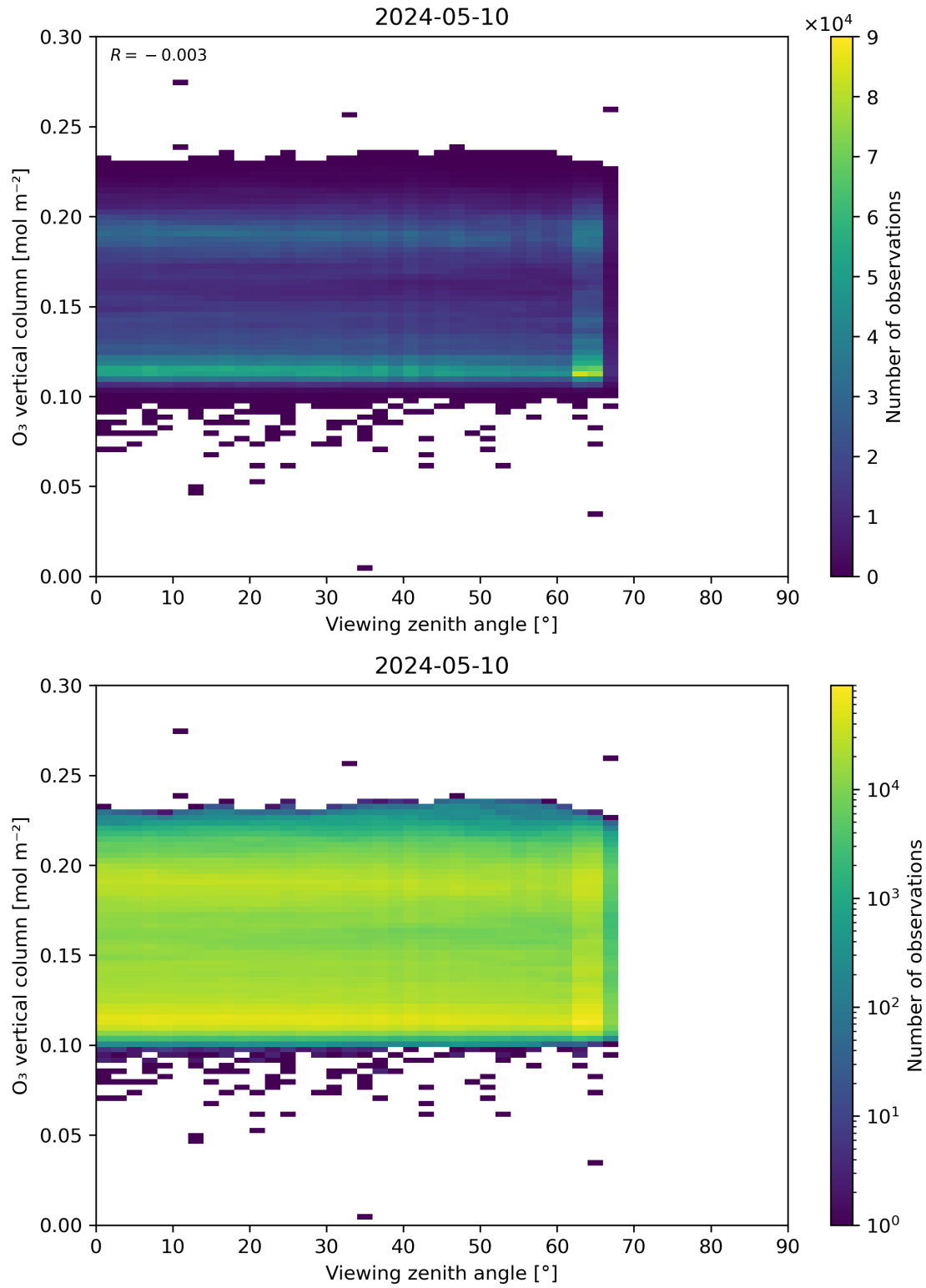
Figure 52: Scatter density plot of “Viewing zenith angle” against “O 3 vertical column” for 2024-05-09 to 2024-05-11.
