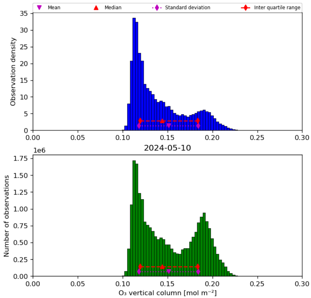
Figure 21: Histogram of “O 3 vertical column” for 2024-05-09 to 2024-05-11
