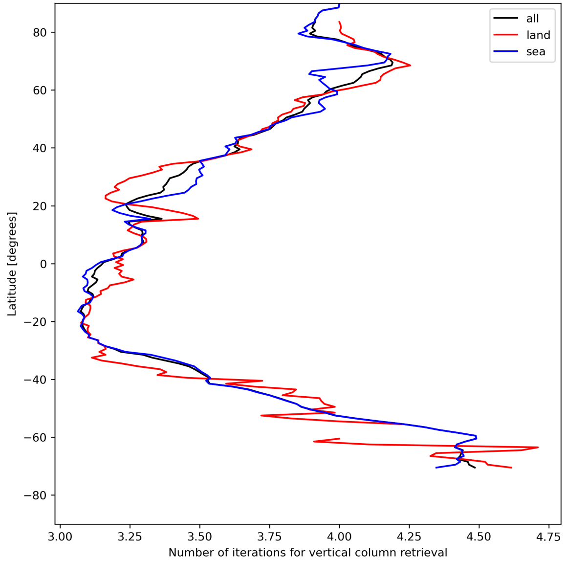
Figure 19: Zonal average of “Number of iterations for vertical column retrieval” for 2024-05-09 to 2024-05-11.
