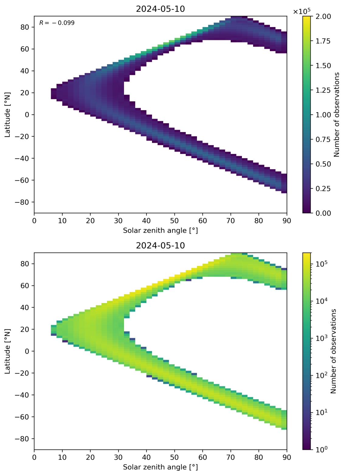
Figure 44: Scatter density plot of “Solar zenith angle” against “Latitude” for 2024-05-09 to 2024-05-11.
