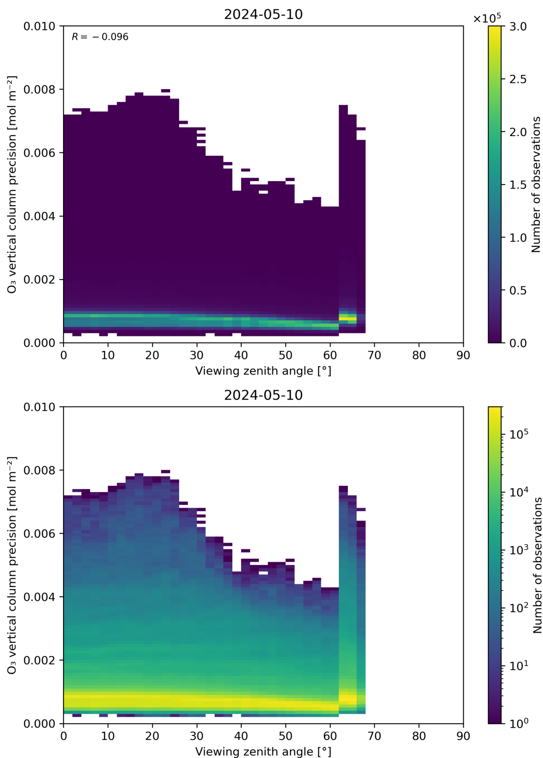
Figure 53: Scatter density plot of “Viewing zenith angle” against “O 3 vertical column precision” for 2024-05-09 to 2024-05-11.
