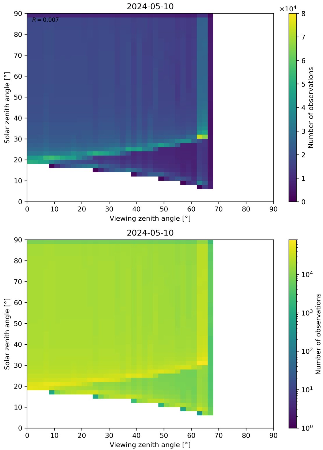
Figure 54: Scatter density plot of “Viewing zenith angle” against “Solar zenith angle” for 2024-05-09 to 2024-05-11.
