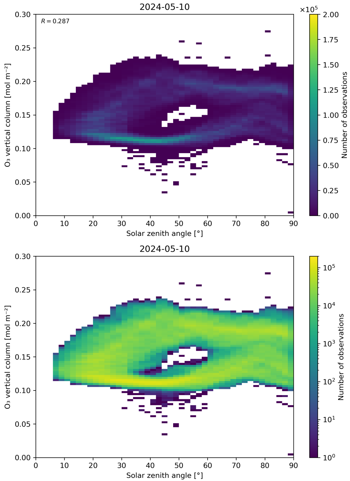
Figure 47: Scatter density plot of “Solar zenith angle” against “O 3 vertical column” for 2024-05-09 to 2024-05-11.
