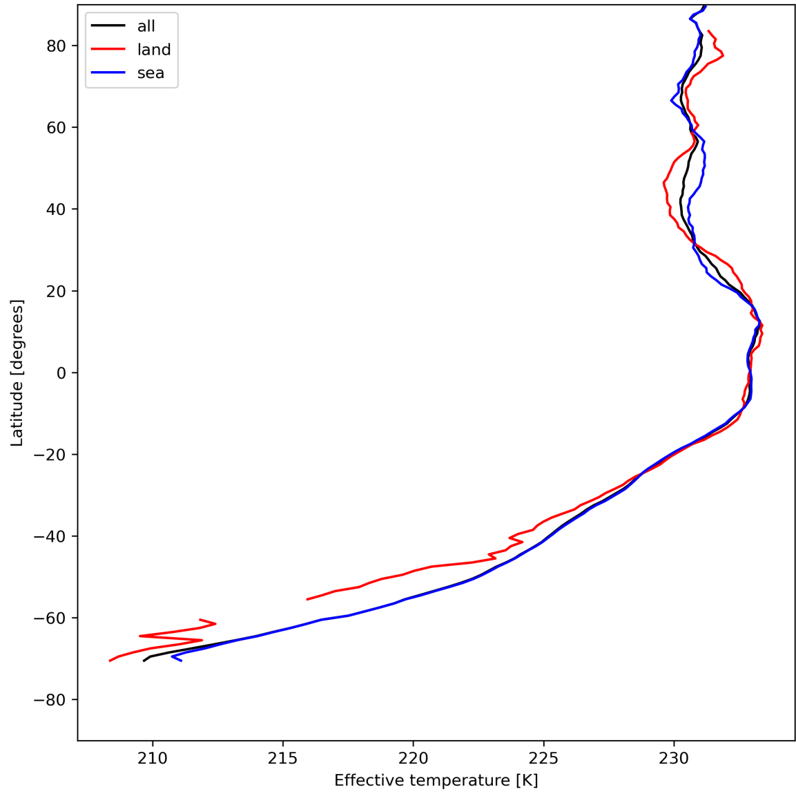
Figure 17: Zonal average of "Effective temperature" for 2024-05-09 to 2024-05-11.
