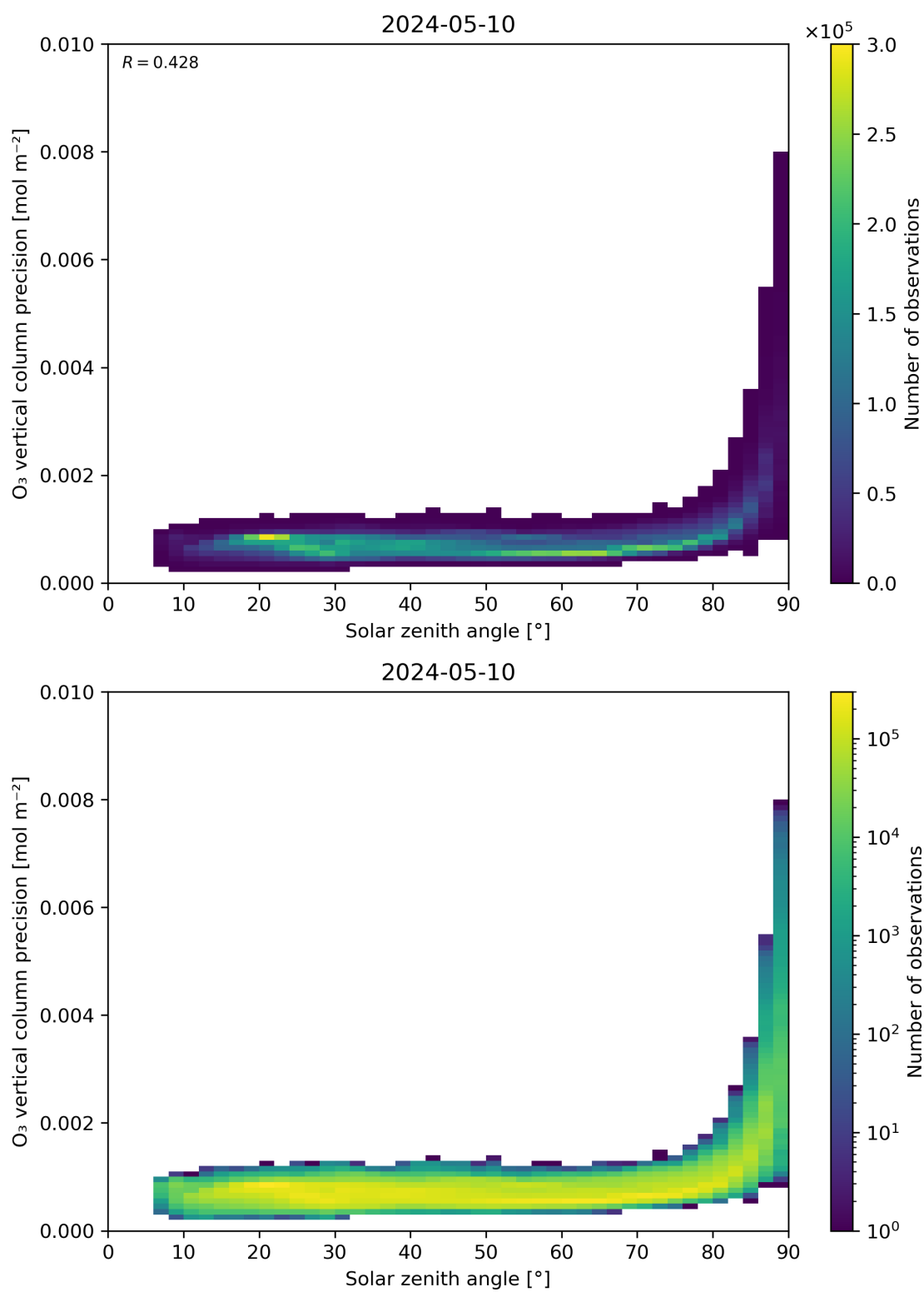
Figure 48: Scatter density plot of “Solar zenith angle” against “O 3 vertical column precision” for 2024-05-09 to 2024-05-11.
