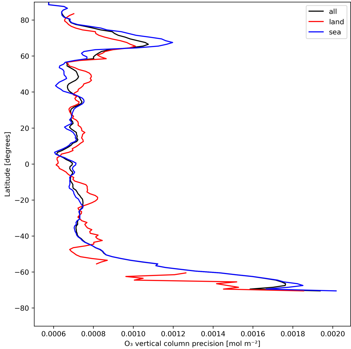
Figure 15: Zonal average of “O 3 vertical column precision” for 2024-05-09 to 2024-05-11.
