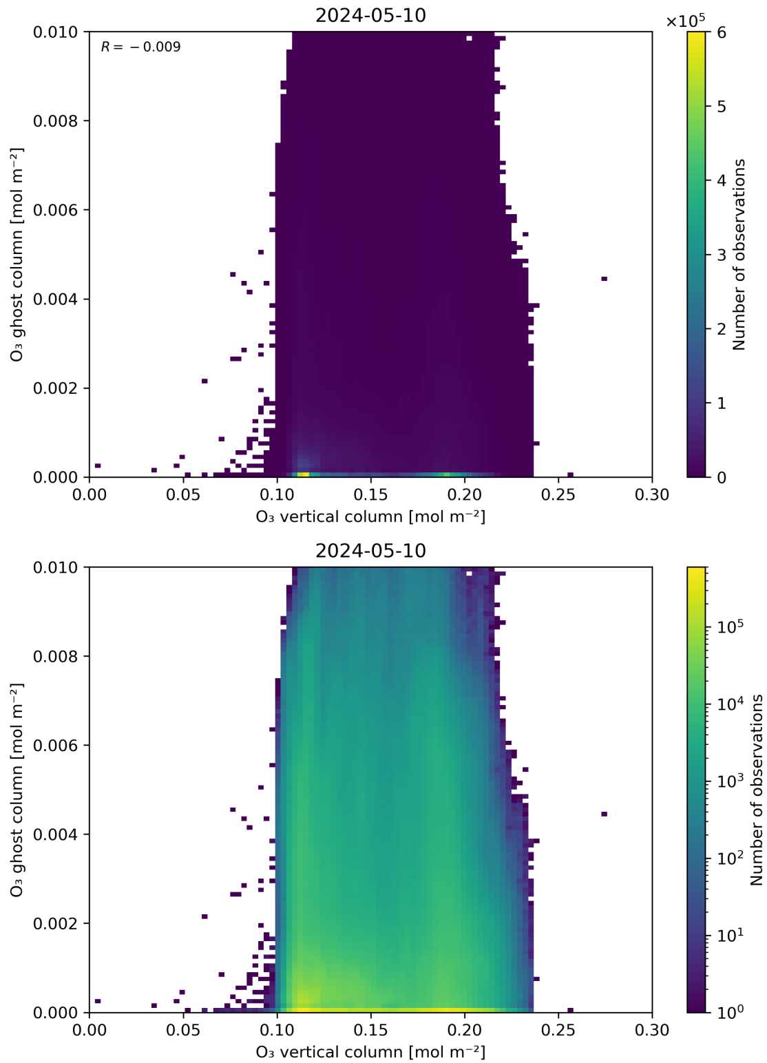
Figure 40: Scatter density plot of “O 3 vertical column” against “O 3 ghost column” for 2024-05-09 to 2024-05-11.
