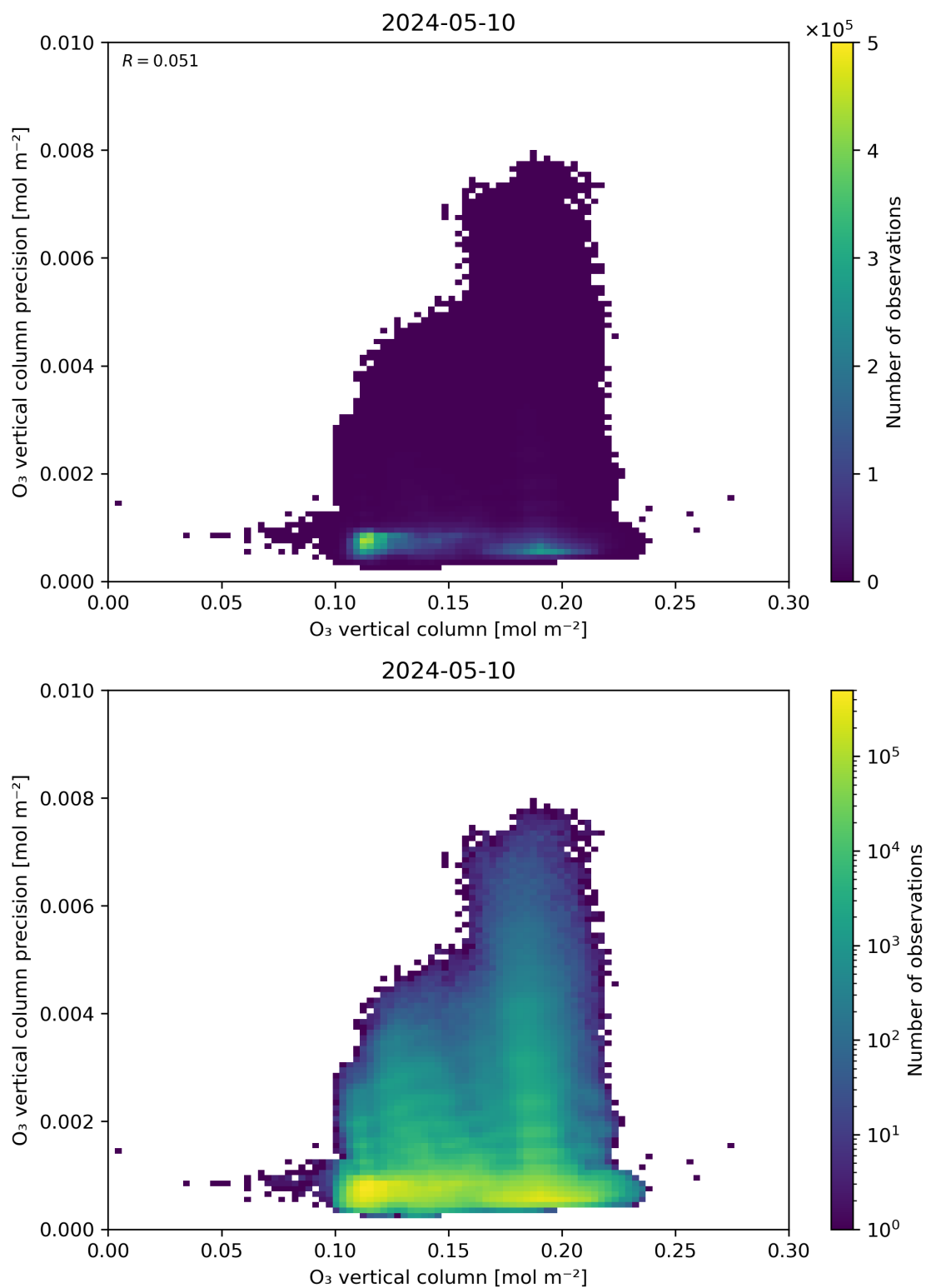
Figure 41: Scatter density plot of “O 3 vertical column” against “O 3 vertical column precision” for 2024-05-09 to 2024-05-11.
