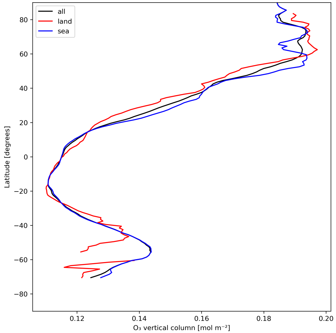
Figure 14: Zonal average of “O 3 vertical column” for 2024-05-09 to 2024-05-11.
