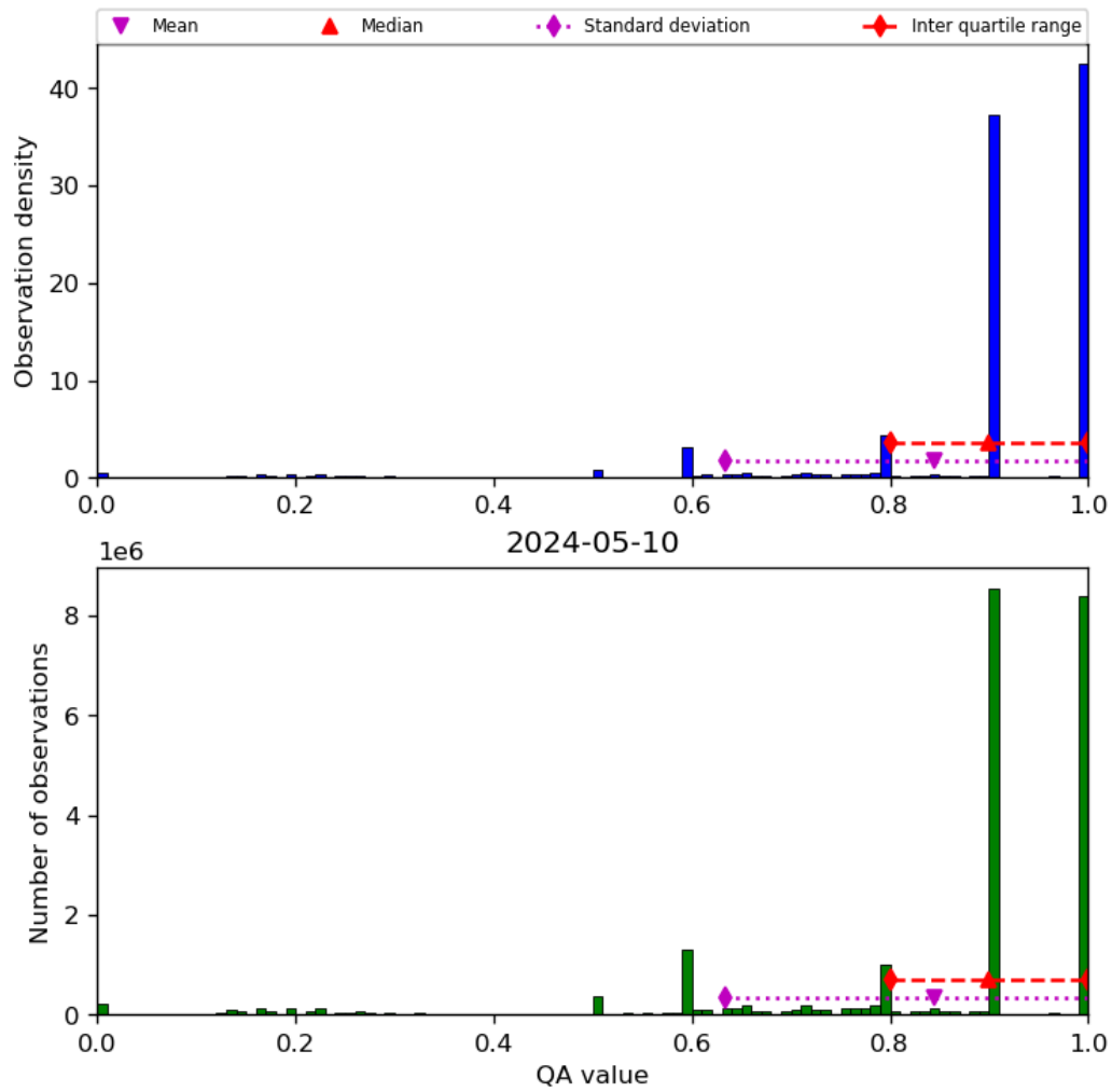
Figure 20: Histogram of “QA value” for 2024-05-09 to 2024-05-11
