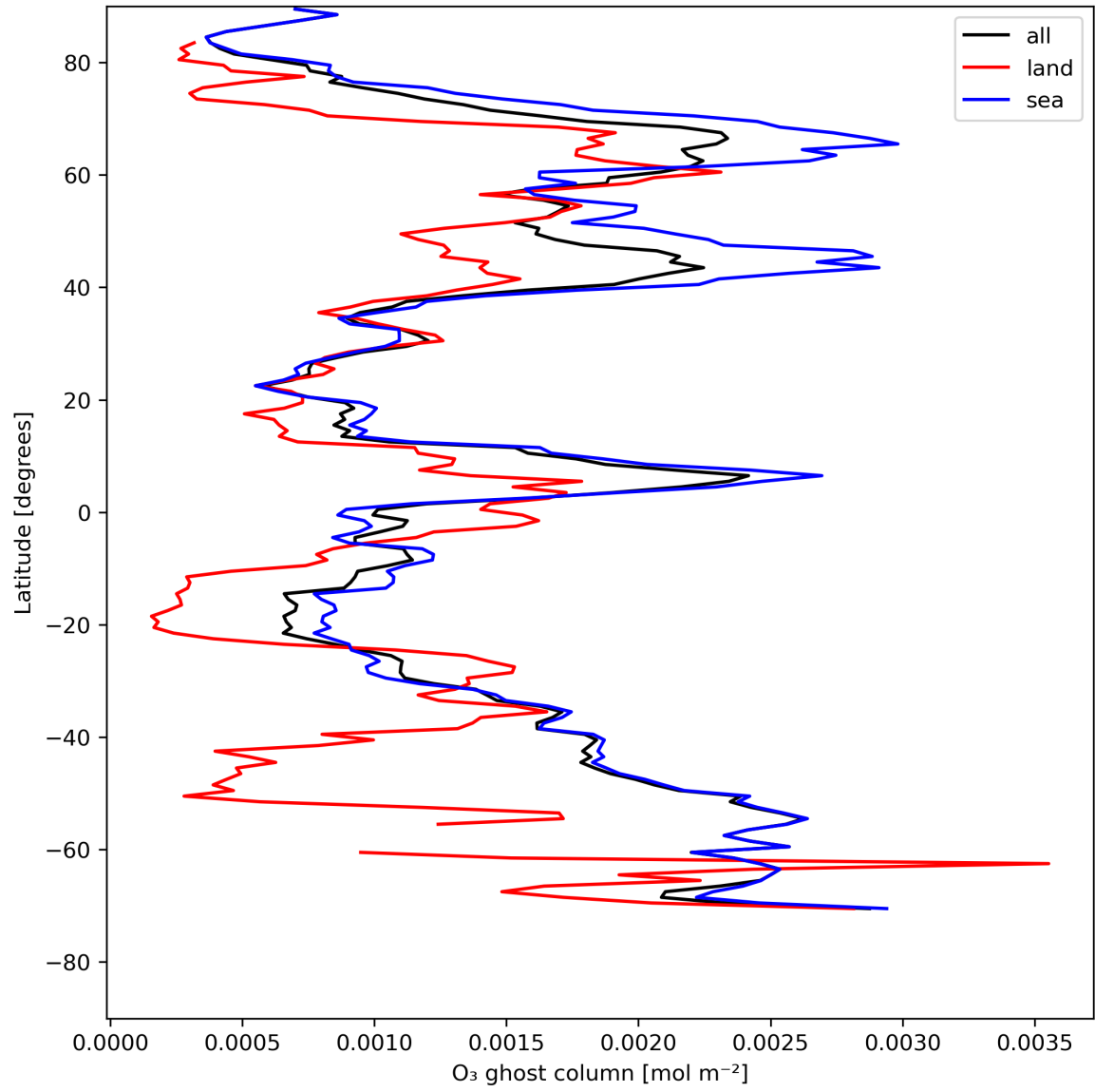
Figure 18: Zonal average of "O 3 ghost column" for 2024-05-09 to 2024-05-11.
