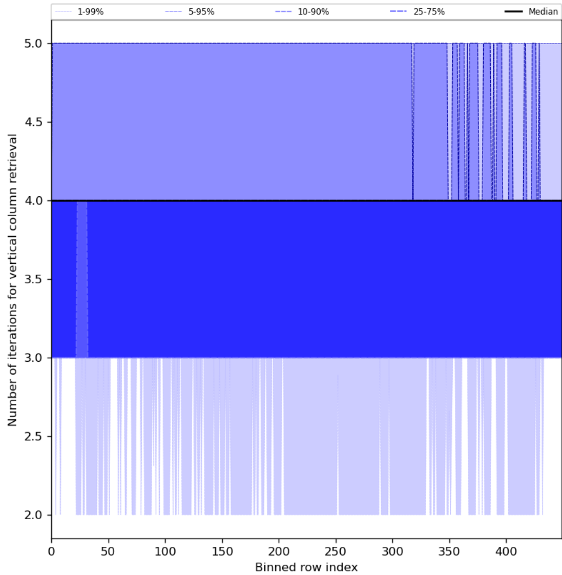
Figure 33: Along track statistics of “Number of iterations for vertical column retrieval” for 2024-05-09 to 2024-05-11
