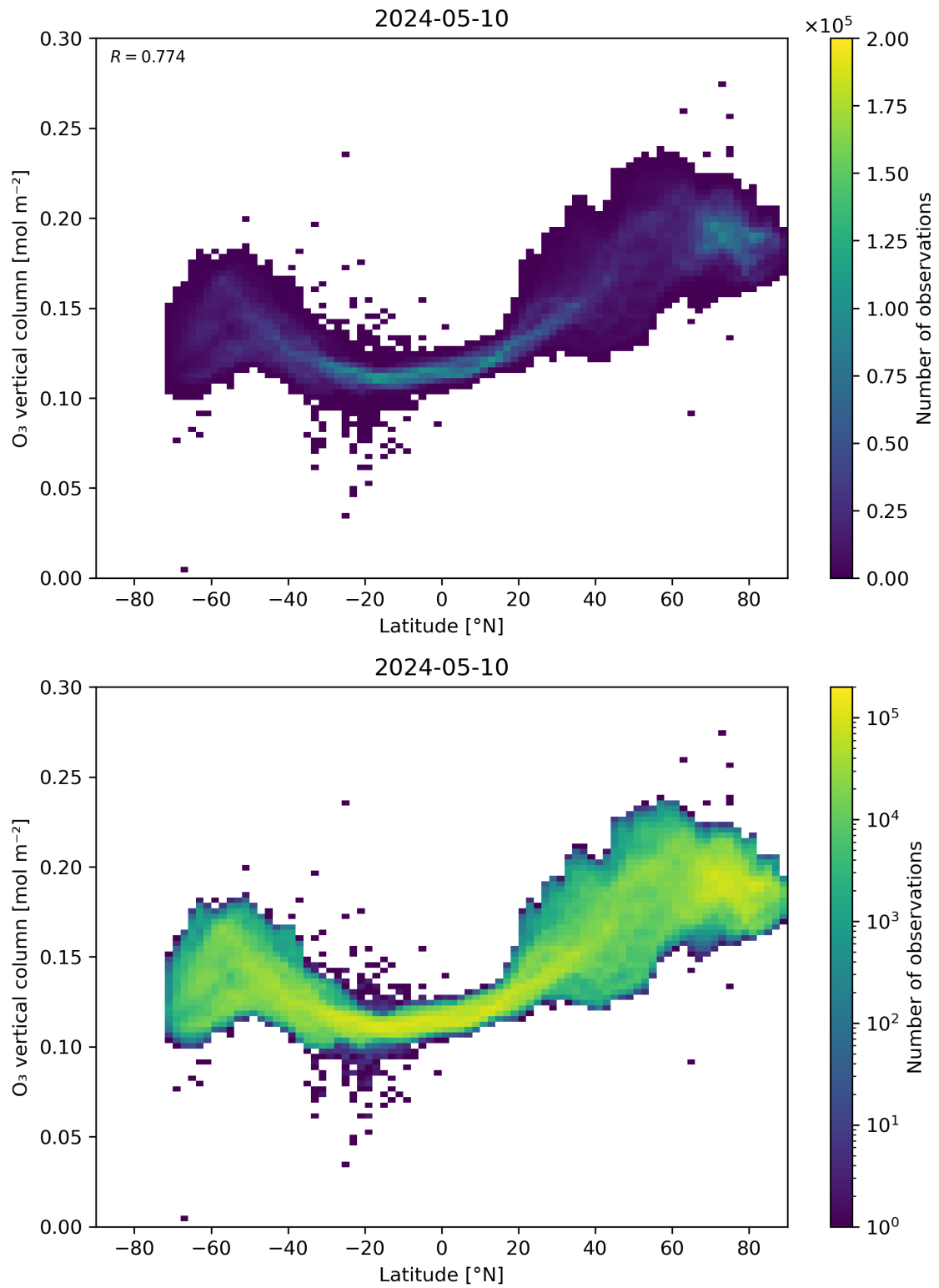
Figure 36: Scatter density plot of “Latitude” against “O 3 vertical column” for 2024-05-09 to 2024-05-11.
