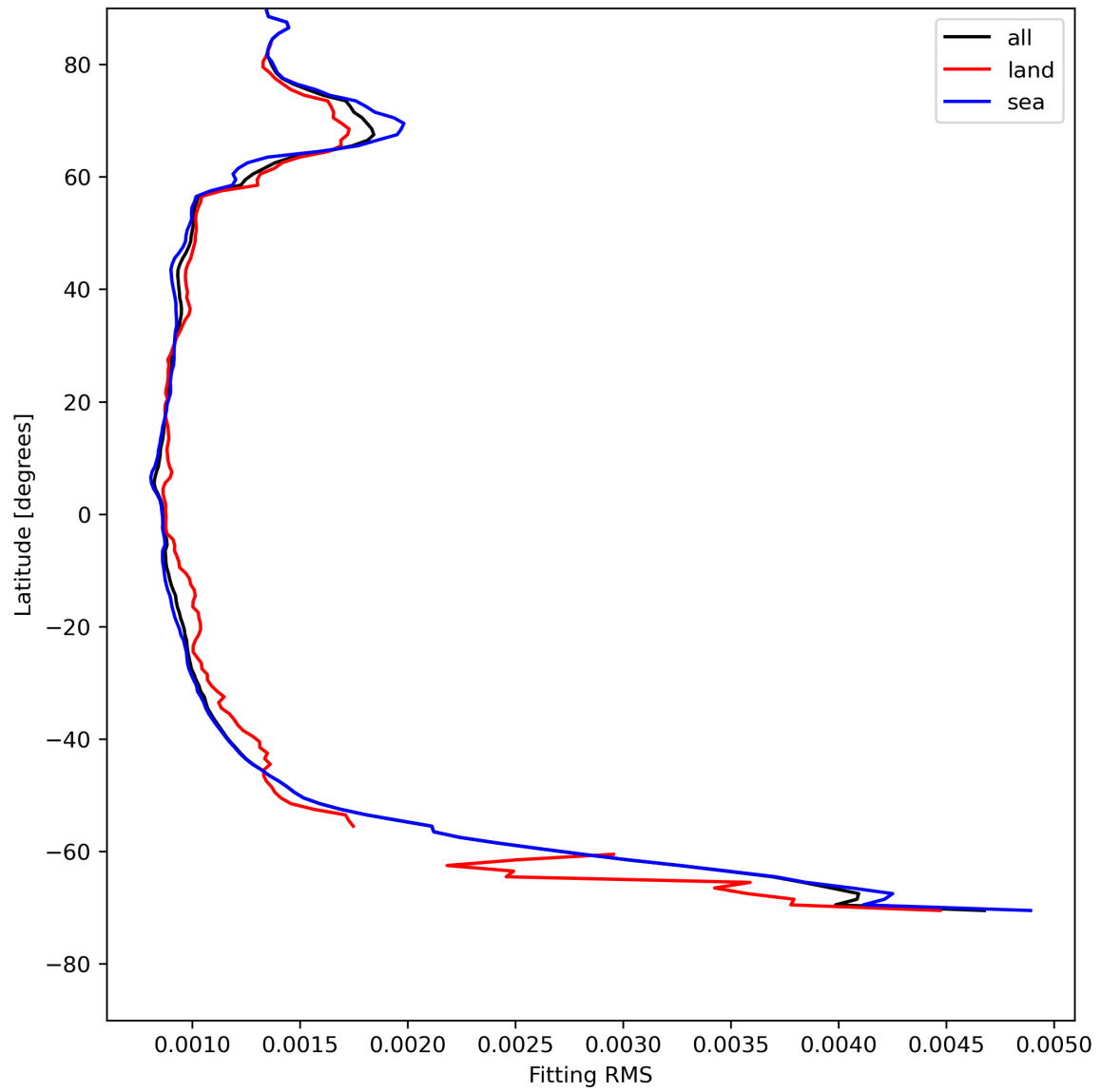
Figure 16: Zonal average of “Fitting RMS” for 2024-05-09 to 2024-05-11.
