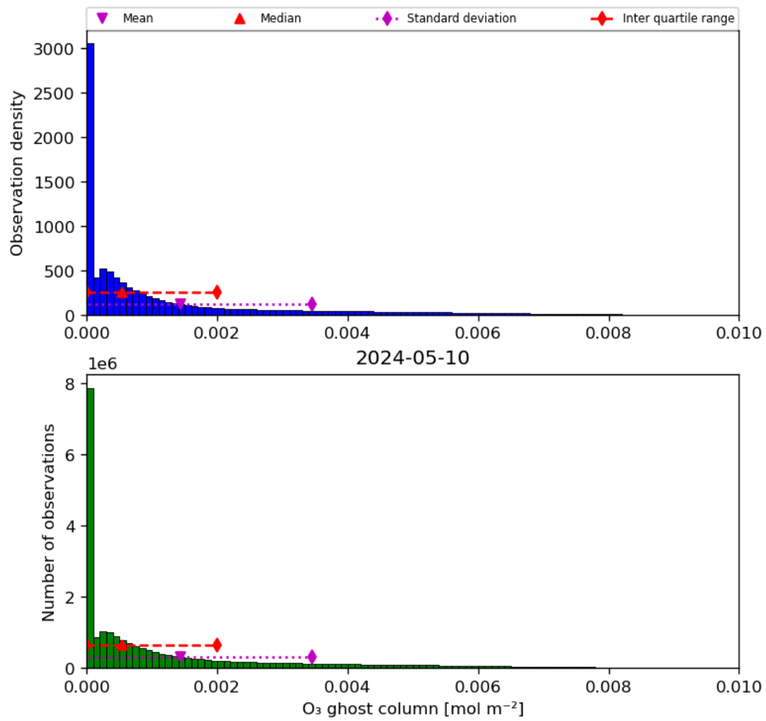
Figure 25: Histogram of “O 3 ghost column” for 2024-05-09 to 2024-05-11
