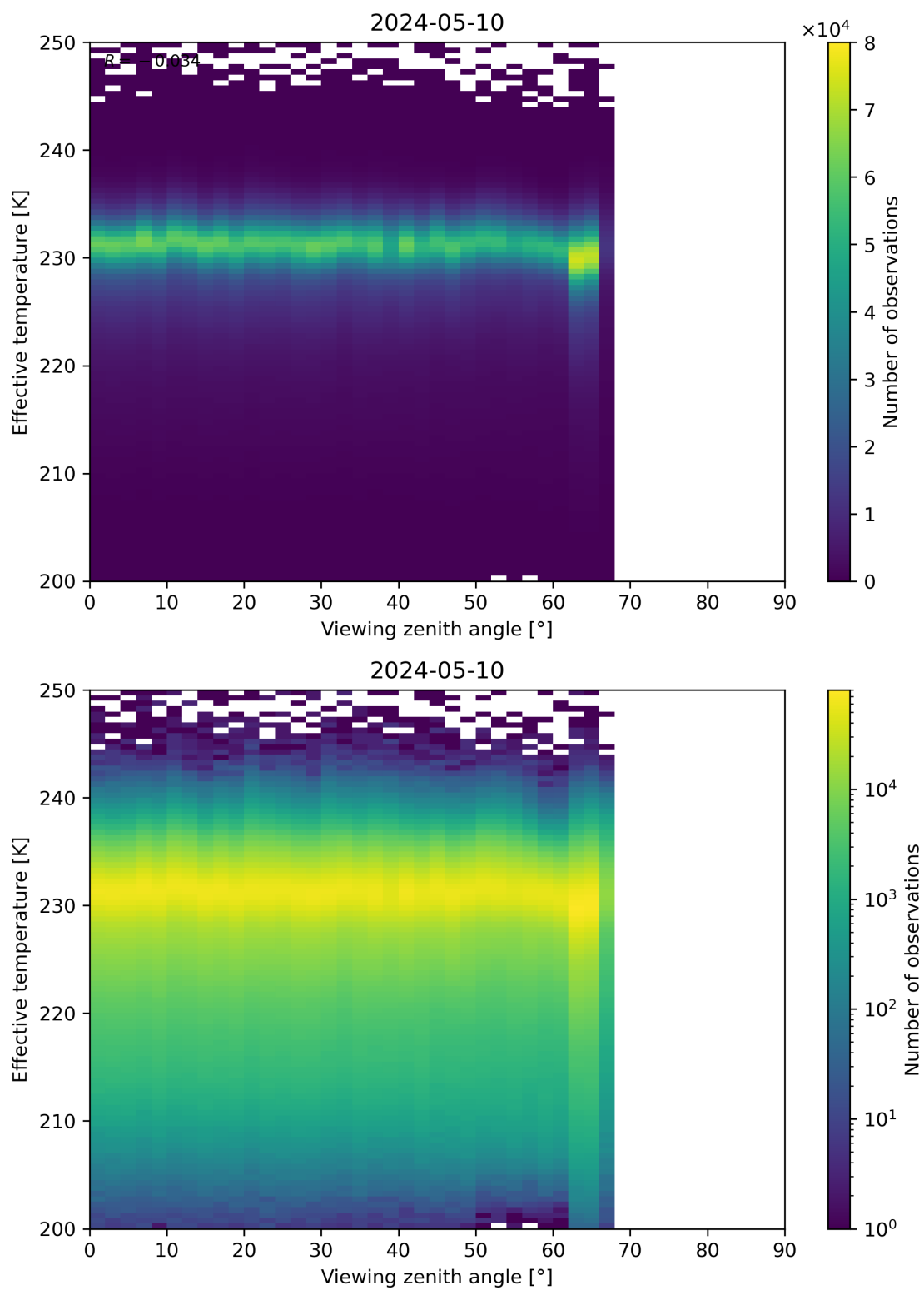
Figure 50: Scatter density plot of “Viewing zenith angle” against “Effective temperature” for 2024-05-09 to 2024-05-11.
