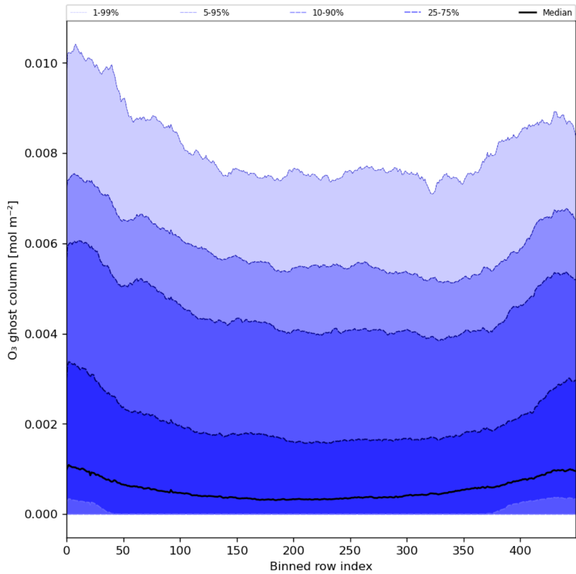
Figure 32: Along track statistics of “O 3 ghost column” for 2024-05-09 to 2024-05-11
