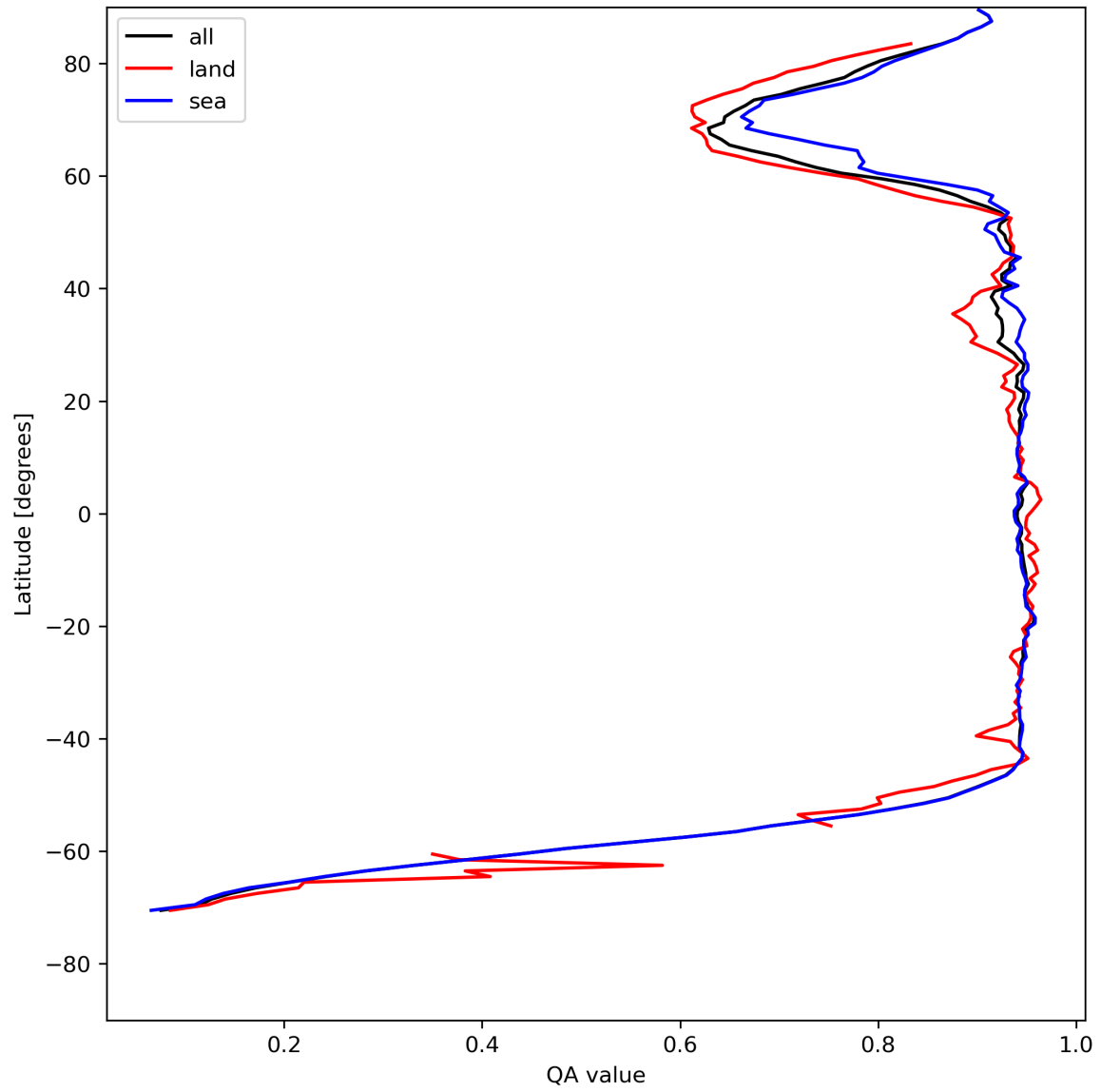
Figure 13: Zonal average of “QA value” for 2024-05-09 to 2024-05-11.
