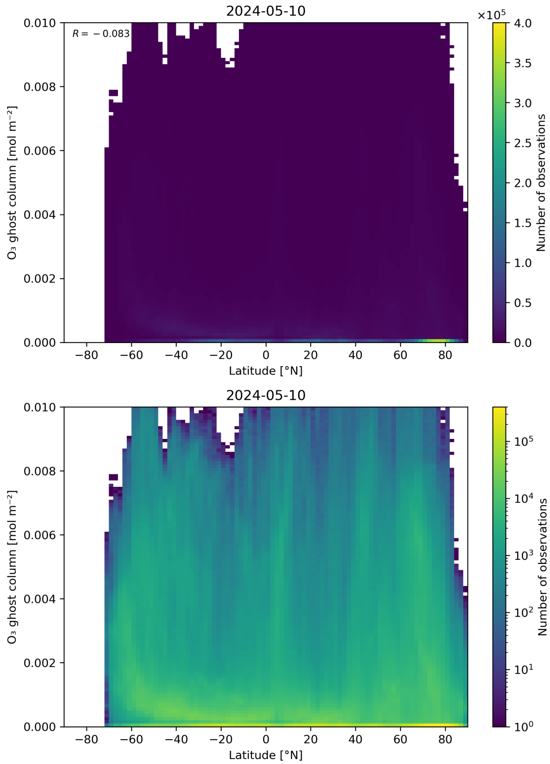
Figure 35: Scatter density plot of “Latitude” against “O 3 ghost column” for 2024-05-09 to 2024-05-11.
