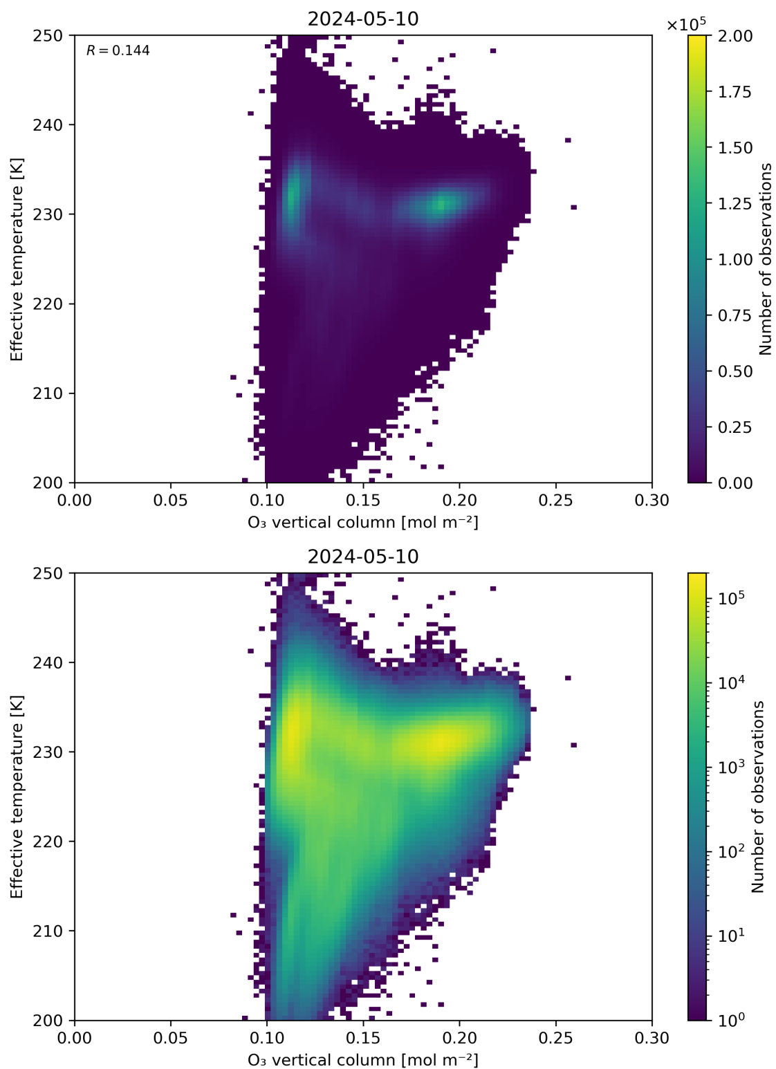
Figure 39: Scatter density plot of “O 3 vertical column” against “Effective temperature” for 2024-05-09 to 2024-05-11.
