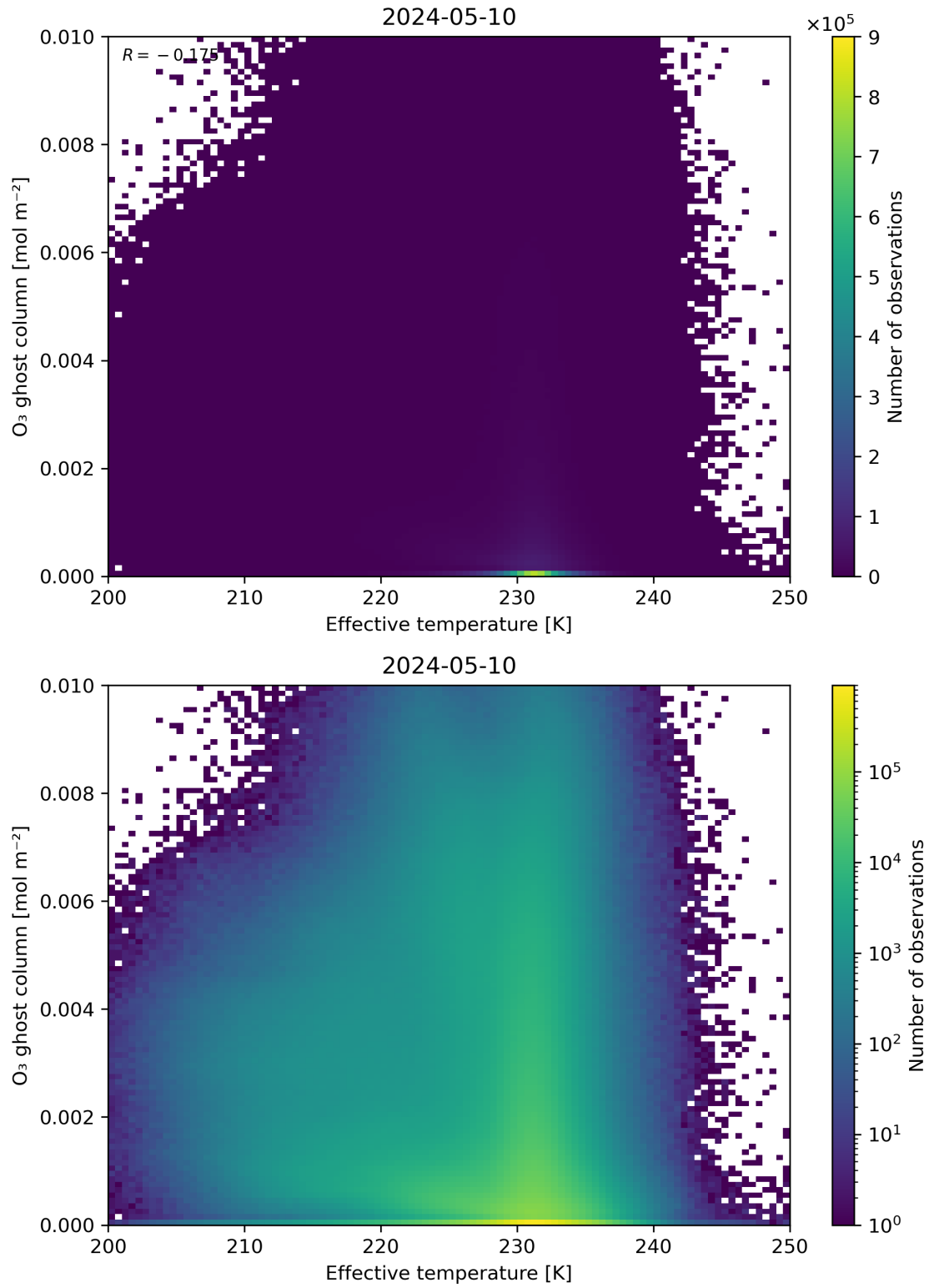
Figure 38: Scatter density plot of “Effective temperature” against “O 3 ghost column” for 2024-05-09 to 2024-05-11.
