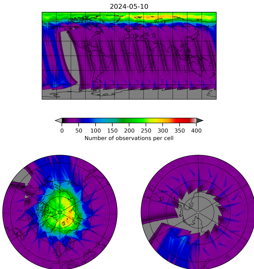
Figure 12: Map of the number of observations for 2024-05-09 to 2024-05-11
