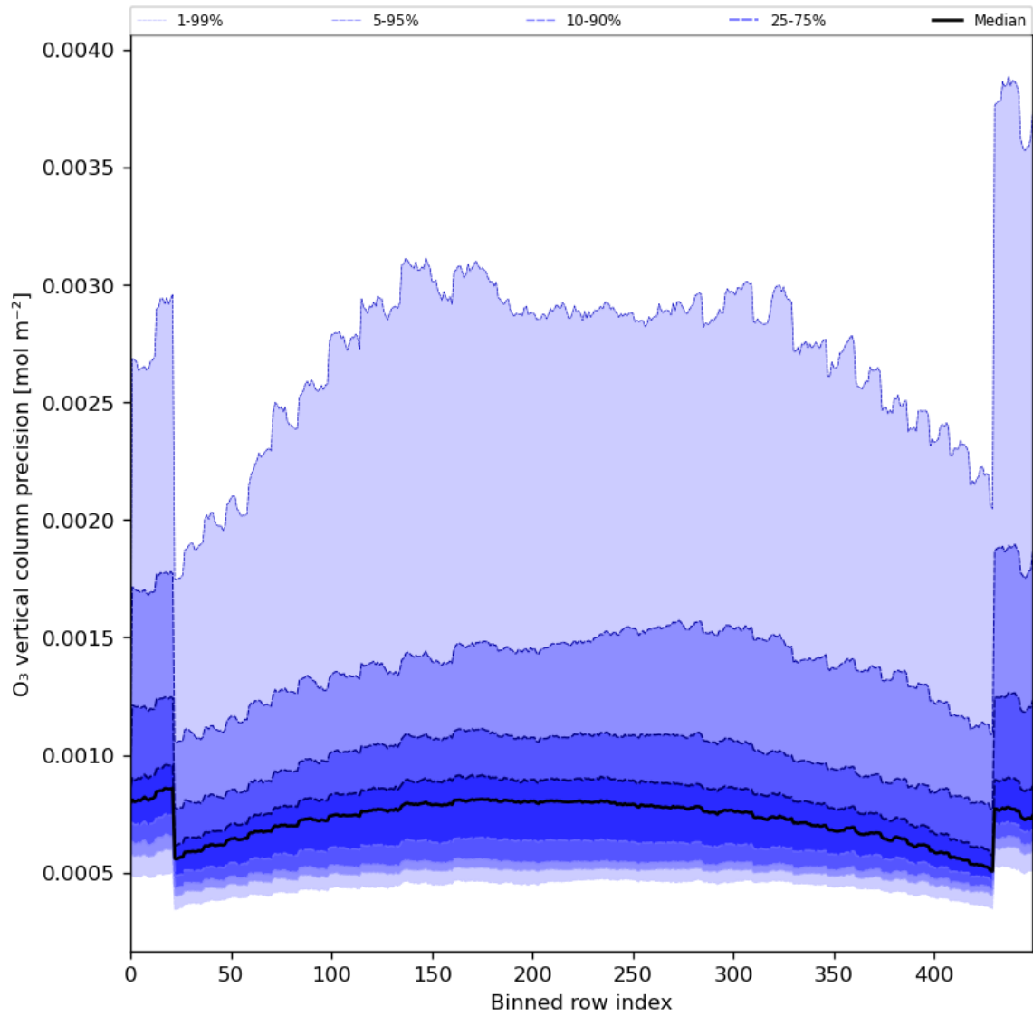
Figure 29: Along track statistics of “O 3 vertical column precision” for 2024-05-09 to 2024-05-11
