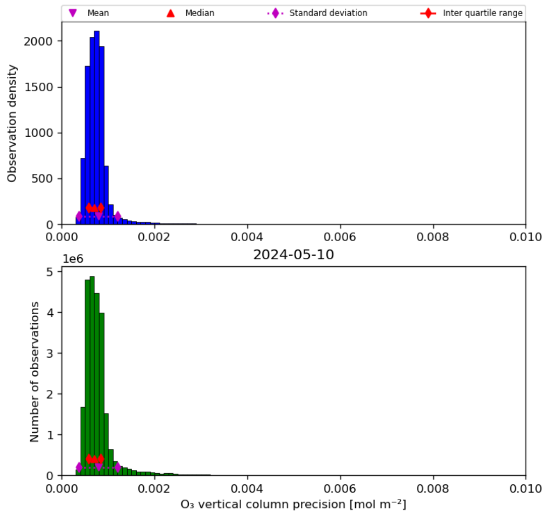
Figure 22: Histogram of “O 3 vertical column precision” for 2024-05-09 to 2024-05-11
