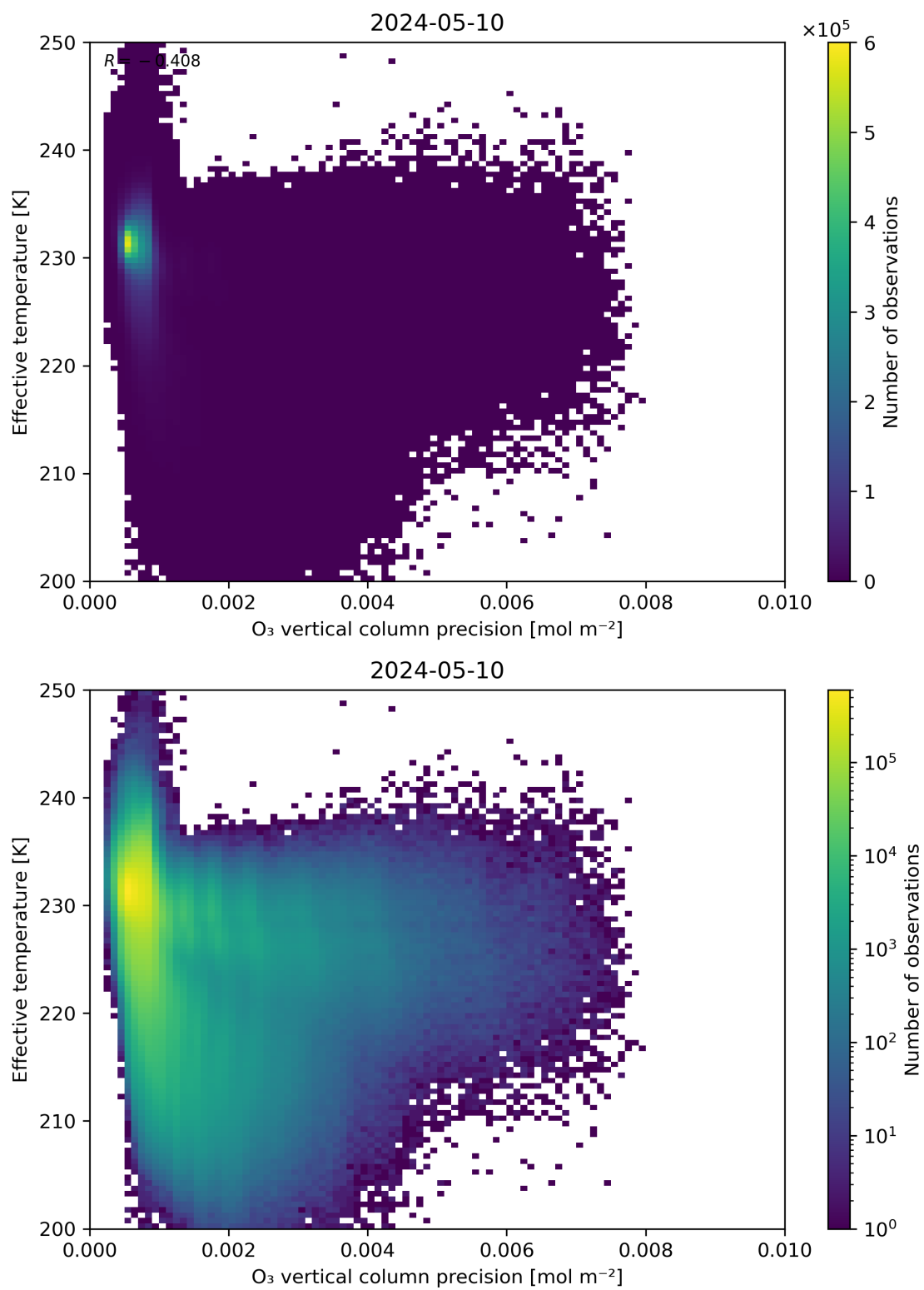
Figure 42: Scatter density plot of “O 3 vertical column precision” against “Effective temperature” for 2024-05-09 to 2024-05-11.
