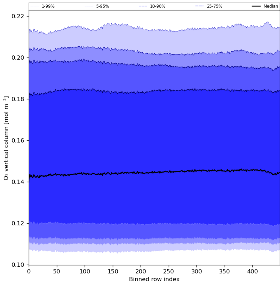
Figure 28: Along track statistics of “O 3 vertical column” for 2024-05-09 to 2024-05-11
