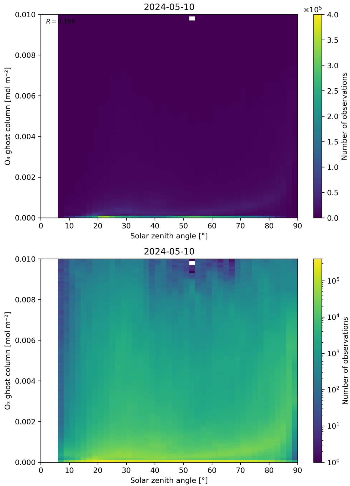
Figure 46: Scatter density plot of “Solar zenith angle” against “O 3 ghost column” for 2024-05-09 to 2024-05-11.
