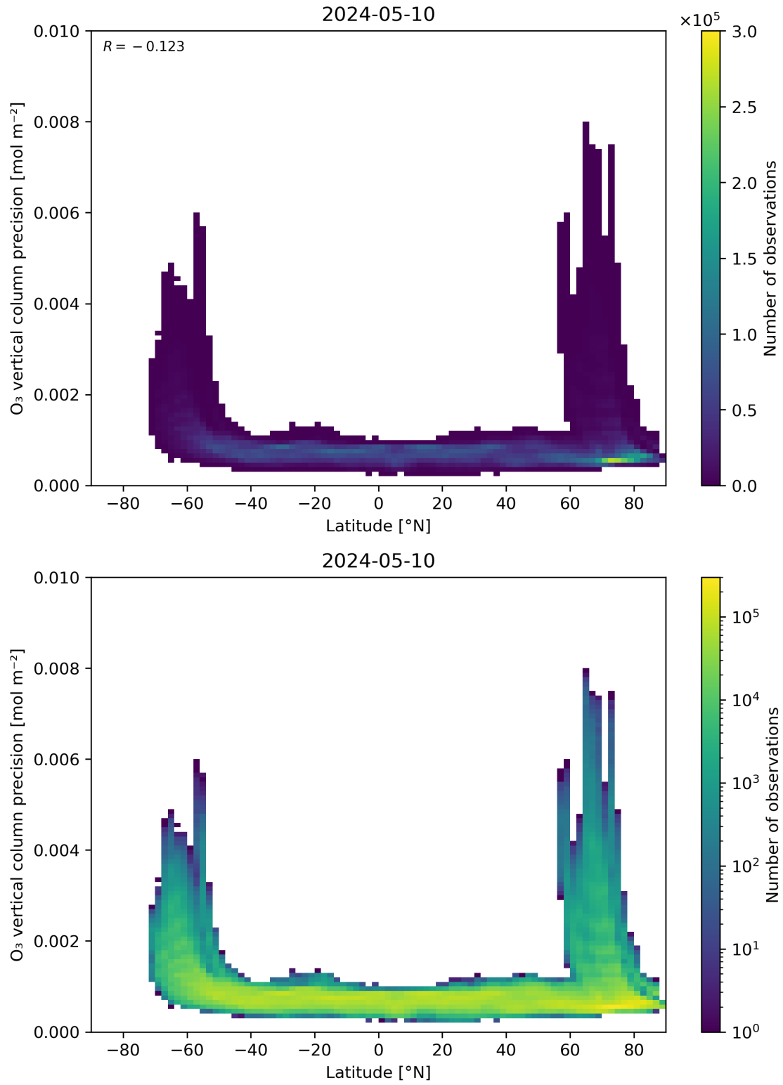
Figure 37: Scatter density plot of “Latitude” against “O 3 vertical column precision” for 2024-05-09 to 2024-05-11.
