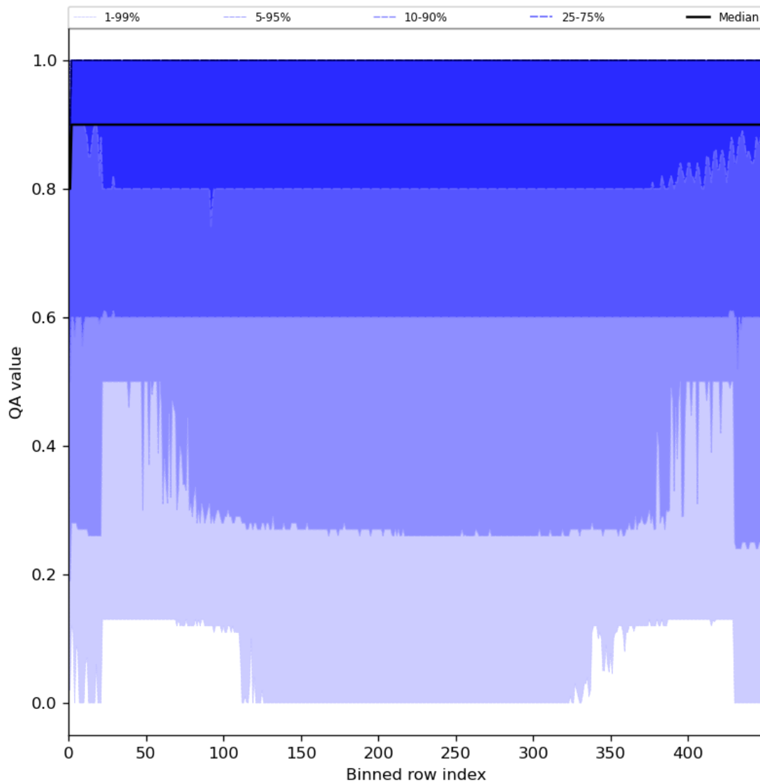
Figure 27: Along track statistics of “QA value” for 2024-05-09 to 2024-05-11
