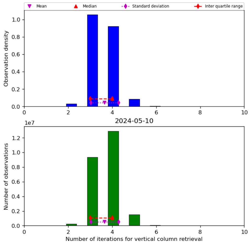
Figure 26: Histogram of “Number of iterations for vertical column retrieval” for 2024-05-09 to 2024-05-11
