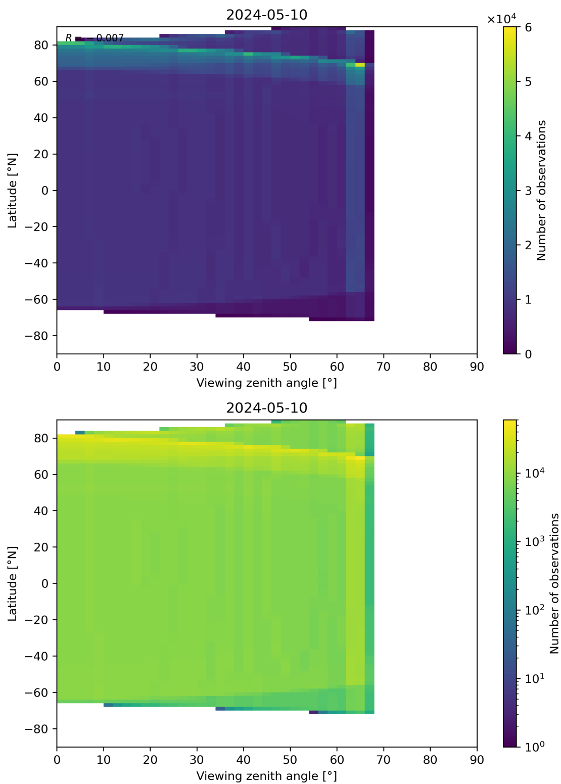
Figure 49: Scatter density plot of “Viewing zenith angle” against “Latitude” for 2024-05-09 to 2024-05-11.
