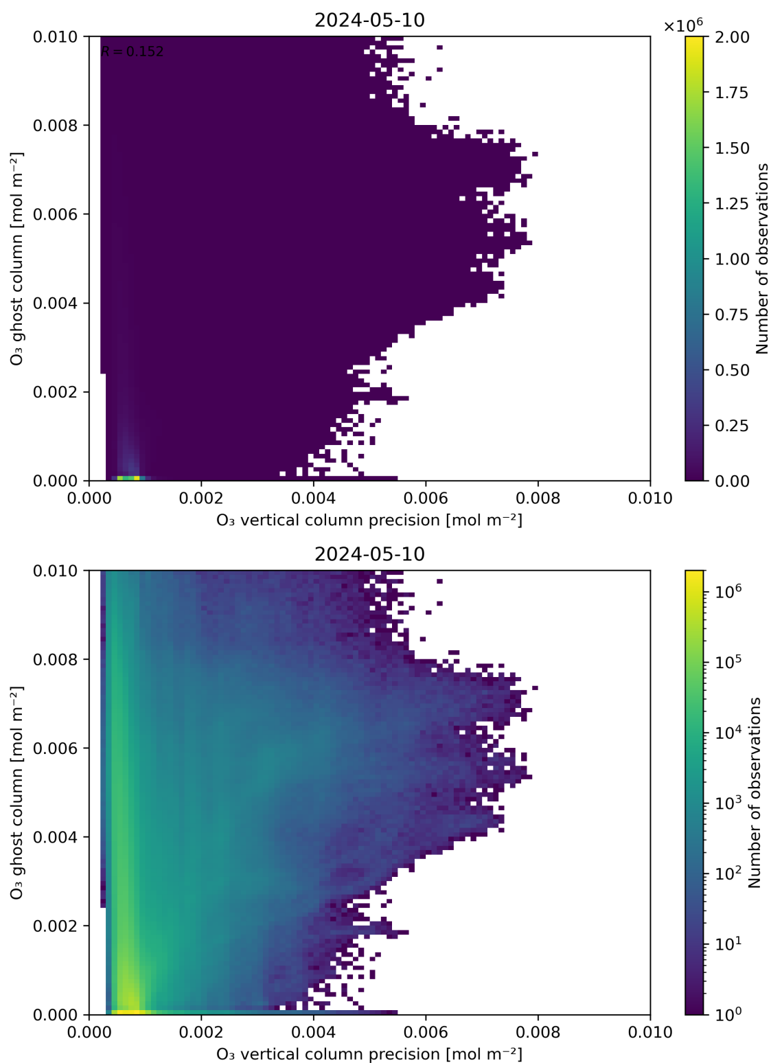
Figure 43: Scatter density plot of “O 3 vertical column precision” against “O 3 ghost column” for 2024-05-09 to 2024-05-11.
