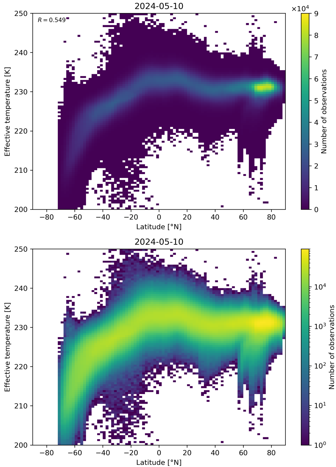
Figure 34: Scatter density plot of “Latitude” against “Effective temperature” for 2024-05-09 to 2024-05-11.
