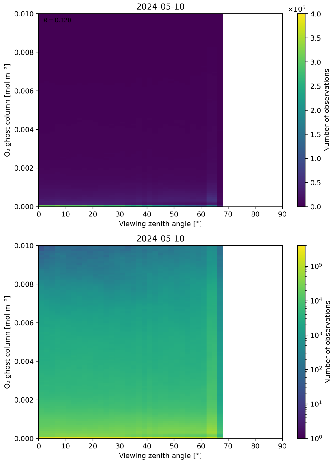
Figure 51: Scatter density plot of “Viewing zenith angle” against “O 3 ghost column” for 2024-05-09 to 2024-05-11.
