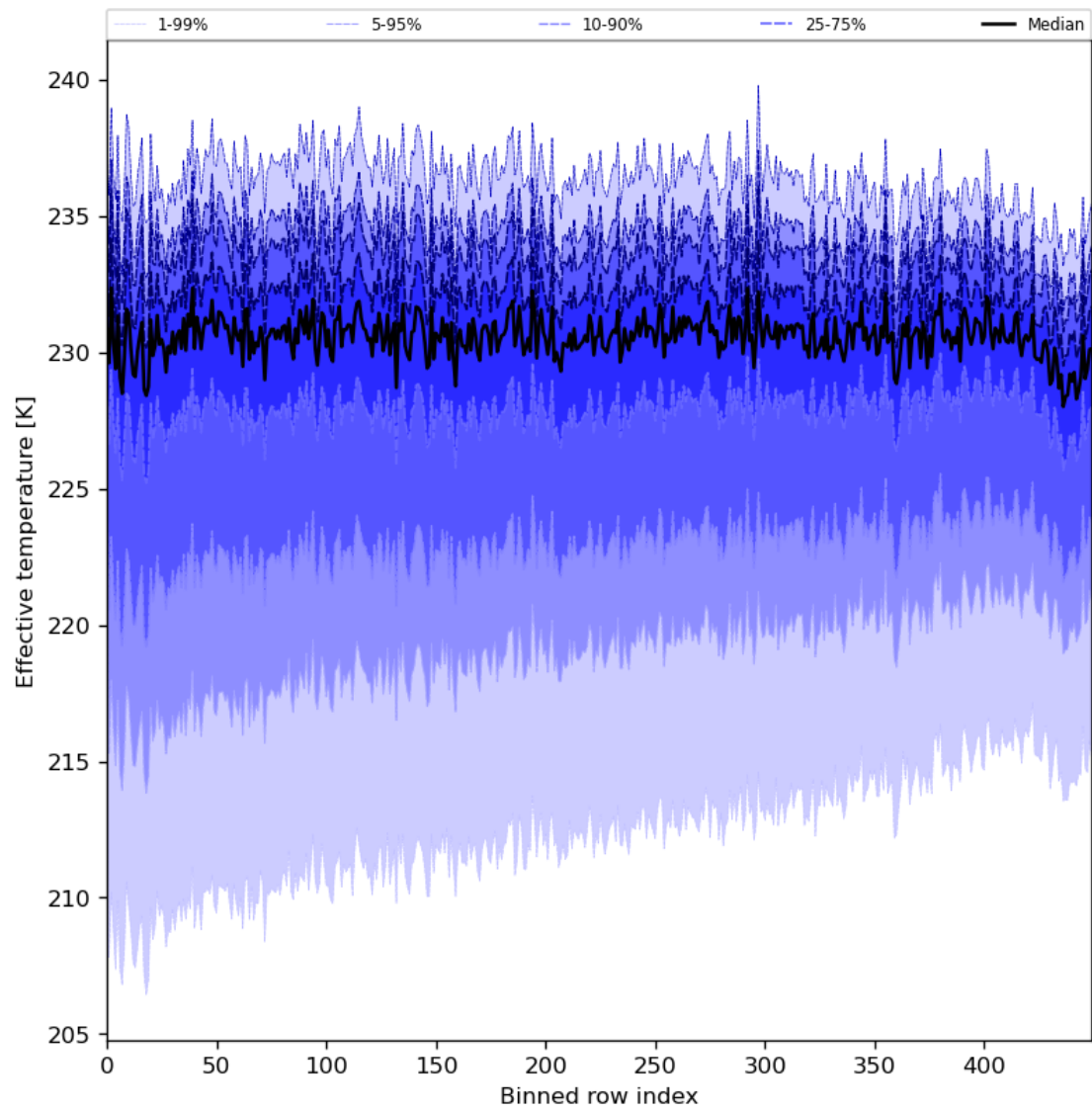
Figure 31: Along track statistics of “Effective temperature” for 2024-05-09 to 2024-05-11
