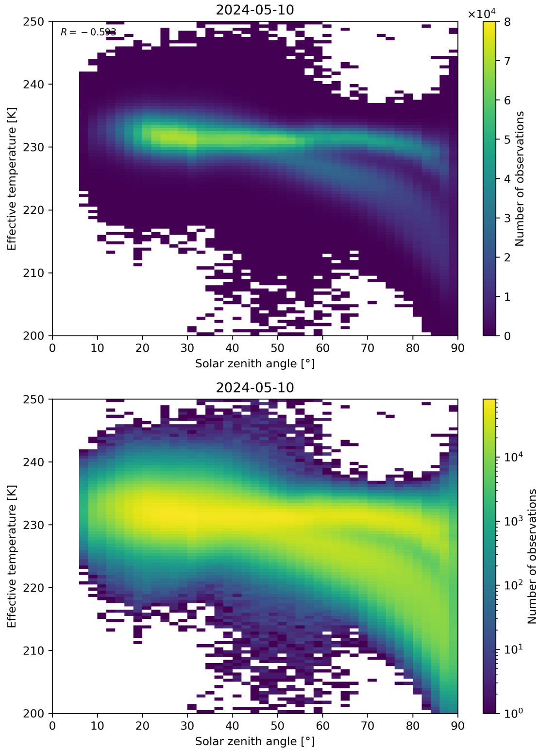
Figure 45: Scatter density plot of “Solar zenith angle” against “Effective temperature” for 2024-05-09 to 2024-05-11.
