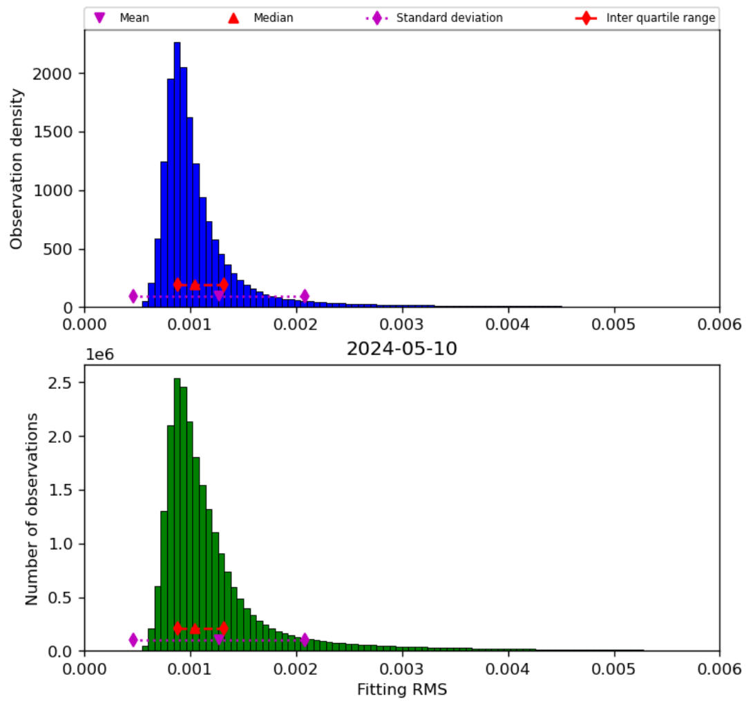
Figure 23: Histogram of “Fitting RMS” for 2024-05-09 to 2024-05-11
