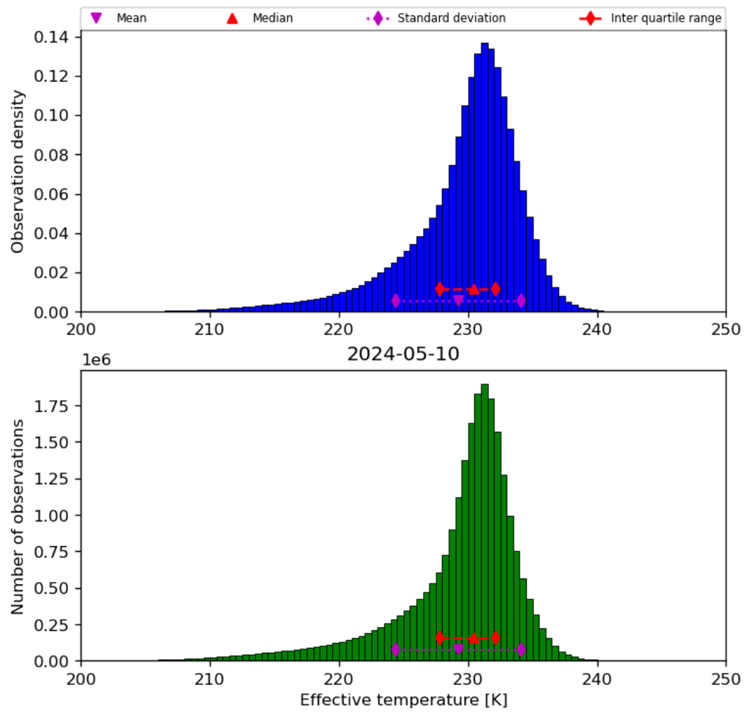
Figure 24: Histogram of “Effective temperature” for 2024-05-09 to 2024-05-11
