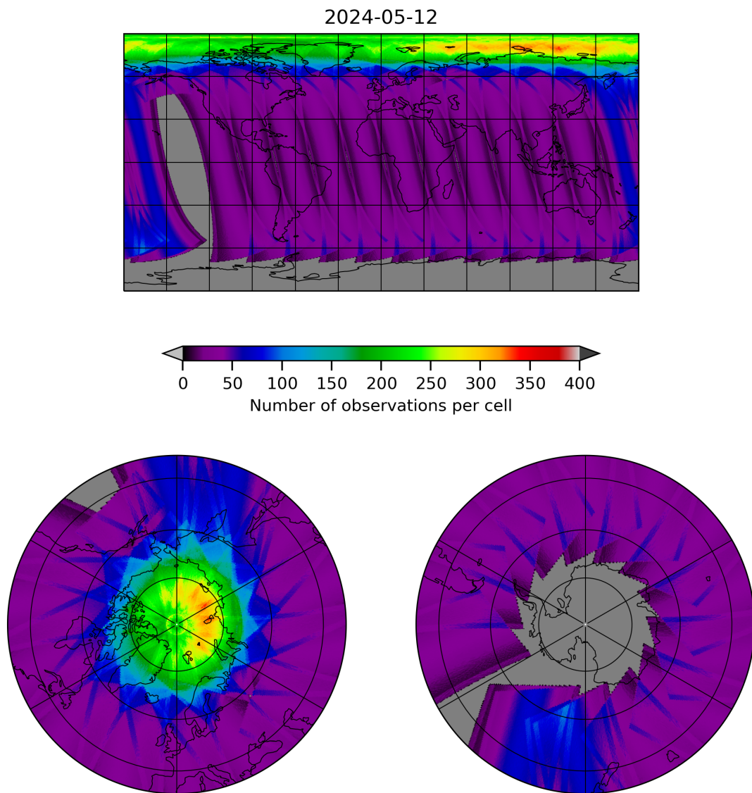
Figure 12: Map of the number of observations for 2024-05-12 to 2024-05-13
