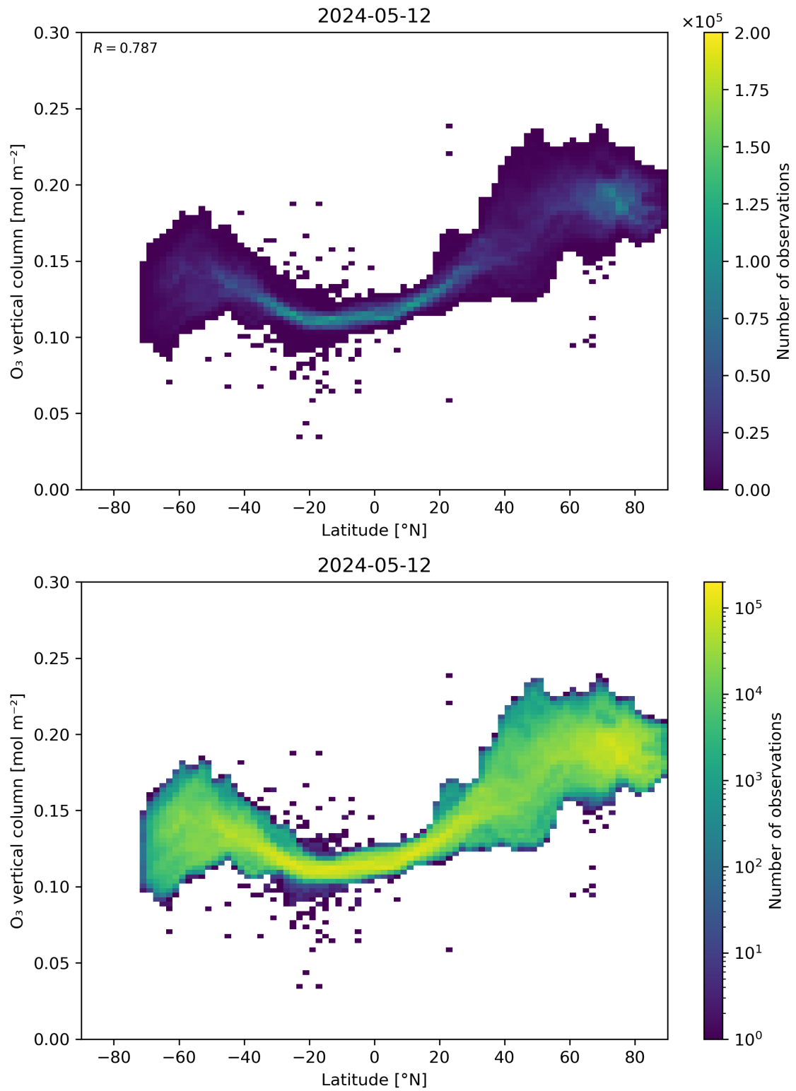
Figure 36: Scatter density plot of “Latitude” against “O 3 vertical column” for 2024-05-12 to 2024-05-13.
