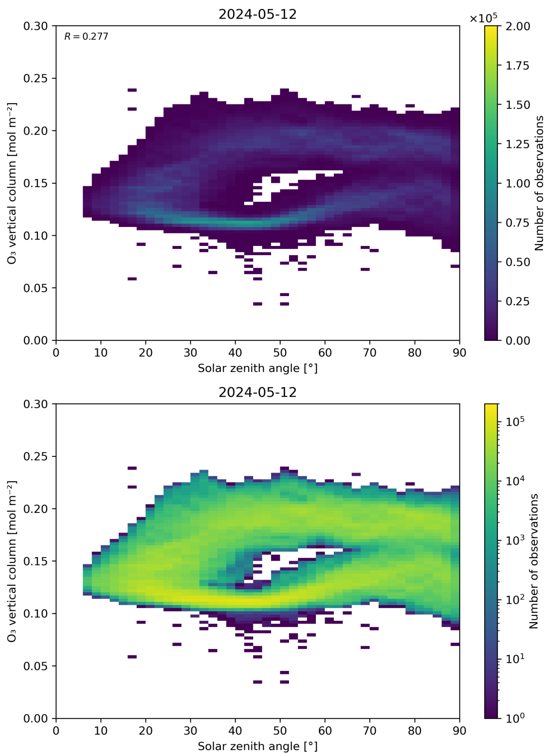
Figure 47: Scatter density plot of “Solar zenith angle” against “O 3 vertical column” for 2024-05-12 to 2024-05-13.
