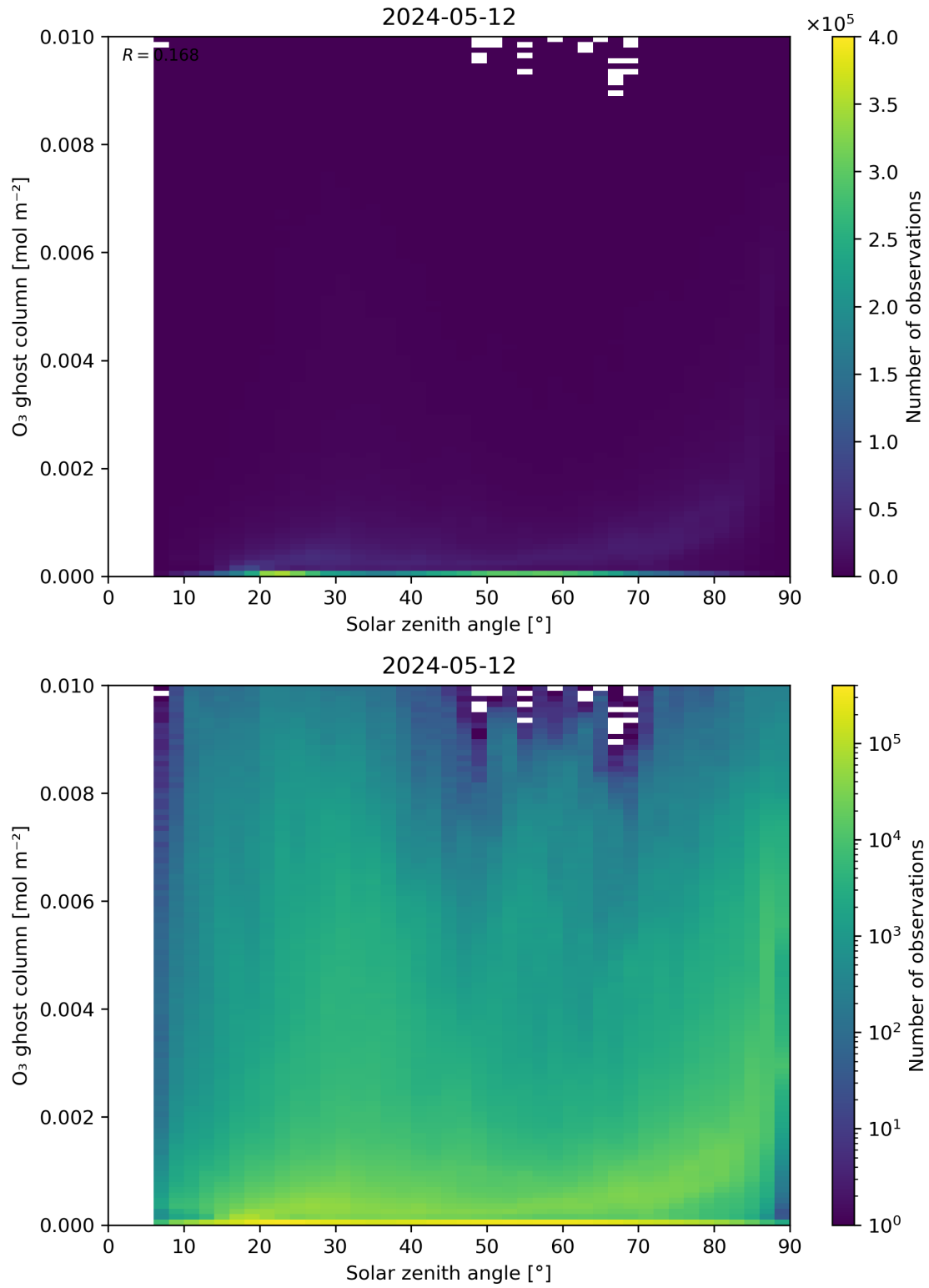
Figure 46: Scatter density plot of “Solar zenith angle” against “O 3 ghost column” for 2024-05-12 to 2024-05-13.
