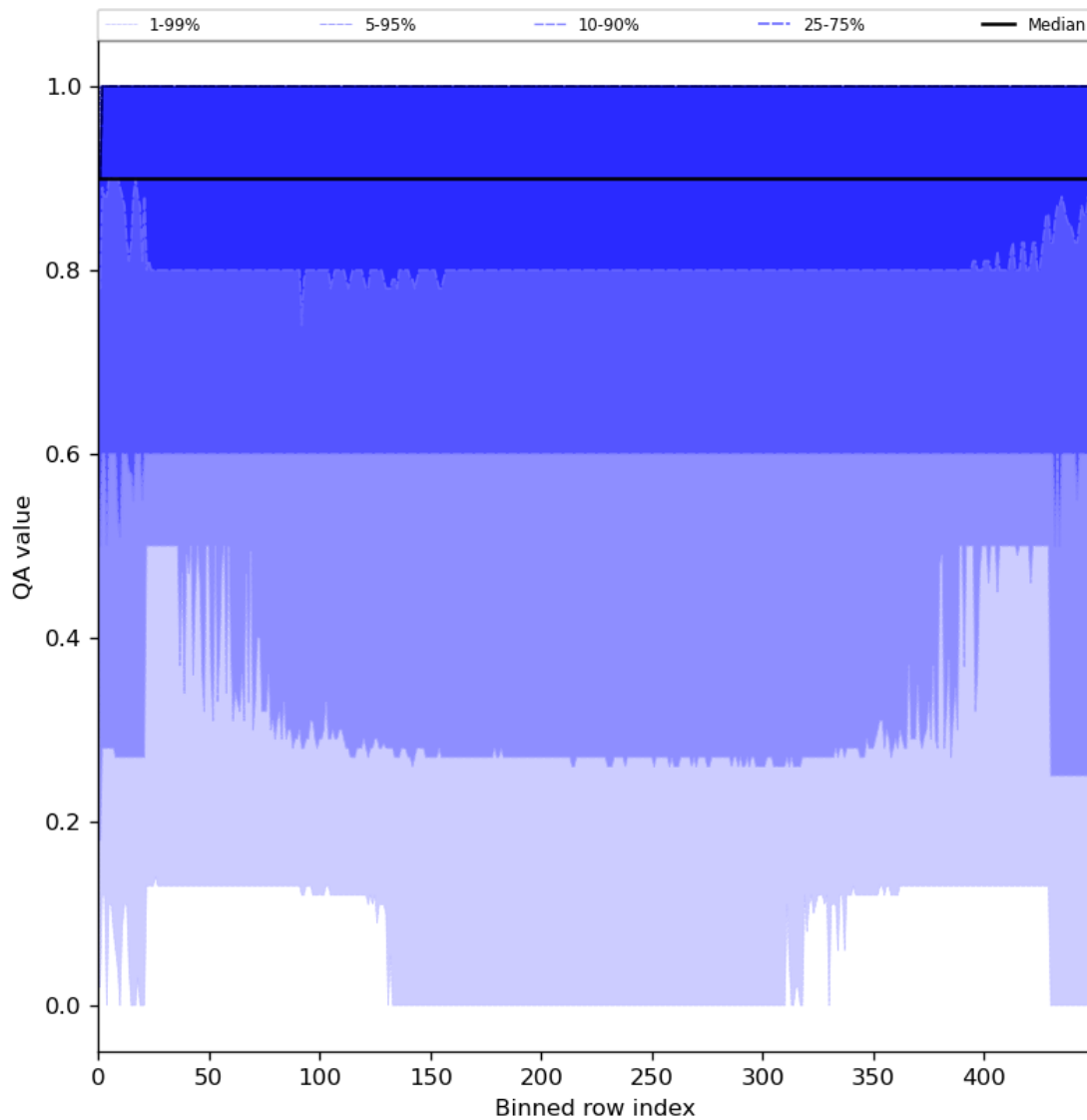
Figure 27: Along track statistics of “QA value” for 2024-05-12 to 2024-05-13
