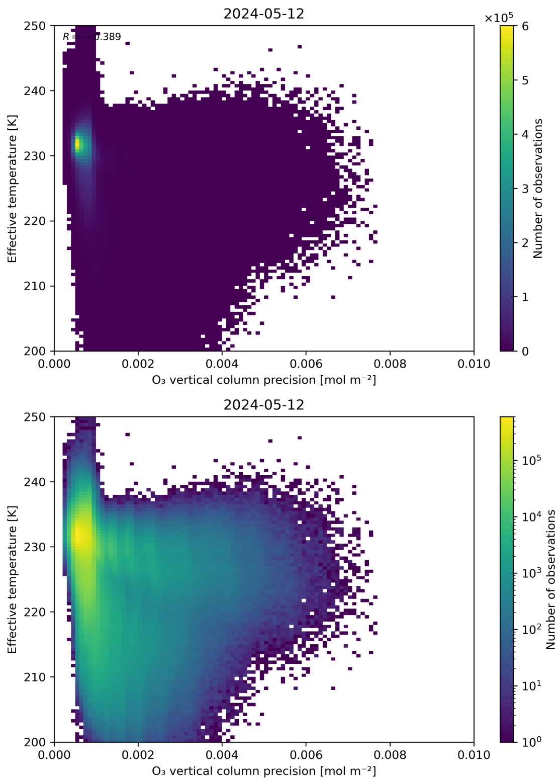
Figure 42: Scatter density plot of “O 3 vertical column precision” against “Effective temperature” for 2024-05-12 to 2024-05-13.
