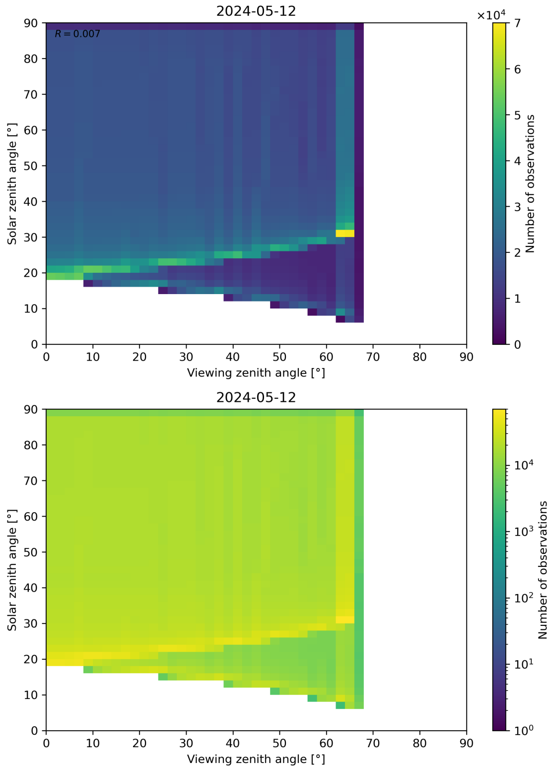
Figure 54: Scatter density plot of “Viewing zenith angle” against “Solar zenith angle” for 2024-05-12 to 2024-05-13.
