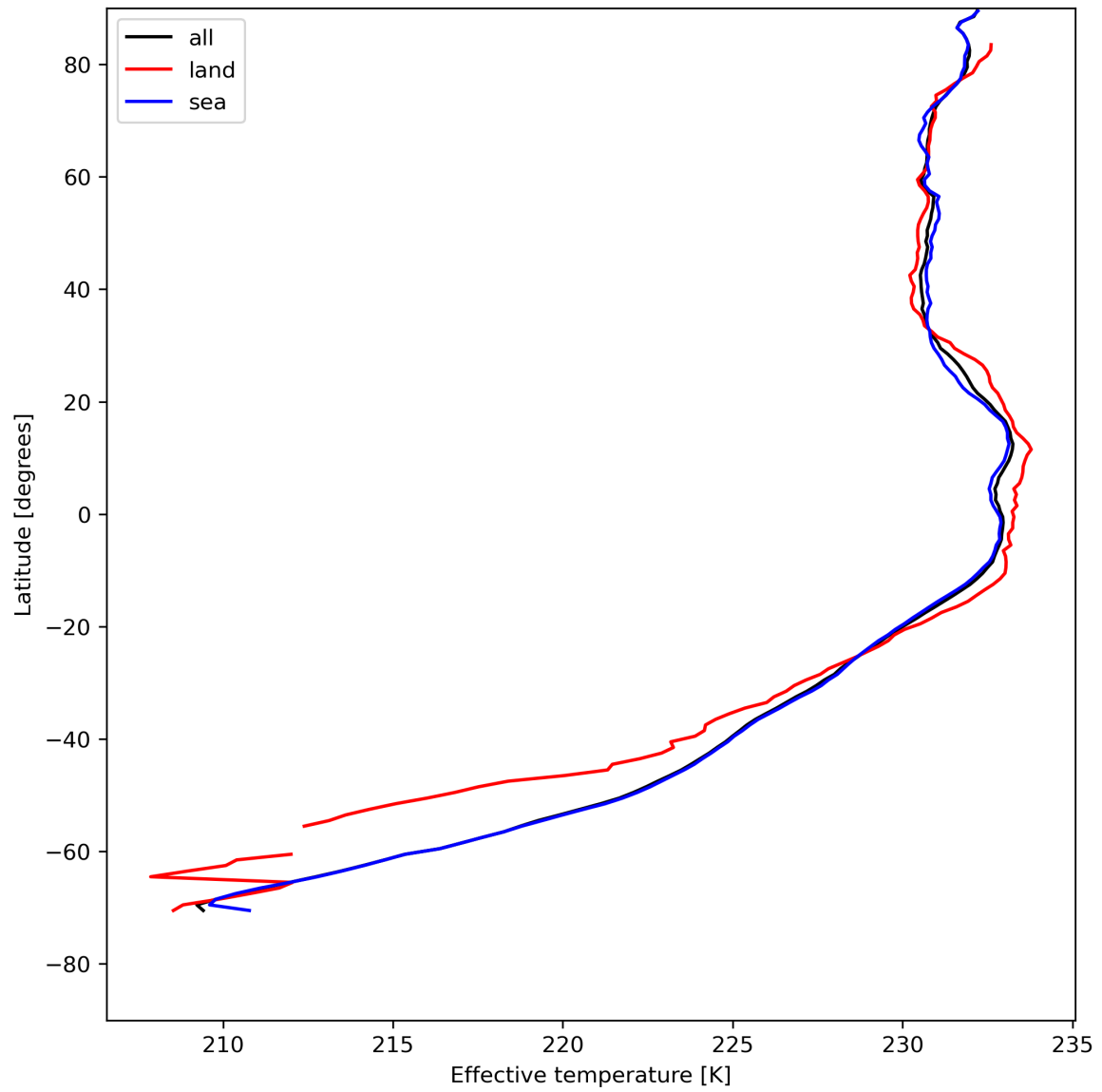
Figure 17: Zonal average of "Effective temperature" for 2024-05-12 to 2024-05-13.
