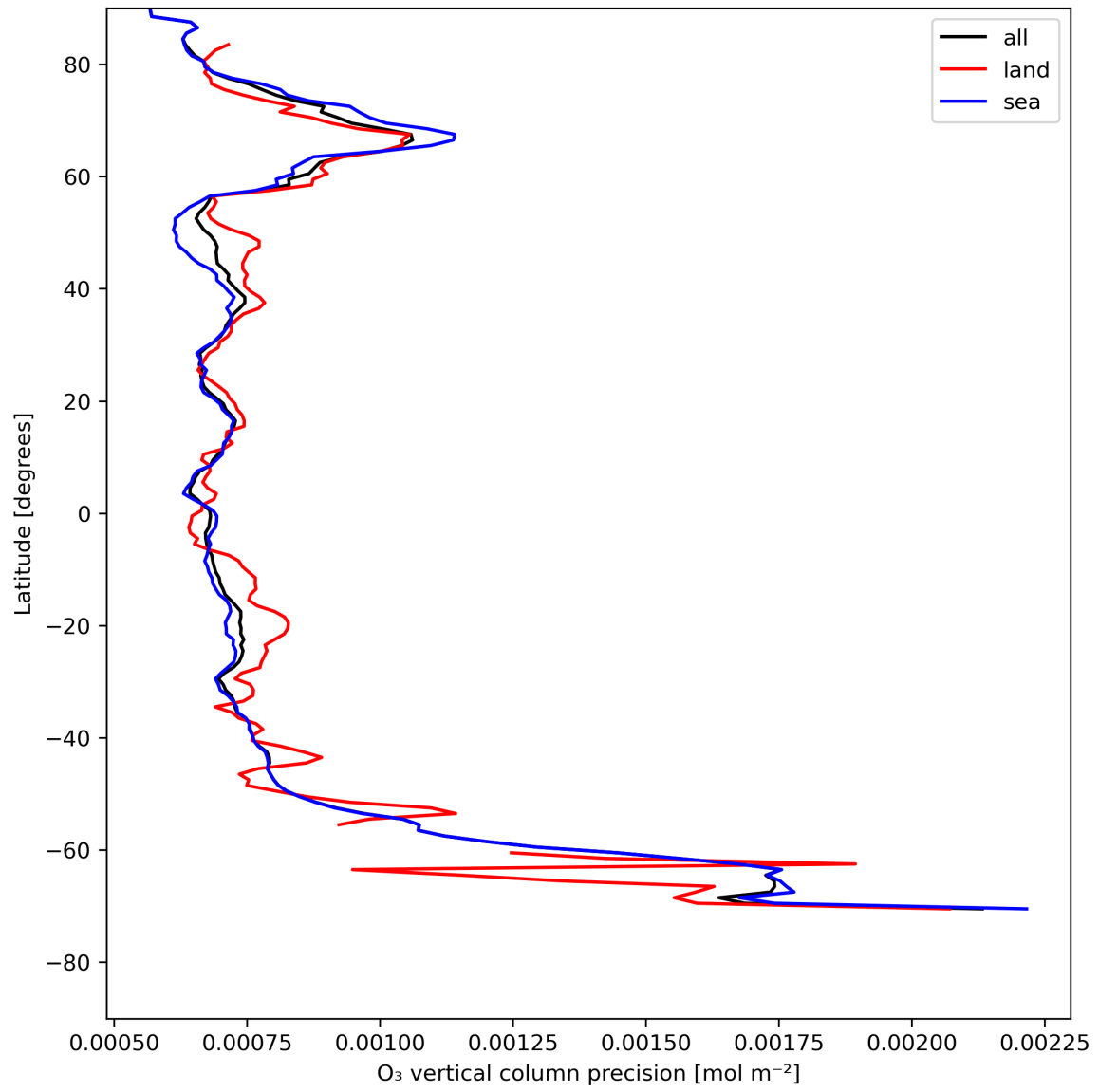
Figure 15: Zonal average of “O 3 vertical column precision” for 2024-05-12 to 2024-05-13.
