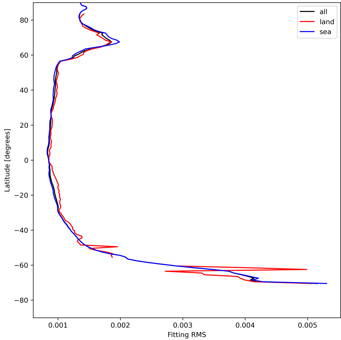
Figure 16: Zonal average of “Fitting RMS” for 2024-05-12 to 2024-05-13.
