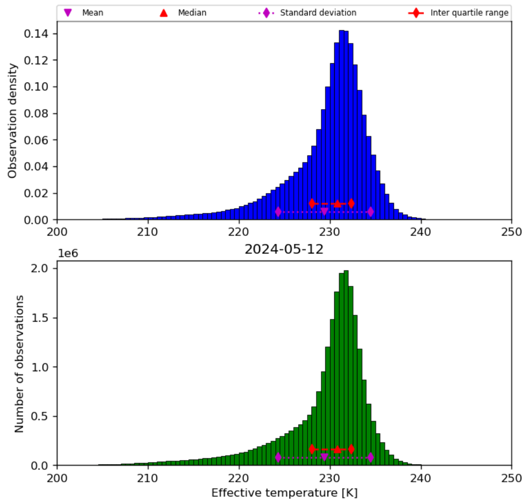
Figure 24: Histogram of “Effective temperature” for 2024-05-12 to 2024-05-13
