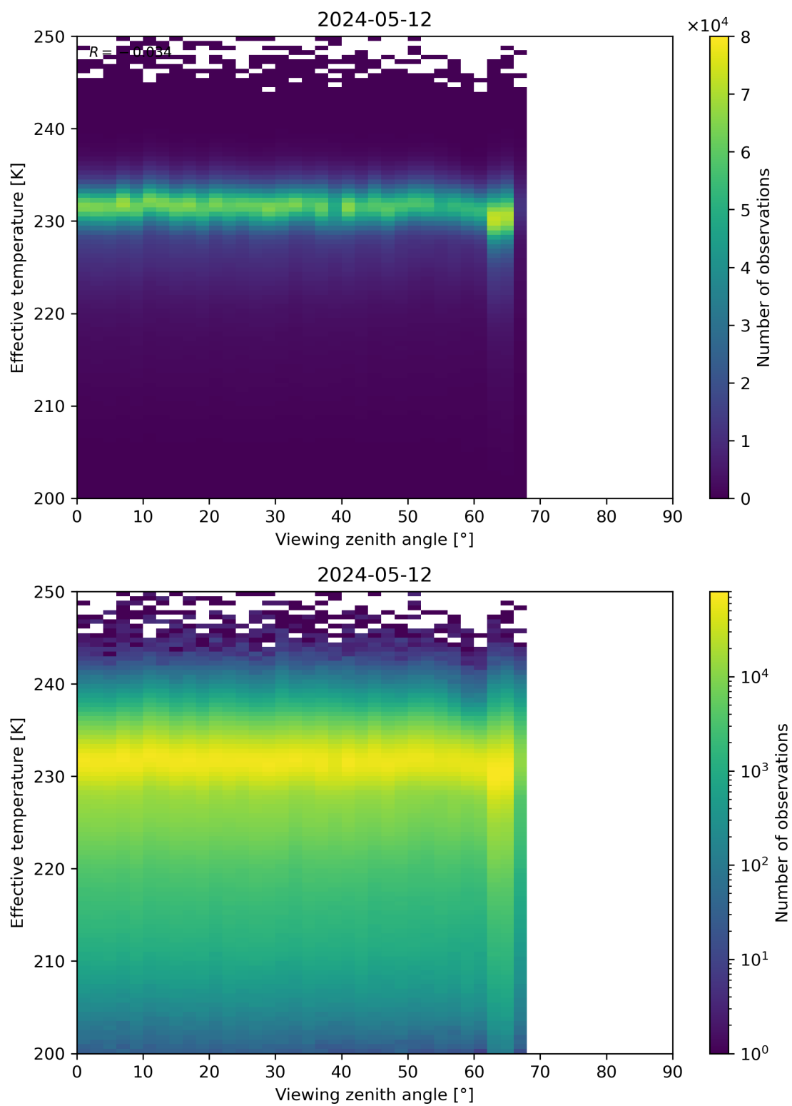
Figure 50: Scatter density plot of “Viewing zenith angle” against “Effective temperature” for 2024-05-12 to 2024-05-13.
