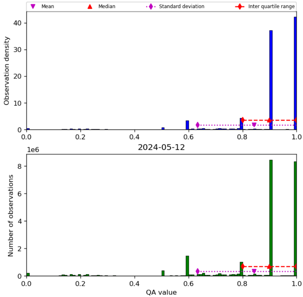
Figure 20: Histogram of “QA value” for 2024-05-12 to 2024-05-13
