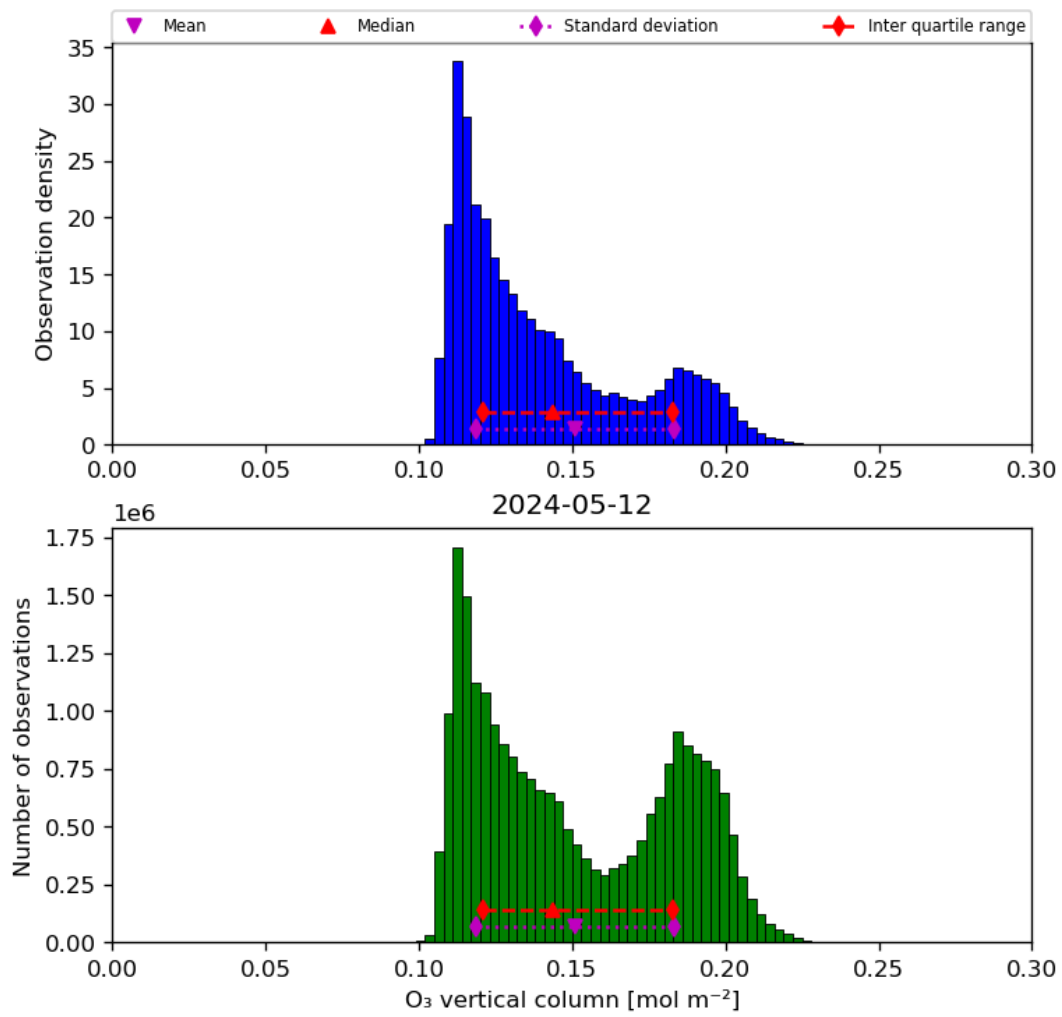
Figure 21: Histogram of “O 3 vertical column” for 2024-05-12 to 2024-05-13
