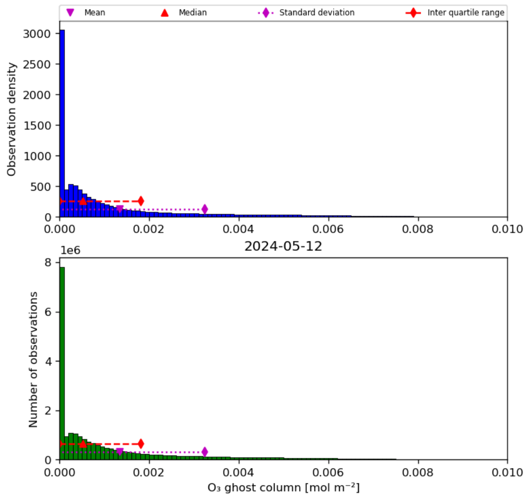
Figure 25: Histogram of “O 3 ghost column” for 2024-05-12 to 2024-05-13
