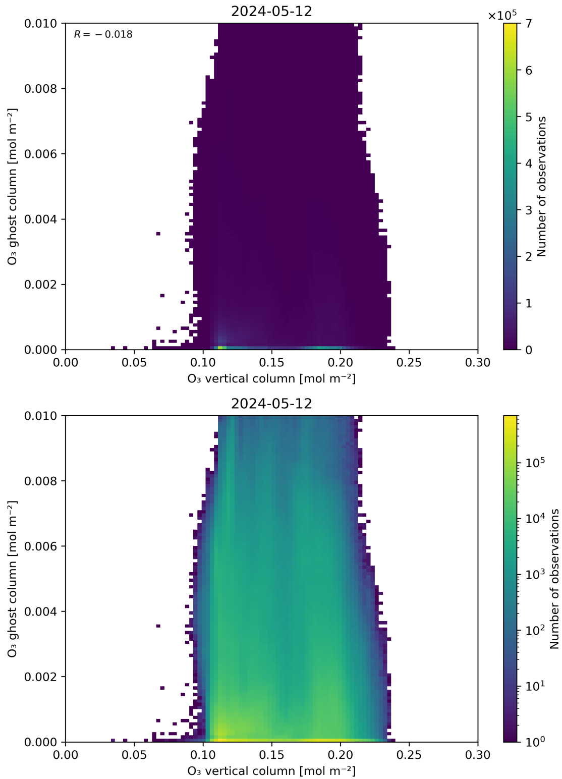
Figure 40: Scatter density plot of “O 3 vertical column” against “O 3 ghost column” for 2024-05-12 to 2024-05-13.
