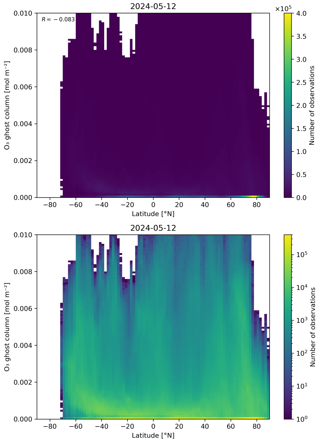
Figure 35: Scatter density plot of “Latitude” against “O 3 ghost column” for 2024-05-12 to 2024-05-13.
