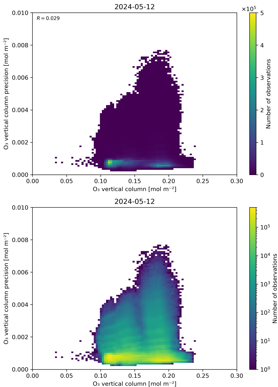
Figure 41: Scatter density plot of “O 3 vertical column” against “O 3 vertical column precision” for 2024-05-12 to 2024-05-13.
