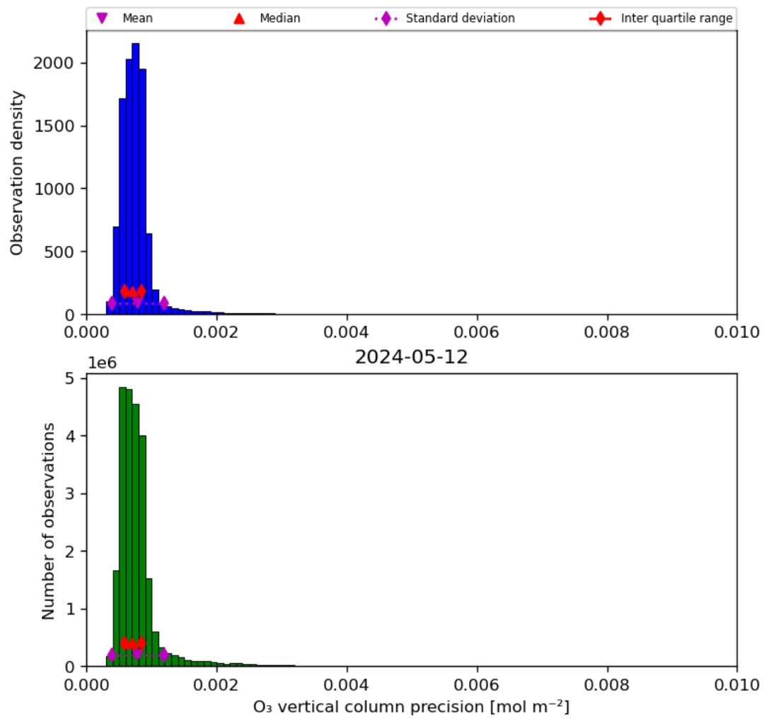
Figure 22: Histogram of “O 3 vertical column precision” for 2024-05-12 to 2024-05-13
