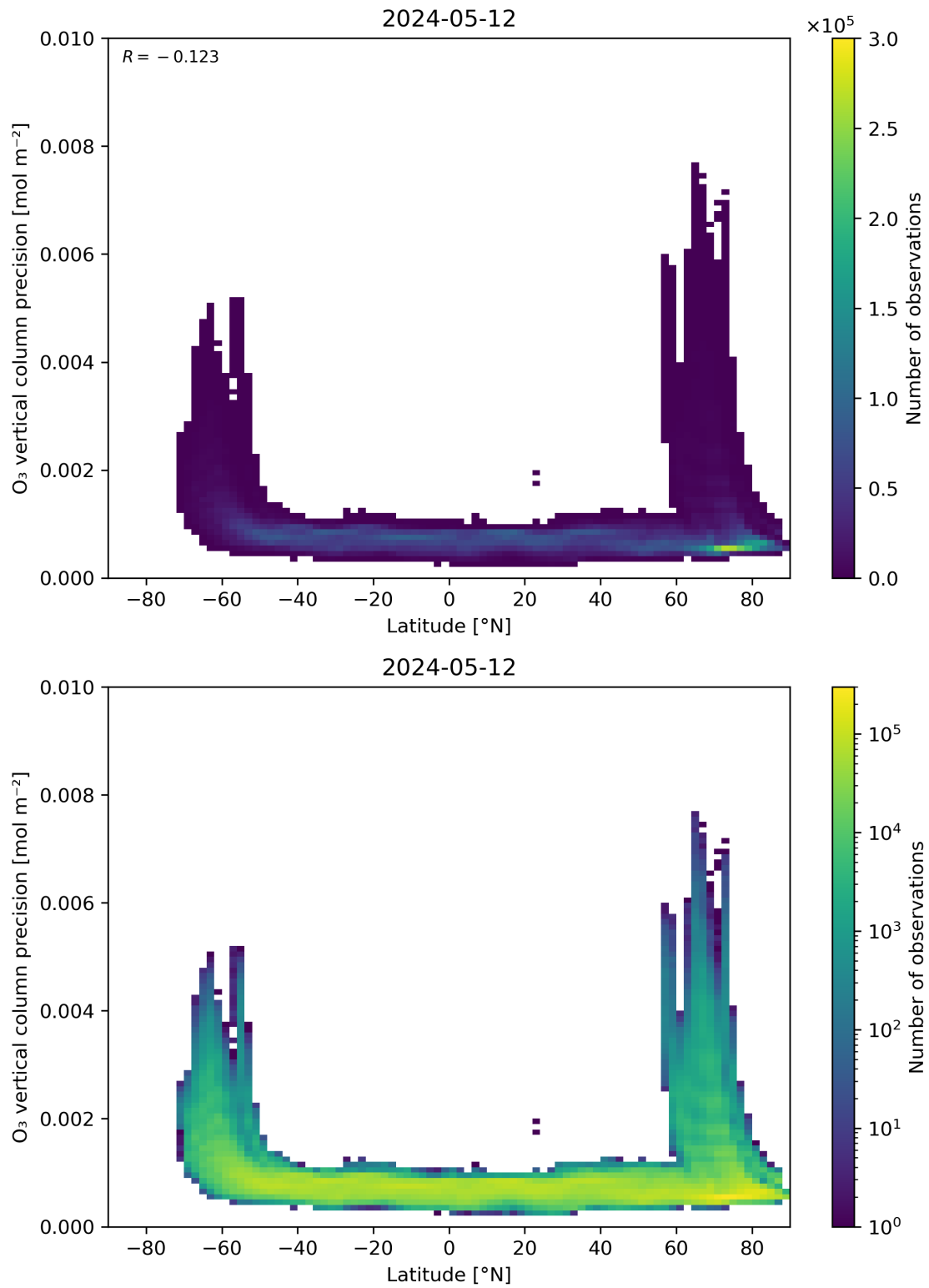
Figure 37: Scatter density plot of “Latitude” against “O 3 vertical column precision” for 2024-05-12 to 2024-05-13.
