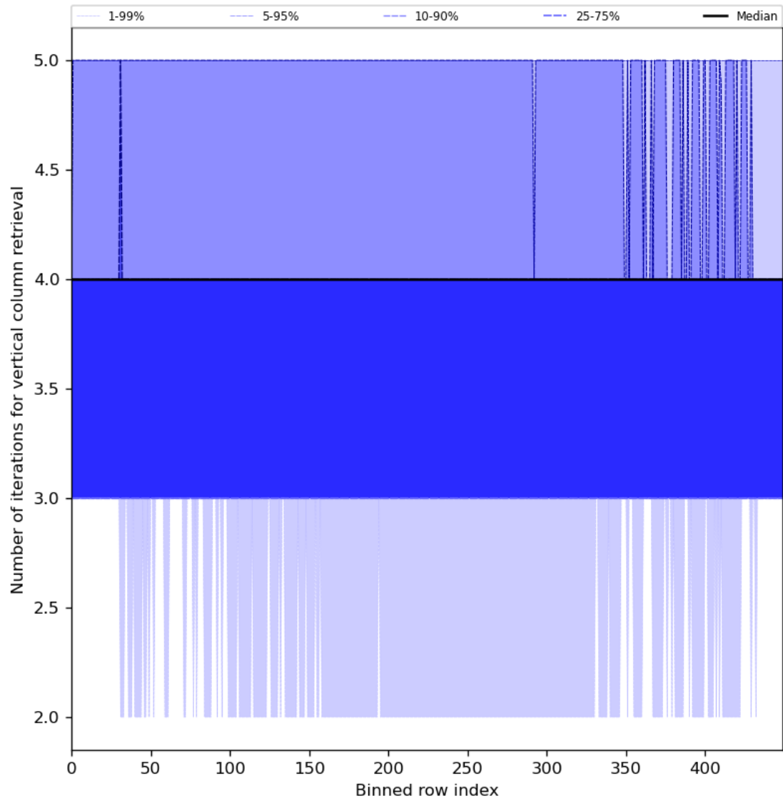
Figure 33: Along track statistics of “Number of iterations for vertical column retrieval” for 2024-05-12 to 2024-05-13
