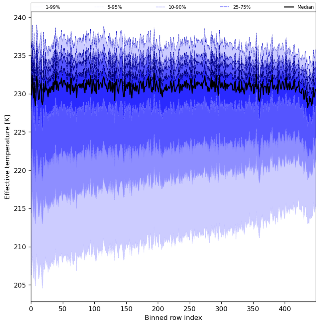
Figure 31: Along track statistics of “Effective temperature” for 2024-05-12 to 2024-05-13
