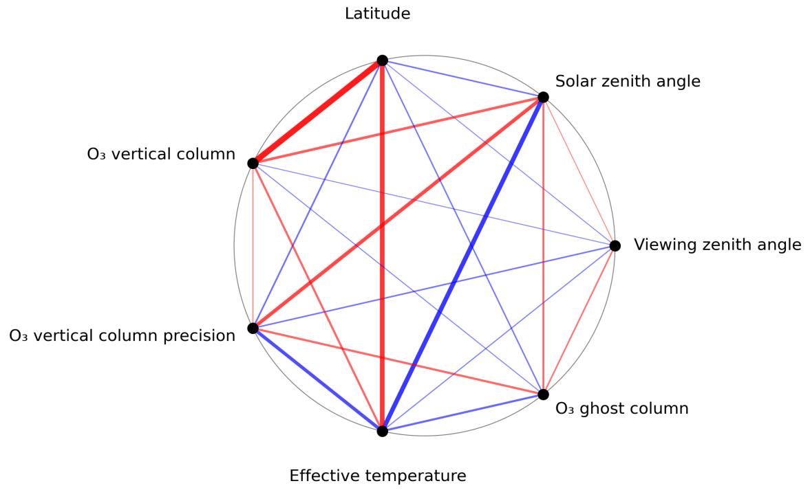
Figure 1: Map of correlation graph for 2024-05-12 to 2024-05-13.
