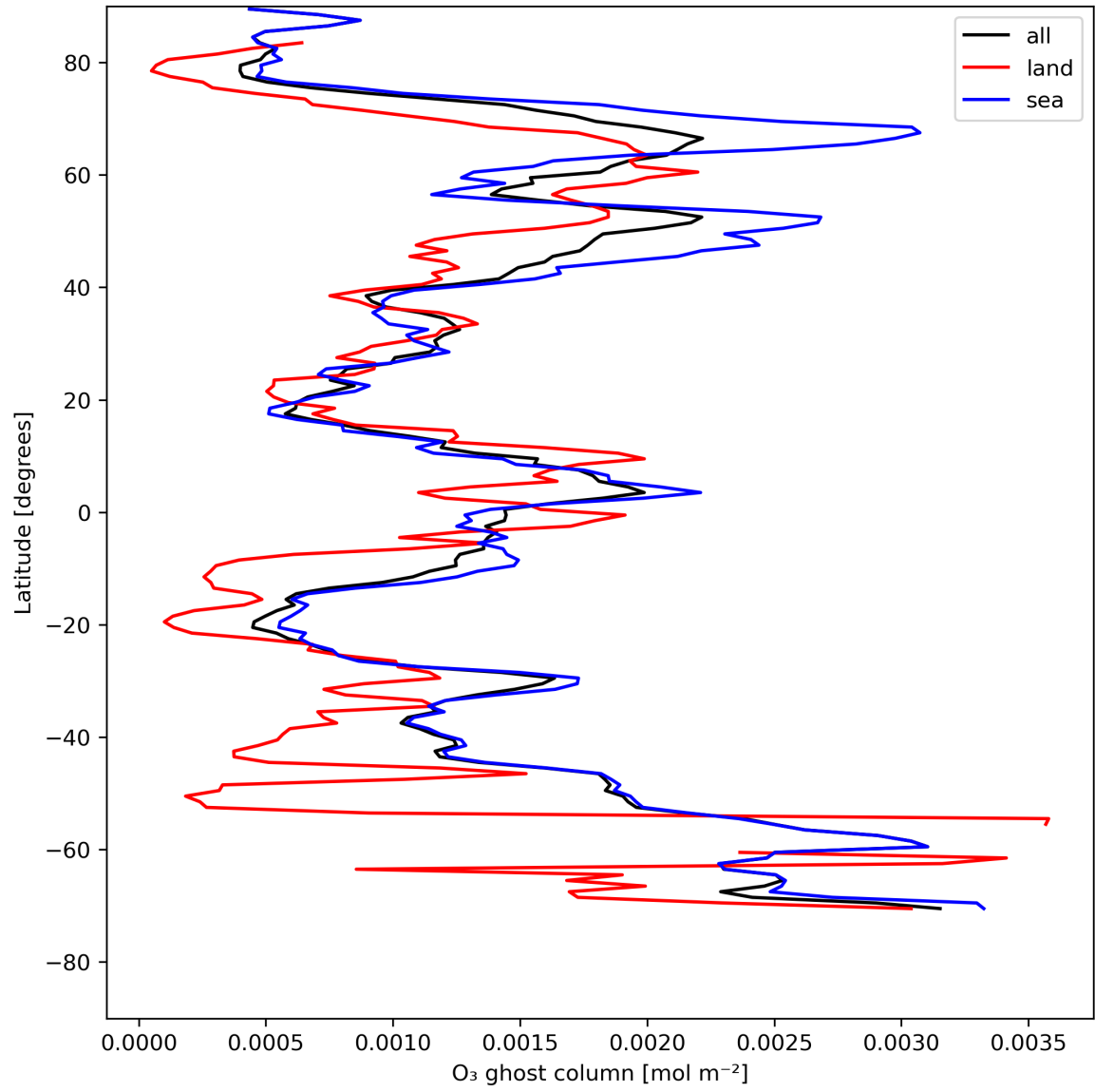
Figure 18: Zonal average of "O 3 ghost column" for 2024-05-12 to 2024-05-13.
