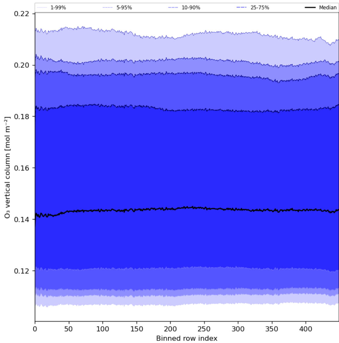
Figure 28: Along track statistics of “O 3 vertical column” for 2024-05-12 to 2024-05-13
