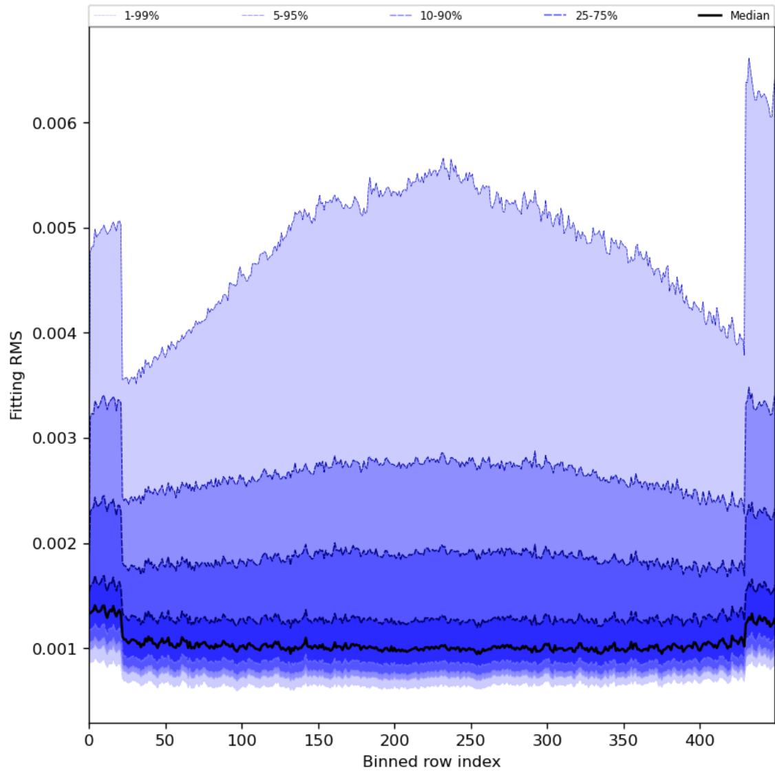
Figure 30: Along track statistics of “Fitting RMS” for 2024-05-12 to 2024-05-13
