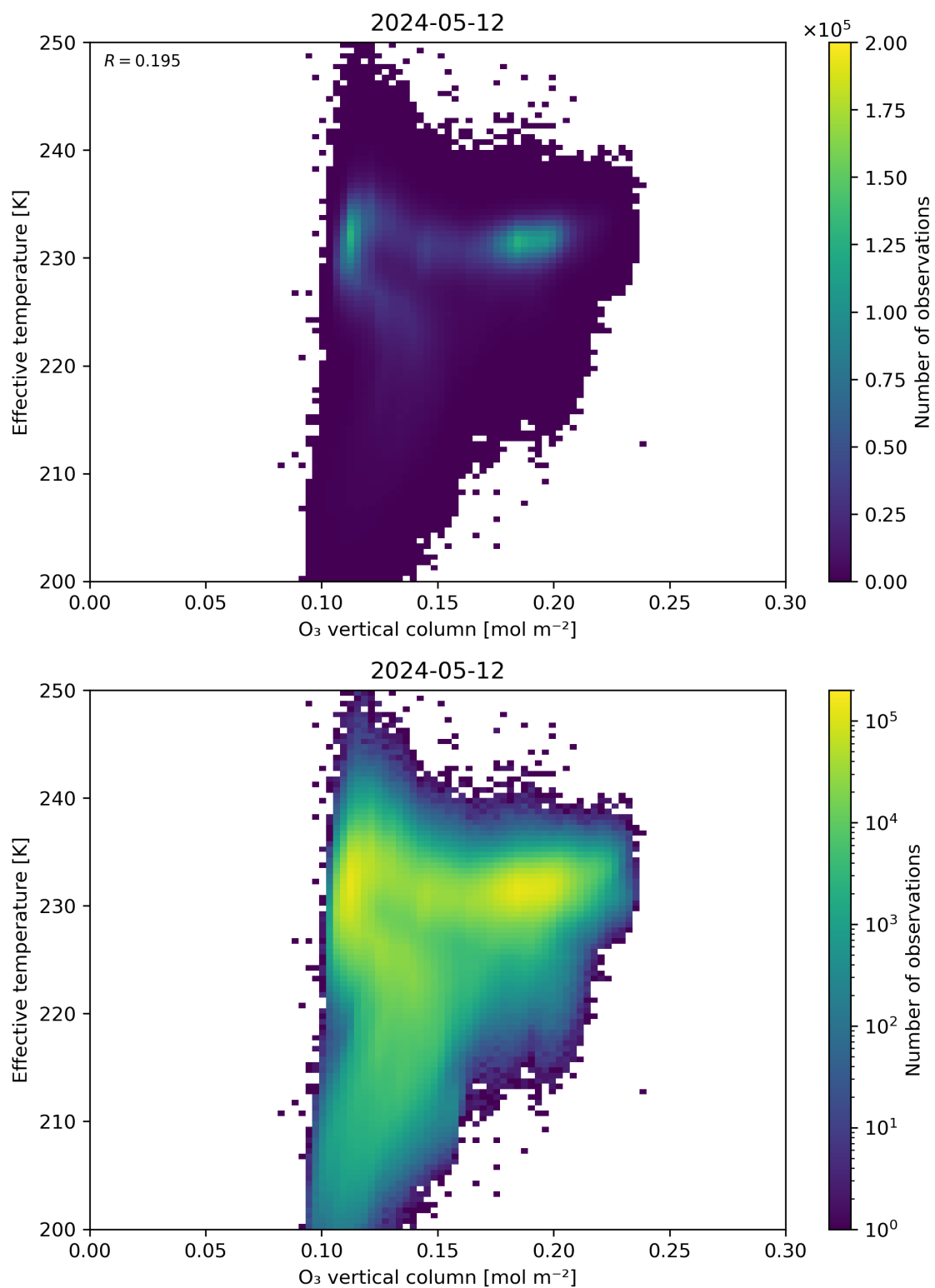
Figure 39: Scatter density plot of “O 3 vertical column” against “Effective temperature” for 2024-05-12 to 2024-05-13.
