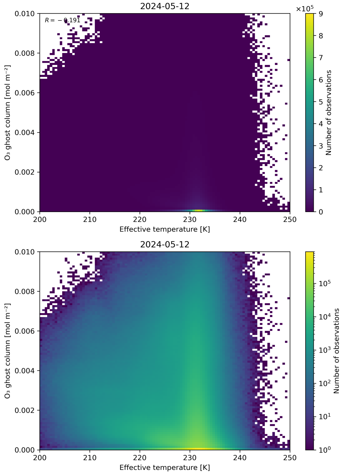
Figure 38: Scatter density plot of “Effective temperature” against “O 3 ghost column” for 2024-05-12 to 2024-05-13.
