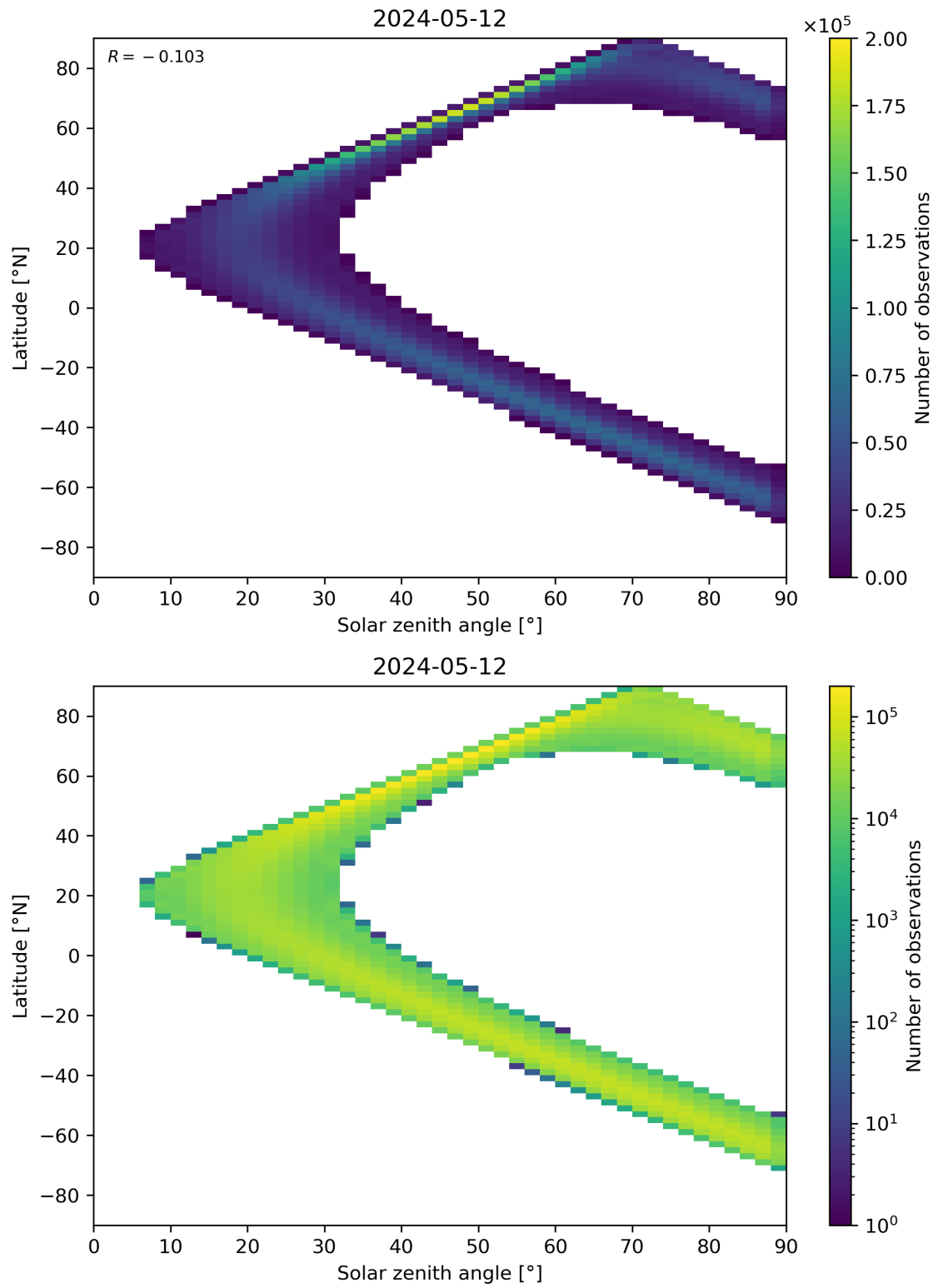
Figure 44: Scatter density plot of “Solar zenith angle” against “Latitude” for 2024-05-12 to 2024-05-13.
