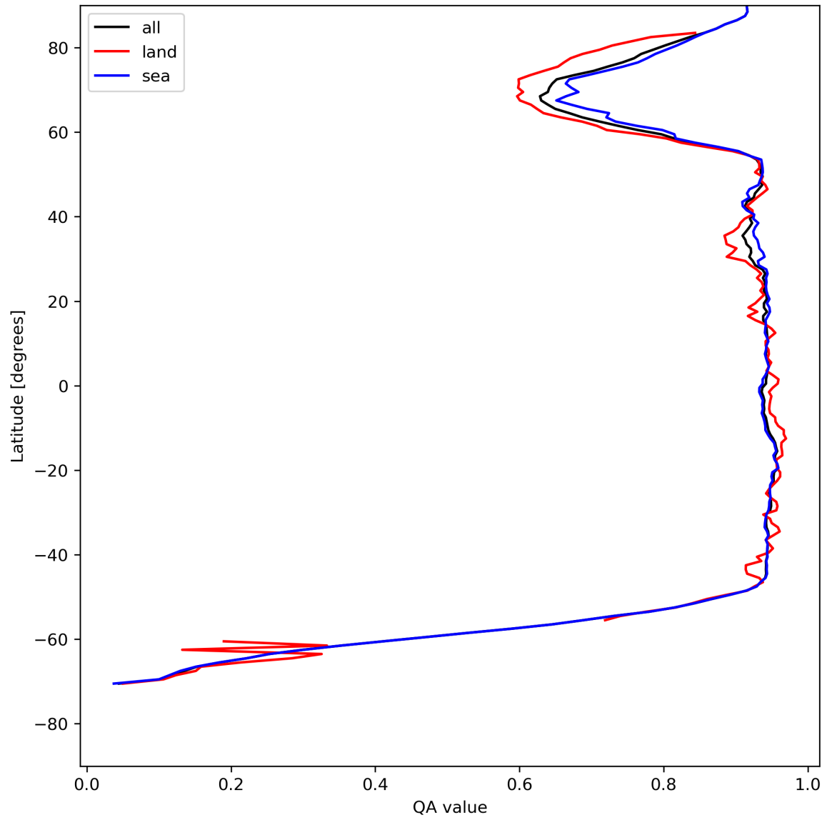
Figure 13: Zonal average of “QA value” for 2024-05-12 to 2024-05-13.
