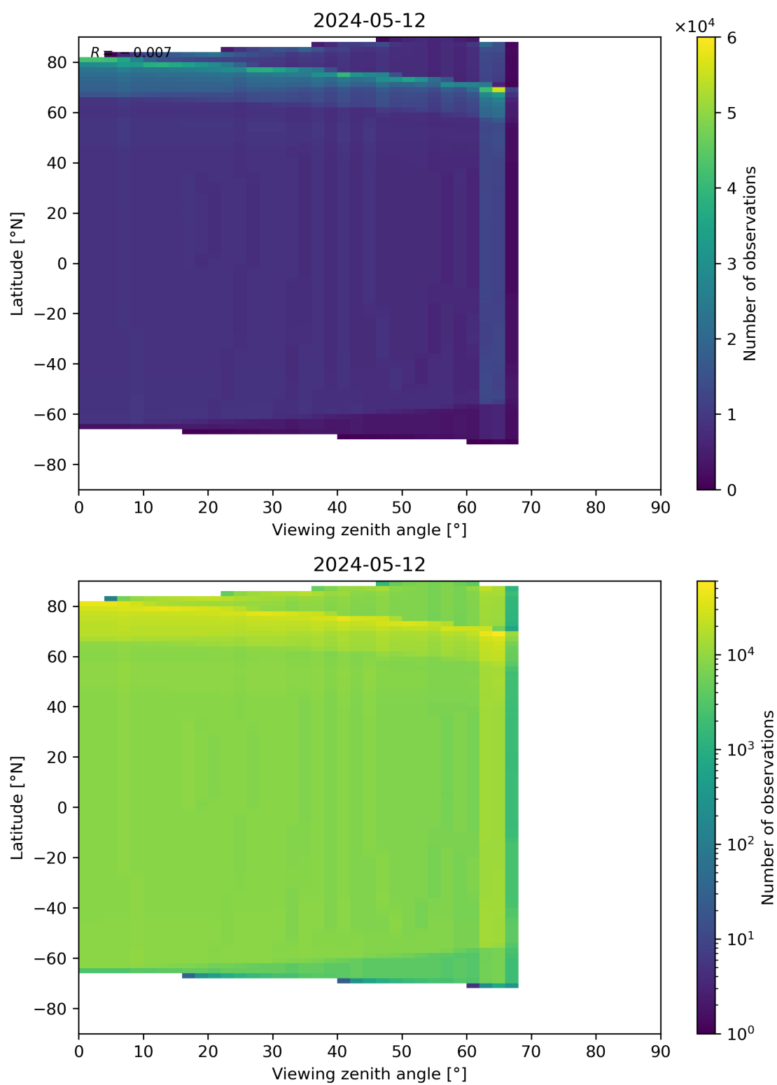
Figure 49: Scatter density plot of “Viewing zenith angle” against “Latitude” for 2024-05-12 to 2024-05-13.
