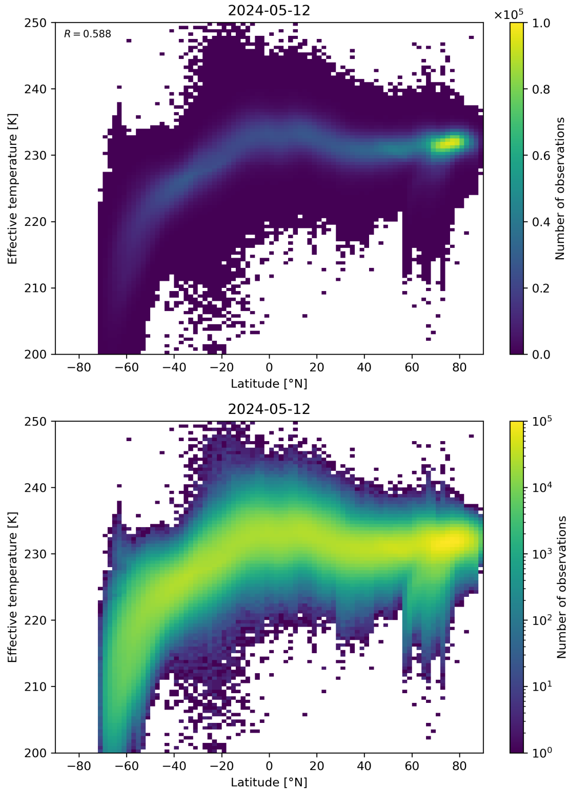
Figure 34: Scatter density plot of “Latitude” against “Effective temperature” for 2024-05-12 to 2024-05-13.
