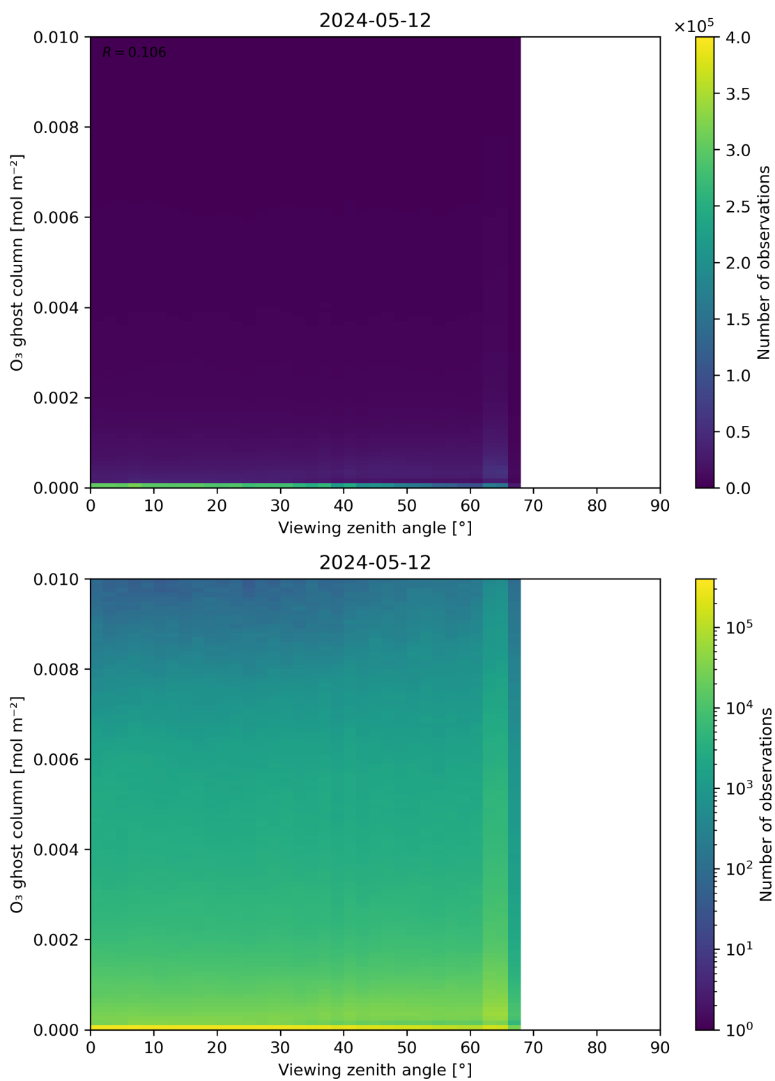
Figure 51: Scatter density plot of “Viewing zenith angle” against “O 3 ghost column” for 2024-05-12 to 2024-05-13.
