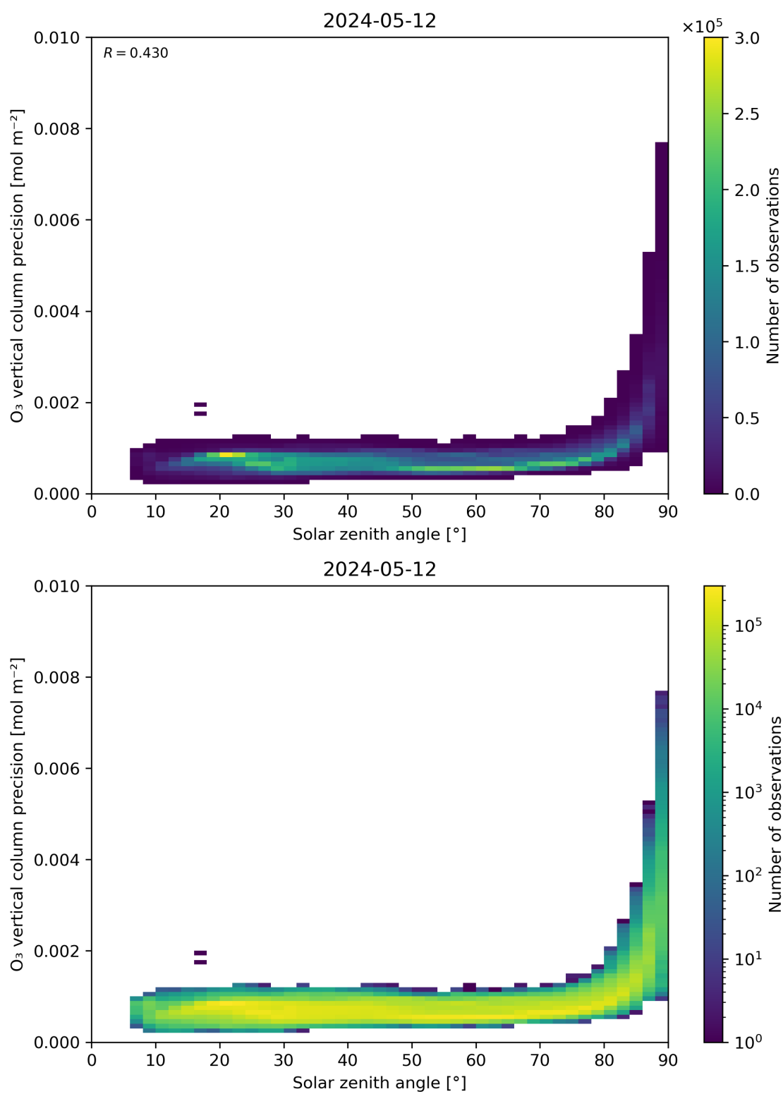
Figure 48: Scatter density plot of “Solar zenith angle” against “O 3 vertical column precision” for 2024-05-12 to 2024-05-13.
