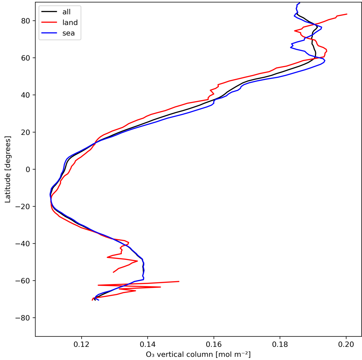
Figure 14: Zonal average of “O 3 vertical column” for 2024-05-12 to 2024-05-13.
