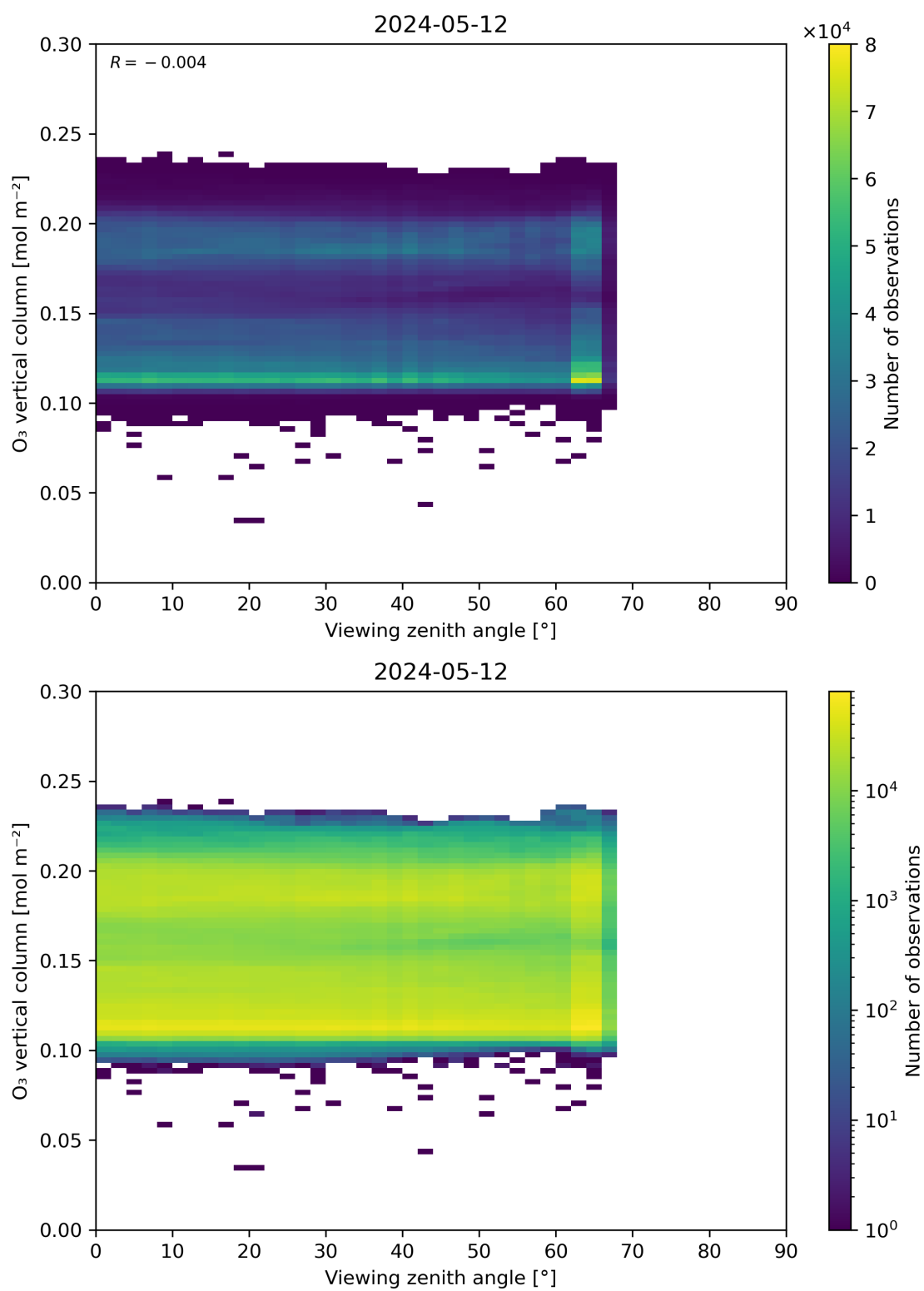
Figure 52: Scatter density plot of “Viewing zenith angle” against “O 3 vertical column” for 2024-05-12 to 2024-05-13.
