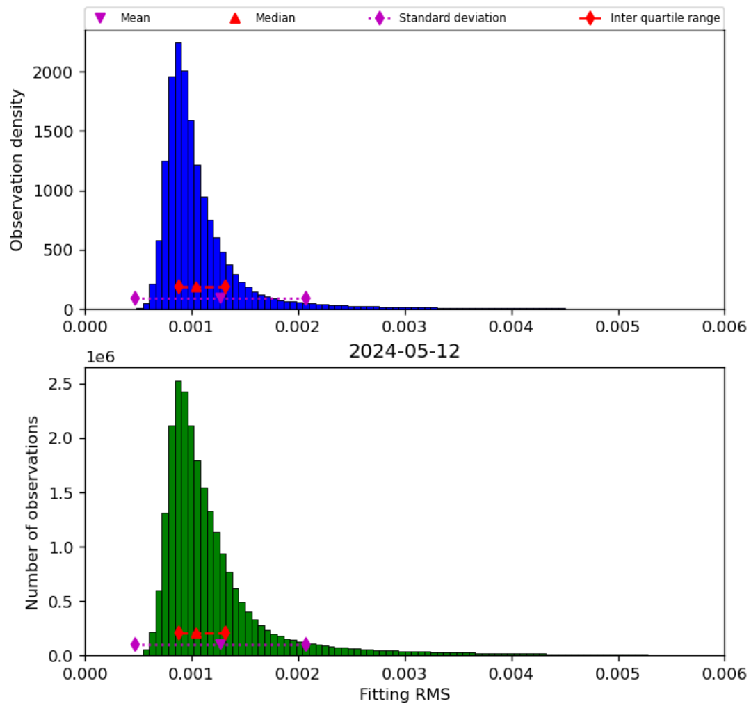
Figure 23: Histogram of “Fitting RMS” for 2024-05-12 to 2024-05-13
