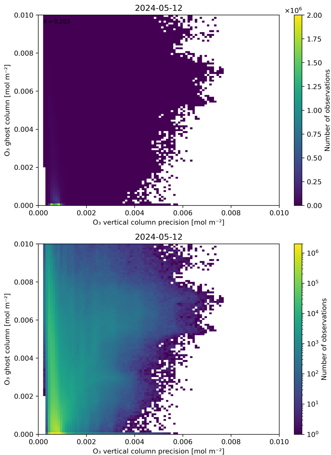
Figure 43: Scatter density plot of “ \text{O}_3 vertical column precision” against “ \text{O}_3 ghost column” for 2024-05-12 to 2024-05-13.
