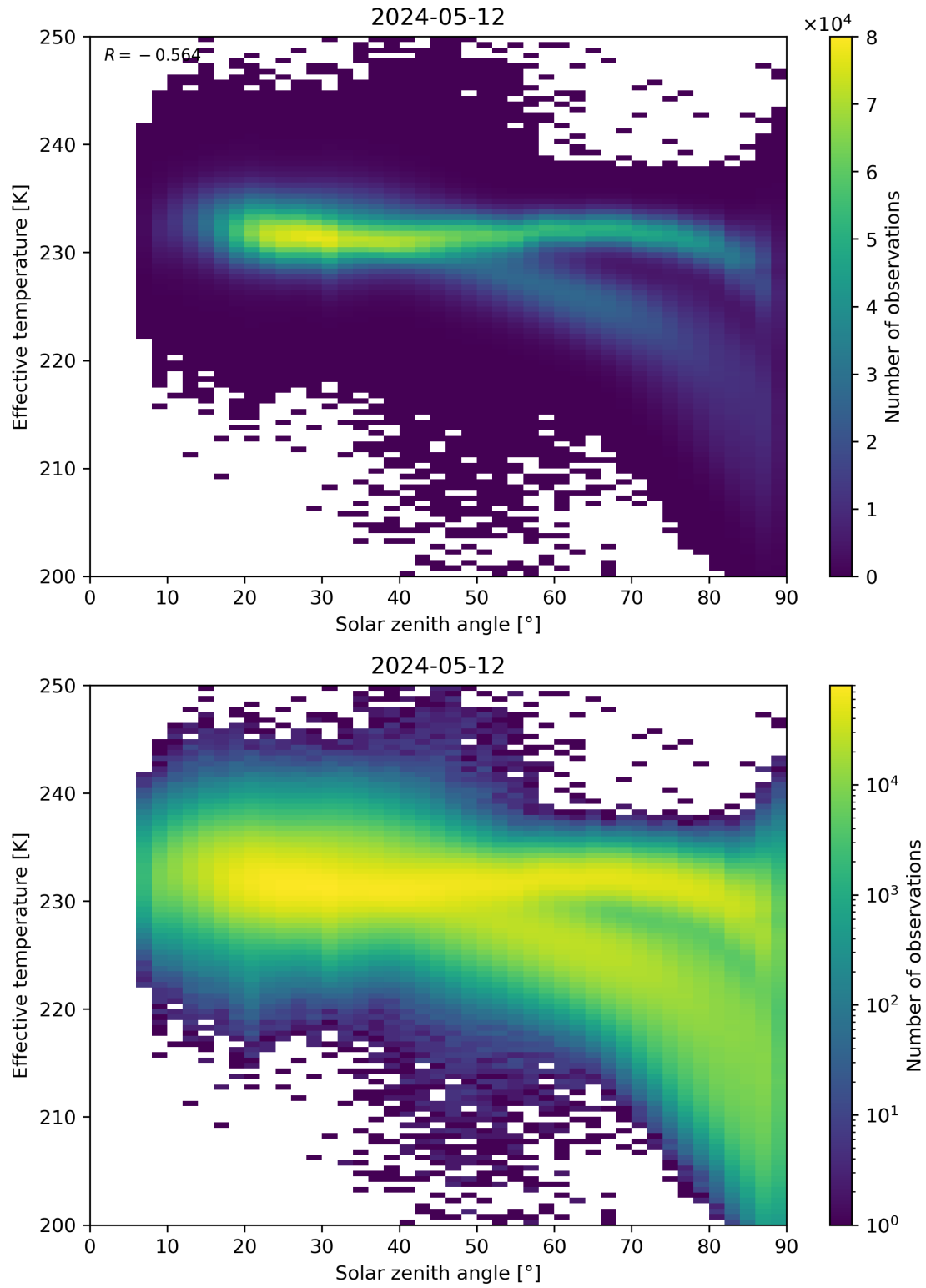
Figure 45: Scatter density plot of “Solar zenith angle” against “Effective temperature” for 2024-05-12 to 2024-05-13.
