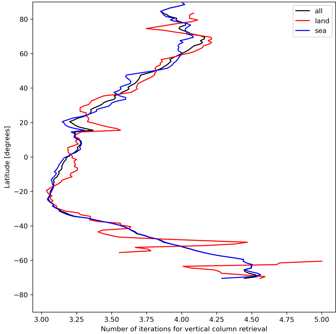
Figure 19: Zonal average of “Number of iterations for vertical column retrieval” for 2024-05-12 to 2024-05-13.
