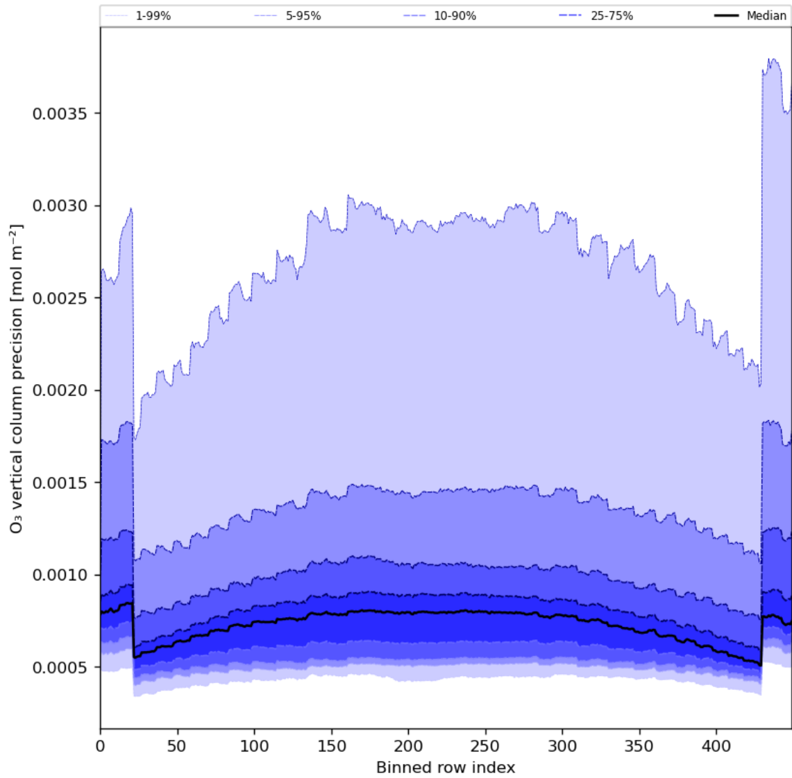
Figure 29: Along track statistics of “O 3 vertical column precision” for 2024-05-12 to 2024-05-13
