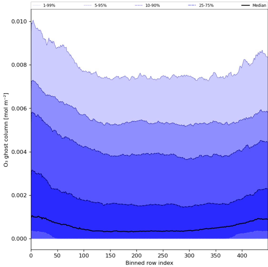
Figure 32: Along track statistics of “O 3 ghost column” for 2024-05-12 to 2024-05-13
