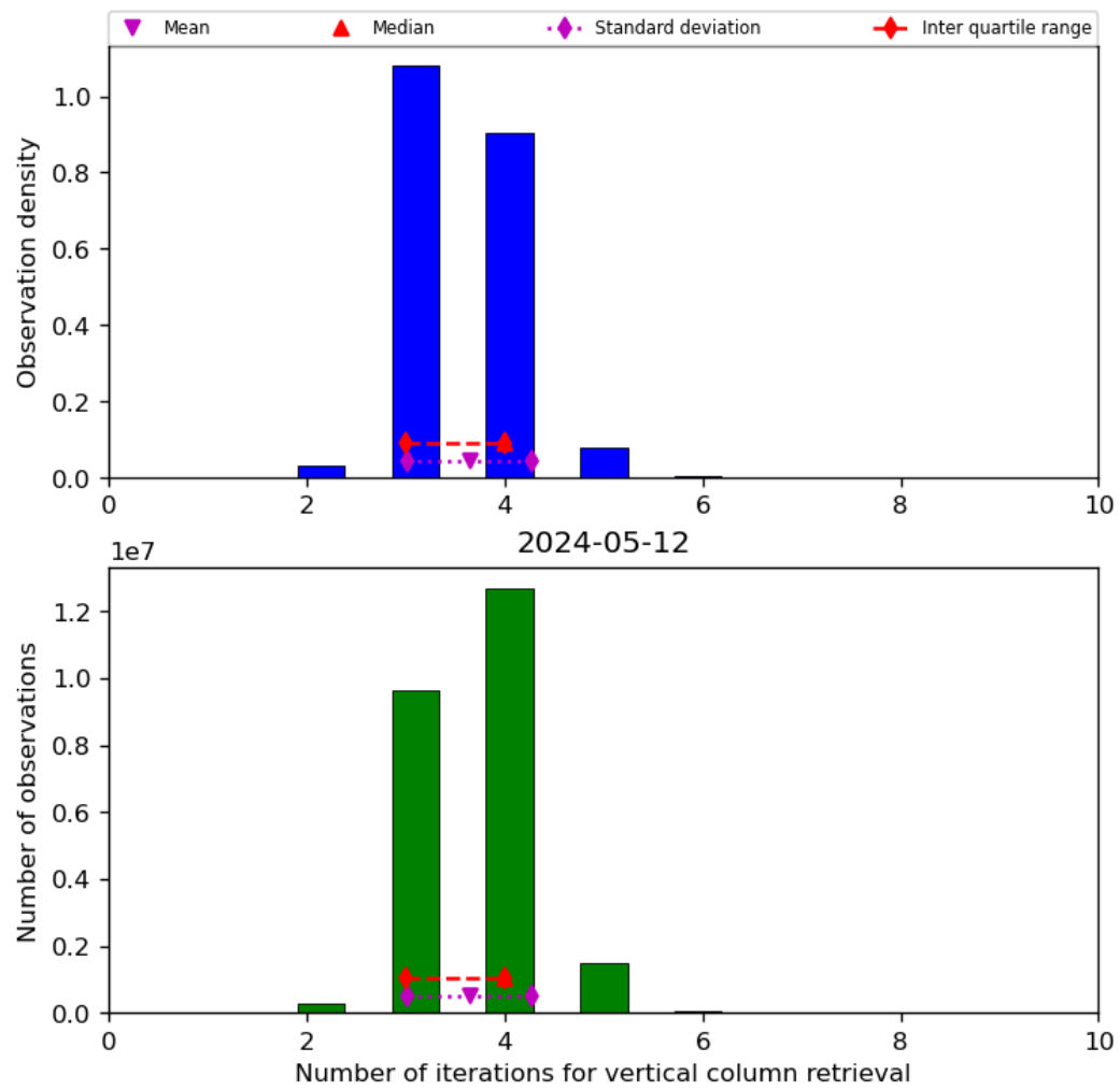
Figure 26: Histogram of “Number of iterations for vertical column retrieval” for 2024-05-12 to 2024-05-13
