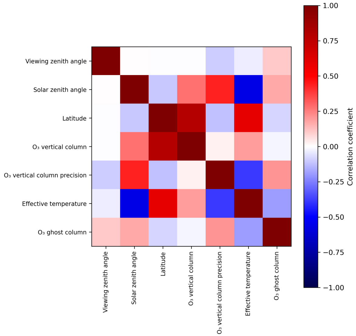
Figure 2: Map of correlation matrix for 2024-05-12 to 2024-05-13.
