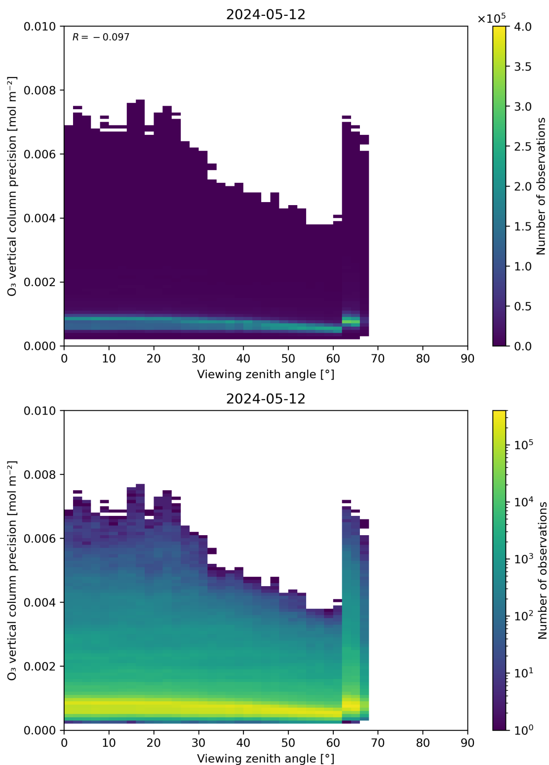
Figure 53: Scatter density plot of “Viewing zenith angle” against “O 3 vertical column precision” for 2024-05-12 to 2024-05-13.
