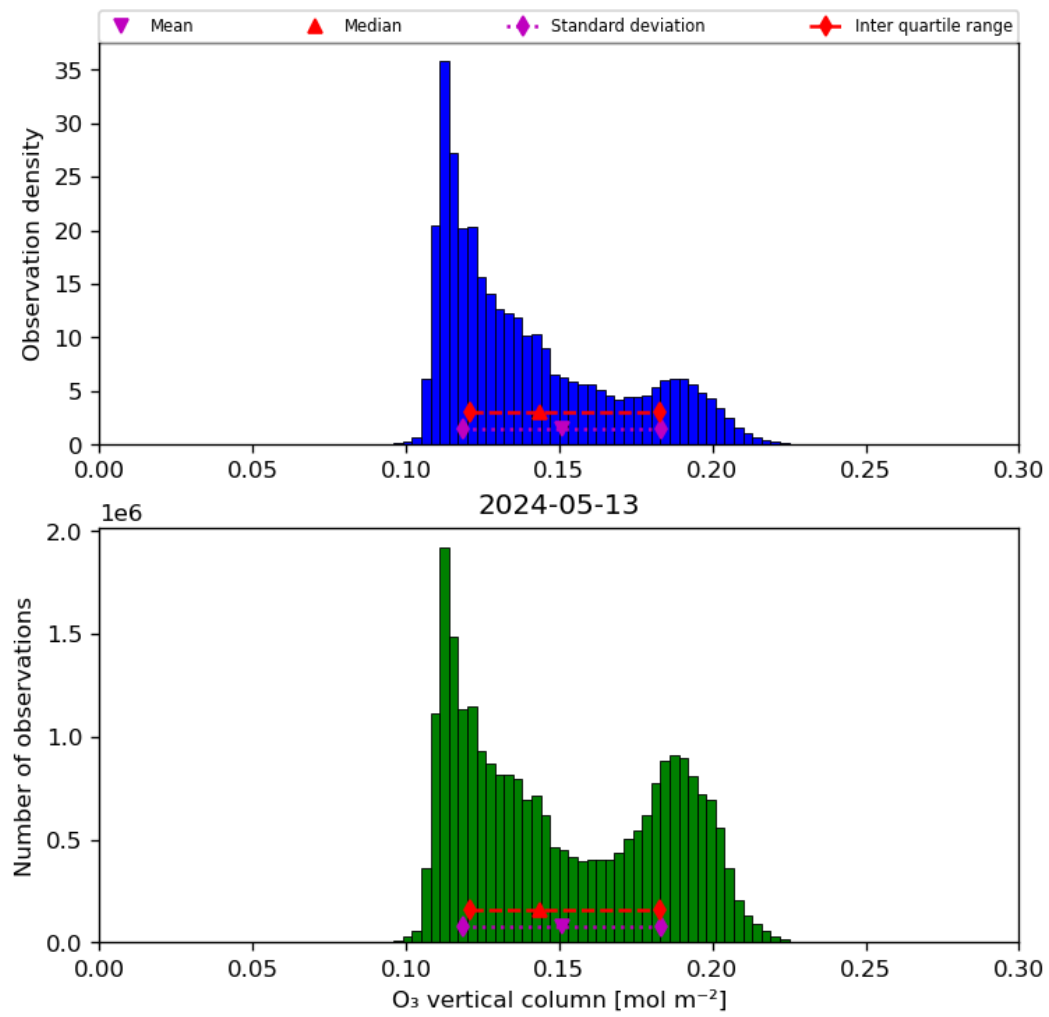
Figure 21: Histogram of “O 3 vertical column” for 2024-05-12 to 2024-05-14
