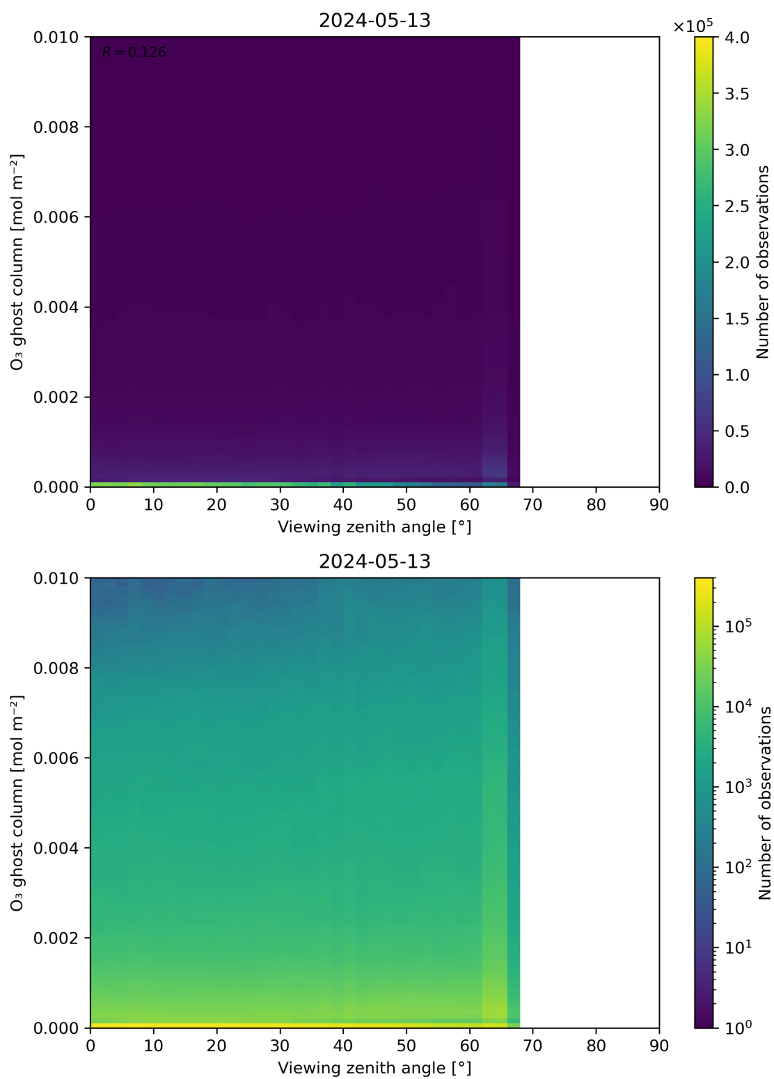
Figure 51: Scatter density plot of “Viewing zenith angle” against “O 3 ghost column” for 2024-05-12 to 2024-05-14.
