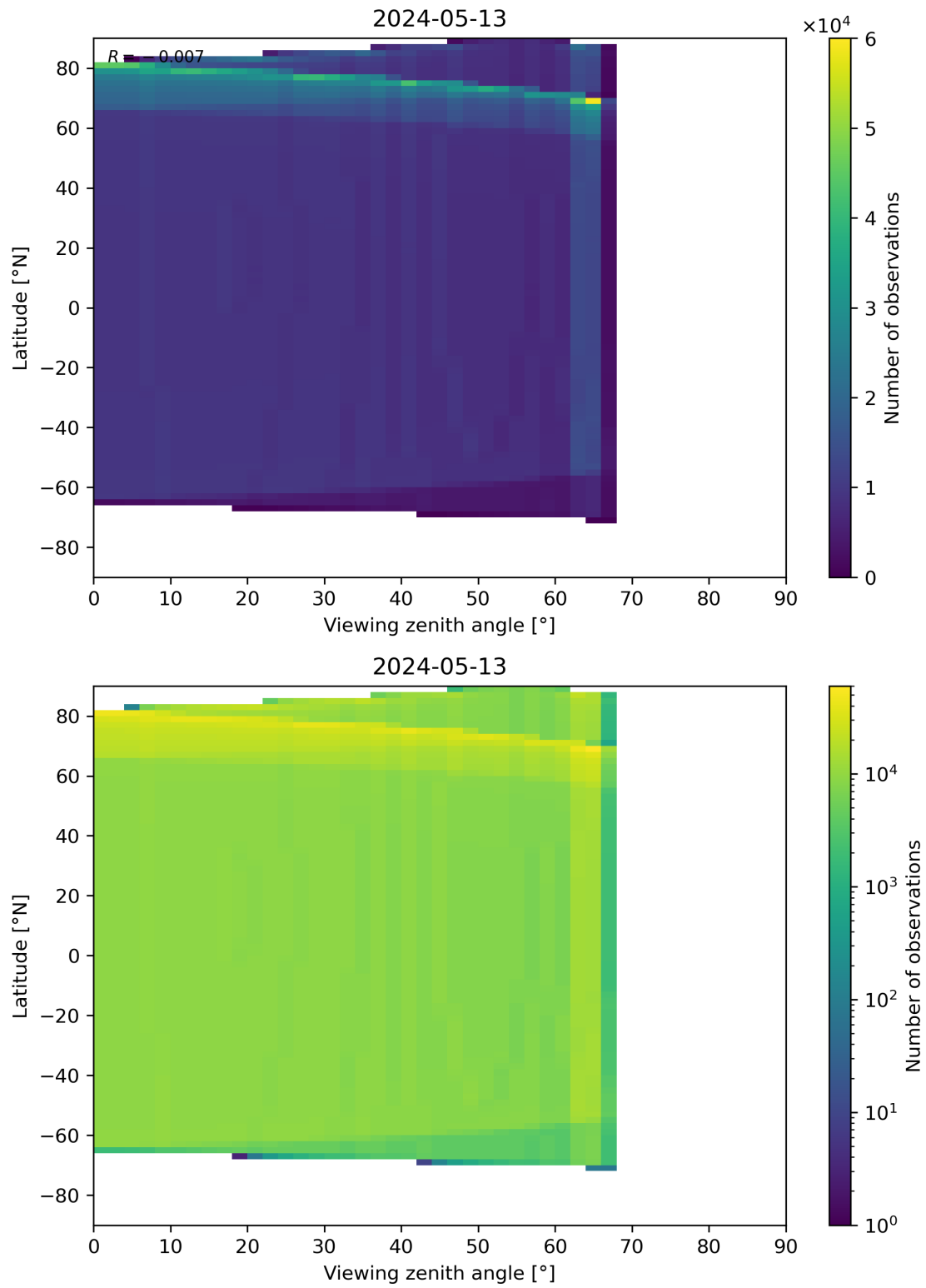
Figure 49: Scatter density plot of “Viewing zenith angle” against “Latitude” for 2024-05-12 to 2024-05-14.
