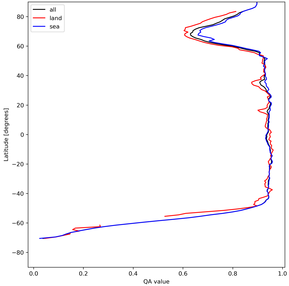
Figure 13: Zonal average of “QA value” for 2024-05-12 to 2024-05-14.
