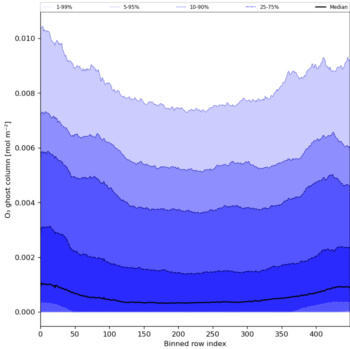
Figure 32: Along track statistics of “O 3 ghost column” for 2024-05-12 to 2024-05-14
