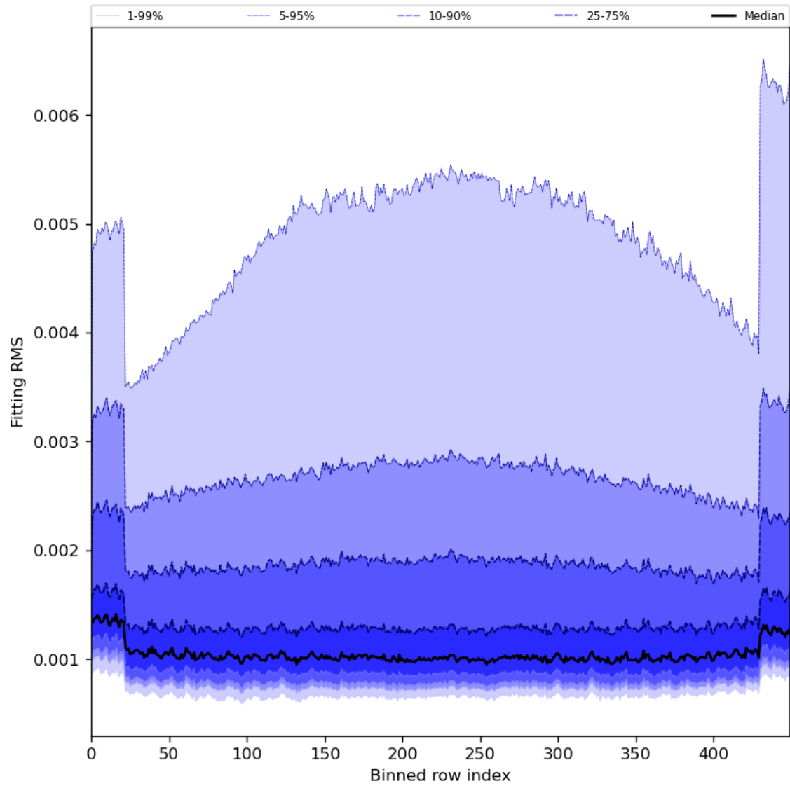
Figure 30: Along track statistics of “Fitting RMS” for 2024-05-12 to 2024-05-14
