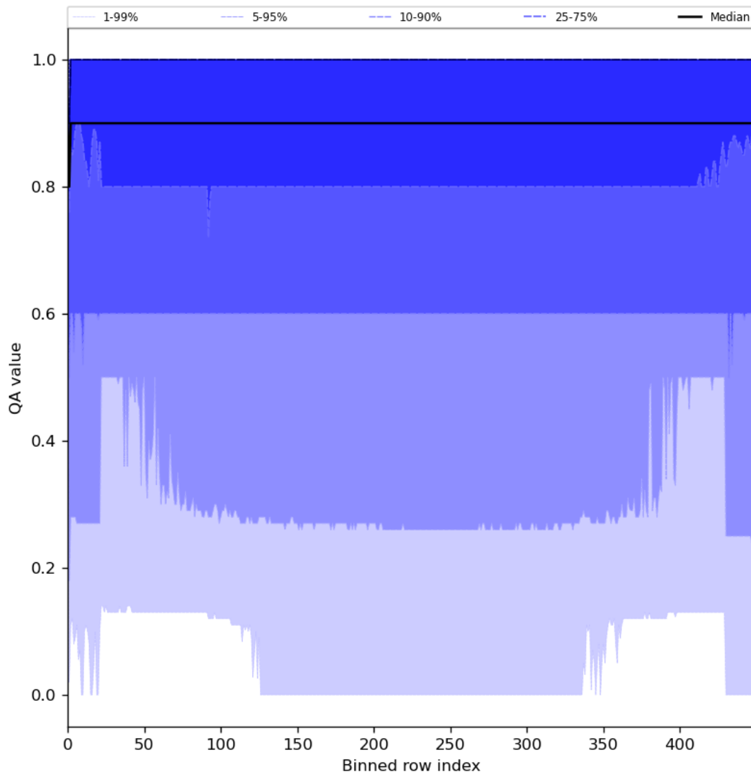
Figure 27: Along track statistics of “QA value” for 2024-05-12 to 2024-05-14
