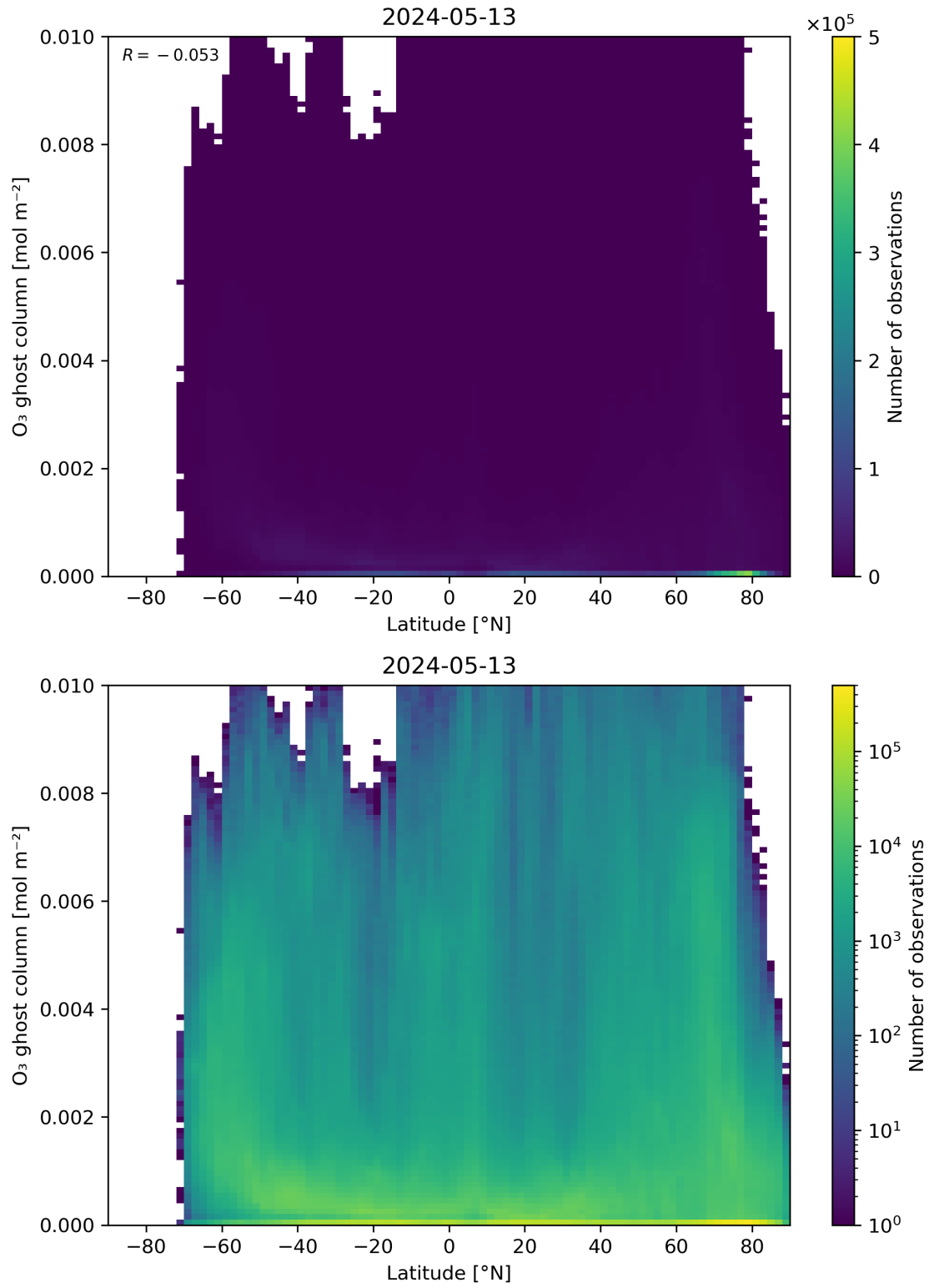
Figure 35: Scatter density plot of “Latitude” against “O 3 ghost column” for 2024-05-12 to 2024-05-14.
