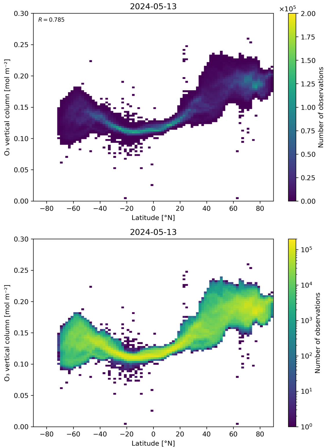
Figure 36: Scatter density plot of “Latitude” against “O 3 vertical column” for 2024-05-12 to 2024-05-14.
