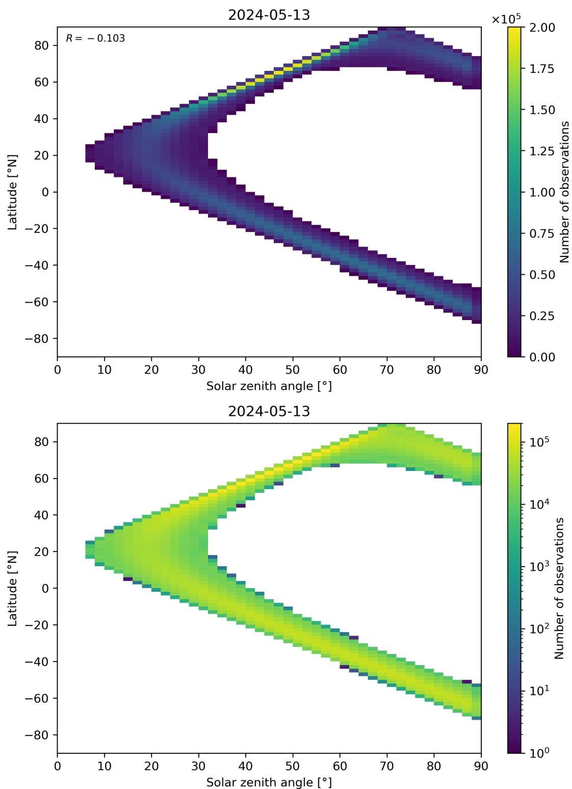
Figure 44: Scatter density plot of “Solar zenith angle” against “Latitude” for 2024-05-12 to 2024-05-14.
