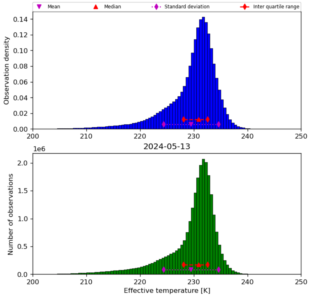
Figure 24: Histogram of “Effective temperature” for 2024-05-12 to 2024-05-14
