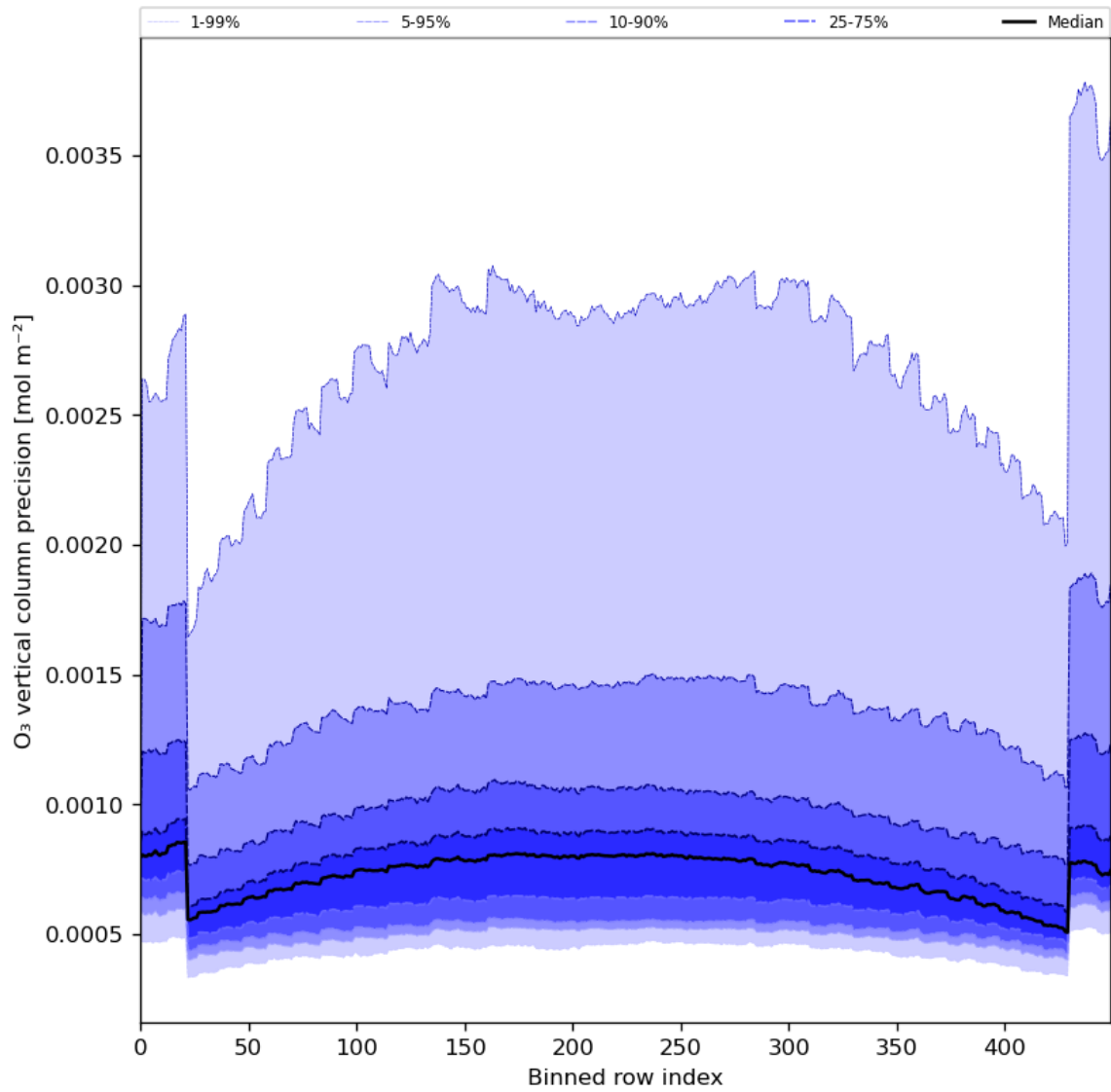
Figure 29: Along track statistics of “O 3 vertical column precision” for 2024-05-12 to 2024-05-14
