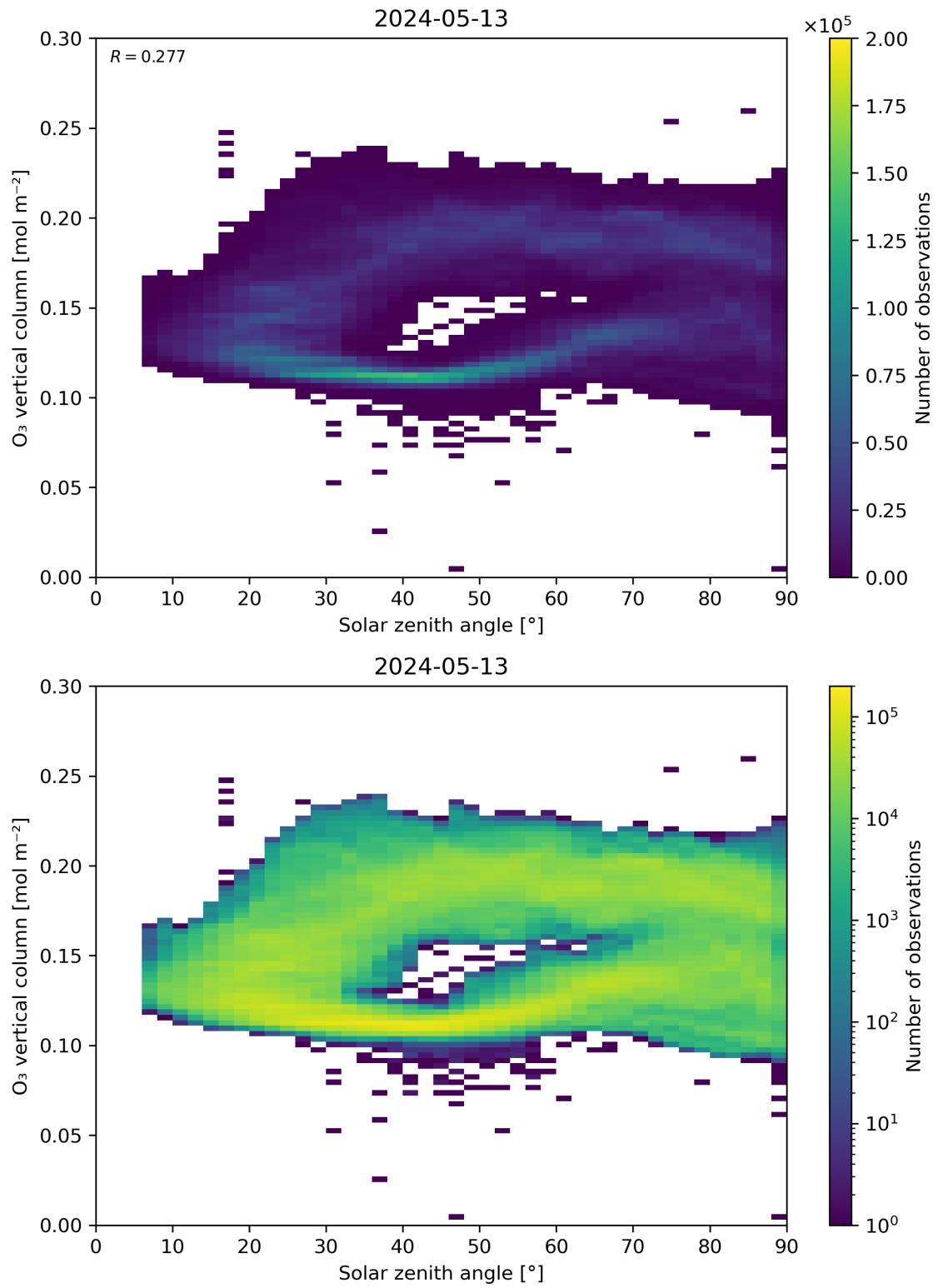
Figure 47: Scatter density plot of “Solar zenith angle” against “O 3 vertical column” for 2024-05-12 to 2024-05-14.
