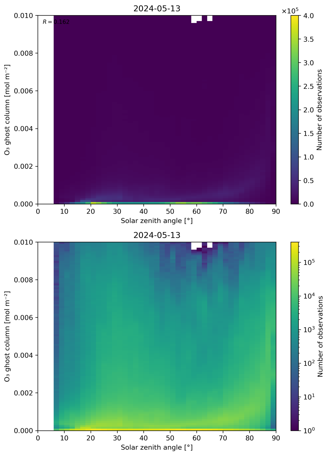
Figure 46: Scatter density plot of “Solar zenith angle” against “O 3 ghost column” for 2024-05-12 to 2024-05-14.
