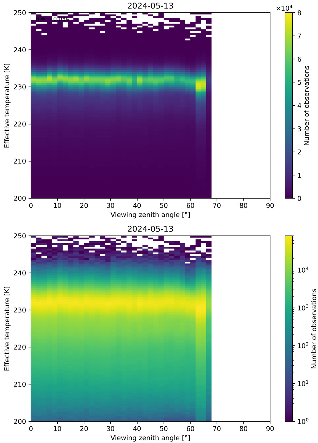
Figure 50: Scatter density plot of “Viewing zenith angle” against “Effective temperature” for 2024-05-12 to 2024-05-14.
