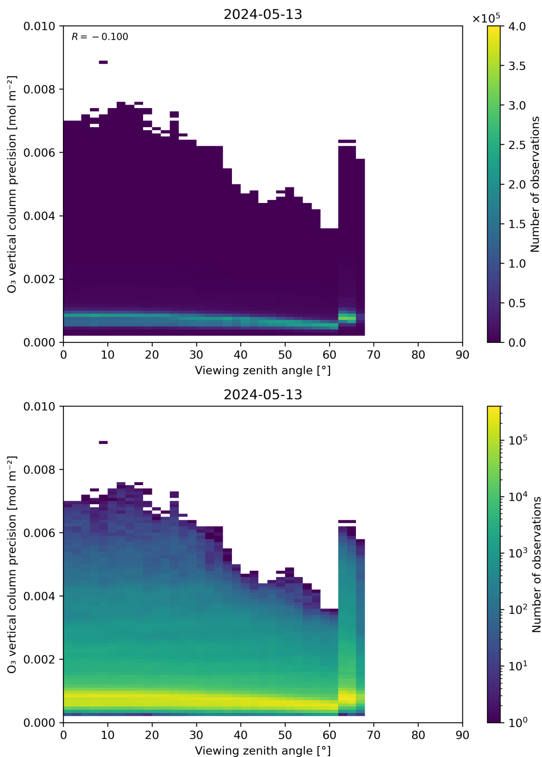
Figure 53: Scatter density plot of “Viewing zenith angle” against “O 3 vertical column precision” for 2024-05-12 to 2024-05-14.
