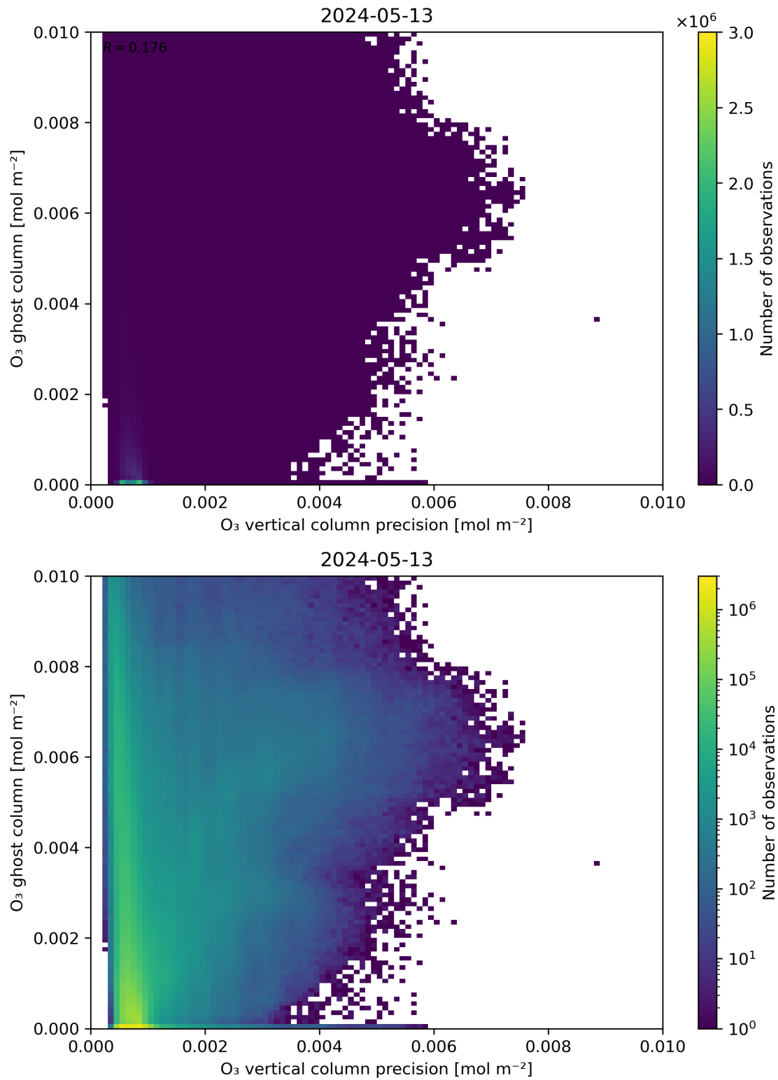
Figure 43: Scatter density plot of “ \text{O}_3 vertical column precision” against “ \text{O}_3 ghost column” for 2024-05-12 to 2024-05-14.
