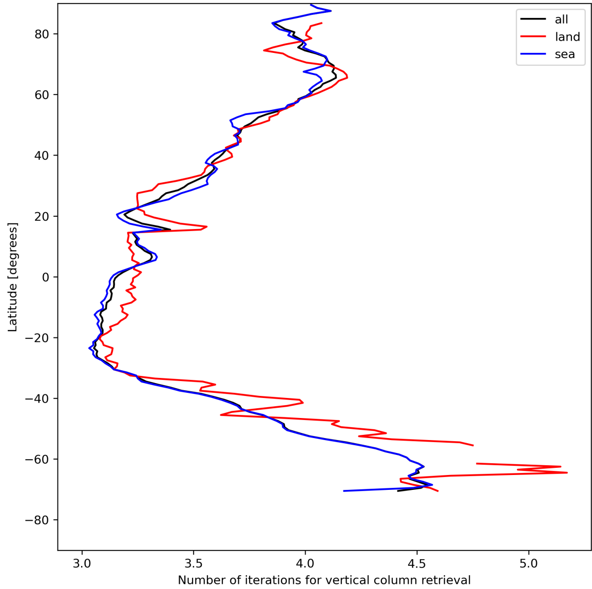
Figure 19: Zonal average of “Number of iterations for vertical column retrieval” for 2024-05-12 to 2024-05-14.
