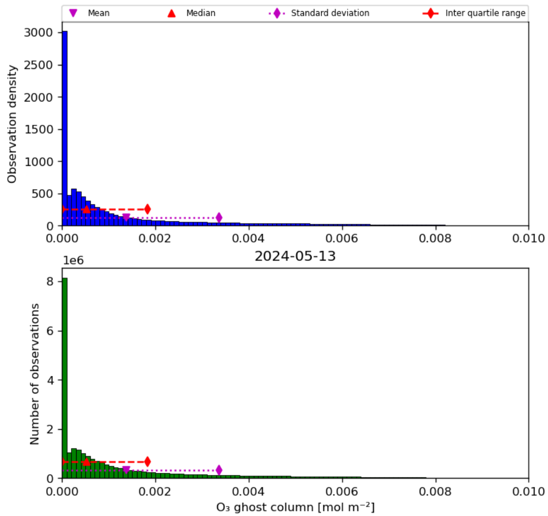
Figure 25: Histogram of “O 3 ghost column” for 2024-05-12 to 2024-05-14
