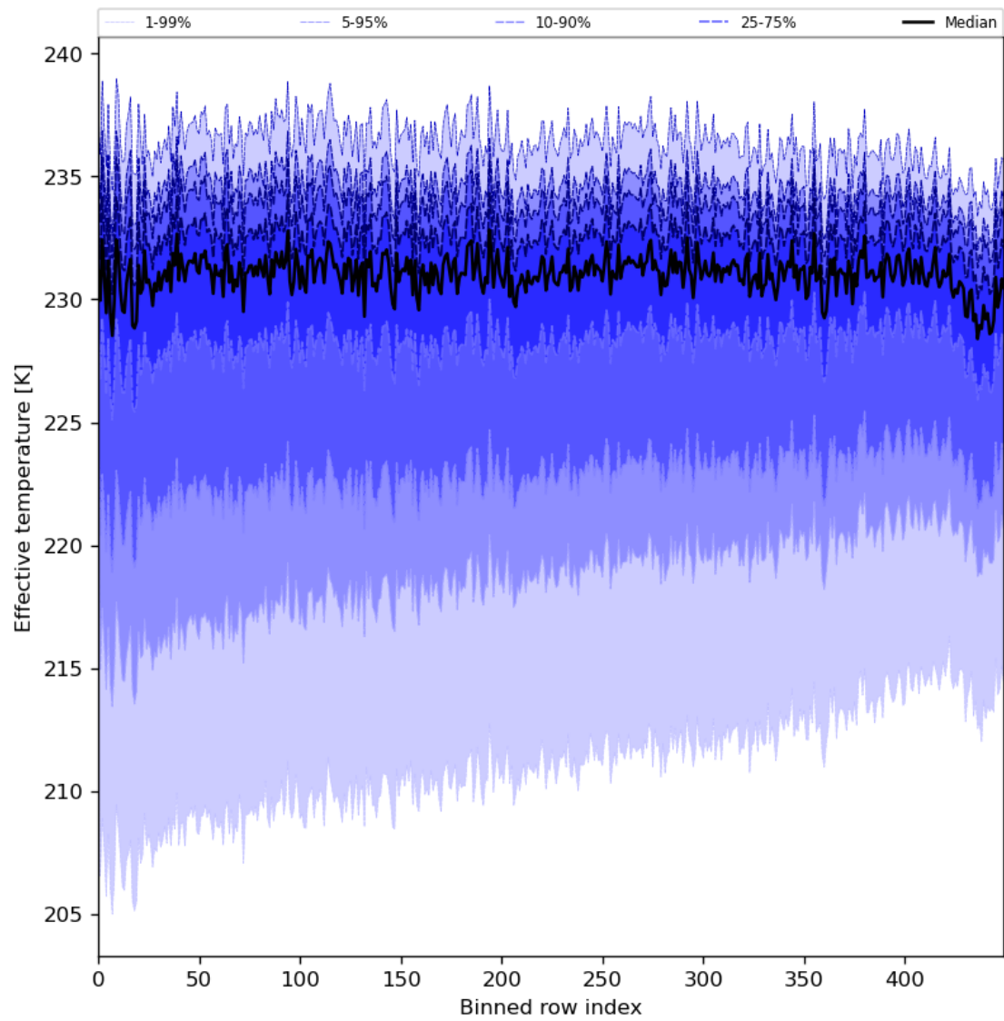
Figure 31: Along track statistics of “Effective temperature” for 2024-05-12 to 2024-05-14
