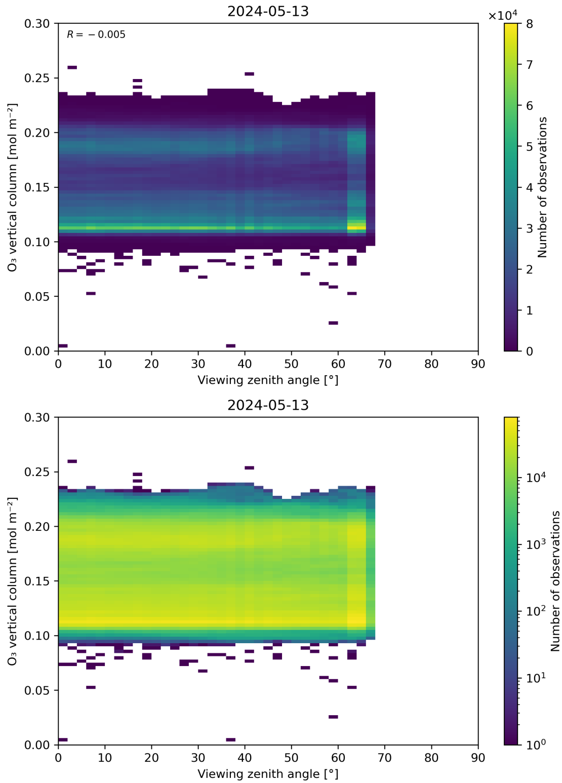
Figure 52: Scatter density plot of “Viewing zenith angle” against “O 3 vertical column” for 2024-05-12 to 2024-05-14.
