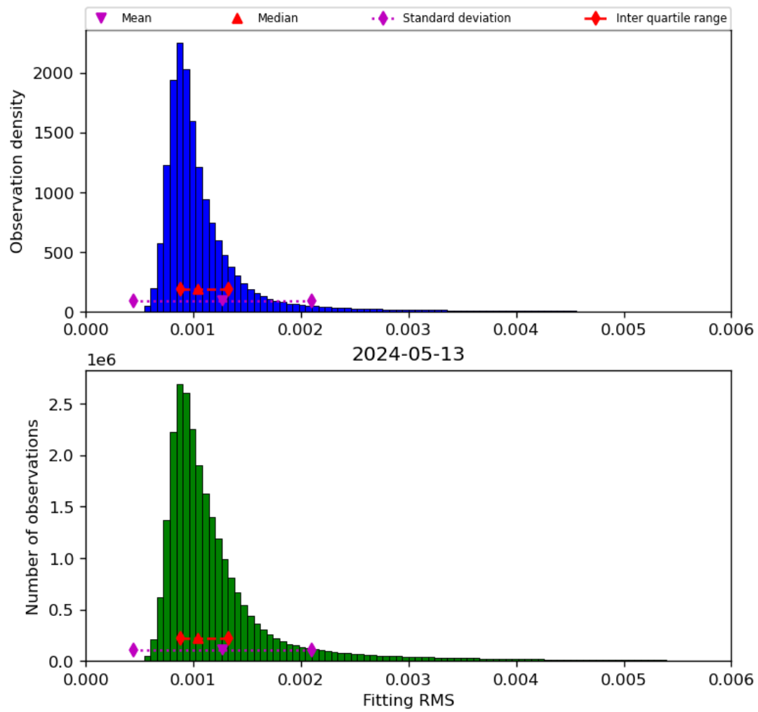
Figure 23: Histogram of “Fitting RMS” for 2024-05-12 to 2024-05-14
