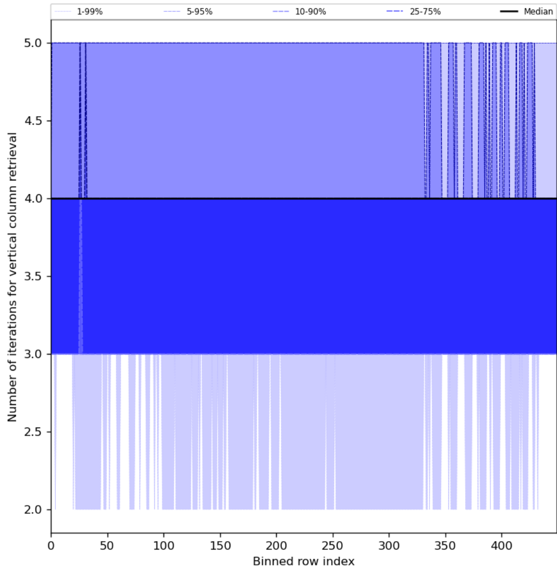
Figure 33: Along track statistics of “Number of iterations for vertical column retrieval” for 2024-05-12 to 2024-05-14
