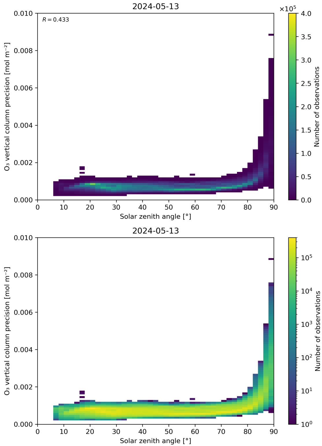
Figure 48: Scatter density plot of “Solar zenith angle” against “O 3 vertical column precision” for 2024-05-12 to 2024-05-14.
