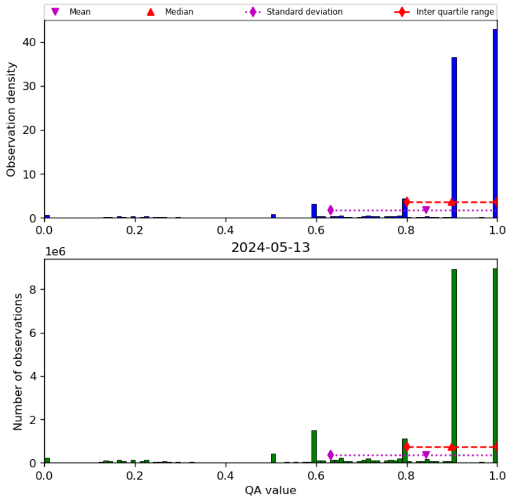
Figure 20: Histogram of “QA value” for 2024-05-12 to 2024-05-14
