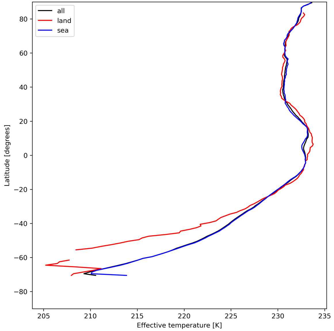
Figure 17: Zonal average of "Effective temperature" for 2024-05-12 to 2024-05-14.
