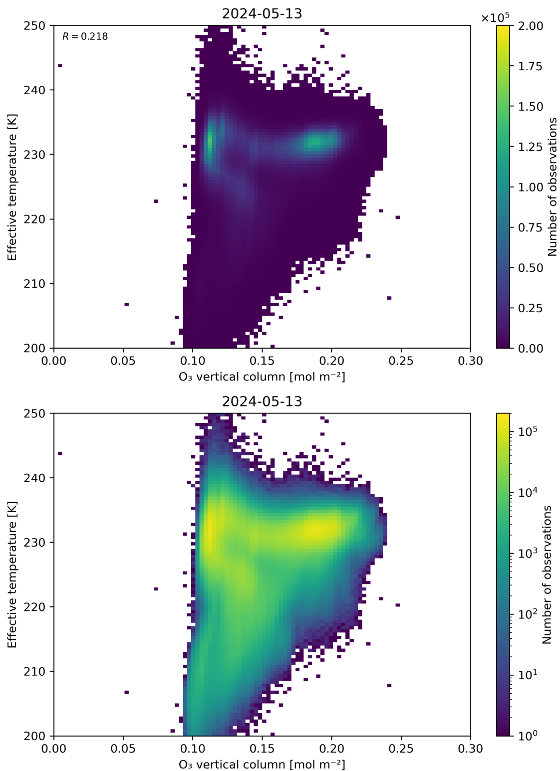
Figure 39: Scatter density plot of “O 3 vertical column” against “Effective temperature” for 2024-05-12 to 2024-05-14.
