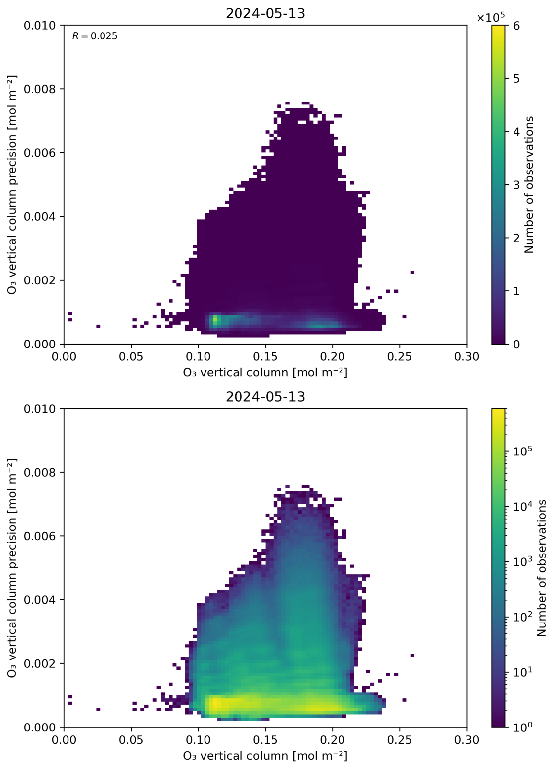
Figure 41: Scatter density plot of “O 3 vertical column” against “O 3 vertical column precision” for 2024-05-12 to 2024-05-14.
