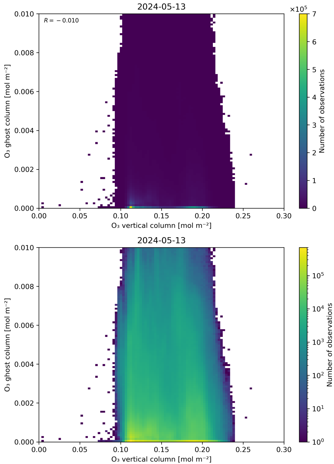
Figure 40: Scatter density plot of “O 3 vertical column” against “O 3 ghost column” for 2024-05-12 to 2024-05-14.
