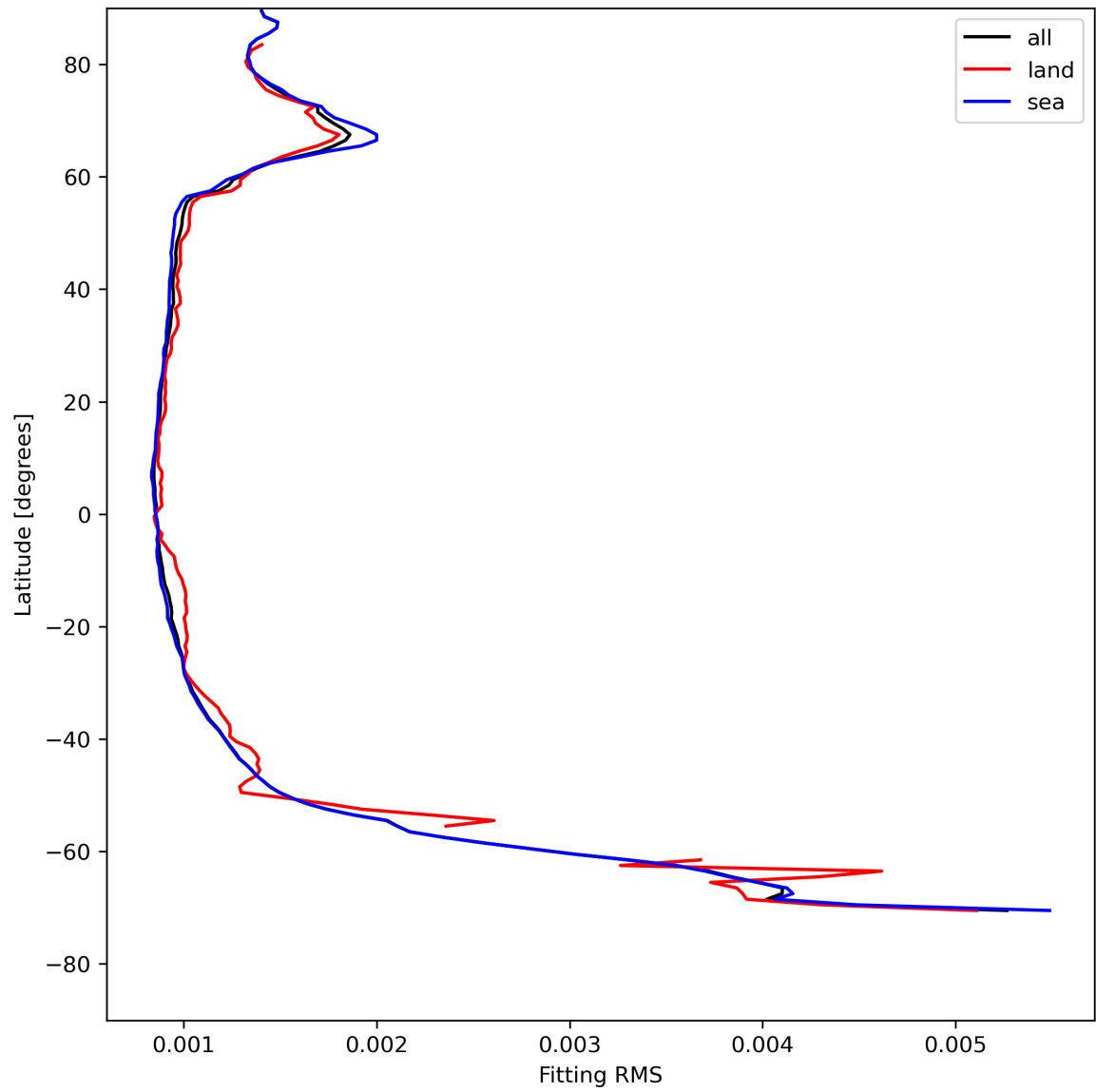
Figure 16: Zonal average of “Fitting RMS” for 2024-05-12 to 2024-05-14.
