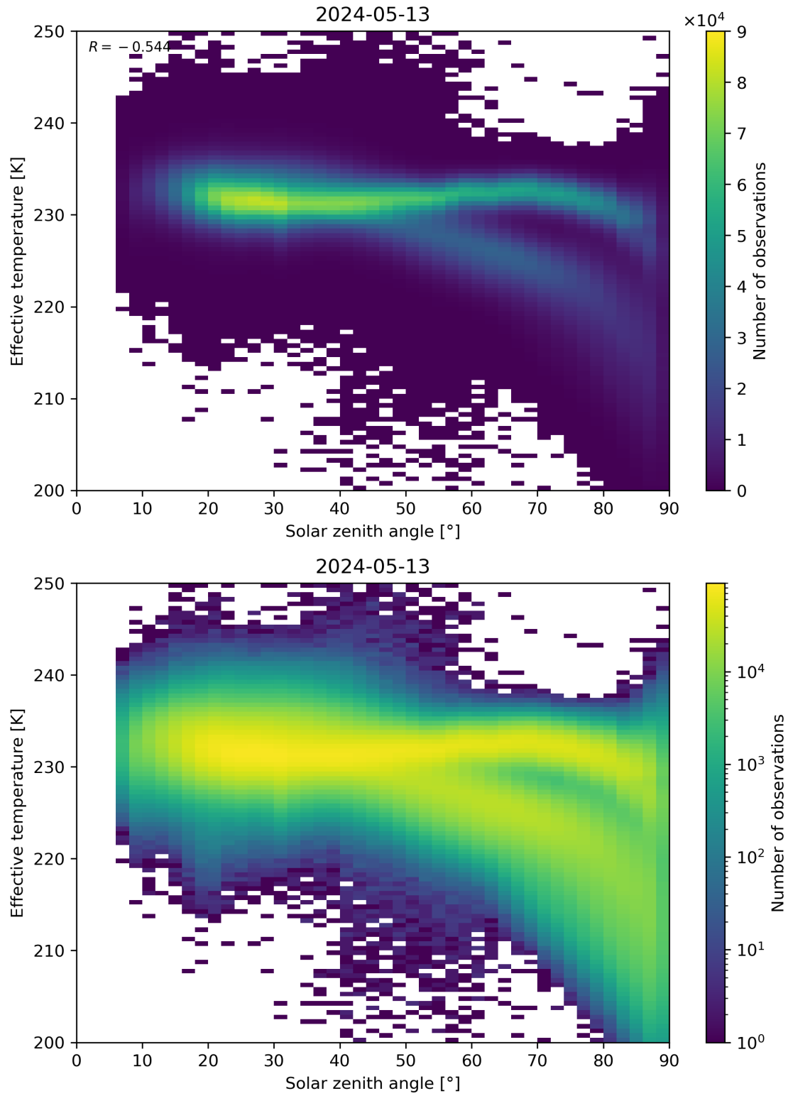
Figure 45: Scatter density plot of “Solar zenith angle” against “Effective temperature” for 2024-05-12 to 2024-05-14.
