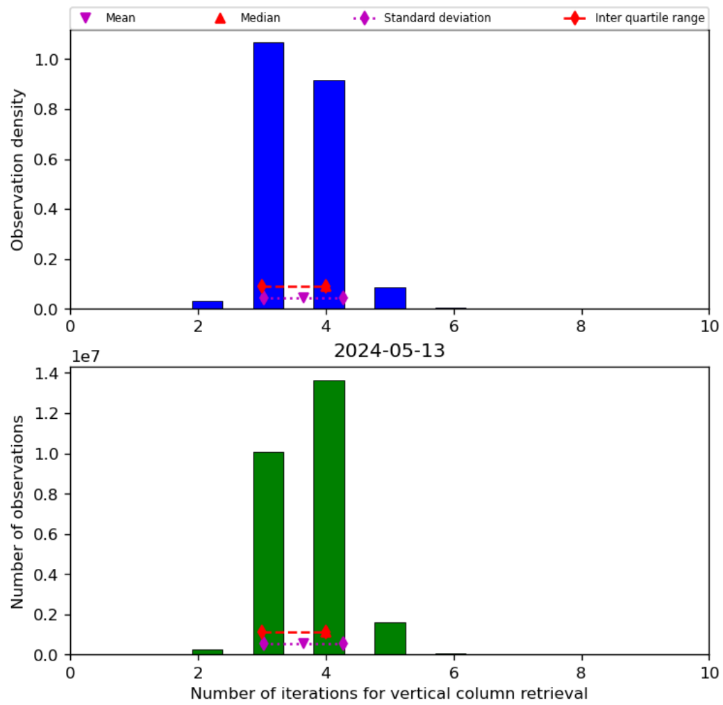
Figure 26: Histogram of “Number of iterations for vertical column retrieval” for 2024-05-12 to 2024-05-14
