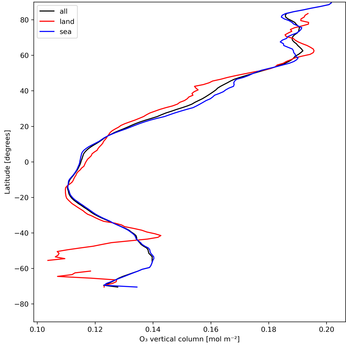
Figure 14: Zonal average of “O 3 vertical column” for 2024-05-12 to 2024-05-14.
