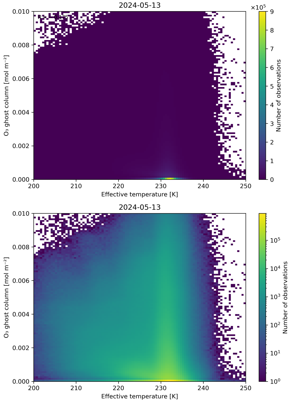
Figure 38: Scatter density plot of “Effective temperature” against “O 3 ghost column” for 2024-05-12 to 2024-05-14.
