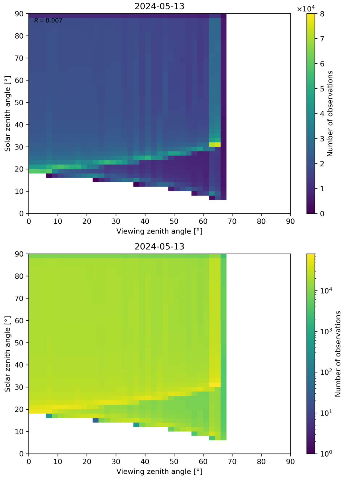
Figure 54: Scatter density plot of “Viewing zenith angle” against “Solar zenith angle” for 2024-05-12 to 2024-05-14.
