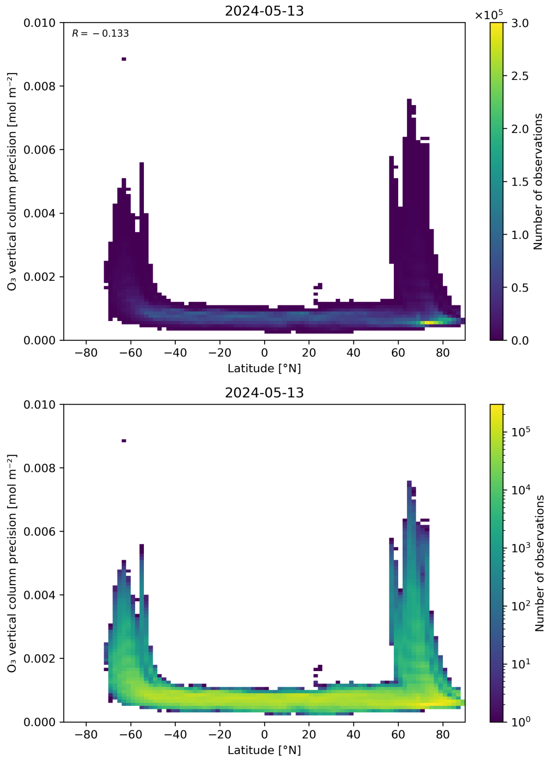
Figure 37: Scatter density plot of “Latitude” against “O 3 vertical column precision” for 2024-05-12 to 2024-05-14.
