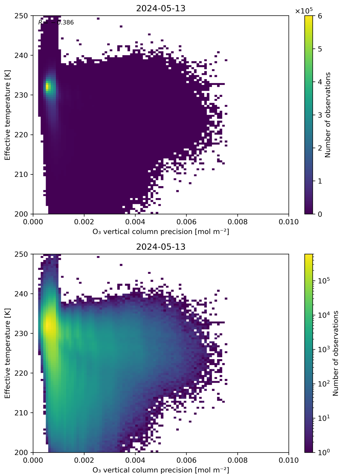
Figure 42: Scatter density plot of “O 3 vertical column precision” against “Effective temperature” for 2024-05-12 to 2024-05-14.
