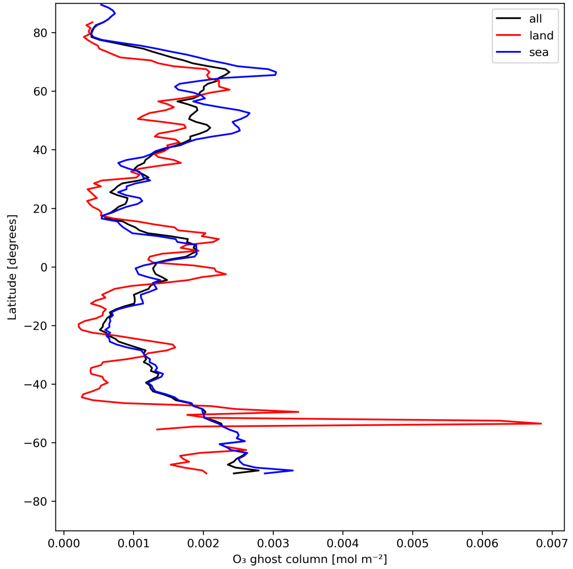
Figure 18: Zonal average of "O 3 ghost column" for 2024-05-12 to 2024-05-14.
