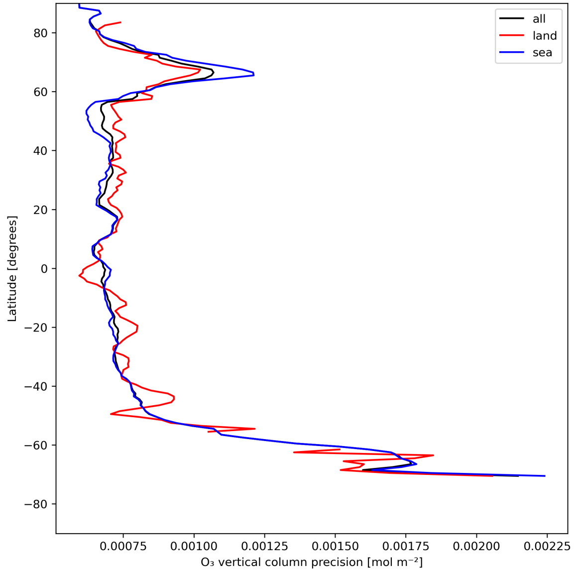
Figure 15: Zonal average of “O 3 vertical column precision” for 2024-05-12 to 2024-05-14.
