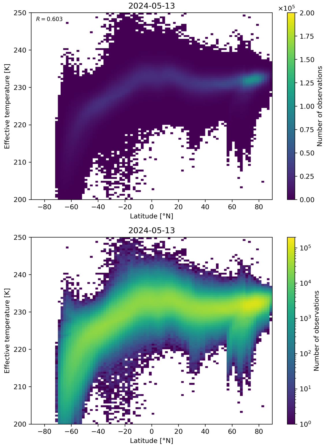
Figure 34: Scatter density plot of “Latitude” against “Effective temperature” for 2024-05-12 to 2024-05-14.
