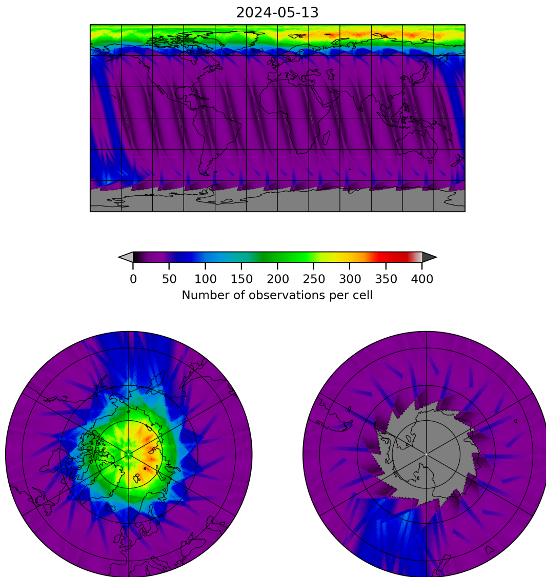
Figure 12: Map of the number of observations for 2024-05-12 to 2024-05-14
