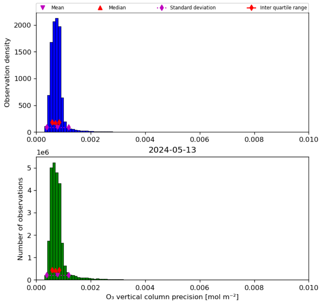
Figure 22: Histogram of “O 3 vertical column precision” for 2024-05-12 to 2024-05-14
