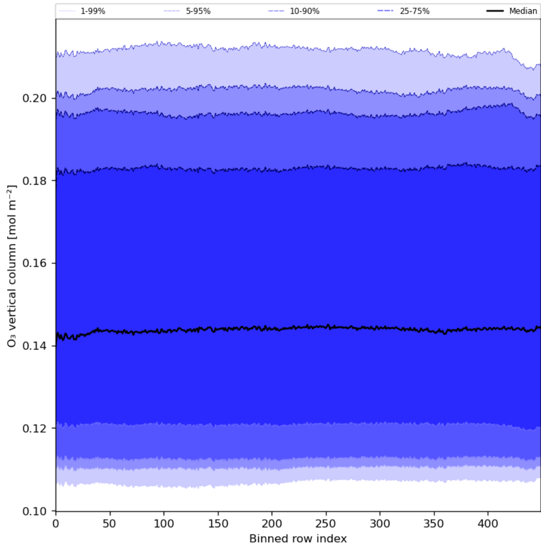
Figure 28: Along track statistics of “O 3 vertical column” for 2024-05-12 to 2024-05-14
