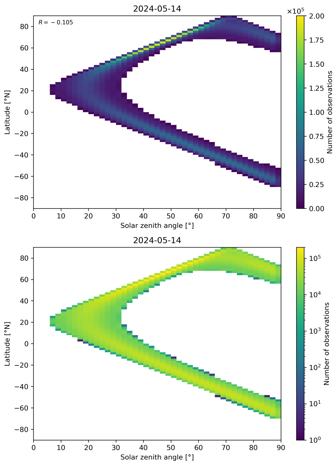
Figure 44: Scatter density plot of “Solar zenith angle” against “Latitude” for 2024-05-13 to 2024-05-15.
