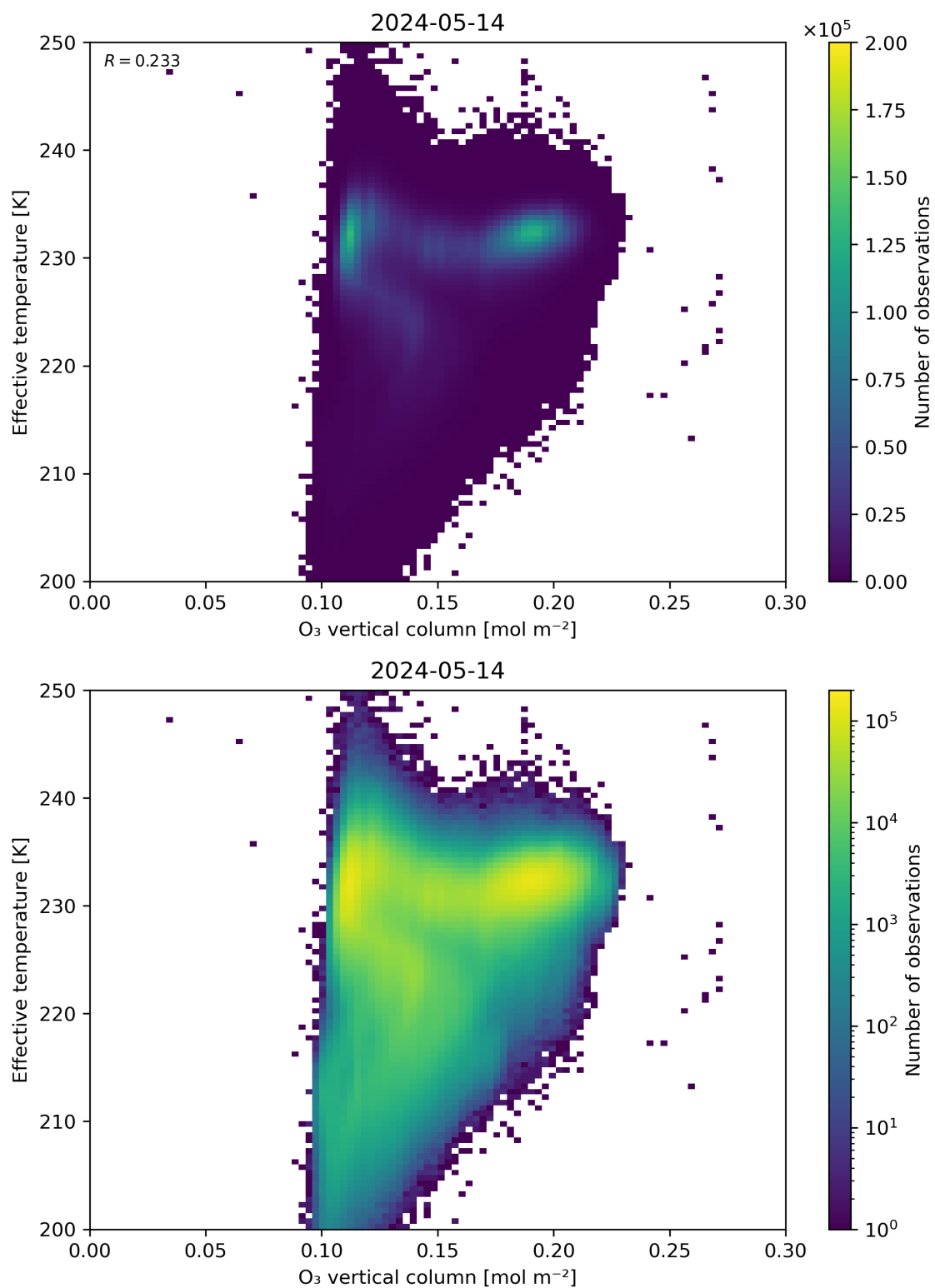
Figure 39: Scatter density plot of “O 3 vertical column” against “Effective temperature” for 2024-05-13 to 2024-05-15.
