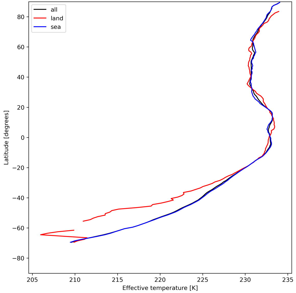
Figure 17: Zonal average of “Effective temperature” for 2024-05-13 to 2024-05-15.
