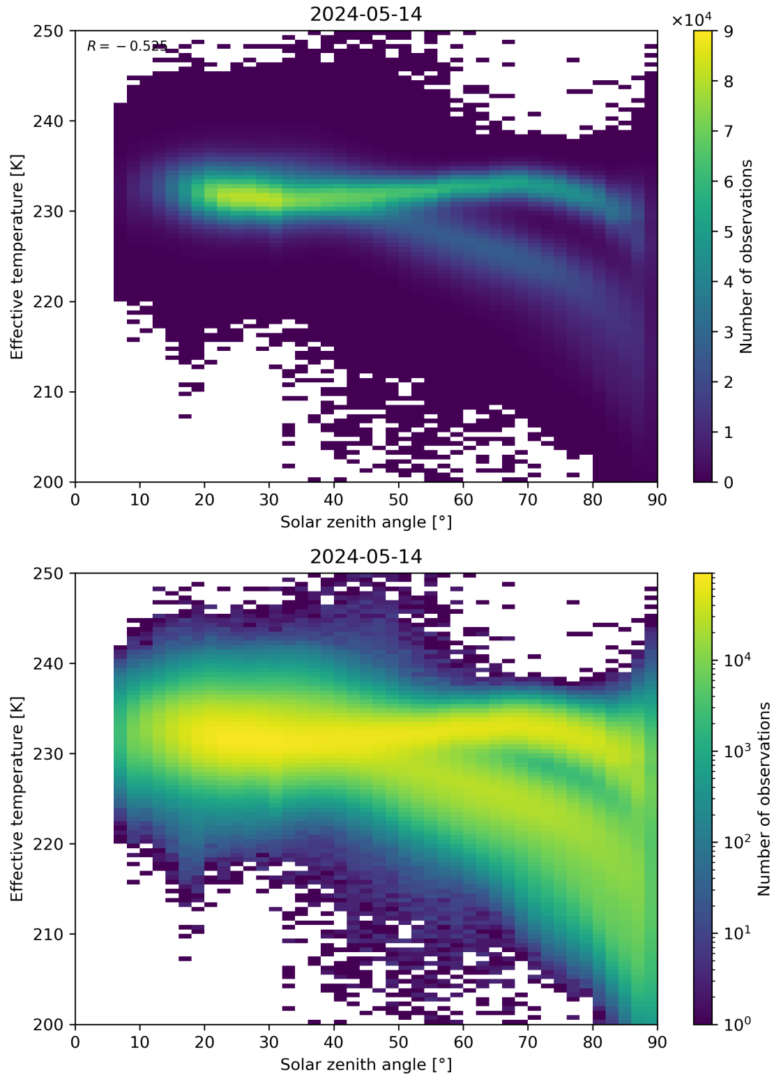
Figure 45: Scatter density plot of “Solar zenith angle” against “Effective temperature” for 2024-05-13 to 2024-05-15.
