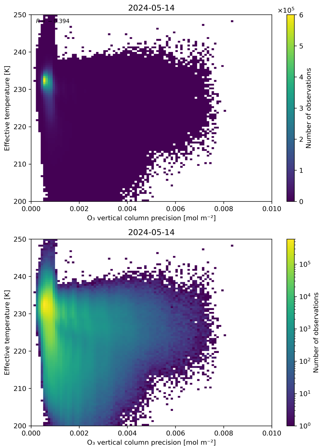
Figure 42: Scatter density plot of “O 3 vertical column precision” against “Effective temperature” for 2024-05-13 to 2024-05-15.
