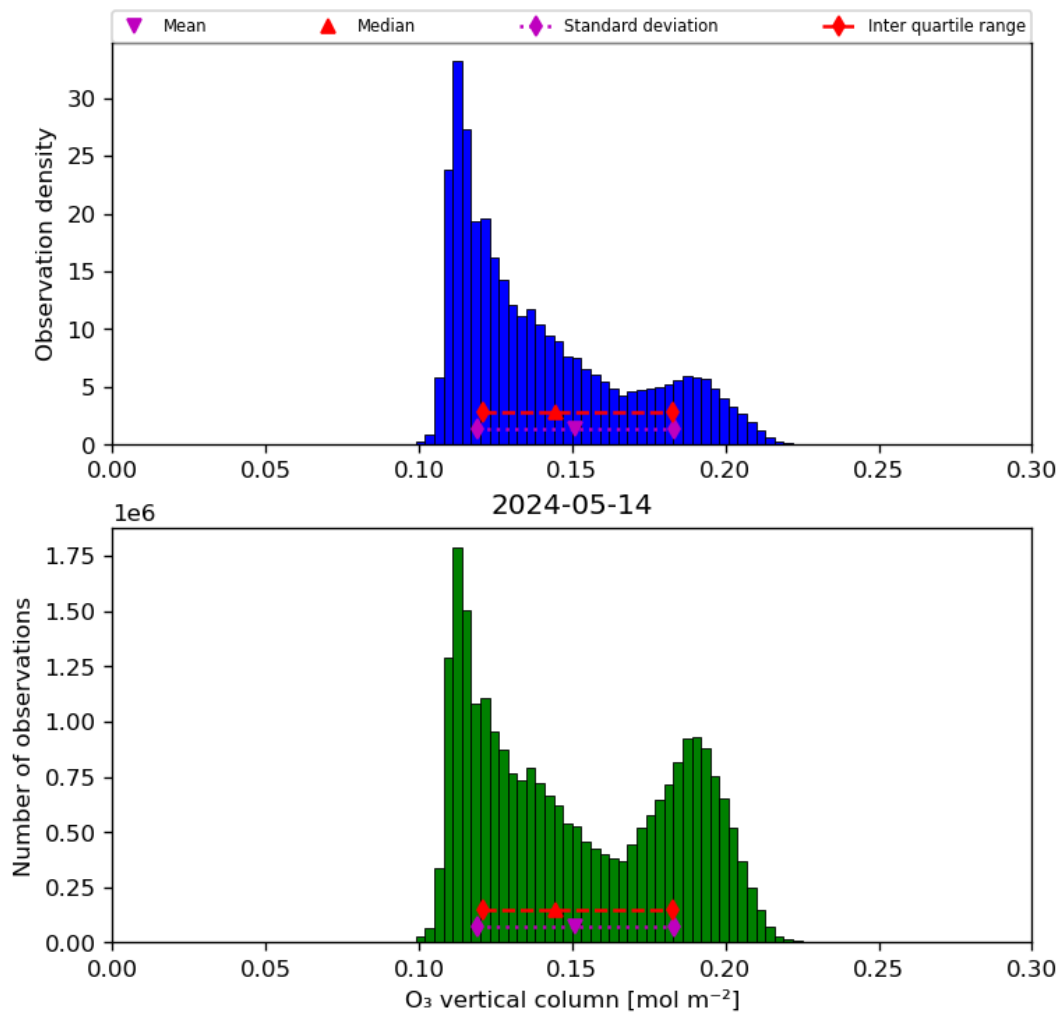
Figure 21: Histogram of “O 3 vertical column” for 2024-05-13 to 2024-05-15
