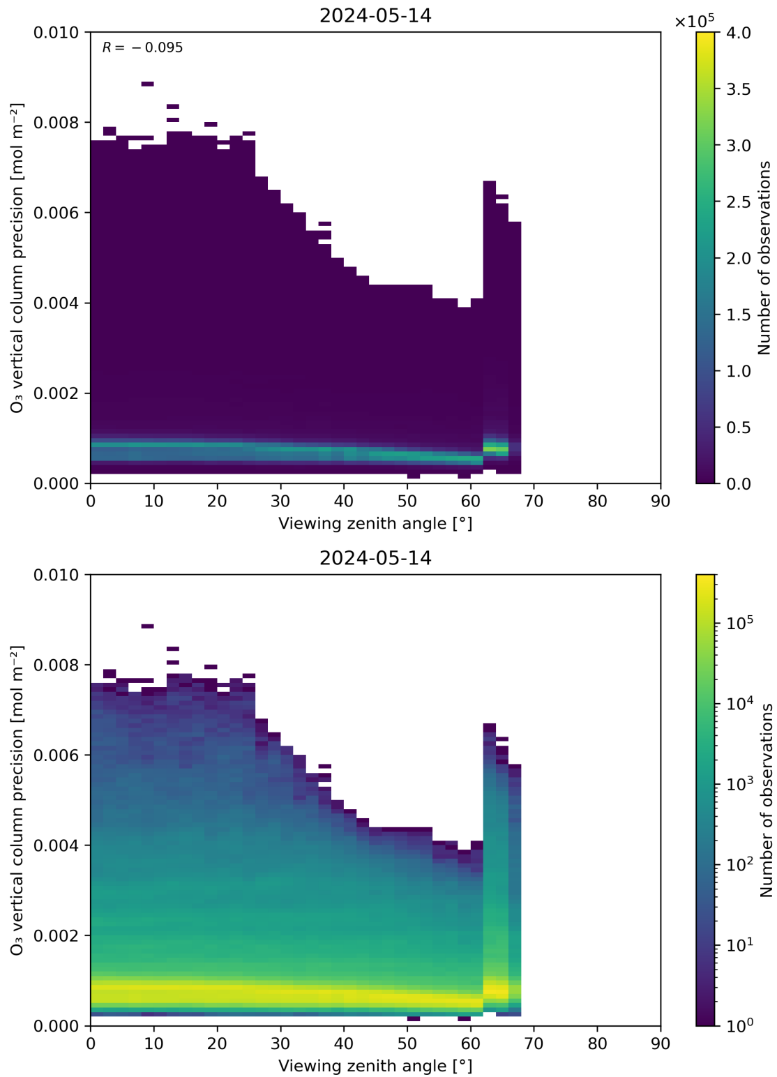
Figure 53: Scatter density plot of “Viewing zenith angle” against “O 3 vertical column precision” for 2024-05-13 to 2024-05-15.
