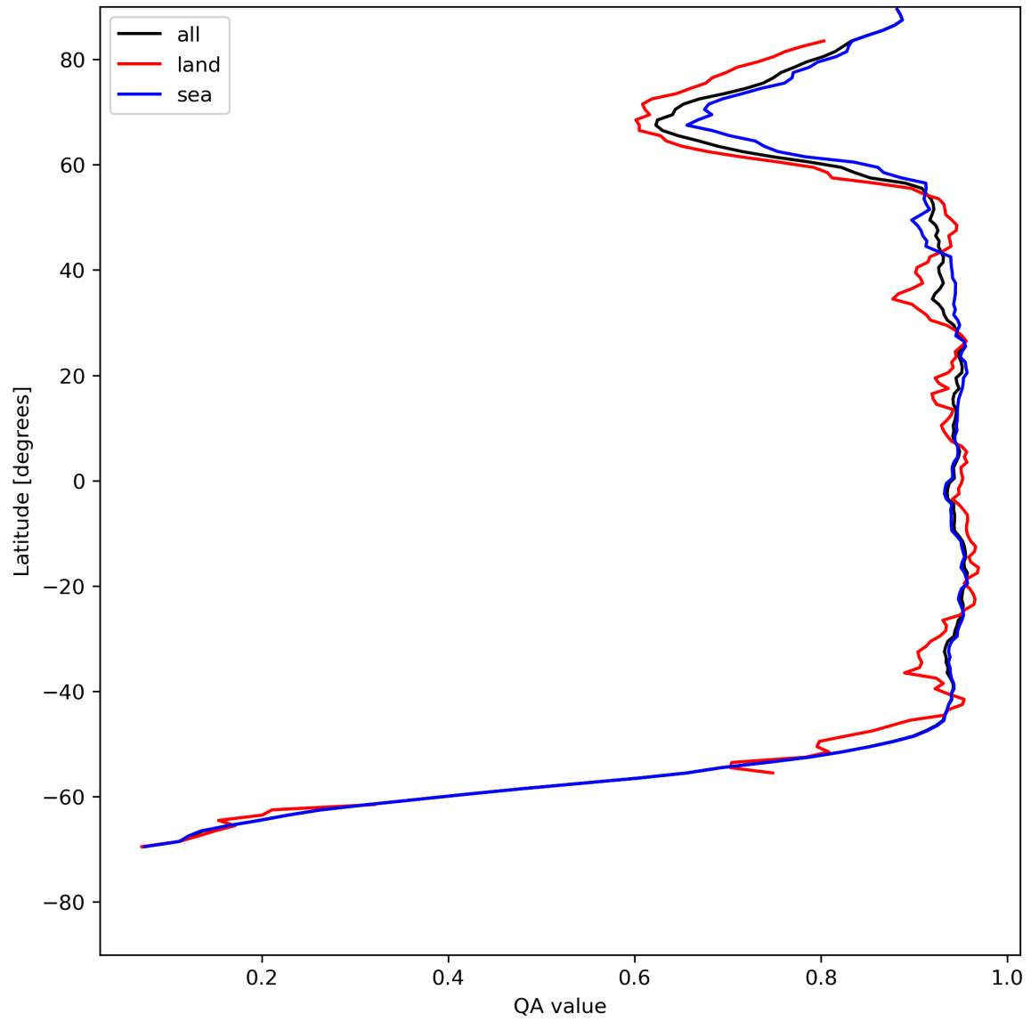
Figure 13: Zonal average of “QA value” for 2024-05-13 to 2024-05-15.
