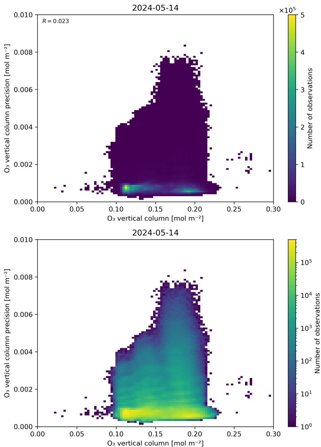
Figure 41: Scatter density plot of “O 3 vertical column” against “O 3 vertical column precision” for 2024-05-13 to 2024-05-15.
