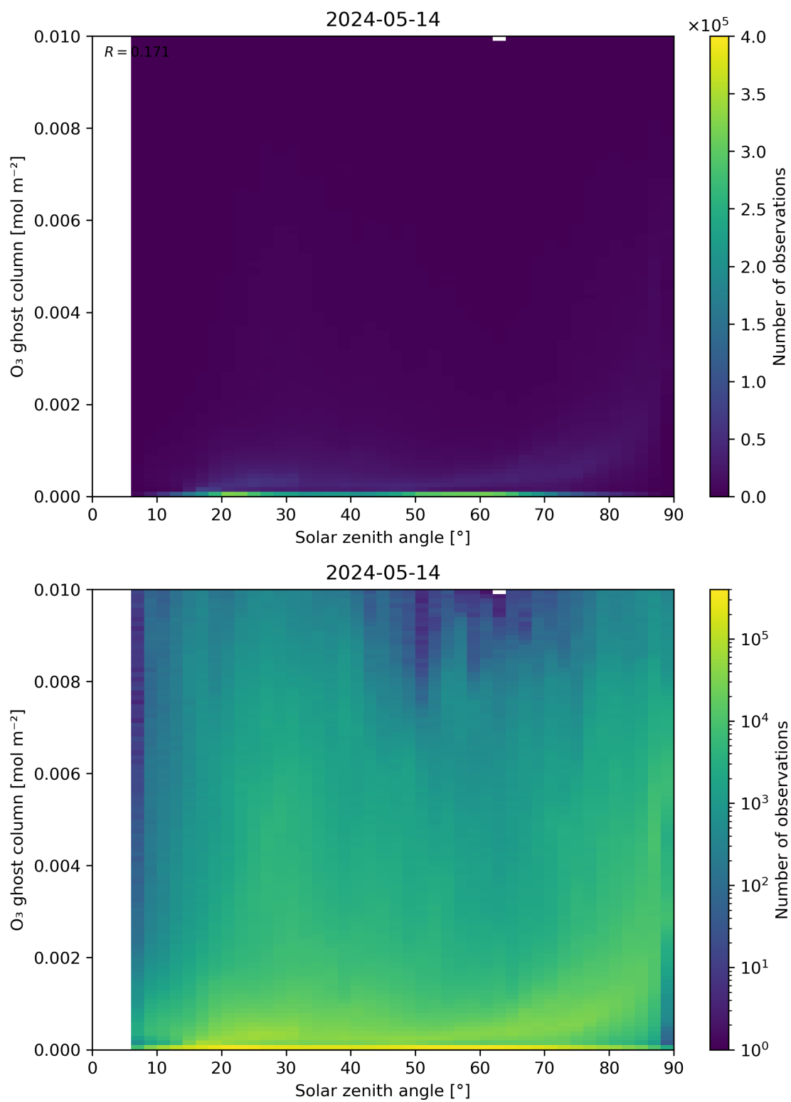
Figure 46: Scatter density plot of “Solar zenith angle” against “O 3 ghost column” for 2024-05-13 to 2024-05-15.
