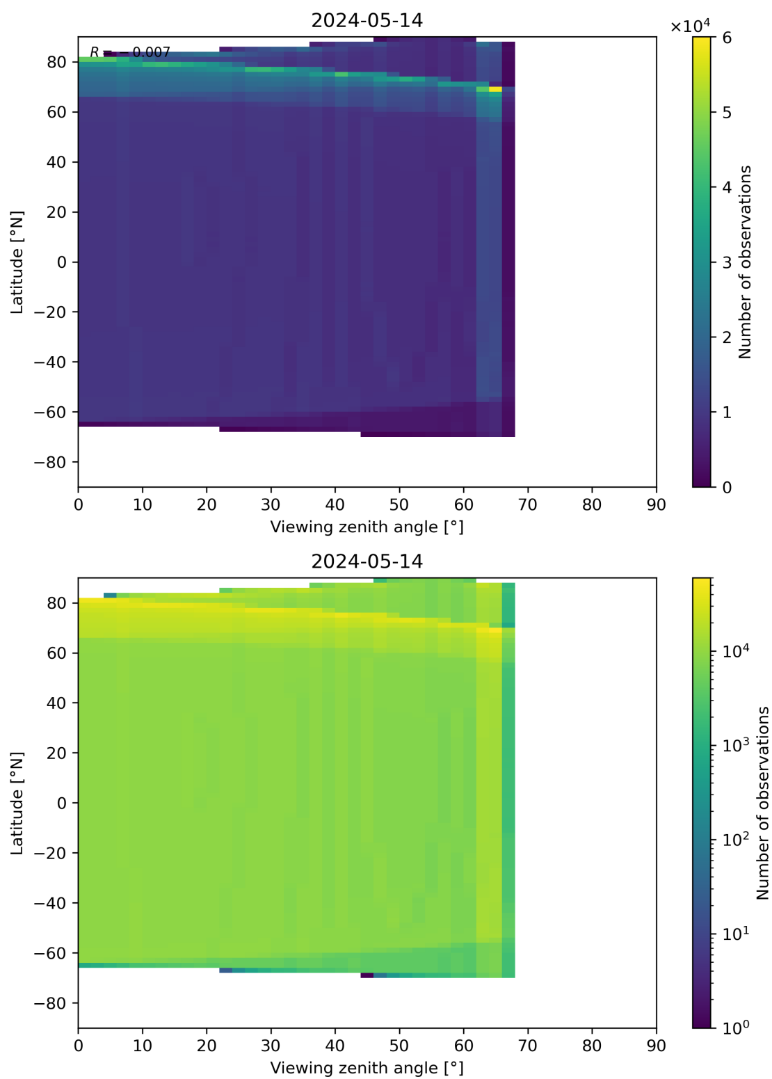
Figure 49: Scatter density plot of “Viewing zenith angle” against “Latitude” for 2024-05-13 to 2024-05-15.
