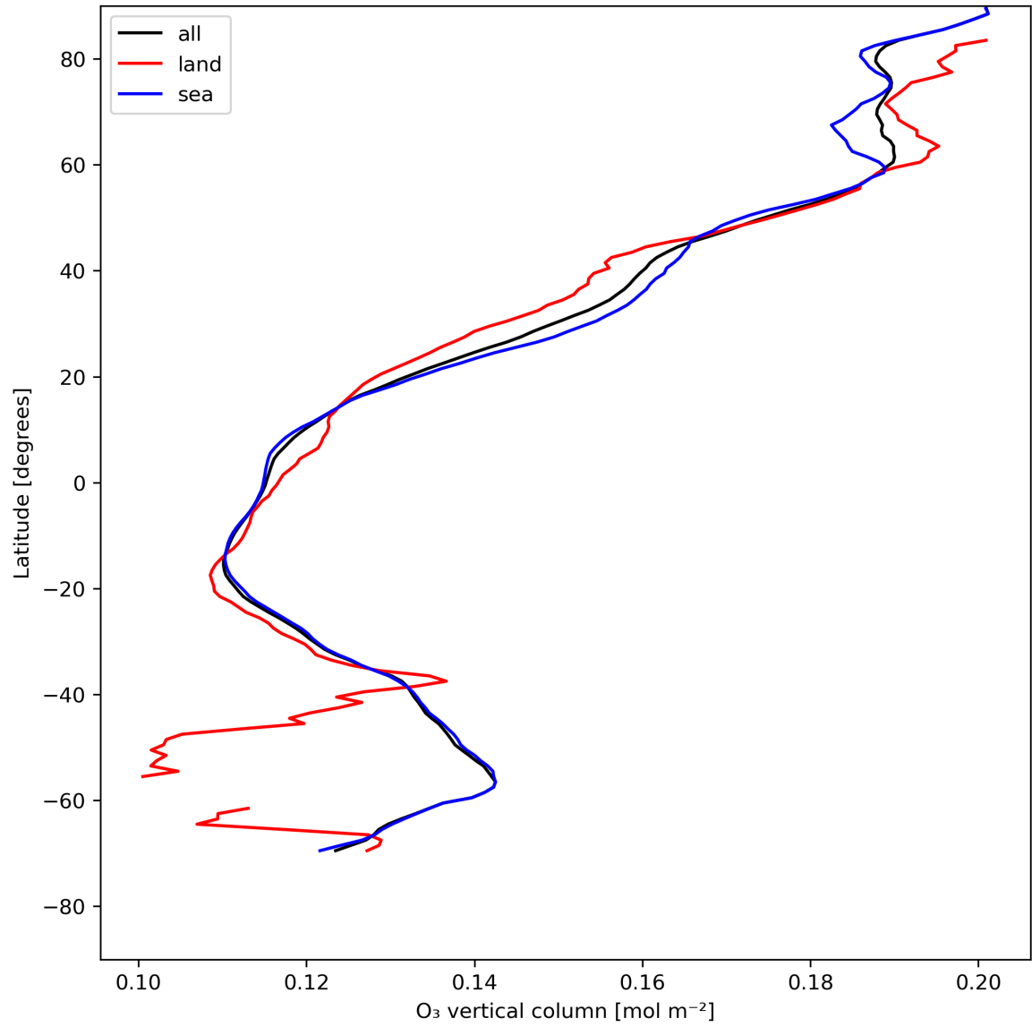
Figure 14: Zonal average of “O 3 vertical column” for 2024-05-13 to 2024-05-15.
