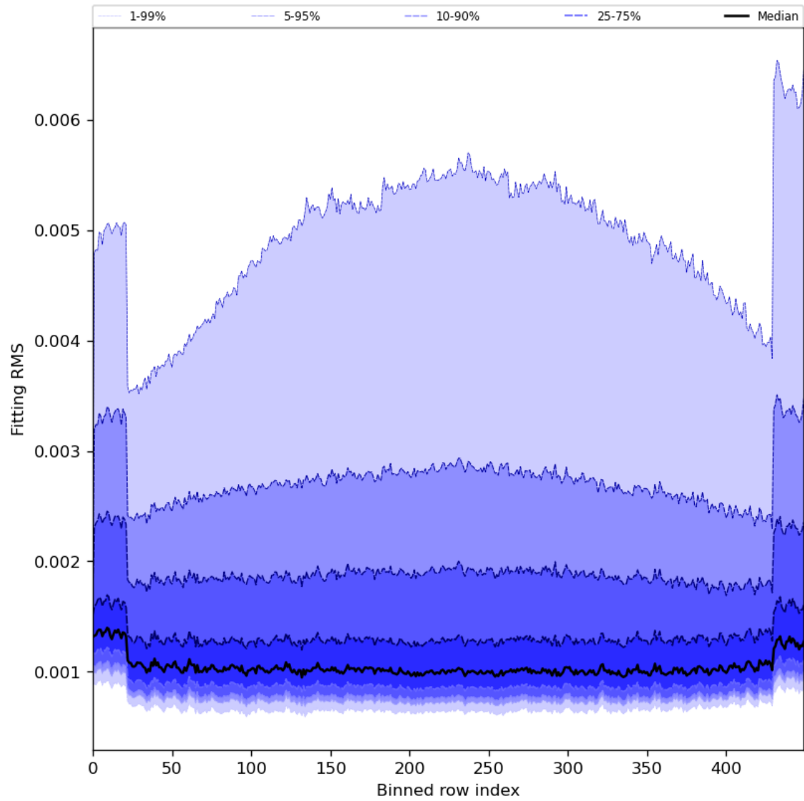
Figure 30: Along track statistics of “Fitting RMS” for 2024-05-13 to 2024-05-15
