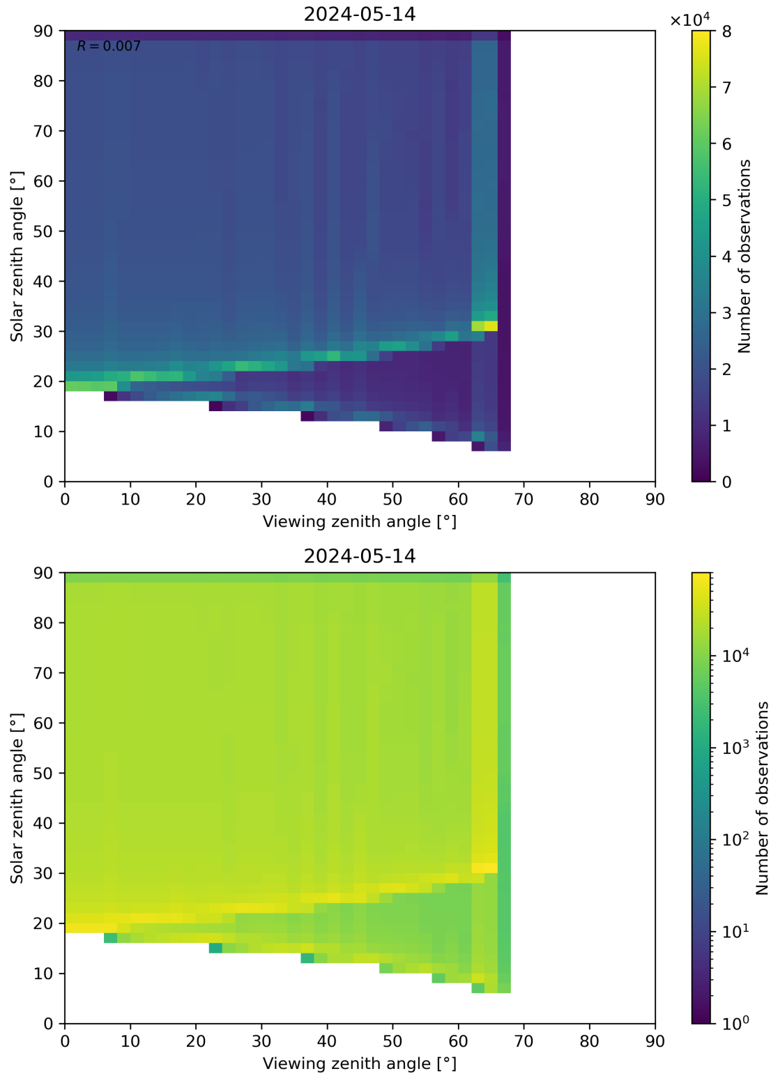
Figure 54: Scatter density plot of “Viewing zenith angle” against “Solar zenith angle” for 2024-05-13 to 2024-05-15.
