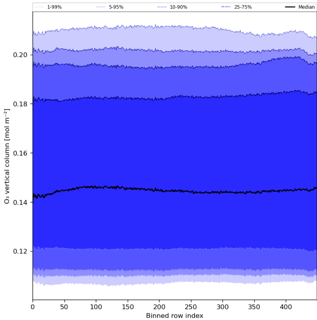
Figure 28: Along track statistics of "O 3 vertical column" for 2024-05-13 to 2024-05-15
