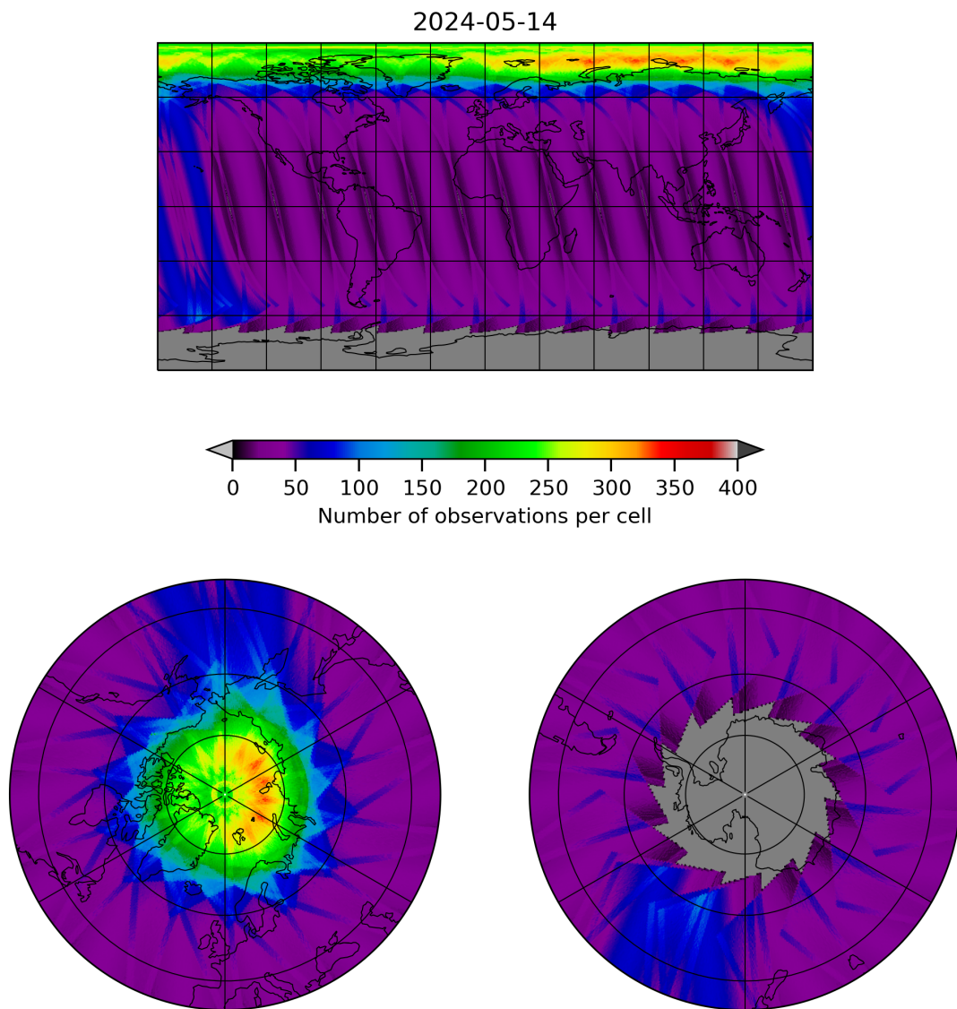
Figure 12: Map of the number of observations for 2024-05-13 to 2024-05-15
