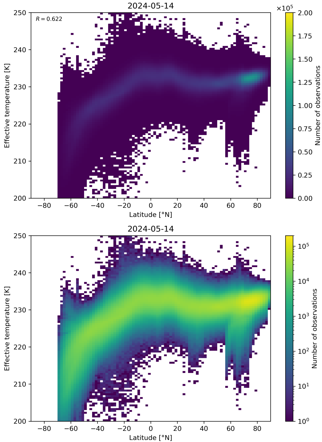
Figure 34: Scatter density plot of “Latitude” against “Effective temperature” for 2024-05-13 to 2024-05-15.
