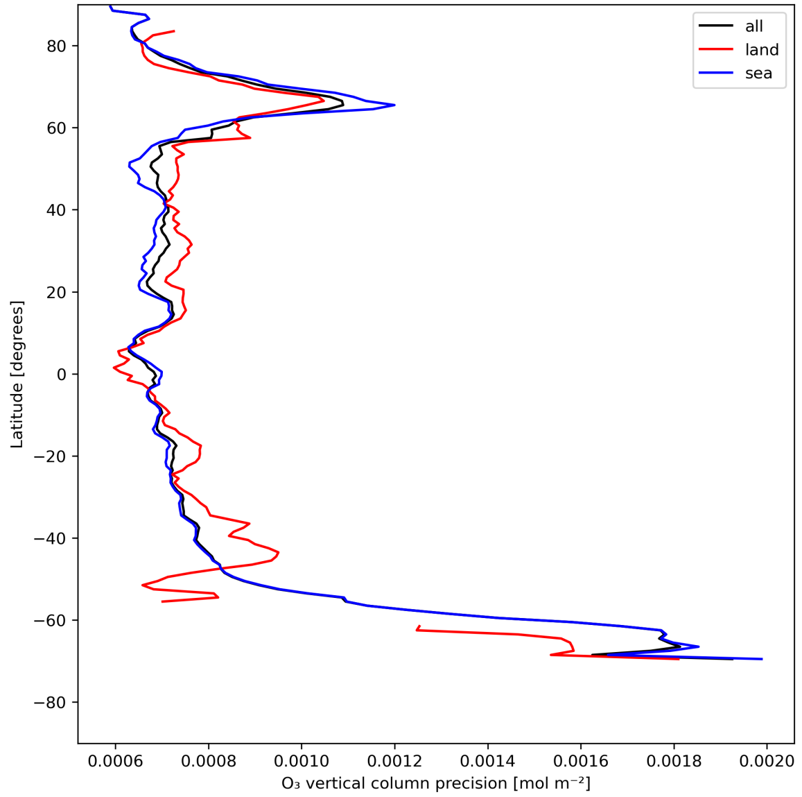
Figure 15: Zonal average of “O 3 vertical column precision” for 2024-05-13 to 2024-05-15.
