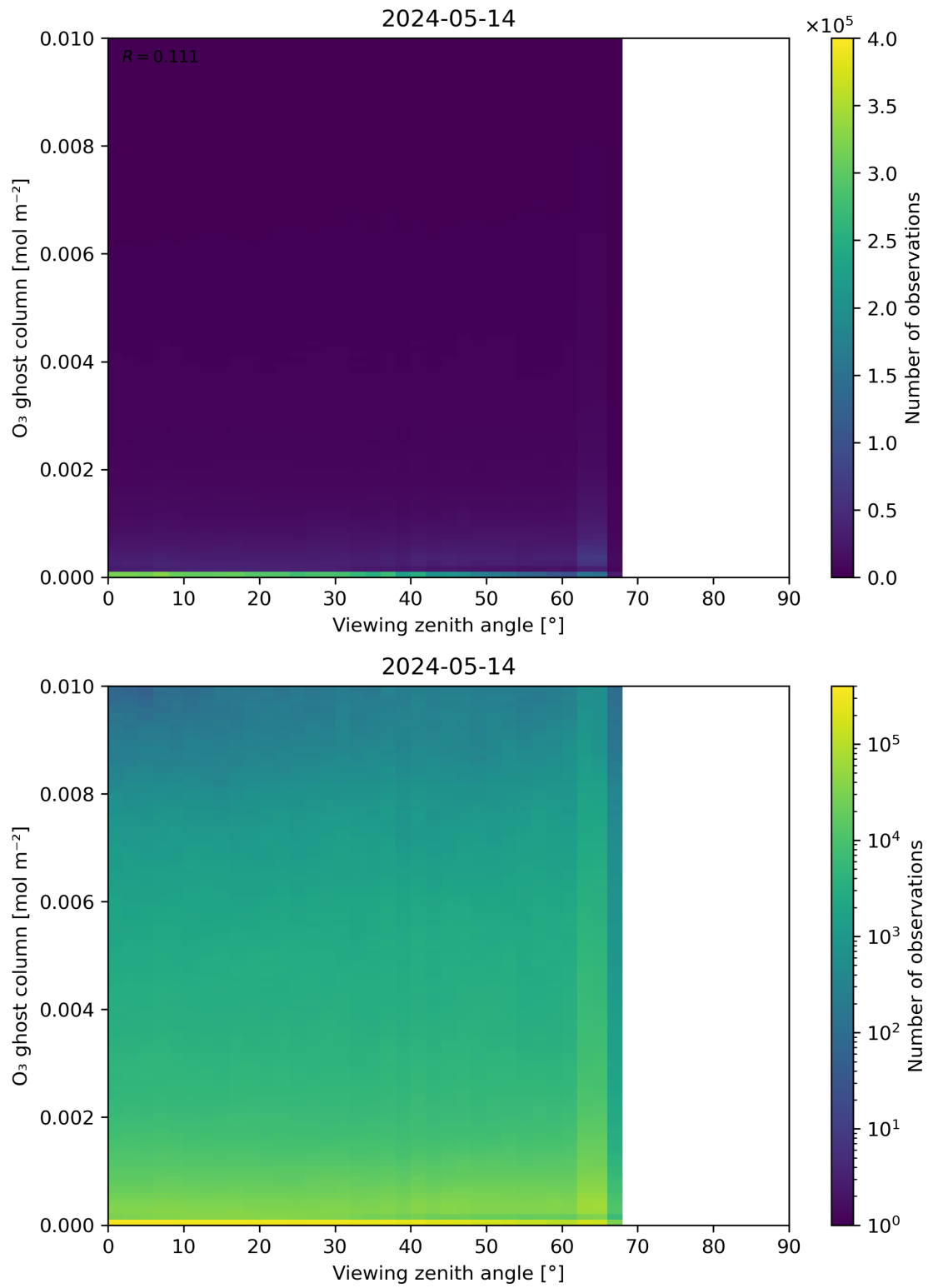
Figure 51: Scatter density plot of “Viewing zenith angle” against “O 3 ghost column” for 2024-05-13 to 2024-05-15.
