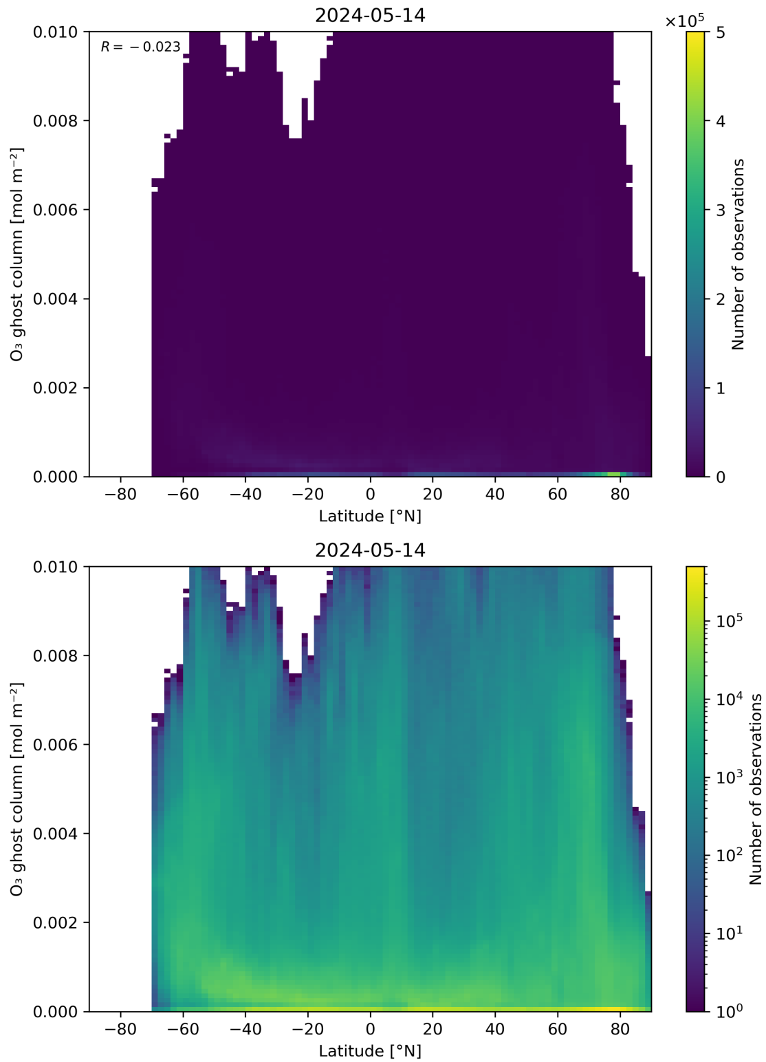
Figure 35: Scatter density plot of “Latitude” against “O 3 ghost column” for 2024-05-13 to 2024-05-15.
