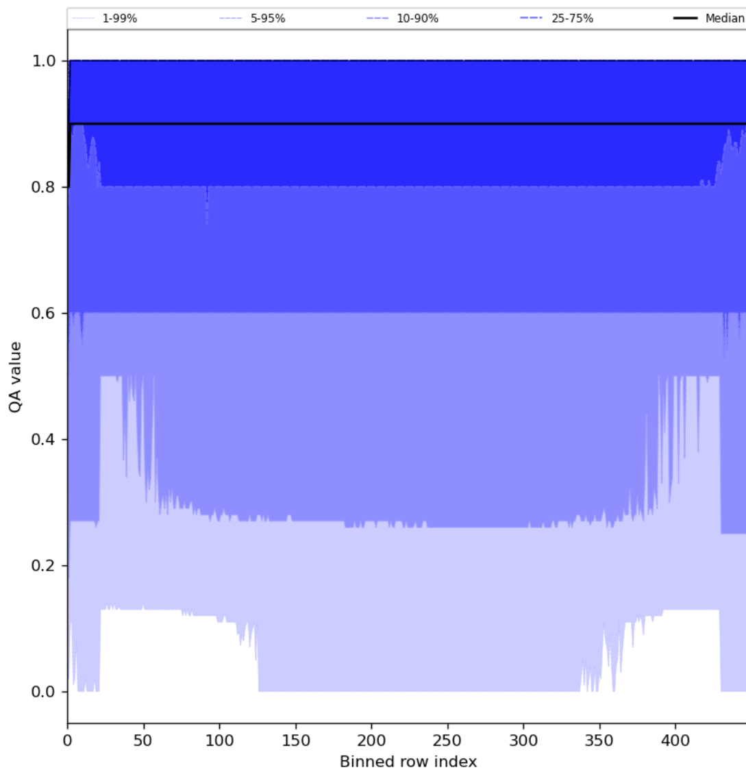
Figure 27: Along track statistics of “QA value” for 2024-05-13 to 2024-05-15
