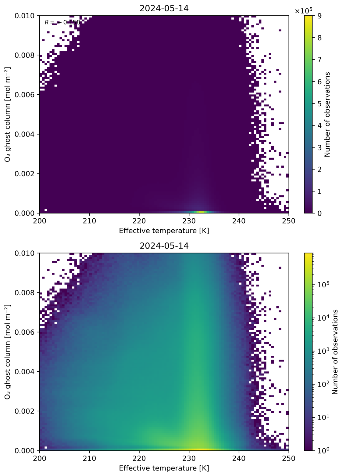
Figure 38: Scatter density plot of “Effective temperature” against “O 3 ghost column” for 2024-05-13 to 2024-05-15.
