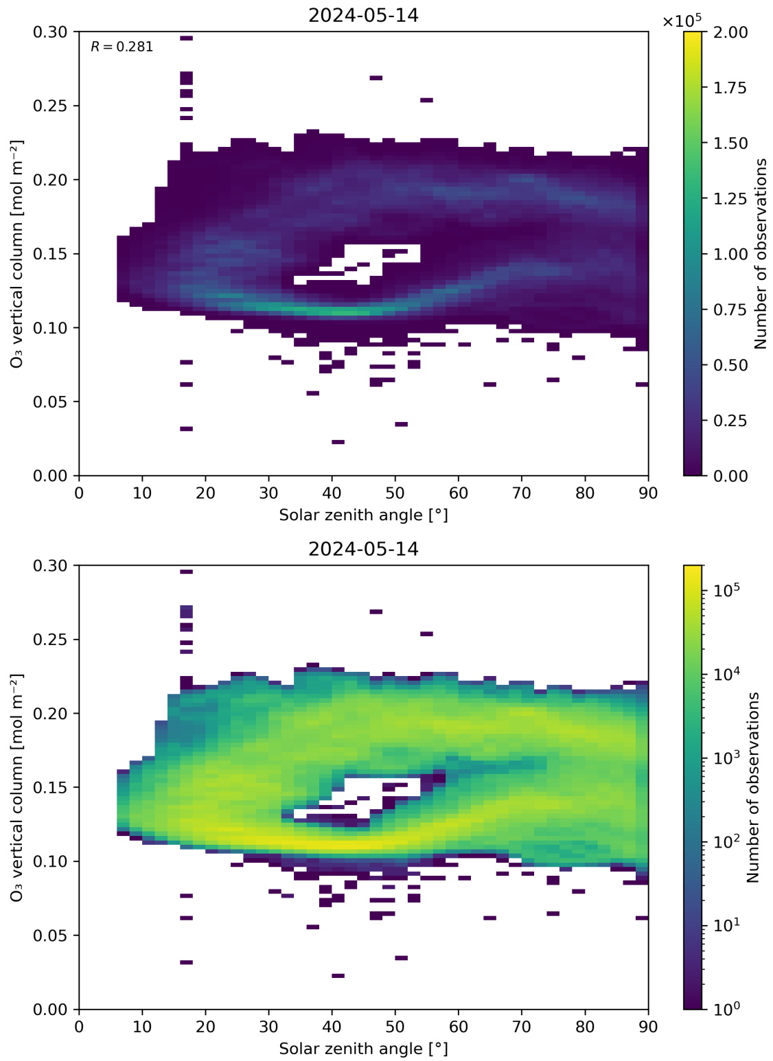
Figure 47: Scatter density plot of “Solar zenith angle” against “O 3 vertical column” for 2024-05-13 to 2024-05-15.
