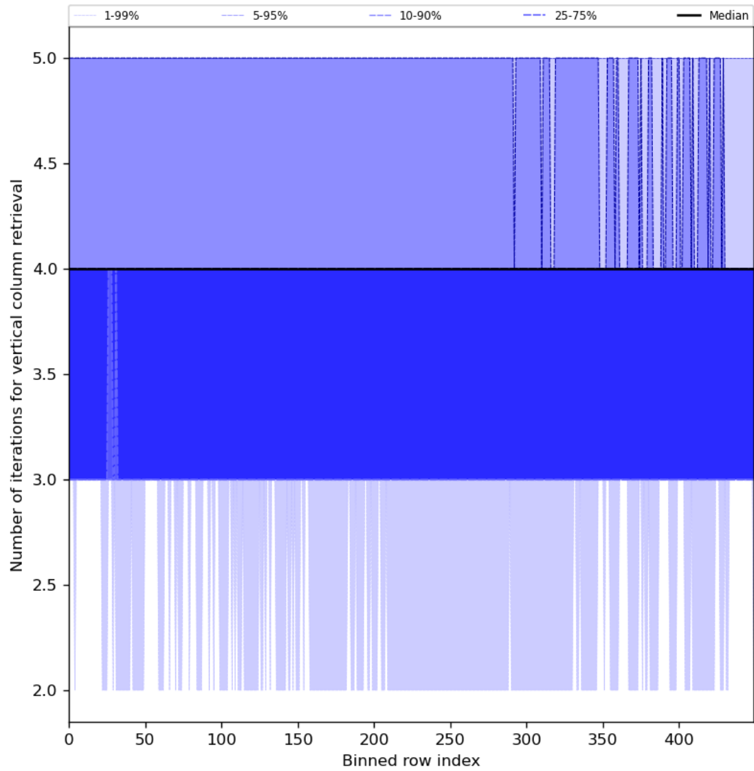
Figure 33: Along track statistics of “Number of iterations for vertical column retrieval” for 2024-05-13 to 2024-05-15
