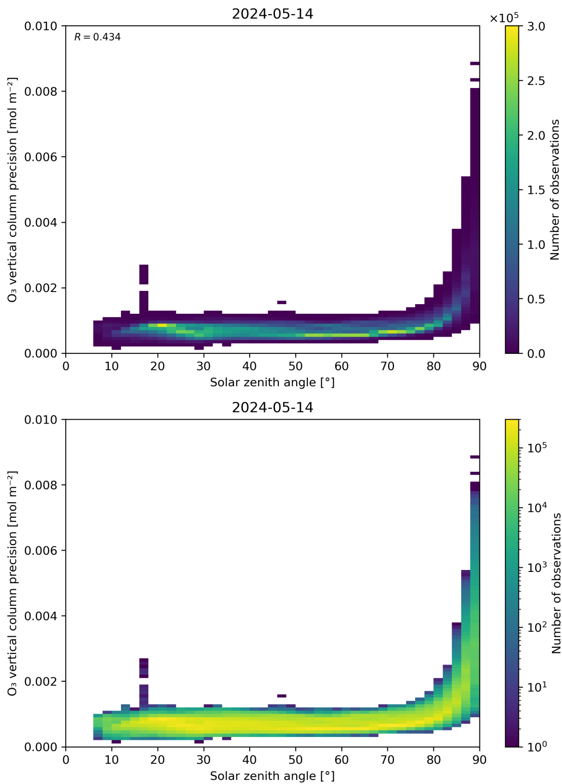
Figure 48: Scatter density plot of “Solar zenith angle” against “O 3 vertical column precision” for 2024-05-13 to 2024-05-15.
