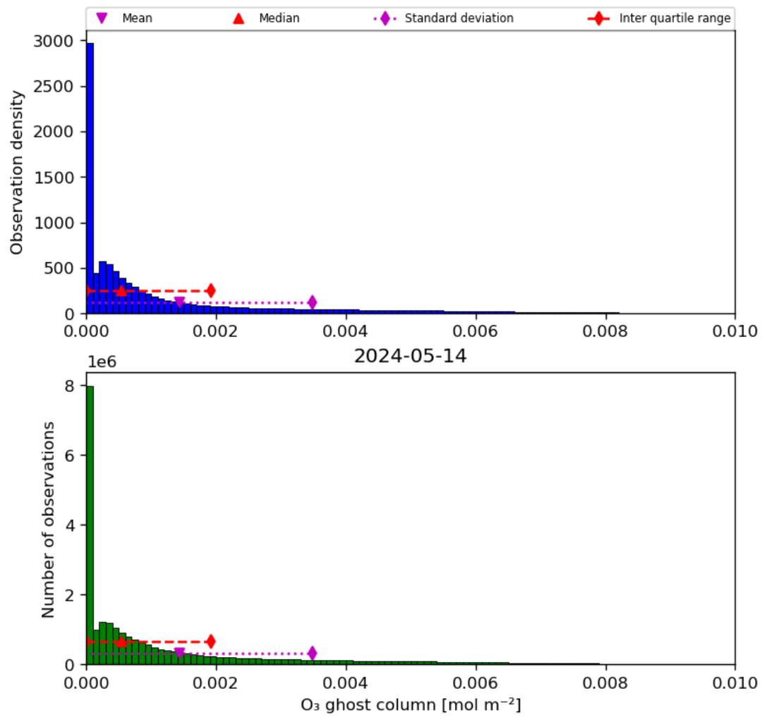
Figure 25: Histogram of “O 3 ghost column” for 2024-05-13 to 2024-05-15
