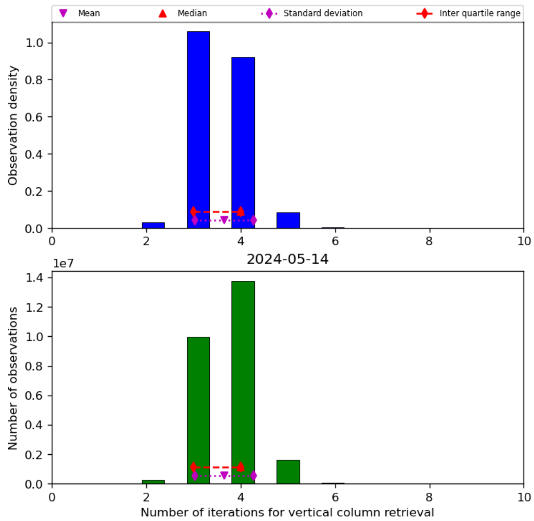
Figure 26: Histogram of “Number of iterations for vertical column retrieval” for 2024-05-13 to 2024-05-15
