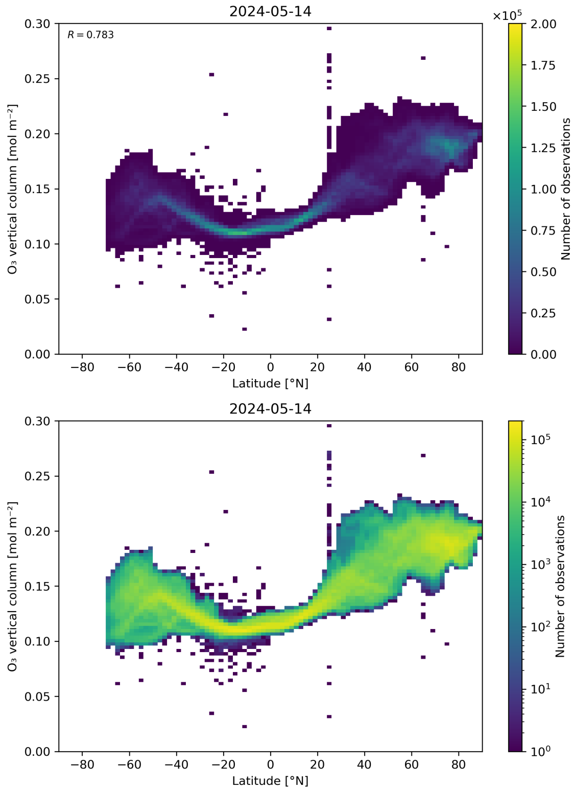
Figure 36: Scatter density plot of “Latitude” against “O 3 vertical column” for 2024-05-13 to 2024-05-15.
