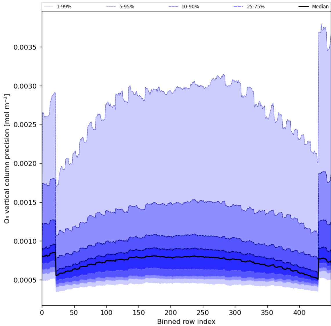
Figure 29: Along track statistics of “O 3 vertical column precision” for 2024-05-13 to 2024-05-15
