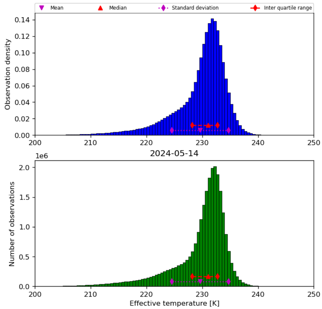
Figure 24: Histogram of “Effective temperature” for 2024-05-13 to 2024-05-15
