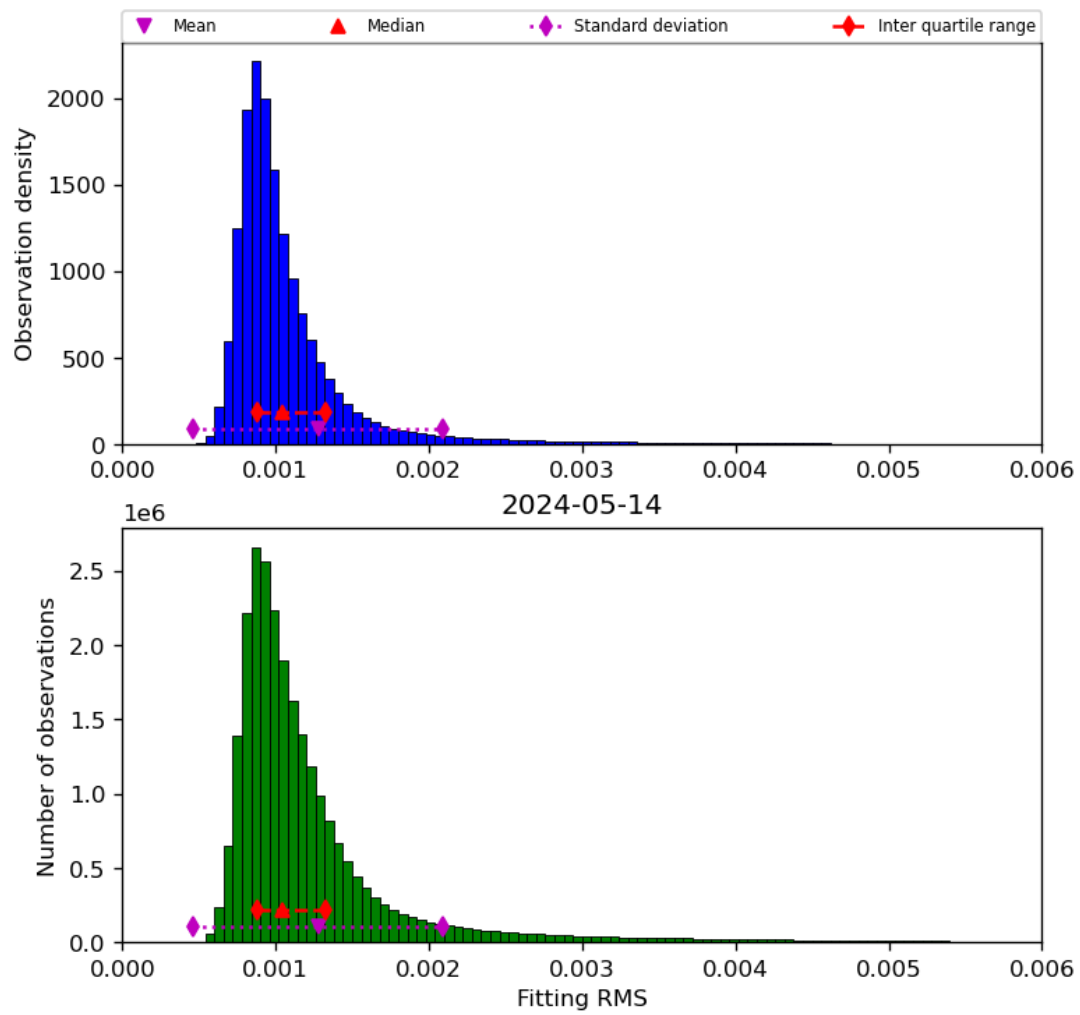
Figure 23: Histogram of “Fitting RMS” for 2024-05-13 to 2024-05-15
