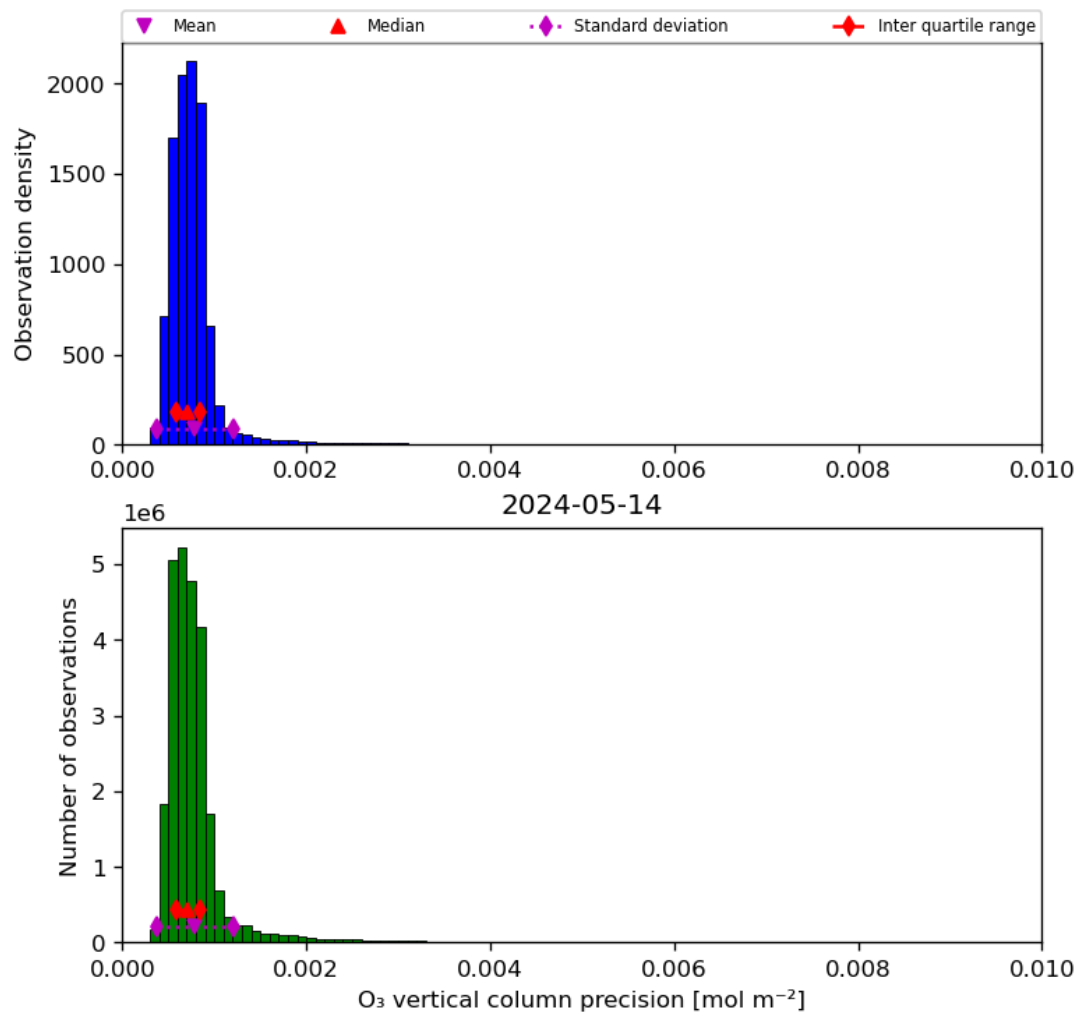
Figure 22: Histogram of “O 3 vertical column precision” for 2024-05-13 to 2024-05-15
