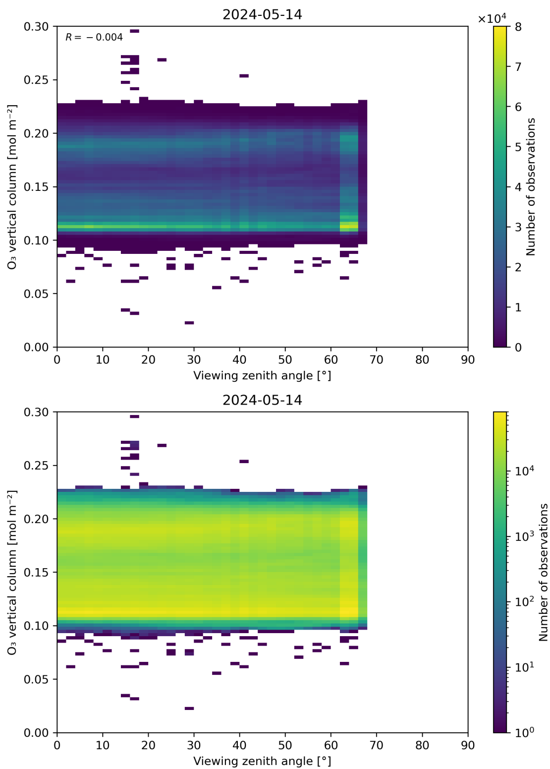
Figure 52: Scatter density plot of “Viewing zenith angle” against “O 3 vertical column” for 2024-05-13 to 2024-05-15.
