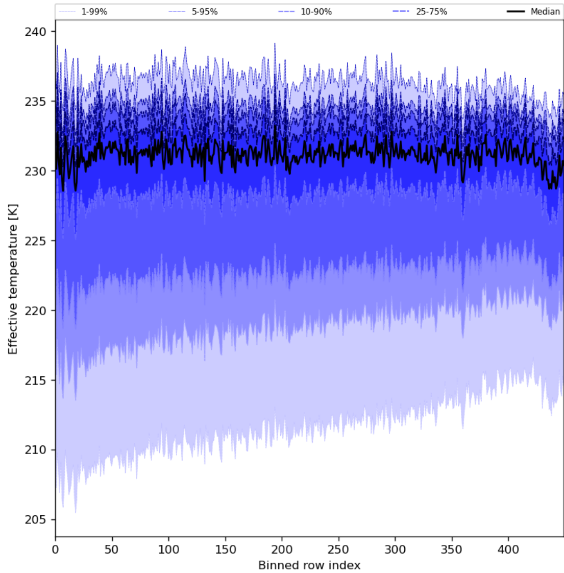
Figure 31: Along track statistics of “Effective temperature” for 2024-05-13 to 2024-05-15
