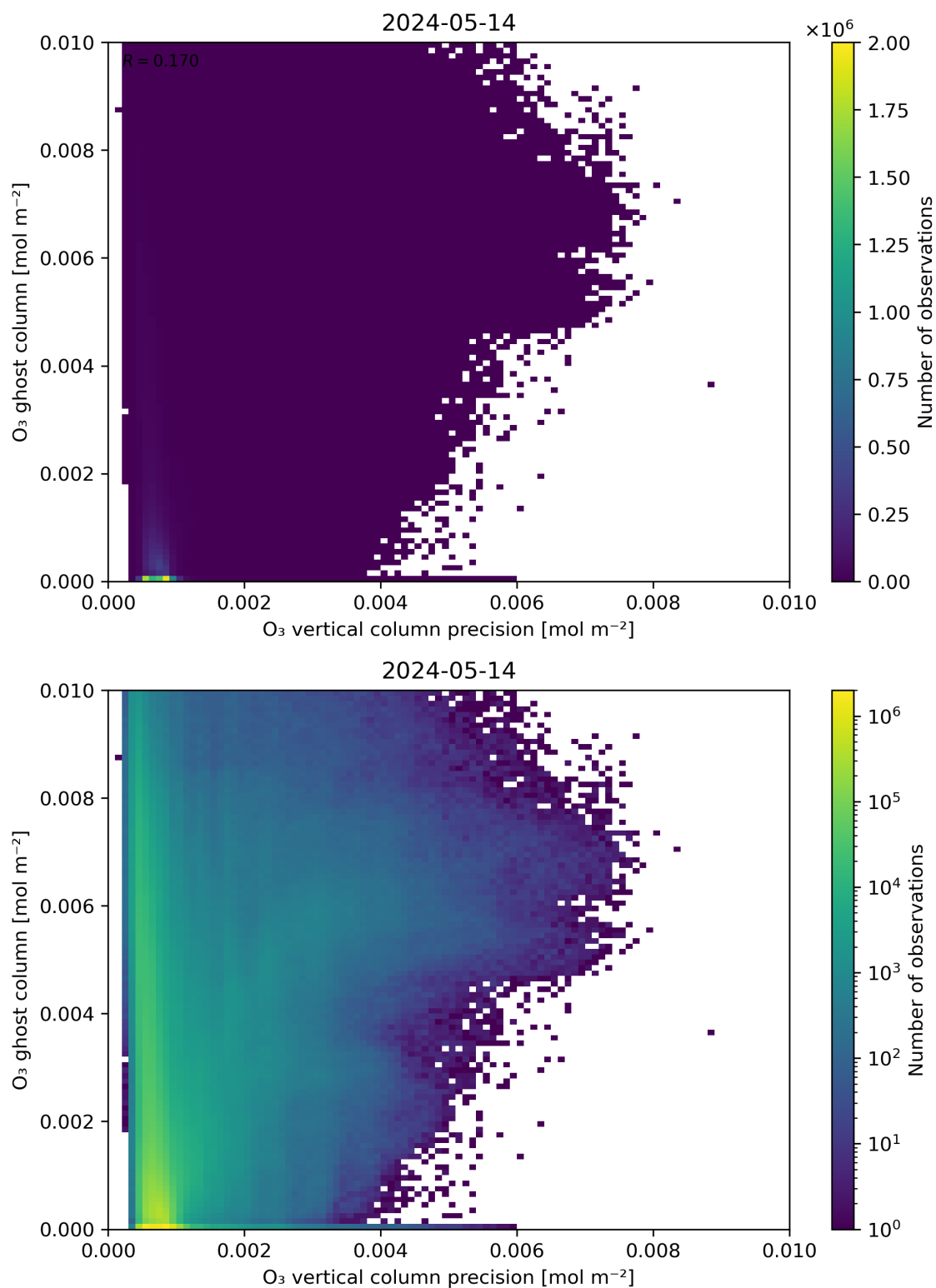
Figure 43: Scatter density plot of “ \text{O}_3 vertical column precision” against “ \text{O}_3 ghost column” for 2024-05-13 to 2024-05-15.
