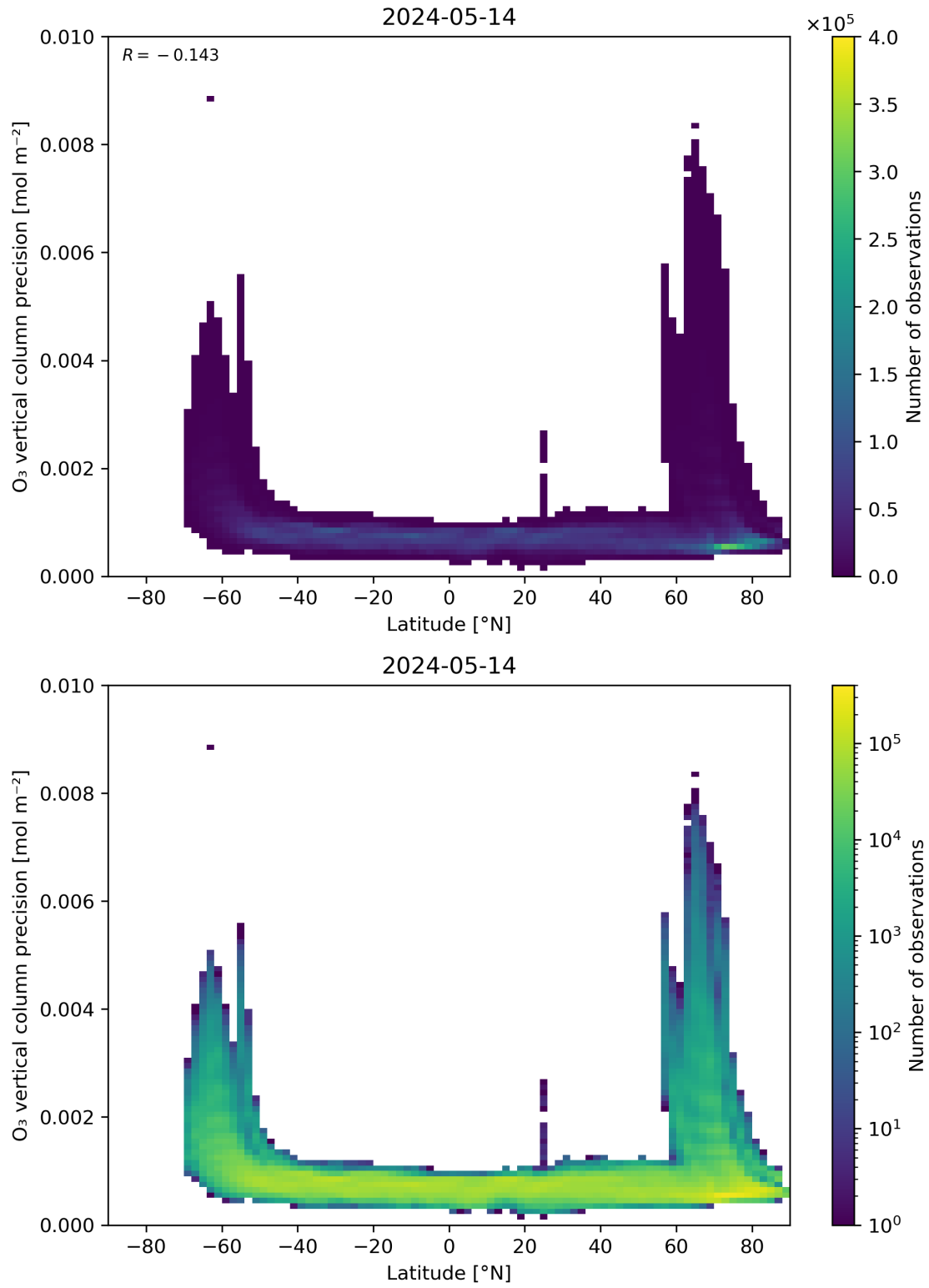
Figure 37: Scatter density plot of “Latitude” against “O 3 vertical column precision” for 2024-05-13 to 2024-05-15.
