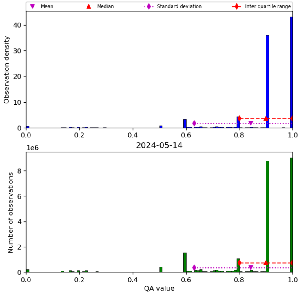
Figure 20: Histogram of “QA value” for 2024-05-13 to 2024-05-15
