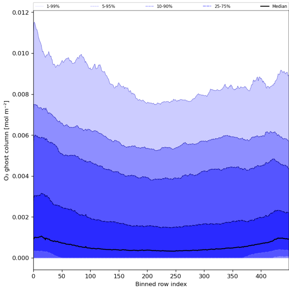
Figure 32: Along track statistics of "O 3 ghost column" for 2024-05-13 to 2024-05-15
