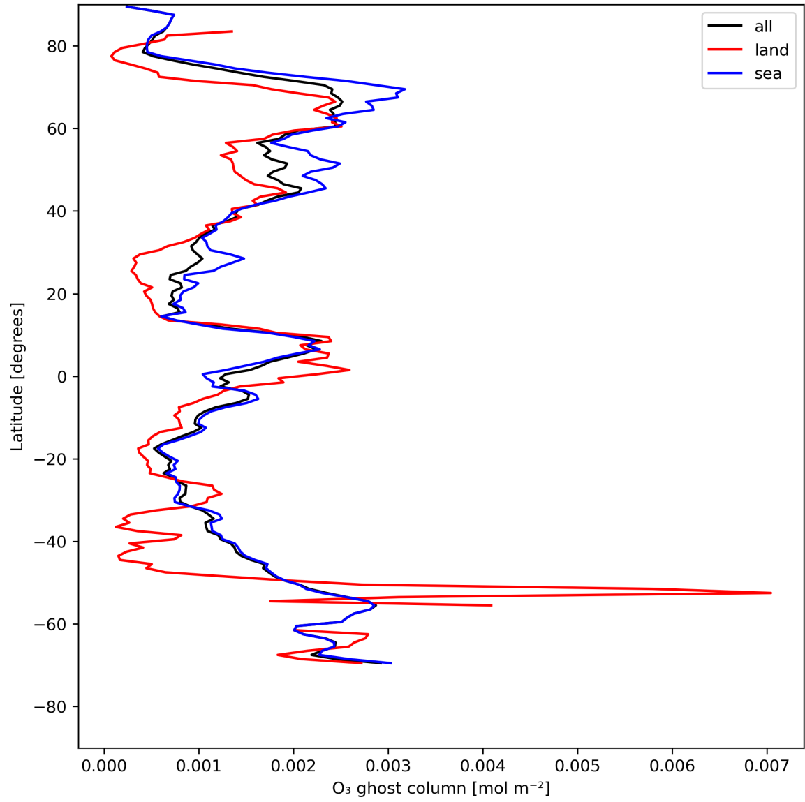
Figure 18: Zonal average of "O 3 ghost column" for 2024-05-13 to 2024-05-15.
