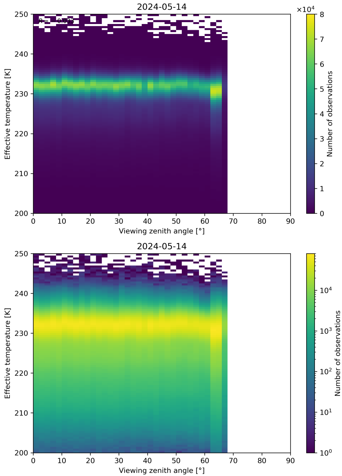
Figure 50: Scatter density plot of “Viewing zenith angle” against “Effective temperature” for 2024-05-13 to 2024-05-15.
