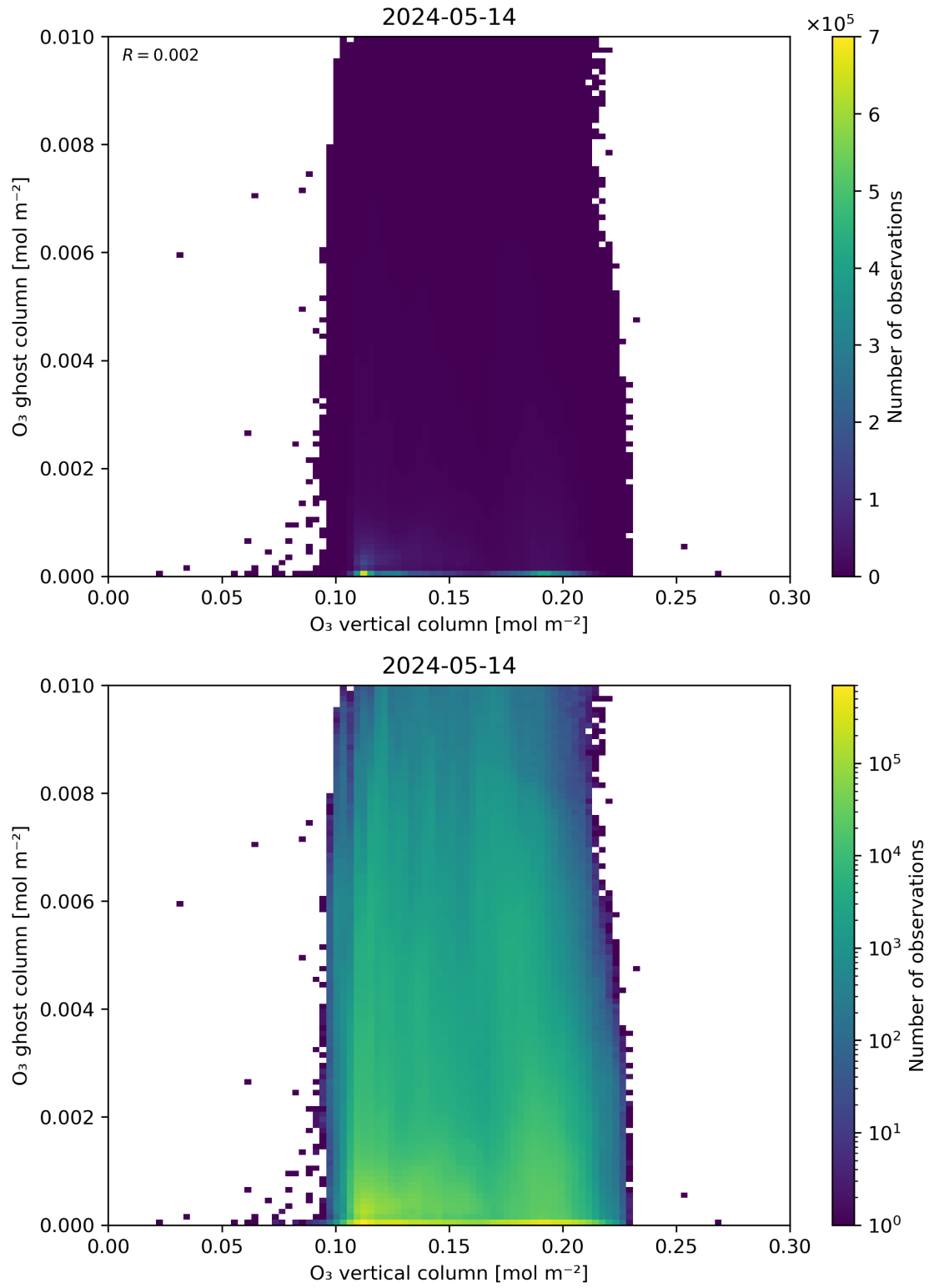
Figure 40: Scatter density plot of “O 3 vertical column” against “O 3 ghost column” for 2024-05-13 to 2024-05-15.
