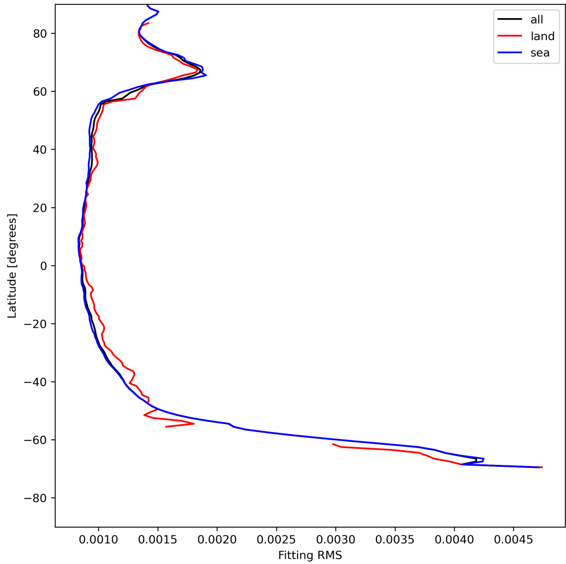
Figure 16: Zonal average of “Fitting RMS” for 2024-05-13 to 2024-05-15.
