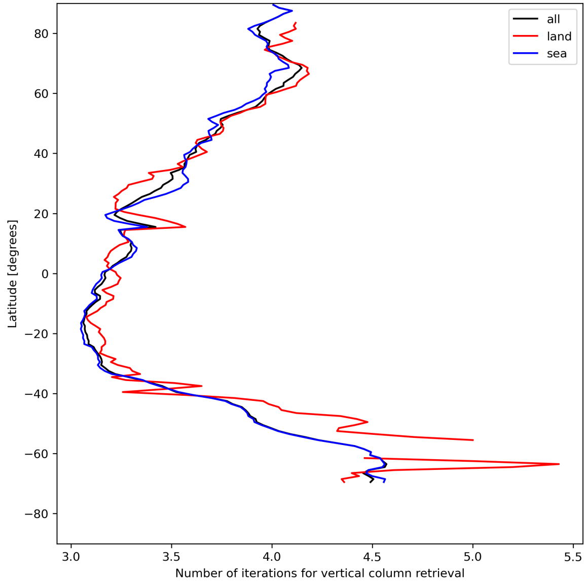
Figure 19: Zonal average of “Number of iterations for vertical column retrieval” for 2024-05-13 to 2024-05-15.
