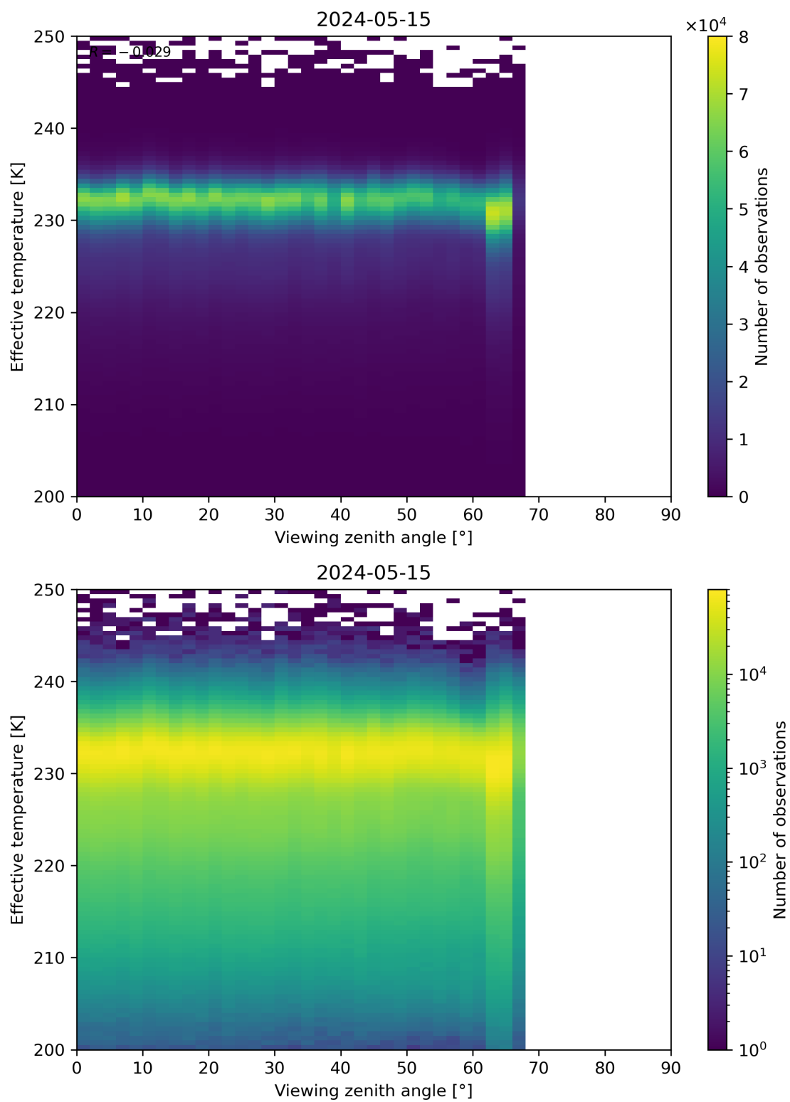
Figure 50: Scatter density plot of “Viewing zenith angle” against “Effective temperature” for 2024-05-14 to 2024-05-16.
