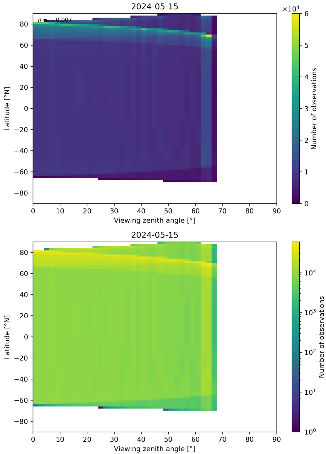
Figure 49: Scatter density plot of “Viewing zenith angle” against “Latitude” for 2024-05-14 to 2024-05-16.
