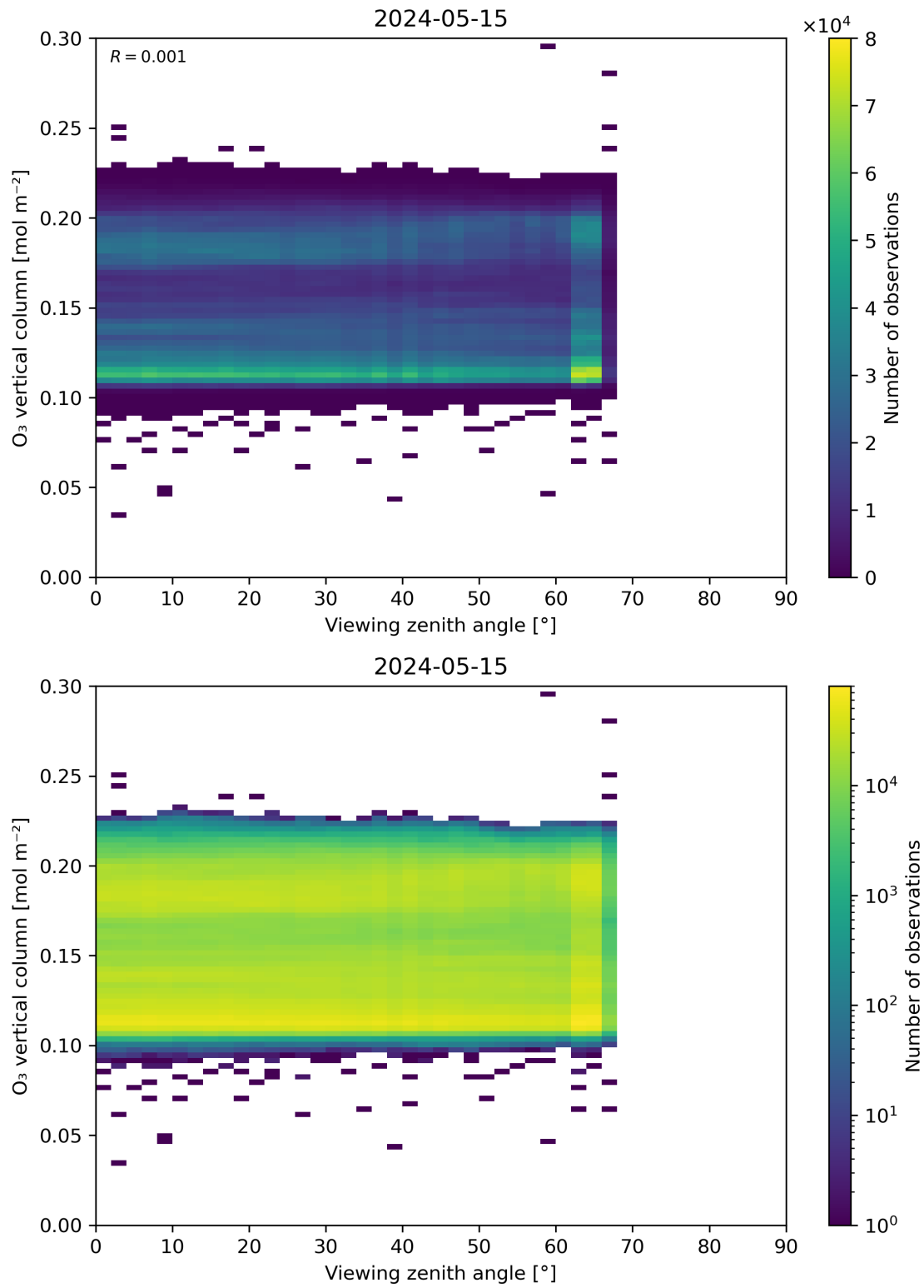
Figure 52: Scatter density plot of “Viewing zenith angle” against “O 3 vertical column” for 2024-05-14 to 2024-05-16.
