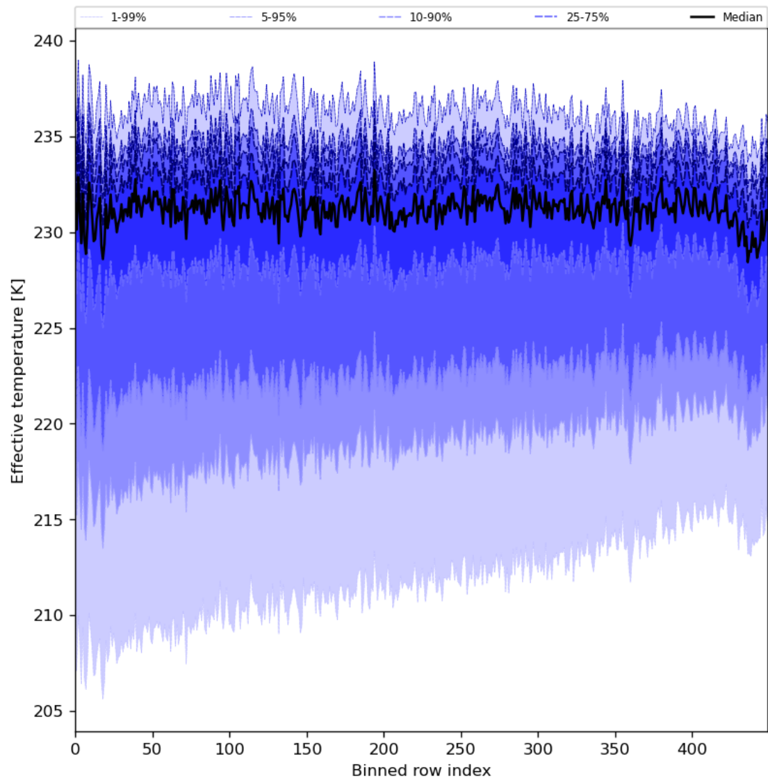
Figure 31: Along track statistics of “Effective temperature” for 2024-05-14 to 2024-05-16
