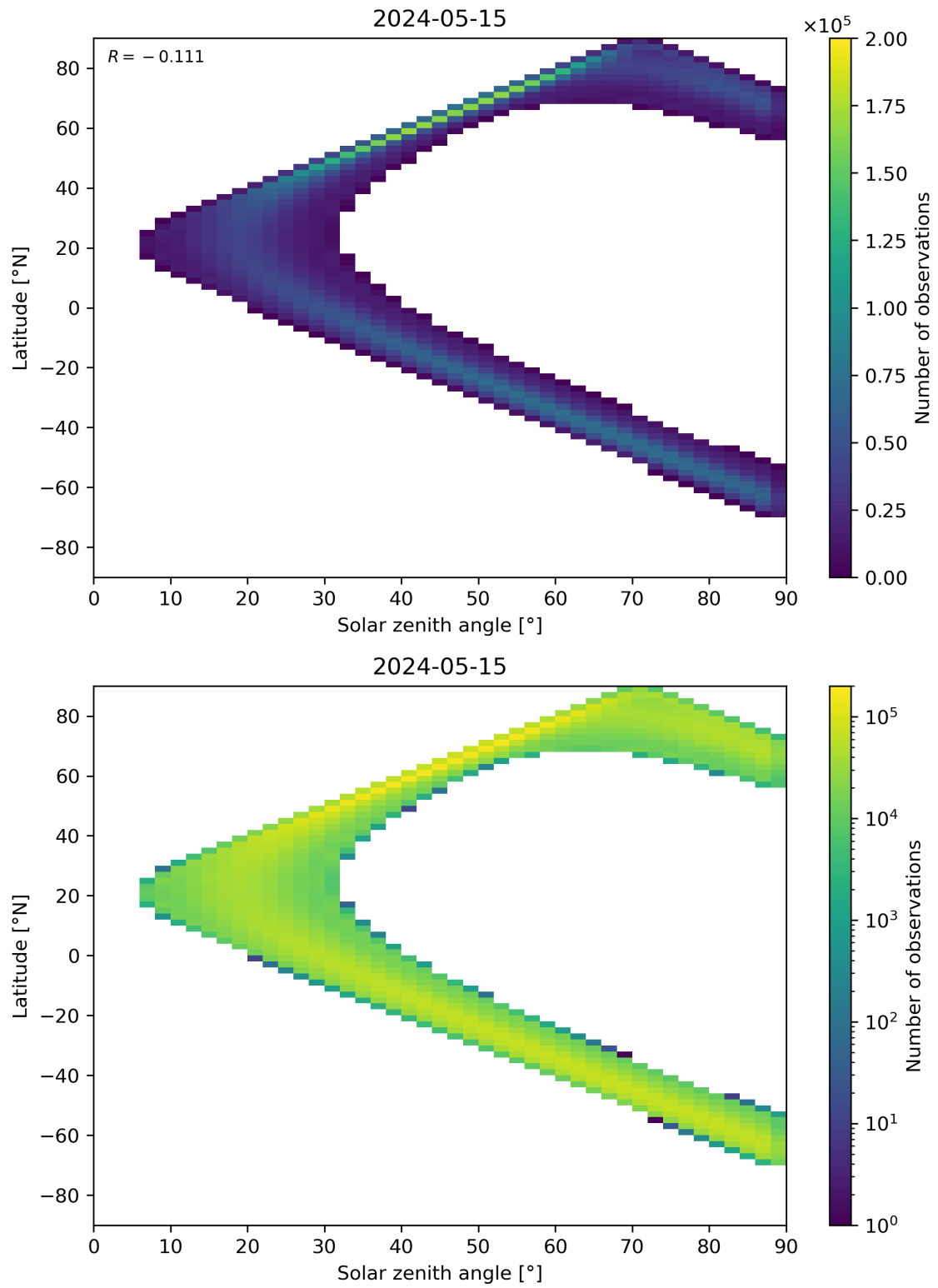
Figure 44: Scatter density plot of “Solar zenith angle” against “Latitude” for 2024-05-14 to 2024-05-16.
