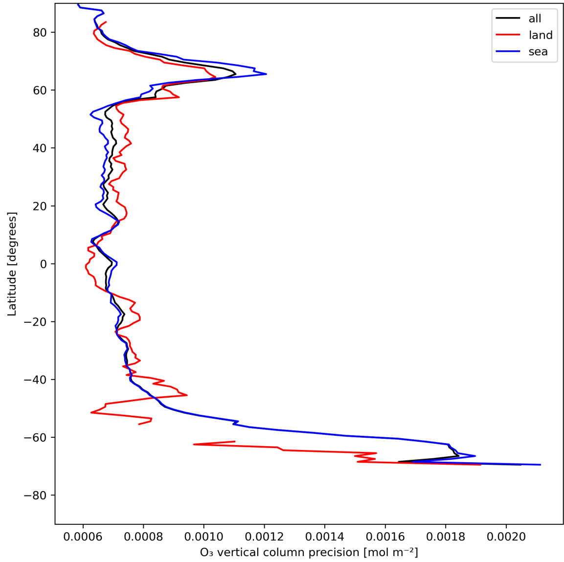
Figure 15: Zonal average of “O 3 vertical column precision” for 2024-05-14 to 2024-05-16.
