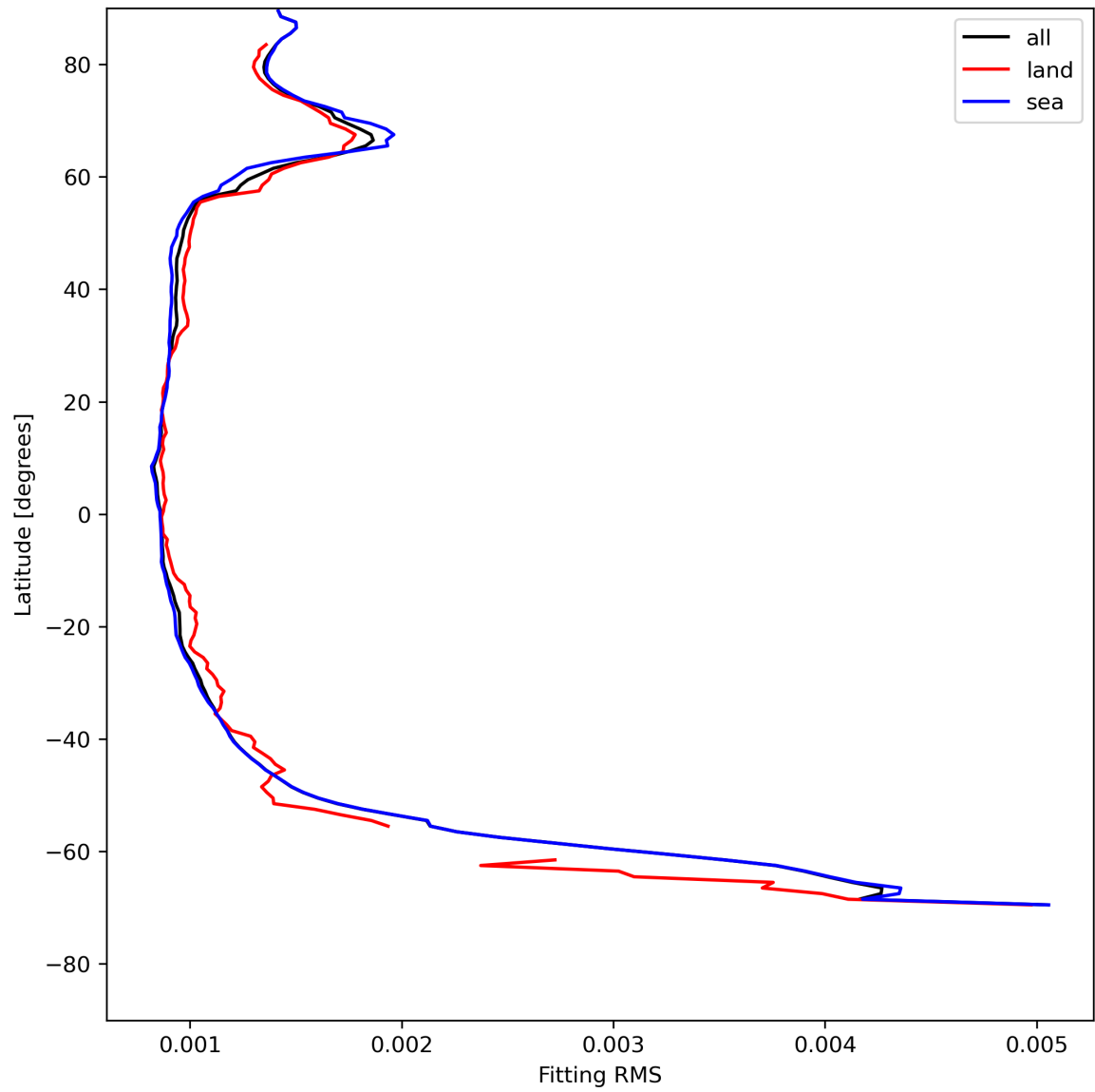
Figure 16: Zonal average of “Fitting RMS” for 2024-05-14 to 2024-05-16.
