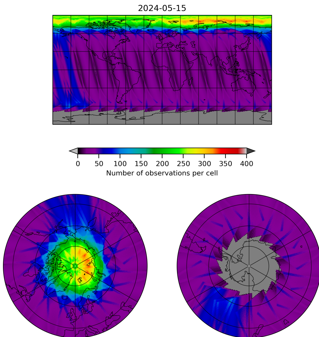
Figure 12: Map of the number of observations for 2024-05-14 to 2024-05-16
