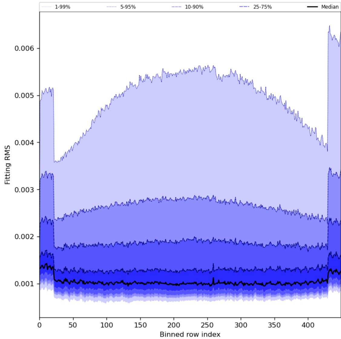
Figure 30: Along track statistics of “Fitting RMS” for 2024-05-14 to 2024-05-16
