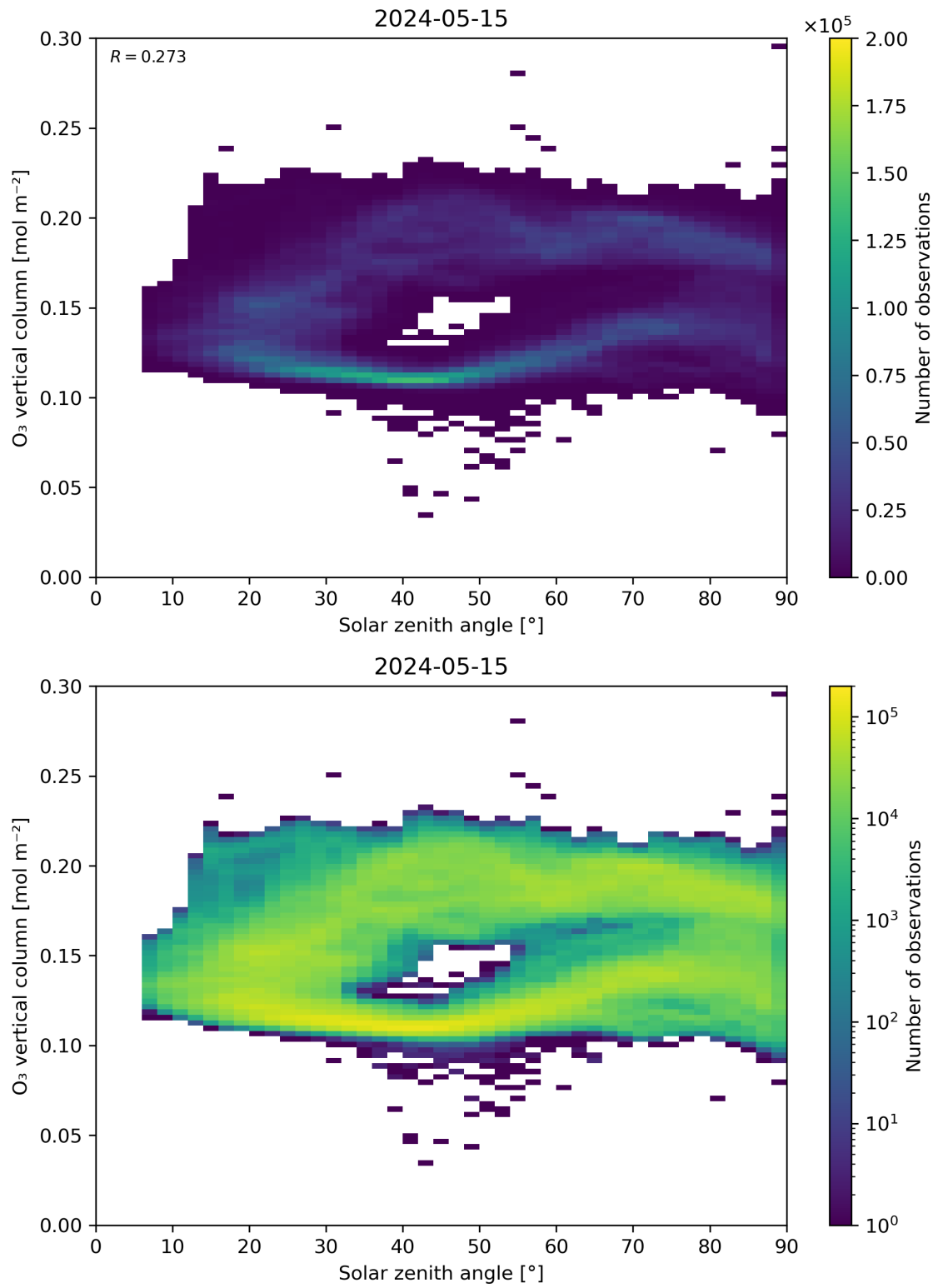
Figure 47: Scatter density plot of “Solar zenith angle” against “O 3 vertical column” for 2024-05-14 to 2024-05-16.
