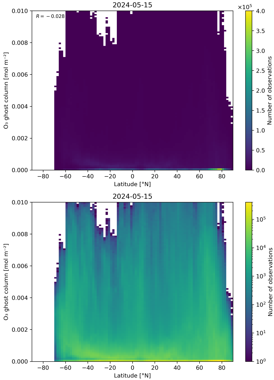
Figure 35: Scatter density plot of “Latitude” against “O 3 ghost column” for 2024-05-14 to 2024-05-16.
