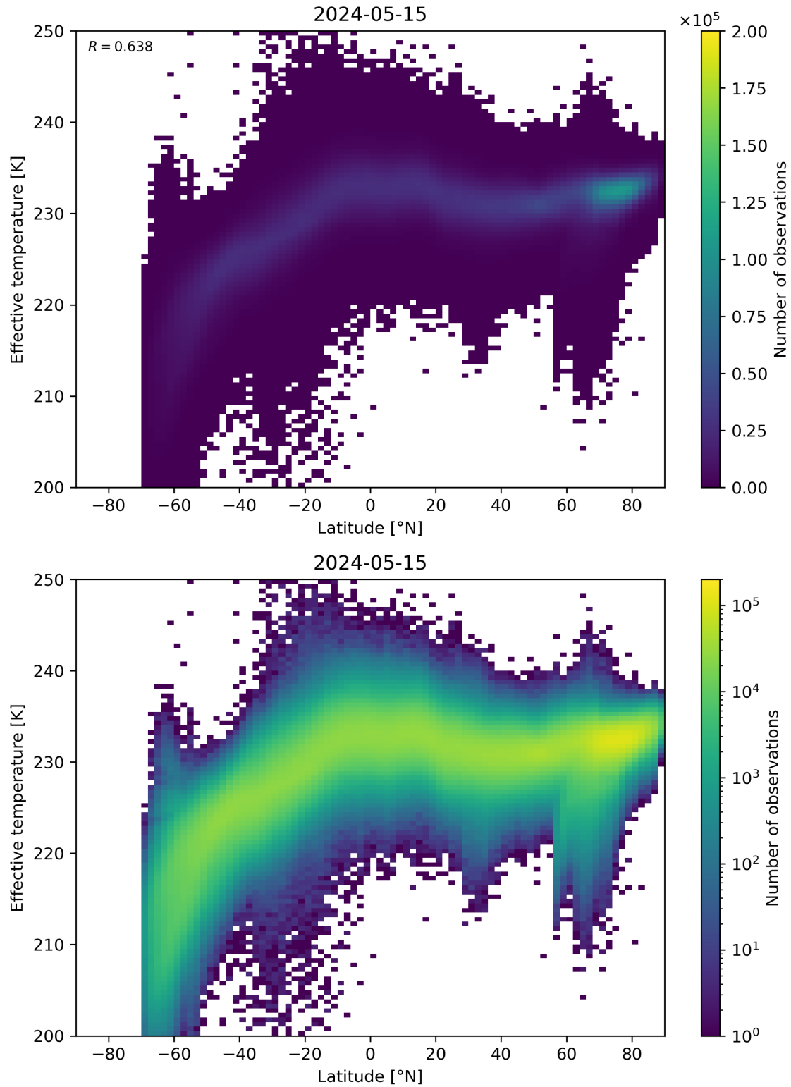
Figure 34: Scatter density plot of “Latitude” against “Effective temperature” for 2024-05-14 to 2024-05-16.
