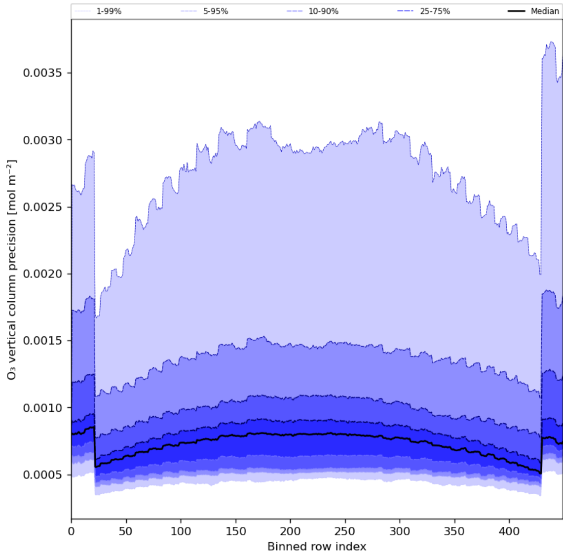
Figure 29: Along track statistics of “O 3 vertical column precision” for 2024-05-14 to 2024-05-16
