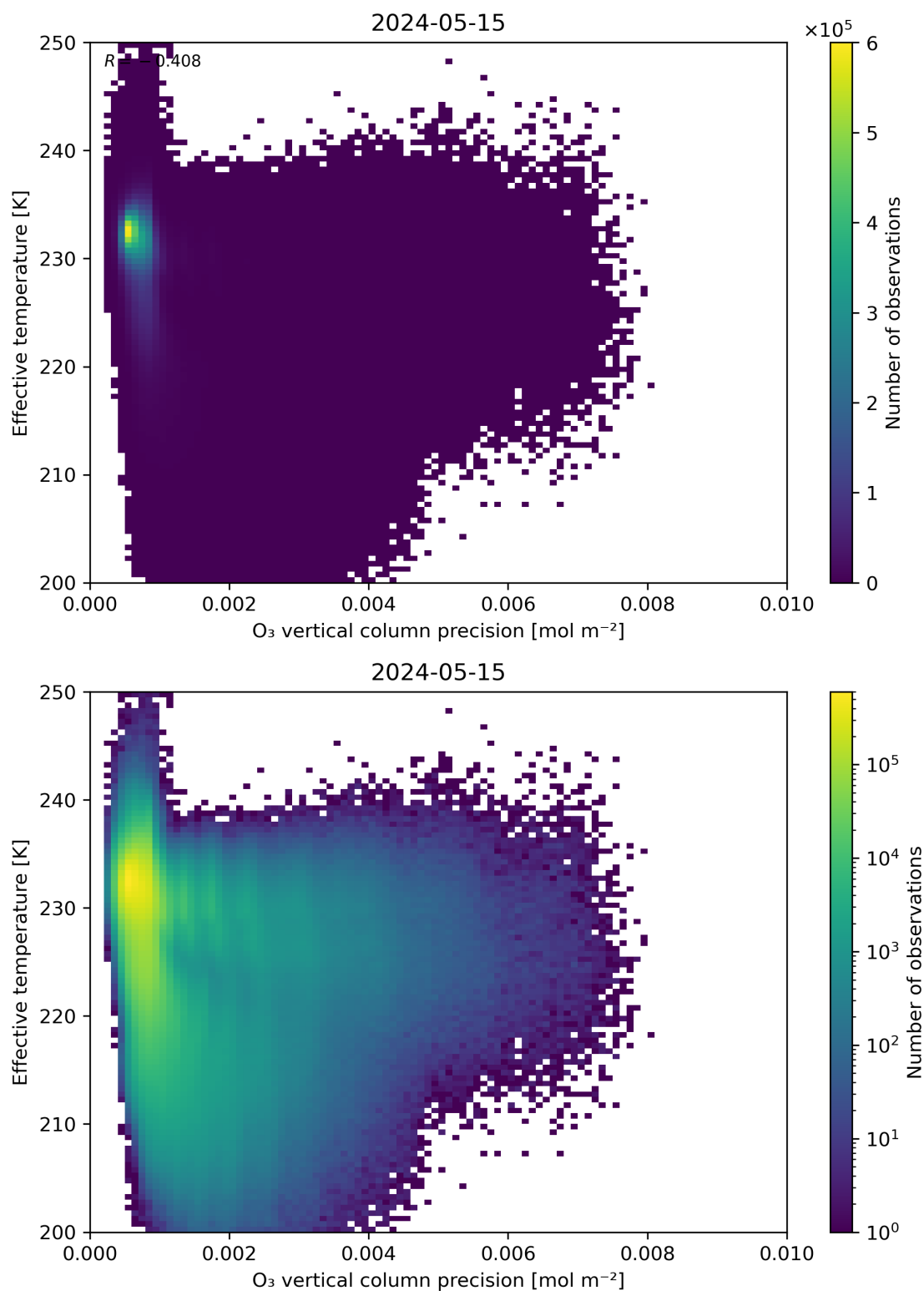
Figure 42: Scatter density plot of “O 3 vertical column precision” against “Effective temperature” for 2024-05-14 to 2024-05-16.
