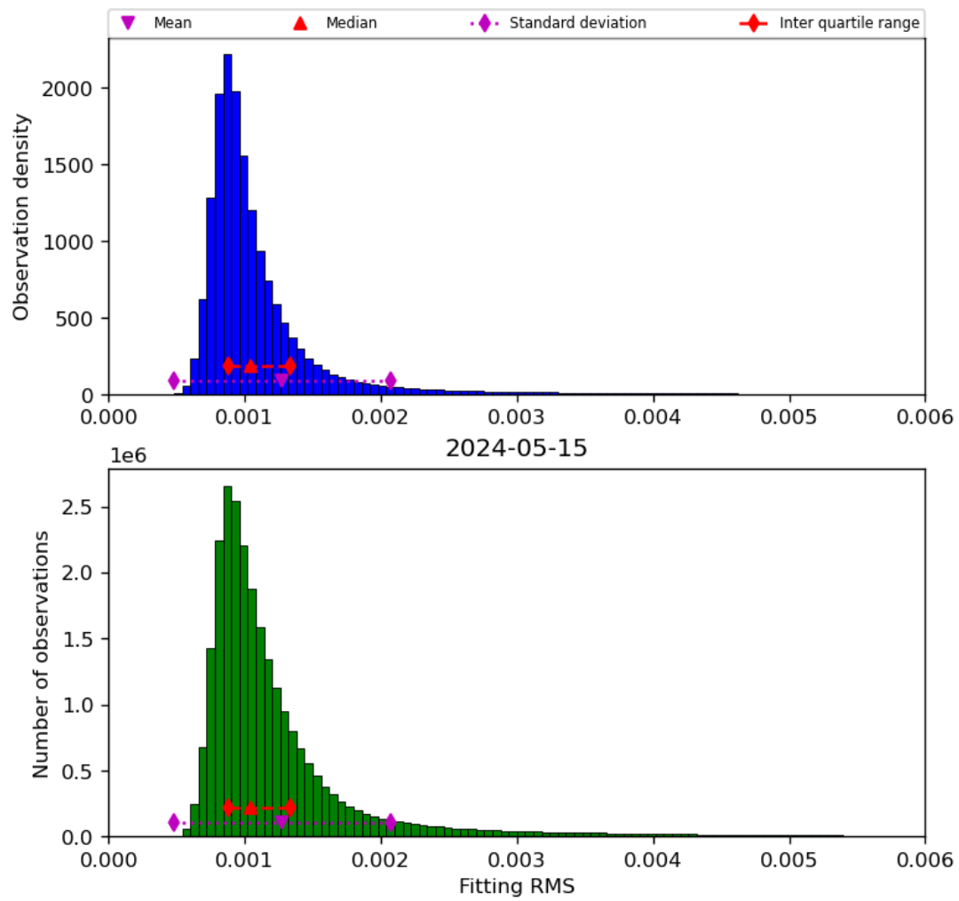
Figure 23: Histogram of “Fitting RMS” for 2024-05-14 to 2024-05-16
