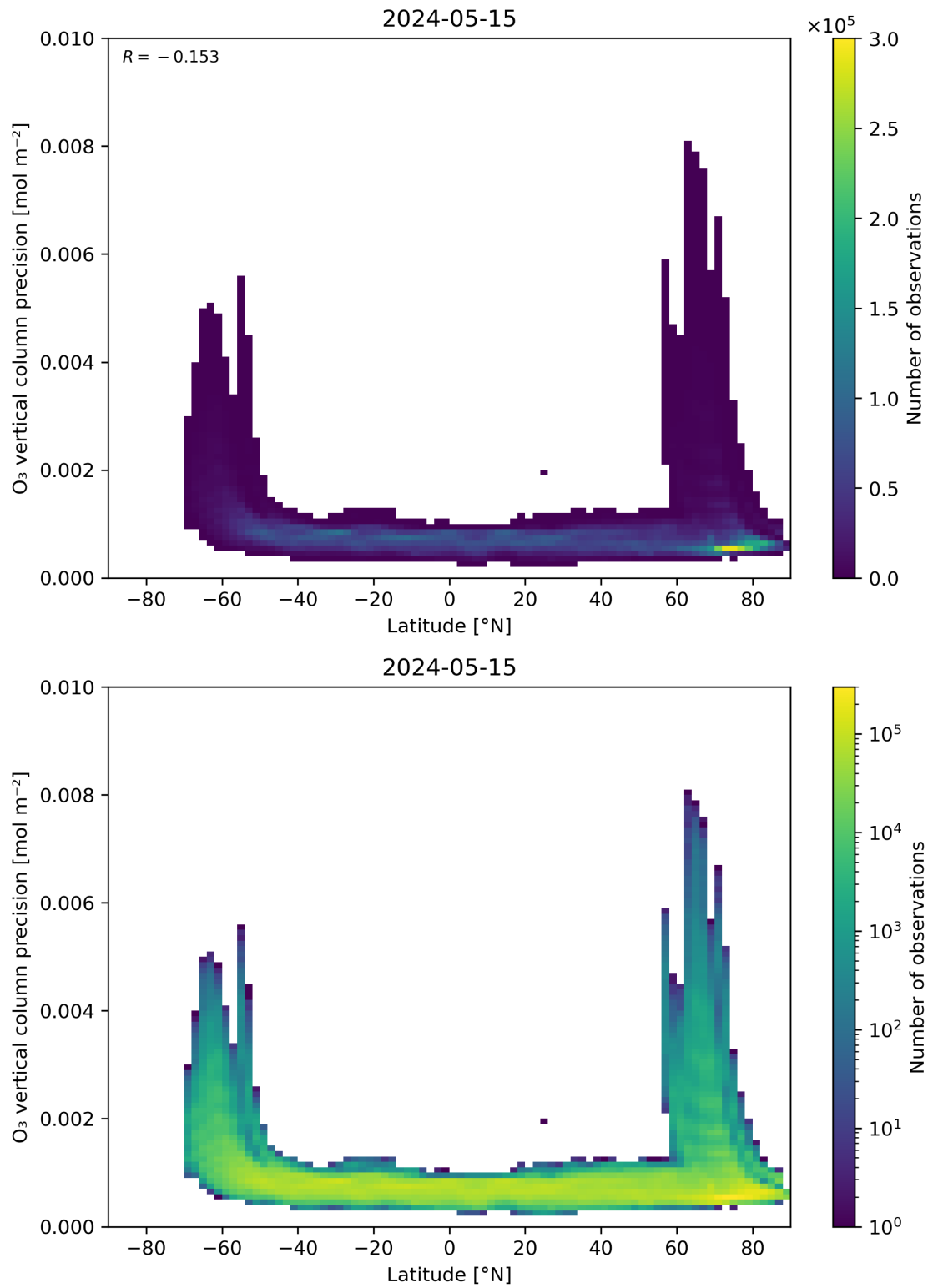
Figure 37: Scatter density plot of “Latitude” against “O 3 vertical column precision” for 2024-05-14 to 2024-05-16.
