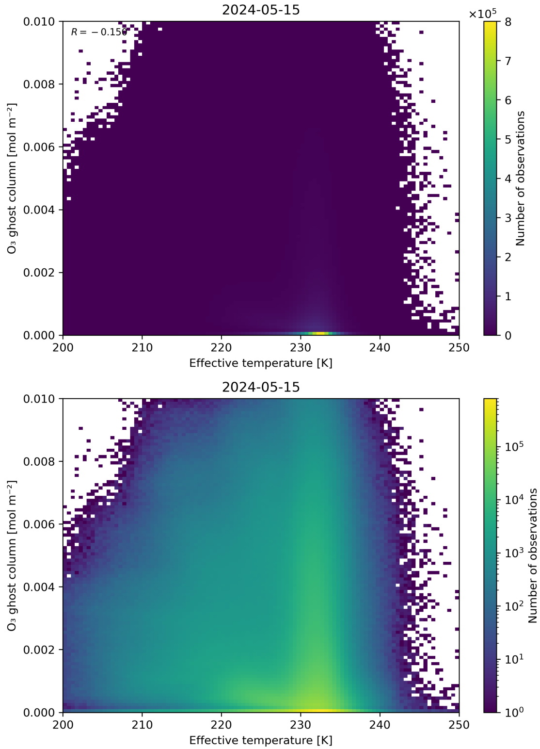
Figure 38: Scatter density plot of “Effective temperature” against “O 3 ghost column” for 2024-05-14 to 2024-05-16.
