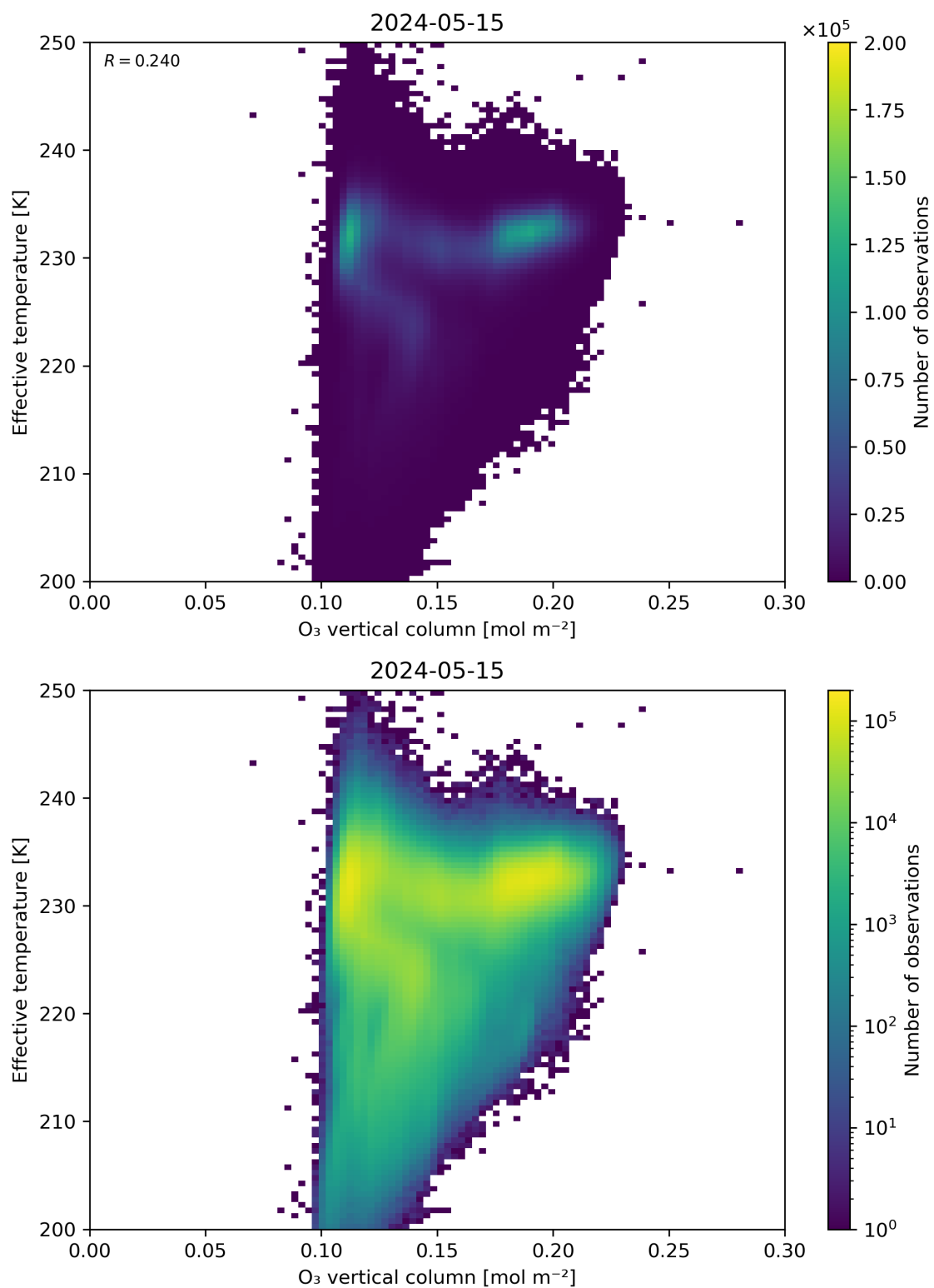
Figure 39: Scatter density plot of “O 3 vertical column” against “Effective temperature” for 2024-05-14 to 2024-05-16.
