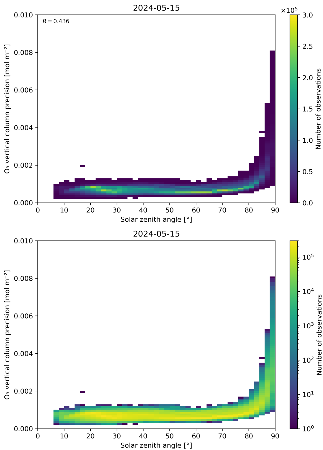
Figure 48: Scatter density plot of “Solar zenith angle” against “O 3 vertical column precision” for 2024-05-14 to 2024-05-16.
