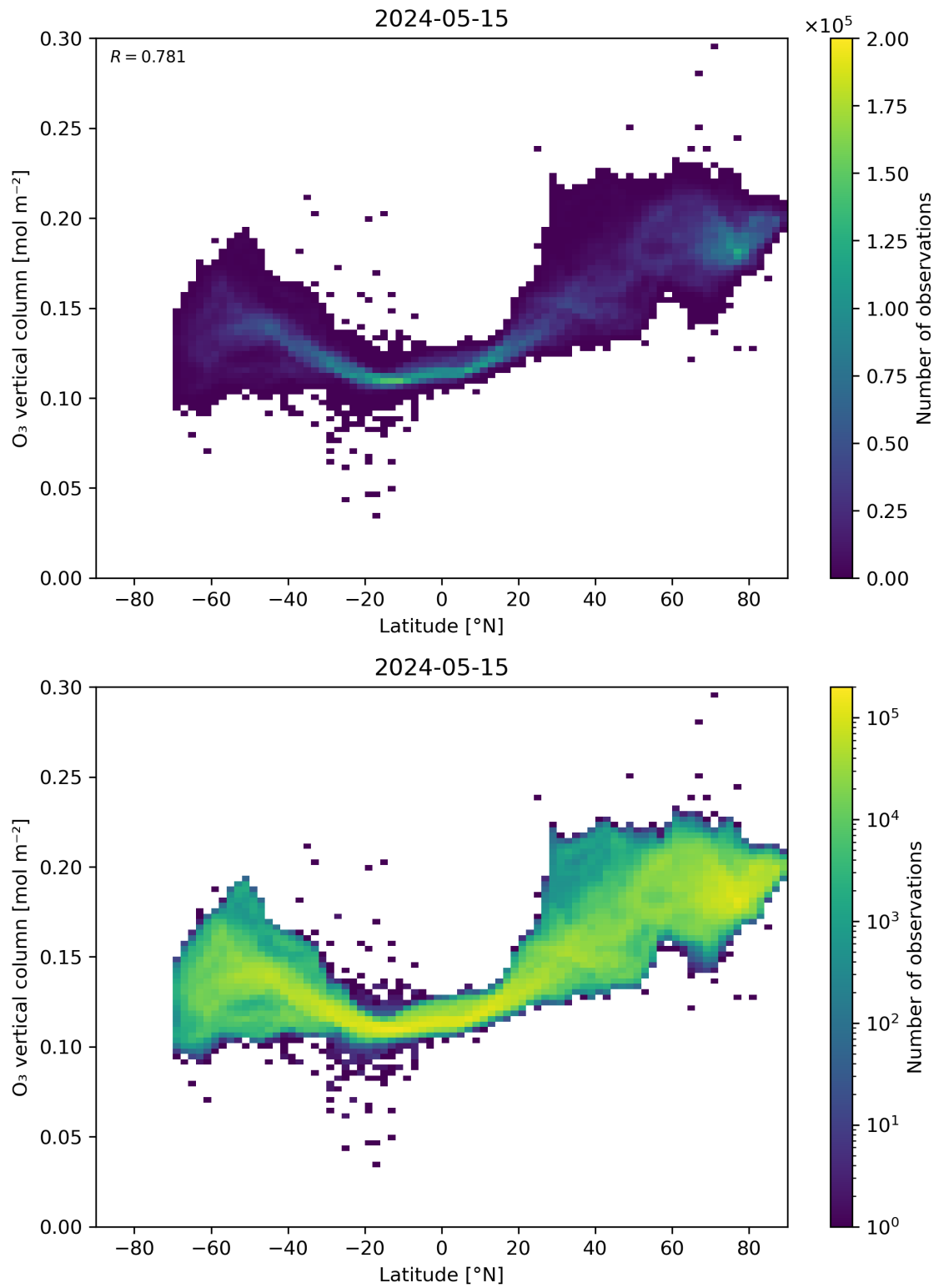
Figure 36: Scatter density plot of “Latitude” against “O 3 vertical column” for 2024-05-14 to 2024-05-16.
