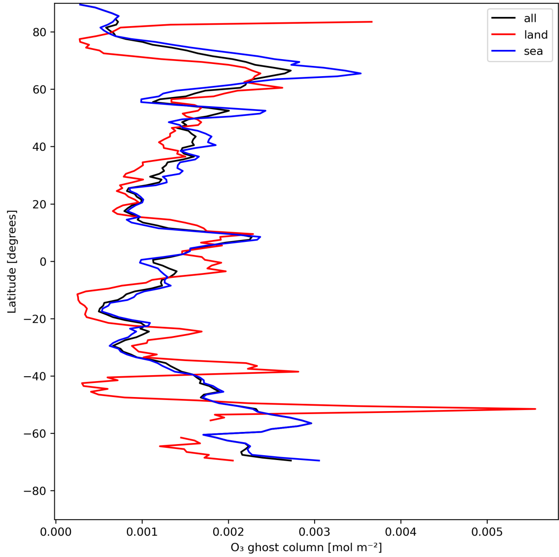
Figure 18: Zonal average of “O 3 ghost column” for 2024-05-14 to 2024-05-16.
