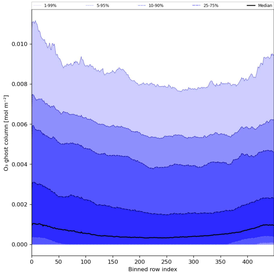
Figure 32: Along track statistics of “O 3 ghost column” for 2024-05-14 to 2024-05-16
