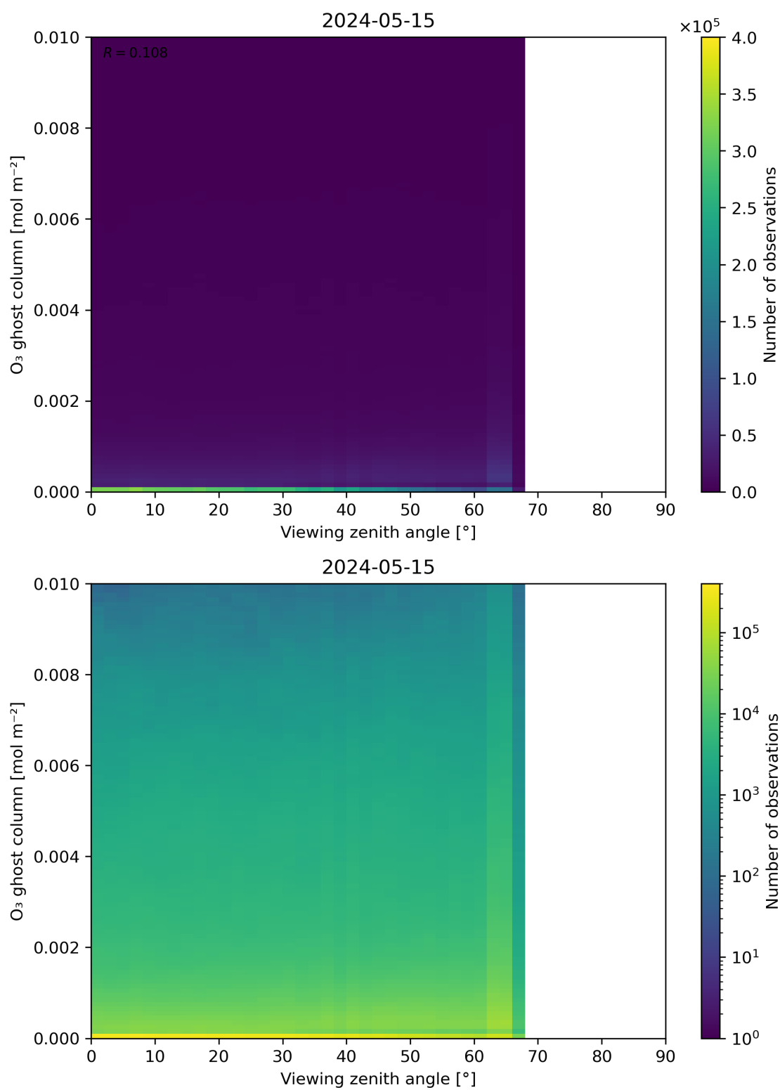
Figure 51: Scatter density plot of “Viewing zenith angle” against “O 3 ghost column” for 2024-05-14 to 2024-05-16.
