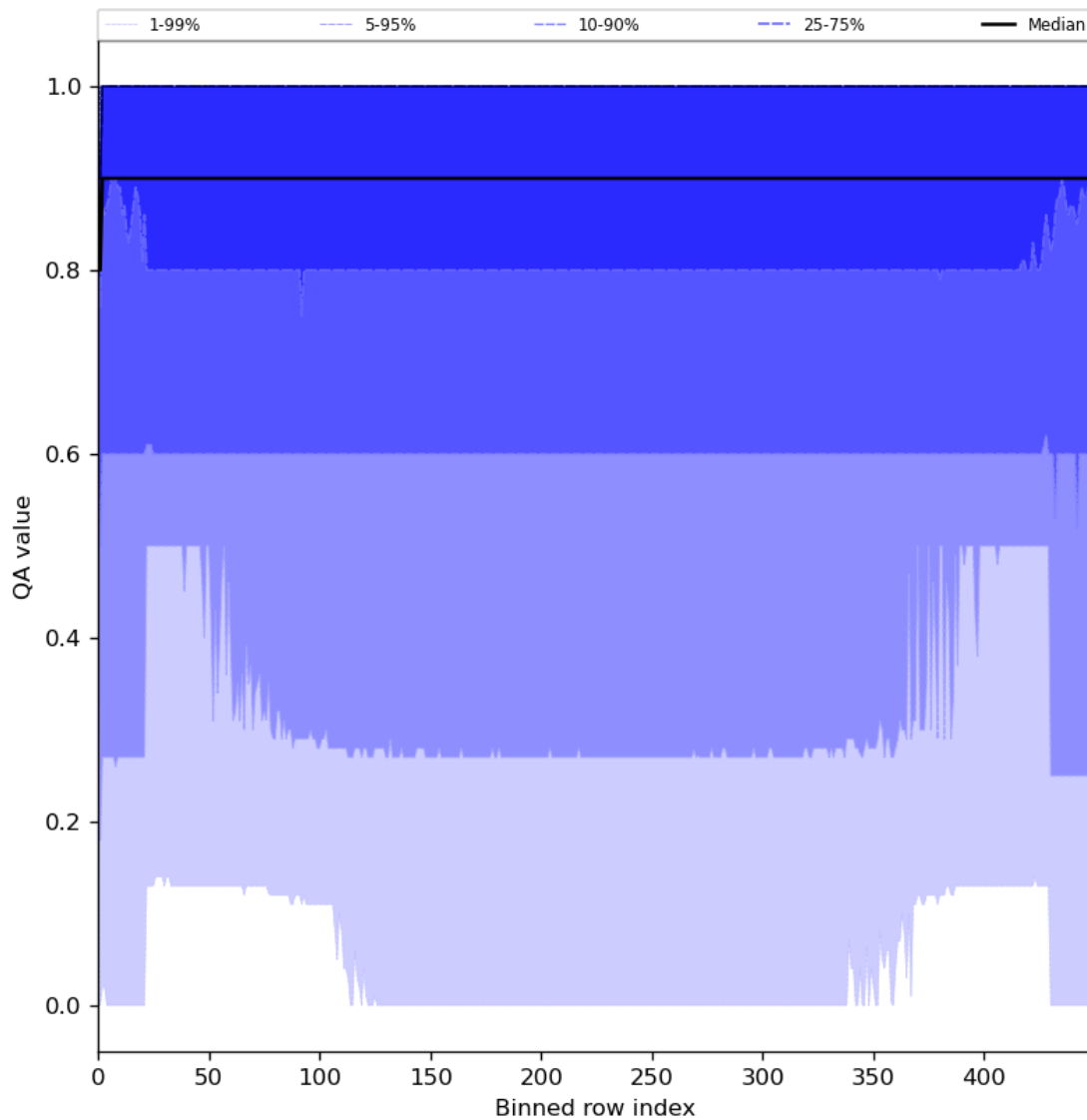
Figure 27: Along track statistics of “QA value” for 2024-05-14 to 2024-05-16
