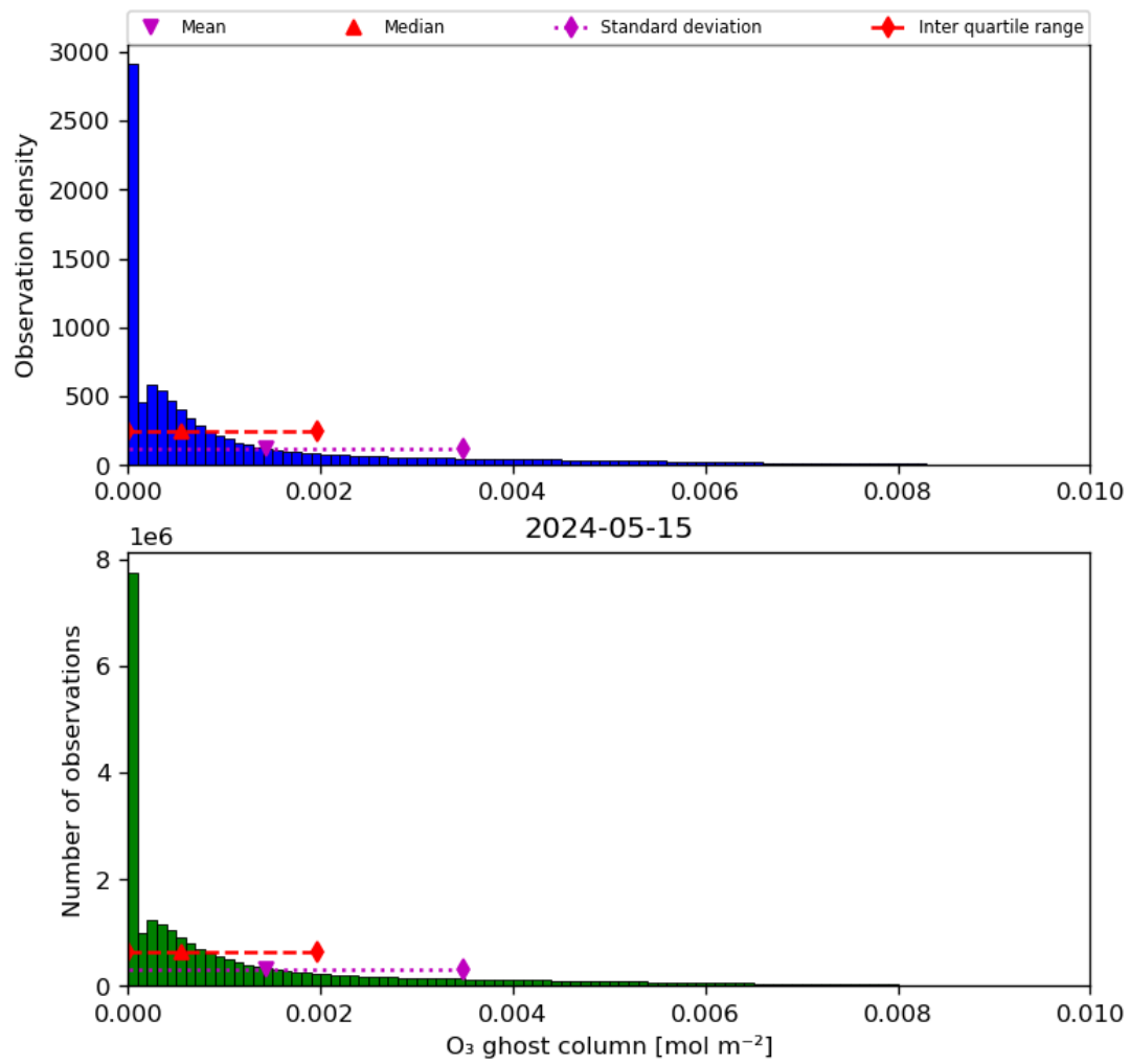
Figure 25: Histogram of “O 3 ghost column” for 2024-05-14 to 2024-05-16
