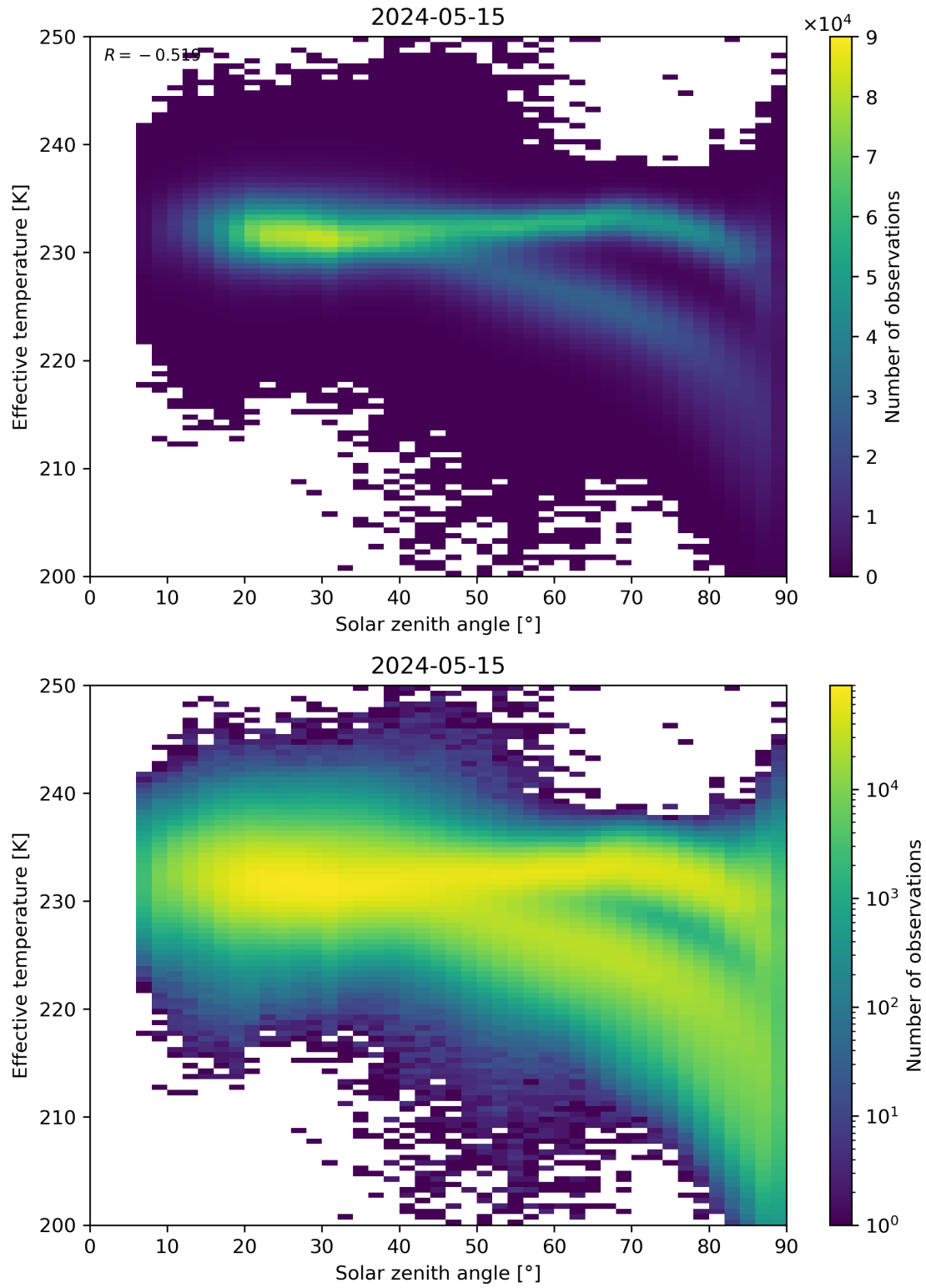
Figure 45: Scatter density plot of “Solar zenith angle” against “Effective temperature” for 2024-05-14 to 2024-05-16.
