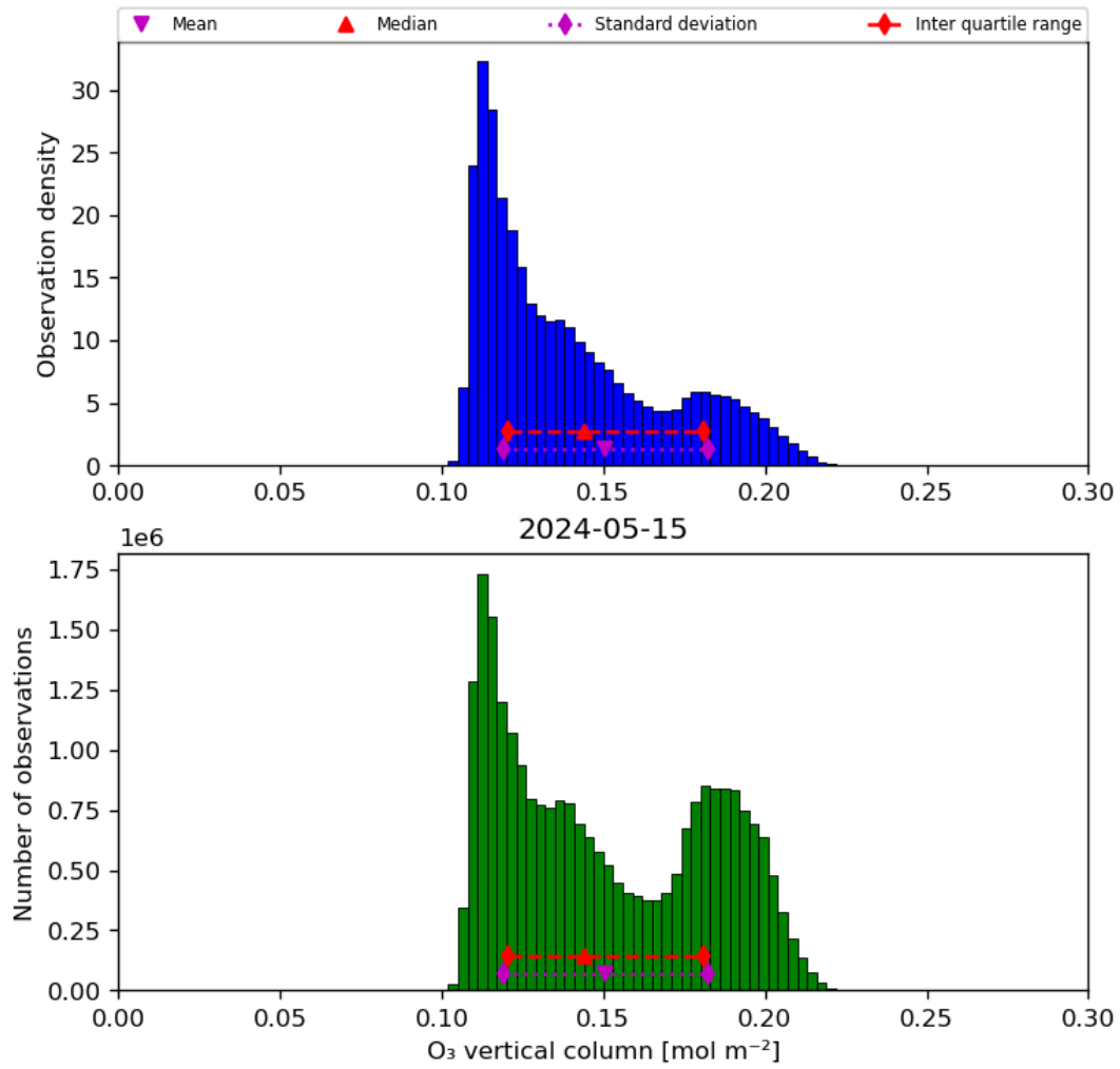
Figure 21: Histogram of “O 3 vertical column” for 2024-05-14 to 2024-05-16
