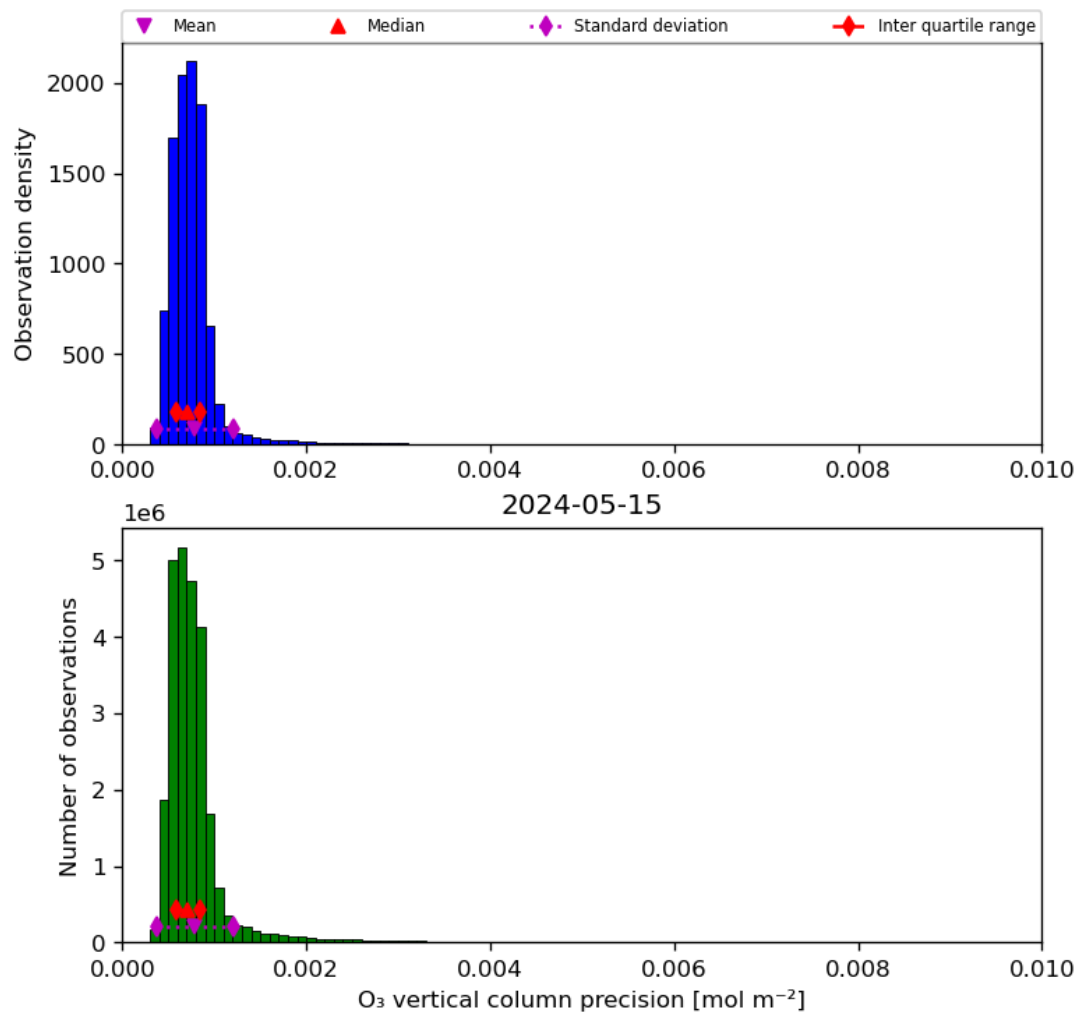
Figure 22: Histogram of “O 3 vertical column precision” for 2024-05-14 to 2024-05-16
