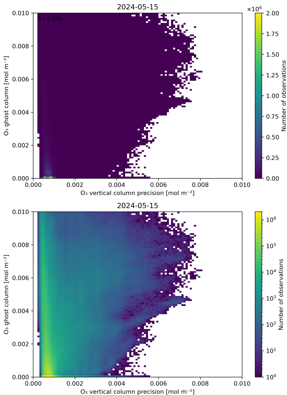
Figure 43: Scatter density plot of “ \text{O}_3 vertical column precision” against “ \text{O}_3 ghost column” for 2024-05-14 to 2024-05-16.
