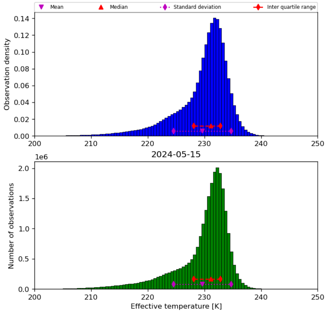
Figure 24: Histogram of “Effective temperature” for 2024-05-14 to 2024-05-16
