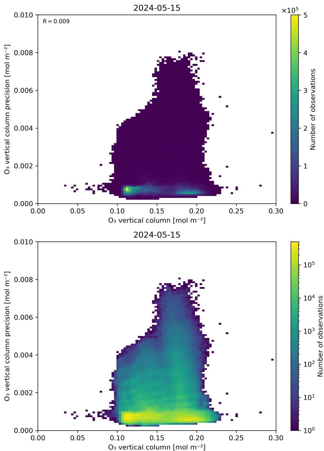
Figure 41: Scatter density plot of “O 3 vertical column” against “O 3 vertical column precision” for 2024-05-14 to 2024-05-16.
