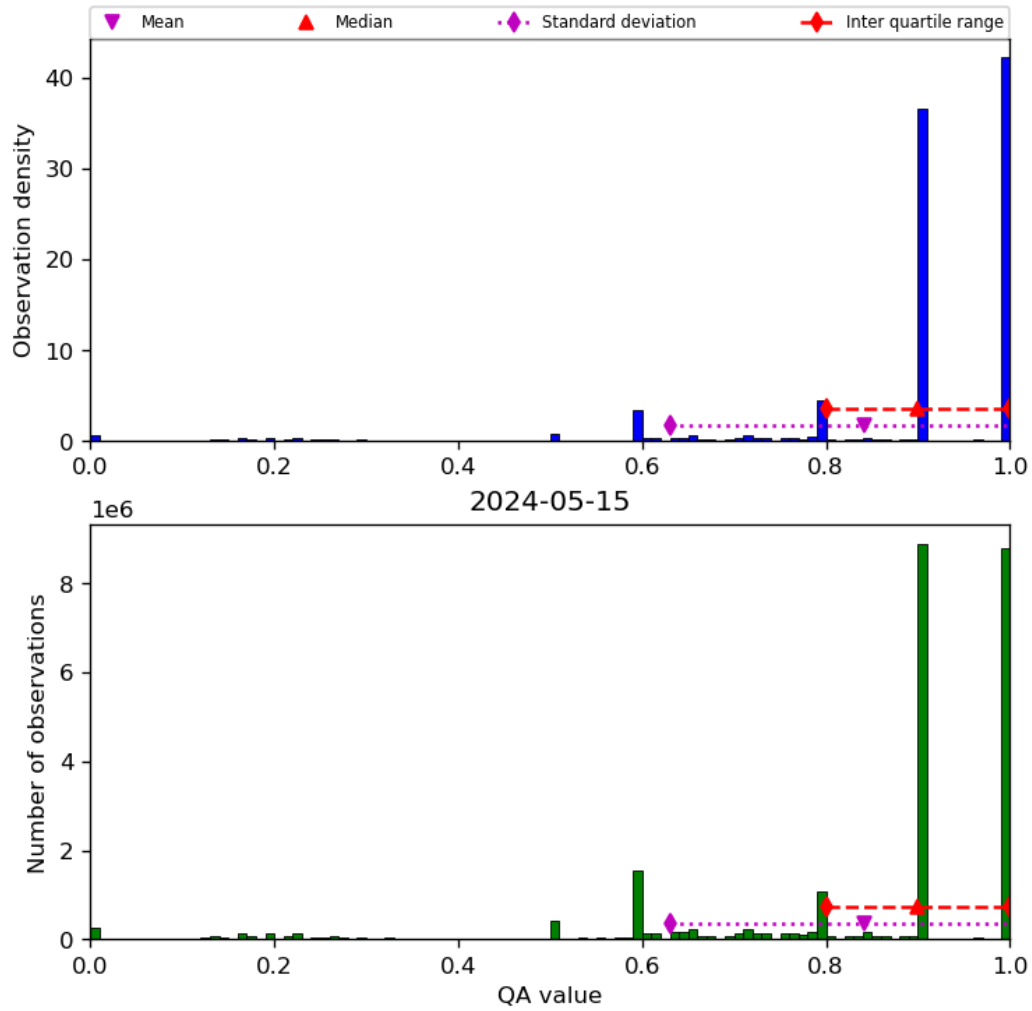
Figure 20: Histogram of “QA value” for 2024-05-14 to 2024-05-16
