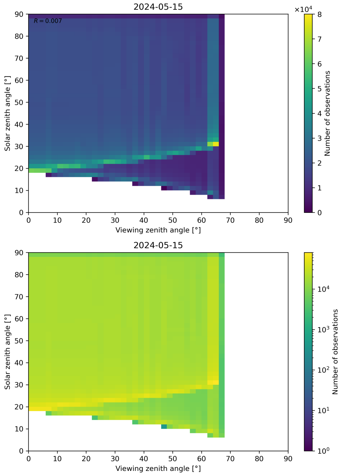
Figure 54: Scatter density plot of “Viewing zenith angle” against “Solar zenith angle” for 2024-05-14 to 2024-05-16.
