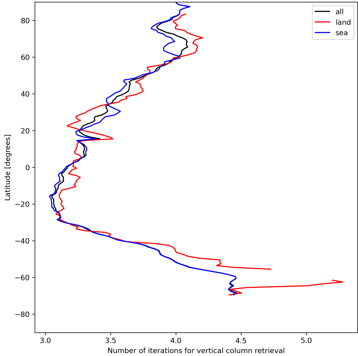
Figure 19: Zonal average of “Number of iterations for vertical column retrieval” for 2024-05-14 to 2024-05-16.
