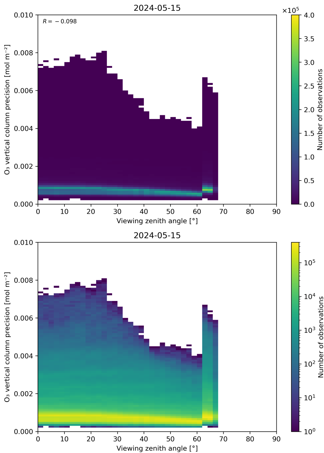
Figure 53: Scatter density plot of “Viewing zenith angle” against “O 3 vertical column precision” for 2024-05-14 to 2024-05-16.
