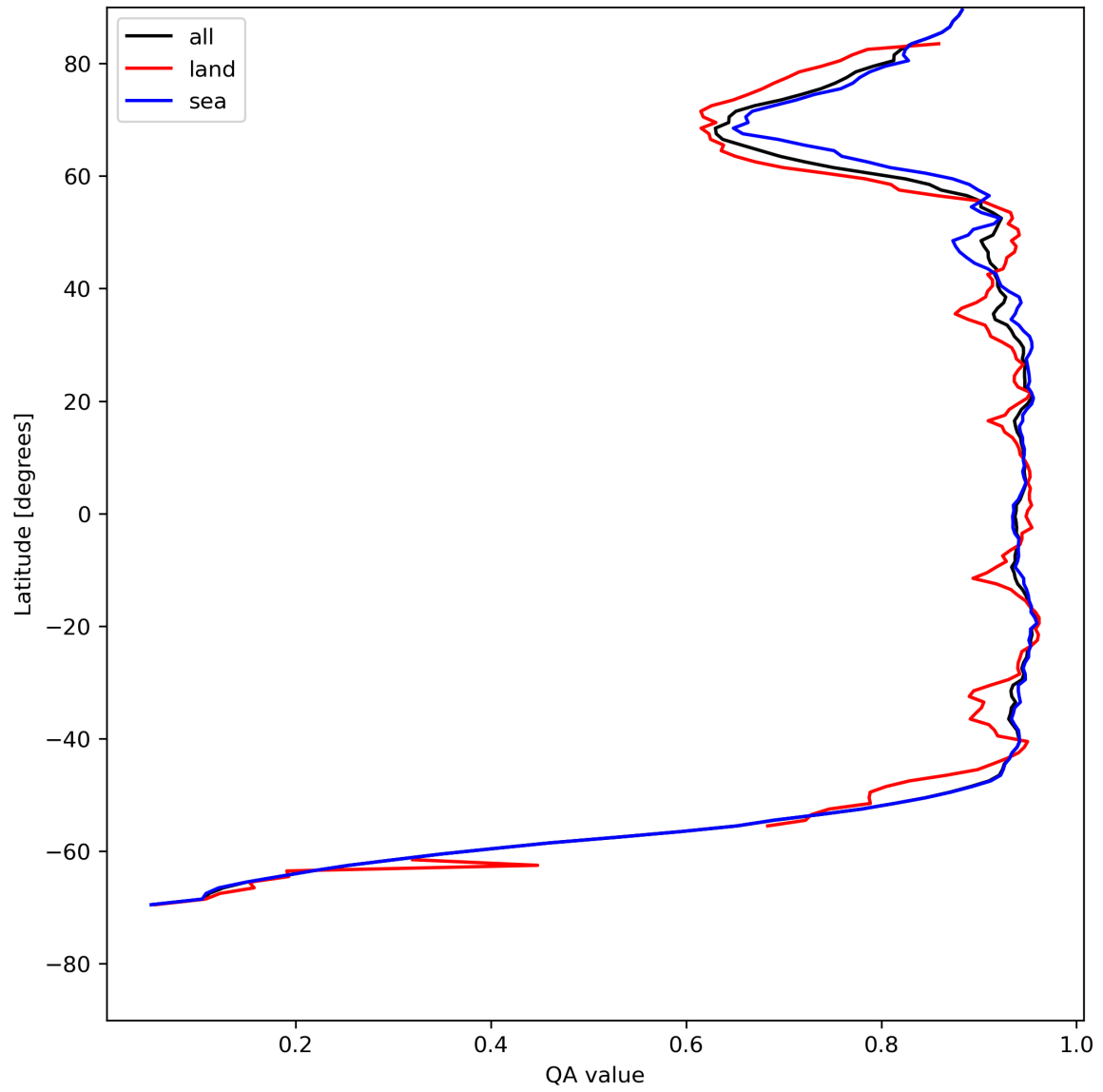
Figure 13: Zonal average of “QA value” for 2024-05-14 to 2024-05-16.
