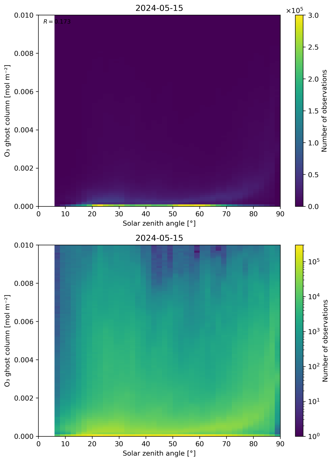
Figure 46: Scatter density plot of “Solar zenith angle” against “O 3 ghost column” for 2024-05-14 to 2024-05-16.
