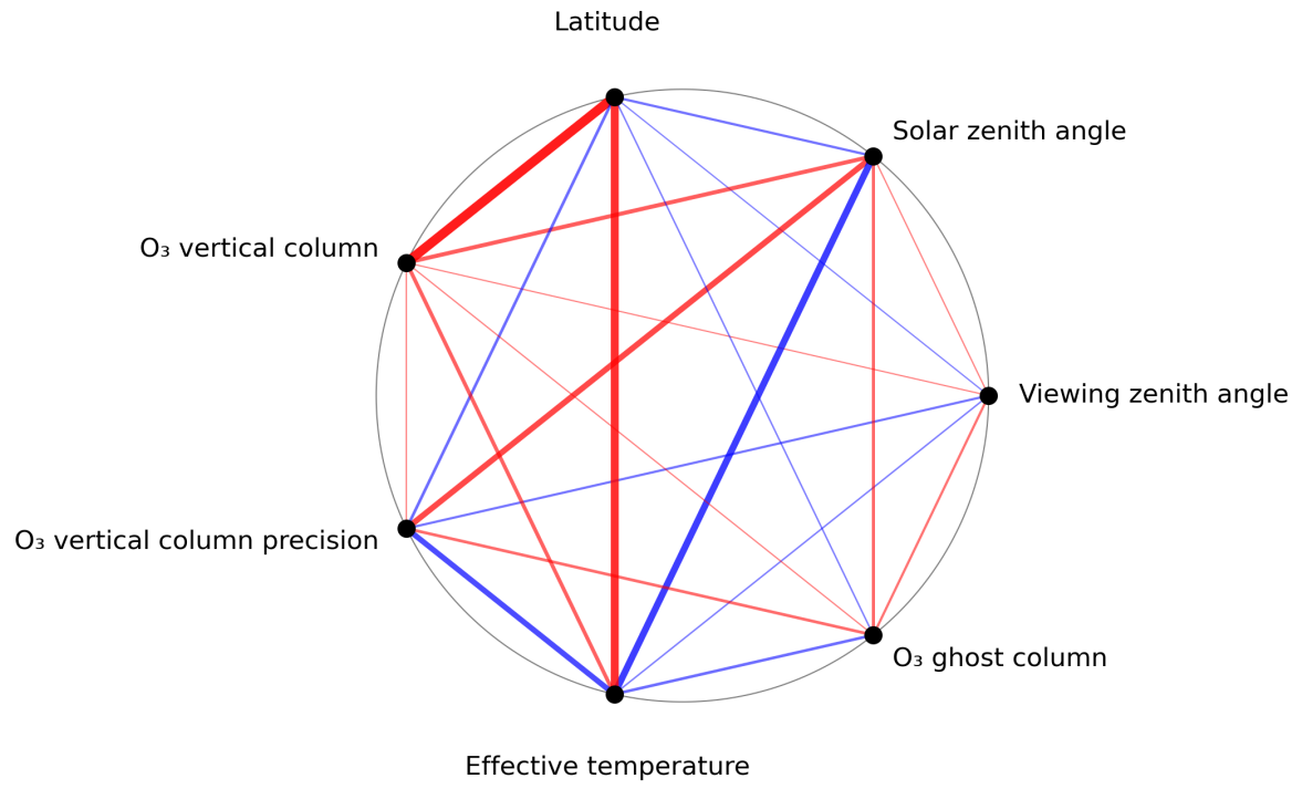
Figure 1: Map of correlation graph for 2024-05-14 to 2024-05-16.
