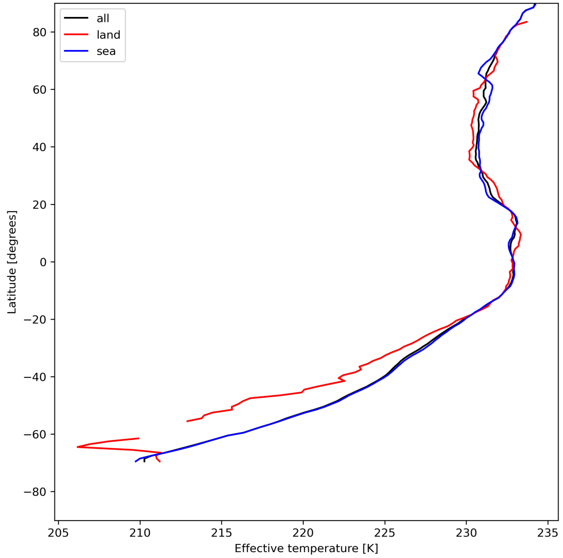
Figure 17: Zonal average of "Effective temperature" for 2024-05-14 to 2024-05-16.
