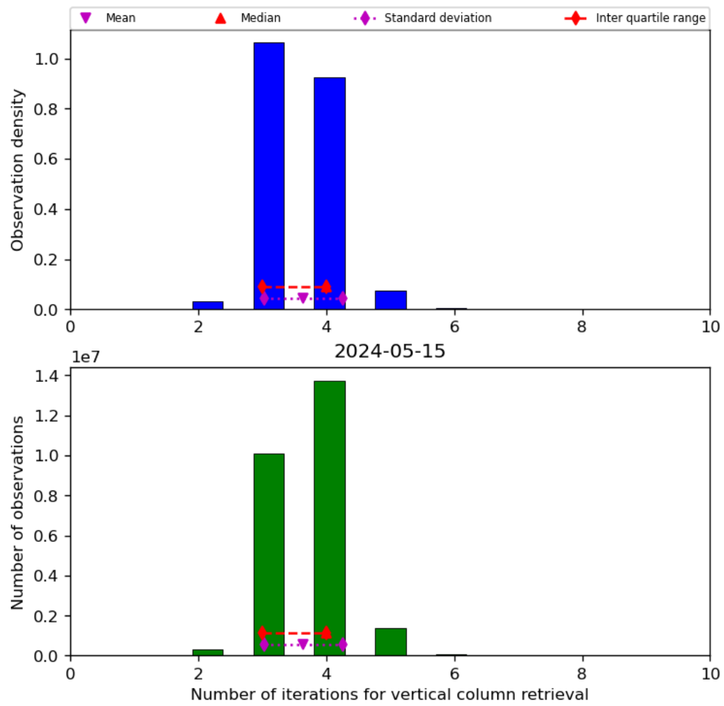
Figure 26: Histogram of “Number of iterations for vertical column retrieval” for 2024-05-14 to 2024-05-16
