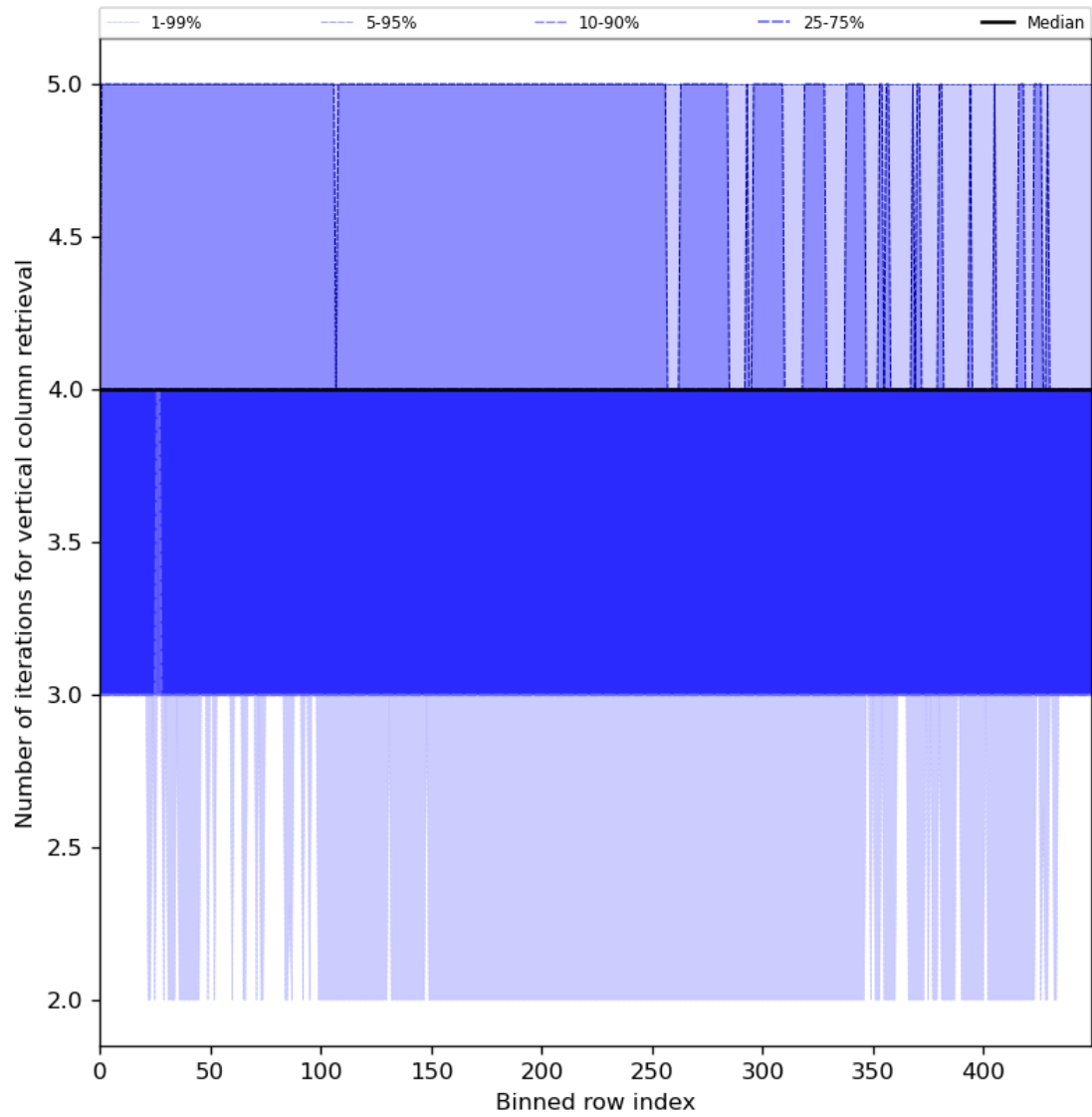
Figure 33: Along track statistics of “Number of iterations for vertical column retrieval” for 2024-05-14 to 2024-05-16
