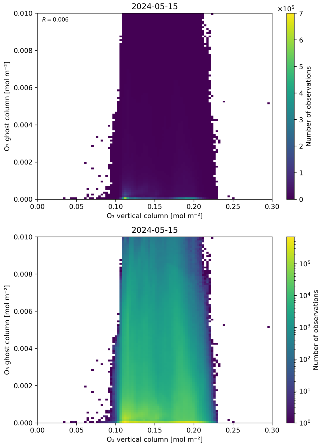
Figure 40: Scatter density plot of “O 3 vertical column” against “O 3 ghost column” for 2024-05-14 to 2024-05-16.
