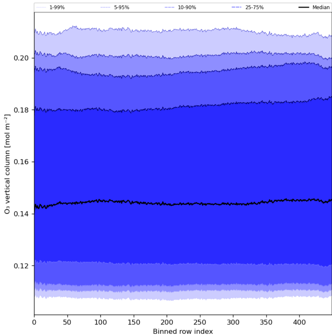
Figure 28: Along track statistics of “O 3 vertical column” for 2024-05-14 to 2024-05-16
