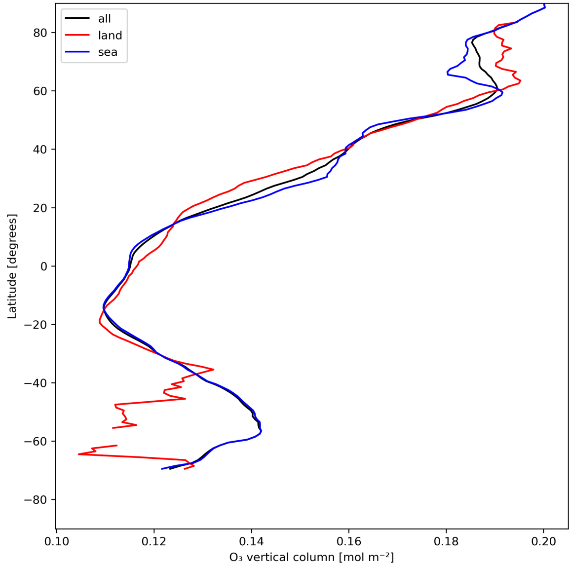
Figure 14: Zonal average of “O 3 vertical column” for 2024-05-14 to 2024-05-16.
