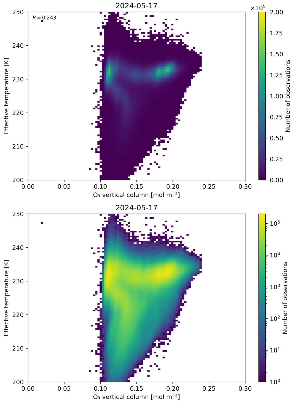
Figure 39: Scatter density plot of “O 3 vertical column” against “Effective temperature” for 2024-05-16 to 2024-05-18.
