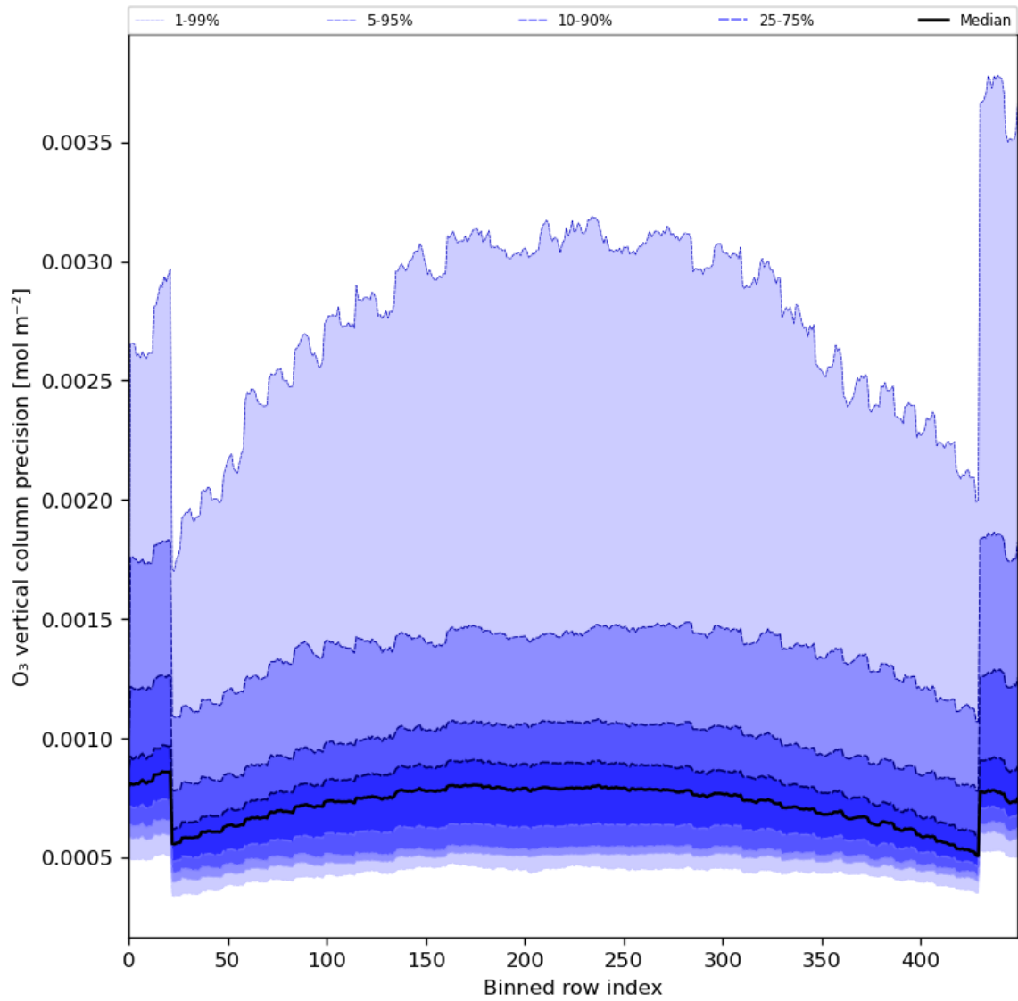
Figure 29: Along track statistics of “O 3 vertical column precision” for 2024-05-16 to 2024-05-18
