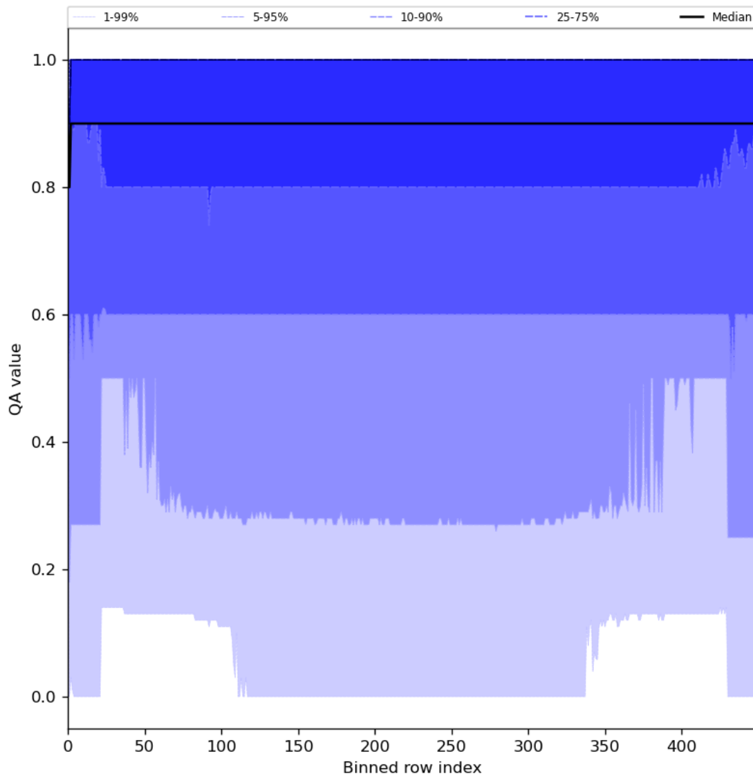
Figure 27: Along track statistics of “QA value” for 2024-05-16 to 2024-05-18
