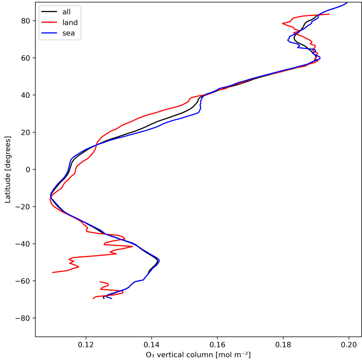
Figure 14: Zonal average of “O 3 vertical column” for 2024-05-16 to 2024-05-18.
