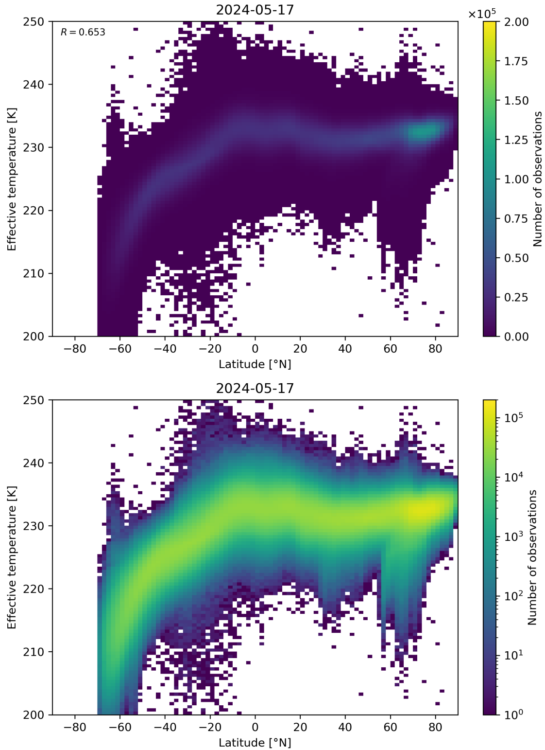
Figure 34: Scatter density plot of “Latitude” against “Effective temperature” for 2024-05-16 to 2024-05-18.
