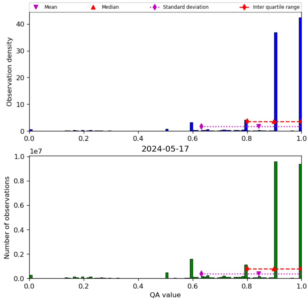
Figure 20: Histogram of “QA value” for 2024-05-16 to 2024-05-18
