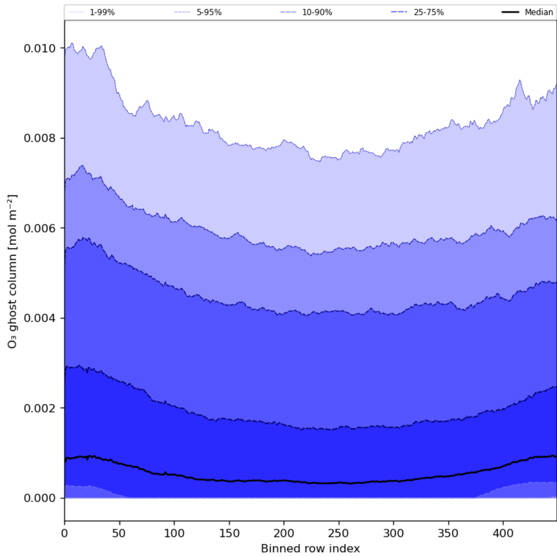
Figure 32: Along track statistics of “O 3 ghost column” for 2024-05-16 to 2024-05-18
