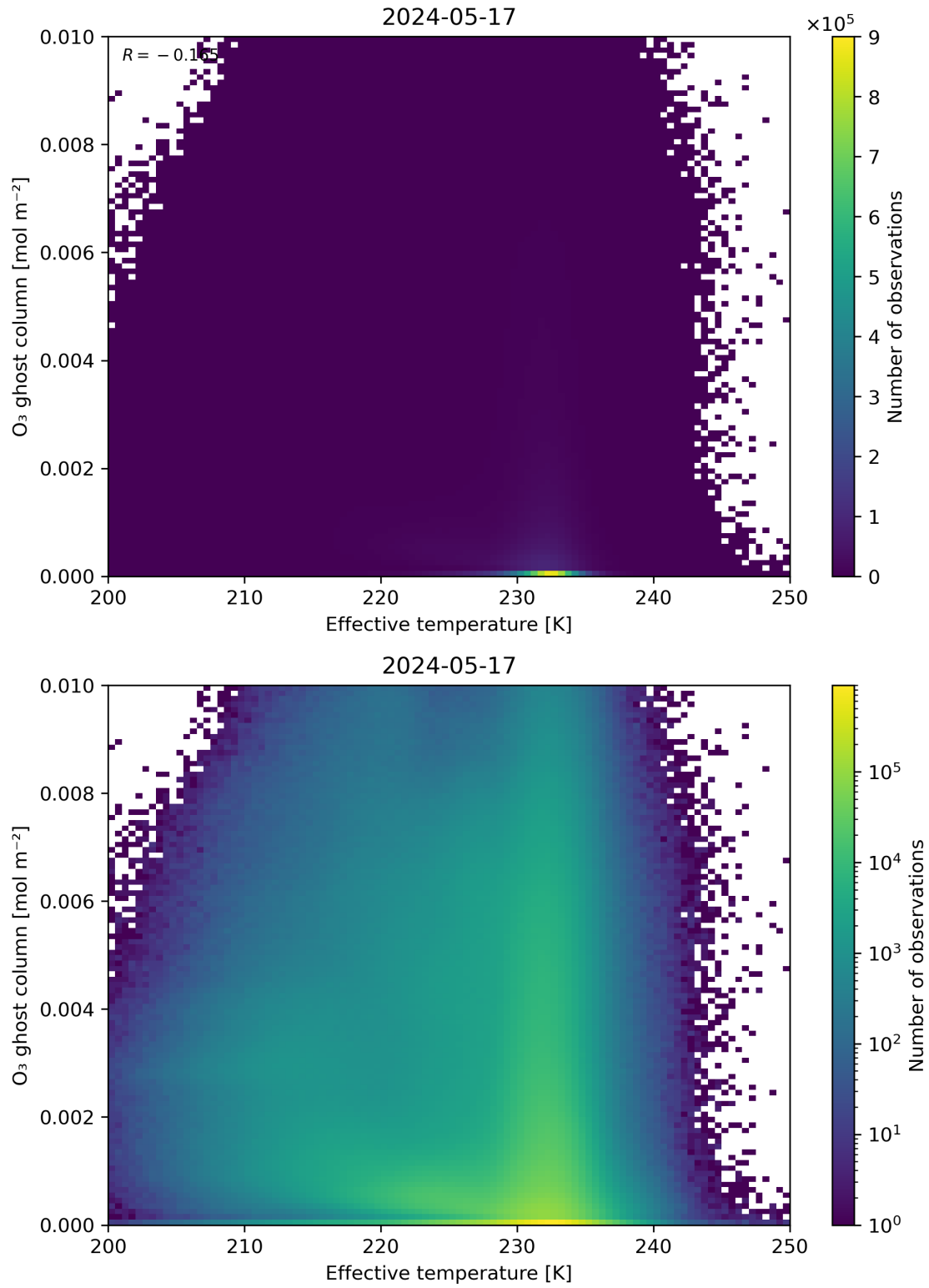
Figure 38: Scatter density plot of “Effective temperature” against “O 3 ghost column” for 2024-05-16 to 2024-05-18.
