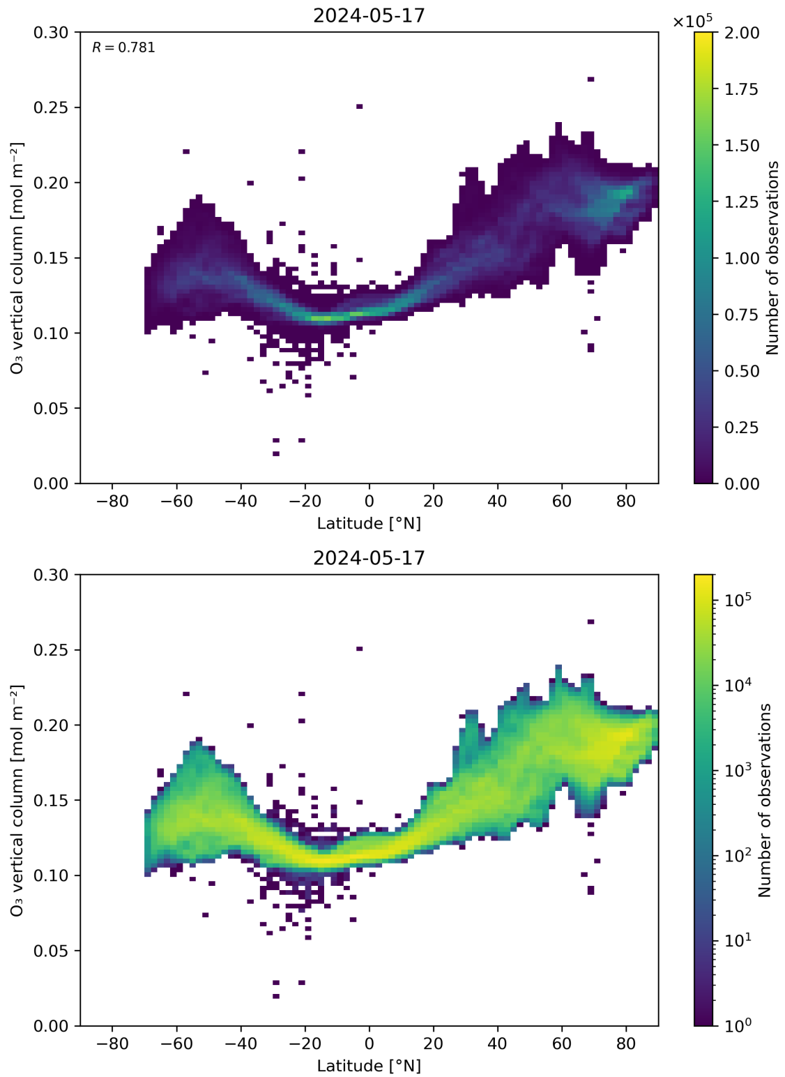
Figure 36: Scatter density plot of “Latitude” against “O 3 vertical column” for 2024-05-16 to 2024-05-18.
