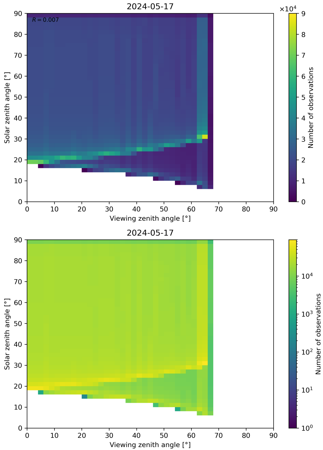
Figure 54: Scatter density plot of “Viewing zenith angle” against “Solar zenith angle” for 2024-05-16 to 2024-05-18.
