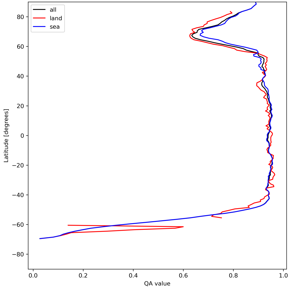
Figure 13: Zonal average of “QA value” for 2024-05-16 to 2024-05-18.
