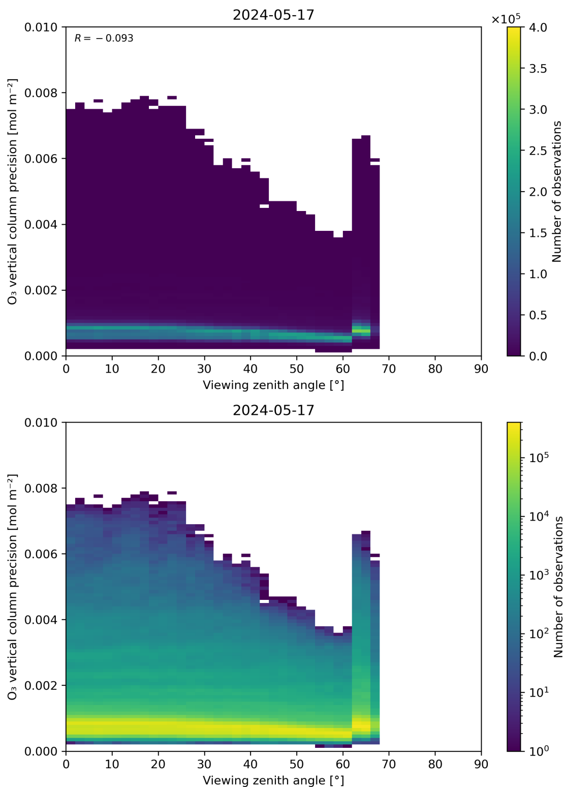
Figure 53: Scatter density plot of “Viewing zenith angle” against “O 3 vertical column precision” for 2024-05-16 to 2024-05-18.
