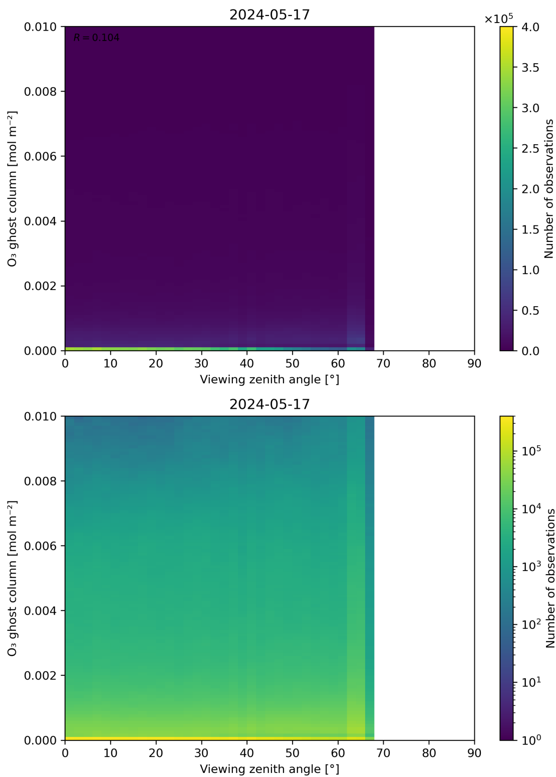
Figure 51: Scatter density plot of “Viewing zenith angle” against “O 3 ghost column” for 2024-05-16 to 2024-05-18.
