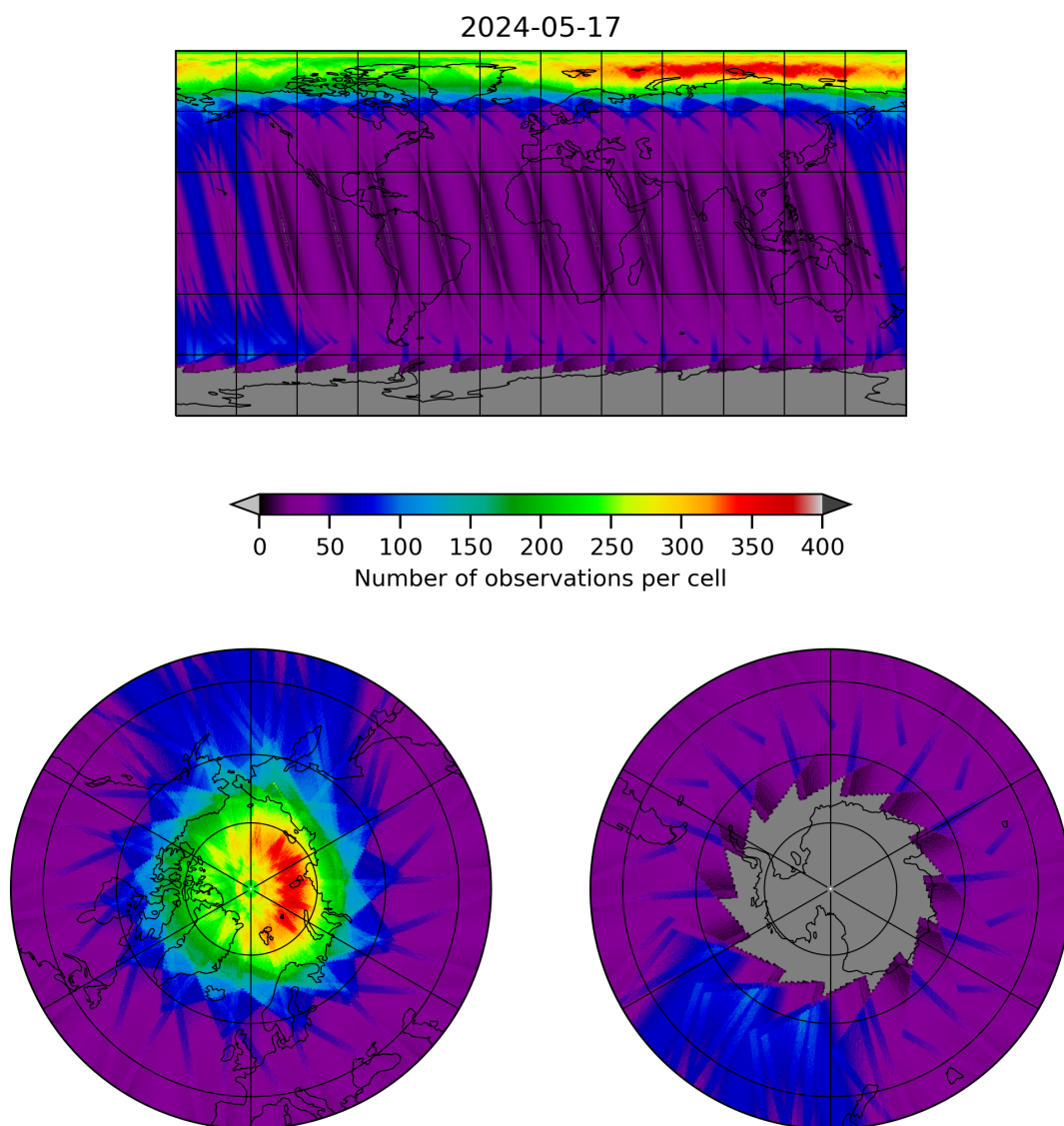
Figure 12: Map of the number of observations for 2024-05-16 to 2024-05-18
