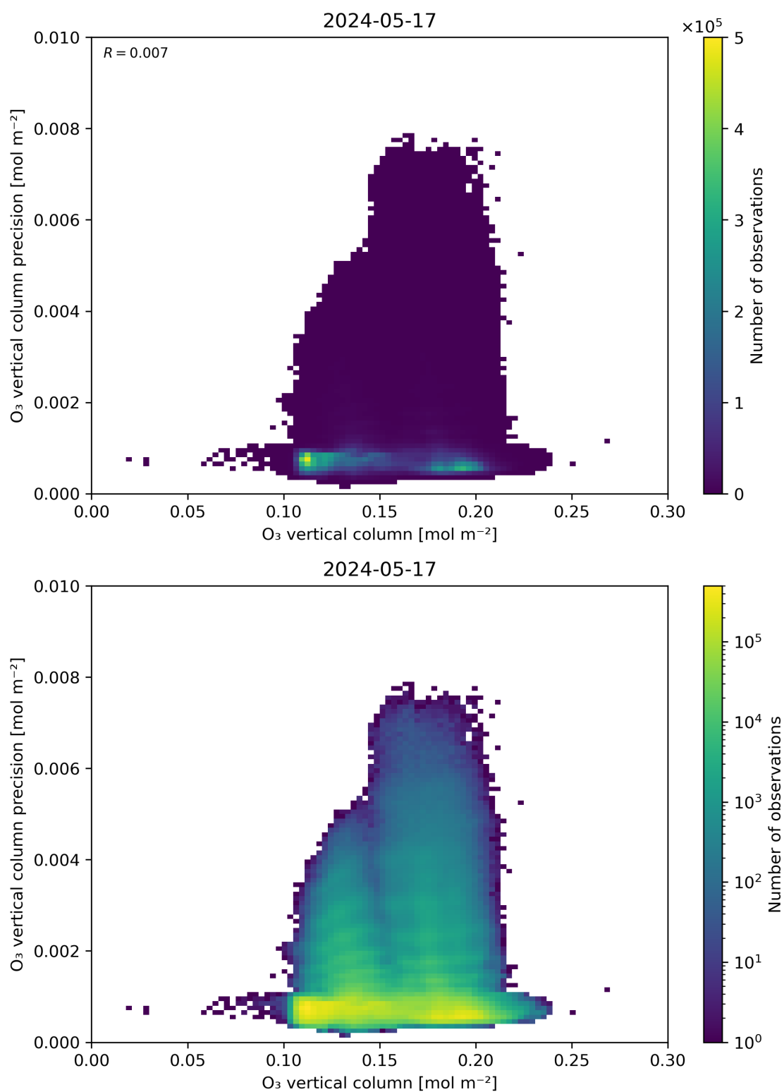
Figure 41: Scatter density plot of “O 3 vertical column” against “O 3 vertical column precision” for 2024-05-16 to 2024-05-18.
