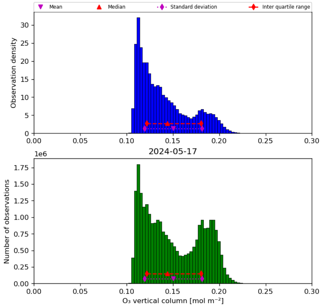
Figure 21: Histogram of “O 3 vertical column” for 2024-05-16 to 2024-05-18
