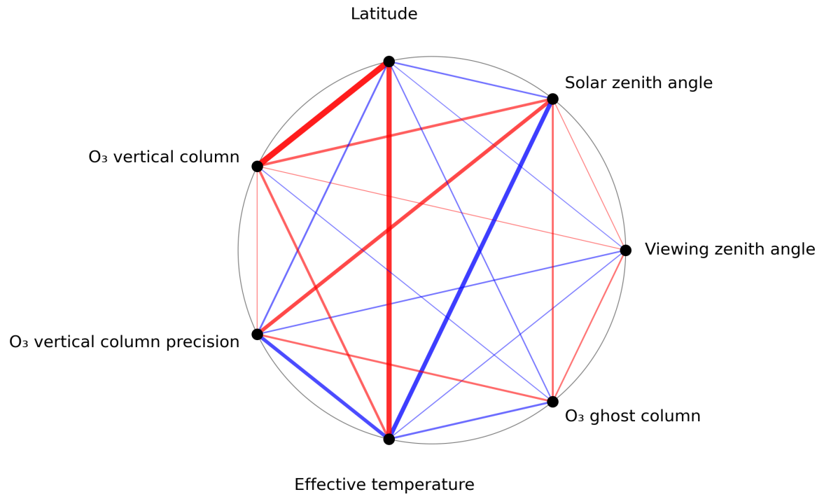
Figure 1: Map of correlation graph for 2024-05-16 to 2024-05-18.
