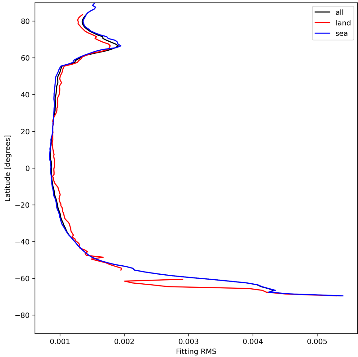
Figure 16: Zonal average of “Fitting RMS” for 2024-05-16 to 2024-05-18.
