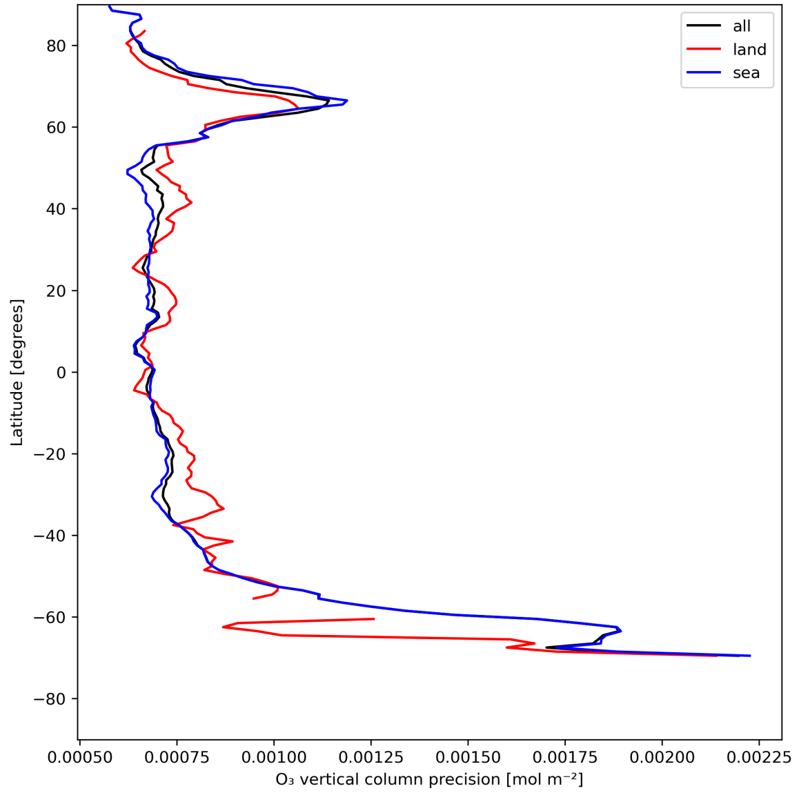
Figure 15: Zonal average of “O 3 vertical column precision” for 2024-05-16 to 2024-05-18.
