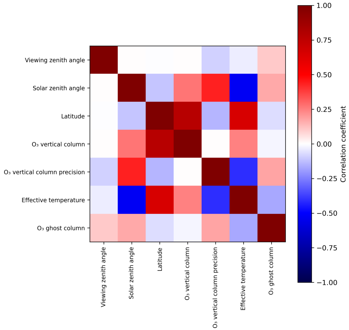
Figure 2: Map of correlation matrix for 2024-05-16 to 2024-05-18.
