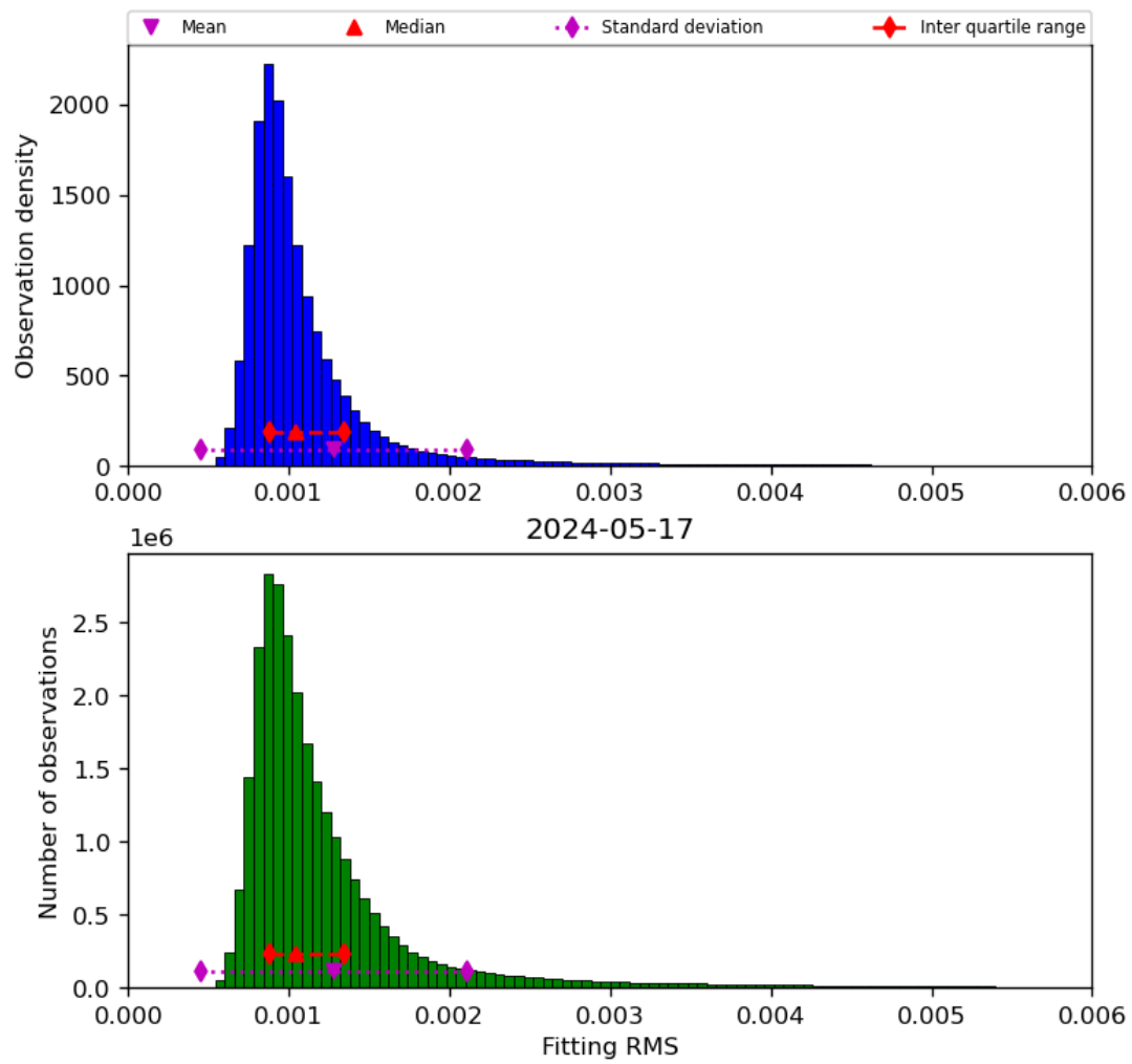
Figure 23: Histogram of “Fitting RMS” for 2024-05-16 to 2024-05-18
