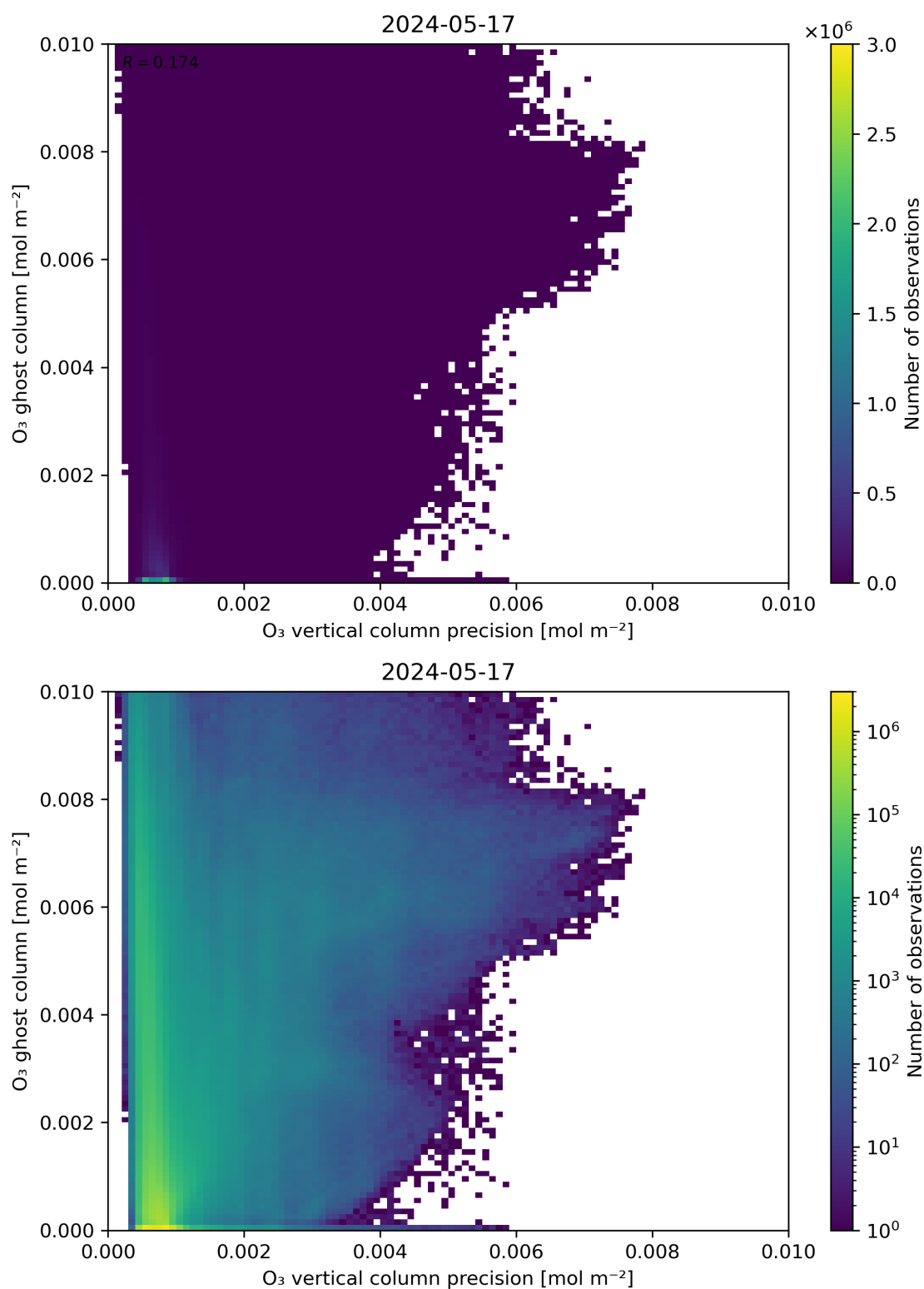
Figure 43: Scatter density plot of “O 3 vertical column precision” against “O 3 ghost column” for 2024-05-16 to 2024-05-18.
