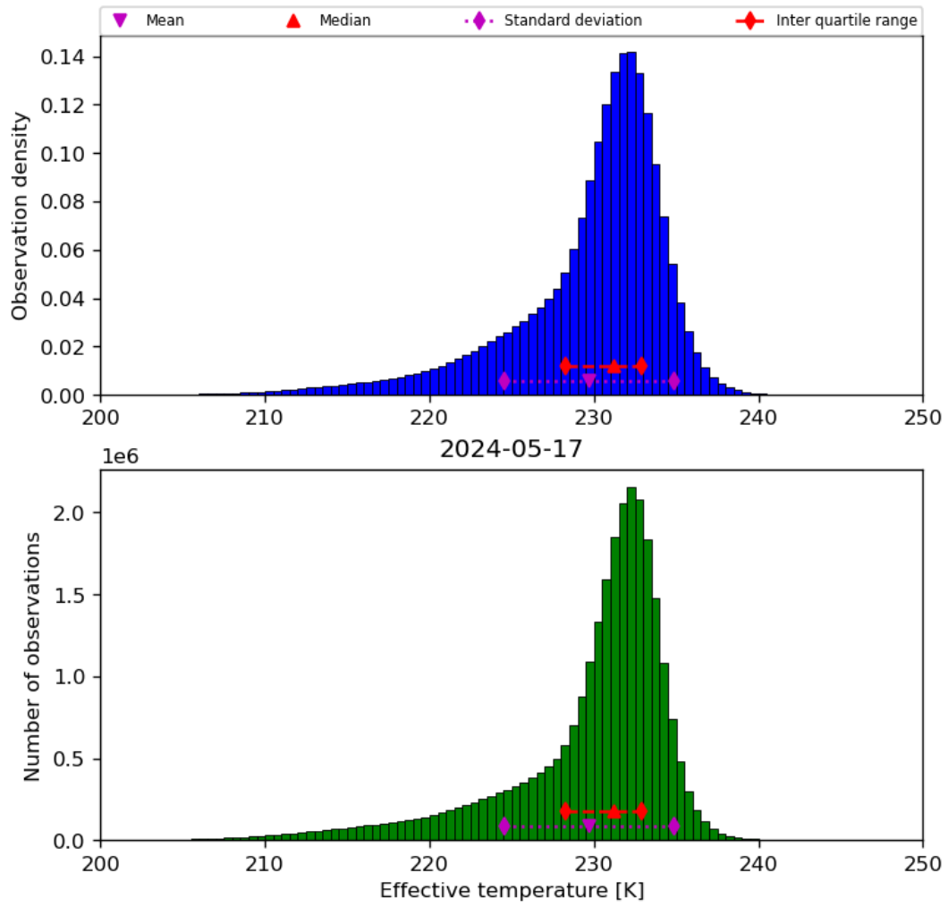
Figure 24: Histogram of “Effective temperature” for 2024-05-16 to 2024-05-18
