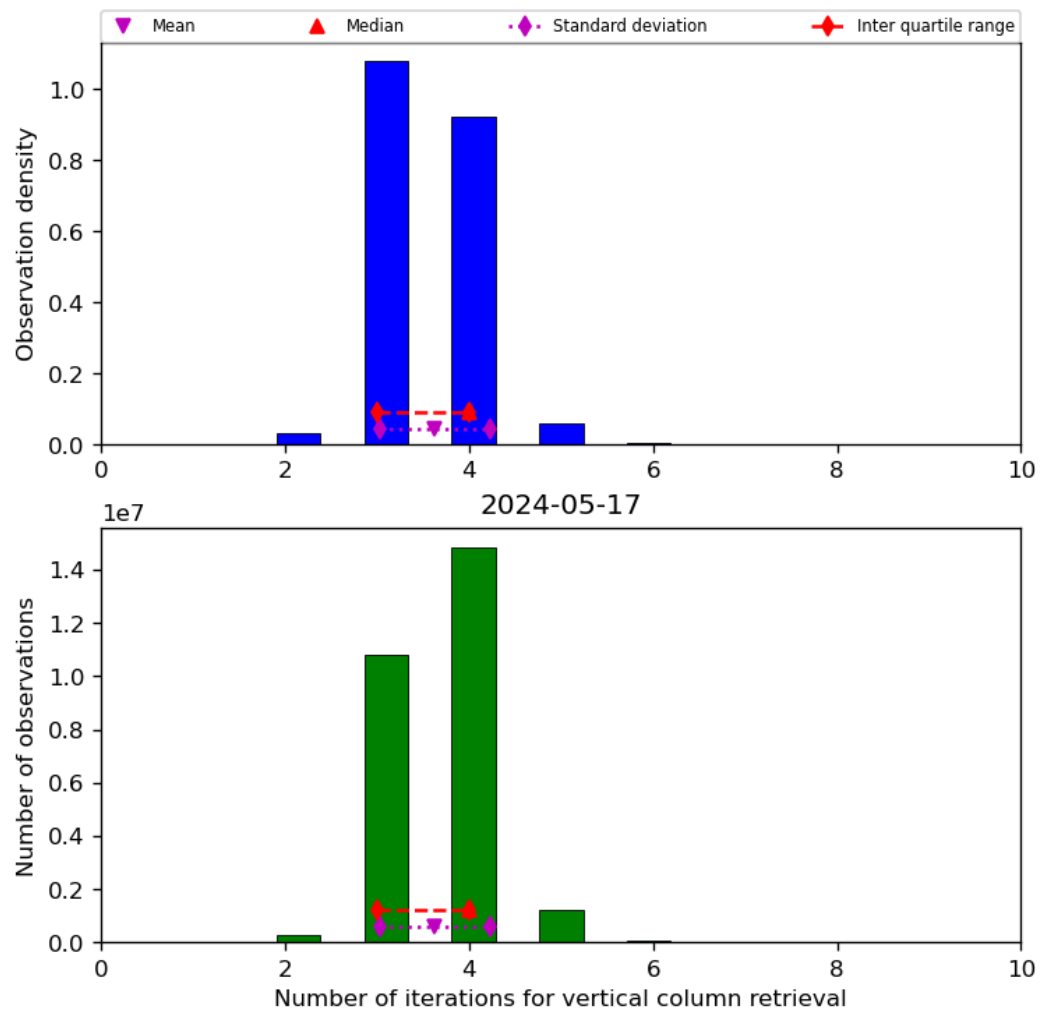
Figure 26: Histogram of “Number of iterations for vertical column retrieval” for 2024-05-16 to 2024-05-18
