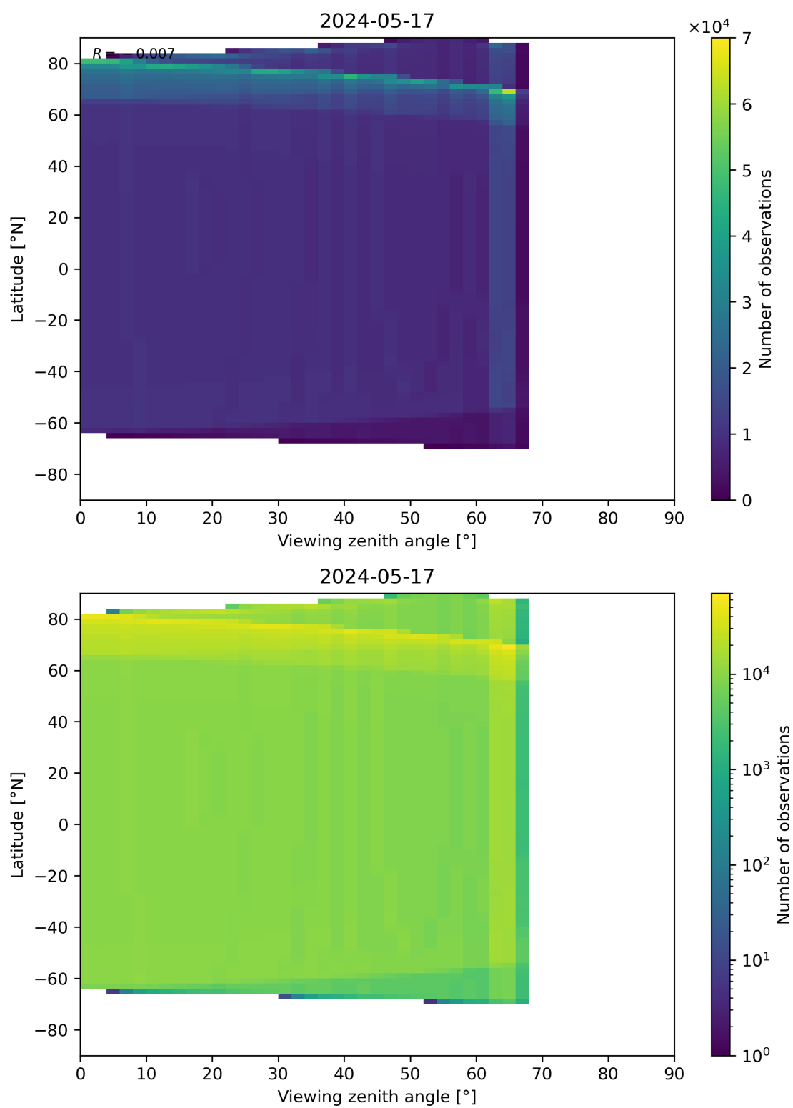
Figure 49: Scatter density plot of “Viewing zenith angle” against “Latitude” for 2024-05-16 to 2024-05-18.
