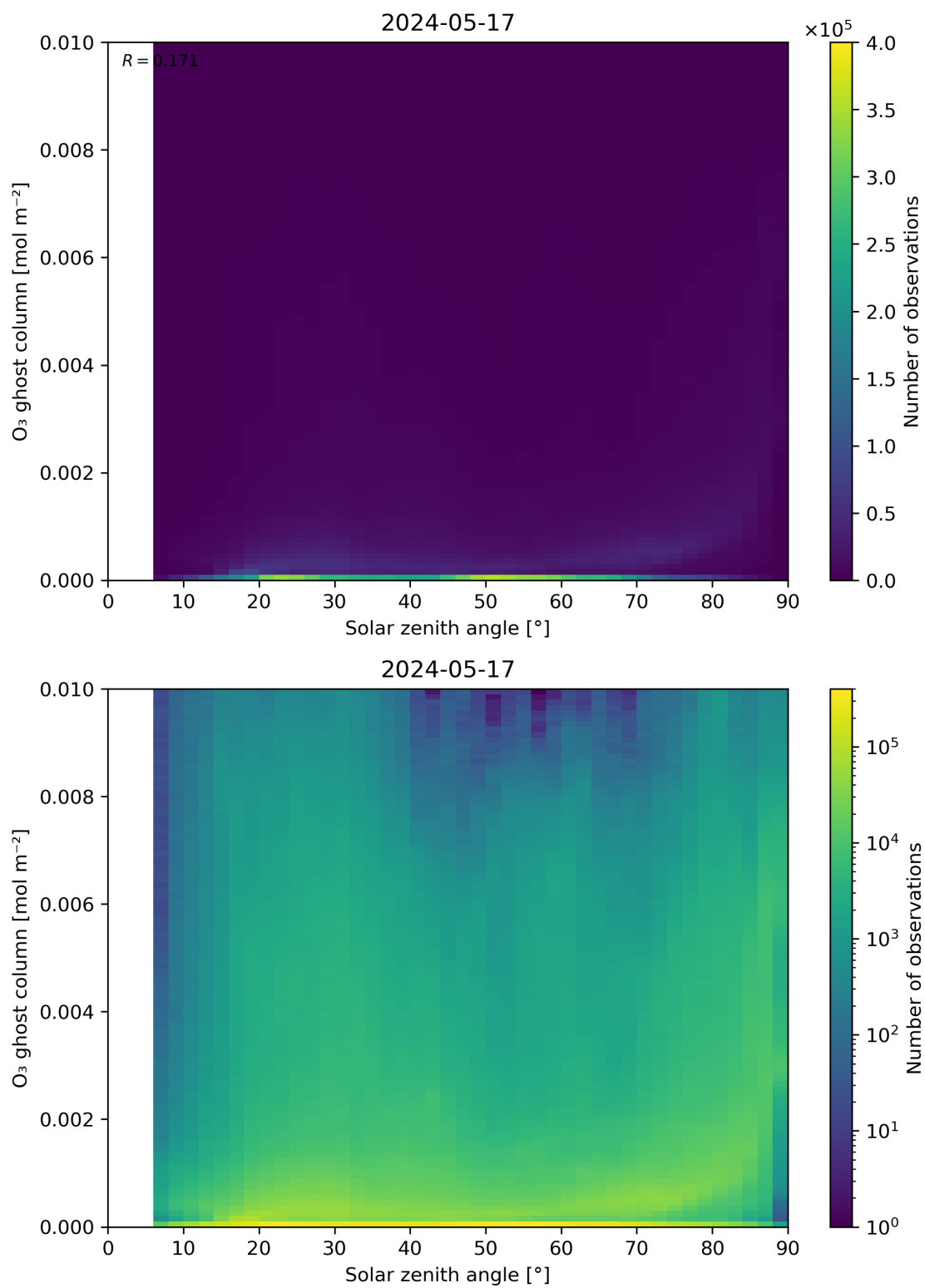
Figure 46: Scatter density plot of “Solar zenith angle” against “O 3 ghost column” for 2024-05-16 to 2024-05-18.
