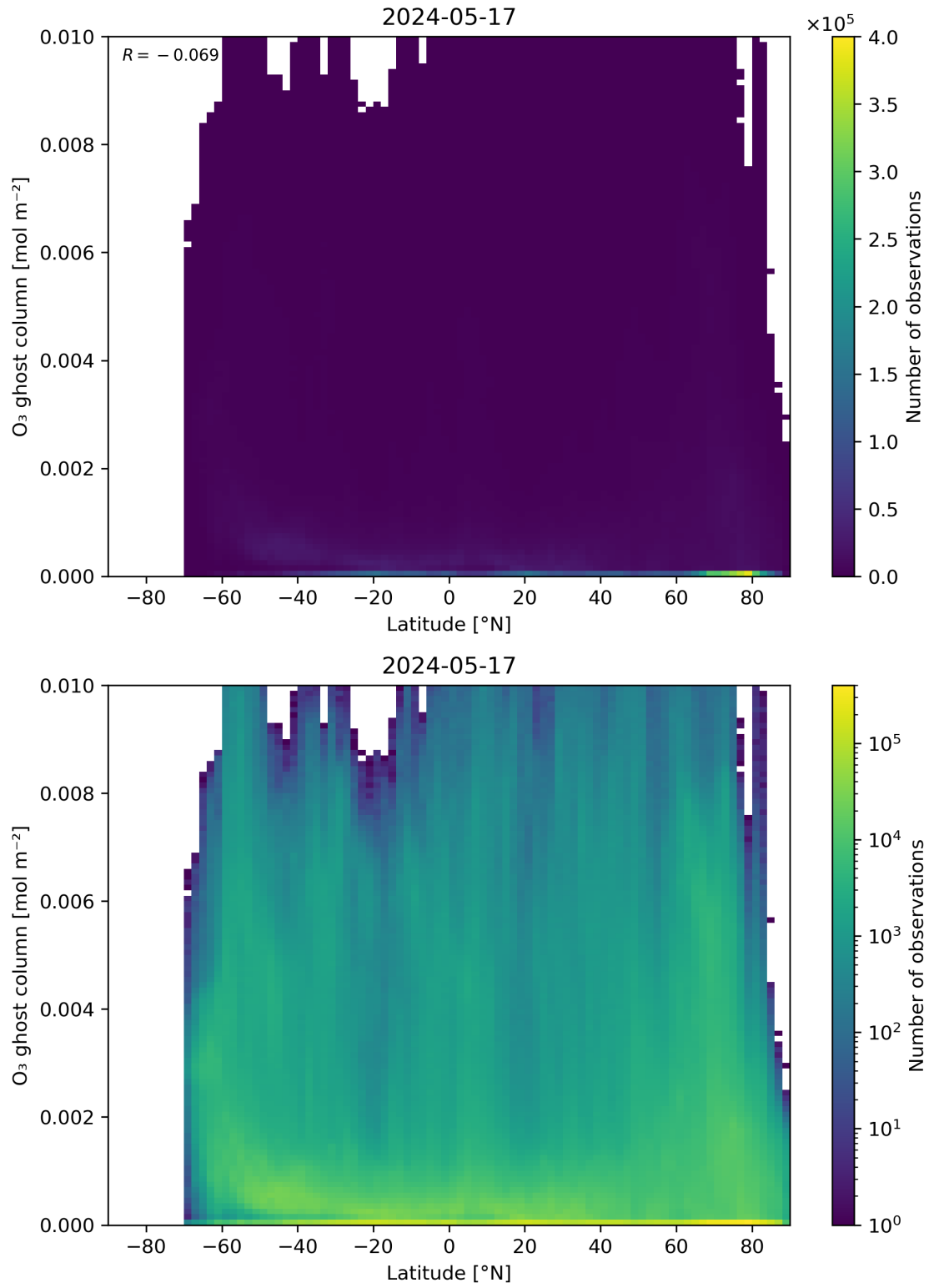
Figure 35: Scatter density plot of “Latitude” against “O 3 ghost column” for 2024-05-16 to 2024-05-18.
