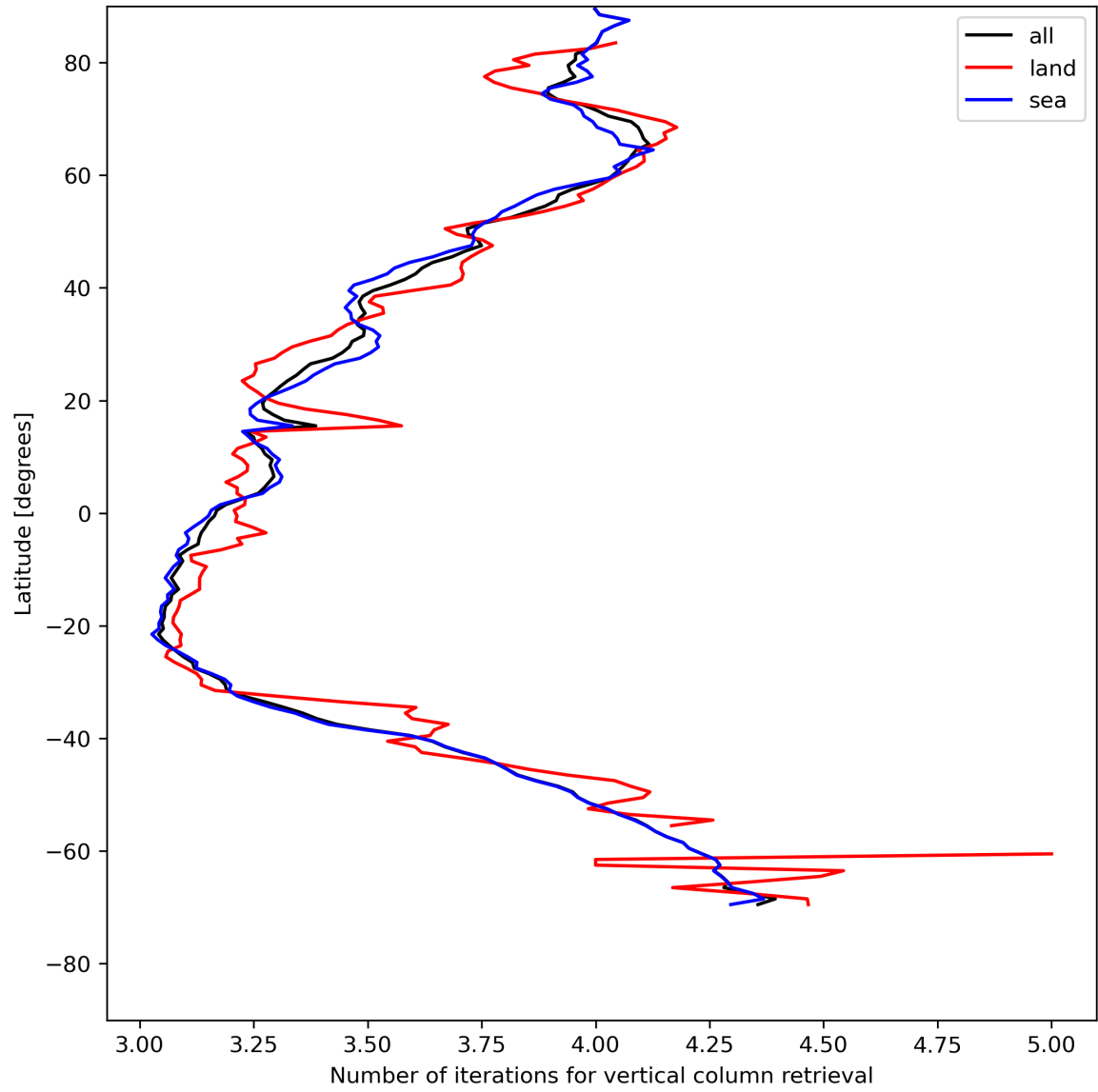
Figure 19: Zonal average of “Number of iterations for vertical column retrieval” for 2024-05-16 to 2024-05-18.
