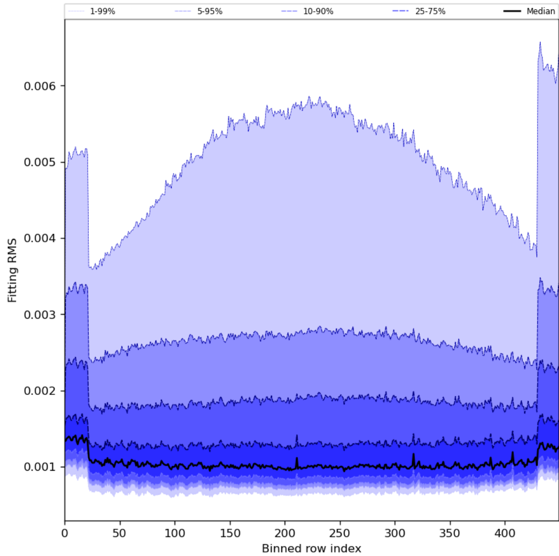
Figure 30: Along track statistics of “Fitting RMS” for 2024-05-16 to 2024-05-18
