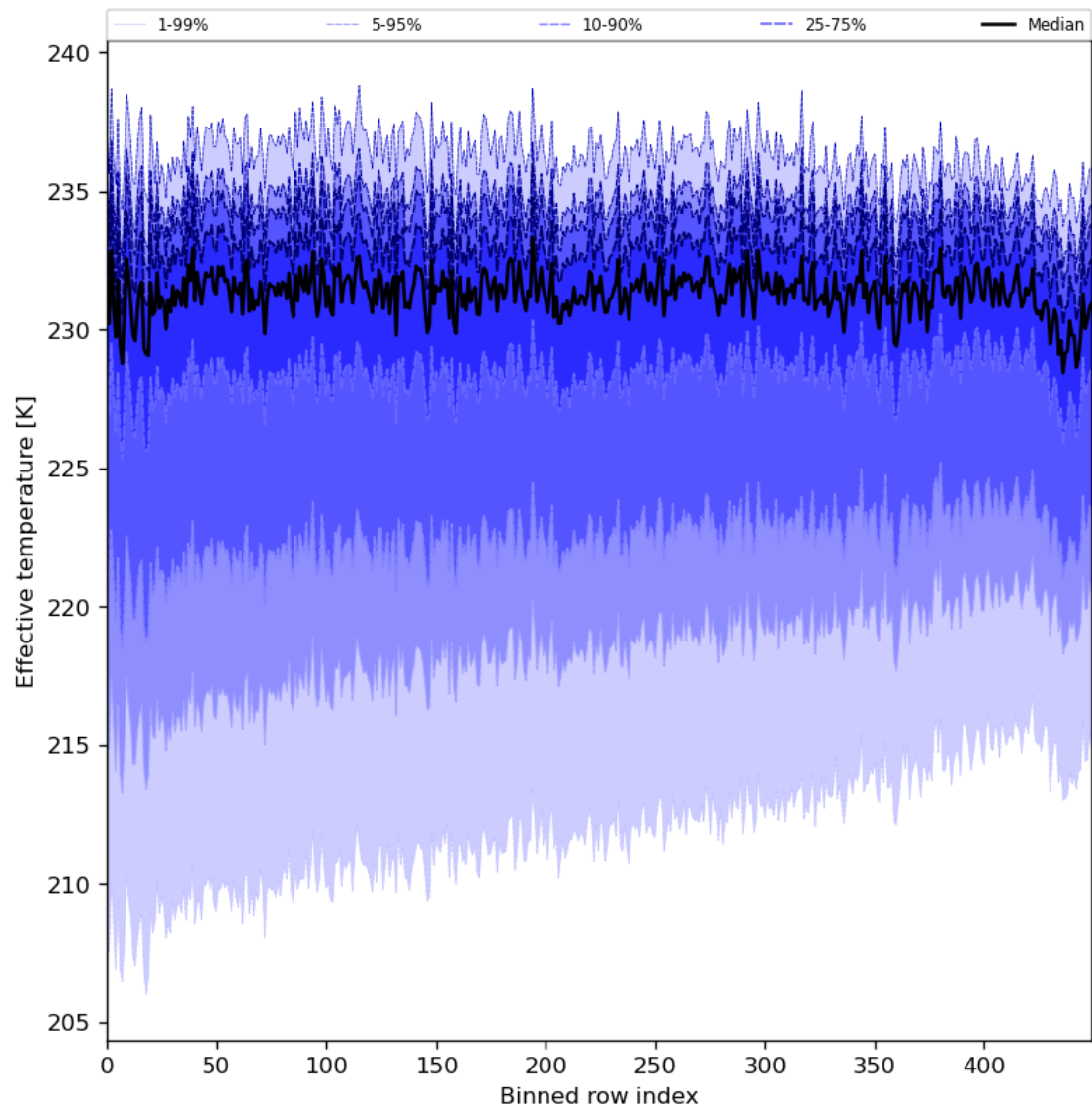
Figure 31: Along track statistics of “Effective temperature” for 2024-05-16 to 2024-05-18
