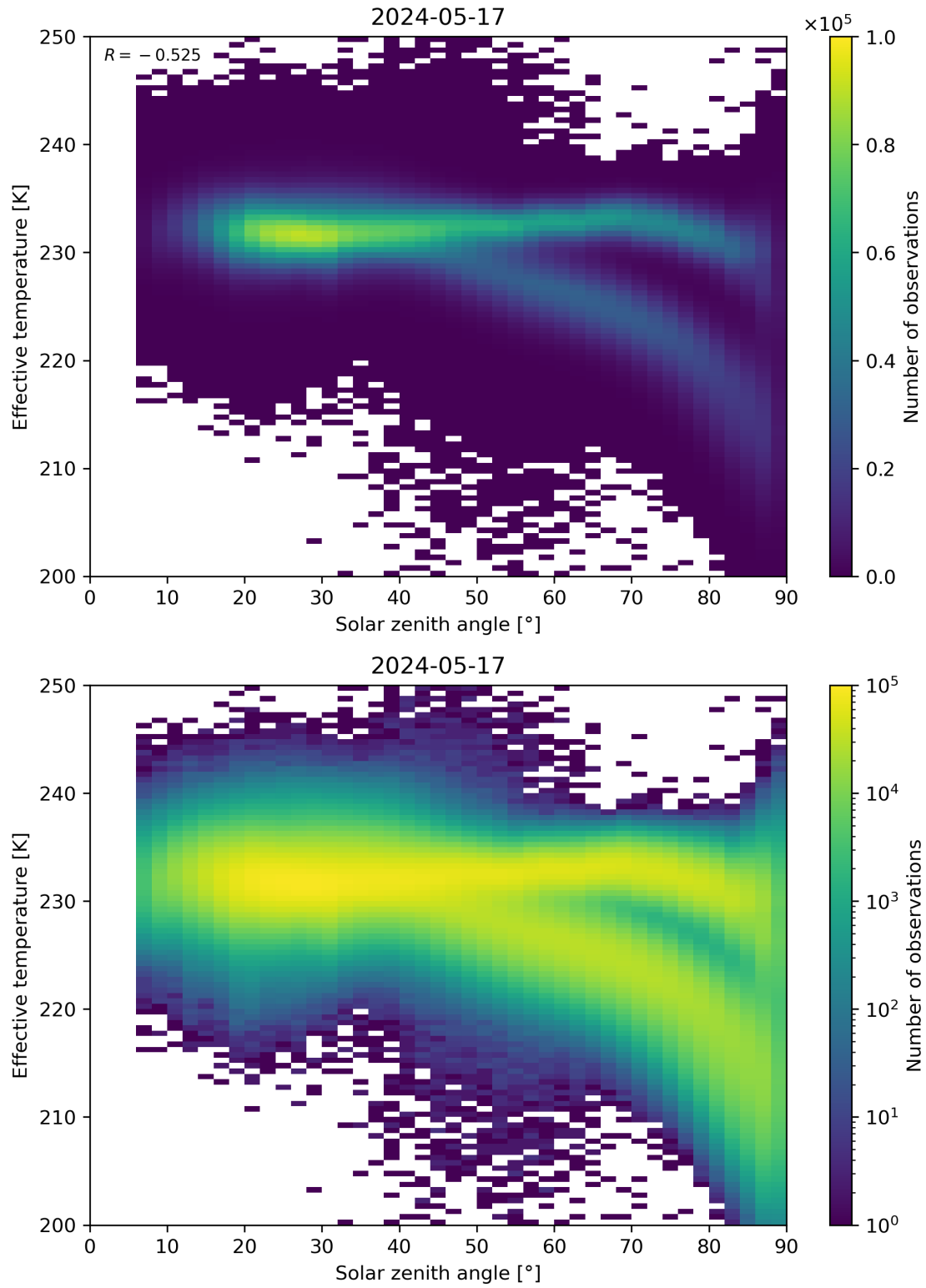
Figure 45: Scatter density plot of “Solar zenith angle” against “Effective temperature” for 2024-05-16 to 2024-05-18.
