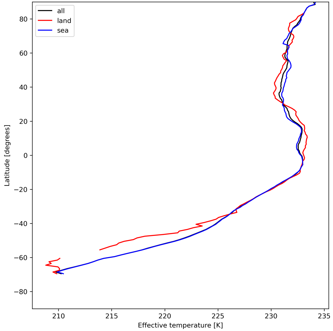
Figure 17: Zonal average of "Effective temperature" for 2024-05-16 to 2024-05-18.
