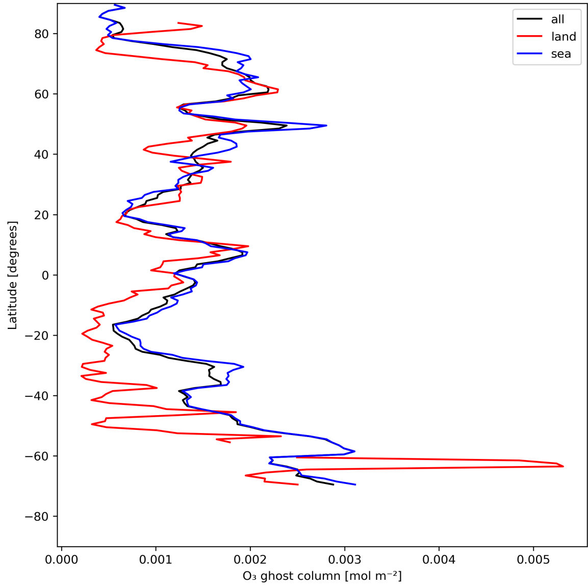
Figure 18: Zonal average of “O 3 ghost column” for 2024-05-16 to 2024-05-18.
