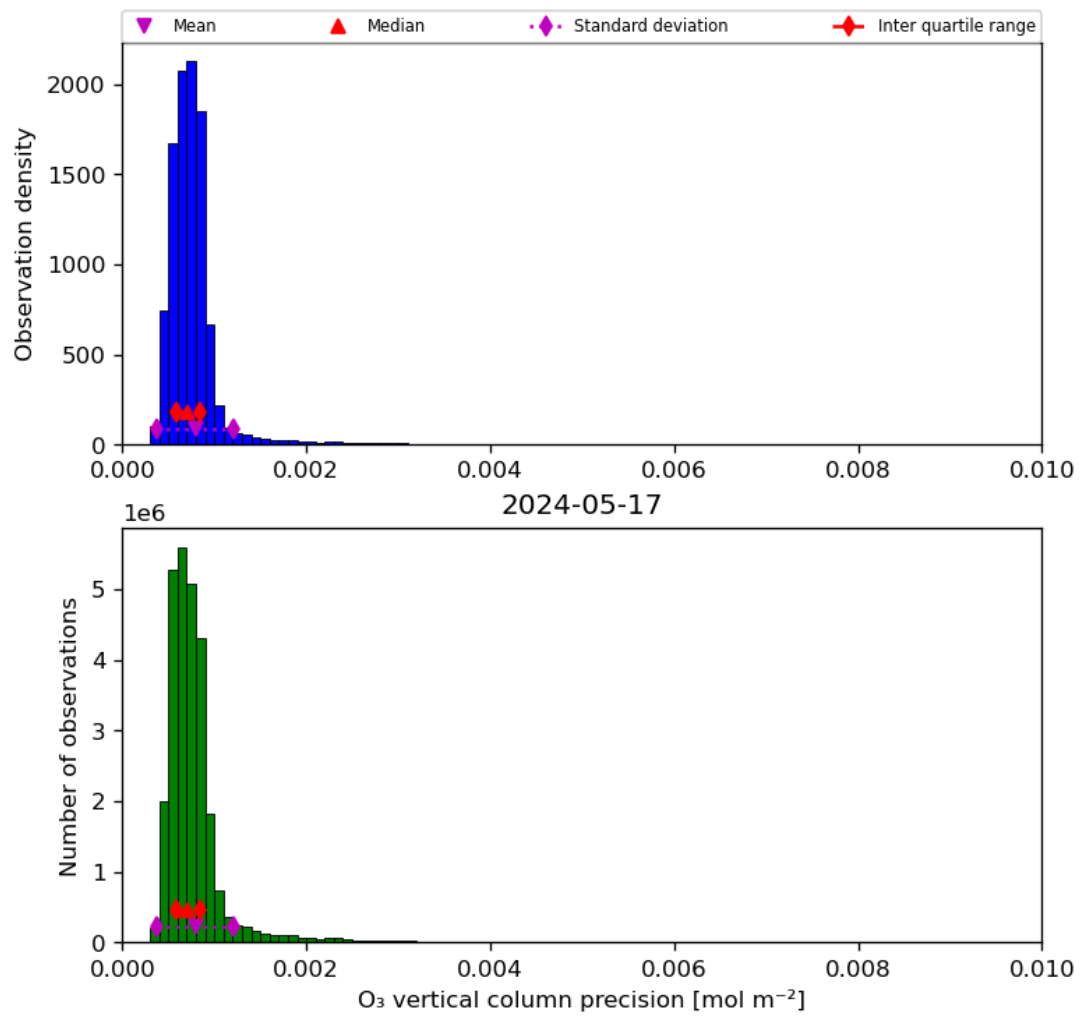
Figure 22: Histogram of “O 3 vertical column precision” for 2024-05-16 to 2024-05-18
