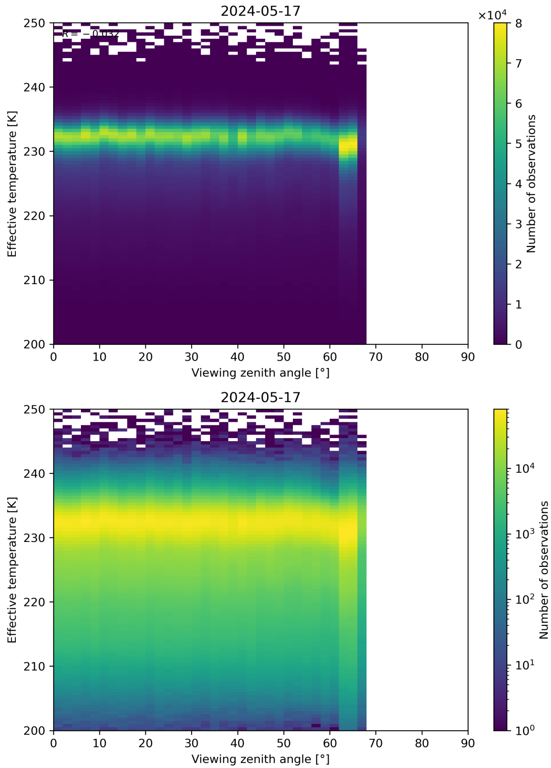
Figure 50: Scatter density plot of “Viewing zenith angle” against “Effective temperature” for 2024-05-16 to 2024-05-18.
