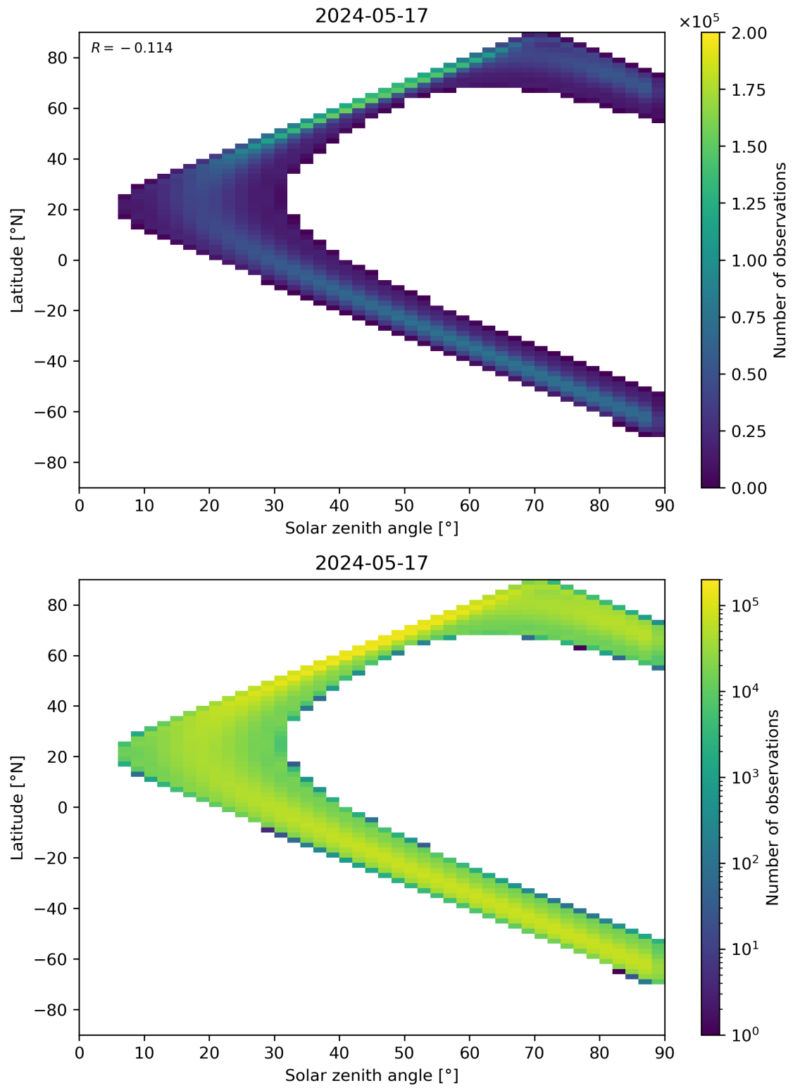
Figure 44: Scatter density plot of “Solar zenith angle” against “Latitude” for 2024-05-16 to 2024-05-18.
