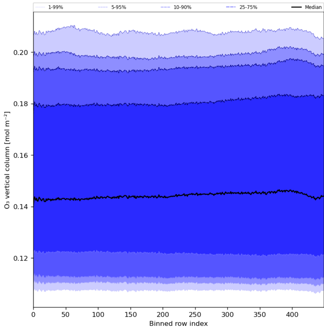
Figure 28: Along track statistics of “O 3 vertical column” for 2024-05-16 to 2024-05-18
