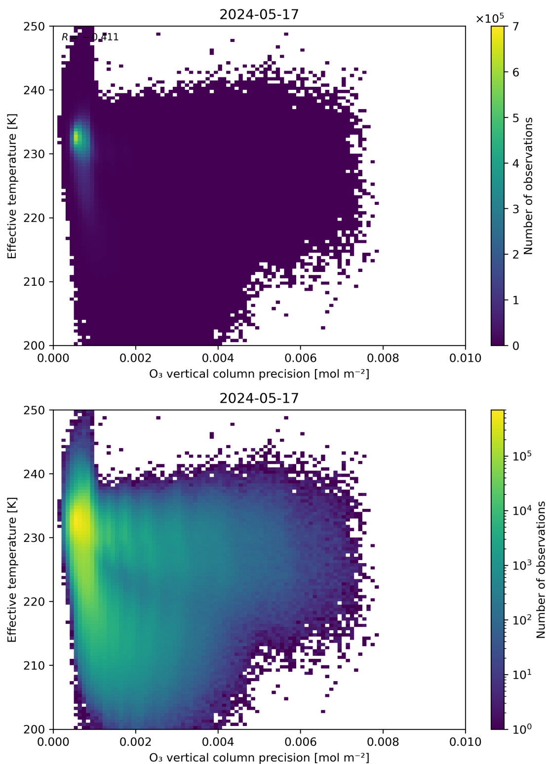
Figure 42: Scatter density plot of “O 3 vertical column precision” against “Effective temperature” for 2024-05-16 to 2024-05-18.
