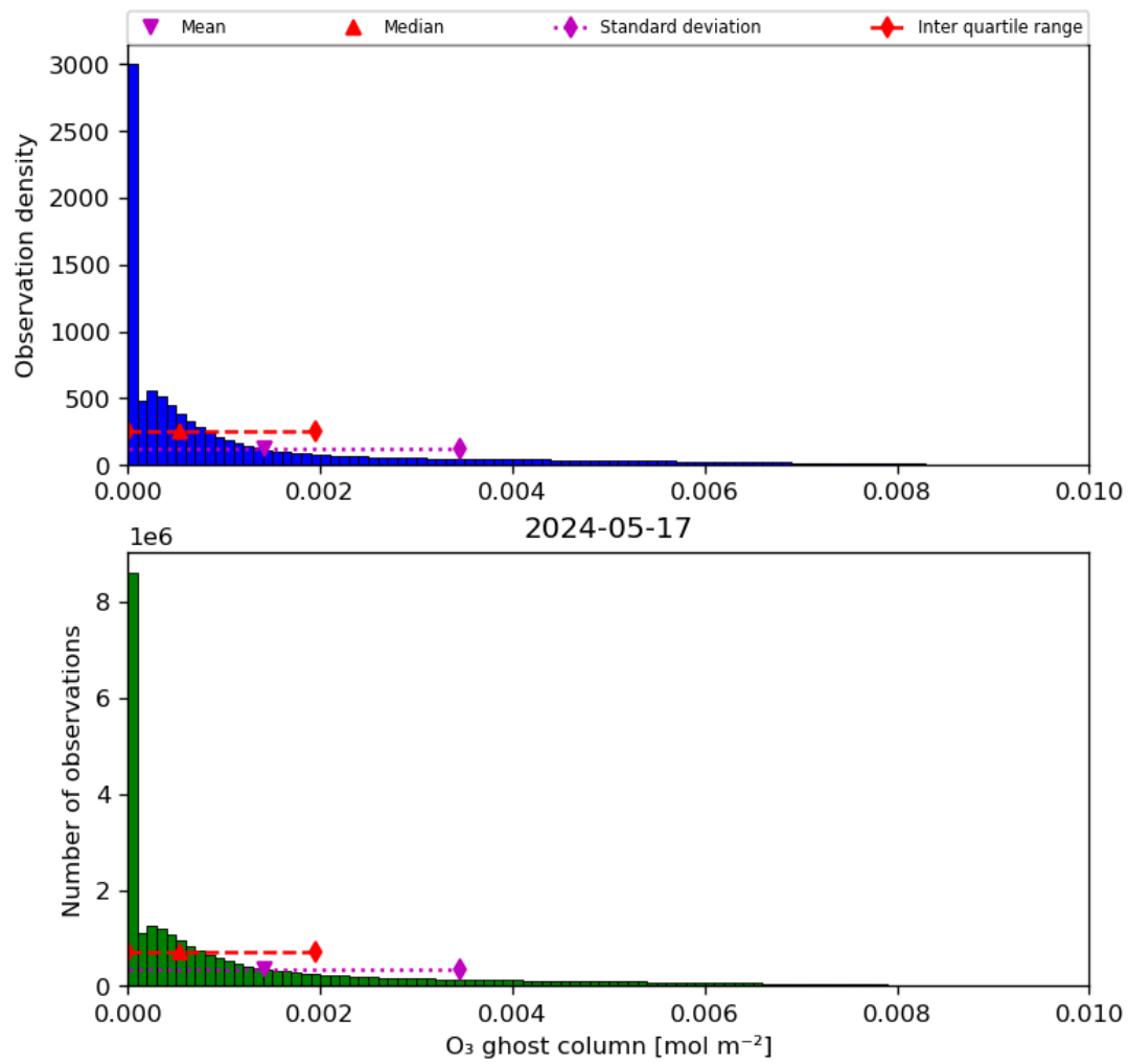
Figure 25: Histogram of “O 3 ghost column” for 2024-05-16 to 2024-05-18
