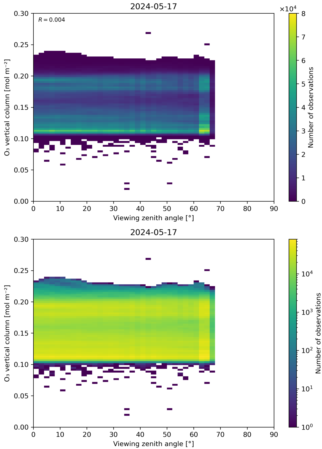
Figure 52: Scatter density plot of “Viewing zenith angle” against “O 3 vertical column” for 2024-05-16 to 2024-05-18.
