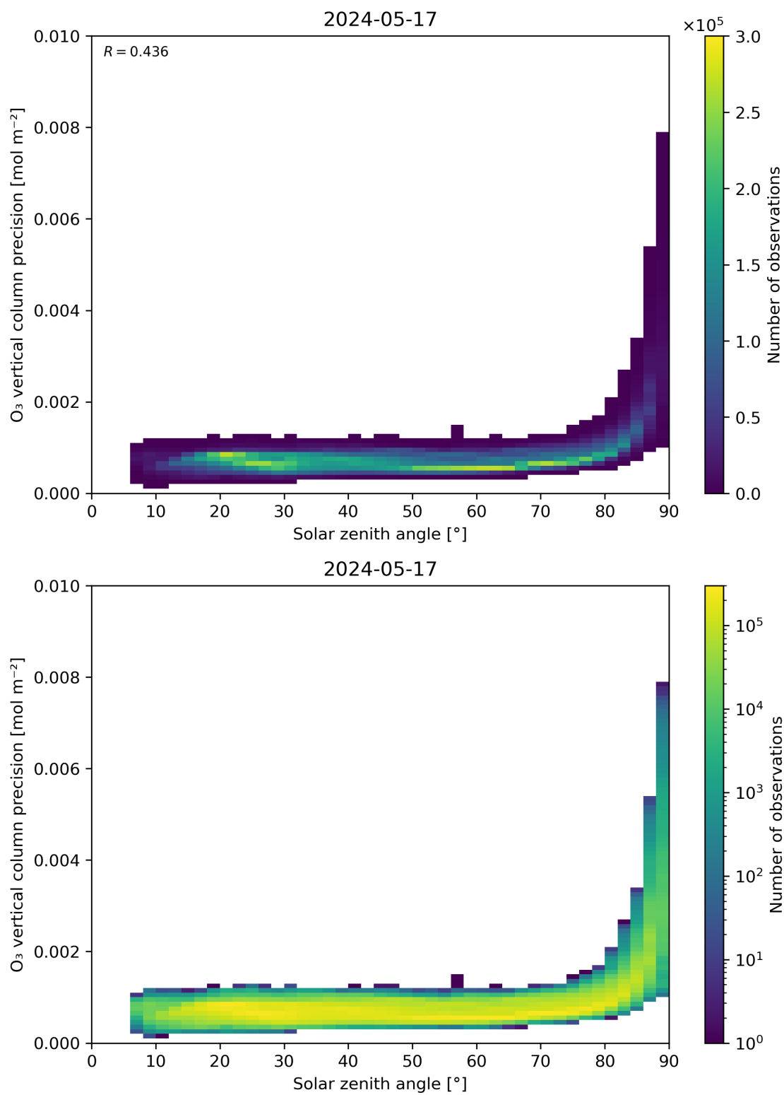
Figure 48: Scatter density plot of “Solar zenith angle” against “O 3 vertical column precision” for 2024-05-16 to 2024-05-18.
