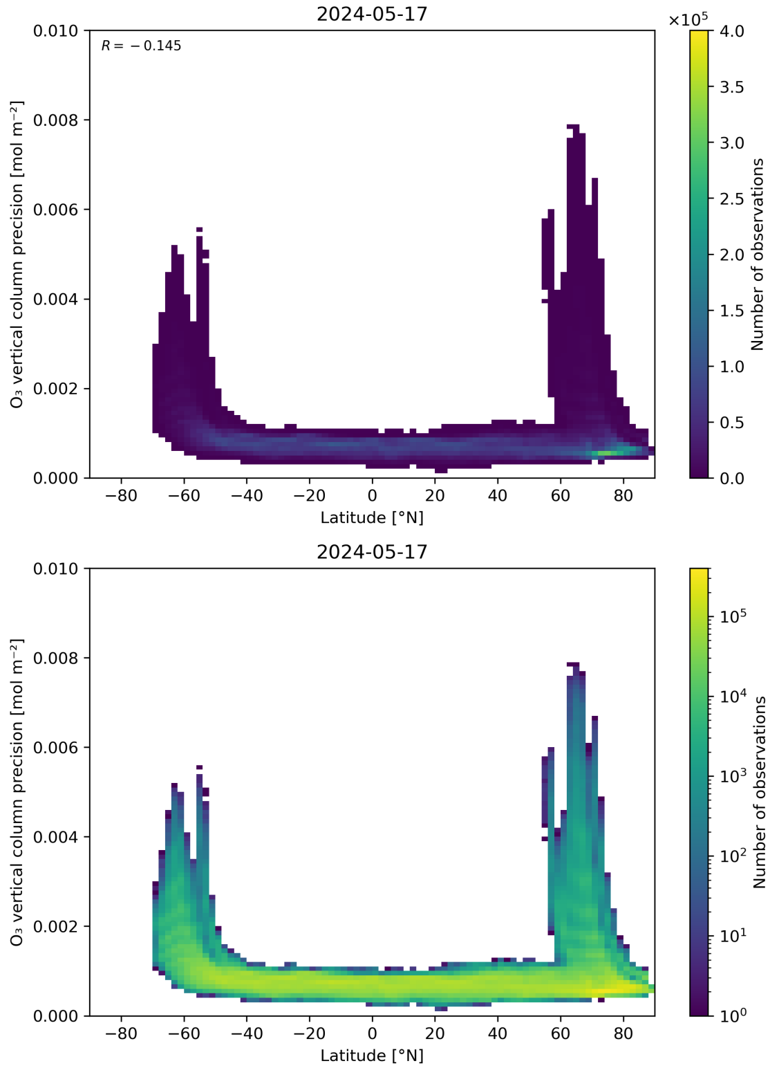
Figure 37: Scatter density plot of “Latitude” against “O 3 vertical column precision” for 2024-05-16 to 2024-05-18.
