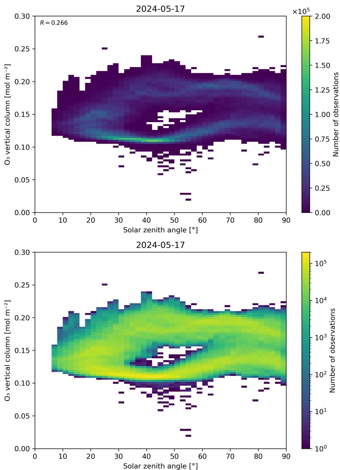
Figure 47: Scatter density plot of “Solar zenith angle” against “O 3 vertical column” for 2024-05-16 to 2024-05-18.
