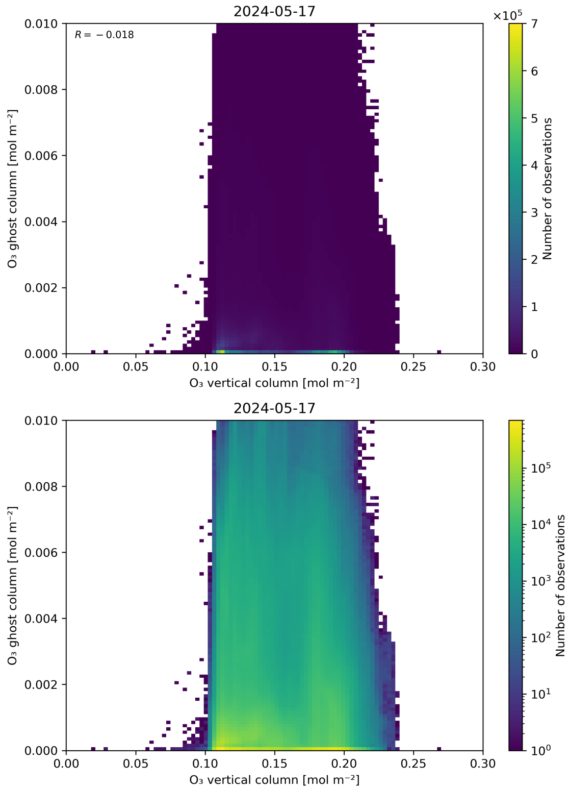
Figure 40: Scatter density plot of “O 3 vertical column” against “O 3 ghost column” for 2024-05-16 to 2024-05-18.
