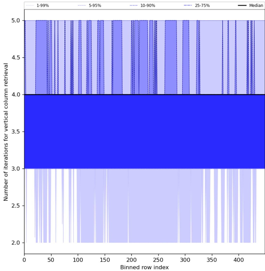
Figure 33: Along track statistics of “Number of iterations for vertical column retrieval” for 2024-05-16 to 2024-05-18
