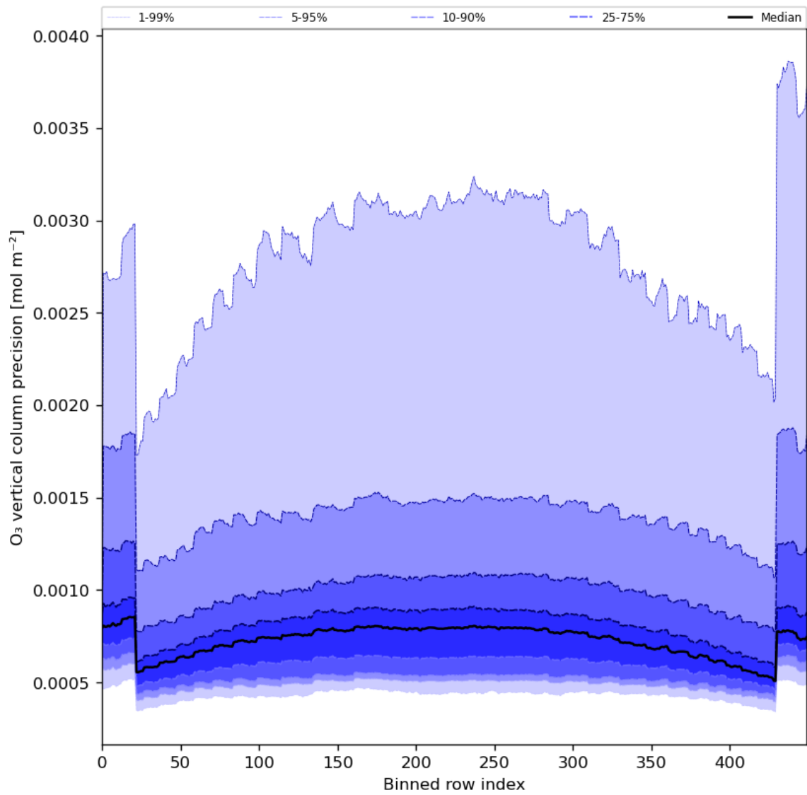
Figure 29: Along track statistics of “O 3 vertical column precision” for 2024-05-18 to 2024-05-19
