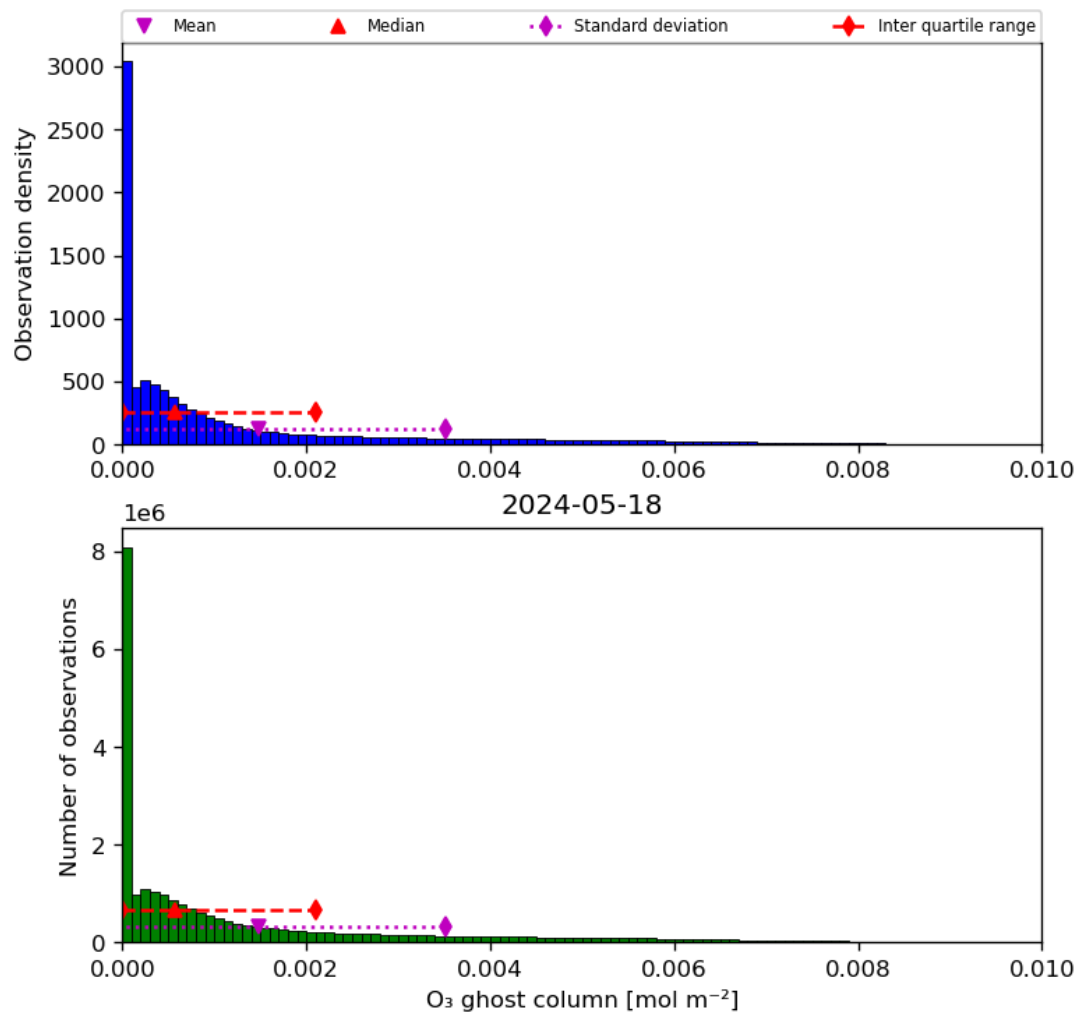
Figure 25: Histogram of “O 3 ghost column” for 2024-05-18 to 2024-05-19
