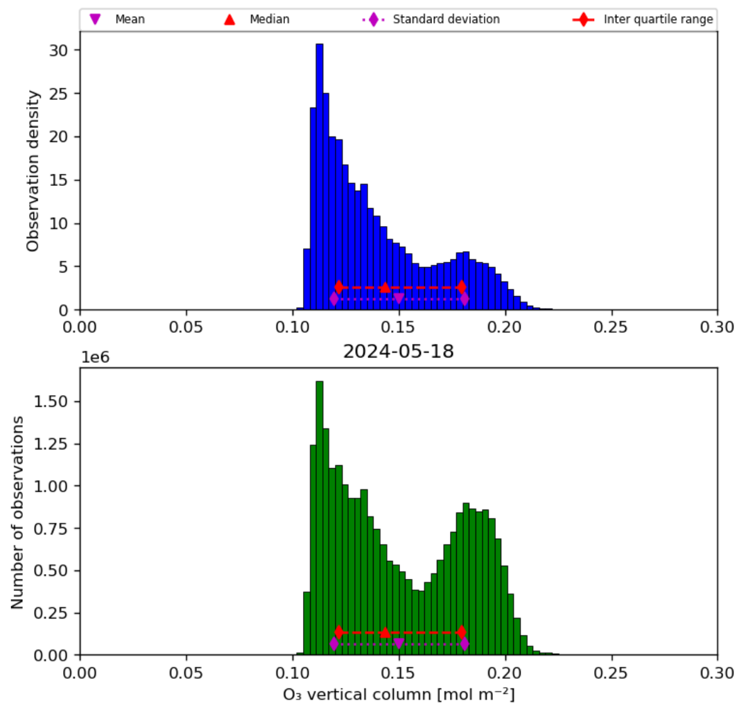
Figure 21: Histogram of “O 3 vertical column” for 2024-05-18 to 2024-05-19
