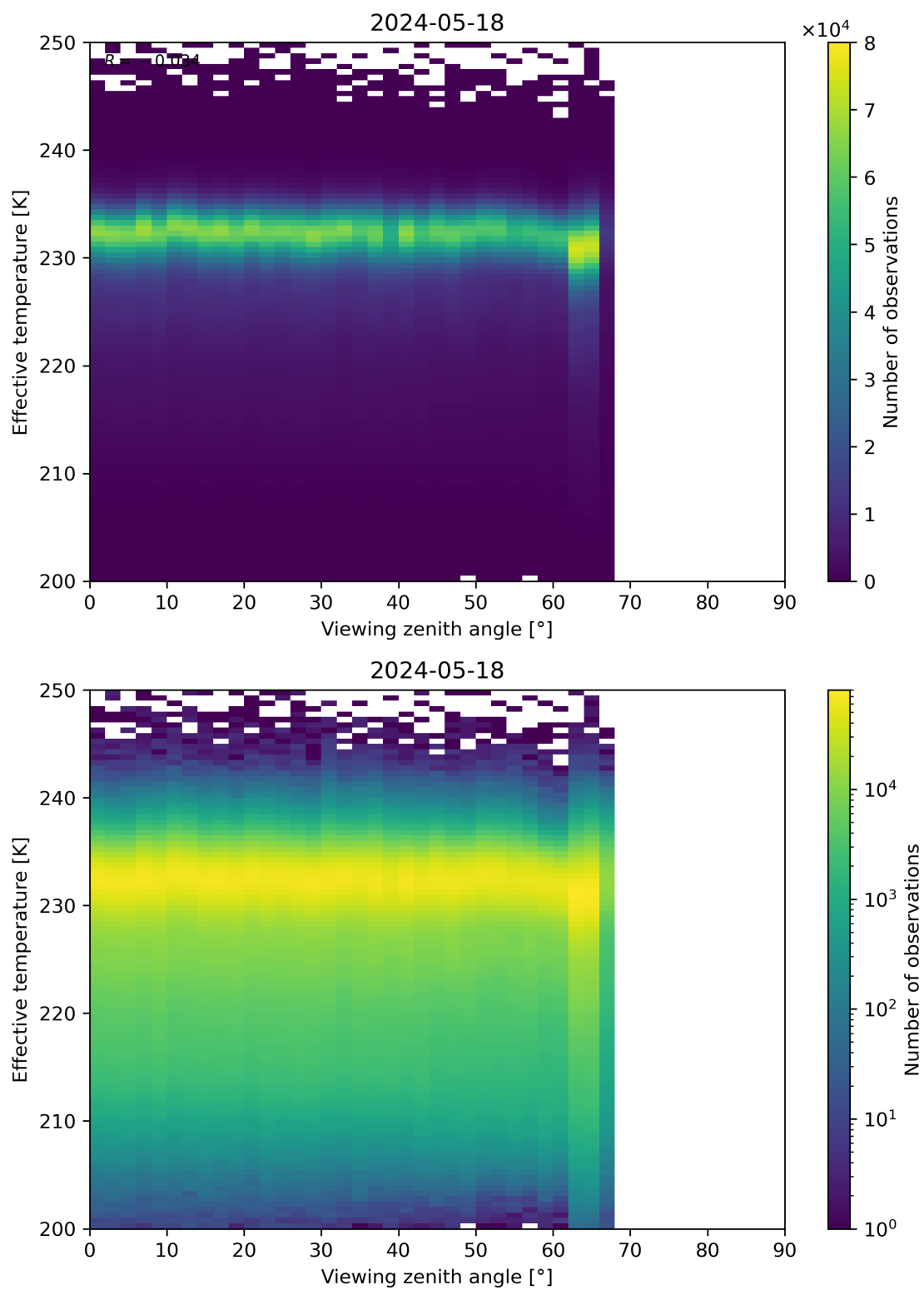
Figure 50: Scatter density plot of “Viewing zenith angle” against “Effective temperature” for 2024-05-18 to 2024-05-19.
