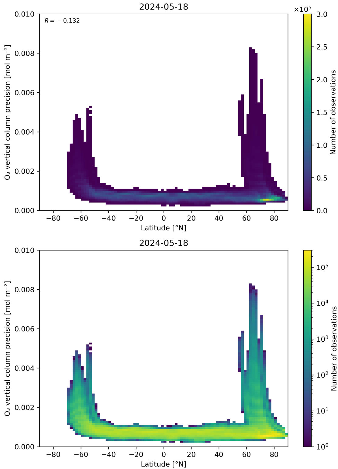
Figure 37: Scatter density plot of “Latitude” against “O 3 vertical column precision” for 2024-05-18 to 2024-05-19.
