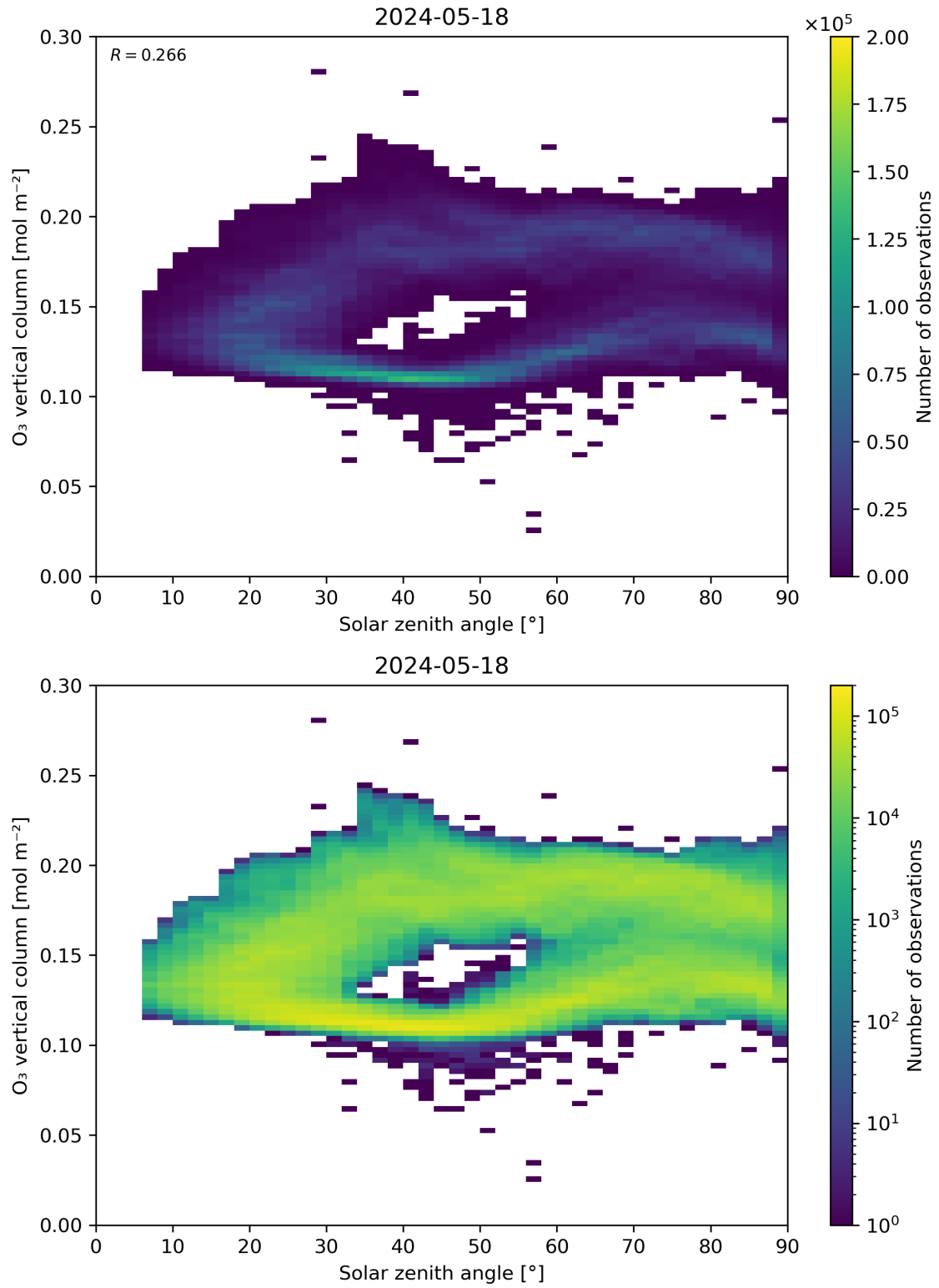
Figure 47: Scatter density plot of “Solar zenith angle” against “O 3 vertical column” for 2024-05-18 to 2024-05-19.
