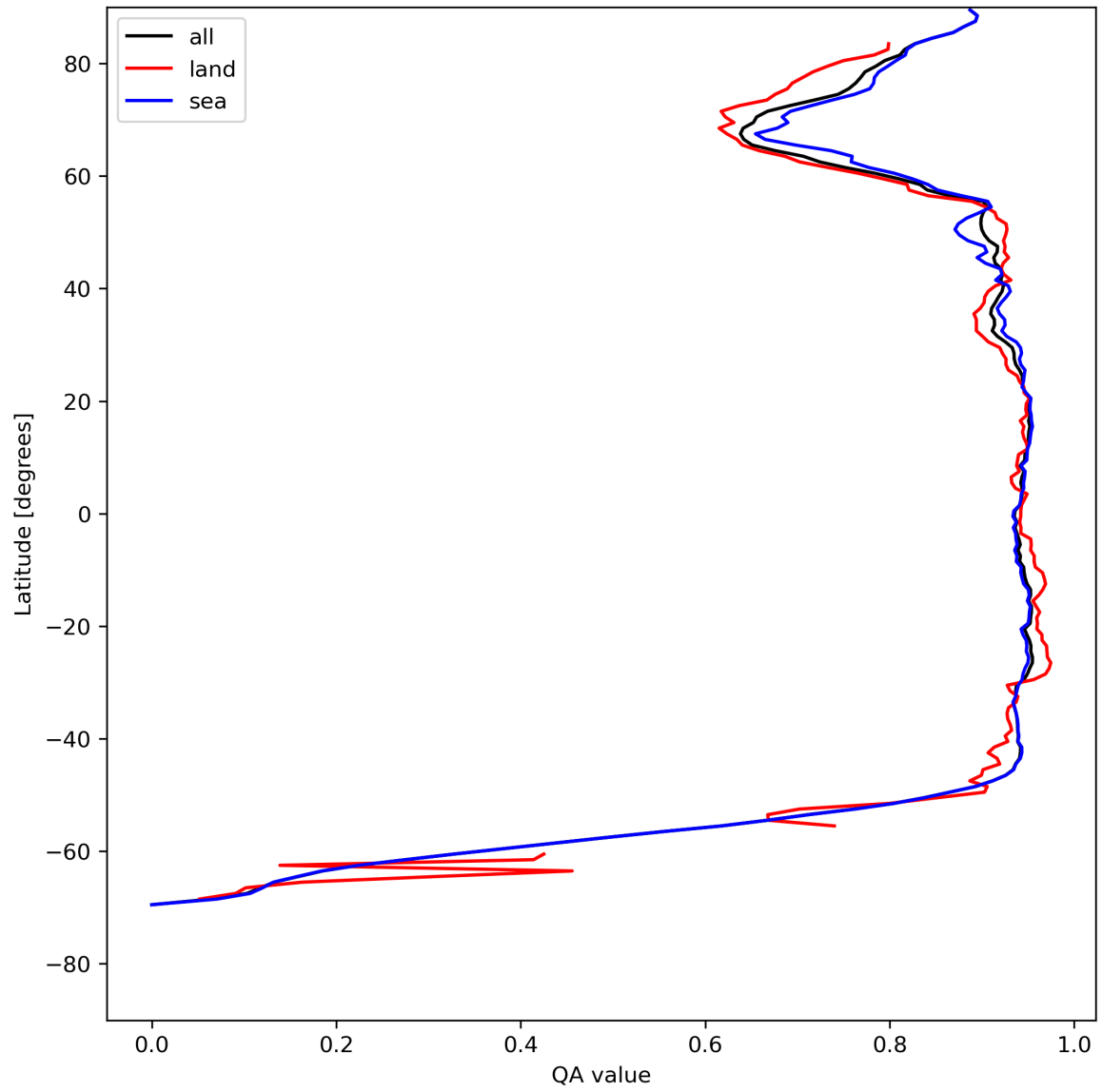
Figure 13: Zonal average of “QA value” for 2024-05-18 to 2024-05-19.
