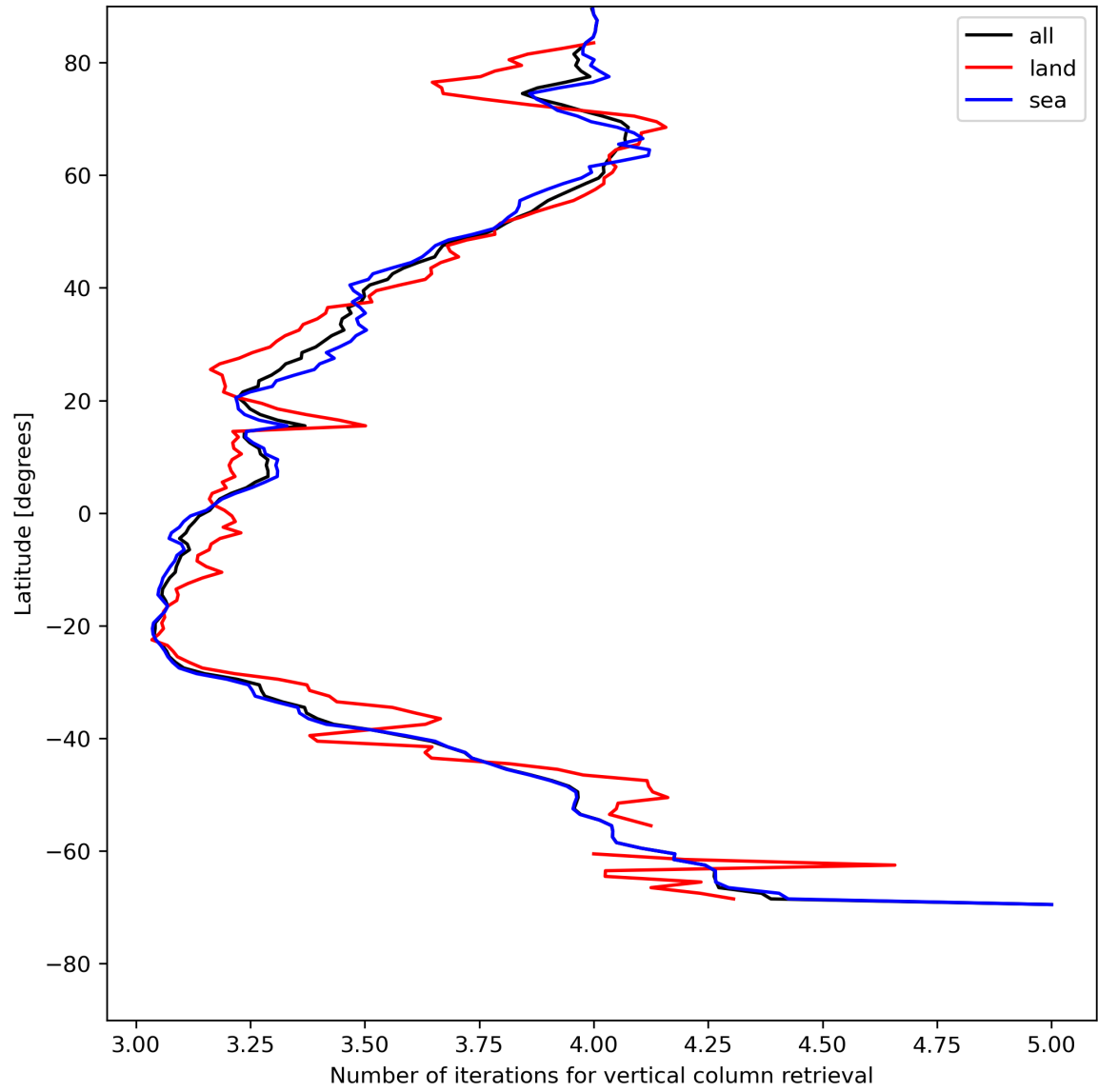
Figure 19: Zonal average of “Number of iterations for vertical column retrieval” for 2024-05-18 to 2024-05-19.
