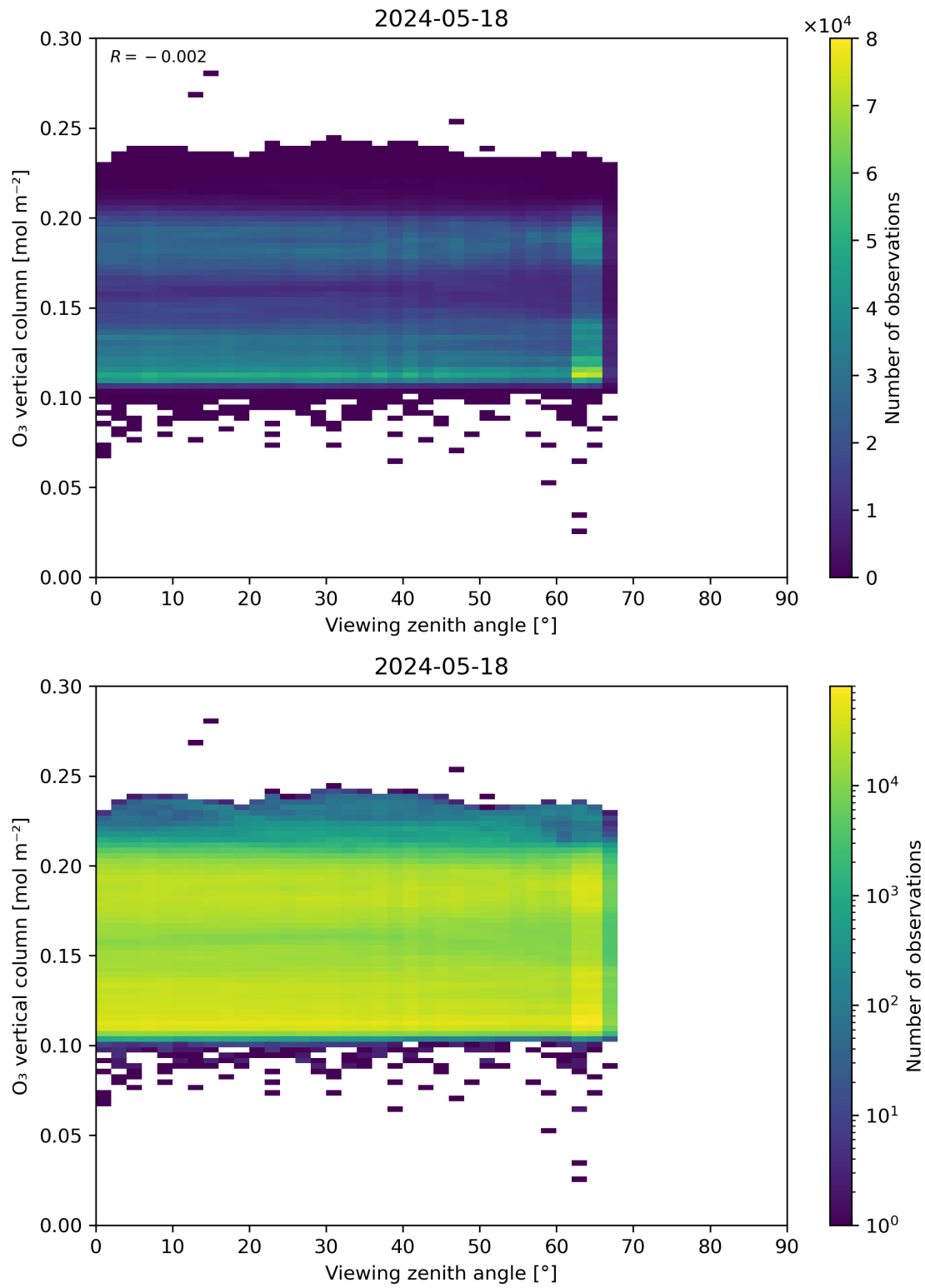
Figure 52: Scatter density plot of “Viewing zenith angle” against “O 3 vertical column” for 2024-05-18 to 2024-05-19.
