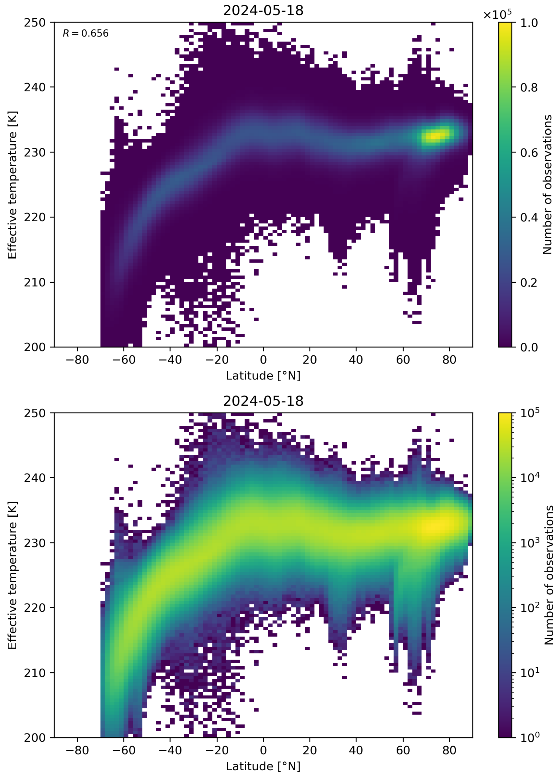
Figure 34: Scatter density plot of “Latitude” against “Effective temperature” for 2024-05-18 to 2024-05-19.
