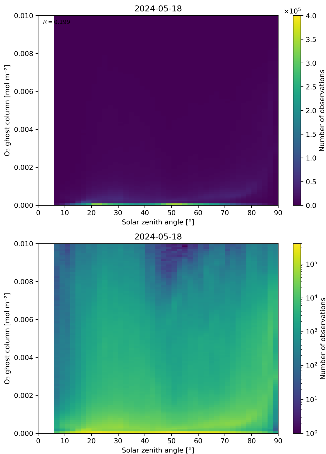
Figure 46: Scatter density plot of “Solar zenith angle” against “O 3 ghost column” for 2024-05-18 to 2024-05-19.
