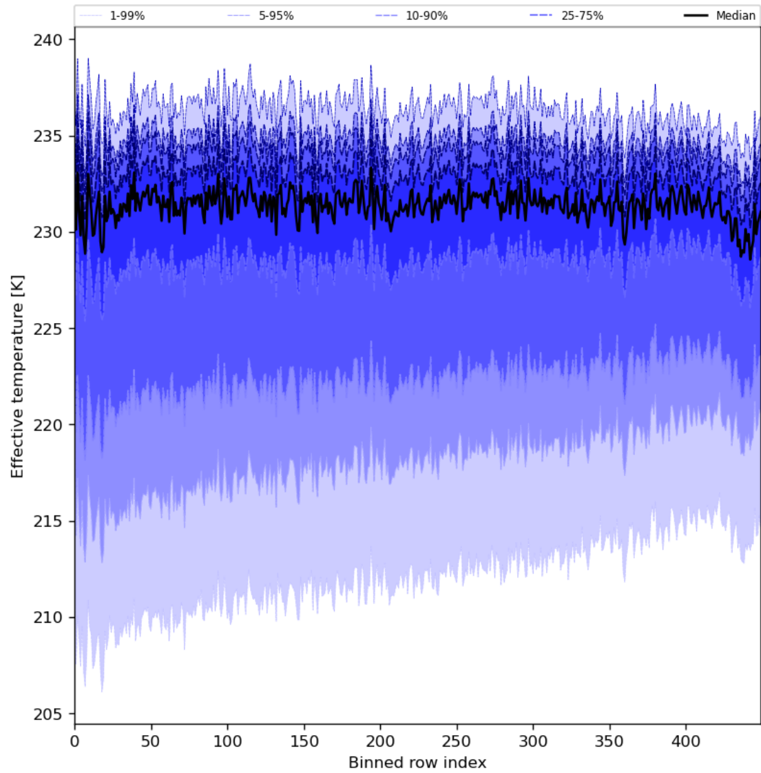
Figure 31: Along track statistics of “Effective temperature” for 2024-05-18 to 2024-05-19
