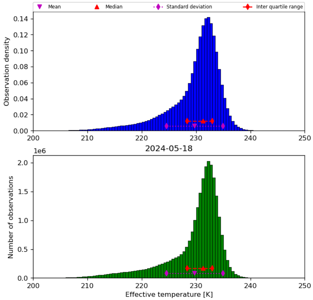
Figure 24: Histogram of “Effective temperature” for 2024-05-18 to 2024-05-19
