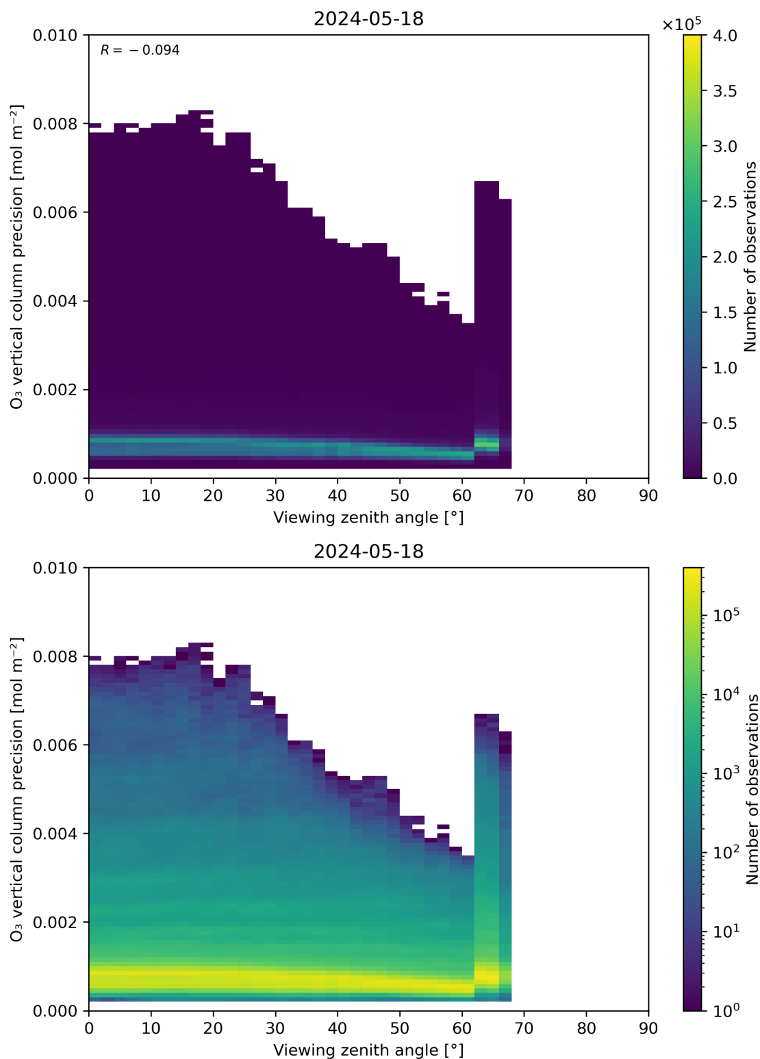
Figure 53: Scatter density plot of “Viewing zenith angle” against “O 3 vertical column precision” for 2024-05-18 to 2024-05-19.
