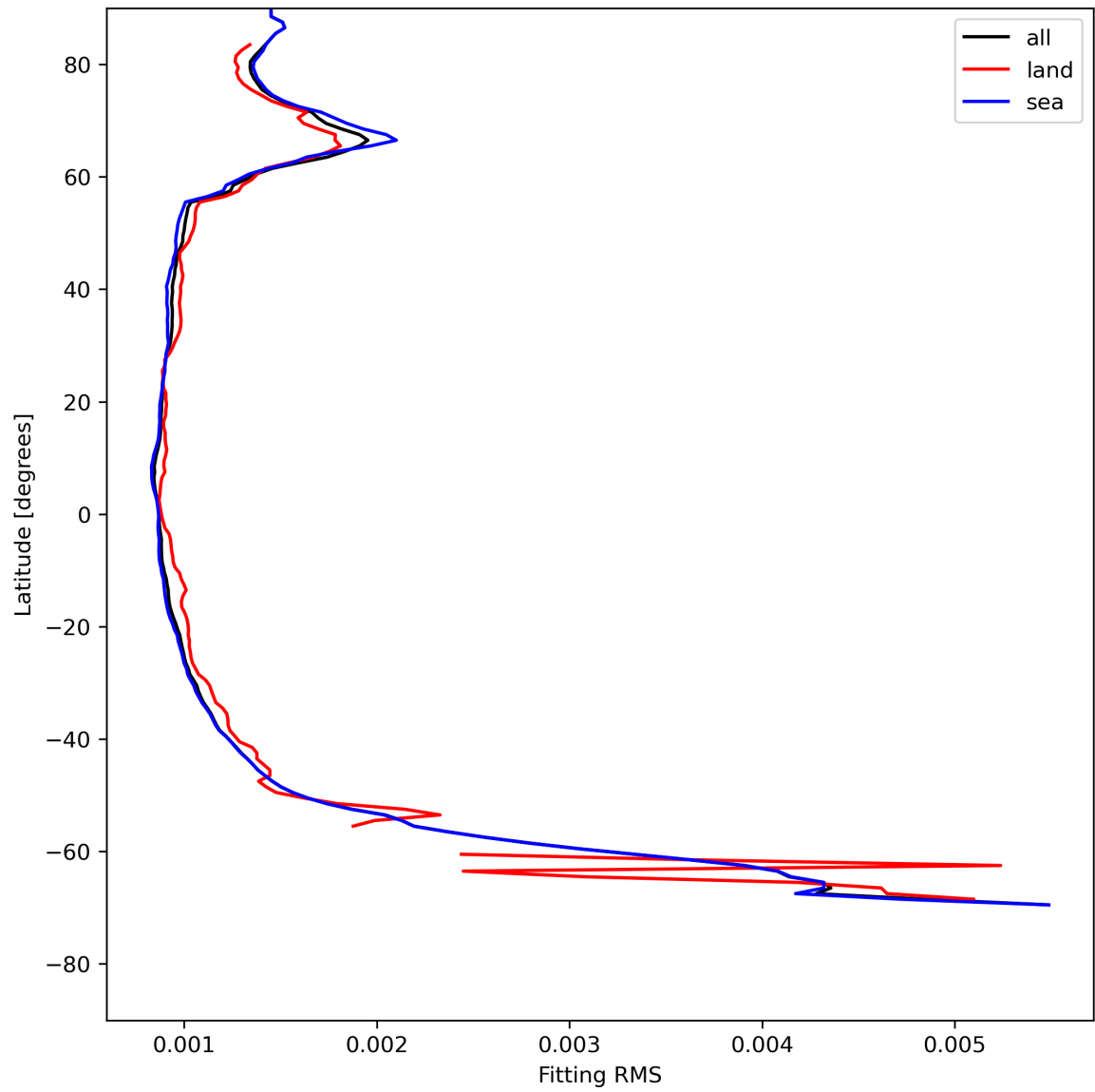
Figure 16: Zonal average of “Fitting RMS” for 2024-05-18 to 2024-05-19.
