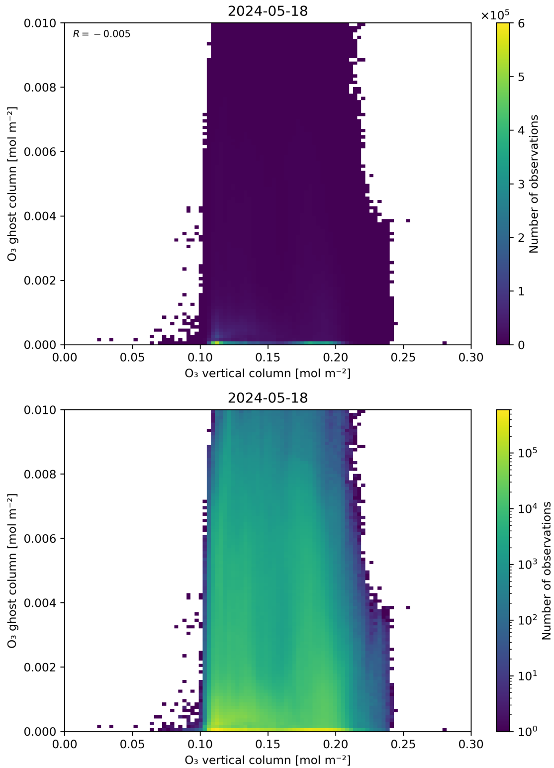
Figure 40: Scatter density plot of “O 3 vertical column” against “O 3 ghost column” for 2024-05-18 to 2024-05-19.
