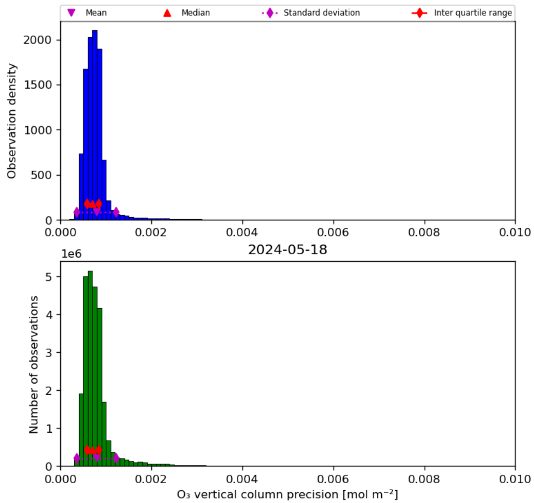
Figure 22: Histogram of “O 3 vertical column precision” for 2024-05-18 to 2024-05-19
