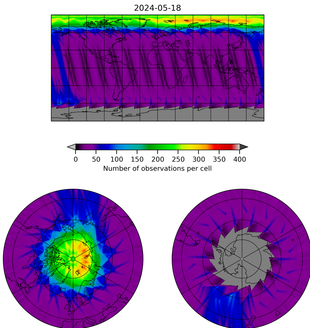
Figure 12: Map of the number of observations for 2024-05-18 to 2024-05-19
