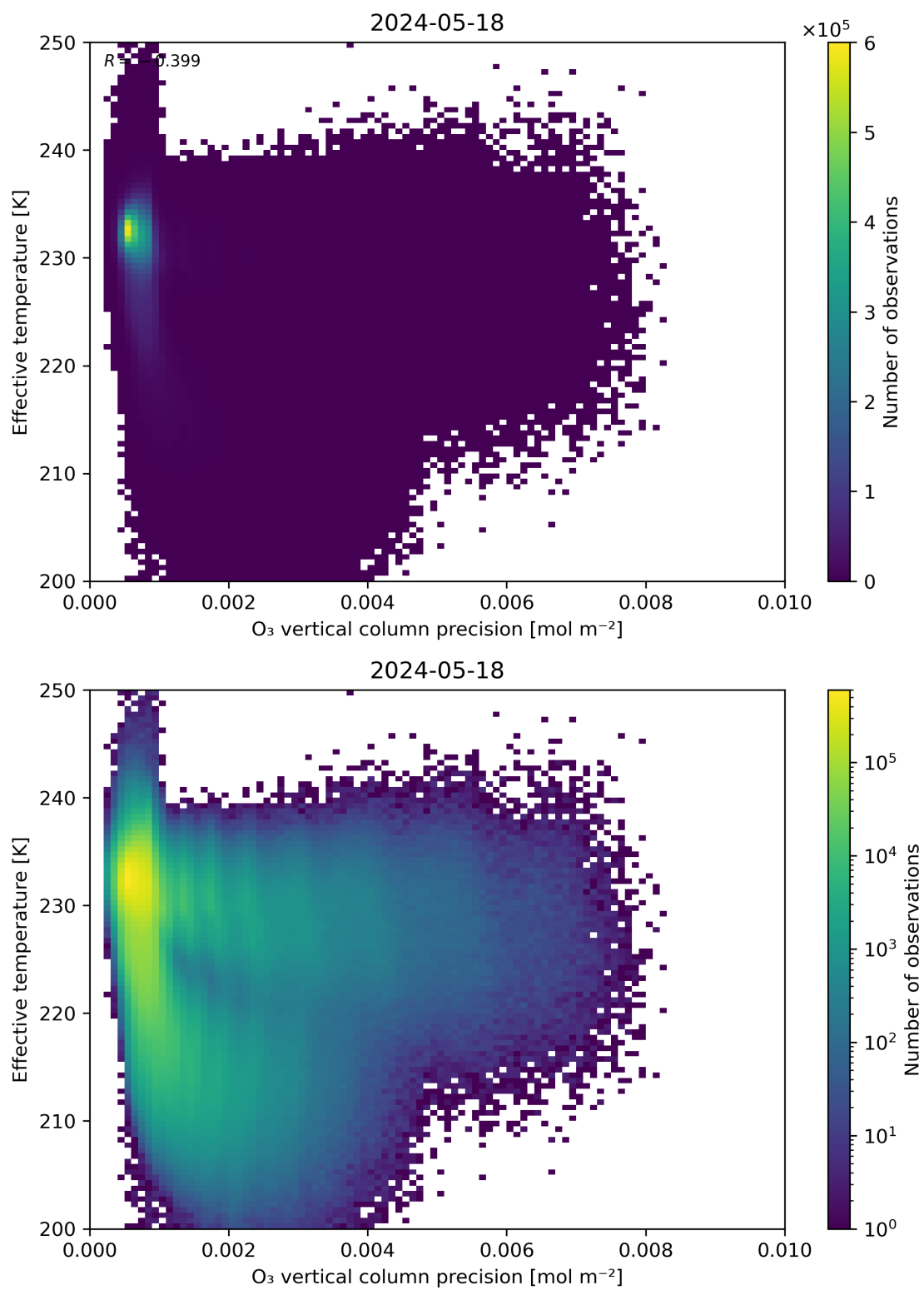
Figure 42: Scatter density plot of “O 3 vertical column precision” against “Effective temperature” for 2024-05-18 to 2024-05-19.
