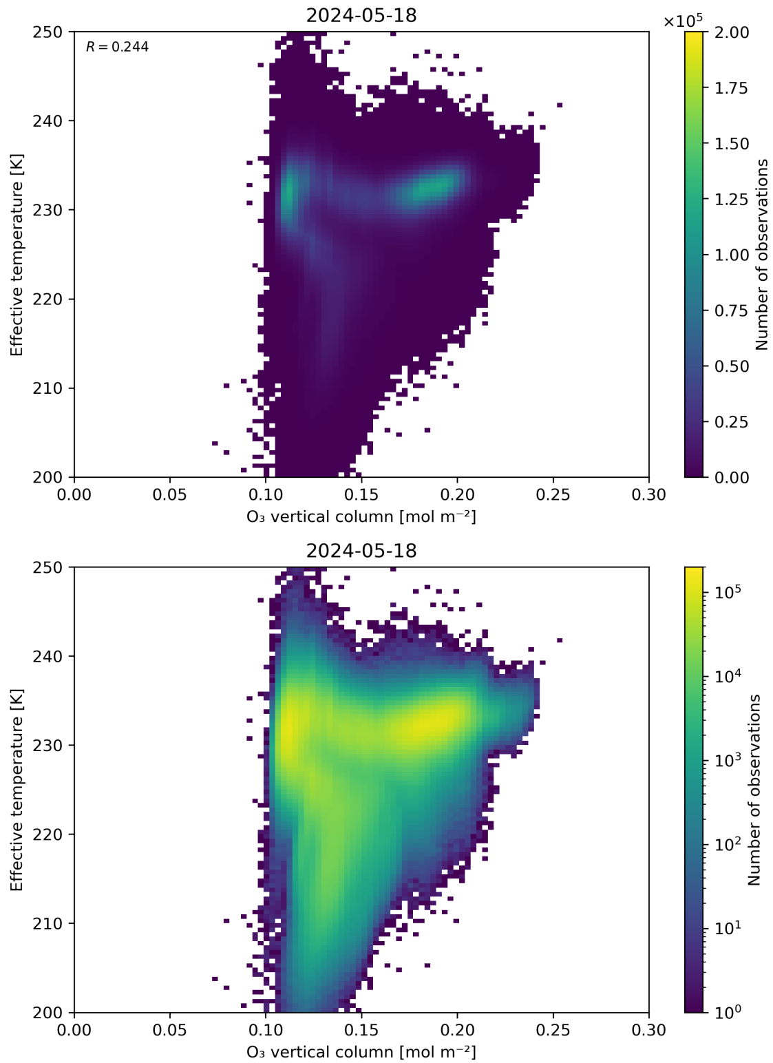
Figure 39: Scatter density plot of “O 3 vertical column” against “Effective temperature” for 2024-05-18 to 2024-05-19.
