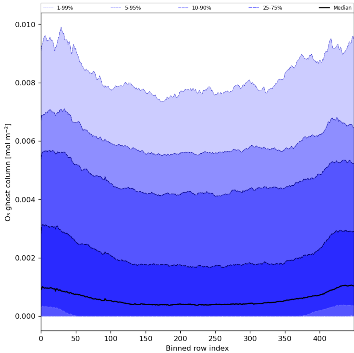
Figure 32: Along track statistics of “O 3 ghost column” for 2024-05-18 to 2024-05-19
