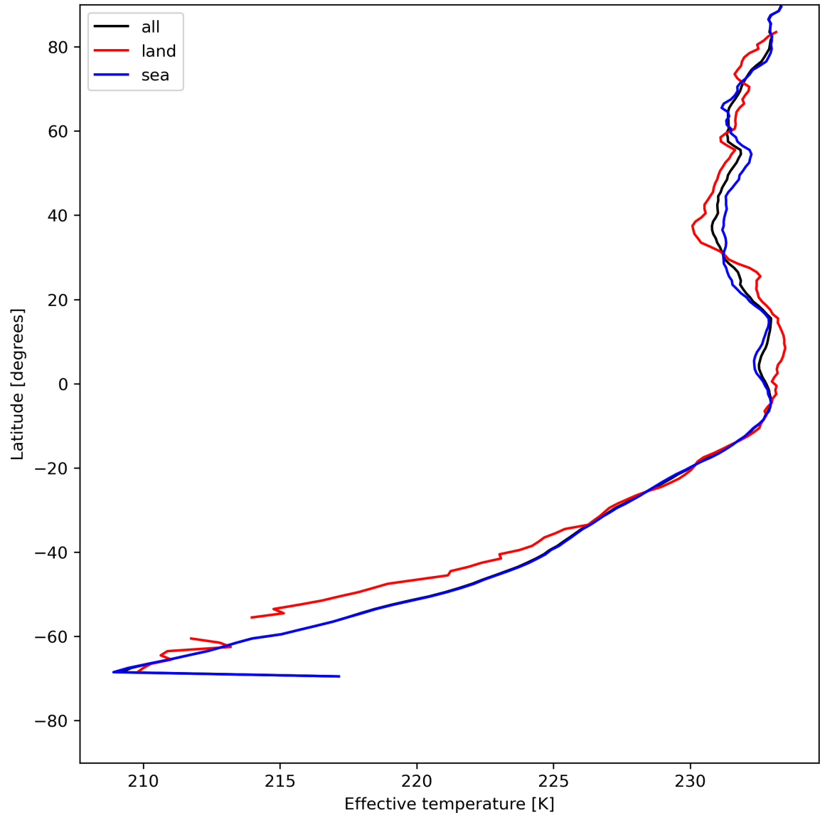
Figure 17: Zonal average of "Effective temperature" for 2024-05-18 to 2024-05-19.
