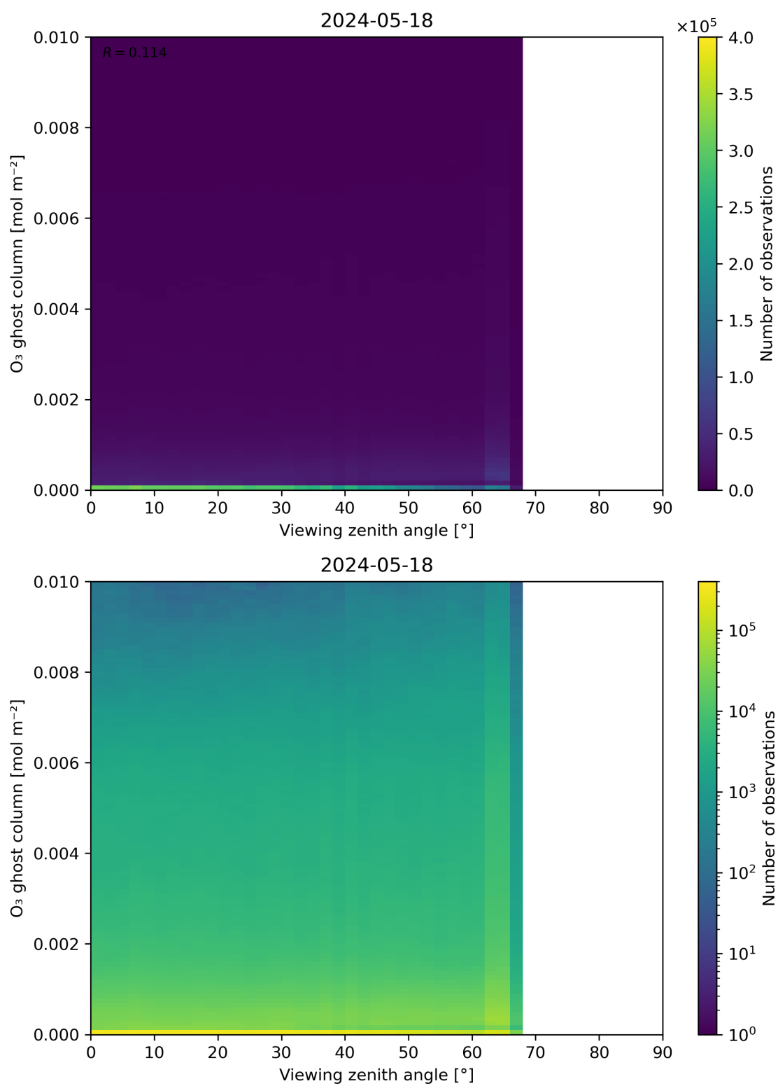
Figure 51: Scatter density plot of “Viewing zenith angle” against “O 3 ghost column” for 2024-05-18 to 2024-05-19.
