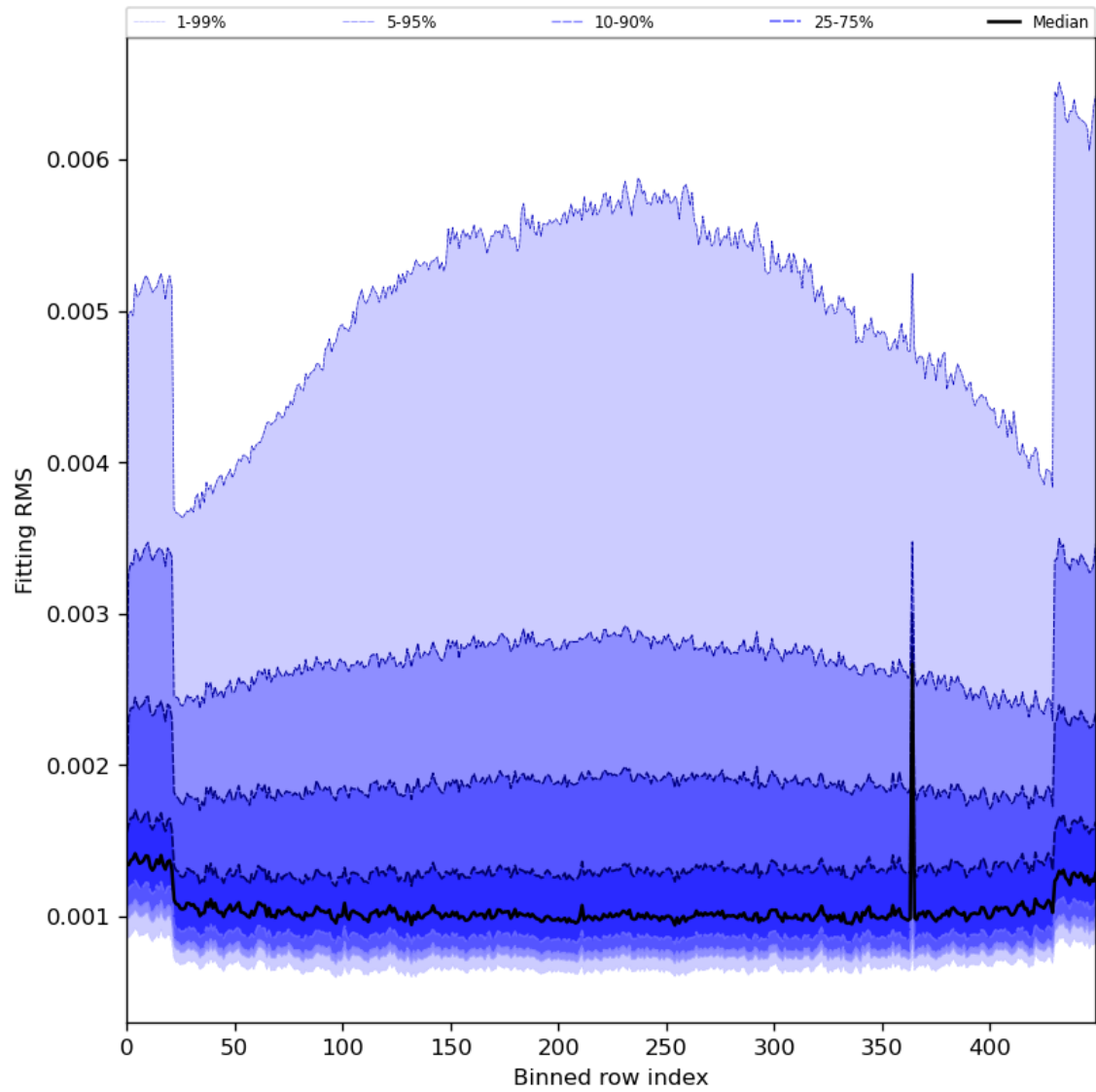
Figure 30: Along track statistics of “Fitting RMS” for 2024-05-18 to 2024-05-19
