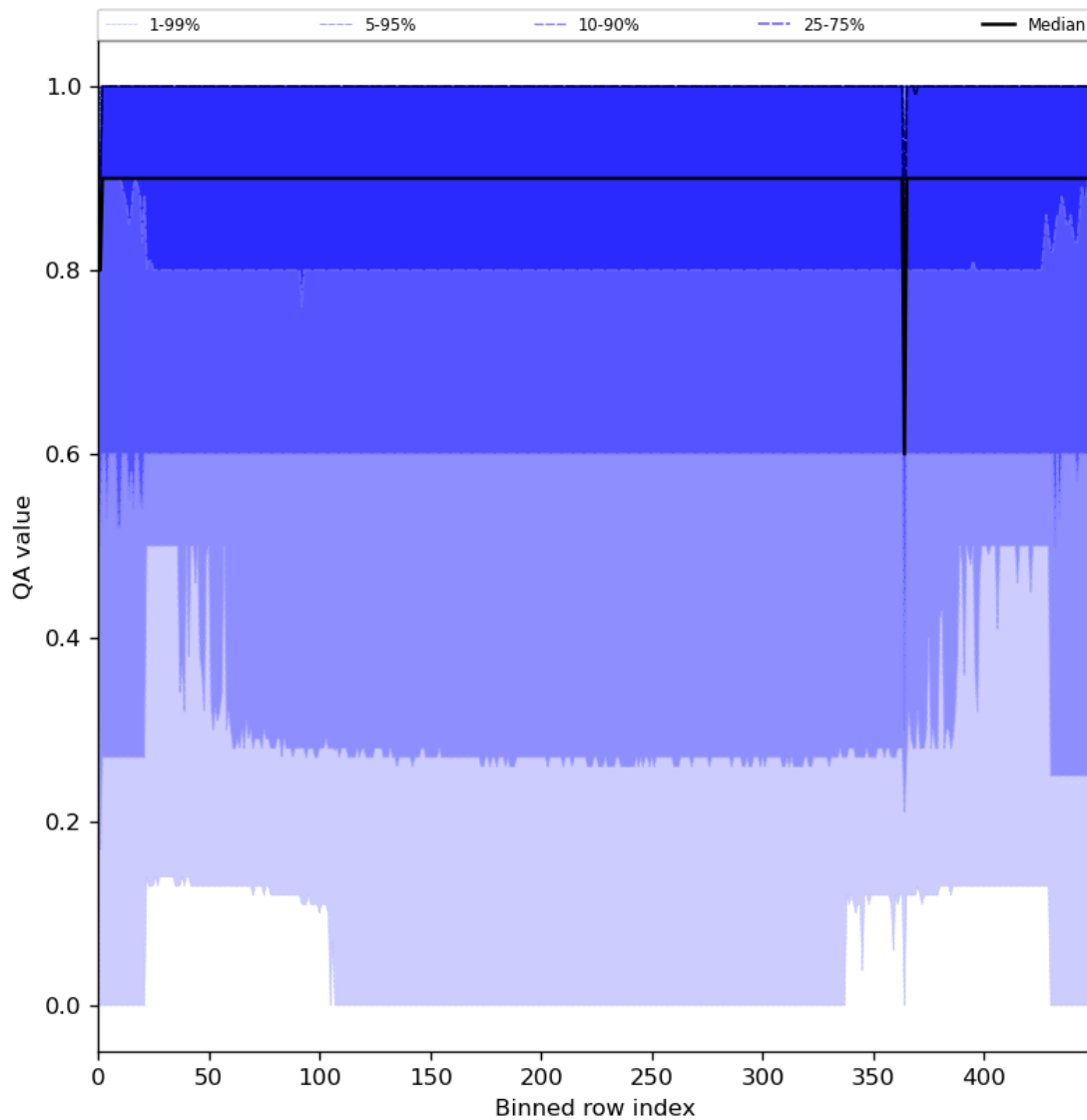
Figure 27: Along track statistics of “QA value” for 2024-05-18 to 2024-05-19
