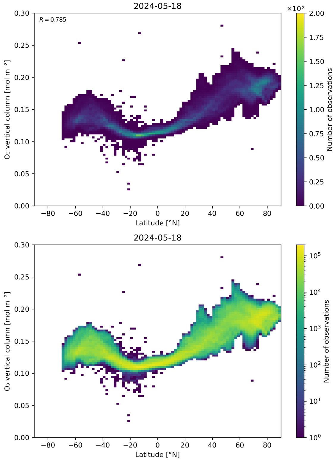
Figure 36: Scatter density plot of “Latitude” against “O 3 vertical column” for 2024-05-18 to 2024-05-19.
