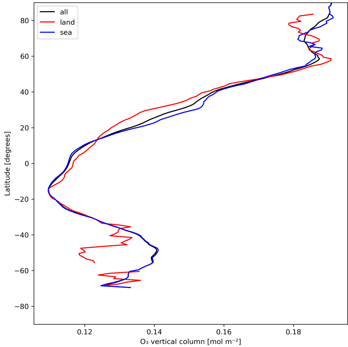
Figure 14: Zonal average of “O 3 vertical column” for 2024-05-18 to 2024-05-19.
