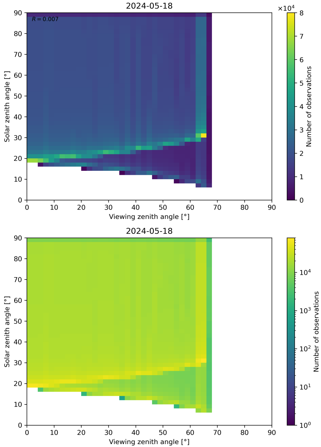
Figure 54: Scatter density plot of “Viewing zenith angle” against “Solar zenith angle” for 2024-05-18 to 2024-05-19.
