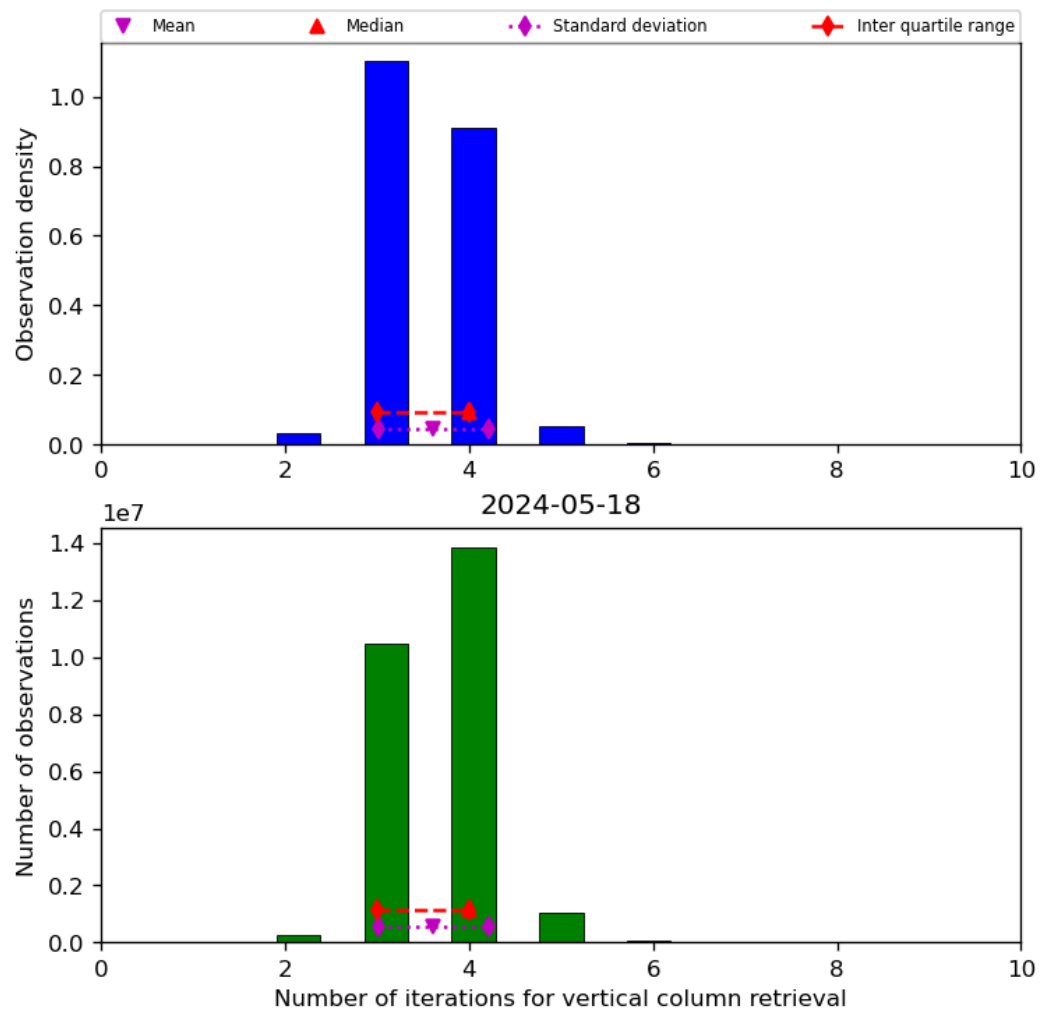
Figure 26: Histogram of “Number of iterations for vertical column retrieval” for 2024-05-18 to 2024-05-19
