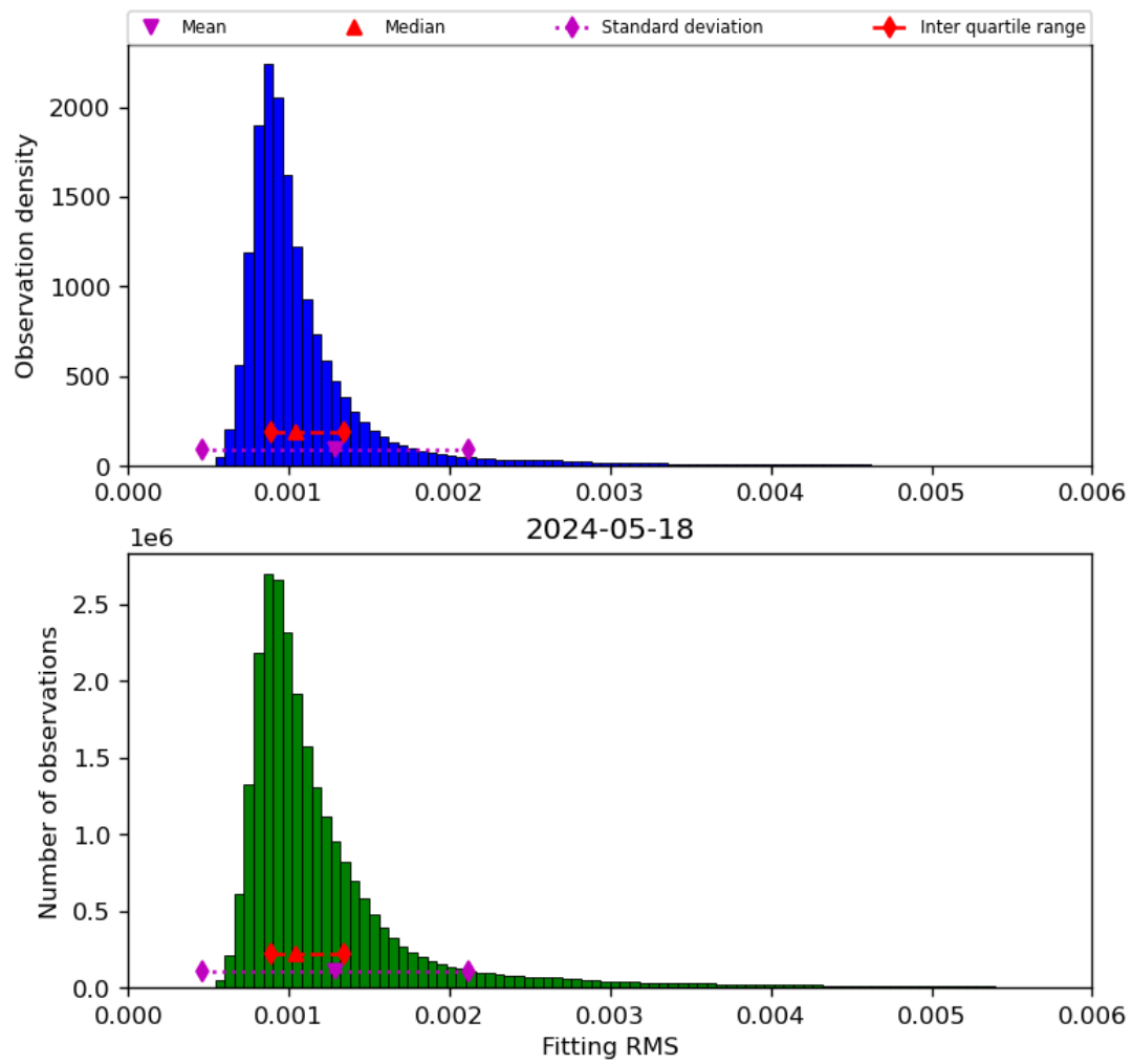
Figure 23: Histogram of “Fitting RMS” for 2024-05-18 to 2024-05-19
