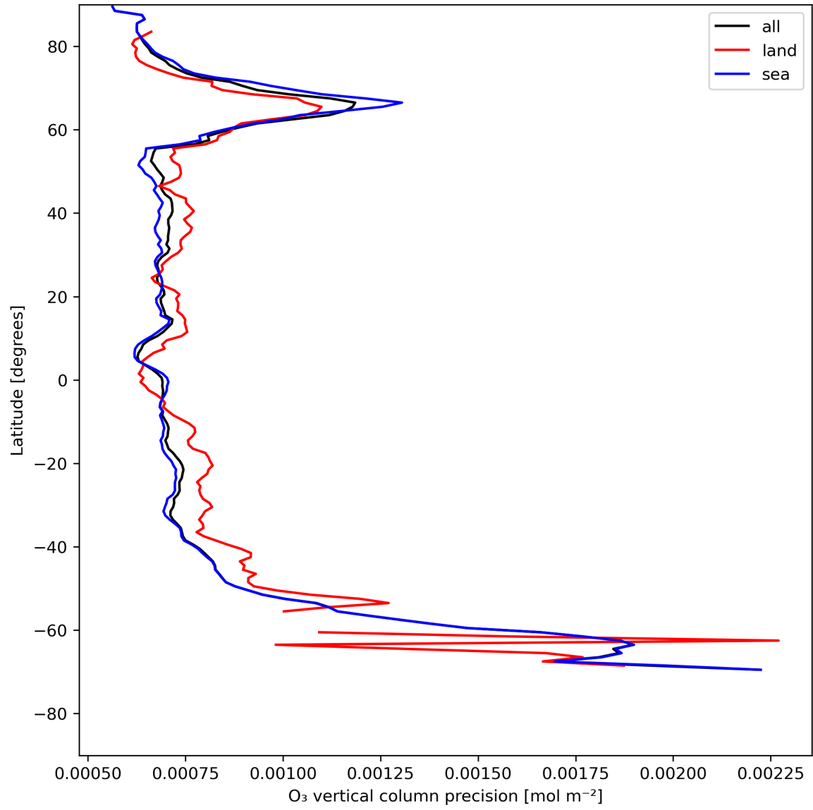
Figure 15: Zonal average of "O 3 vertical column precision" for 2024-05-18 to 2024-05-19.
