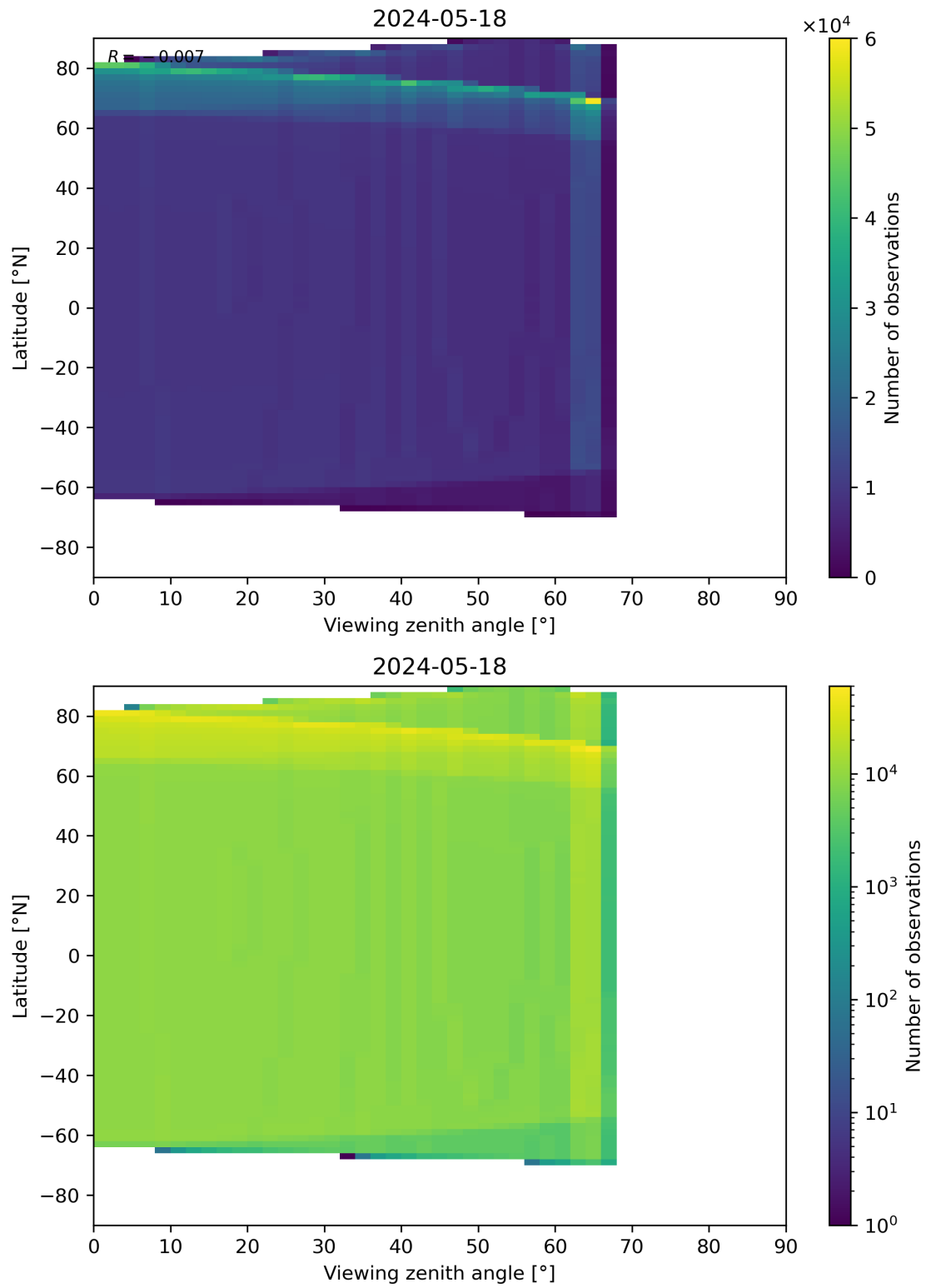
Figure 49: Scatter density plot of “Viewing zenith angle” against “Latitude” for 2024-05-18 to 2024-05-19.
