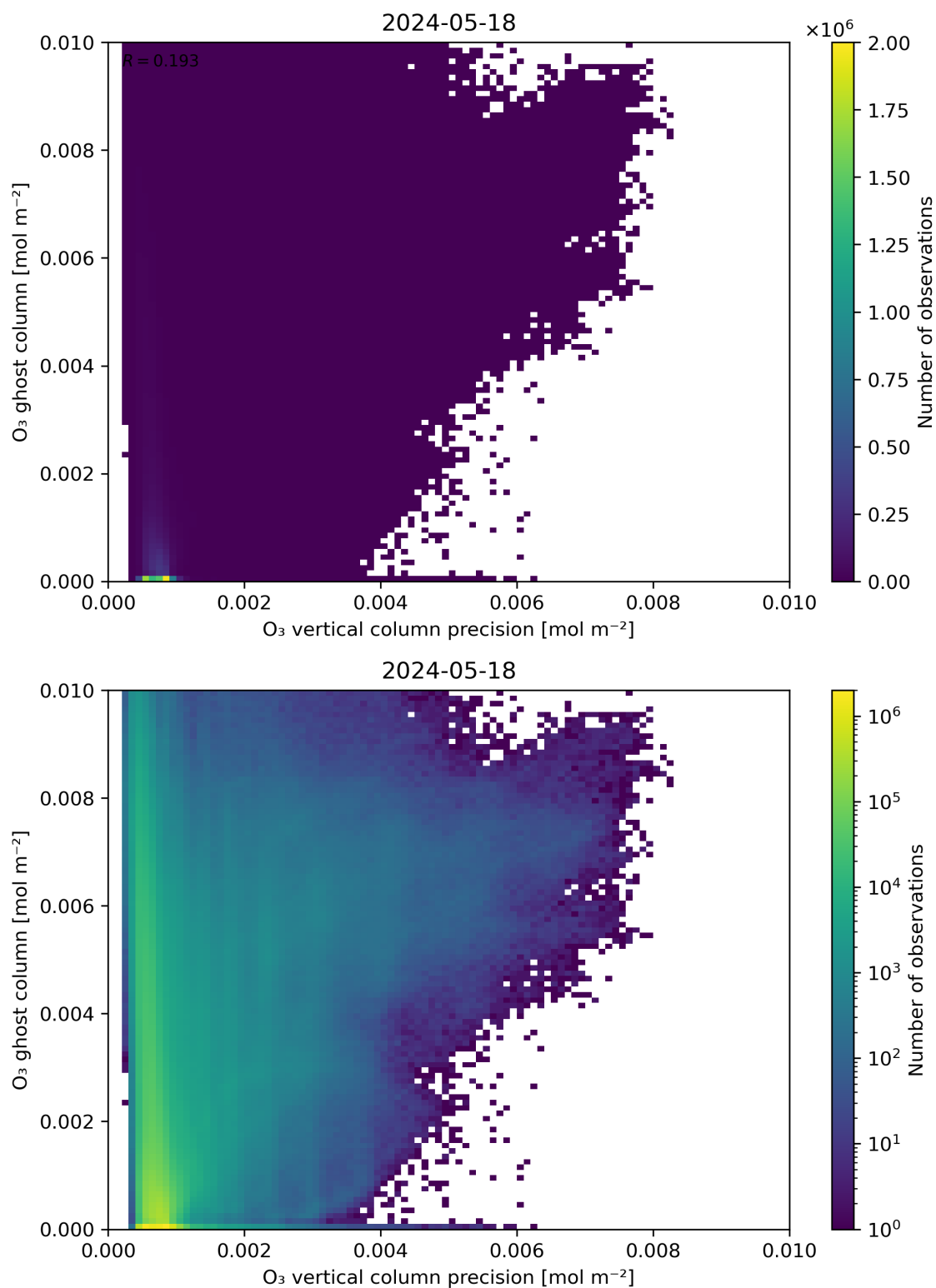
Figure 43: Scatter density plot of “O 3 vertical column precision” against “O 3 ghost column” for 2024-05-18 to 2024-05-19.
