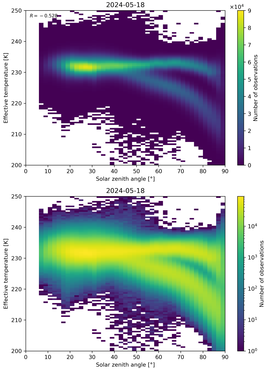
Figure 45: Scatter density plot of “Solar zenith angle” against “Effective temperature” for 2024-05-18 to 2024-05-19.
