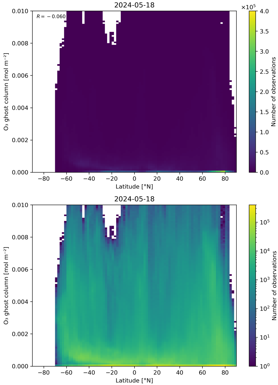
Figure 35: Scatter density plot of “Latitude” against “O 3 ghost column” for 2024-05-18 to 2024-05-19.
