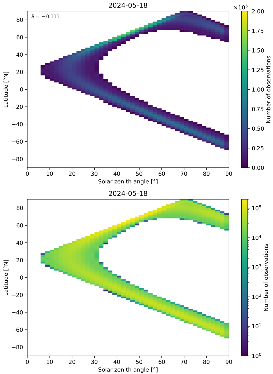
Figure 44: Scatter density plot of “Solar zenith angle” against “Latitude” for 2024-05-18 to 2024-05-19.
