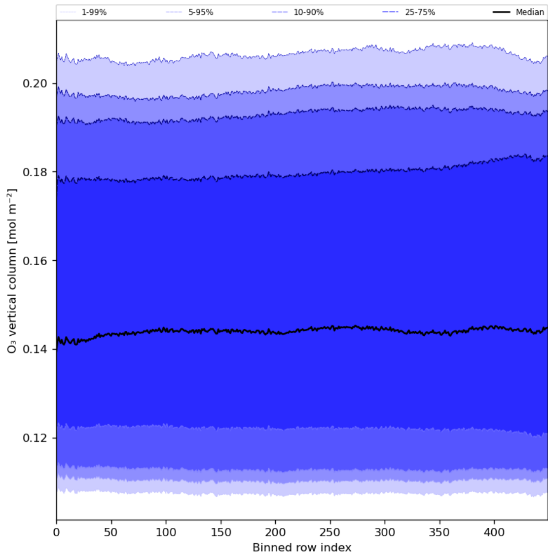
Figure 28: Along track statistics of “O 3 vertical column” for 2024-05-18 to 2024-05-19
