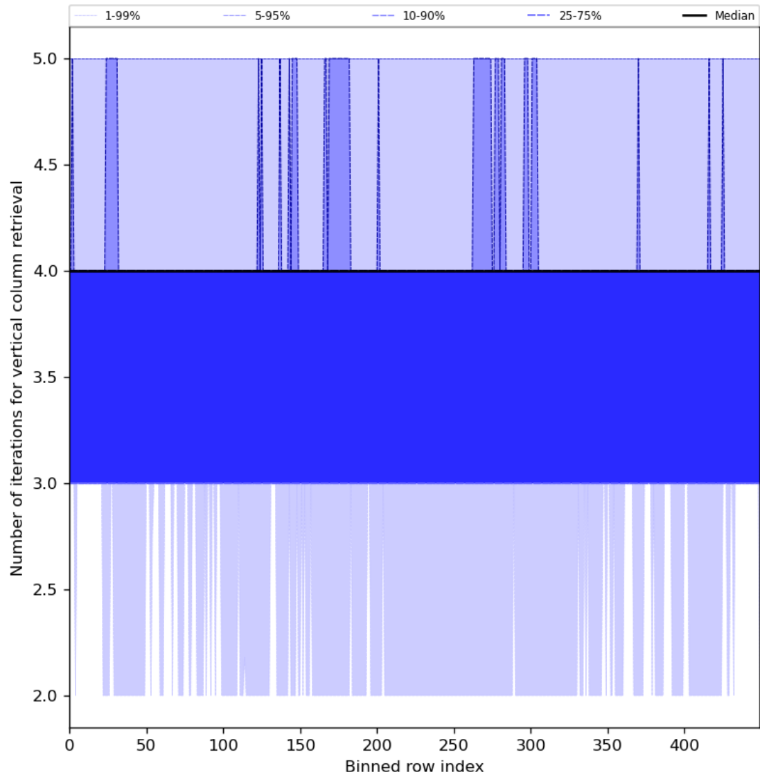
Figure 33: Along track statistics of “Number of iterations for vertical column retrieval” for 2024-05-18 to 2024-05-19
