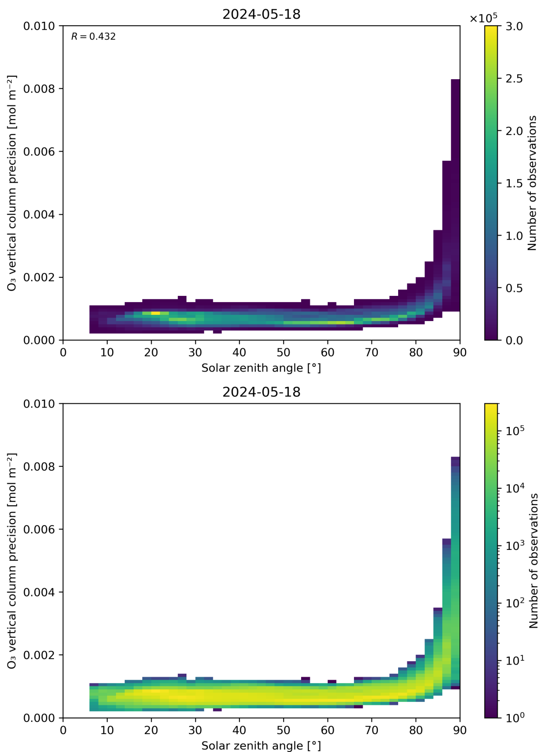
Figure 48: Scatter density plot of “Solar zenith angle” against “O 3 vertical column precision” for 2024-05-18 to 2024-05-19.
