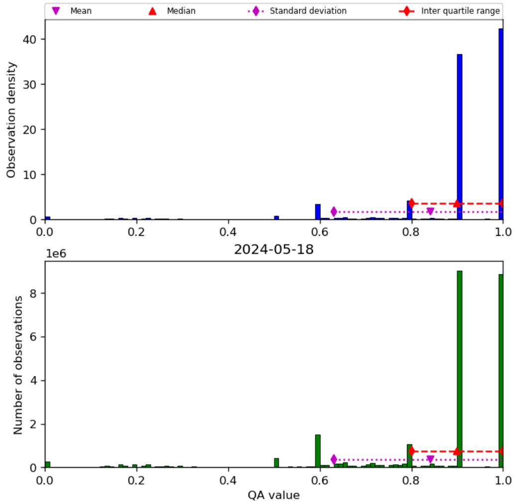
Figure 20: Histogram of “QA value” for 2024-05-18 to 2024-05-19
