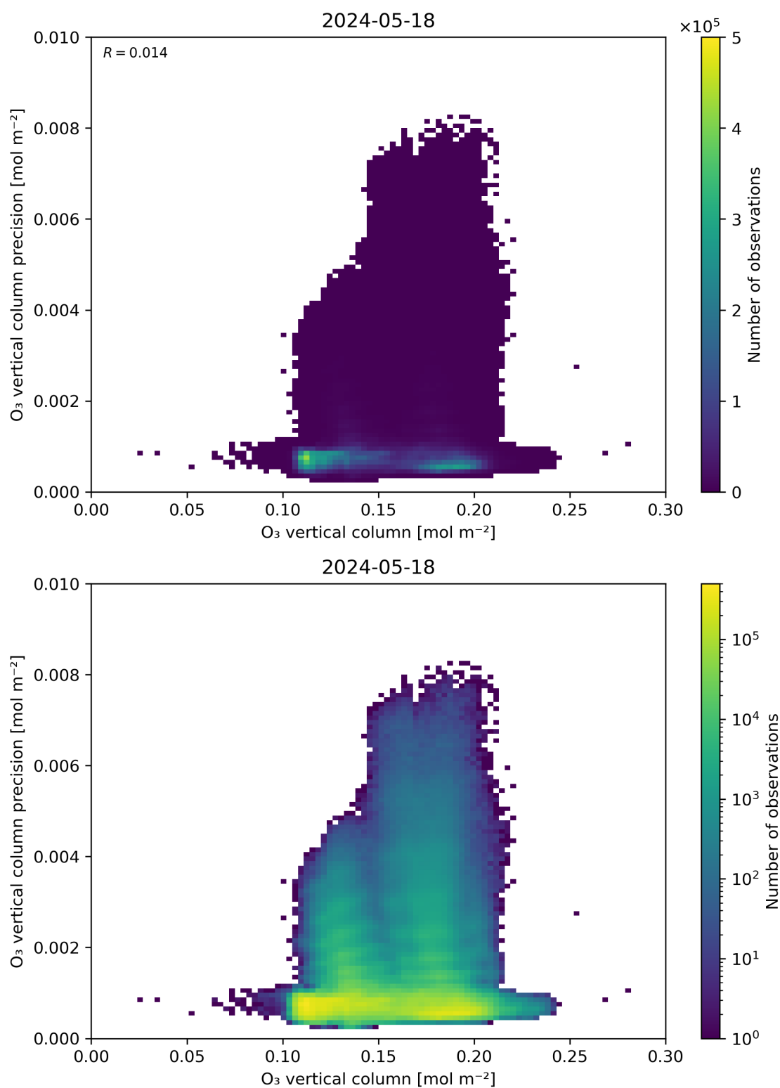
Figure 41: Scatter density plot of “O 3 vertical column” against “O 3 vertical column precision” for 2024-05-18 to 2024-05-19.
