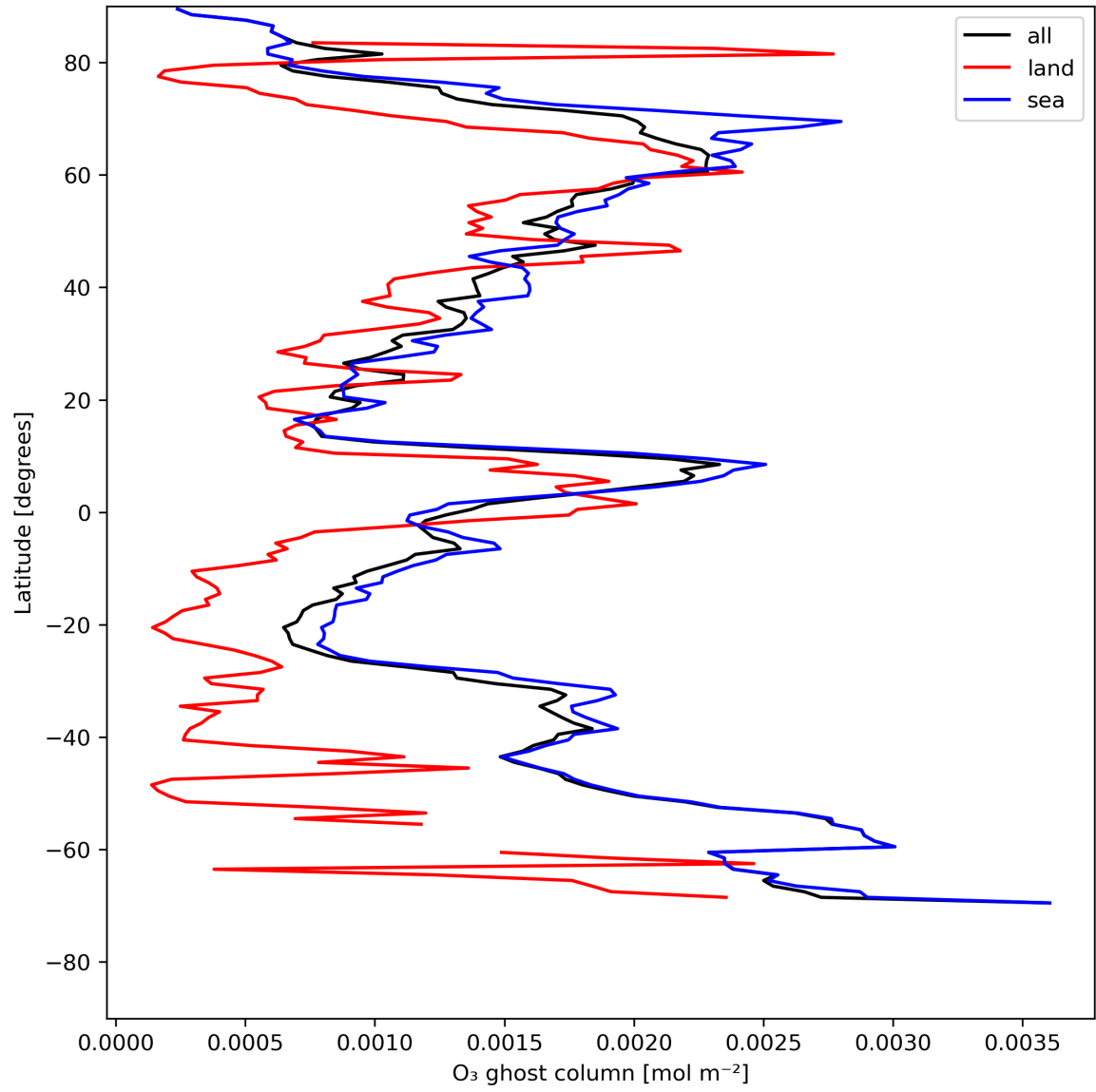
Figure 18: Zonal average of “O 3 ghost column” for 2024-05-18 to 2024-05-19.
