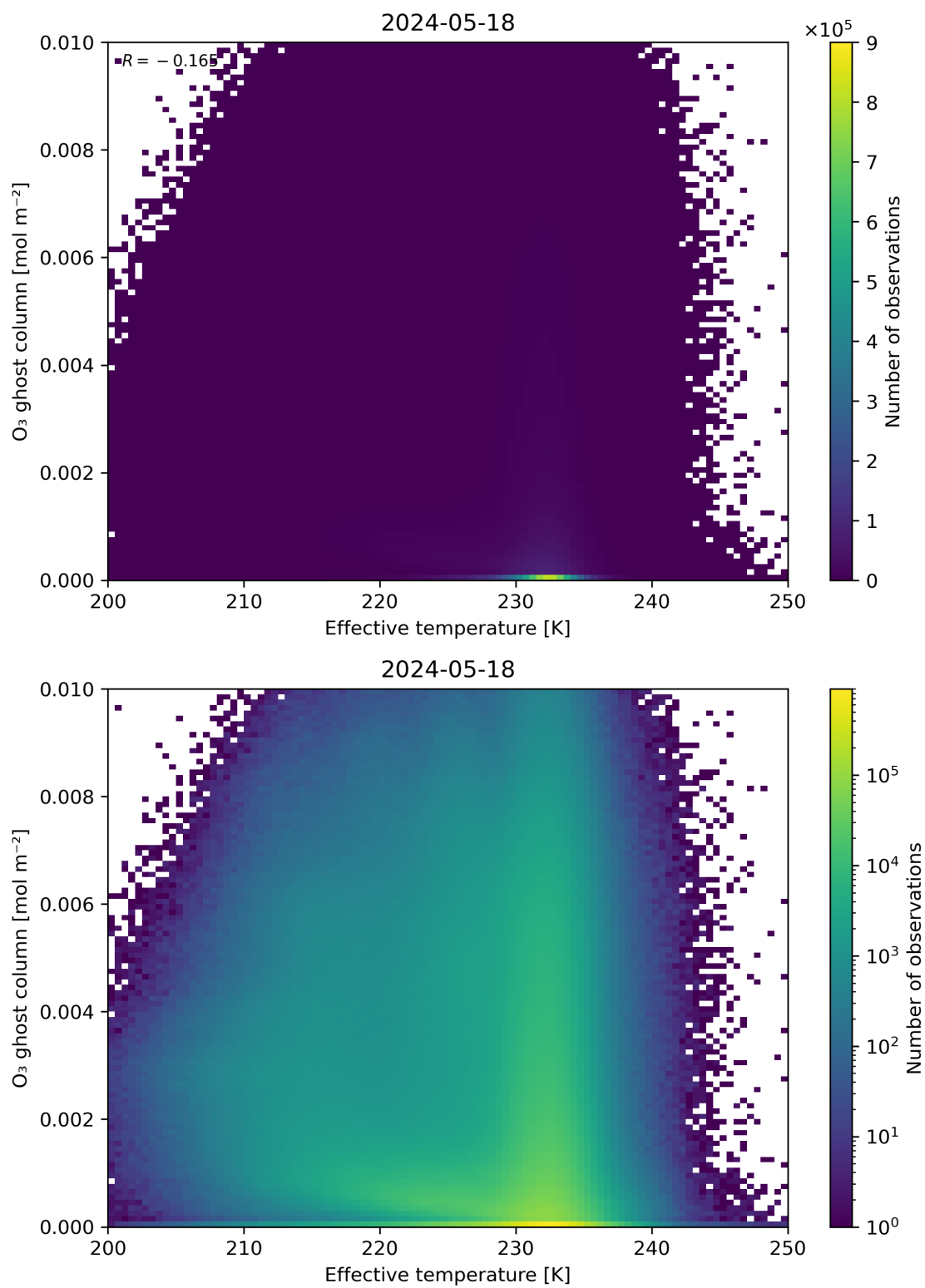
Figure 38: Scatter density plot of “Effective temperature” against “O 3 ghost column” for 2024-05-18 to 2024-05-19.
