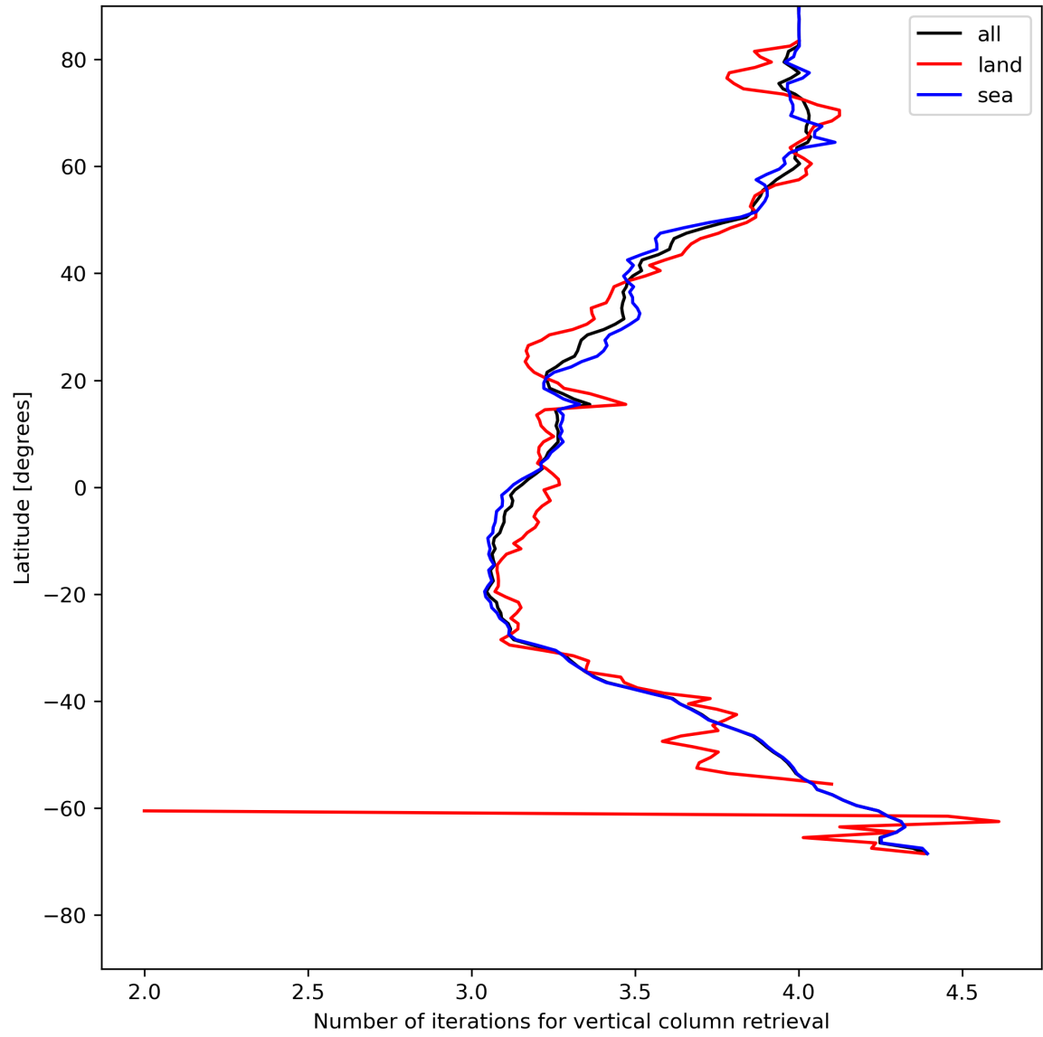
Figure 19: Zonal average of “Number of iterations for vertical column retrieval” for 2024-05-18 to 2024-05-20.
