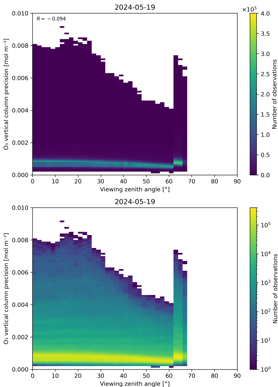
Figure 53: Scatter density plot of “Viewing zenith angle” against “O 3 vertical column precision” for 2024-05-18 to 2024-05-20.
