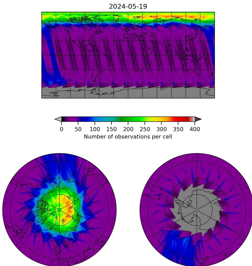
Figure 12: Map of the number of observations for 2024-05-18 to 2024-05-20
