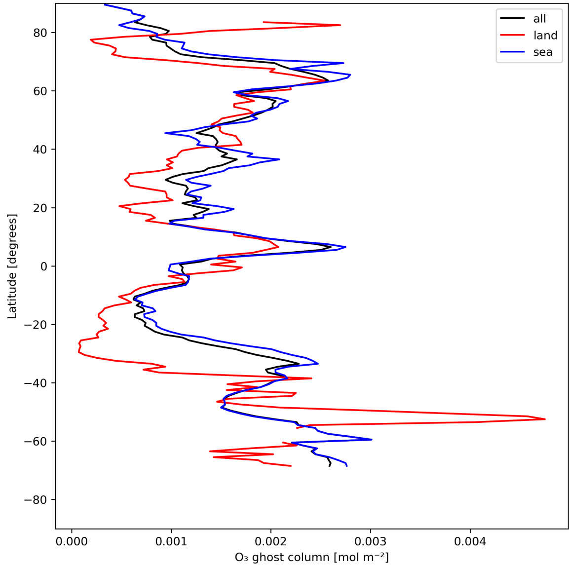
Figure 18: Zonal average of "O 3 ghost column" for 2024-05-18 to 2024-05-20.
