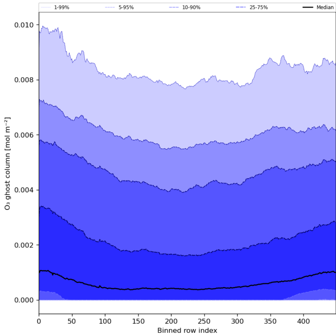
Figure 32: Along track statistics of “O 3 ghost column” for 2024-05-18 to 2024-05-20
