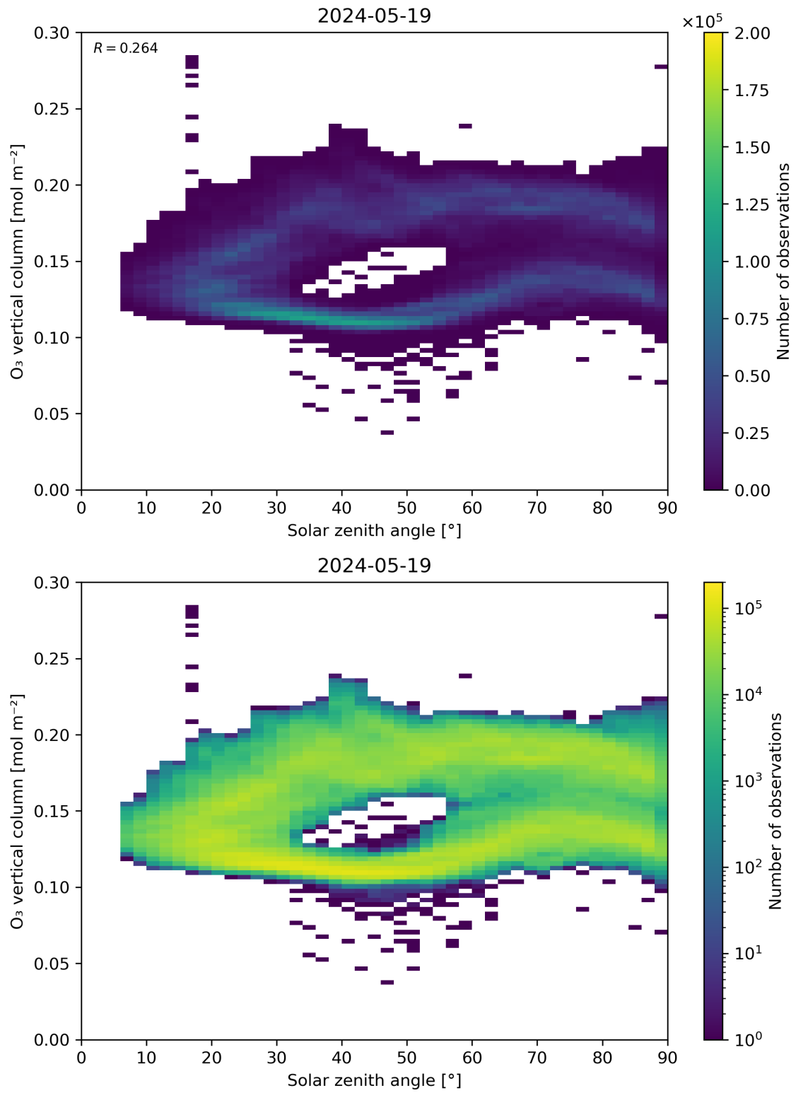
Figure 47: Scatter density plot of “Solar zenith angle” against “O 3 vertical column” for 2024-05-18 to 2024-05-20.
