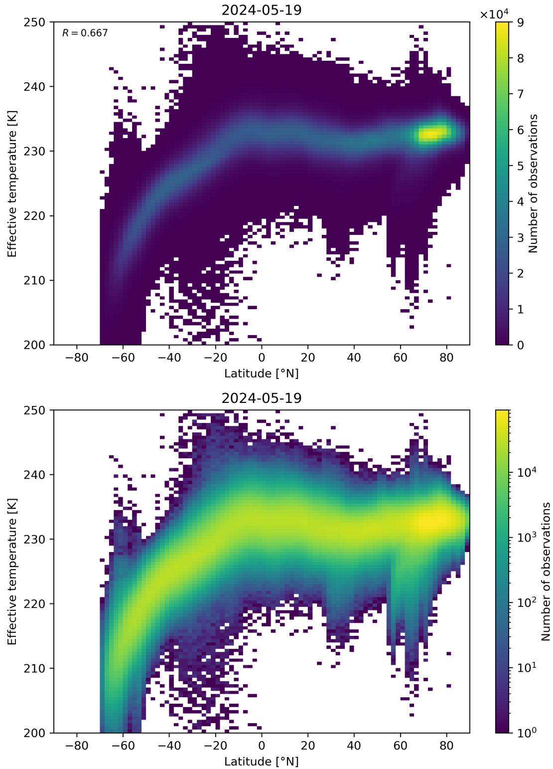
Figure 34: Scatter density plot of “Latitude” against “Effective temperature” for 2024-05-18 to 2024-05-20.
