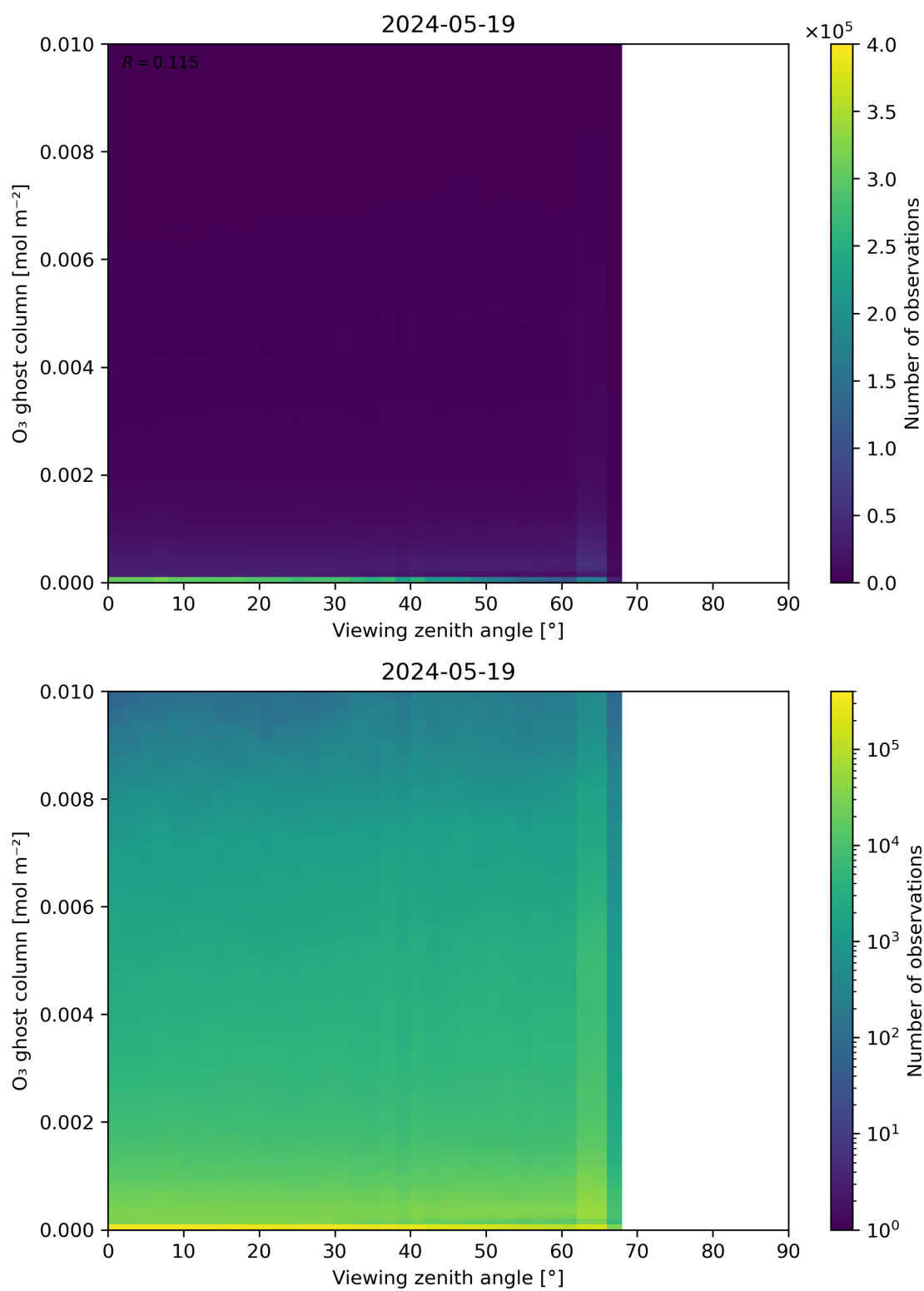
Figure 51: Scatter density plot of “Viewing zenith angle” against “O 3 ghost column” for 2024-05-18 to 2024-05-20.
