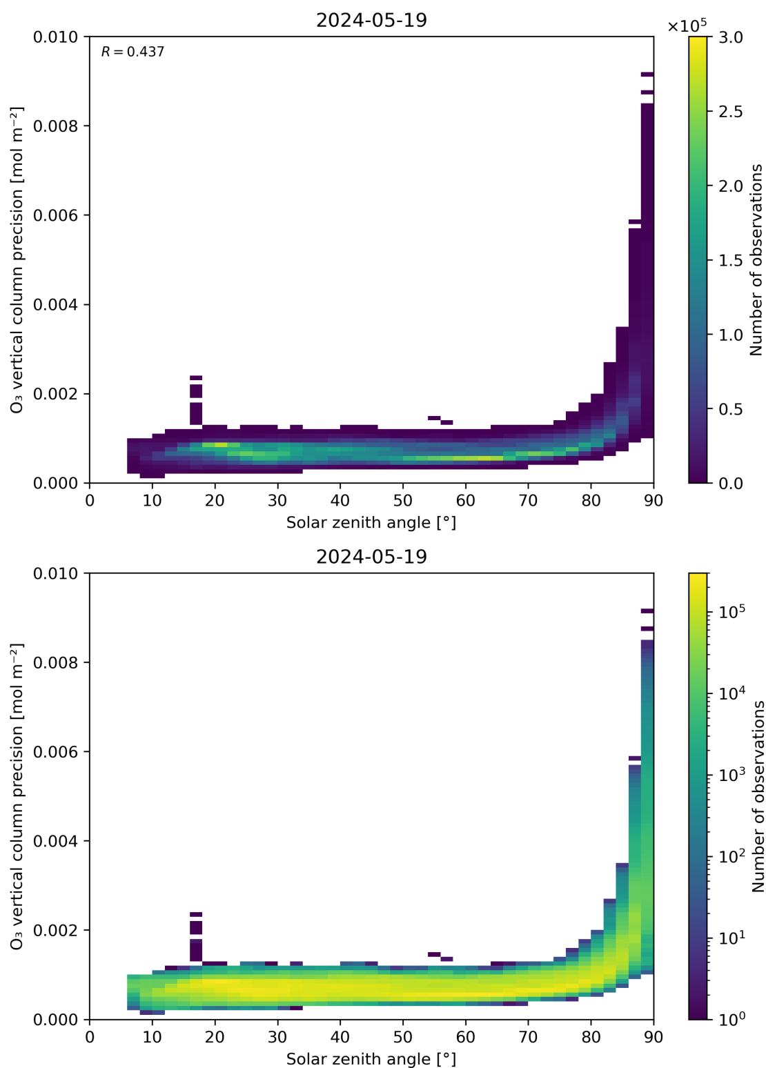
Figure 48: Scatter density plot of “Solar zenith angle” against “O 3 vertical column precision” for 2024-05-18 to 2024-05-20.
