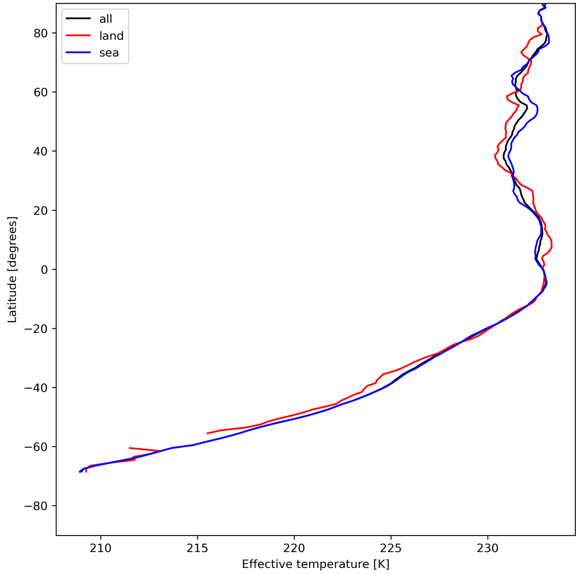
Figure 17: Zonal average of "Effective temperature" for 2024-05-18 to 2024-05-20.
