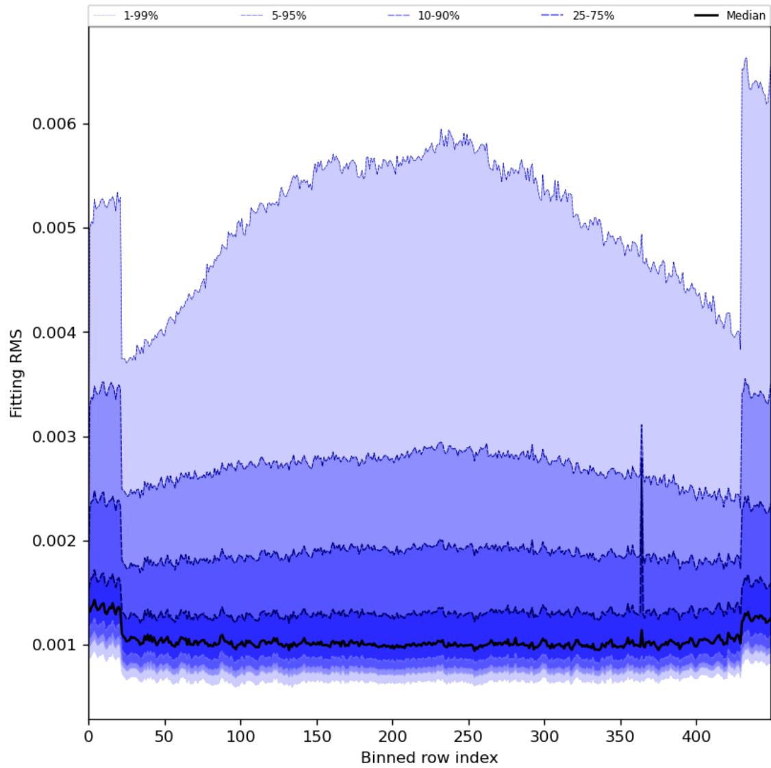
Figure 30: Along track statistics of “Fitting RMS” for 2024-05-18 to 2024-05-20
