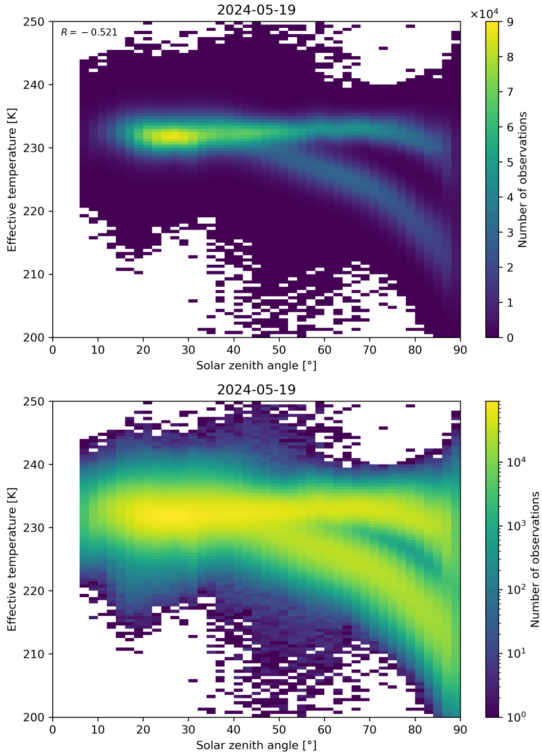
Figure 45: Scatter density plot of “Solar zenith angle” against “Effective temperature” for 2024-05-18 to 2024-05-20.
