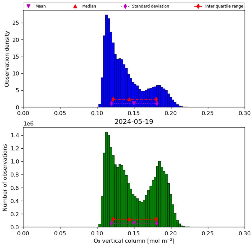
Figure 21: Histogram of “O 3 vertical column” for 2024-05-18 to 2024-05-20
