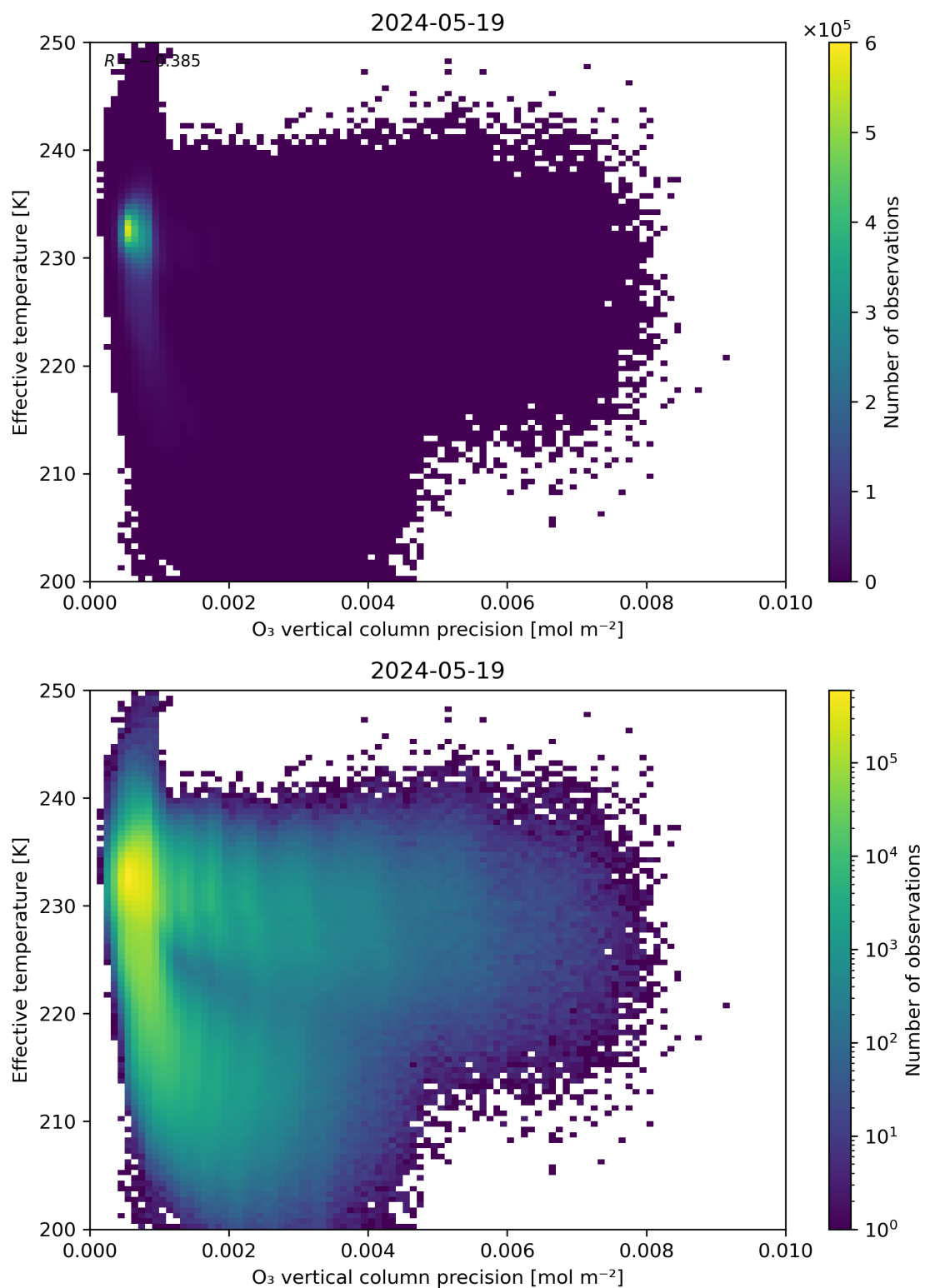
Figure 42: Scatter density plot of “O 3 vertical column precision” against “Effective temperature” for 2024-05-18 to 2024-05-20.
