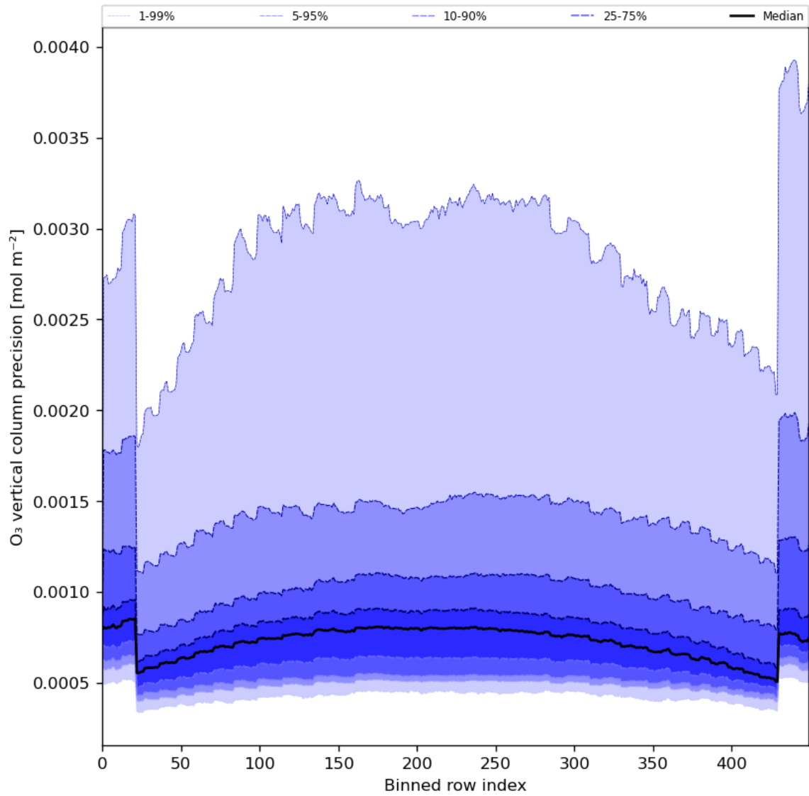
Figure 29: Along track statistics of “O 3 vertical column precision” for 2024-05-18 to 2024-05-20
