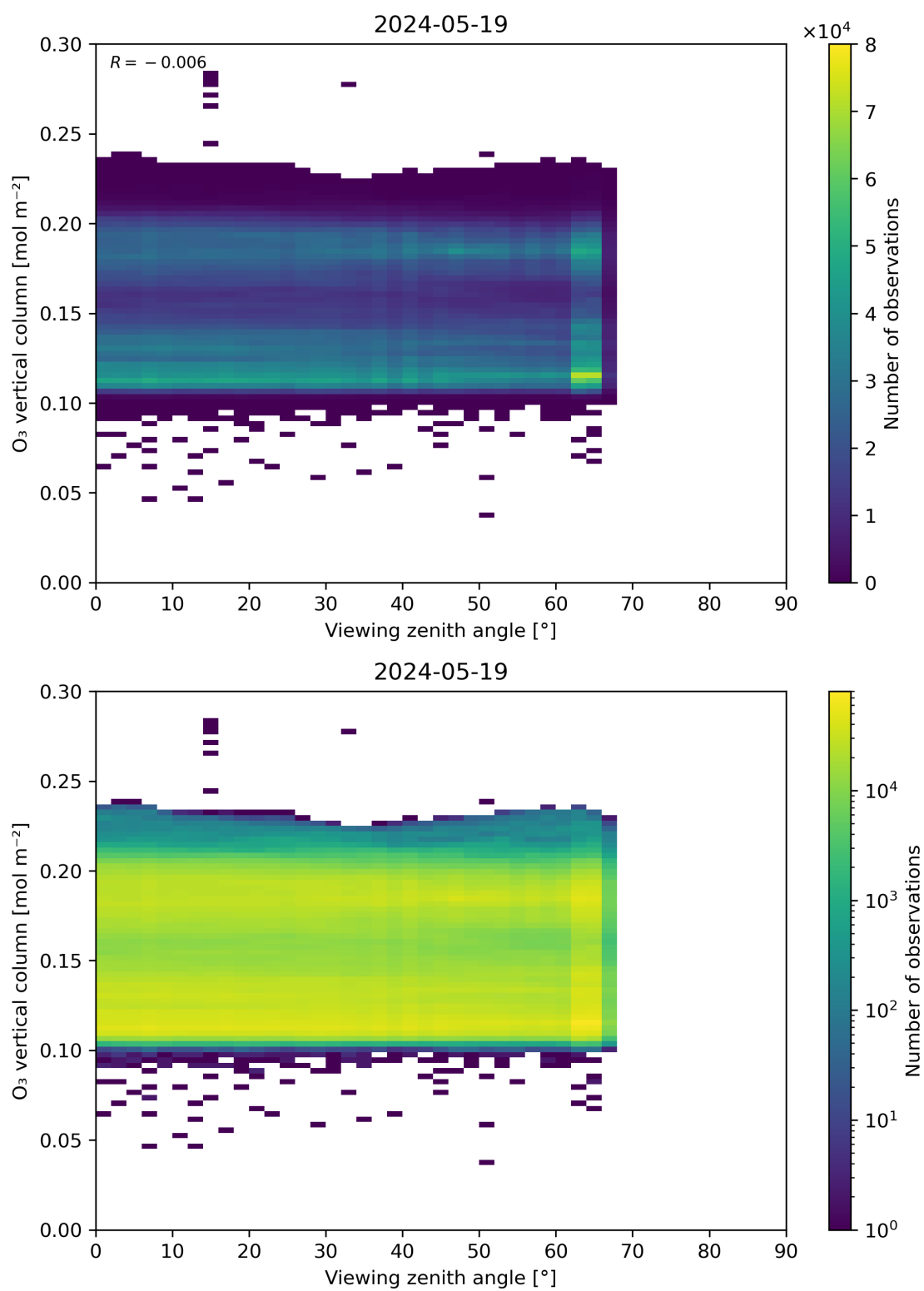
Figure 52: Scatter density plot of “Viewing zenith angle” against “O 3 vertical column” for 2024-05-18 to 2024-05-20.
