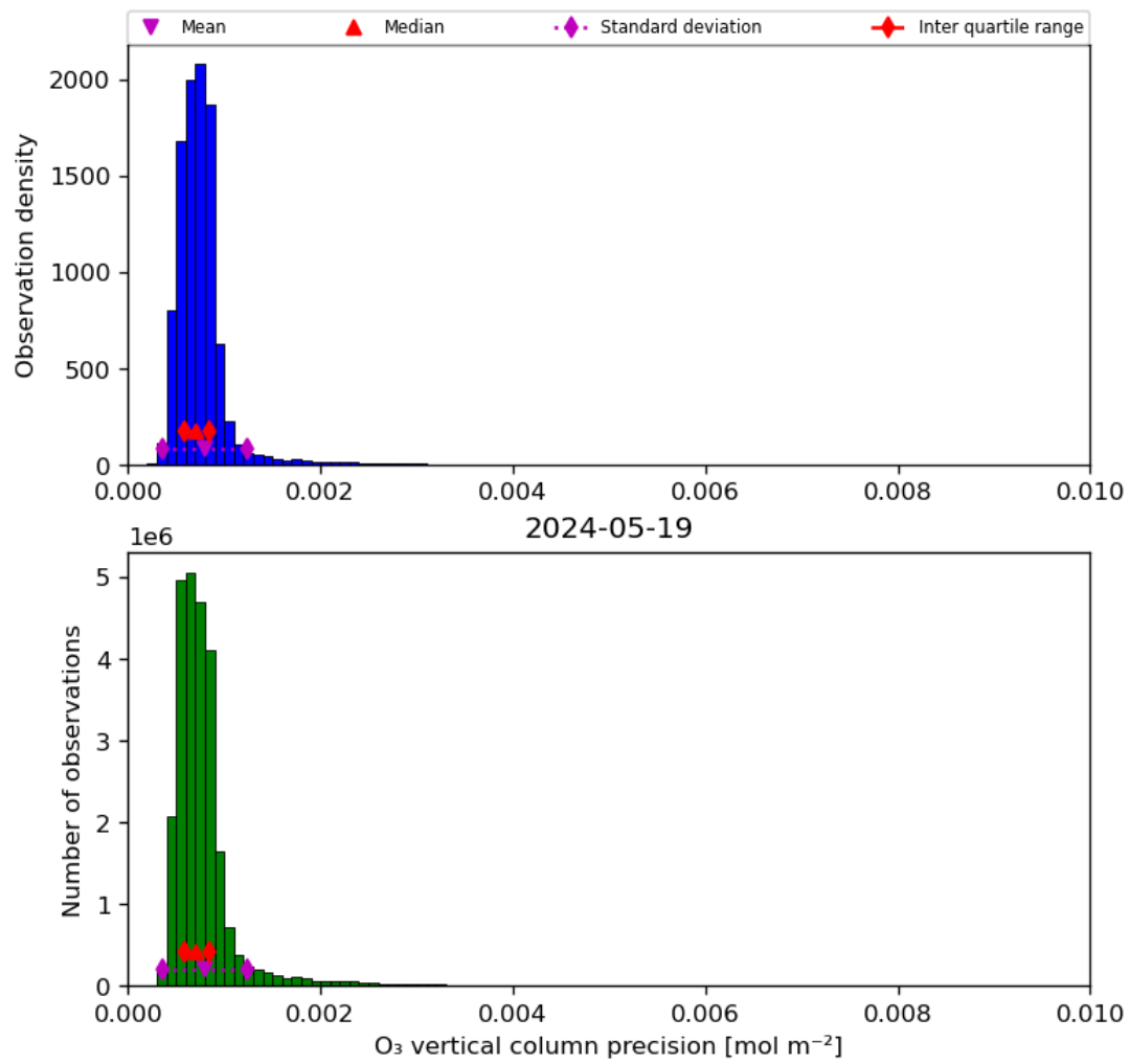
Figure 22: Histogram of “O 3 vertical column precision” for 2024-05-18 to 2024-05-20
