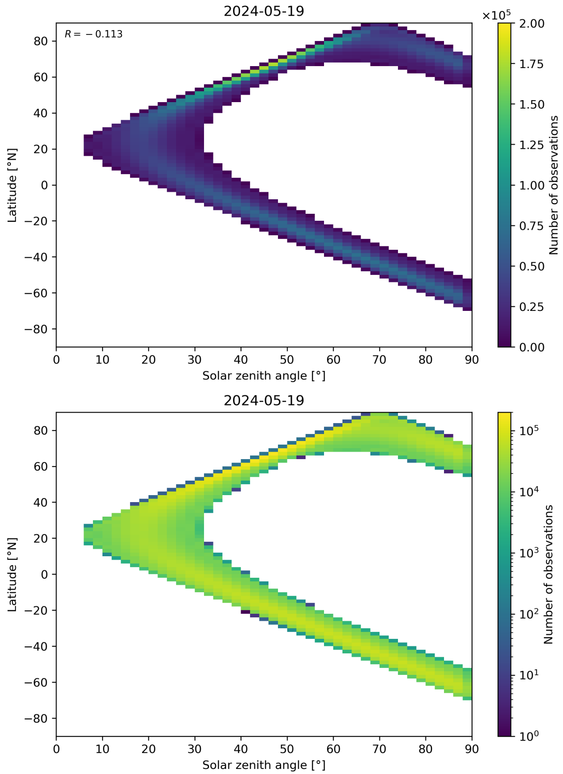
Figure 44: Scatter density plot of “Solar zenith angle” against “Latitude” for 2024-05-18 to 2024-05-20.
