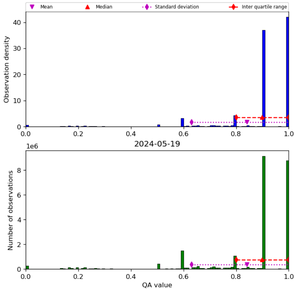
Figure 20: Histogram of “QA value” for 2024-05-18 to 2024-05-20
