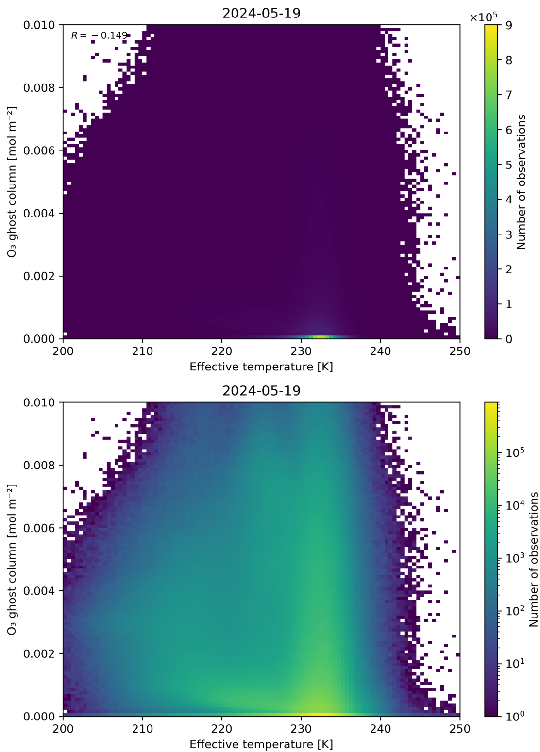
Figure 38: Scatter density plot of “Effective temperature” against “O 3 ghost column” for 2024-05-18 to 2024-05-20.
