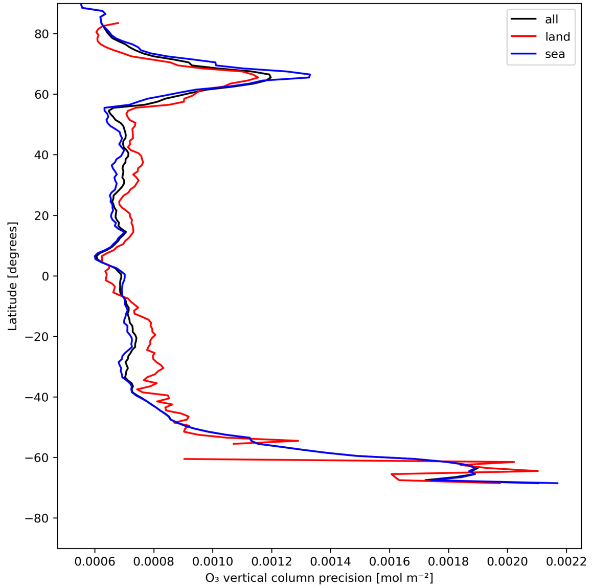
Figure 15: Zonal average of "O 3 vertical column precision" for 2024-05-18 to 2024-05-20.
