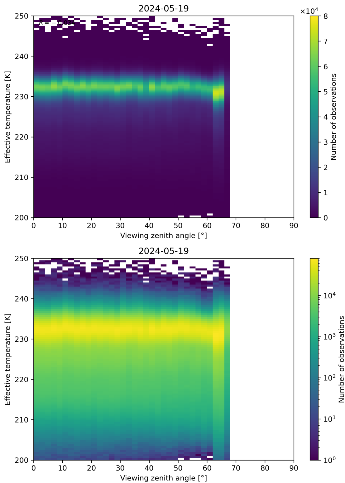
Figure 50: Scatter density plot of “Viewing zenith angle” against “Effective temperature” for 2024-05-18 to 2024-05-20.
