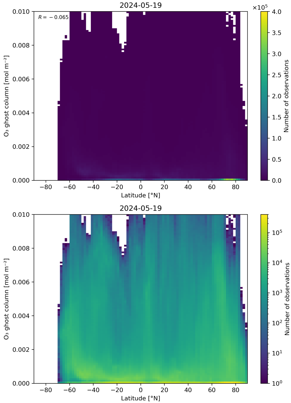
Figure 35: Scatter density plot of “Latitude” against “O 3 ghost column” for 2024-05-18 to 2024-05-20.
