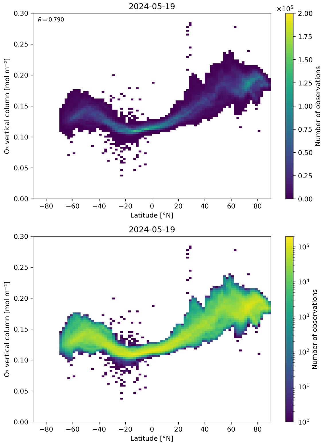
Figure 36: Scatter density plot of “Latitude” against “O 3 vertical column” for 2024-05-18 to 2024-05-20.
