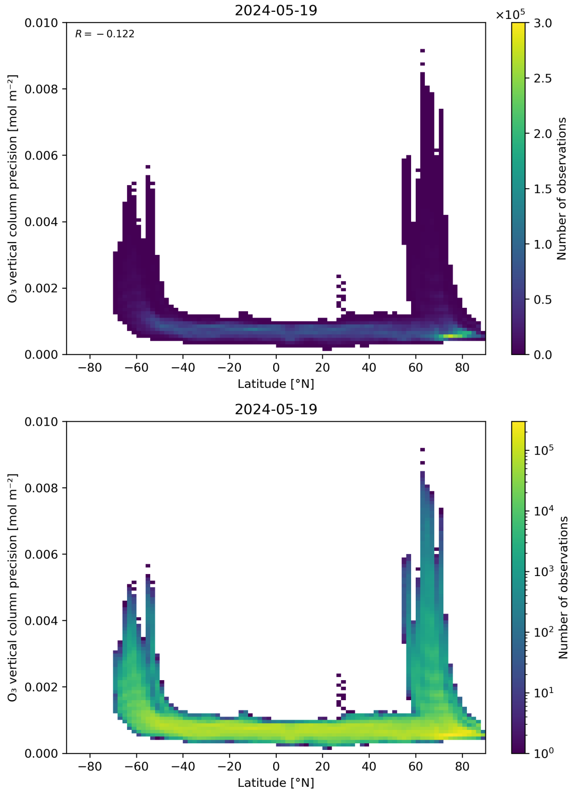
Figure 37: Scatter density plot of “Latitude” against “O 3 vertical column precision” for 2024-05-18 to 2024-05-20.
