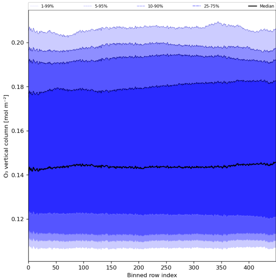
Figure 28: Along track statistics of “O 3 vertical column” for 2024-05-18 to 2024-05-20
