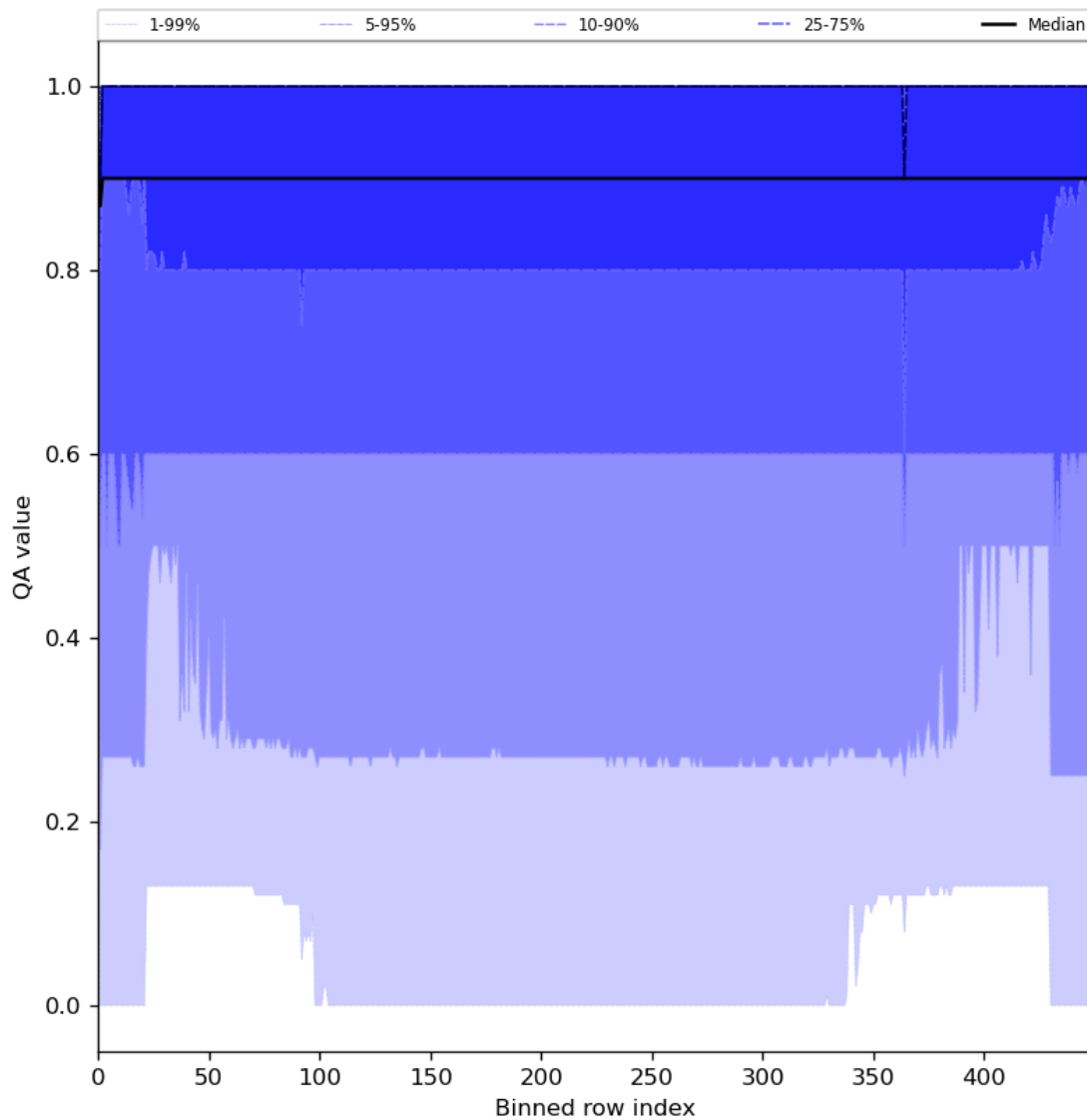
Figure 27: Along track statistics of “QA value” for 2024-05-18 to 2024-05-20
