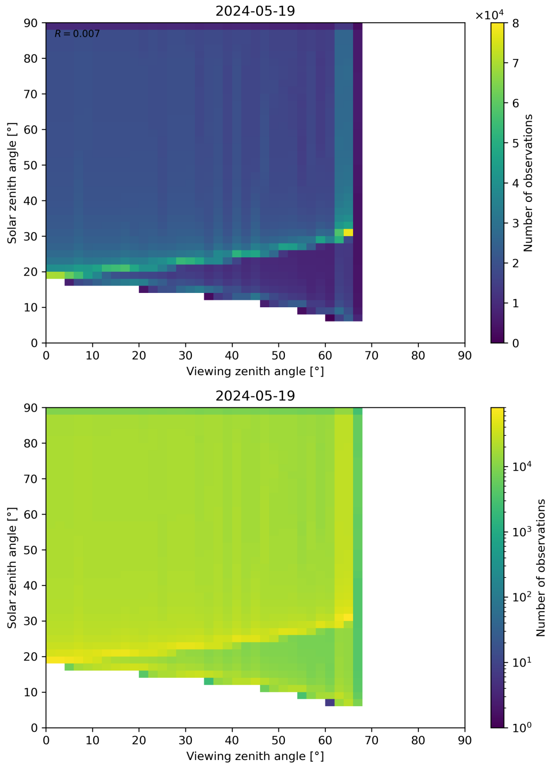
Figure 54: Scatter density plot of “Viewing zenith angle” against “Solar zenith angle” for 2024-05-18 to 2024-05-20.
