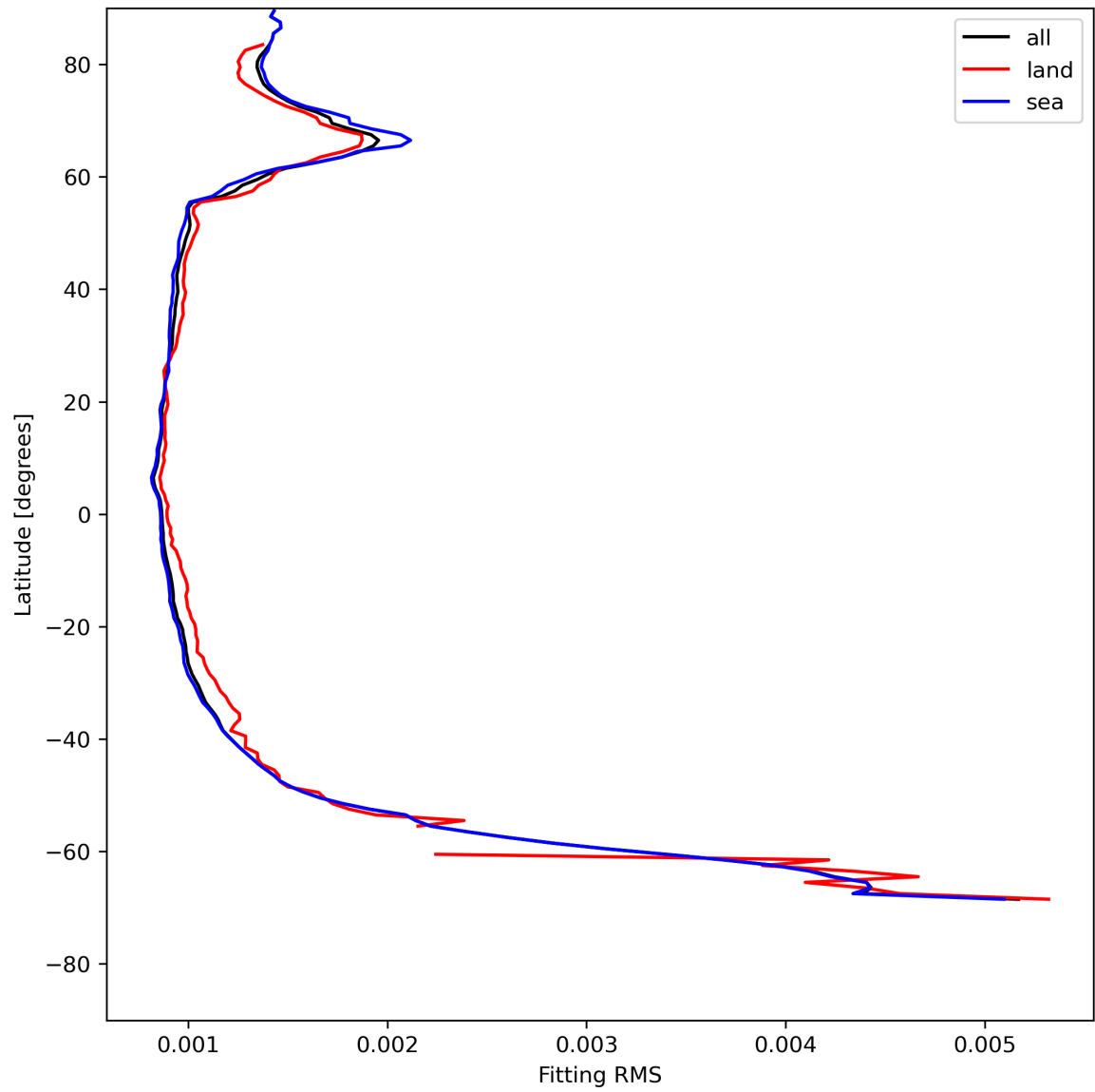
Figure 16: Zonal average of “Fitting RMS” for 2024-05-18 to 2024-05-20.
