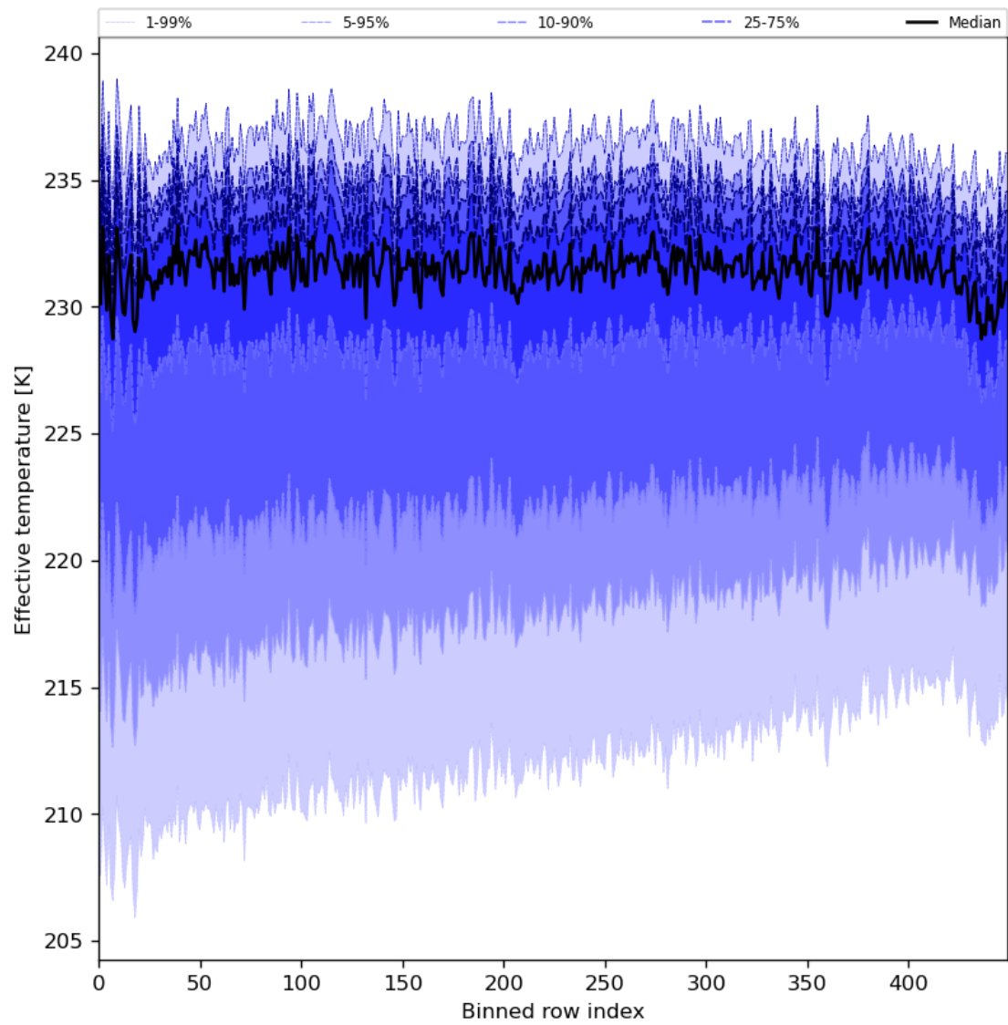
Figure 31: Along track statistics of “Effective temperature” for 2024-05-18 to 2024-05-20
