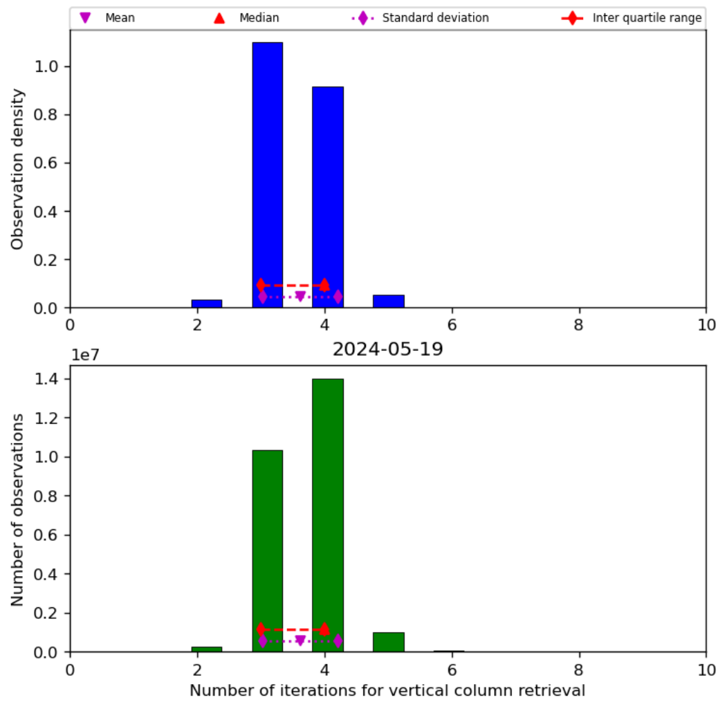
Figure 26: Histogram of “Number of iterations for vertical column retrieval” for 2024-05-18 to 2024-05-20
