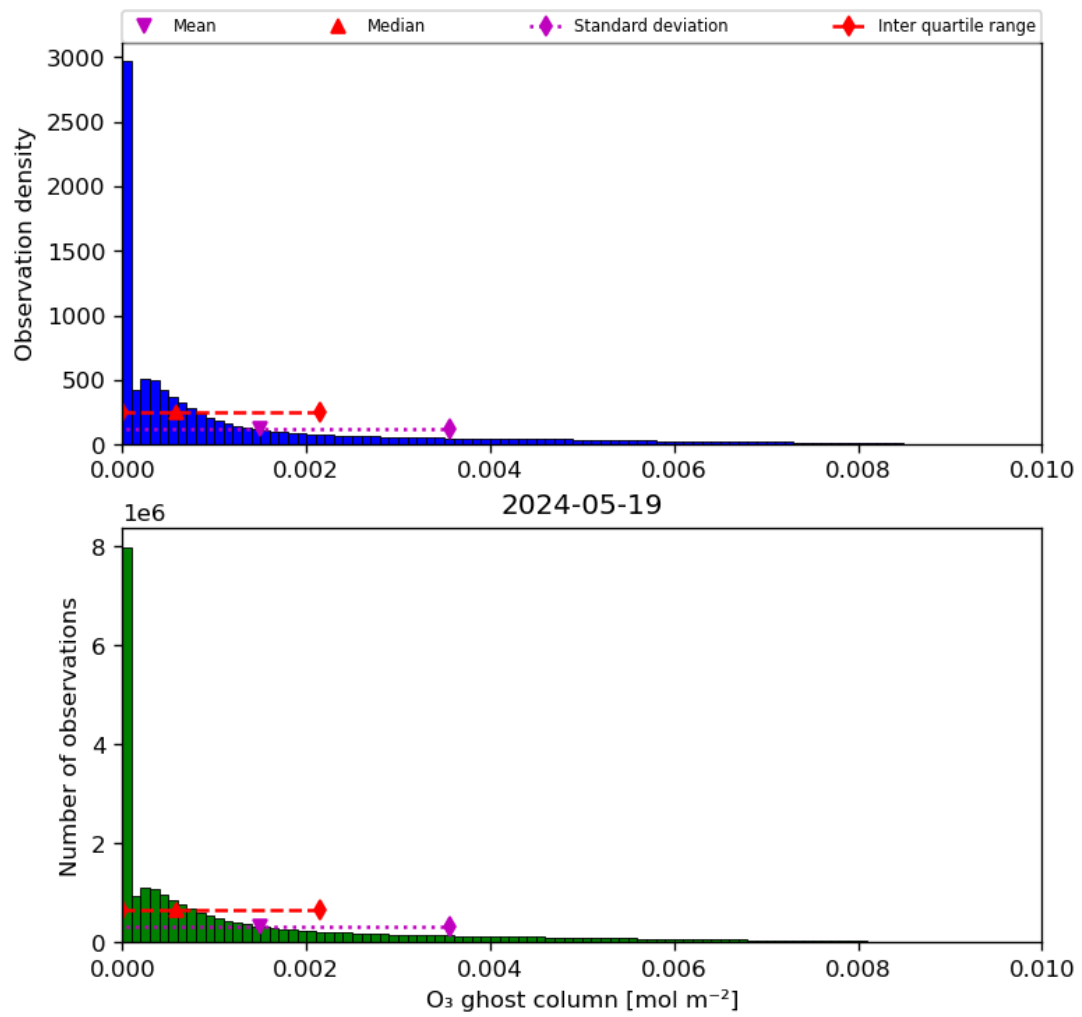
Figure 25: Histogram of “O 3 ghost column” for 2024-05-18 to 2024-05-20
