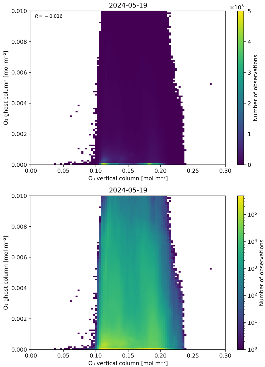
Figure 40: Scatter density plot of “O 3 vertical column” against “O 3 ghost column” for 2024-05-18 to 2024-05-20.
