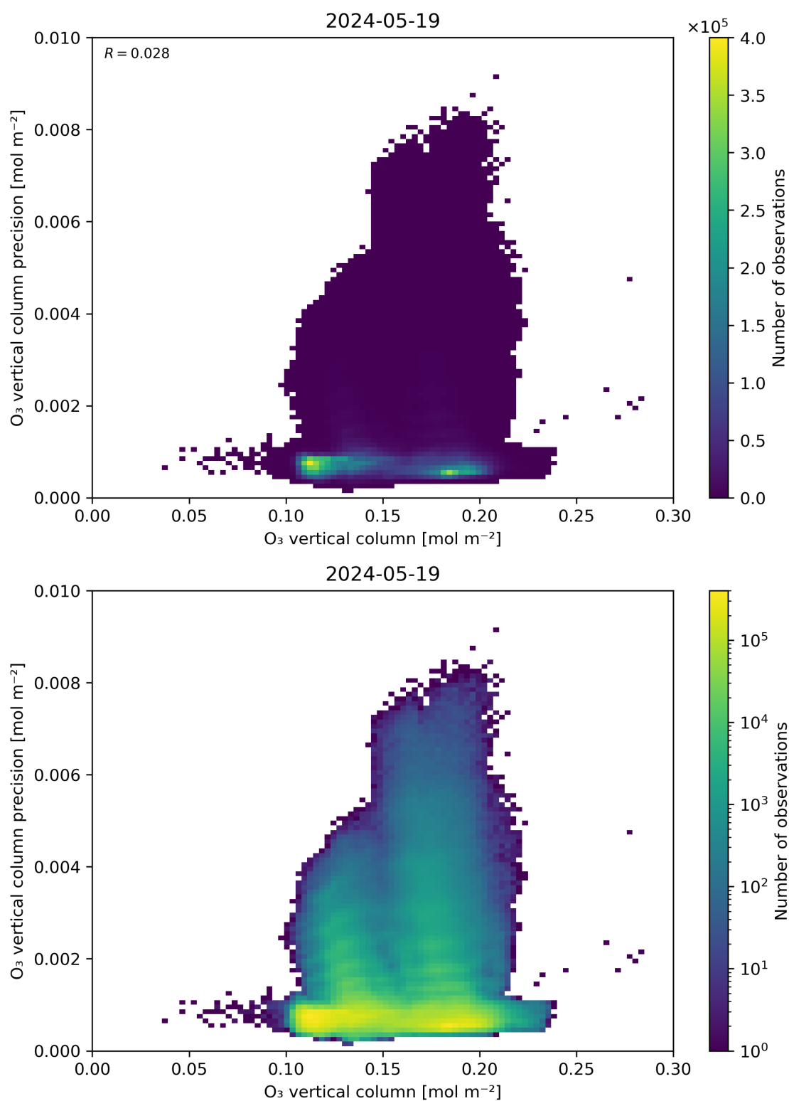
Figure 41: Scatter density plot of “O 3 vertical column” against “O 3 vertical column precision” for 2024-05-18 to 2024-05-20.
