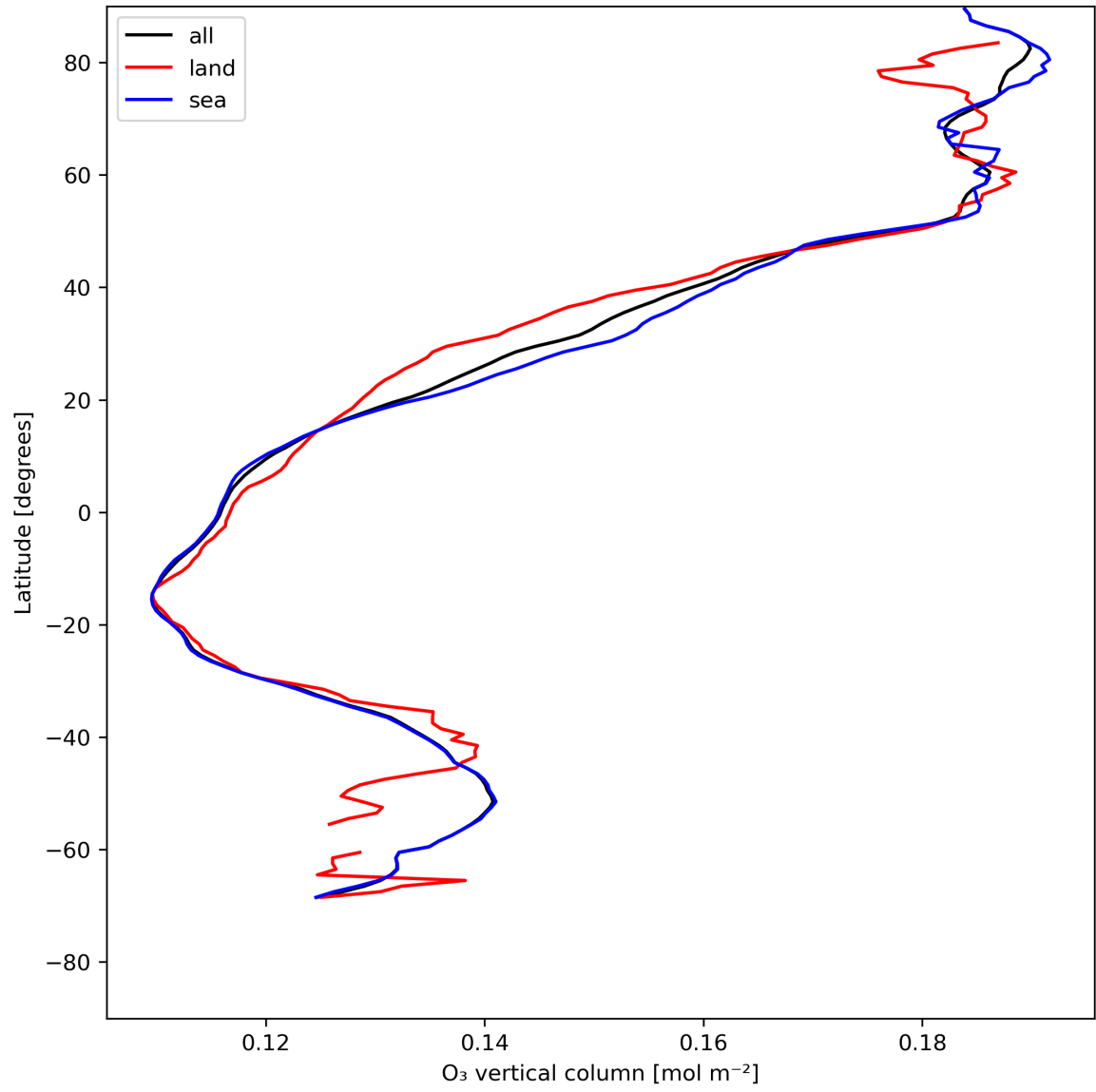
Figure 14: Zonal average of “O 3 vertical column” for 2024-05-18 to 2024-05-20.
