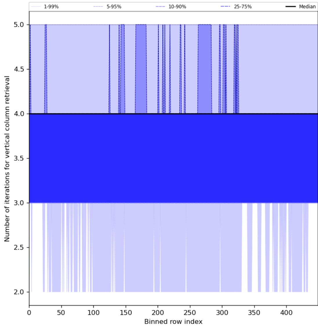
Figure 33: Along track statistics of “Number of iterations for vertical column retrieval” for 2024-05-18 to 2024-05-20
