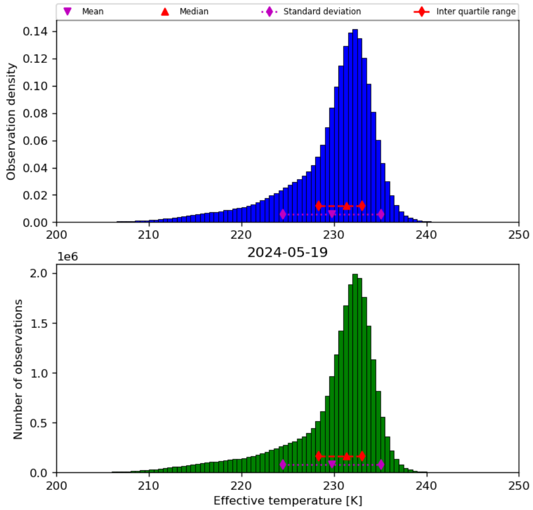
Figure 24: Histogram of “Effective temperature” for 2024-05-18 to 2024-05-20
