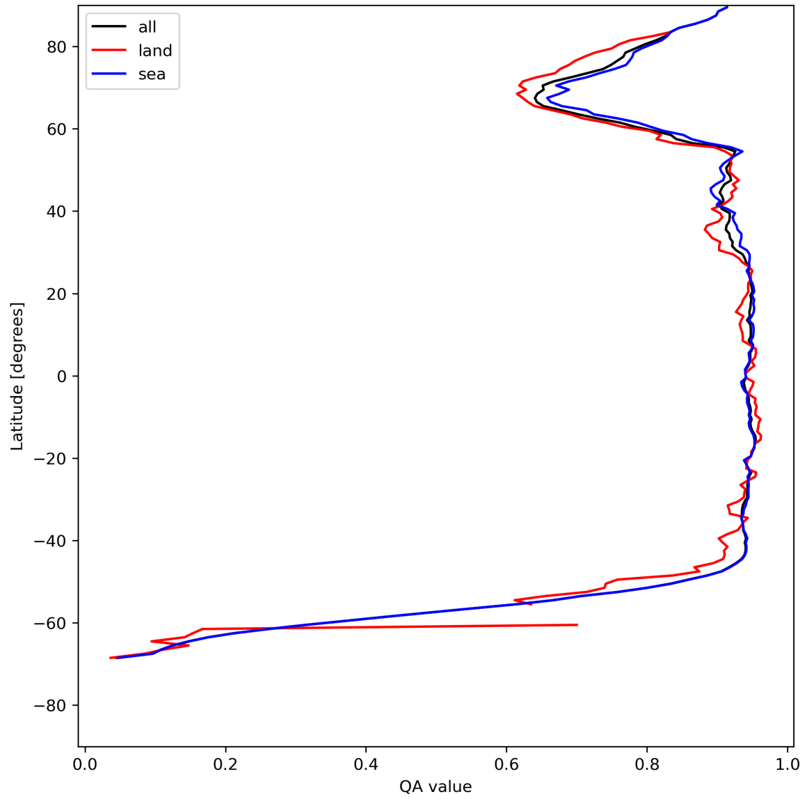
Figure 13: Zonal average of “QA value” for 2024-05-18 to 2024-05-20.
