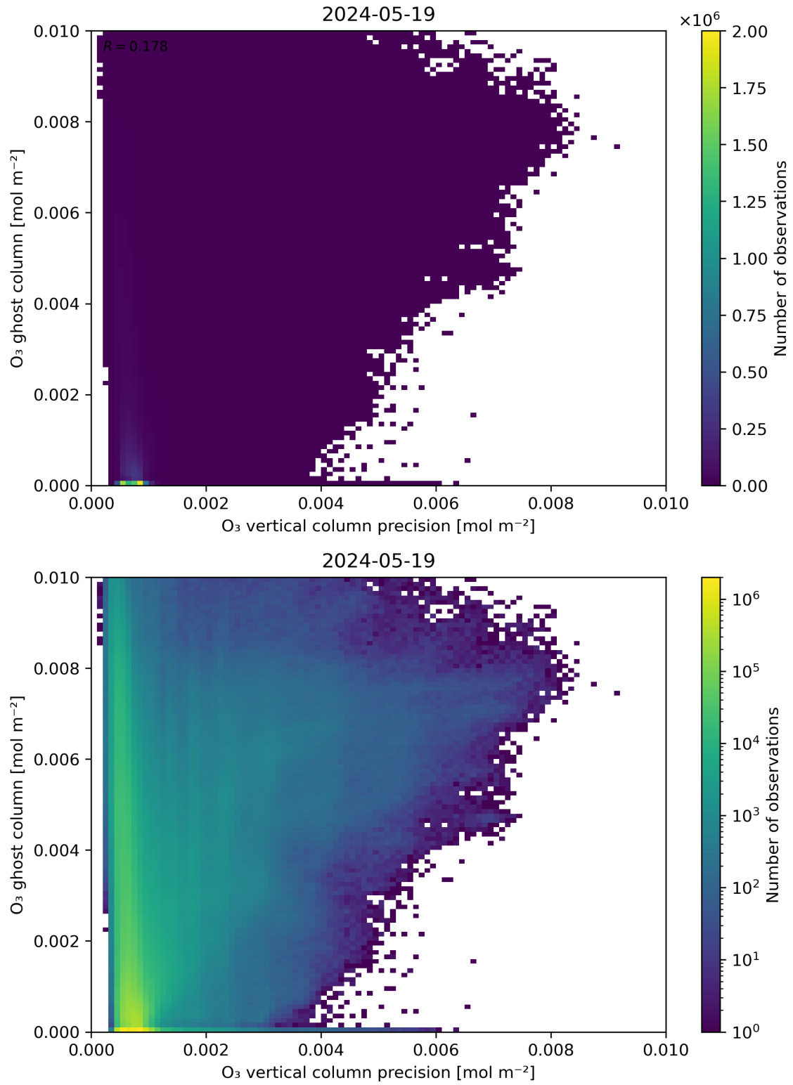
Figure 43: Scatter density plot of “O 3 vertical column precision” against “O 3 ghost column” for 2024-05-18 to 2024-05-20.
