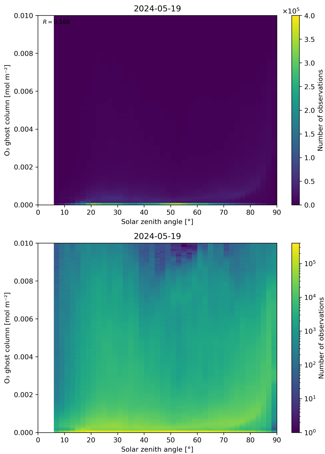
Figure 46: Scatter density plot of “Solar zenith angle” against “O 3 ghost column” for 2024-05-18 to 2024-05-20.
