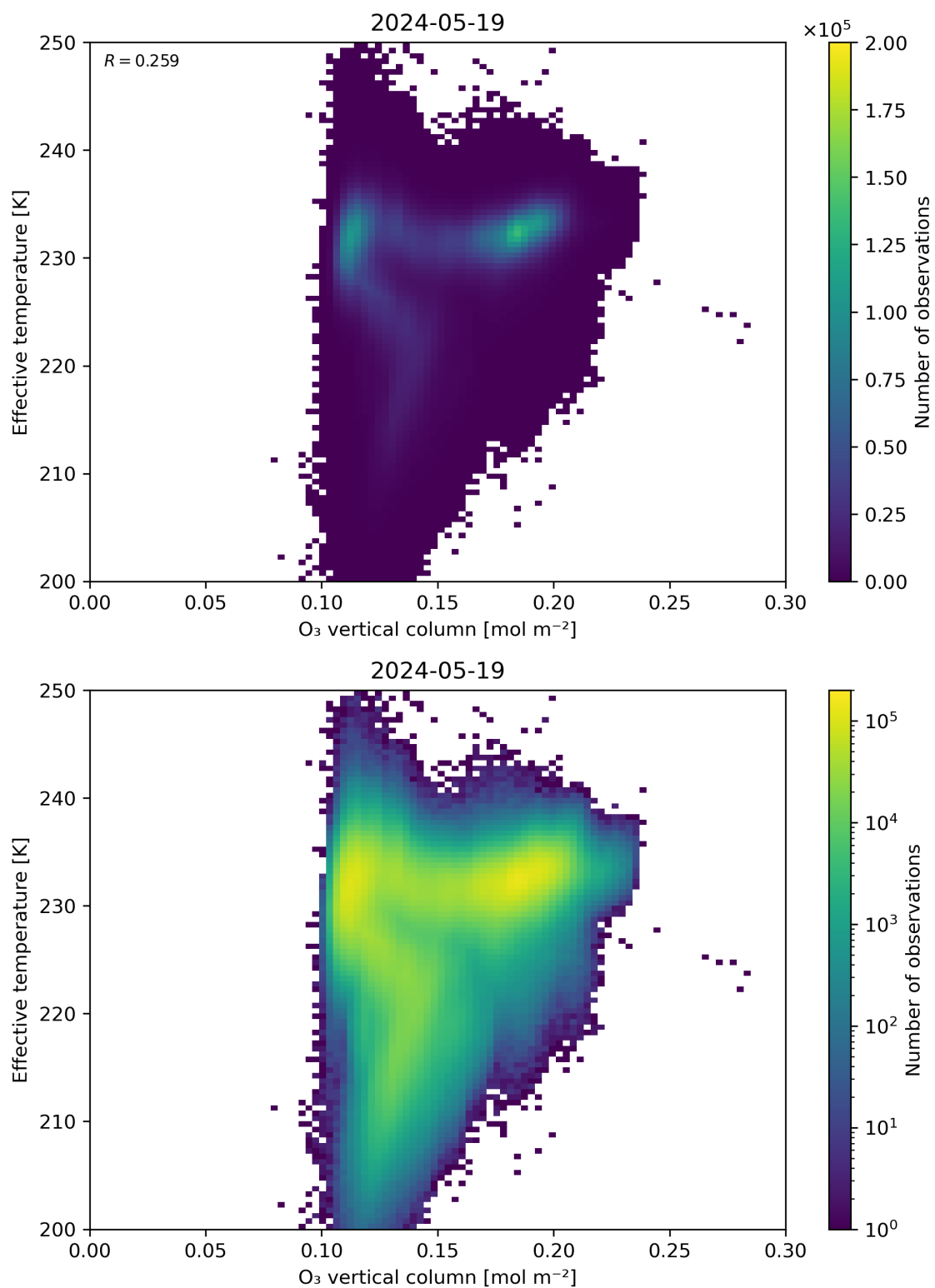
Figure 39: Scatter density plot of “O 3 vertical column” against “Effective temperature” for 2024-05-18 to 2024-05-20.
