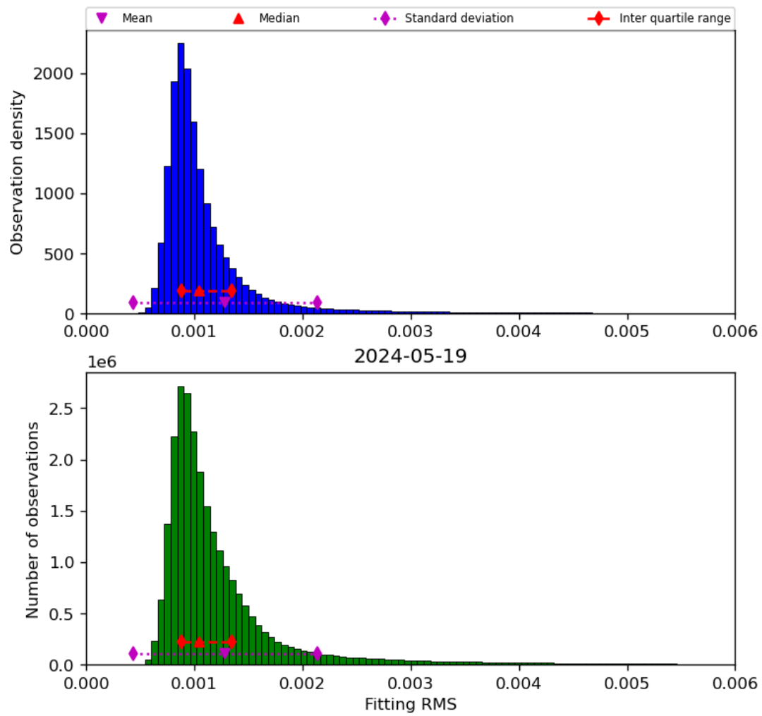
Figure 23: Histogram of “Fitting RMS” for 2024-05-18 to 2024-05-20
