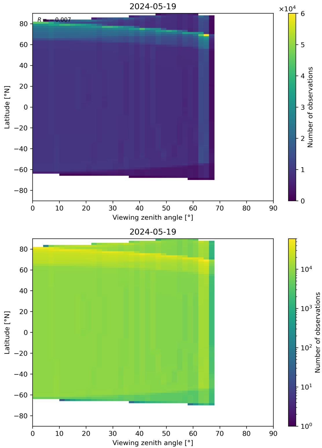
Figure 49: Scatter density plot of “Viewing zenith angle” against “Latitude” for 2024-05-18 to 2024-05-20.
