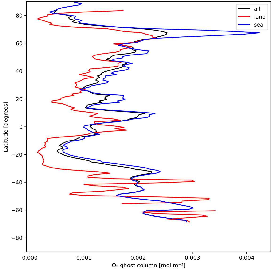
Figure 18: Zonal average of "O 3 ghost column" for 2024-05-19 to 2024-05-21.
