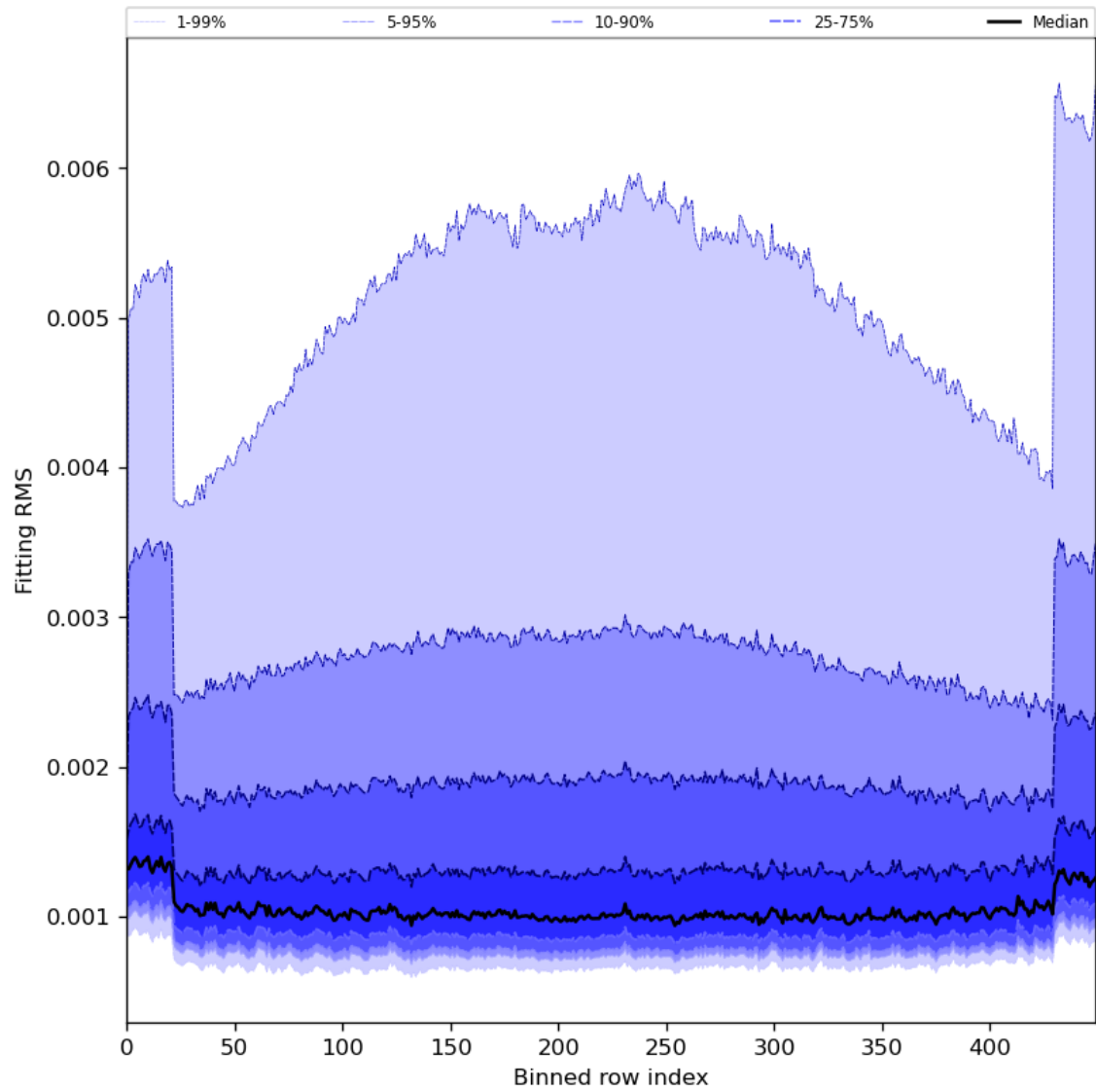
Figure 30: Along track statistics of “Fitting RMS” for 2024-05-19 to 2024-05-21
