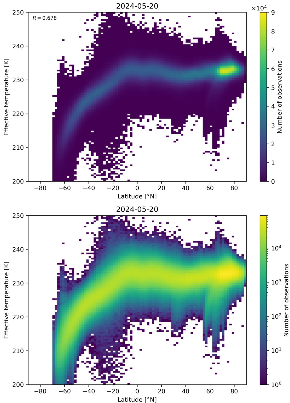
Figure 34: Scatter density plot of “Latitude” against “Effective temperature” for 2024-05-19 to 2024-05-21.
