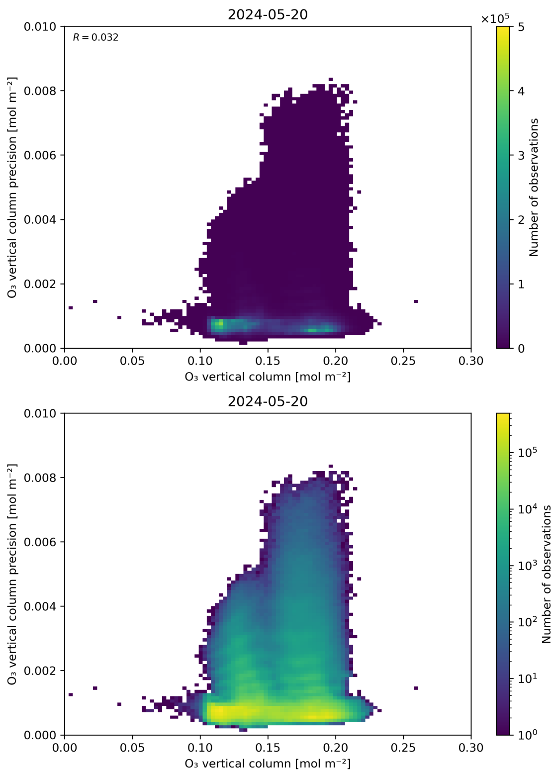
Figure 41: Scatter density plot of “O 3 vertical column” against “O 3 vertical column precision” for 2024-05-19 to 2024-05-21.
