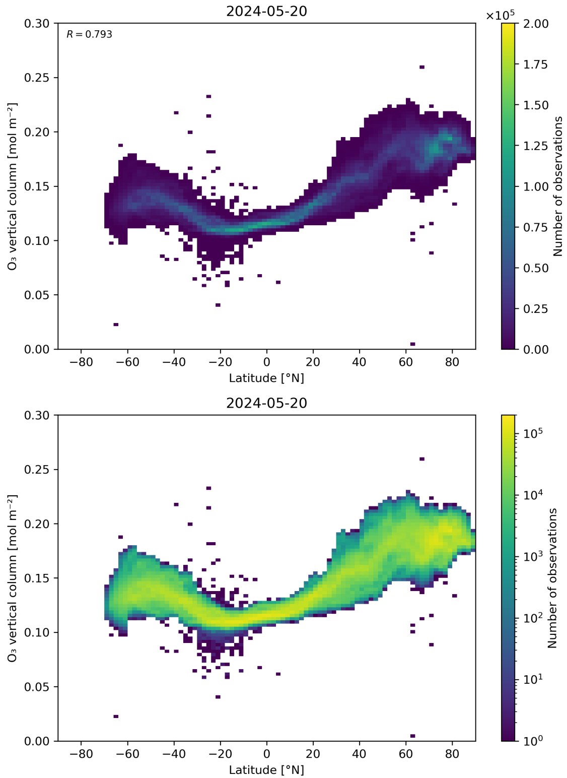
Figure 36: Scatter density plot of “Latitude” against “O 3 vertical column” for 2024-05-19 to 2024-05-21.
