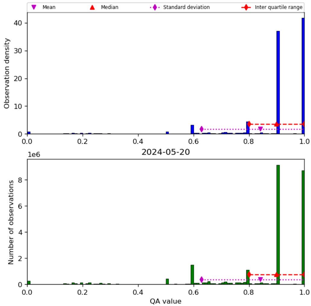
Figure 20: Histogram of “QA value” for 2024-05-19 to 2024-05-21
