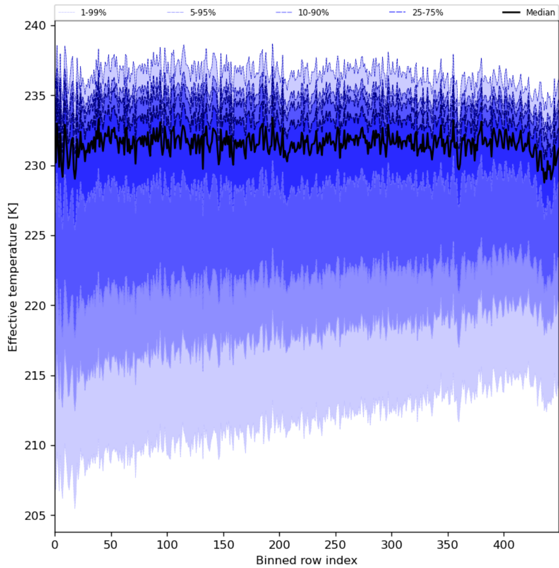
Figure 31: Along track statistics of “Effective temperature” for 2024-05-19 to 2024-05-21
