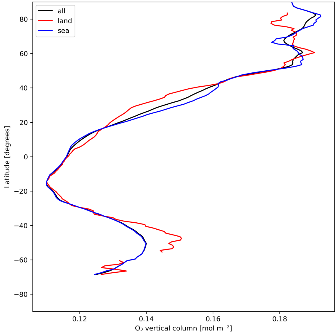
Figure 14: Zonal average of “O 3 vertical column” for 2024-05-19 to 2024-05-21.
