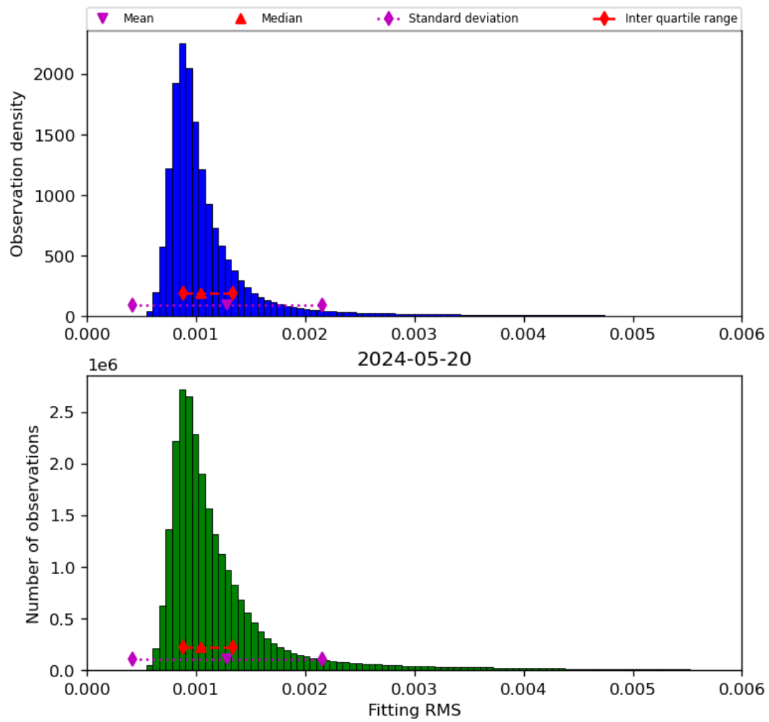
Figure 23: Histogram of “Fitting RMS” for 2024-05-19 to 2024-05-21
