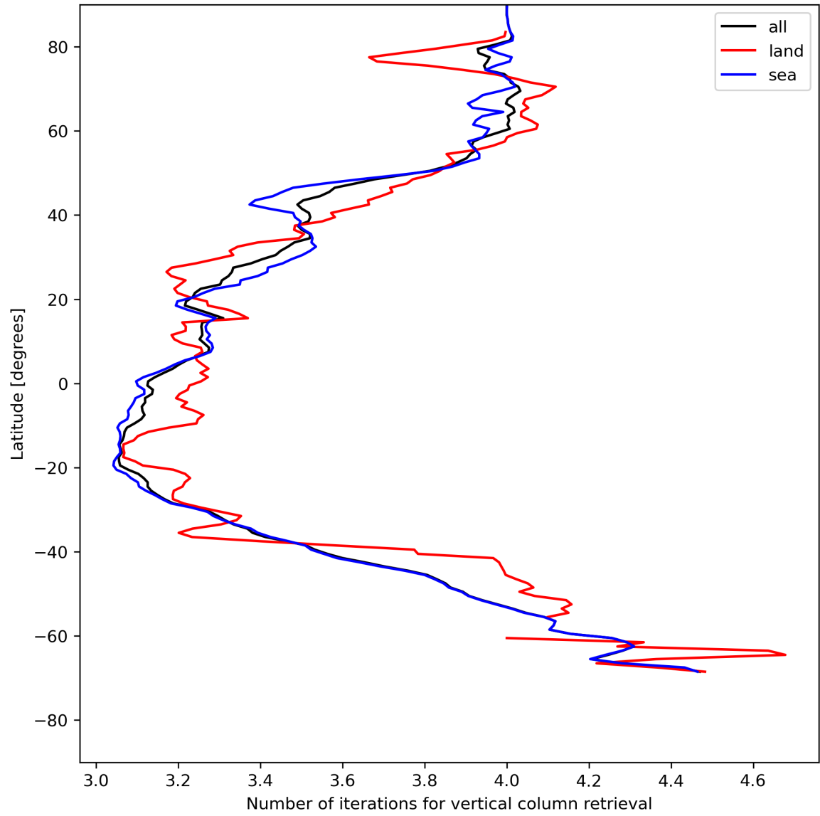
Figure 19: Zonal average of “Number of iterations for vertical column retrieval” for 2024-05-19 to 2024-05-21.
