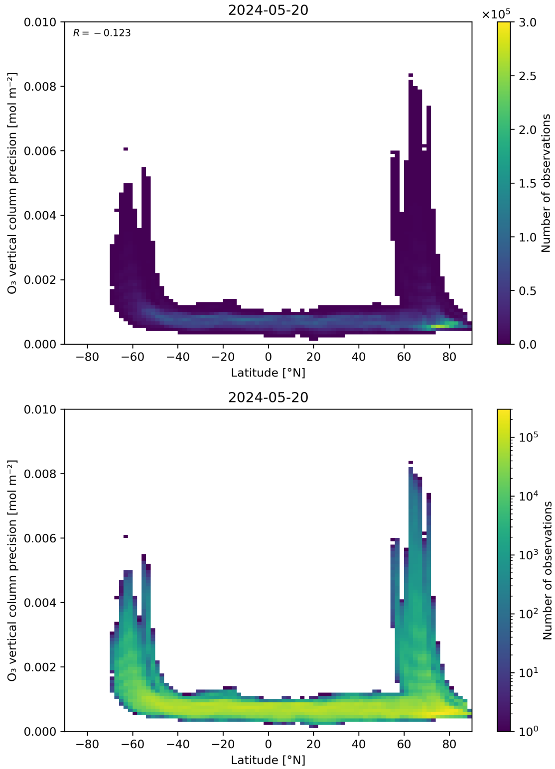
Figure 37: Scatter density plot of “Latitude” against “O 3 vertical column precision” for 2024-05-19 to 2024-05-21.
