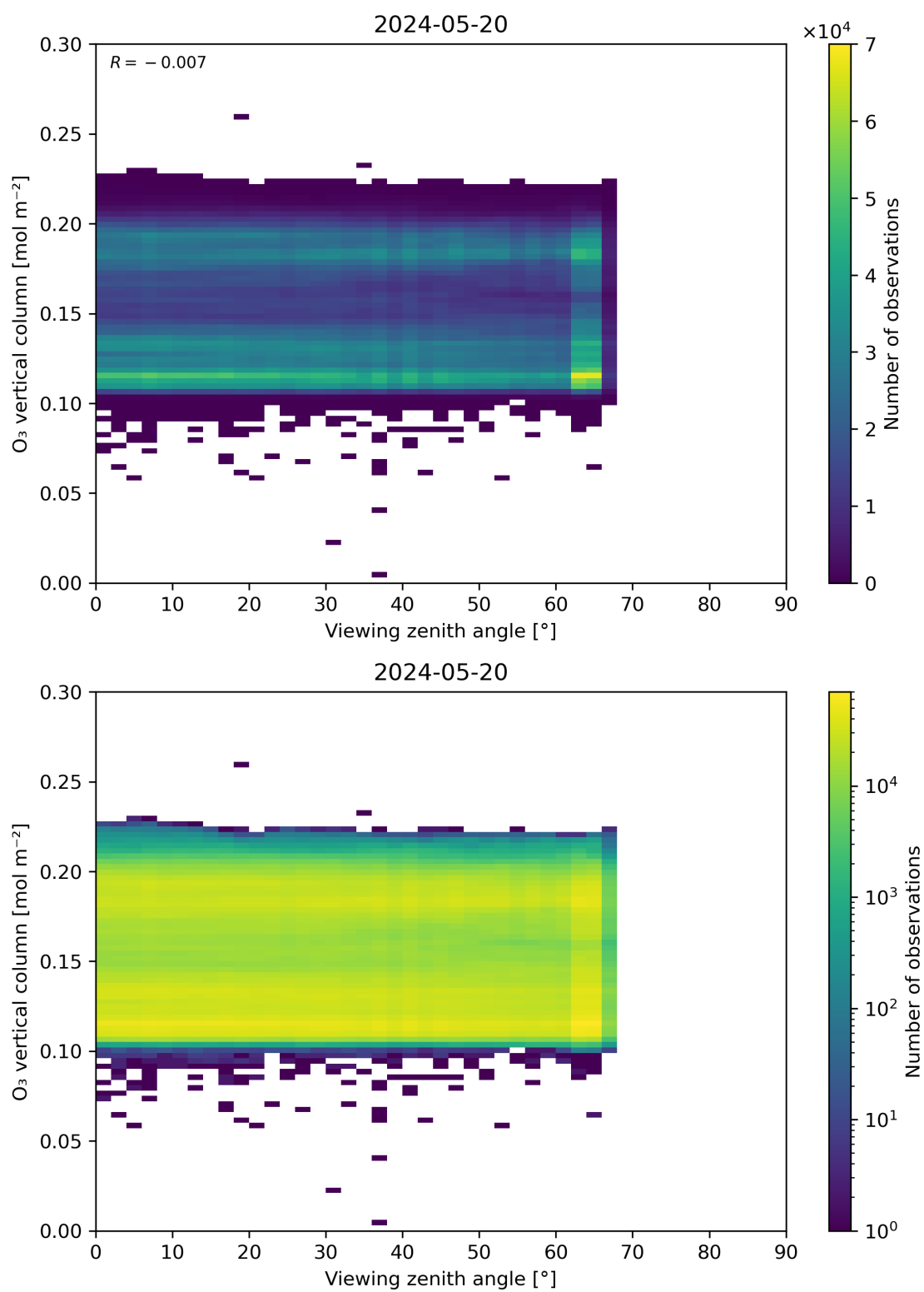
Figure 52: Scatter density plot of “Viewing zenith angle” against “O 3 vertical column” for 2024-05-19 to 2024-05-21.
