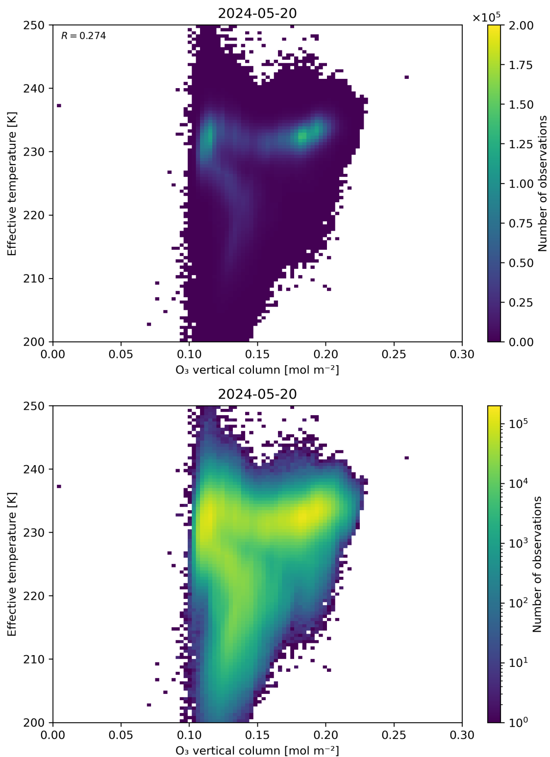
Figure 39: Scatter density plot of “O 3 vertical column” against “Effective temperature” for 2024-05-19 to 2024-05-21.
