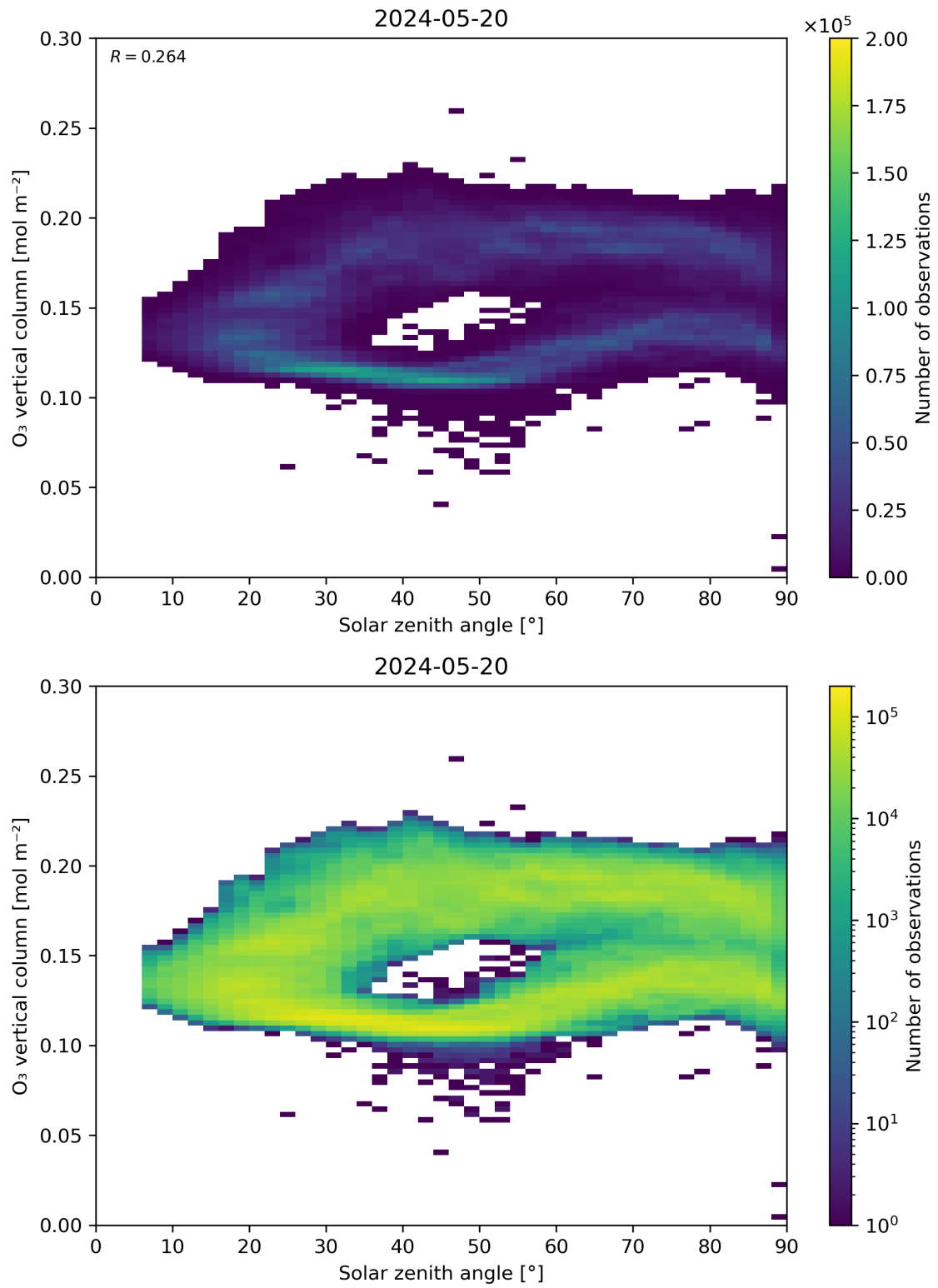
Figure 47: Scatter density plot of “Solar zenith angle” against “O 3 vertical column” for 2024-05-19 to 2024-05-21.
