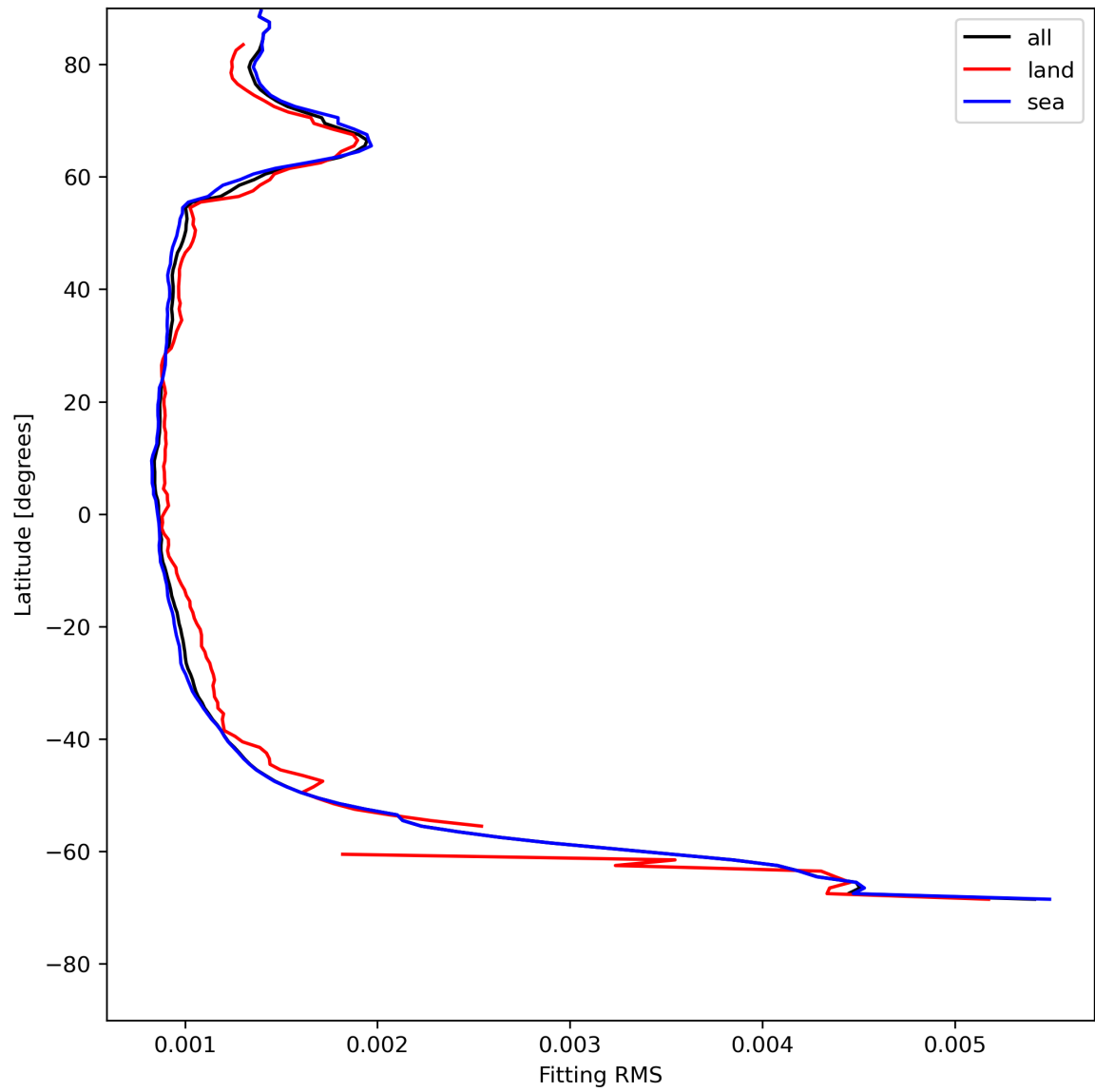
Figure 16: Zonal average of “Fitting RMS” for 2024-05-19 to 2024-05-21.
