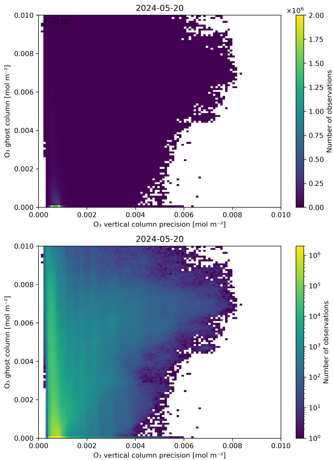
Figure 43: Scatter density plot of “ \text{O}_3 vertical column precision” against “ \text{O}_3 ghost column” for 2024-05-19 to 2024-05-21.
