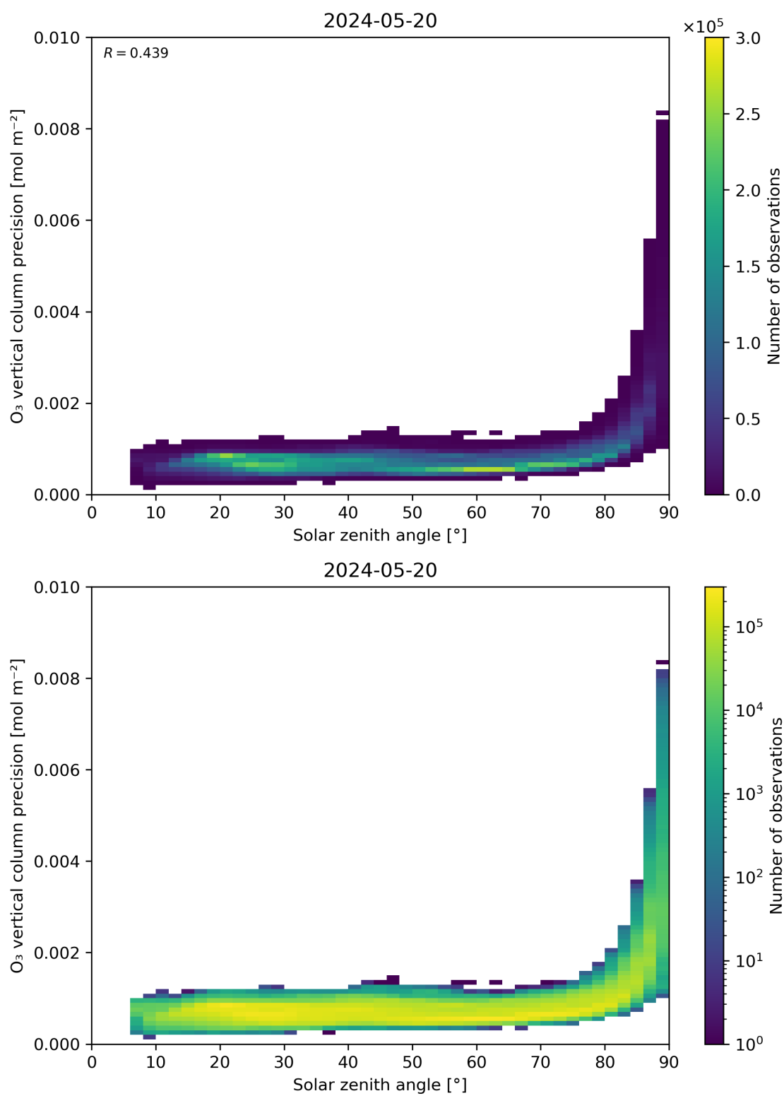
Figure 48: Scatter density plot of “Solar zenith angle” against “O 3 vertical column precision” for 2024-05-19 to 2024-05-21.
