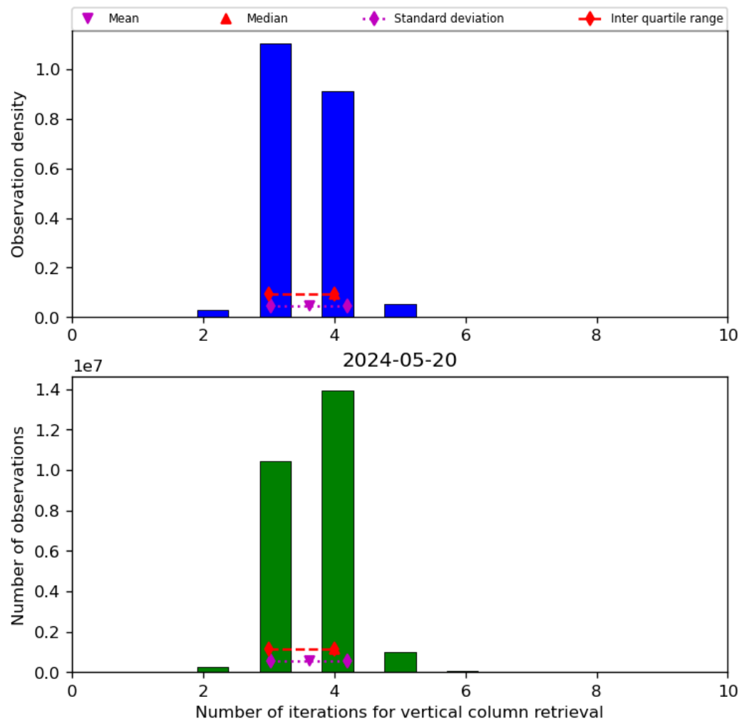
Figure 26: Histogram of “Number of iterations for vertical column retrieval” for 2024-05-19 to 2024-05-21
