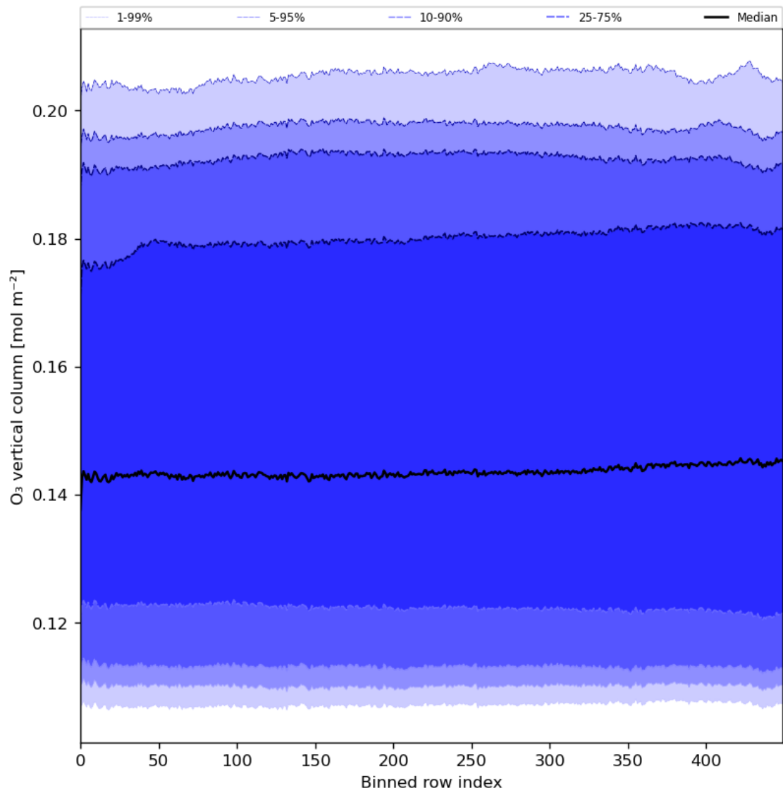
Figure 28: Along track statistics of “O 3 vertical column” for 2024-05-19 to 2024-05-21
