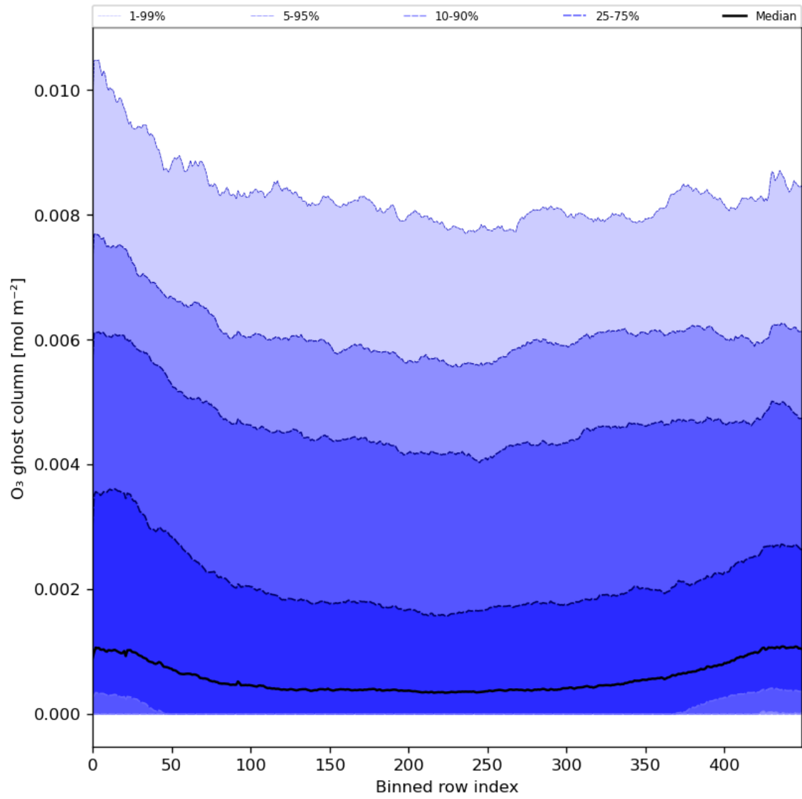
Figure 32: Along track statistics of “O 3 ghost column” for 2024-05-19 to 2024-05-21
