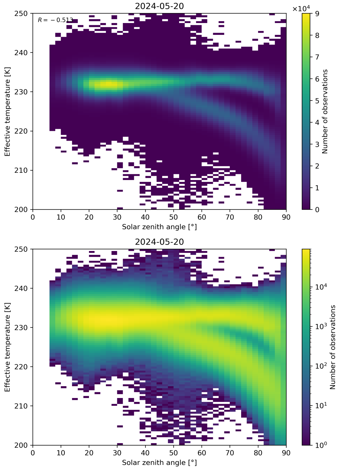
Figure 45: Scatter density plot of “Solar zenith angle” against “Effective temperature” for 2024-05-19 to 2024-05-21.
