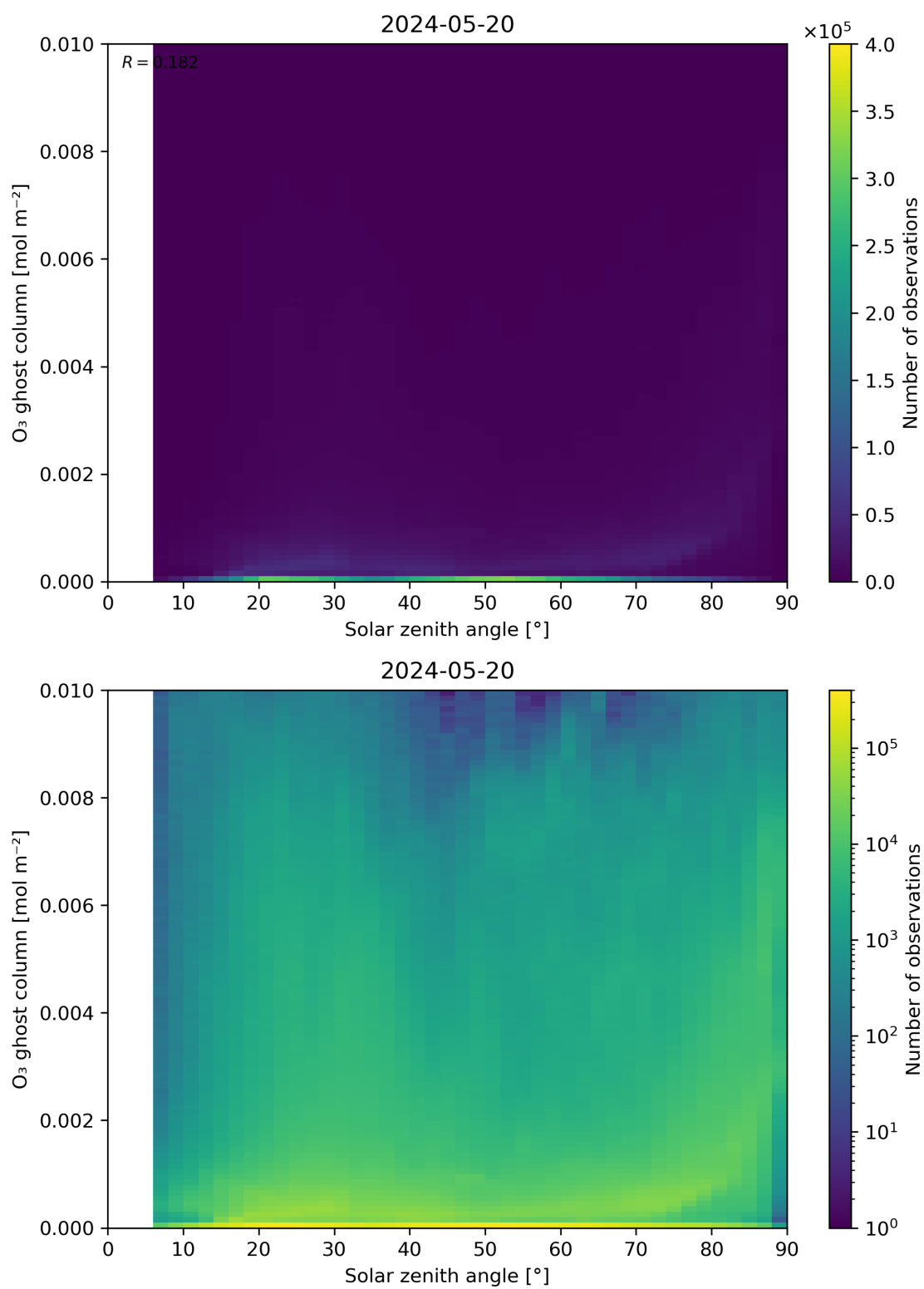
Figure 46: Scatter density plot of “Solar zenith angle” against “O 3 ghost column” for 2024-05-19 to 2024-05-21.
