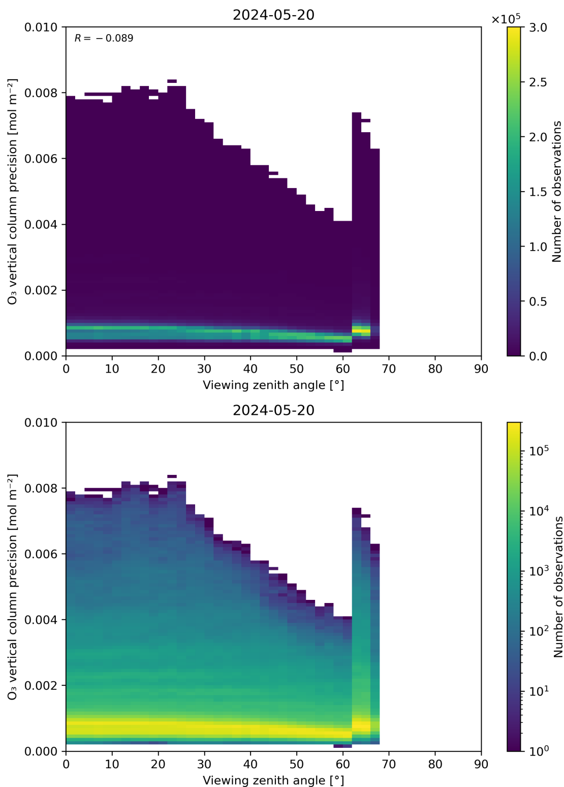
Figure 53: Scatter density plot of “Viewing zenith angle” against “O 3 vertical column precision” for 2024-05-19 to 2024-05-21.
