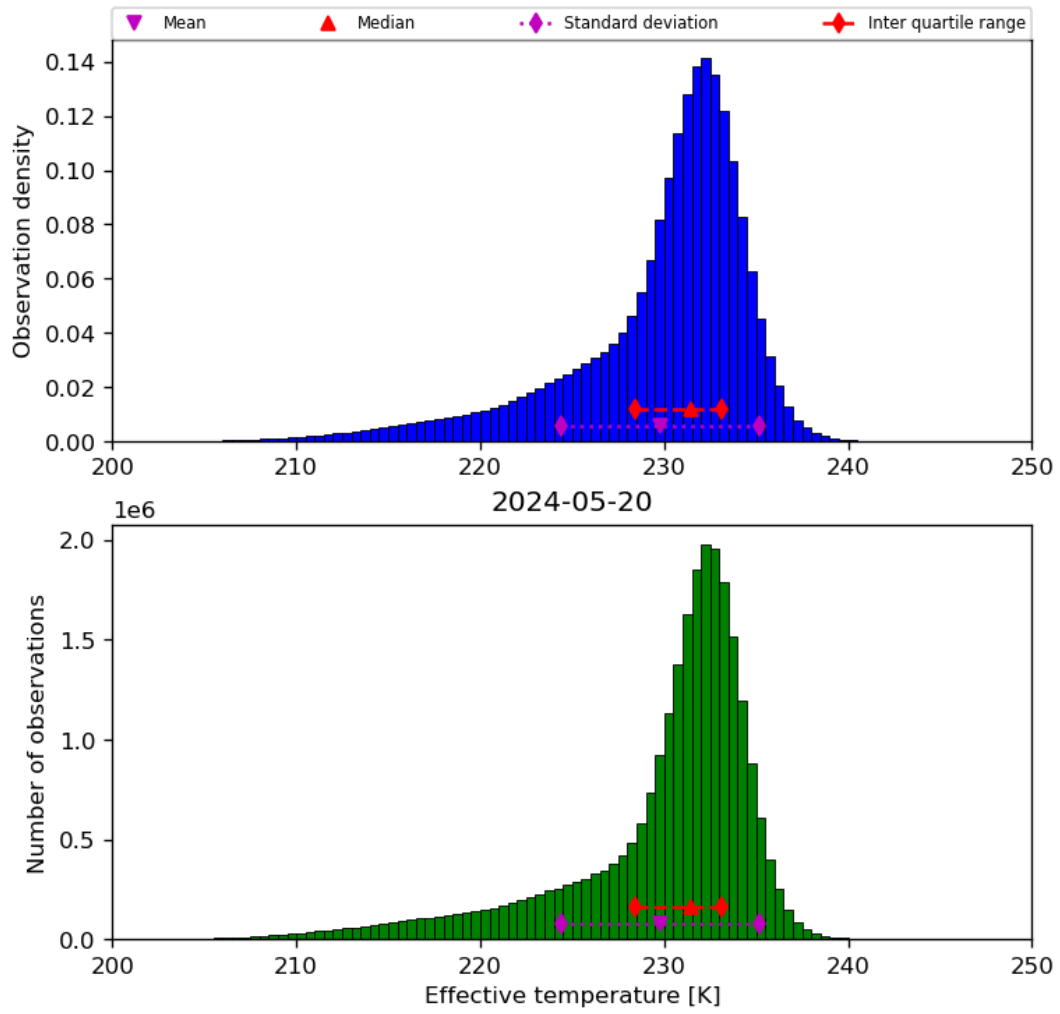
Figure 24: Histogram of “Effective temperature” for 2024-05-19 to 2024-05-21
