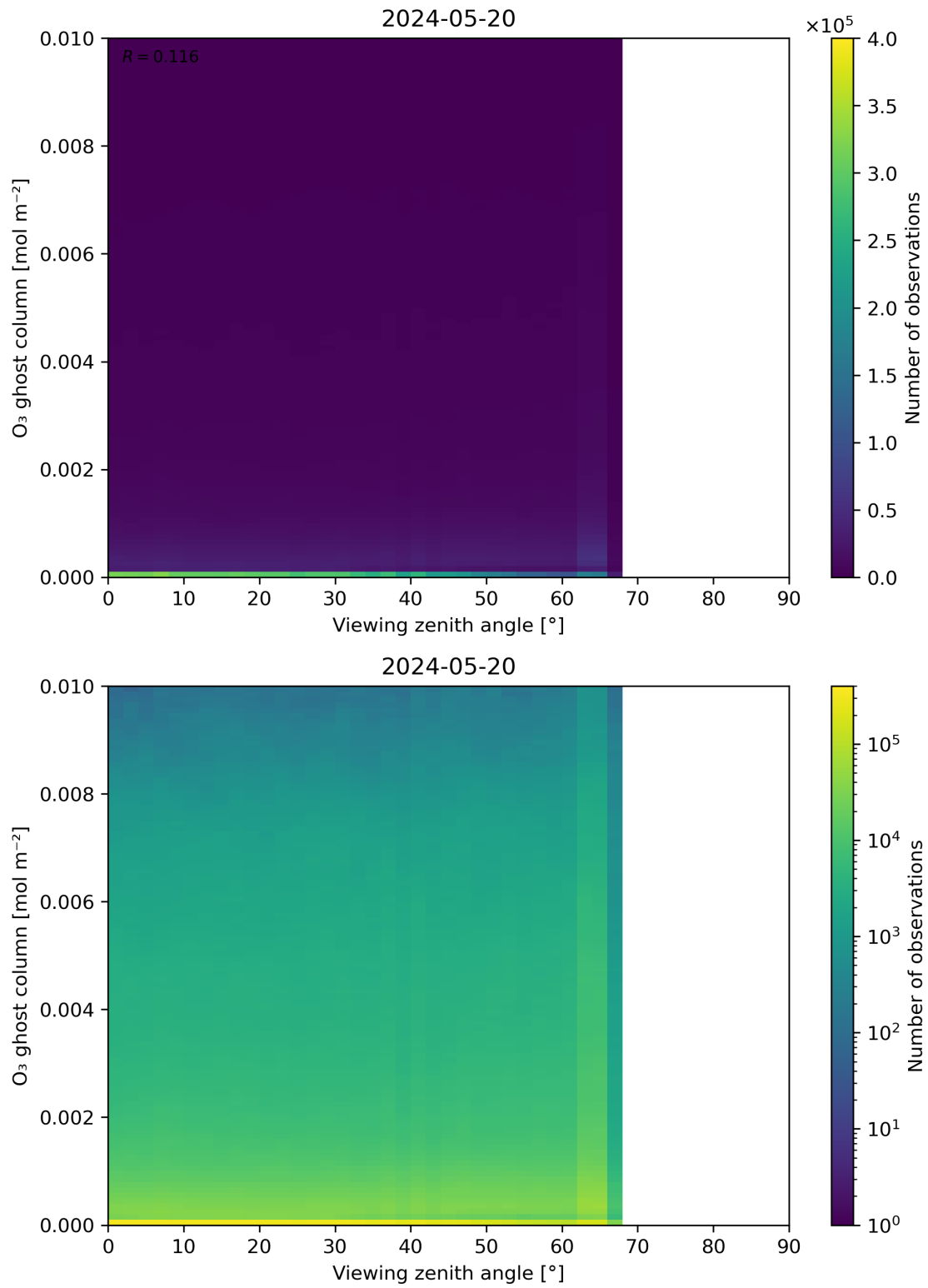
Figure 51: Scatter density plot of “Viewing zenith angle” against “O 3 ghost column” for 2024-05-19 to 2024-05-21.
