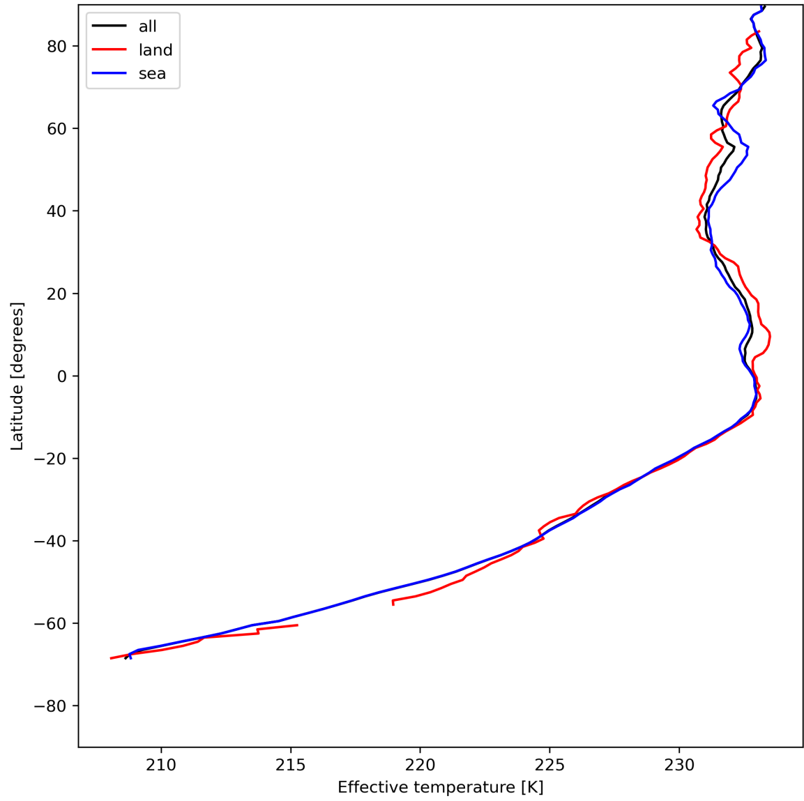
Figure 17: Zonal average of "Effective temperature" for 2024-05-19 to 2024-05-21.
