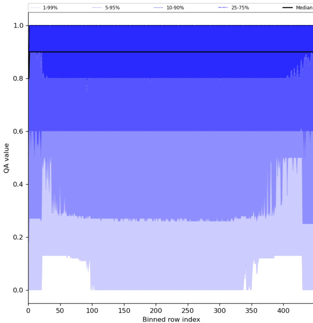
Figure 27: Along track statistics of “QA value” for 2024-05-19 to 2024-05-21
