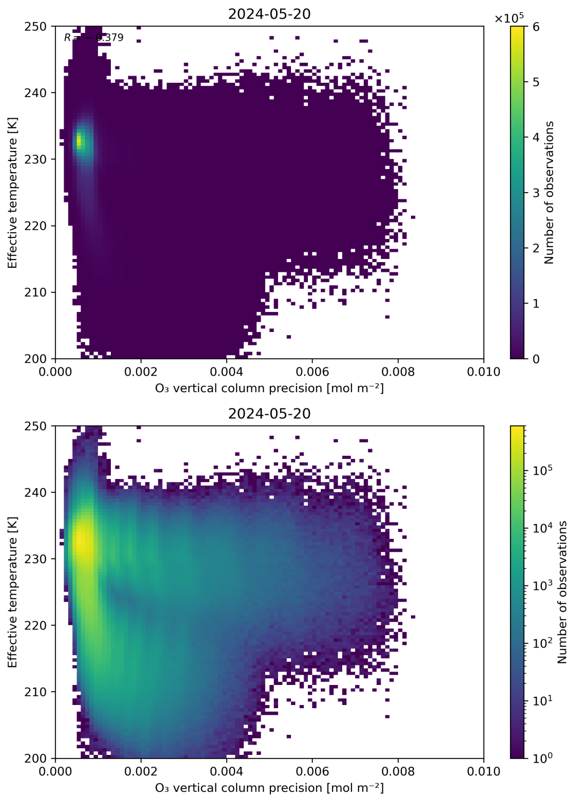
Figure 42: Scatter density plot of “O 3 vertical column precision” against “Effective temperature” for 2024-05-19 to 2024-05-21.
