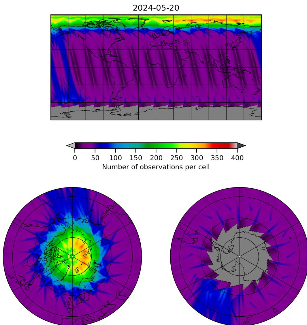
Figure 12: Map of the number of observations for 2024-05-19 to 2024-05-21
