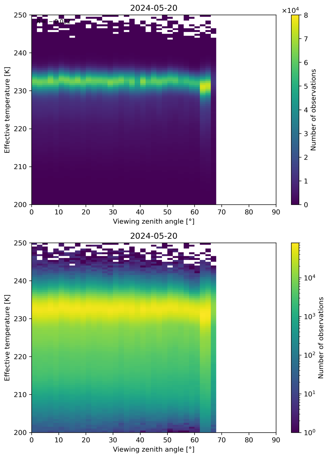
Figure 50: Scatter density plot of “Viewing zenith angle” against “Effective temperature” for 2024-05-19 to 2024-05-21.
