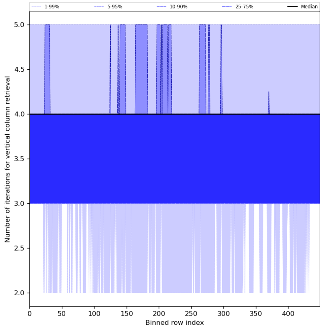
Figure 33: Along track statistics of “Number of iterations for vertical column retrieval” for 2024-05-19 to 2024-05-21
