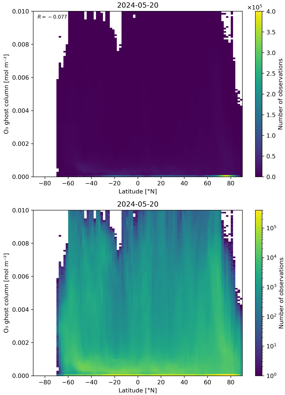
Figure 35: Scatter density plot of “Latitude” against “O 3 ghost column” for 2024-05-19 to 2024-05-21.
