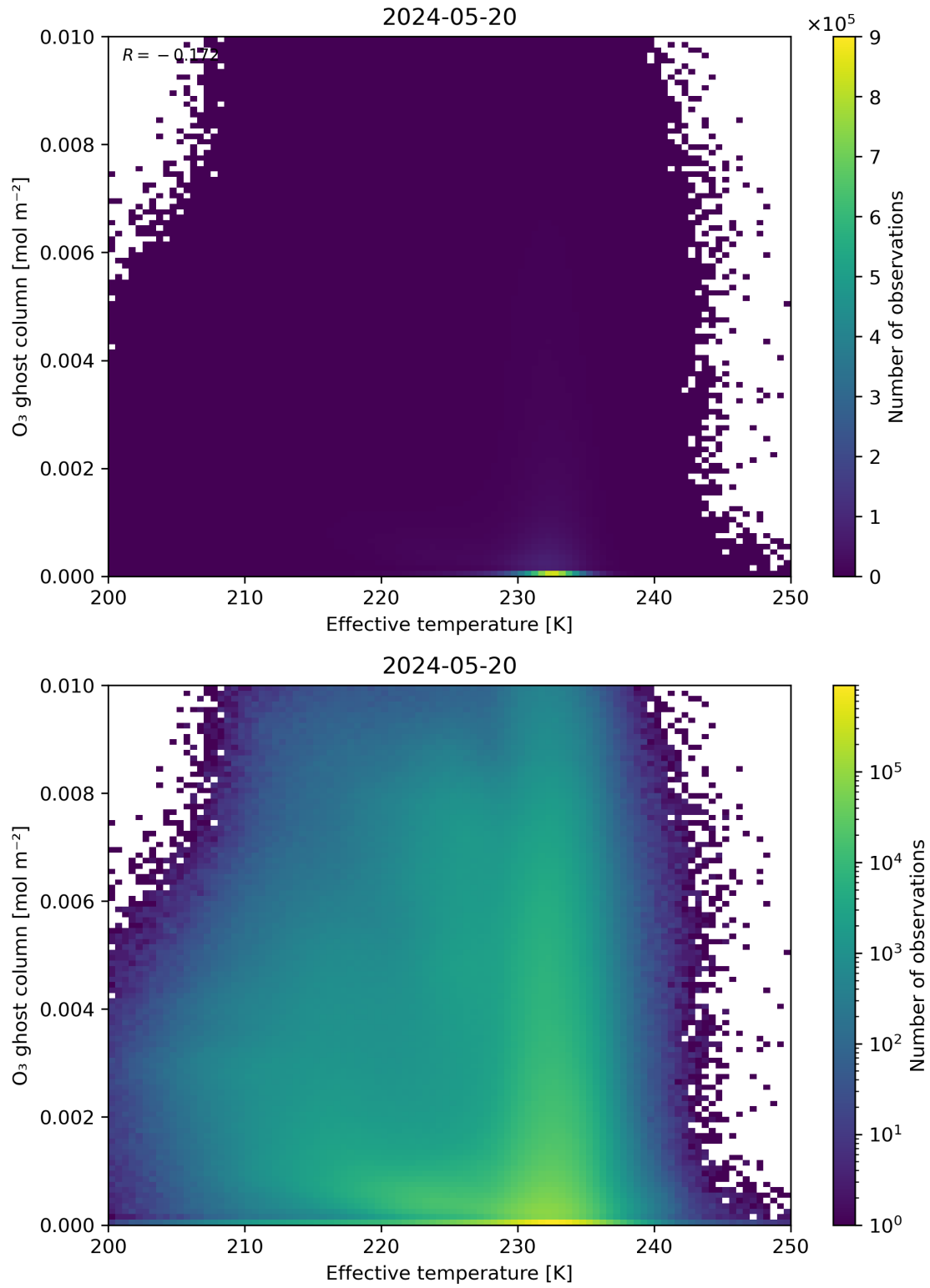
Figure 38: Scatter density plot of “Effective temperature” against “O 3 ghost column” for 2024-05-19 to 2024-05-21.
