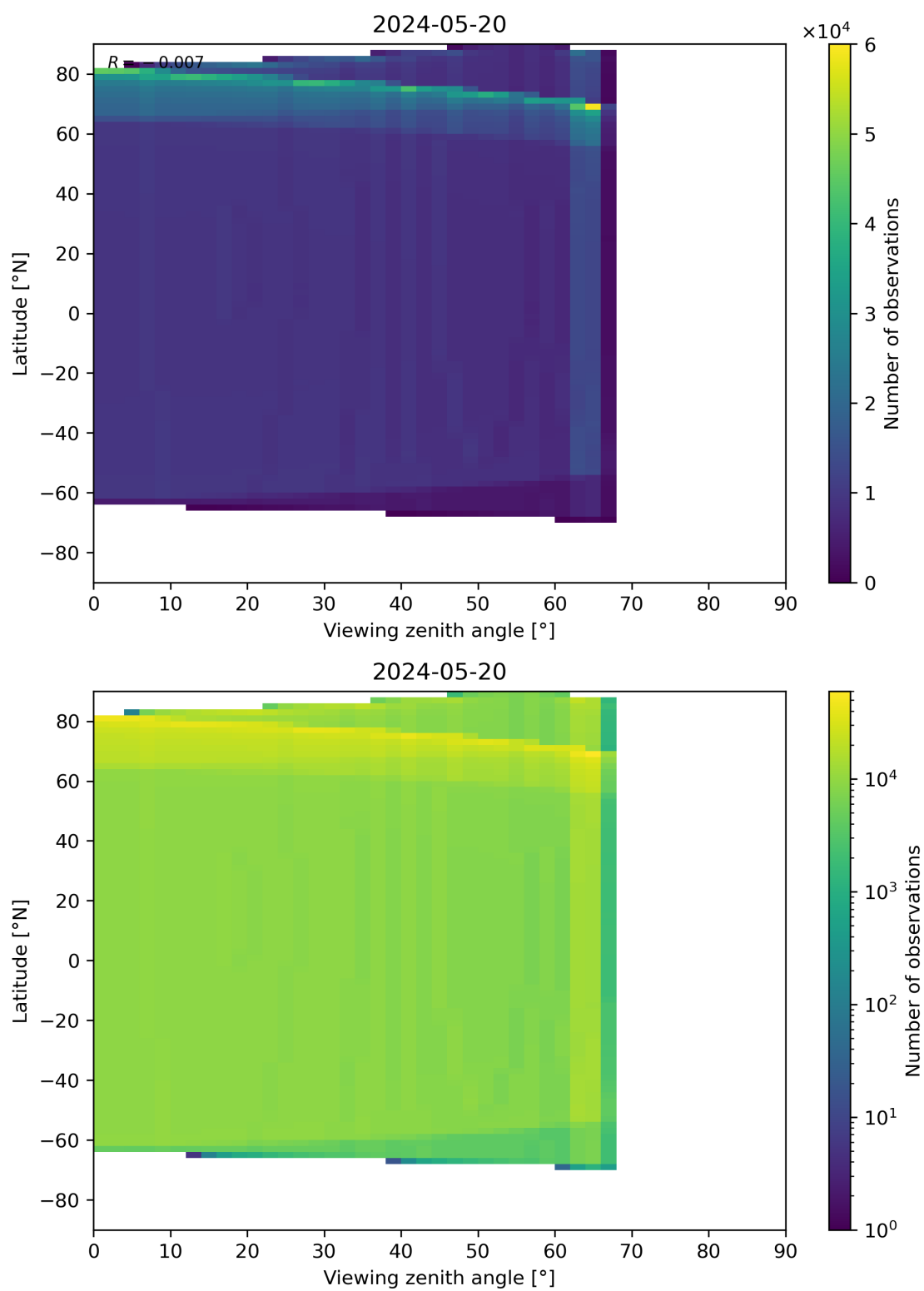
Figure 49: Scatter density plot of “Viewing zenith angle” against “Latitude” for 2024-05-19 to 2024-05-21.
