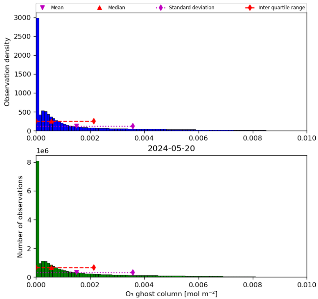
Figure 25: Histogram of “O 3 ghost column” for 2024-05-19 to 2024-05-21
