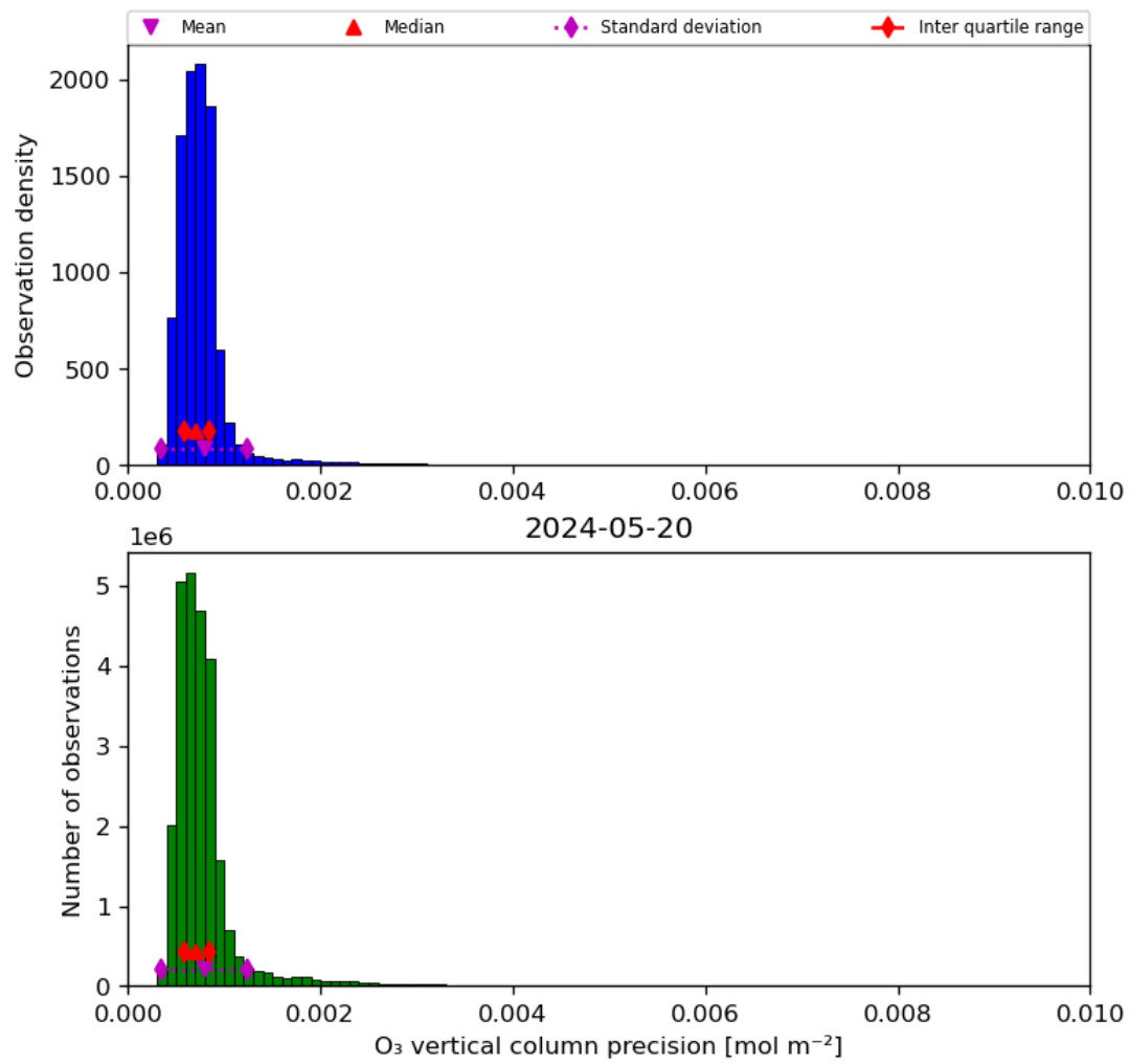
Figure 22: Histogram of “O 3 vertical column precision” for 2024-05-19 to 2024-05-21
