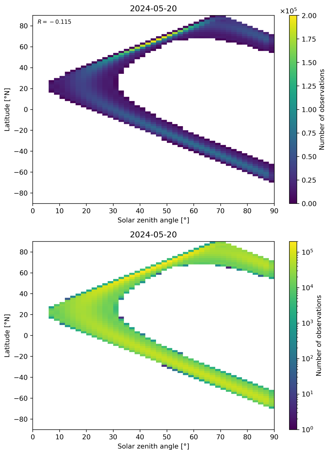
Figure 44: Scatter density plot of “Solar zenith angle” against “Latitude” for 2024-05-19 to 2024-05-21.
