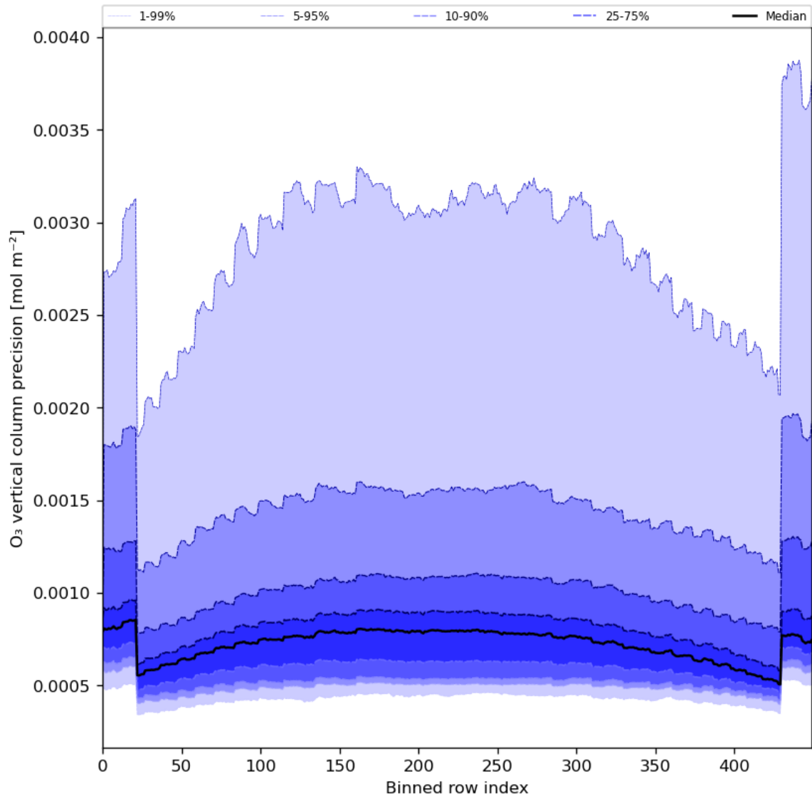
Figure 29: Along track statistics of “O 3 vertical column precision” for 2024-05-19 to 2024-05-21
