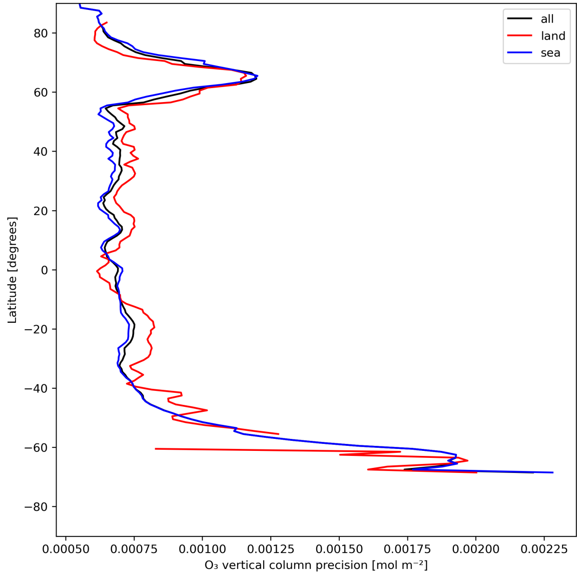
Figure 15: Zonal average of "O 3 vertical column precision" for 2024-05-19 to 2024-05-21.
