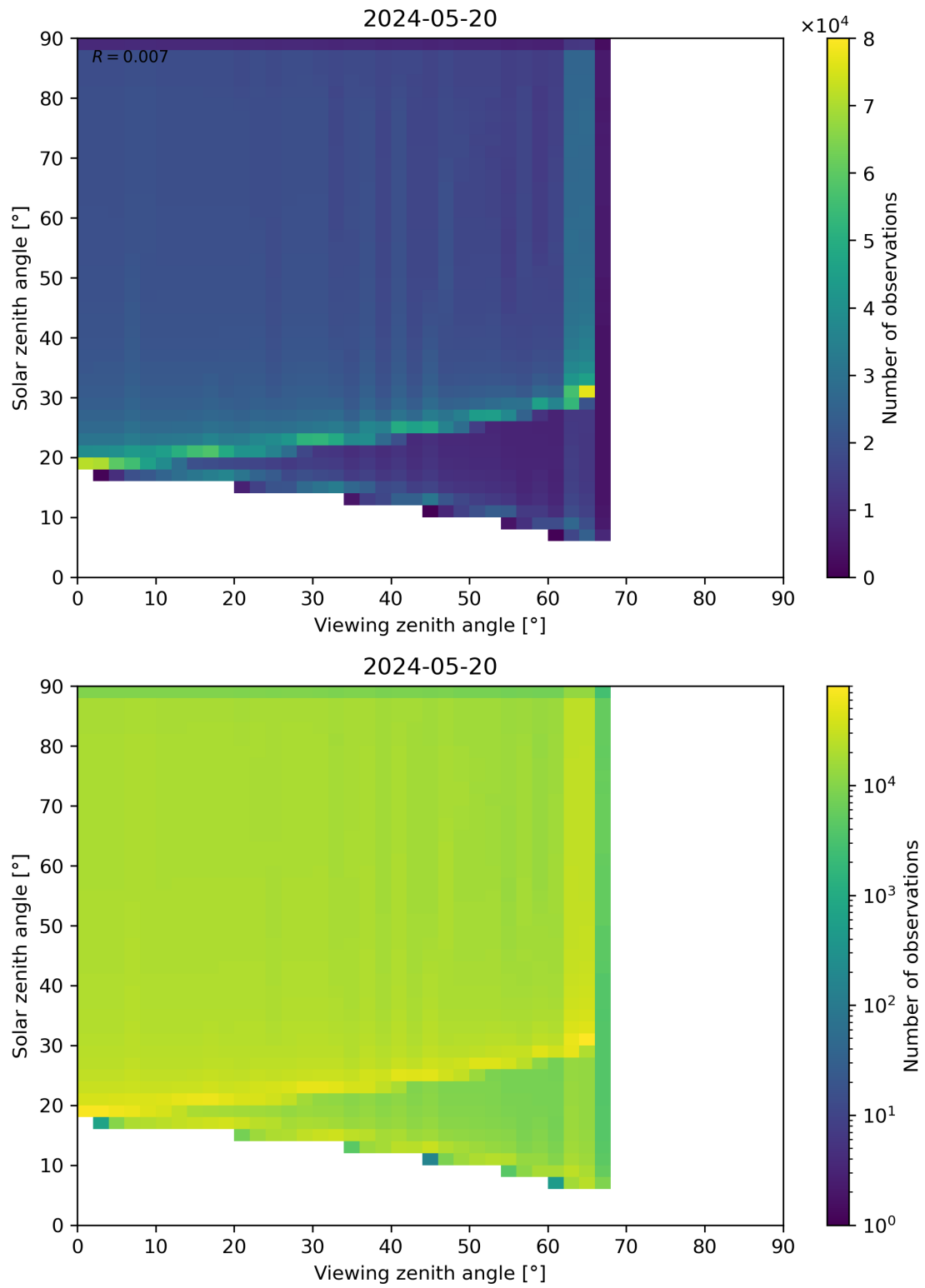
Figure 54: Scatter density plot of “Viewing zenith angle” against “Solar zenith angle” for 2024-05-19 to 2024-05-21.
