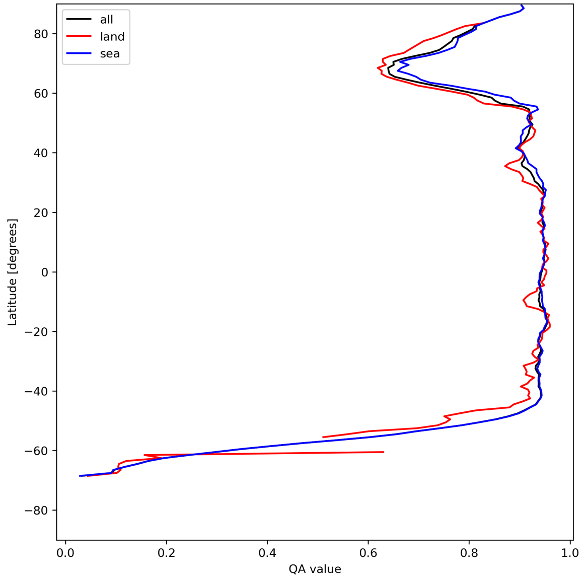
Figure 13: Zonal average of “QA value” for 2024-05-19 to 2024-05-21.
