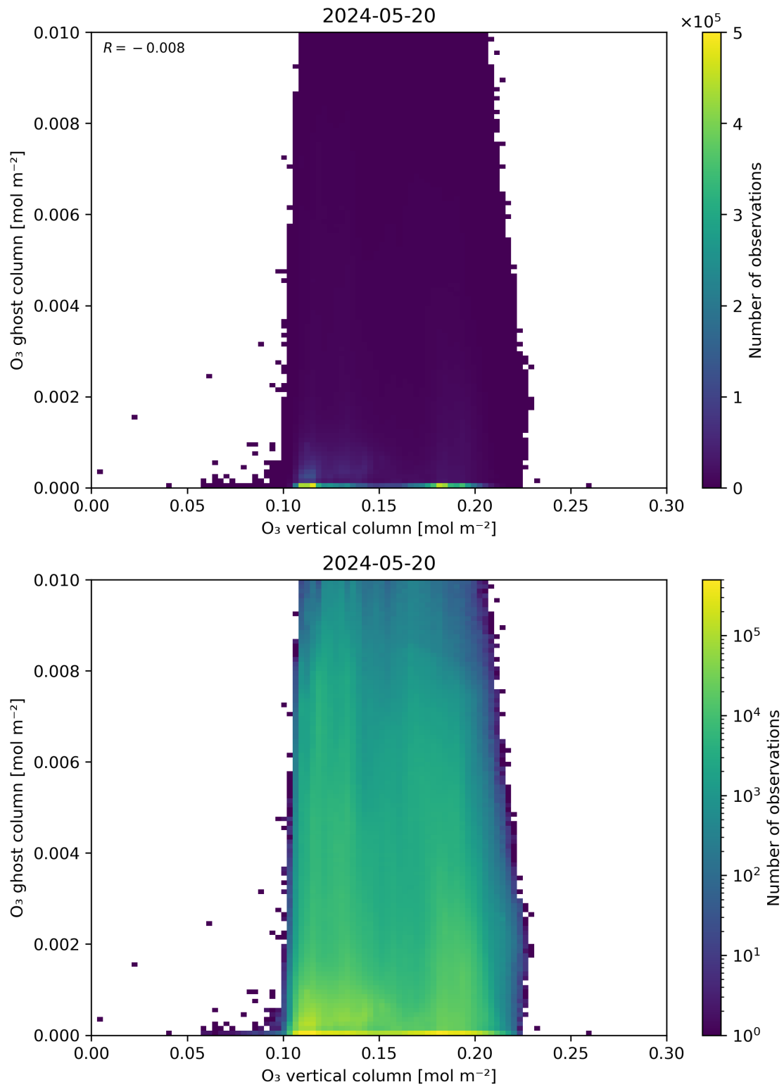
Figure 40: Scatter density plot of “O 3 vertical column” against “O 3 ghost column” for 2024-05-19 to 2024-05-21.
