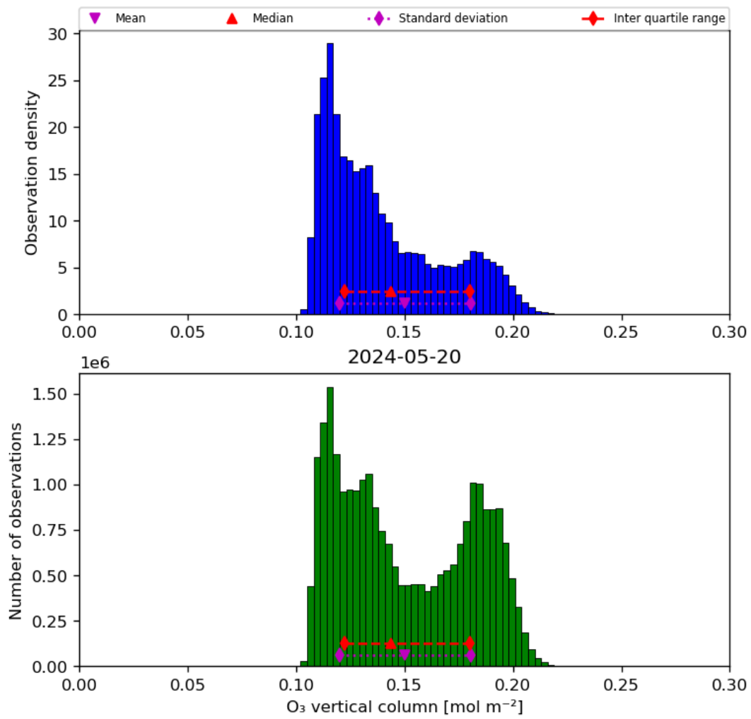
Figure 21: Histogram of “O 3 vertical column” for 2024-05-19 to 2024-05-21
