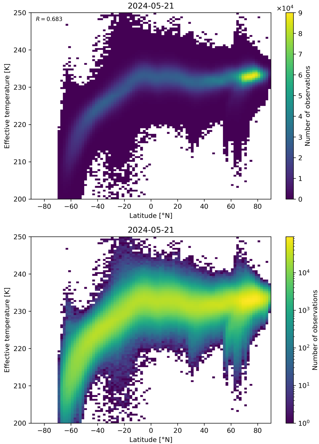
Figure 34: Scatter density plot of “Latitude” against “Effective temperature” for 2024-05-20 to 2024-05-22.
