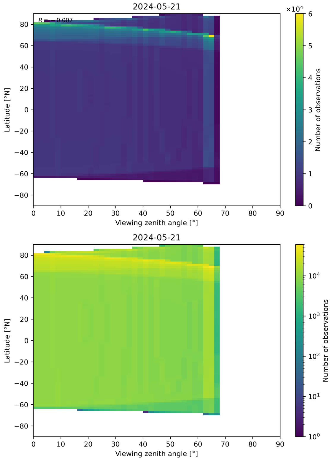
Figure 49: Scatter density plot of “Viewing zenith angle” against “Latitude” for 2024-05-20 to 2024-05-22.
