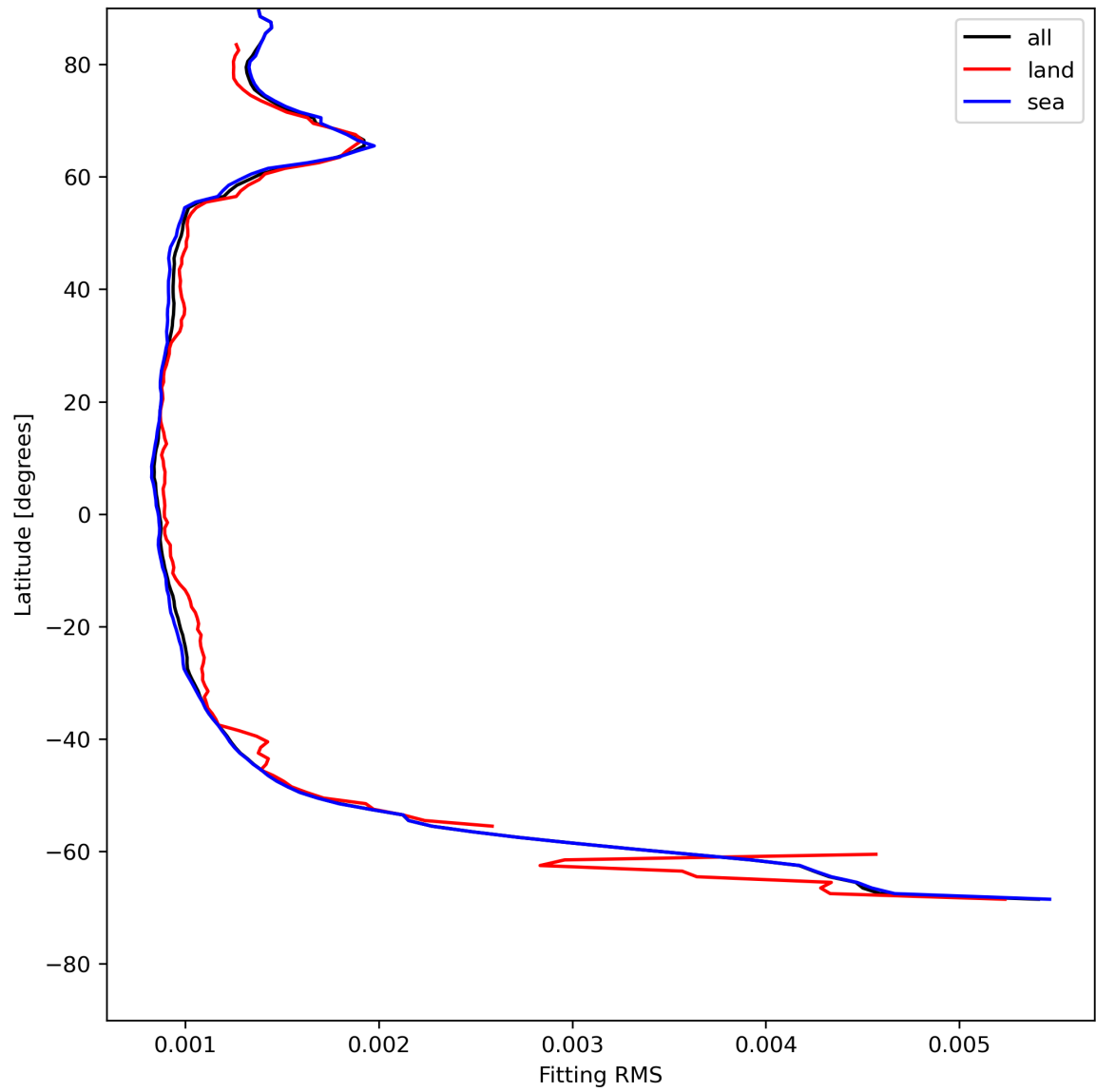
Figure 16: Zonal average of “Fitting RMS” for 2024-05-20 to 2024-05-22.
