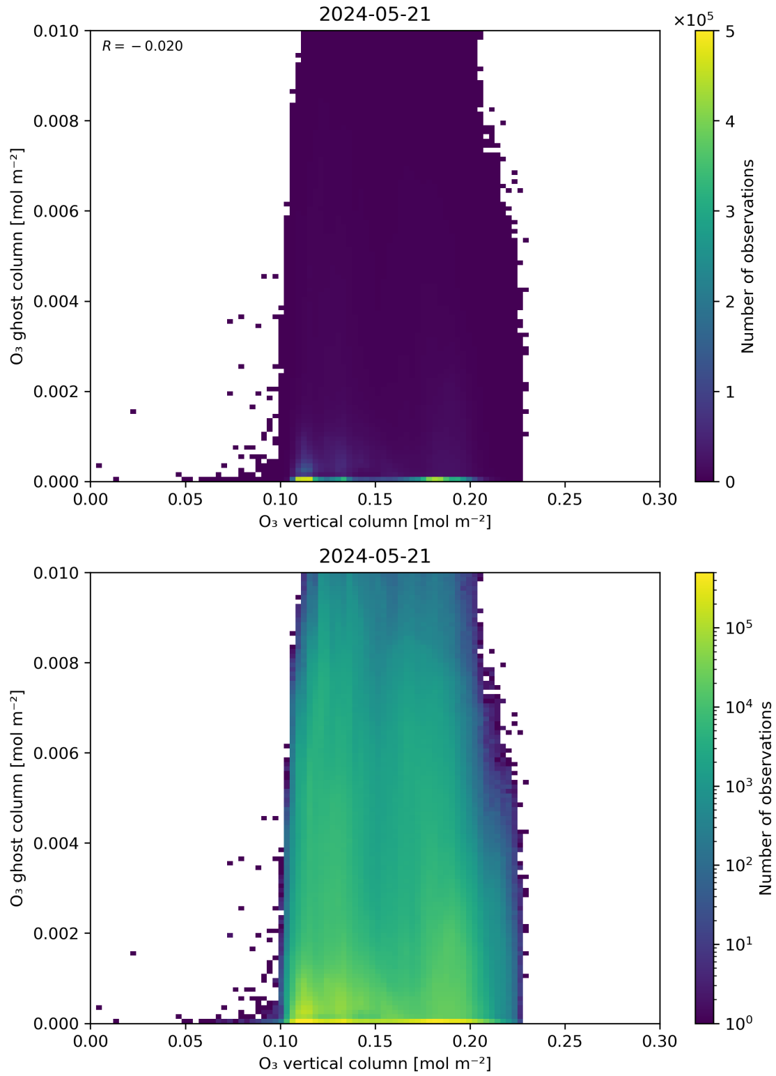
Figure 40: Scatter density plot of “O 3 vertical column” against “O 3 ghost column” for 2024-05-20 to 2024-05-22.
