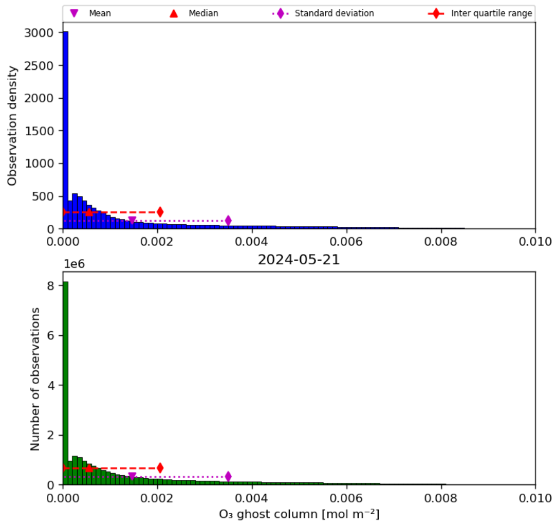
Figure 25: Histogram of “O 3 ghost column” for 2024-05-20 to 2024-05-22
