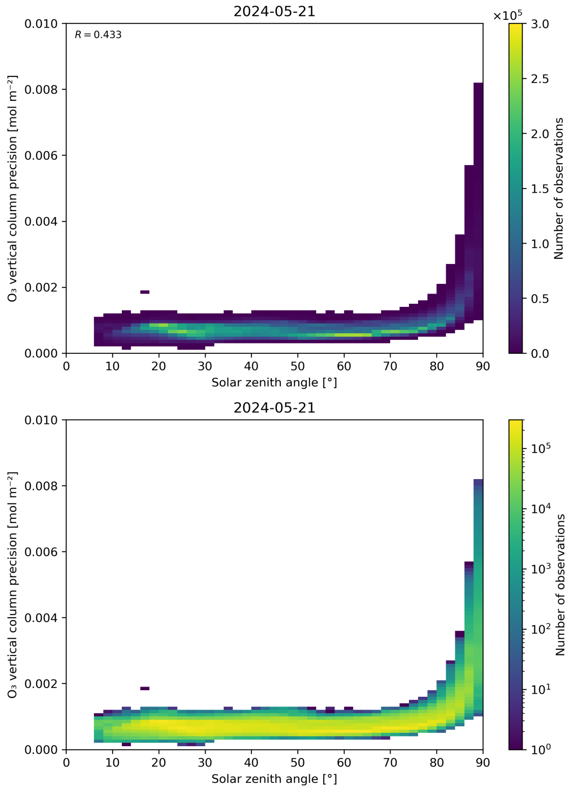
Figure 48: Scatter density plot of “Solar zenith angle” against “O 3 vertical column precision” for 2024-05-20 to 2024-05-22.
