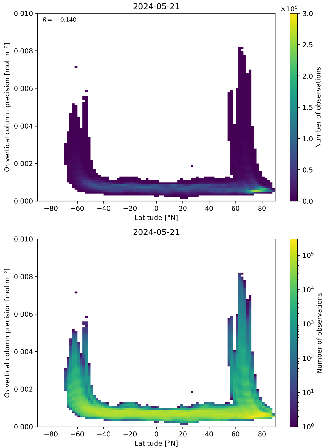
Figure 37: Scatter density plot of “Latitude” against “O 3 vertical column precision” for 2024-05-20 to 2024-05-22.
