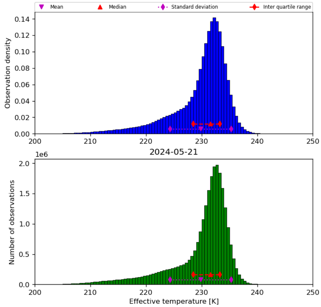
Figure 24: Histogram of “Effective temperature” for 2024-05-20 to 2024-05-22
