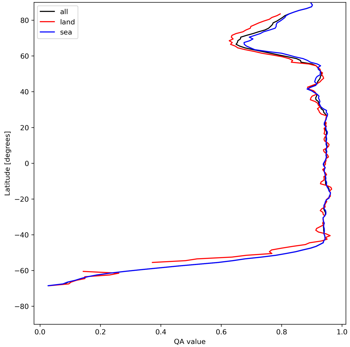
Figure 13: Zonal average of “QA value” for 2024-05-20 to 2024-05-22.
