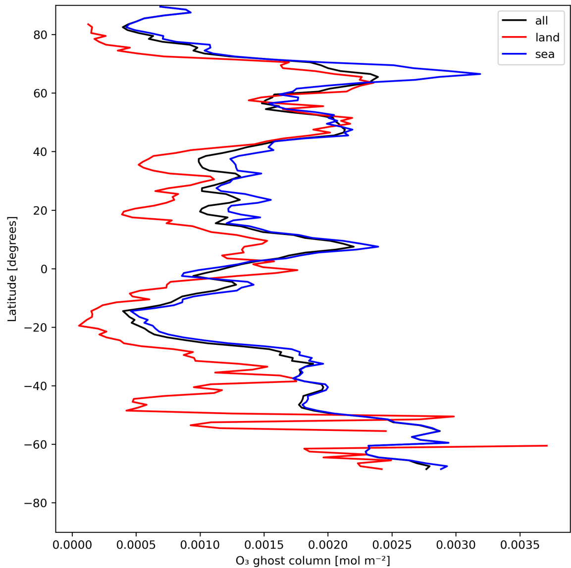
Figure 18: Zonal average of “O 3 ghost column” for 2024-05-20 to 2024-05-22.
