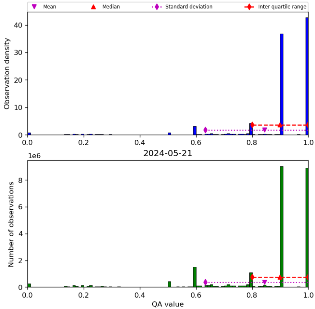
Figure 20: Histogram of “QA value” for 2024-05-20 to 2024-05-22
