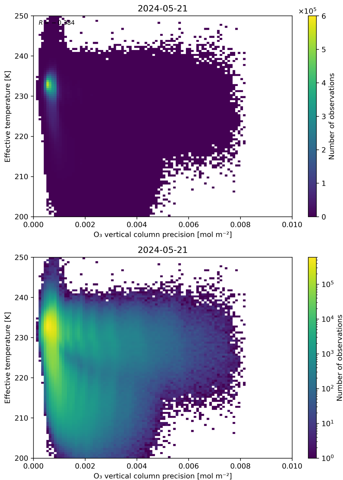
Figure 42: Scatter density plot of “O 3 vertical column precision” against “Effective temperature” for 2024-05-20 to 2024-05-22.
