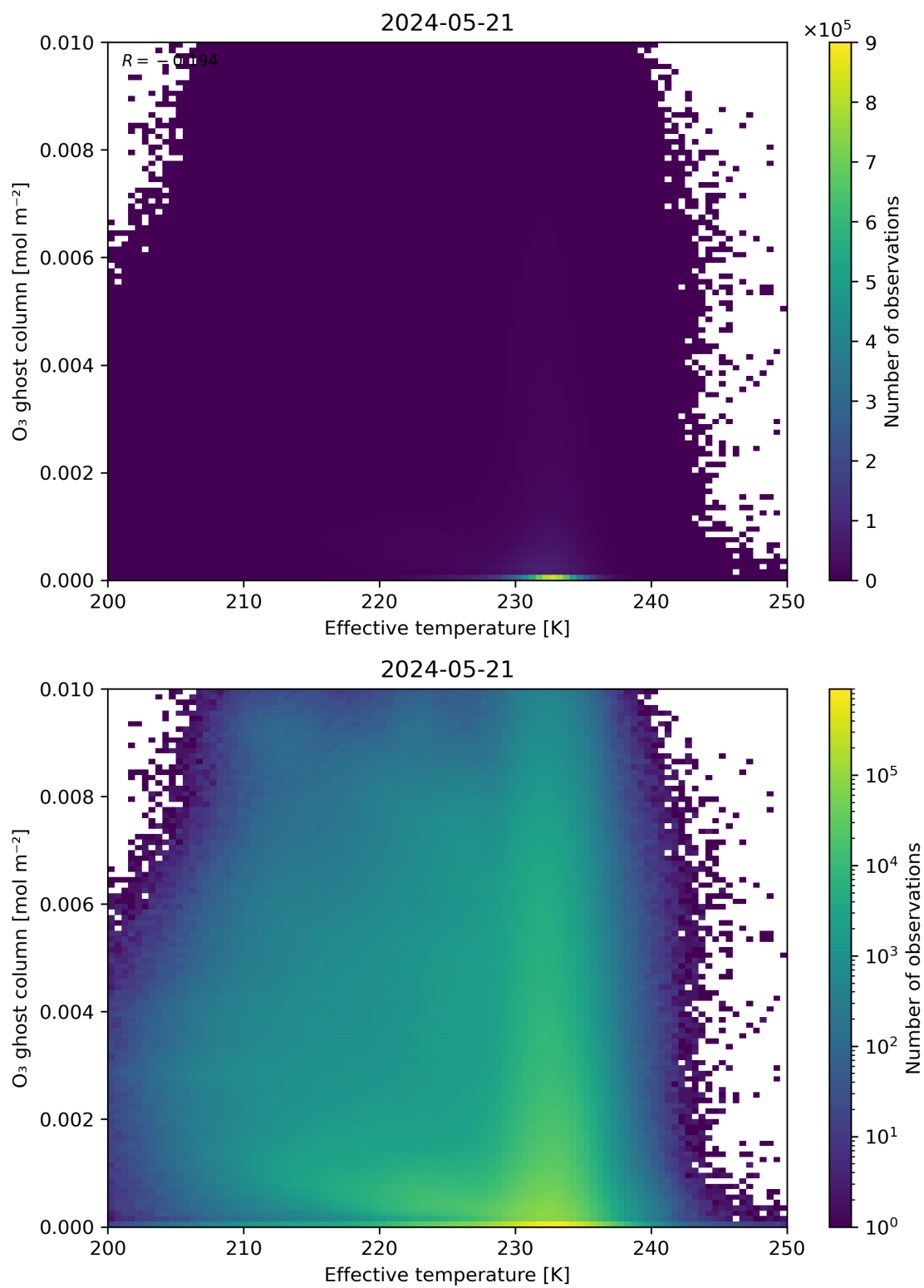
Figure 38: Scatter density plot of “Effective temperature” against “O 3 ghost column” for 2024-05-20 to 2024-05-22.
