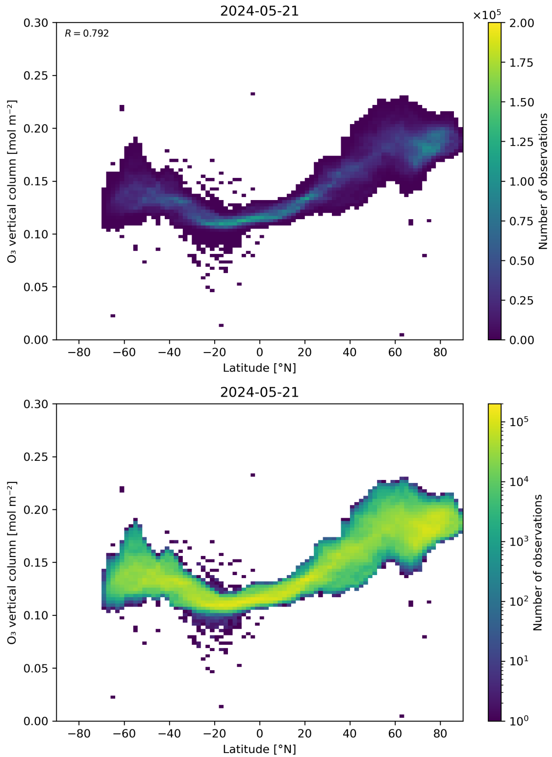
Figure 36: Scatter density plot of “Latitude” against “O 3 vertical column” for 2024-05-20 to 2024-05-22.
