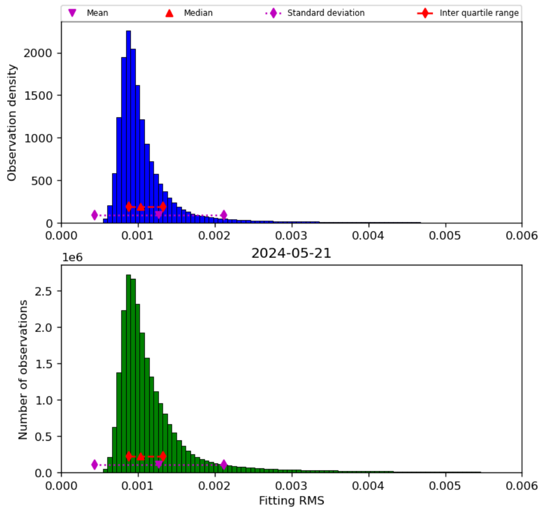
Figure 23: Histogram of “Fitting RMS” for 2024-05-20 to 2024-05-22
