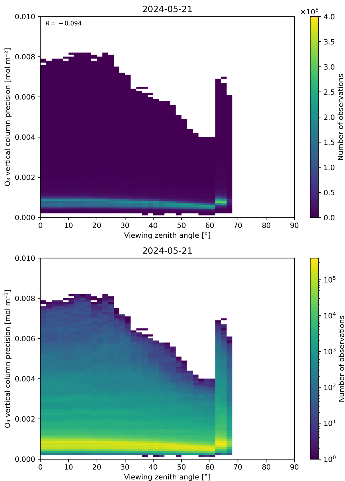
Figure 53: Scatter density plot of “Viewing zenith angle” against “O 3 vertical column precision” for 2024-05-20 to 2024-05-22.
