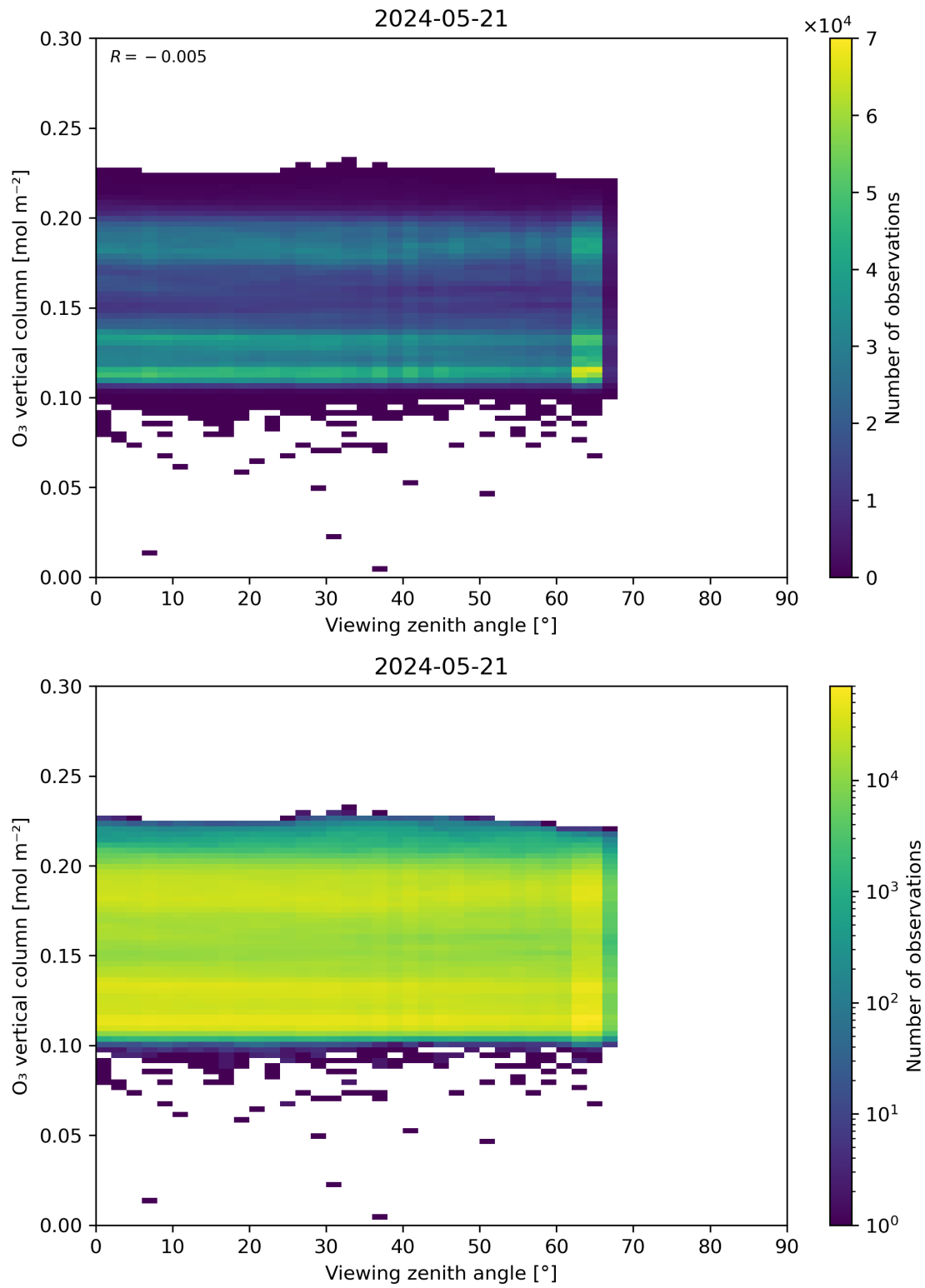
Figure 52: Scatter density plot of “Viewing zenith angle” against “O 3 vertical column” for 2024-05-20 to 2024-05-22.
