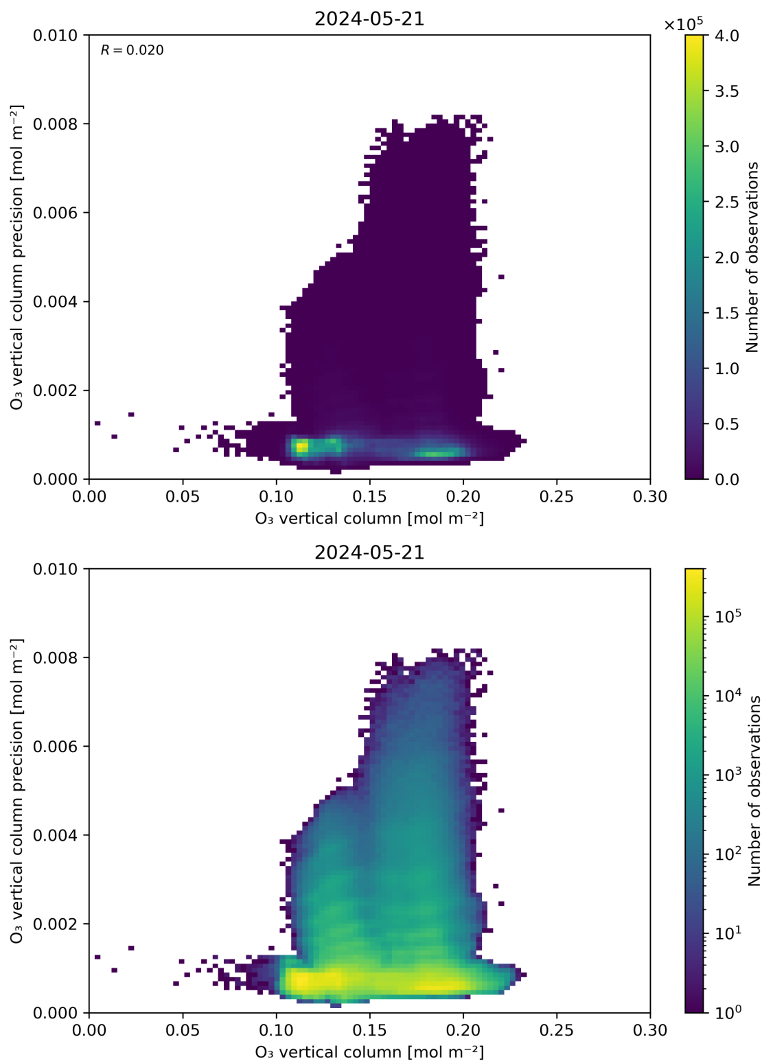
Figure 41: Scatter density plot of “O 3 vertical column” against “O 3 vertical column precision” for 2024-05-20 to 2024-05-22.
