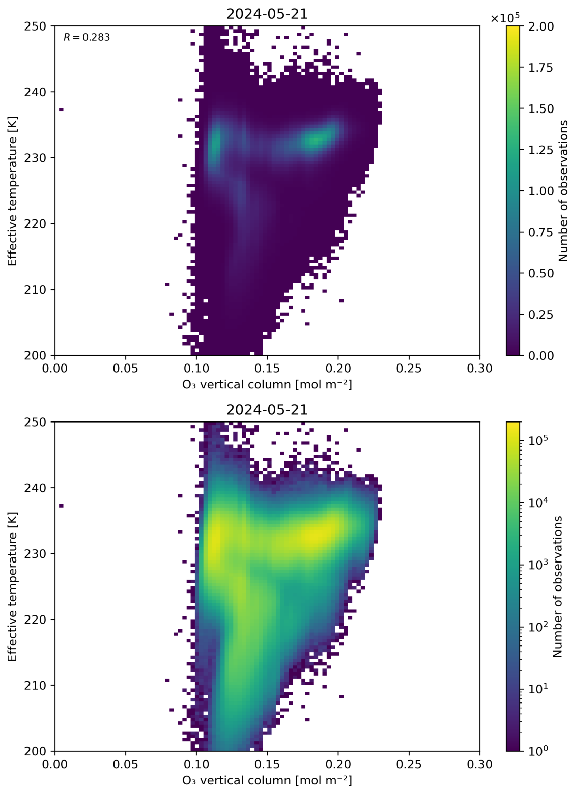
Figure 39: Scatter density plot of “O 3 vertical column” against “Effective temperature” for 2024-05-20 to 2024-05-22.
