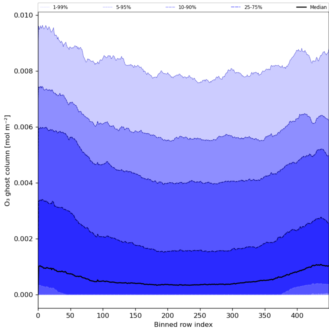
Figure 32: Along track statistics of “O 3 ghost column” for 2024-05-20 to 2024-05-22
