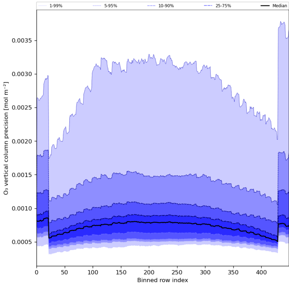
Figure 29: Along track statistics of “O 3 vertical column precision” for 2024-05-20 to 2024-05-22
