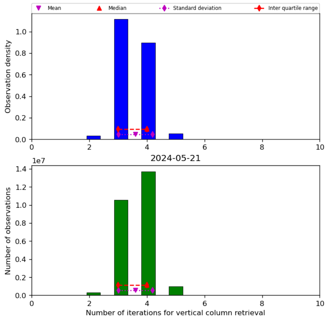
Figure 26: Histogram of “Number of iterations for vertical column retrieval” for 2024-05-20 to 2024-05-22
