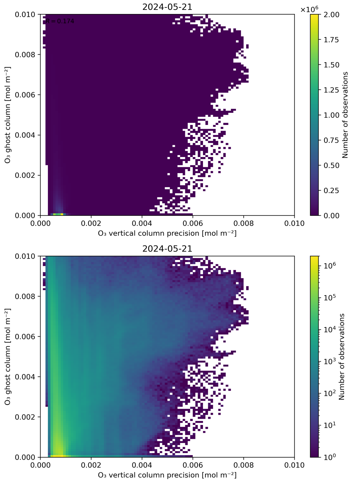
Figure 43: Scatter density plot of “ \text{O}_3 vertical column precision” against “ \text{O}_3 ghost column” for 2024-05-20 to 2024-05-22.
