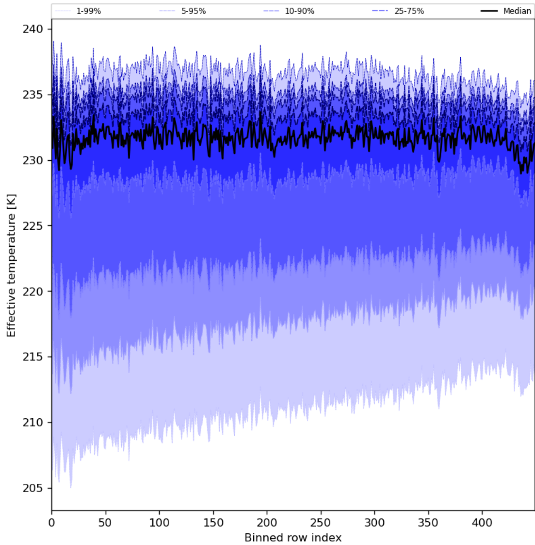
Figure 31: Along track statistics of “Effective temperature” for 2024-05-20 to 2024-05-22
