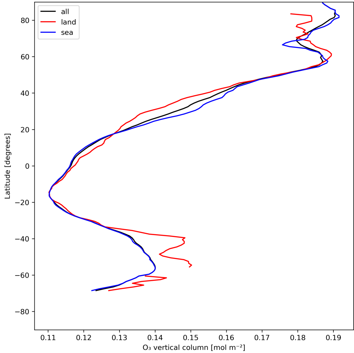
Figure 14: Zonal average of “O 3 vertical column” for 2024-05-20 to 2024-05-22.
