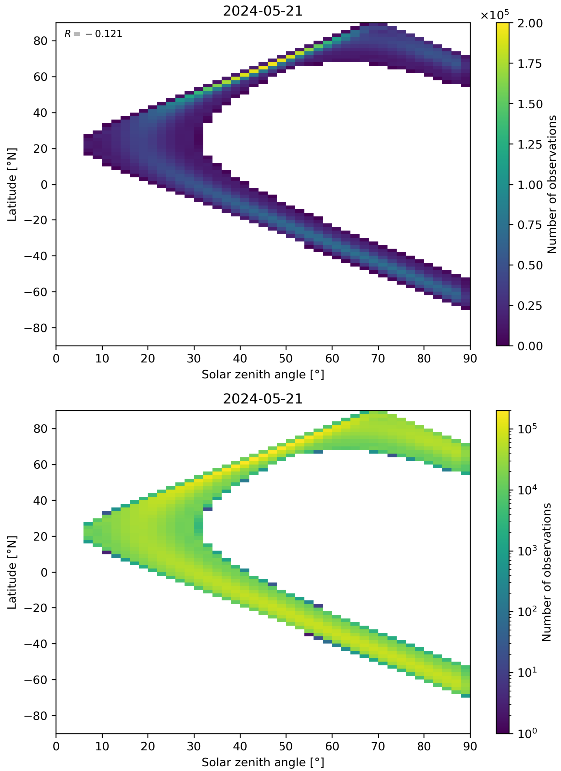
Figure 44: Scatter density plot of “Solar zenith angle” against “Latitude” for 2024-05-20 to 2024-05-22.
