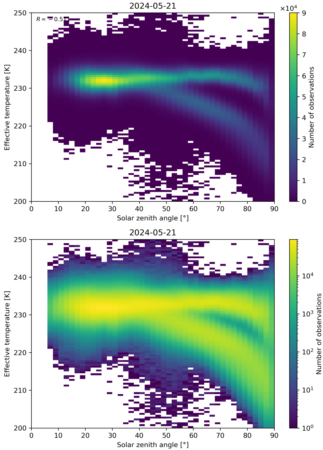
Figure 45: Scatter density plot of “Solar zenith angle” against “Effective temperature” for 2024-05-20 to 2024-05-22.
