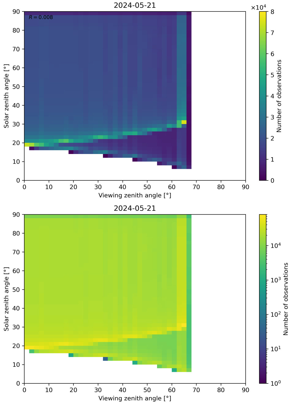
Figure 54: Scatter density plot of “Viewing zenith angle” against “Solar zenith angle” for 2024-05-20 to 2024-05-22.
