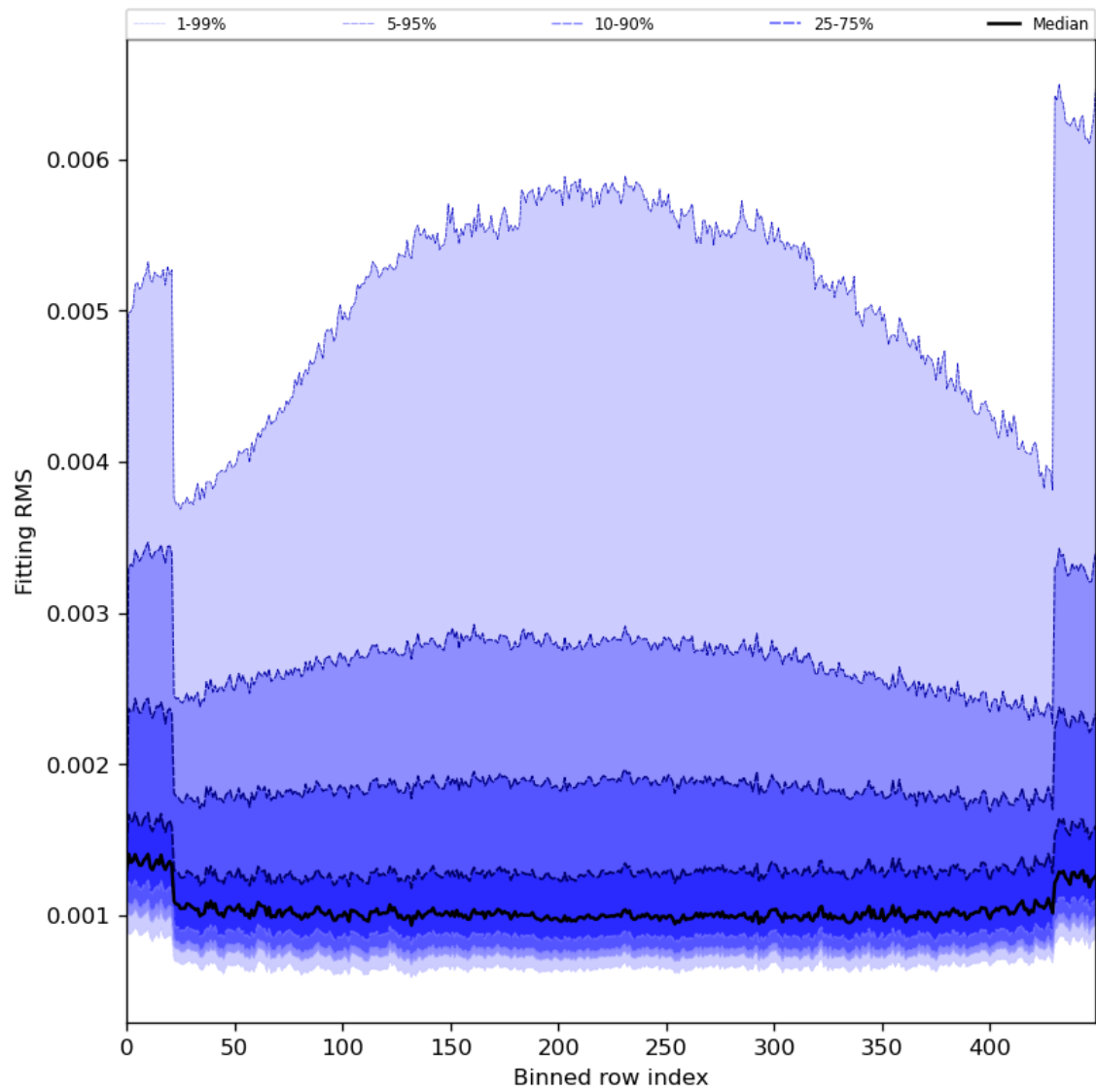
Figure 30: Along track statistics of “Fitting RMS” for 2024-05-20 to 2024-05-22
