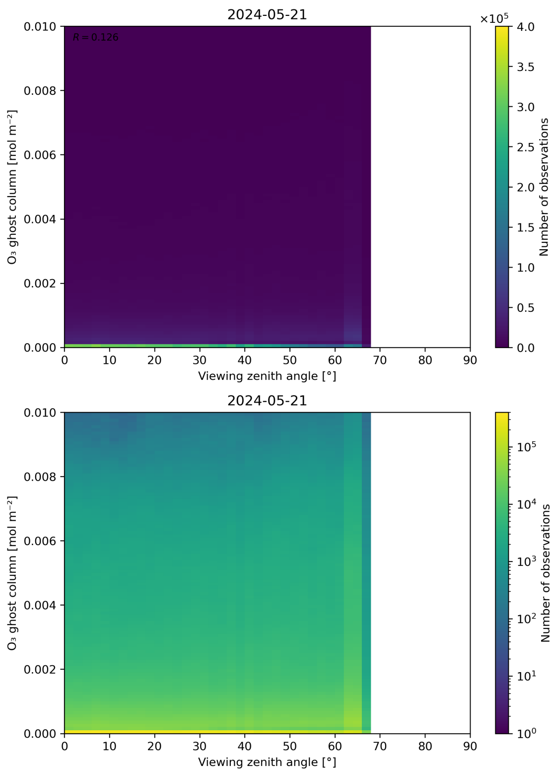
Figure 51: Scatter density plot of “Viewing zenith angle” against “O 3 ghost column” for 2024-05-20 to 2024-05-22.
