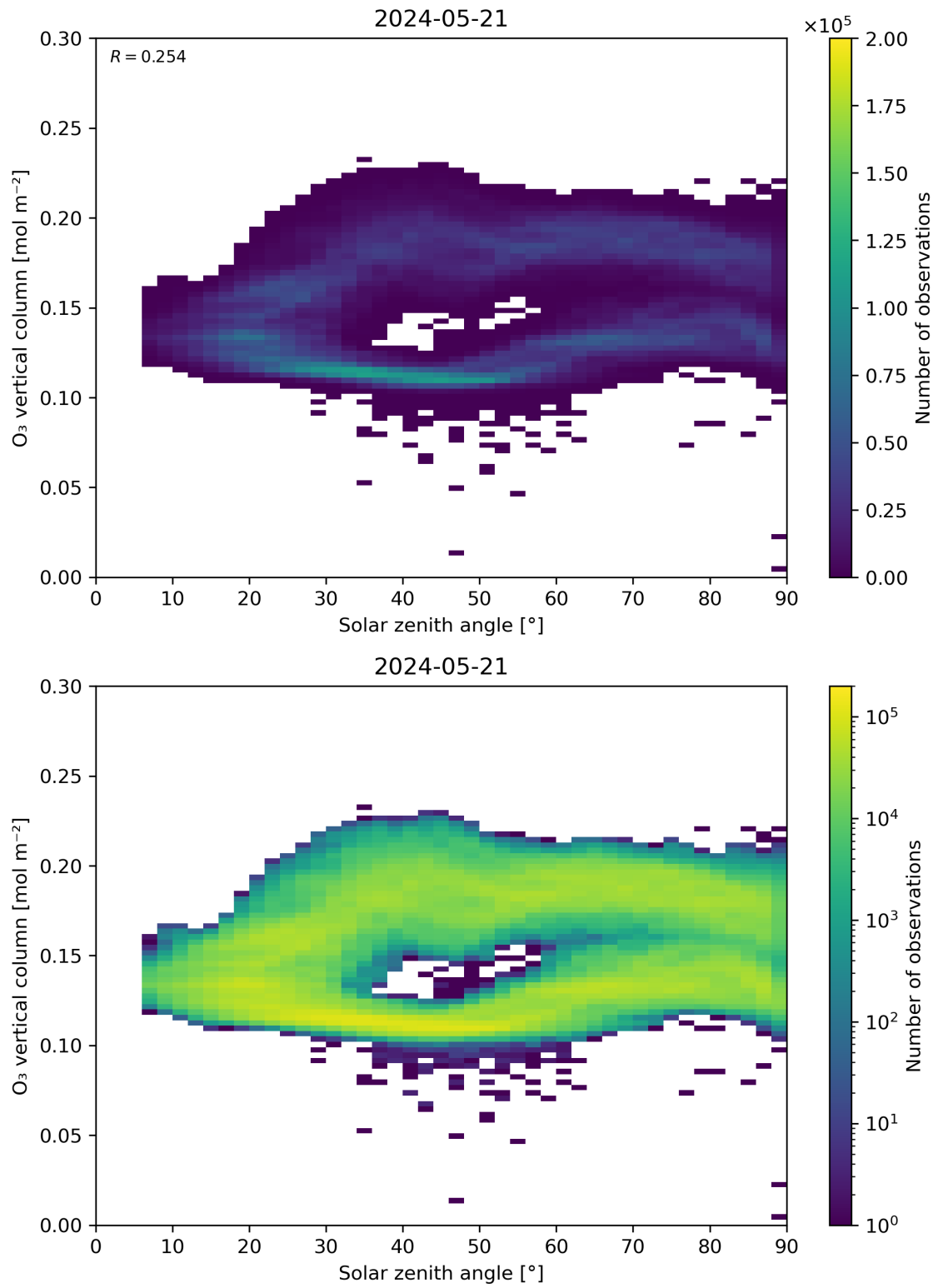
Figure 47: Scatter density plot of “Solar zenith angle” against “O 3 vertical column” for 2024-05-20 to 2024-05-22.
