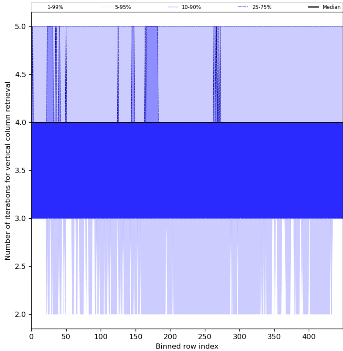
Figure 33: Along track statistics of “Number of iterations for vertical column retrieval” for 2024-05-20 to 2024-05-22
