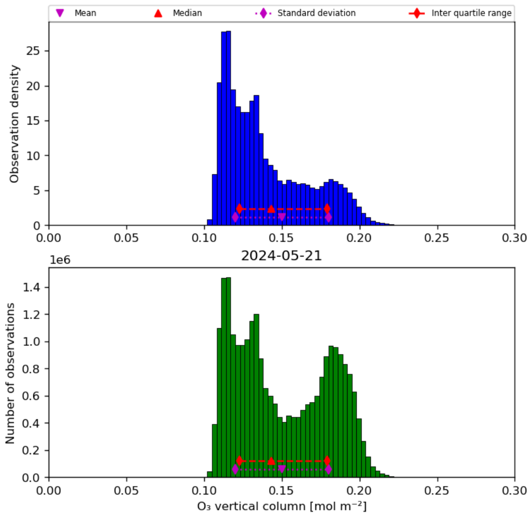
Figure 21: Histogram of “O 3 vertical column” for 2024-05-20 to 2024-05-22
