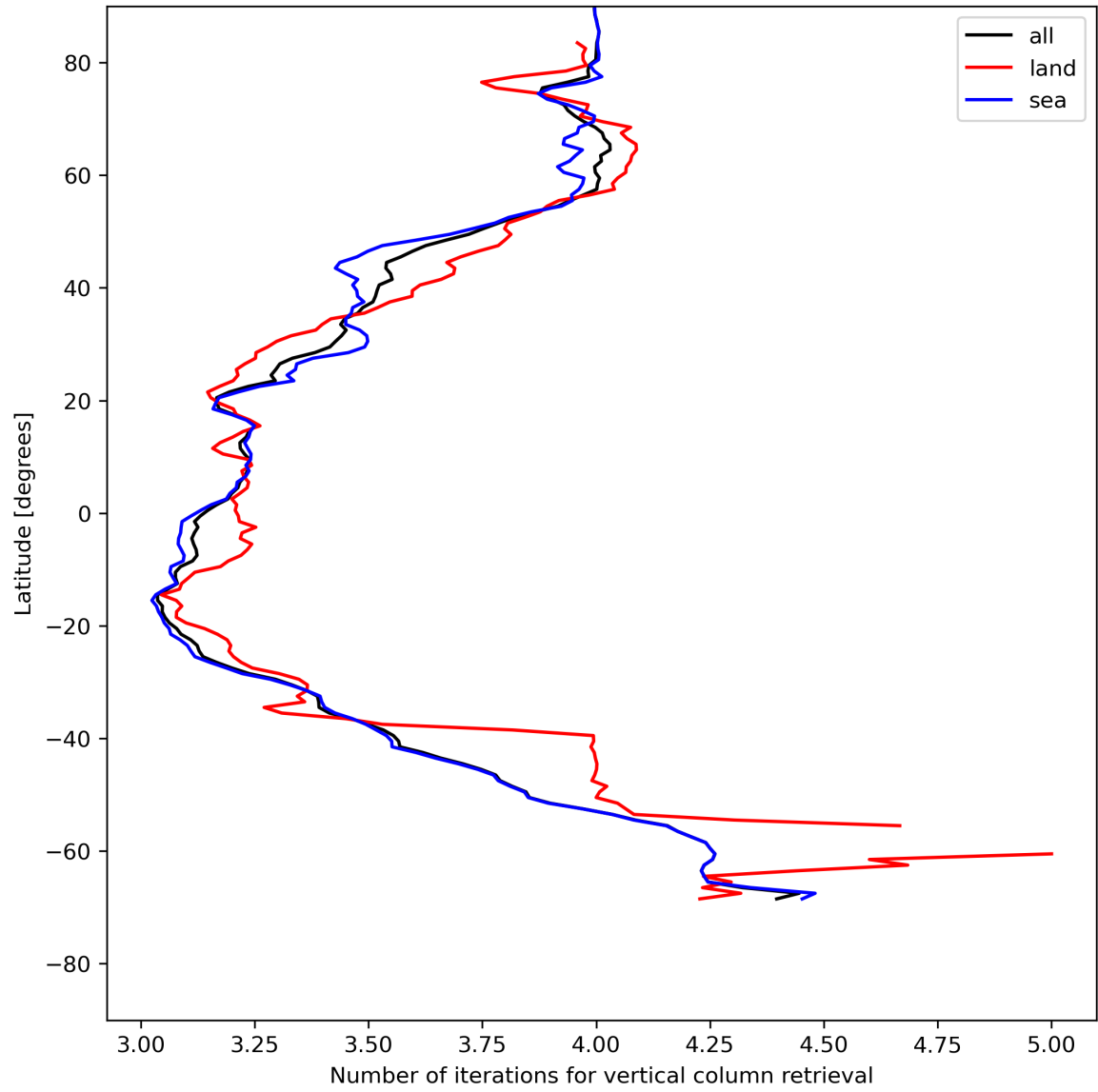
Figure 19: Zonal average of “Number of iterations for vertical column retrieval” for 2024-05-20 to 2024-05-22.
