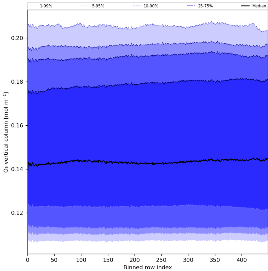
Figure 28: Along track statistics of “O 3 vertical column” for 2024-05-20 to 2024-05-22
