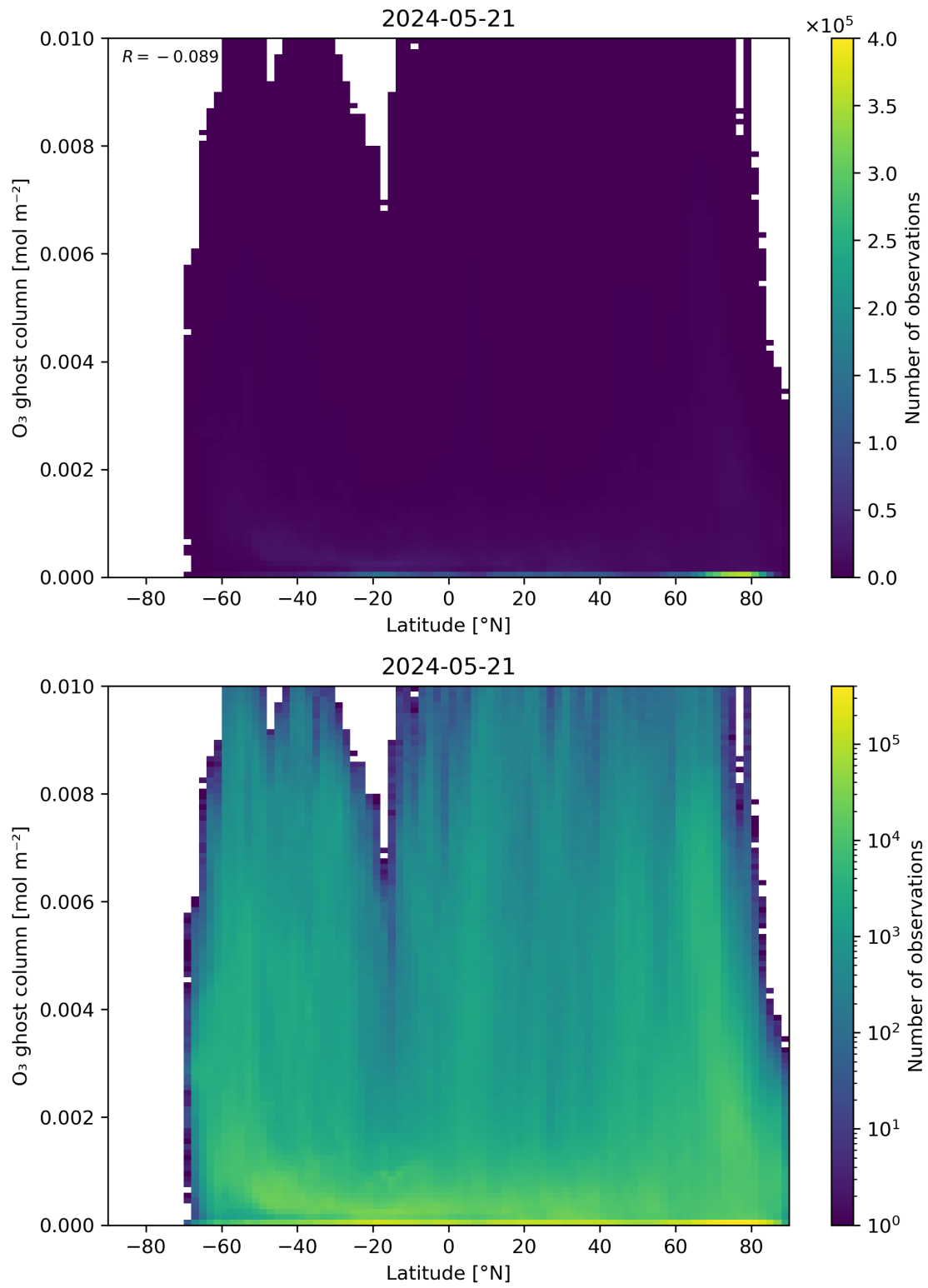
Figure 35: Scatter density plot of “Latitude” against “O 3 ghost column” for 2024-05-20 to 2024-05-22.
