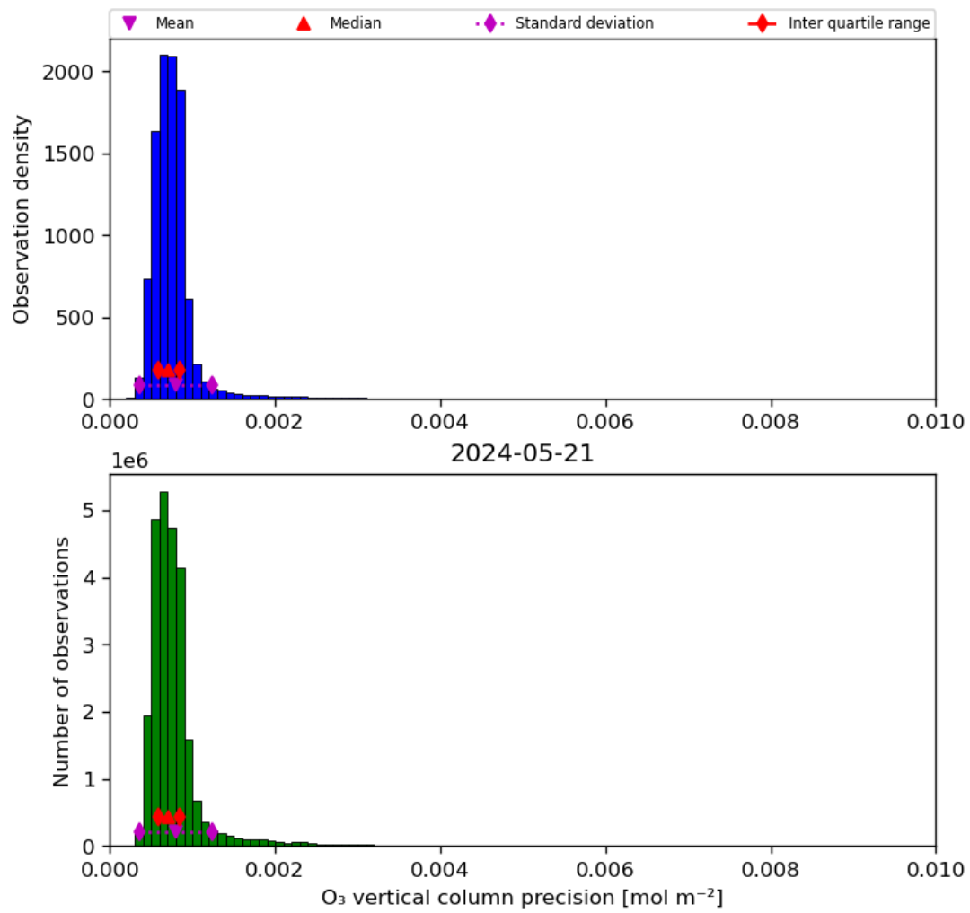
Figure 22: Histogram of "O 3 vertical column precision" for 2024-05-20 to 2024-05-22
