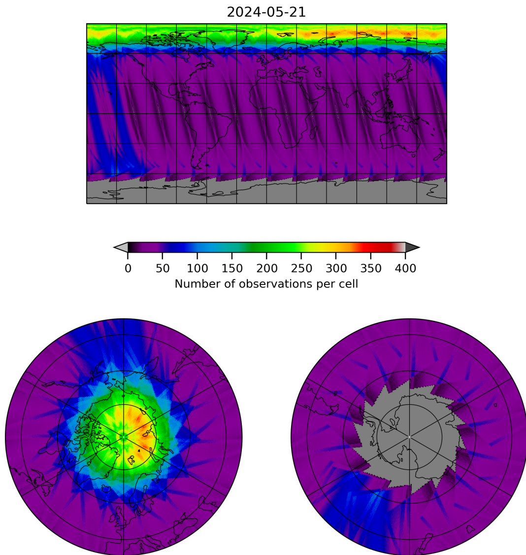
Figure 12: Map of the number of observations for 2024-05-20 to 2024-05-22
