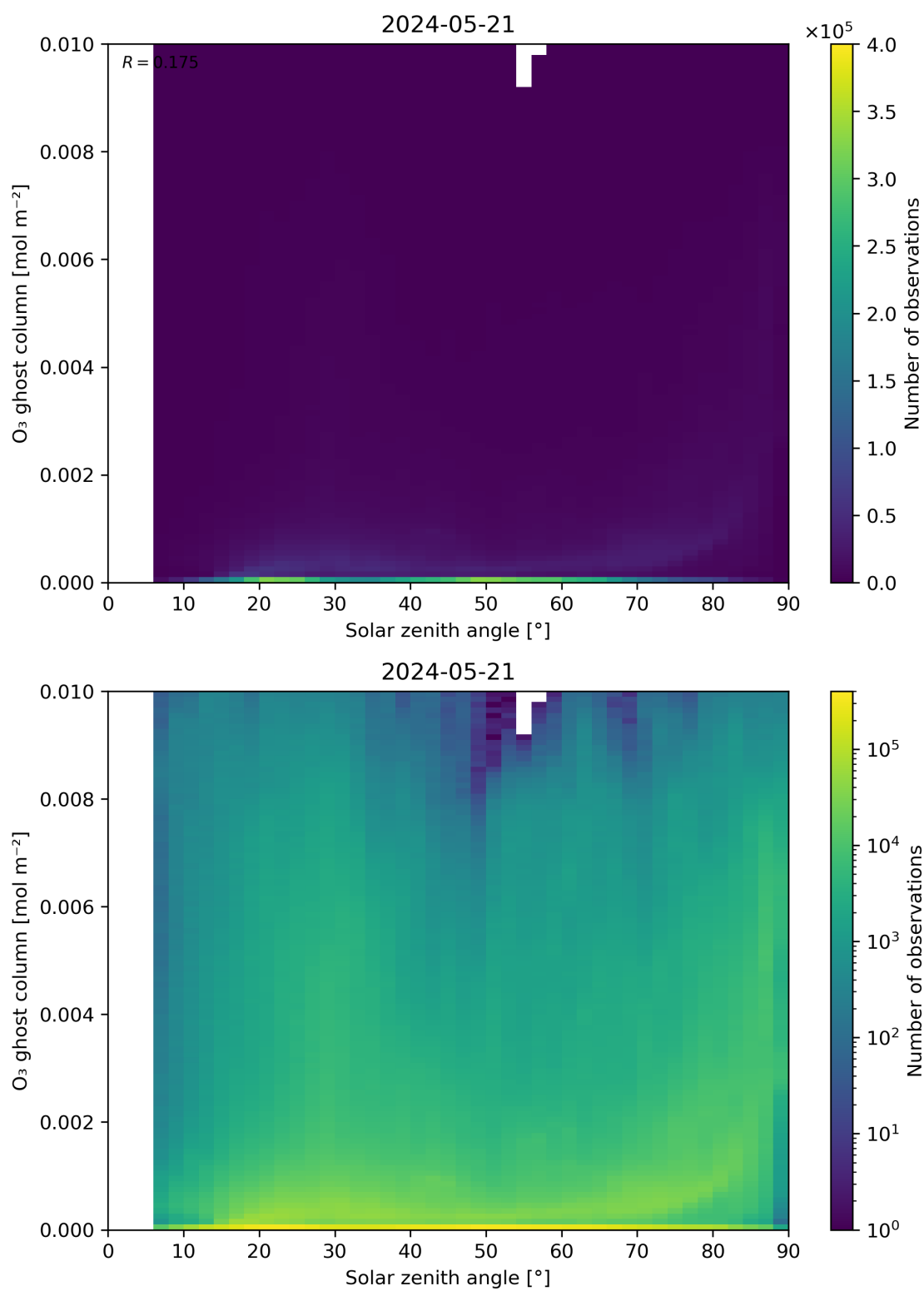
Figure 46: Scatter density plot of “Solar zenith angle” against “O 3 ghost column” for 2024-05-20 to 2024-05-22.
