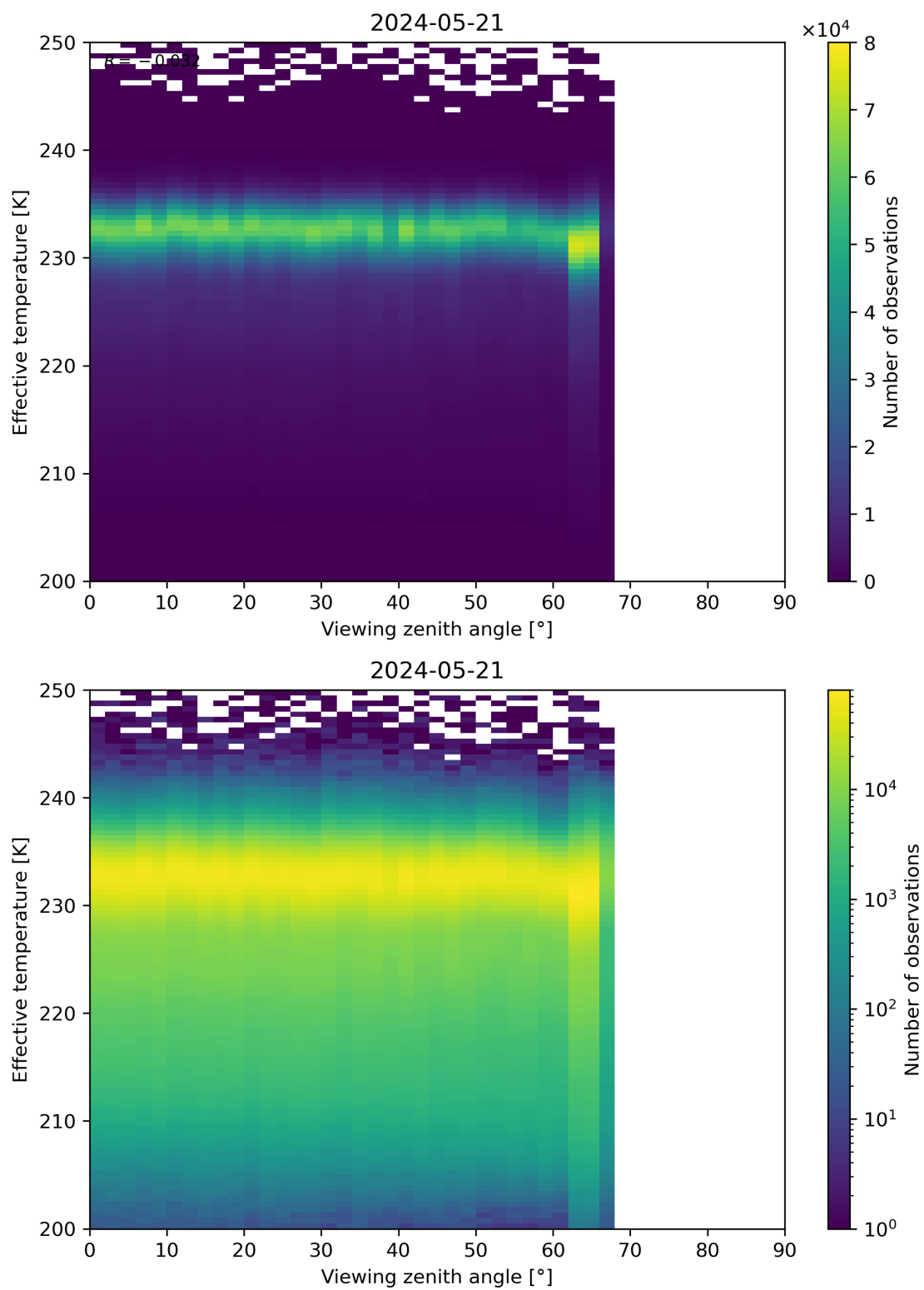
Figure 50: Scatter density plot of “Viewing zenith angle” against “Effective temperature” for 2024-05-20 to 2024-05-22.
