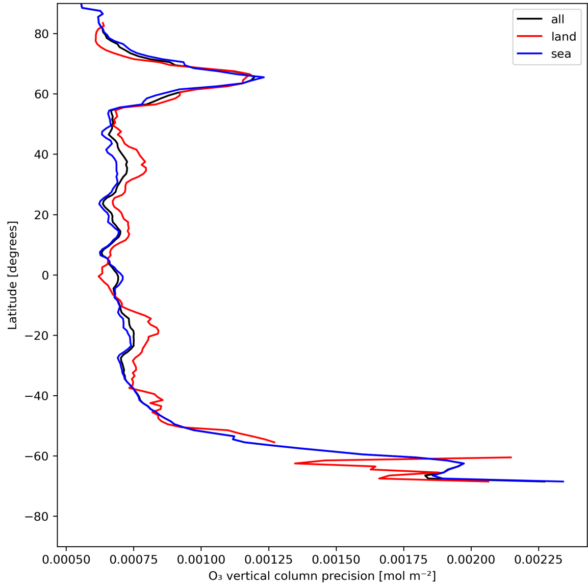
Figure 15: Zonal average of “O 3 vertical column precision” for 2024-05-20 to 2024-05-22.
