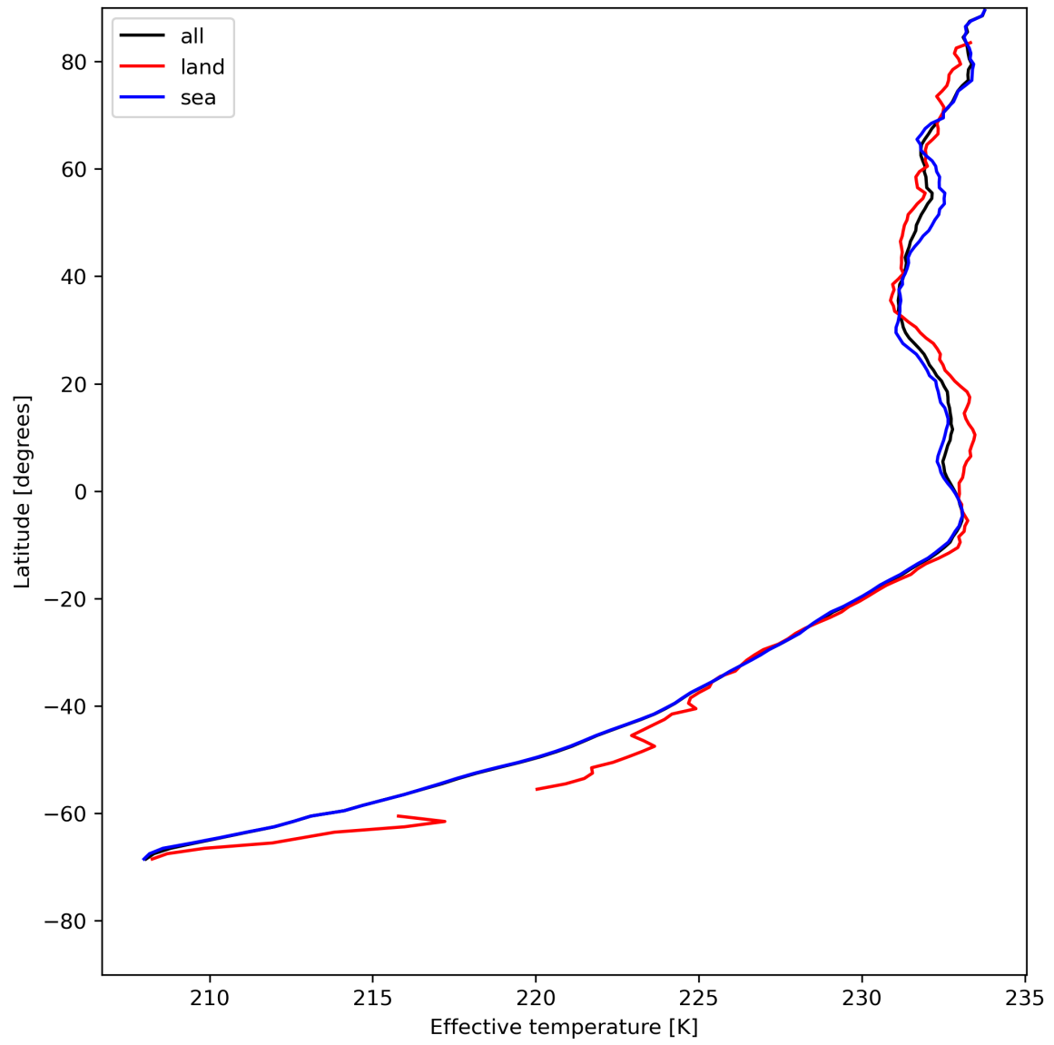
Figure 17: Zonal average of "Effective temperature" for 2024-05-20 to 2024-05-22.
