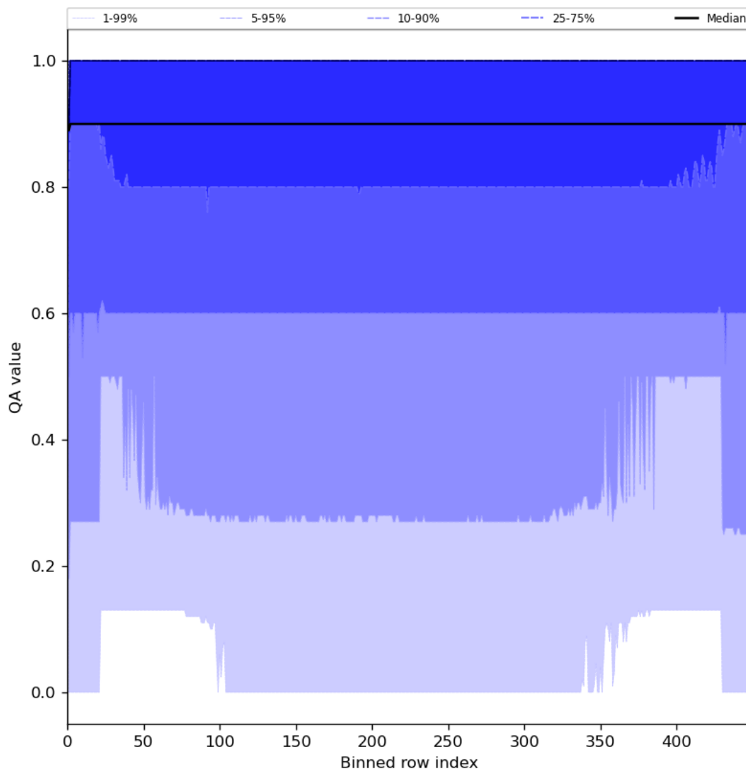
Figure 27: Along track statistics of “QA value” for 2024-05-20 to 2024-05-22
