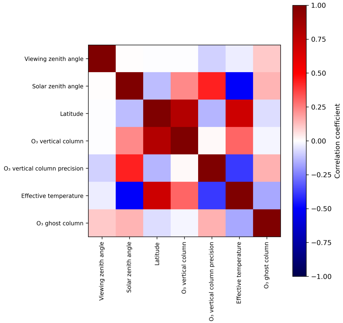
Figure 2: Map of correlation matrix for 2024-05-21 to 2024-05-23.
