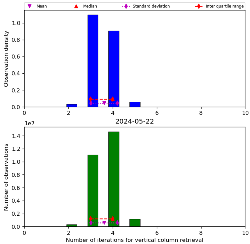
Figure 26: Histogram of “Number of iterations for vertical column retrieval” for 2024-05-21 to 2024-05-23
