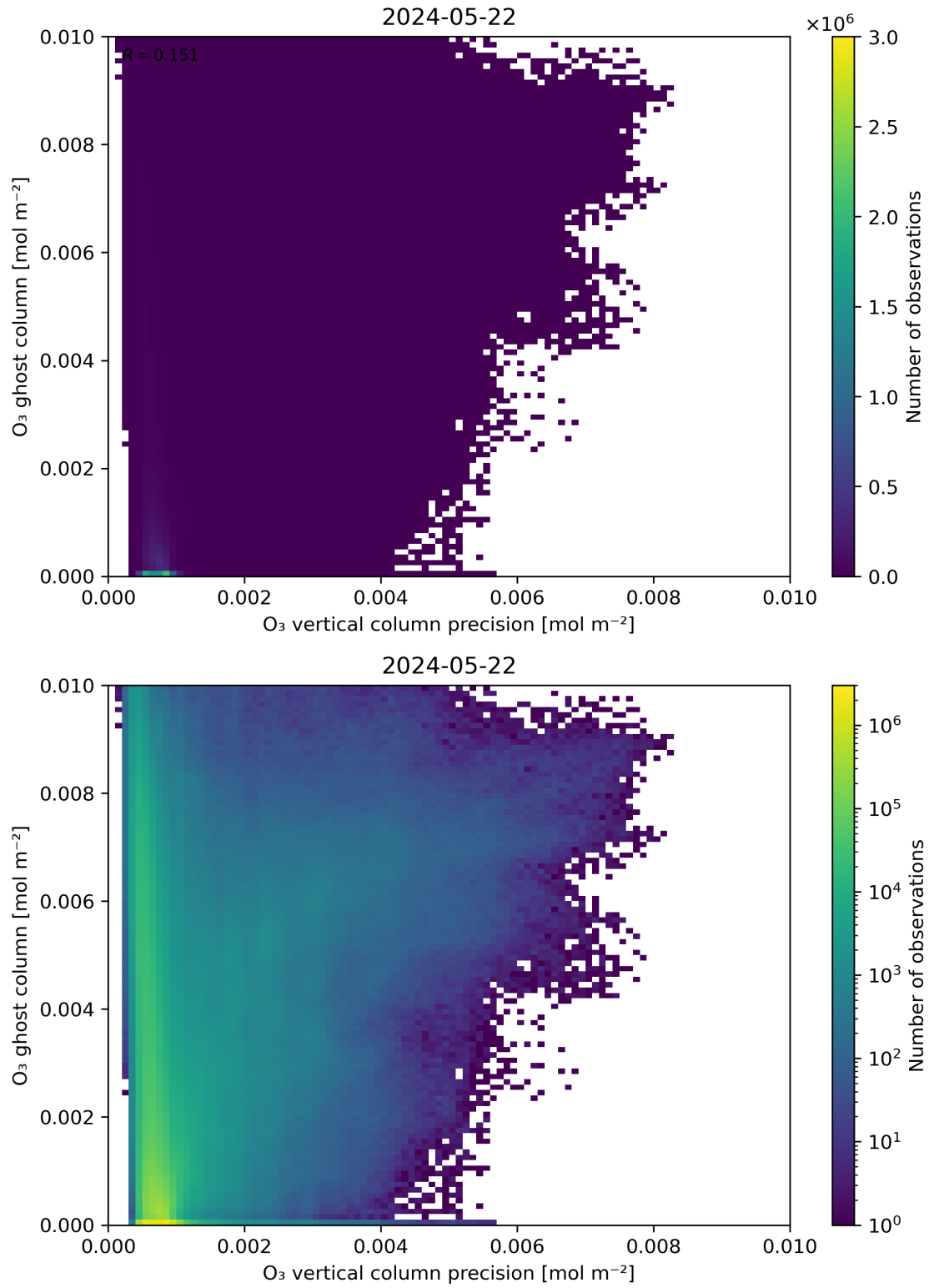
Figure 43: Scatter density plot of “ \text{O}_3 vertical column precision” against “ \text{O}_3 ghost column” for 2024-05-21 to 2024-05-23.
