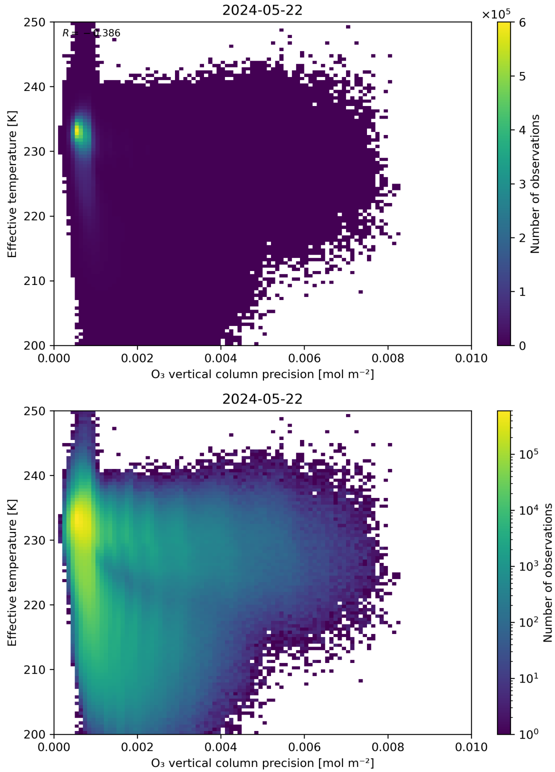
Figure 42: Scatter density plot of “O 3 vertical column precision” against “Effective temperature” for 2024-05-21 to 2024-05-23.
