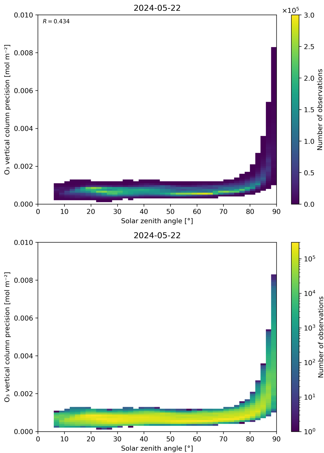
Figure 48: Scatter density plot of “Solar zenith angle” against “O 3 vertical column precision” for 2024-05-21 to 2024-05-23.
