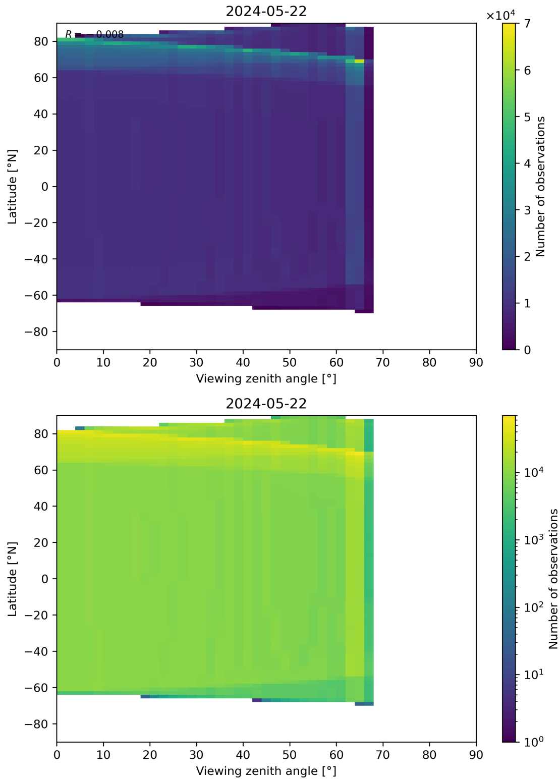
Figure 49: Scatter density plot of “Viewing zenith angle” against “Latitude” for 2024-05-21 to 2024-05-23.
