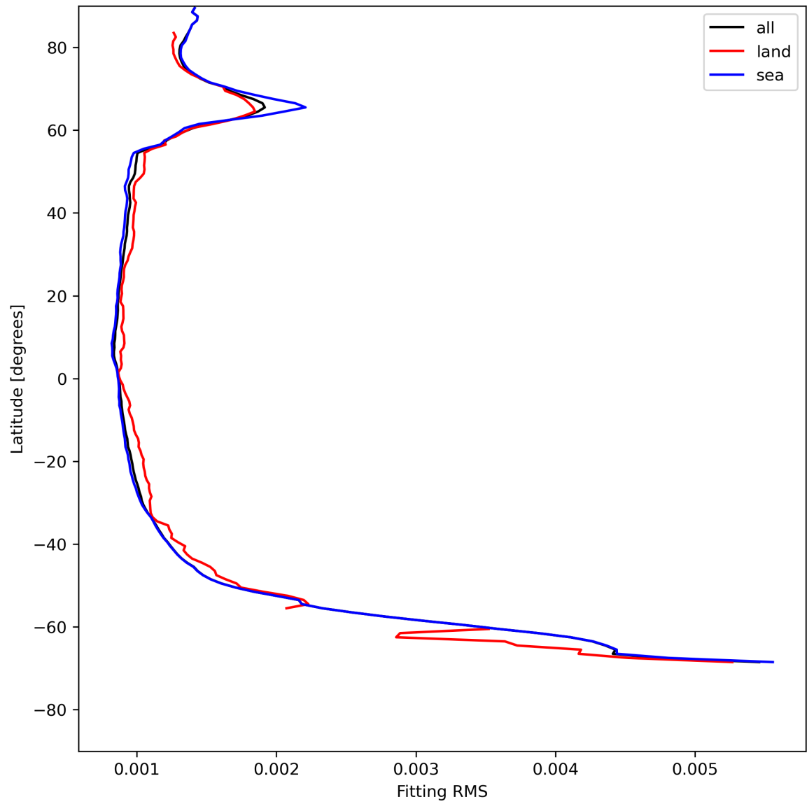
Figure 16: Zonal average of “Fitting RMS” for 2024-05-21 to 2024-05-23.
