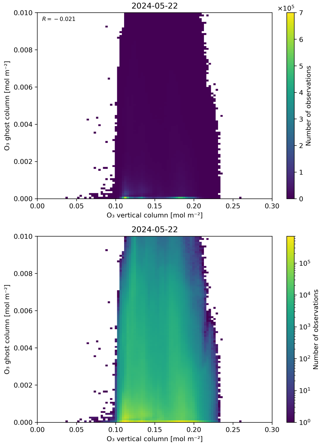
Figure 40: Scatter density plot of “O 3 vertical column” against “O 3 ghost column” for 2024-05-21 to 2024-05-23.
