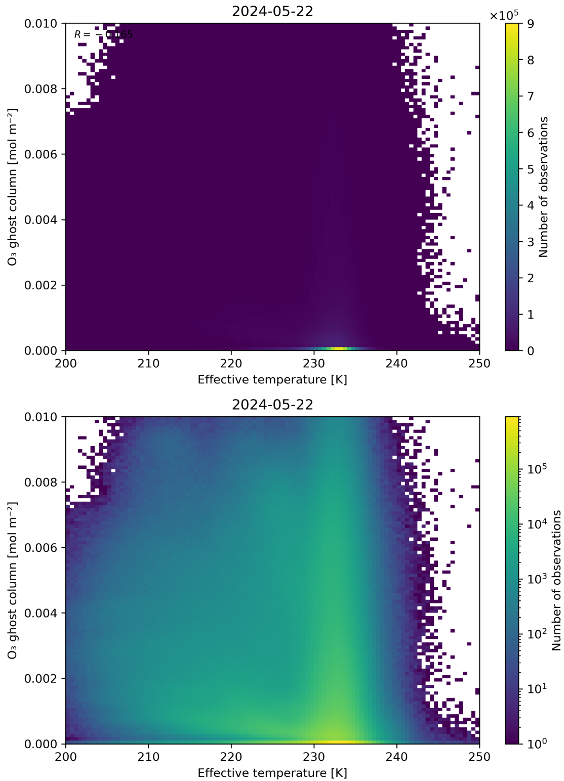
Figure 38: Scatter density plot of “Effective temperature” against “O 3 ghost column” for 2024-05-21 to 2024-05-23.
