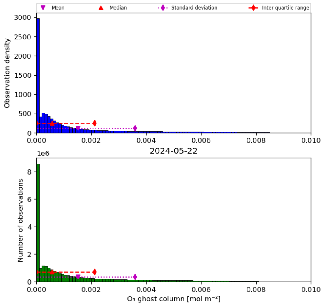
Figure 25: Histogram of "O 3 ghost column" for 2024-05-21 to 2024-05-23
