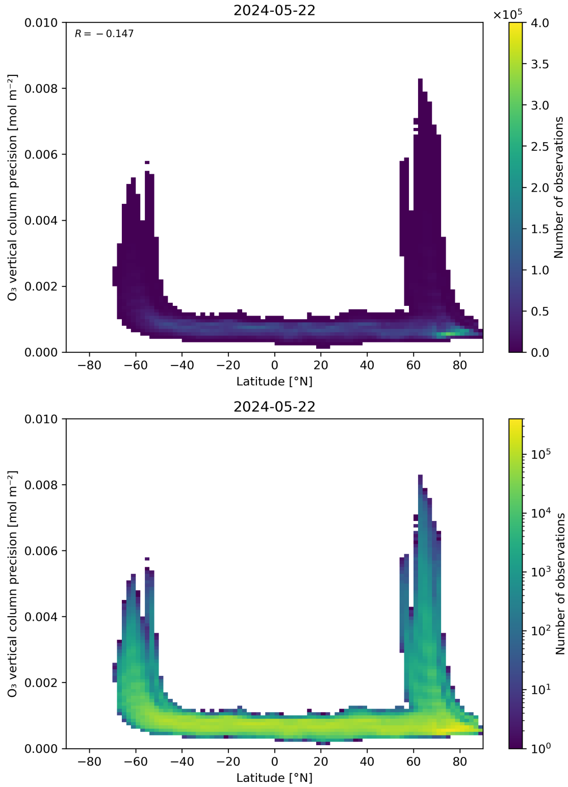
Figure 37: Scatter density plot of “Latitude” against “O 3 vertical column precision” for 2024-05-21 to 2024-05-23.
