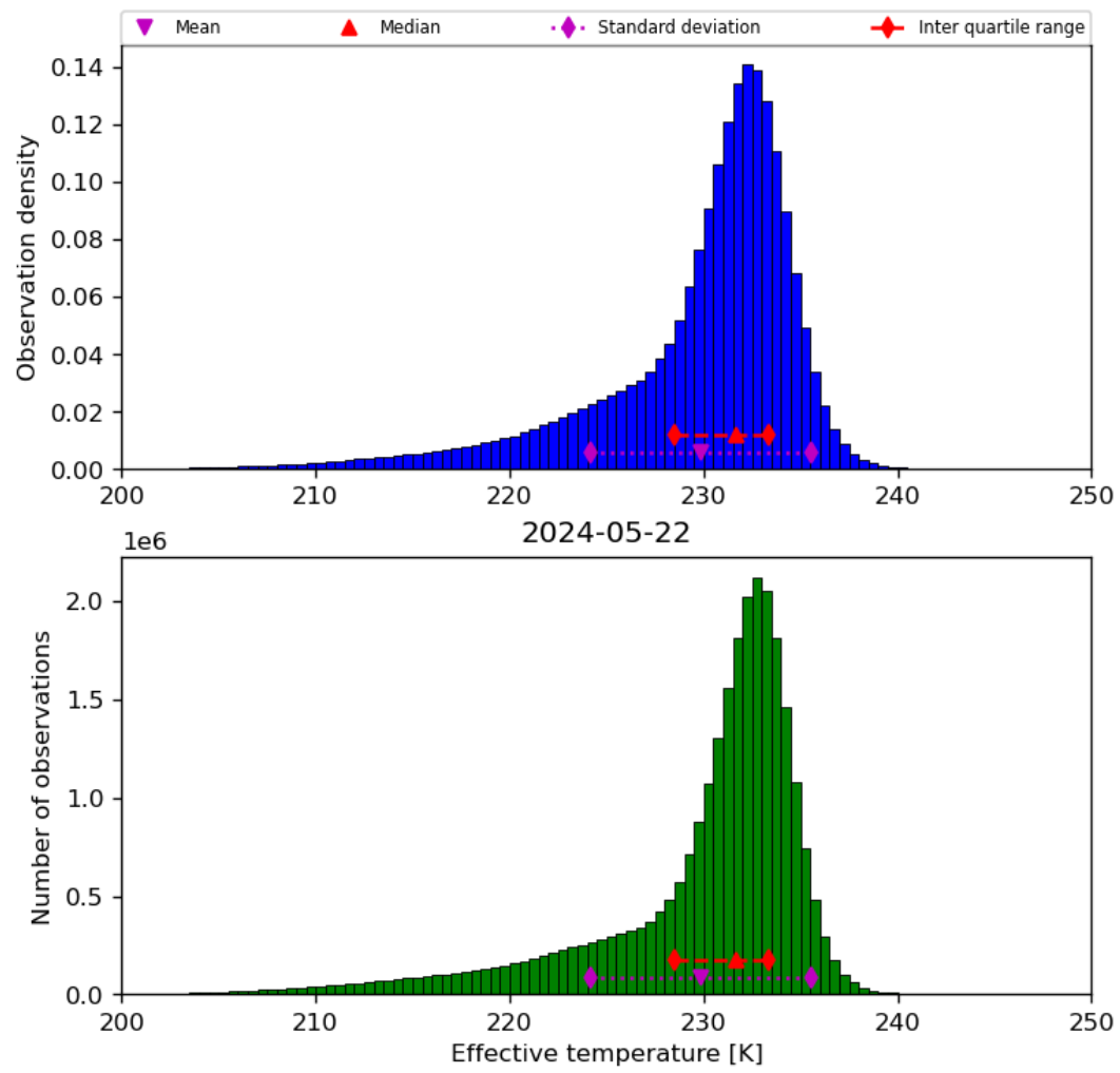
Figure 24: Histogram of “Effective temperature” for 2024-05-21 to 2024-05-23
