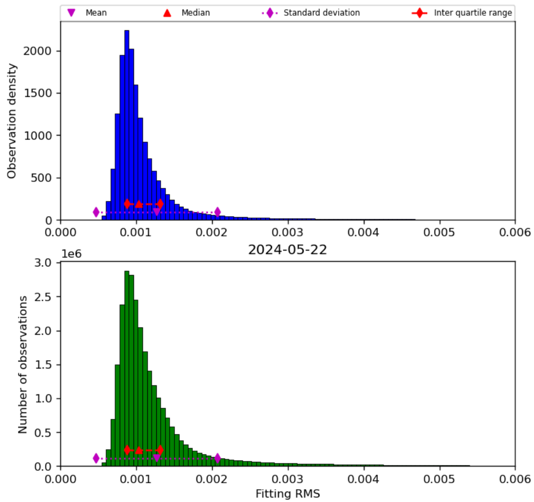
Figure 23: Histogram of “Fitting RMS” for 2024-05-21 to 2024-05-23
