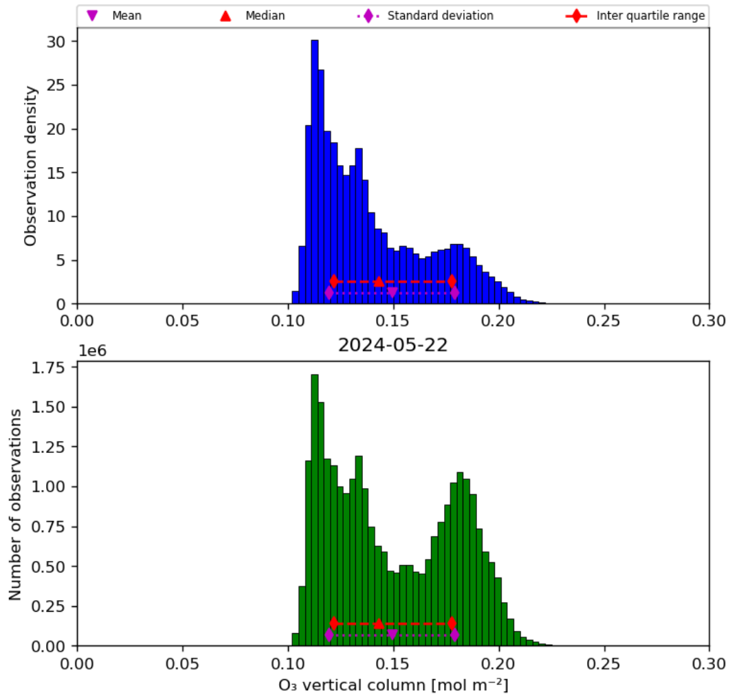
Figure 21: Histogram of “O 3 vertical column” for 2024-05-21 to 2024-05-23
