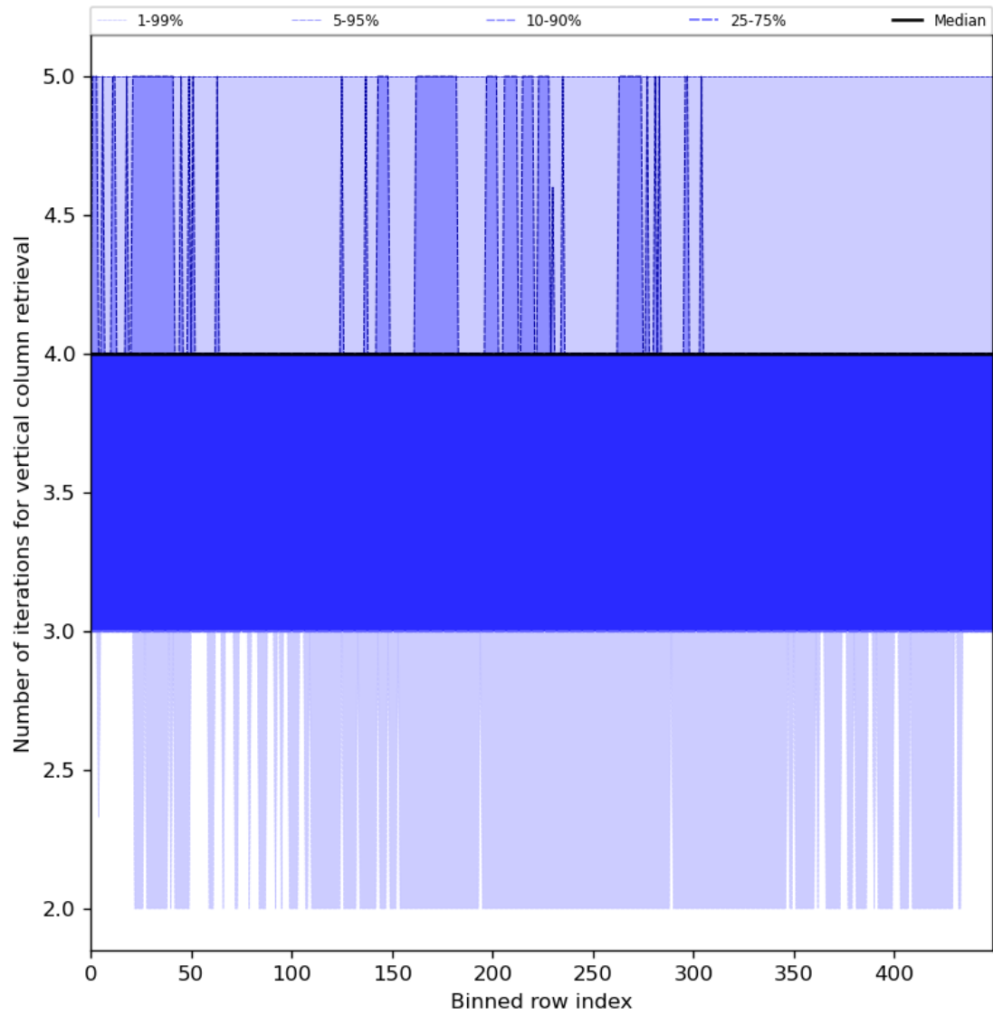
Figure 33: Along track statistics of “Number of iterations for vertical column retrieval” for 2024-05-21 to 2024-05-23
