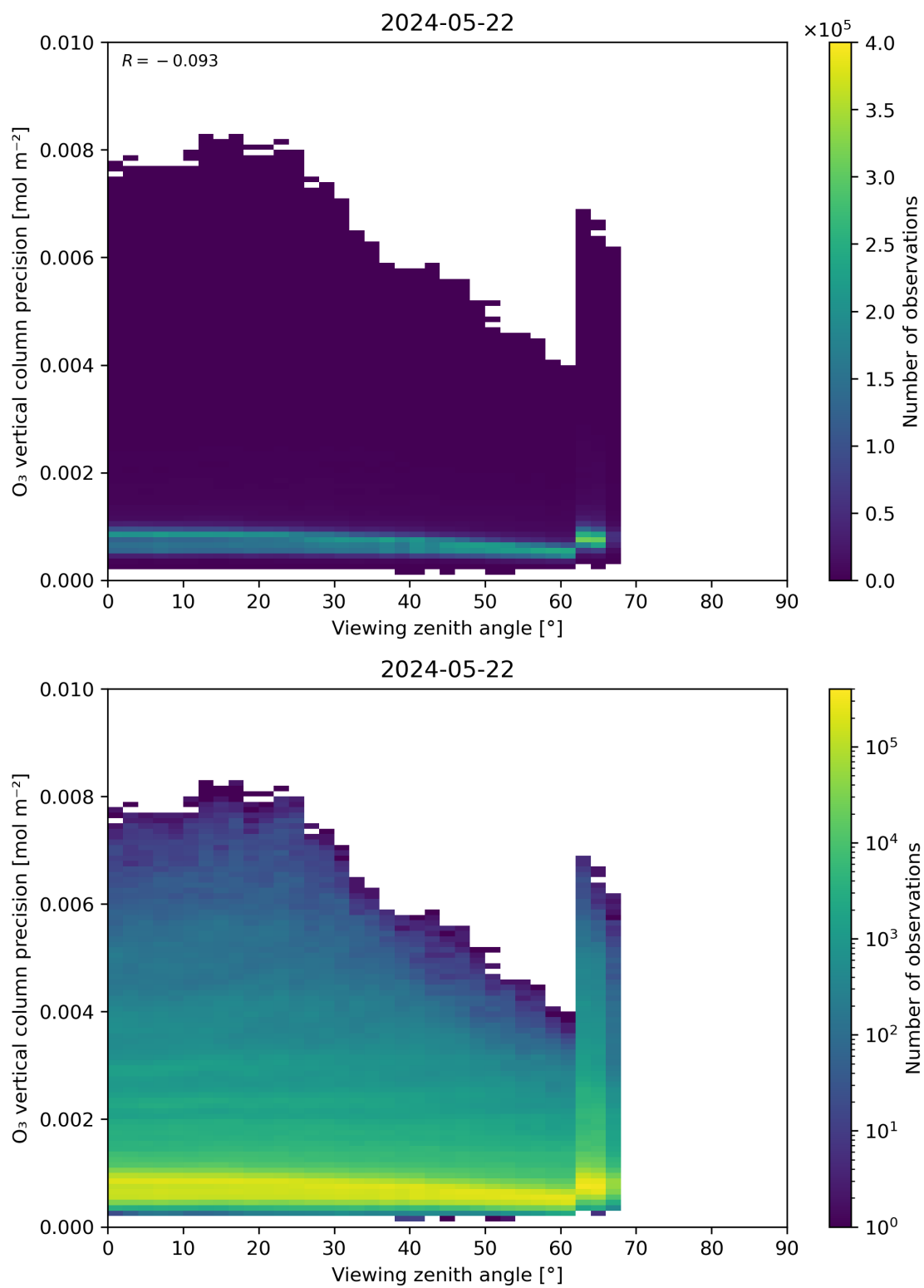
Figure 53: Scatter density plot of “Viewing zenith angle” against “O 3 vertical column precision” for 2024-05-21 to 2024-05-23.
