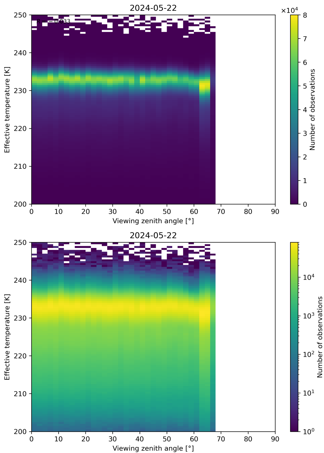
Figure 50: Scatter density plot of “Viewing zenith angle” against “Effective temperature” for 2024-05-21 to 2024-05-23.
