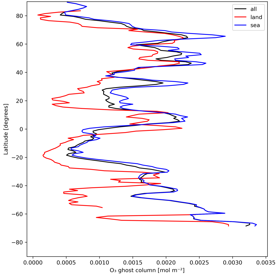
Figure 18: Zonal average of "O 3 ghost column" for 2024-05-21 to 2024-05-23.
