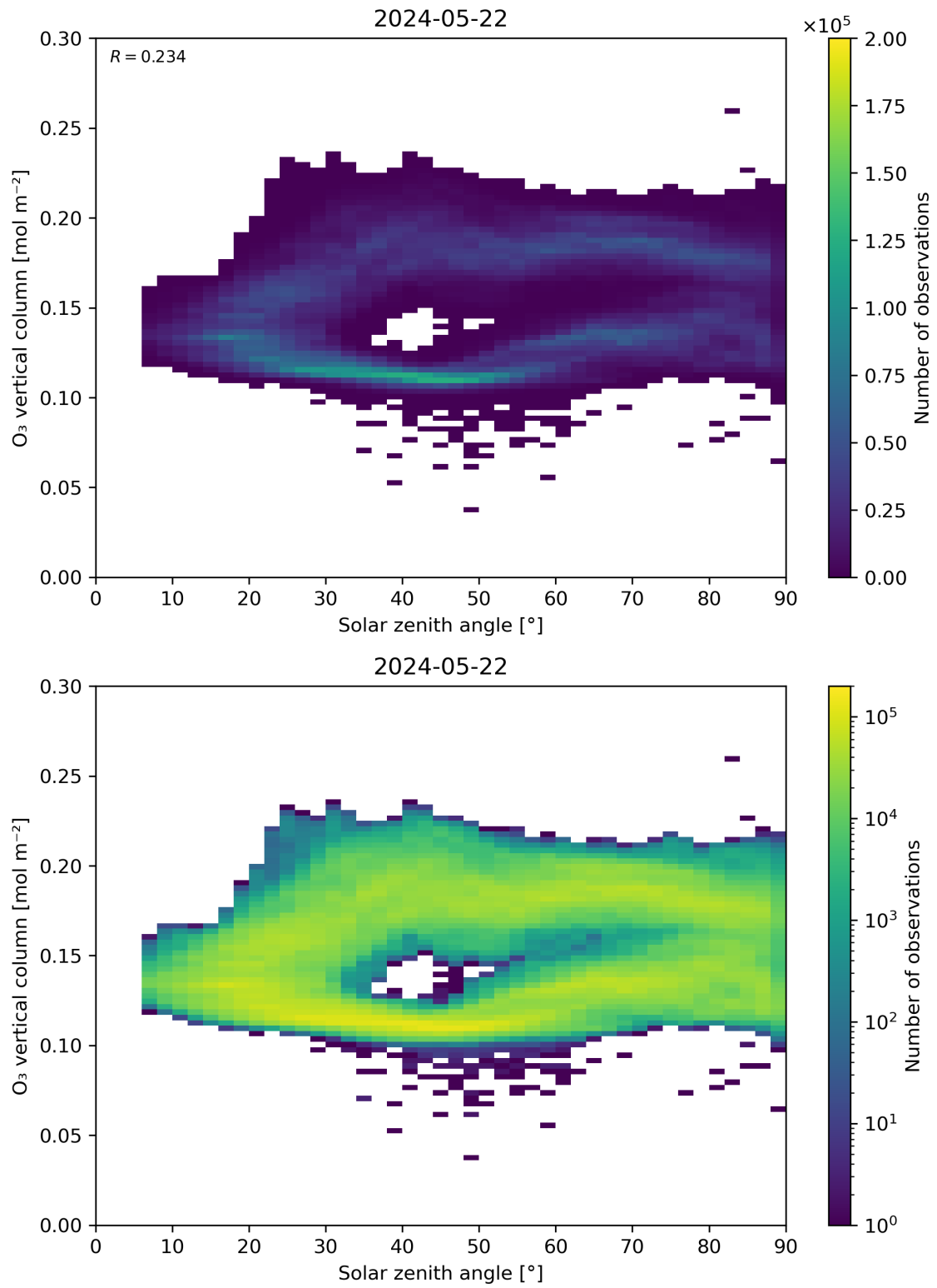
Figure 47: Scatter density plot of “Solar zenith angle” against “O 3 vertical column” for 2024-05-21 to 2024-05-23.
