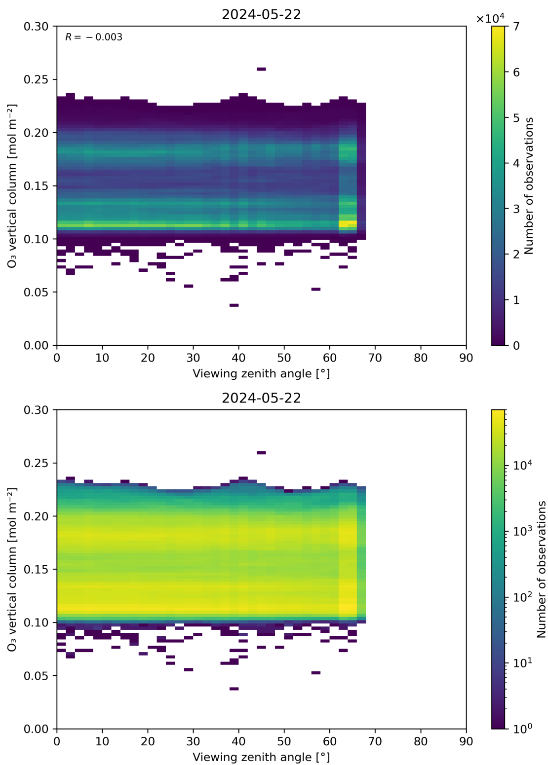
Figure 52: Scatter density plot of “Viewing zenith angle” against “O 3 vertical column” for 2024-05-21 to 2024-05-23.
