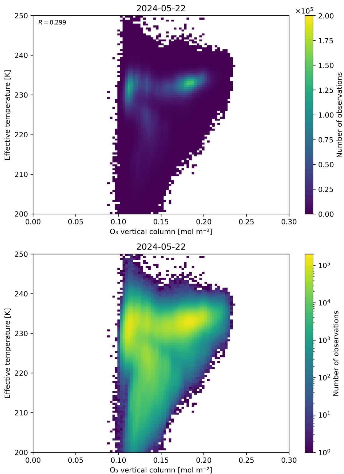
Figure 39: Scatter density plot of “O 3 vertical column” against “Effective temperature” for 2024-05-21 to 2024-05-23.
