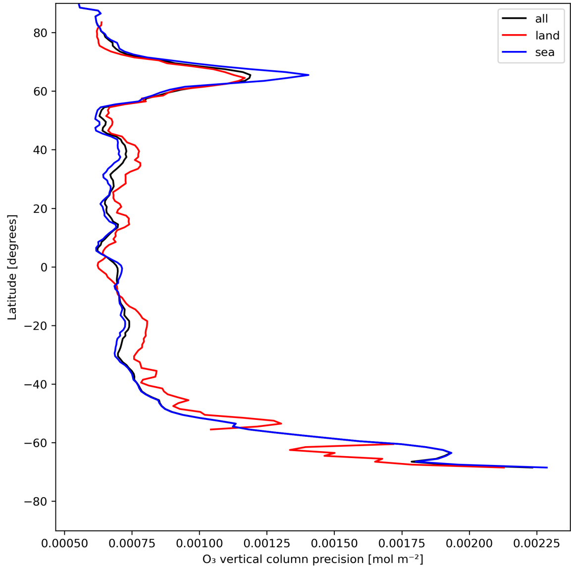
Figure 15: Zonal average of “O 3 vertical column precision” for 2024-05-21 to 2024-05-23.
