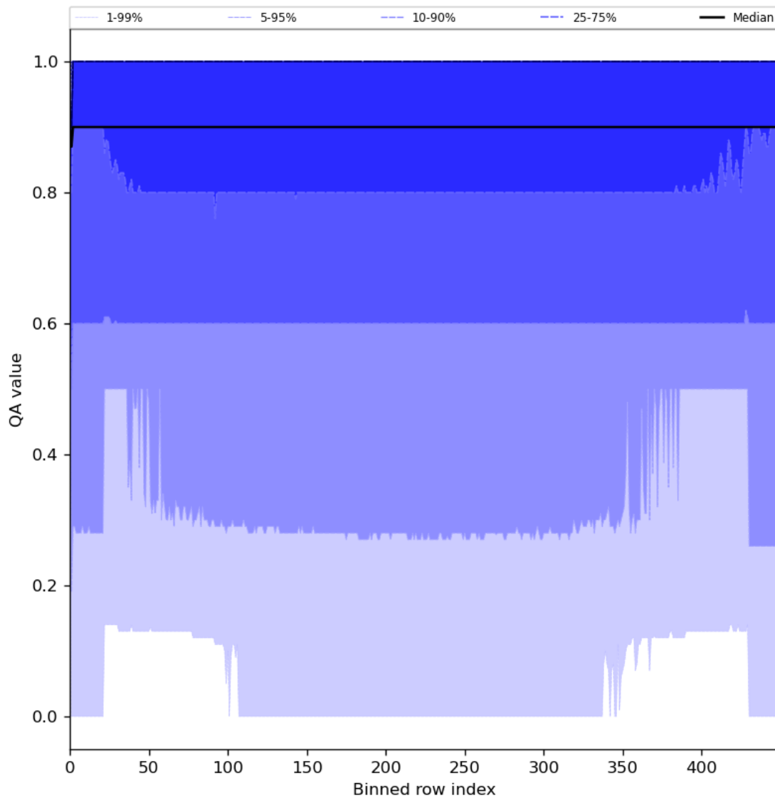
Figure 27: Along track statistics of “QA value” for 2024-05-21 to 2024-05-23
