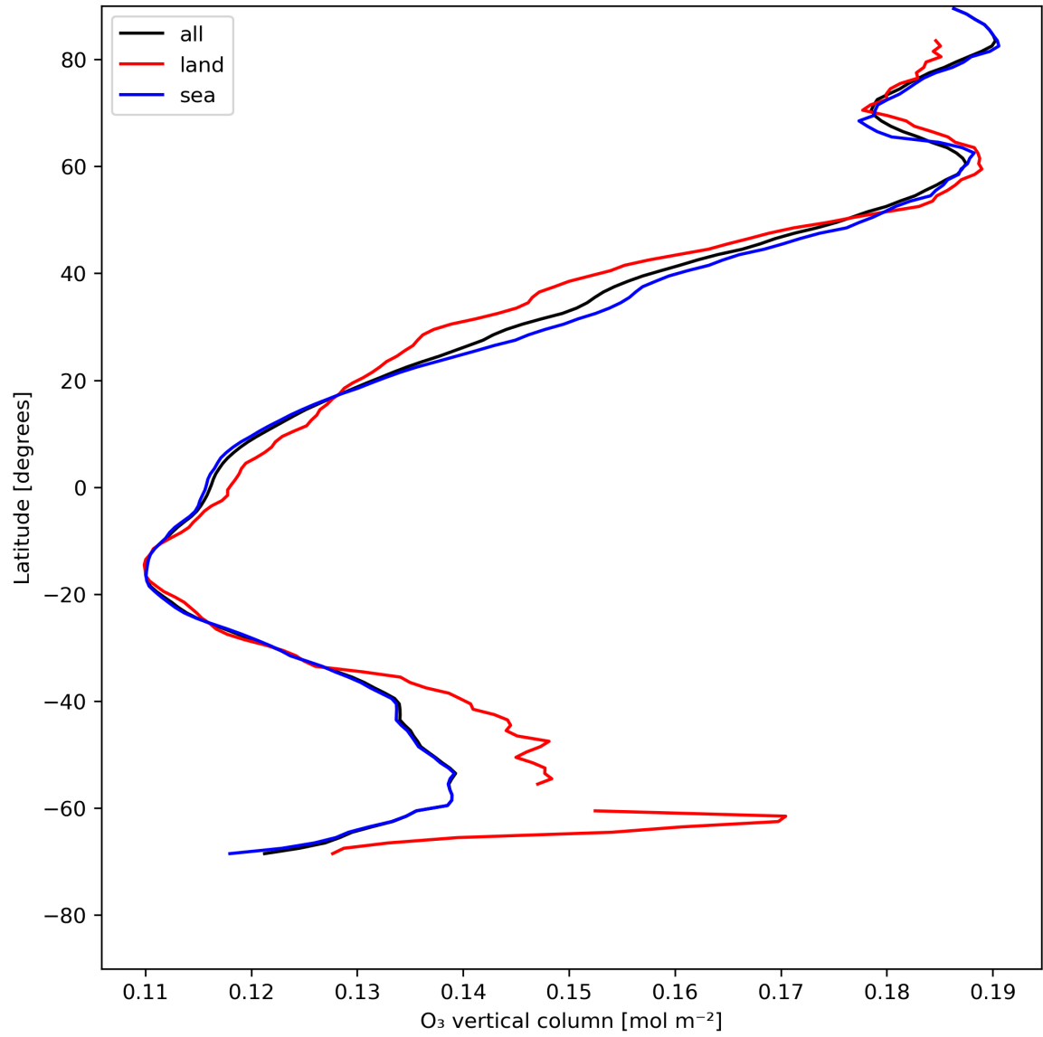
Figure 14: Zonal average of “O 3 vertical column” for 2024-05-21 to 2024-05-23.
