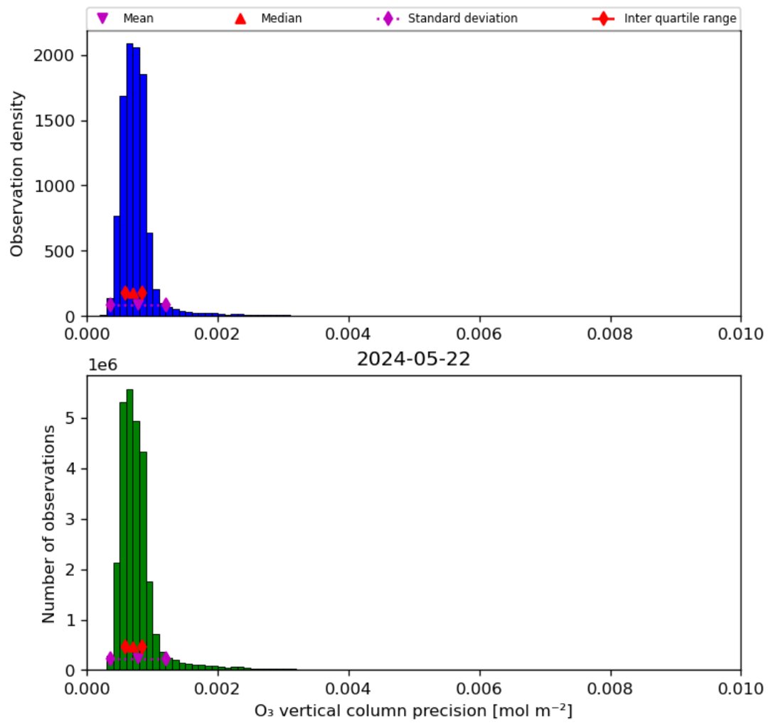
Figure 22: Histogram of “O 3 vertical column precision” for 2024-05-21 to 2024-05-23
