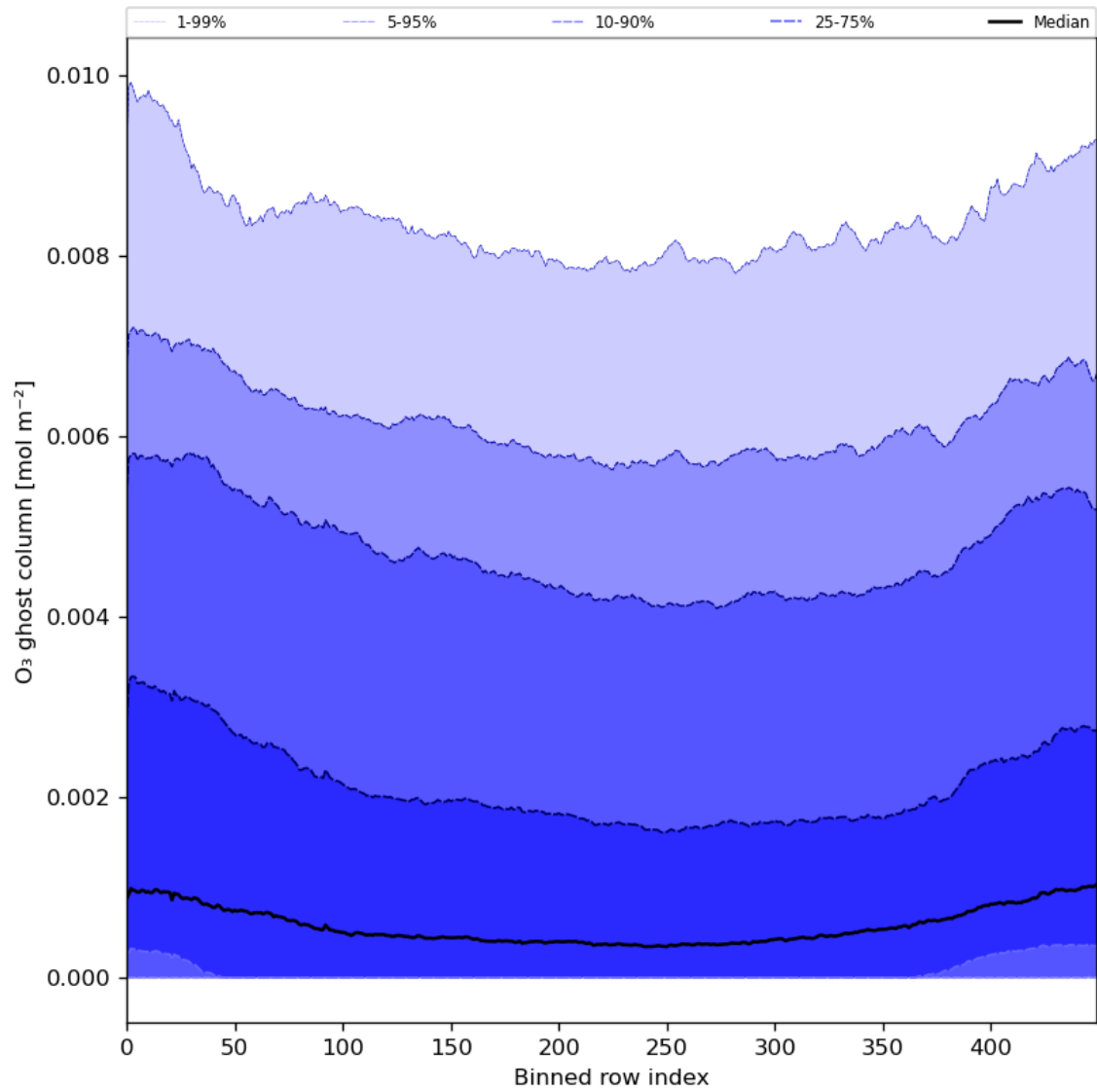
Figure 32: Along track statistics of “O 3 ghost column” for 2024-05-21 to 2024-05-23
