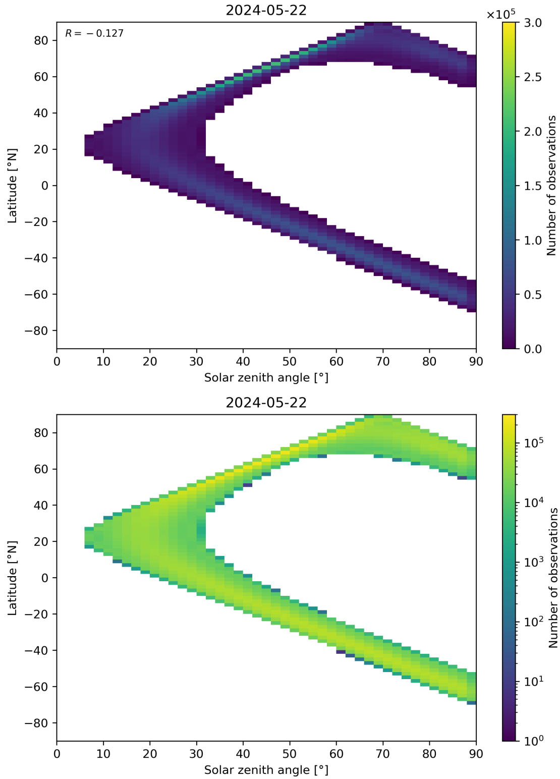
Figure 44: Scatter density plot of “Solar zenith angle” against “Latitude” for 2024-05-21 to 2024-05-23.
