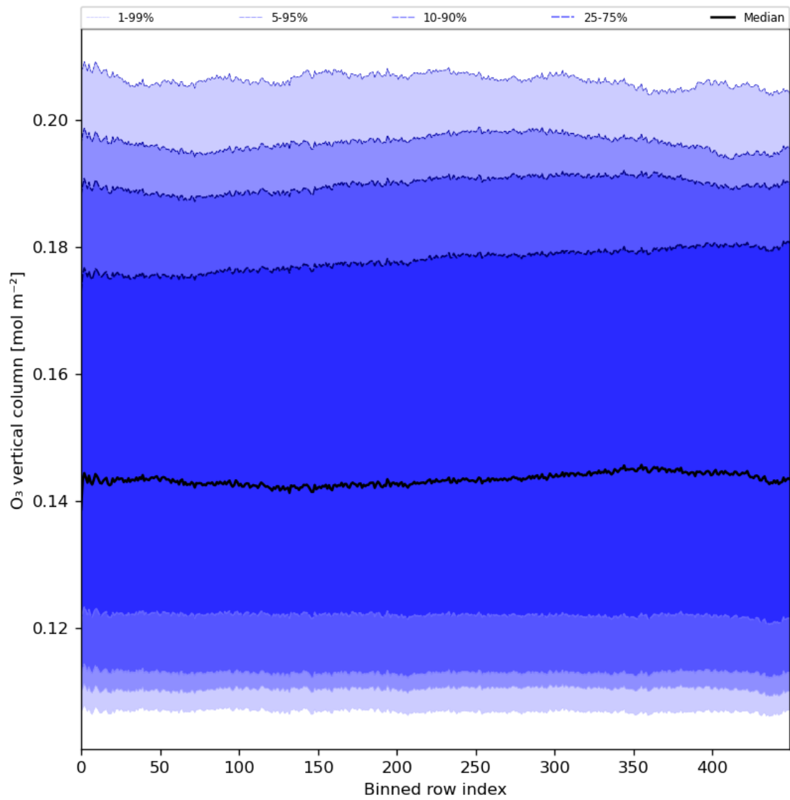
Figure 28: Along track statistics of “O 3 vertical column” for 2024-05-21 to 2024-05-23
