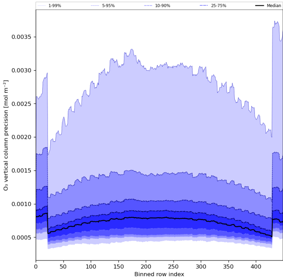
Figure 29: Along track statistics of “O 3 vertical column precision” for 2024-05-21 to 2024-05-23
