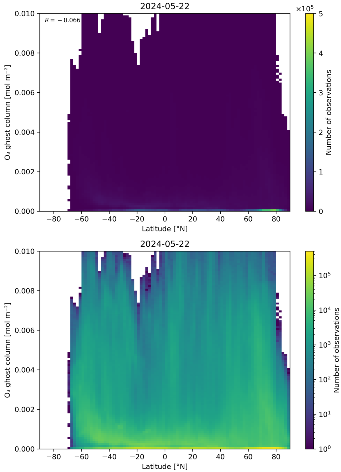
Figure 35: Scatter density plot of “Latitude” against “O 3 ghost column” for 2024-05-21 to 2024-05-23.
