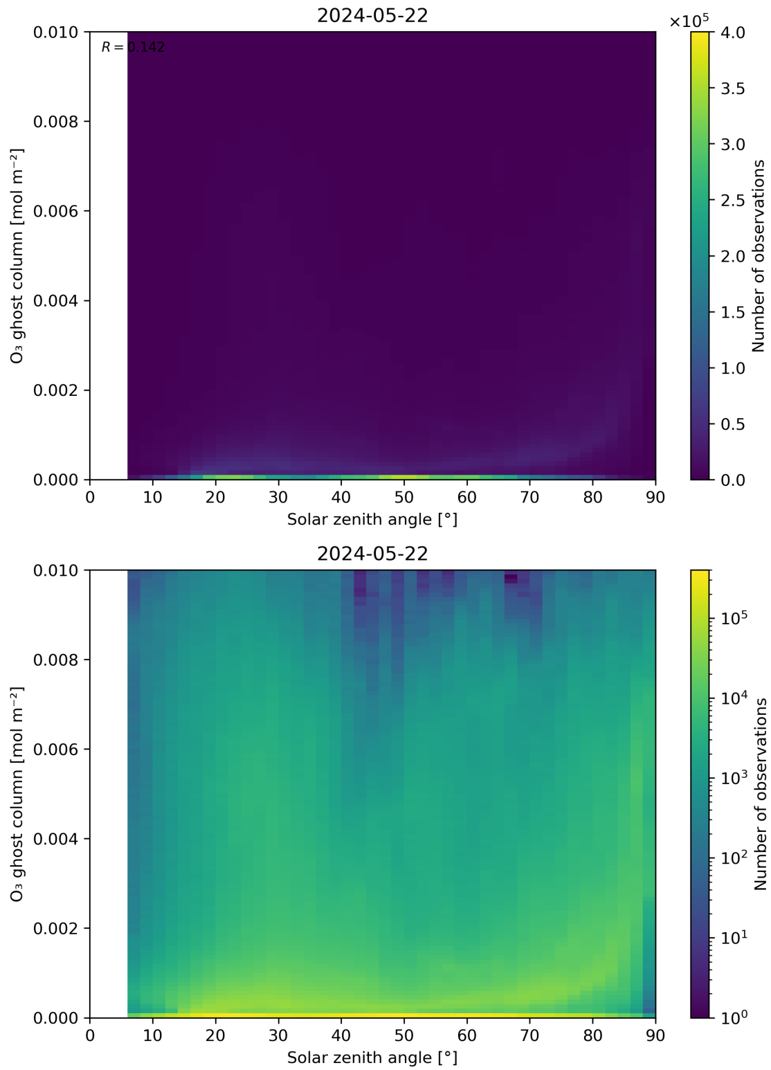
Figure 46: Scatter density plot of “Solar zenith angle” against “O 3 ghost column” for 2024-05-21 to 2024-05-23.
