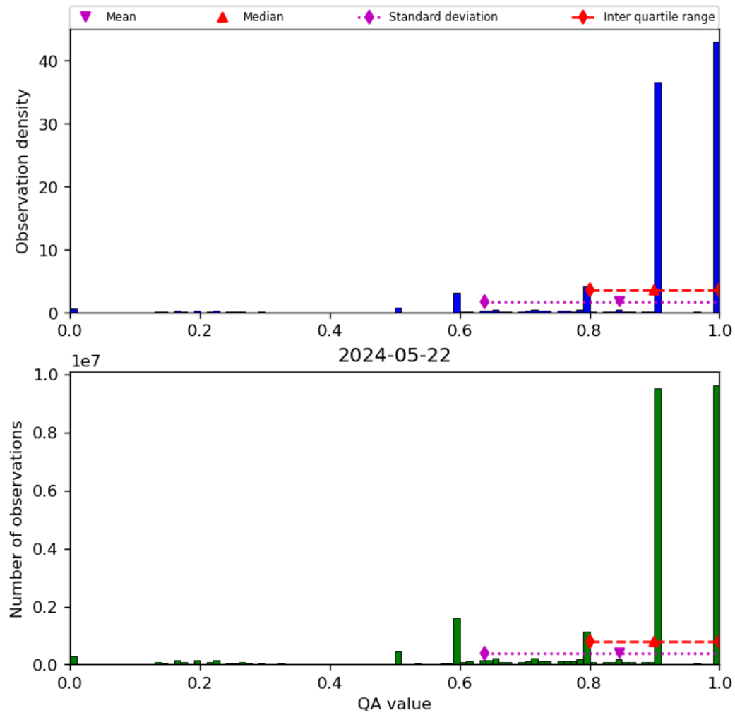
Figure 20: Histogram of “QA value” for 2024-05-21 to 2024-05-23
