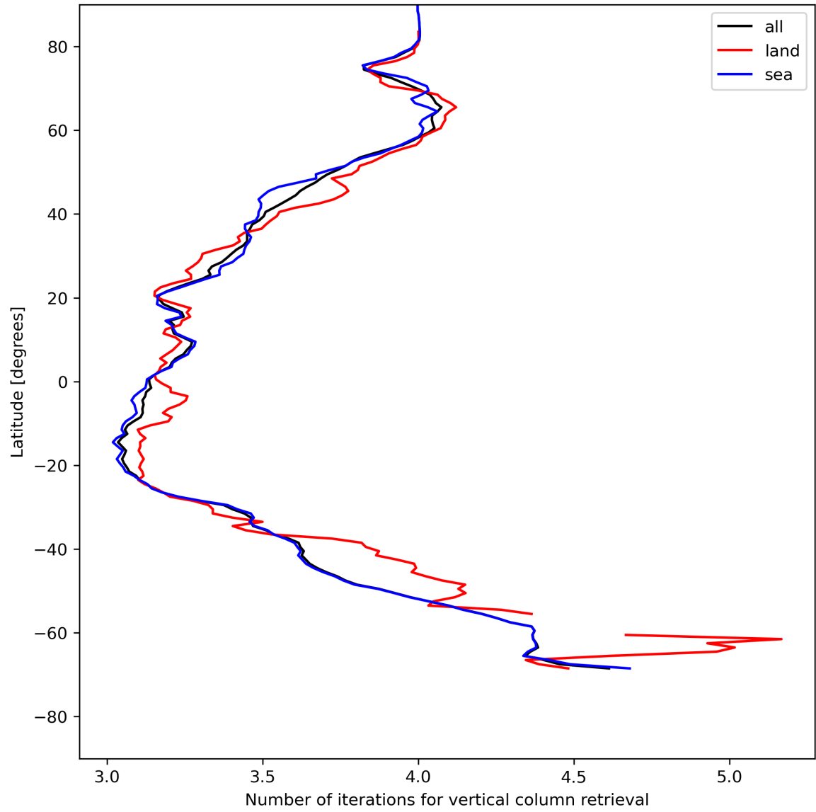
Figure 19: Zonal average of “Number of iterations for vertical column retrieval” for 2024-05-21 to 2024-05-23.
