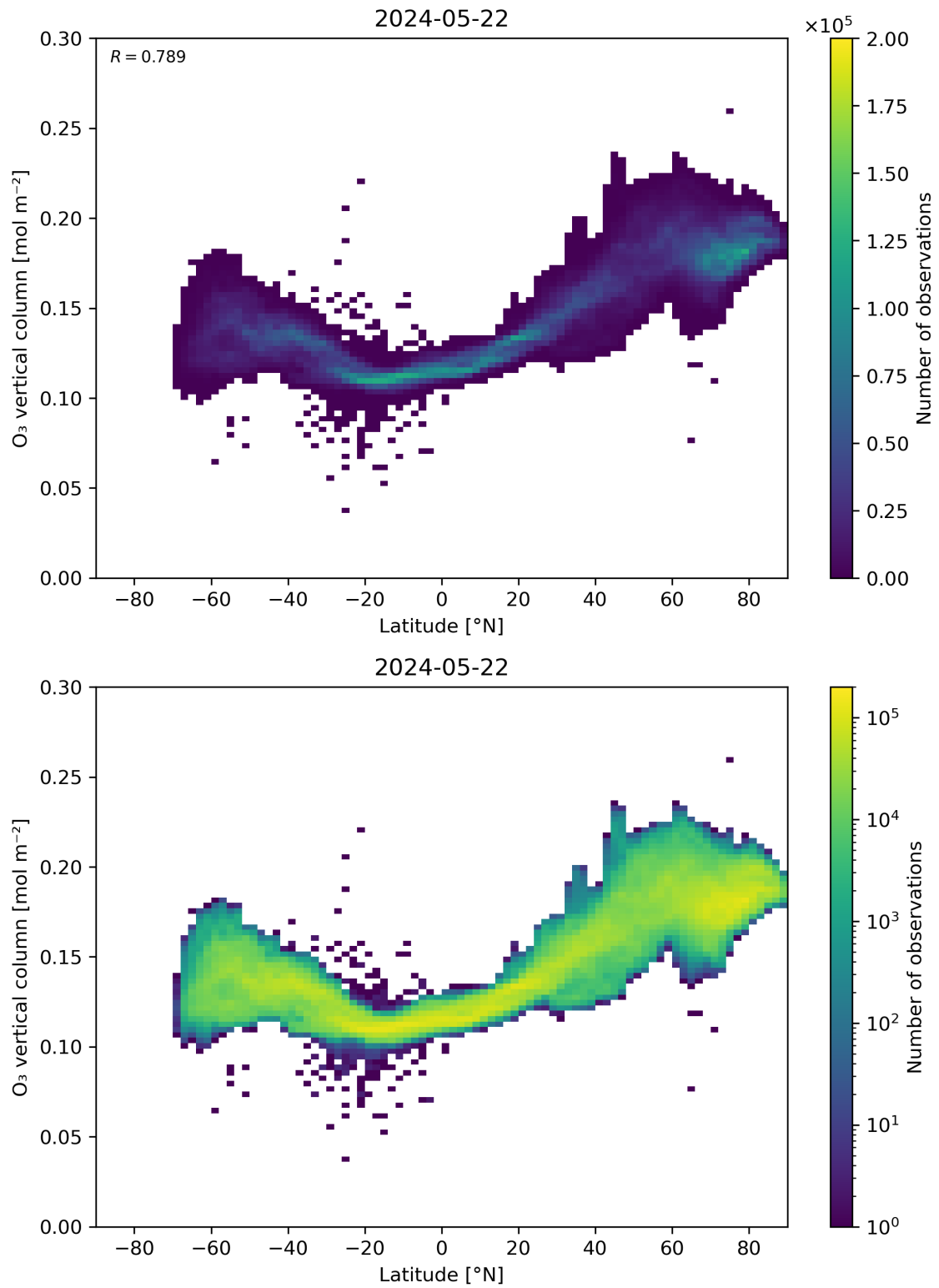
Figure 36: Scatter density plot of “Latitude” against “O 3 vertical column” for 2024-05-21 to 2024-05-23.
