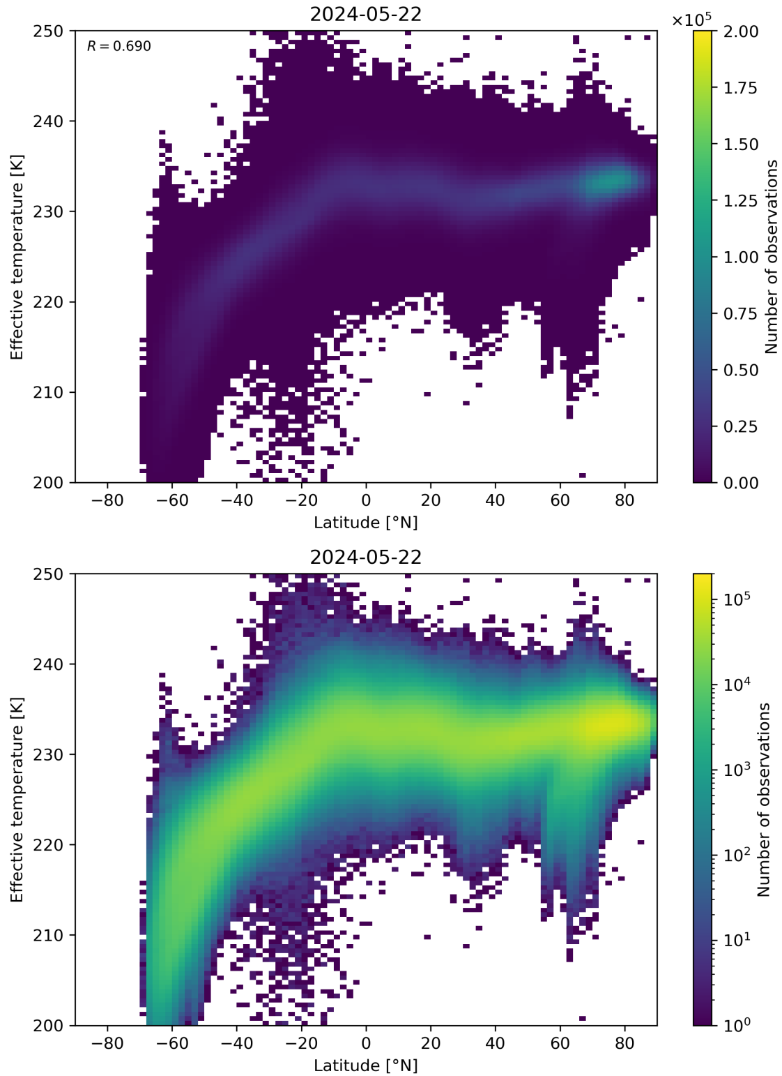
Figure 34: Scatter density plot of “Latitude” against “Effective temperature” for 2024-05-21 to 2024-05-23.
