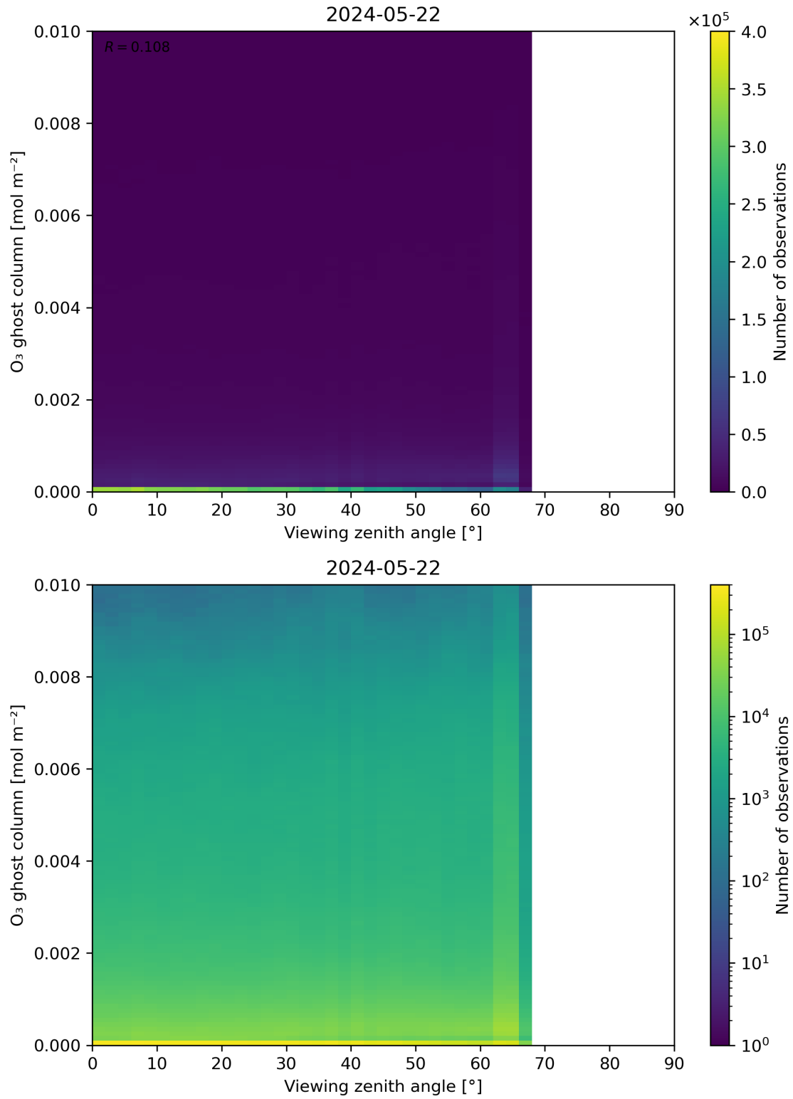
Figure 51: Scatter density plot of “Viewing zenith angle” against “O 3 ghost column” for 2024-05-21 to 2024-05-23.
