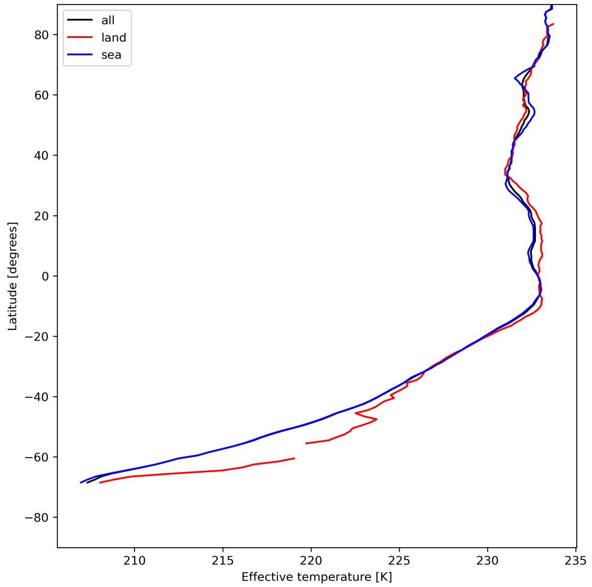
Figure 17: Zonal average of "Effective temperature" for 2024-05-21 to 2024-05-23.
