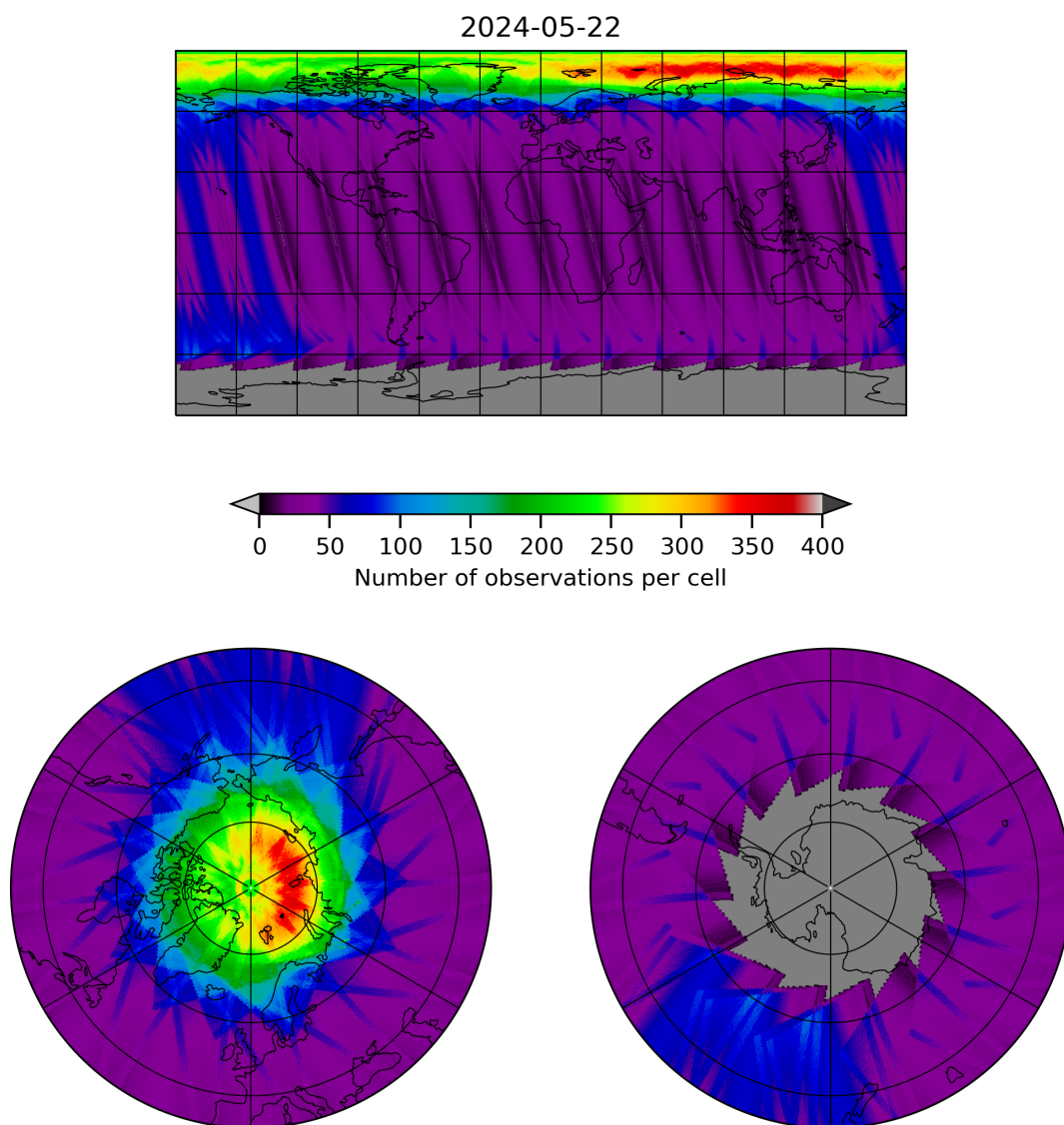
Figure 12: Map of the number of observations for 2024-05-21 to 2024-05-23
