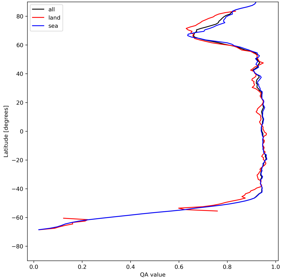
Figure 13: Zonal average of “QA value” for 2024-05-21 to 2024-05-23.
