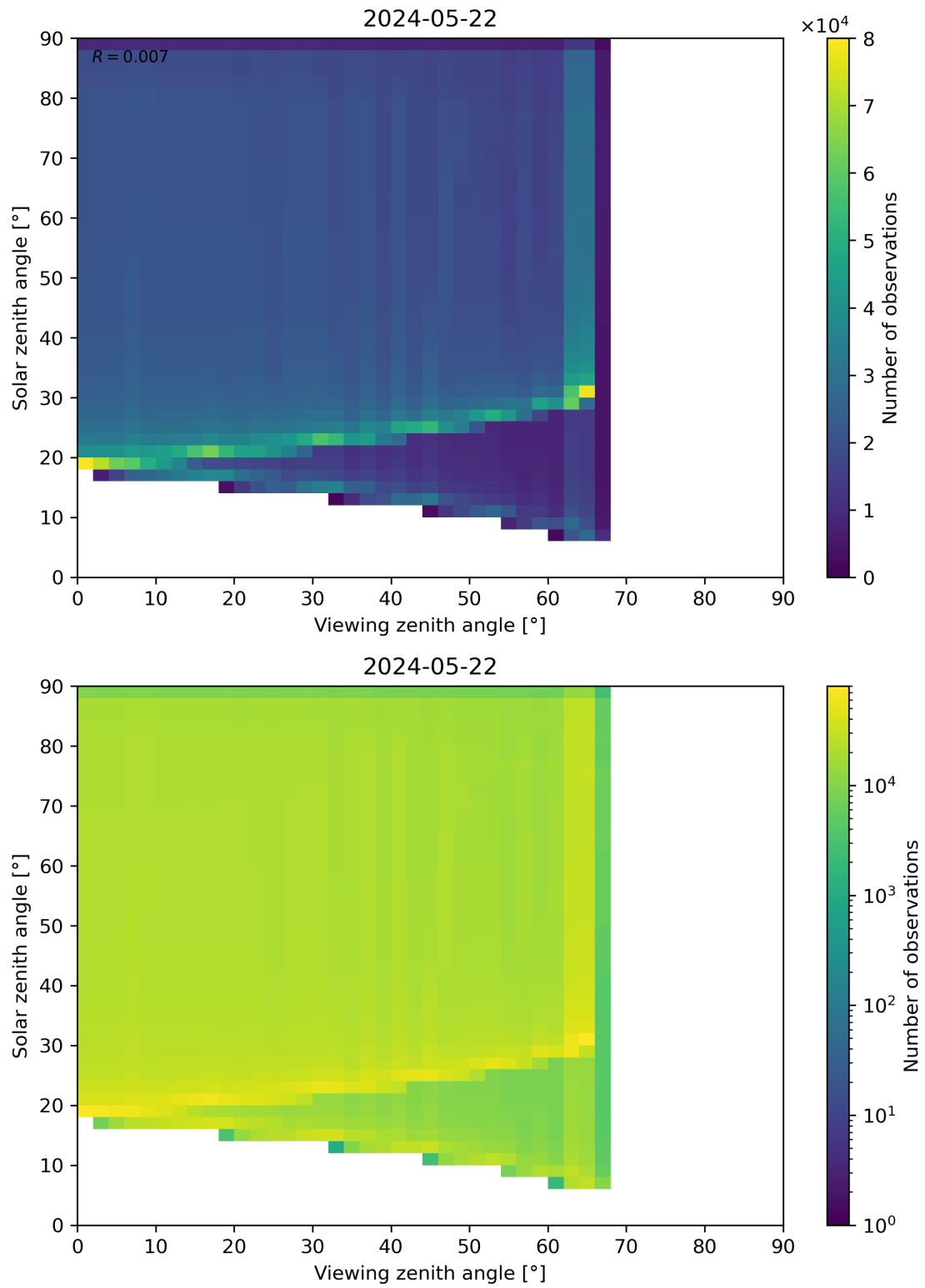
Figure 54: Scatter density plot of “Viewing zenith angle” against “Solar zenith angle” for 2024-05-21 to 2024-05-23.
