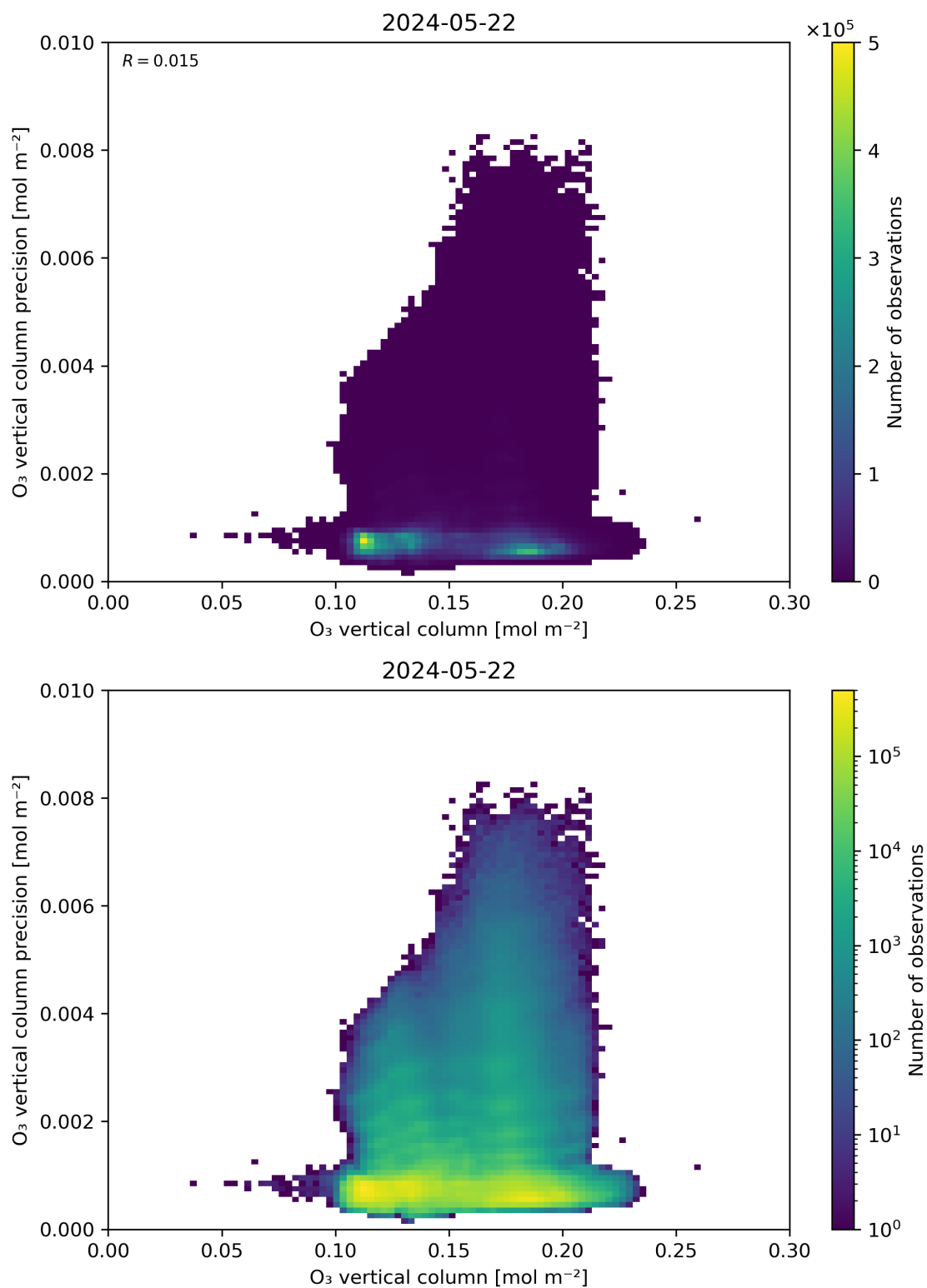
Figure 41: Scatter density plot of “O 3 vertical column” against “O 3 vertical column precision” for 2024-05-21 to 2024-05-23.
