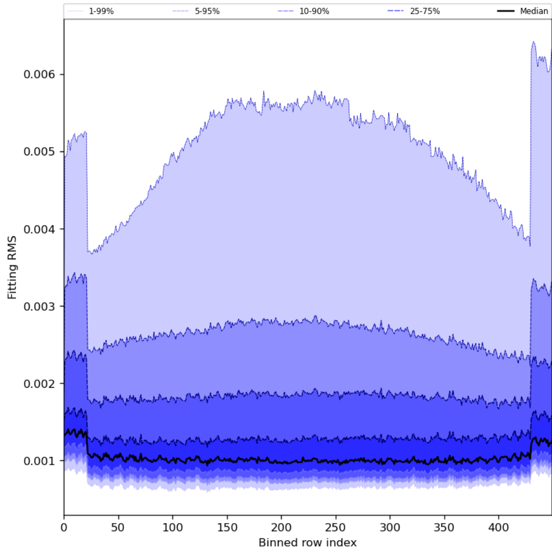
Figure 30: Along track statistics of “Fitting RMS” for 2024-05-21 to 2024-05-23
