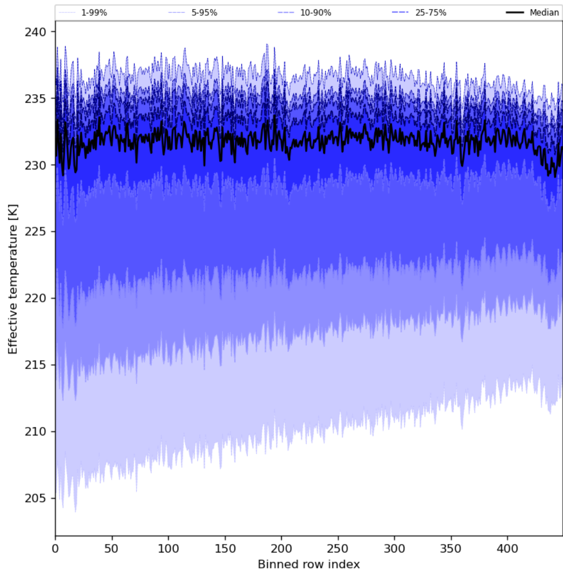
Figure 31: Along track statistics of “Effective temperature” for 2024-05-21 to 2024-05-23
