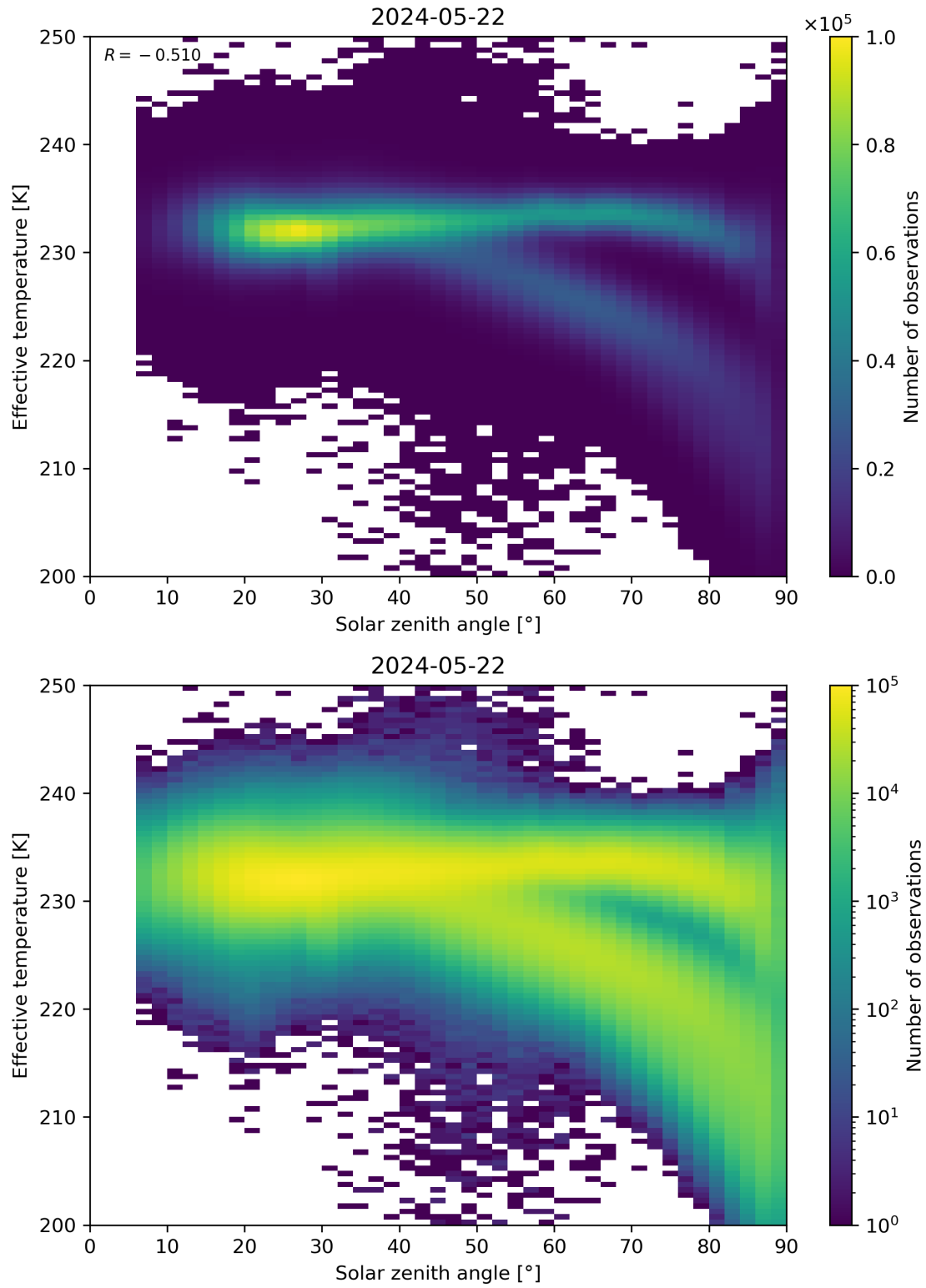
Figure 45: Scatter density plot of “Solar zenith angle” against “Effective temperature” for 2024-05-21 to 2024-05-23.
