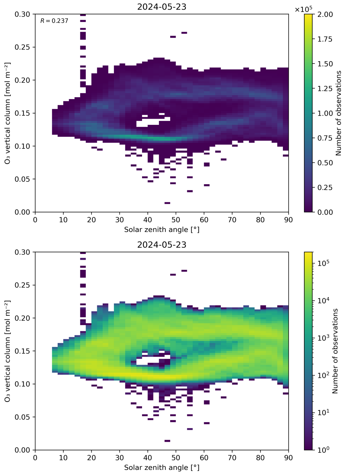
Figure 47: Scatter density plot of “Solar zenith angle” against “O 3 vertical column” for 2024-05-23 to 2024-05-24.
