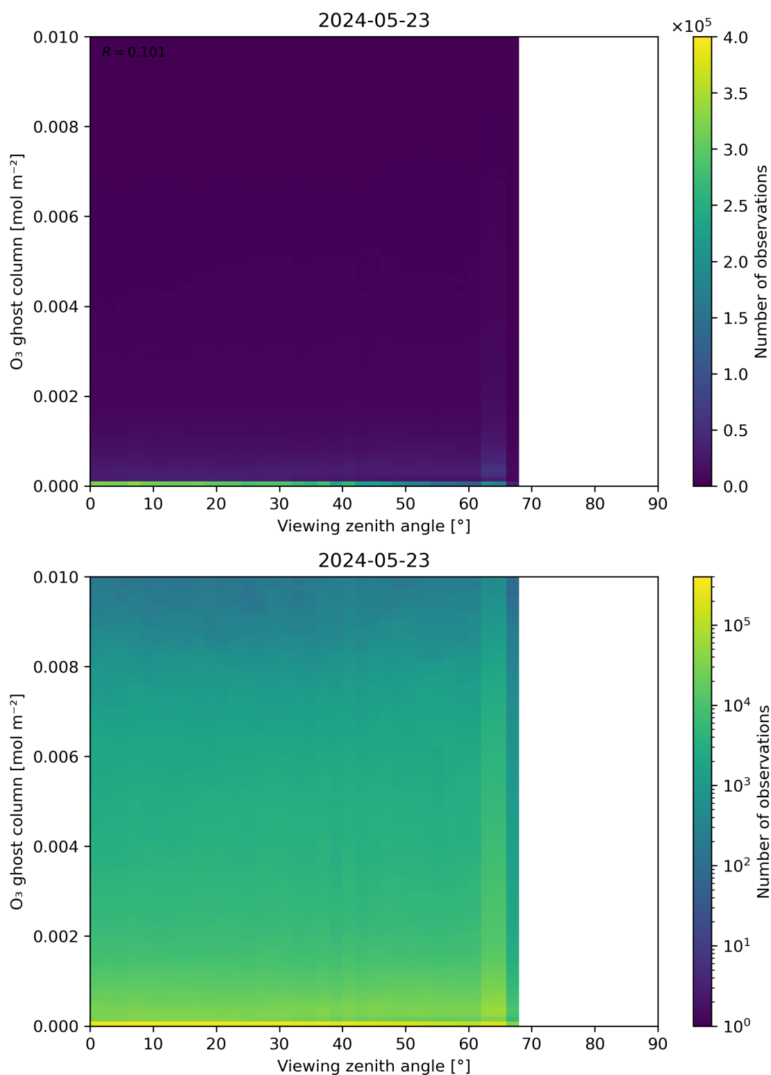
Figure 51: Scatter density plot of “Viewing zenith angle” against “O 3 ghost column” for 2024-05-23 to 2024-05-24.
