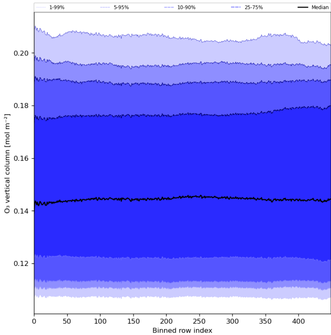
Figure 28: Along track statistics of “O 3 vertical column” for 2024-05-23 to 2024-05-24
