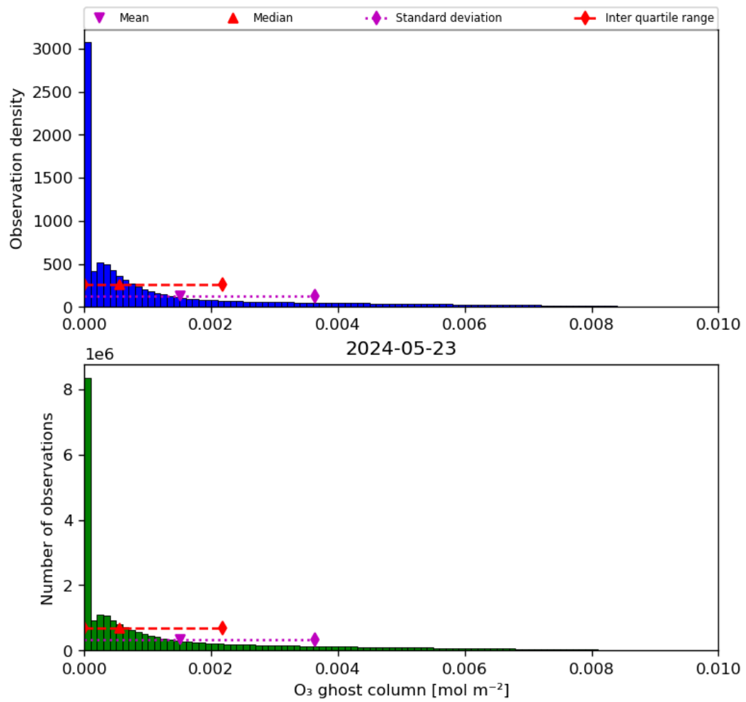
Figure 25: Histogram of “O 3 ghost column” for 2024-05-23 to 2024-05-24
