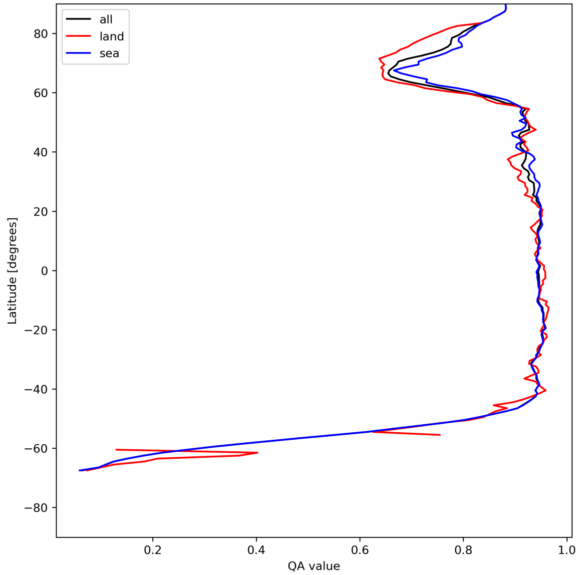
Figure 13: Zonal average of “QA value” for 2024-05-23 to 2024-05-24.
