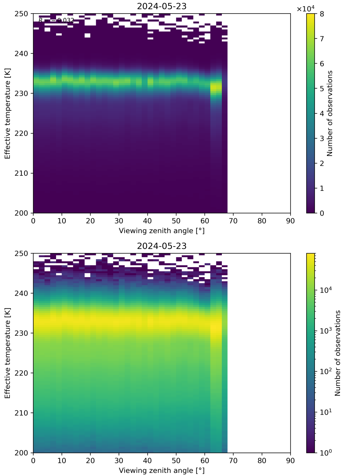
Figure 50: Scatter density plot of “Viewing zenith angle” against “Effective temperature” for 2024-05-23 to 2024-05-24.
