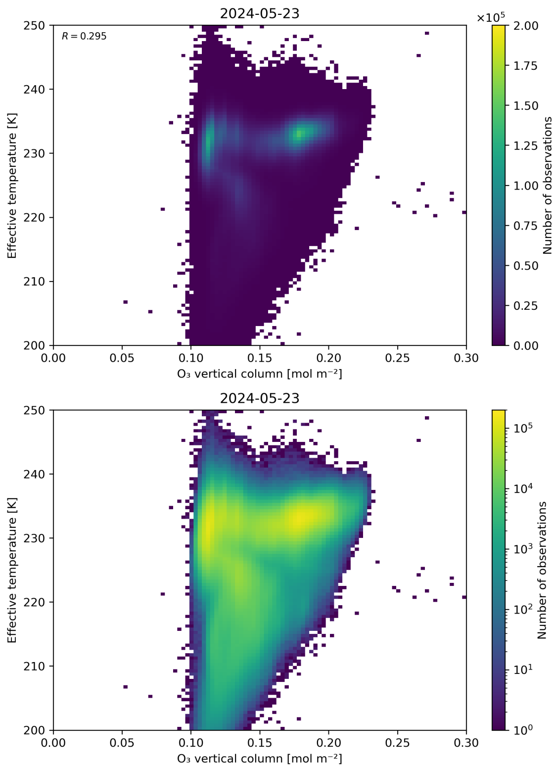
Figure 39: Scatter density plot of “O 3 vertical column” against “Effective temperature” for 2024-05-23 to 2024-05-24.
