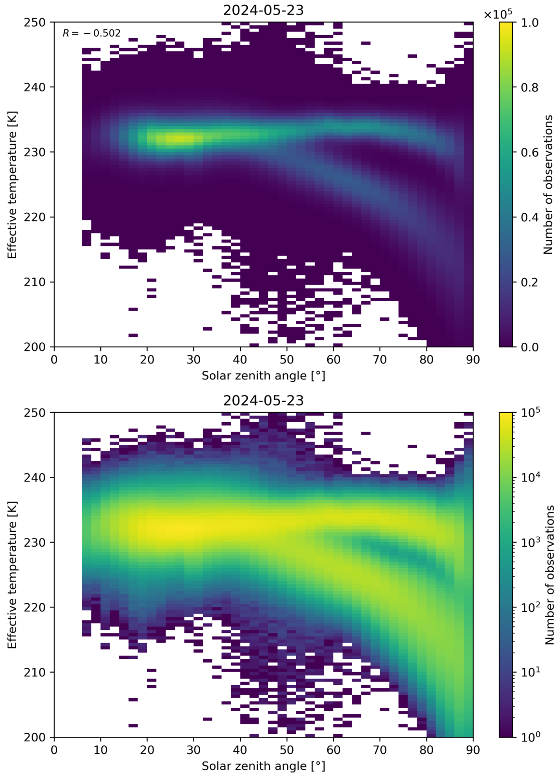
Figure 45: Scatter density plot of “Solar zenith angle” against “Effective temperature” for 2024-05-23 to 2024-05-24.
