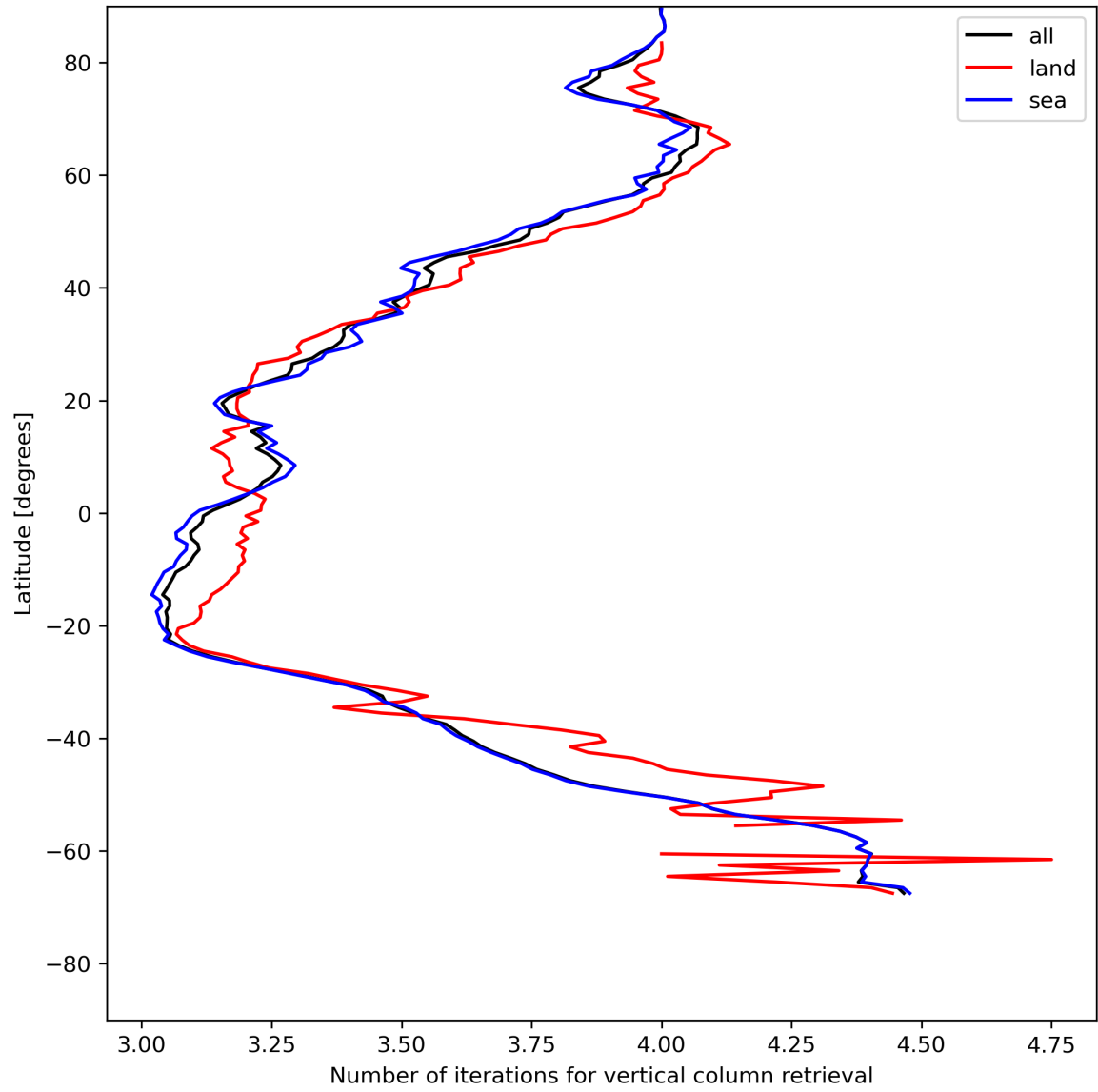
Figure 19: Zonal average of “Number of iterations for vertical column retrieval” for 2024-05-23 to 2024-05-24.
