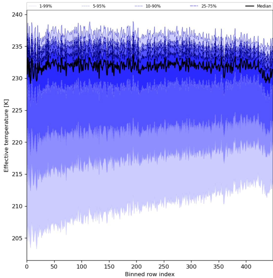
Figure 31: Along track statistics of “Effective temperature” for 2024-05-23 to 2024-05-24
