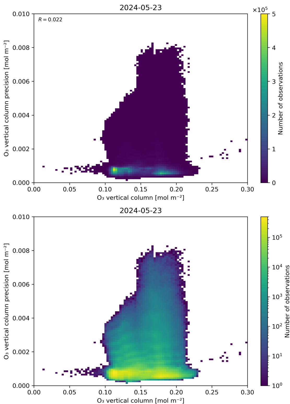
Figure 41: Scatter density plot of “O 3 vertical column” against “O 3 vertical column precision” for 2024-05-23 to 2024-05-24.
