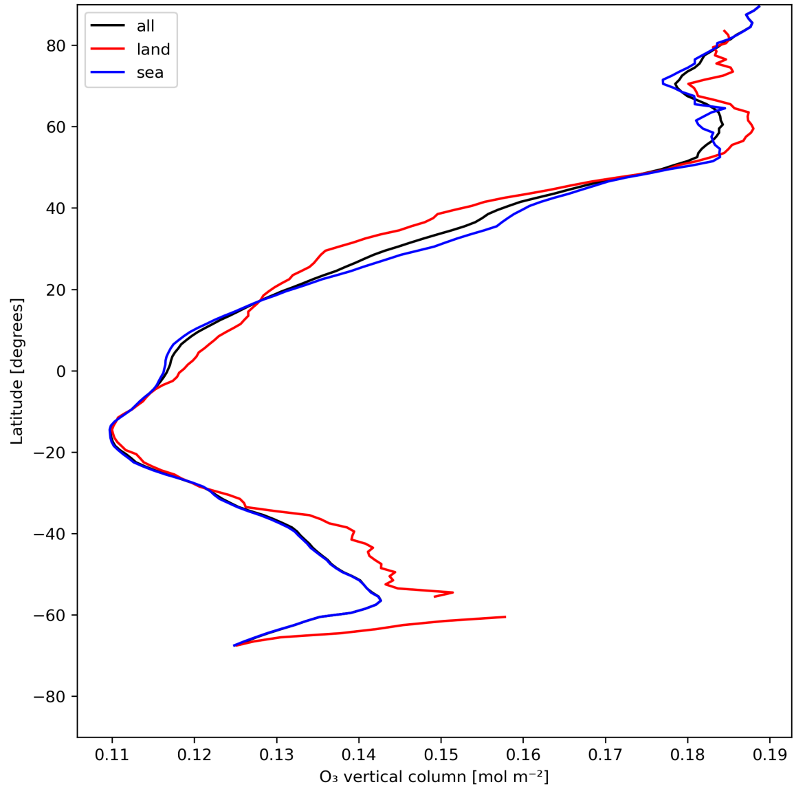
Figure 14: Zonal average of “O 3 vertical column” for 2024-05-23 to 2024-05-24.
