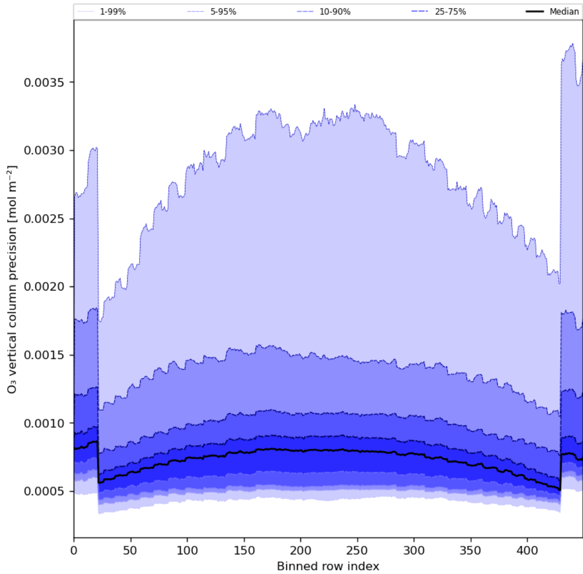
Figure 29: Along track statistics of “O 3 vertical column precision” for 2024-05-23 to 2024-05-24
