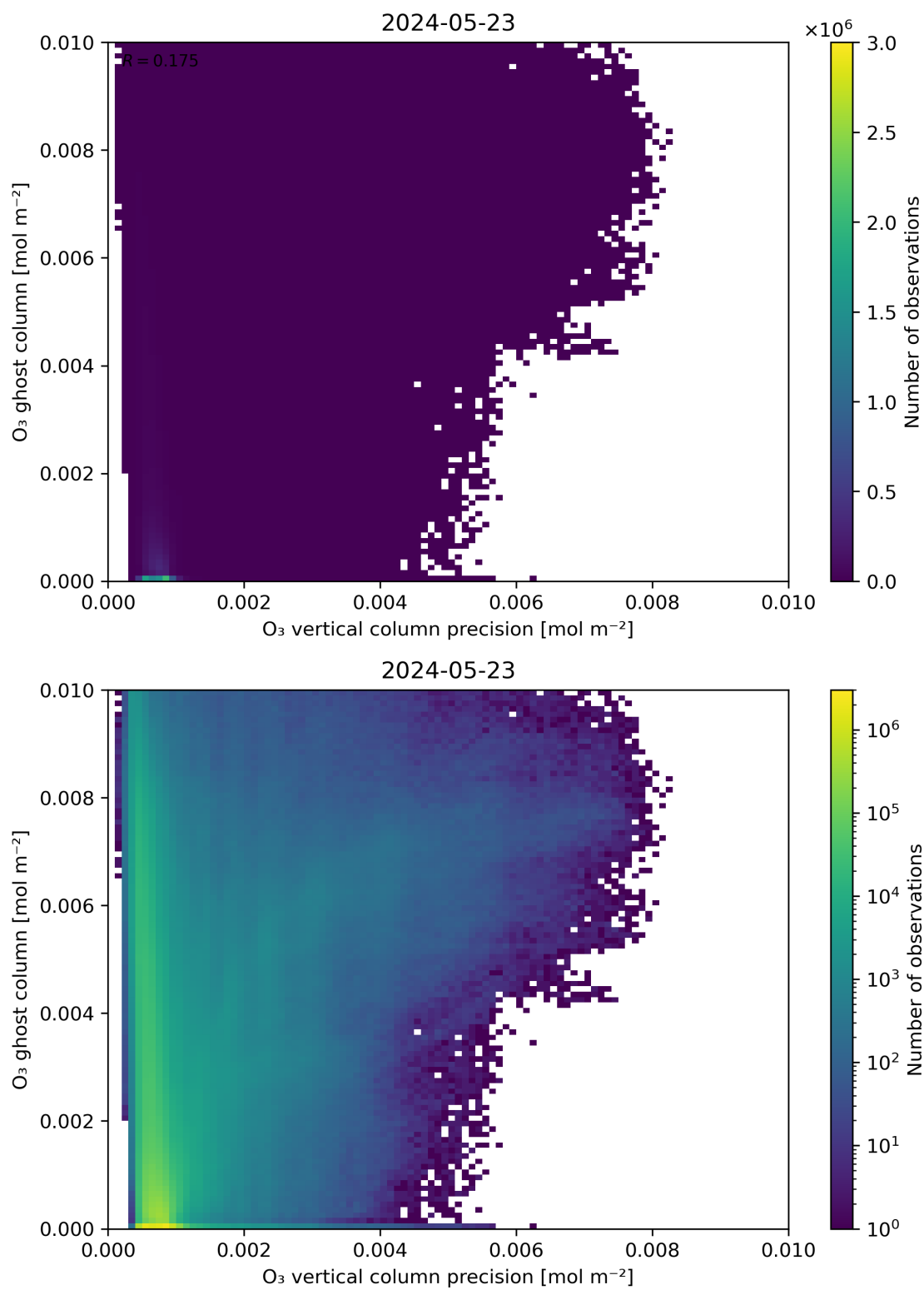
Figure 43: Scatter density plot of “ \text{O}_3 vertical column precision” against “ \text{O}_3 ghost column” for 2024-05-23 to 2024-05-24.
