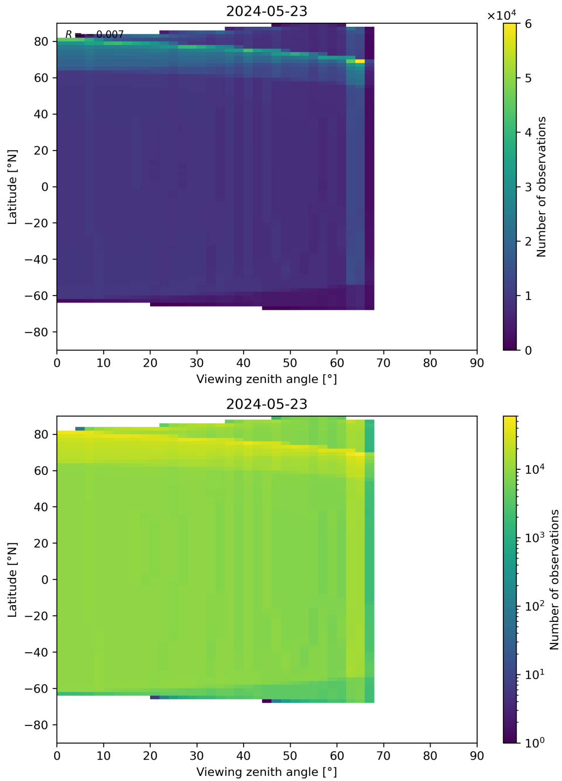
Figure 49: Scatter density plot of “Viewing zenith angle” against “Latitude” for 2024-05-23 to 2024-05-24.
