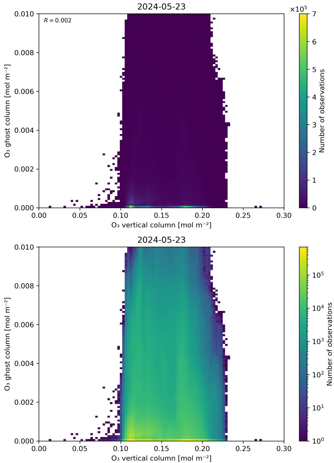
Figure 40: Scatter density plot of “O 3 vertical column” against “O 3 ghost column” for 2024-05-23 to 2024-05-24.
