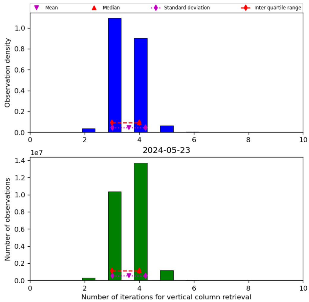
Figure 26: Histogram of “Number of iterations for vertical column retrieval” for 2024-05-23 to 2024-05-24
