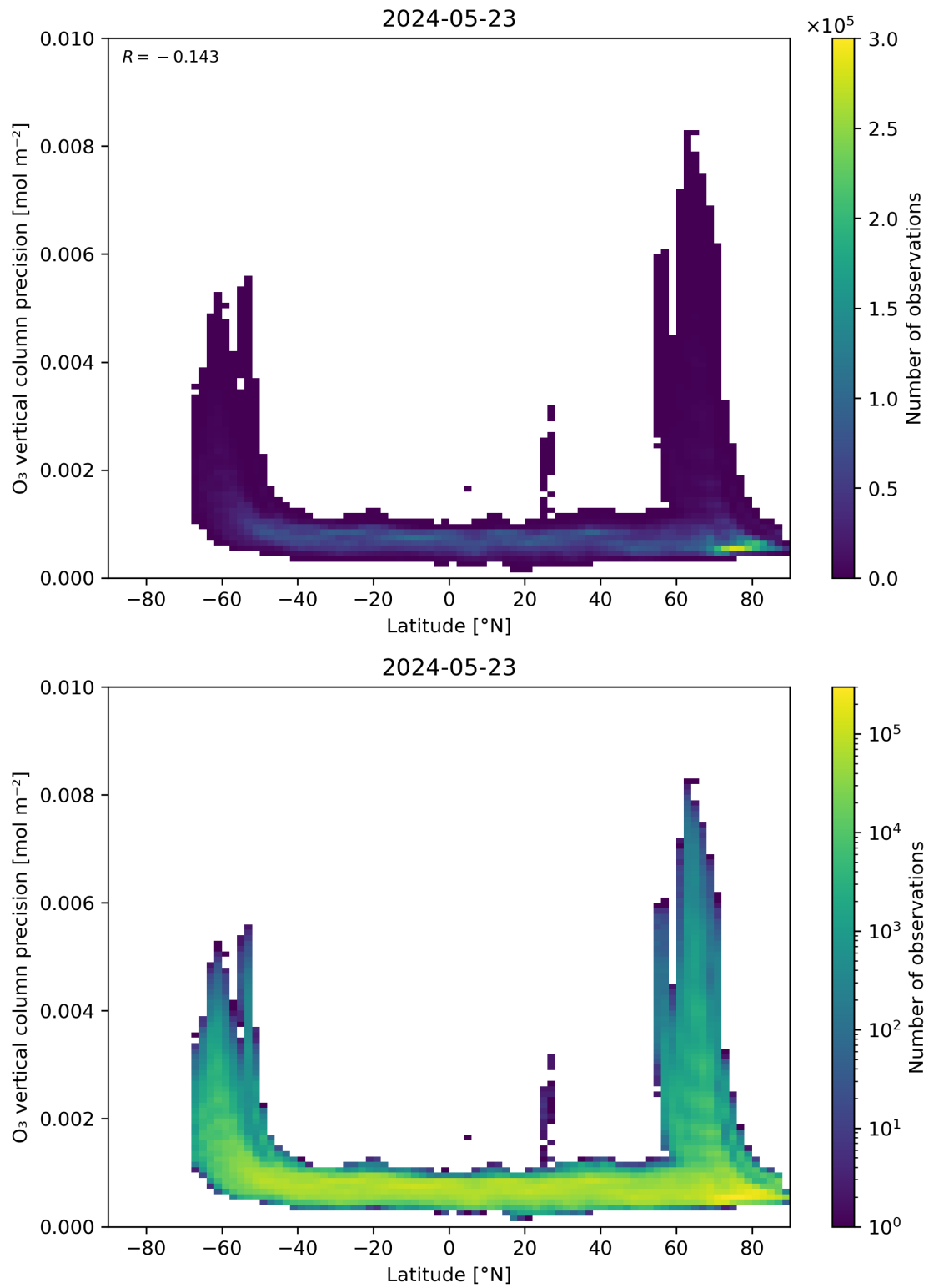
Figure 37: Scatter density plot of “Latitude” against “O 3 vertical column precision” for 2024-05-23 to 2024-05-24.
