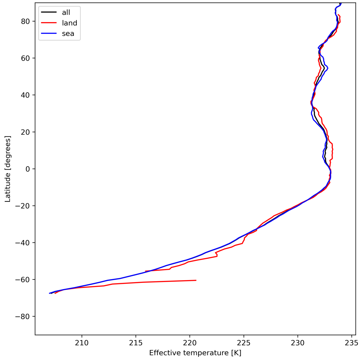
Figure 17: Zonal average of “Effective temperature” for 2024-05-23 to 2024-05-24.
