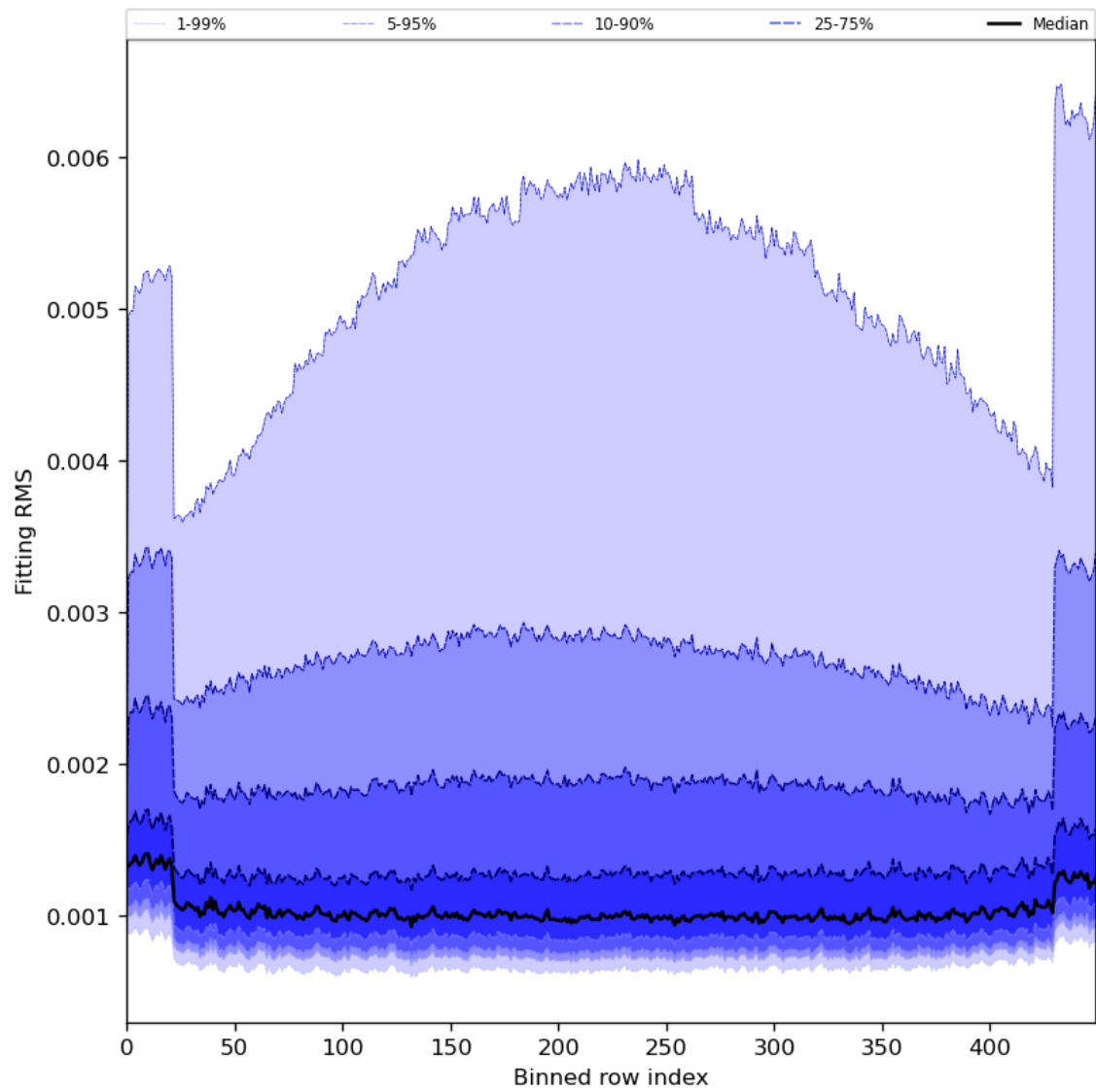
Figure 30: Along track statistics of “Fitting RMS” for 2024-05-23 to 2024-05-24
