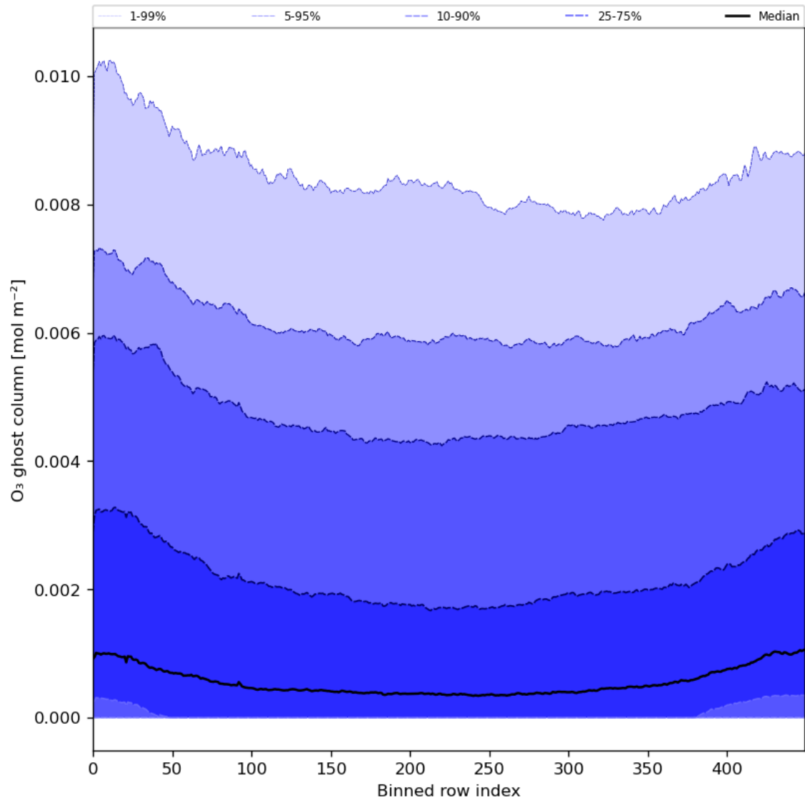
Figure 32: Along track statistics of “O 3 ghost column” for 2024-05-23 to 2024-05-24
