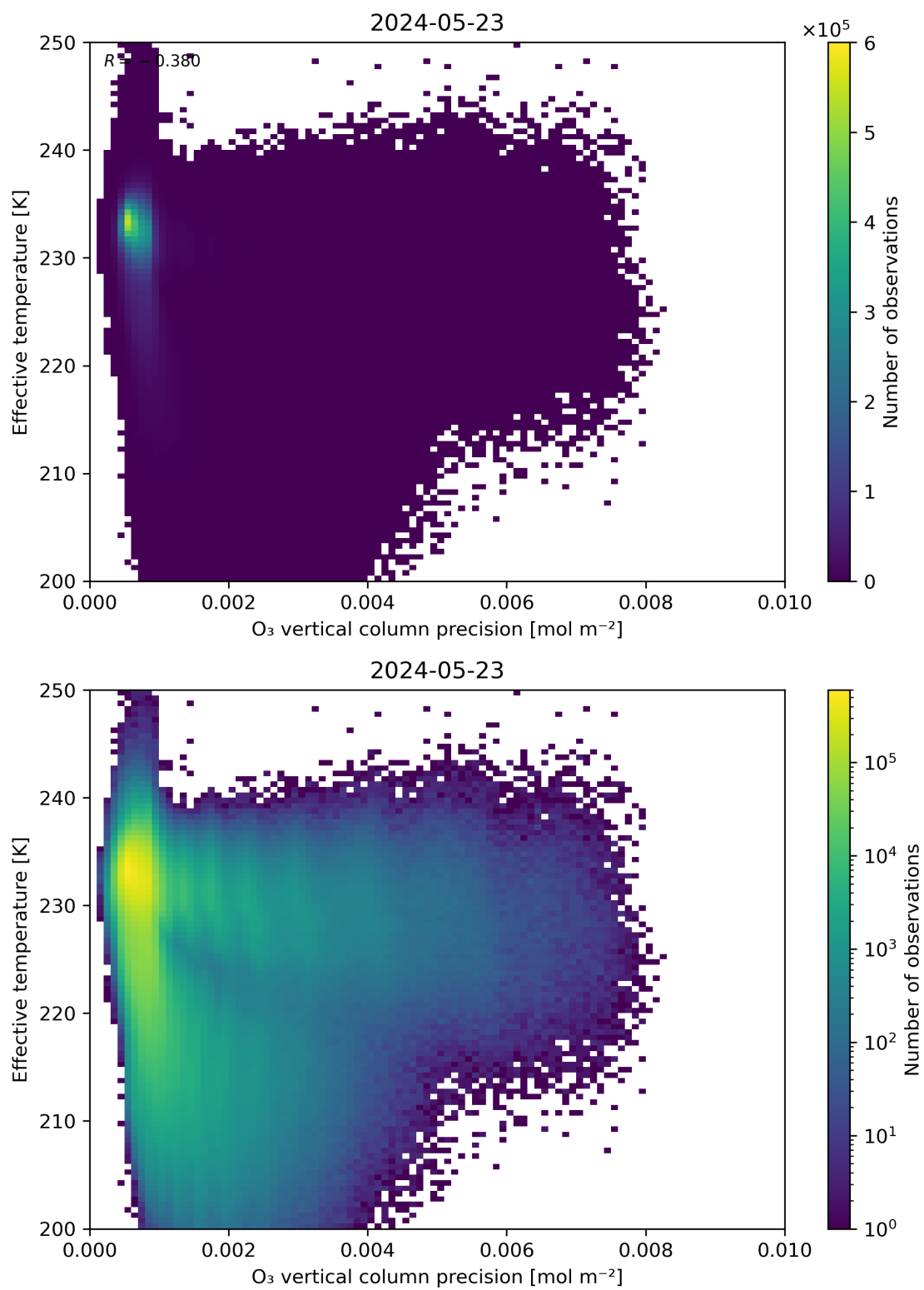
Figure 42: Scatter density plot of “O 3 vertical column precision” against “Effective temperature” for 2024-05-23 to 2024-05-24.
