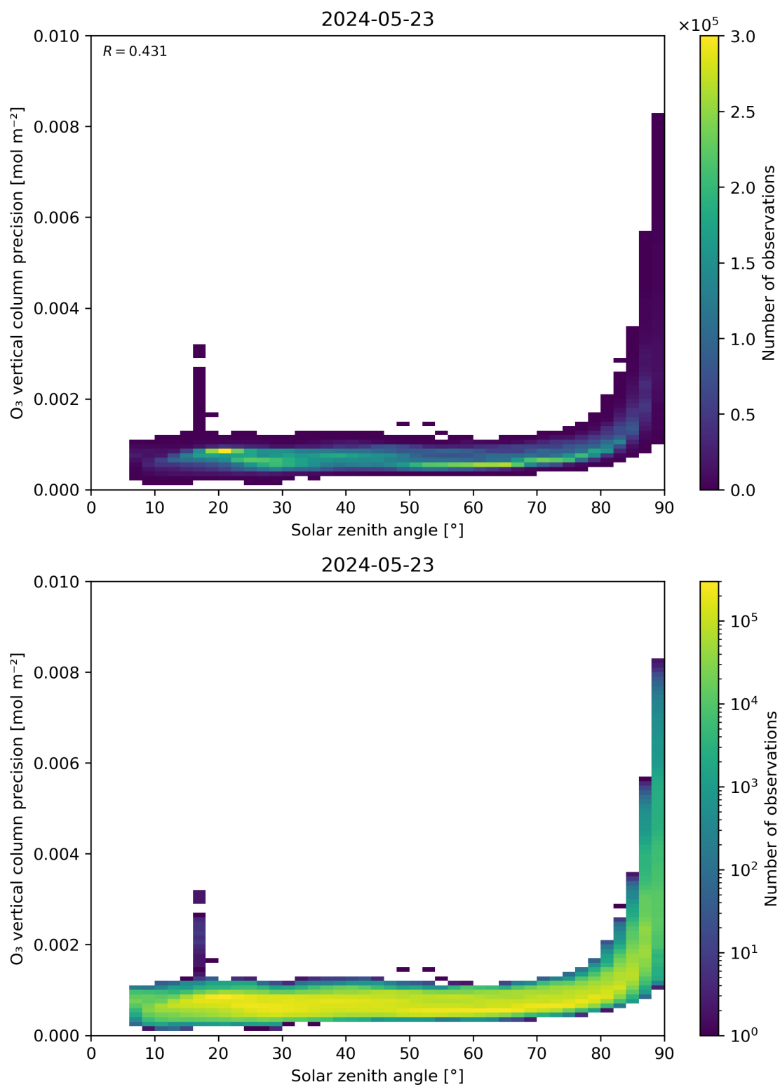
Figure 48: Scatter density plot of “Solar zenith angle” against “O 3 vertical column precision” for 2024-05-23 to 2024-05-24.
