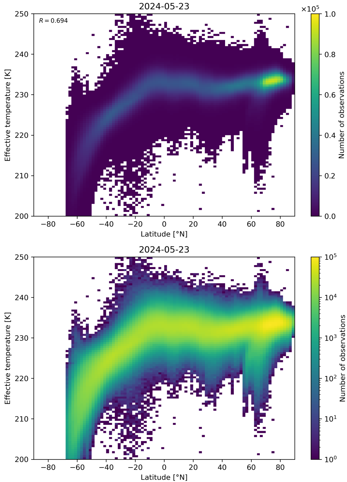
Figure 34: Scatter density plot of “Latitude” against “Effective temperature” for 2024-05-23 to 2024-05-24.
