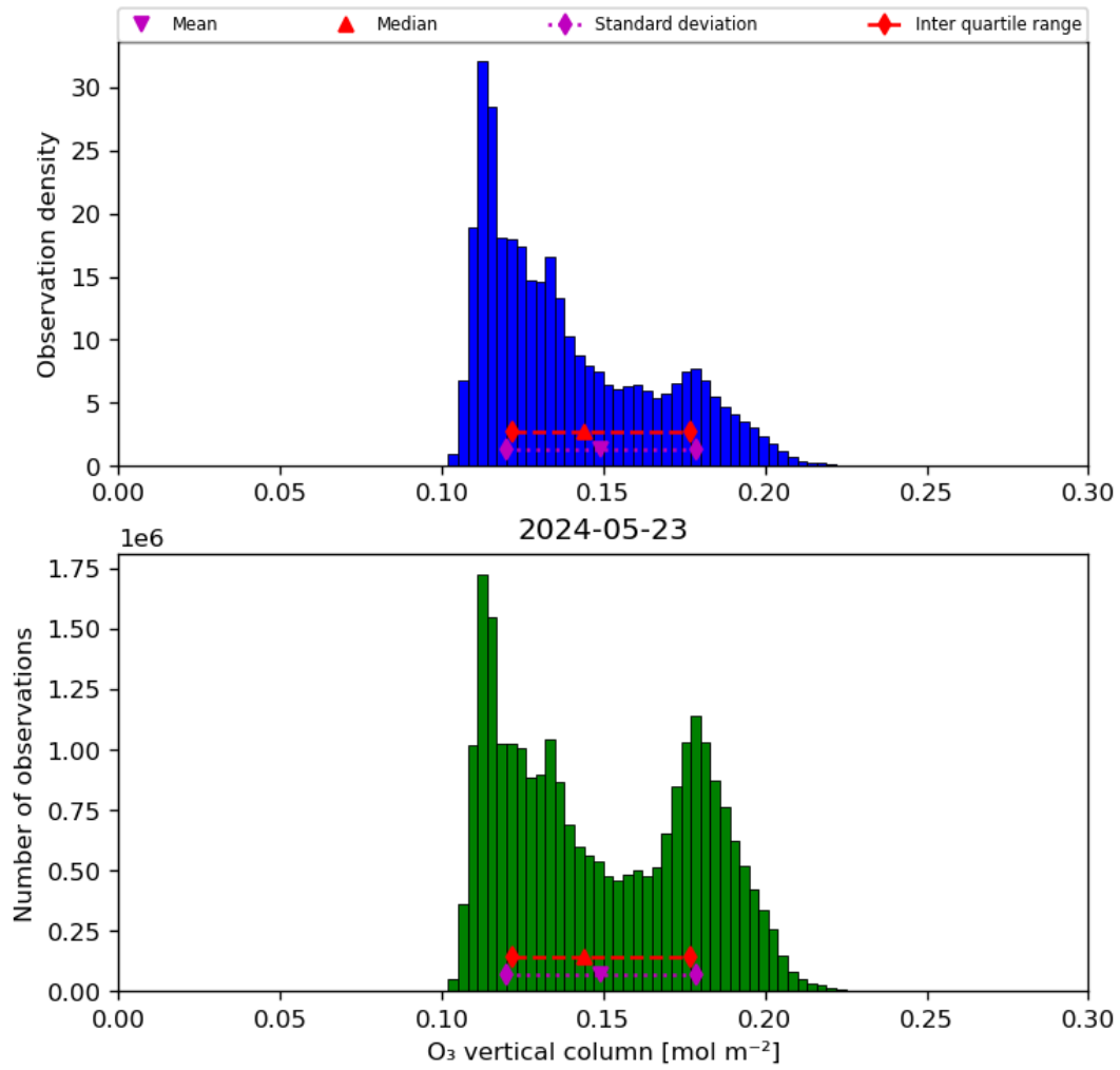
Figure 21: Histogram of “O 3 vertical column” for 2024-05-23 to 2024-05-24
