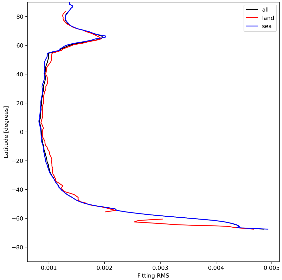
Figure 16: Zonal average of “Fitting RMS” for 2024-05-23 to 2024-05-24.
