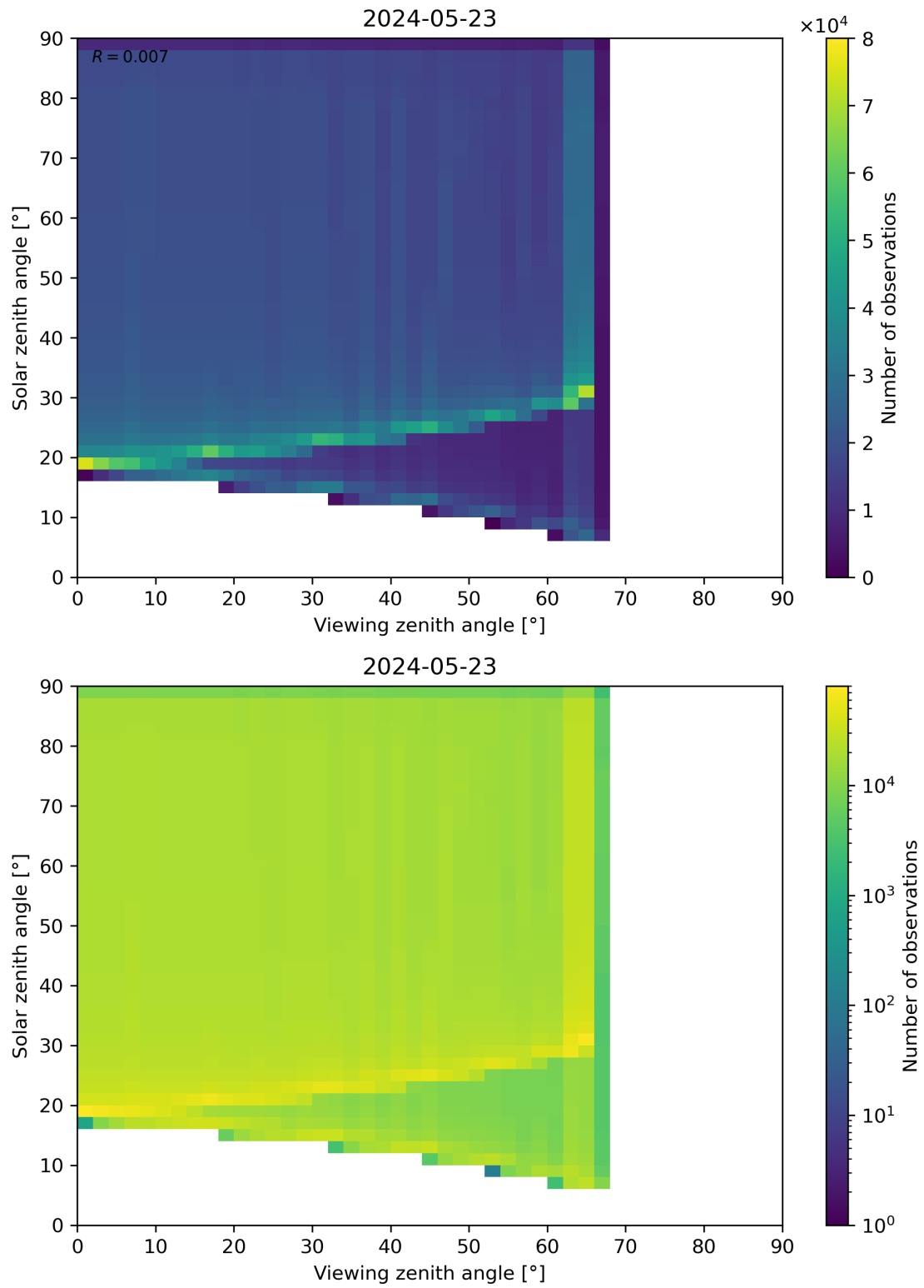
Figure 54: Scatter density plot of “Viewing zenith angle” against “Solar zenith angle” for 2024-05-23 to 2024-05-24.
