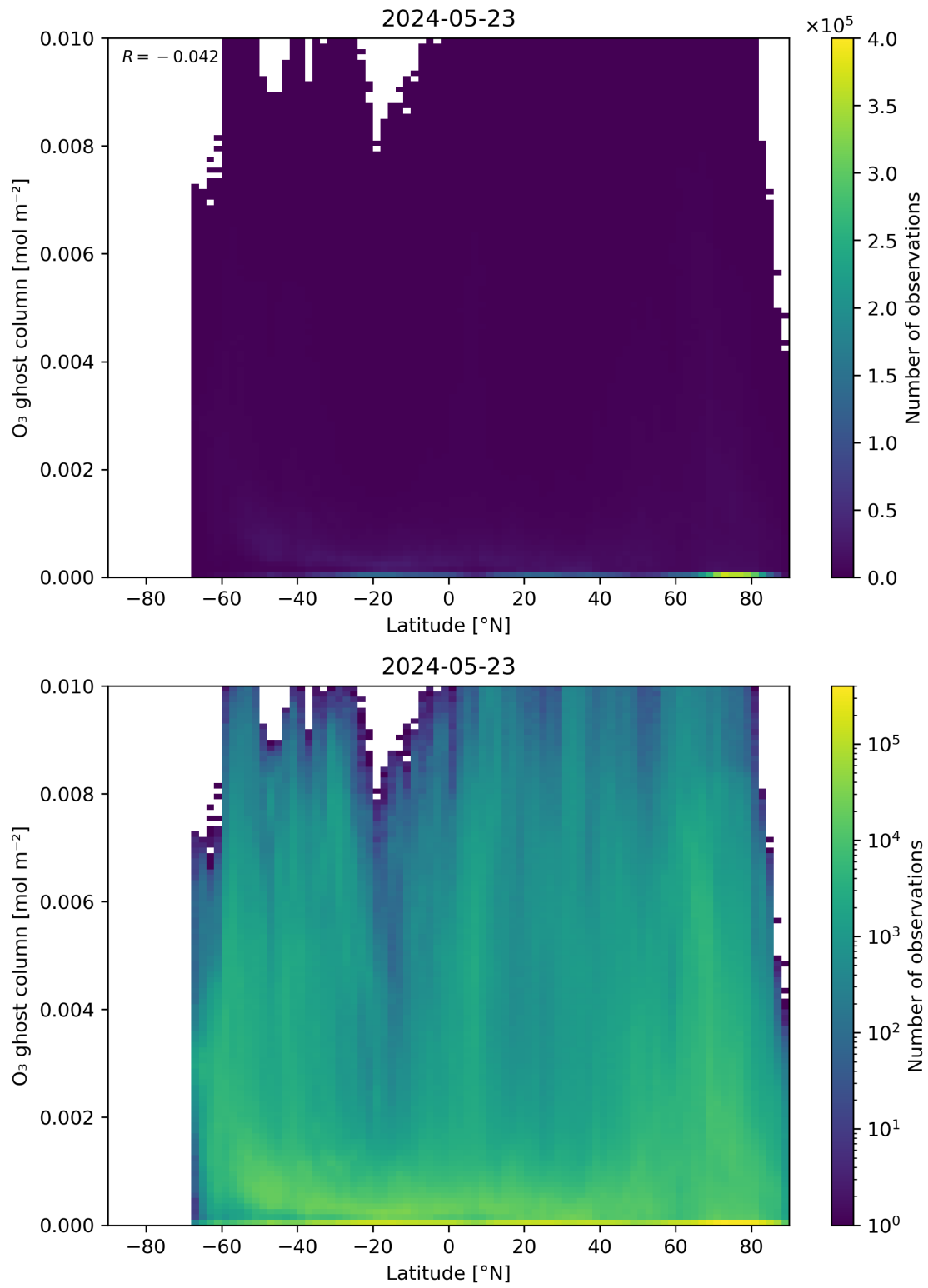
Figure 35: Scatter density plot of “Latitude” against “O 3 ghost column” for 2024-05-23 to 2024-05-24.
