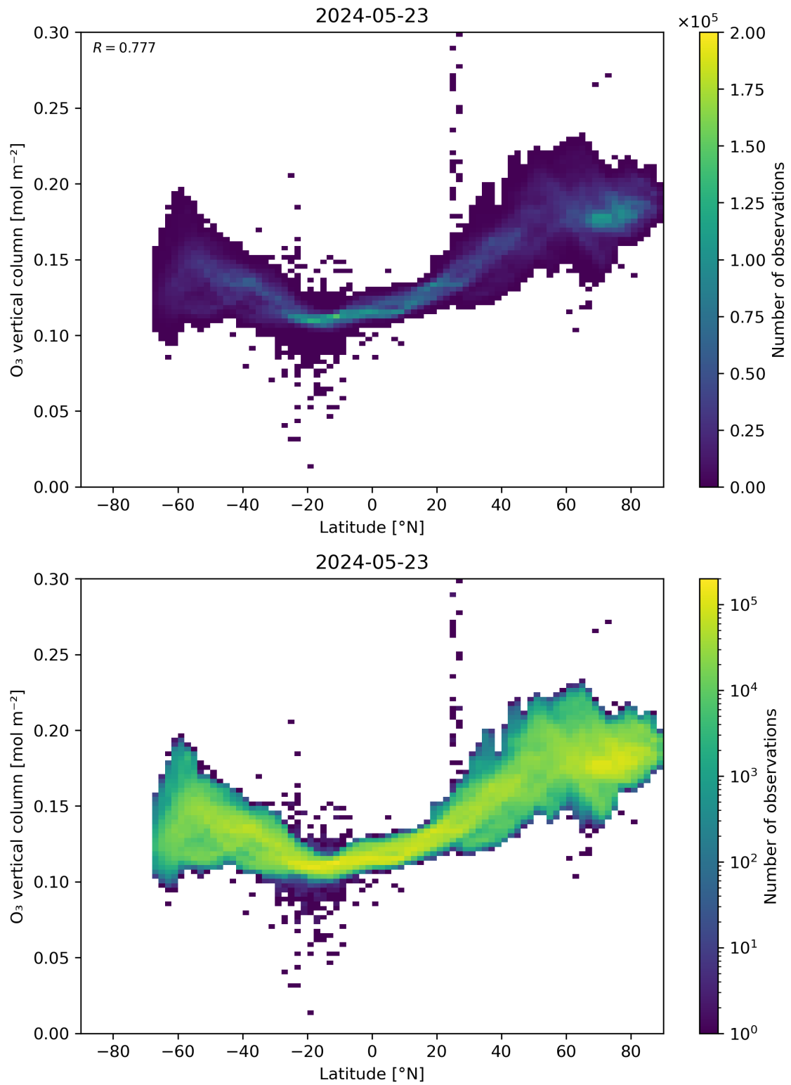
Figure 36: Scatter density plot of “Latitude” against “O 3 vertical column” for 2024-05-23 to 2024-05-24.
