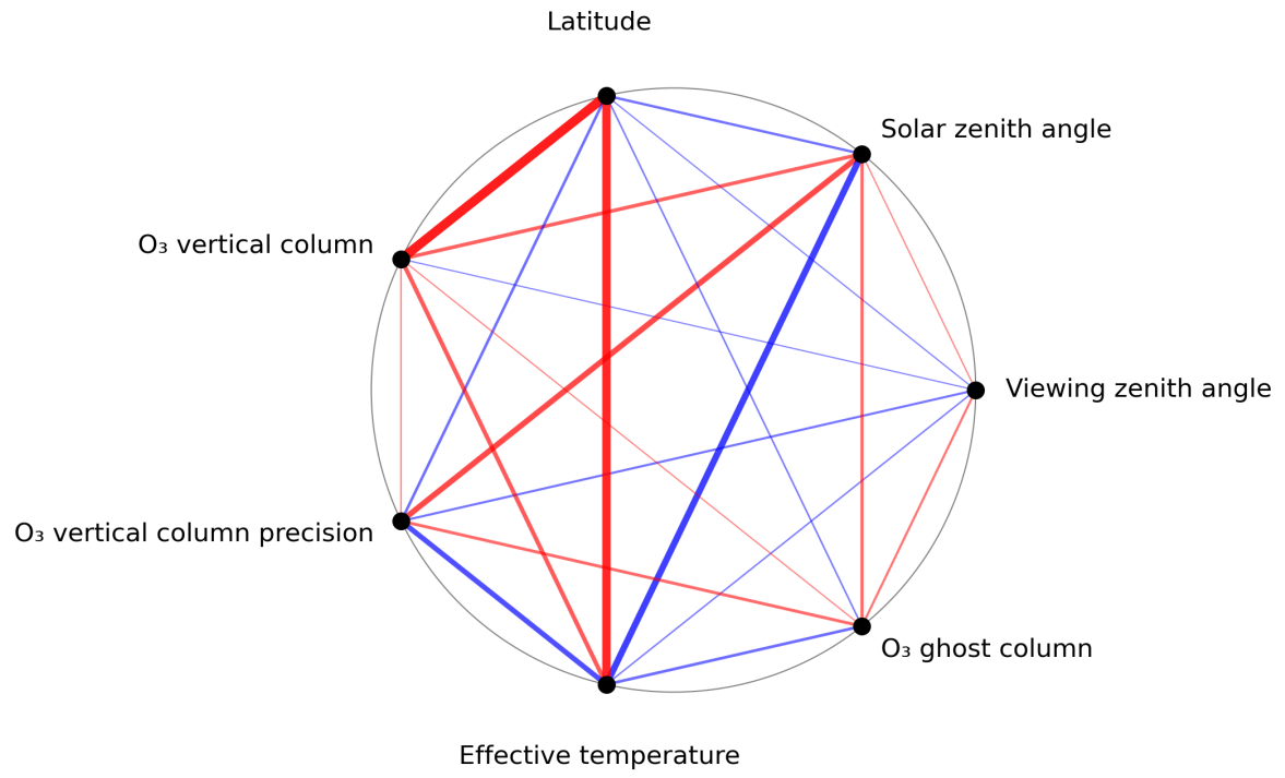
Figure 1: Map of correlation graph for 2024-05-23 to 2024-05-24.
