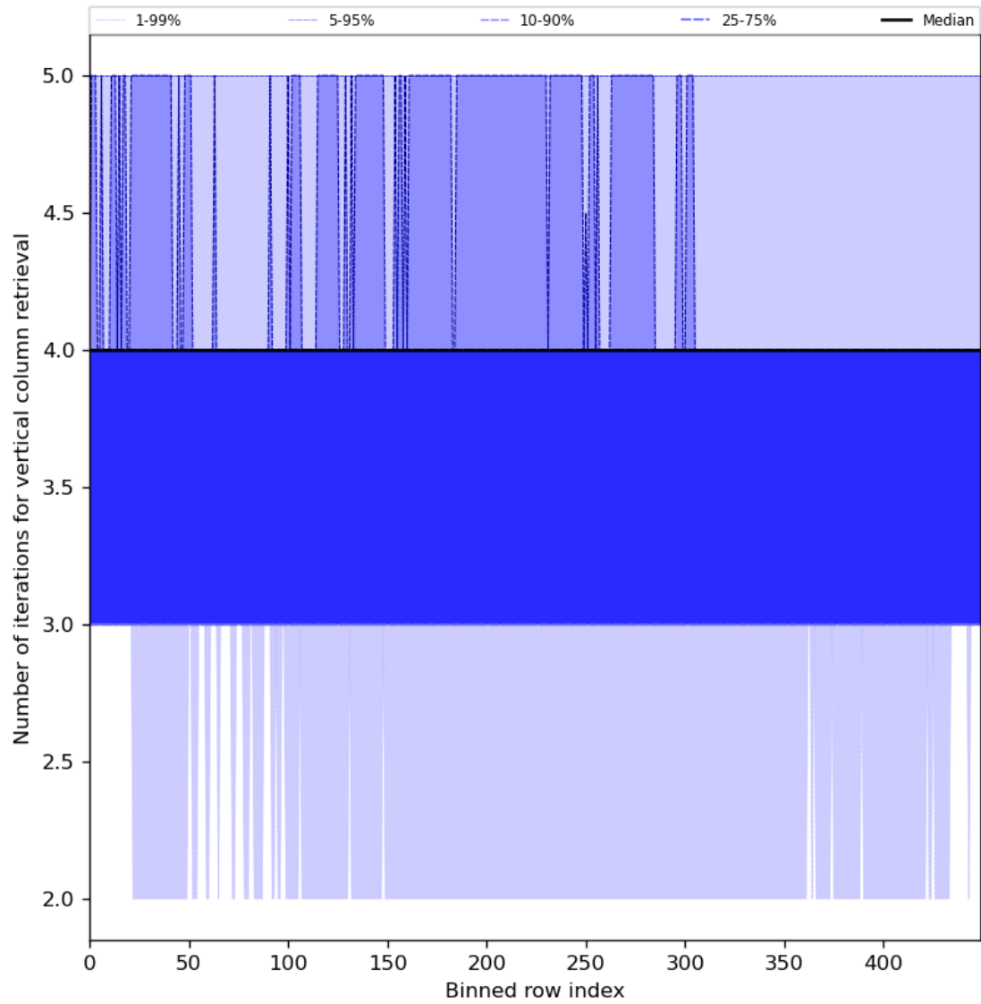
Figure 33: Along track statistics of “Number of iterations for vertical column retrieval” for 2024-05-23 to 2024-05-24
