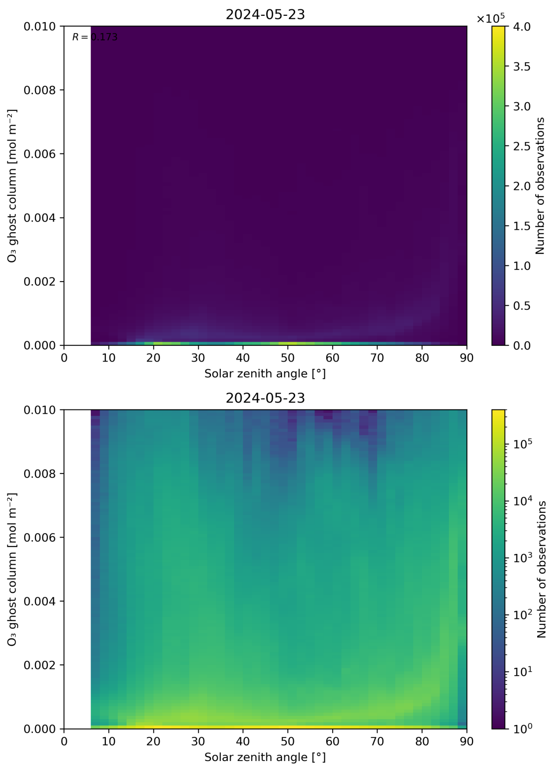
Figure 46: Scatter density plot of “Solar zenith angle” against “O 3 ghost column” for 2024-05-23 to 2024-05-24.
