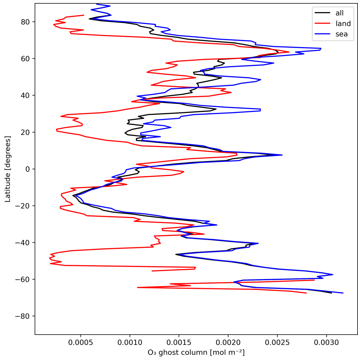
Figure 18: Zonal average of “O 3 ghost column” for 2024-05-23 to 2024-05-24.
