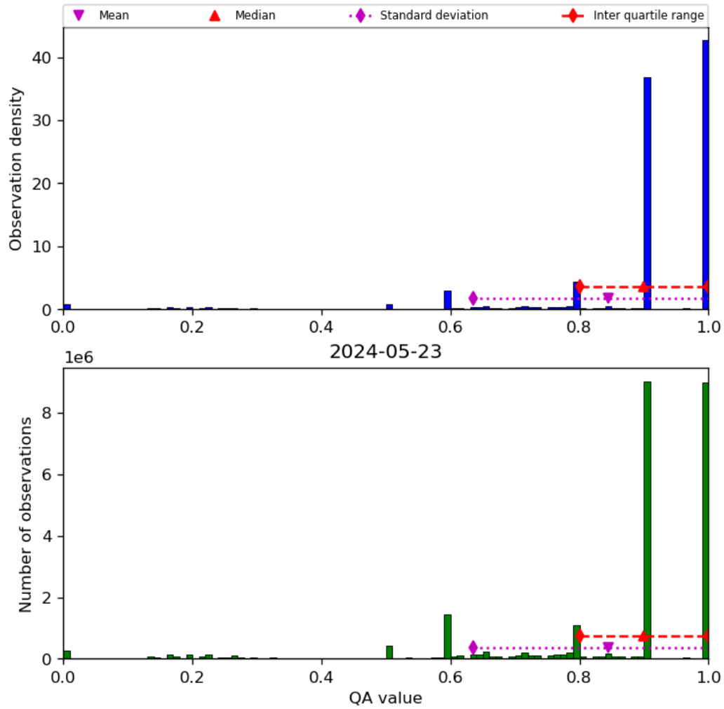
Figure 20: Histogram of “QA value” for 2024-05-23 to 2024-05-24
