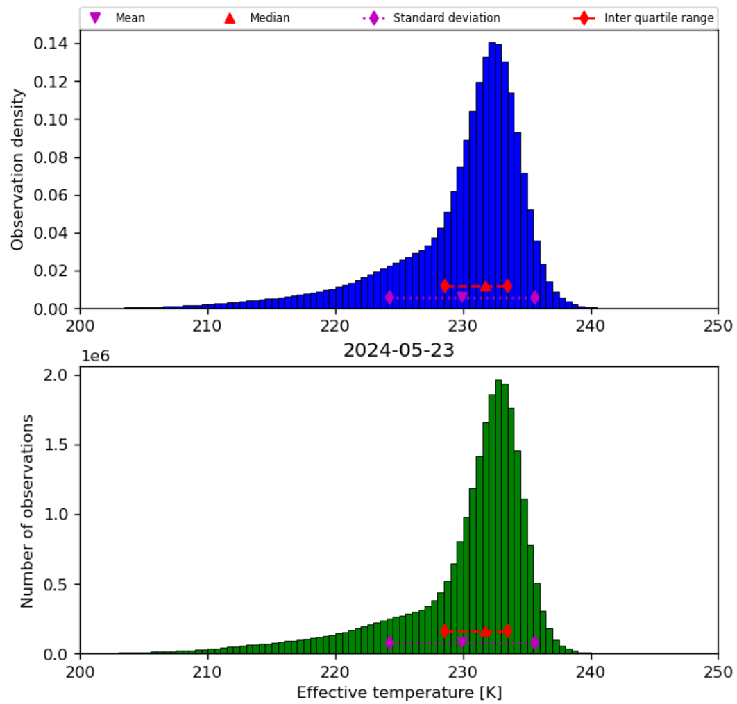
Figure 24: Histogram of “Effective temperature” for 2024-05-23 to 2024-05-24
