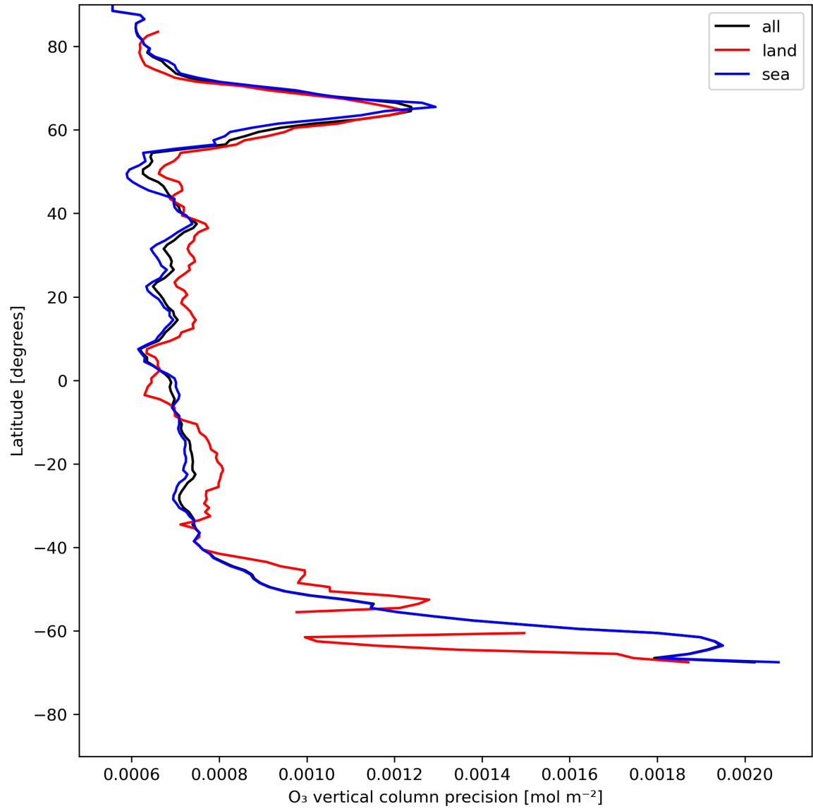
Figure 15: Zonal average of "O 3 vertical column precision" for 2024-05-23 to 2024-05-24.
