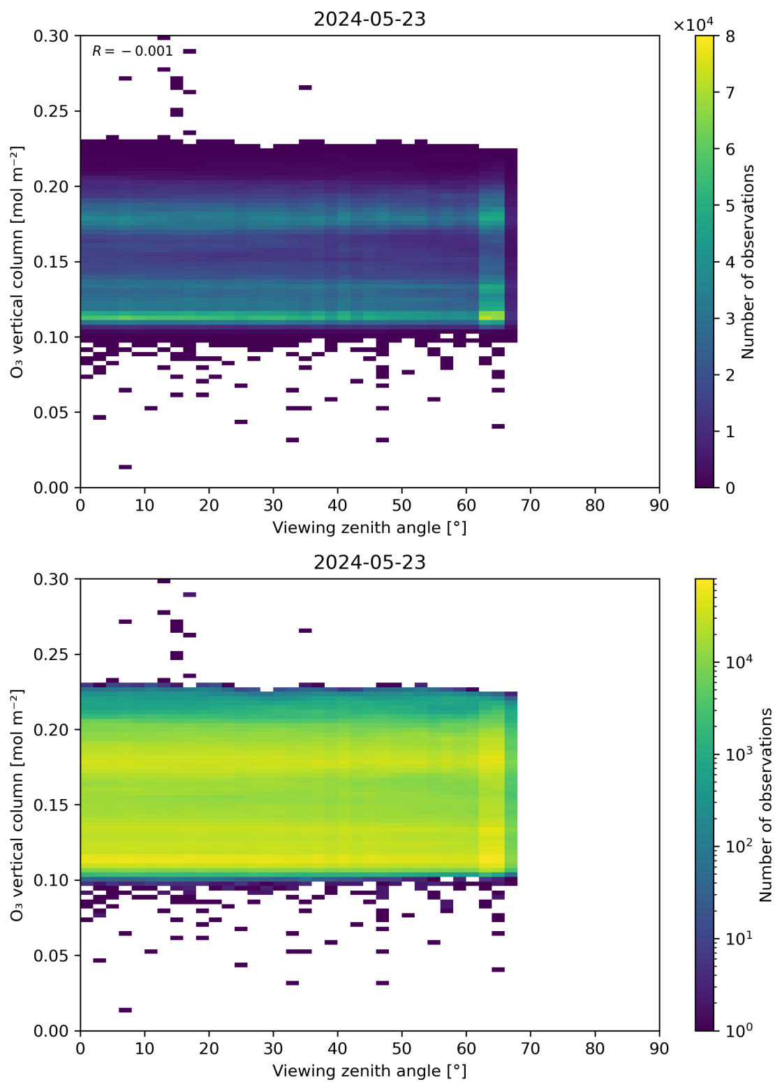
Figure 52: Scatter density plot of “Viewing zenith angle” against “O 3 vertical column” for 2024-05-23 to 2024-05-24.
