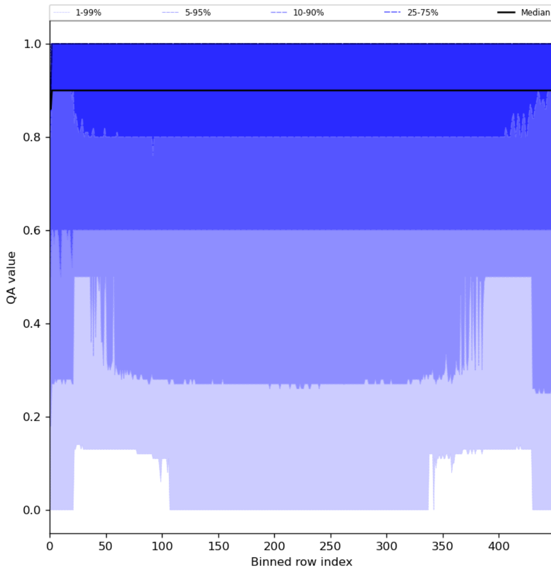
Figure 27: Along track statistics of “QA value” for 2024-05-23 to 2024-05-24
