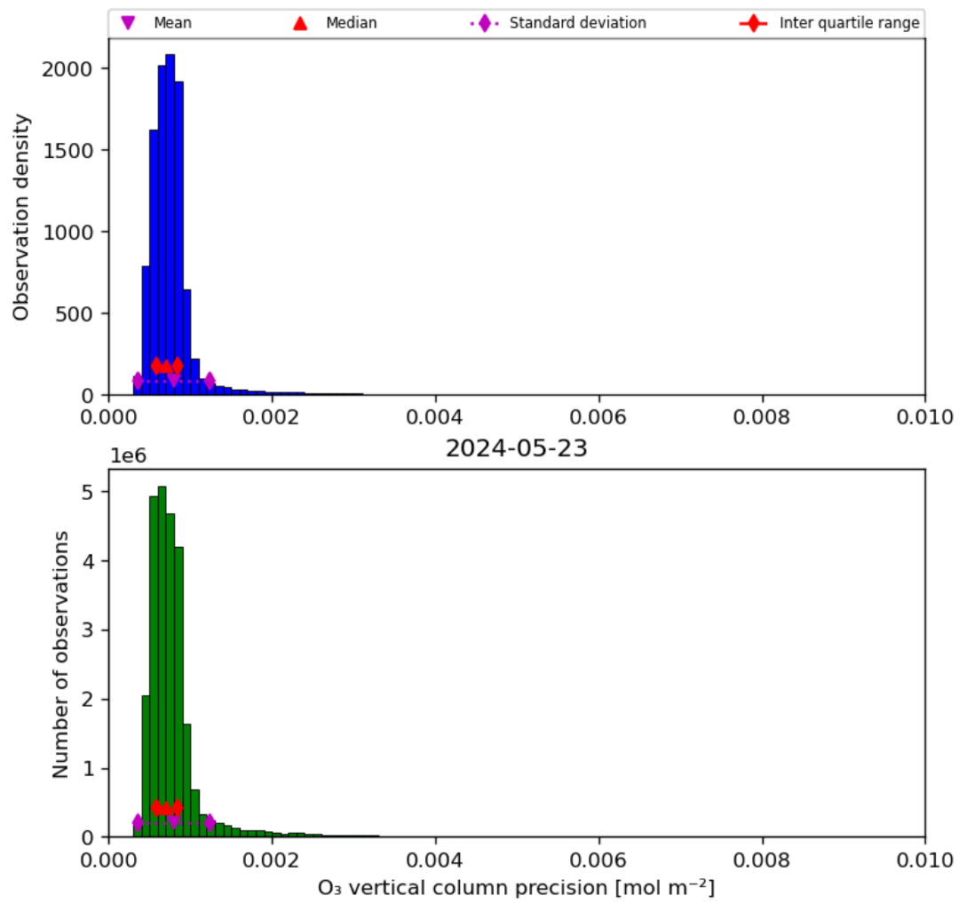
Figure 22: Histogram of “O 3 vertical column precision” for 2024-05-23 to 2024-05-24
