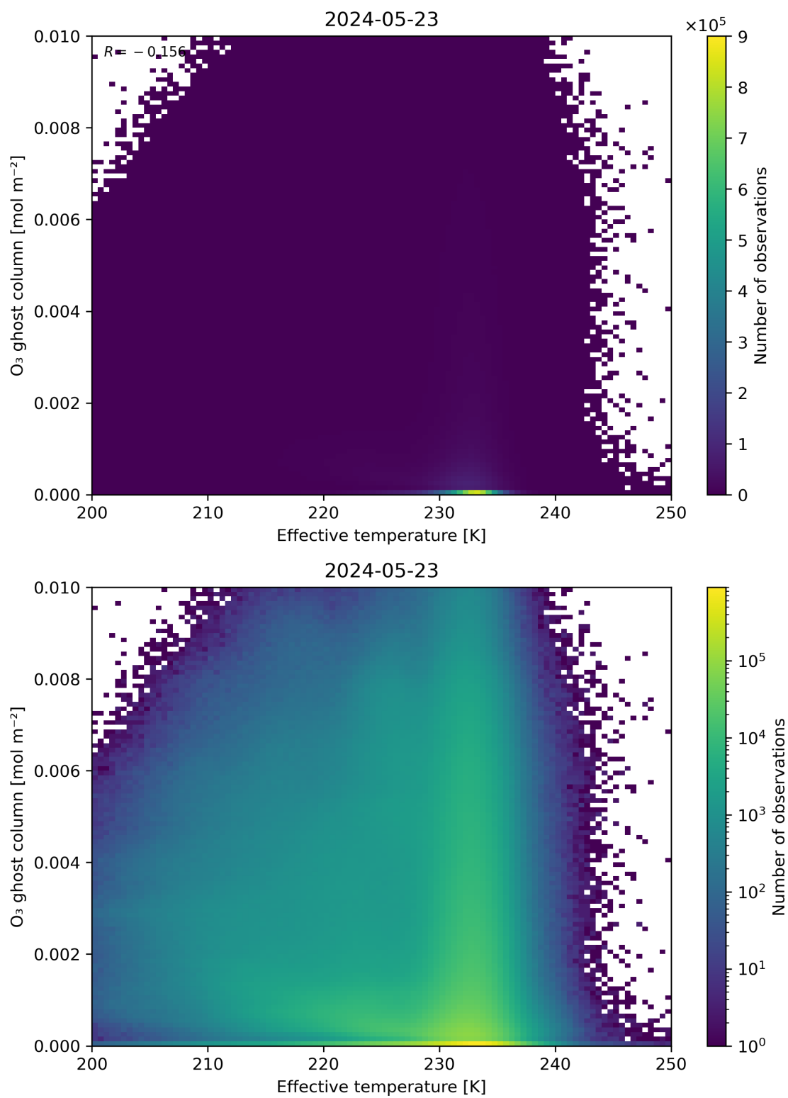
Figure 38: Scatter density plot of “Effective temperature” against “O 3 ghost column” for 2024-05-23 to 2024-05-24.
