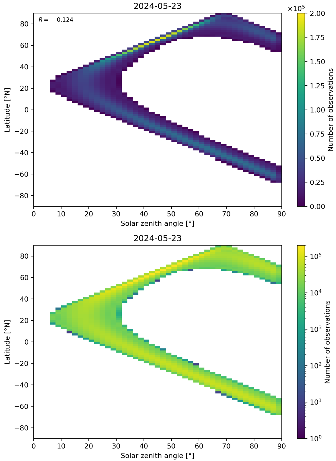
Figure 44: Scatter density plot of “Solar zenith angle” against “Latitude” for 2024-05-23 to 2024-05-24.
