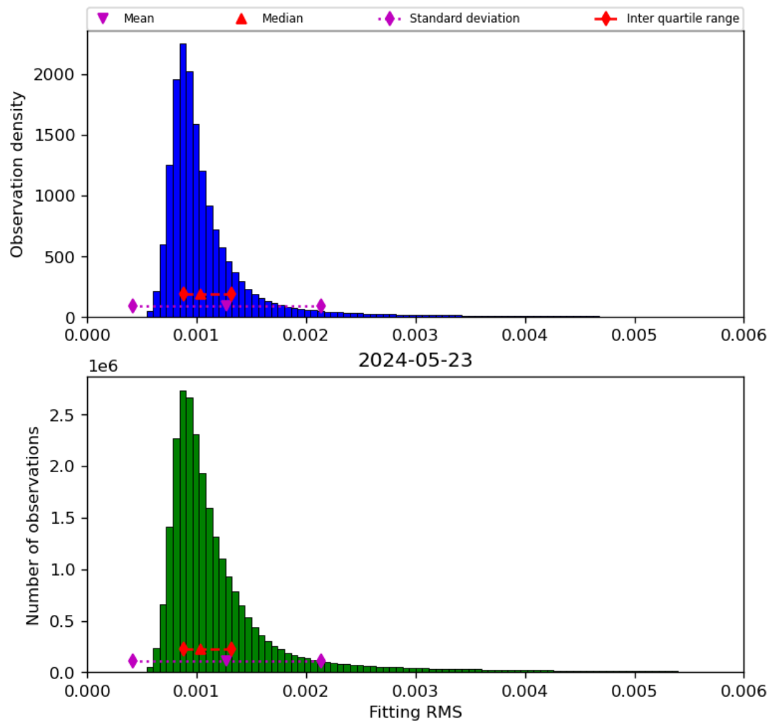
Figure 23: Histogram of “Fitting RMS” for 2024-05-23 to 2024-05-24
