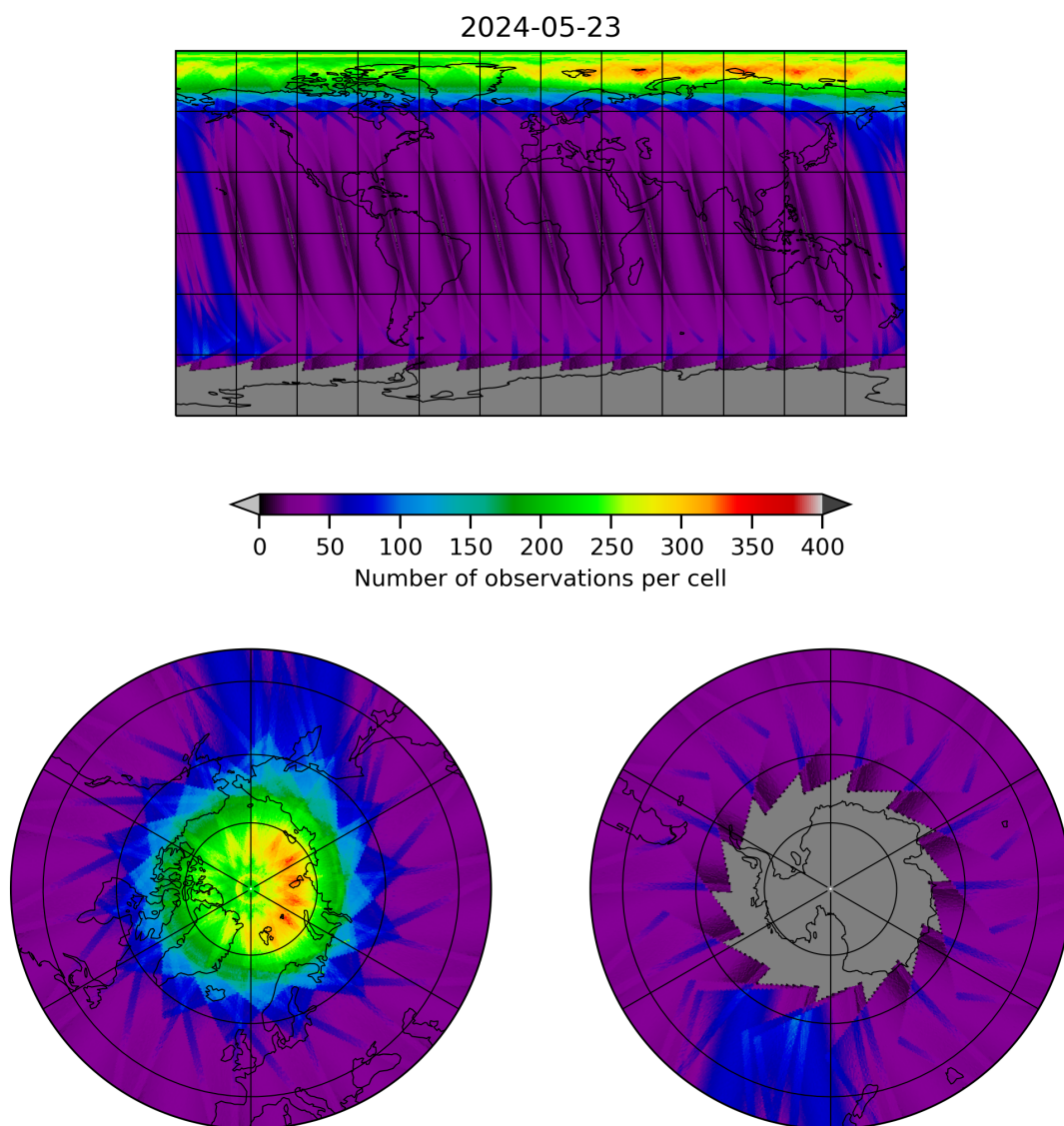
Figure 12: Map of the number of observations for 2024-05-23 to 2024-05-24
