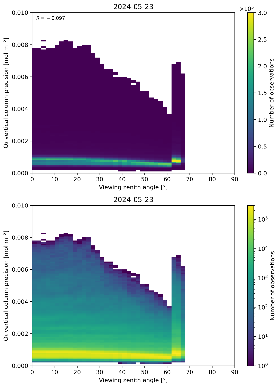
Figure 53: Scatter density plot of “Viewing zenith angle” against “O 3 vertical column precision” for 2024-05-23 to 2024-05-24.
