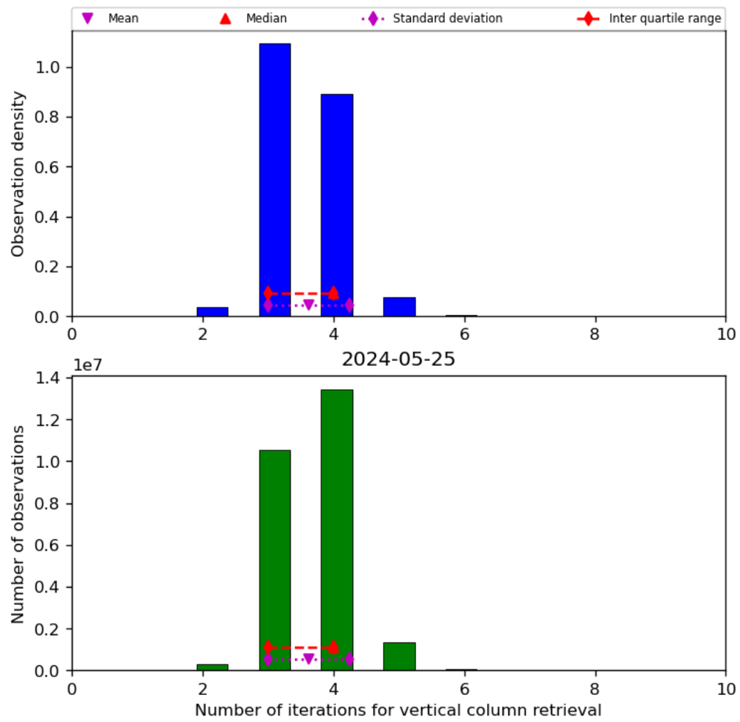
Figure 26: Histogram of “Number of iterations for vertical column retrieval” for 2024-05-24 to 2024-05-26
