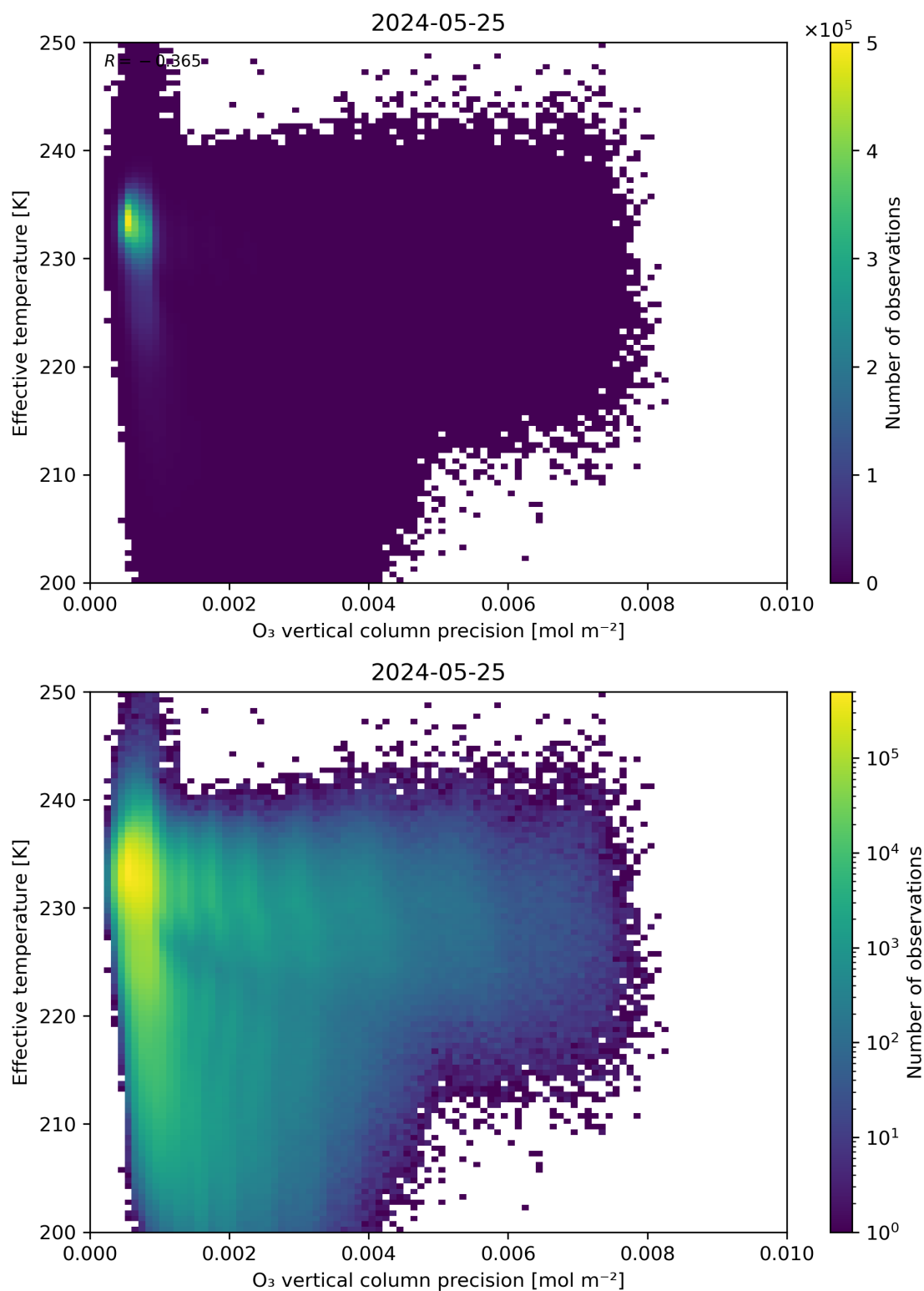
Figure 42: Scatter density plot of “O 3 vertical column precision” against “Effective temperature” for 2024-05-24 to 2024-05-26.
