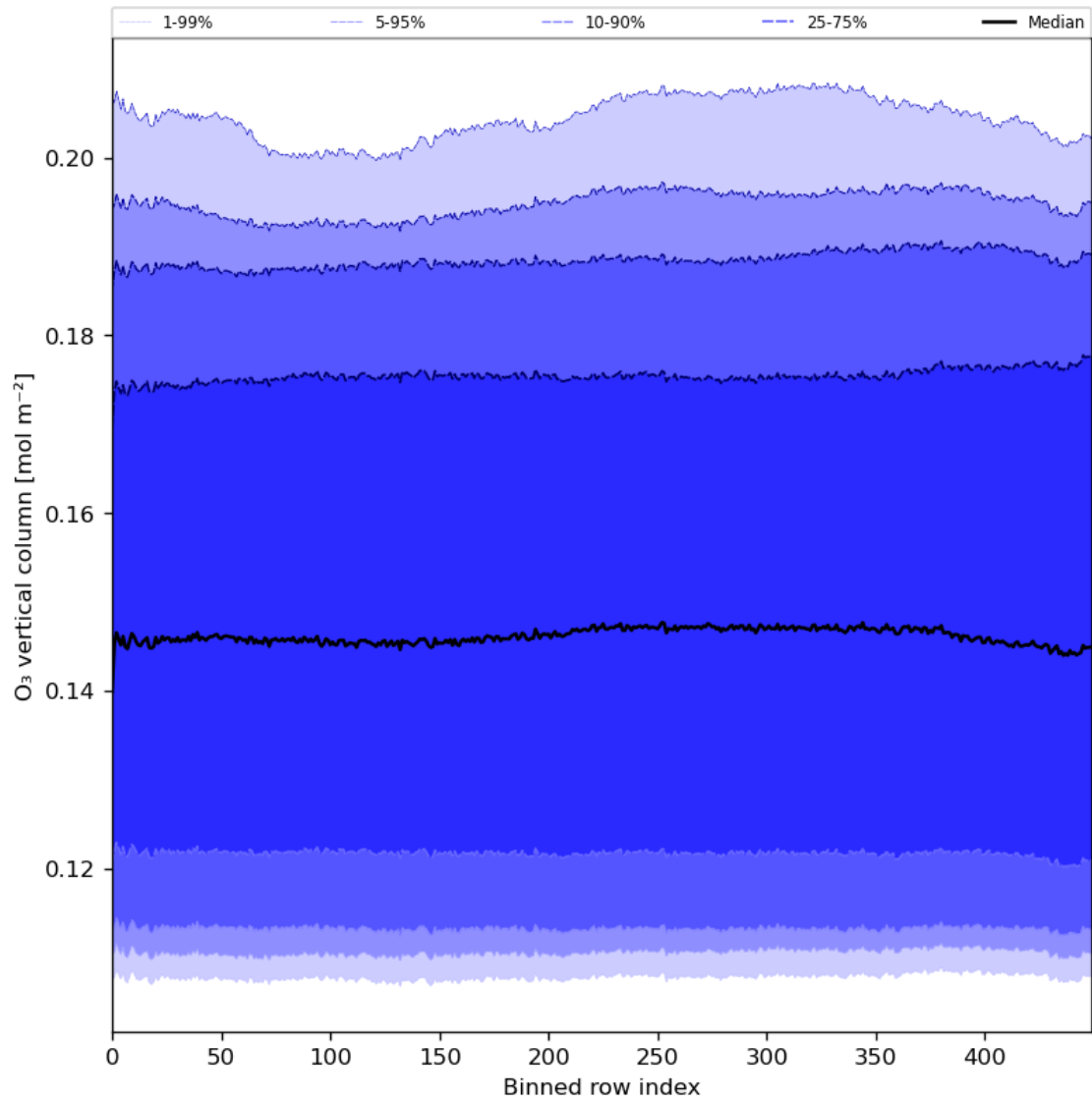
Figure 28: Along track statistics of “O 3 vertical column” for 2024-05-24 to 2024-05-26
