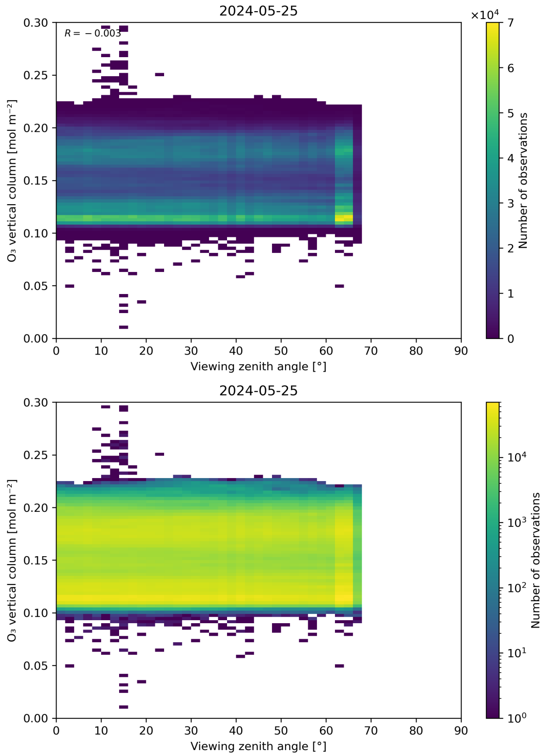
Figure 52: Scatter density plot of “Viewing zenith angle” against “O 3 vertical column” for 2024-05-24 to 2024-05-26.
