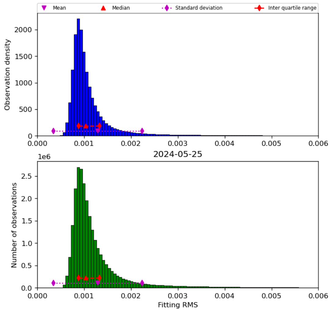
Figure 23: Histogram of “Fitting RMS” for 2024-05-24 to 2024-05-26
