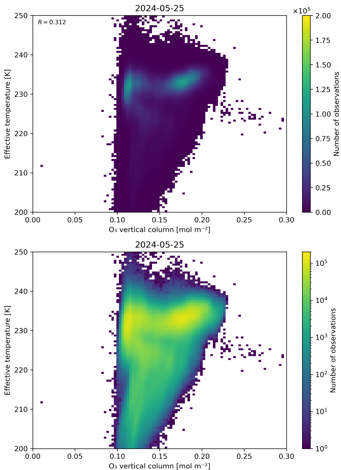
Figure 39: Scatter density plot of “O 3 vertical column” against “Effective temperature” for 2024-05-24 to 2024-05-26.
