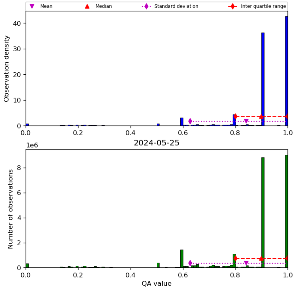
Figure 20: Histogram of “QA value” for 2024-05-24 to 2024-05-26
