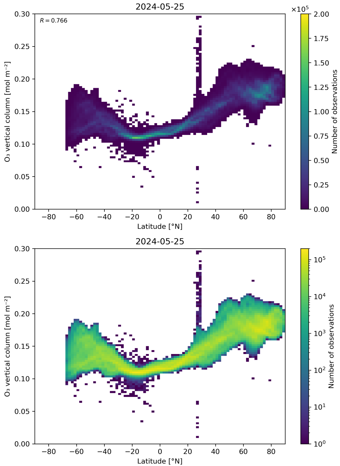
Figure 36: Scatter density plot of “Latitude” against “O 3 vertical column” for 2024-05-24 to 2024-05-26.
