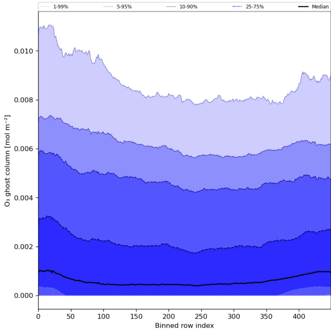
Figure 32: Along track statistics of "O 3 ghost column" for 2024-05-24 to 2024-05-26
