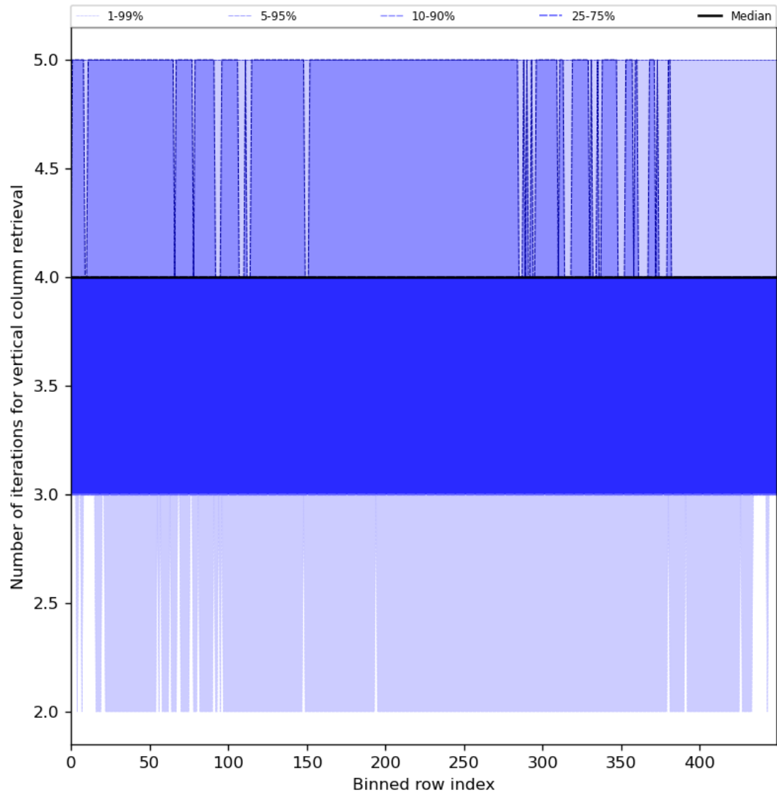
Figure 33: Along track statistics of “Number of iterations for vertical column retrieval” for 2024-05-24 to 2024-05-26
