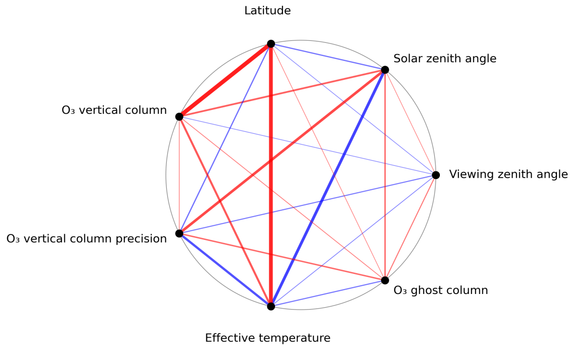
Figure 1: Map of correlation graph for 2024-05-24 to 2024-05-26.
