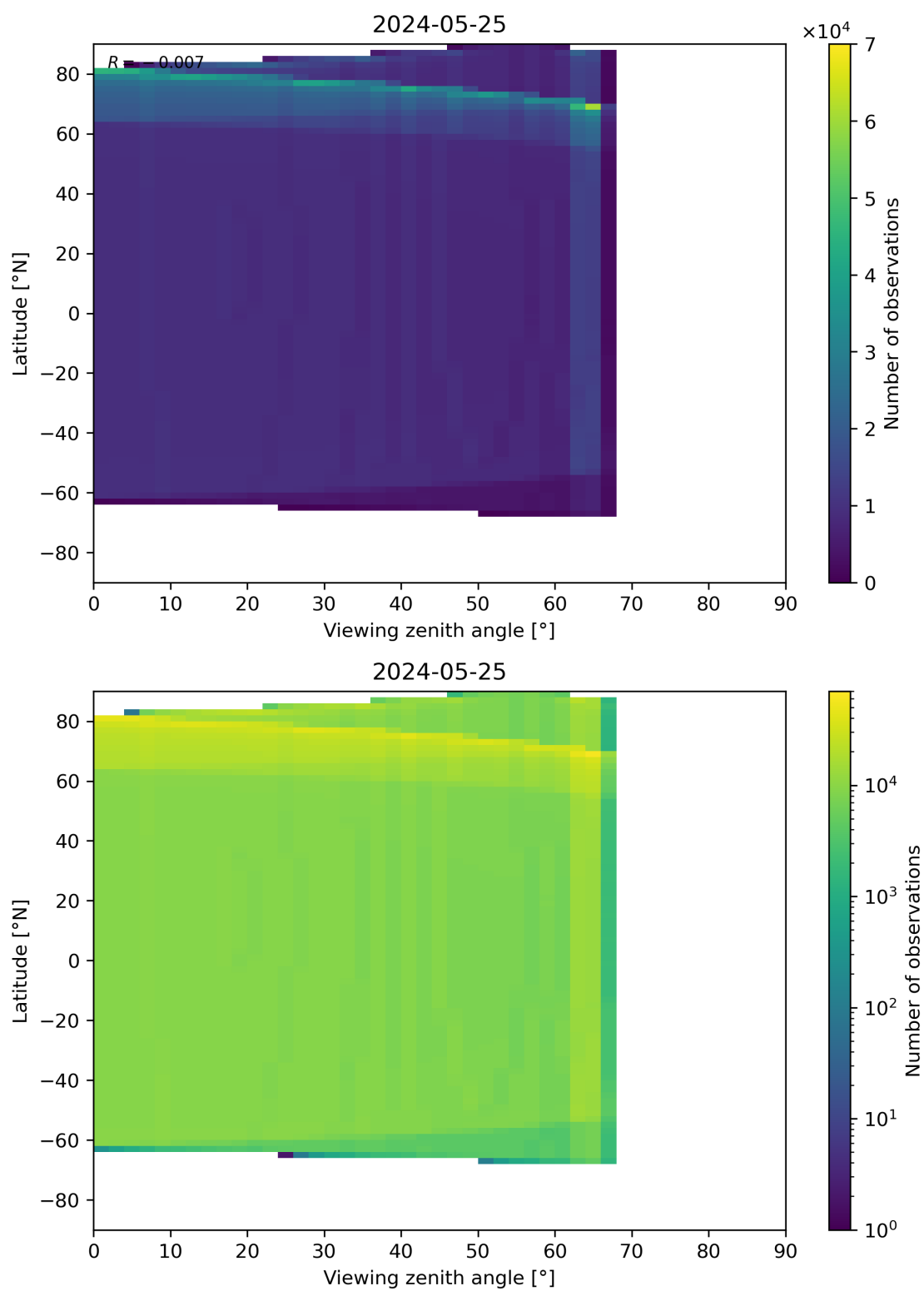
Figure 49: Scatter density plot of “Viewing zenith angle” against “Latitude” for 2024-05-24 to 2024-05-26.
