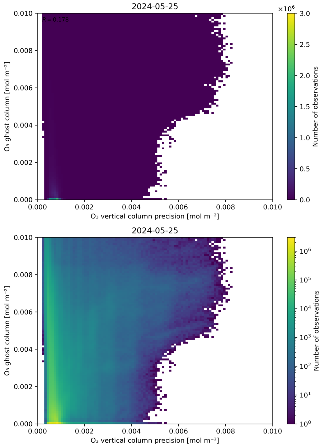
Figure 43: Scatter density plot of “ \text{O}_3 vertical column precision” against “ \text{O}_3 ghost column” for 2024-05-24 to 2024-05-26.
