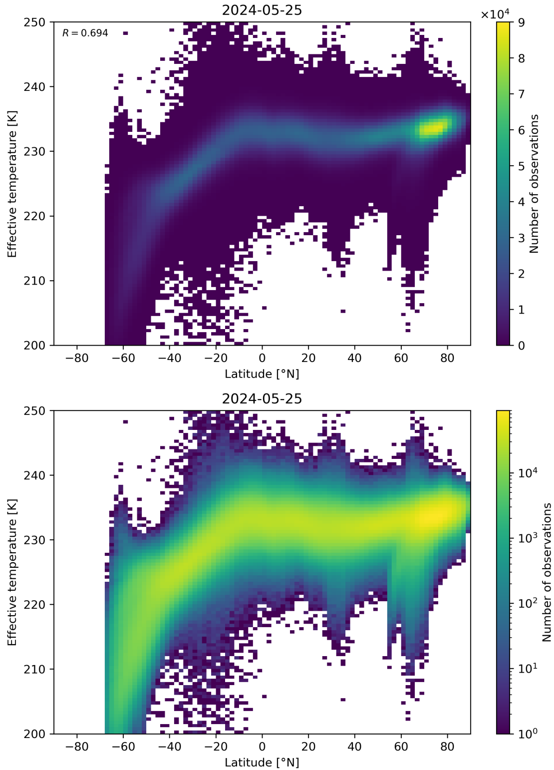
Figure 34: Scatter density plot of “Latitude” against “Effective temperature” for 2024-05-24 to 2024-05-26.
