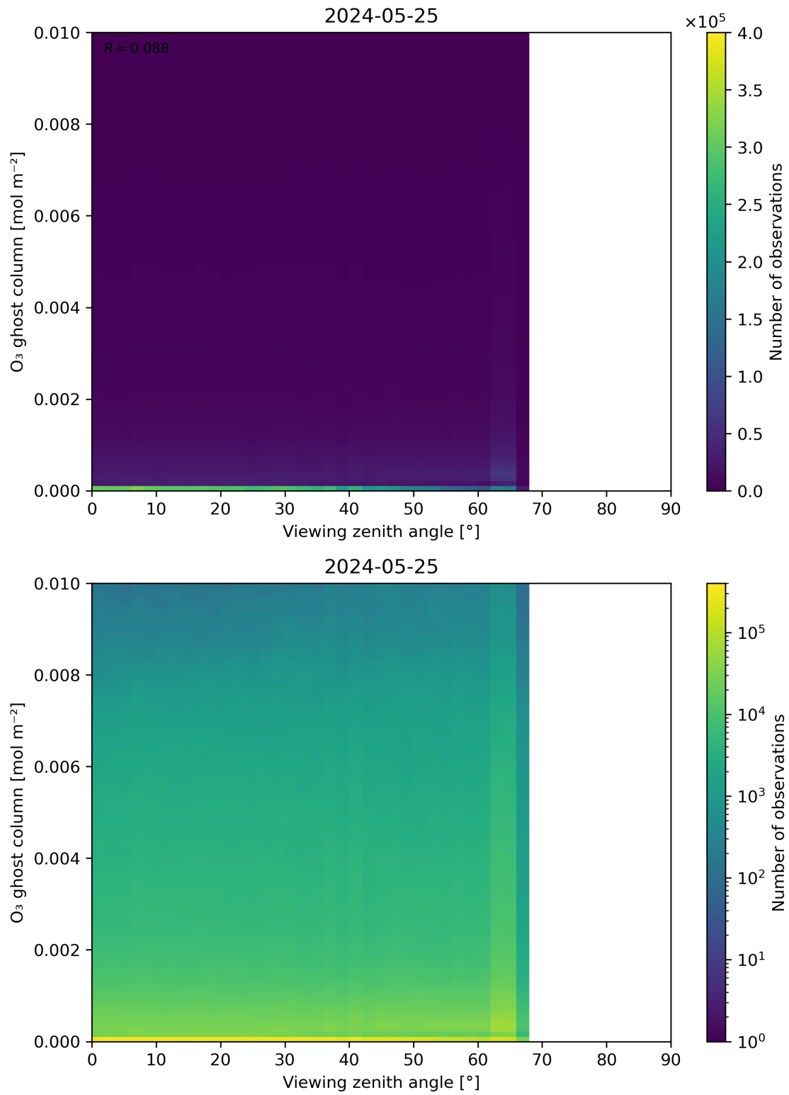
Figure 51: Scatter density plot of “Viewing zenith angle” against “O 3 ghost column” for 2024-05-24 to 2024-05-26.
