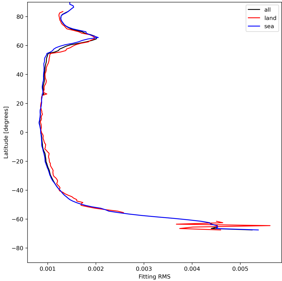
Figure 16: Zonal average of “Fitting RMS” for 2024-05-24 to 2024-05-26.
