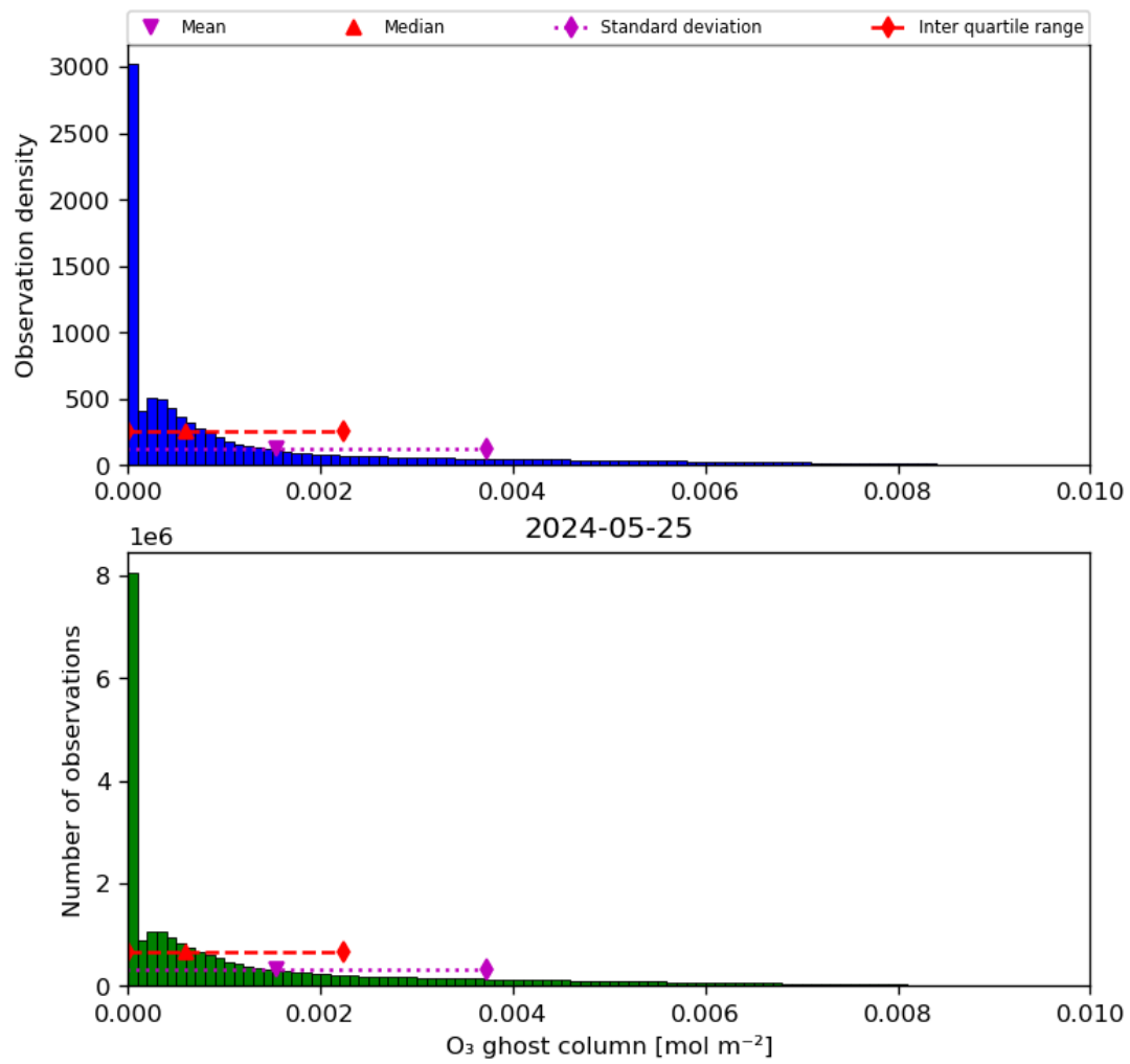
Figure 25: Histogram of “O 3 ghost column” for 2024-05-24 to 2024-05-26
