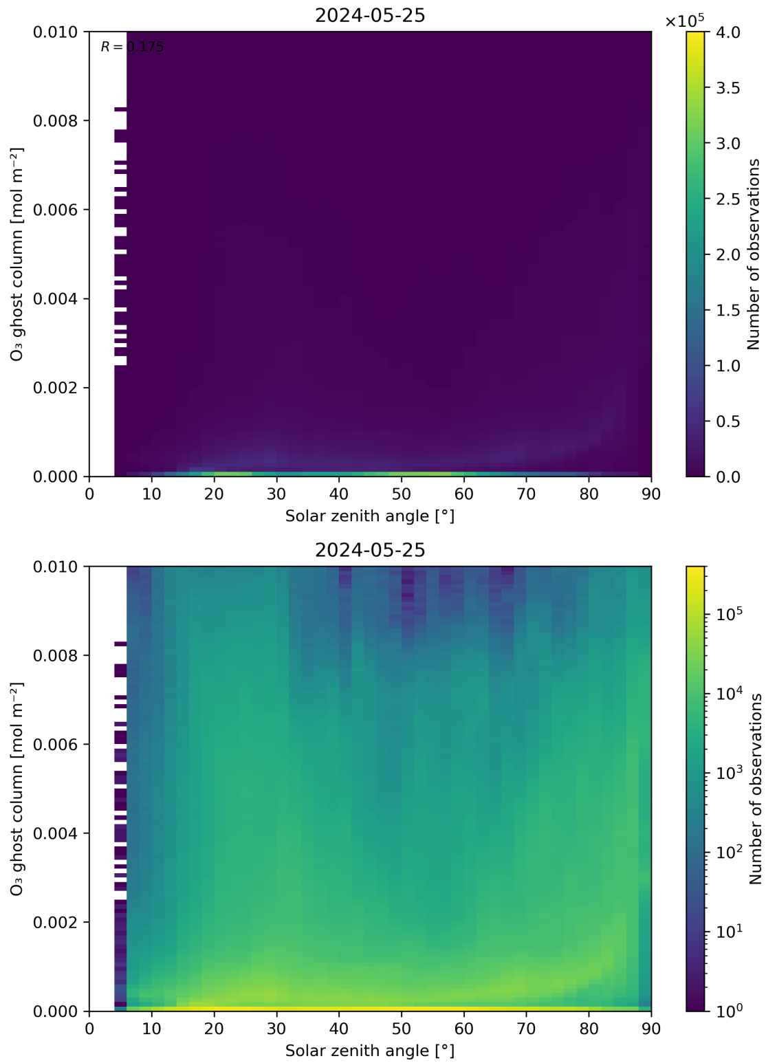
Figure 46: Scatter density plot of “Solar zenith angle” against “O 3 ghost column” for 2024-05-24 to 2024-05-26.
