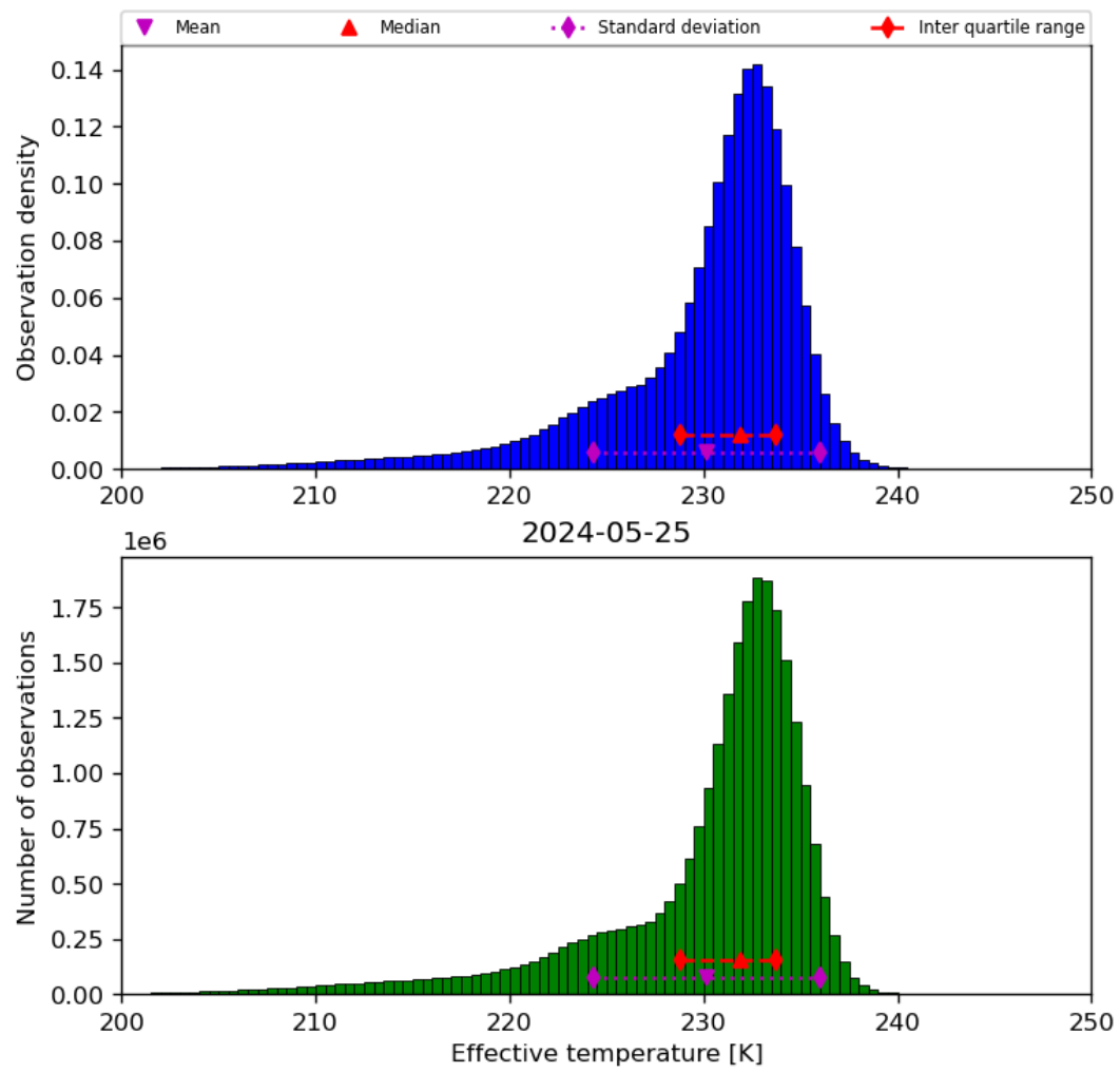
Figure 24: Histogram of “Effective temperature” for 2024-05-24 to 2024-05-26
