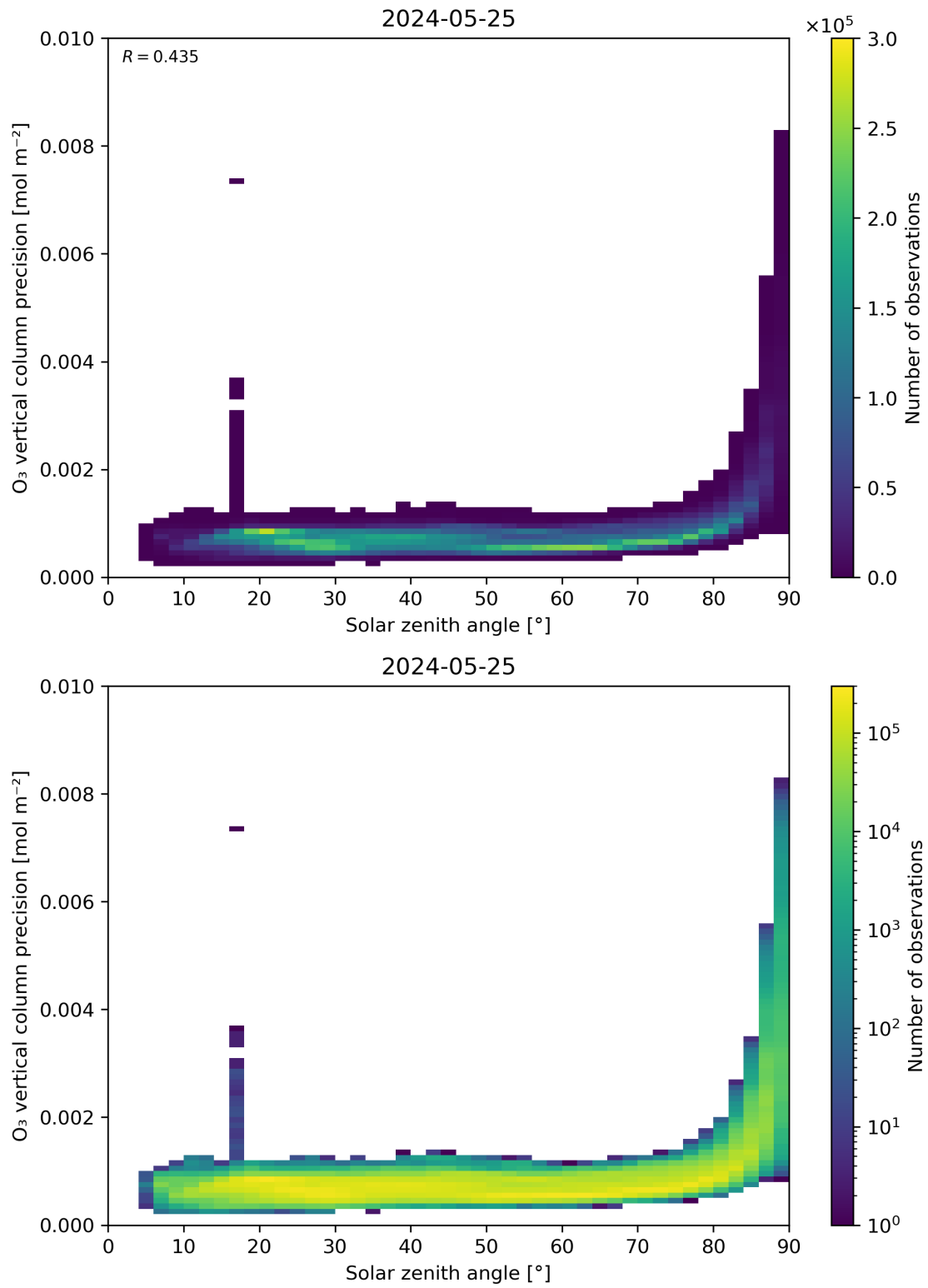
Figure 48: Scatter density plot of “Solar zenith angle” against “O 3 vertical column precision” for 2024-05-24 to 2024-05-26.
