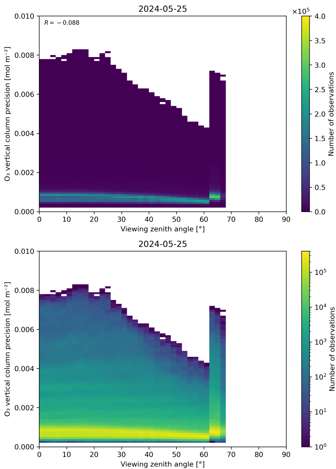
Figure 53: Scatter density plot of “Viewing zenith angle” against “O 3 vertical column precision” for 2024-05-24 to 2024-05-26.
