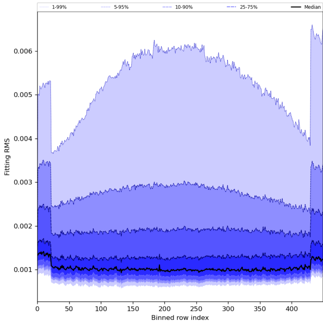
Figure 30: Along track statistics of “Fitting RMS” for 2024-05-24 to 2024-05-26
