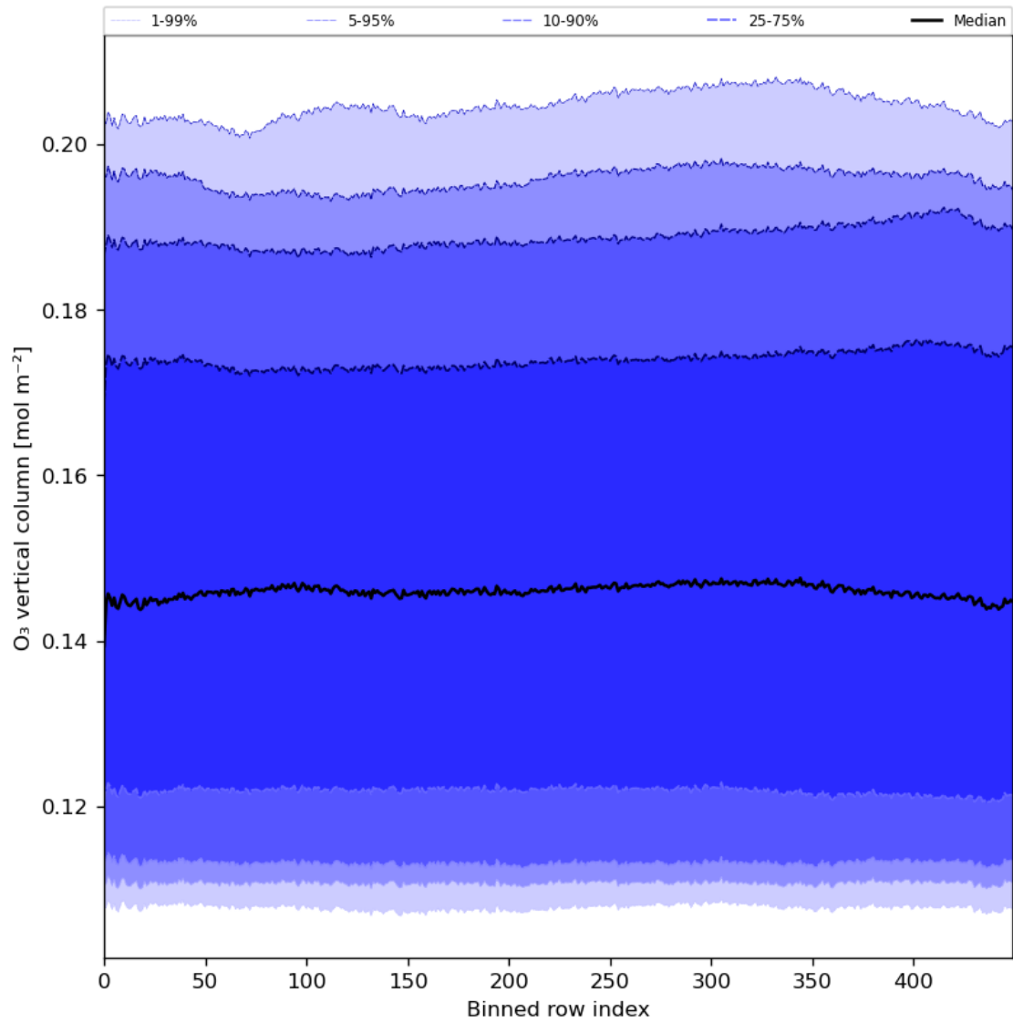
Figure 28: Along track statistics of “O 3 vertical column” for 2024-05-25 to 2024-05-27
