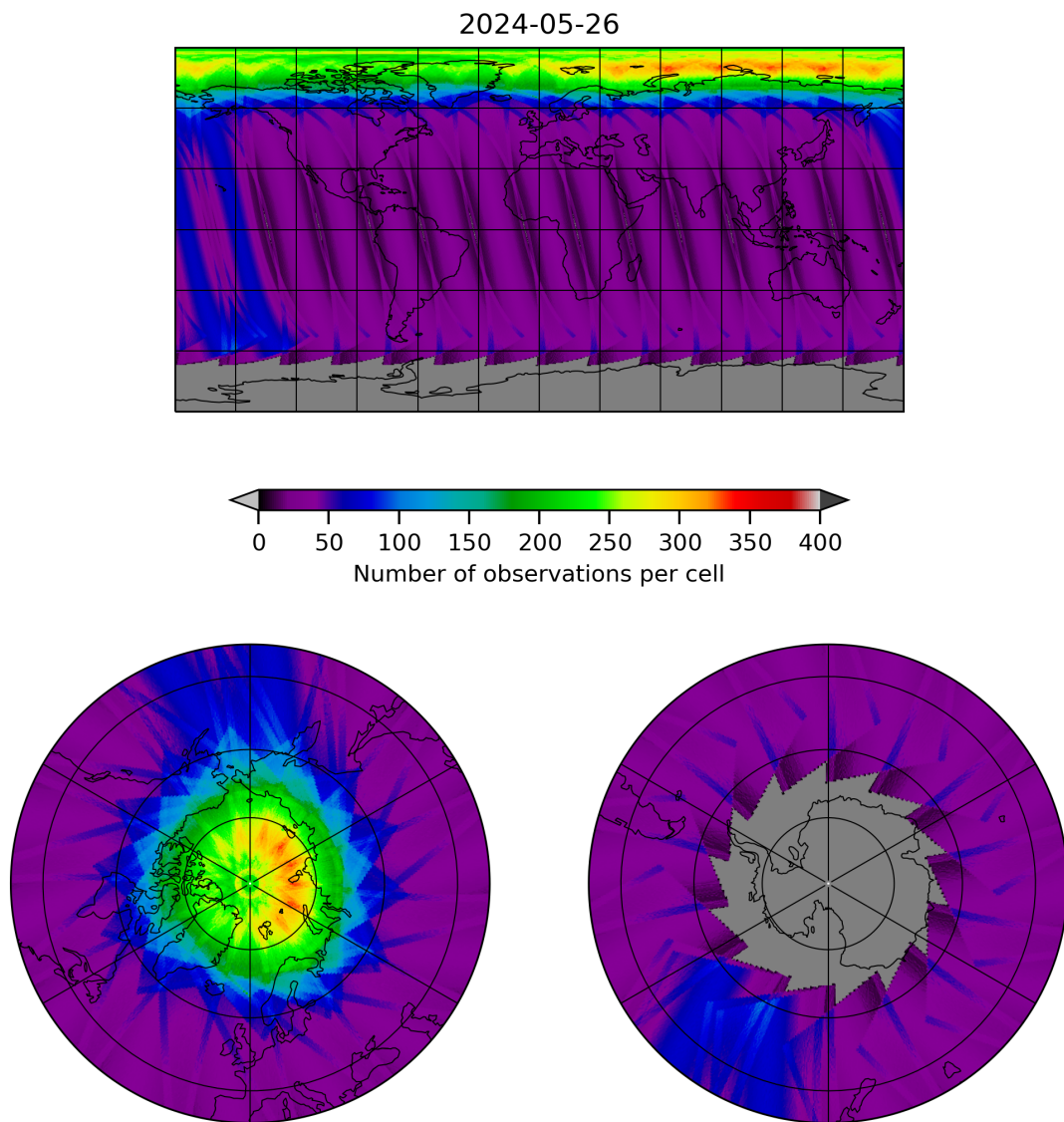
Figure 12: Map of the number of observations for 2024-05-25 to 2024-05-27
