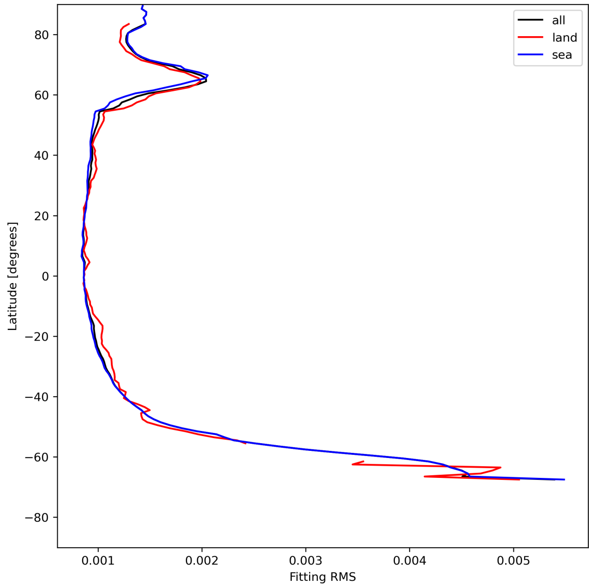
Figure 16: Zonal average of “Fitting RMS” for 2024-05-25 to 2024-05-27.
