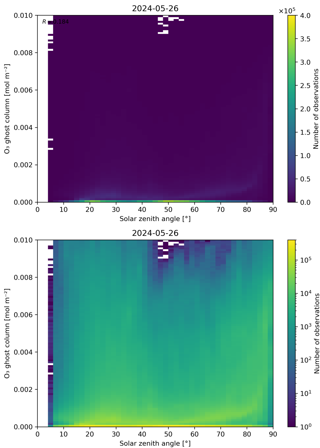
Figure 46: Scatter density plot of “Solar zenith angle” against “O 3 ghost column” for 2024-05-25 to 2024-05-27.
