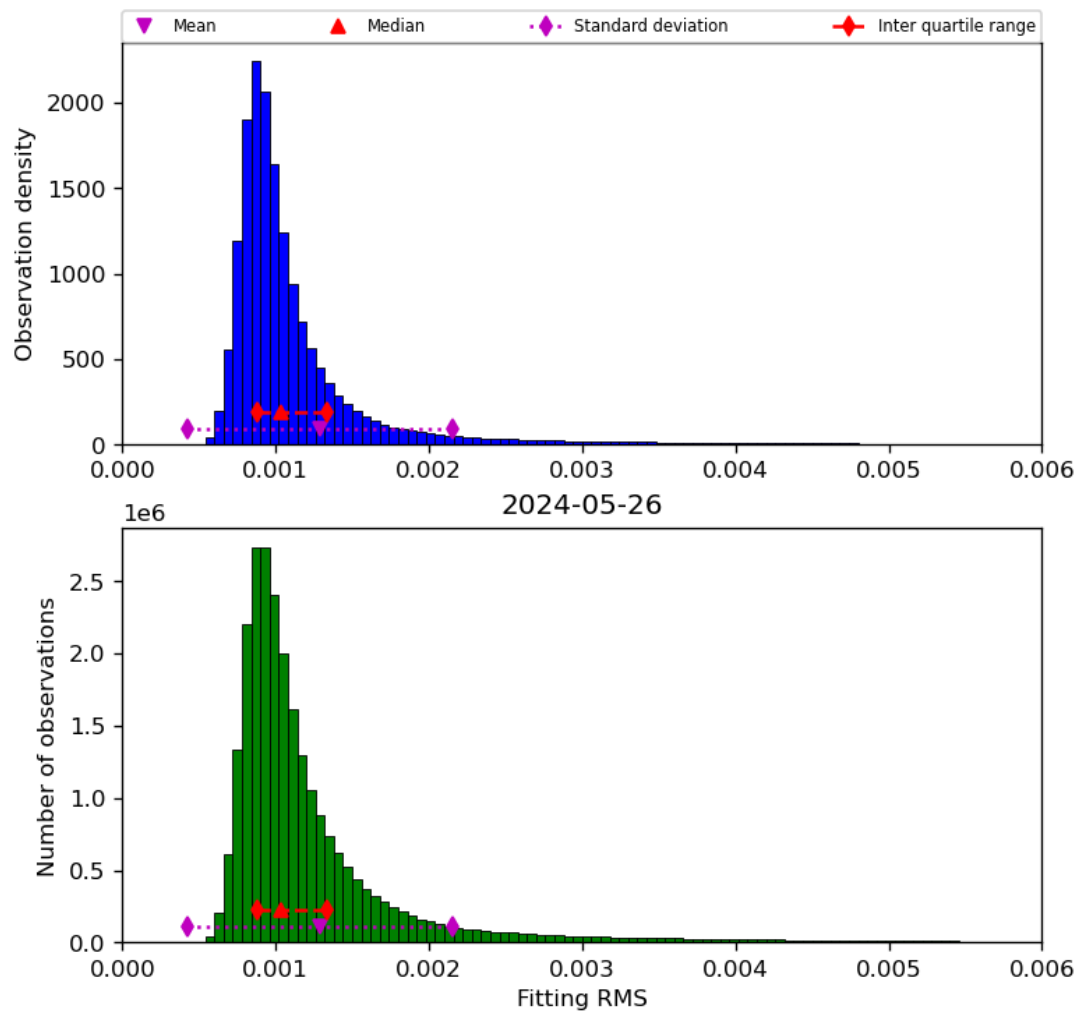
Figure 23: Histogram of “Fitting RMS” for 2024-05-25 to 2024-05-27
