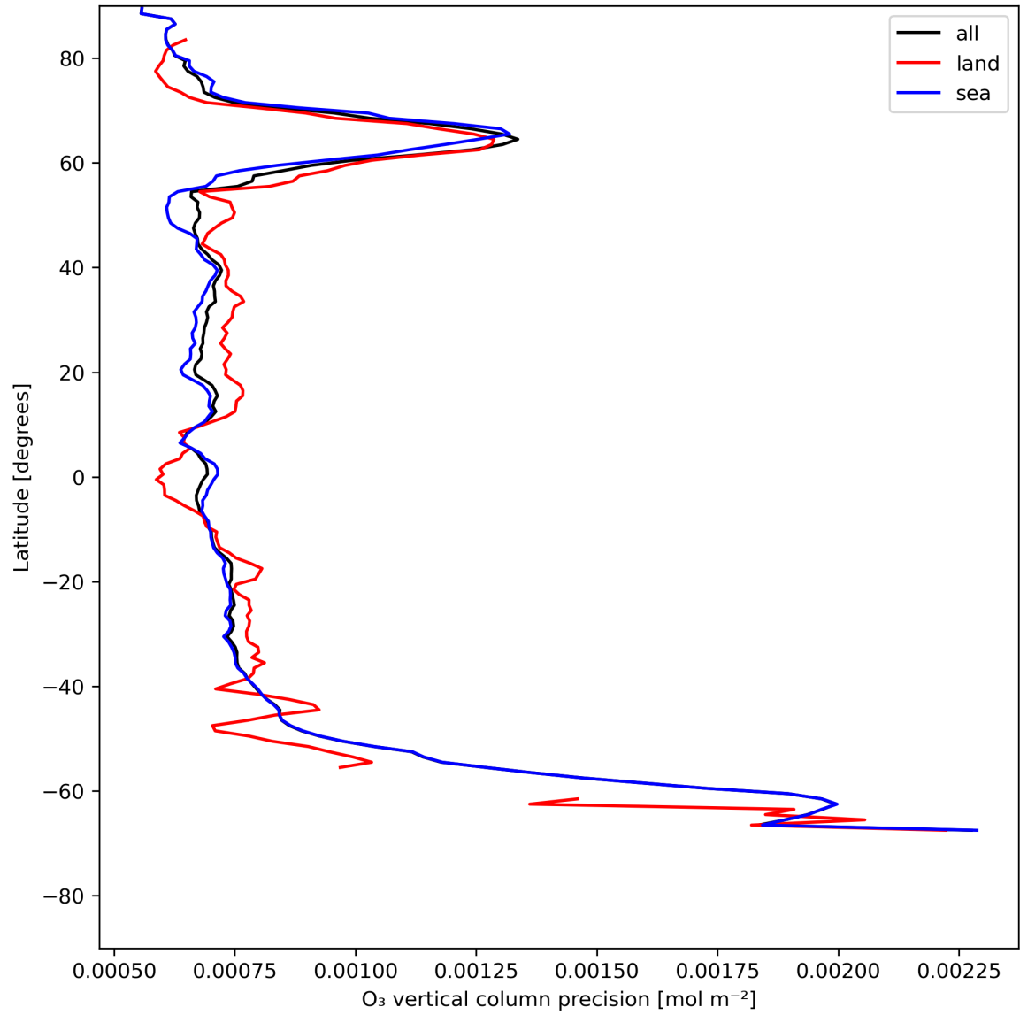
Figure 15: Zonal average of “O 3 vertical column precision” for 2024-05-25 to 2024-05-27.
