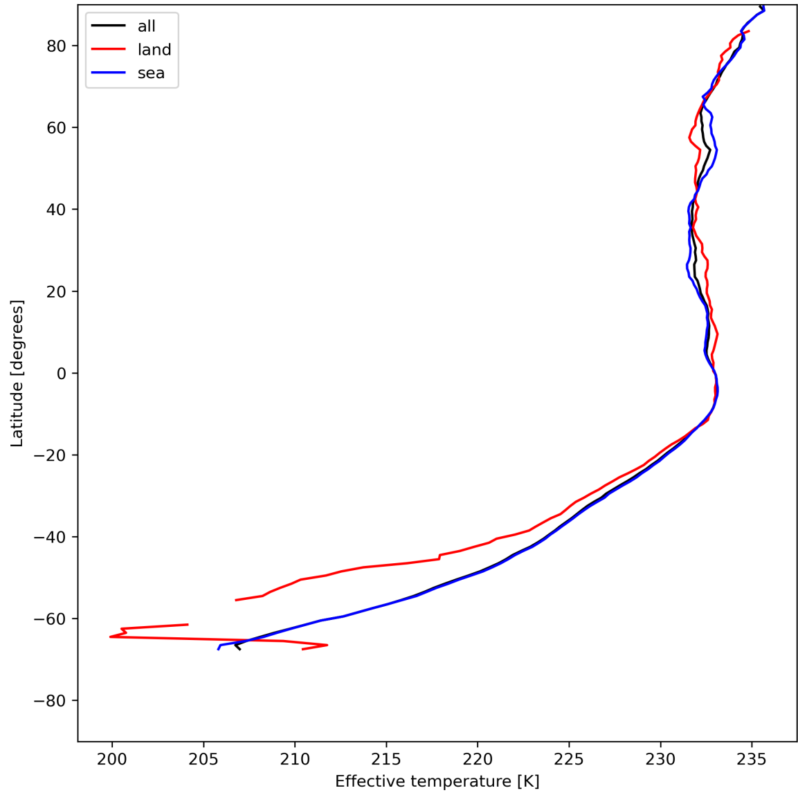
Figure 17: Zonal average of "Effective temperature" for 2024-05-25 to 2024-05-27.
