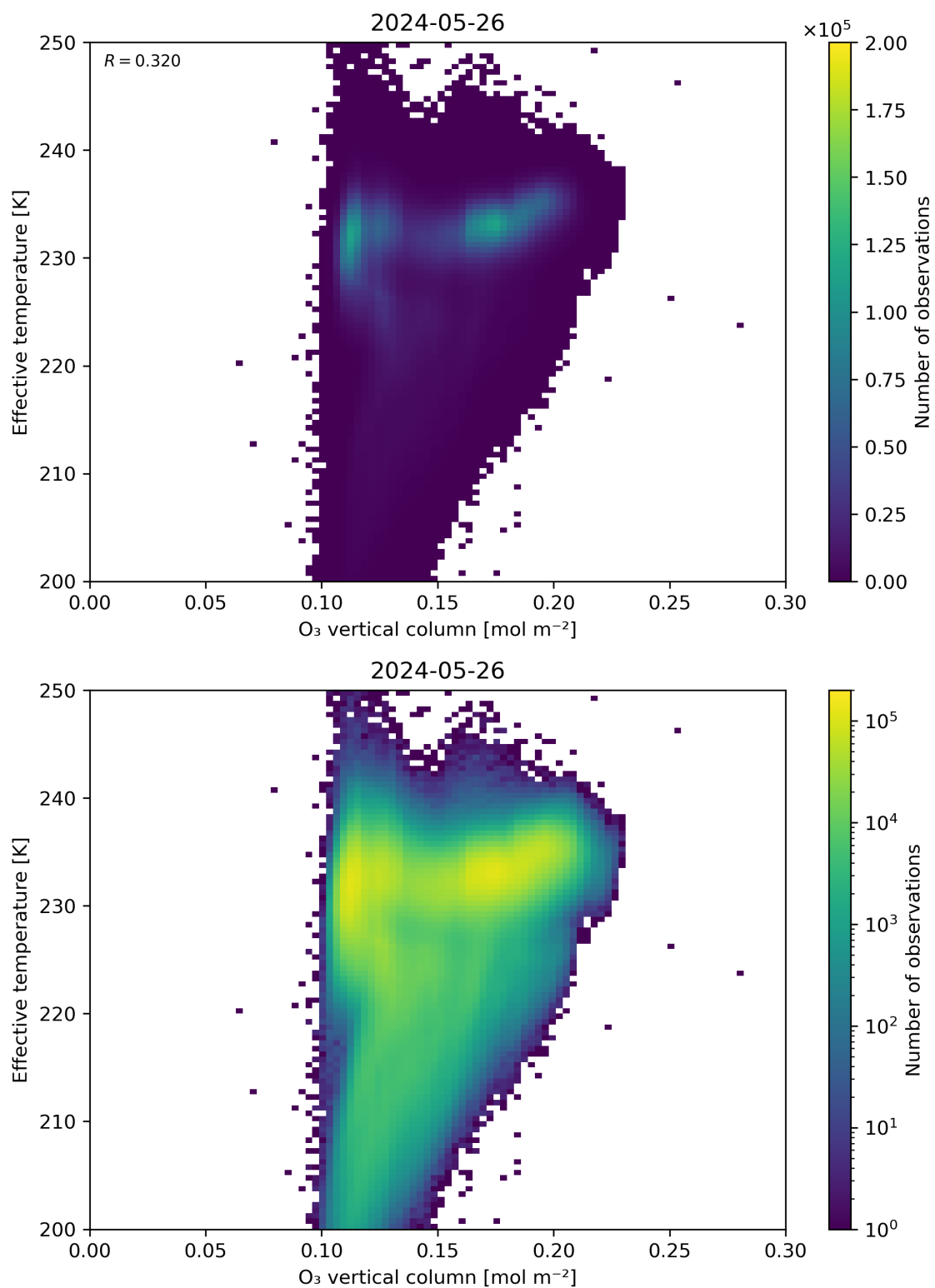
Figure 39: Scatter density plot of “O 3 vertical column” against “Effective temperature” for 2024-05-25 to 2024-05-27.
