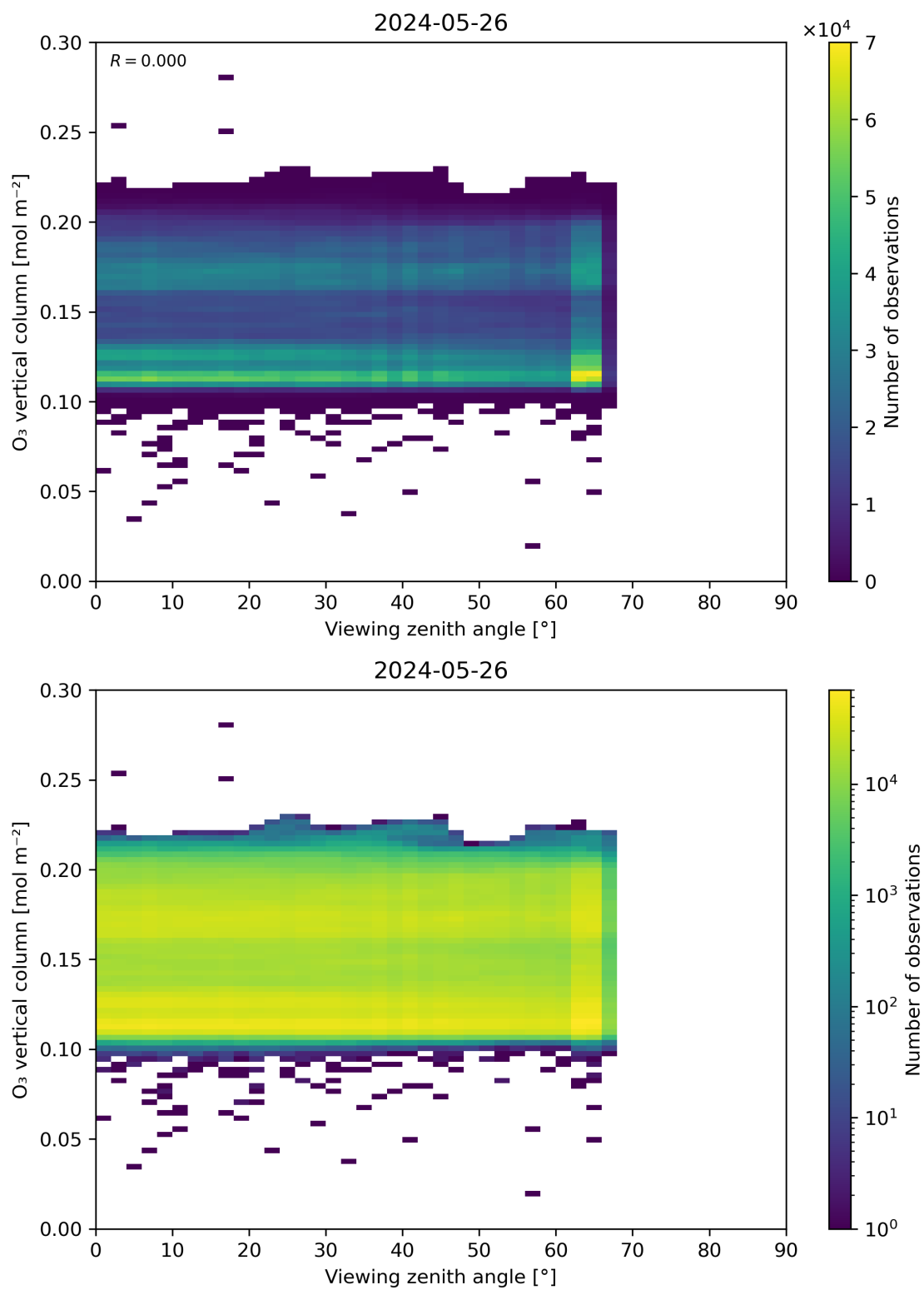
Figure 52: Scatter density plot of “Viewing zenith angle” against “O 3 vertical column” for 2024-05-25 to 2024-05-27.
