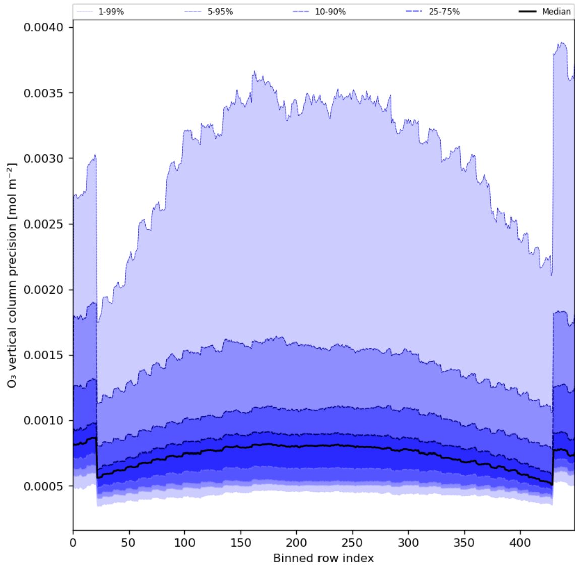
Figure 29: Along track statistics of “O 3 vertical column precision” for 2024-05-25 to 2024-05-27
