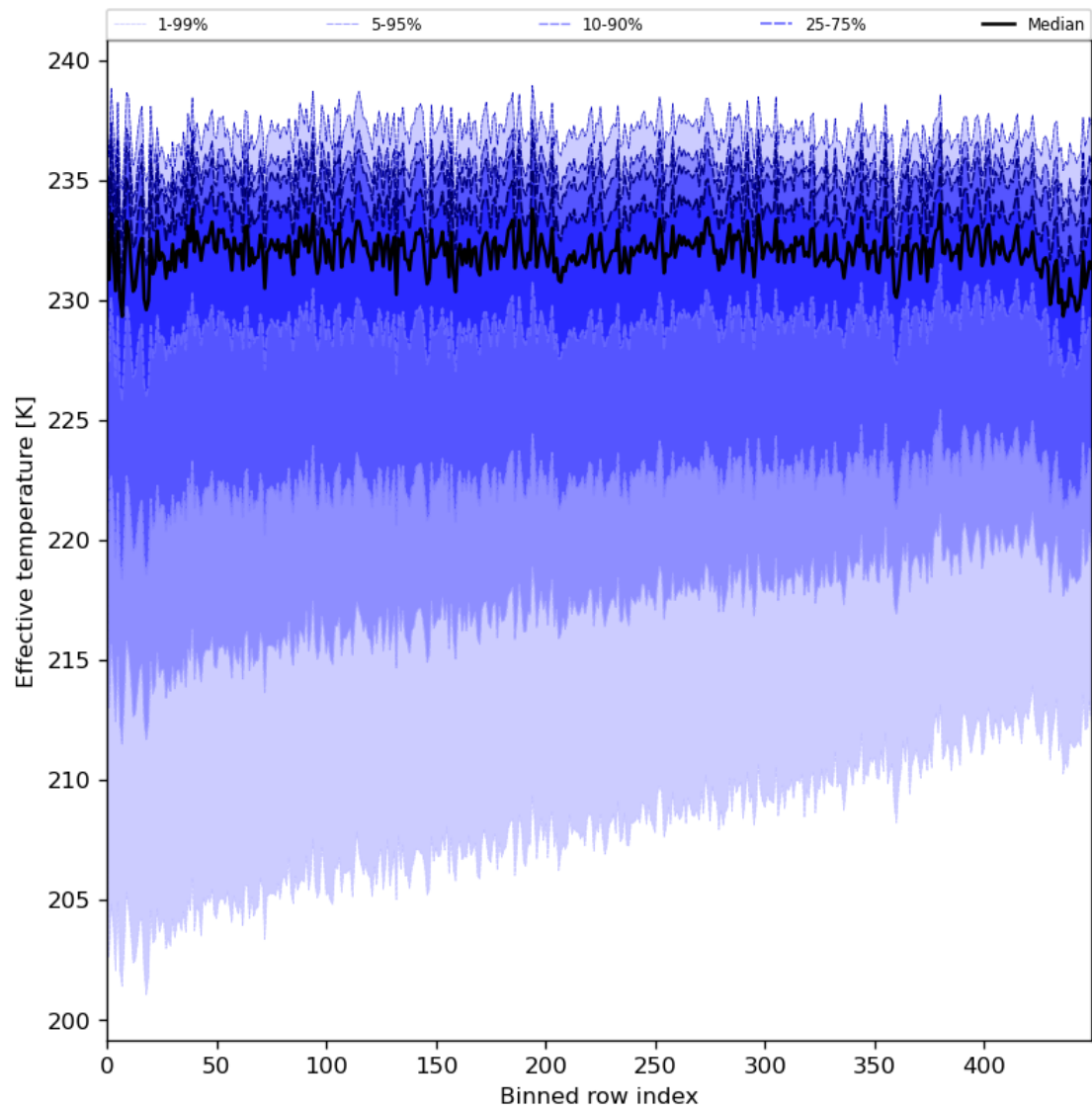
Figure 31: Along track statistics of “Effective temperature” for 2024-05-25 to 2024-05-27
