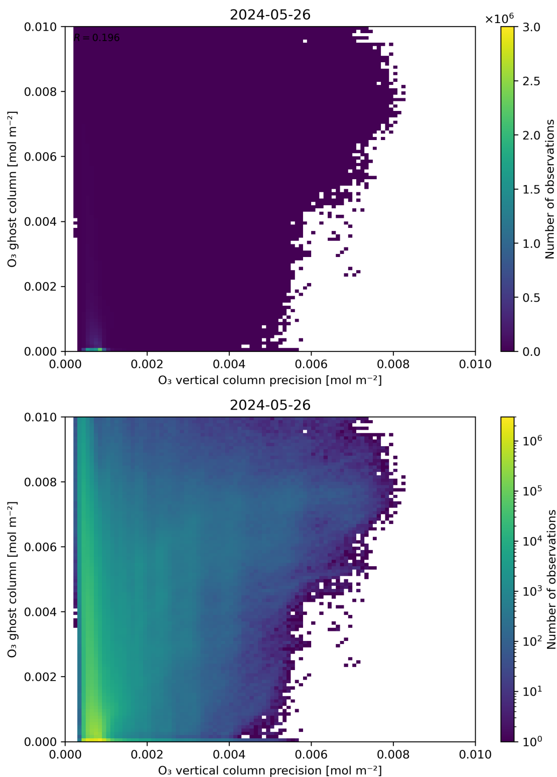
Figure 43: Scatter density plot of “ \text{O}_3 vertical column precision” against “ \text{O}_3 ghost column” for 2024-05-25 to 2024-05-27.
