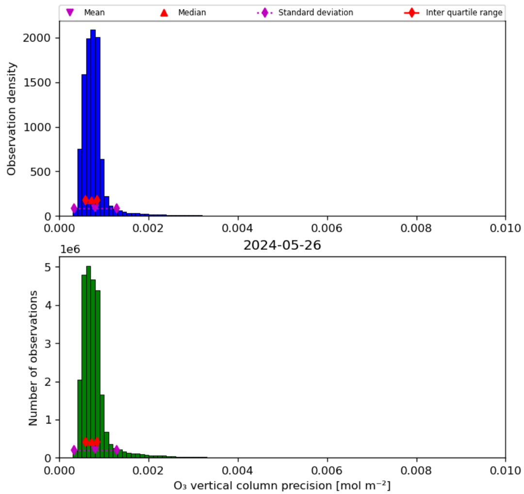
Figure 22: Histogram of “O 3 vertical column precision” for 2024-05-25 to 2024-05-27
