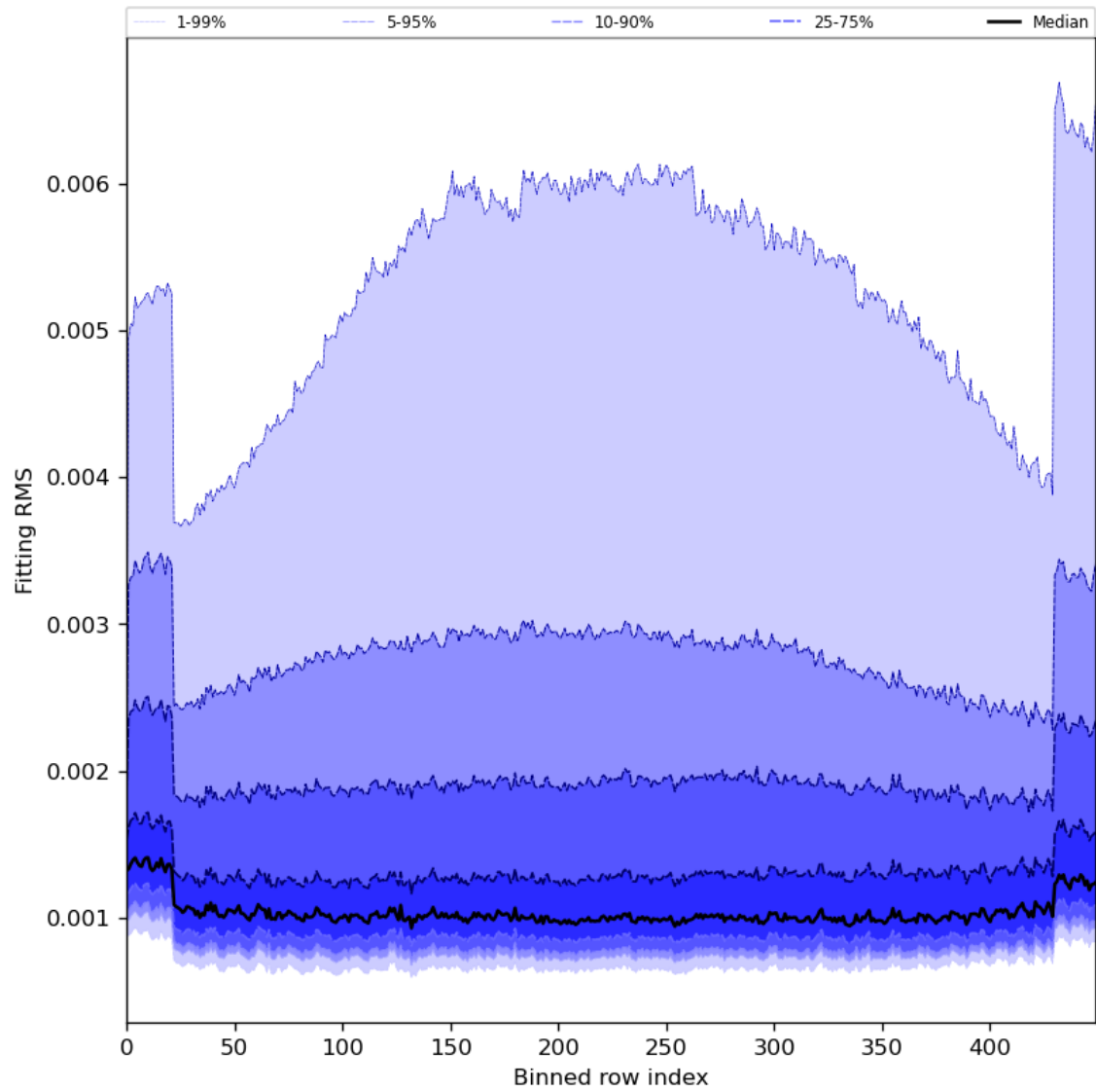
Figure 30: Along track statistics of “Fitting RMS” for 2024-05-25 to 2024-05-27
