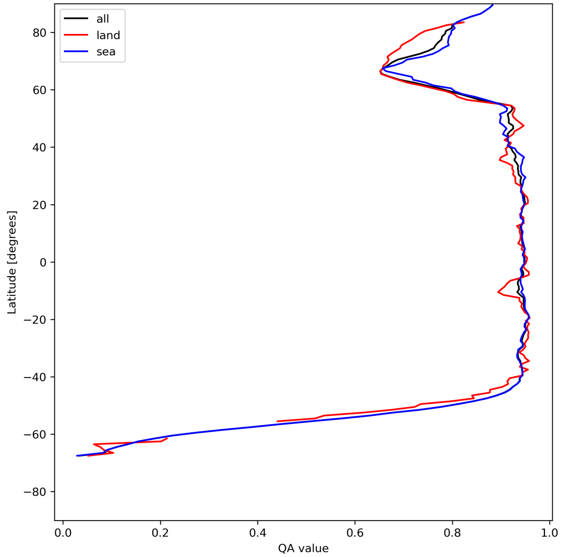
Figure 13: Zonal average of “QA value” for 2024-05-25 to 2024-05-27.
