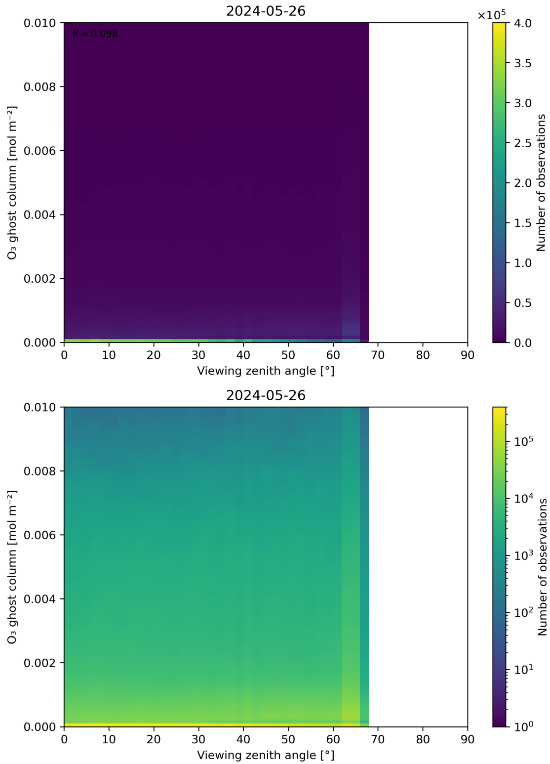
Figure 51: Scatter density plot of “Viewing zenith angle” against “O 3 ghost column” for 2024-05-25 to 2024-05-27.
