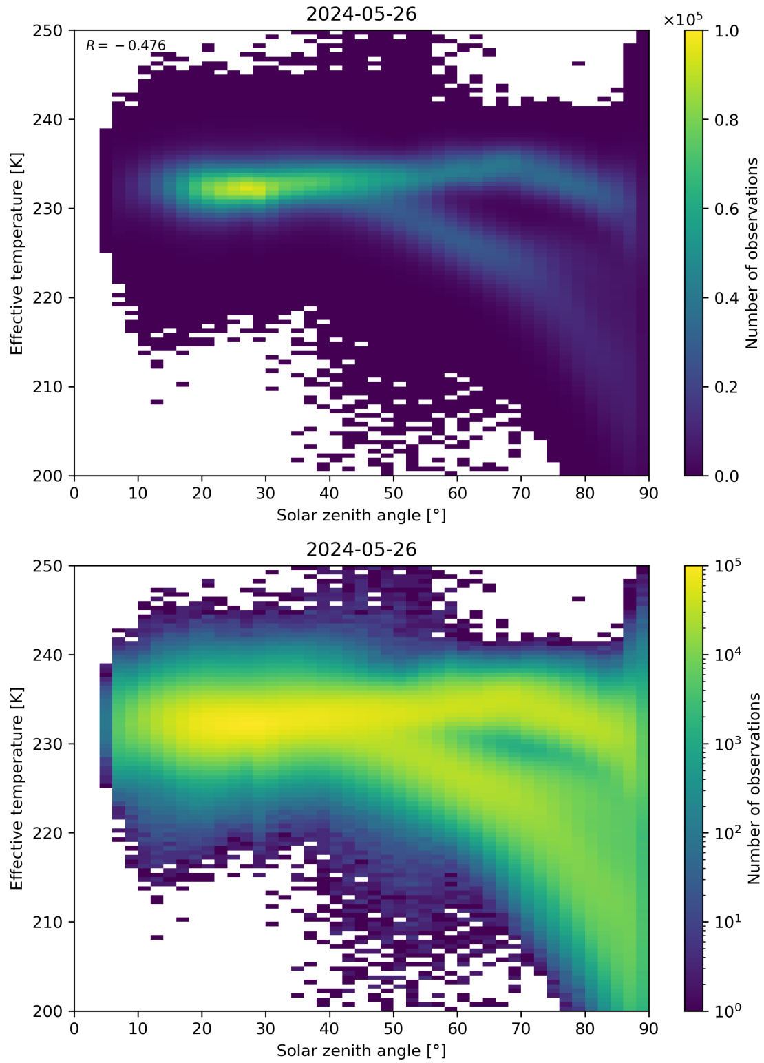
Figure 45: Scatter density plot of “Solar zenith angle” against “Effective temperature” for 2024-05-25 to 2024-05-27.
