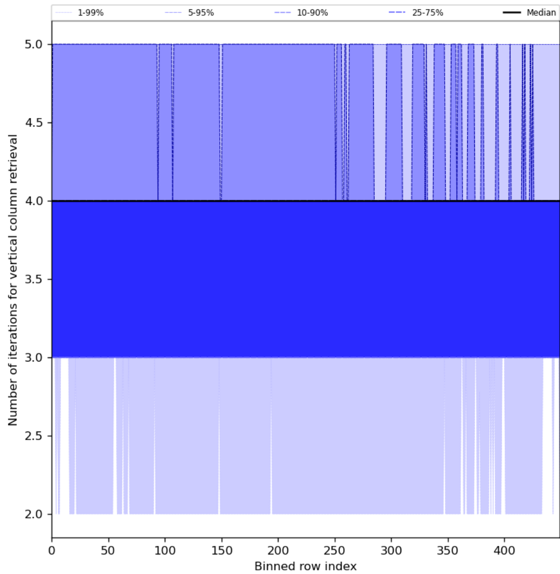
Figure 33: Along track statistics of “Number of iterations for vertical column retrieval” for 2024-05-25 to 2024-05-27
