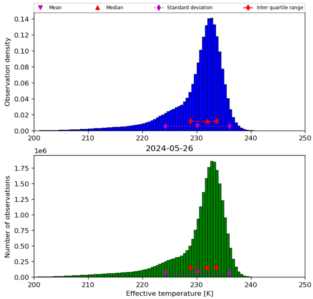
Figure 24: Histogram of “Effective temperature” for 2024-05-25 to 2024-05-27
