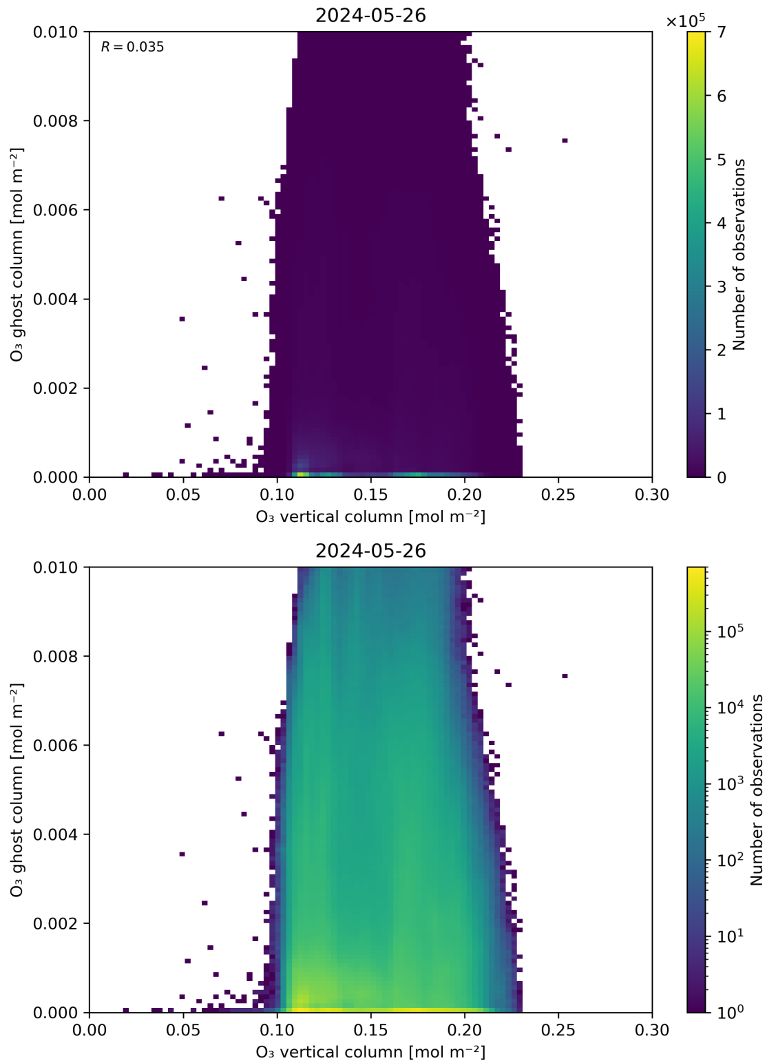
Figure 40: Scatter density plot of “O 3 vertical column” against “O 3 ghost column” for 2024-05-25 to 2024-05-27.
