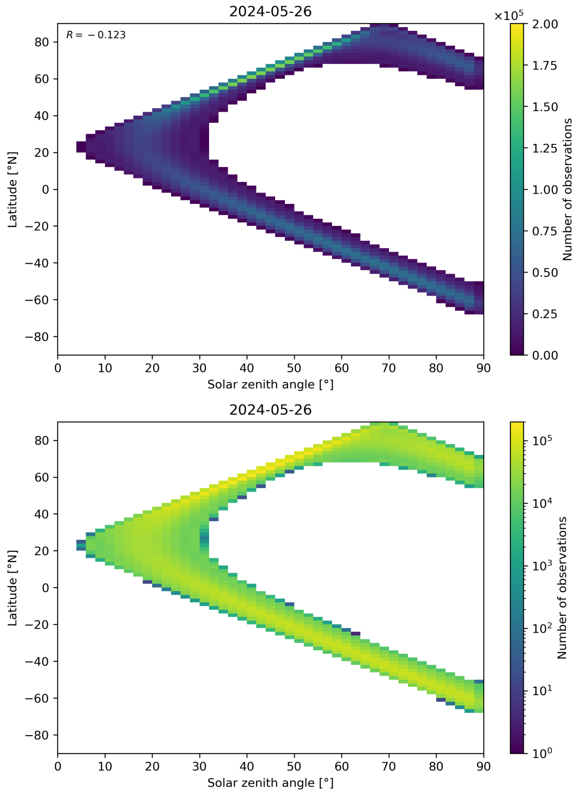
Figure 44: Scatter density plot of “Solar zenith angle” against “Latitude” for 2024-05-25 to 2024-05-27.
