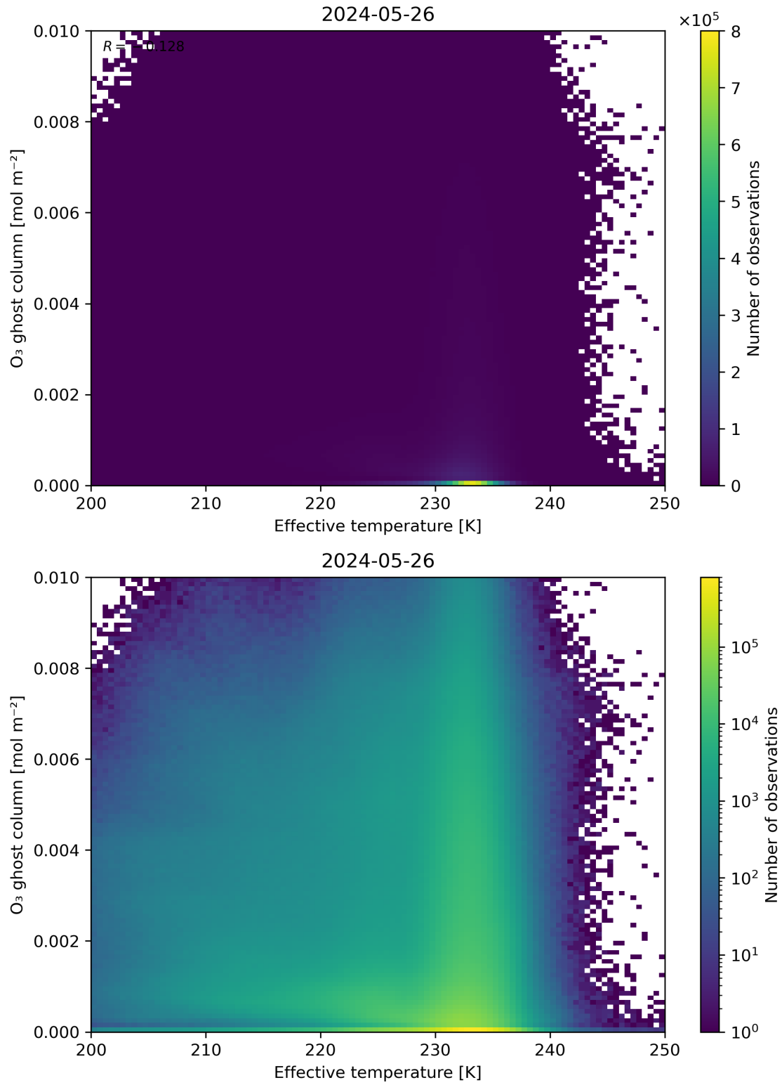
Figure 38: Scatter density plot of “Effective temperature” against “O 3 ghost column” for 2024-05-25 to 2024-05-27.
