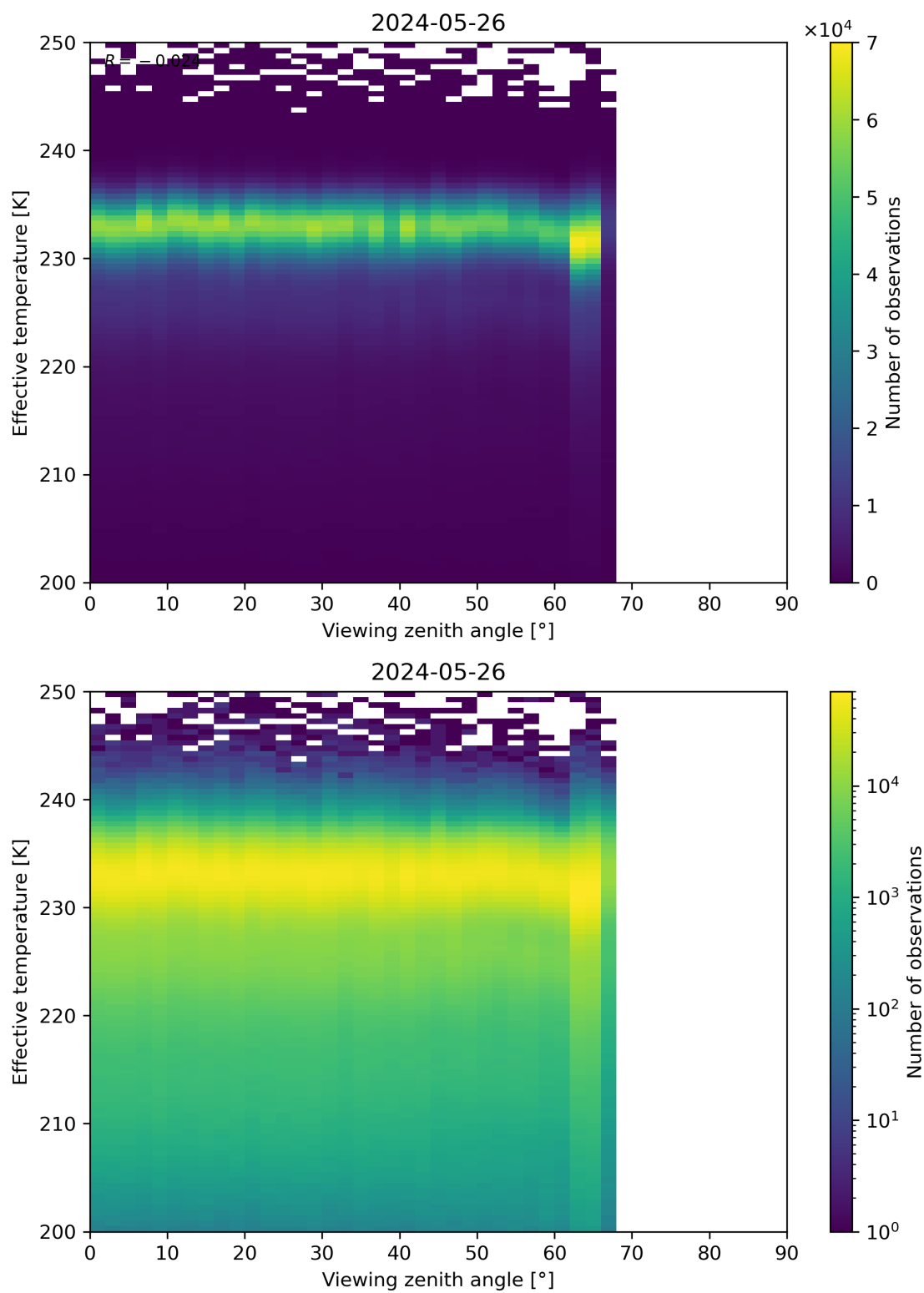
Figure 50: Scatter density plot of “Viewing zenith angle” against “Effective temperature” for 2024-05-25 to 2024-05-27.
