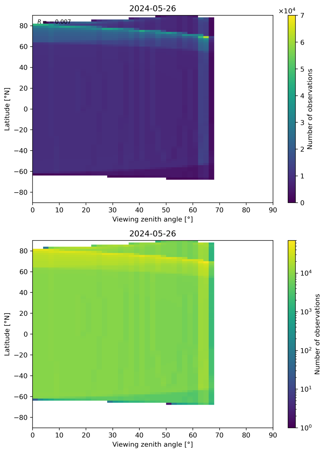
Figure 49: Scatter density plot of “Viewing zenith angle” against “Latitude” for 2024-05-25 to 2024-05-27.
