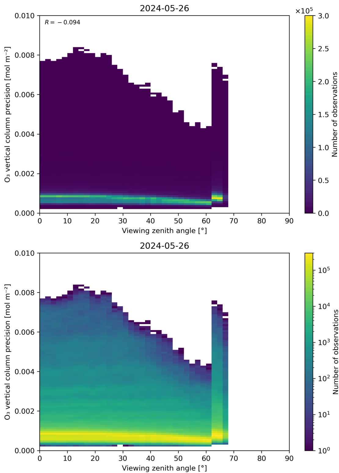
Figure 53: Scatter density plot of “Viewing zenith angle” against “O 3 vertical column precision” for 2024-05-25 to 2024-05-27.
