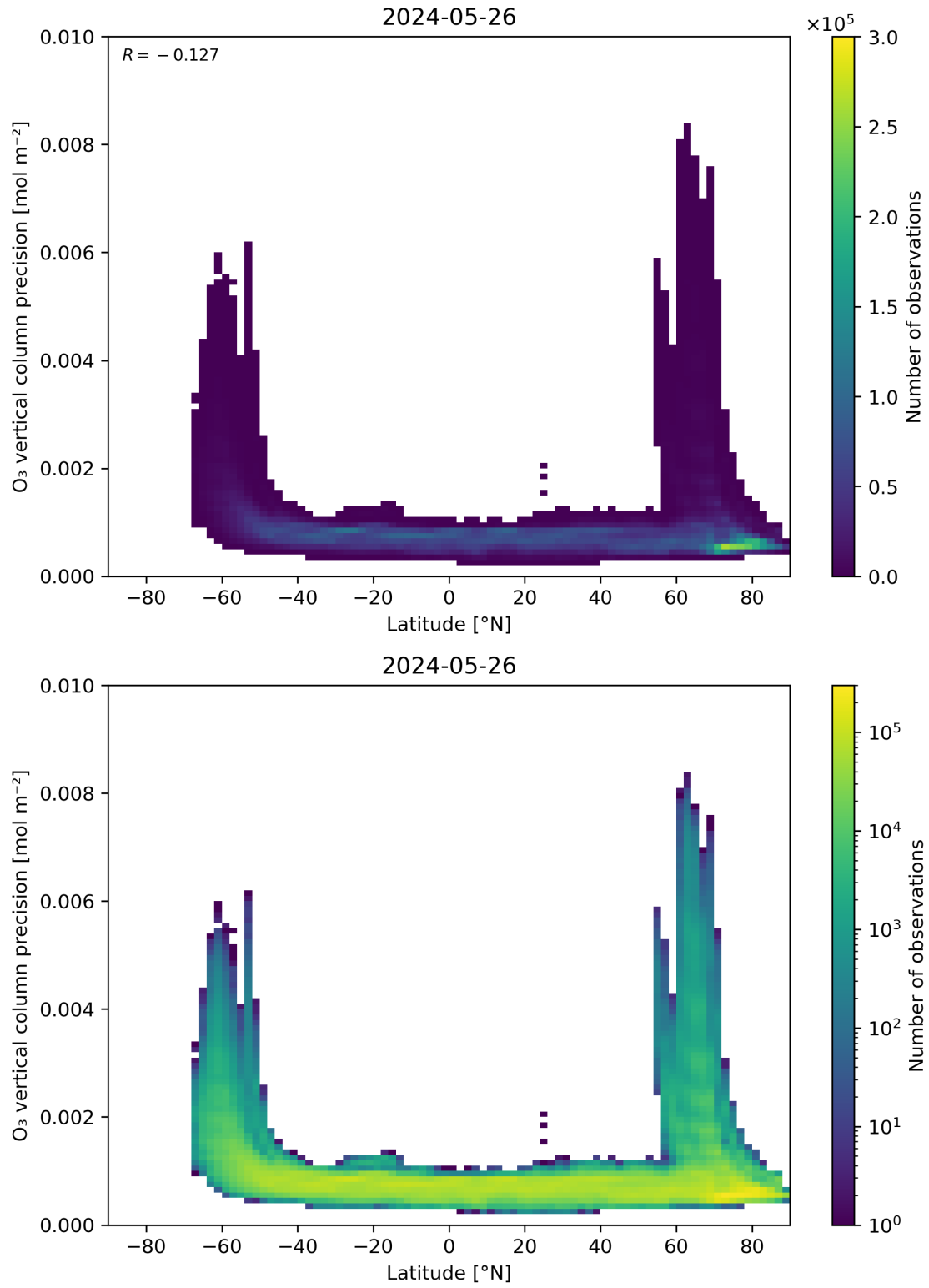
Figure 37: Scatter density plot of “Latitude” against “O 3 vertical column precision” for 2024-05-25 to 2024-05-27.
