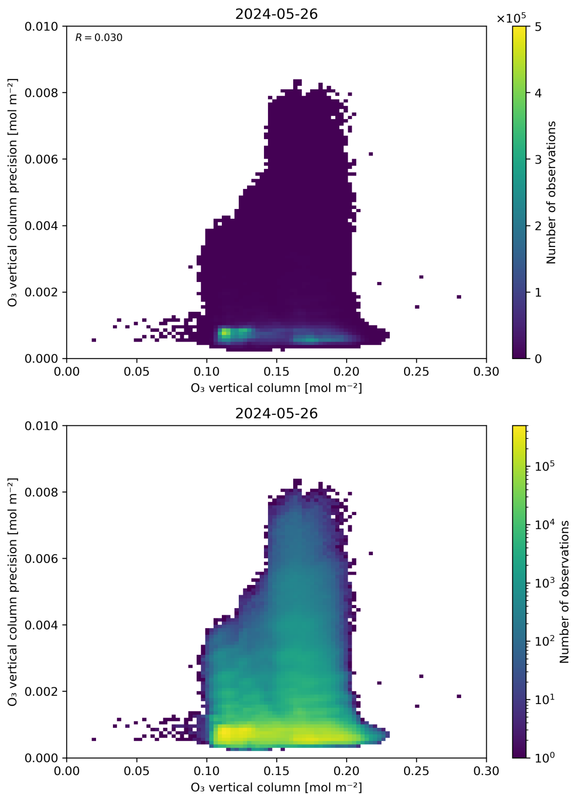
Figure 41: Scatter density plot of “O 3 vertical column” against “O 3 vertical column precision” for 2024-05-25 to 2024-05-27.
