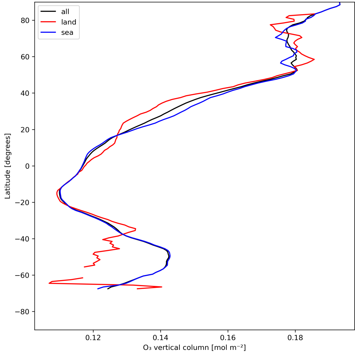
Figure 14: Zonal average of “O 3 vertical column” for 2024-05-25 to 2024-05-27.
