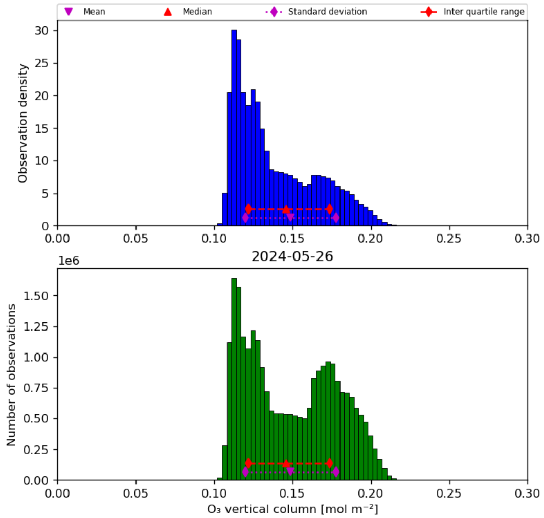
Figure 21: Histogram of “O 3 vertical column” for 2024-05-25 to 2024-05-27
