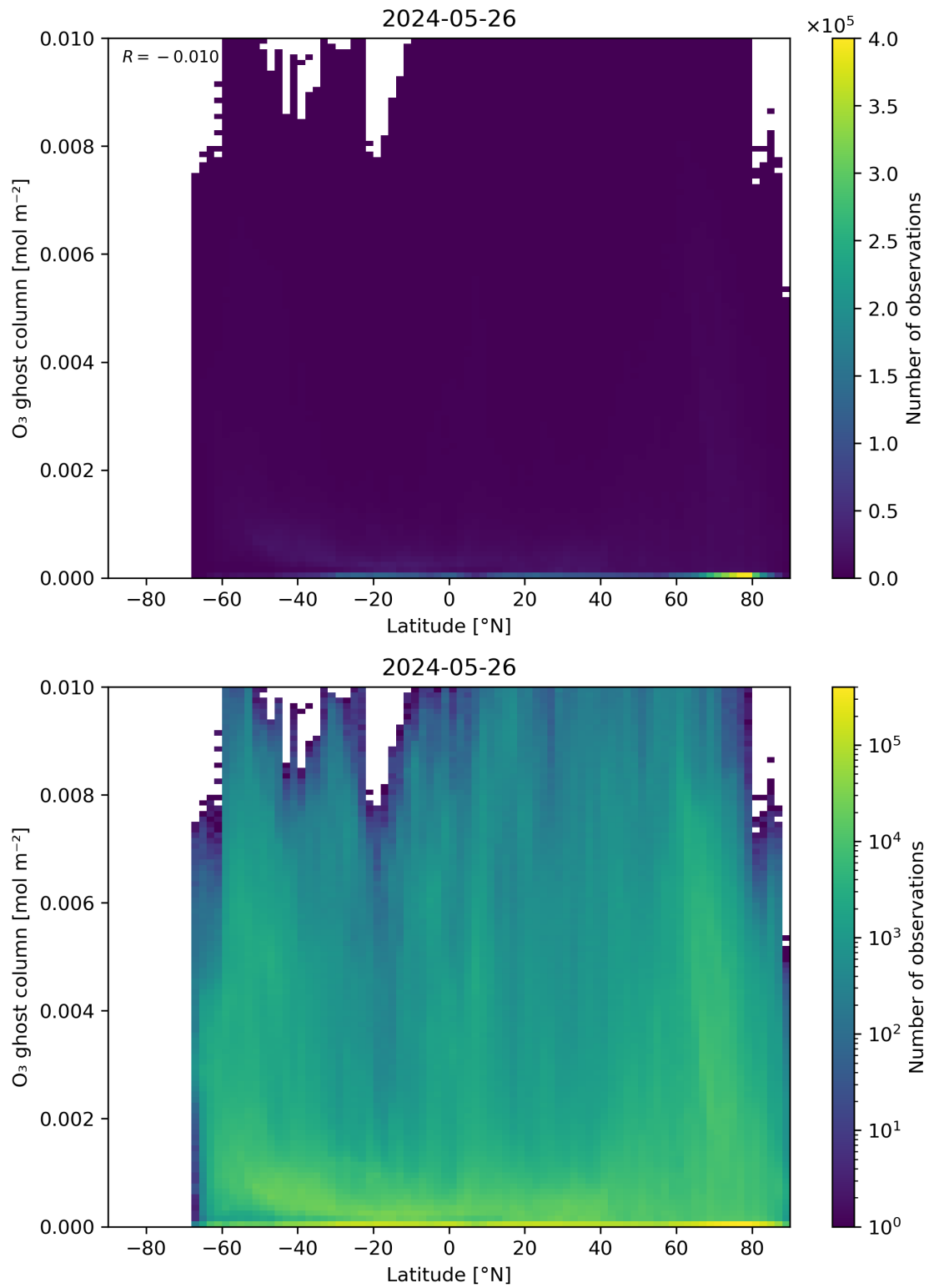
Figure 35: Scatter density plot of “Latitude” against “O 3 ghost column” for 2024-05-25 to 2024-05-27.
