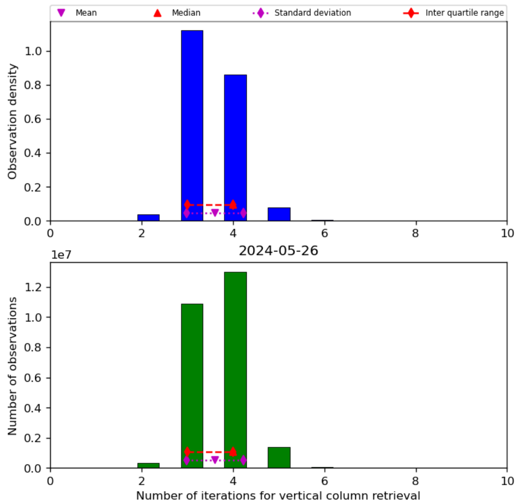
Figure 26: Histogram of “Number of iterations for vertical column retrieval” for 2024-05-25 to 2024-05-27
