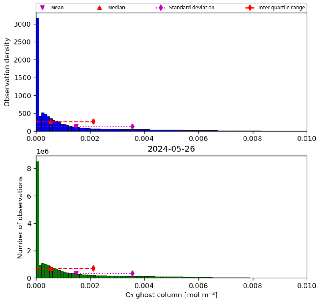
Figure 25: Histogram of “O 3 ghost column” for 2024-05-25 to 2024-05-27
