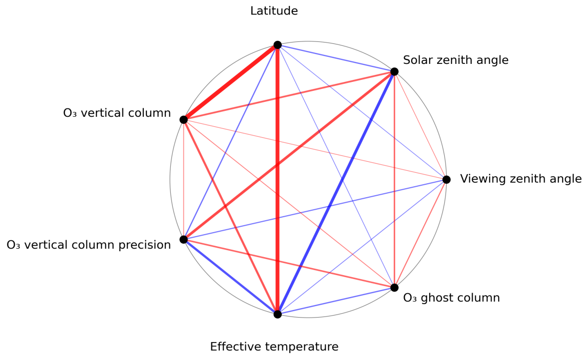
Figure 1: Map of correlation graph for 2024-05-25 to 2024-05-27.
