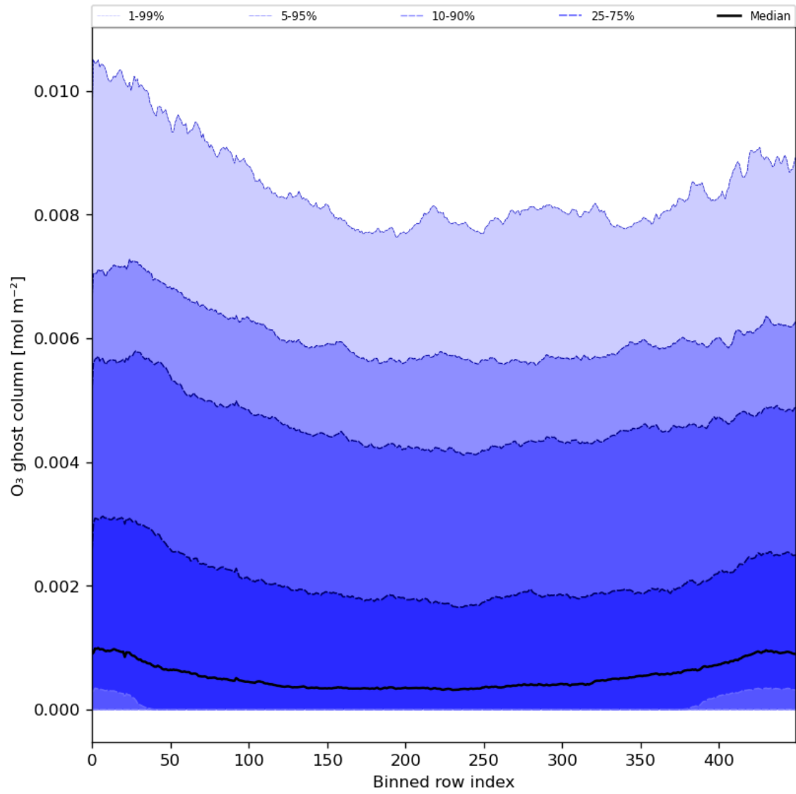
Figure 32: Along track statistics of “O 3 ghost column” for 2024-05-25 to 2024-05-27
