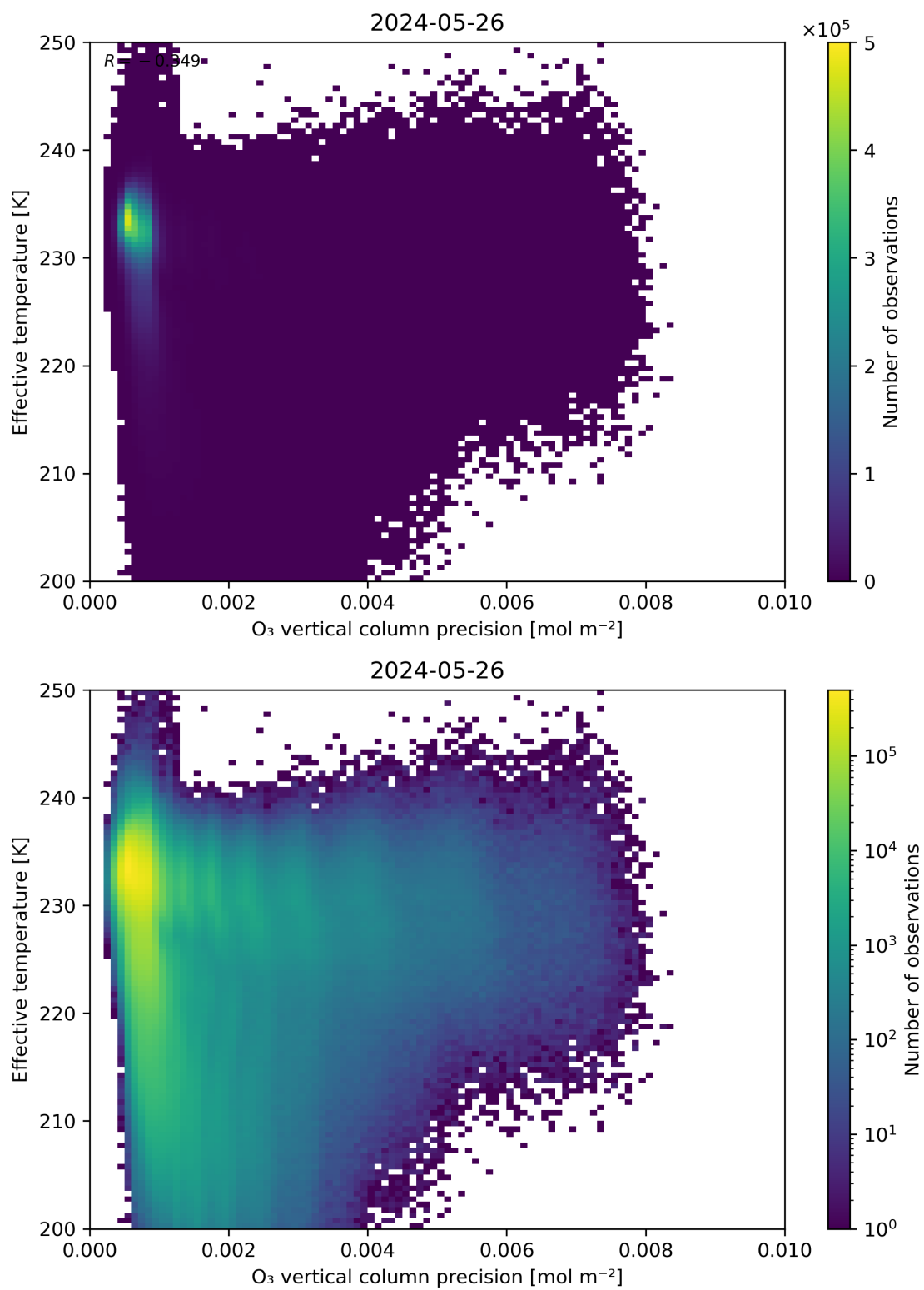
Figure 42: Scatter density plot of “O 3 vertical column precision” against “Effective temperature” for 2024-05-25 to 2024-05-27.
