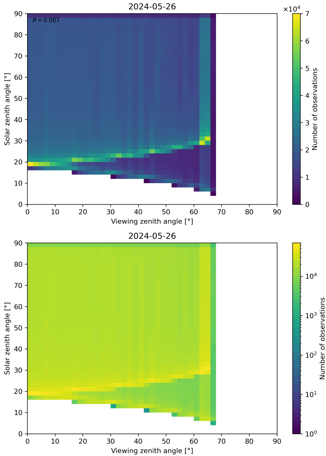
Figure 54: Scatter density plot of “Viewing zenith angle” against “Solar zenith angle” for 2024-05-25 to 2024-05-27.
