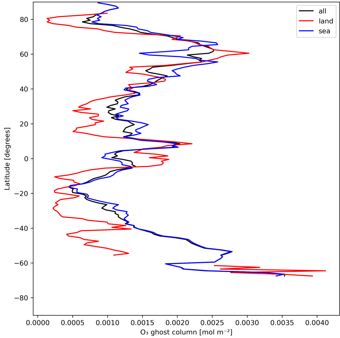
Figure 18: Zonal average of "O 3 ghost column" for 2024-05-25 to 2024-05-27.
