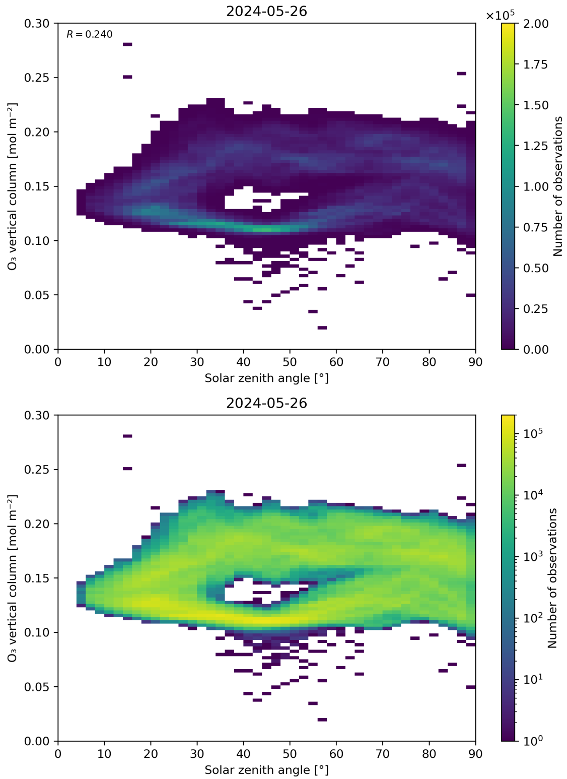
Figure 47: Scatter density plot of “Solar zenith angle” against “O 3 vertical column” for 2024-05-25 to 2024-05-27.
