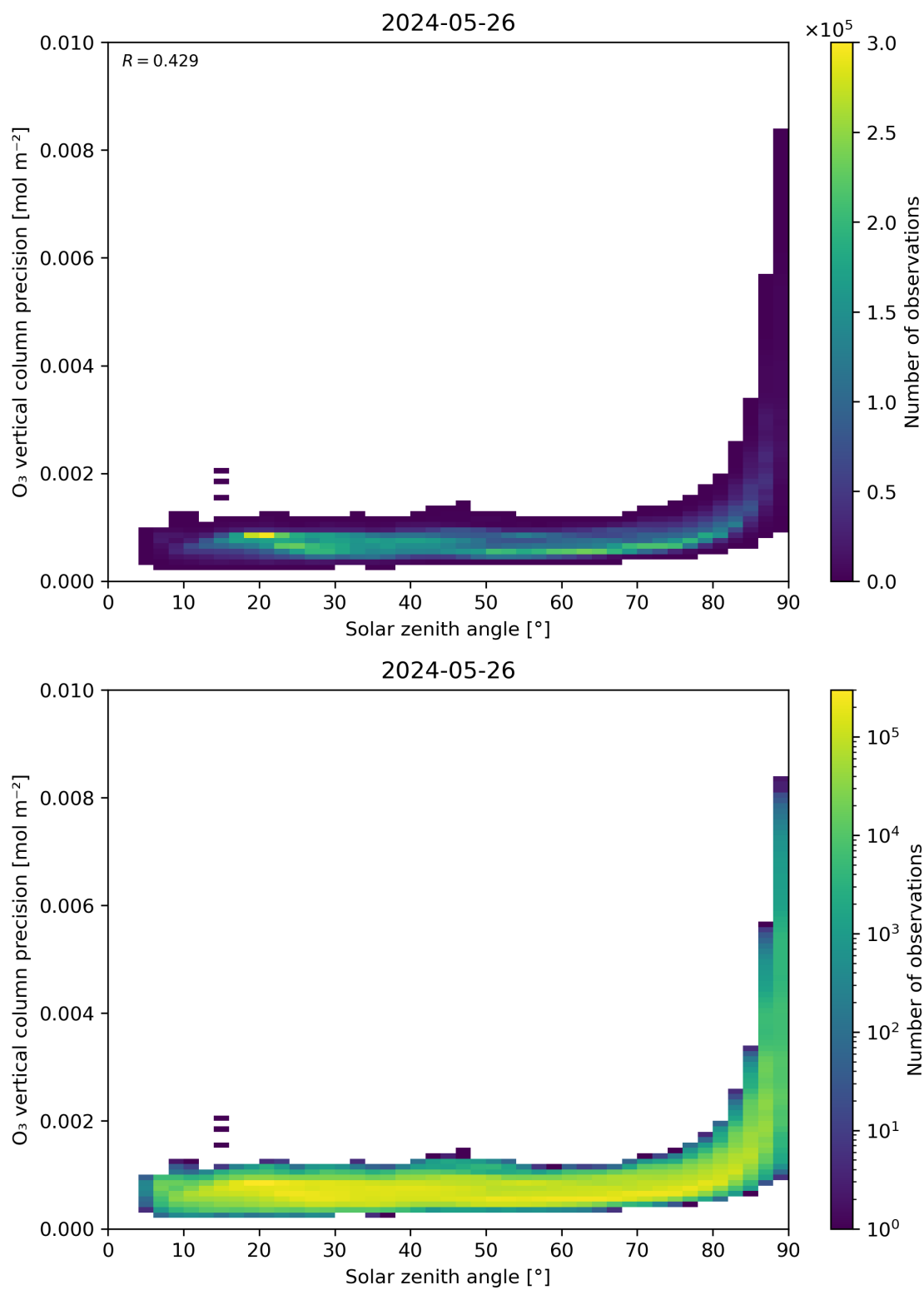
Figure 48: Scatter density plot of “Solar zenith angle” against “O 3 vertical column precision” for 2024-05-25 to 2024-05-27.
