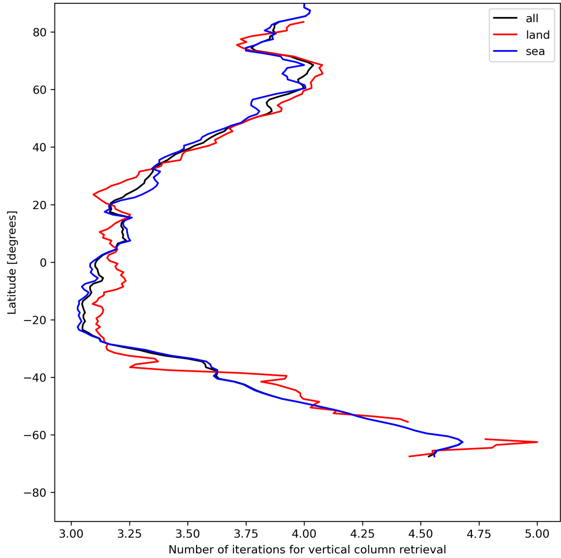
Figure 19: Zonal average of “Number of iterations for vertical column retrieval” for 2024-05-25 to 2024-05-27.
