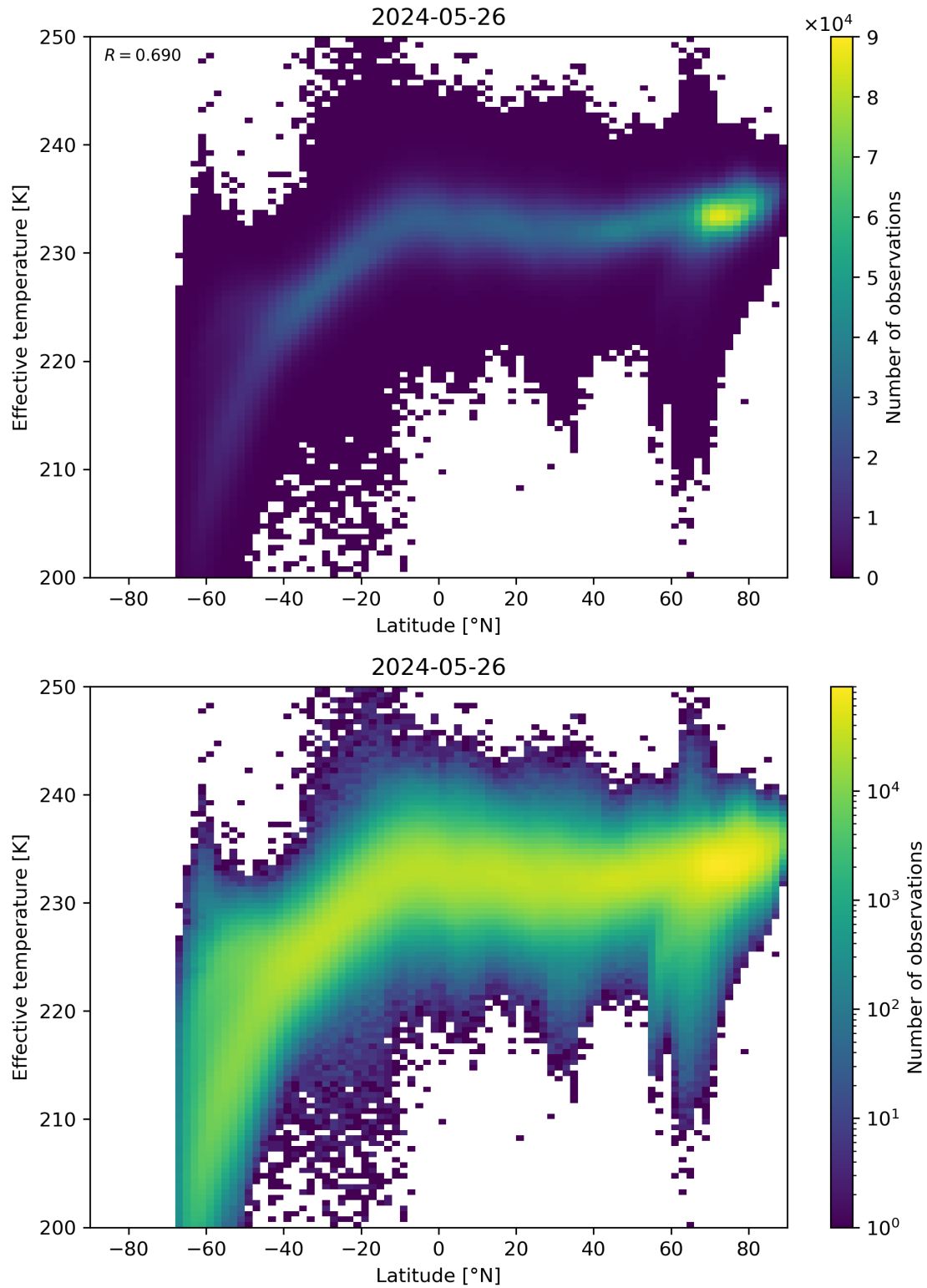
Figure 34: Scatter density plot of “Latitude” against “Effective temperature” for 2024-05-25 to 2024-05-27.
