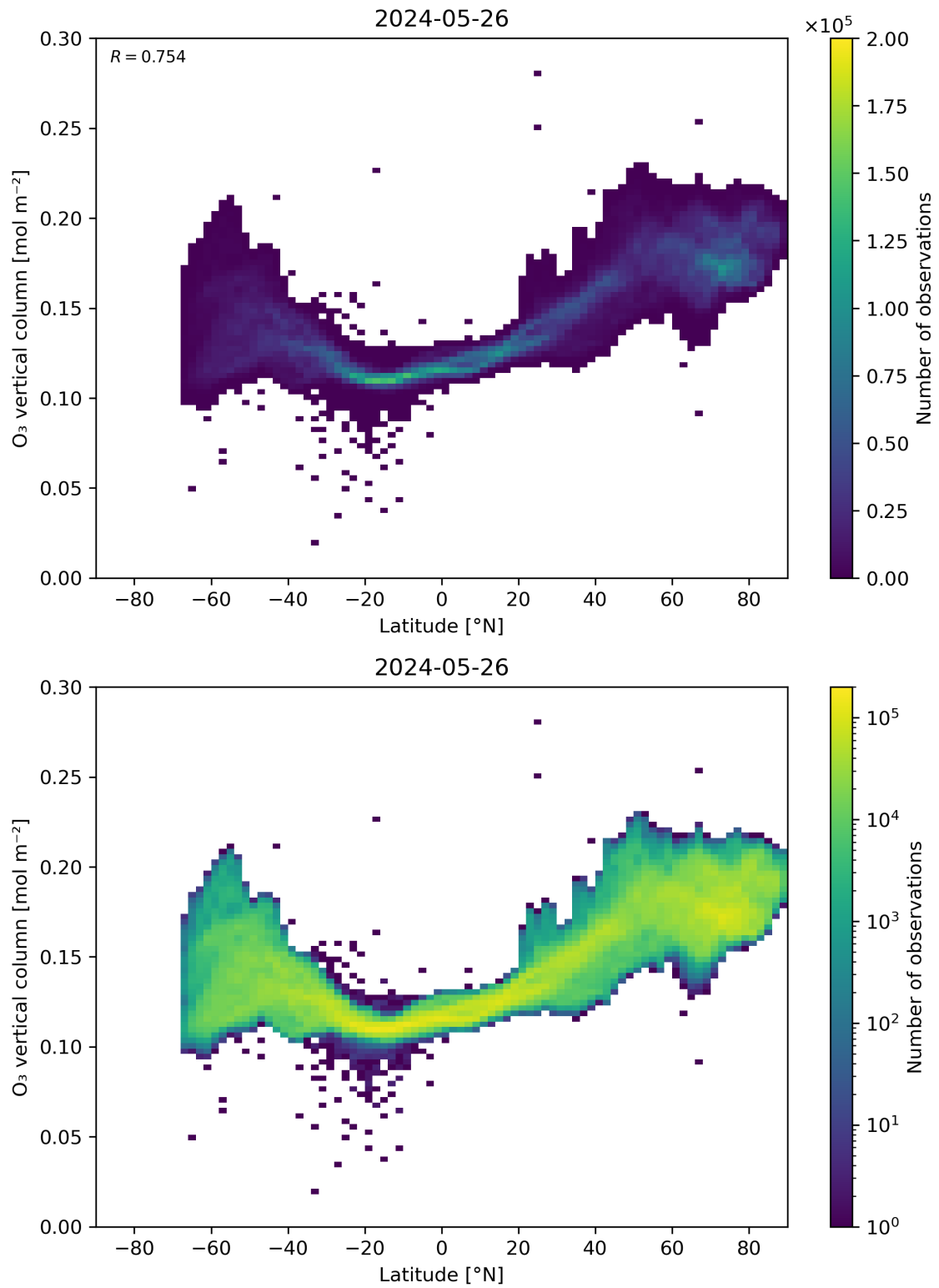
Figure 36: Scatter density plot of “Latitude” against “O 3 vertical column” for 2024-05-25 to 2024-05-27.
