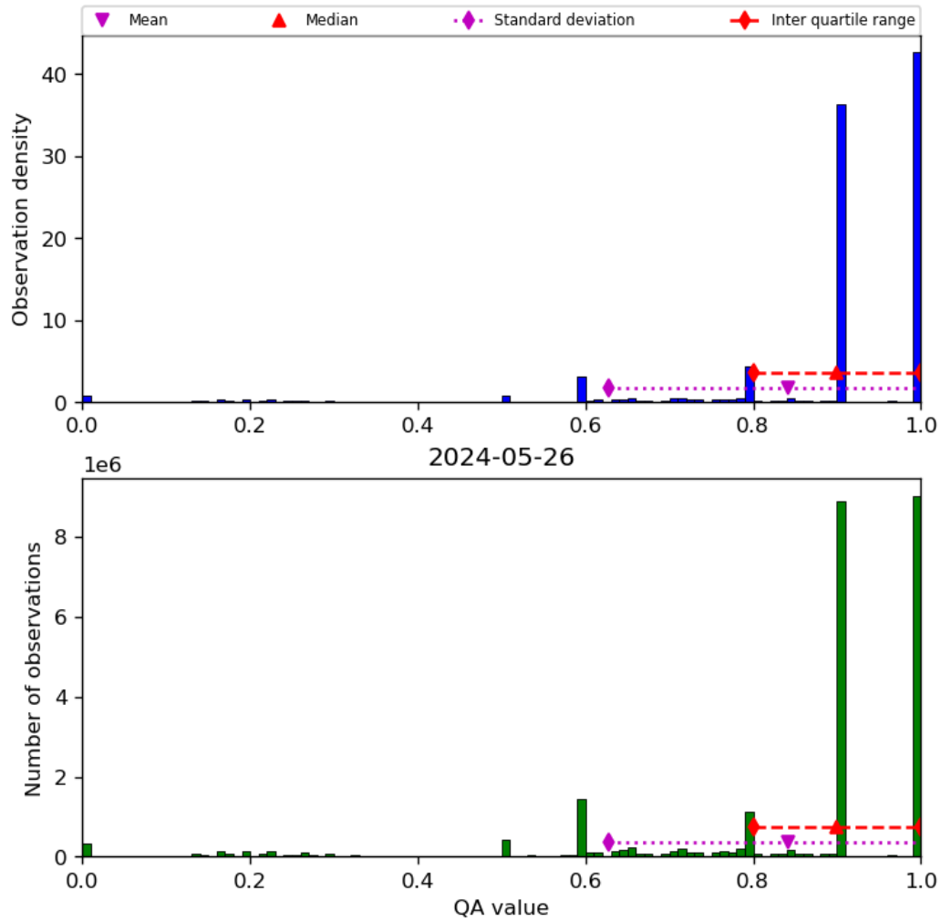
Figure 20: Histogram of “QA value” for 2024-05-25 to 2024-05-27
