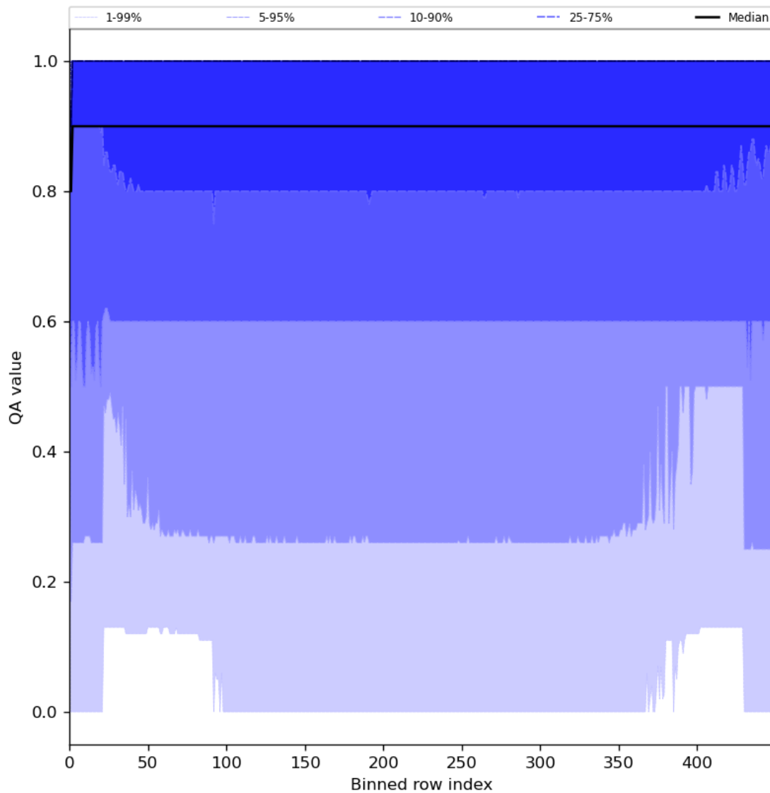
Figure 27: Along track statistics of “QA value” for 2024-05-25 to 2024-05-27
