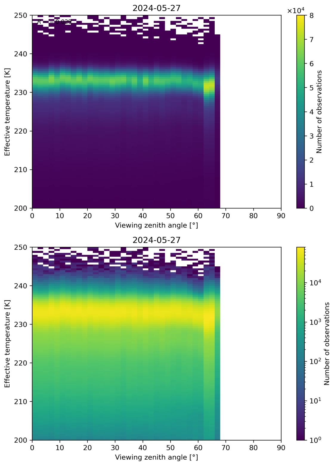
Figure 50: Scatter density plot of “Viewing zenith angle” against “Effective temperature” for 2024-05-26 to 2024-05-28.
