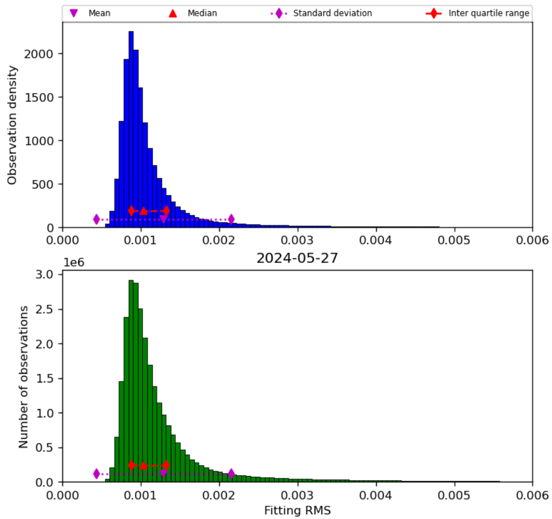
Figure 23: Histogram of “Fitting RMS” for 2024-05-26 to 2024-05-28
