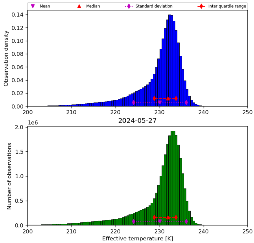
Figure 24: Histogram of “Effective temperature” for 2024-05-26 to 2024-05-28
