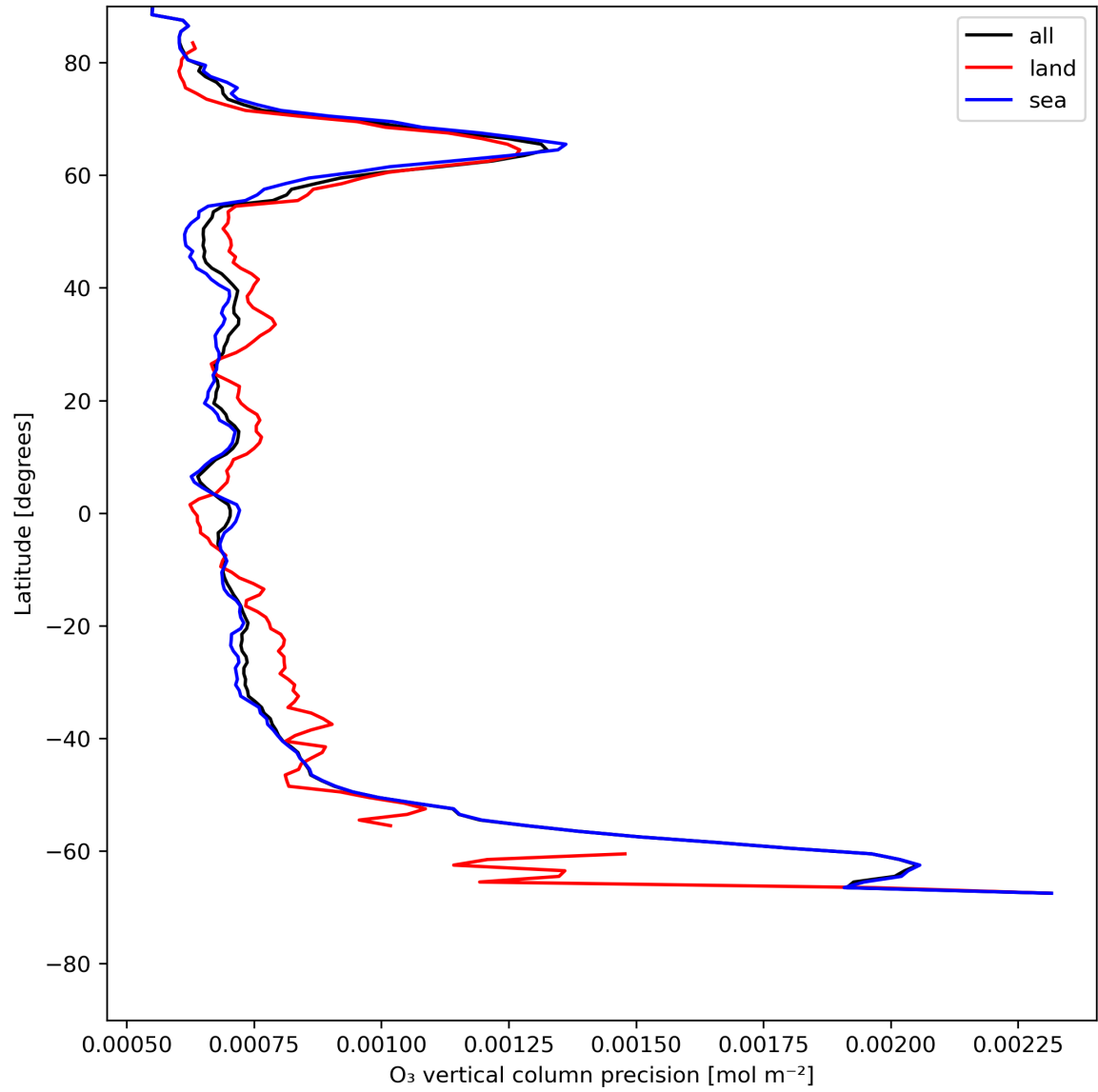
Figure 15: Zonal average of “O 3 vertical column precision” for 2024-05-26 to 2024-05-28.
