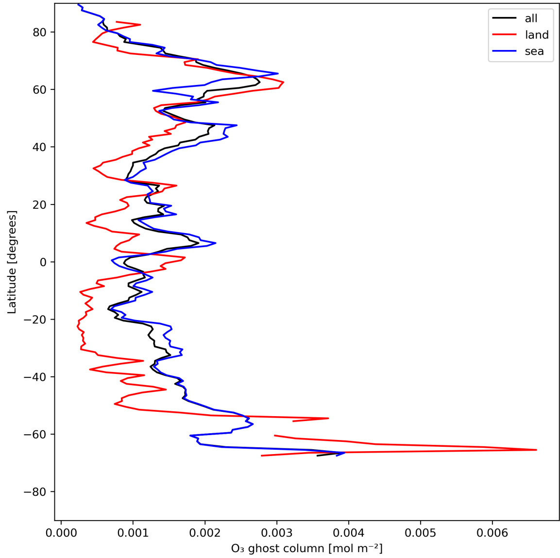
Figure 18: Zonal average of "O 3 ghost column" for 2024-05-26 to 2024-05-28.
