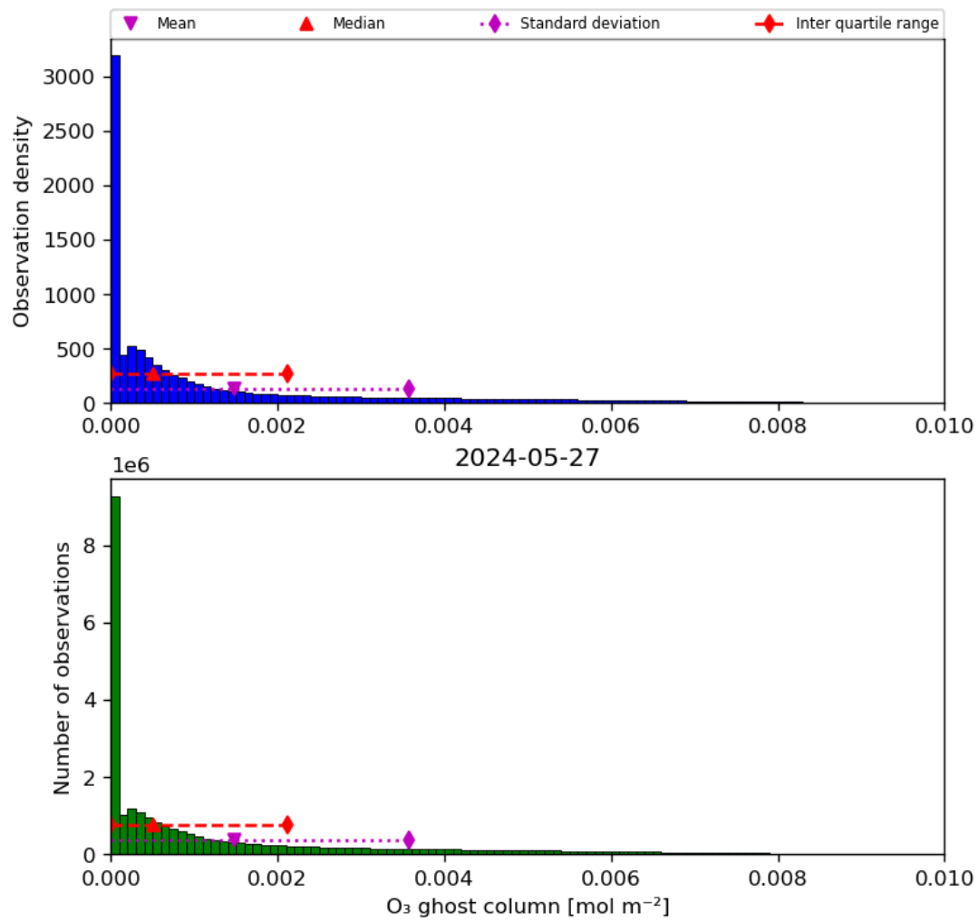
Figure 25: Histogram of "O 3 ghost column" for 2024-05-26 to 2024-05-28
