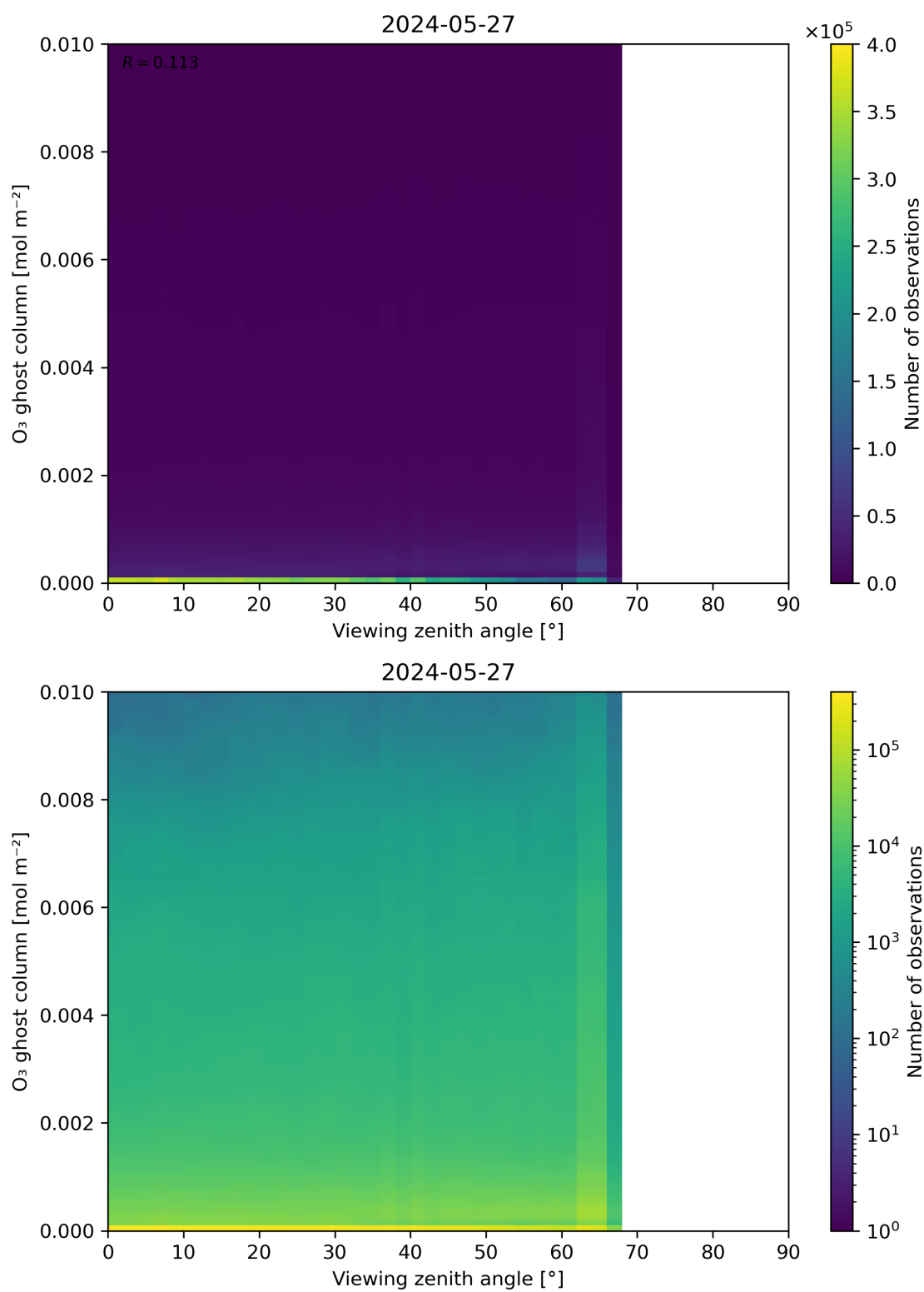
Figure 51: Scatter density plot of “Viewing zenith angle” against “O 3 ghost column” for 2024-05-26 to 2024-05-28.
