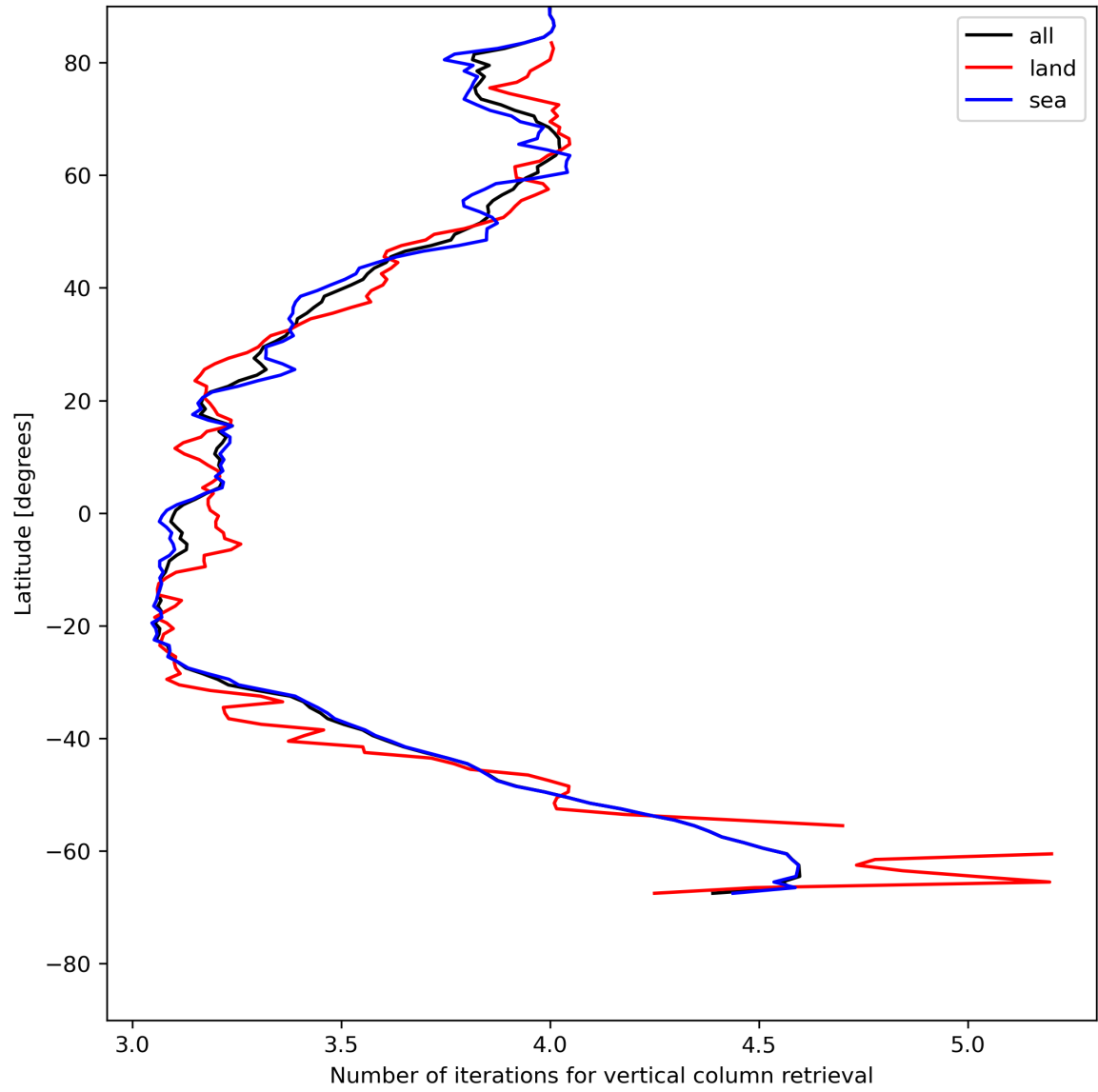
Figure 19: Zonal average of “Number of iterations for vertical column retrieval” for 2024-05-26 to 2024-05-28.
