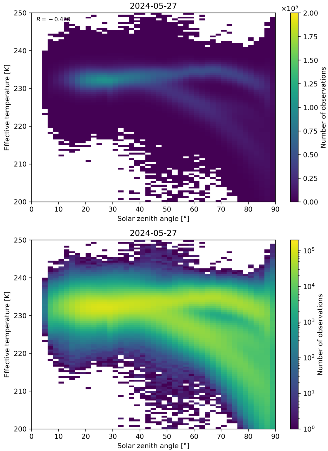
Figure 45: Scatter density plot of “Solar zenith angle” against “Effective temperature” for 2024-05-26 to 2024-05-28.
