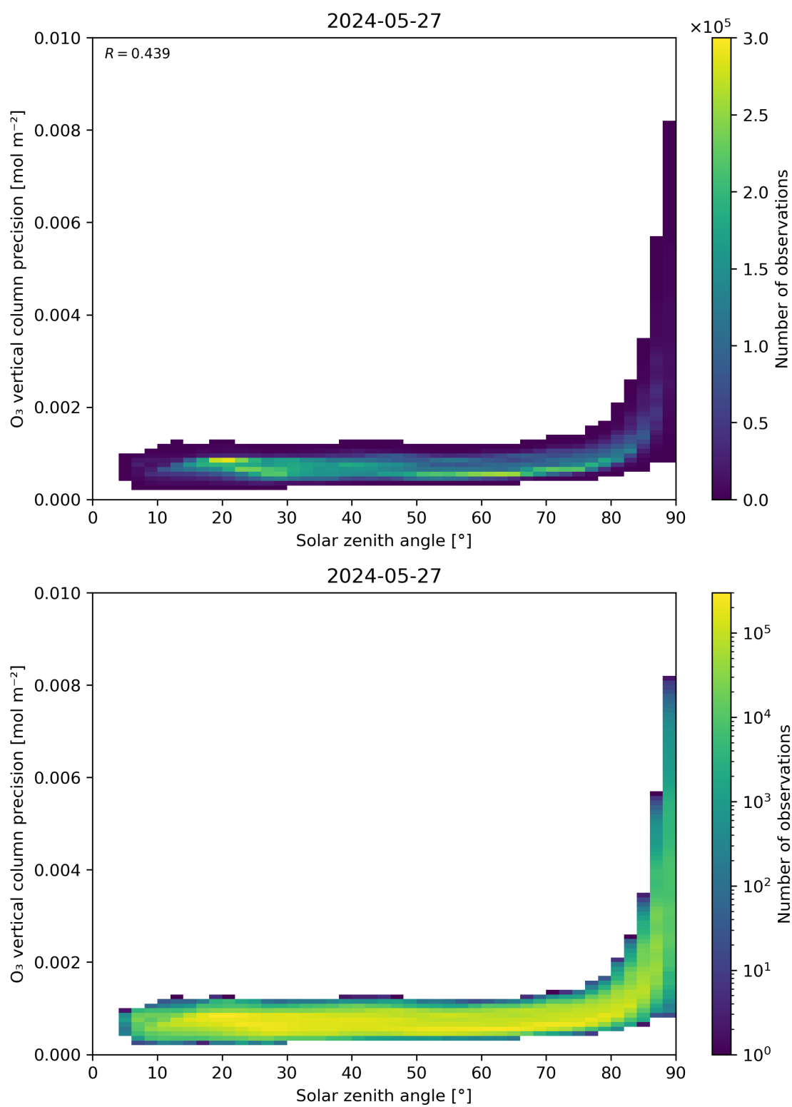
Figure 48: Scatter density plot of “Solar zenith angle” against “O 3 vertical column precision” for 2024-05-26 to 2024-05-28.
