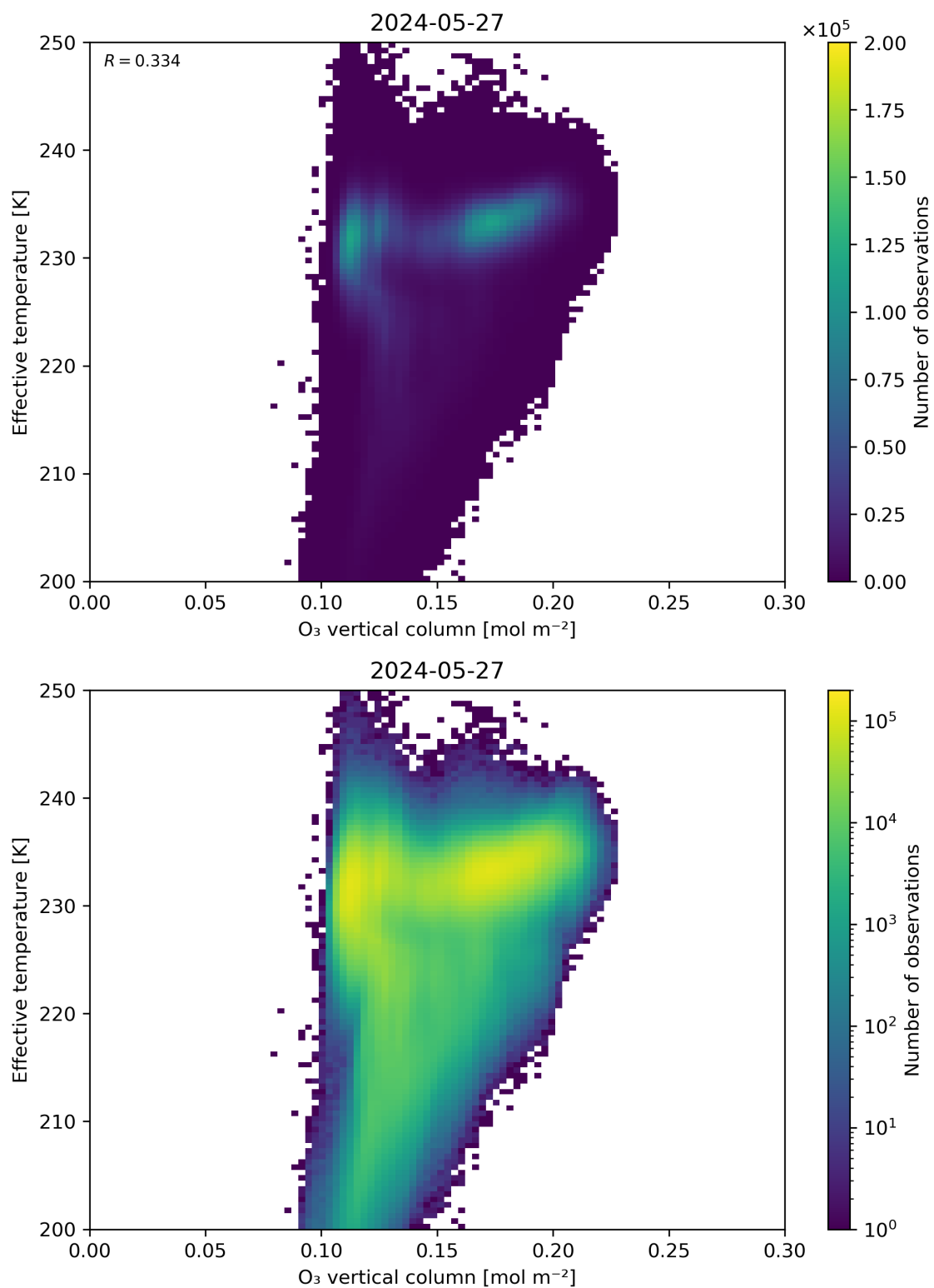
Figure 39: Scatter density plot of “O 3 vertical column” against “Effective temperature” for 2024-05-26 to 2024-05-28.
