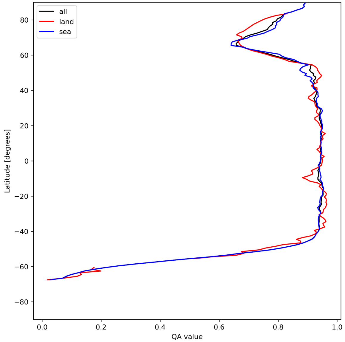
Figure 13: Zonal average of “QA value” for 2024-05-26 to 2024-05-28.
