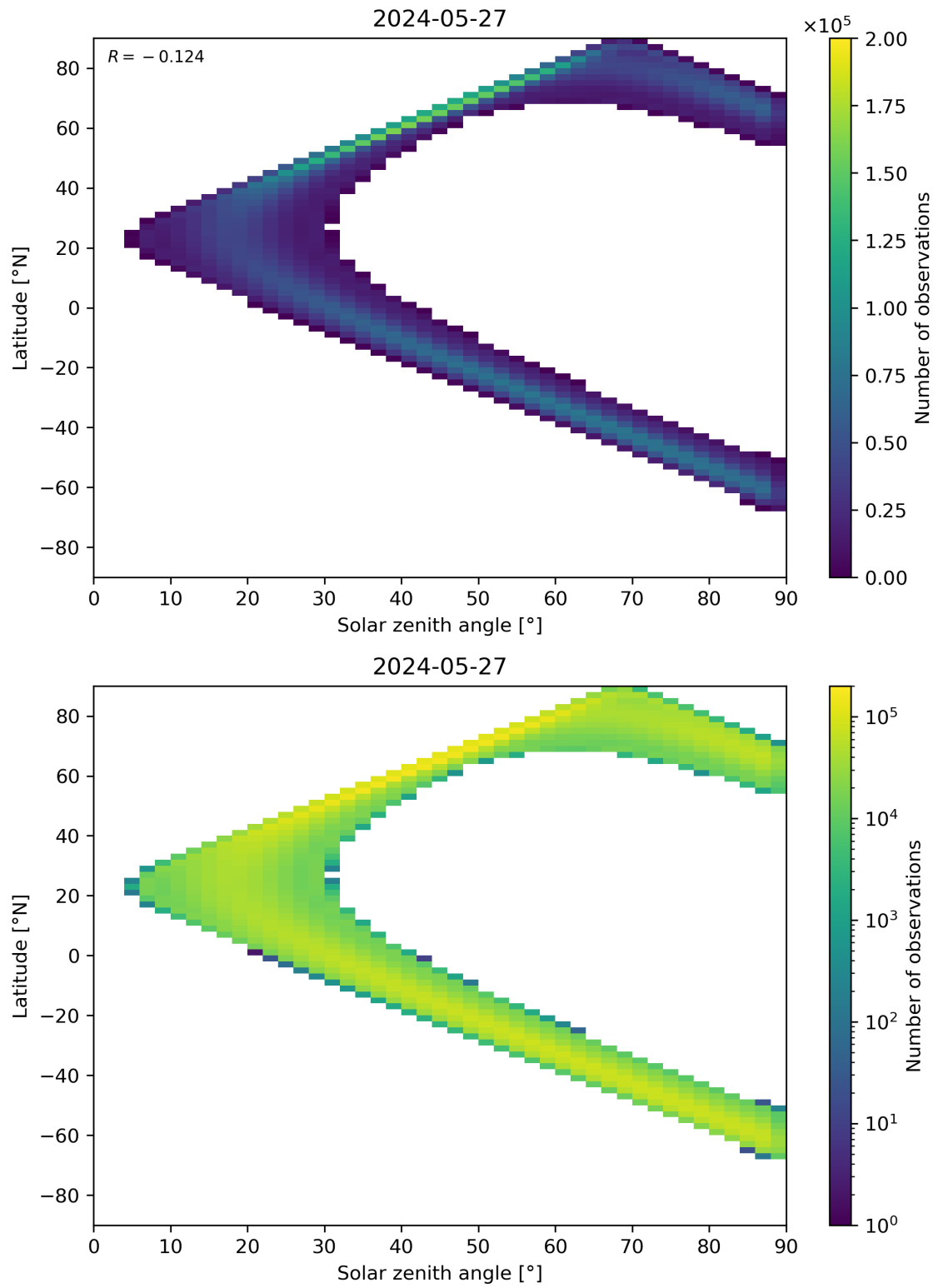
Figure 44: Scatter density plot of “Solar zenith angle” against “Latitude” for 2024-05-26 to 2024-05-28.
