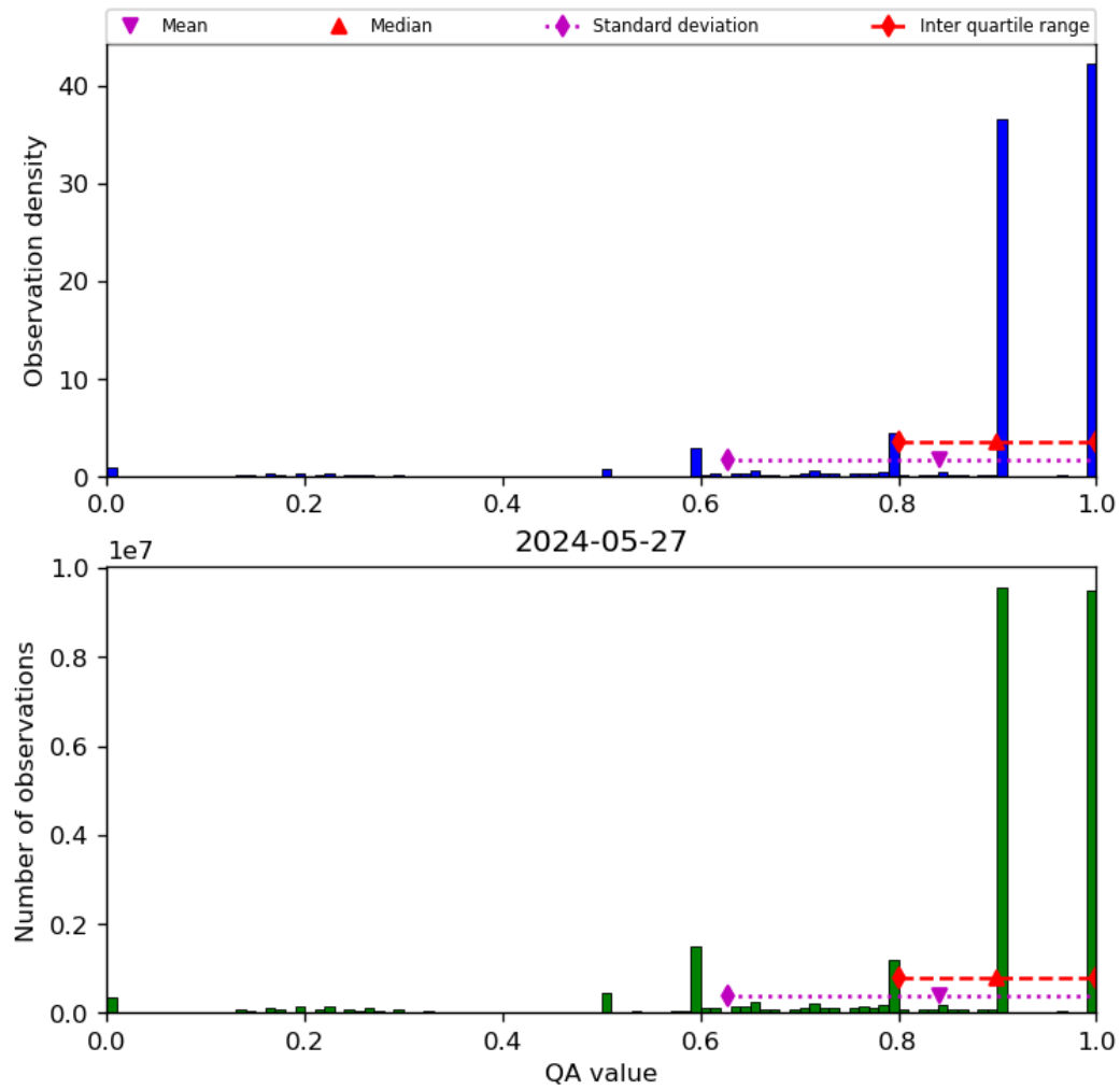
Figure 20: Histogram of “QA value” for 2024-05-26 to 2024-05-28
