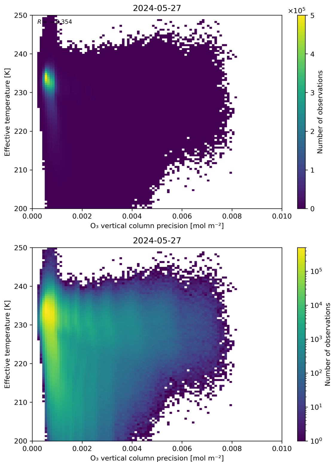
Figure 42: Scatter density plot of “O 3 vertical column precision” against “Effective temperature” for 2024-05-26 to 2024-05-28.
