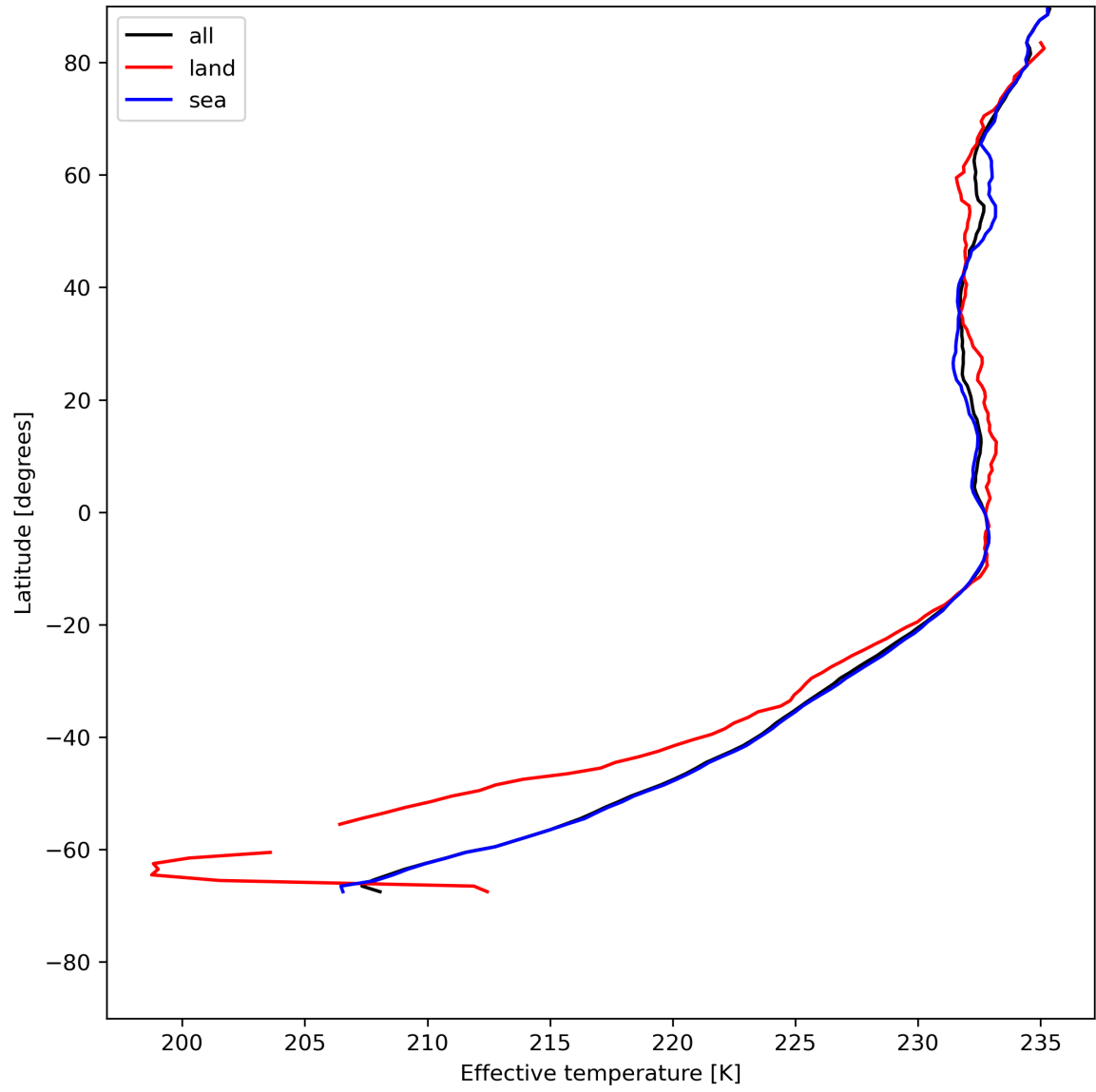
Figure 17: Zonal average of "Effective temperature" for 2024-05-26 to 2024-05-28.
