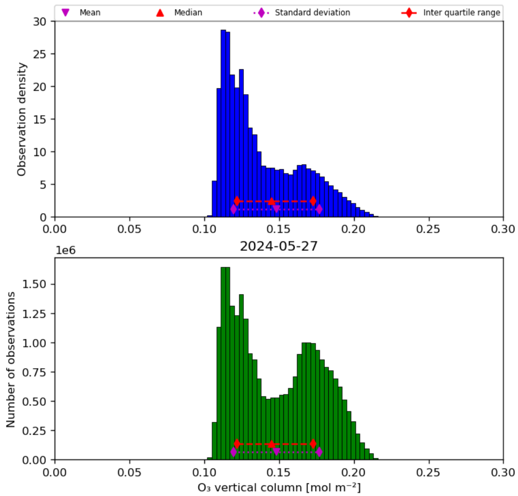
Figure 21: Histogram of “O 3 vertical column” for 2024-05-26 to 2024-05-28
