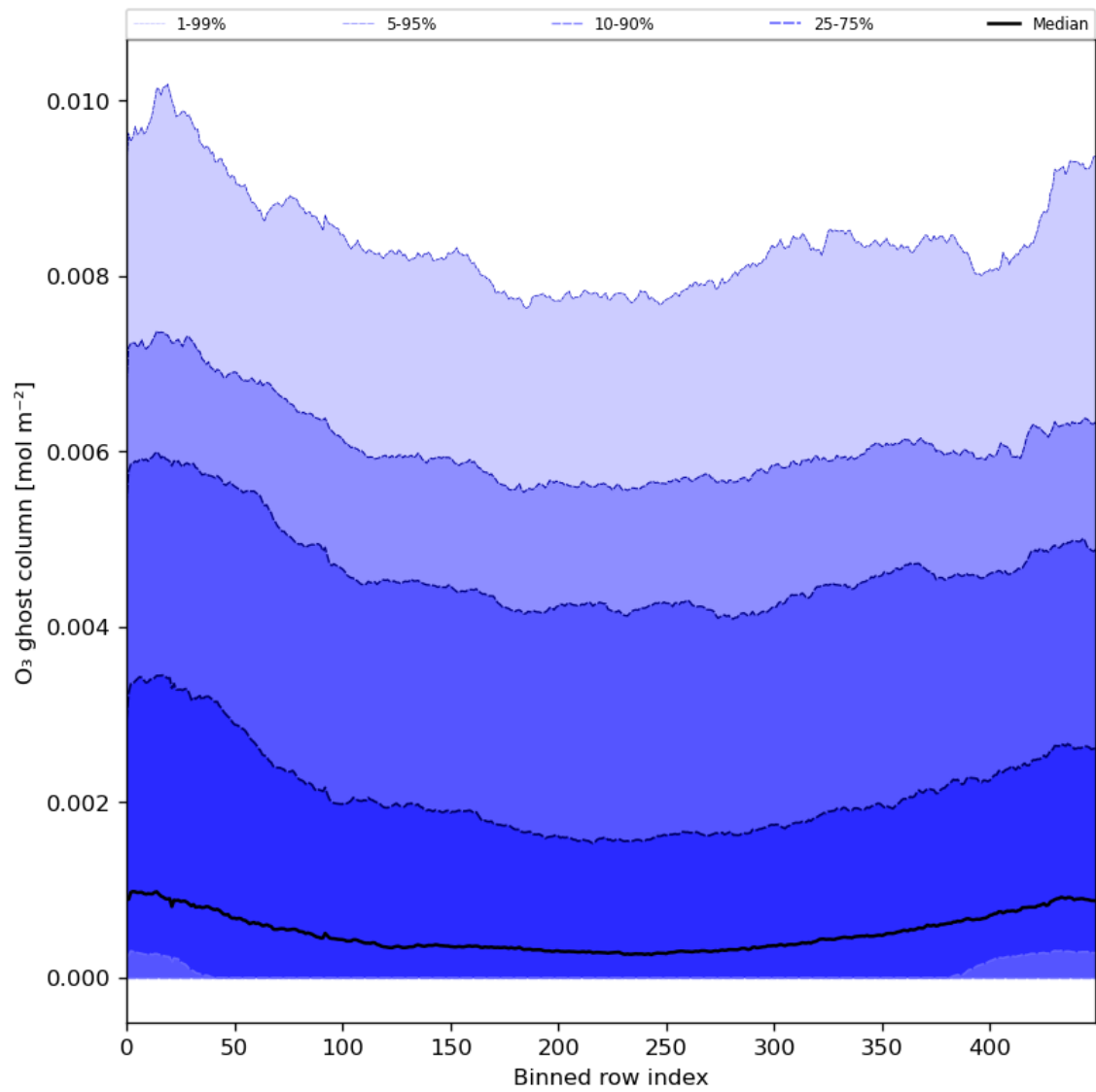
Figure 32: Along track statistics of “O 3 ghost column” for 2024-05-26 to 2024-05-28
