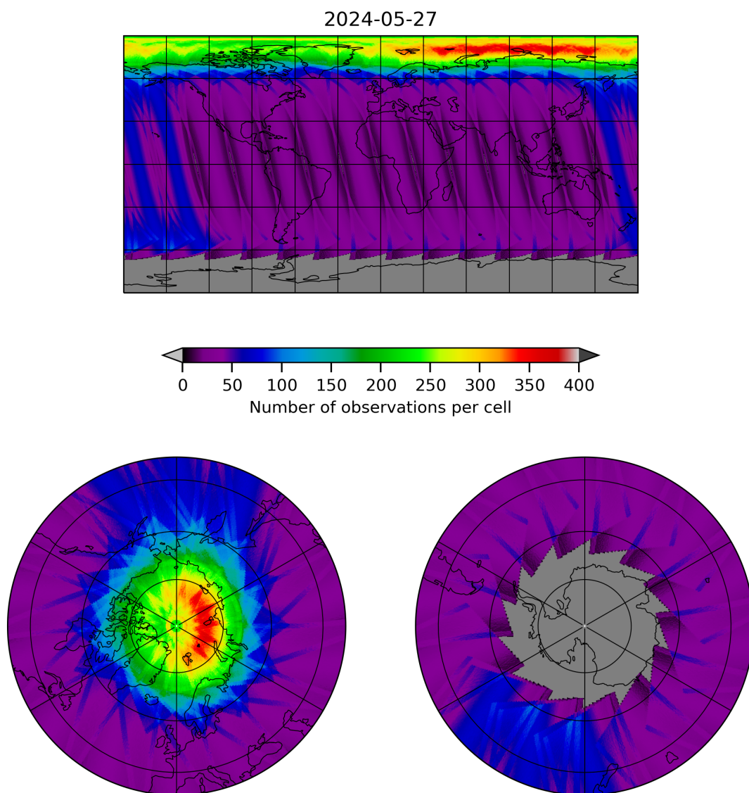
Figure 12: Map of the number of observations for 2024-05-26 to 2024-05-28
