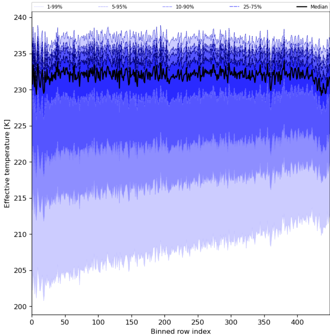
Figure 31: Along track statistics of “Effective temperature” for 2024-05-26 to 2024-05-28
