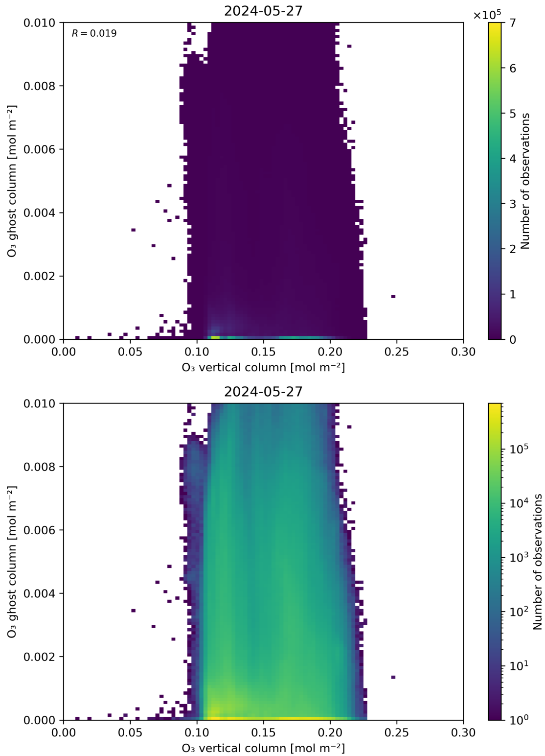
Figure 40: Scatter density plot of “O 3 vertical column” against “O 3 ghost column” for 2024-05-26 to 2024-05-28.
