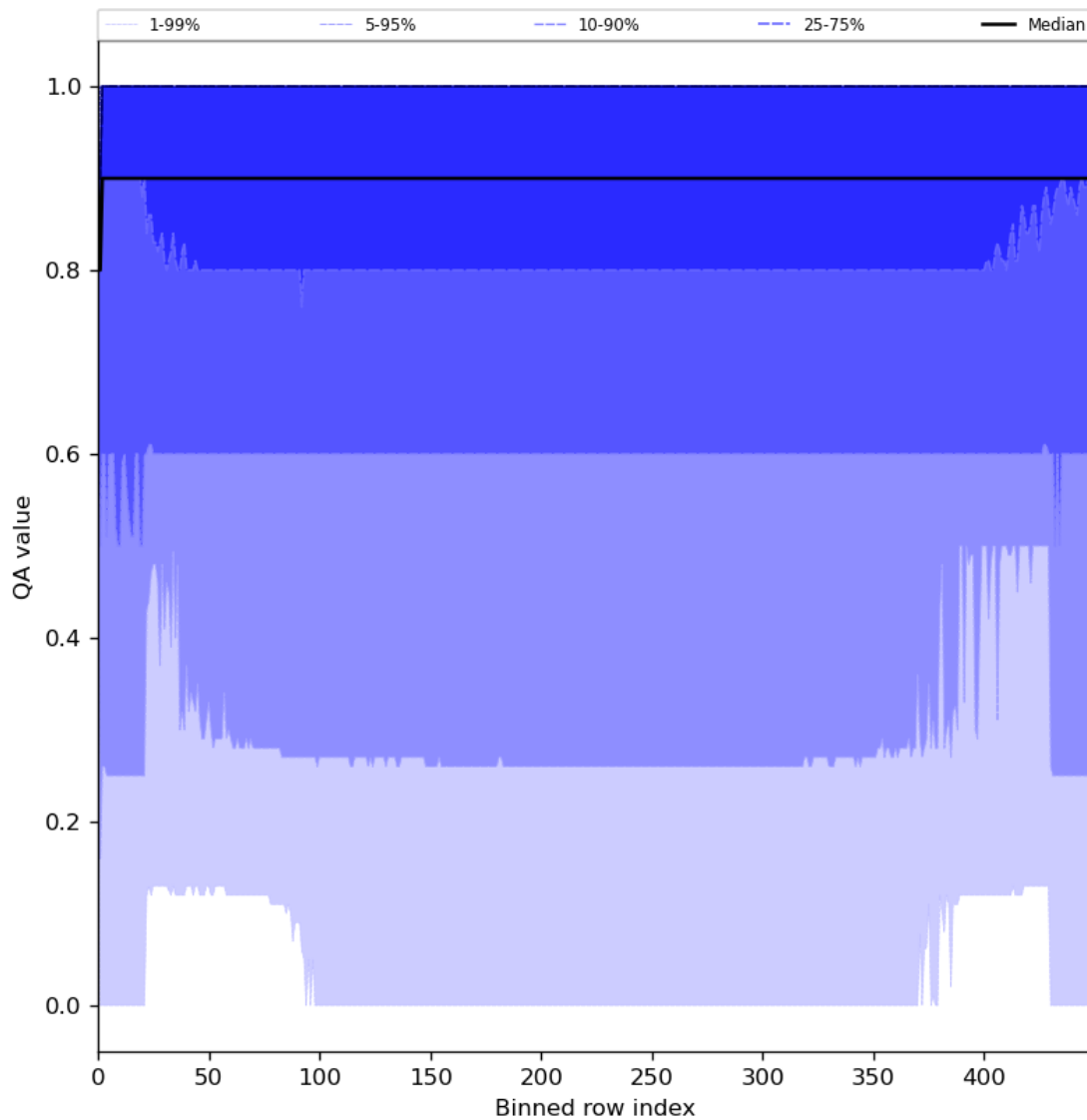
Figure 27: Along track statistics of “QA value” for 2024-05-26 to 2024-05-28
