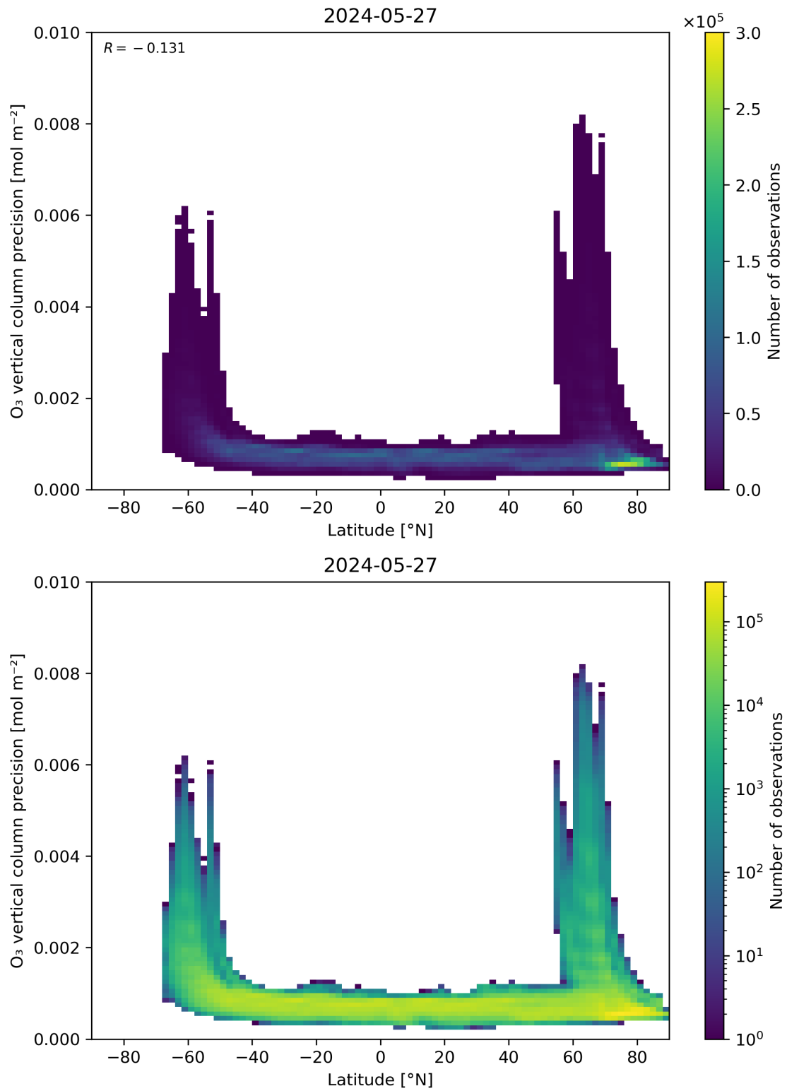
Figure 37: Scatter density plot of “Latitude” against “O 3 vertical column precision” for 2024-05-26 to 2024-05-28.
