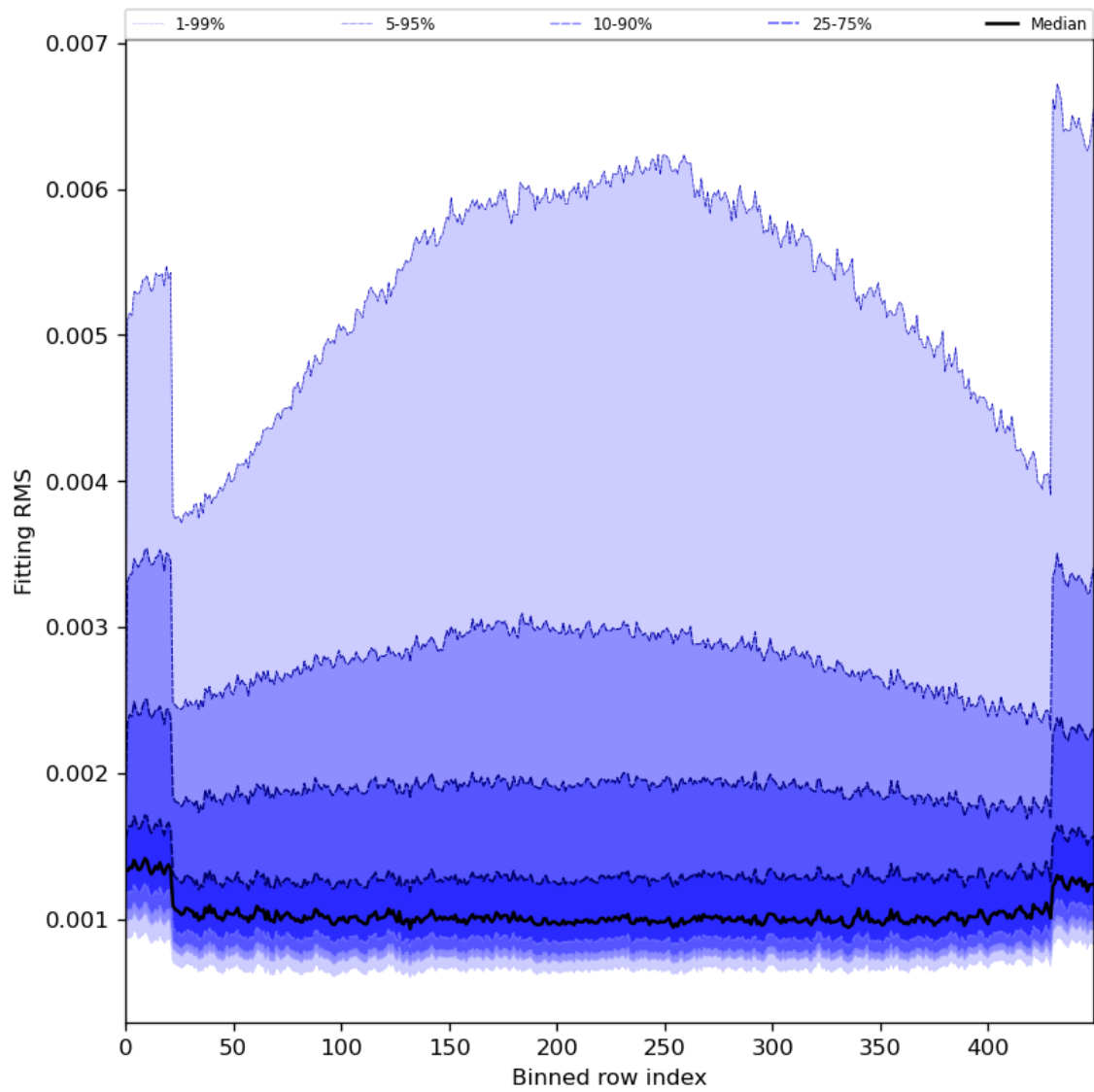
Figure 30: Along track statistics of “Fitting RMS” for 2024-05-26 to 2024-05-28
