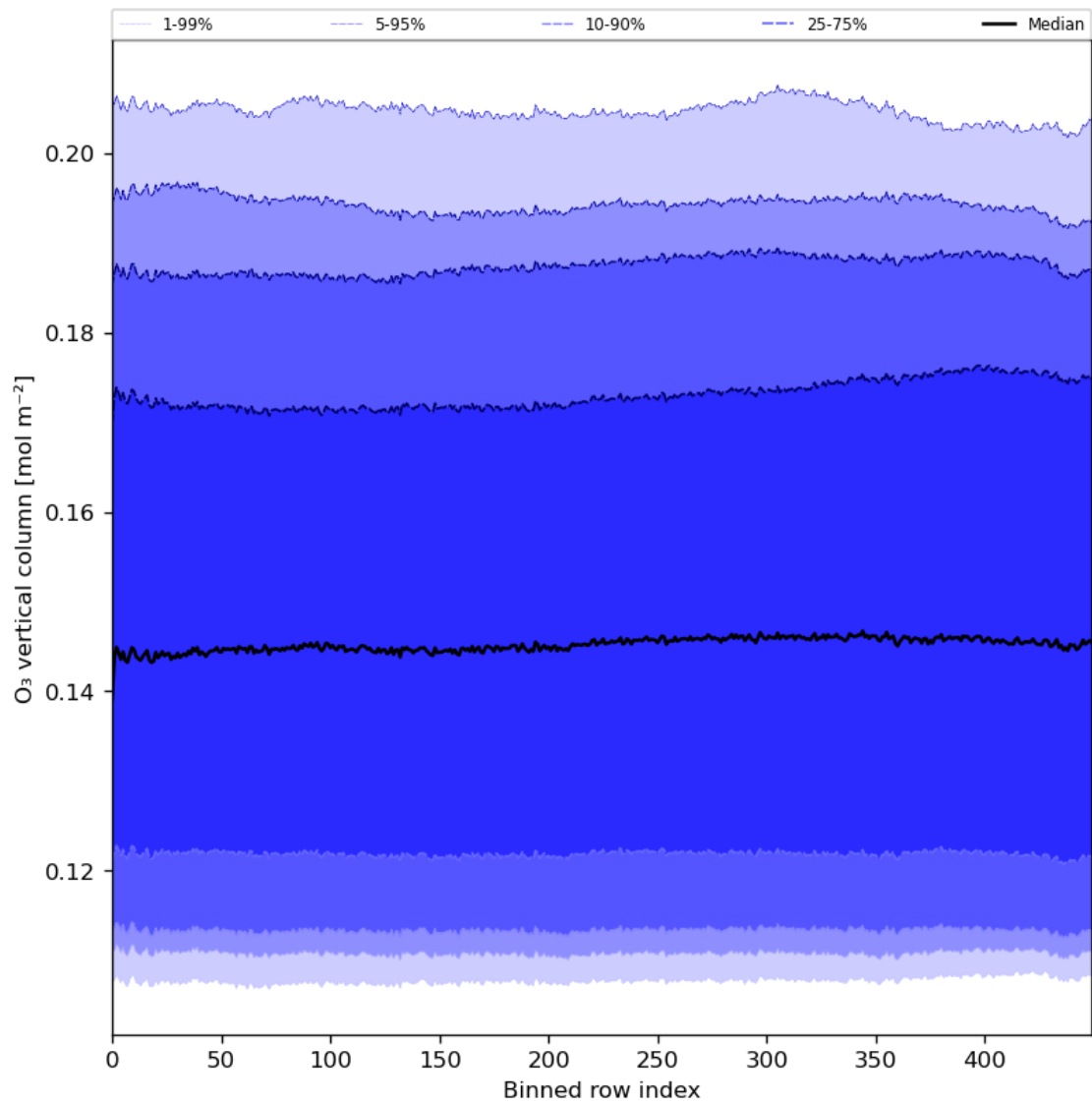
Figure 28: Along track statistics of “O 3 vertical column” for 2024-05-26 to 2024-05-28
