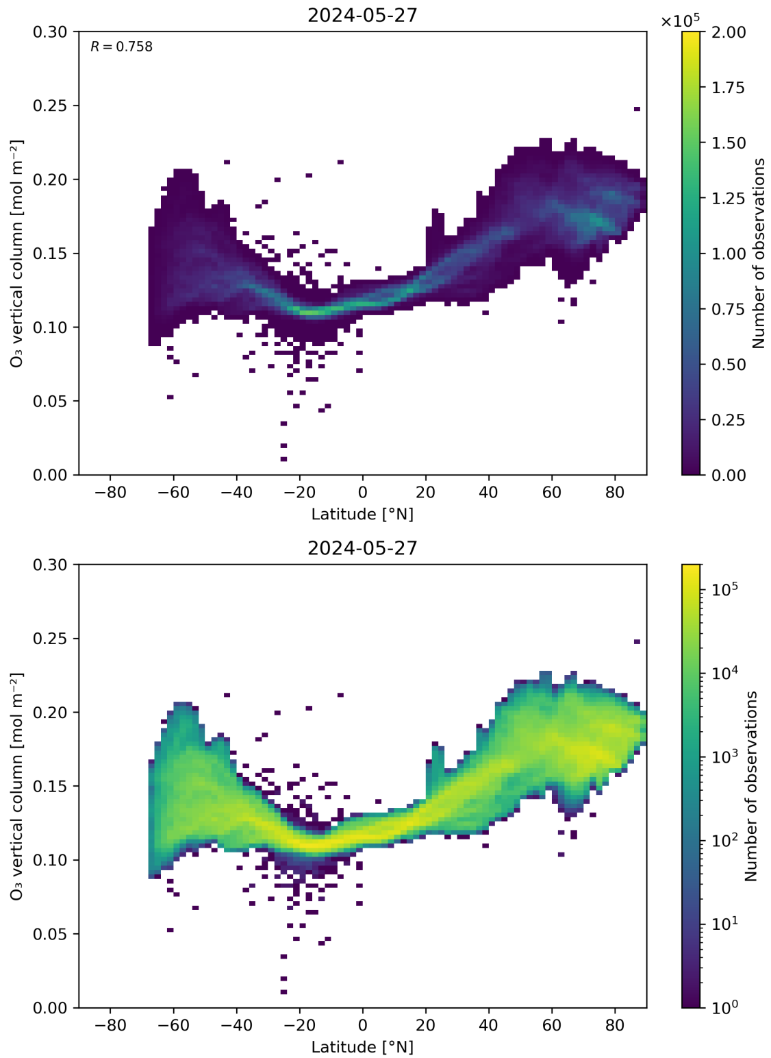
Figure 36: Scatter density plot of “Latitude” against “O 3 vertical column” for 2024-05-26 to 2024-05-28.
