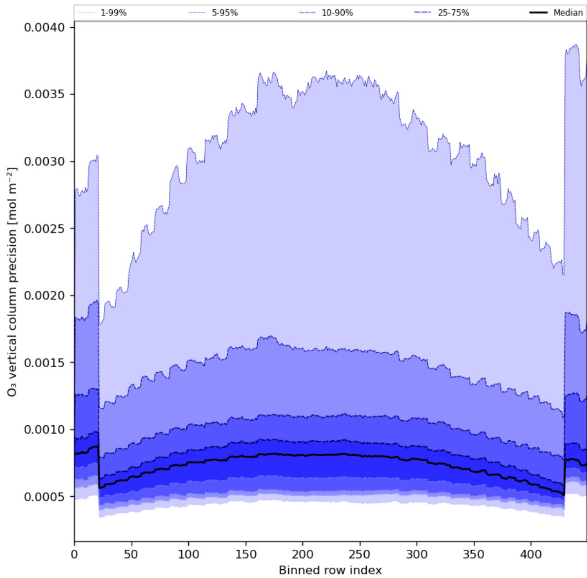
Figure 29: Along track statistics of “O 3 vertical column precision” for 2024-05-26 to 2024-05-28
