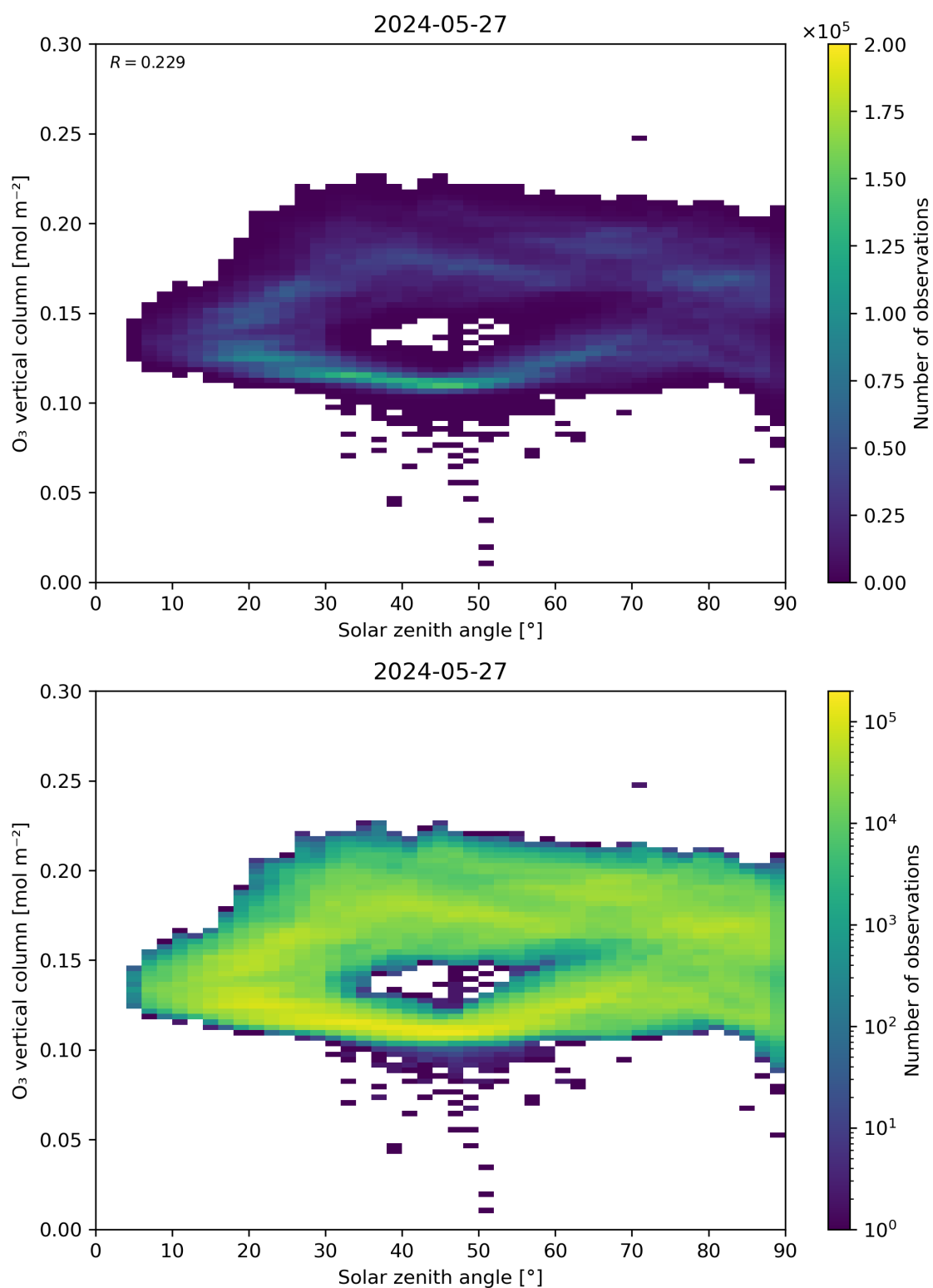
Figure 47: Scatter density plot of “Solar zenith angle” against “O 3 vertical column” for 2024-05-26 to 2024-05-28.
