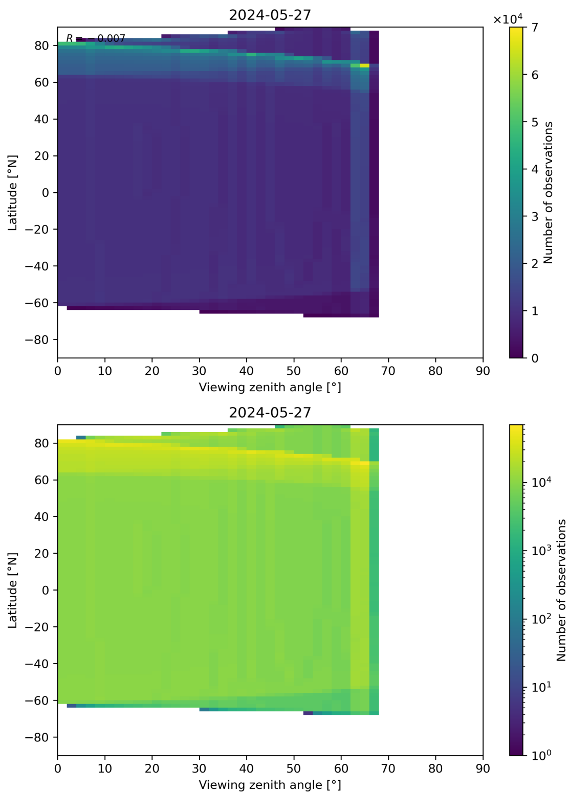
Figure 49: Scatter density plot of “Viewing zenith angle” against “Latitude” for 2024-05-26 to 2024-05-28.
