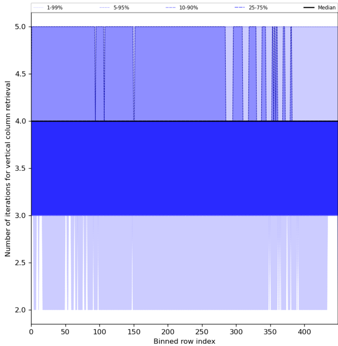
Figure 33: Along track statistics of “Number of iterations for vertical column retrieval” for 2024-05-26 to 2024-05-28
