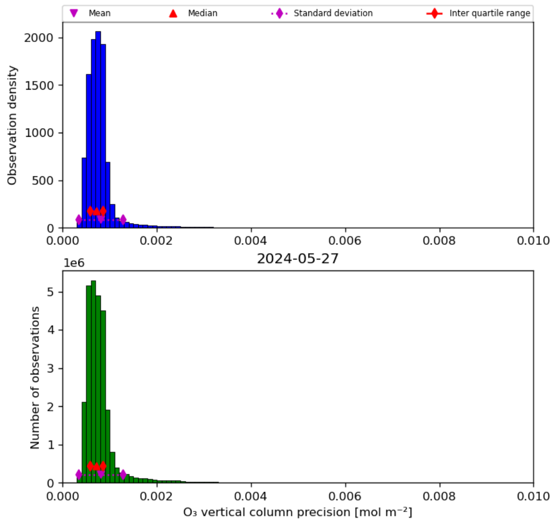
Figure 22: Histogram of “O 3 vertical column precision” for 2024-05-26 to 2024-05-28
