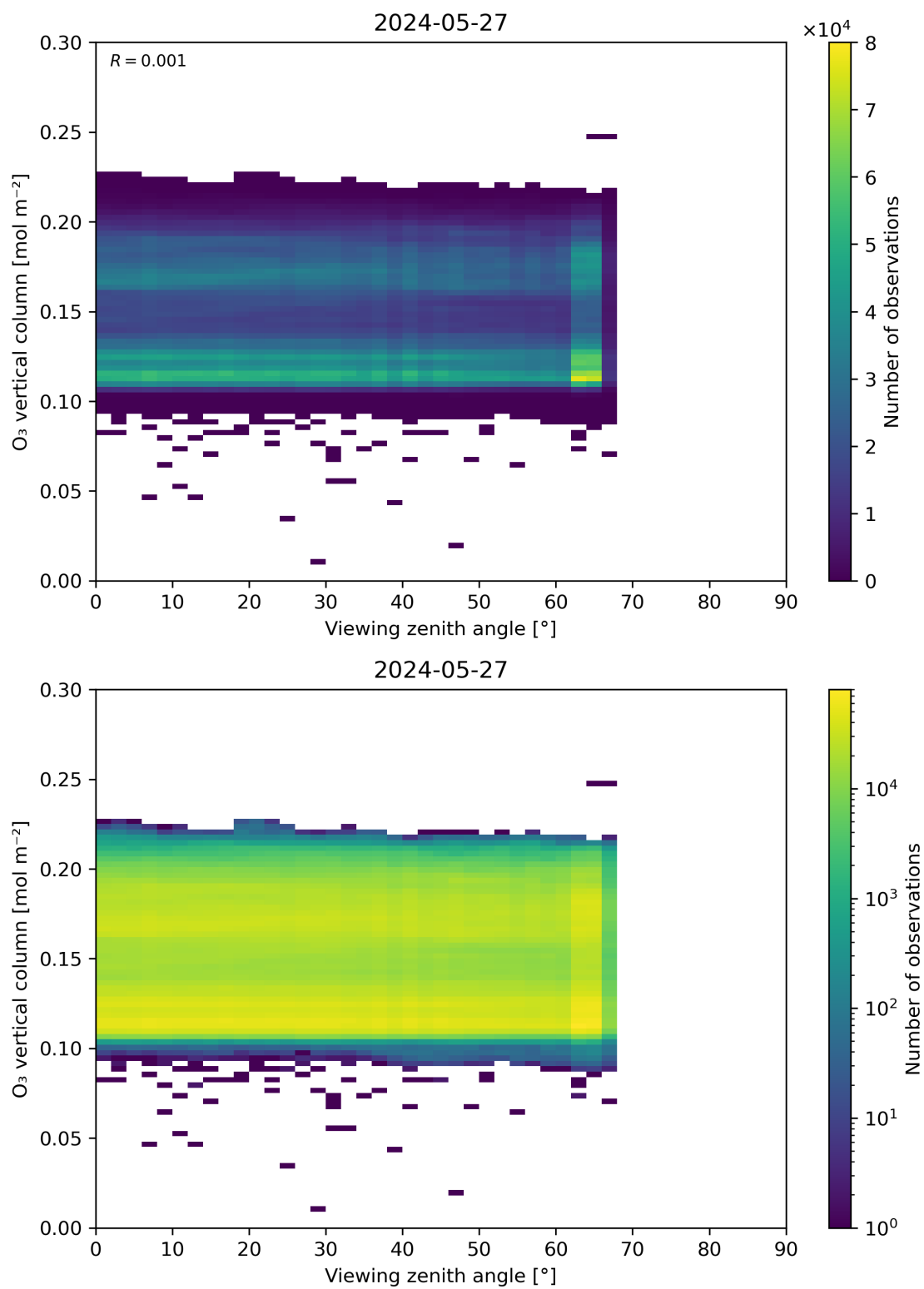
Figure 52: Scatter density plot of “Viewing zenith angle” against “O 3 vertical column” for 2024-05-26 to 2024-05-28.
