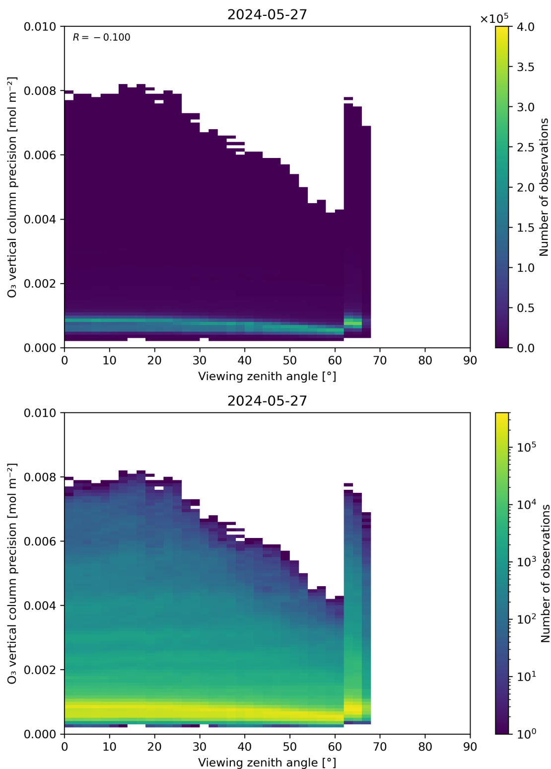
Figure 53: Scatter density plot of “Viewing zenith angle” against “O 3 vertical column precision” for 2024-05-26 to 2024-05-28.
