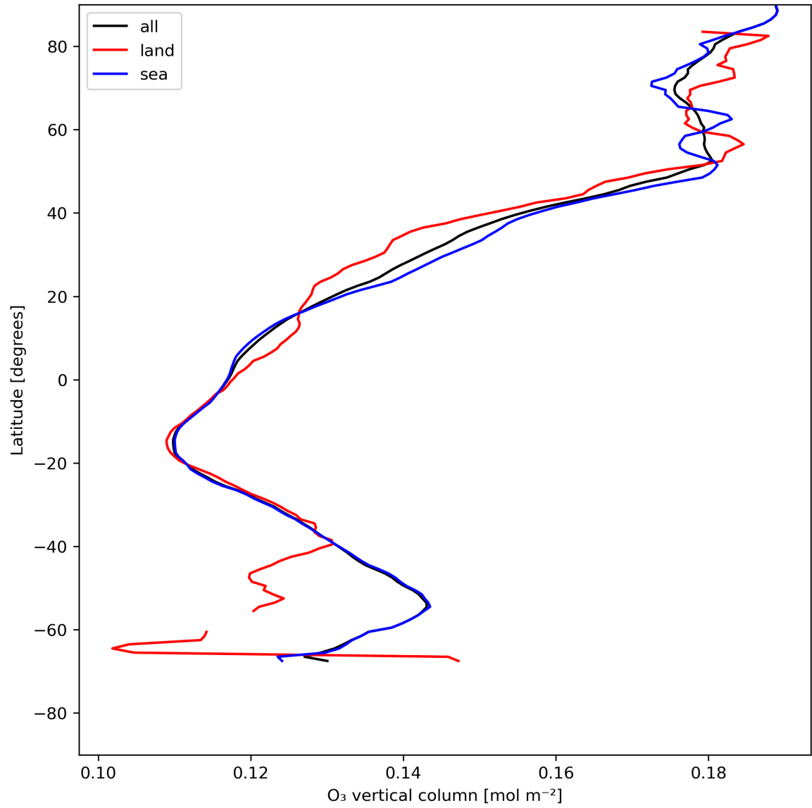
Figure 14: Zonal average of “O 3 vertical column” for 2024-05-26 to 2024-05-28.
