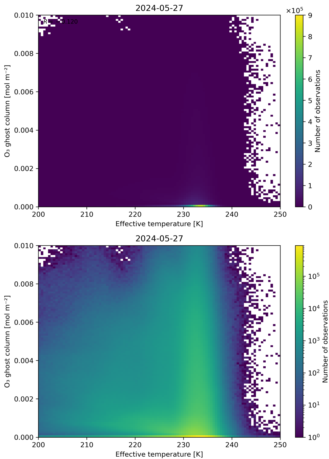
Figure 38: Scatter density plot of “Effective temperature” against “O 3 ghost column” for 2024-05-26 to 2024-05-28.
