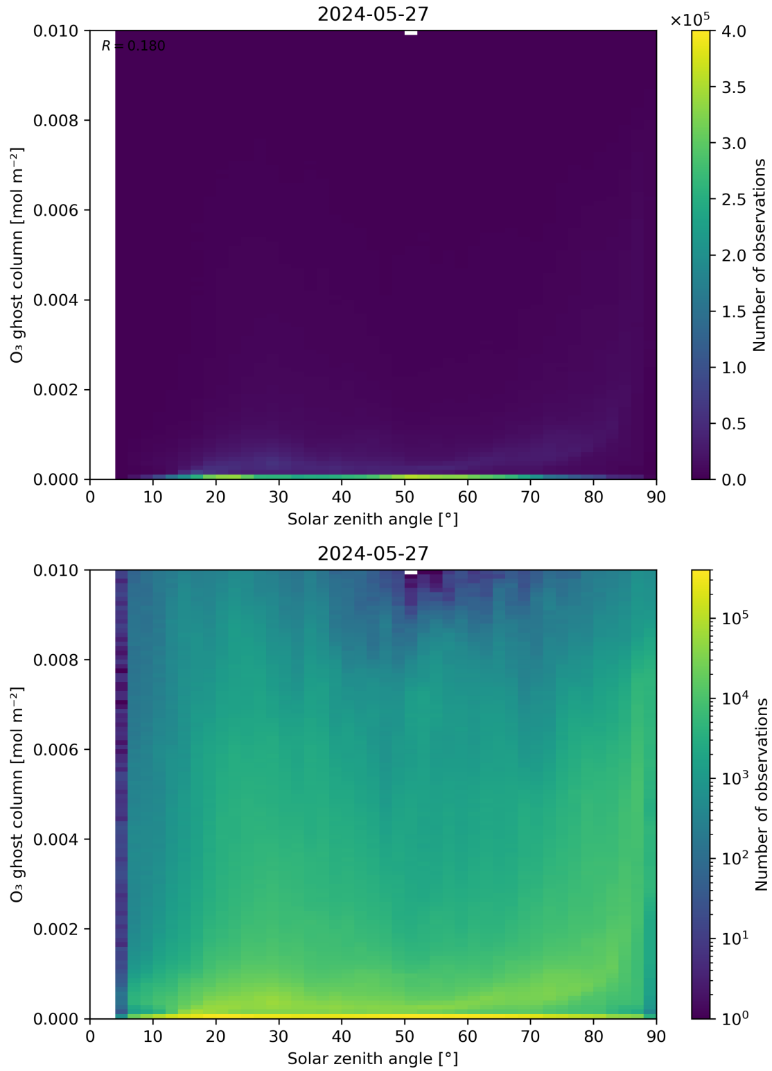
Figure 46: Scatter density plot of “Solar zenith angle” against “O 3 ghost column” for 2024-05-26 to 2024-05-28.
