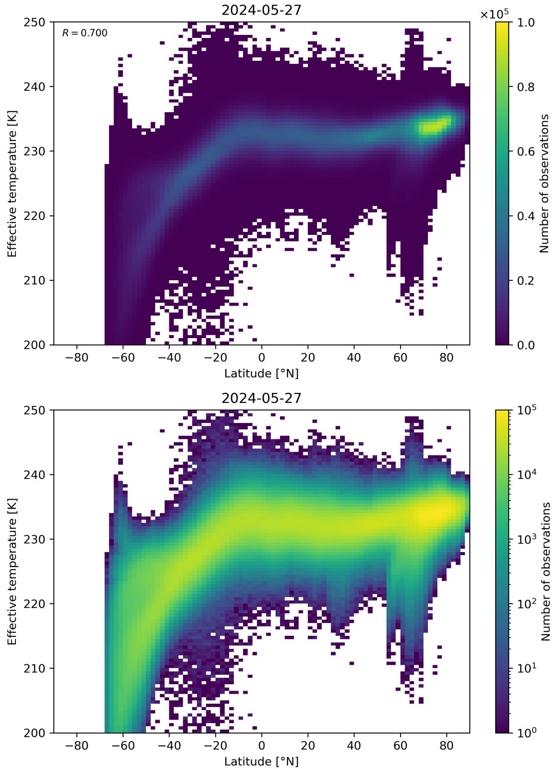
Figure 34: Scatter density plot of “Latitude” against “Effective temperature” for 2024-05-26 to 2024-05-28.
