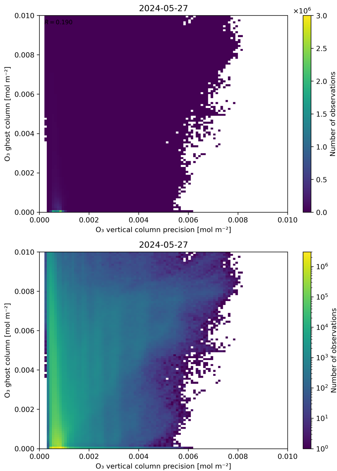
Figure 43: Scatter density plot of “ \text{O}_3 vertical column precision” against “ \text{O}_3 ghost column” for 2024-05-26 to 2024-05-28.
