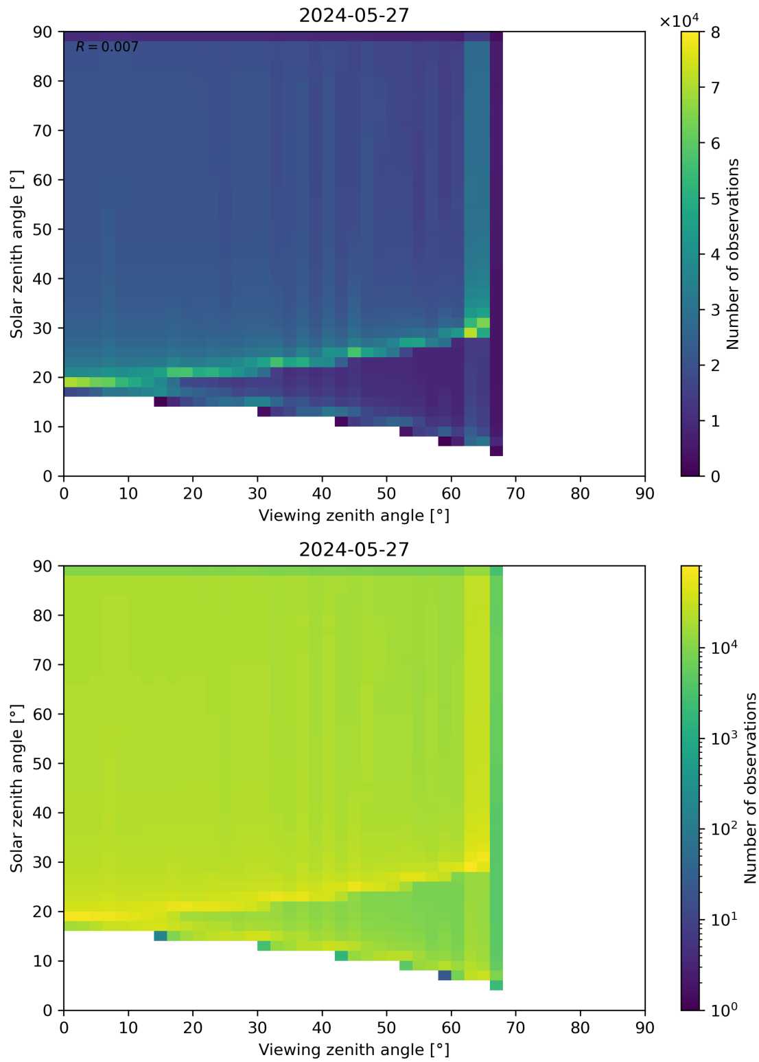
Figure 54: Scatter density plot of “Viewing zenith angle” against “Solar zenith angle” for 2024-05-26 to 2024-05-28.
