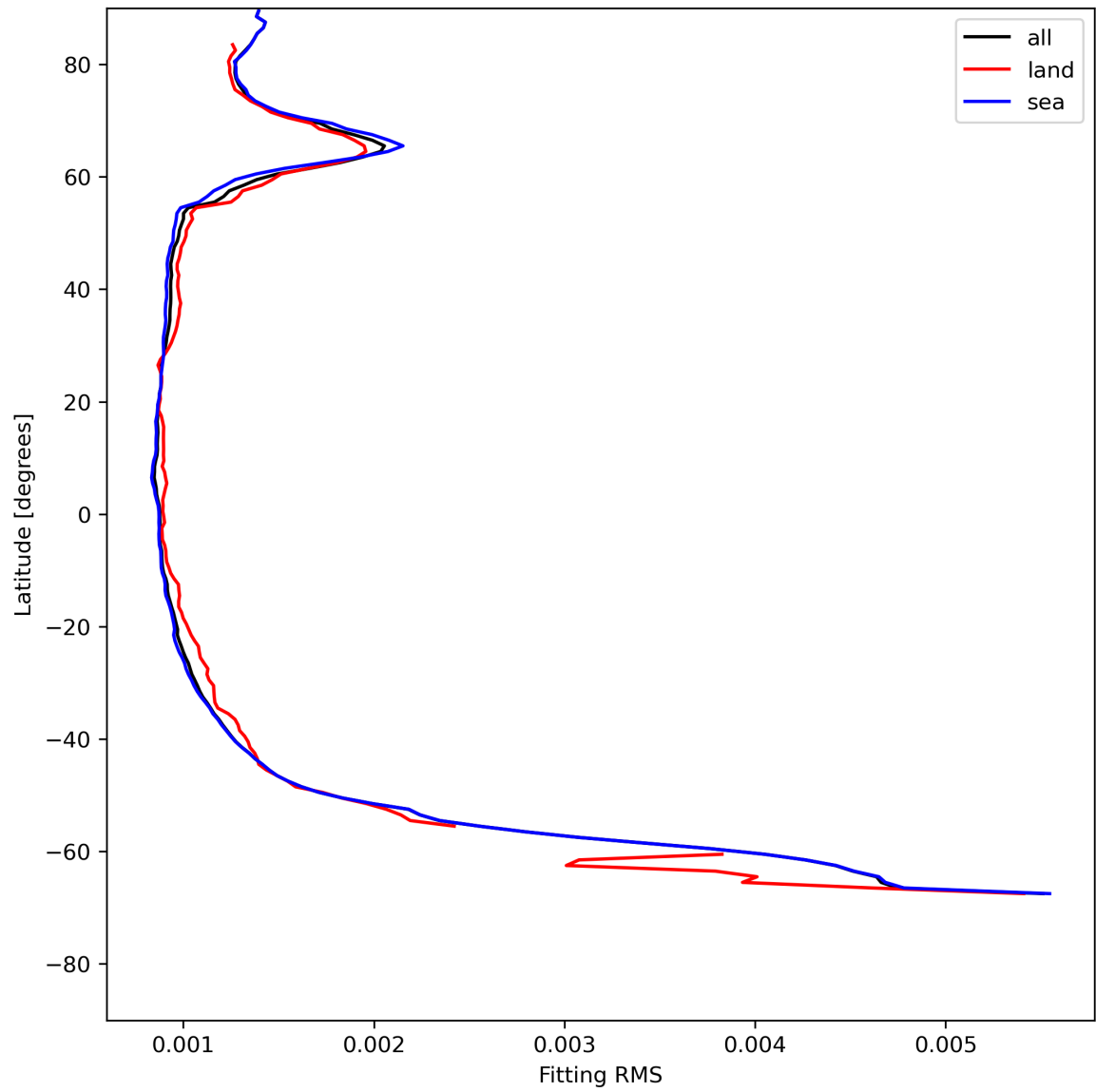
Figure 16: Zonal average of “Fitting RMS” for 2024-05-26 to 2024-05-28.
