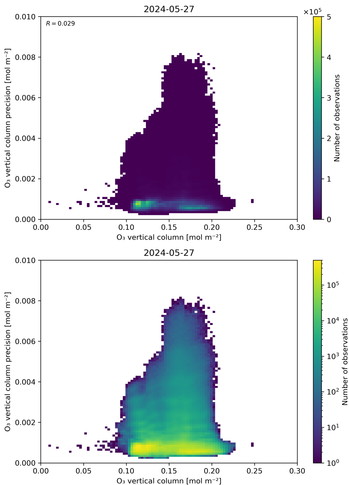
Figure 41: Scatter density plot of “O 3 vertical column” against “O 3 vertical column precision” for 2024-05-26 to 2024-05-28.
