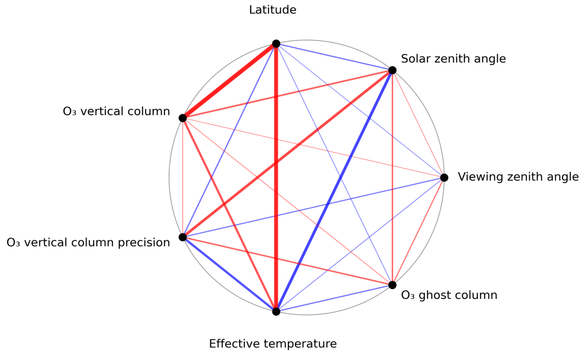
Figure 1: Map of correlation graph for 2024-05-26 to 2024-05-28.
