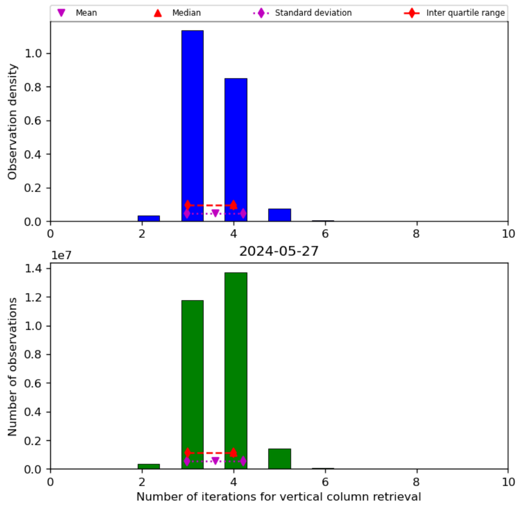
Figure 26: Histogram of “Number of iterations for vertical column retrieval” for 2024-05-26 to 2024-05-28
