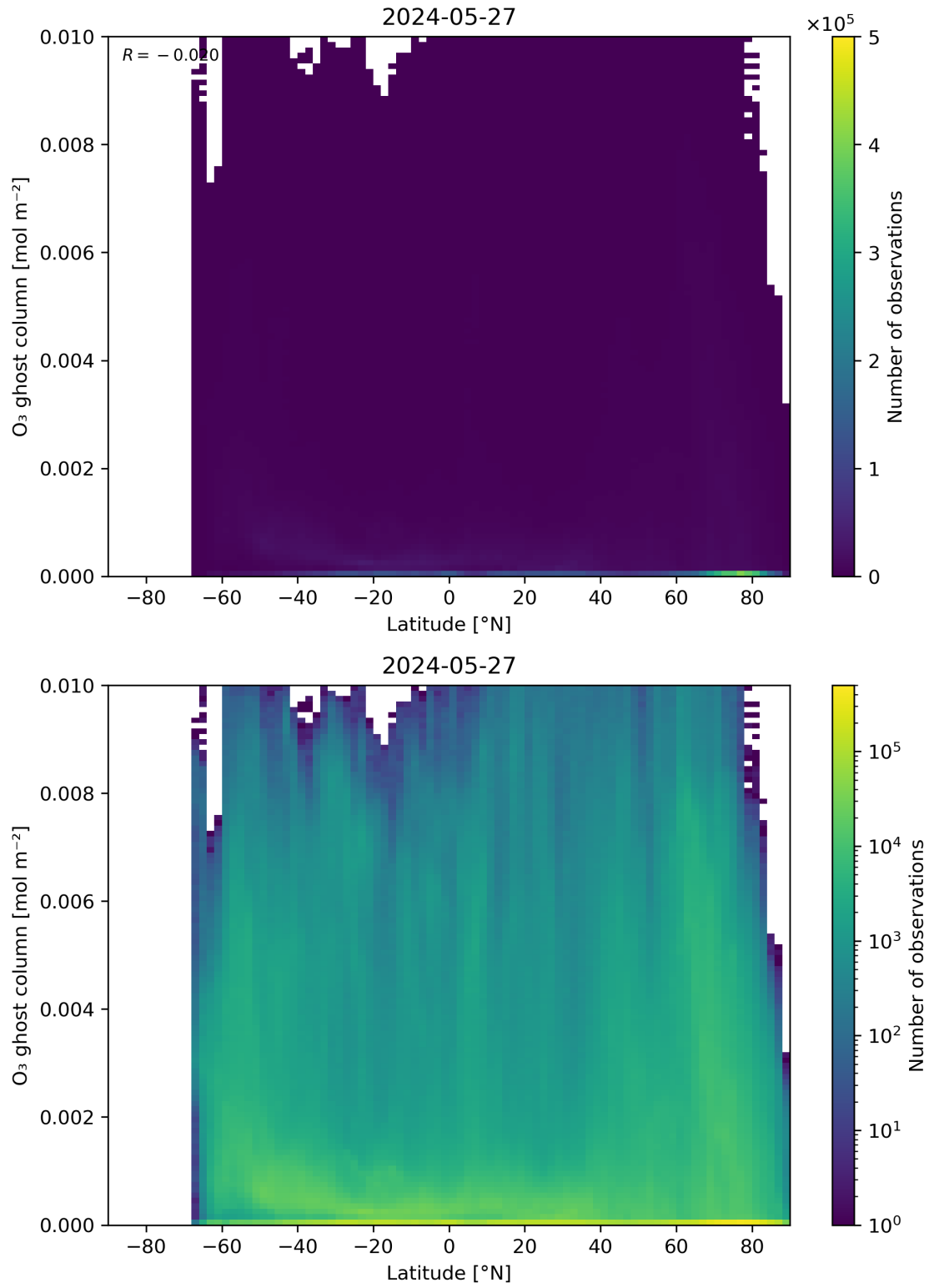
Figure 35: Scatter density plot of “Latitude” against “O 3 ghost column” for 2024-05-26 to 2024-05-28.
