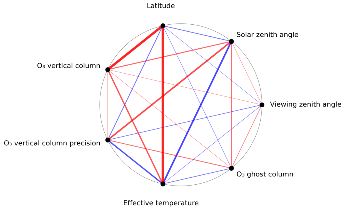
Figure 1: Map of correlation graph for 2024-05-28 to 2024-05-30.
