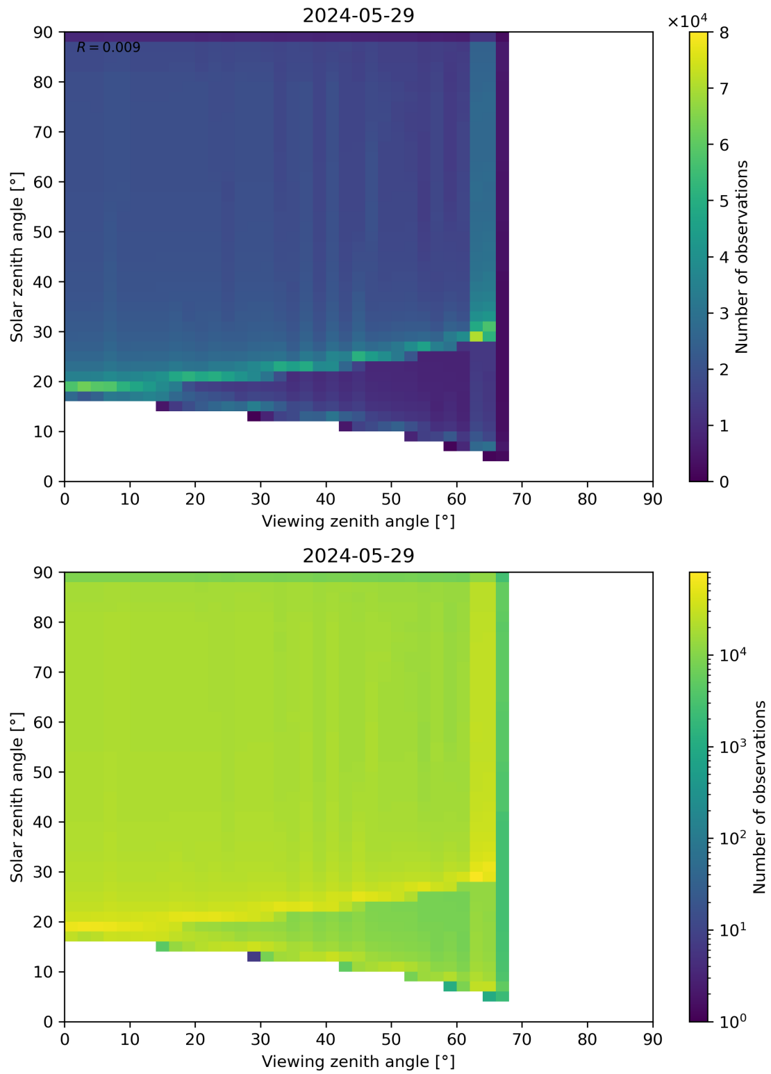
Figure 54: Scatter density plot of “Viewing zenith angle” against “Solar zenith angle” for 2024-05-28 to 2024-05-30.
