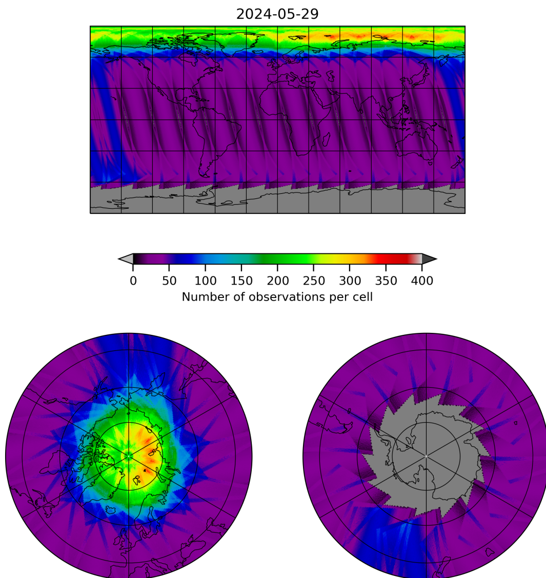
Figure 12: Map of the number of observations for 2024-05-28 to 2024-05-30
