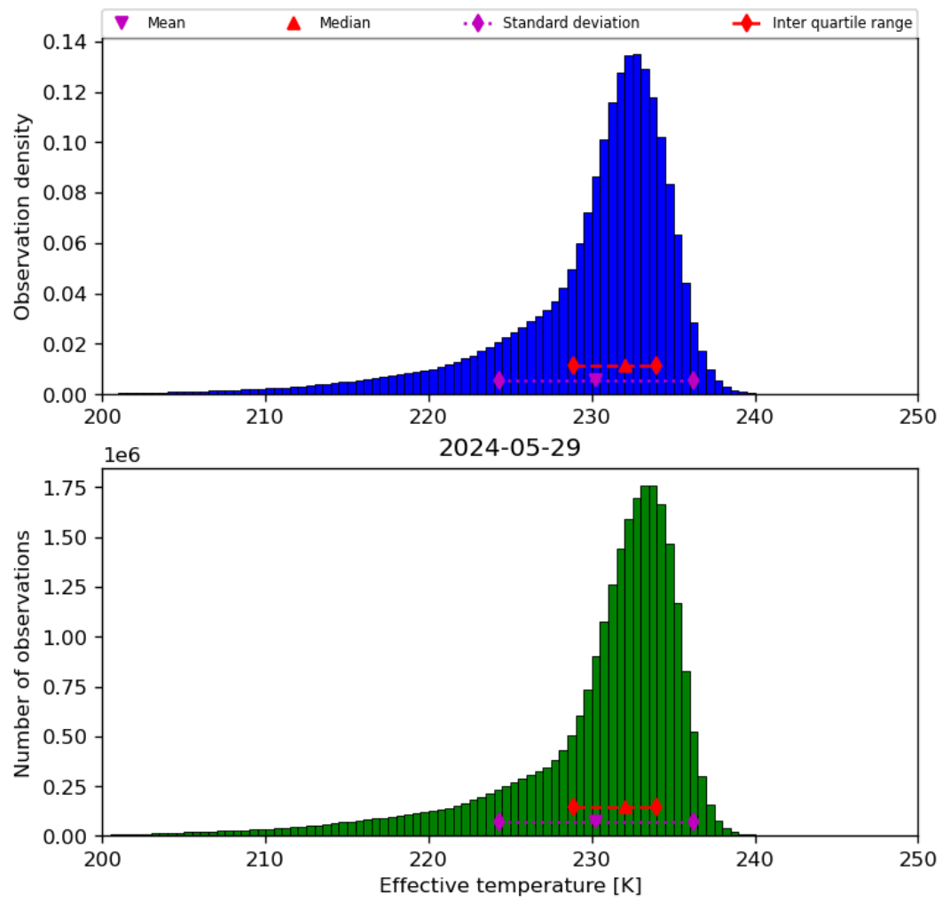
Figure 24: Histogram of “Effective temperature” for 2024-05-28 to 2024-05-30
