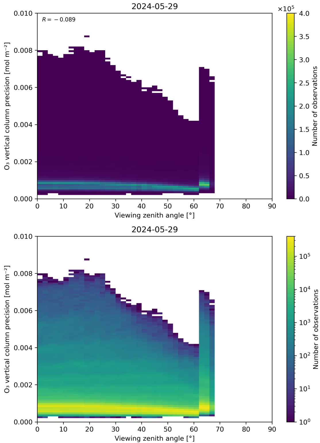
Figure 53: Scatter density plot of “Viewing zenith angle” against “O 3 vertical column precision” for 2024-05-28 to 2024-05-30.
