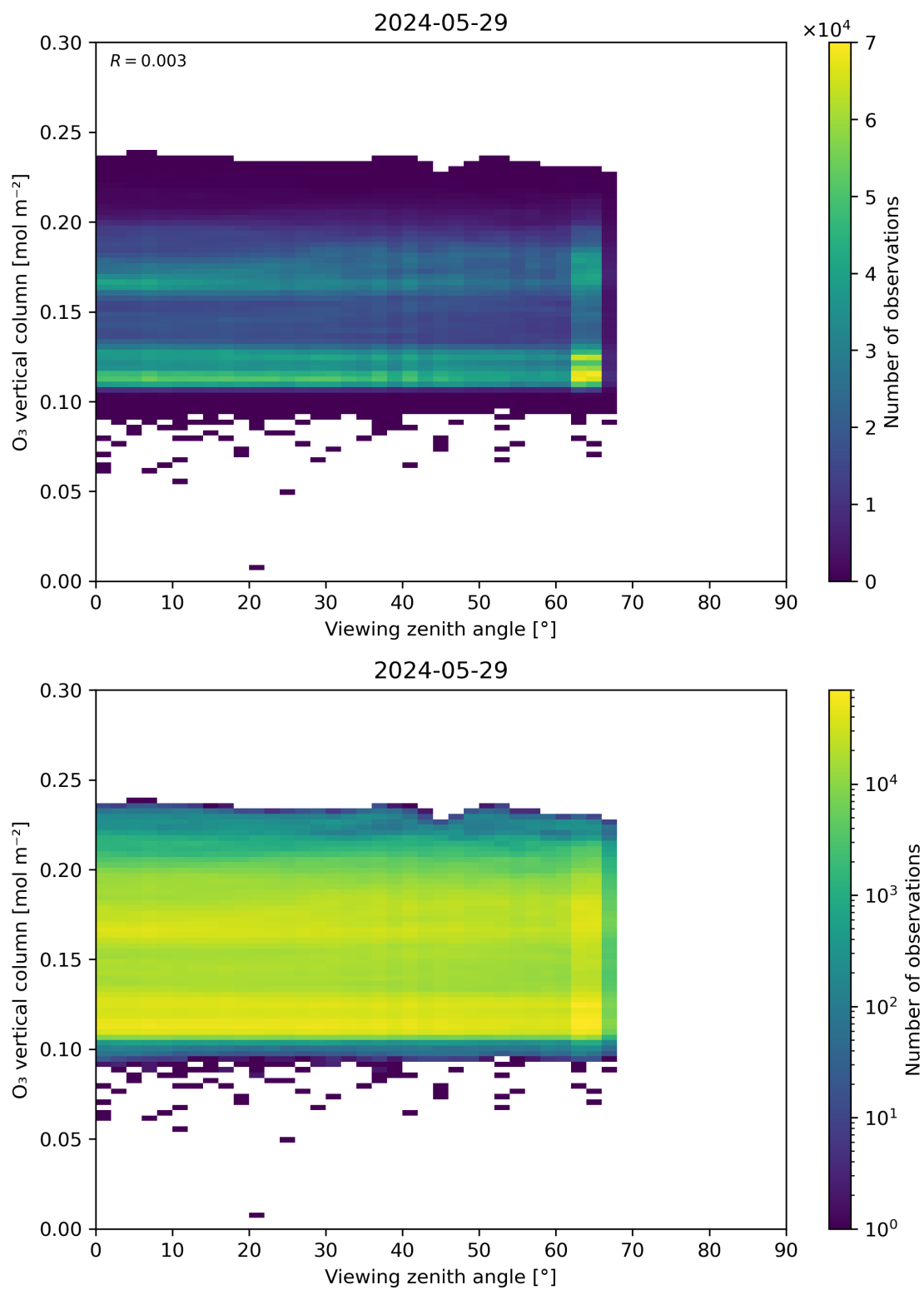
Figure 52: Scatter density plot of “Viewing zenith angle” against “O 3 vertical column” for 2024-05-28 to 2024-05-30.
