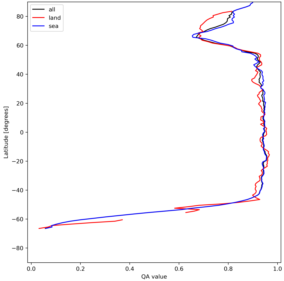
Figure 13: Zonal average of “QA value” for 2024-05-28 to 2024-05-30.
