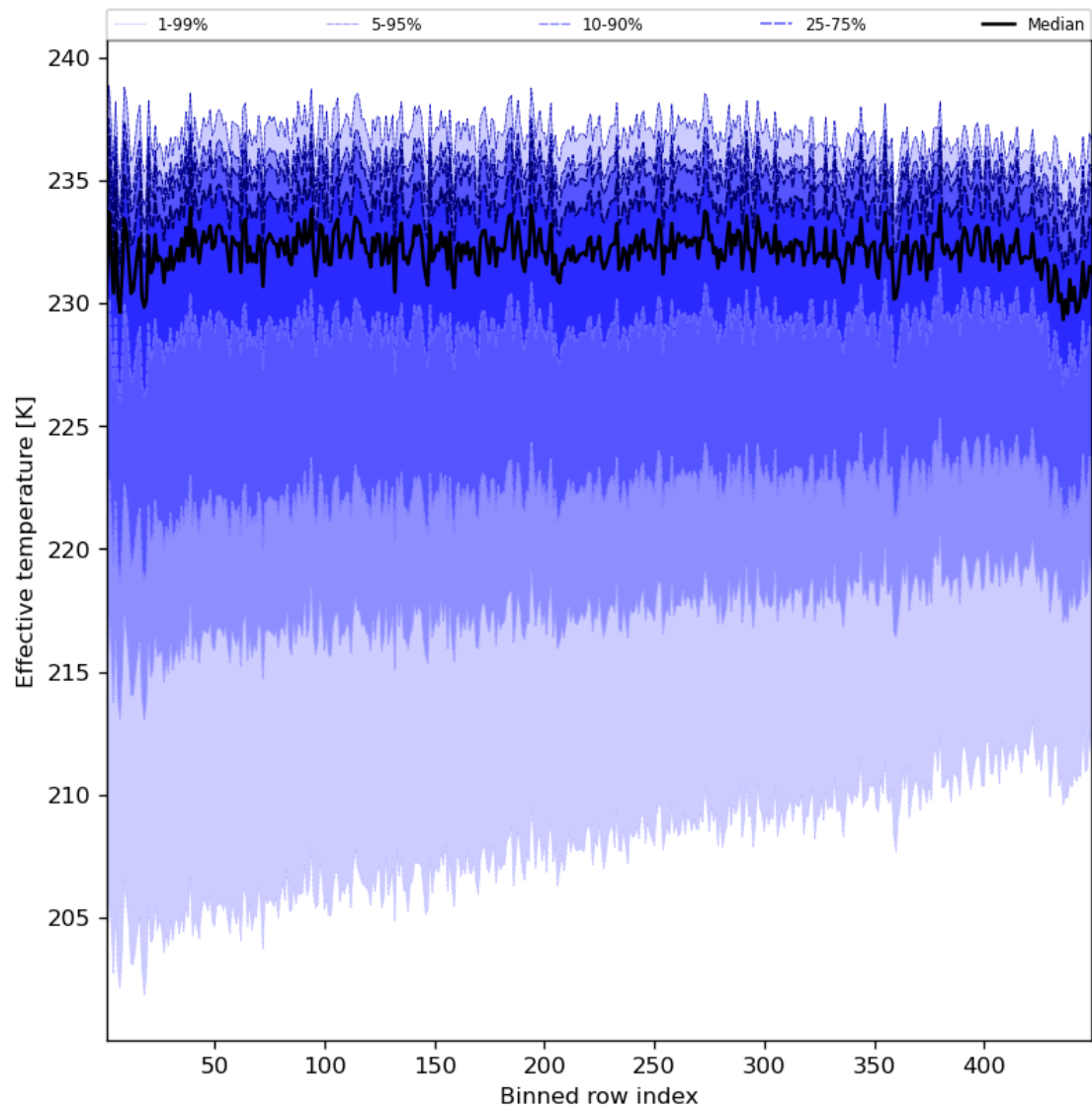
Figure 31: Along track statistics of “Effective temperature” for 2024-05-28 to 2024-05-30
