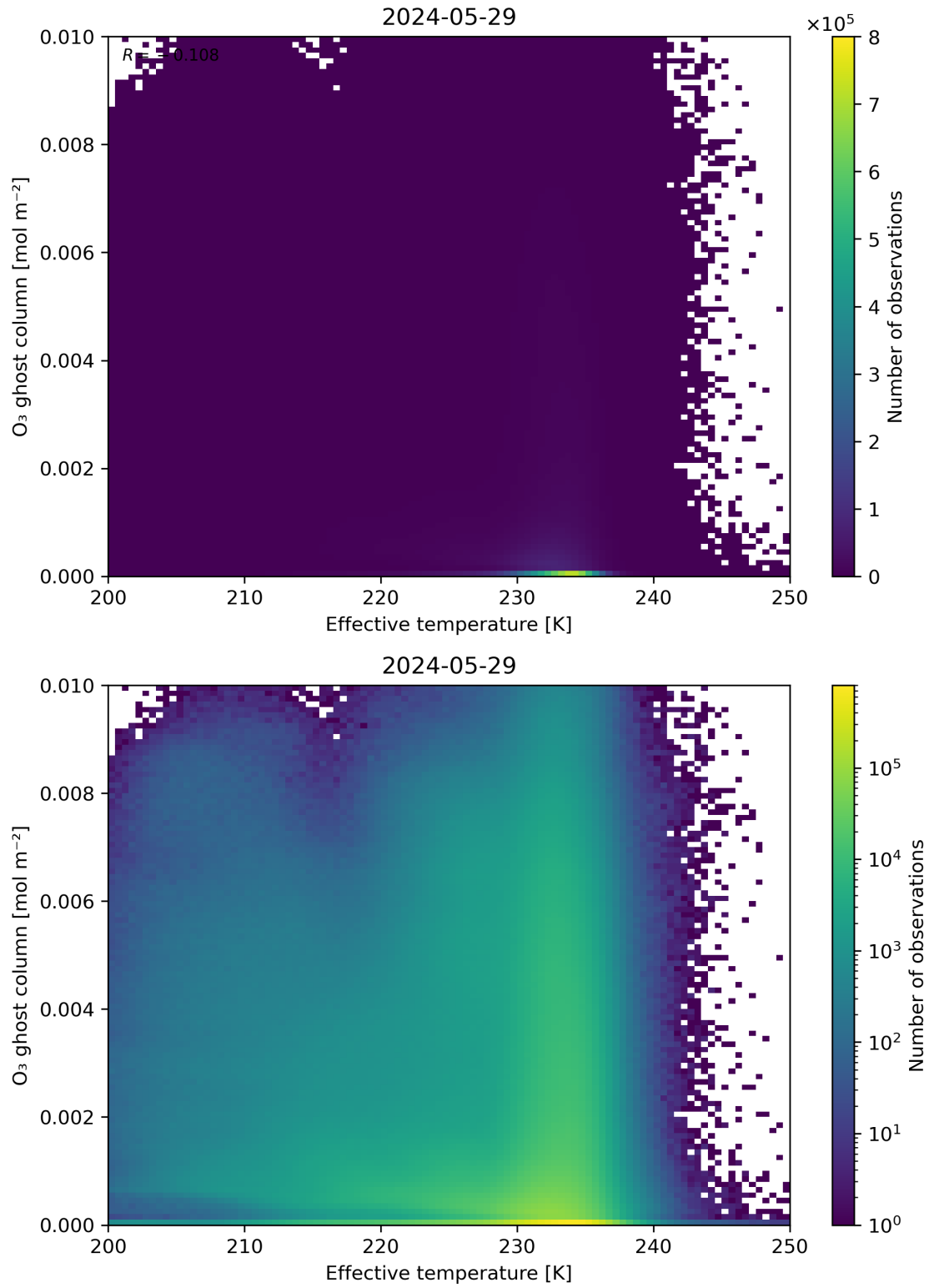
Figure 38: Scatter density plot of “Effective temperature” against “O 3 ghost column” for 2024-05-28 to 2024-05-30.
