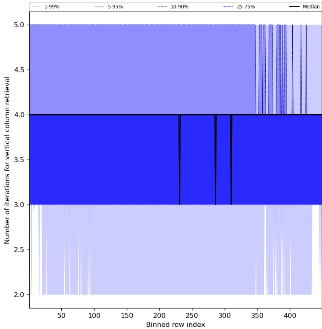
Figure 33: Along track statistics of “Number of iterations for vertical column retrieval” for 2024-05-28 to 2024-05-30
