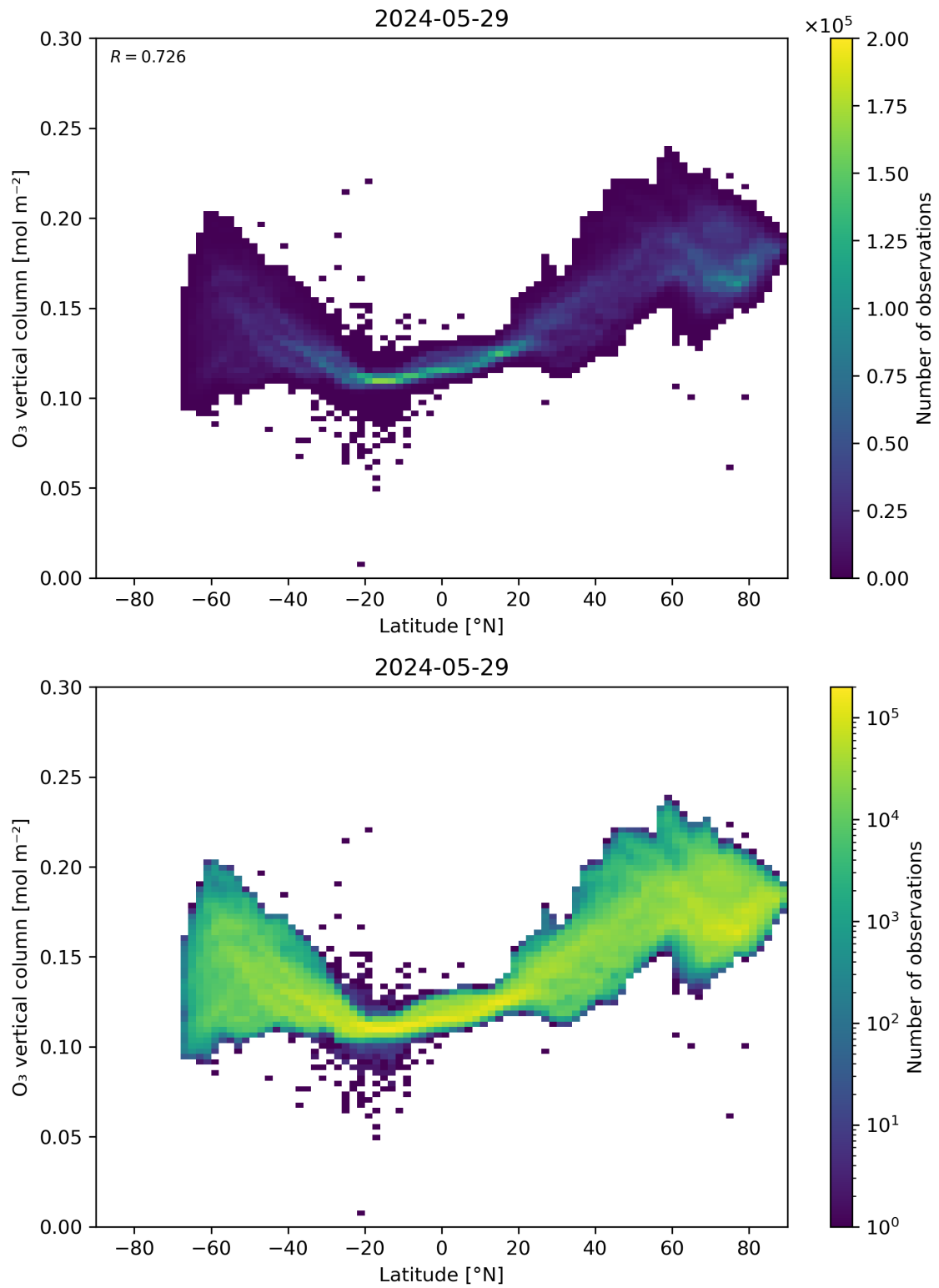
Figure 36: Scatter density plot of “Latitude” against “O 3 vertical column” for 2024-05-28 to 2024-05-30.
