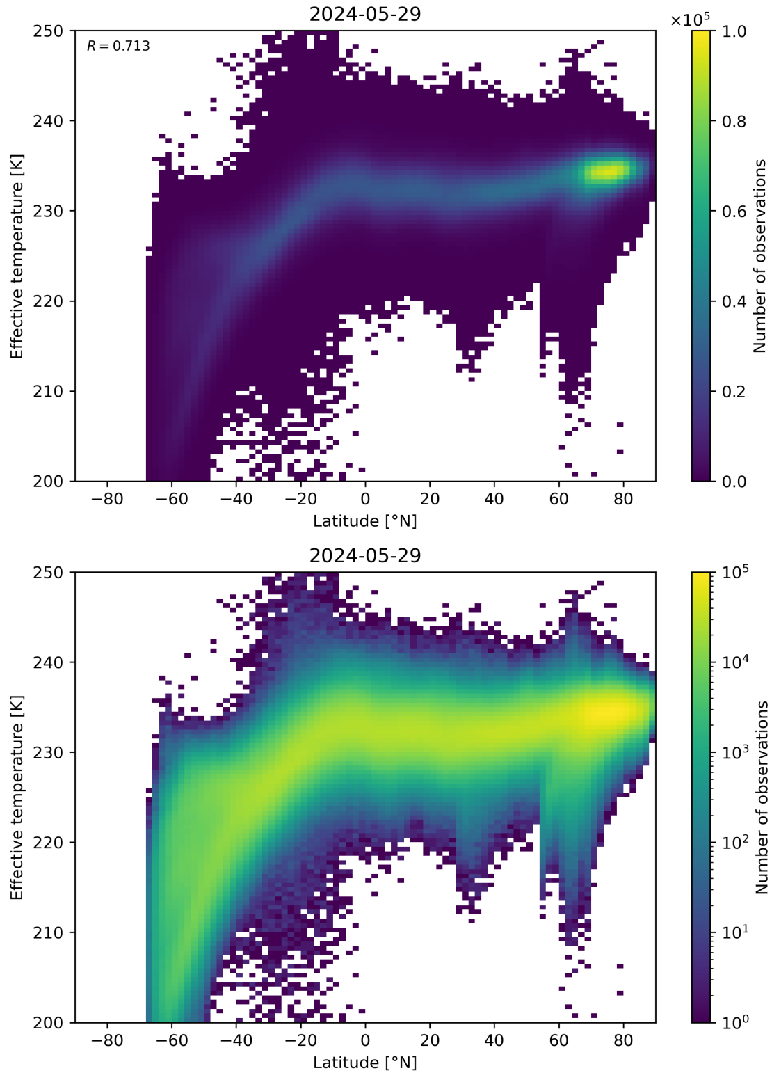
Figure 34: Scatter density plot of “Latitude” against “Effective temperature” for 2024-05-28 to 2024-05-30.
