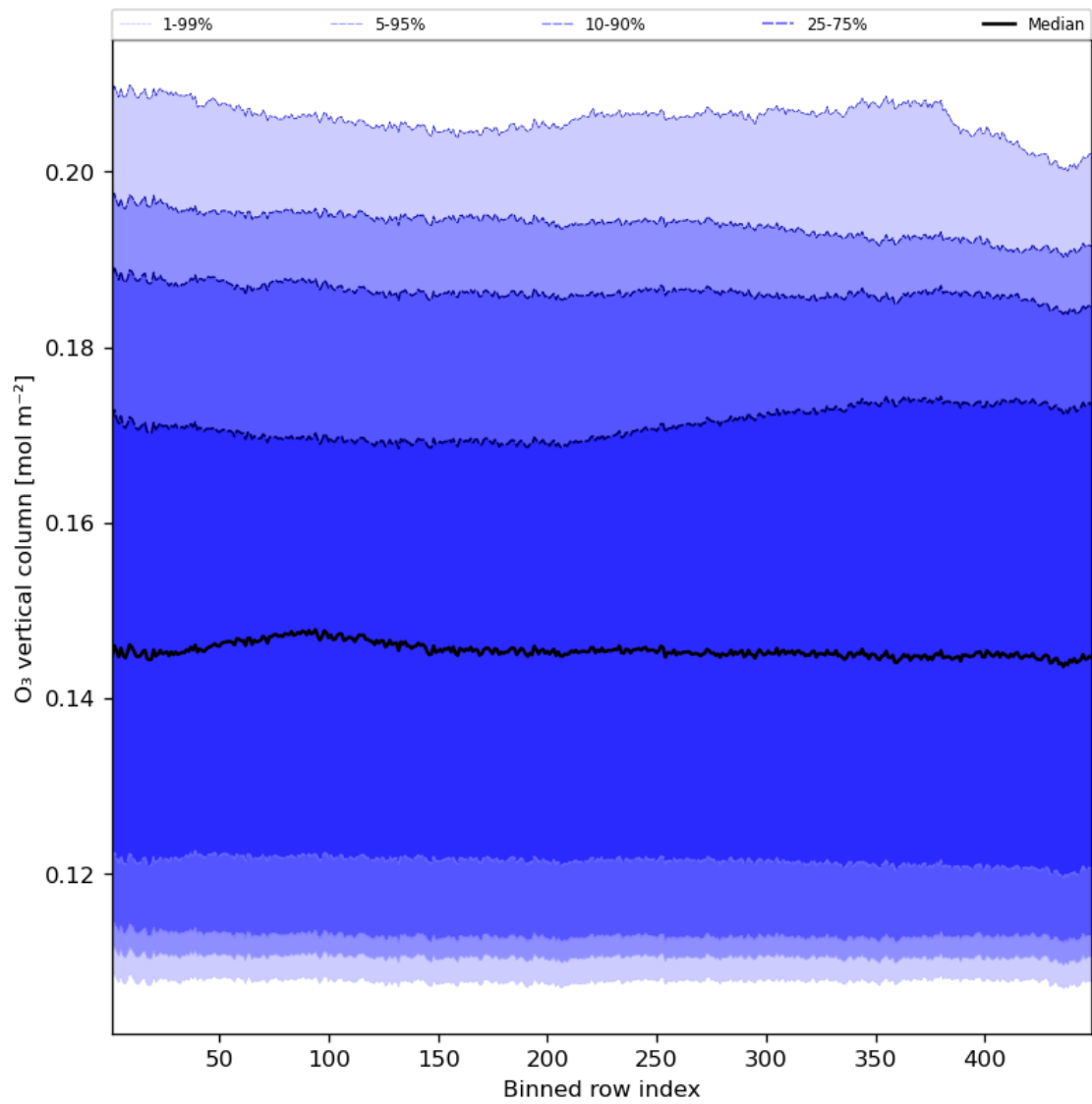
Figure 28: Along track statistics of “O 3 vertical column” for 2024-05-28 to 2024-05-30
