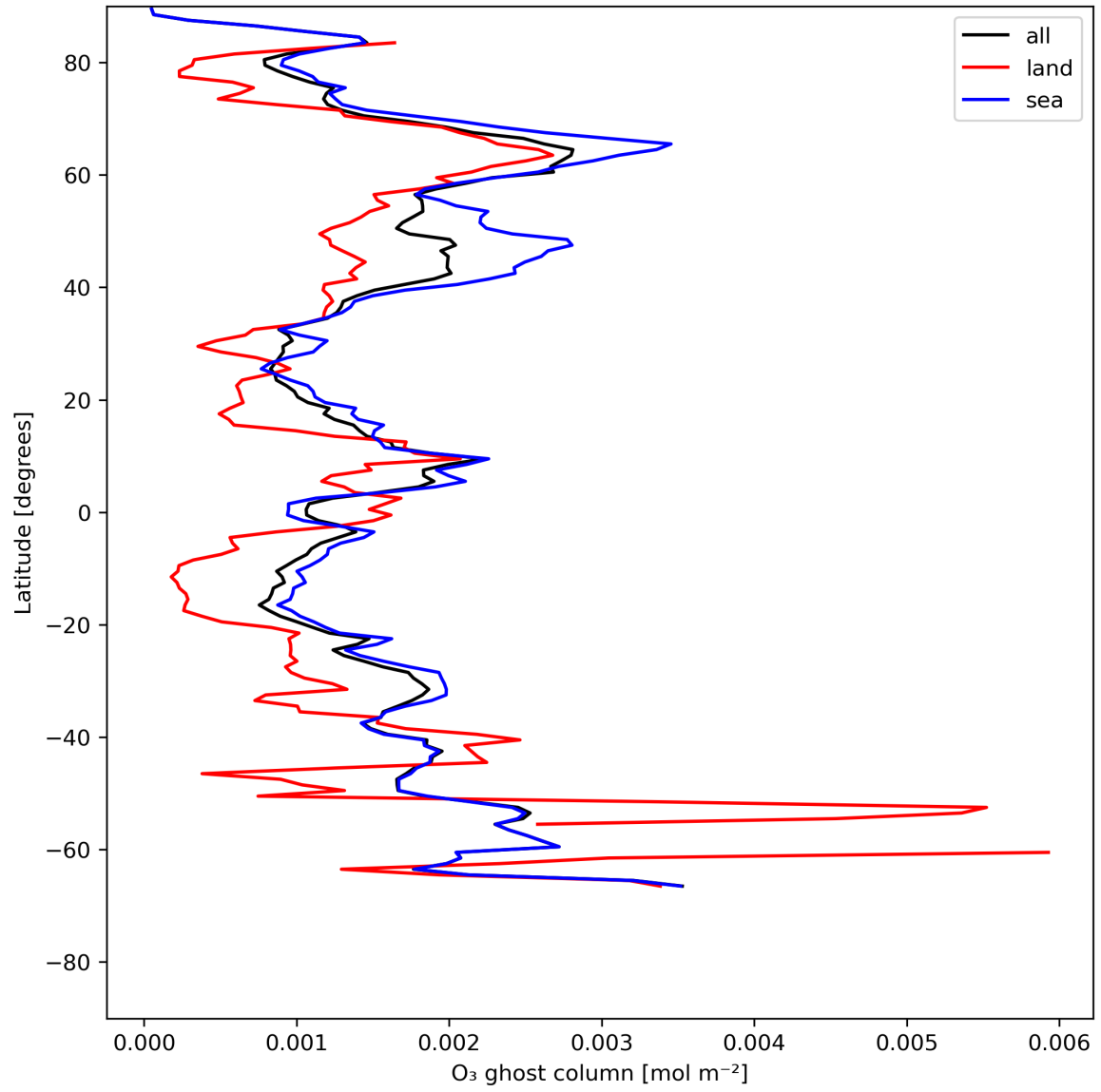
Figure 18: Zonal average of “O 3 ghost column” for 2024-05-28 to 2024-05-30.
