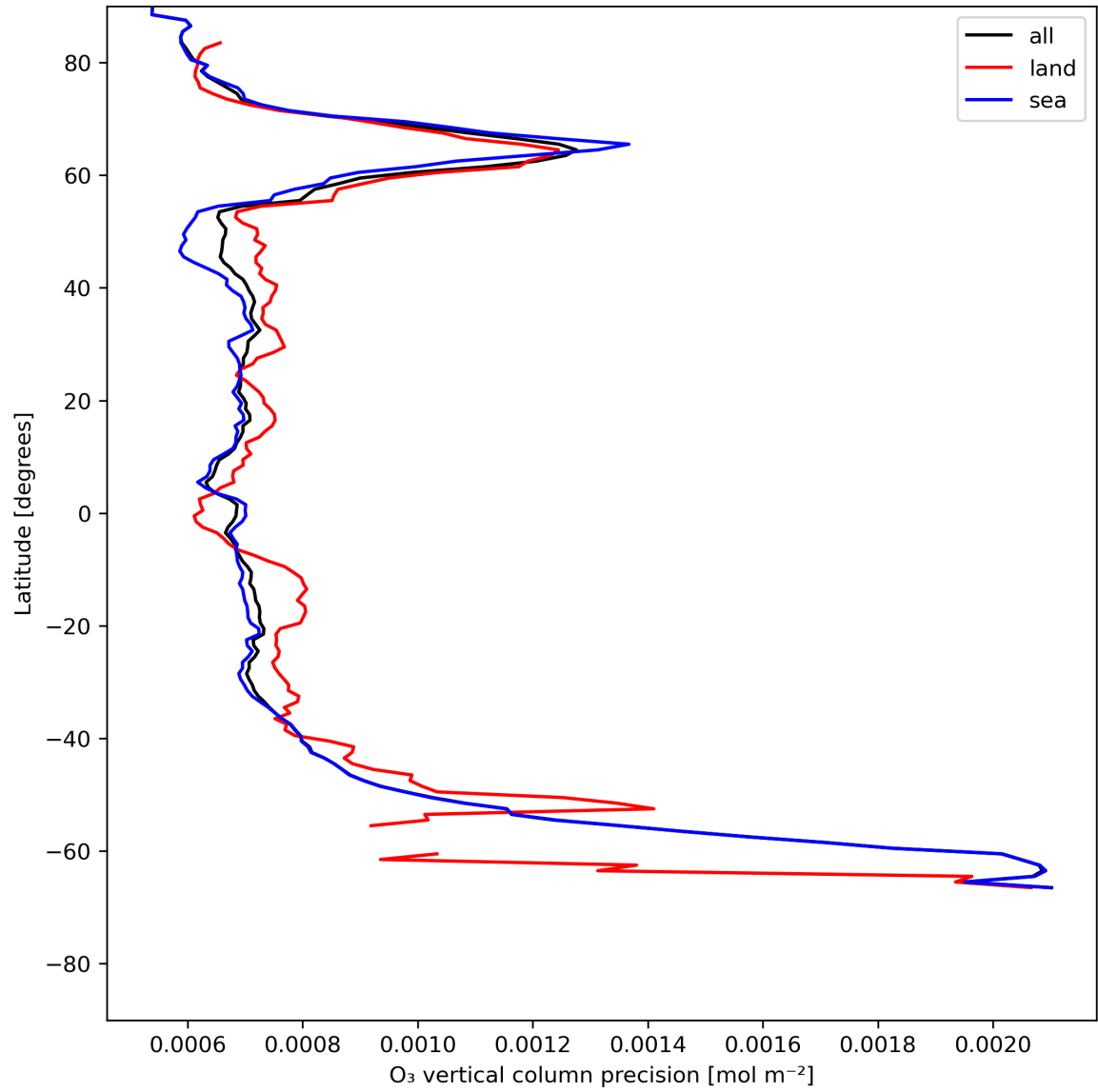
Figure 15: Zonal average of “O 3 vertical column precision” for 2024-05-28 to 2024-05-30.
