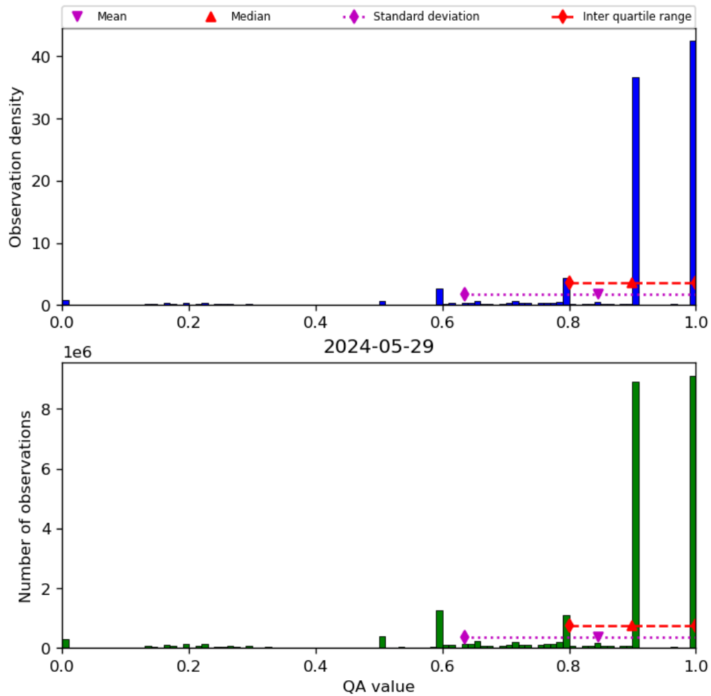
Figure 20: Histogram of “QA value” for 2024-05-28 to 2024-05-30
