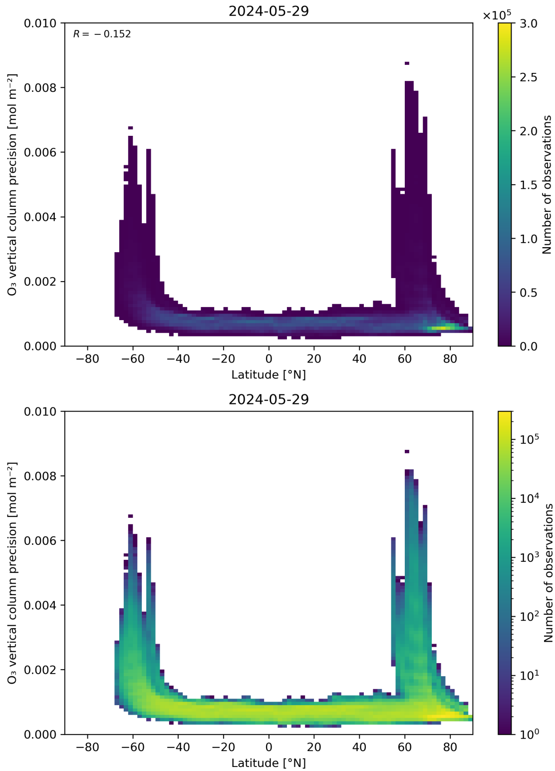
Figure 37: Scatter density plot of “Latitude” against “O 3 vertical column precision” for 2024-05-28 to 2024-05-30.
