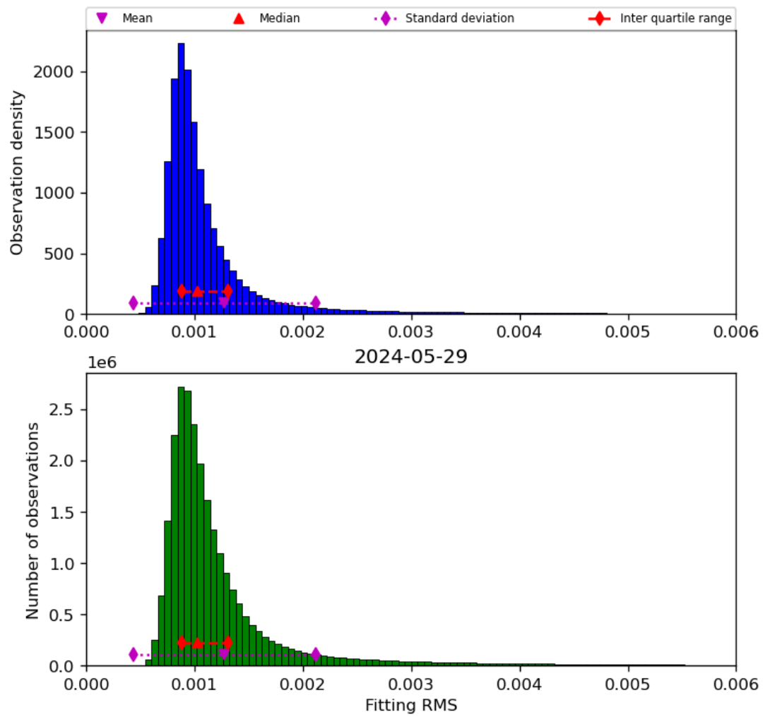
Figure 23: Histogram of “Fitting RMS” for 2024-05-28 to 2024-05-30
