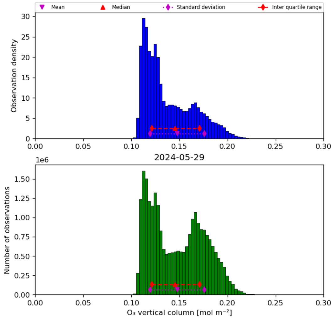
Figure 21: Histogram of “O 3 vertical column” for 2024-05-28 to 2024-05-30
