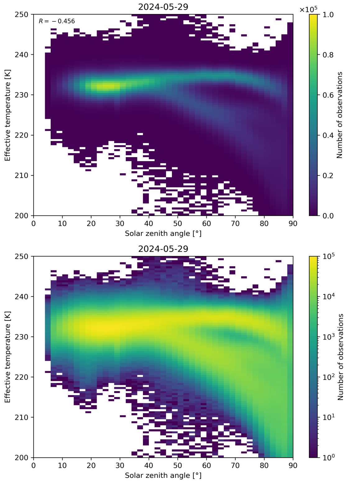
Figure 45: Scatter density plot of “Solar zenith angle” against “Effective temperature” for 2024-05-28 to 2024-05-30.
