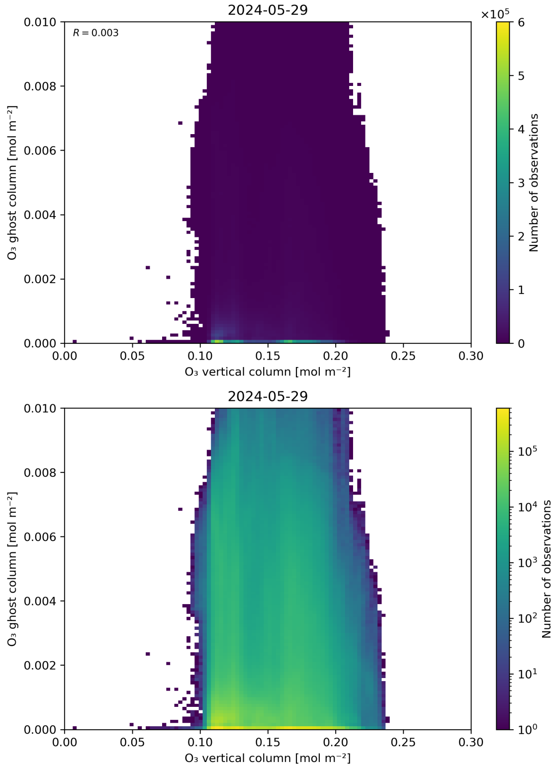
Figure 40: Scatter density plot of “O 3 vertical column” against “O 3 ghost column” for 2024-05-28 to 2024-05-30.
