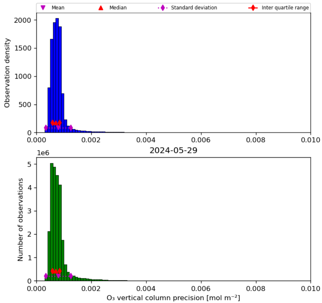
Figure 22: Histogram of “O 3 vertical column precision” for 2024-05-28 to 2024-05-30
