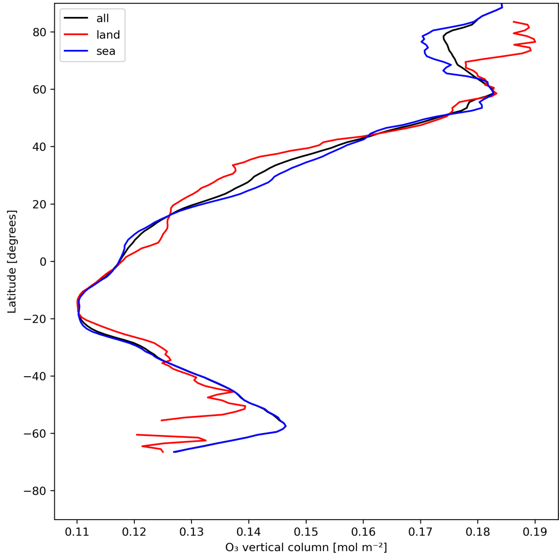
Figure 14: Zonal average of “O 3 vertical column” for 2024-05-28 to 2024-05-30.
