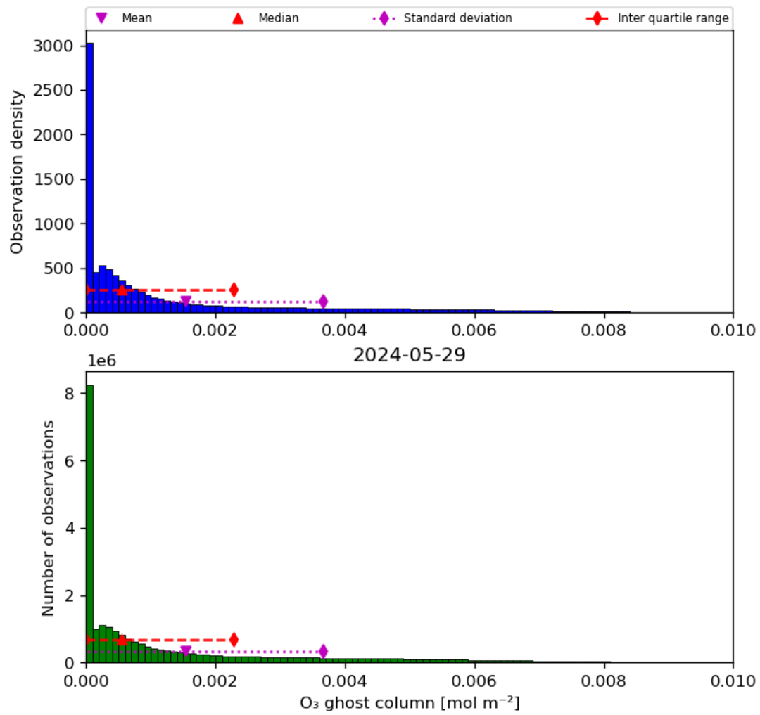
Figure 25: Histogram of “O 3 ghost column” for 2024-05-28 to 2024-05-30
