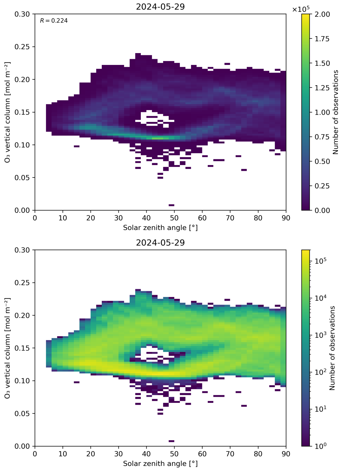
Figure 47: Scatter density plot of “Solar zenith angle” against “O 3 vertical column” for 2024-05-28 to 2024-05-30.
