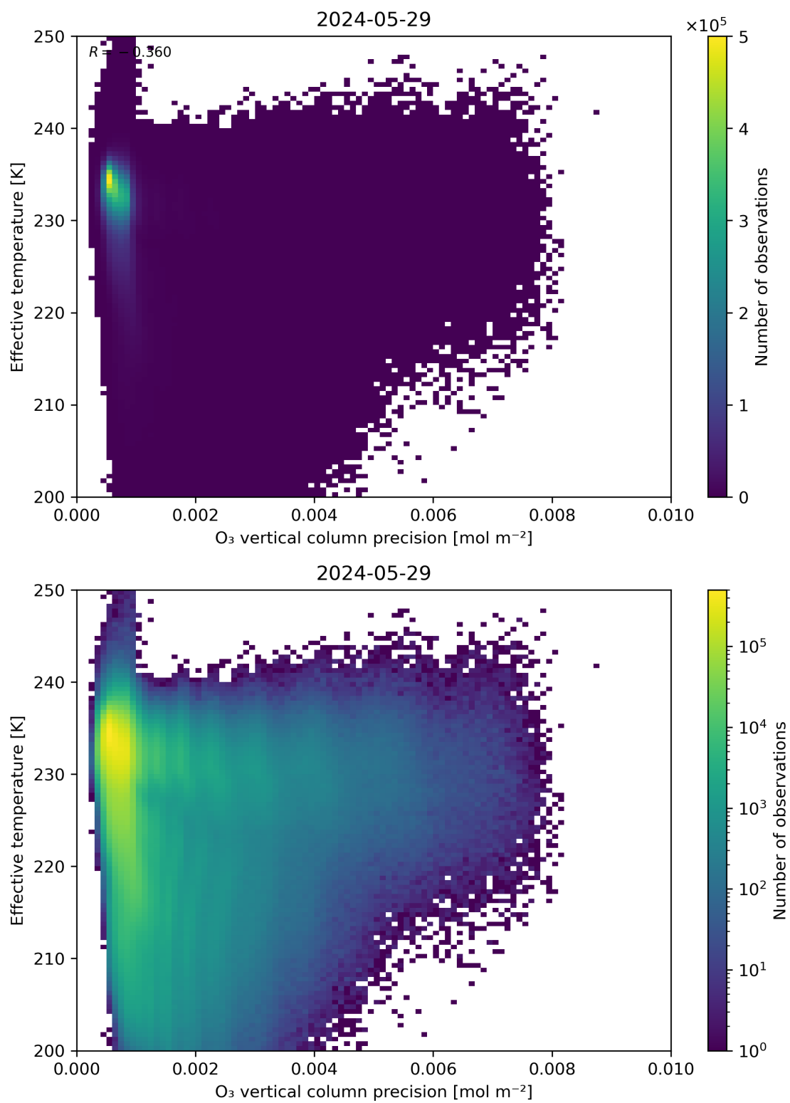
Figure 42: Scatter density plot of “O 3 vertical column precision” against “Effective temperature” for 2024-05-28 to 2024-05-30.
