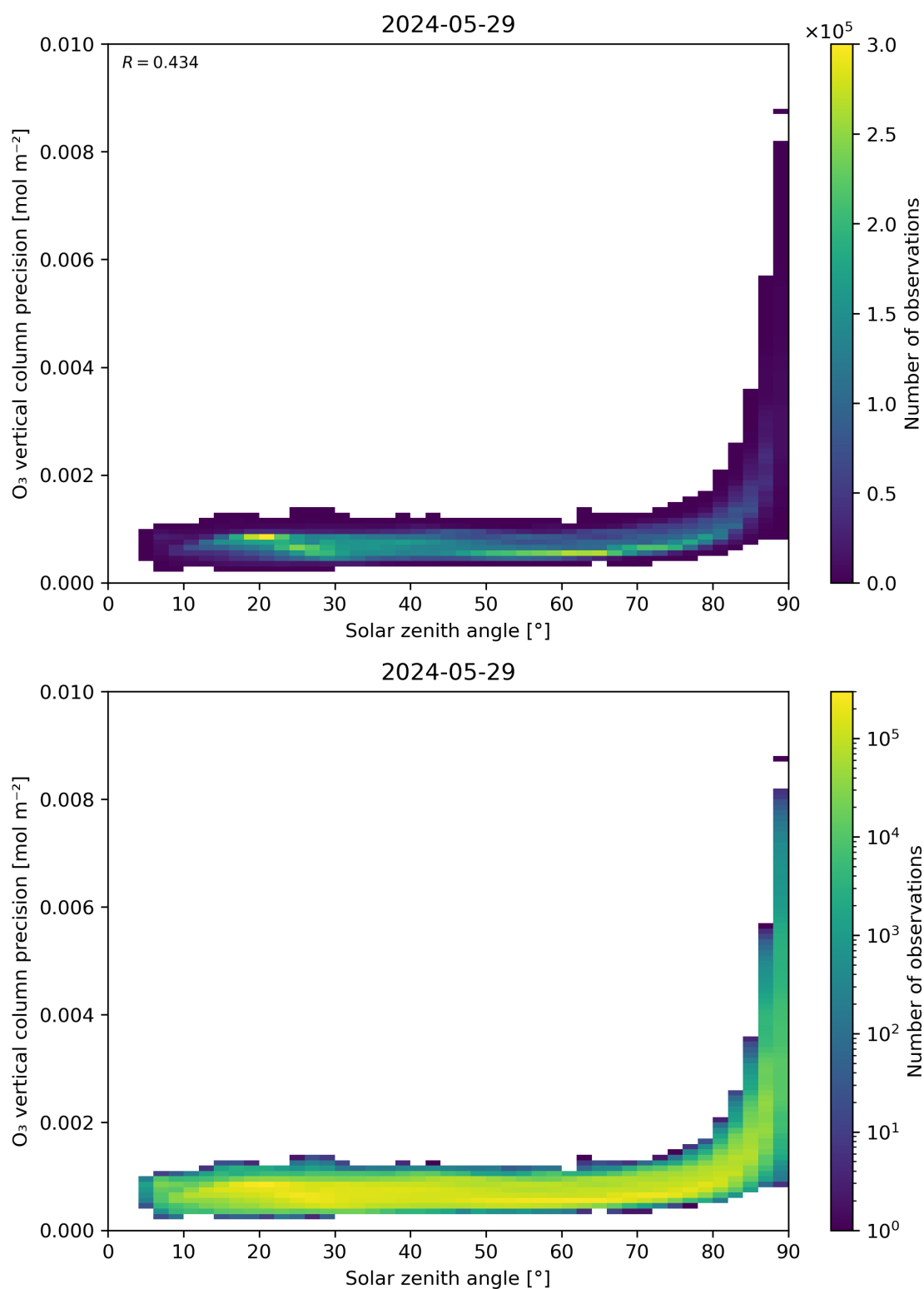
Figure 48: Scatter density plot of “Solar zenith angle” against “O 3 vertical column precision” for 2024-05-28 to 2024-05-30.
