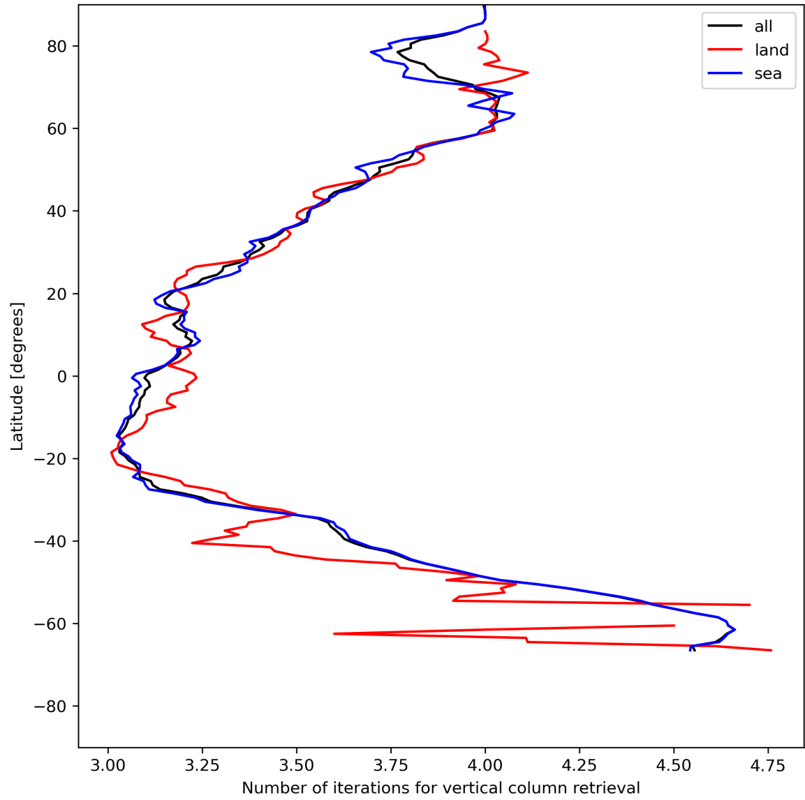
Figure 19: Zonal average of “Number of iterations for vertical column retrieval” for 2024-05-28 to 2024-05-30.
