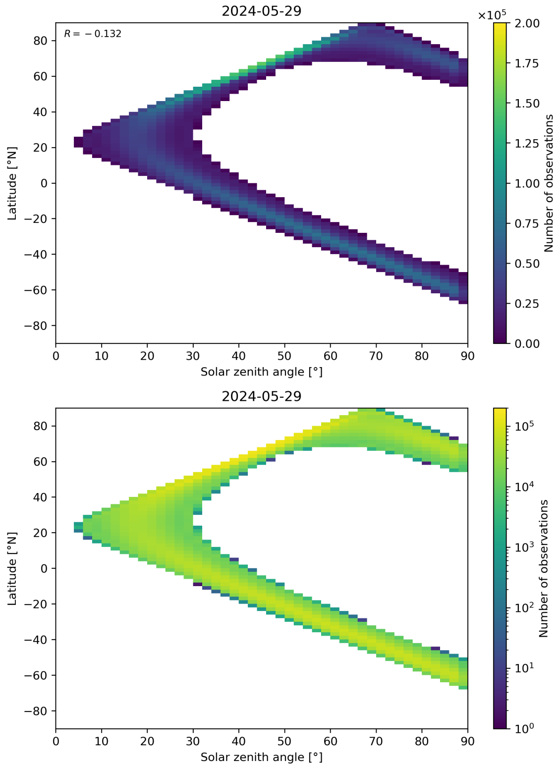
Figure 44: Scatter density plot of “Solar zenith angle” against “Latitude” for 2024-05-28 to 2024-05-30.
