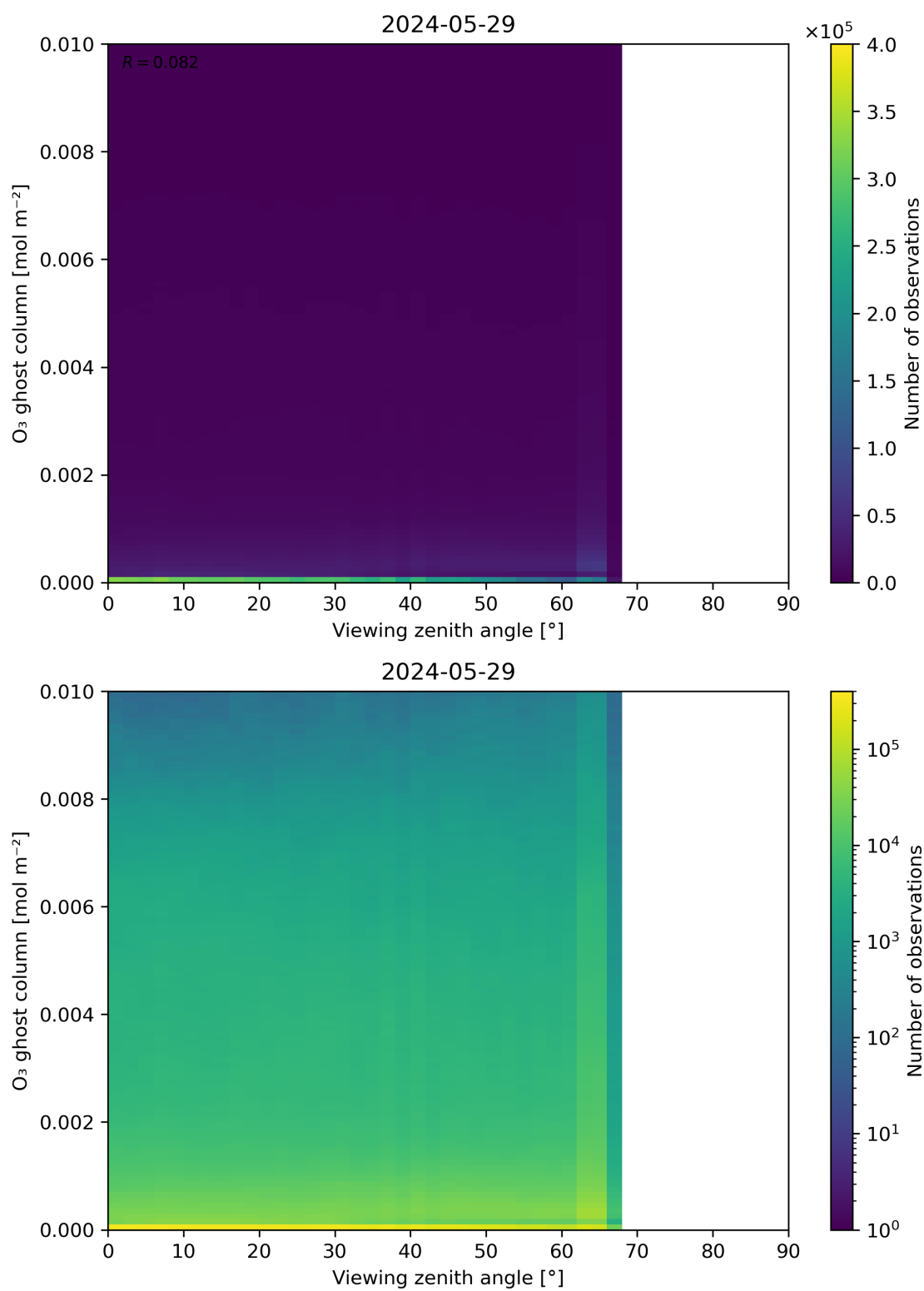
Figure 51: Scatter density plot of “Viewing zenith angle” against “O 3 ghost column” for 2024-05-28 to 2024-05-30.
