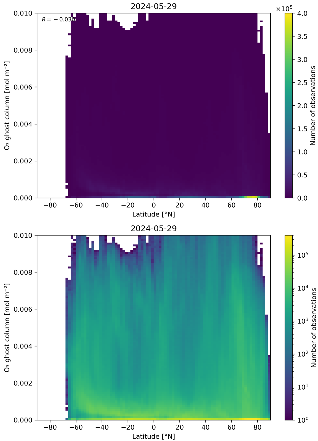
Figure 35: Scatter density plot of “Latitude” against “O 3 ghost column” for 2024-05-28 to 2024-05-30.
