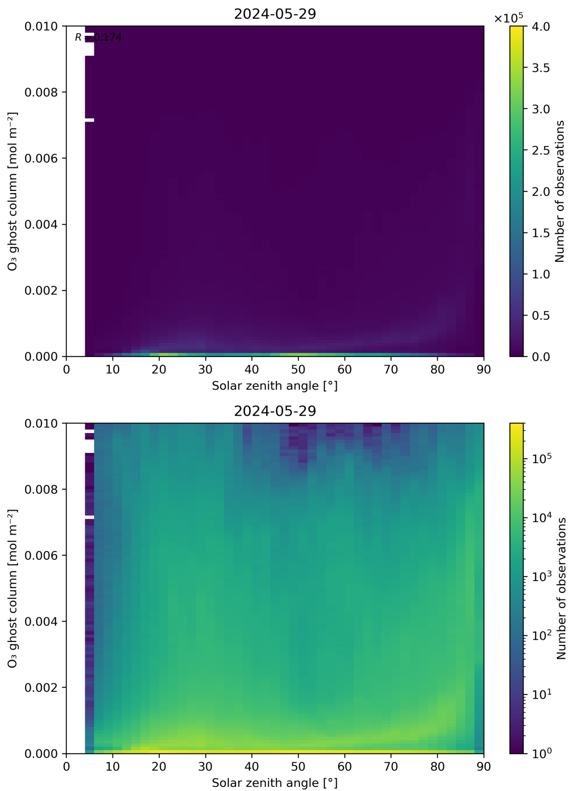
Figure 46: Scatter density plot of “Solar zenith angle” against “O 3 ghost column” for 2024-05-28 to 2024-05-30.
