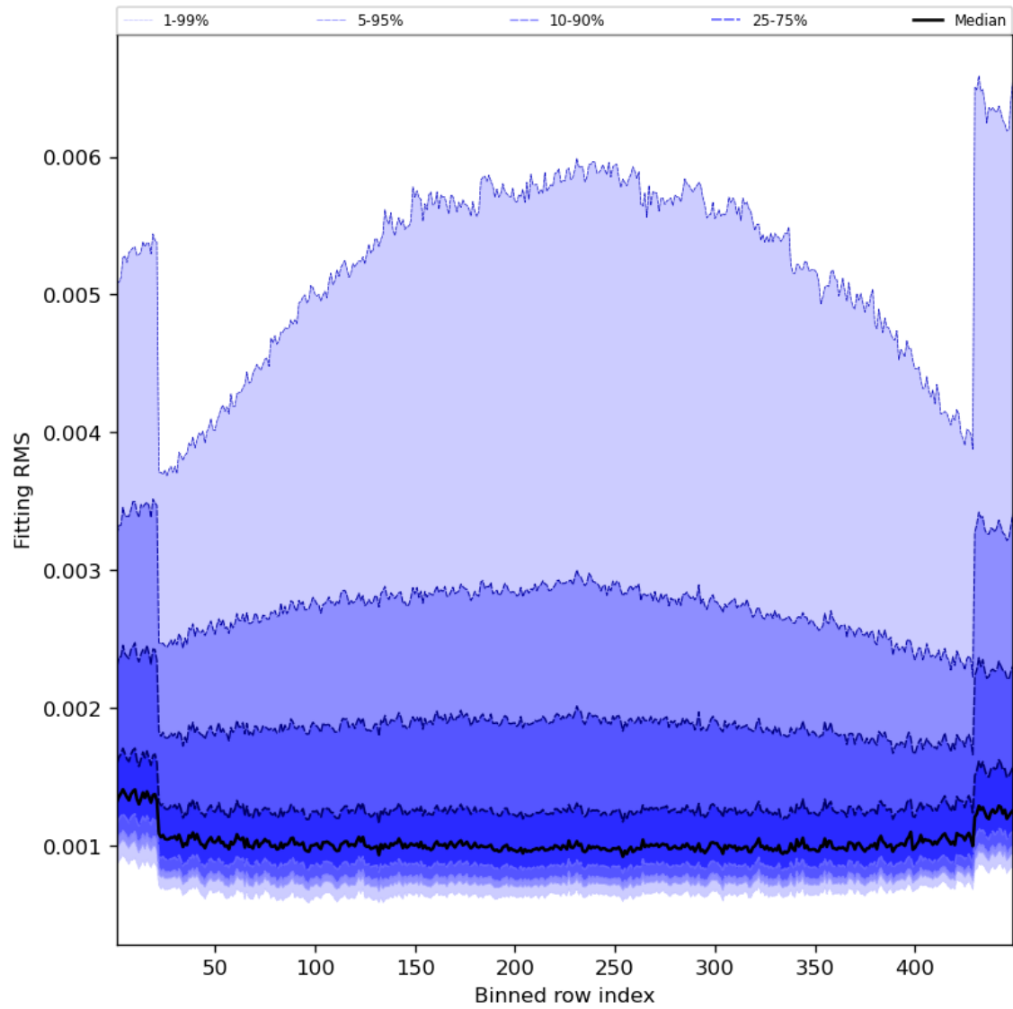
Figure 30: Along track statistics of “Fitting RMS” for 2024-05-28 to 2024-05-30
