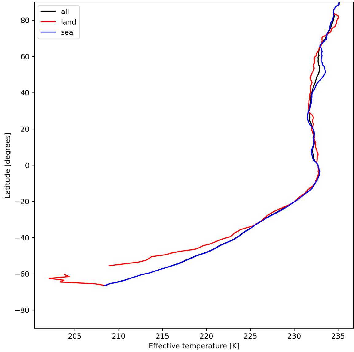
Figure 17: Zonal average of "Effective temperature" for 2024-05-28 to 2024-05-30.
