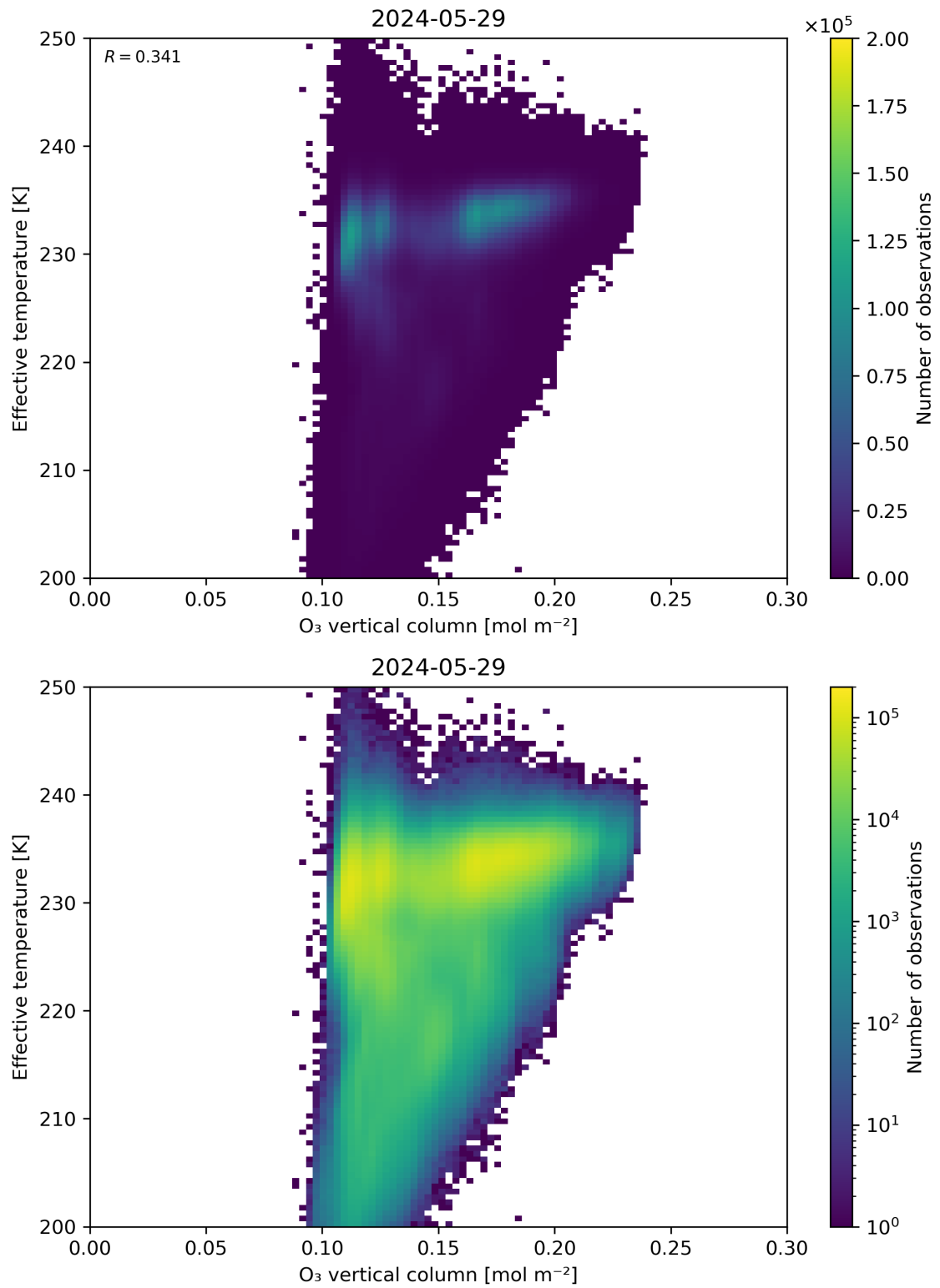
Figure 39: Scatter density plot of “O 3 vertical column” against “Effective temperature” for 2024-05-28 to 2024-05-30.
