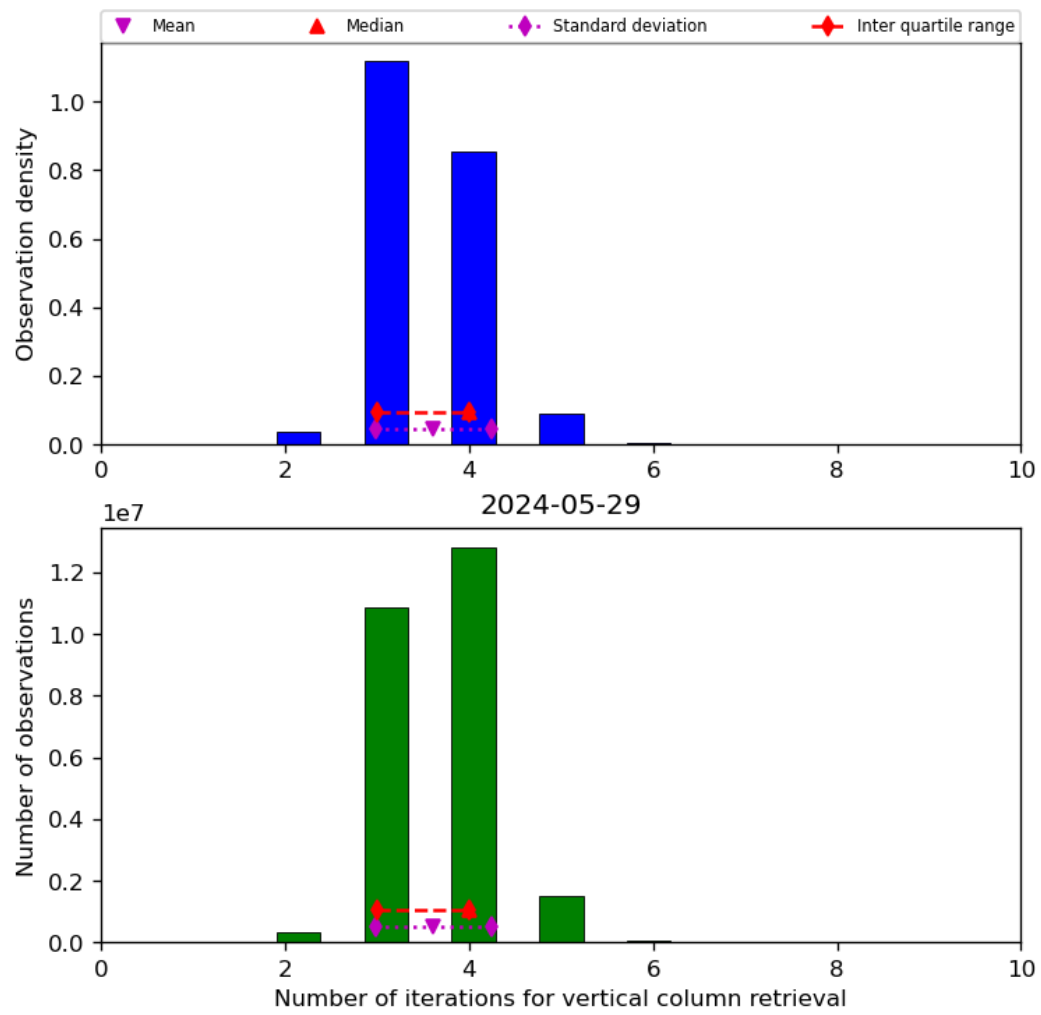
Figure 26: Histogram of “Number of iterations for vertical column retrieval” for 2024-05-28 to 2024-05-30
