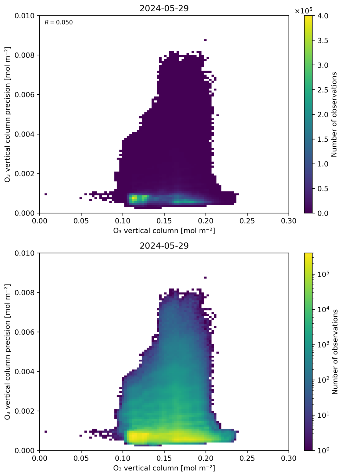
Figure 41: Scatter density plot of “O 3 vertical column” against “O 3 vertical column precision” for 2024-05-28 to 2024-05-30.
