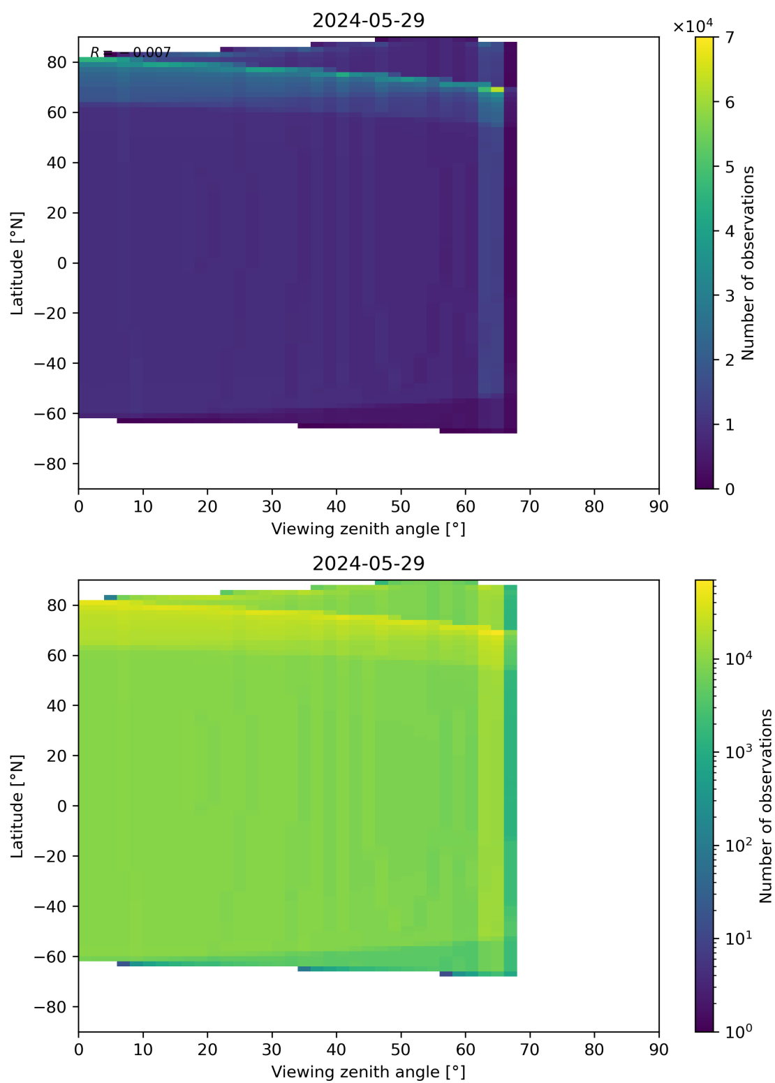
Figure 49: Scatter density plot of “Viewing zenith angle” against “Latitude” for 2024-05-28 to 2024-05-30.
