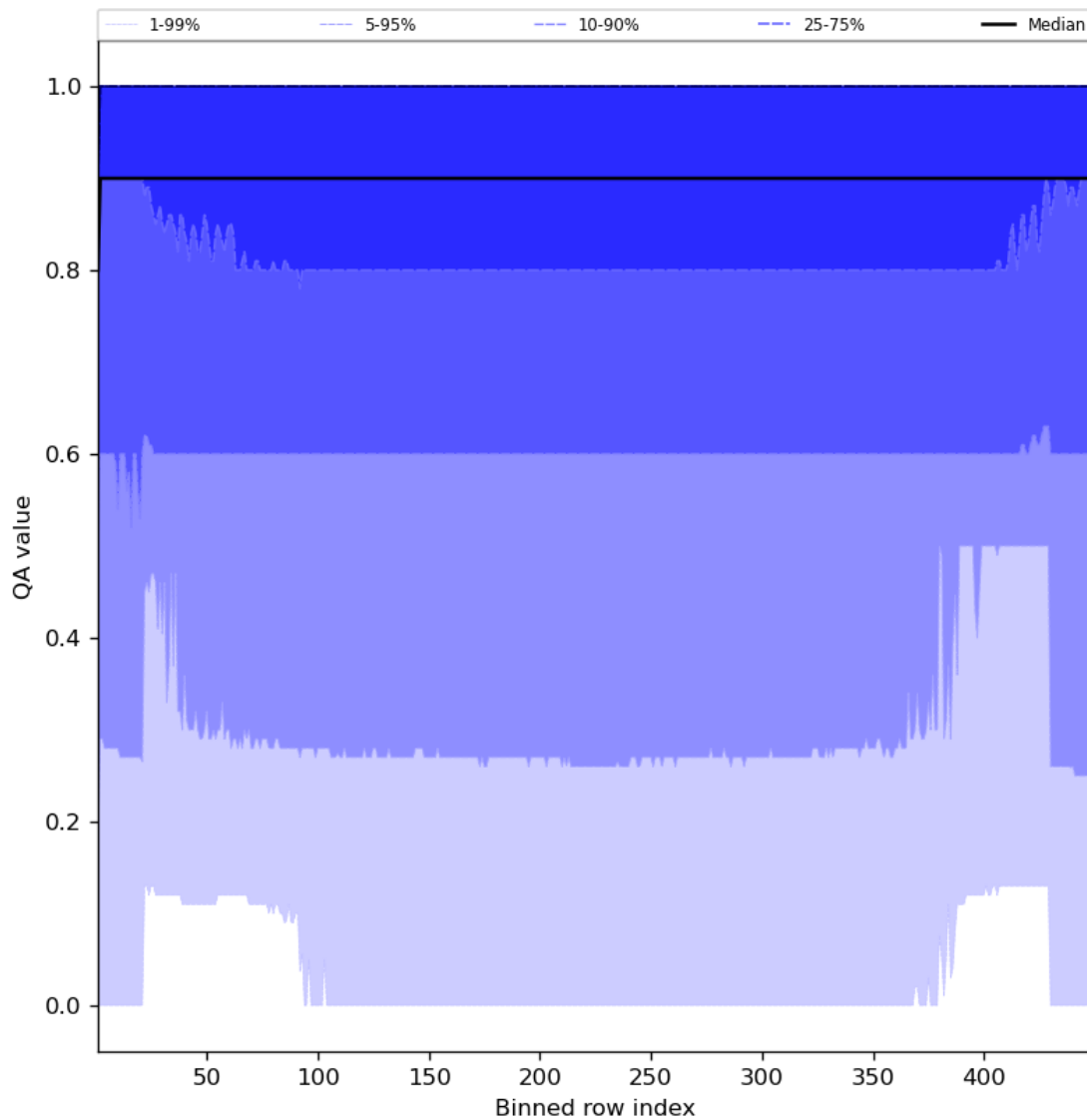
Figure 27: Along track statistics of “QA value” for 2024-05-28 to 2024-05-30
