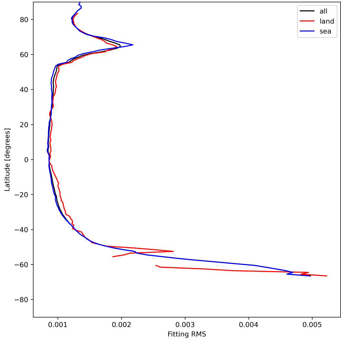
Figure 16: Zonal average of “Fitting RMS” for 2024-05-28 to 2024-05-30.
