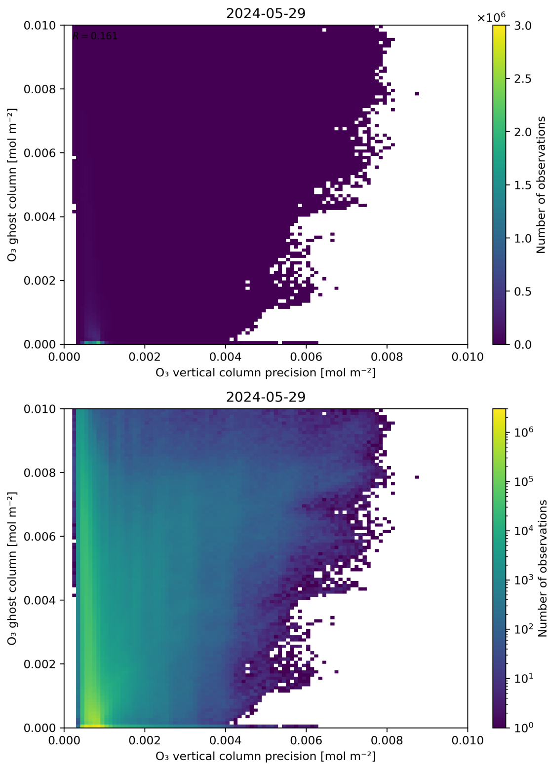
Figure 43: Scatter density plot of “ \text{O}_3 vertical column precision” against “ \text{O}_3 ghost column” for 2024-05-28 to 2024-05-30.
