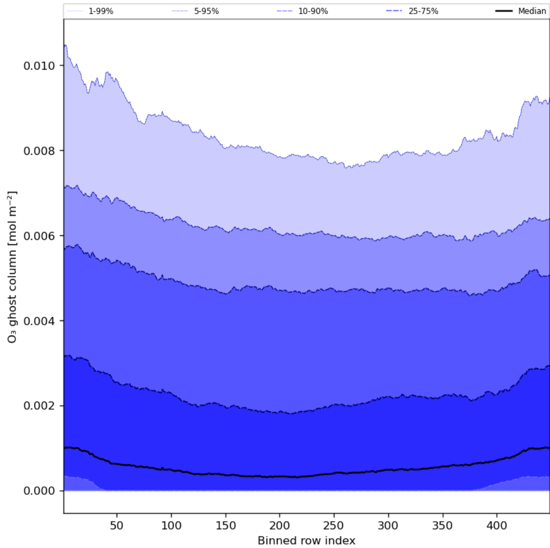
Figure 32: Along track statistics of “O 3 ghost column” for 2024-05-28 to 2024-05-30
