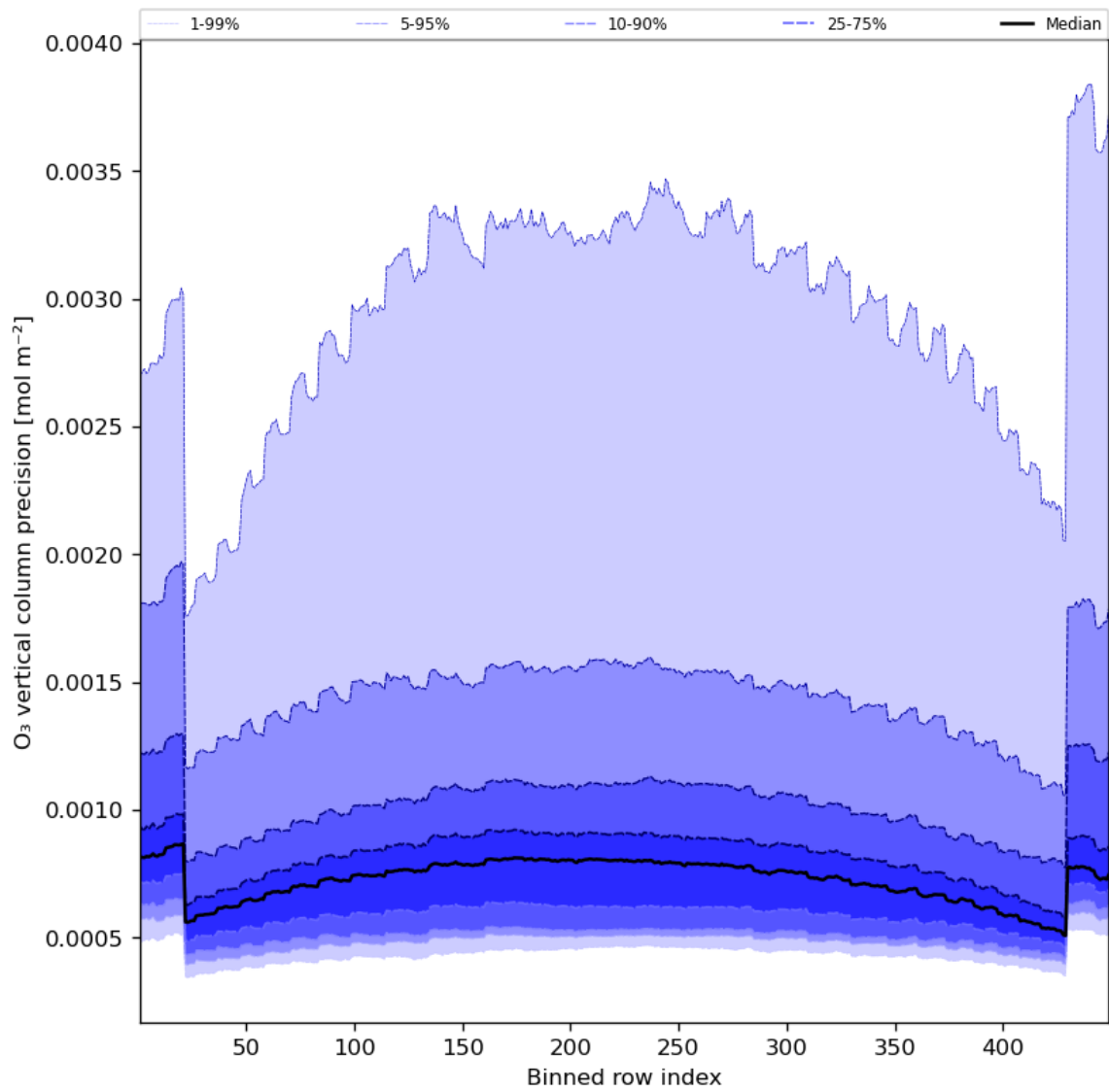
Figure 29: Along track statistics of “O 3 vertical column precision” for 2024-05-28 to 2024-05-30
