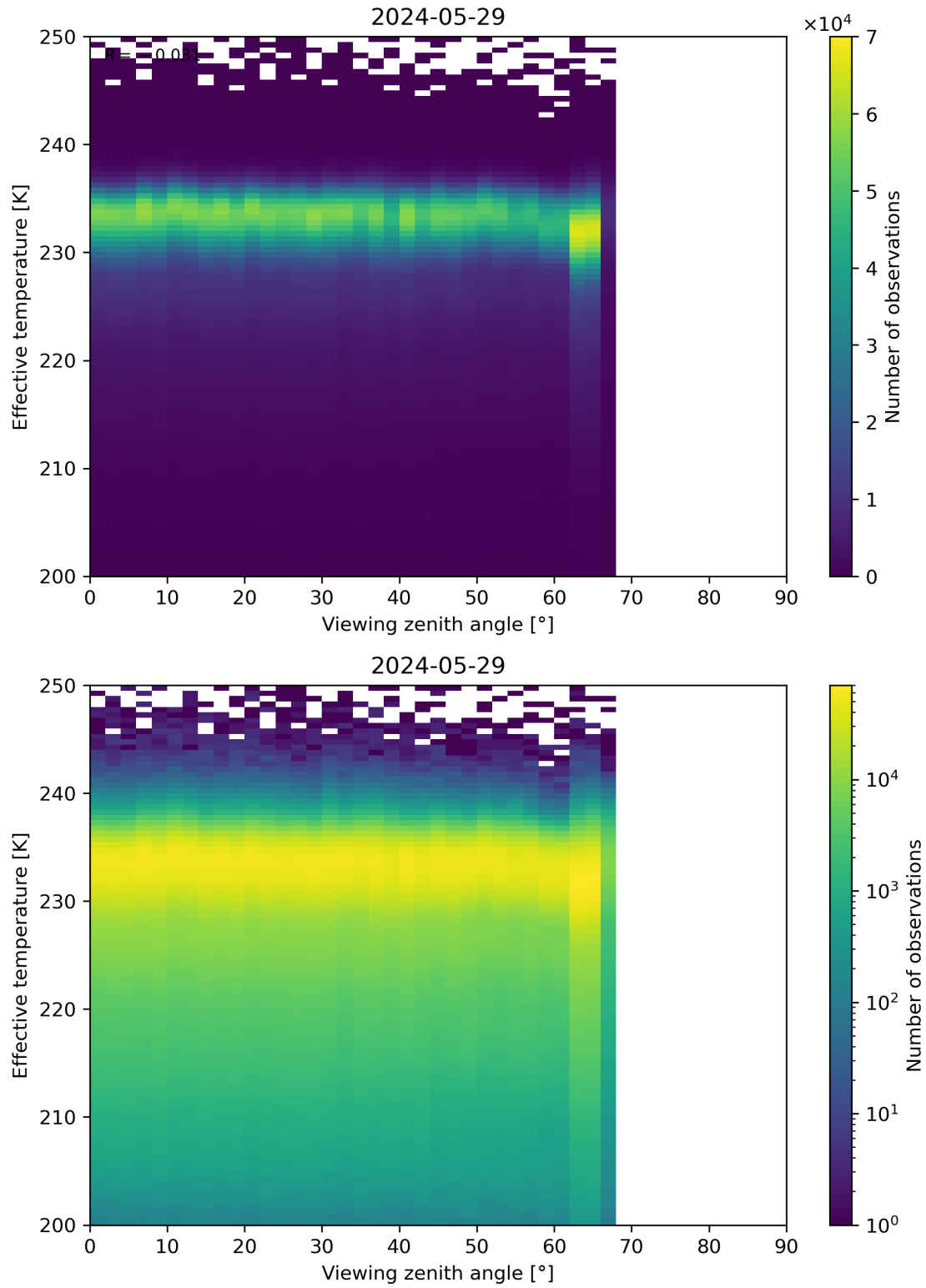
Figure 50: Scatter density plot of “Viewing zenith angle” against “Effective temperature” for 2024-05-28 to 2024-05-30.
