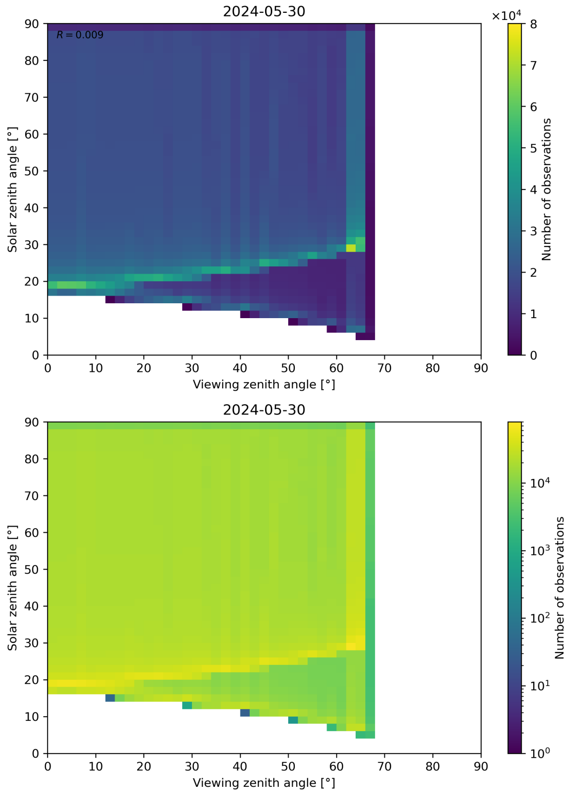
Figure 54: Scatter density plot of “Viewing zenith angle” against “Solar zenith angle” for 2024-05-29 to 2024-05-31.
