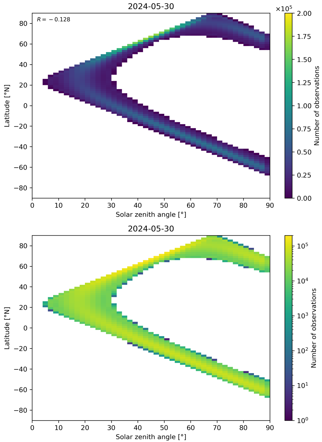
Figure 44: Scatter density plot of “Solar zenith angle” against “Latitude” for 2024-05-29 to 2024-05-31.
