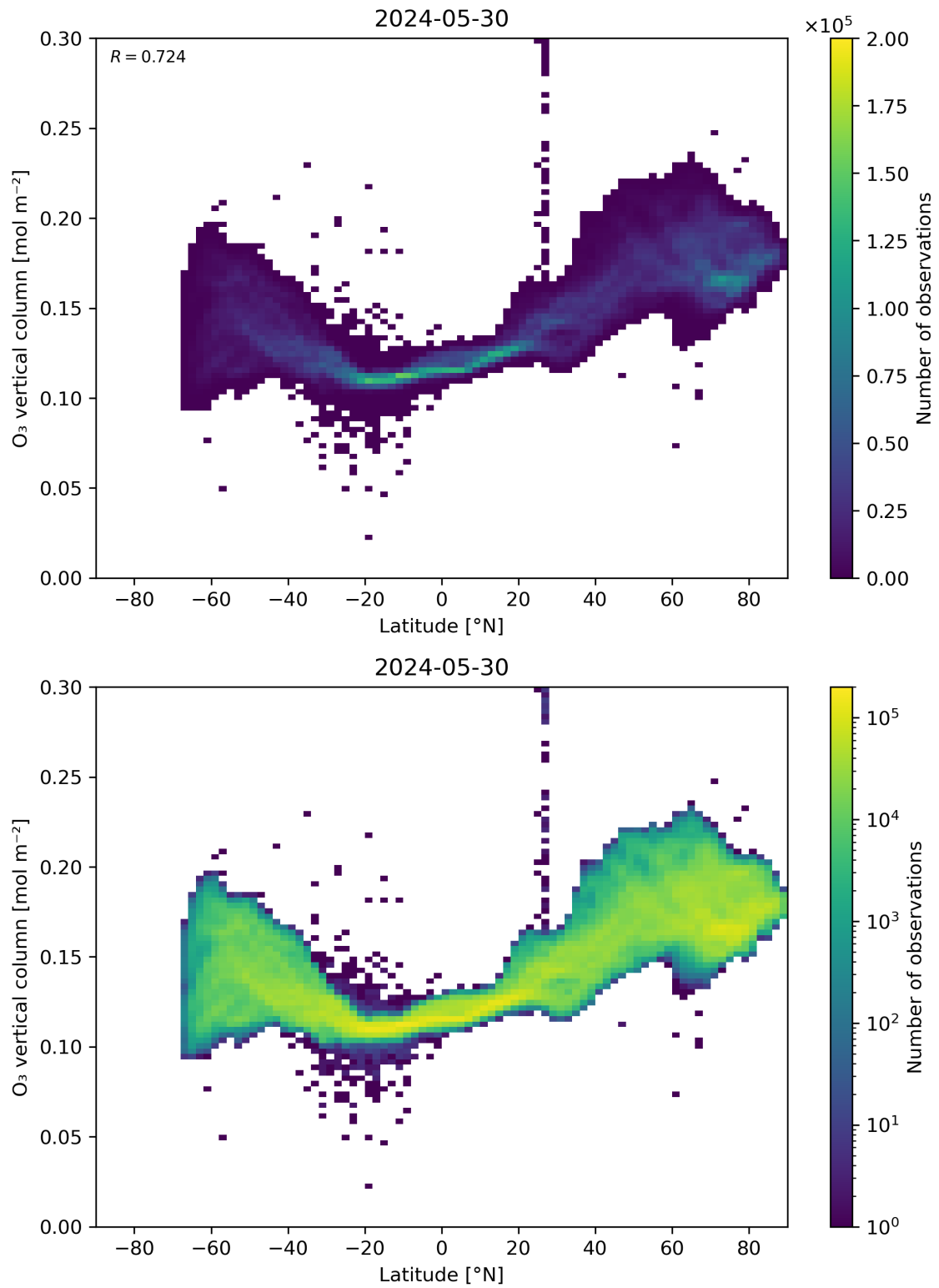
Figure 36: Scatter density plot of “Latitude” against “O 3 vertical column” for 2024-05-29 to 2024-05-31.
