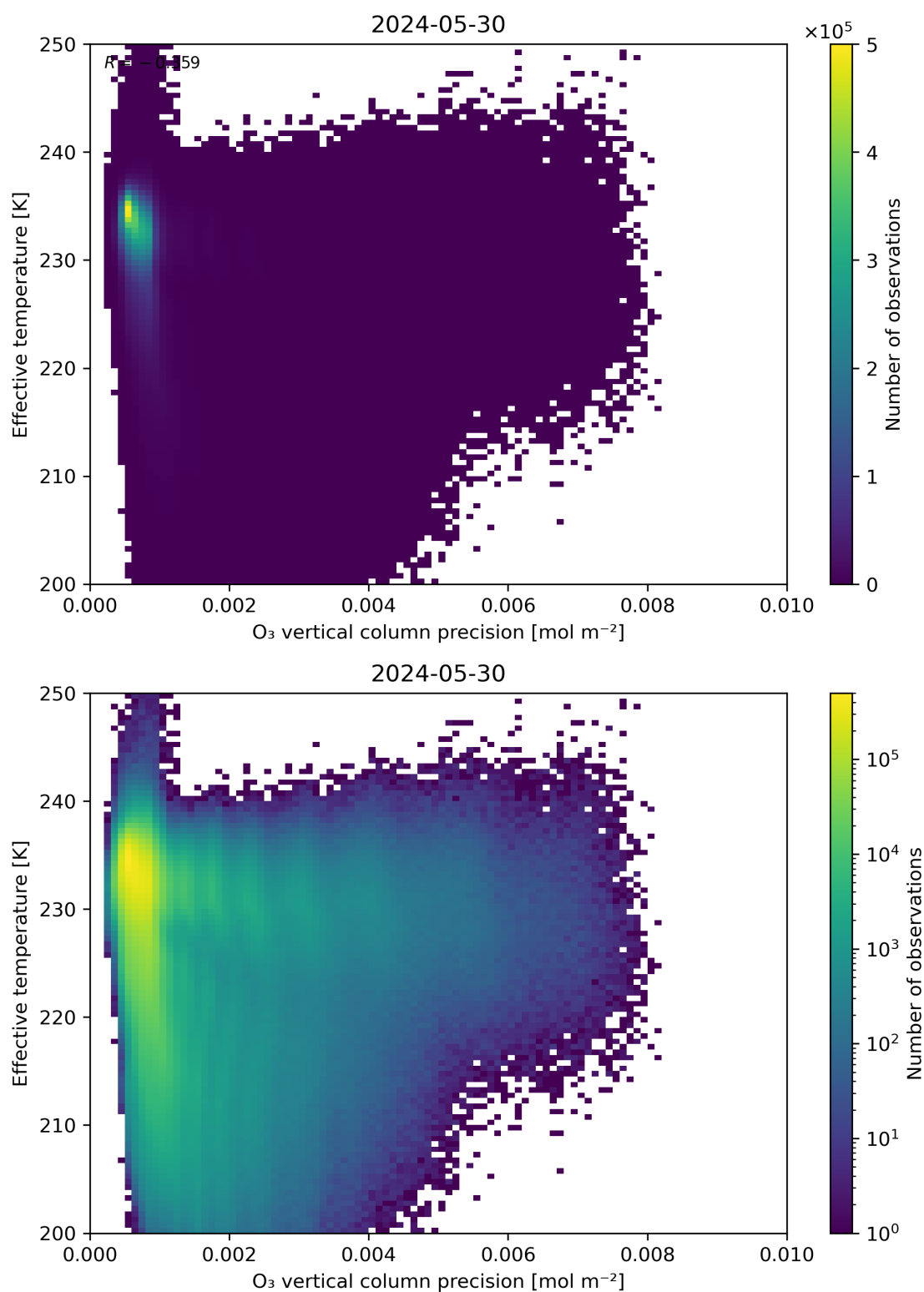
Figure 42: Scatter density plot of “O 3 vertical column precision” against “Effective temperature” for 2024-05-29 to 2024-05-31.
