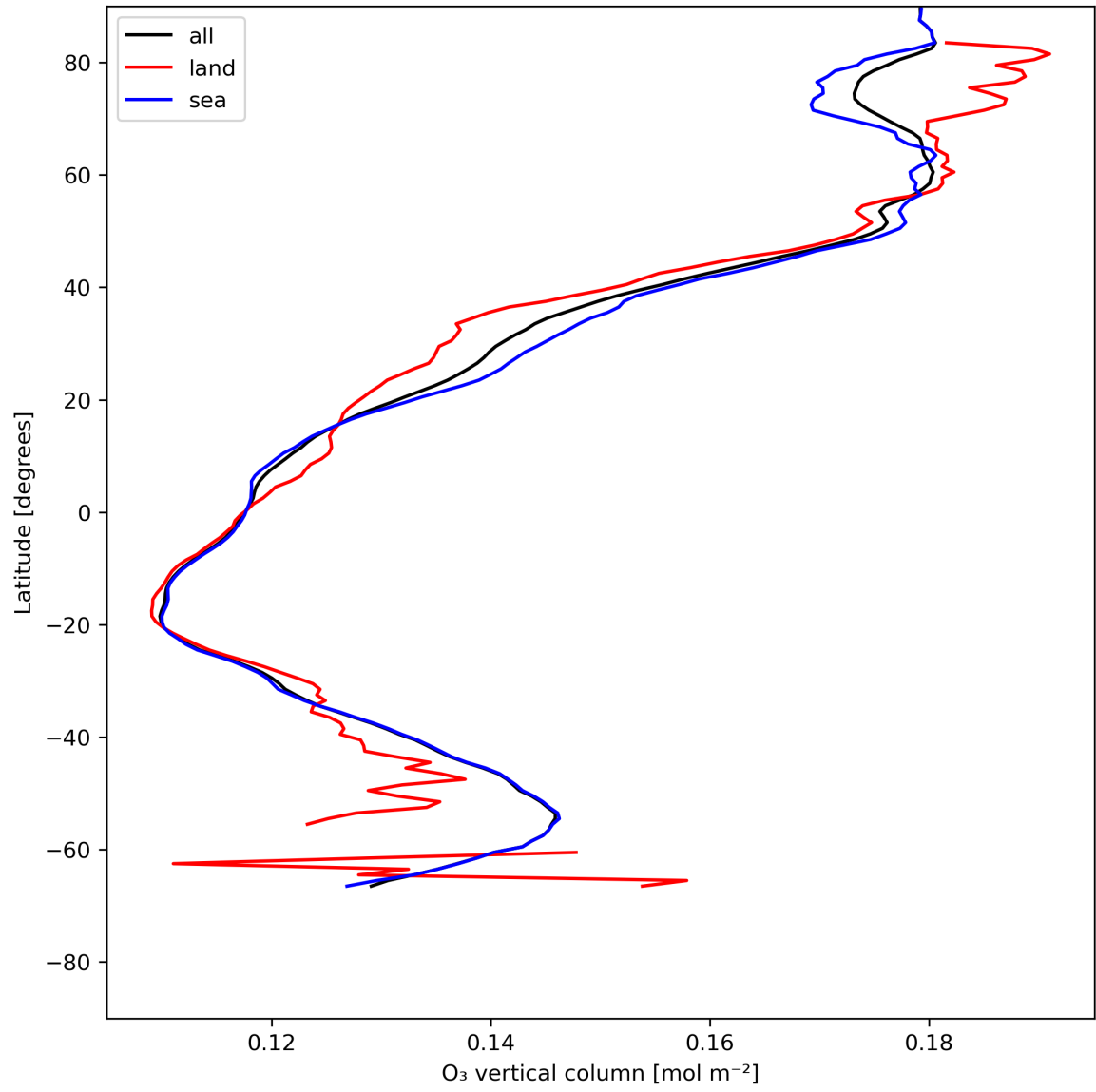
Figure 14: Zonal average of “O 3 vertical column” for 2024-05-29 to 2024-05-31.
