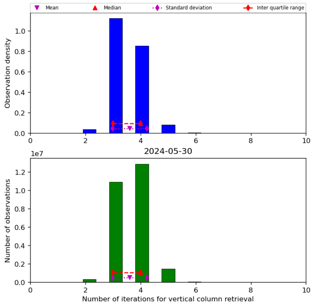
Figure 26: Histogram of “Number of iterations for vertical column retrieval” for 2024-05-29 to 2024-05-31
