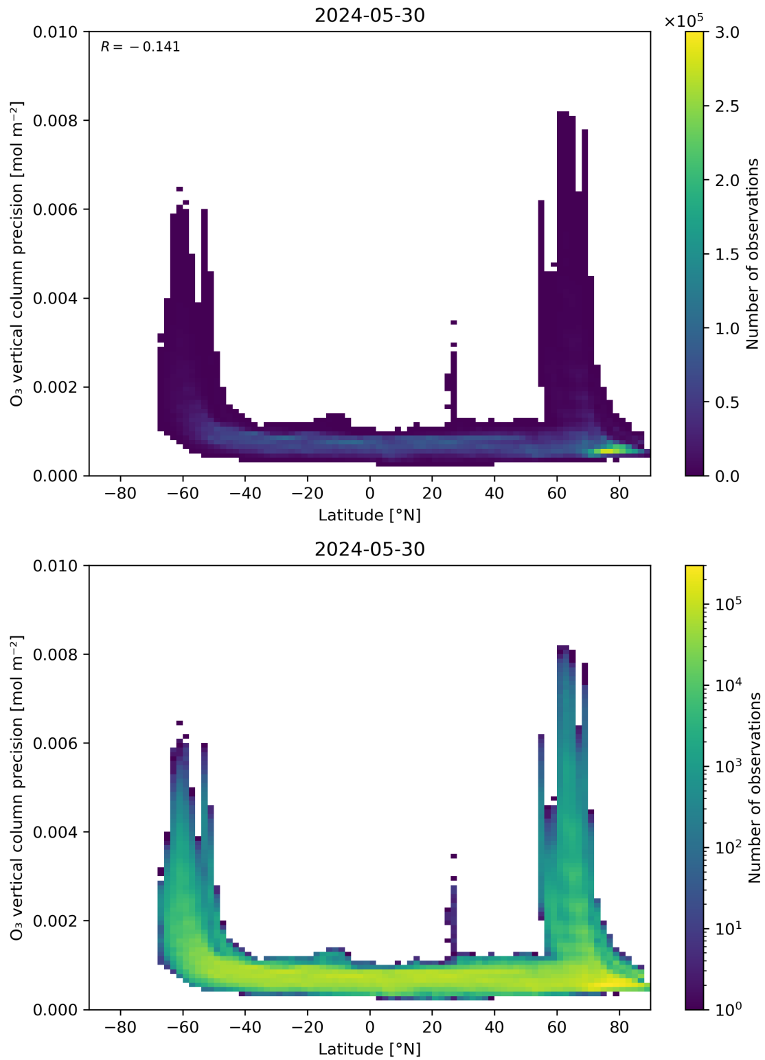
Figure 37: Scatter density plot of “Latitude” against “O 3 vertical column precision” for 2024-05-29 to 2024-05-31.
