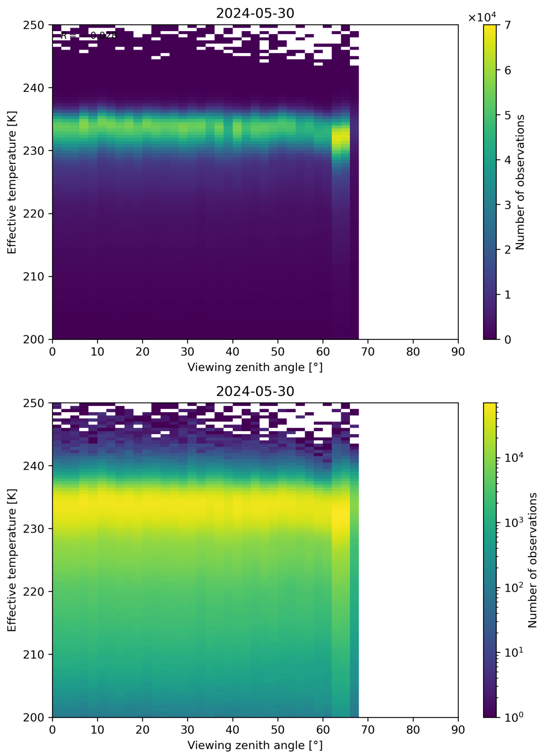
Figure 50: Scatter density plot of “Viewing zenith angle” against “Effective temperature” for 2024-05-29 to 2024-05-31.
