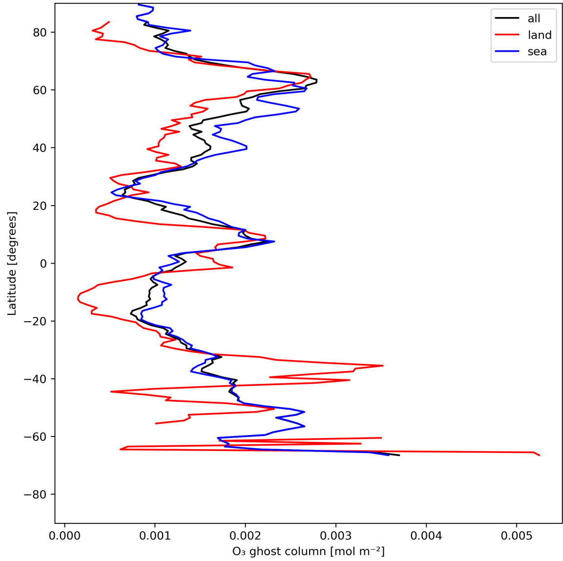
Figure 18: Zonal average of “O 3 ghost column” for 2024-05-29 to 2024-05-31.
