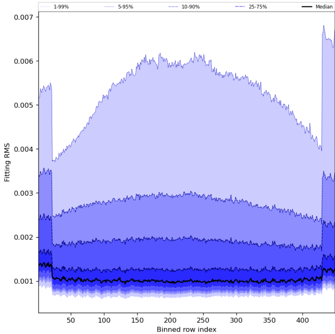
Figure 30: Along track statistics of “Fitting RMS” for 2024-05-29 to 2024-05-31
