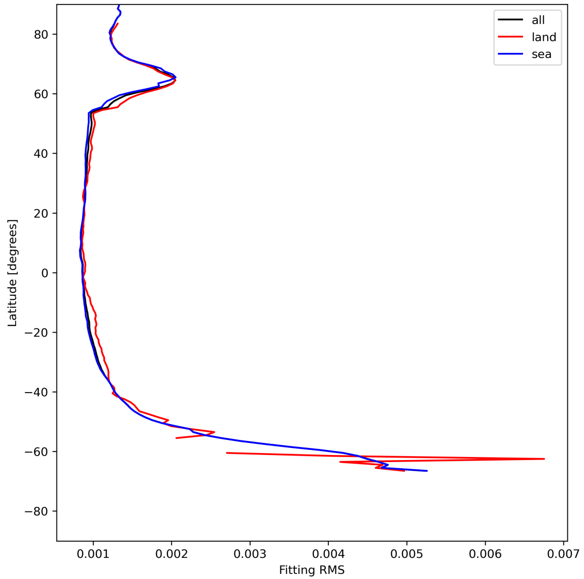
Figure 16: Zonal average of “Fitting RMS” for 2024-05-29 to 2024-05-31.
