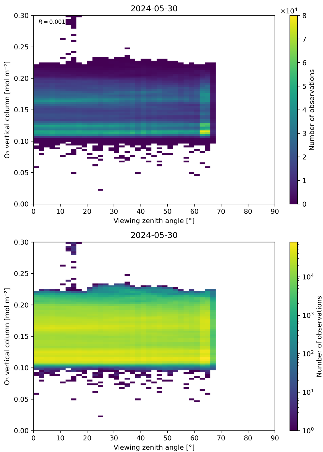
Figure 52: Scatter density plot of “Viewing zenith angle” against “O 3 vertical column” for 2024-05-29 to 2024-05-31.
