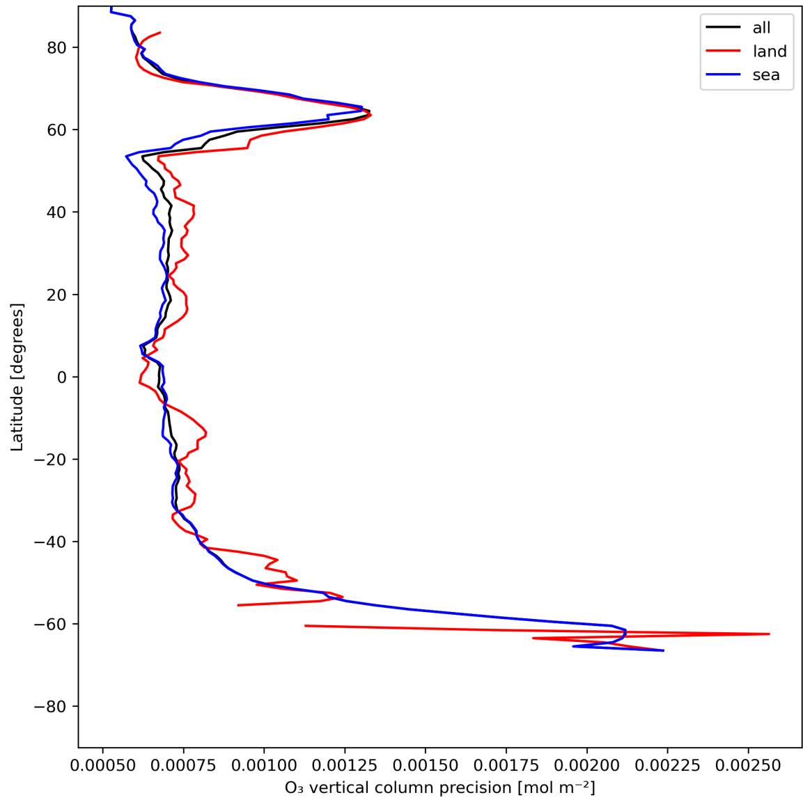
Figure 15: Zonal average of “O 3 vertical column precision” for 2024-05-29 to 2024-05-31.
