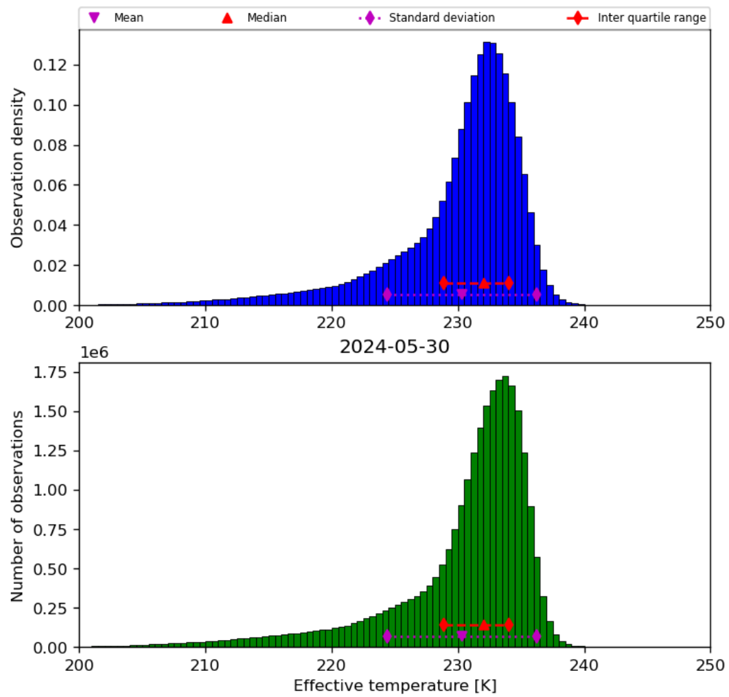
Figure 24: Histogram of “Effective temperature” for 2024-05-29 to 2024-05-31
