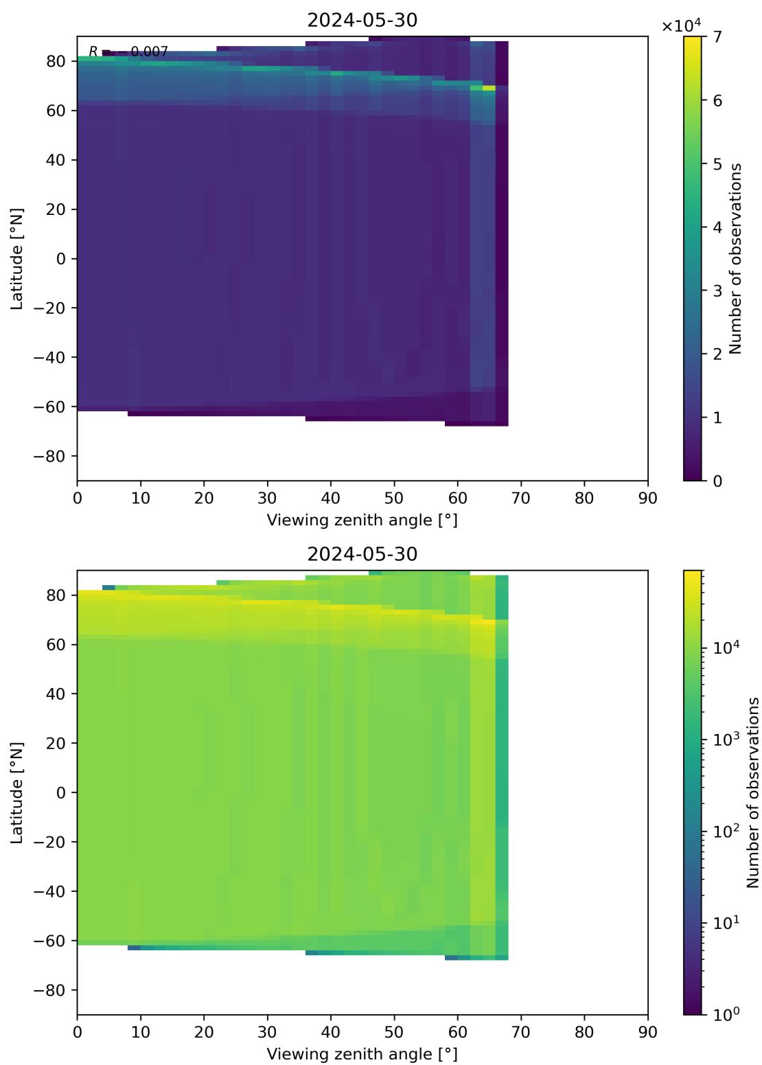
Figure 49: Scatter density plot of “Viewing zenith angle” against “Latitude” for 2024-05-29 to 2024-05-31.
