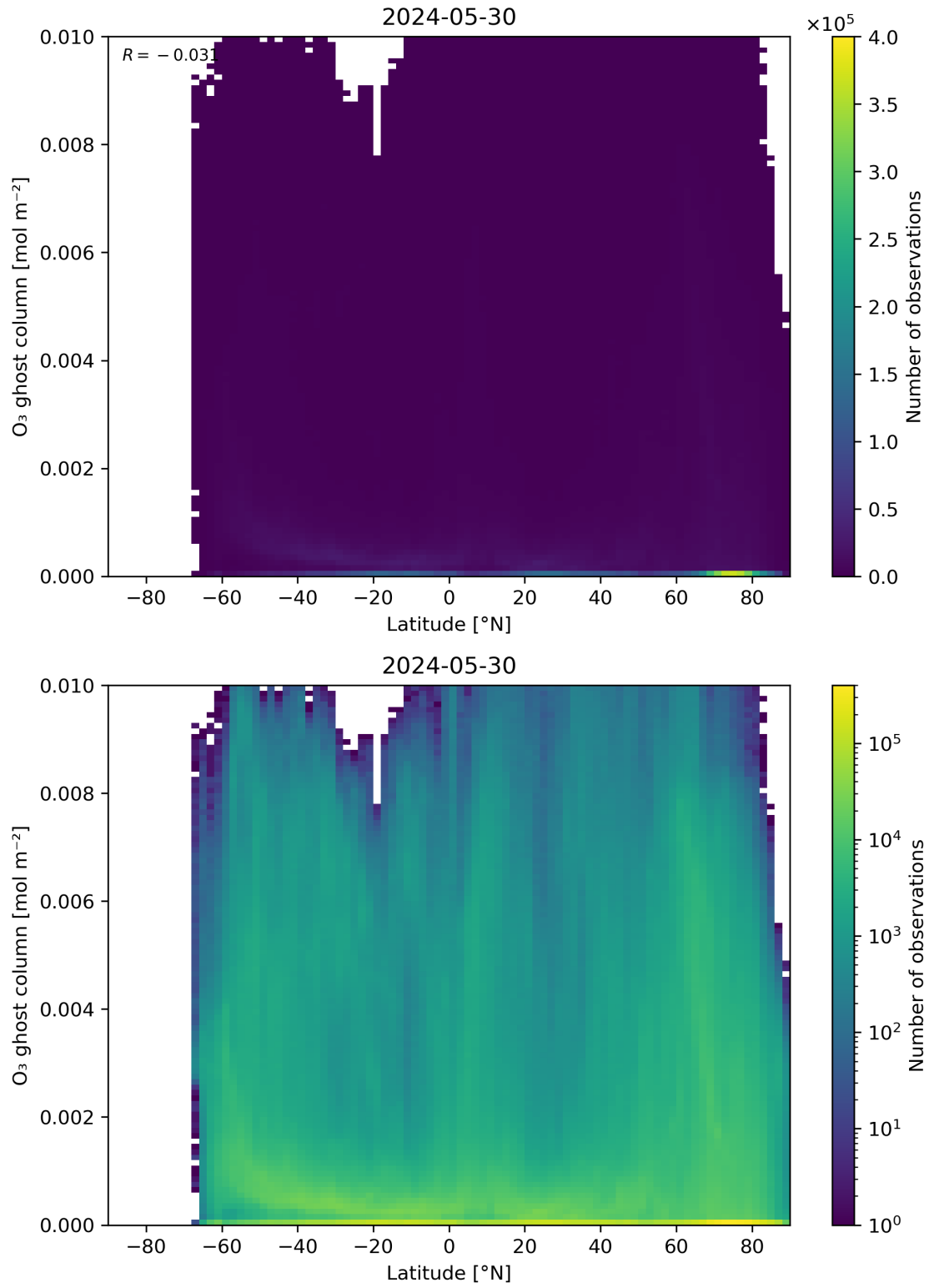
Figure 35: Scatter density plot of “Latitude” against “O 3 ghost column” for 2024-05-29 to 2024-05-31.
