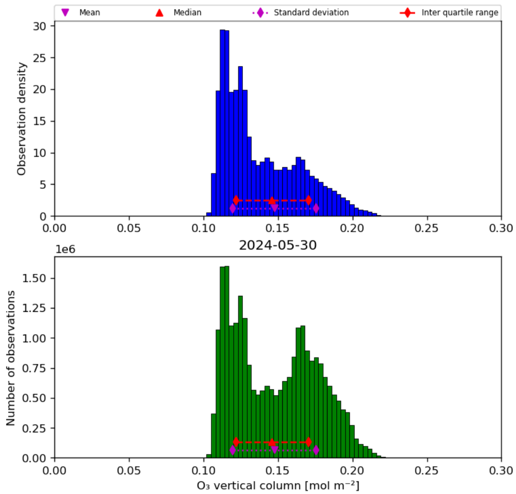
Figure 21: Histogram of “O 3 vertical column” for 2024-05-29 to 2024-05-31
