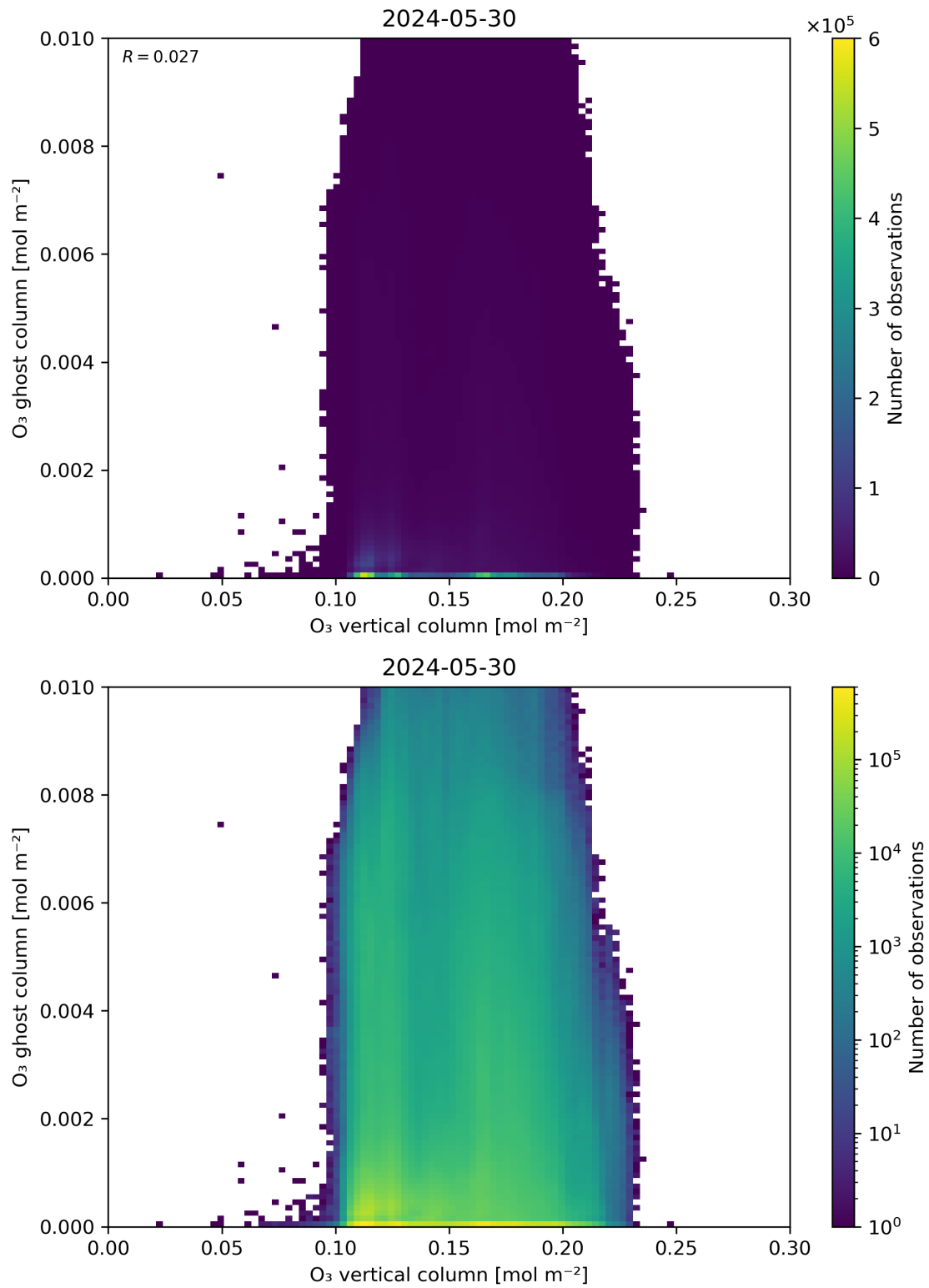
Figure 40: Scatter density plot of “ \text{O}_3 vertical column” against “ \text{O}_3 ghost column” for 2024-05-29 to 2024-05-31.
