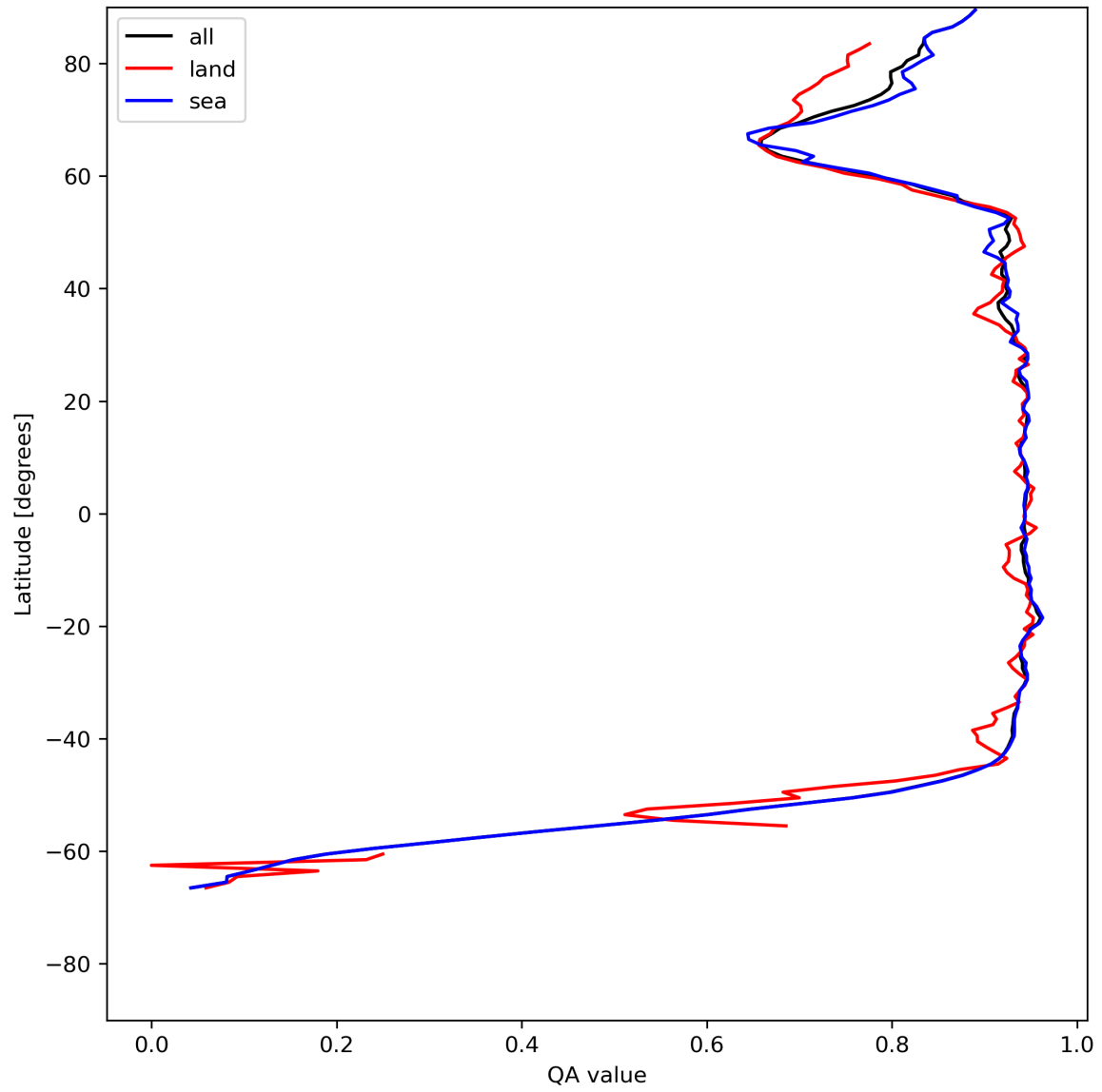
Figure 13: Zonal average of “QA value” for 2024-05-29 to 2024-05-31.
