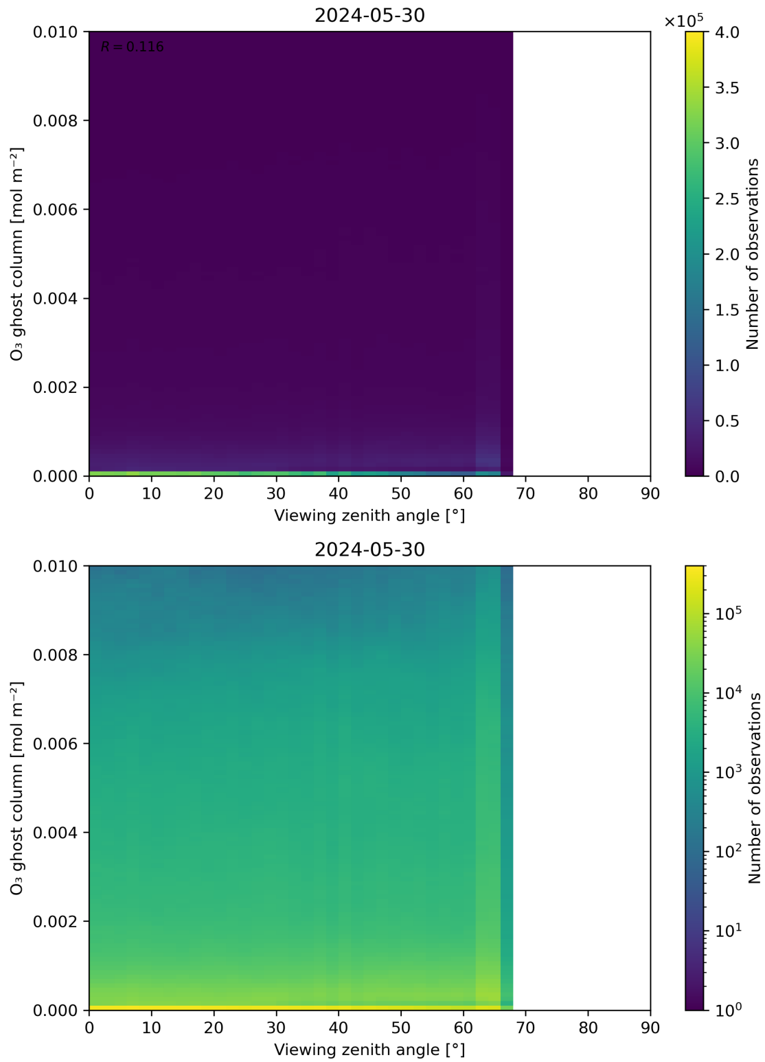
Figure 51: Scatter density plot of “Viewing zenith angle” against “O 3 ghost column” for 2024-05-29 to 2024-05-31.
