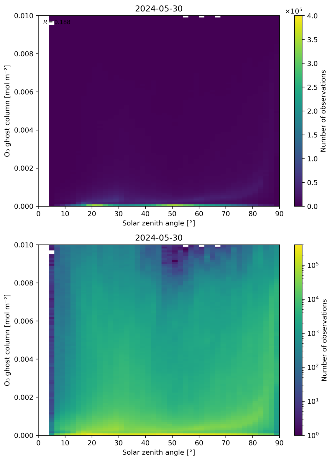
Figure 46: Scatter density plot of “Solar zenith angle” against “O 3 ghost column” for 2024-05-29 to 2024-05-31.
