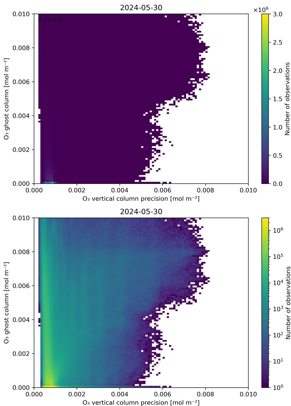
Figure 43: Scatter density plot of “ \text{O}_3 vertical column precision” against “ \text{O}_3 ghost column” for 2024-05-29 to 2024-05-31.
