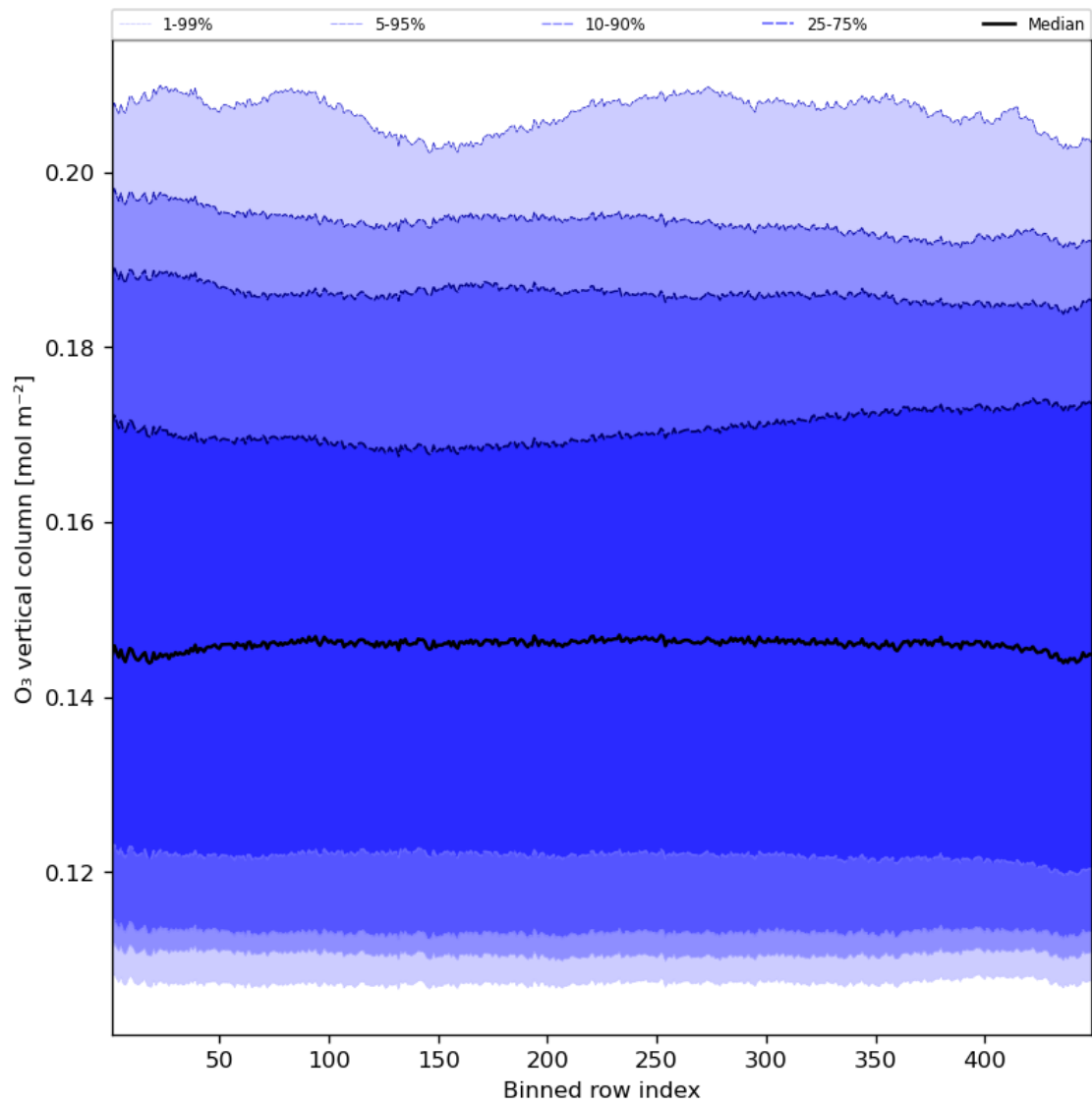
Figure 28: Along track statistics of “O 3 vertical column” for 2024-05-29 to 2024-05-31
