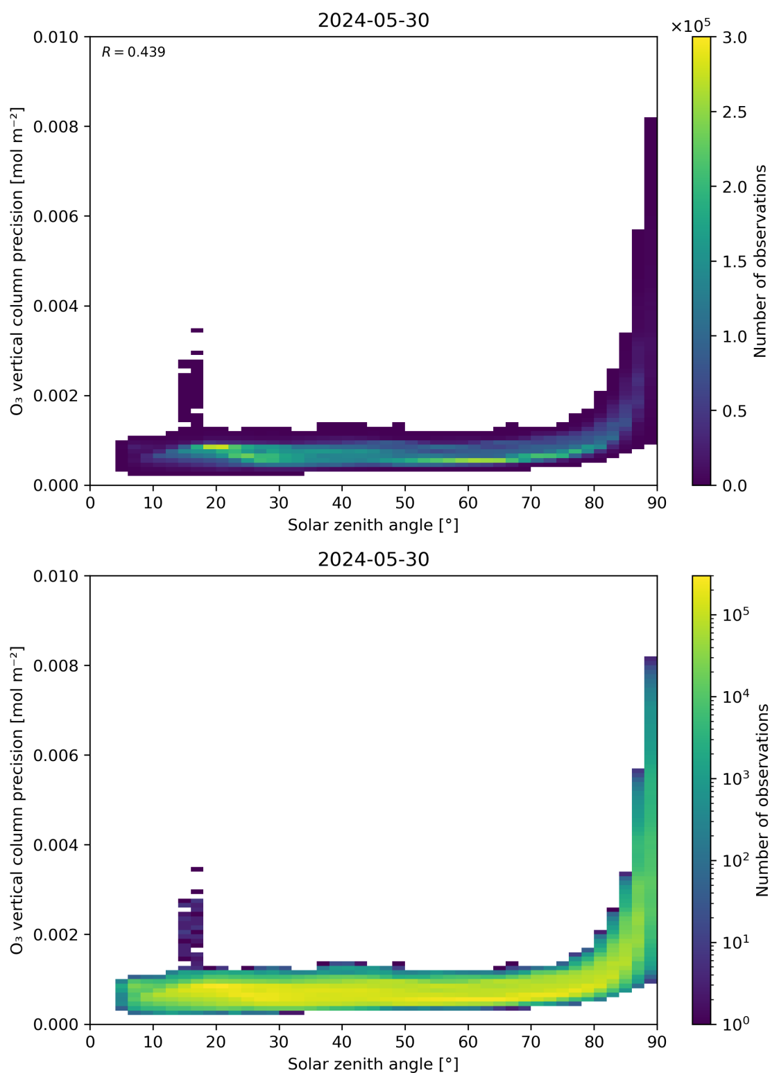
Figure 48: Scatter density plot of “Solar zenith angle” against “O 3 vertical column precision” for 2024-05-29 to 2024-05-31.
