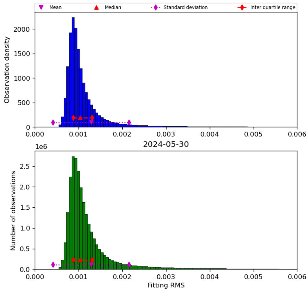
Figure 23: Histogram of “Fitting RMS” for 2024-05-29 to 2024-05-31
