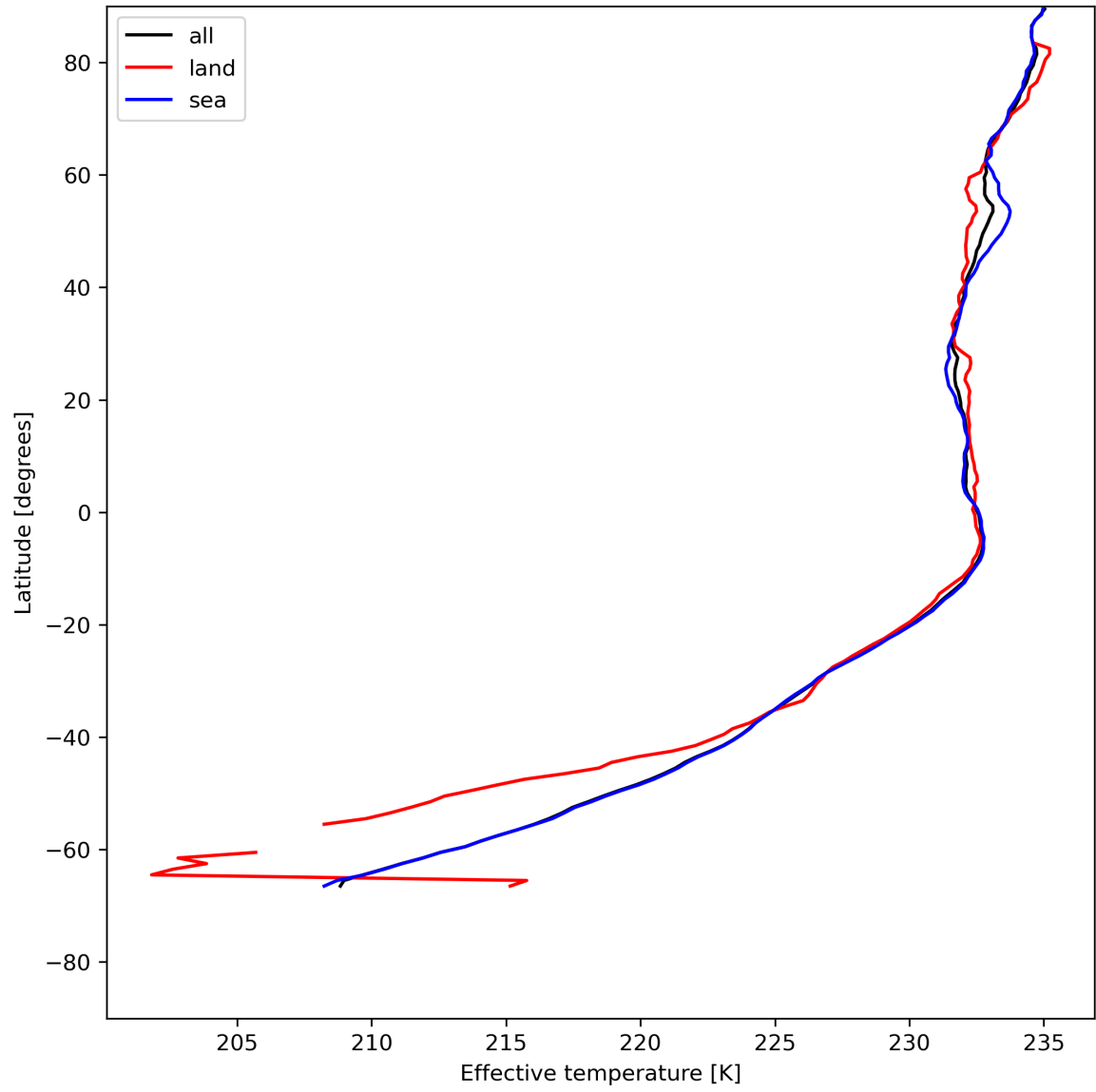
Figure 17: Zonal average of "Effective temperature" for 2024-05-29 to 2024-05-31.
