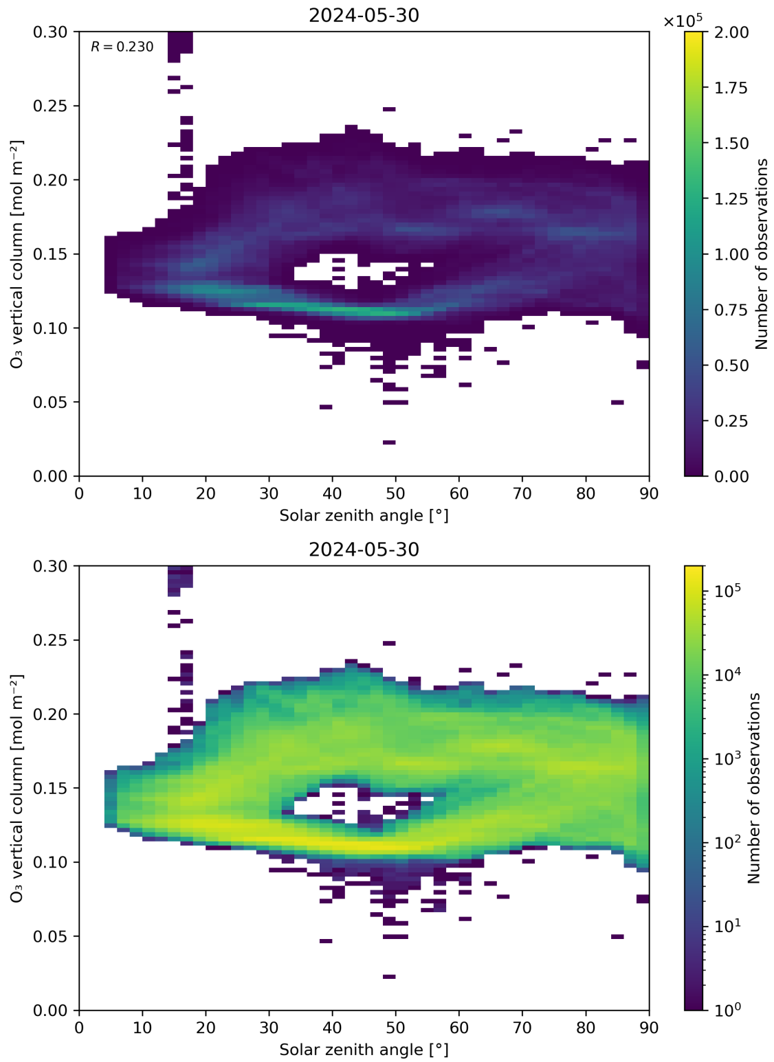
Figure 47: Scatter density plot of “Solar zenith angle” against “O 3 vertical column” for 2024-05-29 to 2024-05-31.
