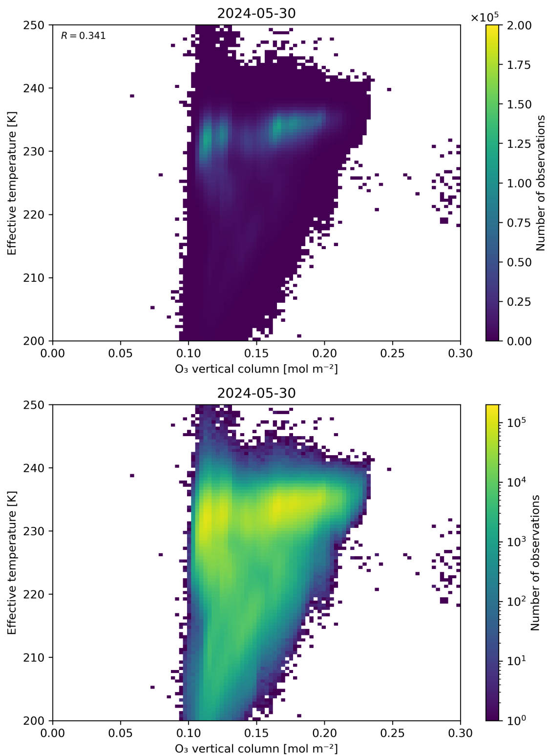
Figure 39: Scatter density plot of “O 3 vertical column” against “Effective temperature” for 2024-05-29 to 2024-05-31.
