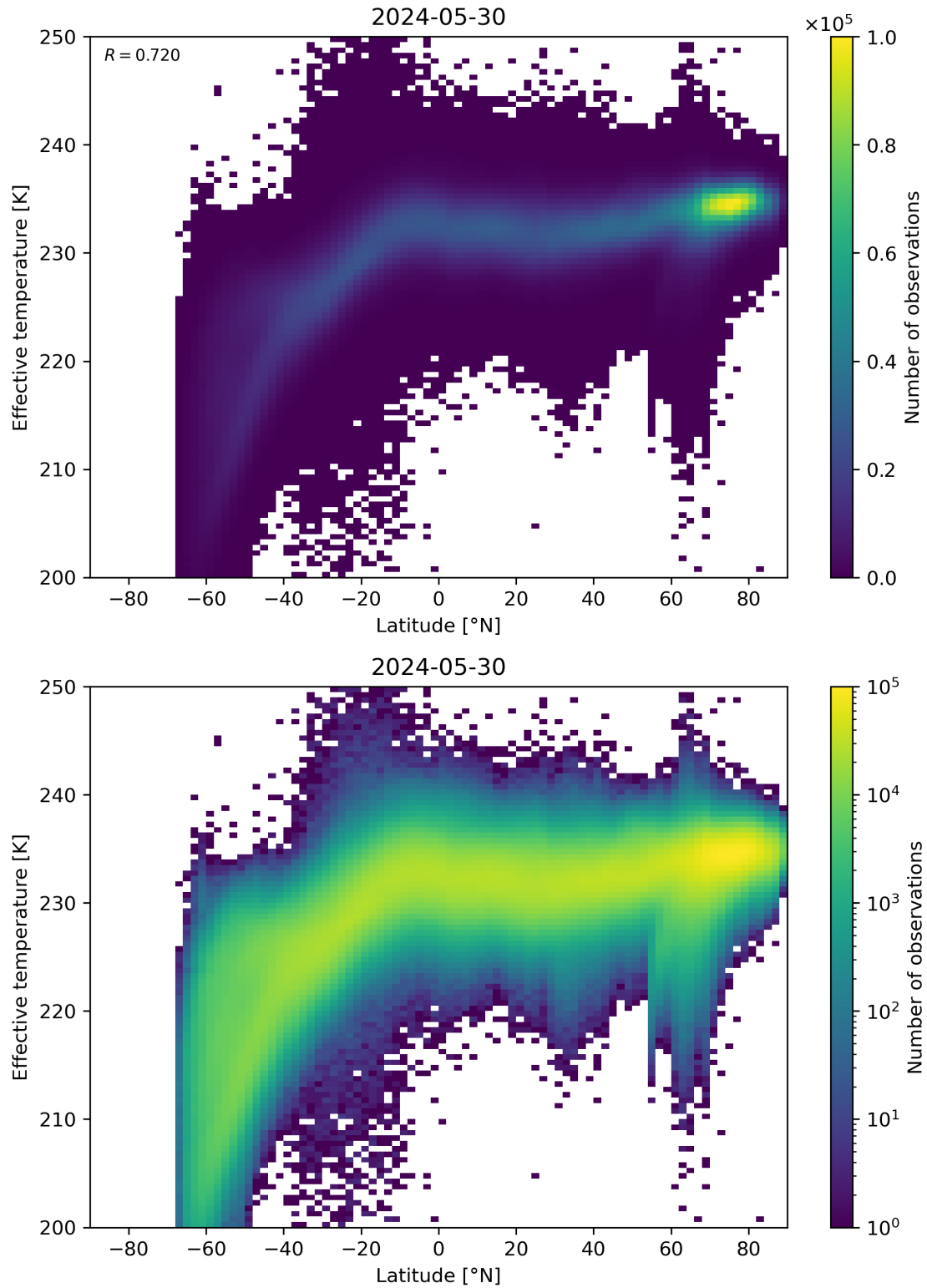
Figure 34: Scatter density plot of “Latitude” against “Effective temperature” for 2024-05-29 to 2024-05-31.
