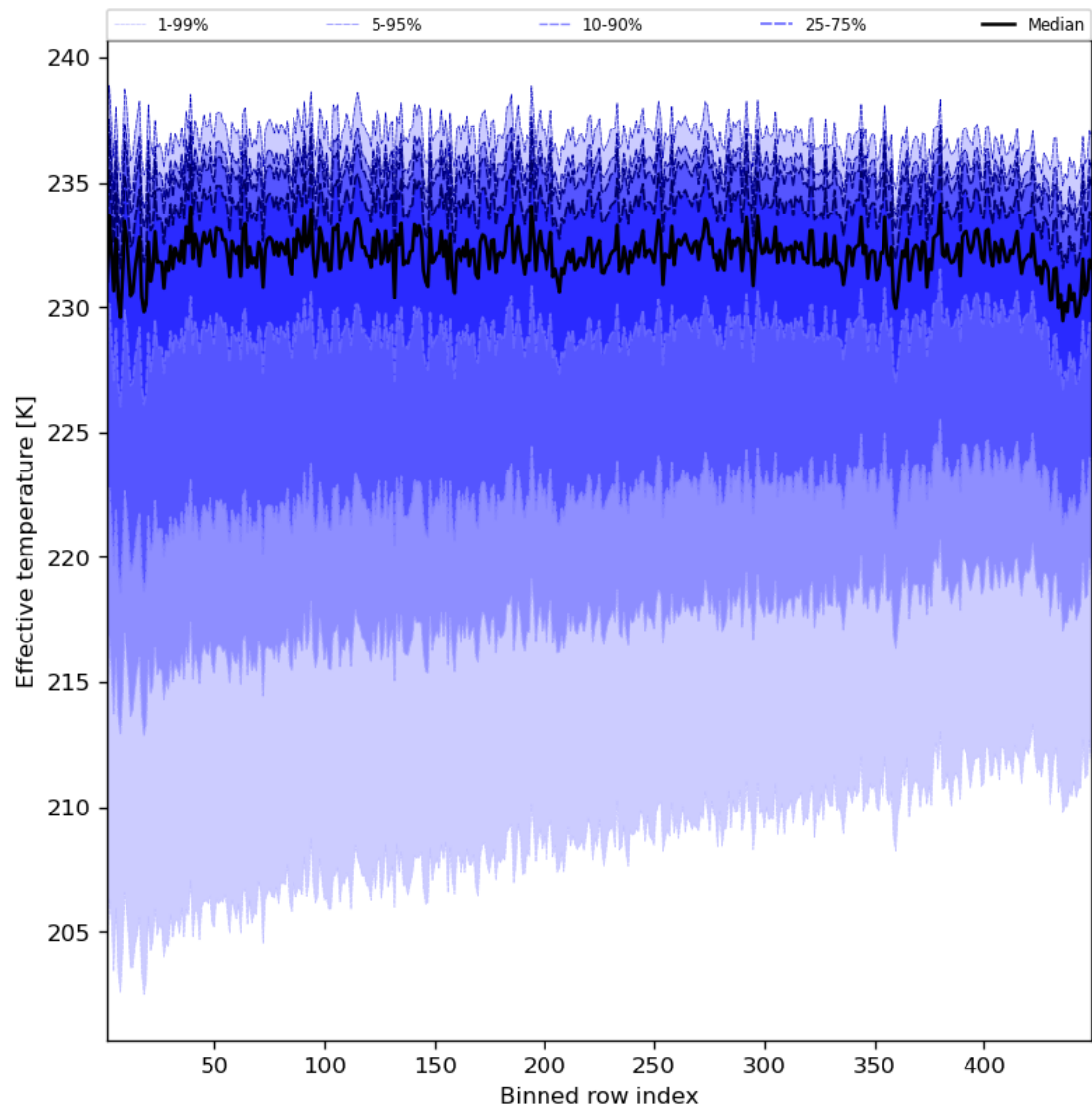
Figure 31: Along track statistics of “Effective temperature” for 2024-05-29 to 2024-05-31
