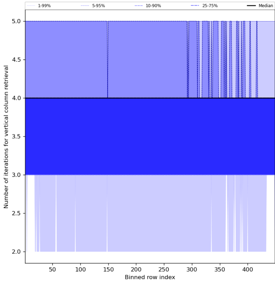
Figure 33: Along track statistics of “Number of iterations for vertical column retrieval” for 2024-05-29 to 2024-05-31
