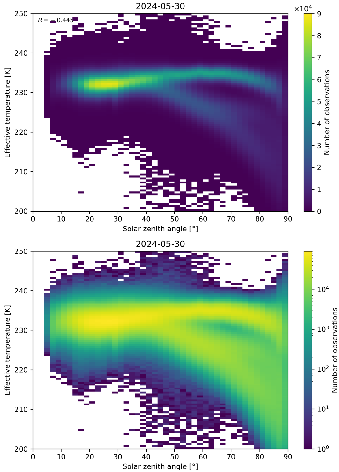
Figure 45: Scatter density plot of “Solar zenith angle” against “Effective temperature” for 2024-05-29 to 2024-05-31.
