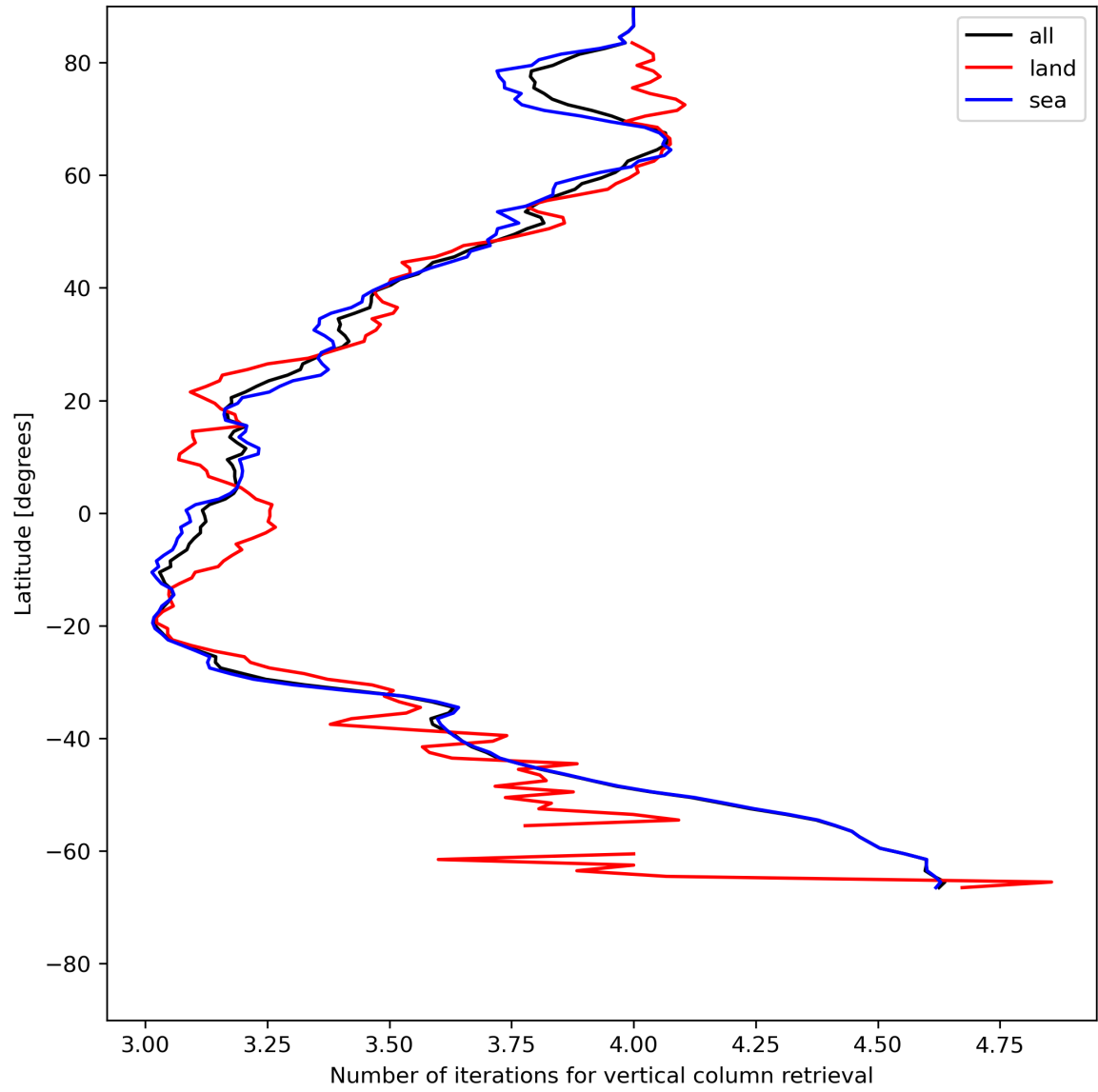
Figure 19: Zonal average of “Number of iterations for vertical column retrieval” for 2024-05-29 to 2024-05-31.
