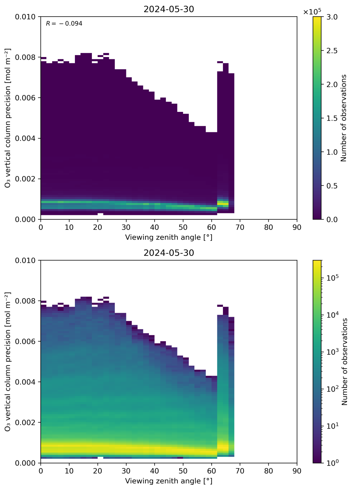
Figure 53: Scatter density plot of “Viewing zenith angle” against “O 3 vertical column precision” for 2024-05-29 to 2024-05-31.
