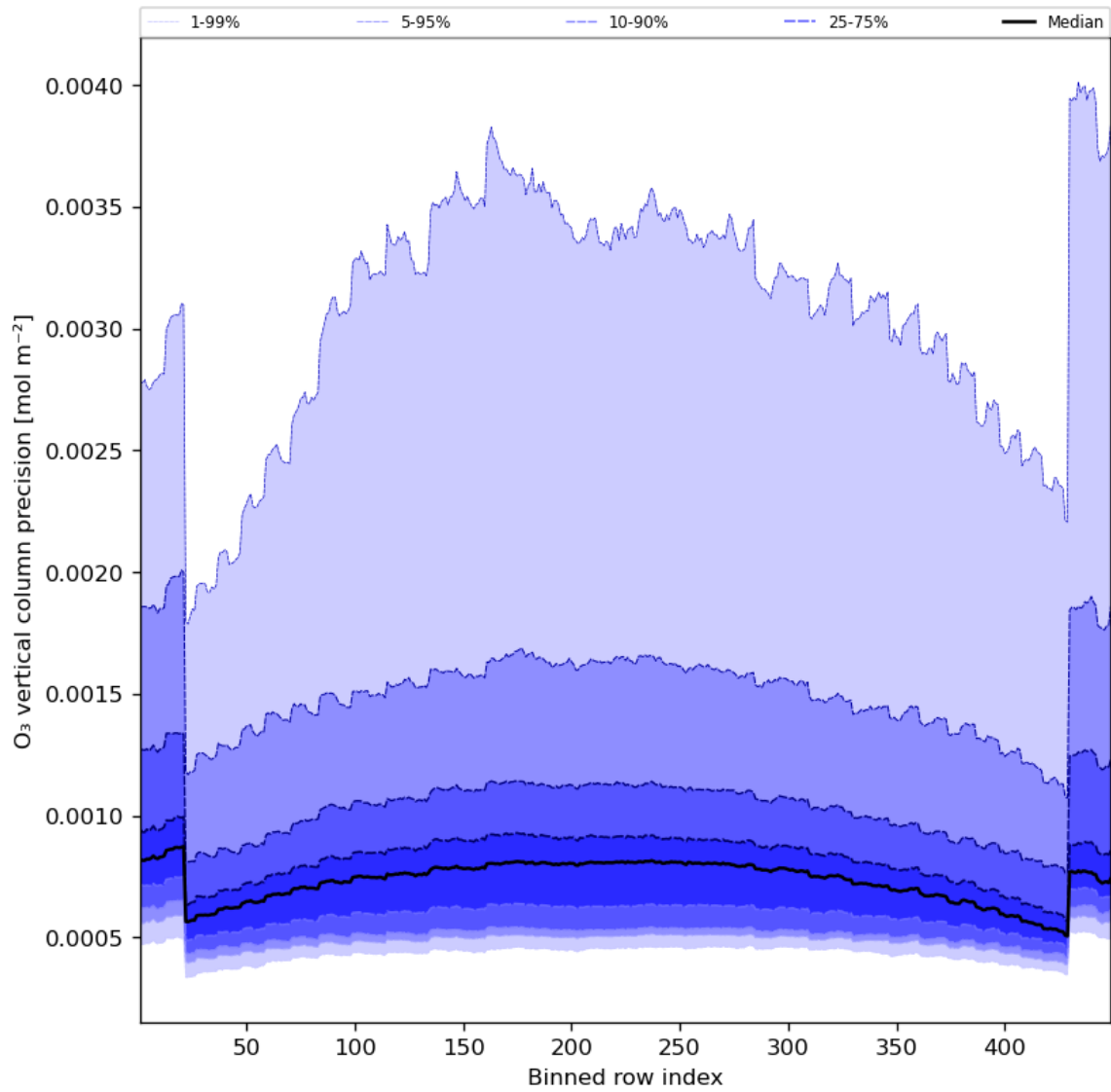
Figure 29: Along track statistics of “O 3 vertical column precision” for 2024-05-29 to 2024-05-31
