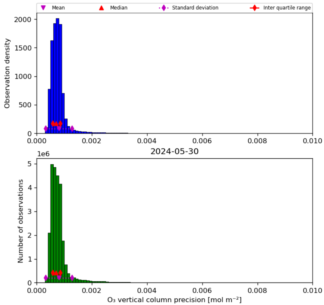
Figure 22: Histogram of “O 3 vertical column precision” for 2024-05-29 to 2024-05-31
