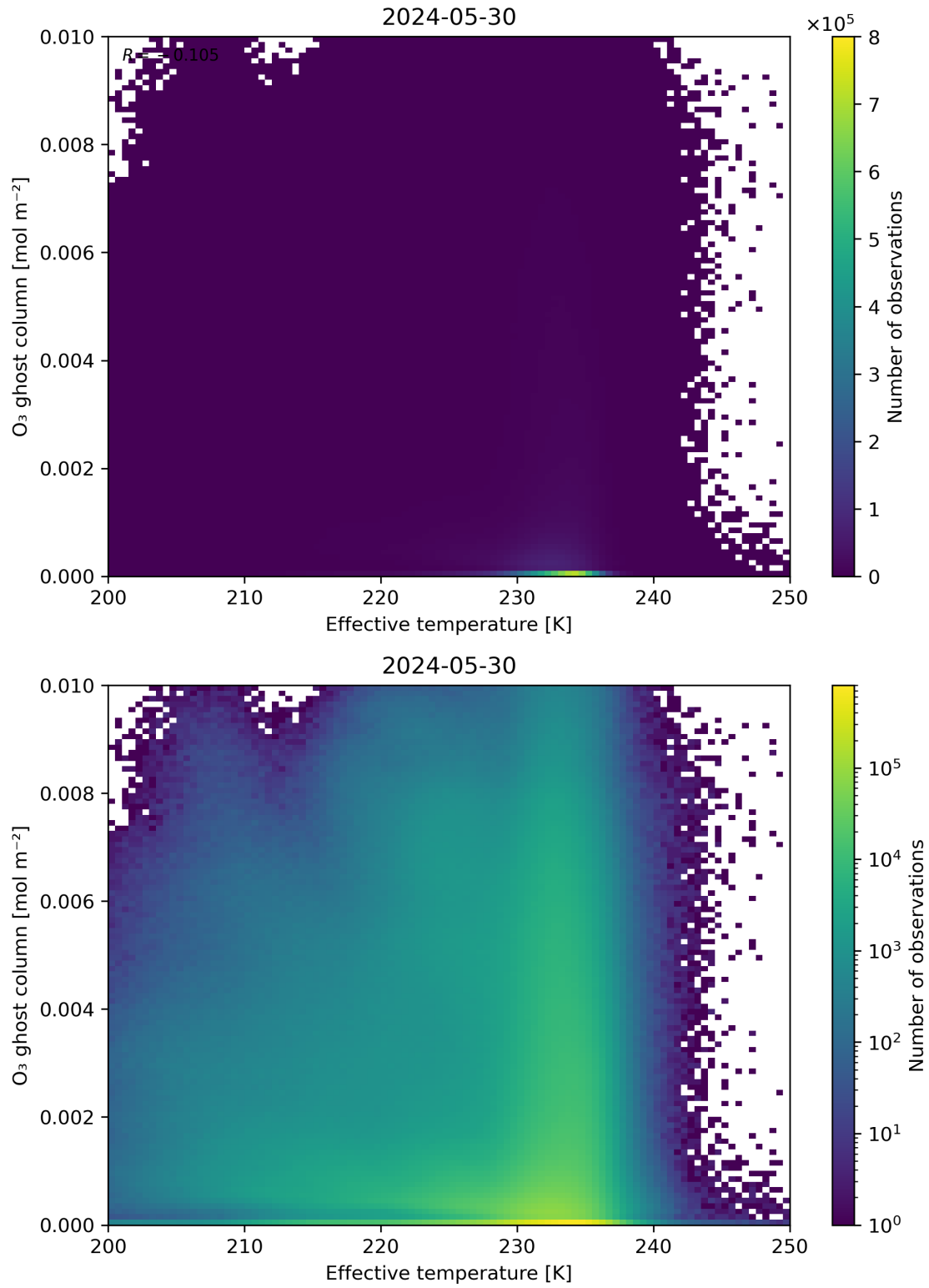
Figure 38: Scatter density plot of “Effective temperature” against “O 3 ghost column” for 2024-05-29 to 2024-05-31.
