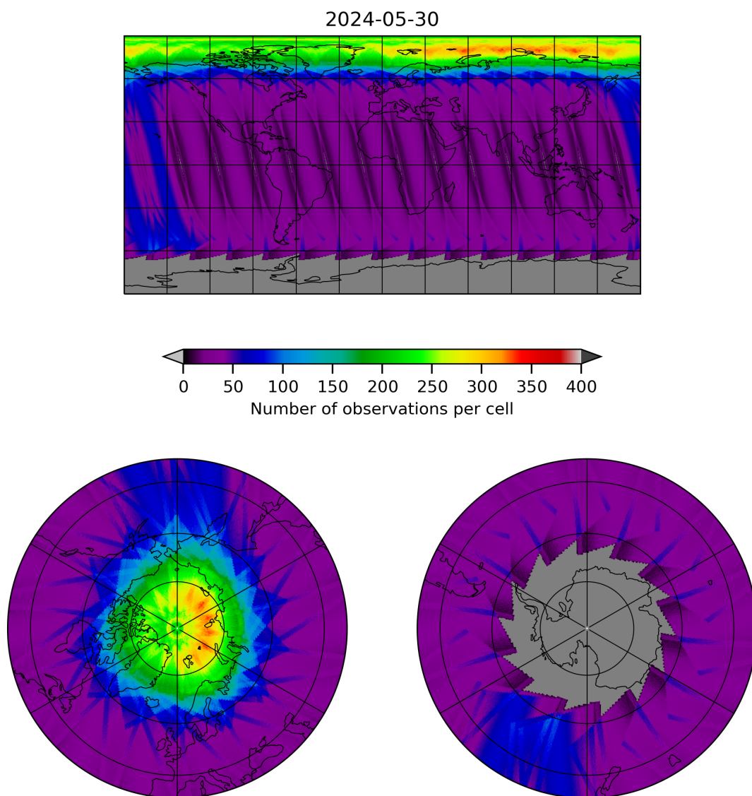
Figure 12: Map of the number of observations for 2024-05-29 to 2024-05-31
