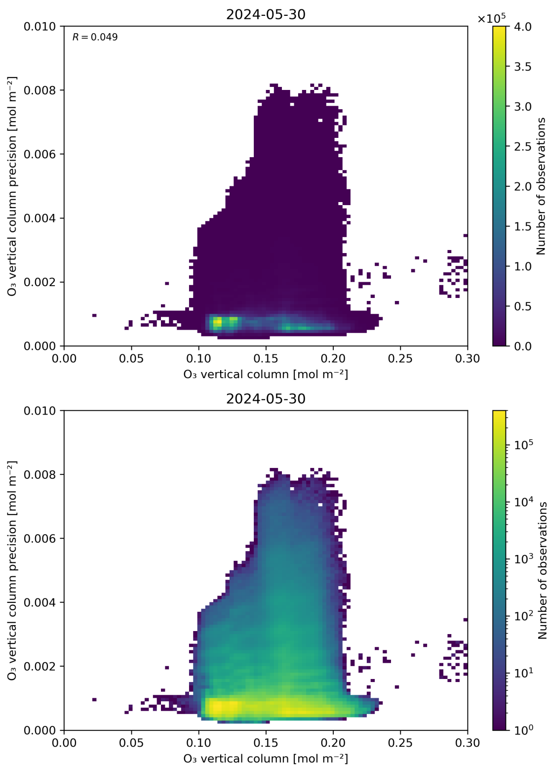
Figure 41: Scatter density plot of “O 3 vertical column” against “O 3 vertical column precision” for 2024-05-29 to 2024-05-31.
