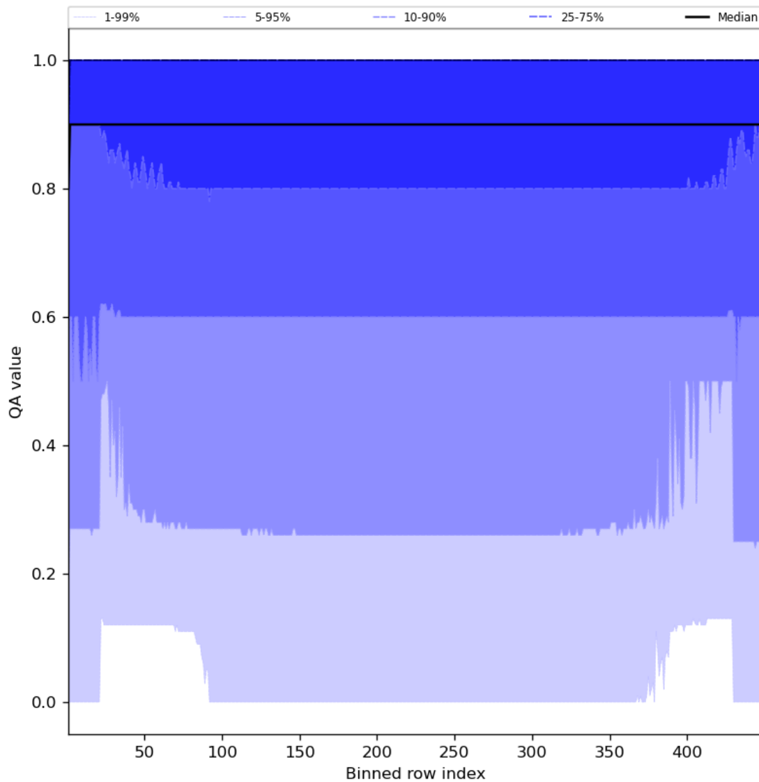
Figure 27: Along track statistics of “QA value” for 2024-05-29 to 2024-05-31
