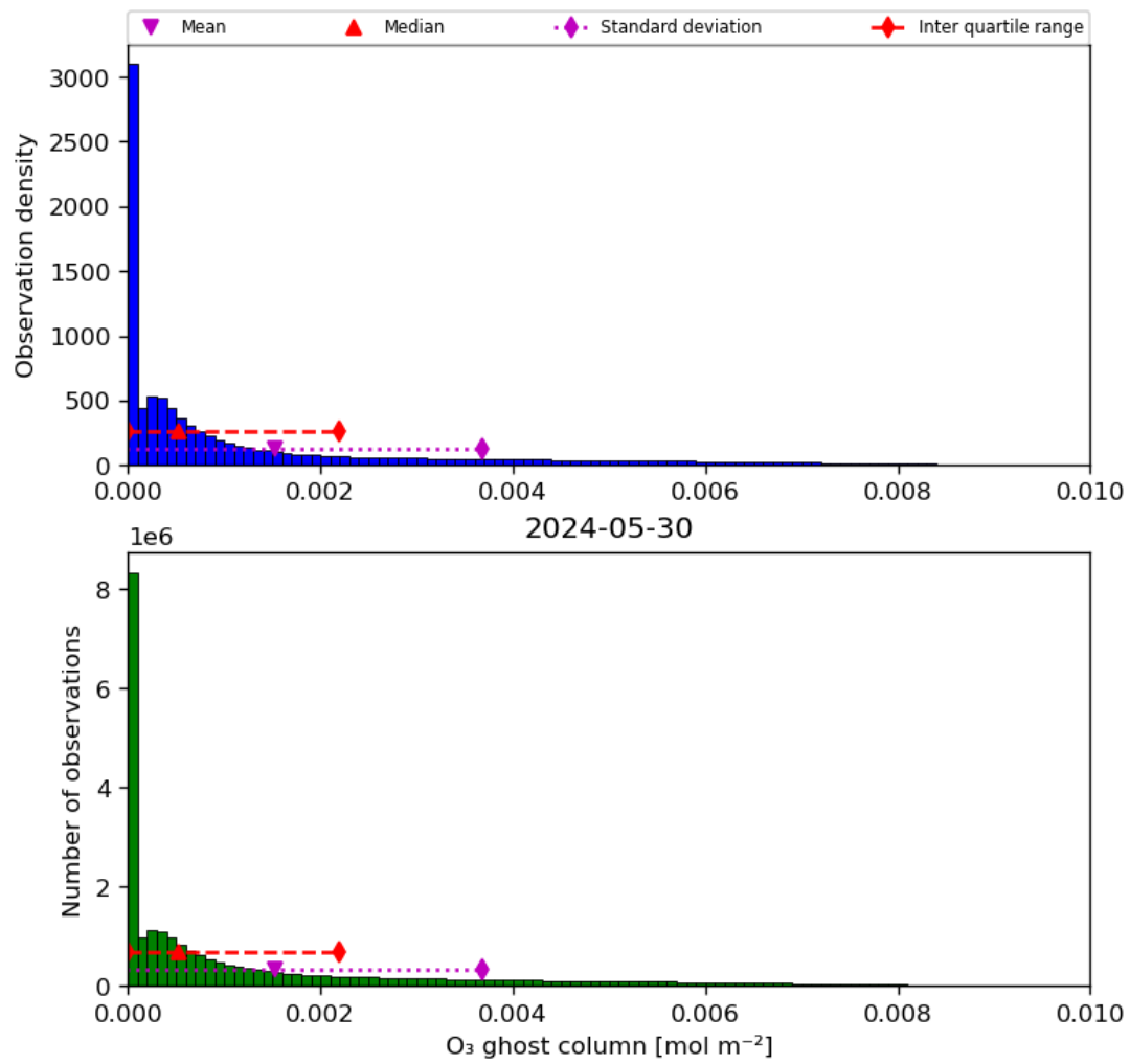
Figure 25: Histogram of “O 3 ghost column” for 2024-05-29 to 2024-05-31
