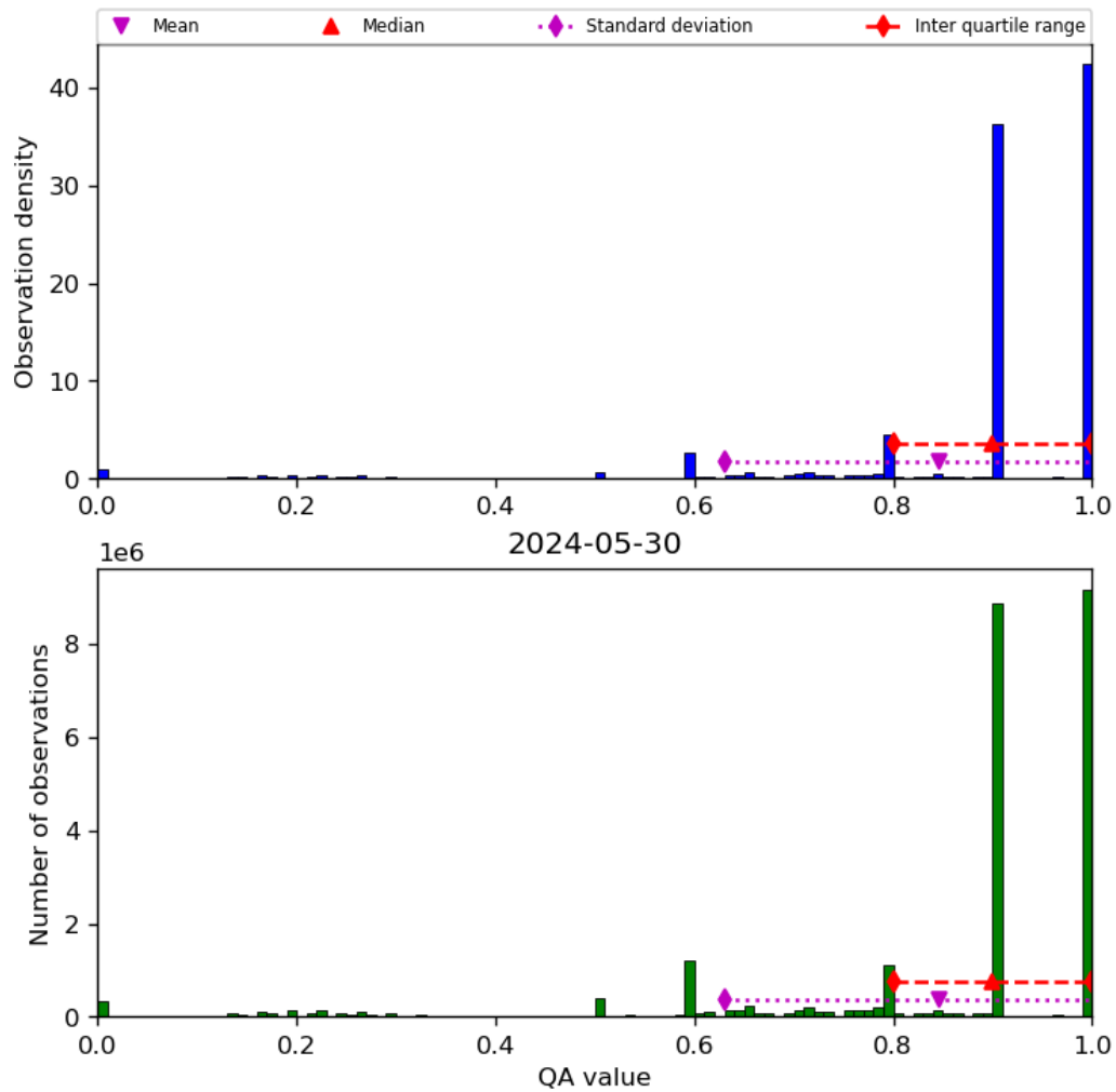
Figure 20: Histogram of “QA value” for 2024-05-29 to 2024-05-31
