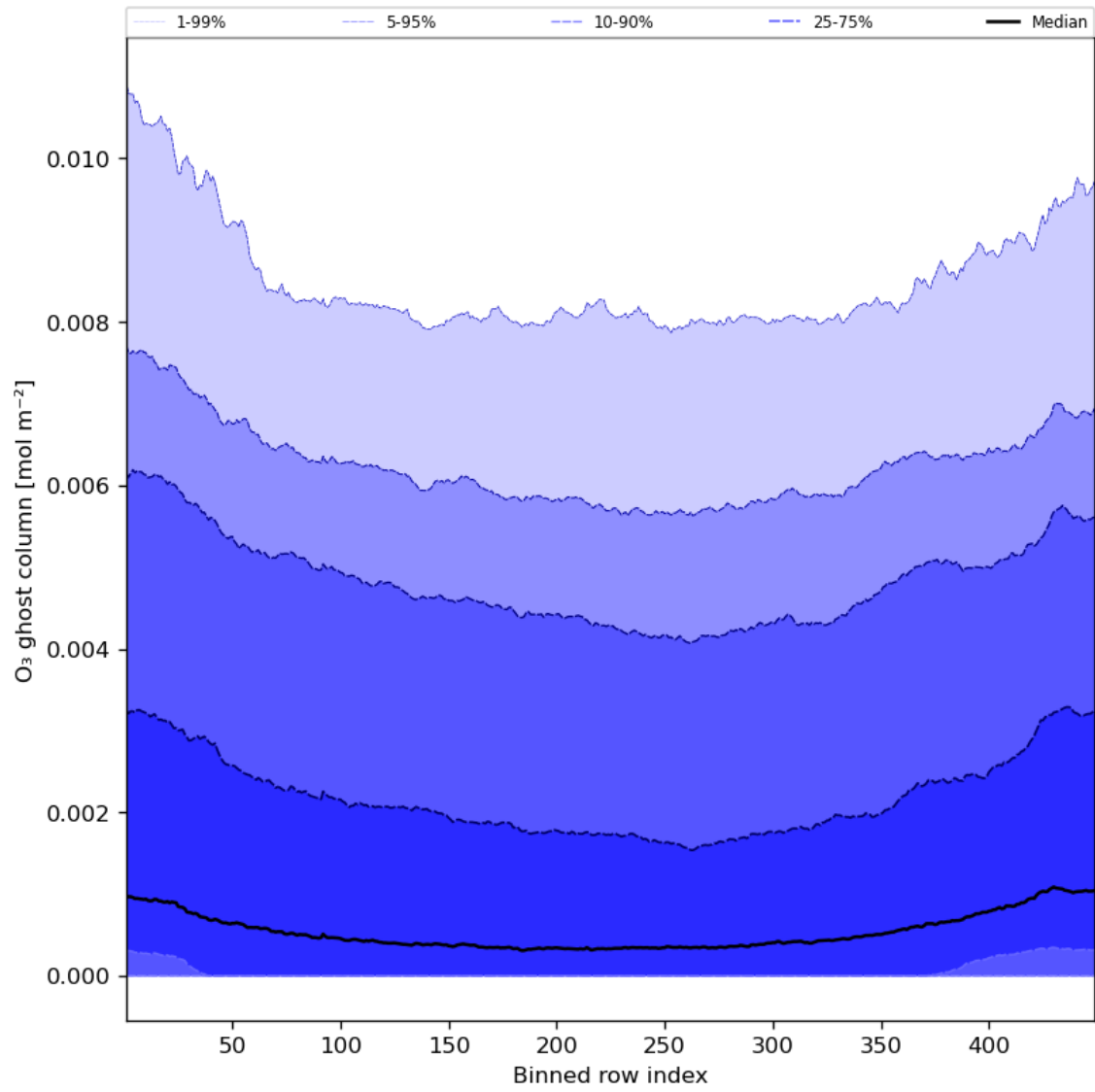
Figure 32: Along track statistics of "O 3 ghost column" for 2024-05-29 to 2024-05-31
