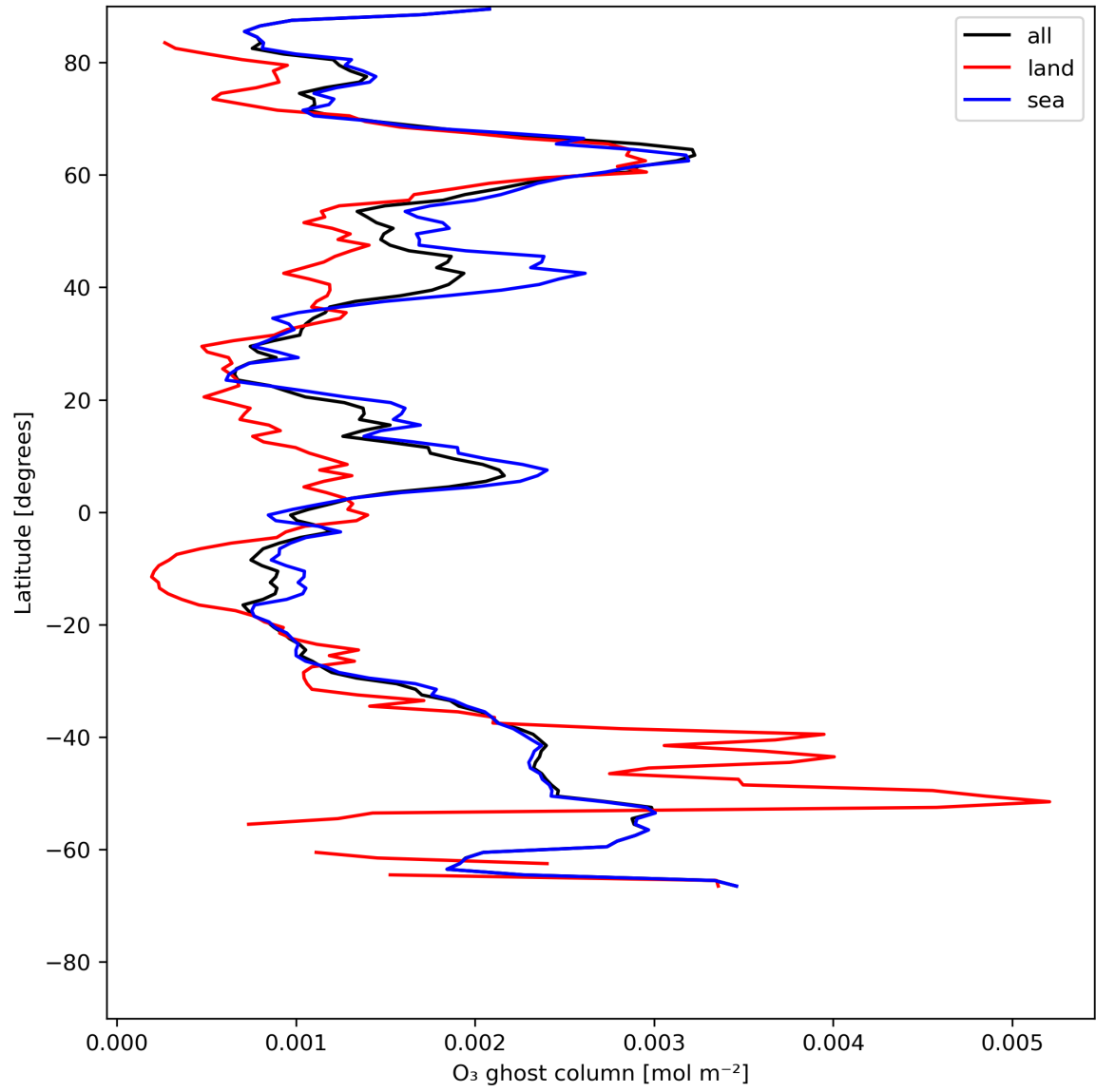
Figure 18: Zonal average of "O 3 ghost column" for 2024-05-30 to 2024-06-01.
