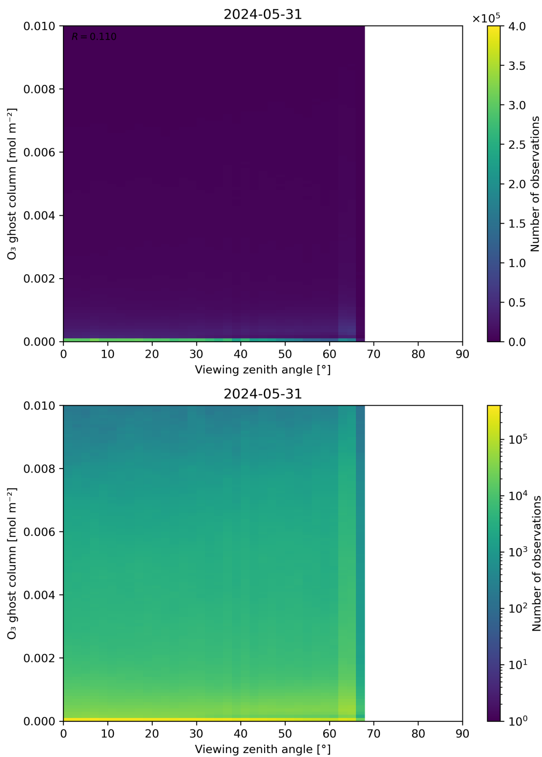
Figure 51: Scatter density plot of “Viewing zenith angle” against “O 3 ghost column” for 2024-05-30 to 2024-06-01.
