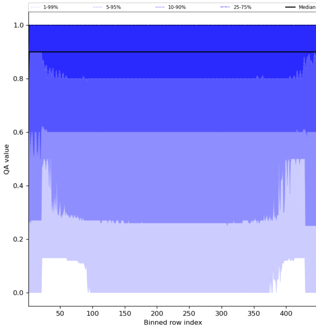
Figure 27: Along track statistics of “QA value” for 2024-05-30 to 2024-06-01
