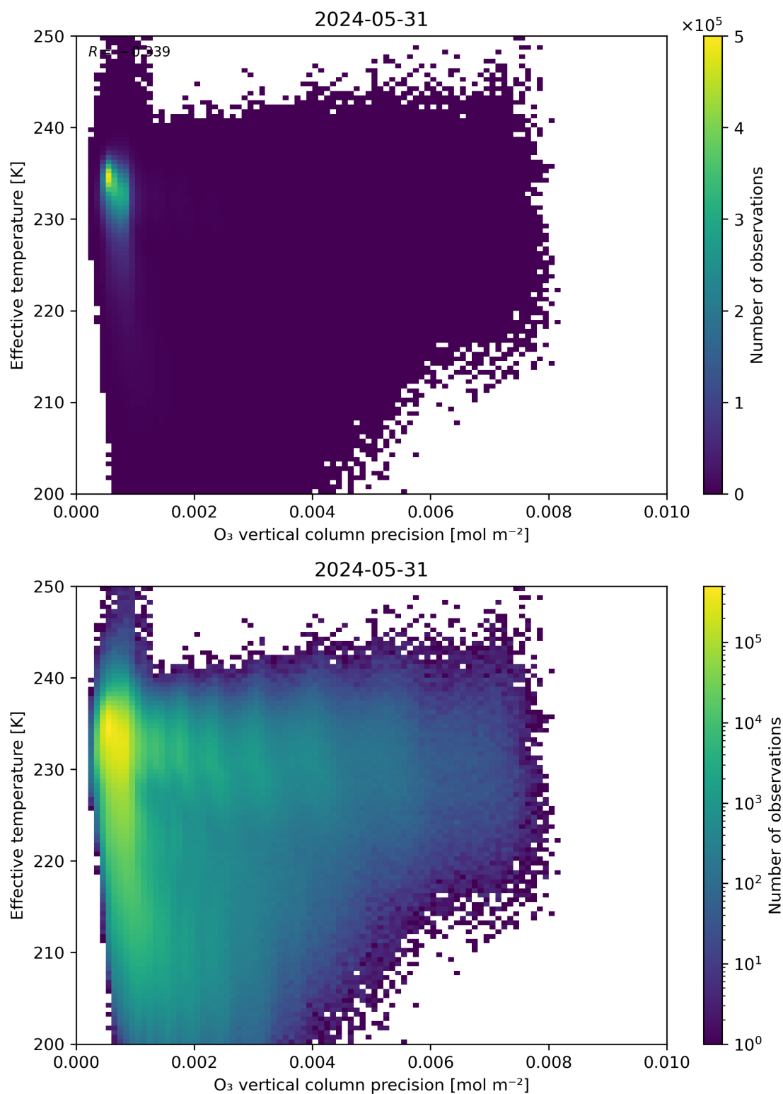
Figure 42: Scatter density plot of “O 3 vertical column precision” against “Effective temperature” for 2024-05-30 to 2024-06-01.
