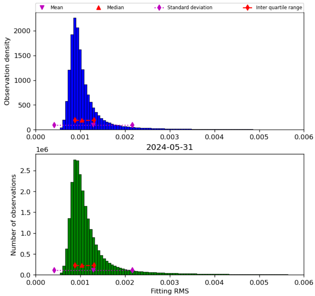
Figure 23: Histogram of “Fitting RMS” for 2024-05-30 to 2024-06-01
