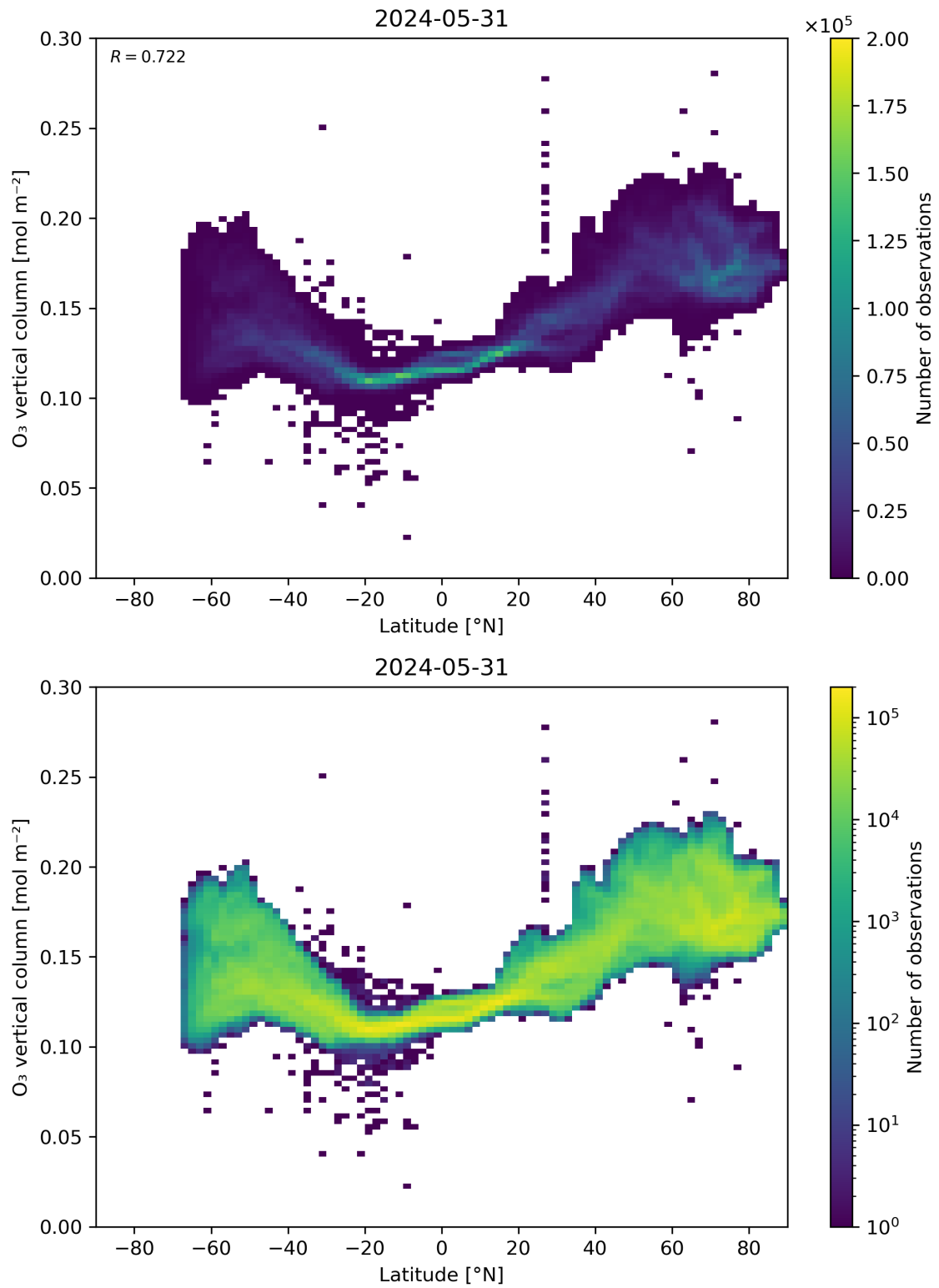
Figure 36: Scatter density plot of “Latitude” against “O 3 vertical column” for 2024-05-30 to 2024-06-01.
