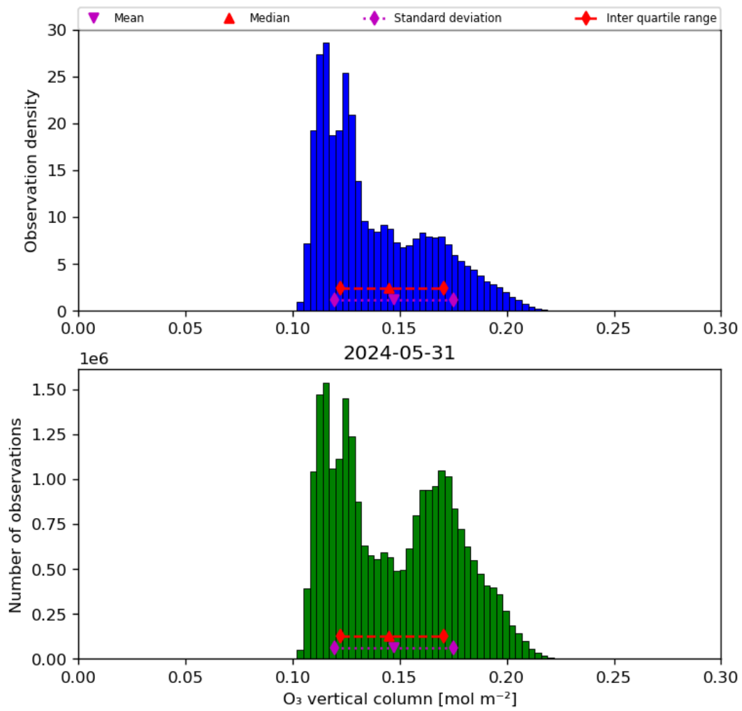
Figure 21: Histogram of “O 3 vertical column” for 2024-05-30 to 2024-06-01
