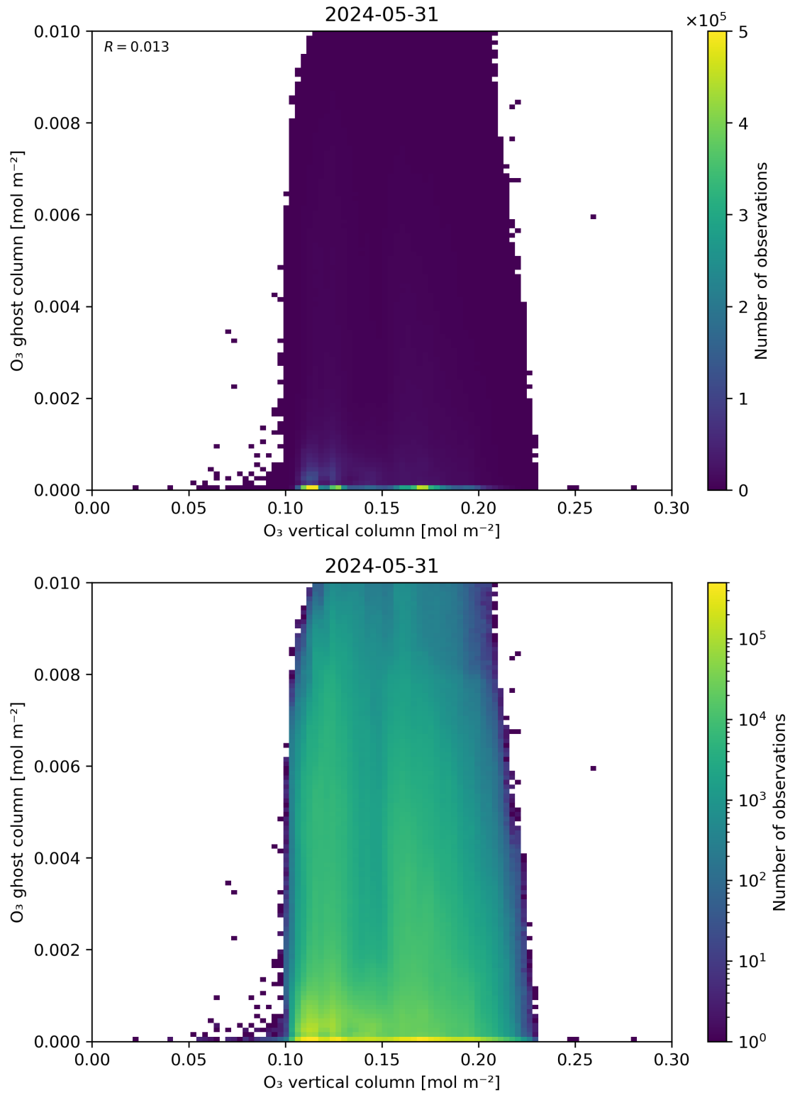
Figure 40: Scatter density plot of “O 3 vertical column” against “O 3 ghost column” for 2024-05-30 to 2024-06-01.
