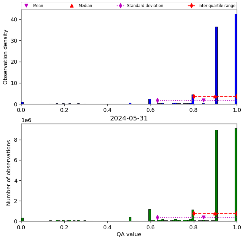
Figure 20: Histogram of “QA value” for 2024-05-30 to 2024-06-01
