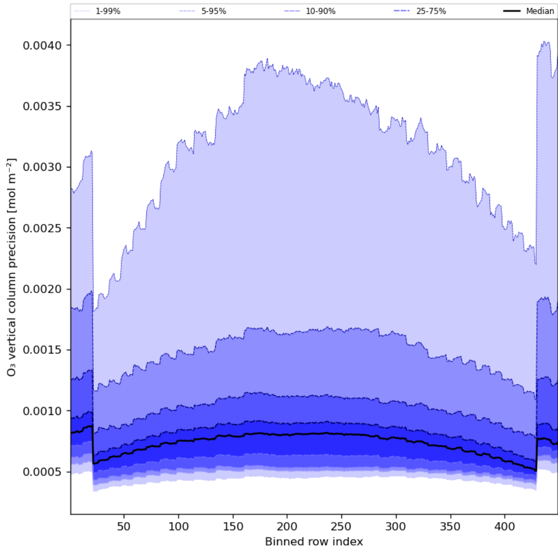
Figure 29: Along track statistics of “O 3 vertical column precision” for 2024-05-30 to 2024-06-01
