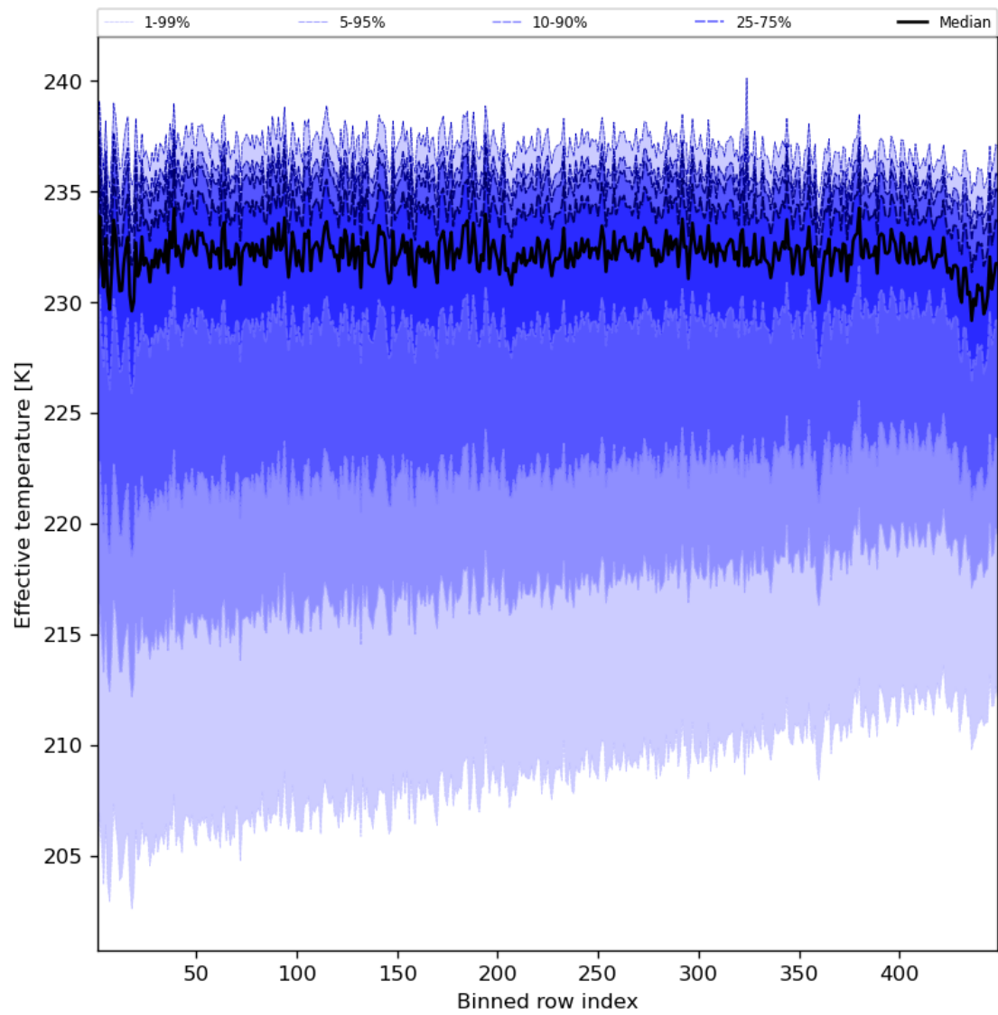
Figure 31: Along track statistics of “Effective temperature” for 2024-05-30 to 2024-06-01
