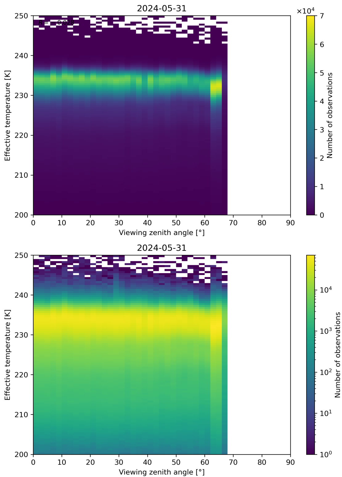
Figure 50: Scatter density plot of “Viewing zenith angle” against “Effective temperature” for 2024-05-30 to 2024-06-01.
