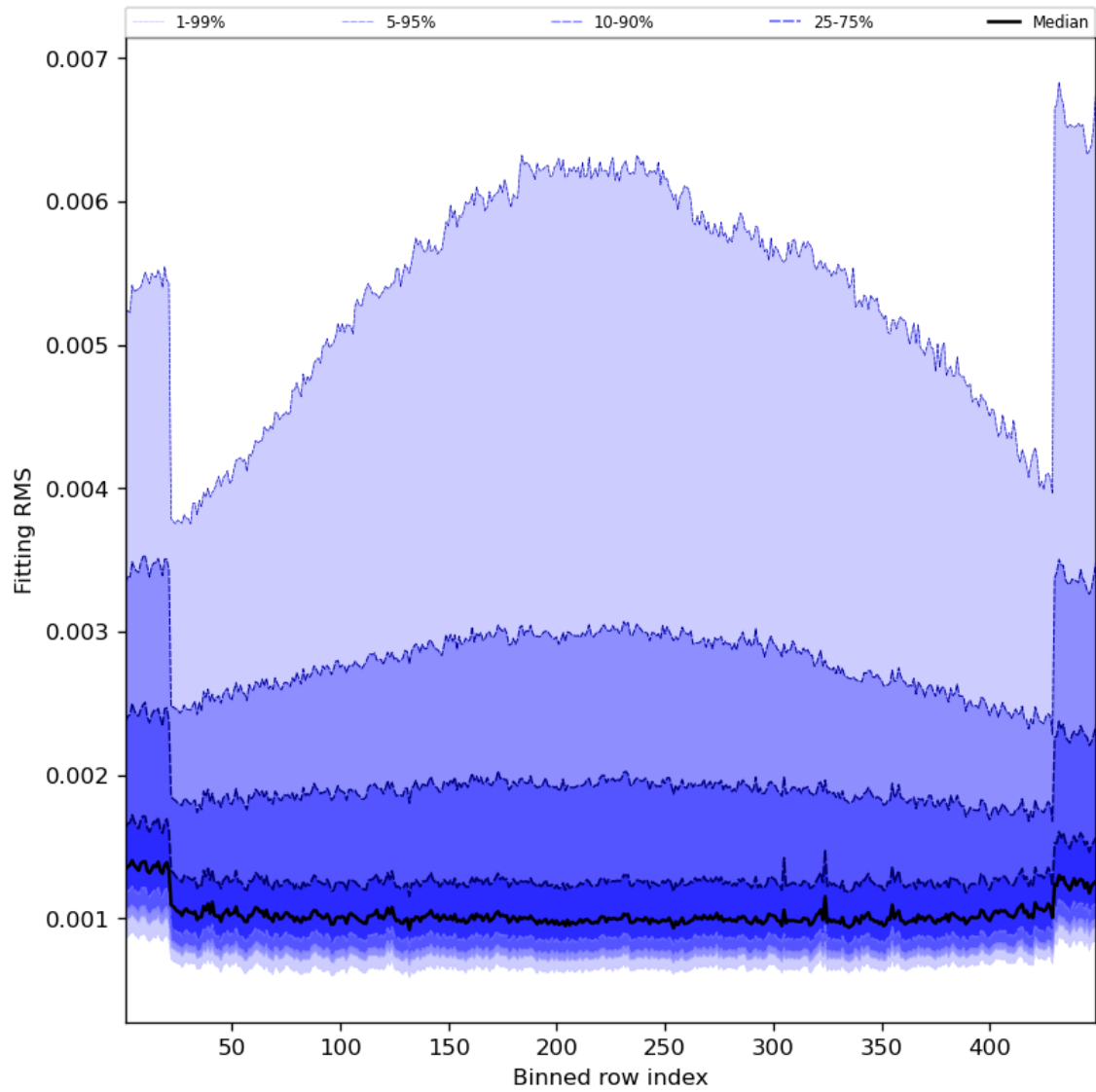
Figure 30: Along track statistics of “Fitting RMS” for 2024-05-30 to 2024-06-01
