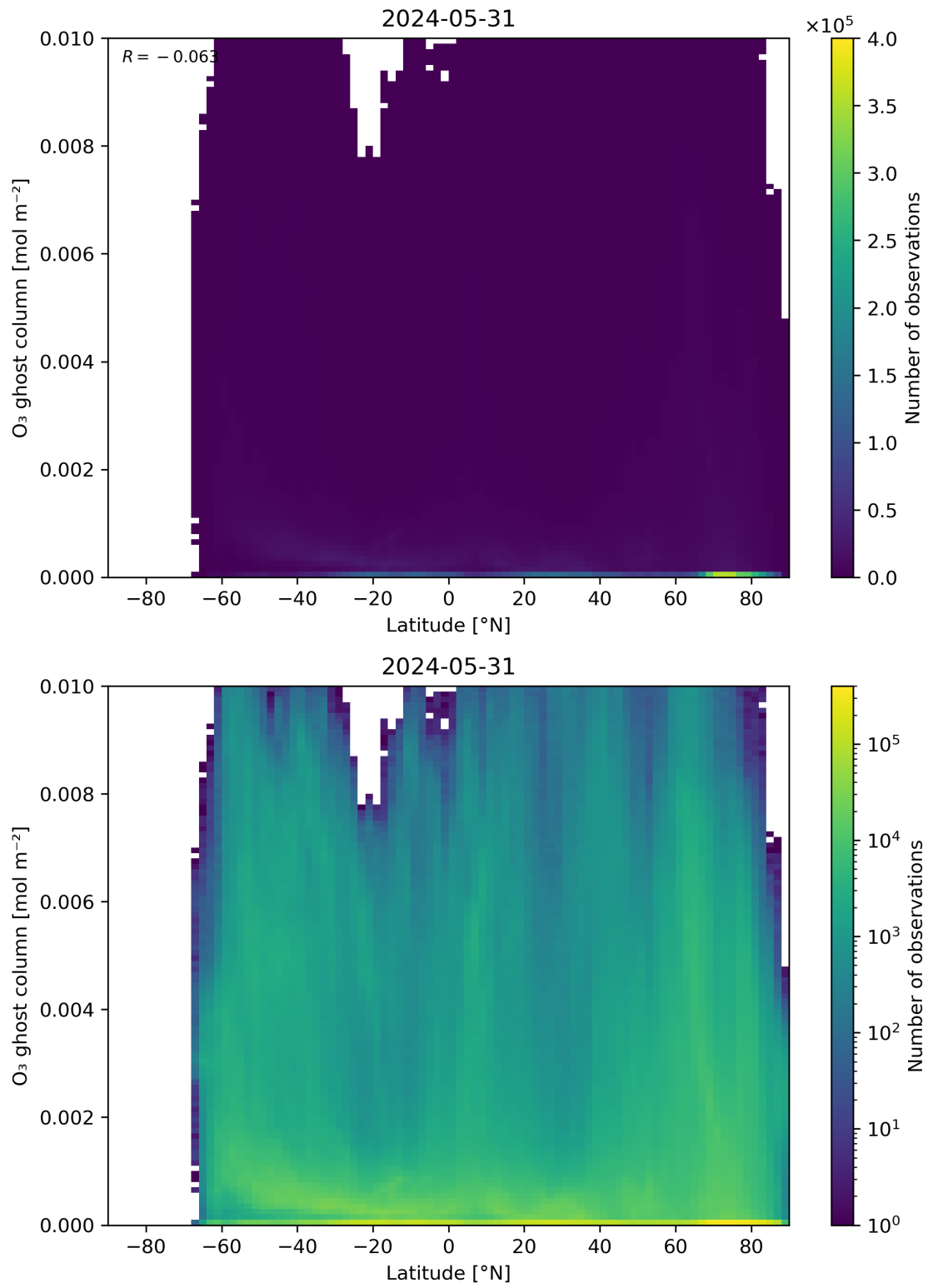
Figure 35: Scatter density plot of “Latitude” against “O 3 ghost column” for 2024-05-30 to 2024-06-01.
