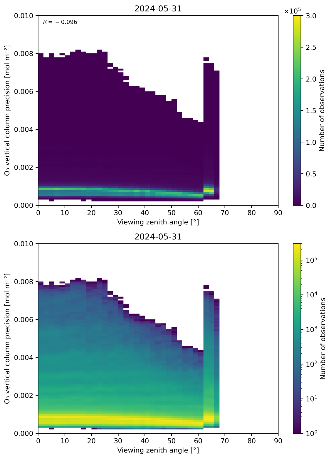
Figure 53: Scatter density plot of “Viewing zenith angle” against “O 3 vertical column precision” for 2024-05-30 to 2024-06-01.
