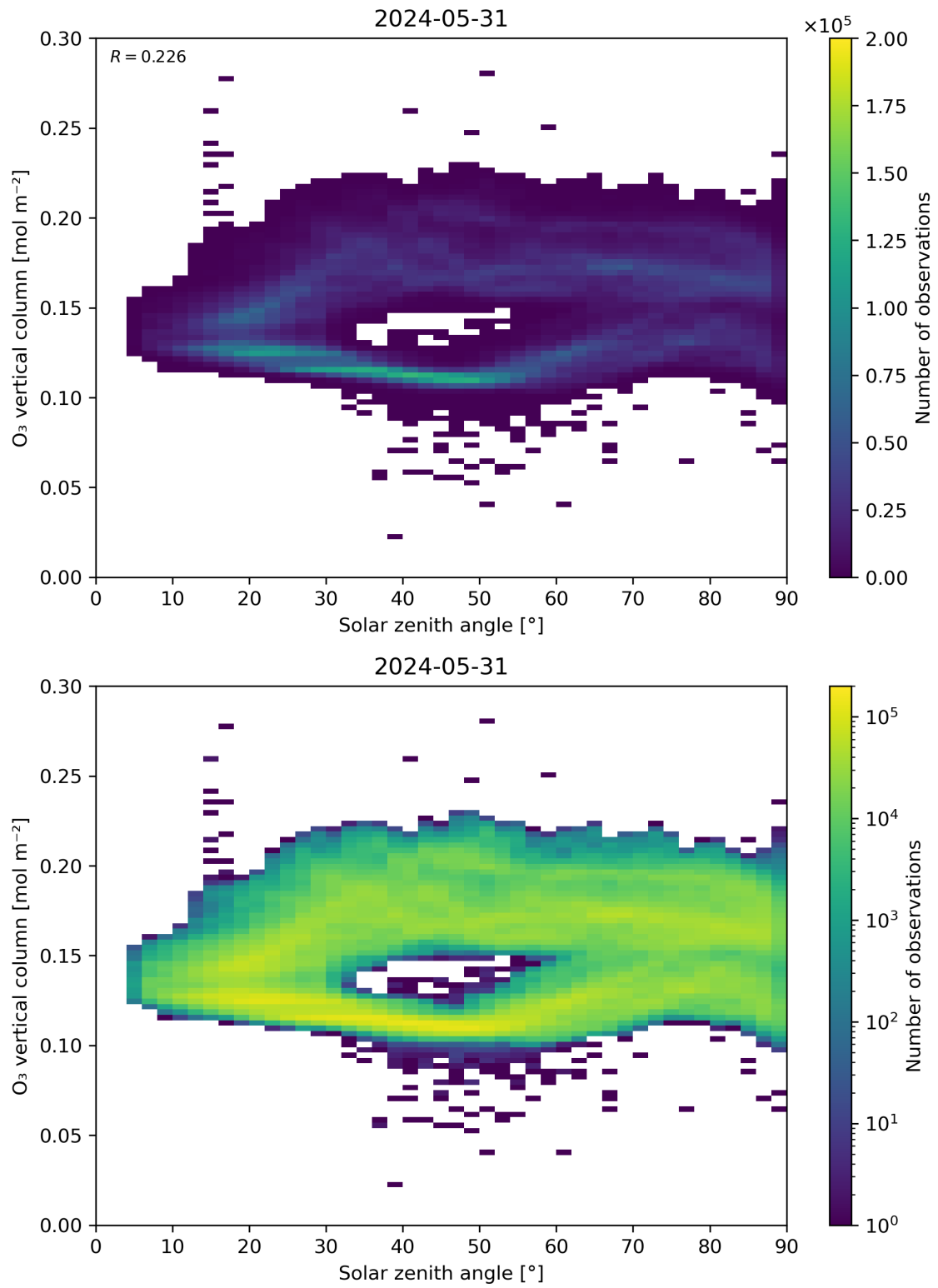
Figure 47: Scatter density plot of “Solar zenith angle” against “O 3 vertical column” for 2024-05-30 to 2024-06-01.
