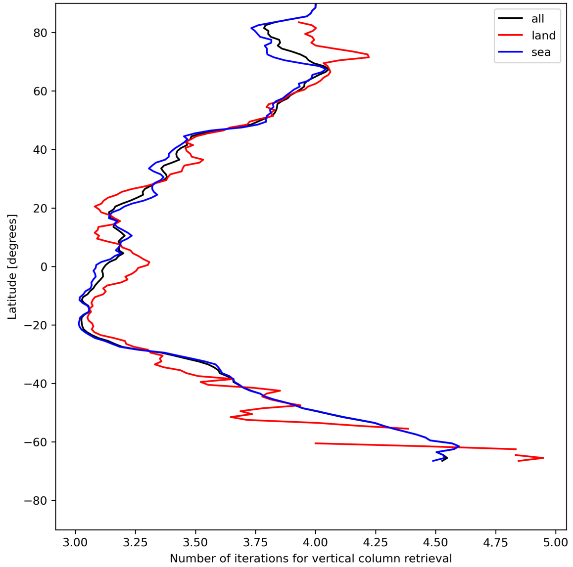
Figure 19: Zonal average of “Number of iterations for vertical column retrieval” for 2024-05-30 to 2024-06-01.
