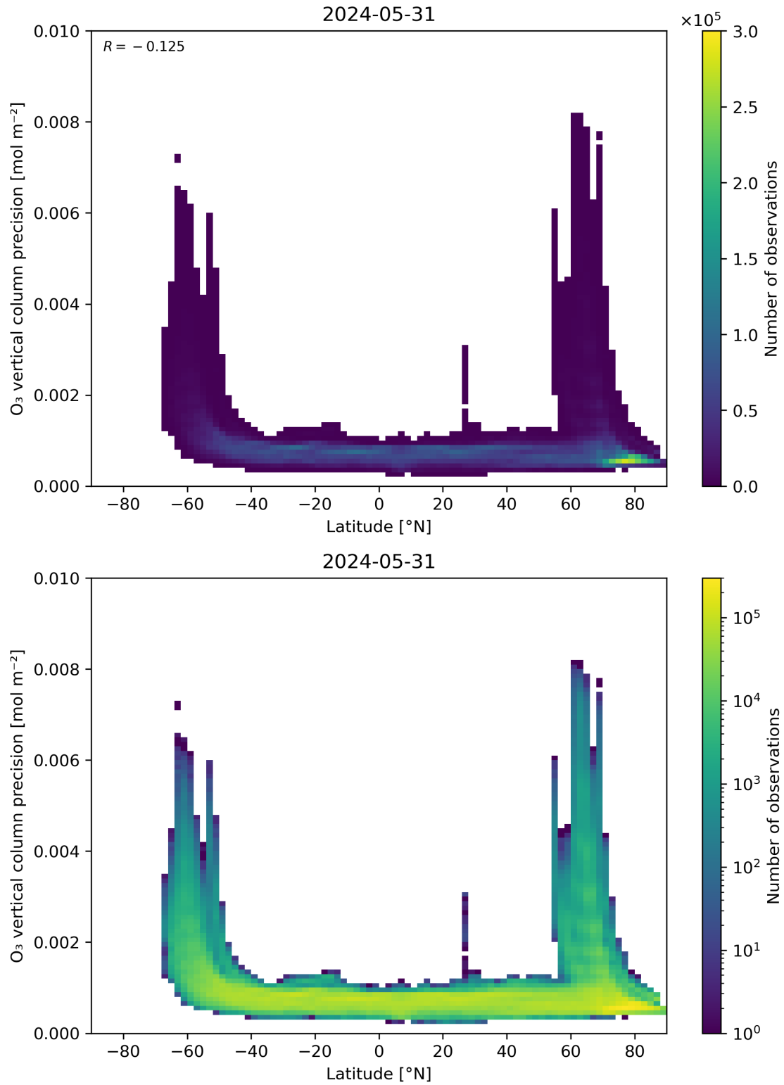
Figure 37: Scatter density plot of “Latitude” against “O 3 vertical column precision” for 2024-05-30 to 2024-06-01.
