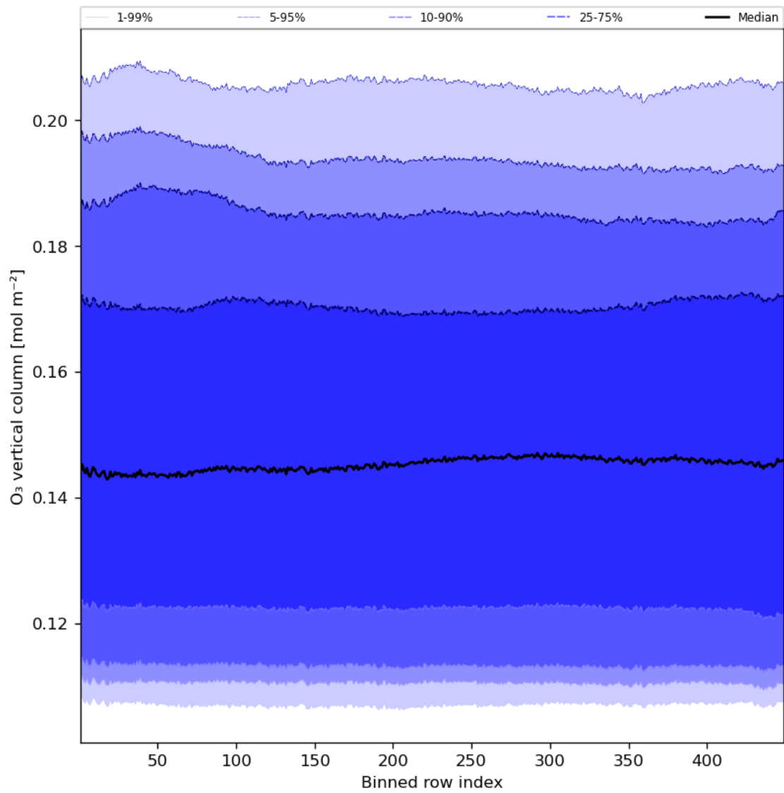
Figure 28: Along track statistics of “O 3 vertical column” for 2024-05-30 to 2024-06-01
