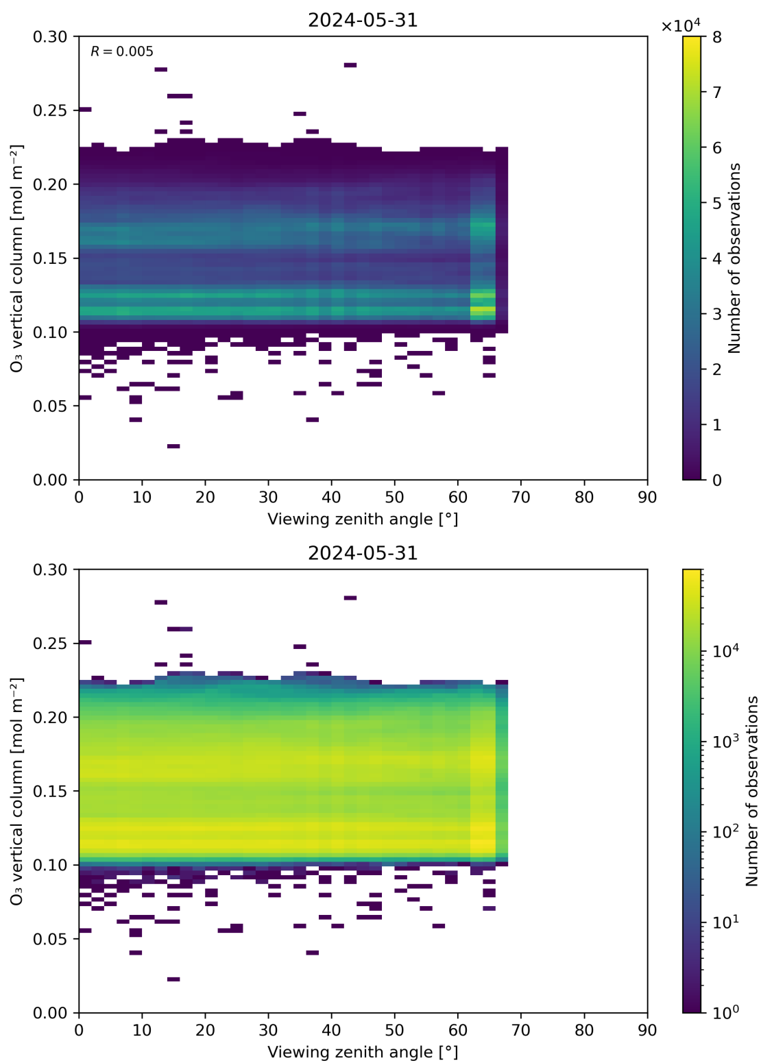
Figure 52: Scatter density plot of “Viewing zenith angle” against “O 3 vertical column” for 2024-05-30 to 2024-06-01.
