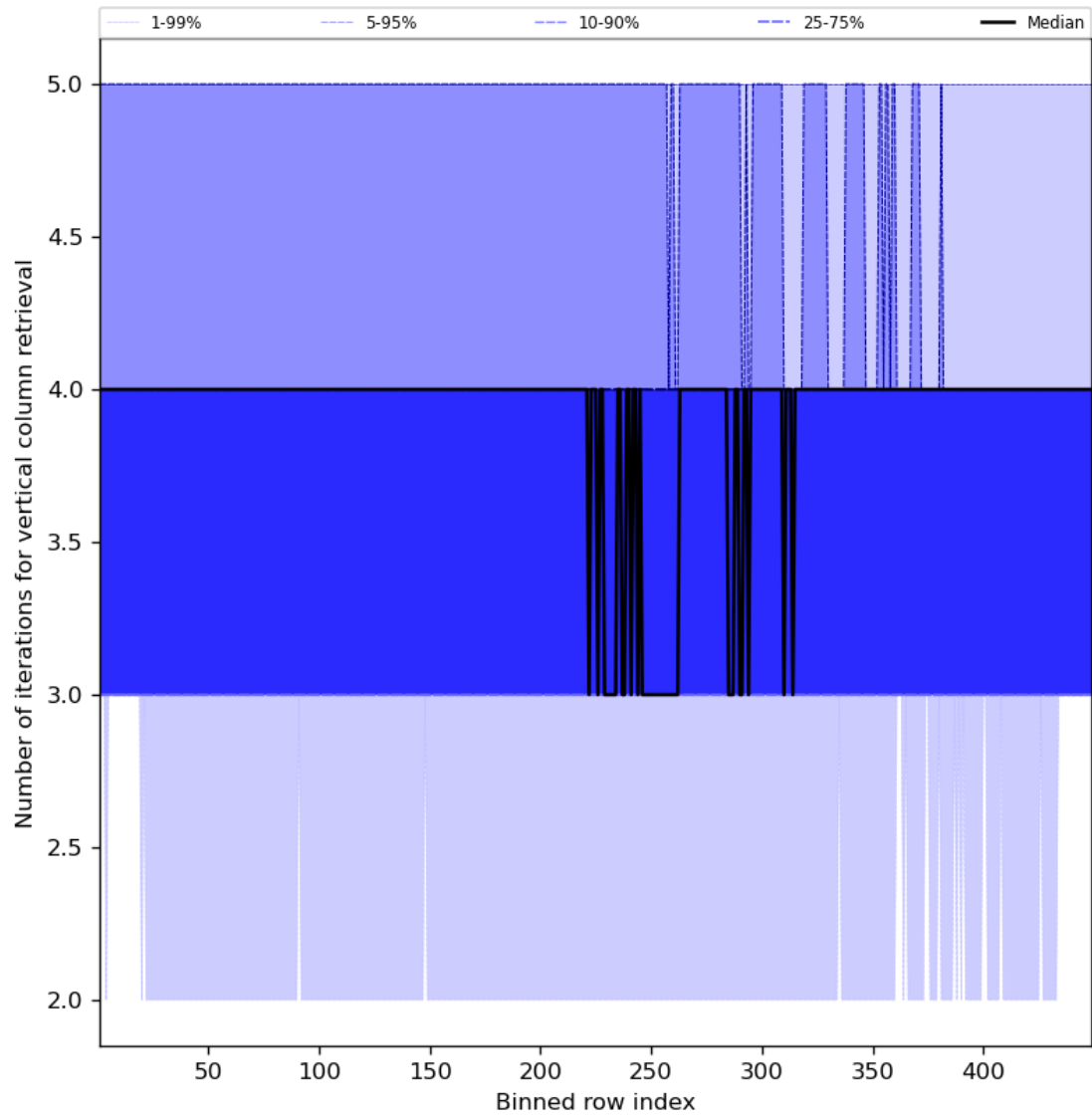
Figure 33: Along track statistics of “Number of iterations for vertical column retrieval” for 2024-05-30 to 2024-06-01
