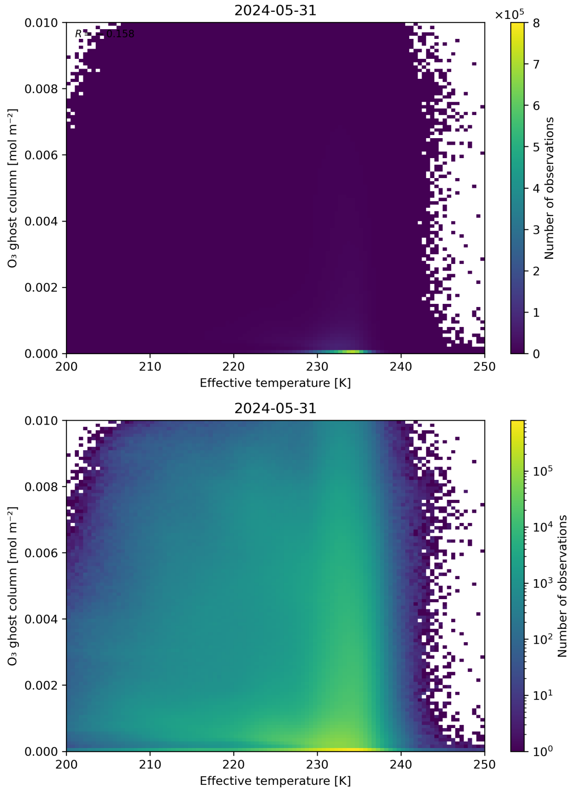
Figure 38: Scatter density plot of “Effective temperature” against “O 3 ghost column” for 2024-05-30 to 2024-06-01.
