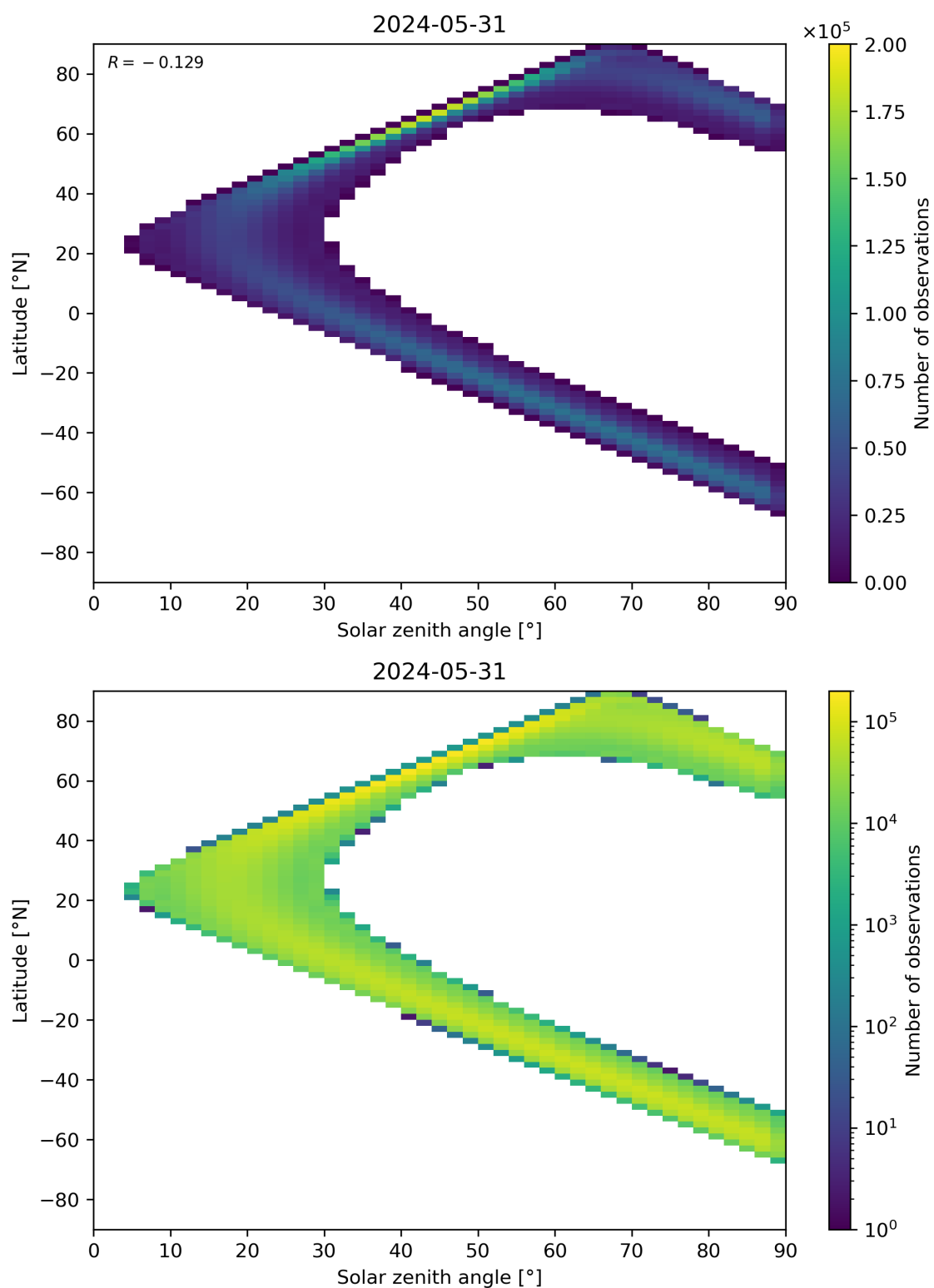
Figure 44: Scatter density plot of “Solar zenith angle” against “Latitude” for 2024-05-30 to 2024-06-01.
