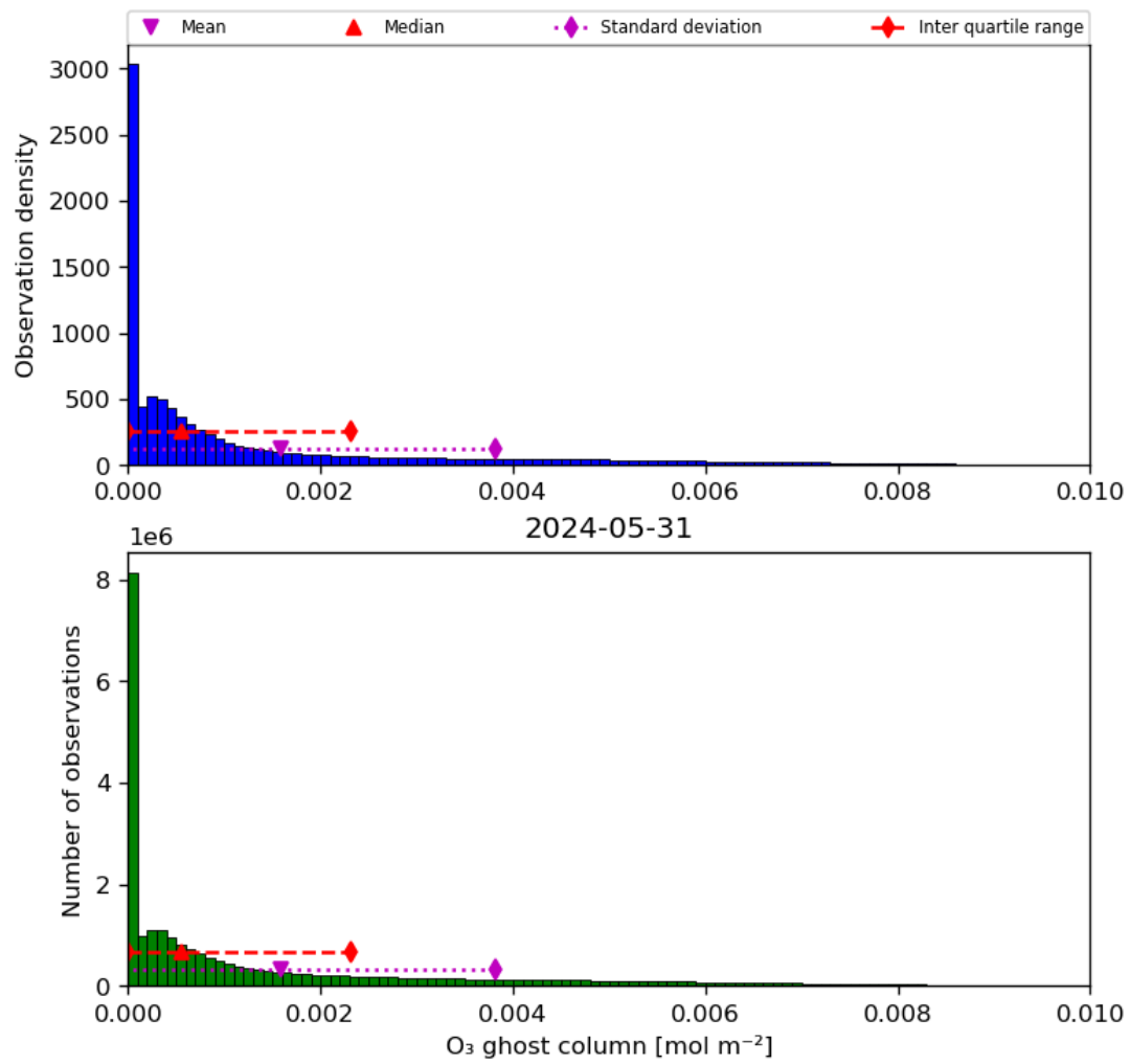
Figure 25: Histogram of “O 3 ghost column” for 2024-05-30 to 2024-06-01
