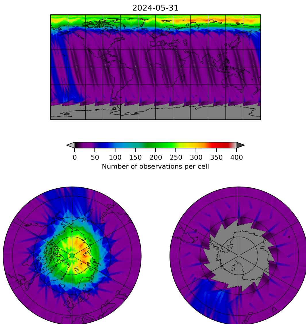
Figure 12: Map of the number of observations for 2024-05-30 to 2024-06-01
