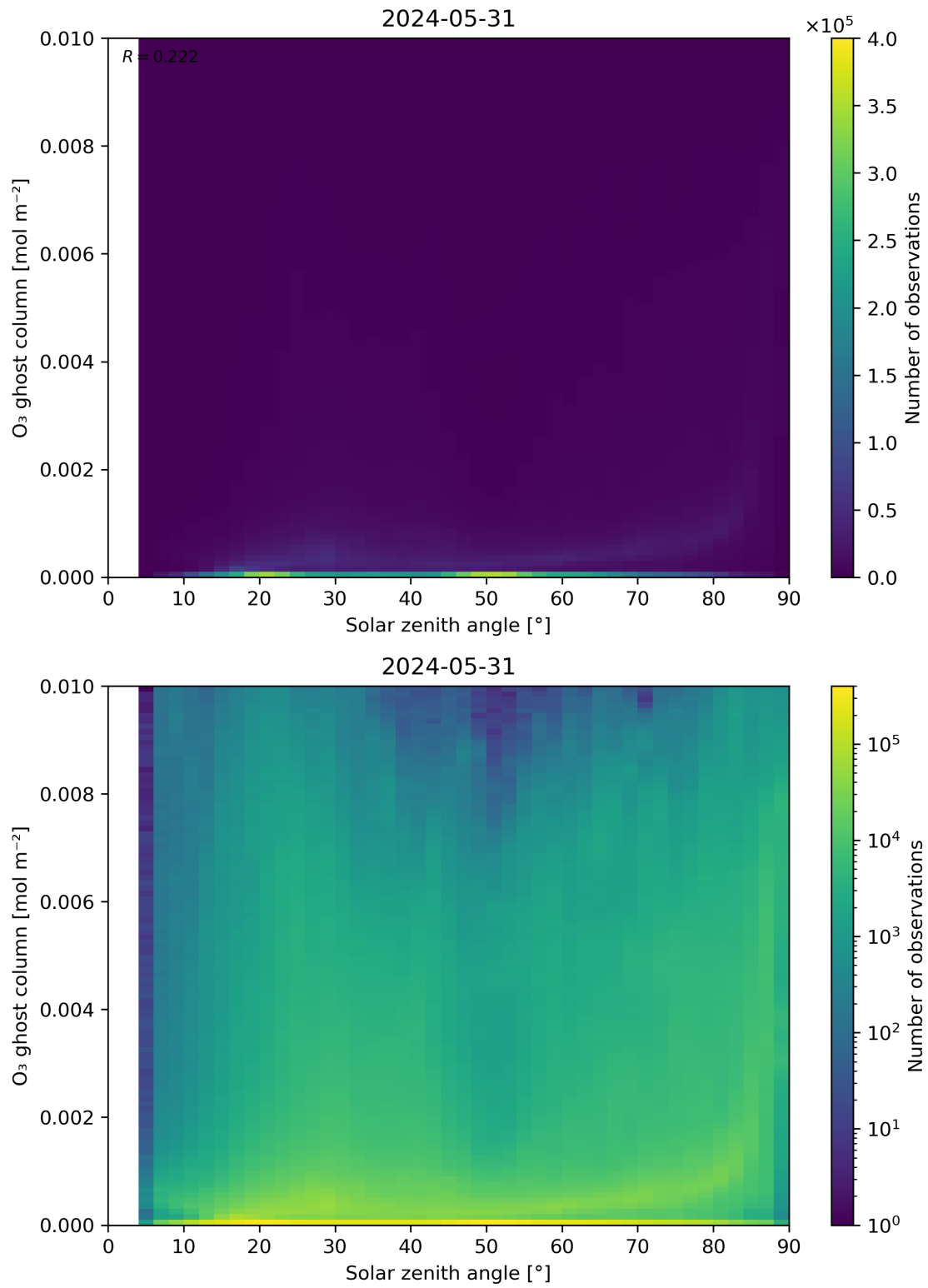
Figure 46: Scatter density plot of “Solar zenith angle” against “O 3 ghost column” for 2024-05-30 to 2024-06-01.
