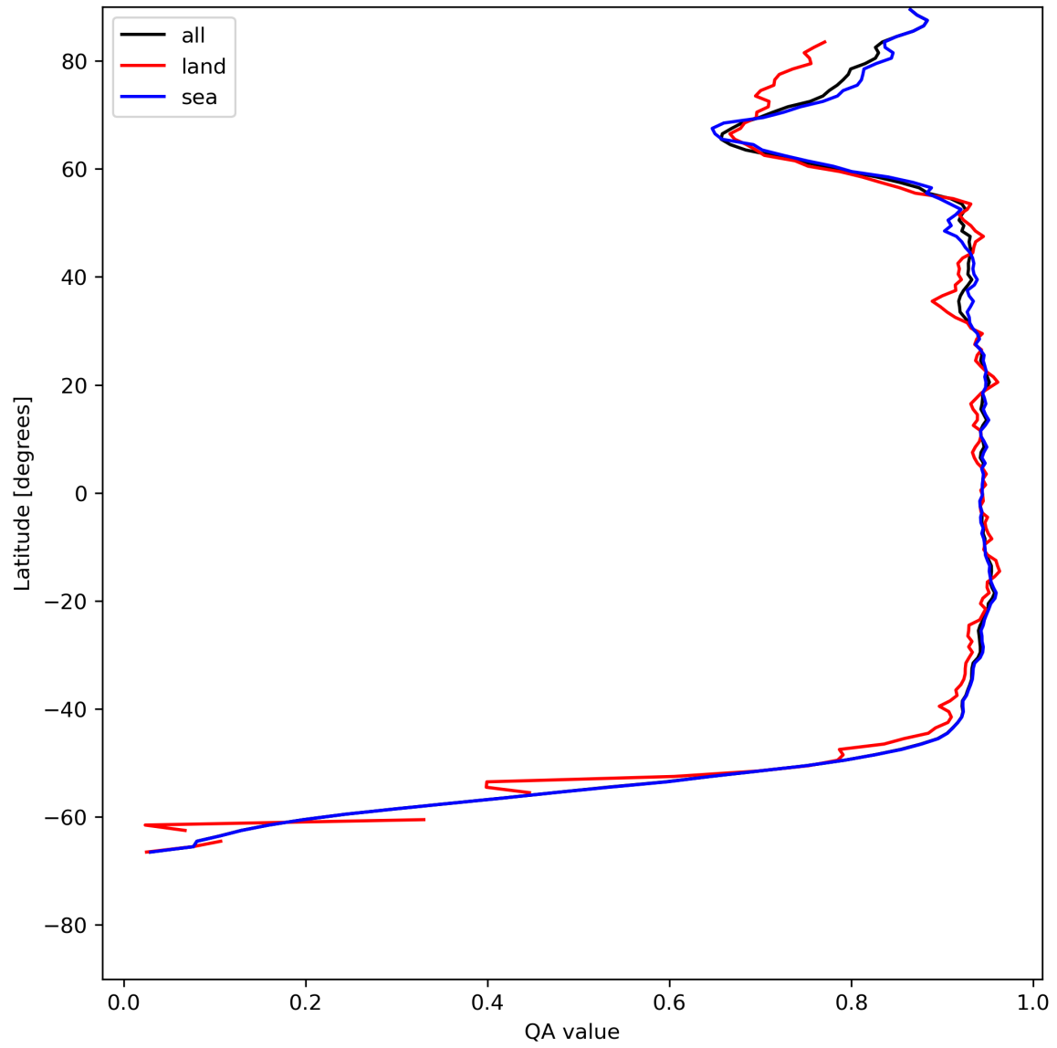
Figure 13: Zonal average of “QA value” for 2024-05-30 to 2024-06-01.
