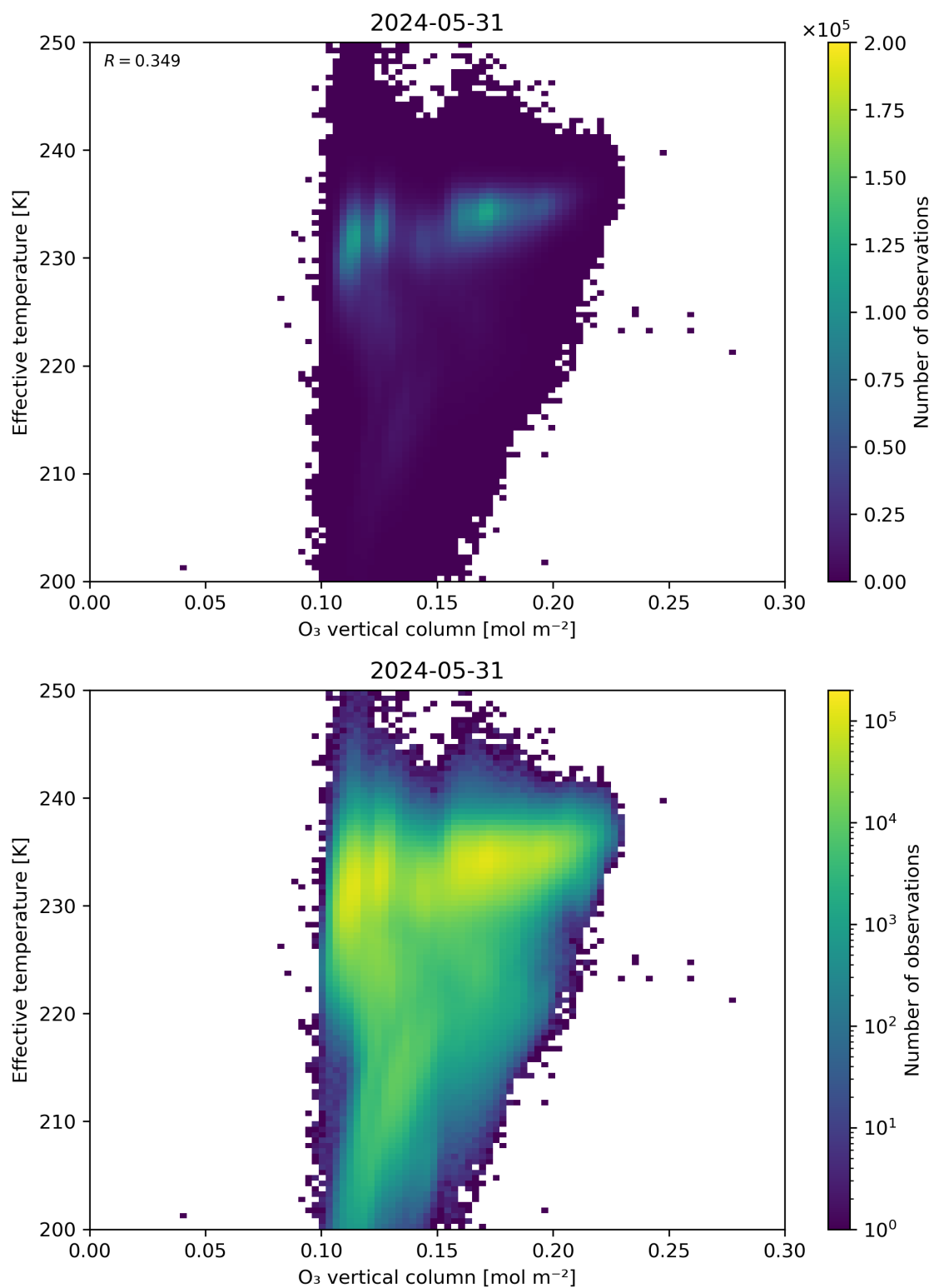
Figure 39: Scatter density plot of “O 3 vertical column” against “Effective temperature” for 2024-05-30 to 2024-06-01.
