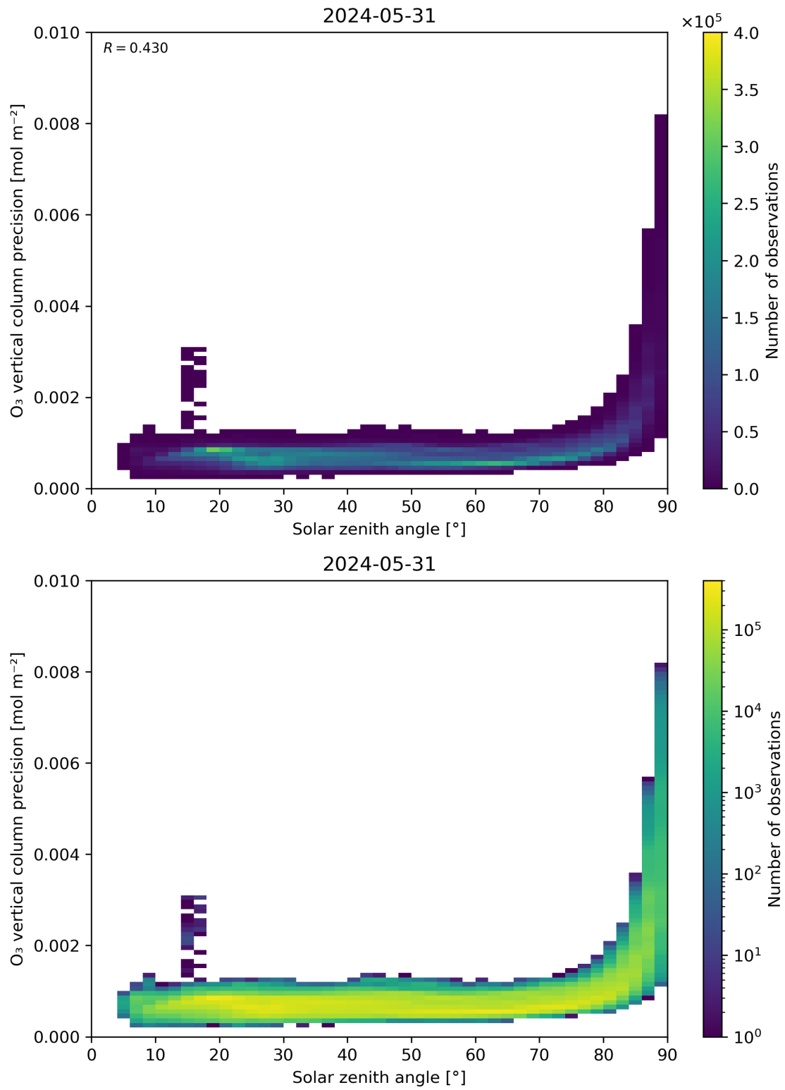
Figure 48: Scatter density plot of “Solar zenith angle” against “O 3 vertical column precision” for 2024-05-30 to 2024-06-01.
