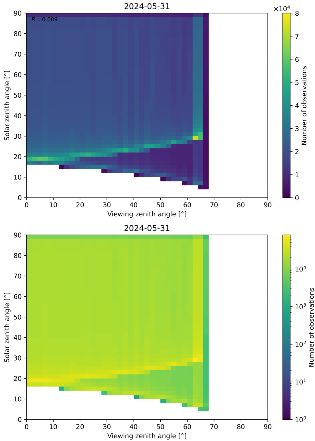
Figure 54: Scatter density plot of “Viewing zenith angle” against “Solar zenith angle” for 2024-05-30 to 2024-06-01.
