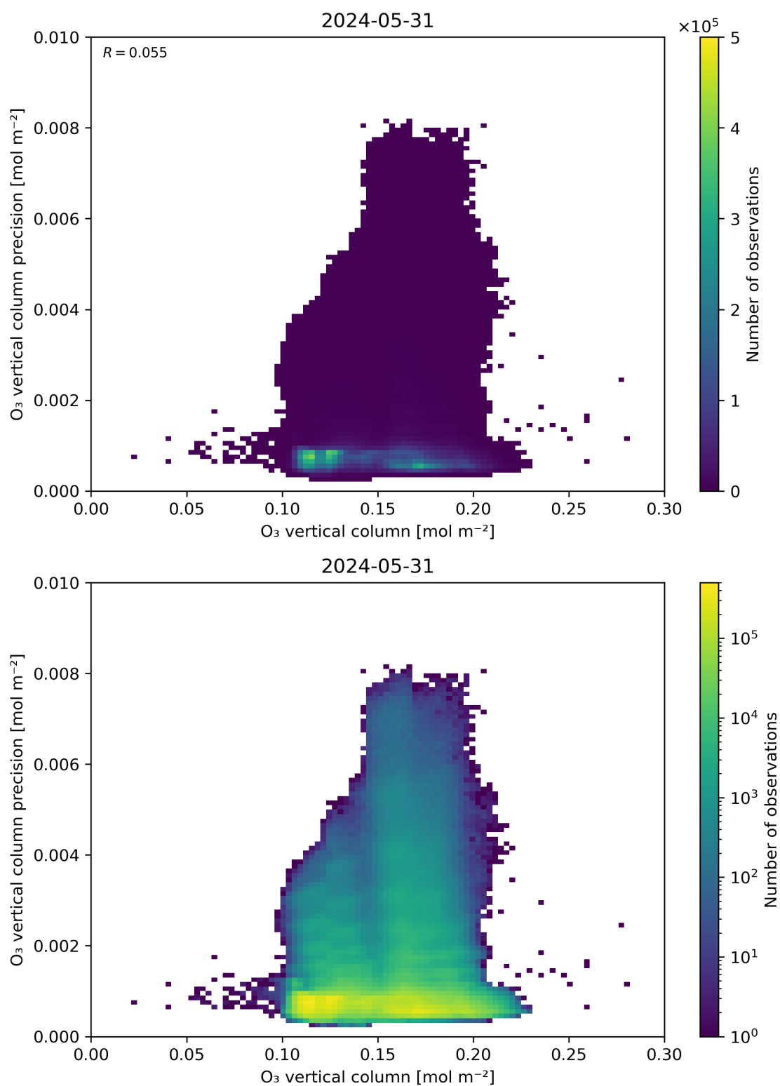
Figure 41: Scatter density plot of “O 3 vertical column” against “O 3 vertical column precision” for 2024-05-30 to 2024-06-01.
