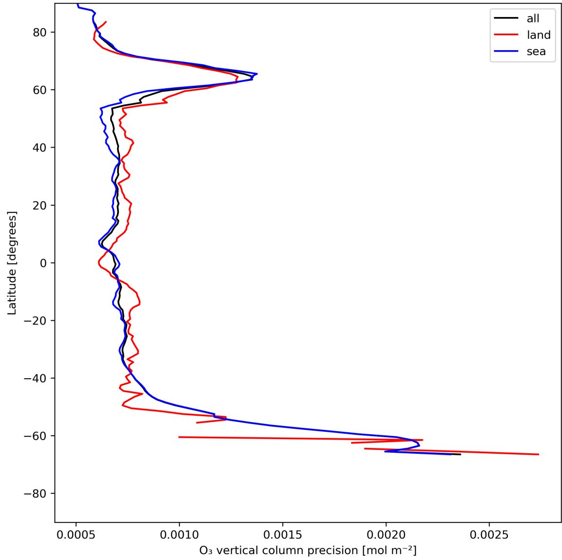
Figure 15: Zonal average of "O 3 vertical column precision" for 2024-05-30 to 2024-06-01.
