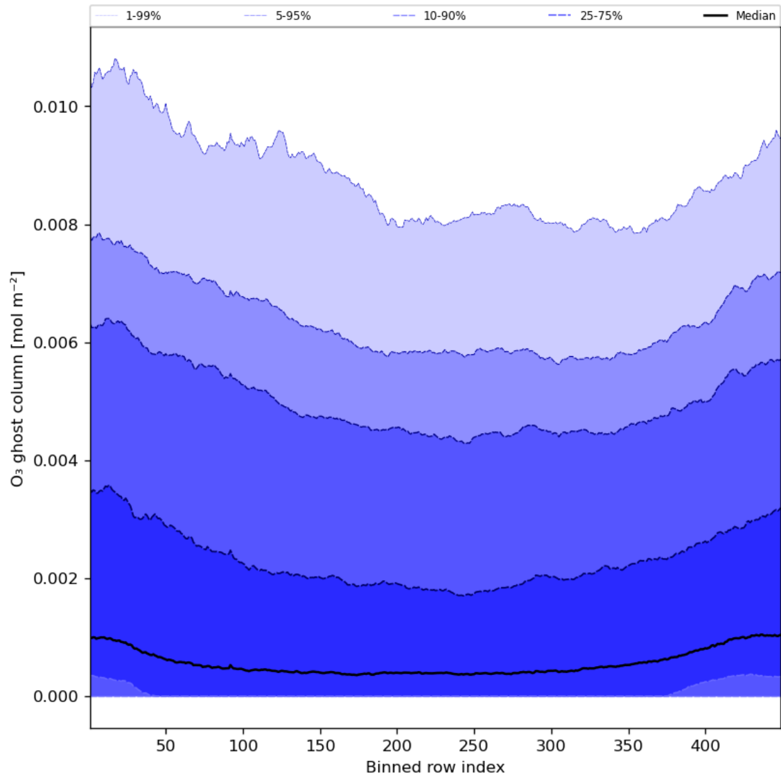
Figure 32: Along track statistics of “O 3 ghost column” for 2024-05-30 to 2024-06-01
