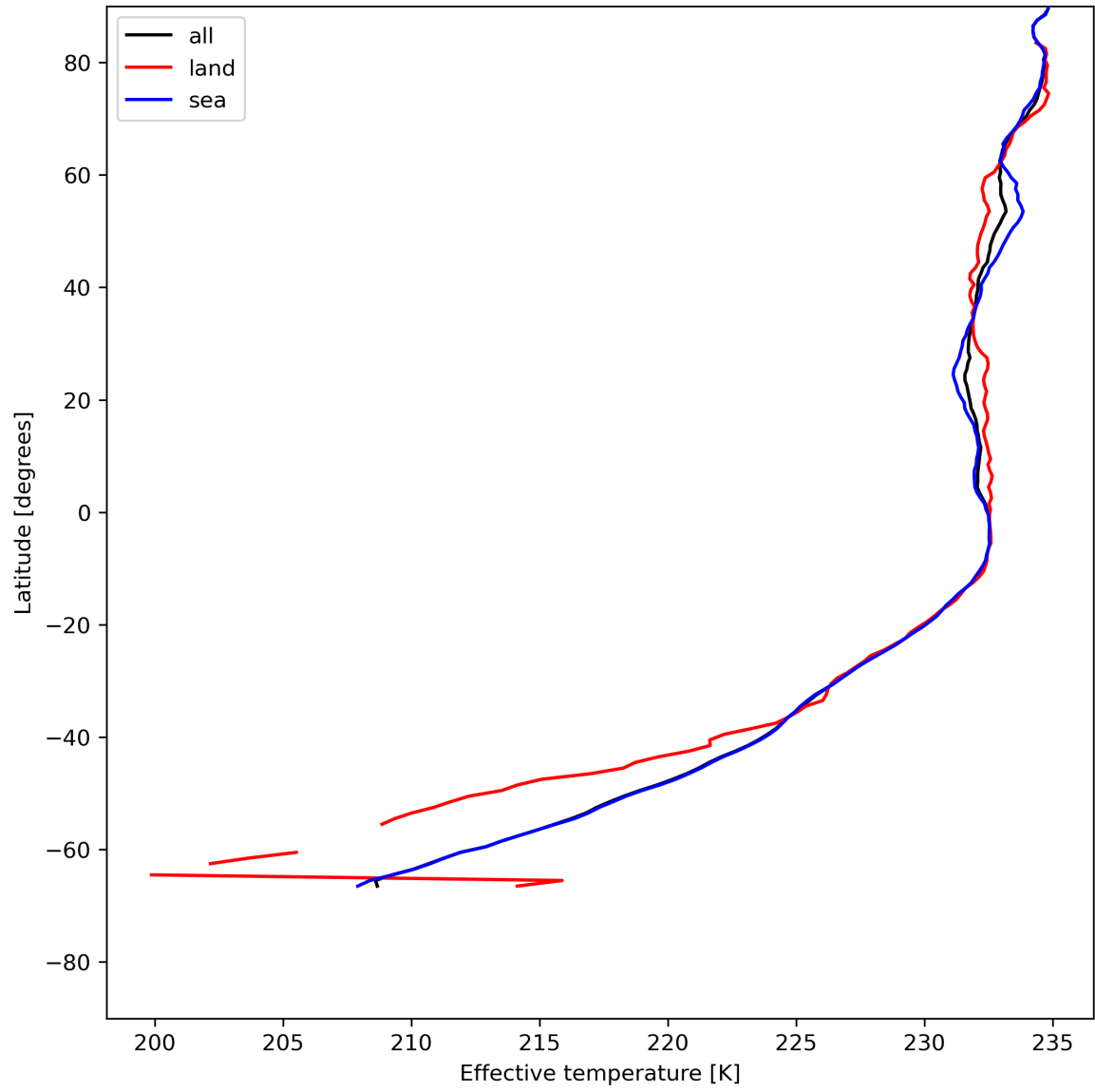
Figure 17: Zonal average of "Effective temperature" for 2024-05-30 to 2024-06-01.
