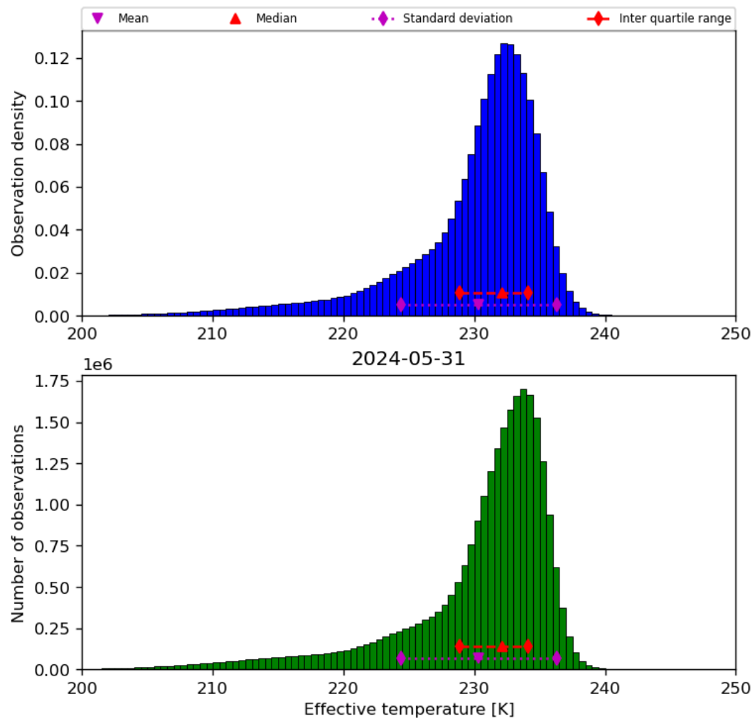
Figure 24: Histogram of “Effective temperature” for 2024-05-30 to 2024-06-01
