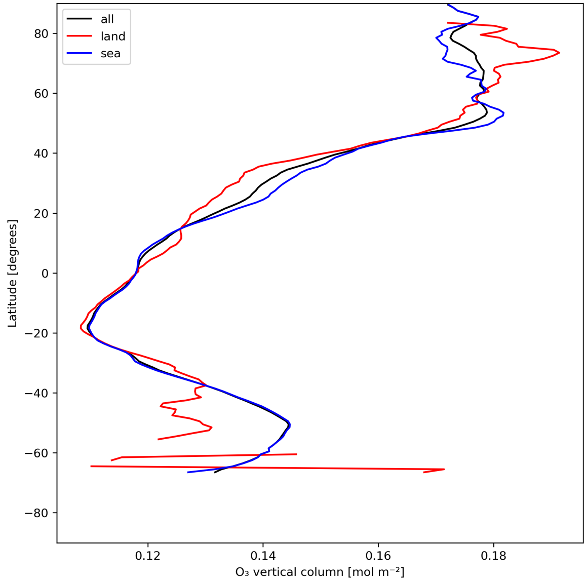
Figure 14: Zonal average of “O 3 vertical column” for 2024-05-30 to 2024-06-01.
