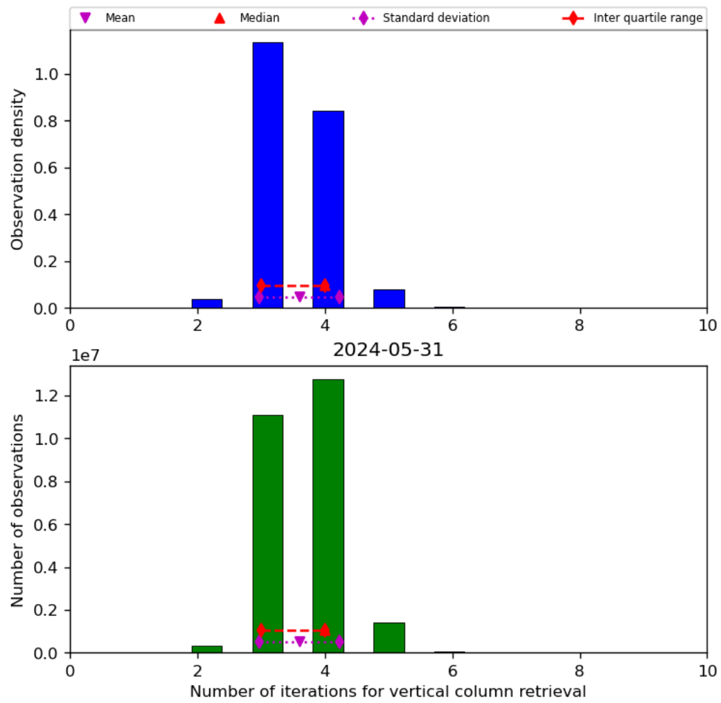
Figure 26: Histogram of “Number of iterations for vertical column retrieval” for 2024-05-30 to 2024-06-01
