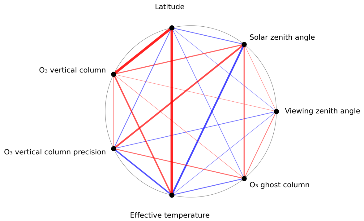
Figure 1: Map of correlation graph for 2024-05-30 to 2024-06-01.
