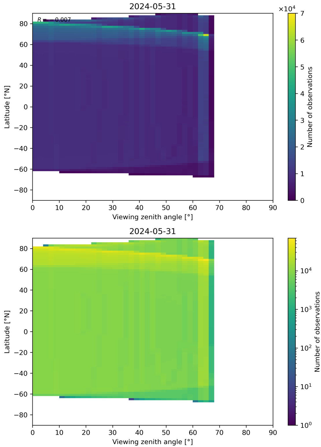
Figure 49: Scatter density plot of “Viewing zenith angle” against “Latitude” for 2024-05-30 to 2024-06-01.
