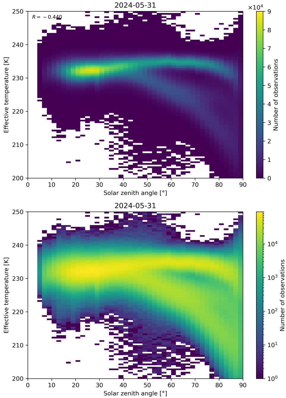
Figure 45: Scatter density plot of “Solar zenith angle” against “Effective temperature” for 2024-05-30 to 2024-06-01.
