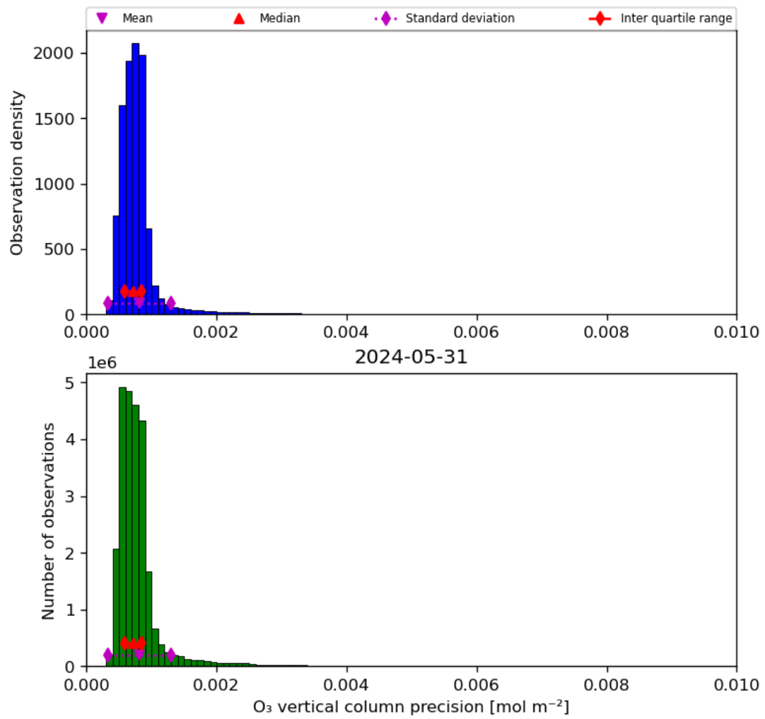
Figure 22: Histogram of “O 3 vertical column precision” for 2024-05-30 to 2024-06-01
