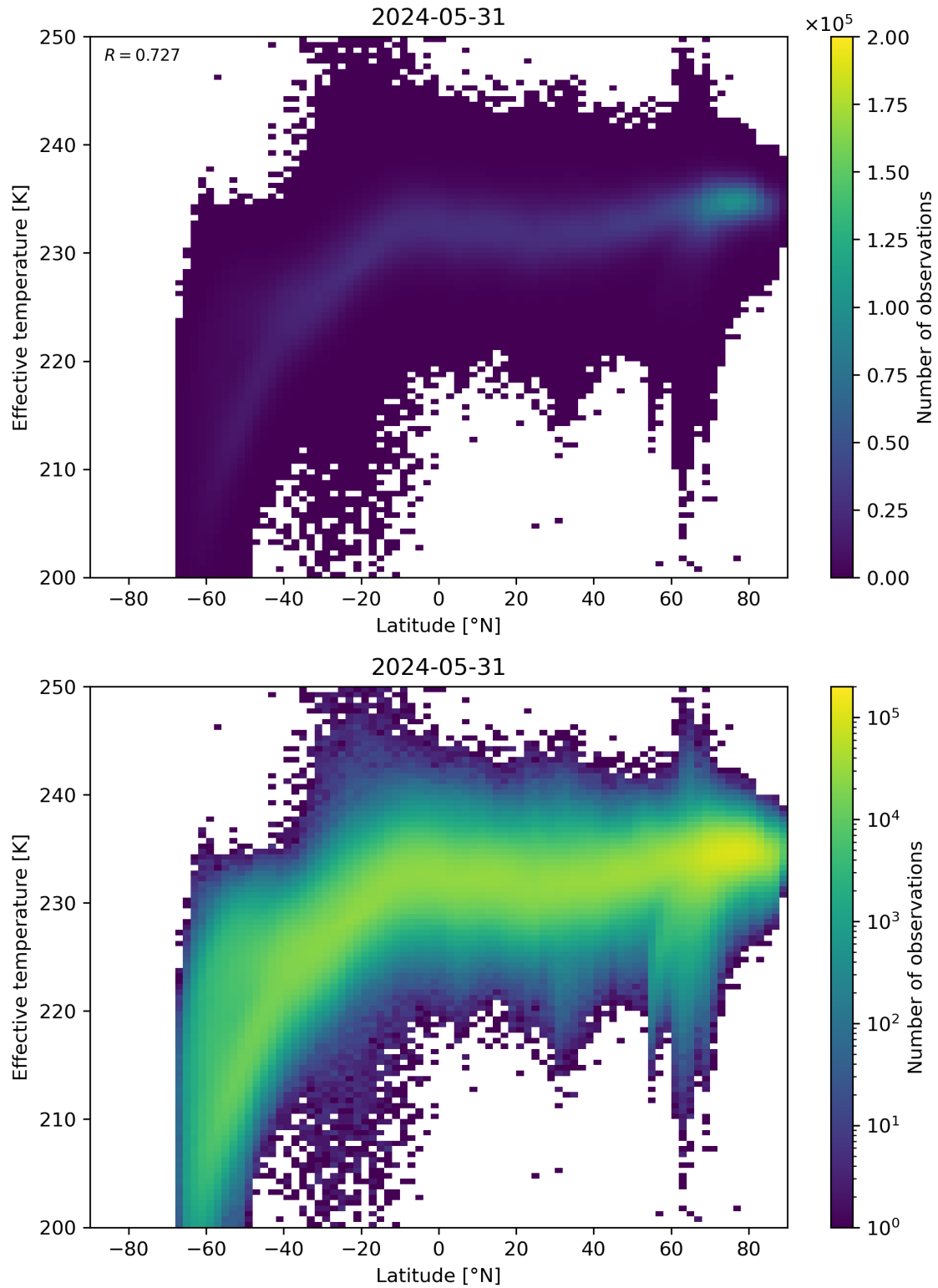
Figure 34: Scatter density plot of “Latitude” against “Effective temperature” for 2024-05-30 to 2024-06-01.
