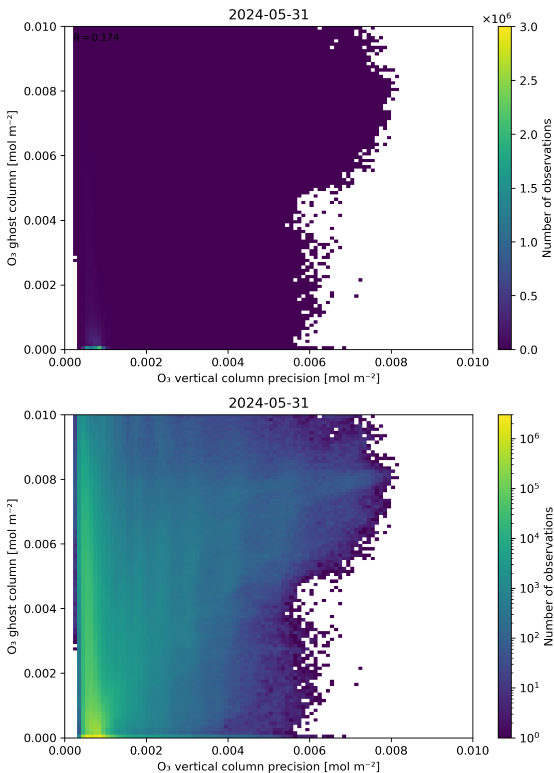
Figure 43: Scatter density plot of “ \text{O}_3 vertical column precision” against “ \text{O}_3 ghost column” for 2024-05-30 to 2024-06-01.
