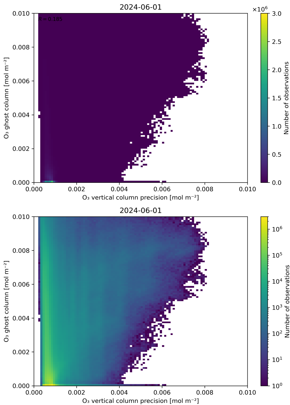
Figure 43: Scatter density plot of “ \text{O}_3 vertical column precision” against “ \text{O}_3 ghost column” for 2024-05-31 to 2024-06-02.
