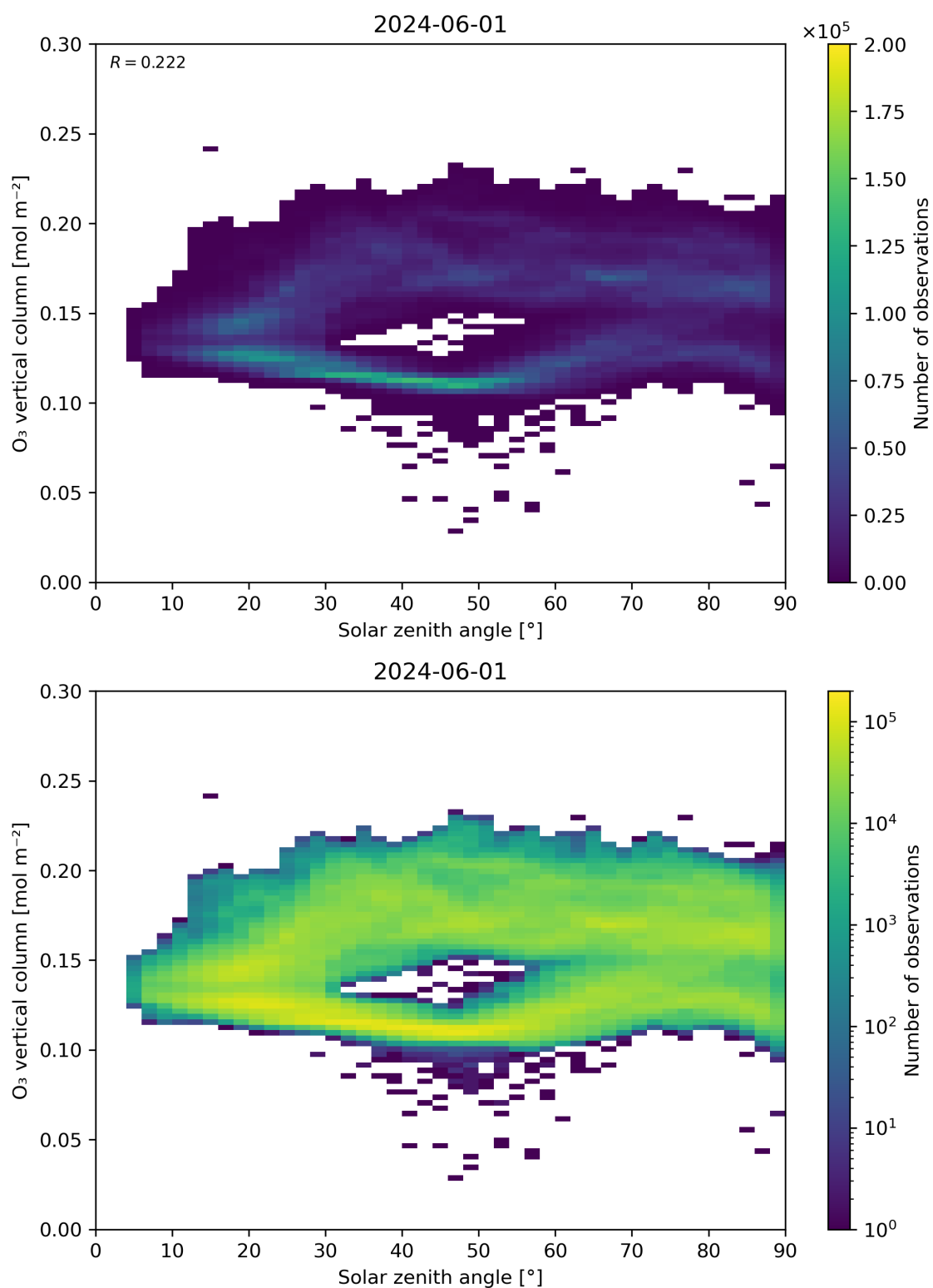
Figure 47: Scatter density plot of “Solar zenith angle” against “O 3 vertical column” for 2024-05-31 to 2024-06-02.
