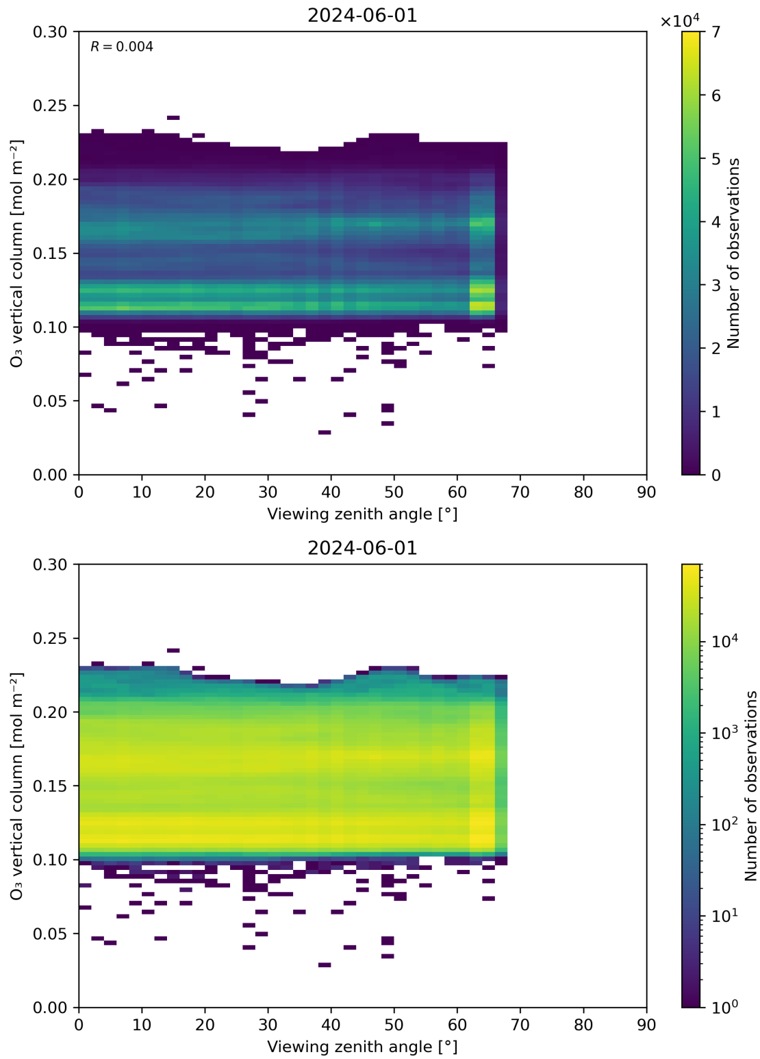
Figure 52: Scatter density plot of “Viewing zenith angle” against “O 3 vertical column” for 2024-05-31 to 2024-06-02.
