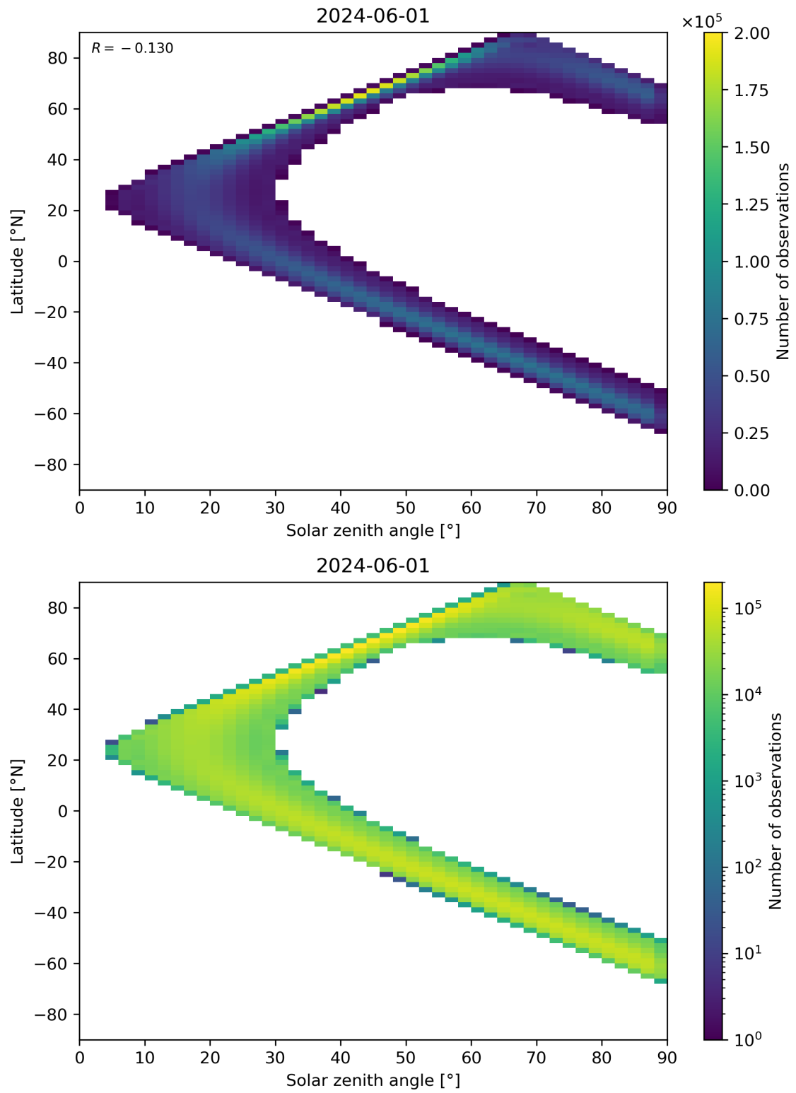
Figure 44: Scatter density plot of “Solar zenith angle” against “Latitude” for 2024-05-31 to 2024-06-02.
