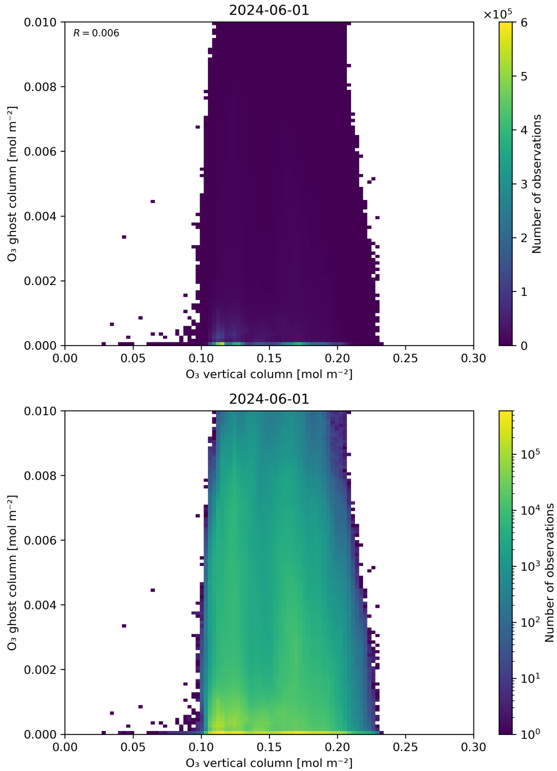
Figure 40: Scatter density plot of “O 3 vertical column” against “O 3 ghost column” for 2024-05-31 to 2024-06-02.
