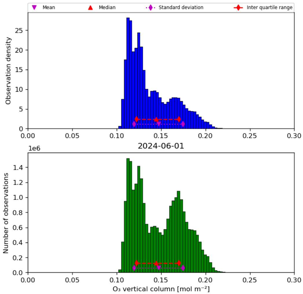
Figure 21: Histogram of “O 3 vertical column” for 2024-05-31 to 2024-06-02
