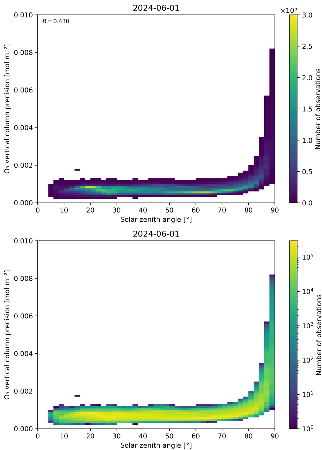
Figure 48: Scatter density plot of “Solar zenith angle” against “O 3 vertical column precision” for 2024-05-31 to 2024-06-02.
