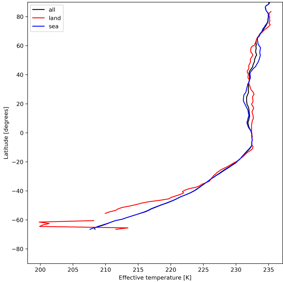
Figure 17: Zonal average of "Effective temperature" for 2024-05-31 to 2024-06-02.
