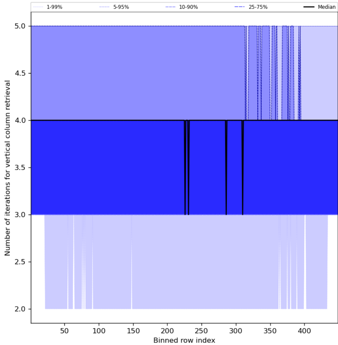
Figure 33: Along track statistics of “Number of iterations for vertical column retrieval” for 2024-05-31 to 2024-06-02
