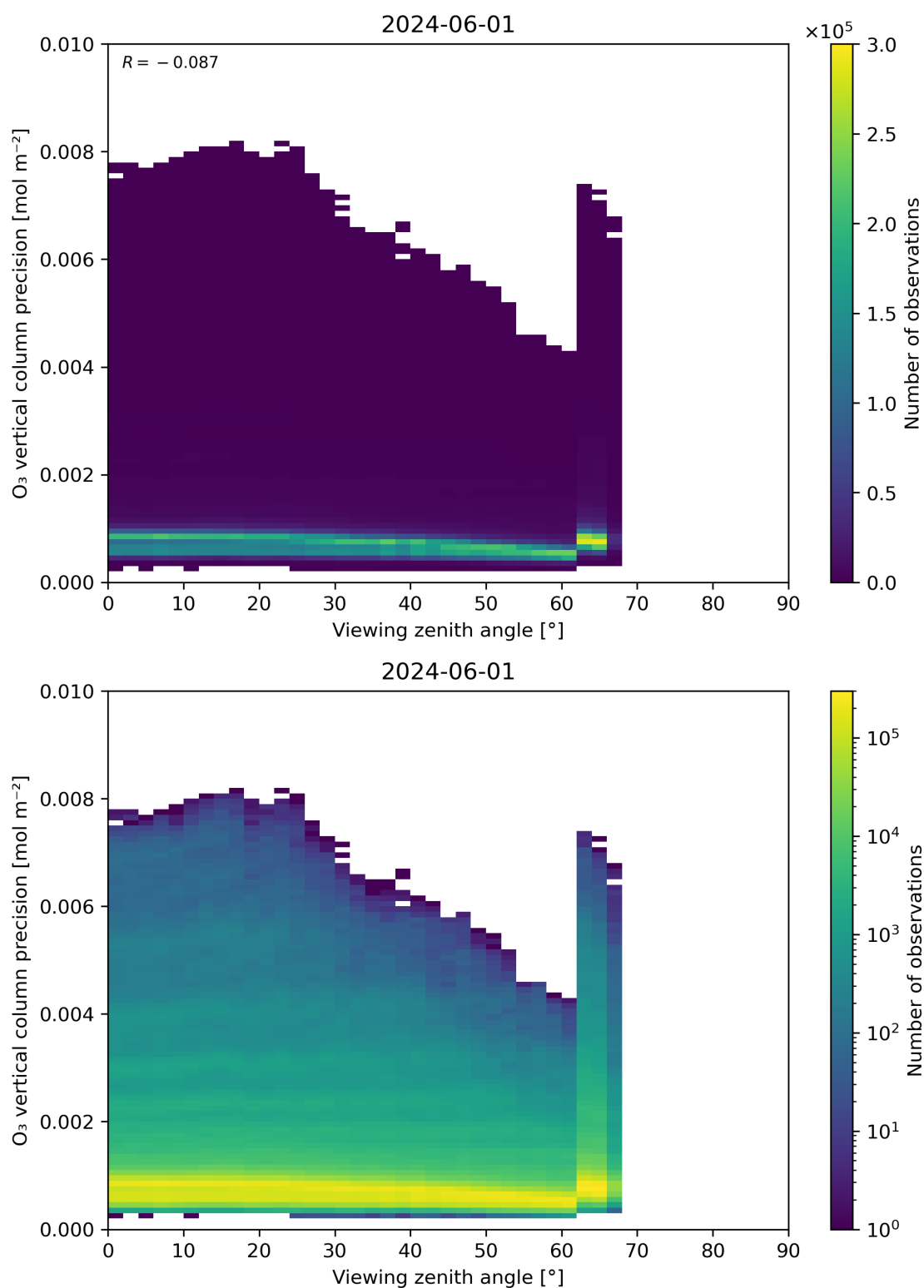
Figure 53: Scatter density plot of “Viewing zenith angle” against “O 3 vertical column precision” for 2024-05-31 to 2024-06-02.
