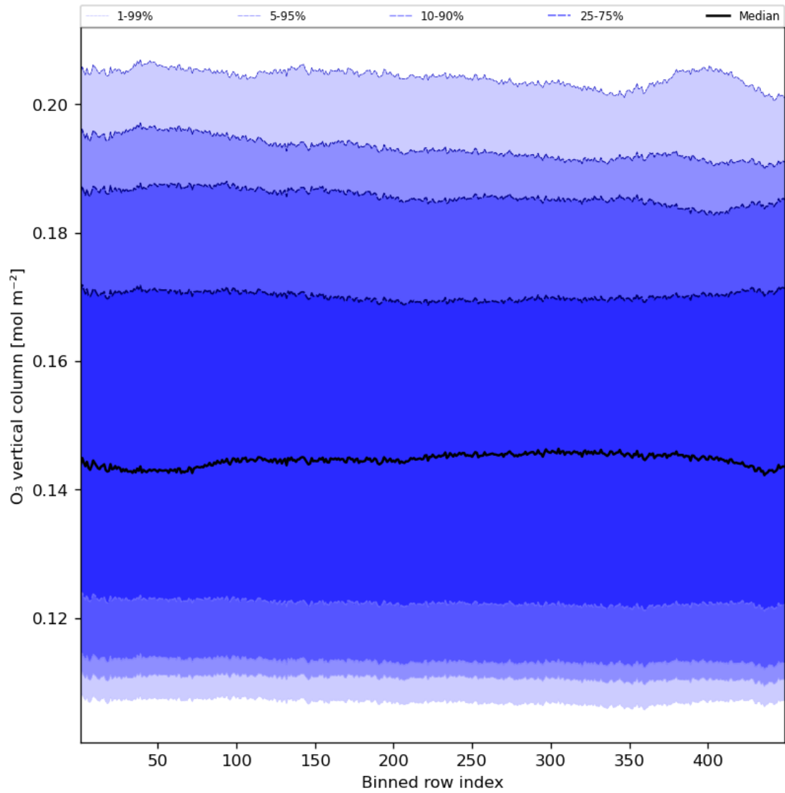
Figure 28: Along track statistics of “O 3 vertical column” for 2024-05-31 to 2024-06-02
