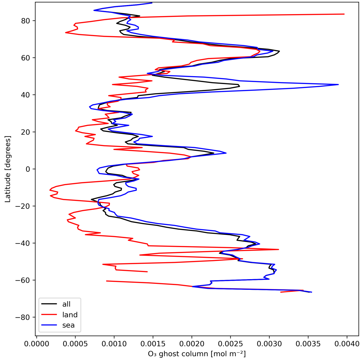
Figure 18: Zonal average of "O 3 ghost column" for 2024-05-31 to 2024-06-02.
