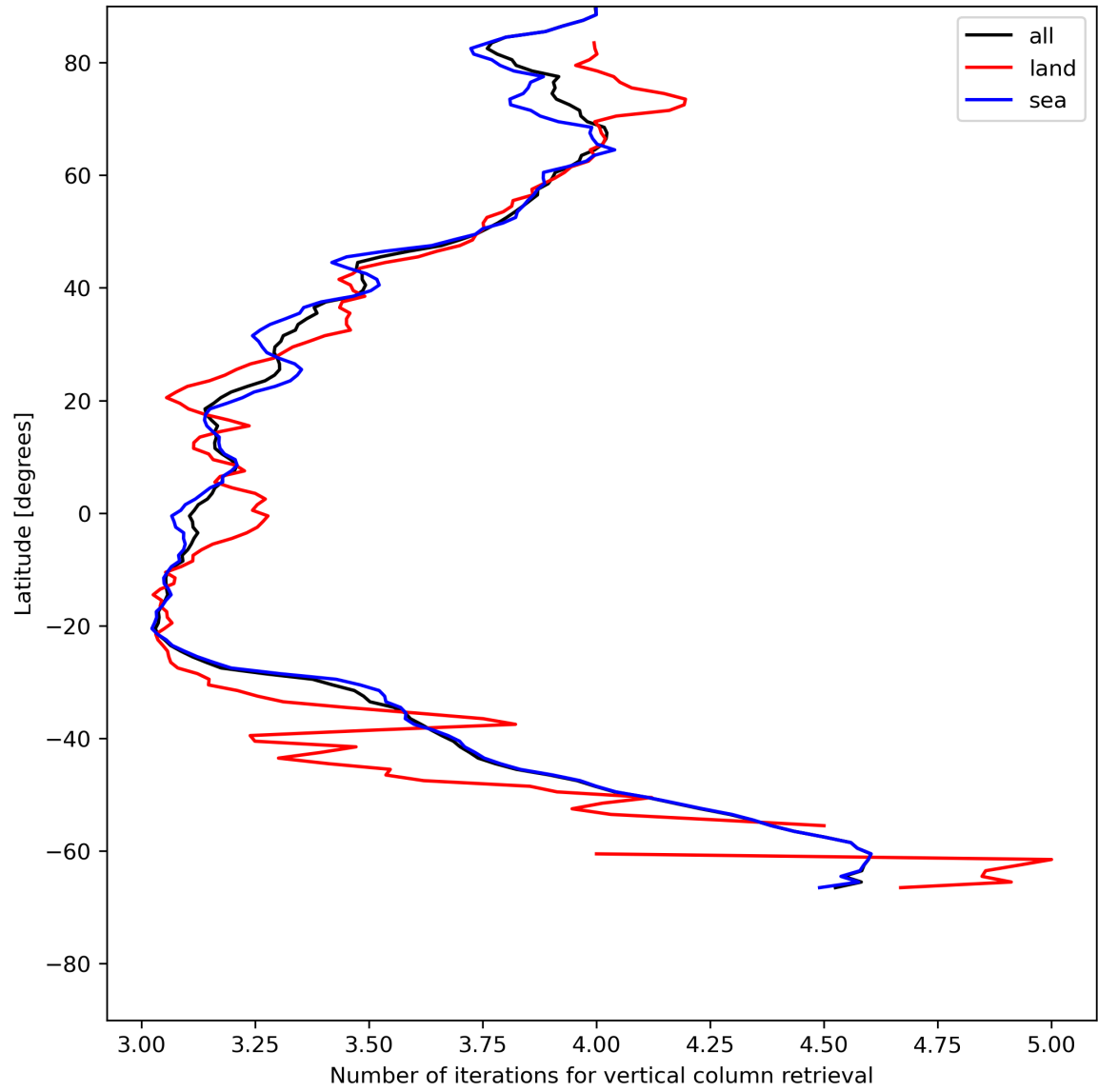
Figure 19: Zonal average of “Number of iterations for vertical column retrieval” for 2024-05-31 to 2024-06-02.
