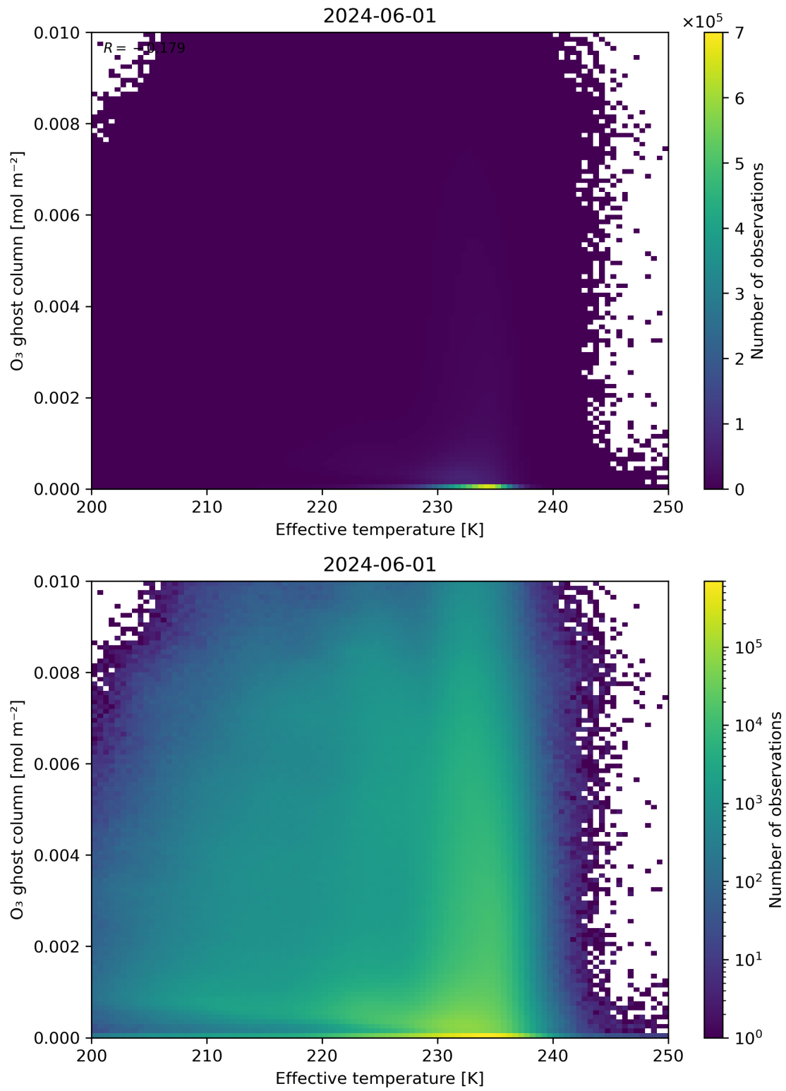
Figure 38: Scatter density plot of “Effective temperature” against “O 3 ghost column” for 2024-05-31 to 2024-06-02.
