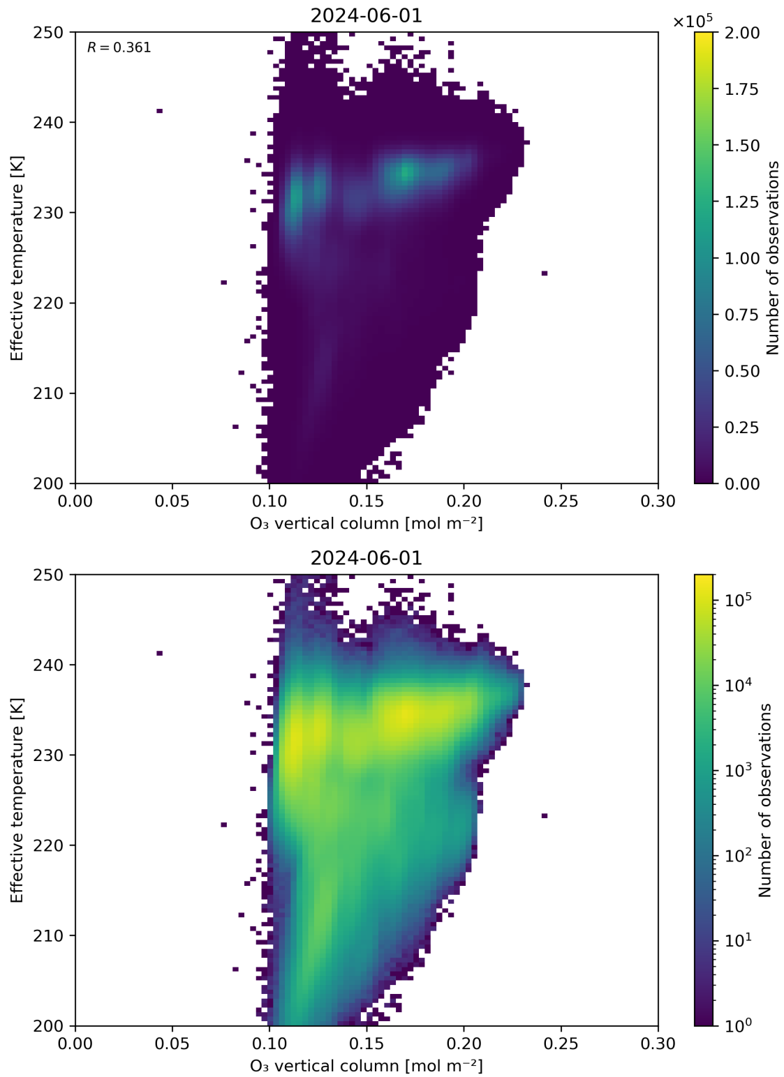
Figure 39: Scatter density plot of “O 3 vertical column” against “Effective temperature” for 2024-05-31 to 2024-06-02.
