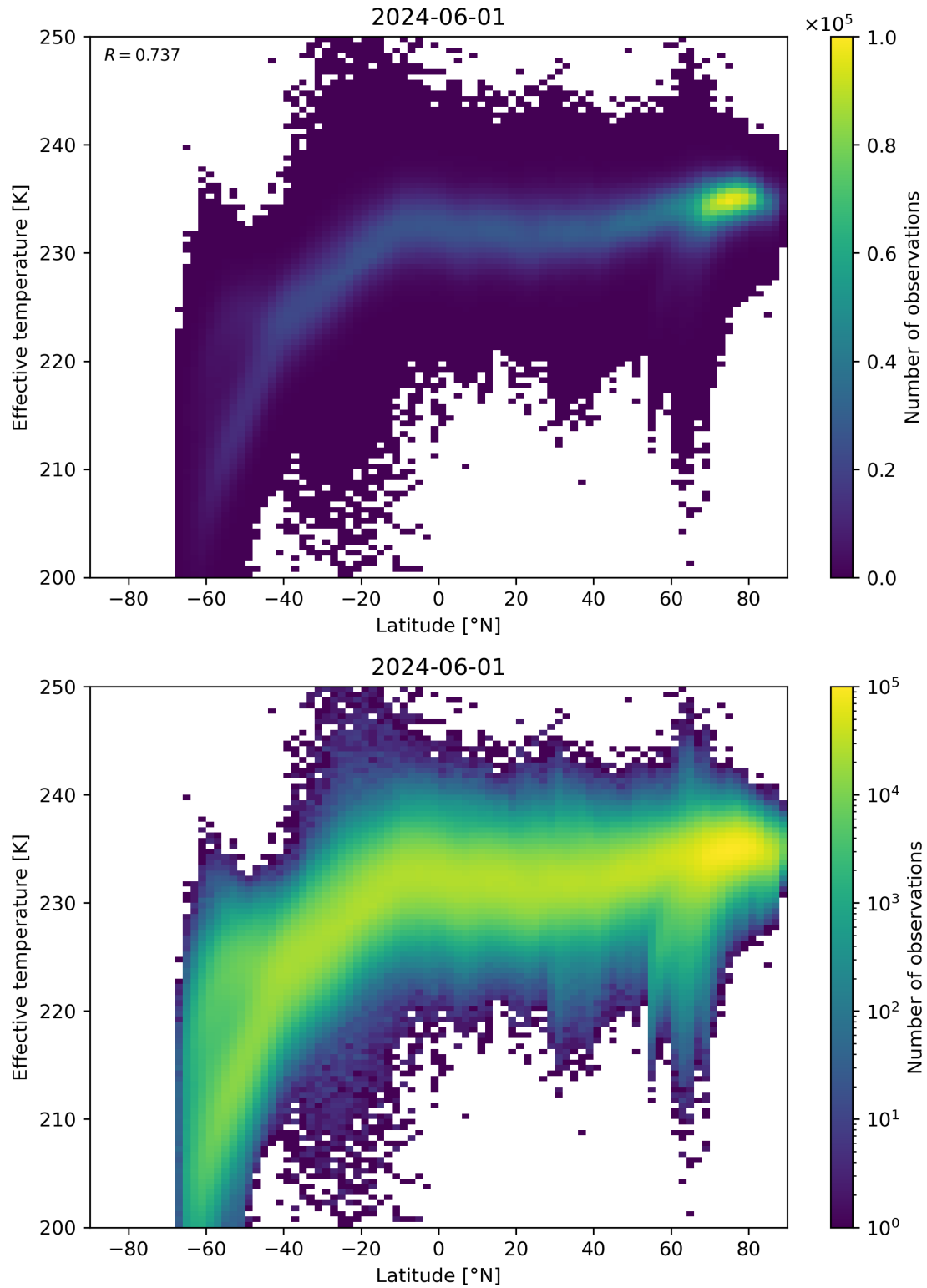
Figure 34: Scatter density plot of “Latitude” against “Effective temperature” for 2024-05-31 to 2024-06-02.
