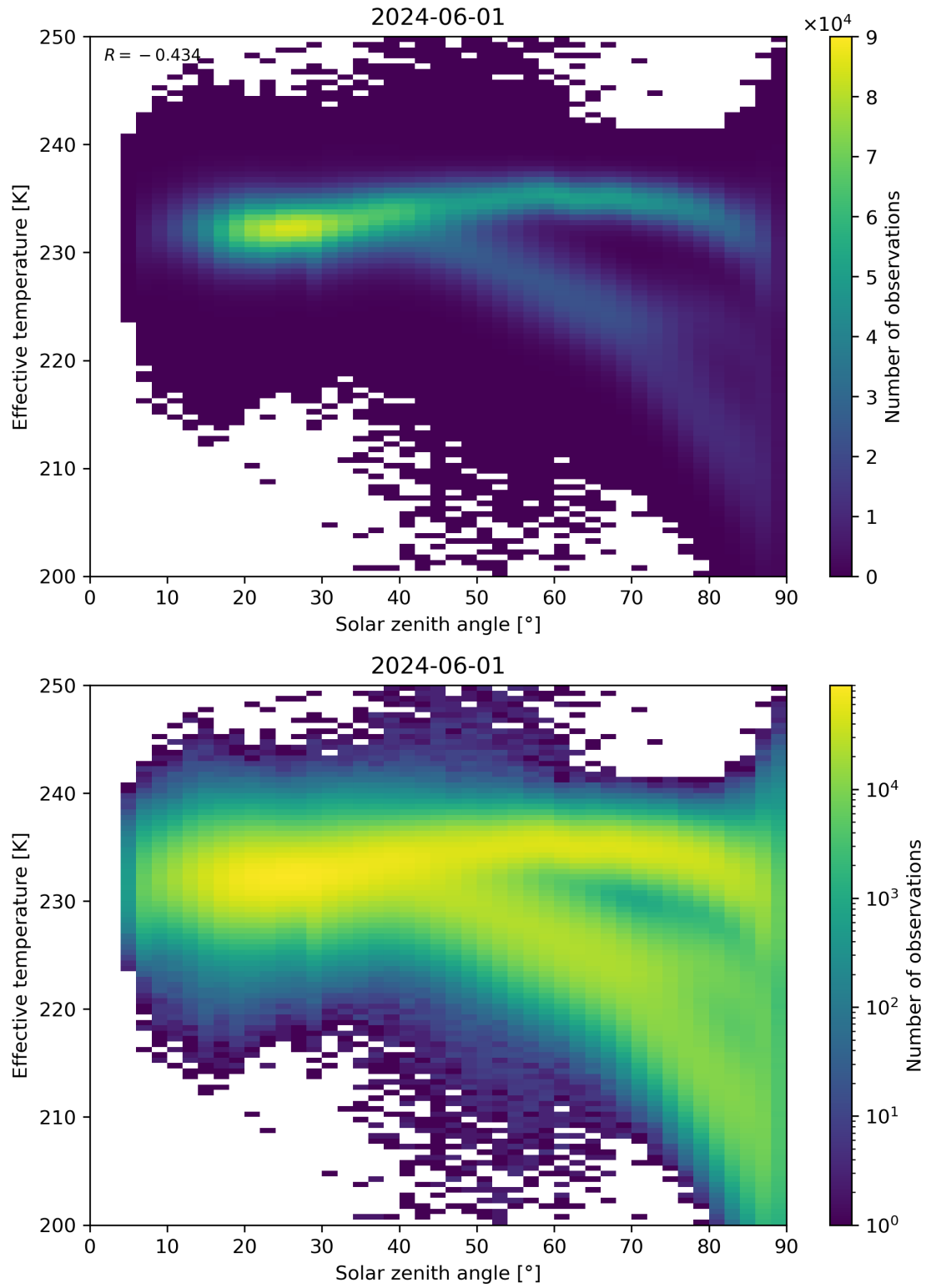
Figure 45: Scatter density plot of “Solar zenith angle” against “Effective temperature” for 2024-05-31 to 2024-06-02.
