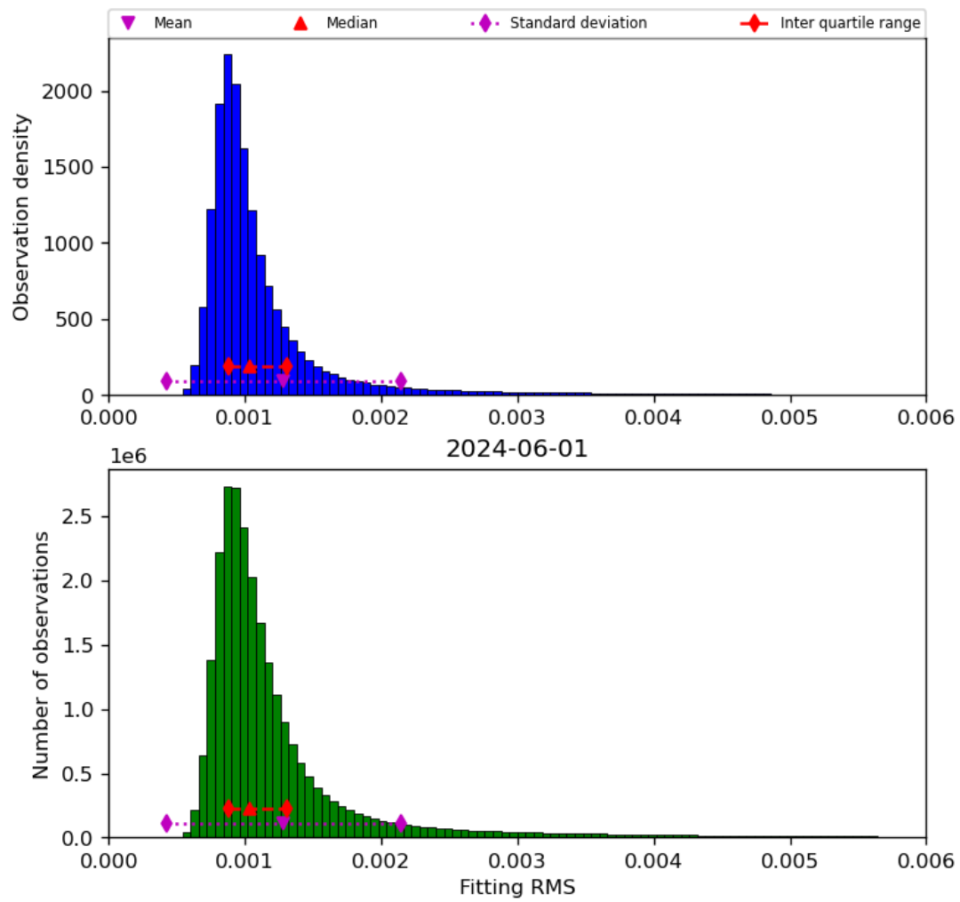
Figure 23: Histogram of “Fitting RMS” for 2024-05-31 to 2024-06-02
