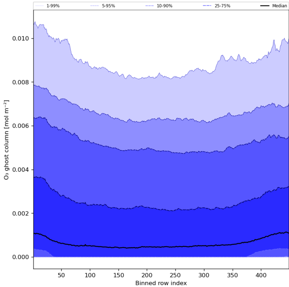
Figure 32: Along track statistics of “O 3 ghost column” for 2024-05-31 to 2024-06-02
