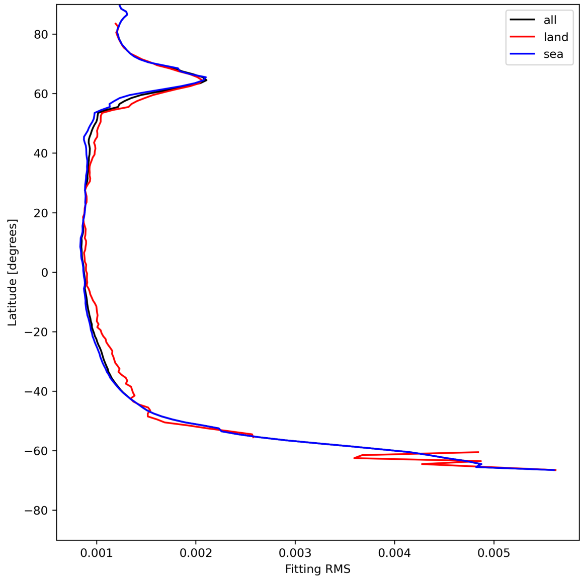
Figure 16: Zonal average of “Fitting RMS” for 2024-05-31 to 2024-06-02.
