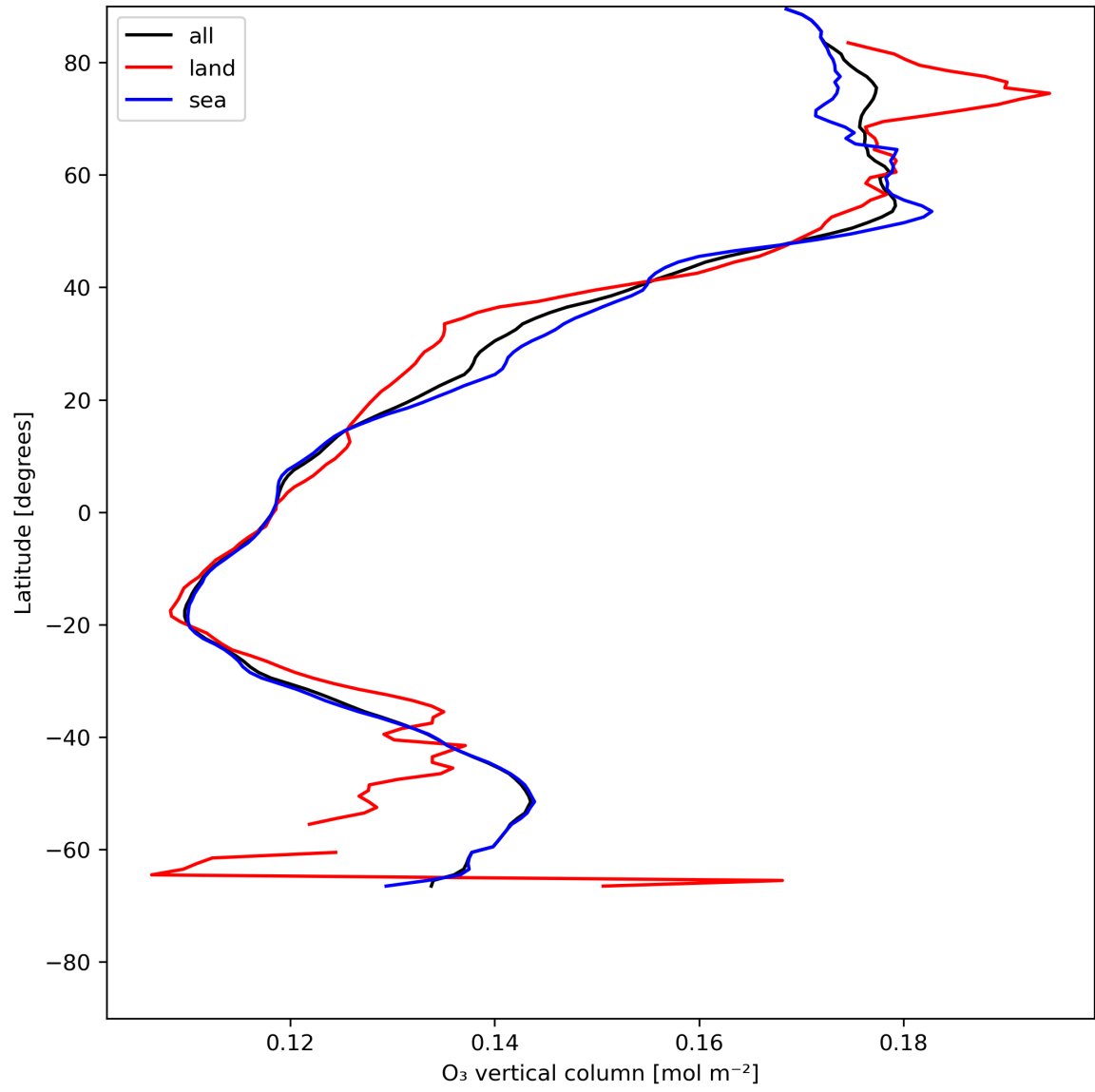
Figure 14: Zonal average of “O 3 vertical column” for 2024-05-31 to 2024-06-02.
