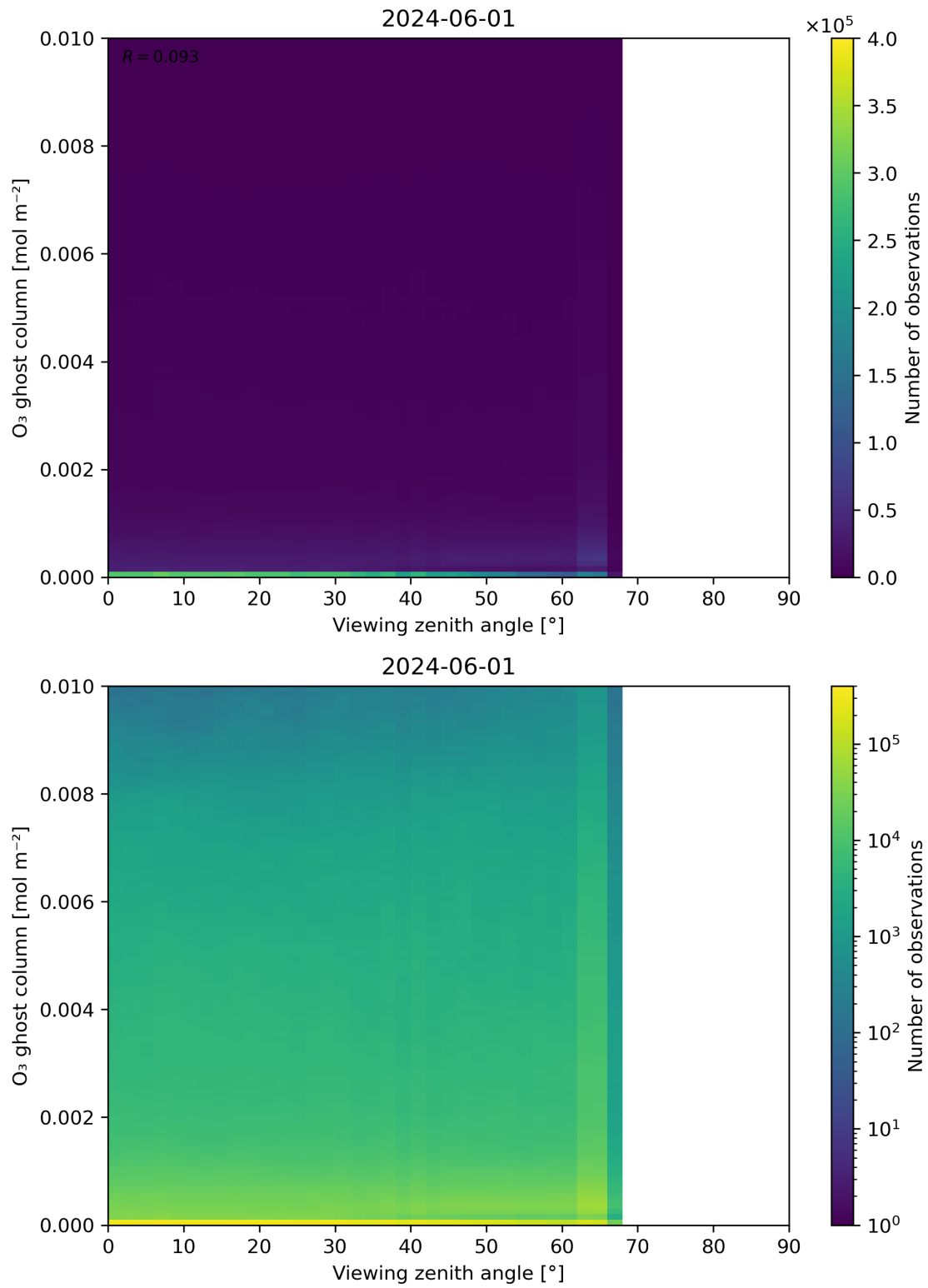
Figure 51: Scatter density plot of “Viewing zenith angle” against “O 3 ghost column” for 2024-05-31 to 2024-06-02.
