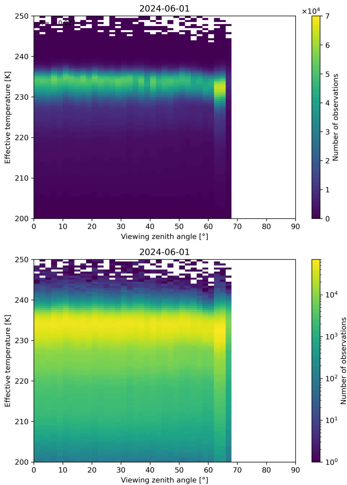
Figure 50: Scatter density plot of “Viewing zenith angle” against “Effective temperature” for 2024-05-31 to 2024-06-02.
