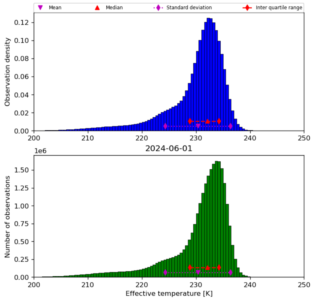
Figure 24: Histogram of “Effective temperature” for 2024-05-31 to 2024-06-02
