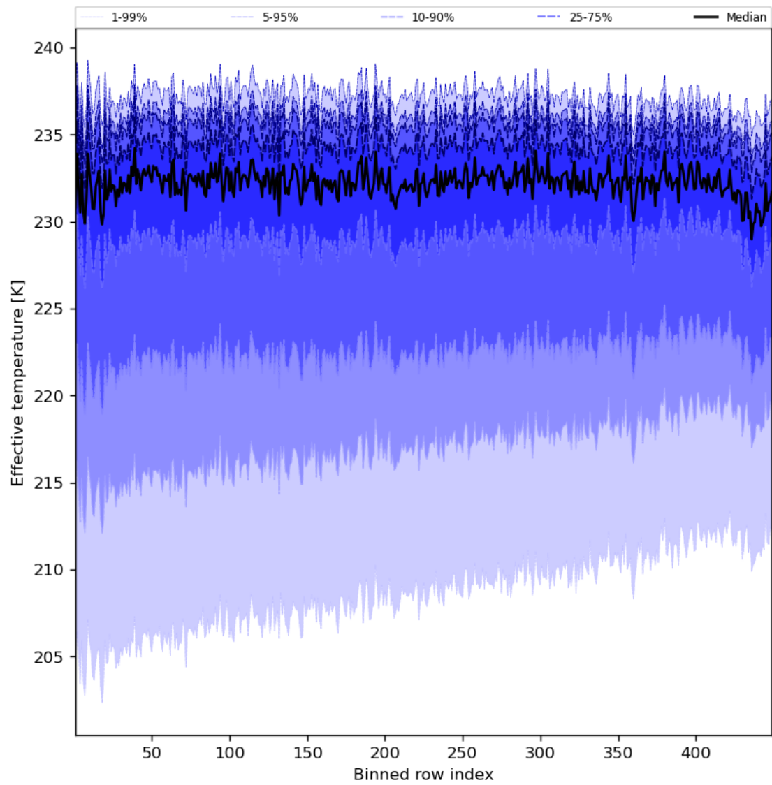
Figure 31: Along track statistics of “Effective temperature” for 2024-05-31 to 2024-06-02
