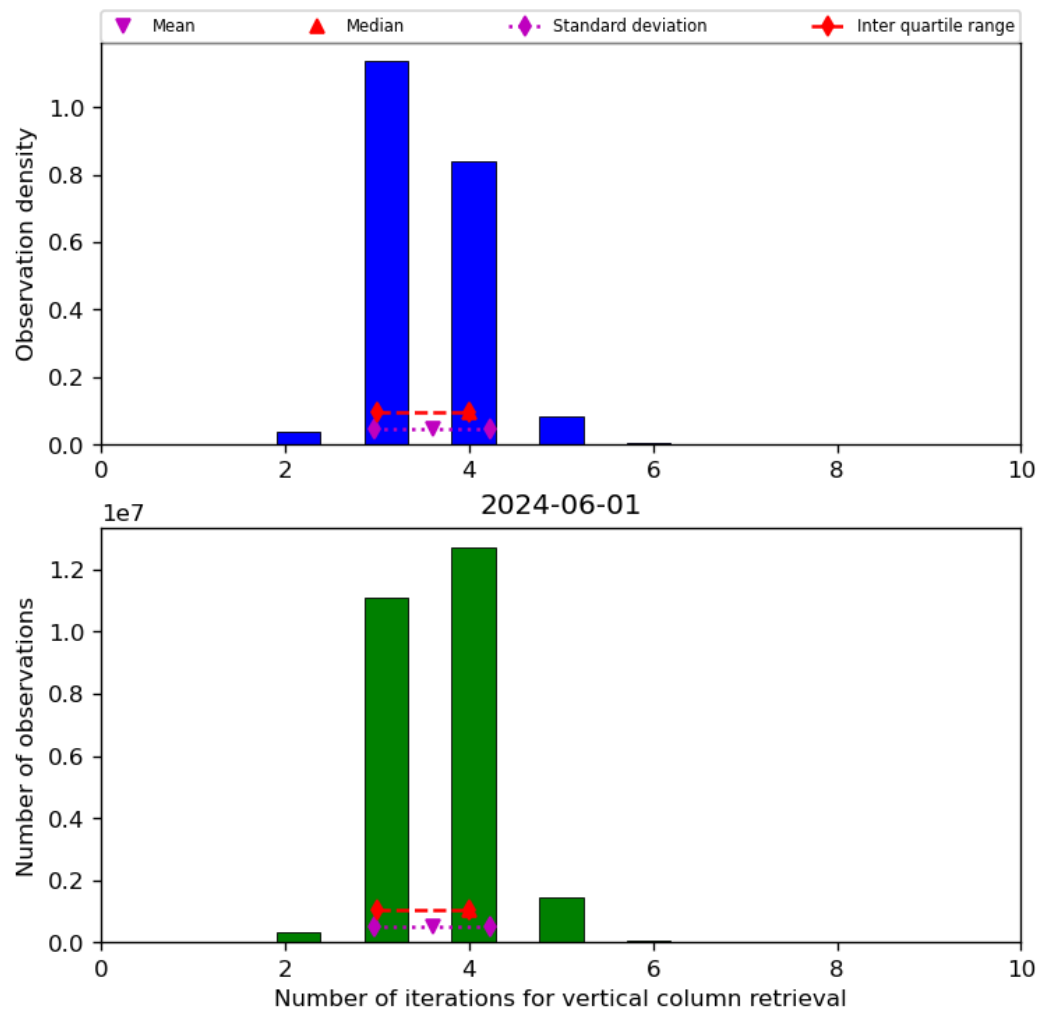
Figure 26: Histogram of “Number of iterations for vertical column retrieval” for 2024-05-31 to 2024-06-02
