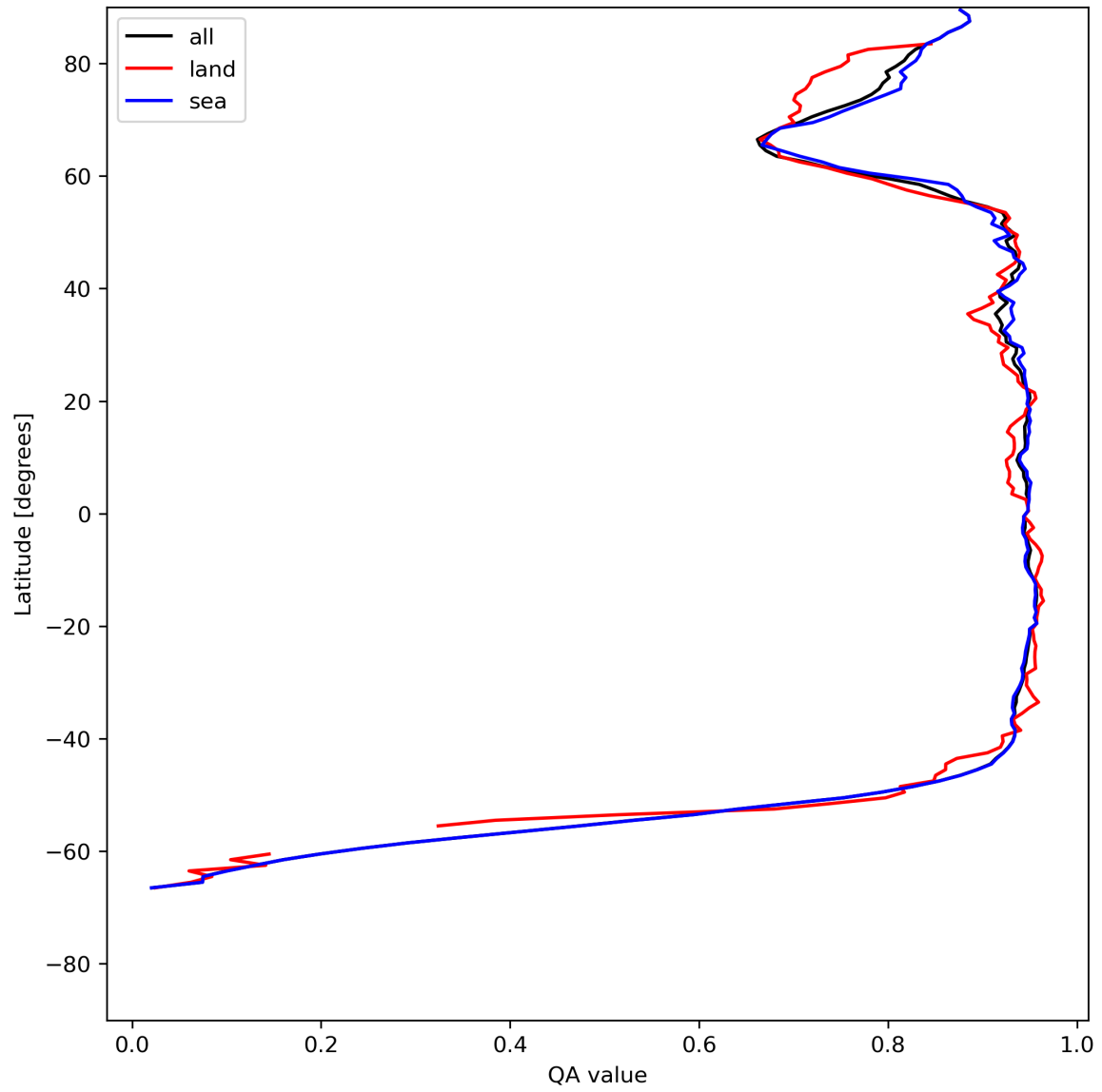
Figure 13: Zonal average of “QA value” for 2024-05-31 to 2024-06-02.
