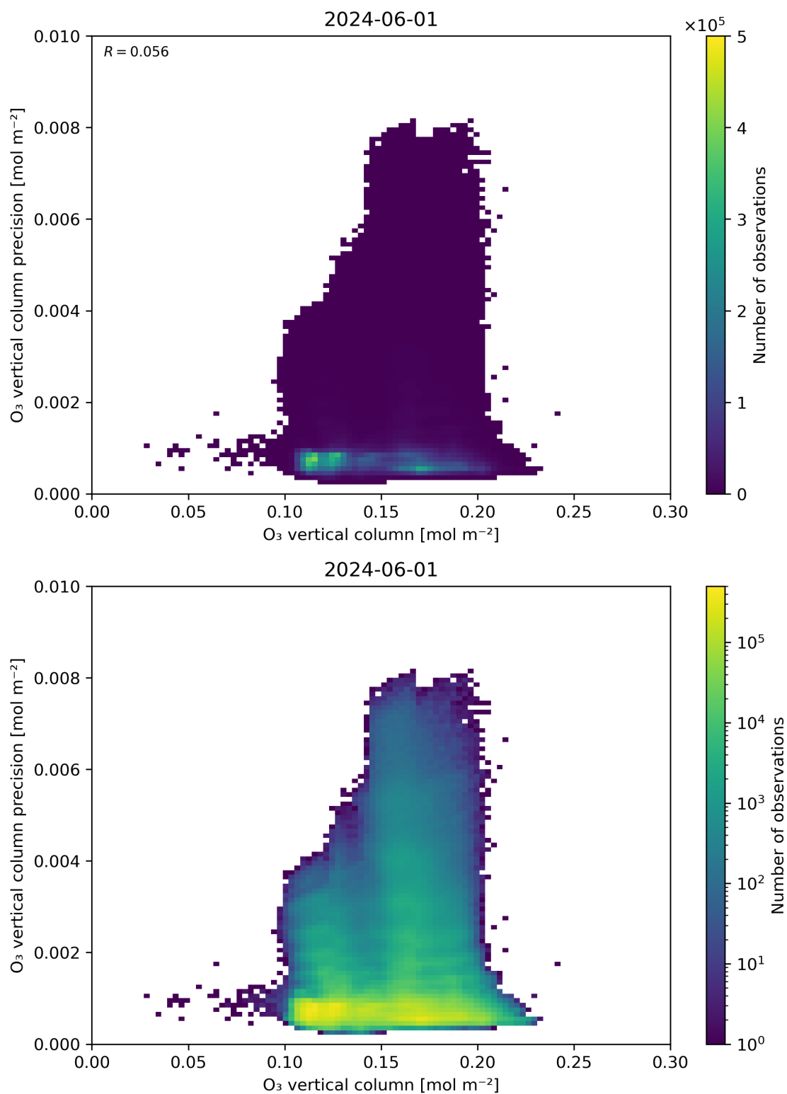
Figure 41: Scatter density plot of “O 3 vertical column” against “O 3 vertical column precision” for 2024-05-31 to 2024-06-02.
