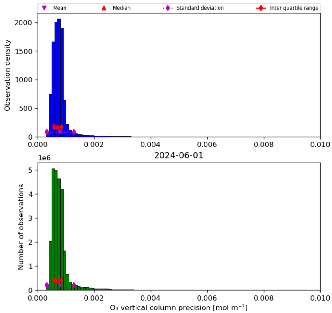
Figure 22: Histogram of “O 3 vertical column precision” for 2024-05-31 to 2024-06-02
