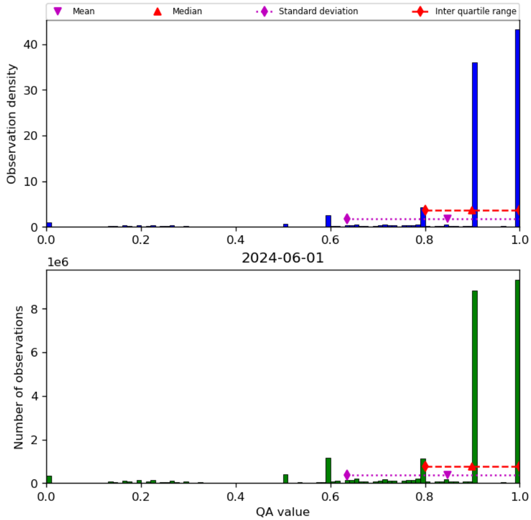
Figure 20: Histogram of “QA value” for 2024-05-31 to 2024-06-02
