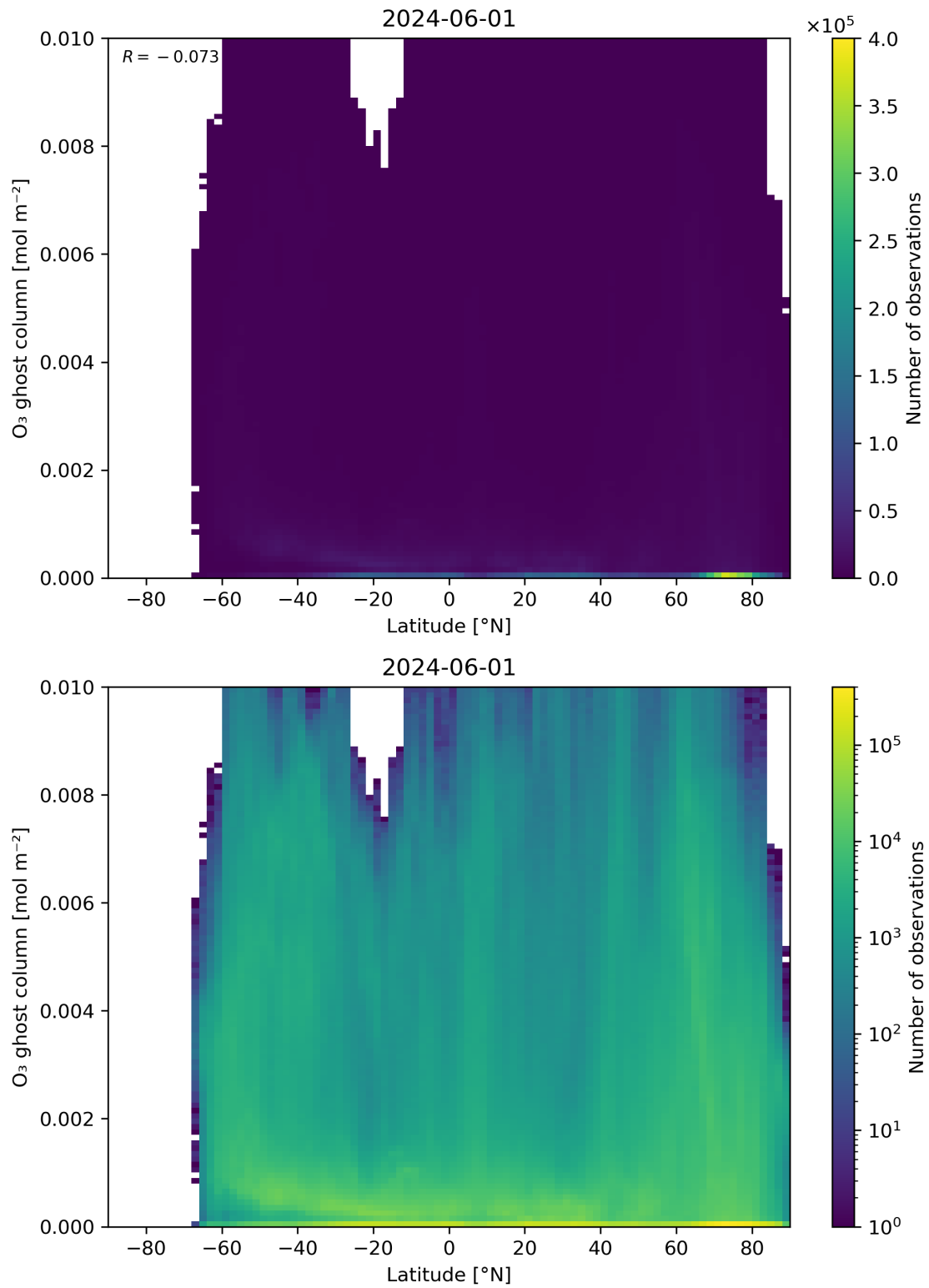
Figure 35: Scatter density plot of “Latitude” against “O 3 ghost column” for 2024-05-31 to 2024-06-02.
