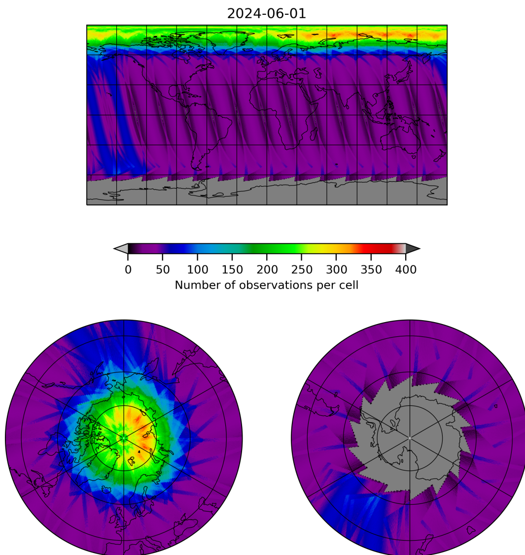
Figure 12: Map of the number of observations for 2024-05-31 to 2024-06-02
