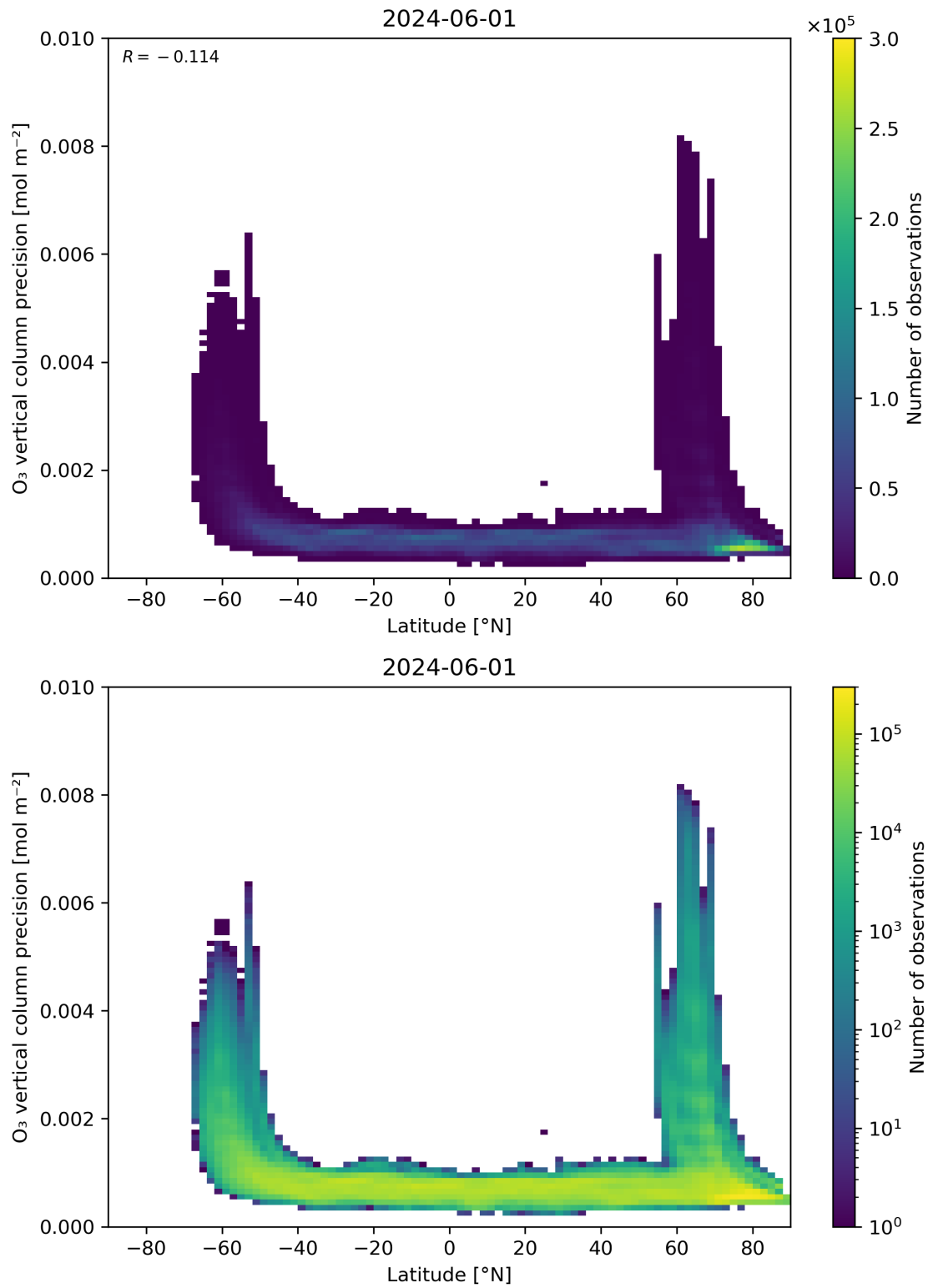
Figure 37: Scatter density plot of “Latitude” against “O 3 vertical column precision” for 2024-05-31 to 2024-06-02.
