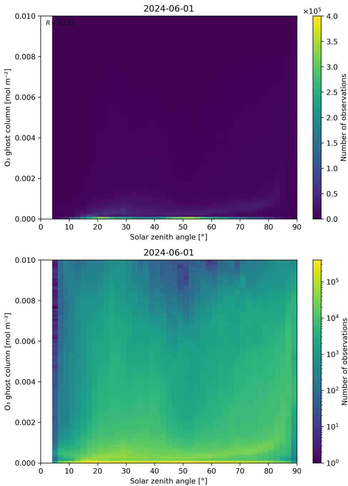
Figure 46: Scatter density plot of “Solar zenith angle” against “O 3 ghost column” for 2024-05-31 to 2024-06-02.
