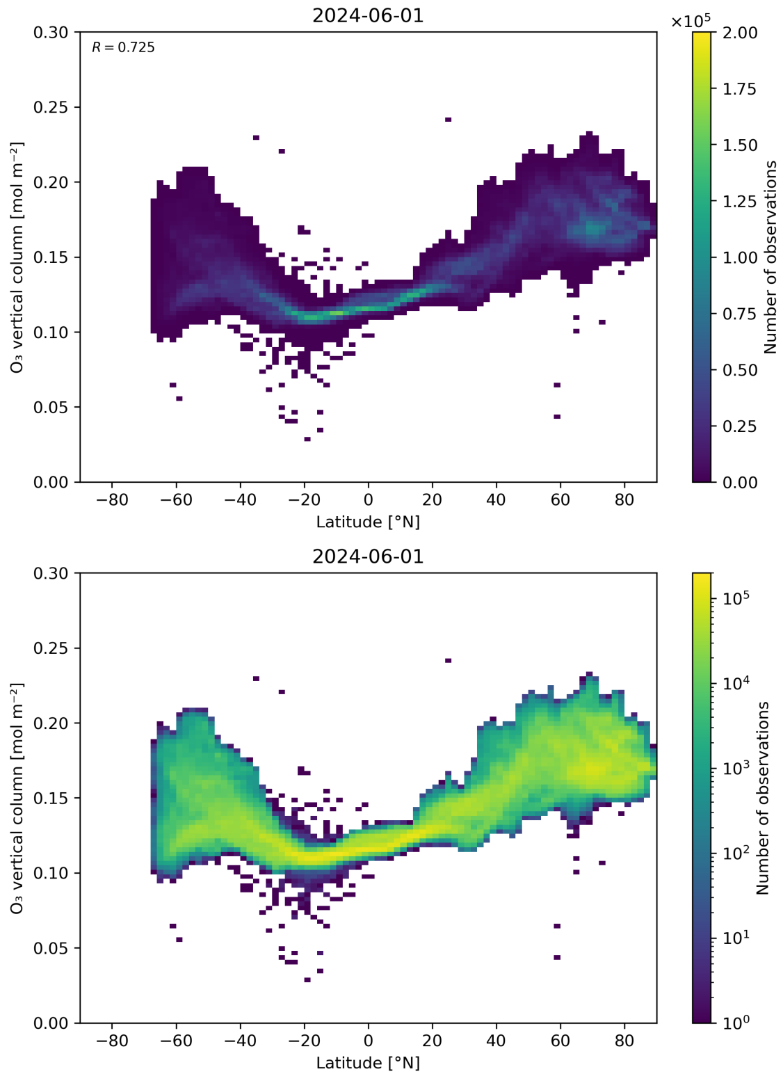
Figure 36: Scatter density plot of “Latitude” against “O 3 vertical column” for 2024-05-31 to 2024-06-02.
