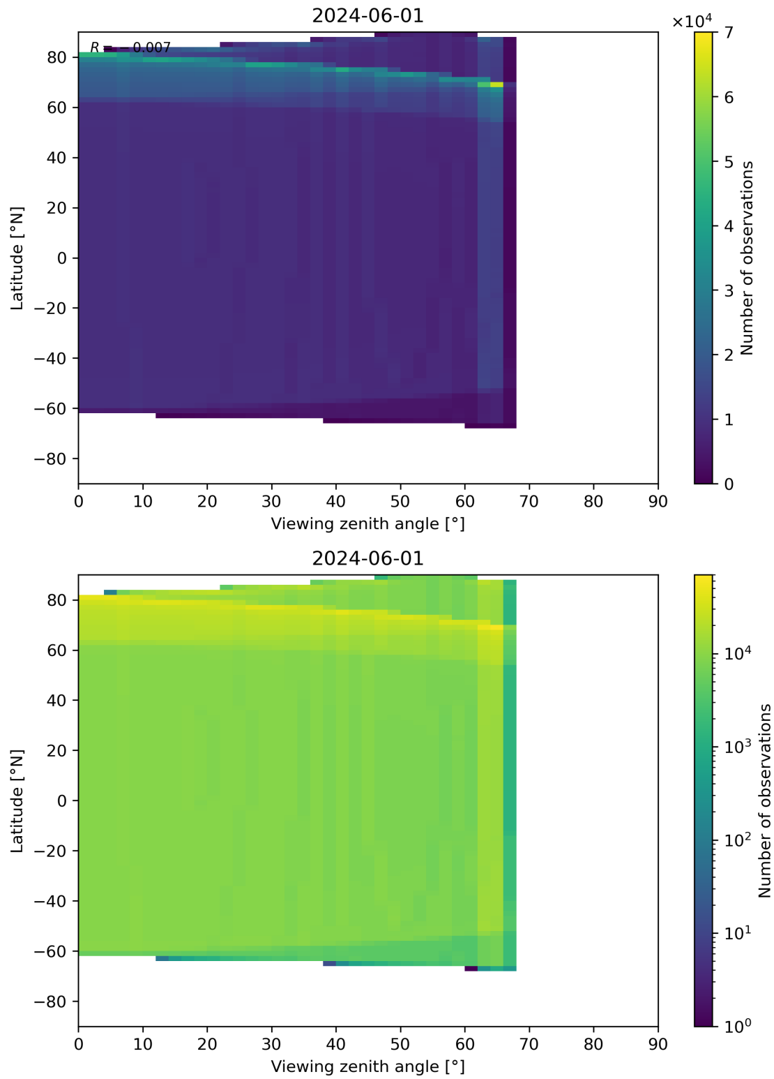
Figure 49: Scatter density plot of “Viewing zenith angle” against “Latitude” for 2024-05-31 to 2024-06-02.
