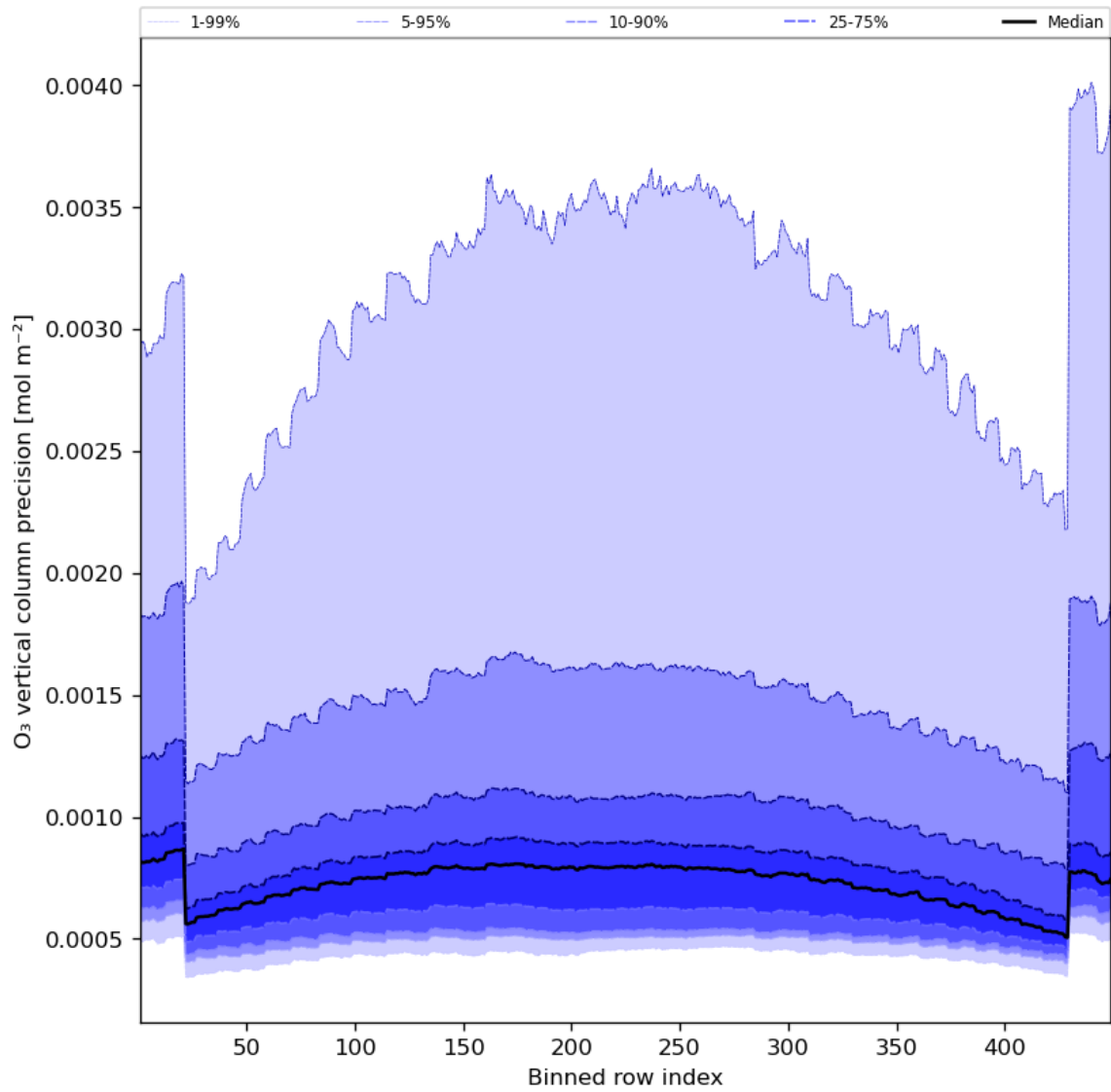
Figure 29: Along track statistics of “O 3 vertical column precision” for 2024-05-31 to 2024-06-02
