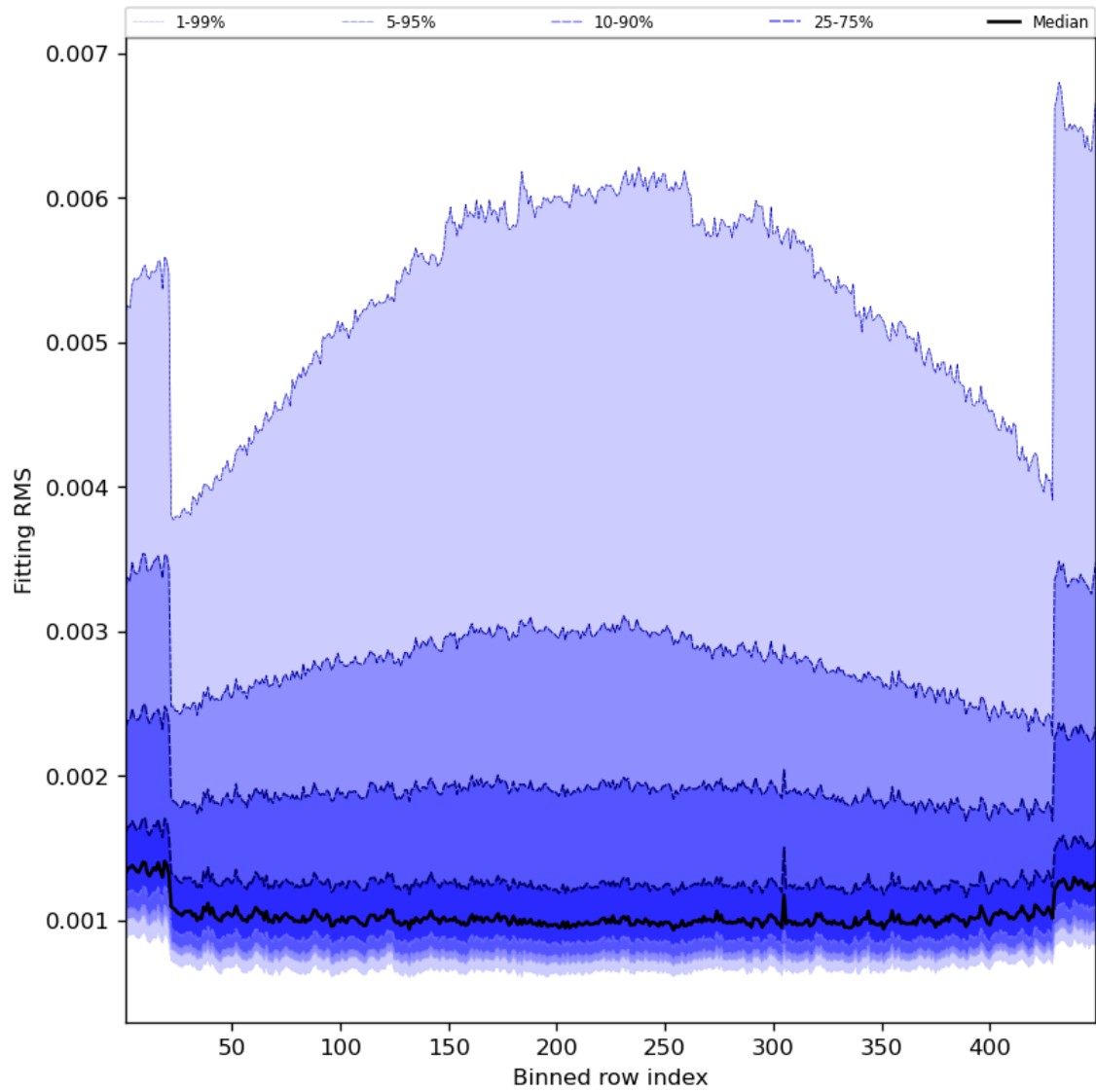
Figure 30: Along track statistics of “Fitting RMS” for 2024-05-31 to 2024-06-02
