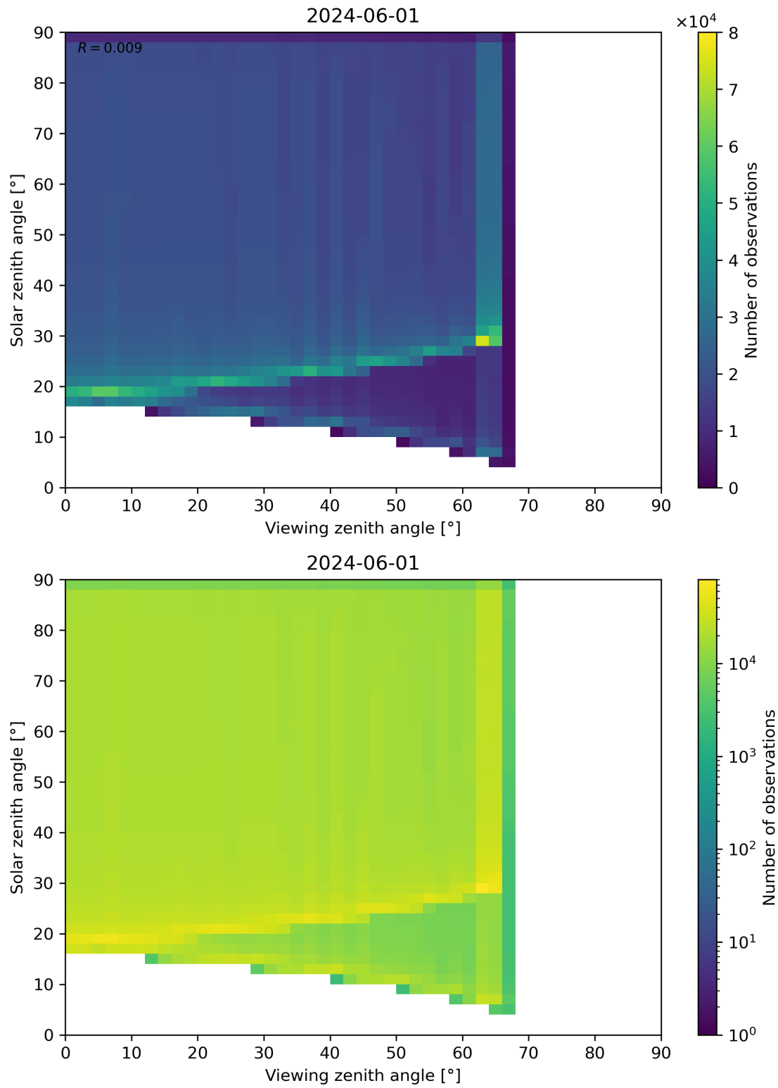
Figure 54: Scatter density plot of “Viewing zenith angle” against “Solar zenith angle” for 2024-05-31 to 2024-06-02.
