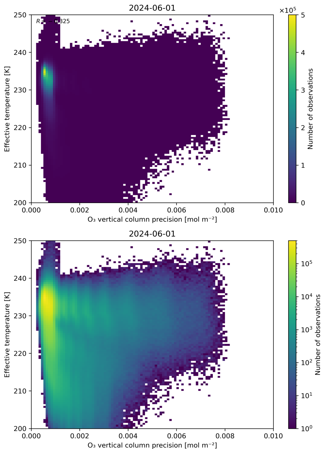
Figure 42: Scatter density plot of “O 3 vertical column precision” against “Effective temperature” for 2024-05-31 to 2024-06-02.
