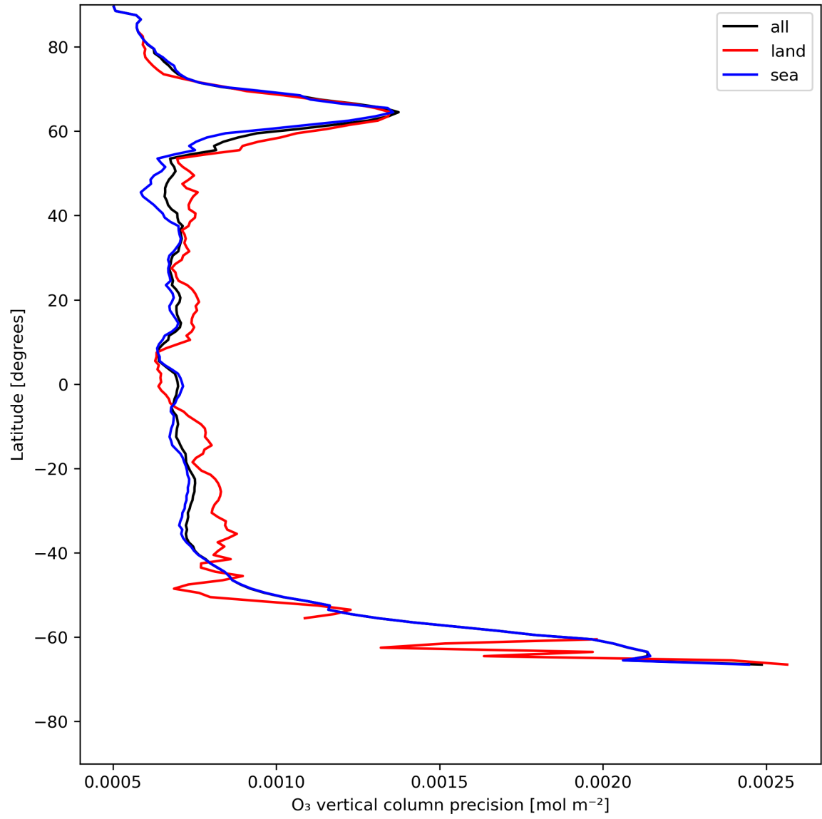
Figure 15: Zonal average of “O 3 vertical column precision” for 2024-05-31 to 2024-06-02.
