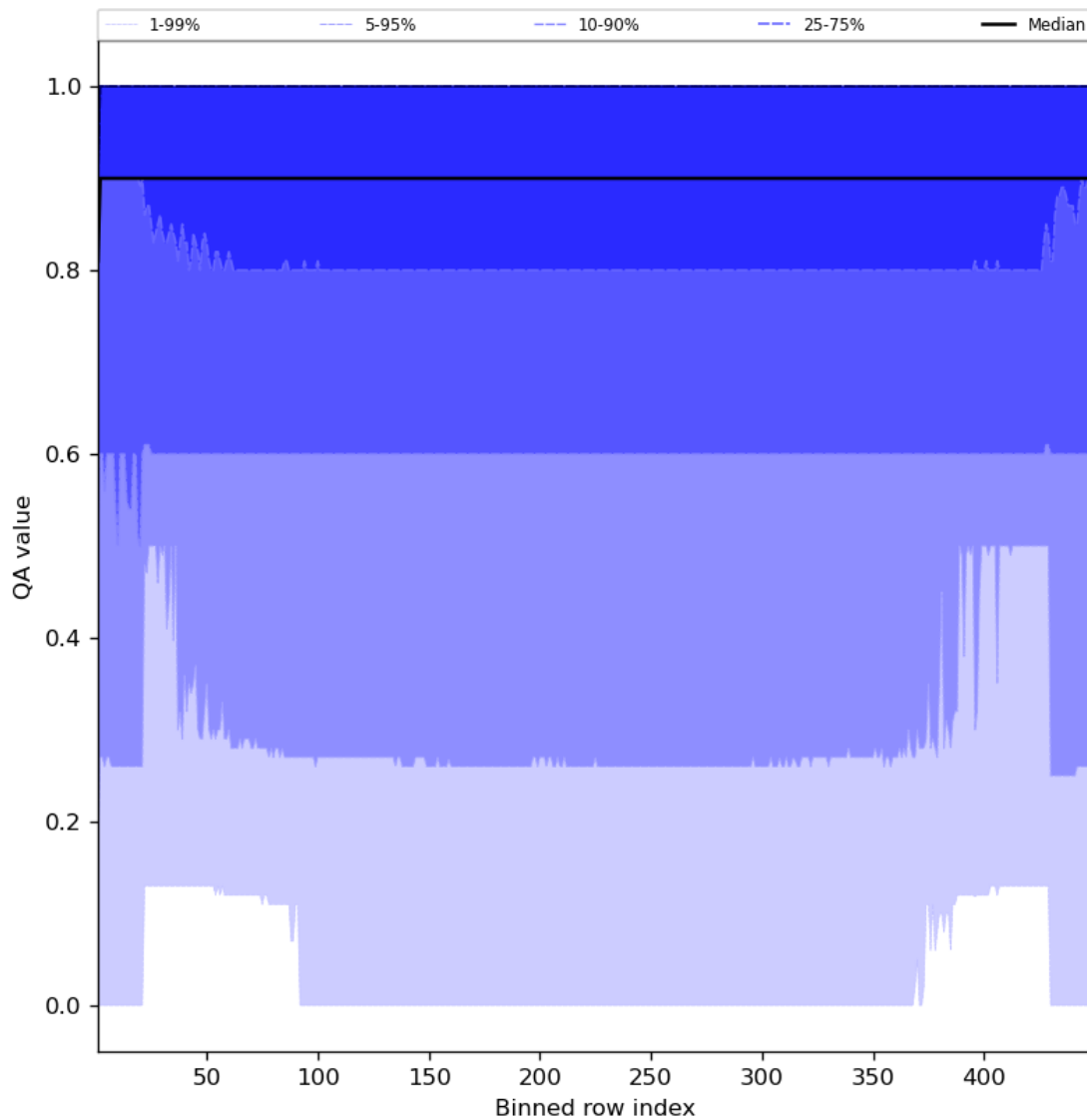
Figure 27: Along track statistics of “QA value” for 2024-05-31 to 2024-06-02
