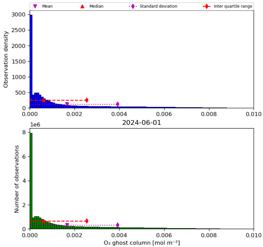
Figure 25: Histogram of “O 3 ghost column” for 2024-05-31 to 2024-06-02
