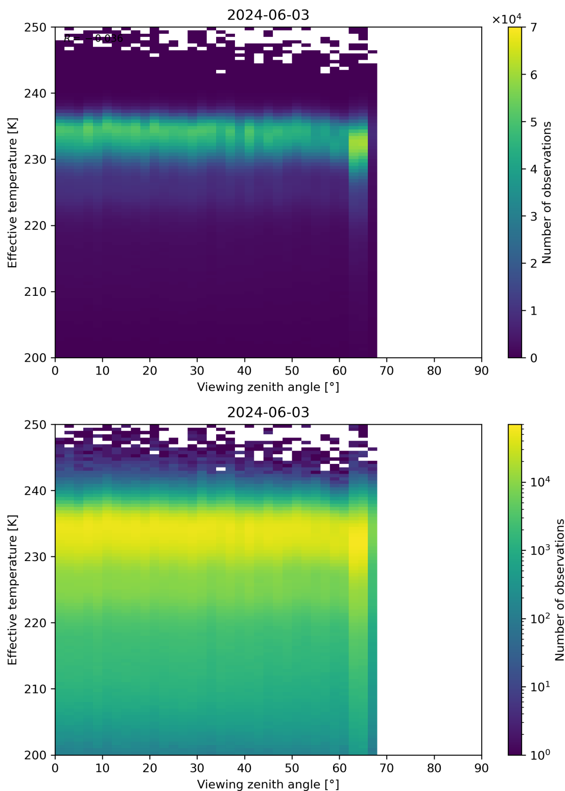
Figure 50: Scatter density plot of “Viewing zenith angle” against “Effective temperature” for 2024-06-03 to 2024-06-04.
