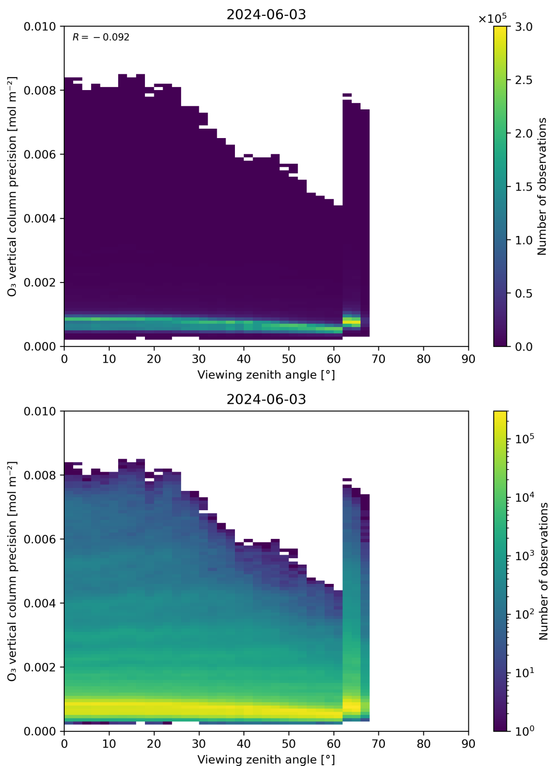
Figure 53: Scatter density plot of “Viewing zenith angle” against “O 3 vertical column precision” for 2024-06-03 to 2024-06-04.
