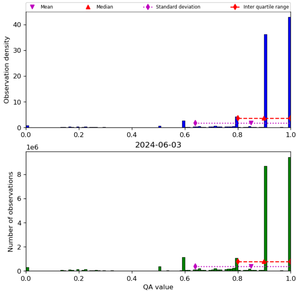
Figure 20: Histogram of “QA value” for 2024-06-03 to 2024-06-04
