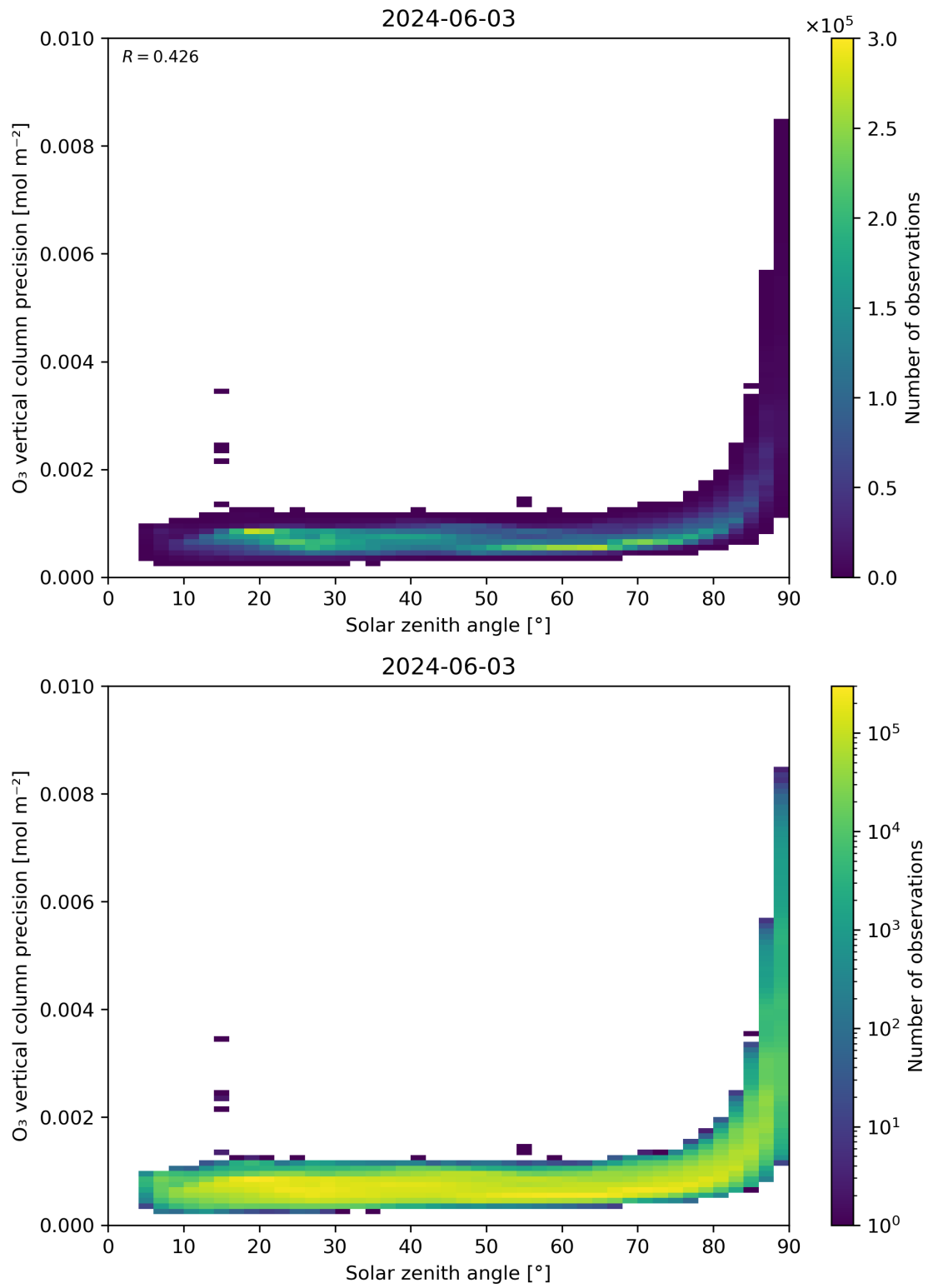
Figure 48: Scatter density plot of “Solar zenith angle” against “O 3 vertical column precision” for 2024-06-03 to 2024-06-04.
