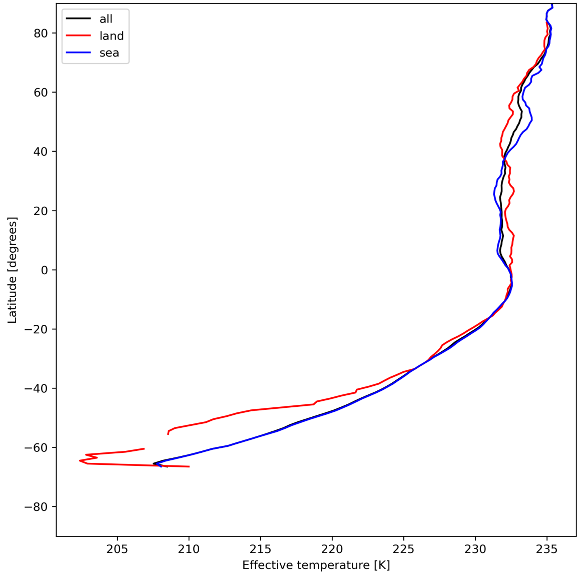
Figure 17: Zonal average of "Effective temperature" for 2024-06-03 to 2024-06-04.
