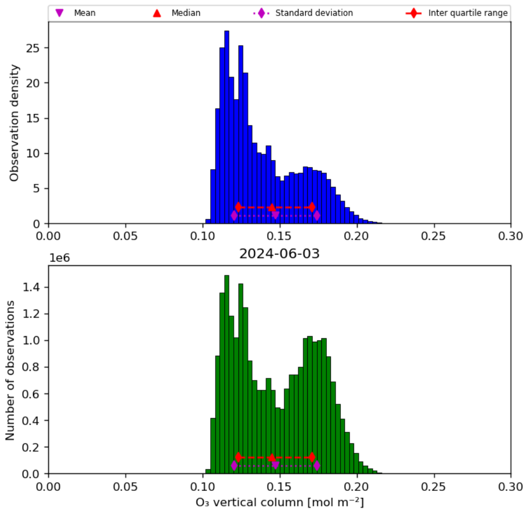
Figure 21: Histogram of “O 3 vertical column” for 2024-06-03 to 2024-06-04
