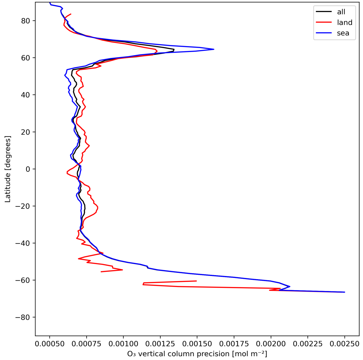
Figure 15: Zonal average of "O 3 vertical column precision" for 2024-06-03 to 2024-06-04.
