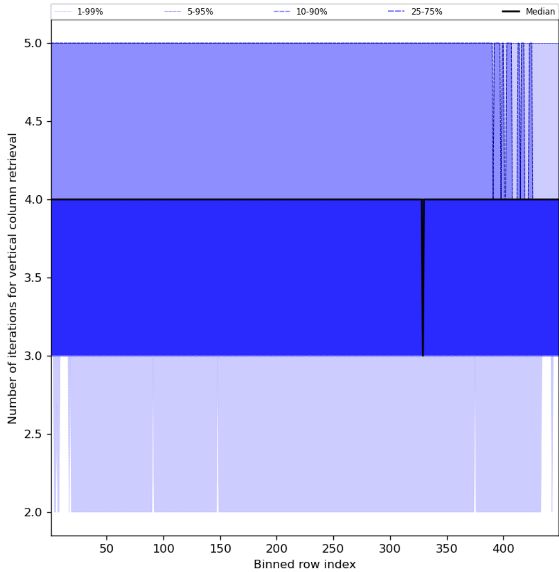
Figure 33: Along track statistics of “Number of iterations for vertical column retrieval” for 2024-06-03 to 2024-06-04
