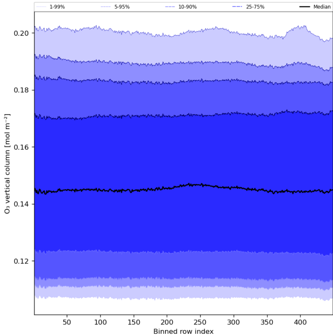
Figure 28: Along track statistics of “O 3 vertical column” for 2024-06-03 to 2024-06-04
