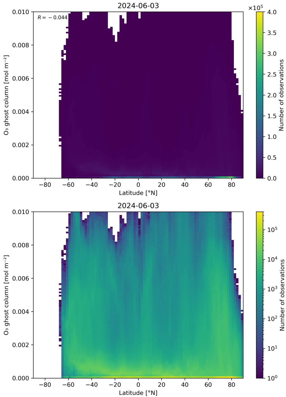
Figure 35: Scatter density plot of “Latitude” against “O 3 ghost column” for 2024-06-03 to 2024-06-04.
