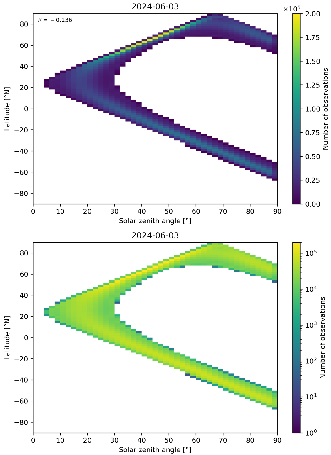
Figure 44: Scatter density plot of “Solar zenith angle” against “Latitude” for 2024-06-03 to 2024-06-04.
