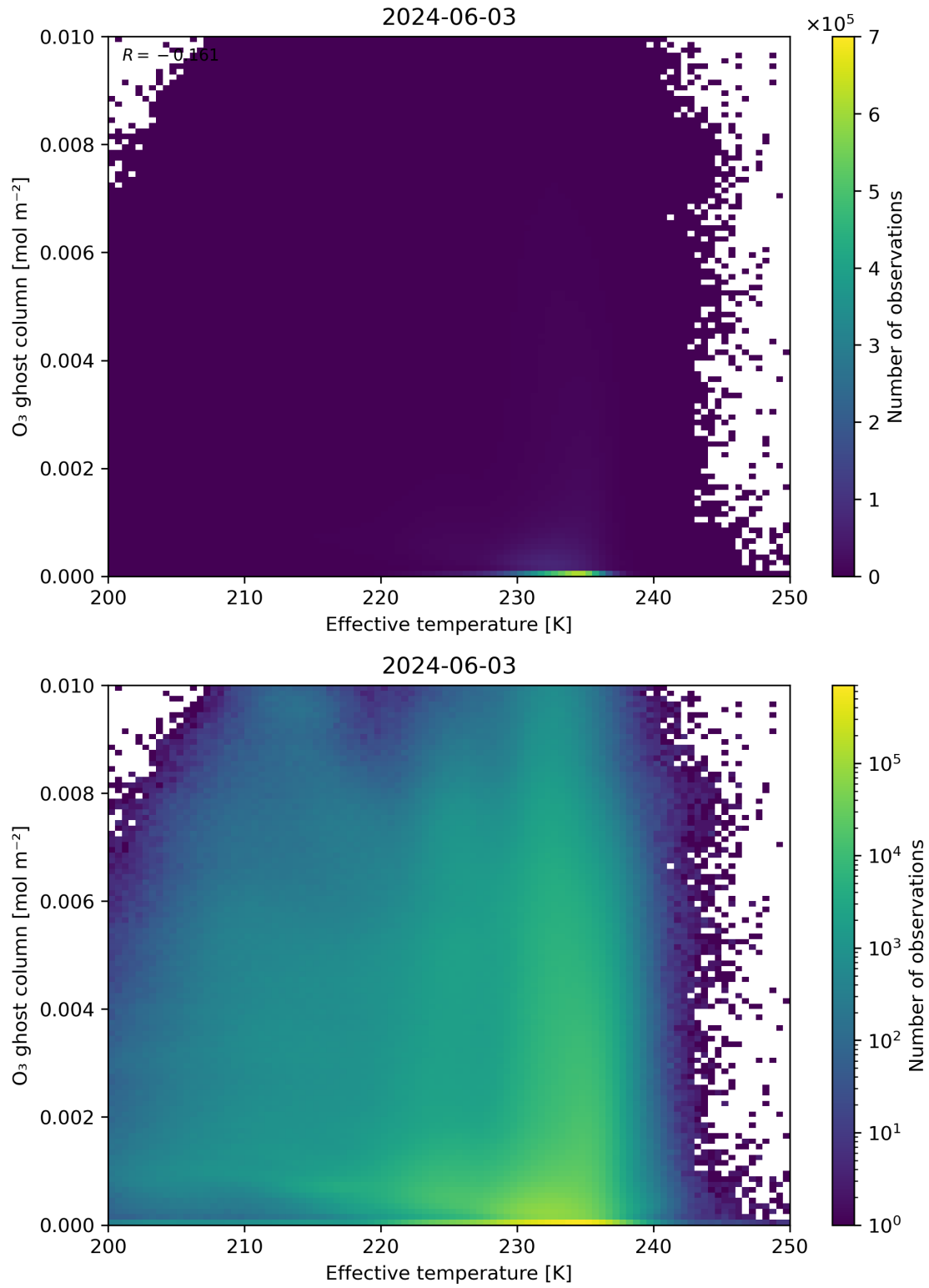
Figure 38: Scatter density plot of “Effective temperature” against “O 3 ghost column” for 2024-06-03 to 2024-06-04.
