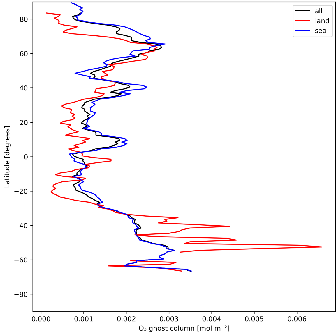
Figure 18: Zonal average of “O 3 ghost column” for 2024-06-03 to 2024-06-04.
