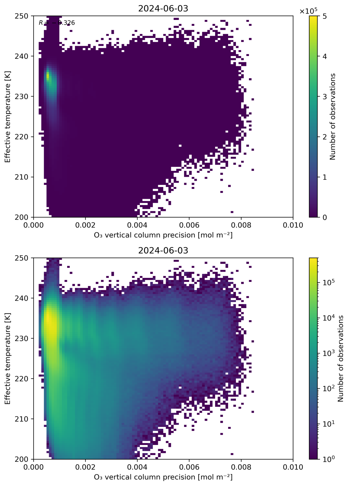
Figure 42: Scatter density plot of “O 3 vertical column precision” against “Effective temperature” for 2024-06-03 to 2024-06-04.
