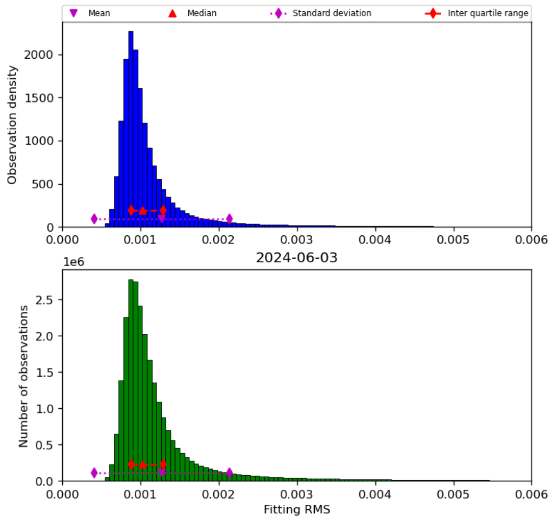
Figure 23: Histogram of “Fitting RMS” for 2024-06-03 to 2024-06-04
