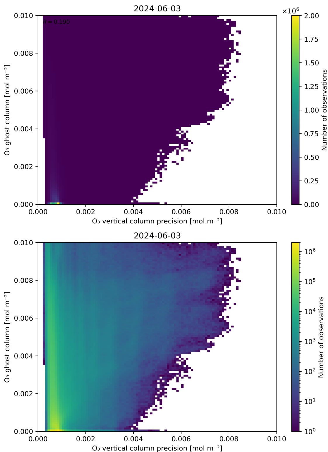
Figure 43: Scatter density plot of “O 3 vertical column precision” against “O 3 ghost column” for 2024-06-03 to 2024-06-04.
