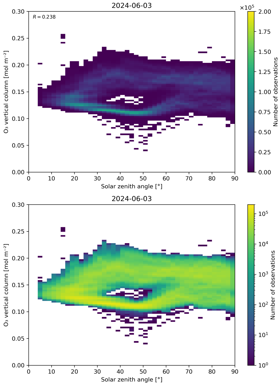
Figure 47: Scatter density plot of “Solar zenith angle” against “O 3 vertical column” for 2024-06-03 to 2024-06-04.
