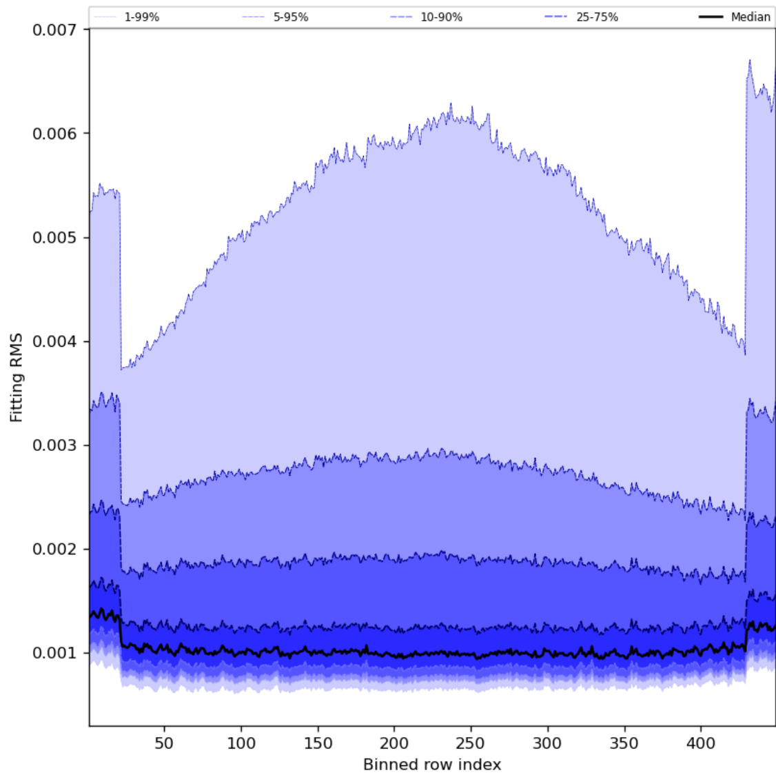
Figure 30: Along track statistics of “Fitting RMS” for 2024-06-03 to 2024-06-04
