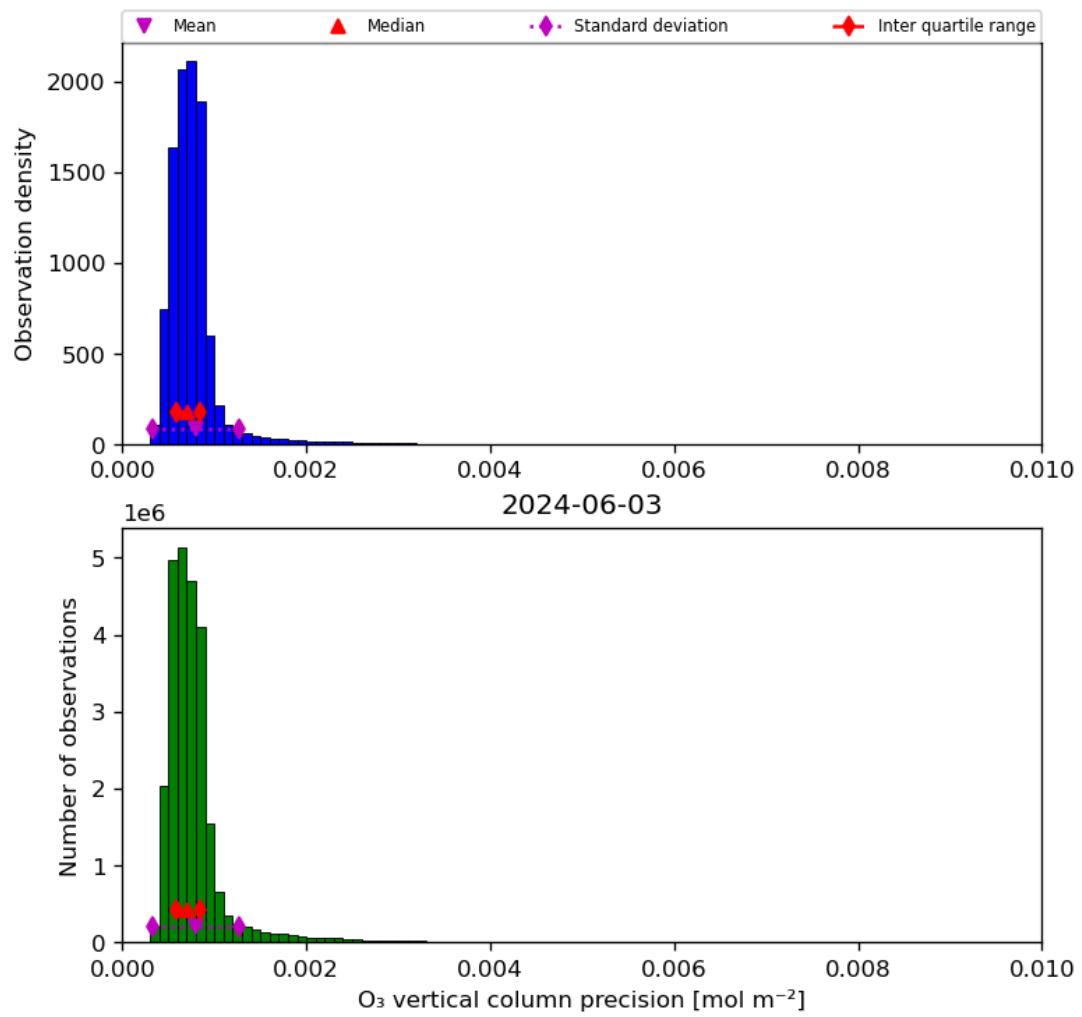
Figure 22: Histogram of “O 3 vertical column precision” for 2024-06-03 to 2024-06-04
