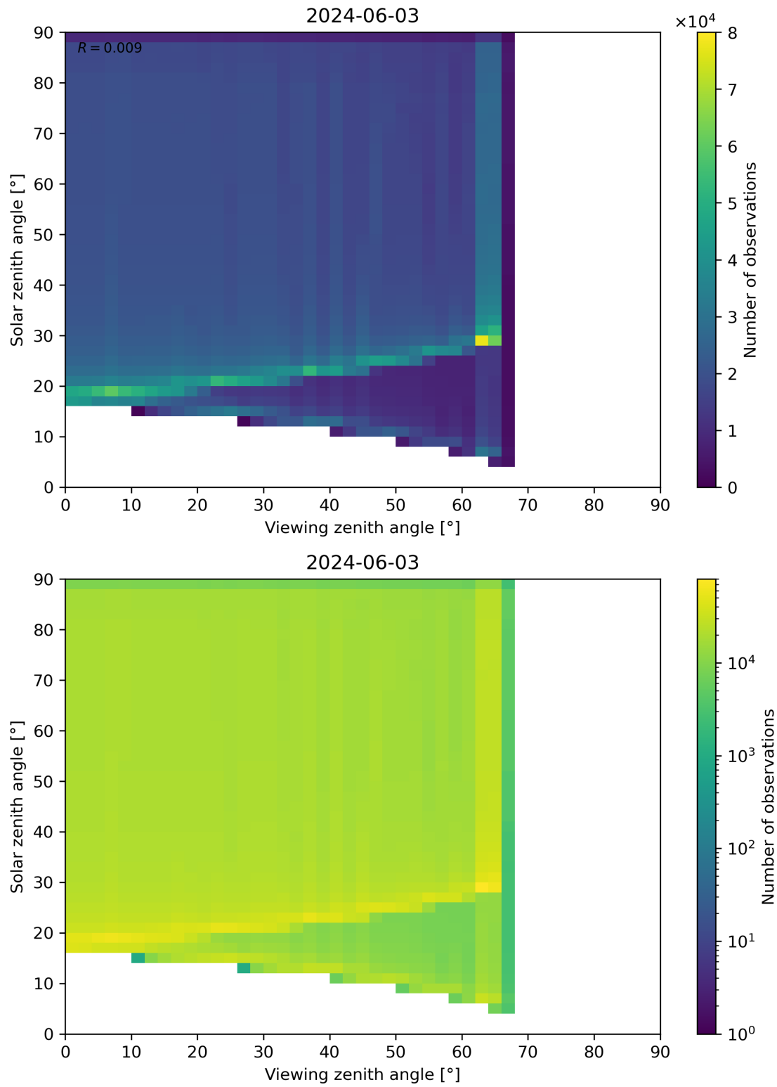
Figure 54: Scatter density plot of “Viewing zenith angle” against “Solar zenith angle” for 2024-06-03 to 2024-06-04.
