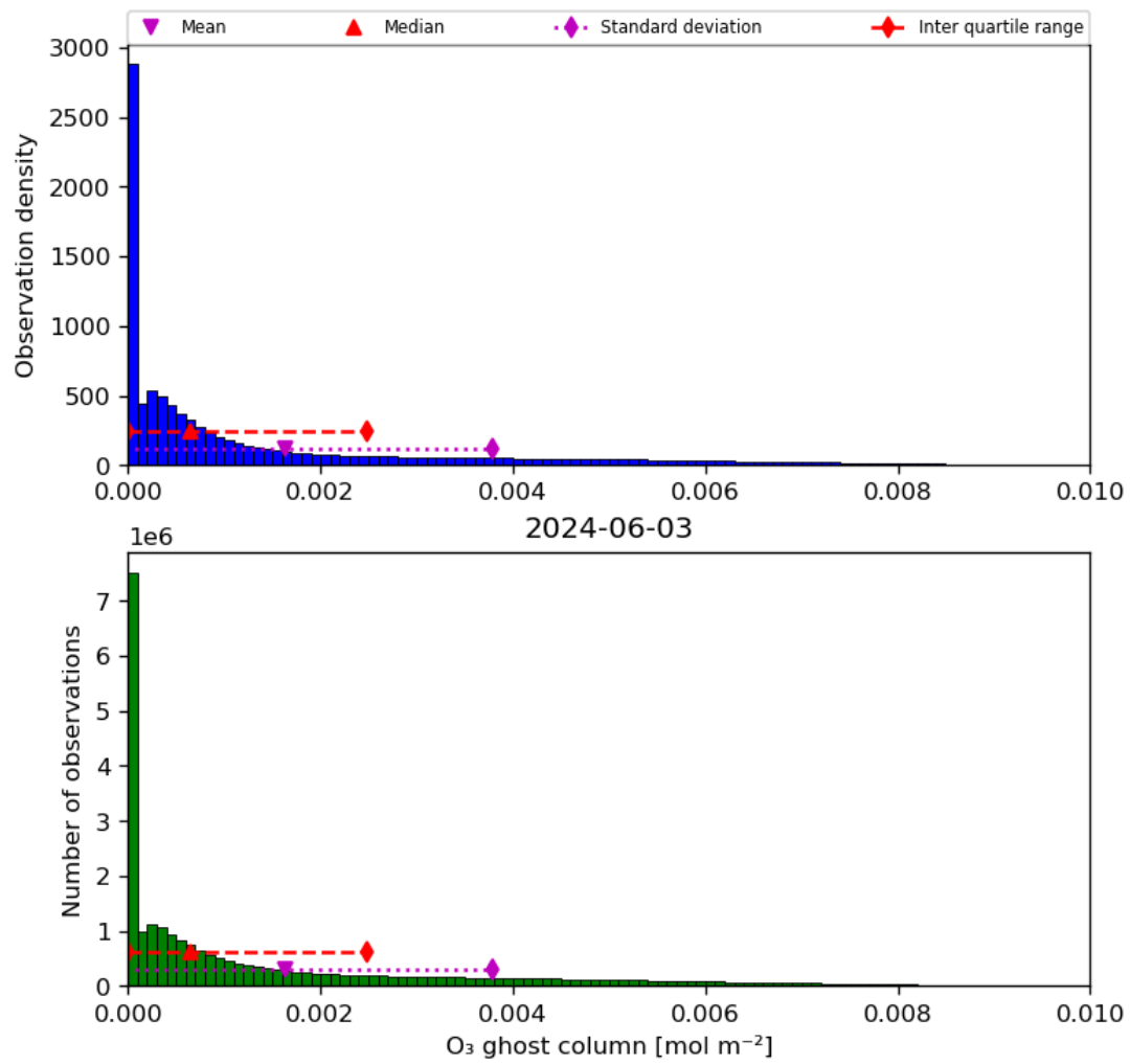
Figure 25: Histogram of “O 3 ghost column” for 2024-06-03 to 2024-06-04
