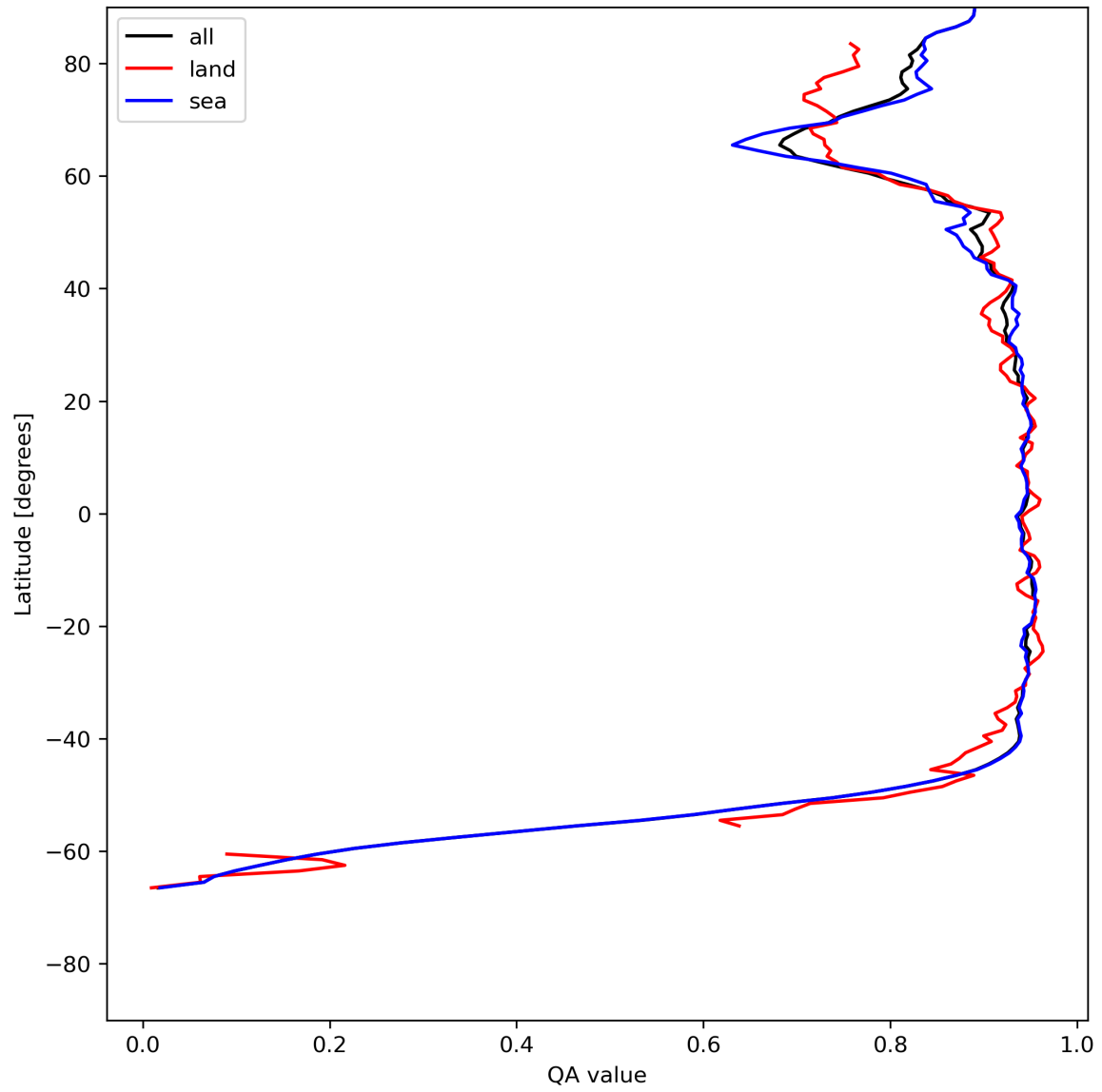
Figure 13: Zonal average of “QA value” for 2024-06-03 to 2024-06-04.
