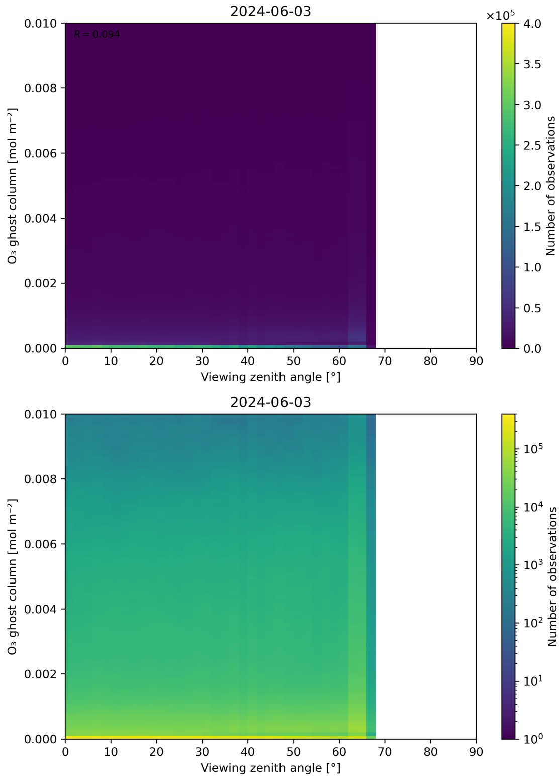
Figure 51: Scatter density plot of “Viewing zenith angle” against “O 3 ghost column” for 2024-06-03 to 2024-06-04.
