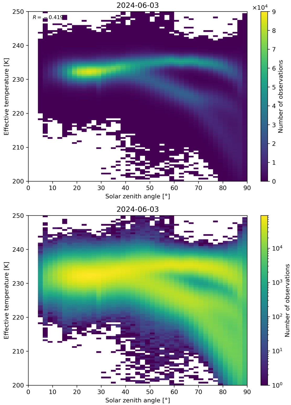
Figure 45: Scatter density plot of “Solar zenith angle” against “Effective temperature” for 2024-06-03 to 2024-06-04.
