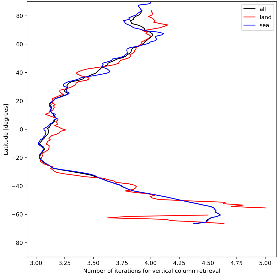
Figure 19: Zonal average of “Number of iterations for vertical column retrieval” for 2024-06-03 to 2024-06-04.
