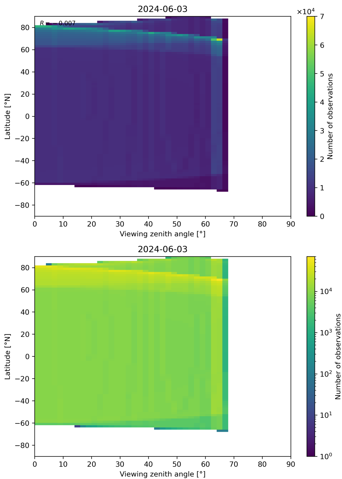
Figure 49: Scatter density plot of “Viewing zenith angle” against “Latitude” for 2024-06-03 to 2024-06-04.
