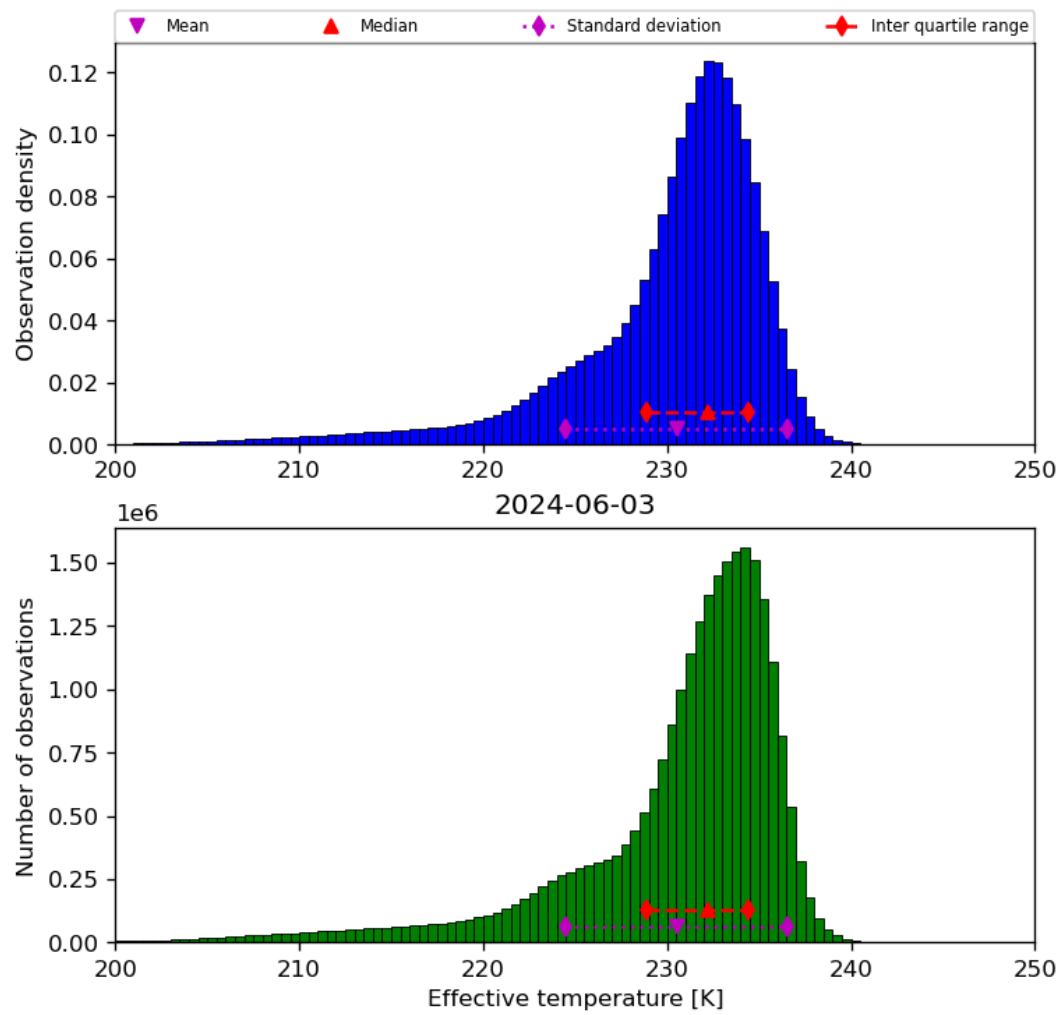
Figure 24: Histogram of “Effective temperature” for 2024-06-03 to 2024-06-04
