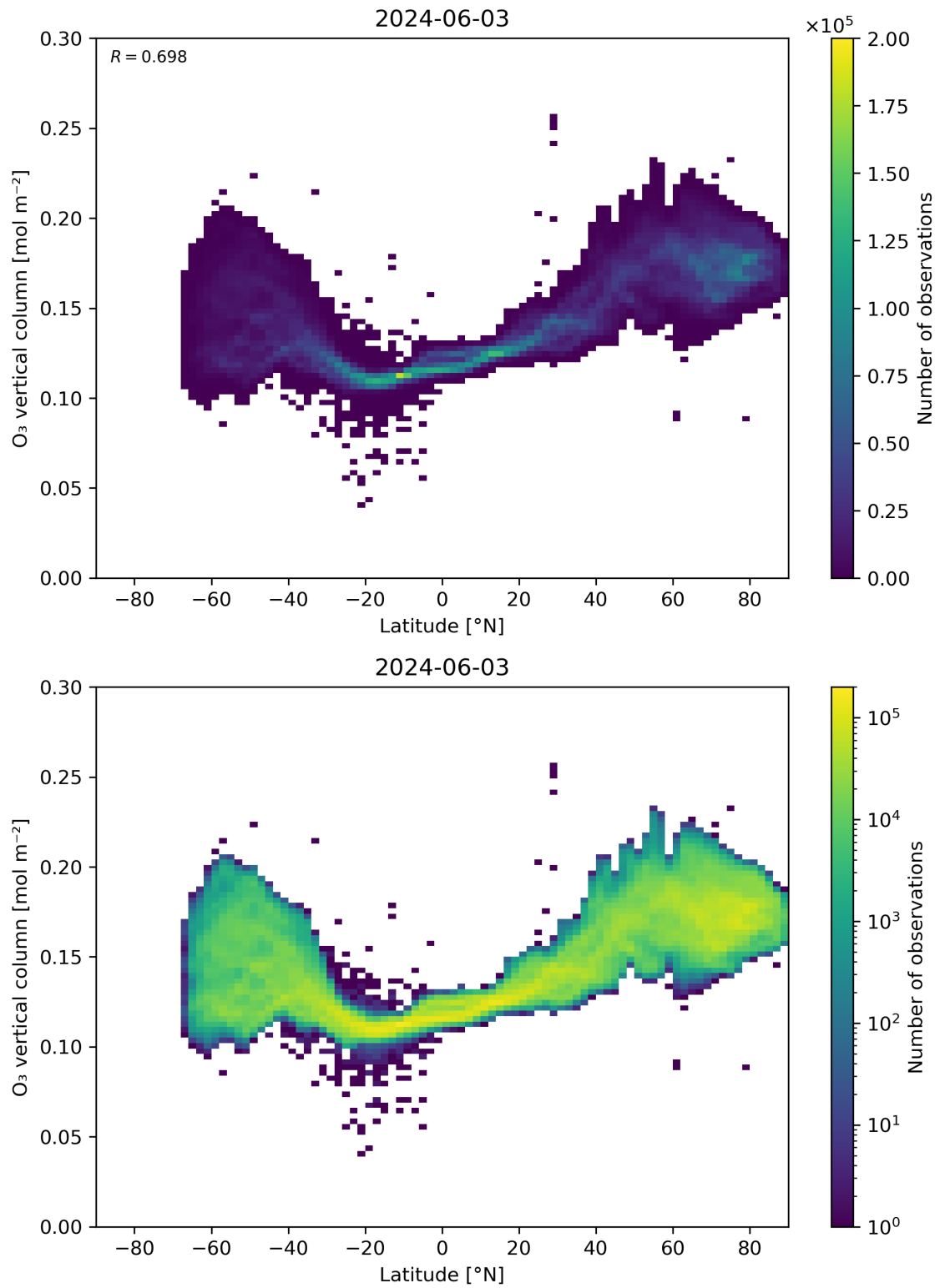
Figure 36: Scatter density plot of “Latitude” against “O 3 vertical column” for 2024-06-03 to 2024-06-04.
