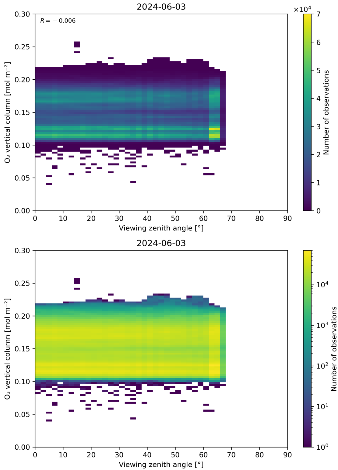
Figure 52: Scatter density plot of “Viewing zenith angle” against “O 3 vertical column” for 2024-06-03 to 2024-06-04.
