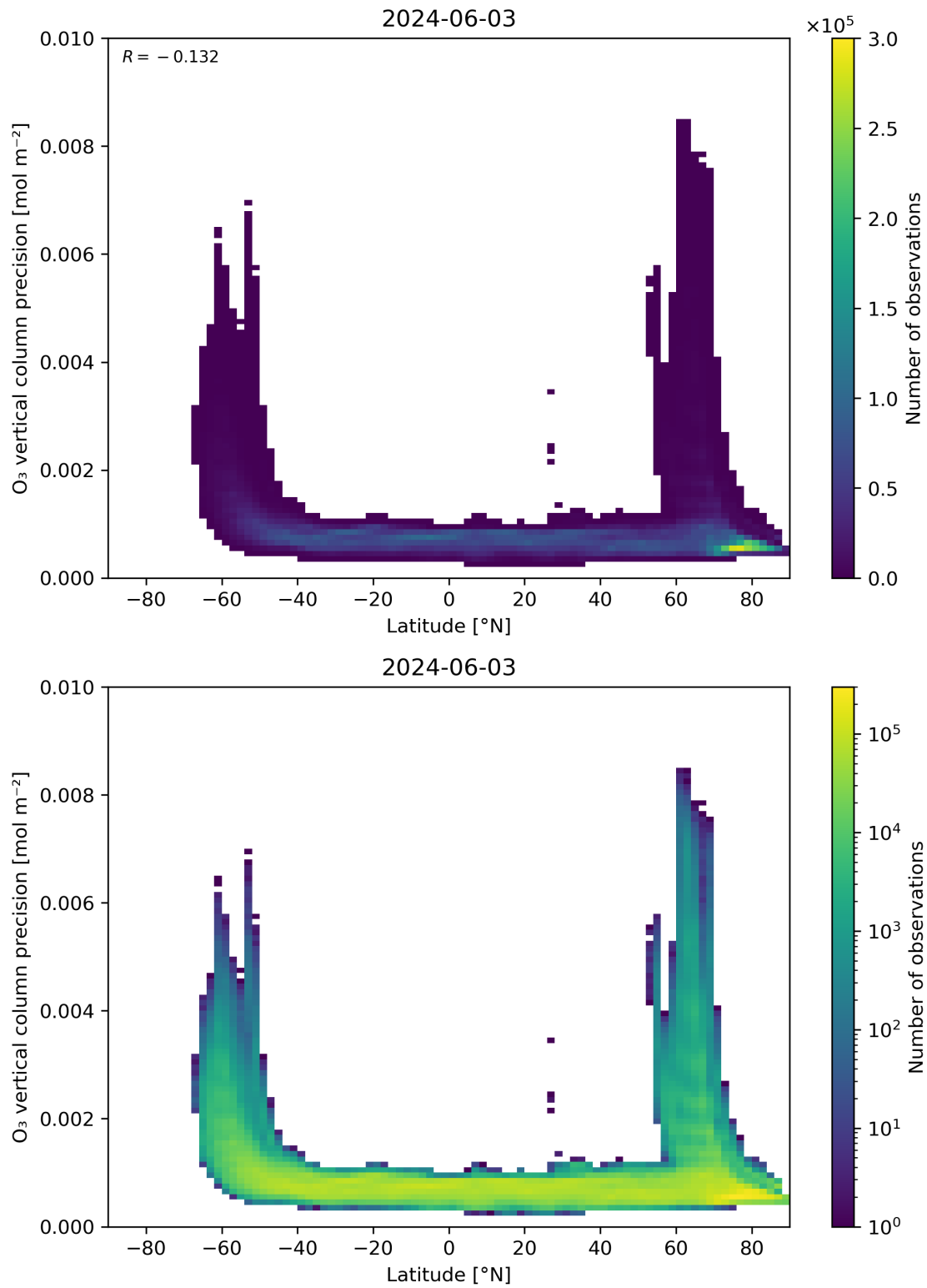
Figure 37: Scatter density plot of “Latitude” against “O 3 vertical column precision” for 2024-06-03 to 2024-06-04.
