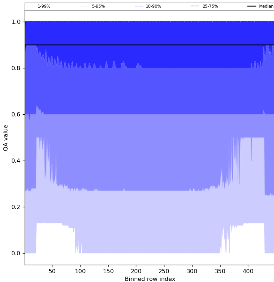
Figure 27: Along track statistics of “QA value” for 2024-06-03 to 2024-06-04
