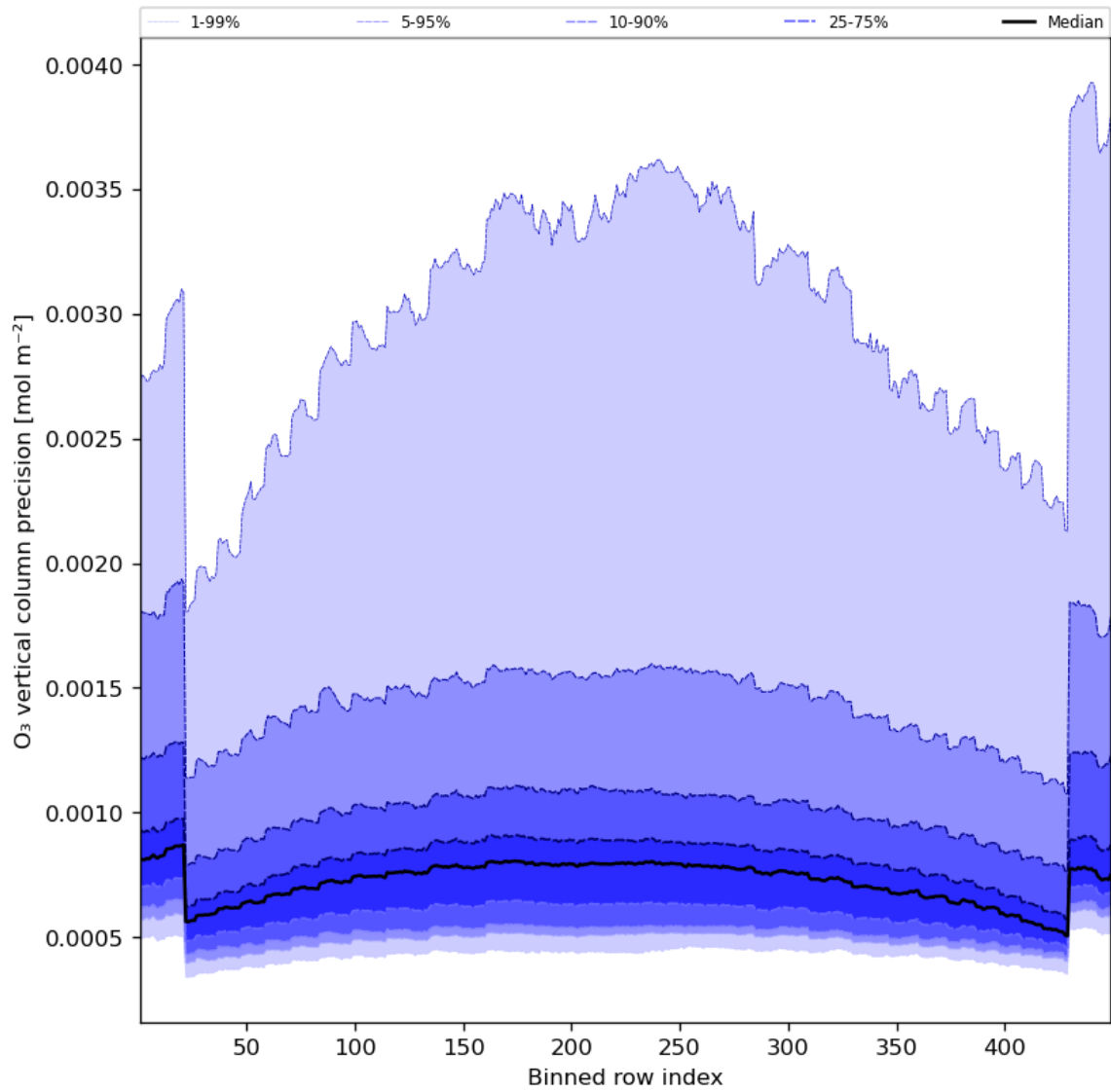
Figure 29: Along track statistics of “O 3 vertical column precision” for 2024-06-03 to 2024-06-04
