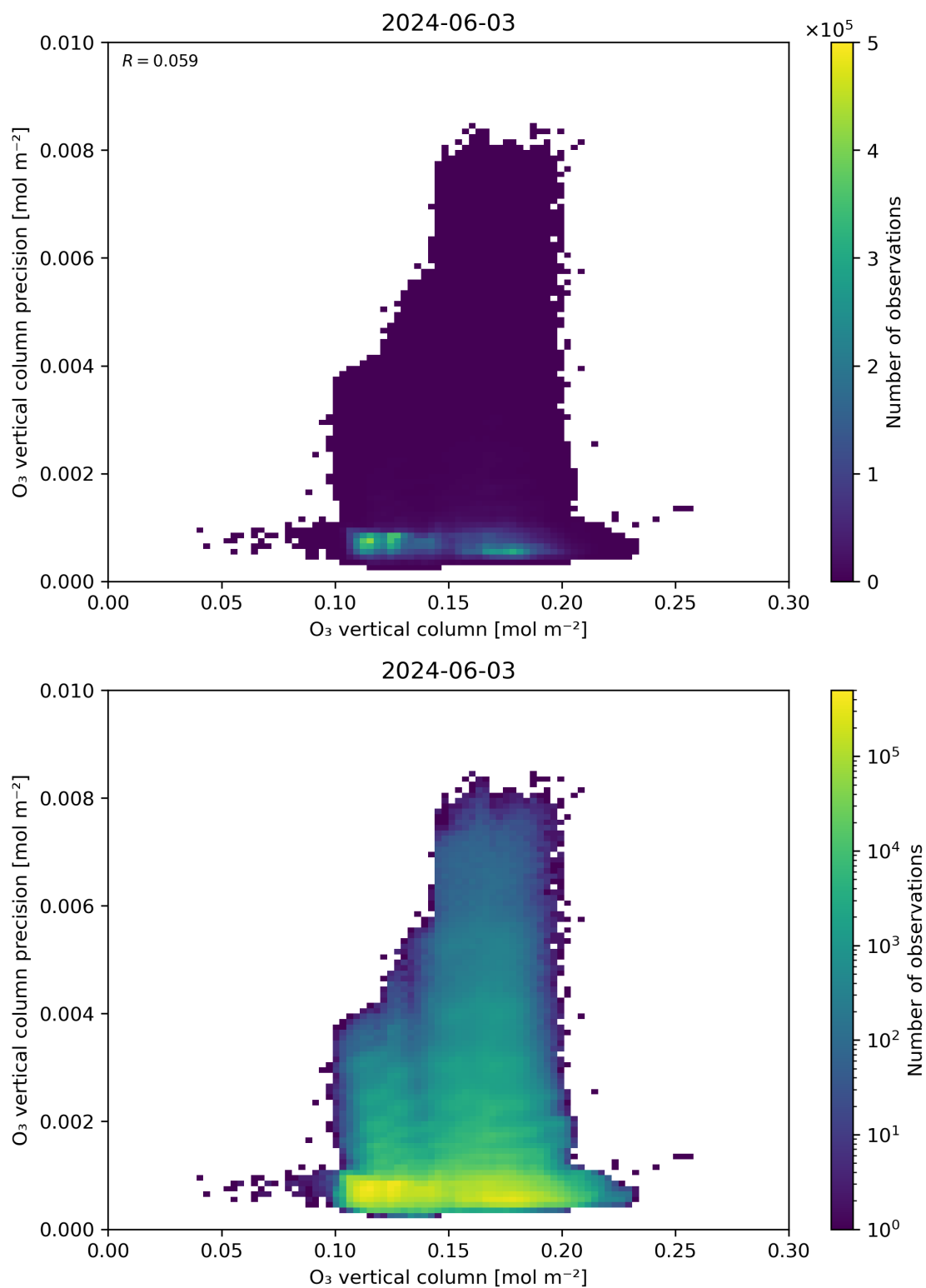
Figure 41: Scatter density plot of “O 3 vertical column” against “O 3 vertical column precision” for 2024-06-03 to 2024-06-04.
