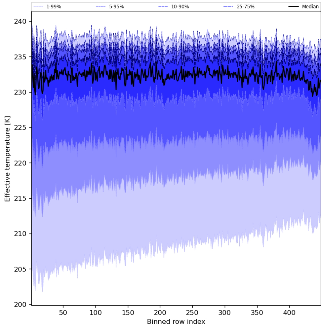
Figure 31: Along track statistics of “Effective temperature” for 2024-06-03 to 2024-06-04
