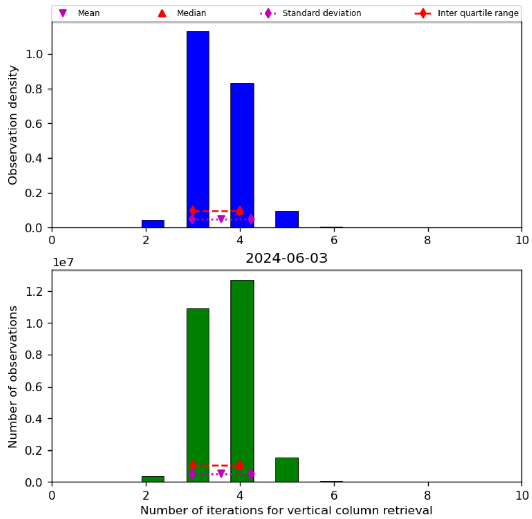
Figure 26: Histogram of “Number of iterations for vertical column retrieval” for 2024-06-03 to 2024-06-04
