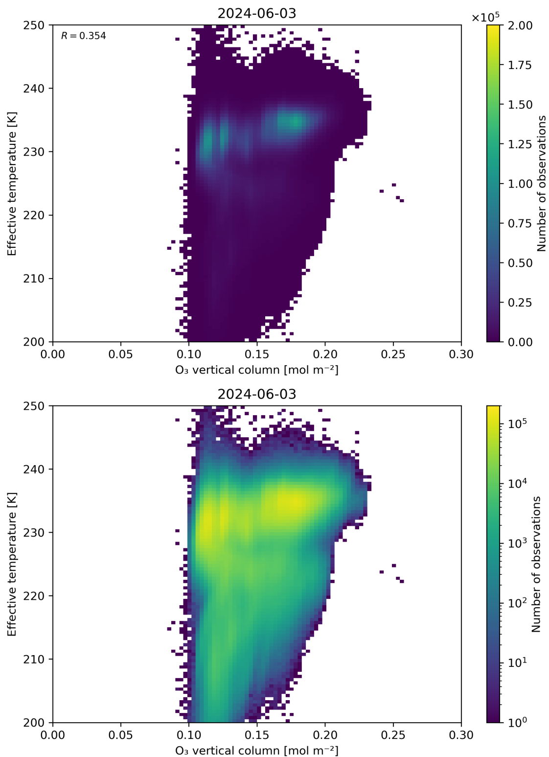
Figure 39: Scatter density plot of “O 3 vertical column” against “Effective temperature” for 2024-06-03 to 2024-06-04.
