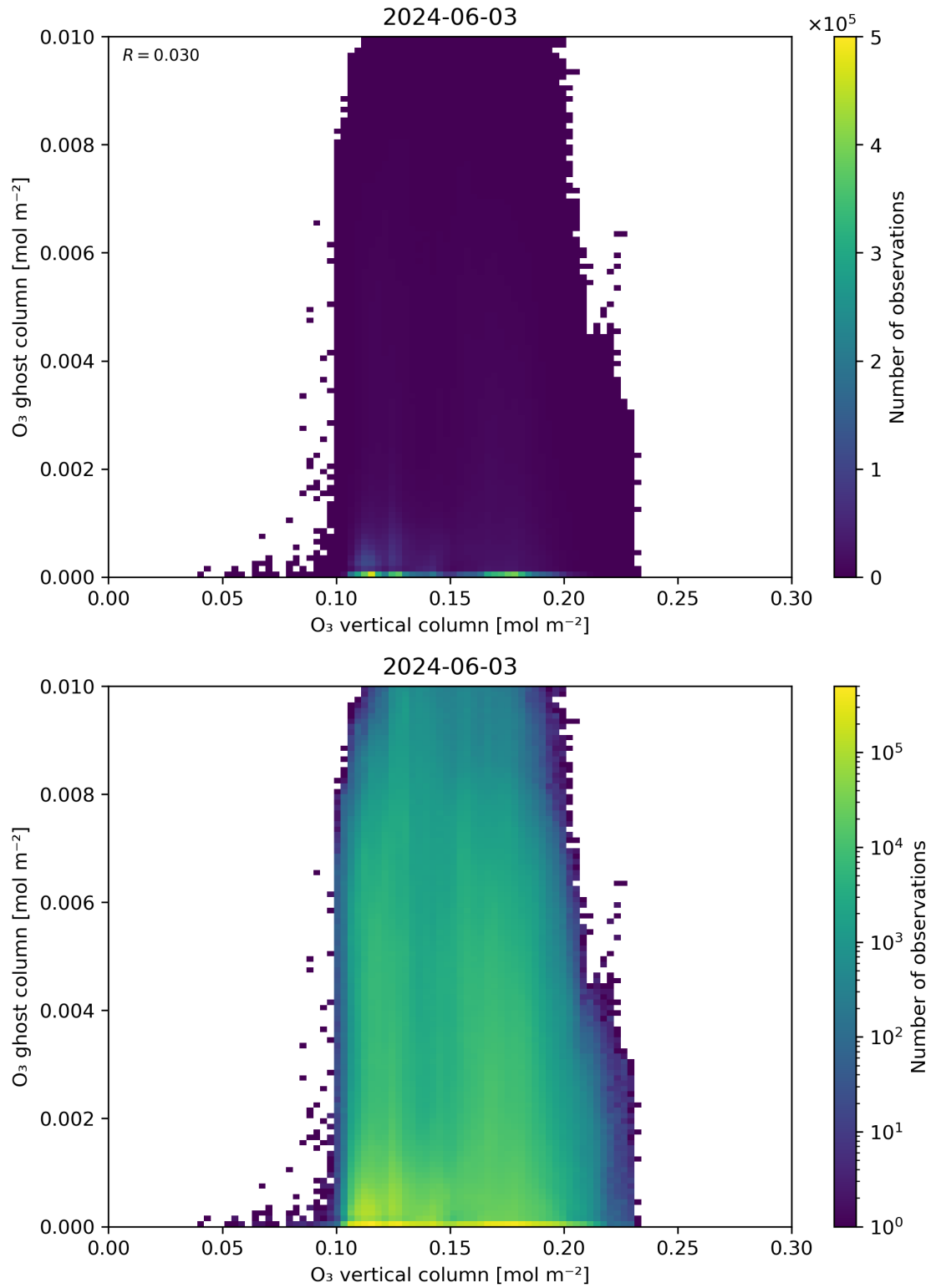
Figure 40: Scatter density plot of “O 3 vertical column” against “O 3 ghost column” for 2024-06-03 to 2024-06-04.
