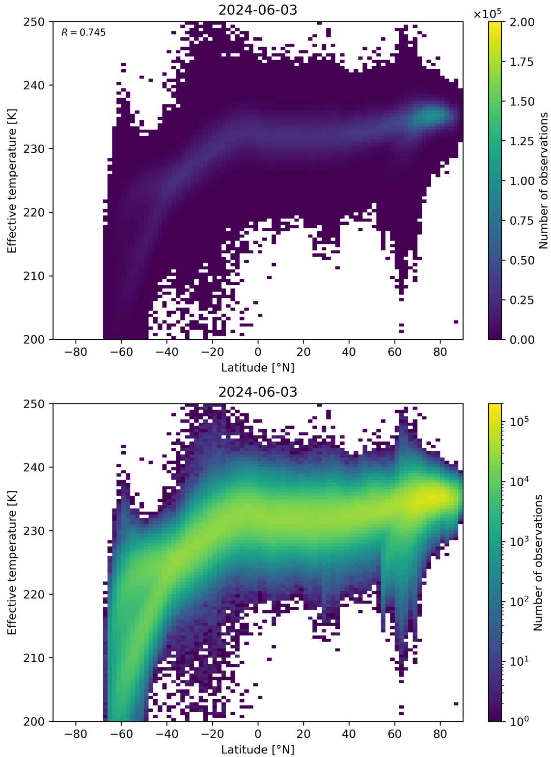
Figure 34: Scatter density plot of “Latitude” against “Effective temperature” for 2024-06-03 to 2024-06-04.
