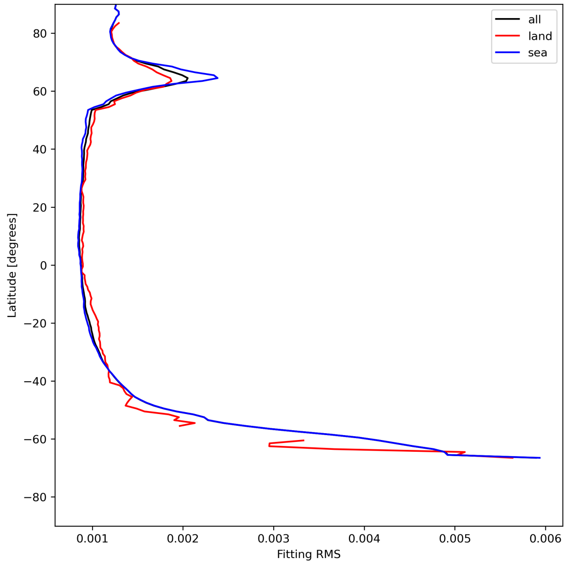
Figure 16: Zonal average of “Fitting RMS” for 2024-06-03 to 2024-06-04.
