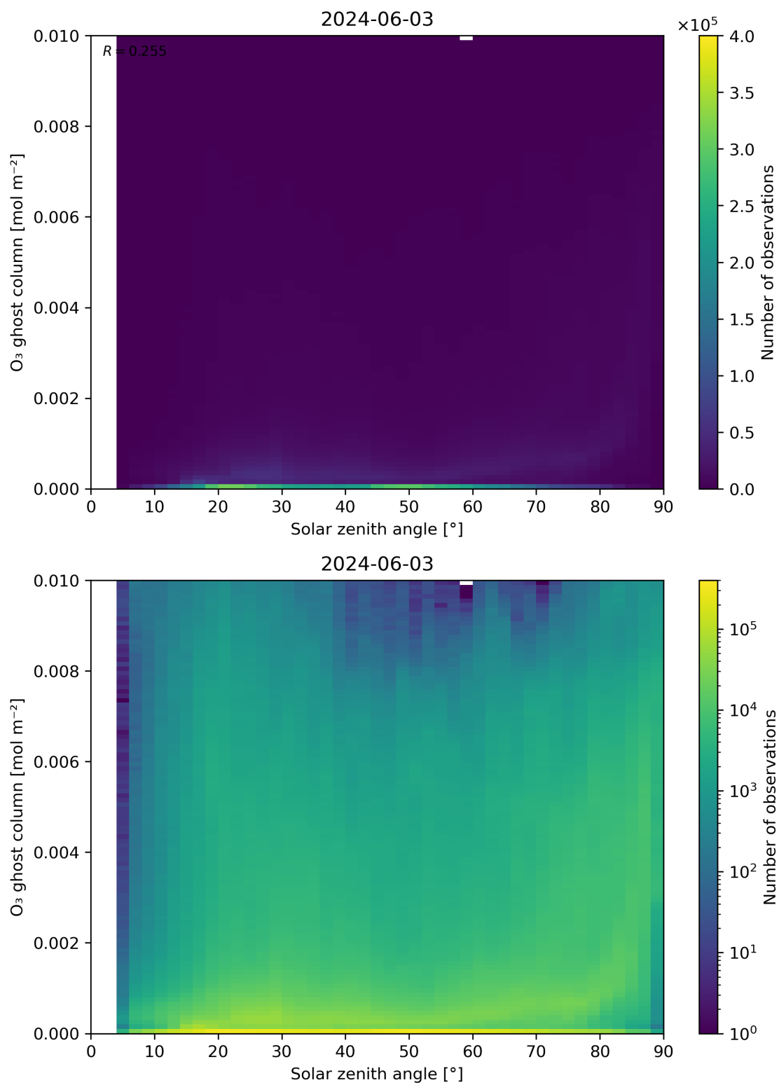
Figure 46: Scatter density plot of “Solar zenith angle” against “O 3 ghost column” for 2024-06-03 to 2024-06-04.
