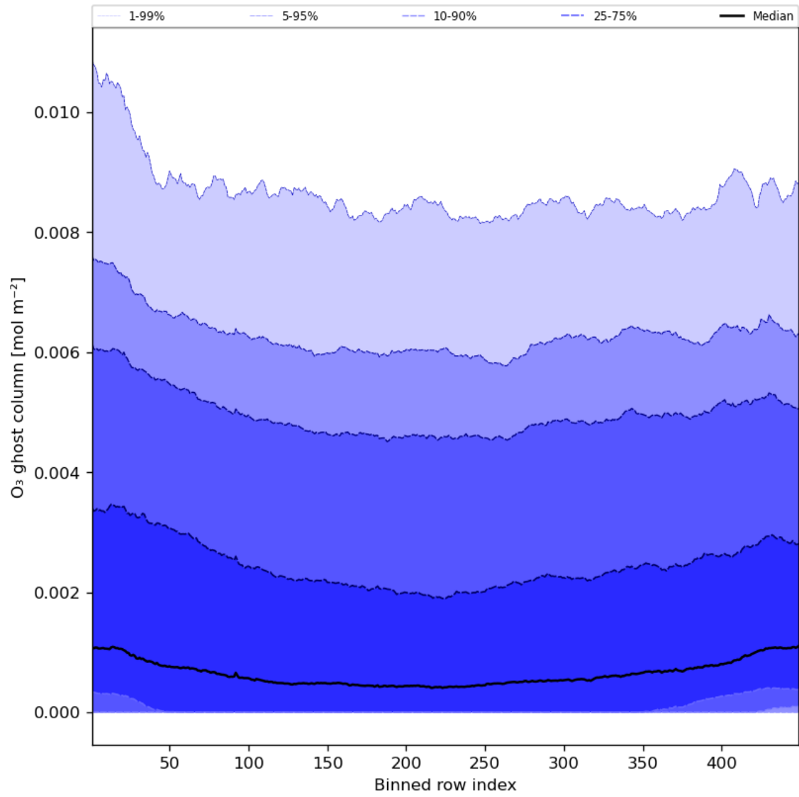
Figure 32: Along track statistics of “O 3 ghost column” for 2024-06-03 to 2024-06-04
