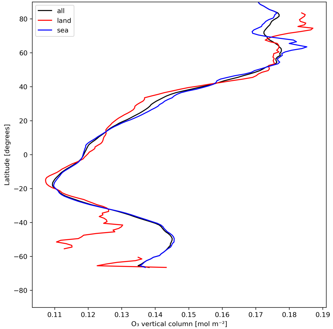
Figure 14: Zonal average of “O 3 vertical column” for 2024-06-03 to 2024-06-04.
