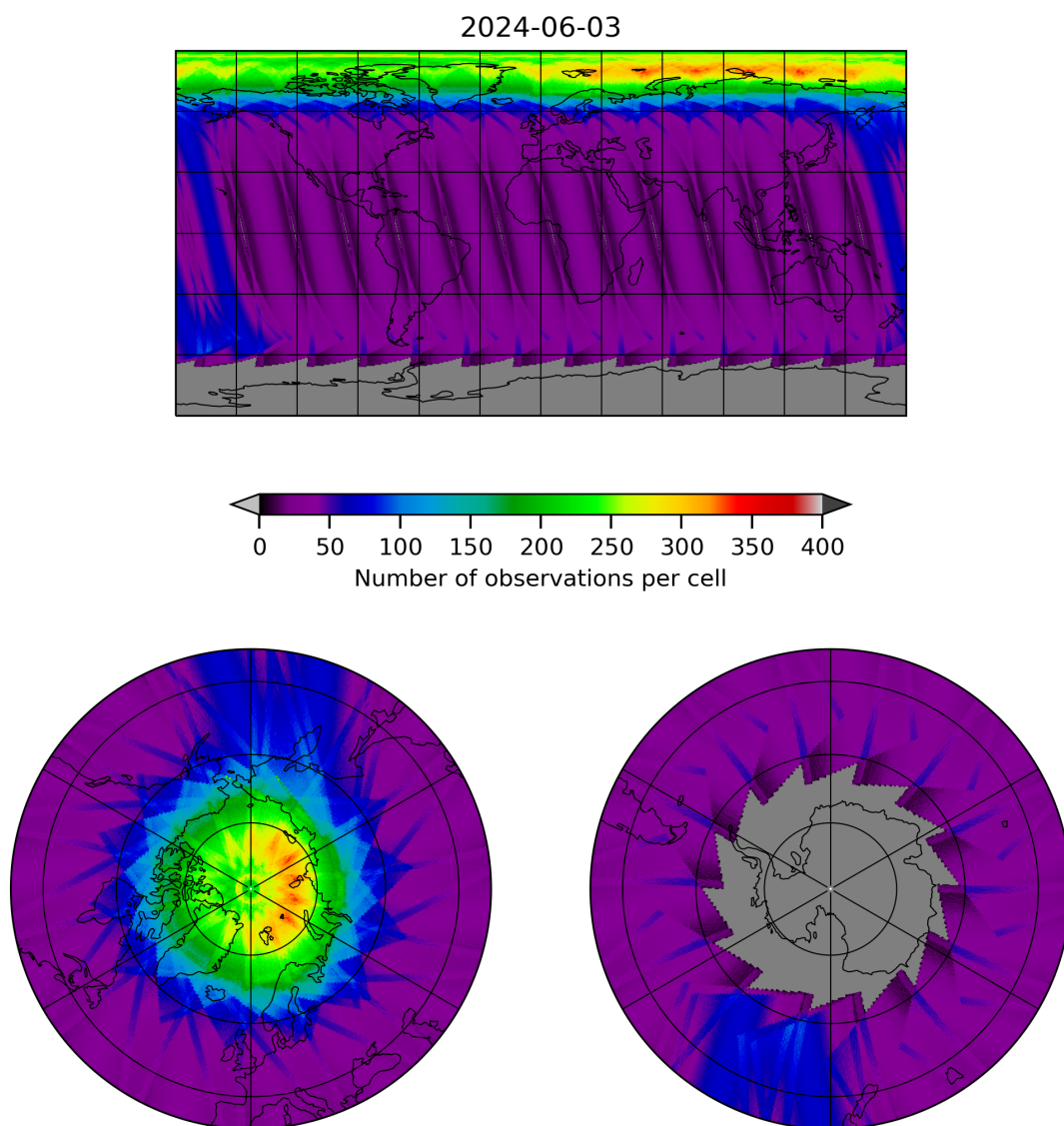
Figure 12: Map of the number of observations for 2024-06-03 to 2024-06-04
