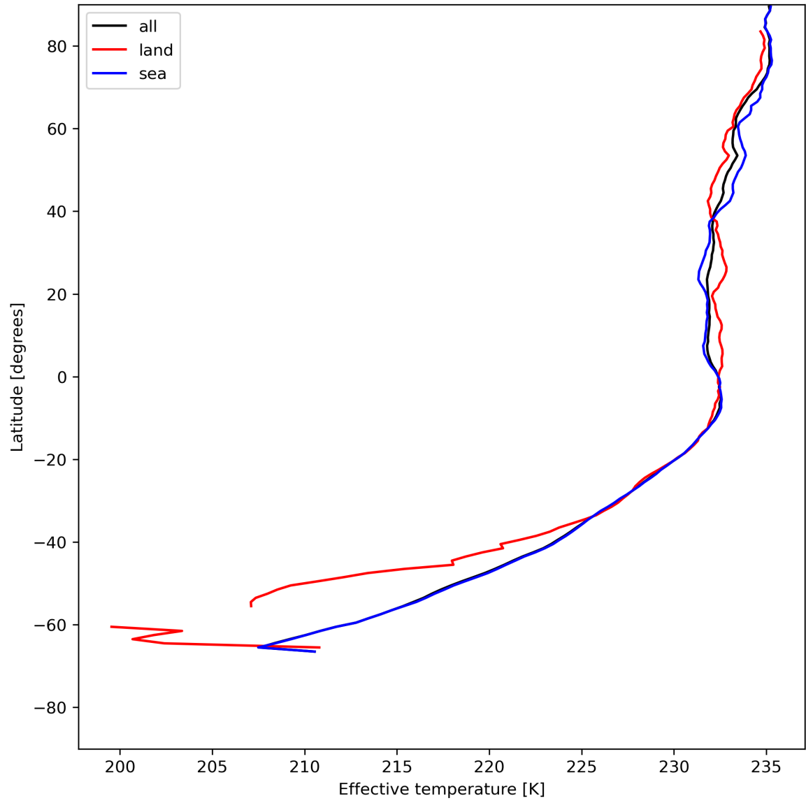
Figure 17: Zonal average of “Effective temperature” for 2024-06-03 to 2024-06-05.
