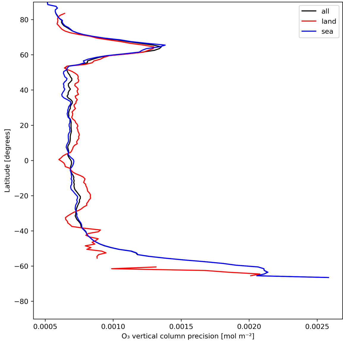
Figure 15: Zonal average of “O 3 vertical column precision” for 2024-06-03 to 2024-06-05.
