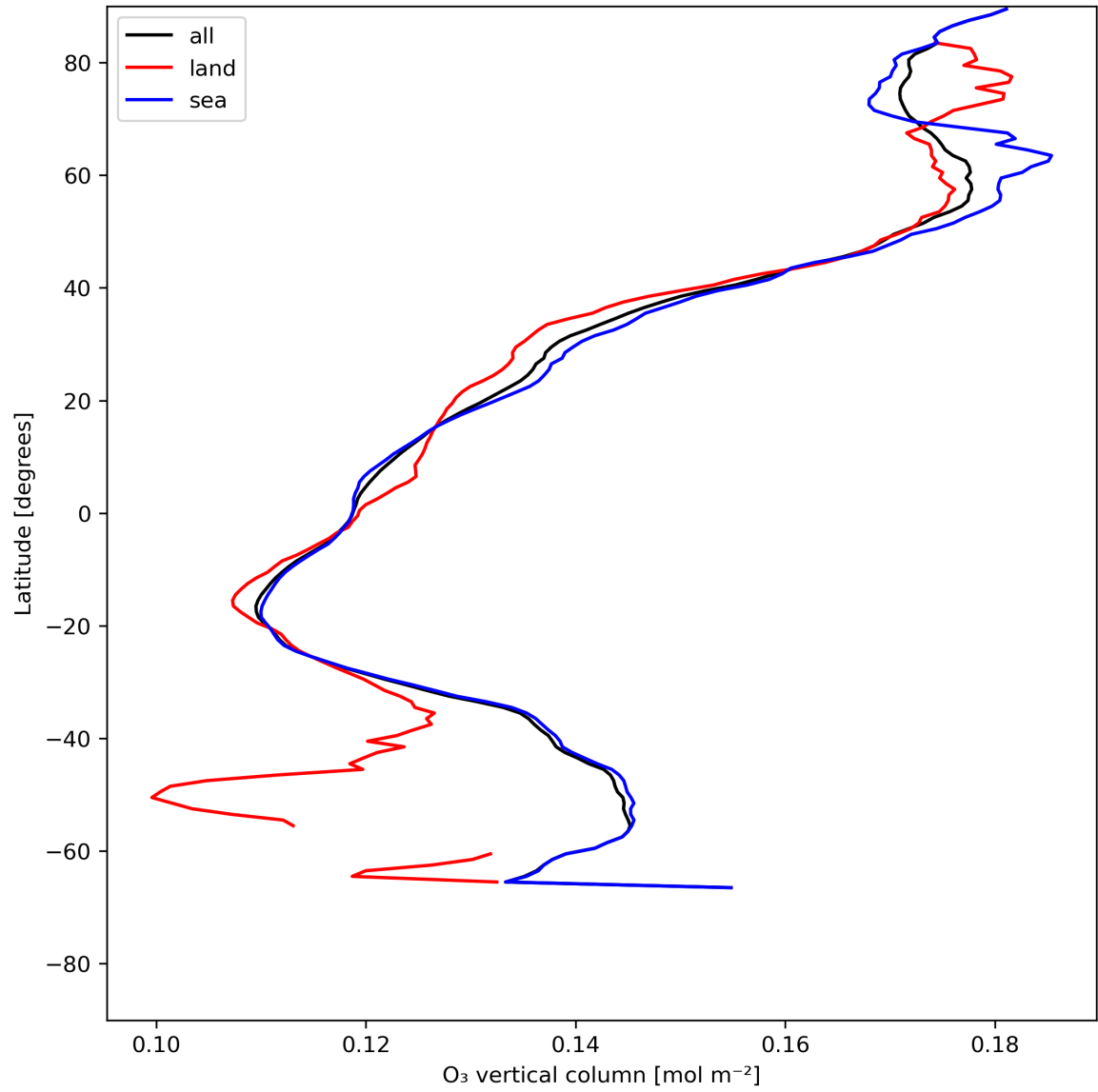
Figure 14: Zonal average of “O 3 vertical column” for 2024-06-03 to 2024-06-05.
