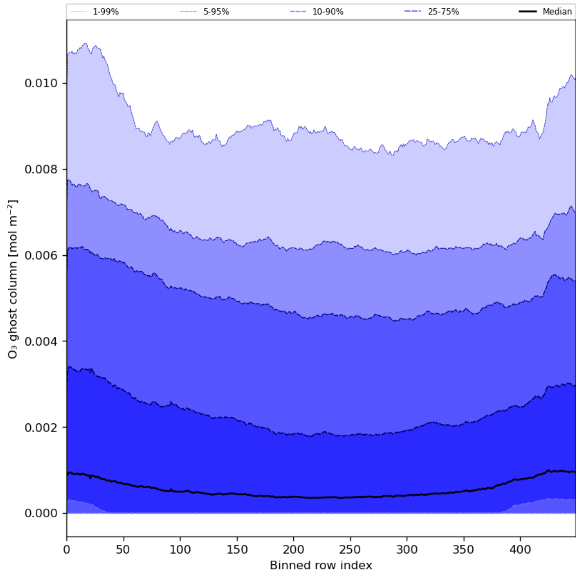
Figure 32: Along track statistics of “O 3 ghost column” for 2024-06-04 to 2024-06-06
