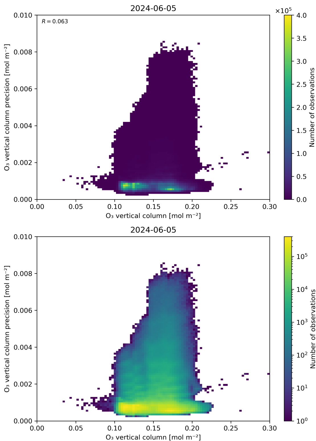
Figure 41: Scatter density plot of “O 3 vertical column” against “O 3 vertical column precision” for 2024-06-04 to 2024-06-06.
