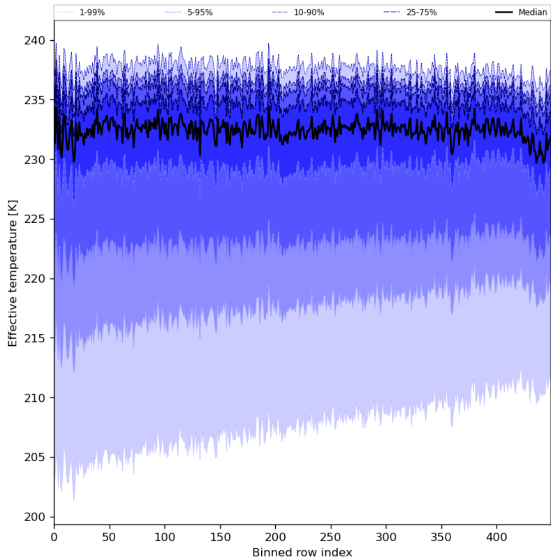
Figure 31: Along track statistics of “Effective temperature” for 2024-06-04 to 2024-06-06
