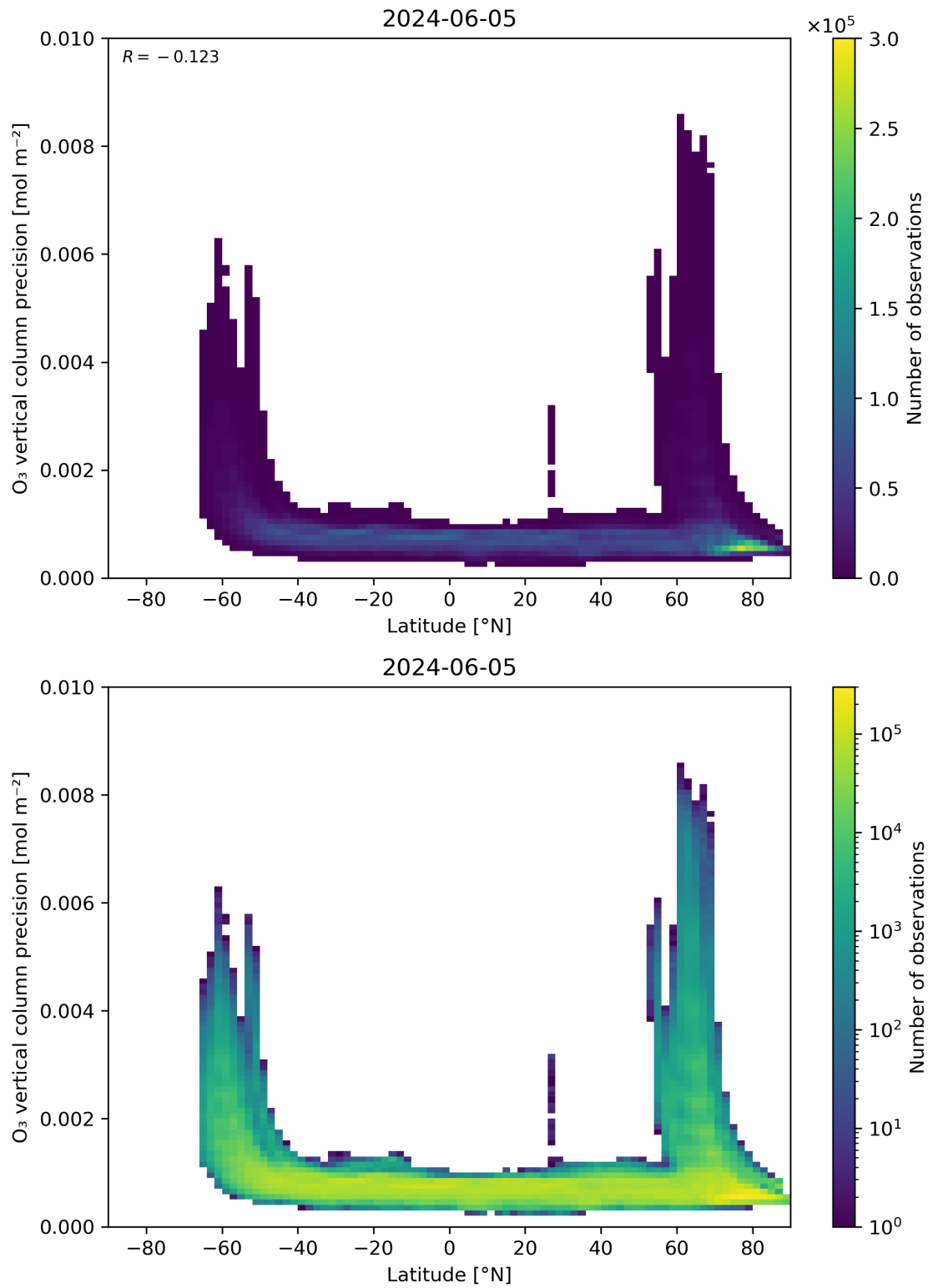
Figure 37: Scatter density plot of “Latitude” against “O 3 vertical column precision” for 2024-06-04 to 2024-06-06.
