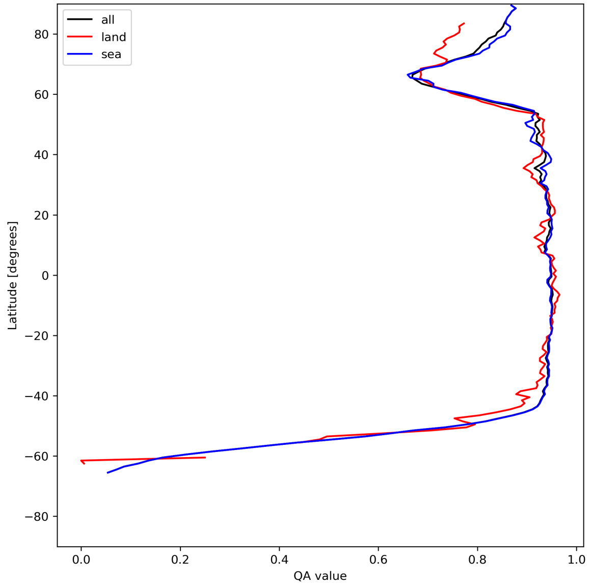
Figure 13: Zonal average of “QA value” for 2024-06-04 to 2024-06-06.
