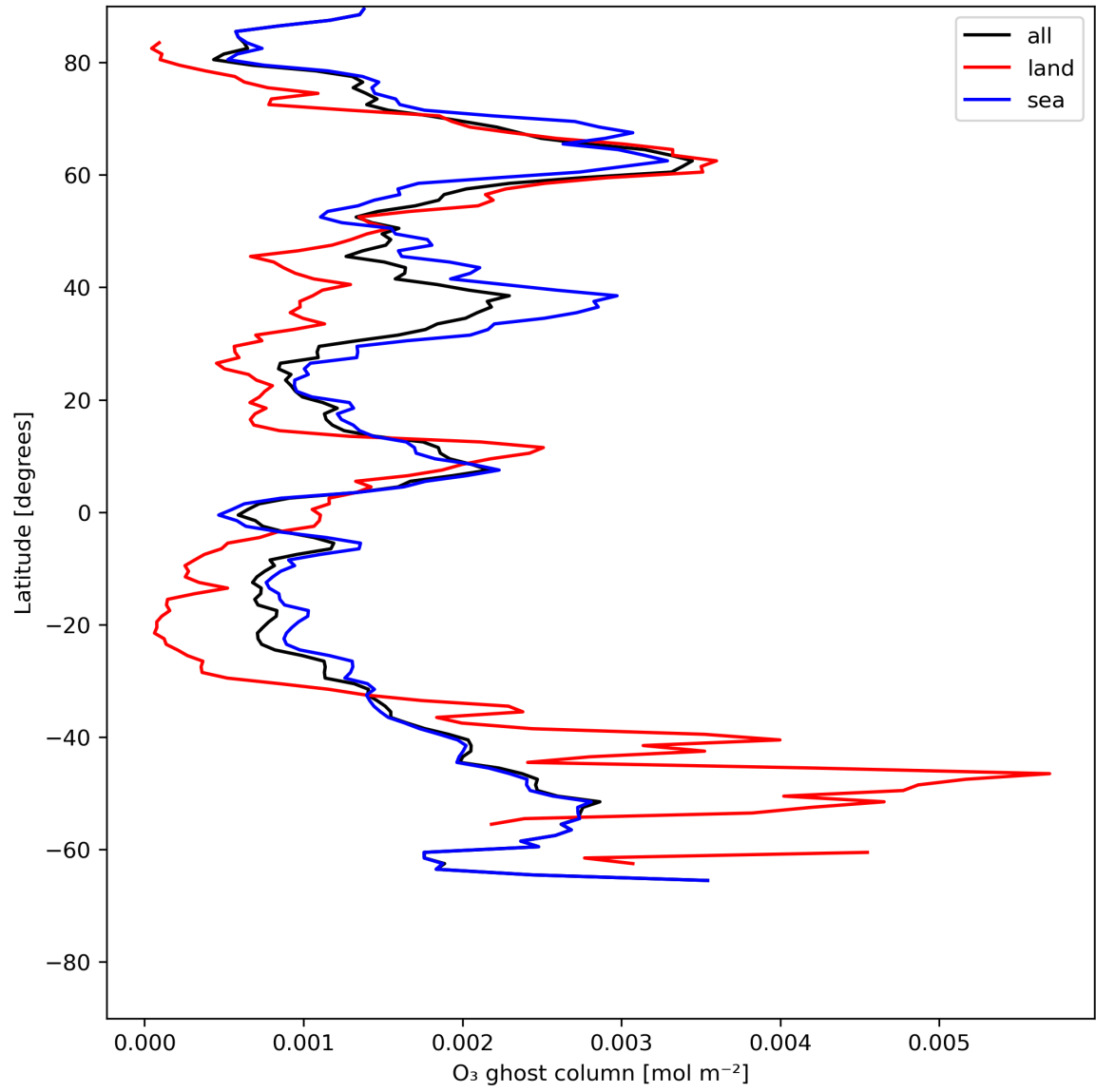
Figure 18: Zonal average of "O 3 ghost column" for 2024-06-04 to 2024-06-06.
