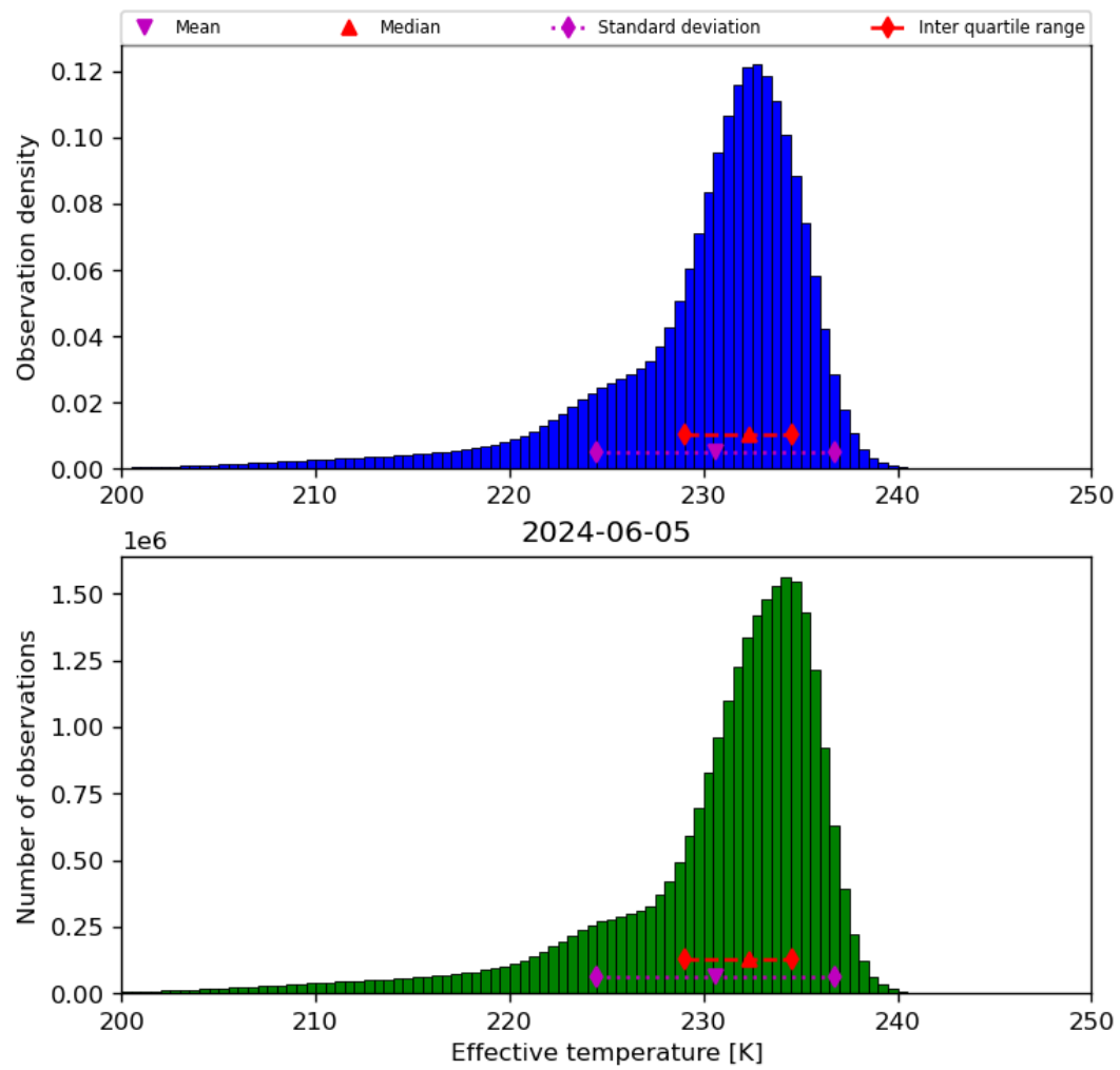
Figure 24: Histogram of “Effective temperature” for 2024-06-04 to 2024-06-06
