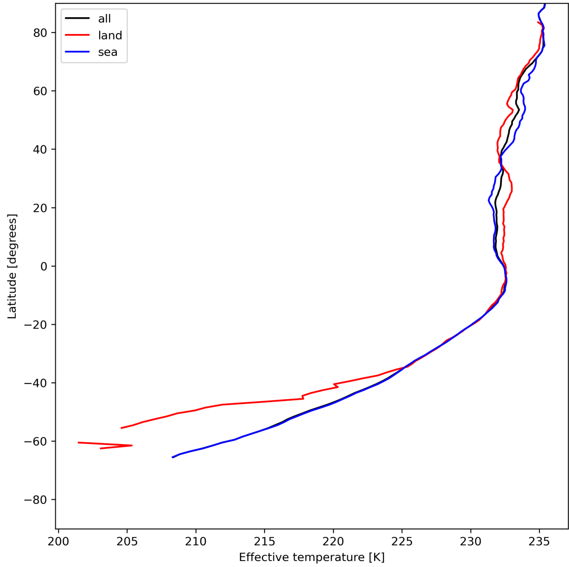
Figure 17: Zonal average of “Effective temperature” for 2024-06-04 to 2024-06-06.
