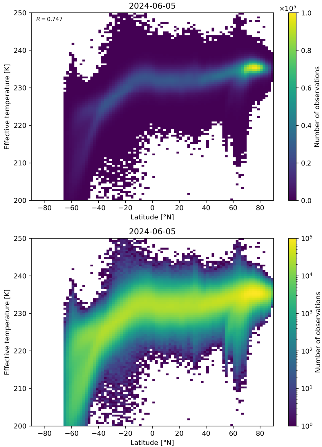
Figure 34: Scatter density plot of “Latitude” against “Effective temperature” for 2024-06-04 to 2024-06-06.
