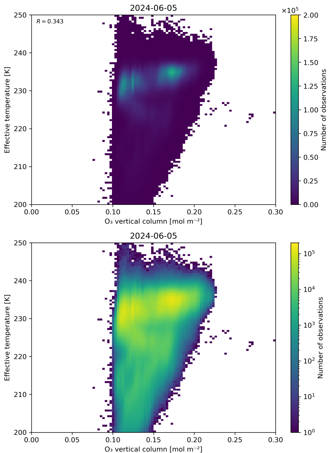
Figure 39: Scatter density plot of “O 3 vertical column” against “Effective temperature” for 2024-06-04 to 2024-06-06.
