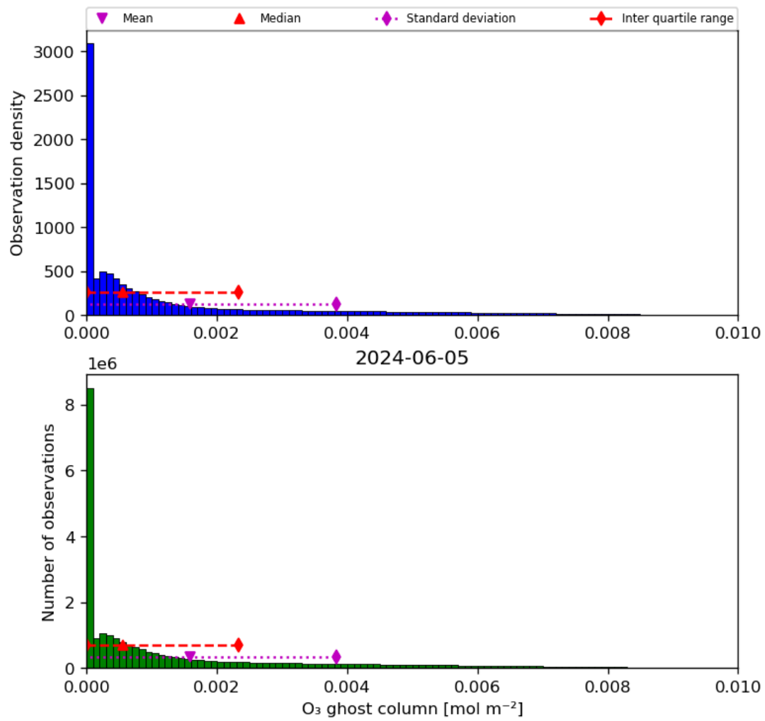
Figure 25: Histogram of "O 3 ghost column" for 2024-06-04 to 2024-06-06
