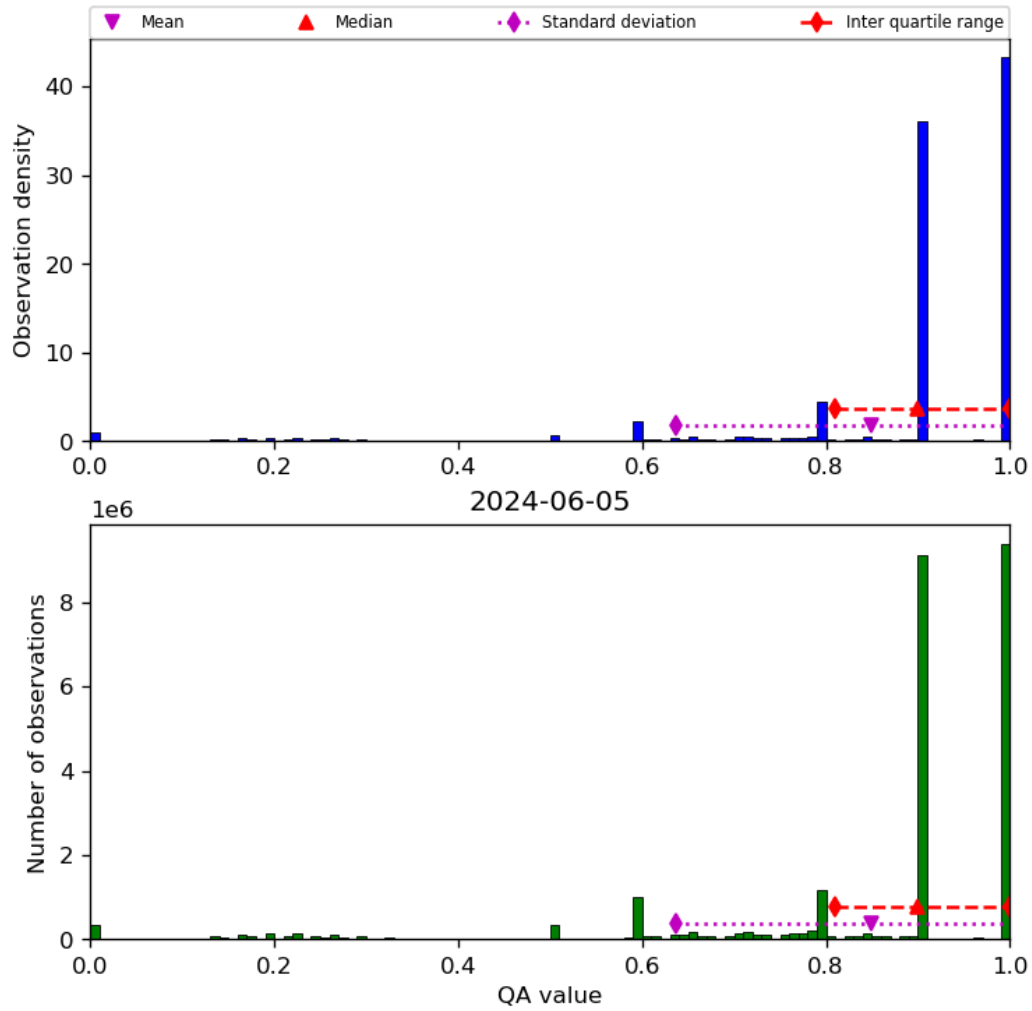
Figure 20: Histogram of “QA value” for 2024-06-04 to 2024-06-06
