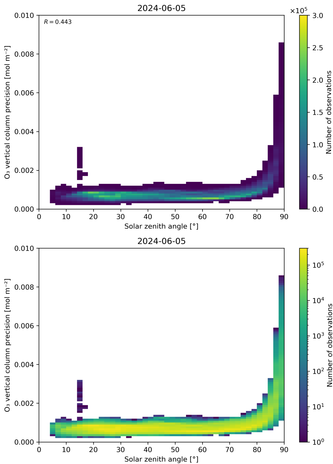
Figure 48: Scatter density plot of “Solar zenith angle” against “O 3 vertical column precision” for 2024-06-04 to 2024-06-06.
