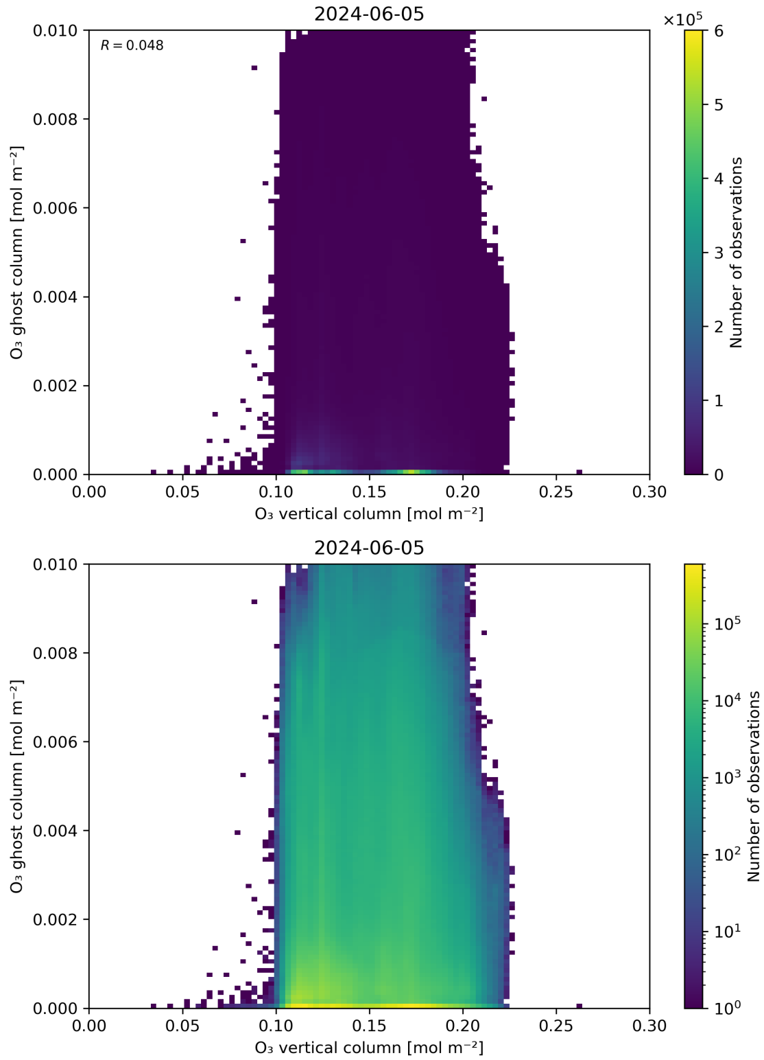
Figure 40: Scatter density plot of “O 3 vertical column” against “O 3 ghost column” for 2024-06-04 to 2024-06-06.
