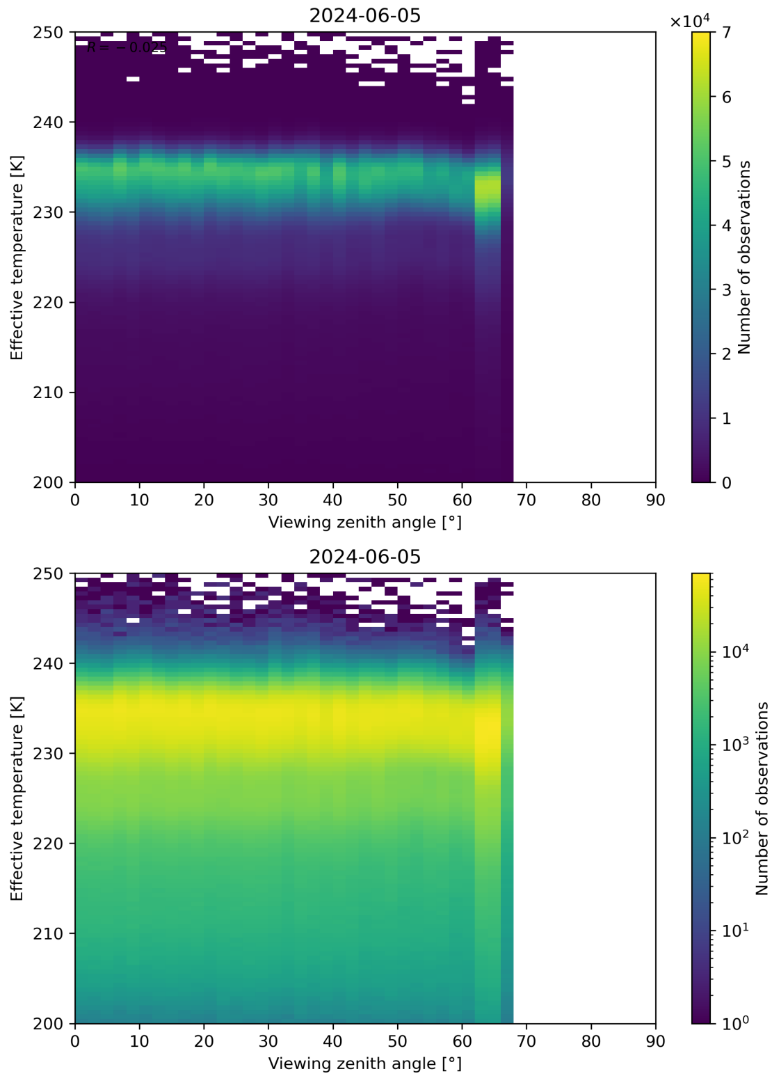
Figure 50: Scatter density plot of “Viewing zenith angle” against “Effective temperature” for 2024-06-04 to 2024-06-06.
