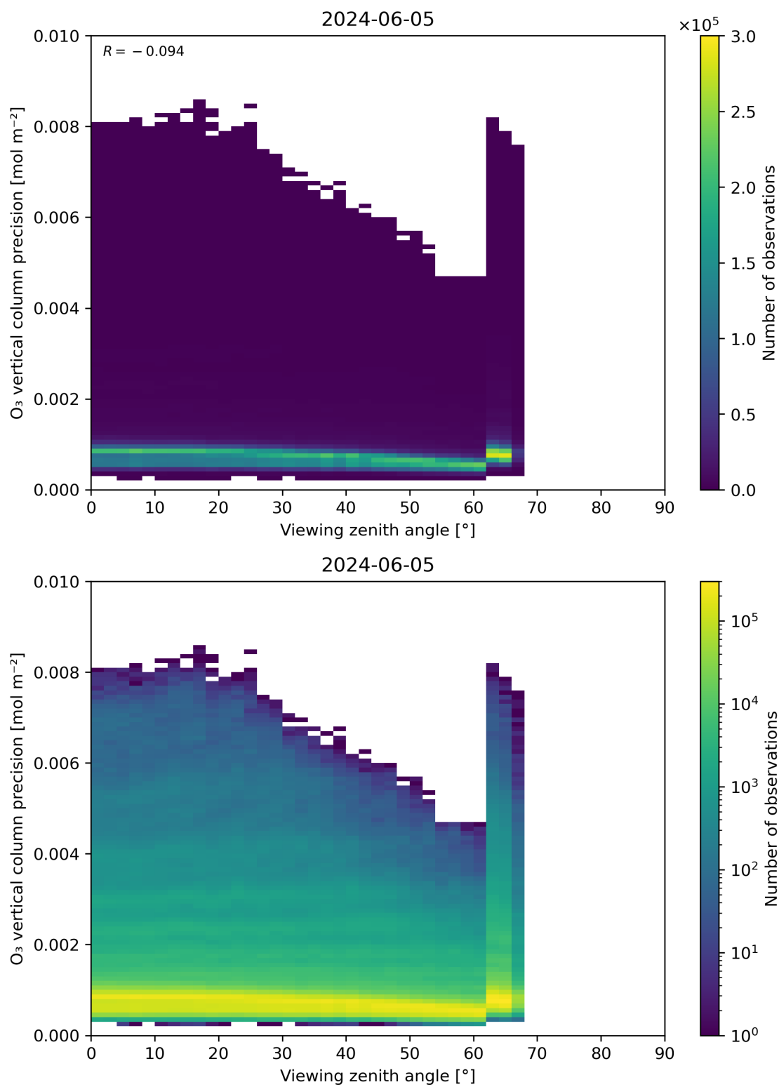
Figure 53: Scatter density plot of “Viewing zenith angle” against “O 3 vertical column precision” for 2024-06-04 to 2024-06-06.
