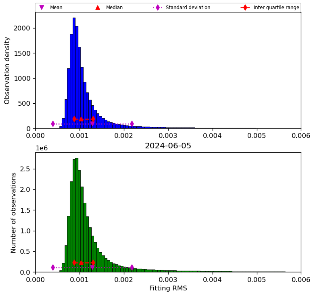
Figure 23: Histogram of “Fitting RMS” for 2024-06-04 to 2024-06-06
