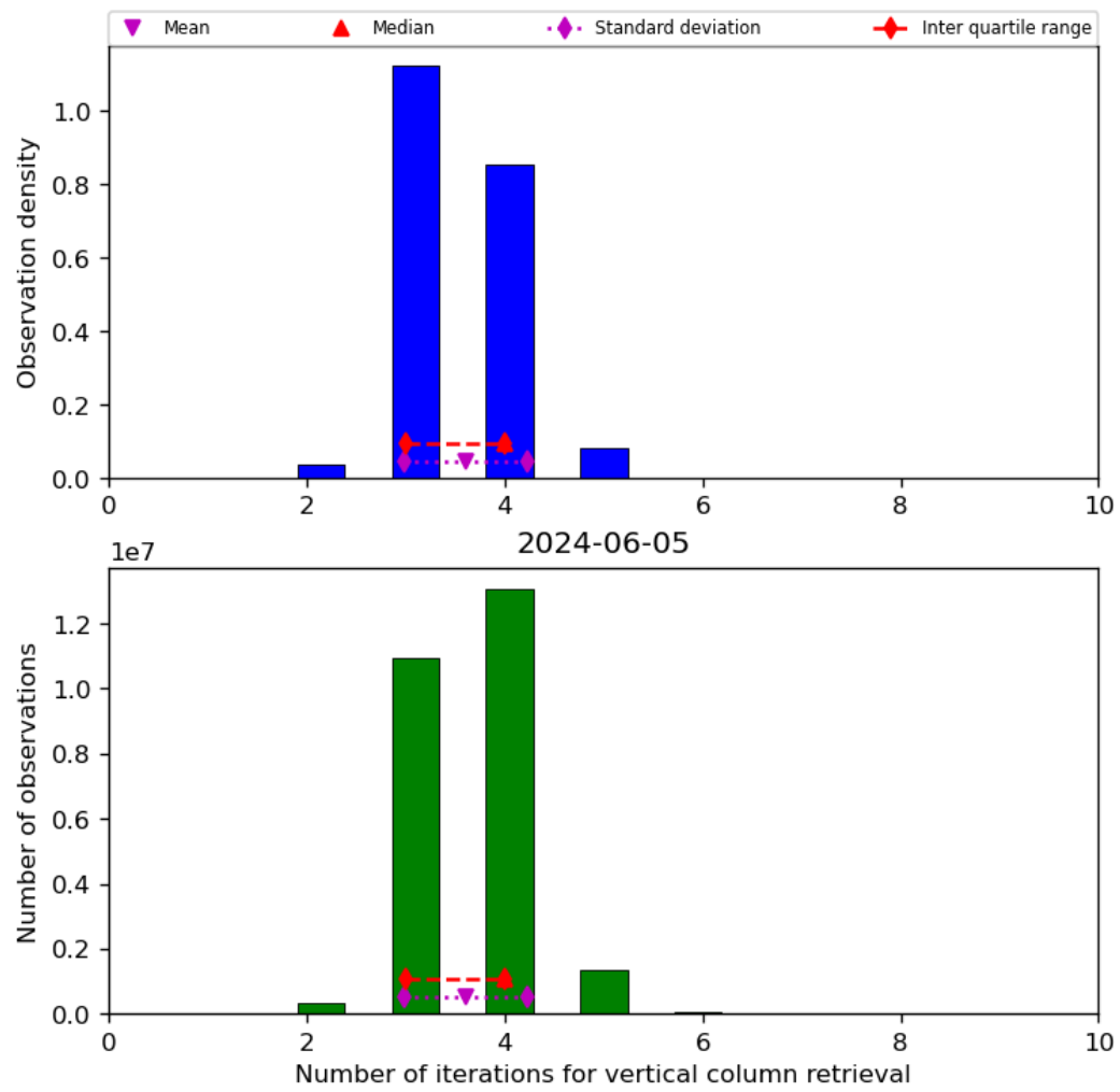
Figure 26: Histogram of “Number of iterations for vertical column retrieval” for 2024-06-04 to 2024-06-06
