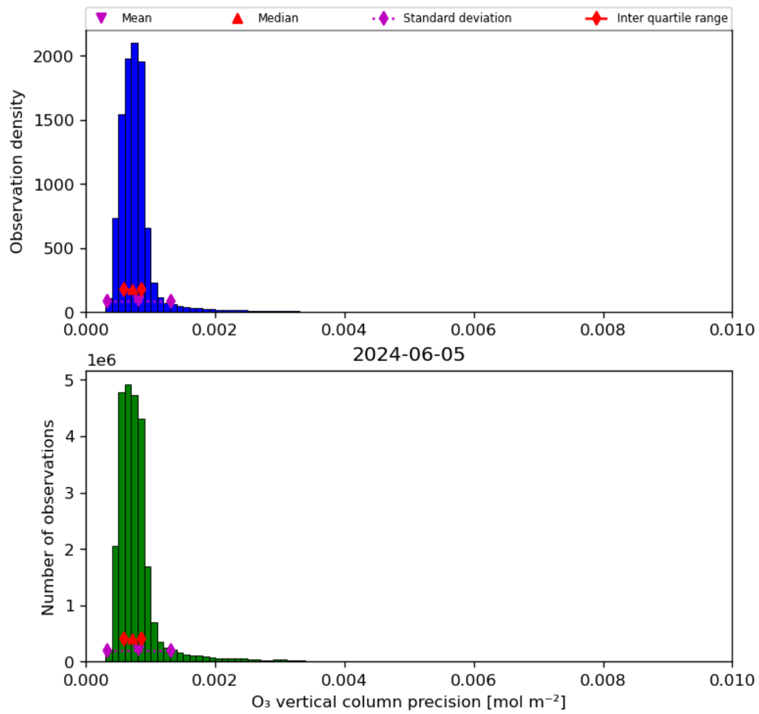
Figure 22: Histogram of “O 3 vertical column precision” for 2024-06-04 to 2024-06-06
