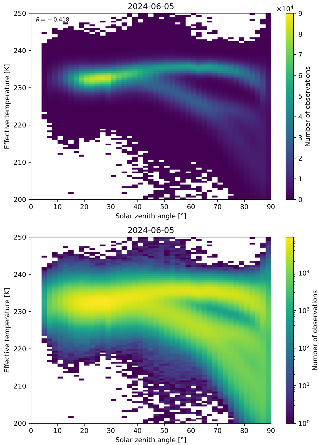
Figure 45: Scatter density plot of “Solar zenith angle” against “Effective temperature” for 2024-06-04 to 2024-06-06.
