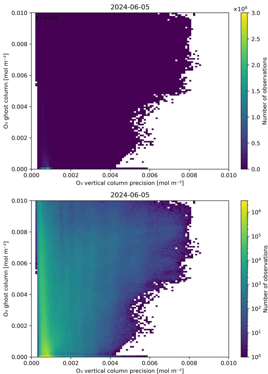
Figure 43: Scatter density plot of “ \text{O}_3 vertical column precision” against “ \text{O}_3 ghost column” for 2024-06-04 to 2024-06-06.
