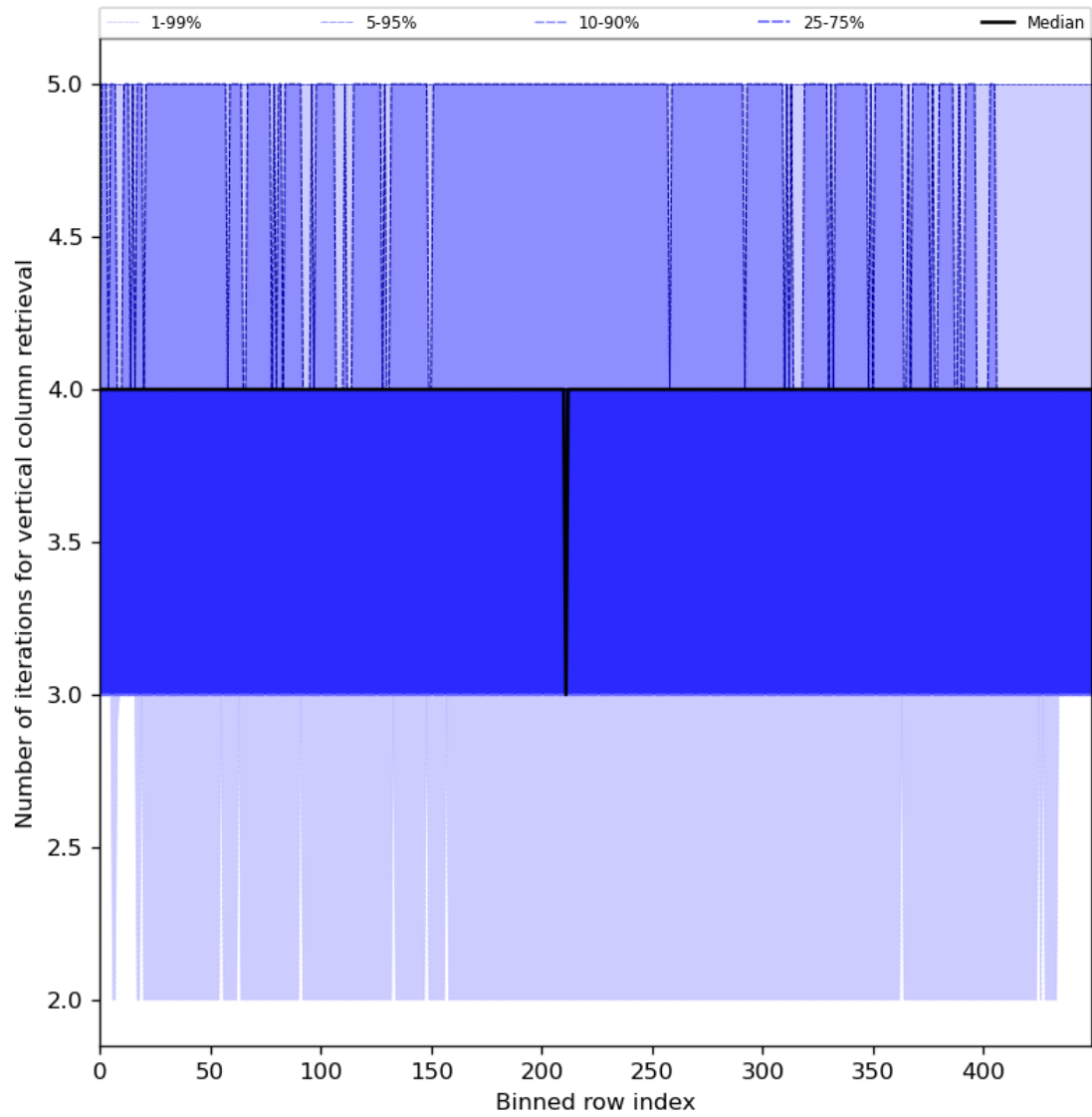
Figure 33: Along track statistics of “Number of iterations for vertical column retrieval” for 2024-06-04 to 2024-06-06
