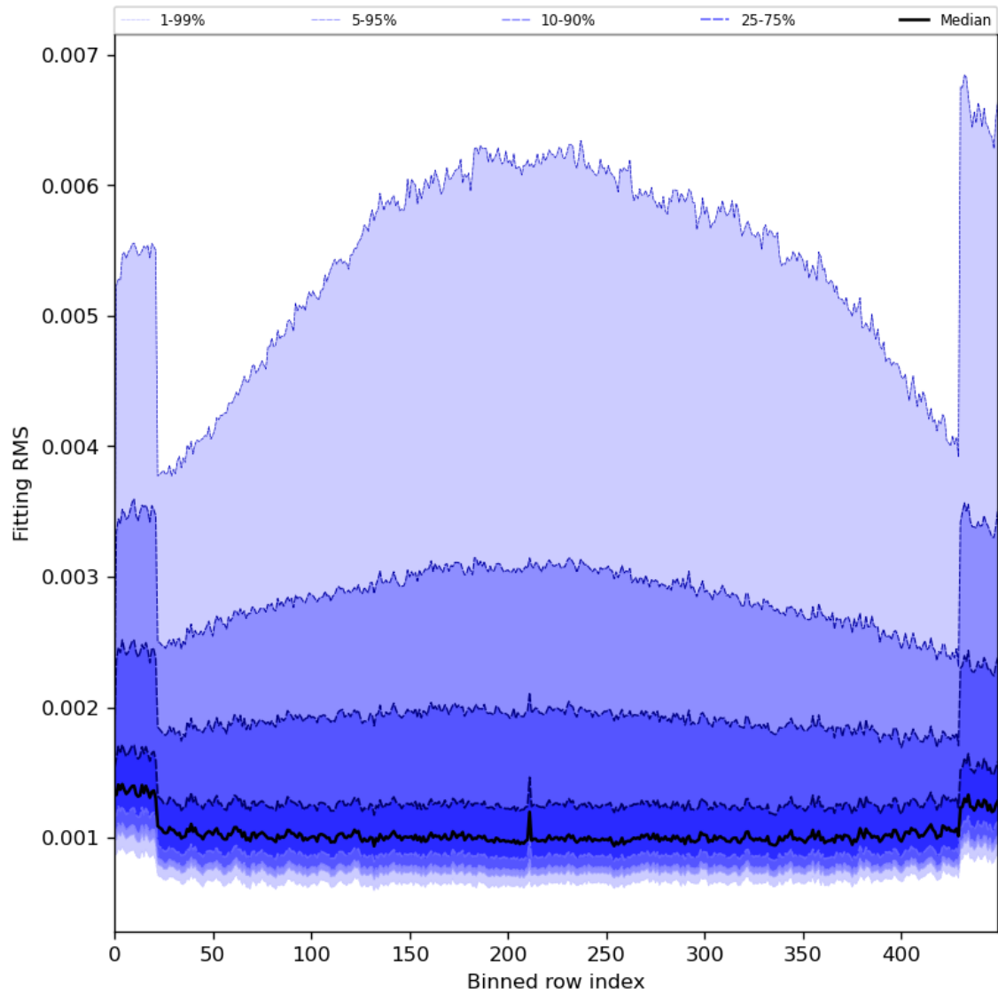
Figure 30: Along track statistics of “Fitting RMS” for 2024-06-04 to 2024-06-06
