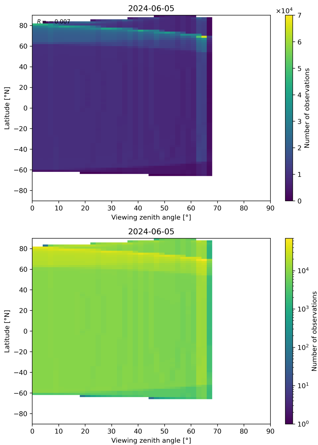
Figure 49: Scatter density plot of “Viewing zenith angle” against “Latitude” for 2024-06-04 to 2024-06-06.
