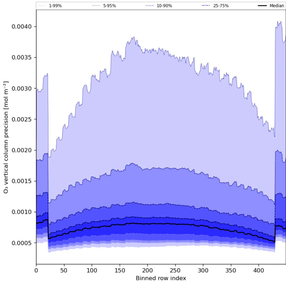
Figure 29: Along track statistics of “O 3 vertical column precision” for 2024-06-04 to 2024-06-06
