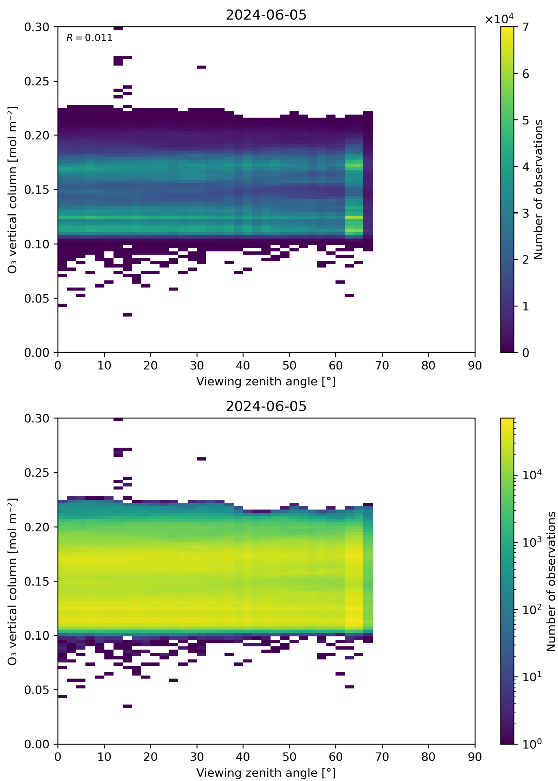
Figure 52: Scatter density plot of “Viewing zenith angle” against “O 3 vertical column” for 2024-06-04 to 2024-06-06.
