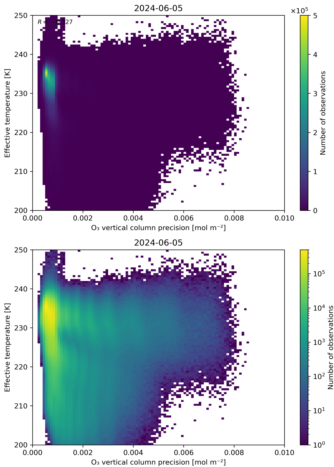
Figure 42: Scatter density plot of “O 3 vertical column precision” against “Effective temperature” for 2024-06-04 to 2024-06-06.
