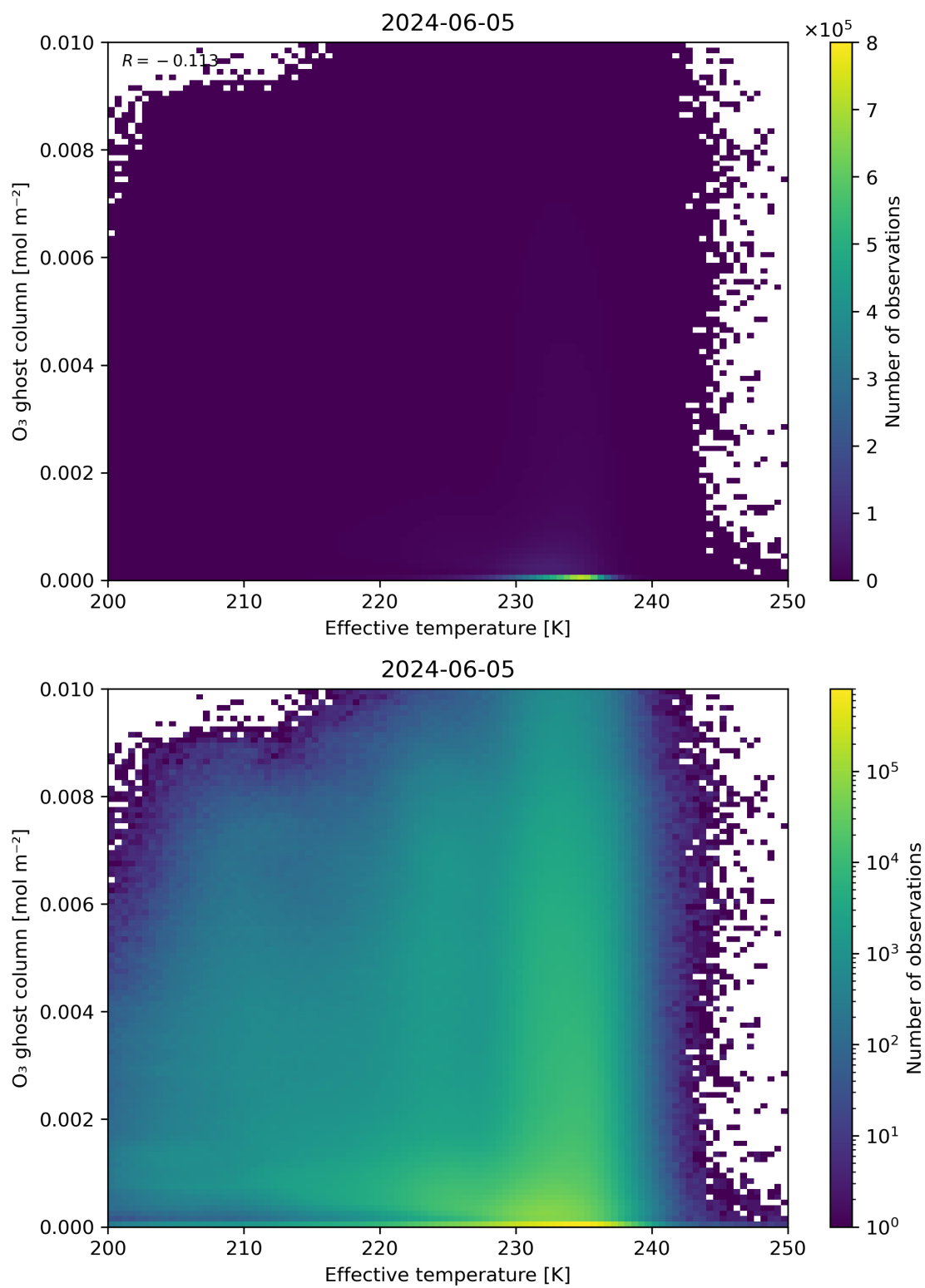
Figure 38: Scatter density plot of “Effective temperature” against “O 3 ghost column” for 2024-06-04 to 2024-06-06.
