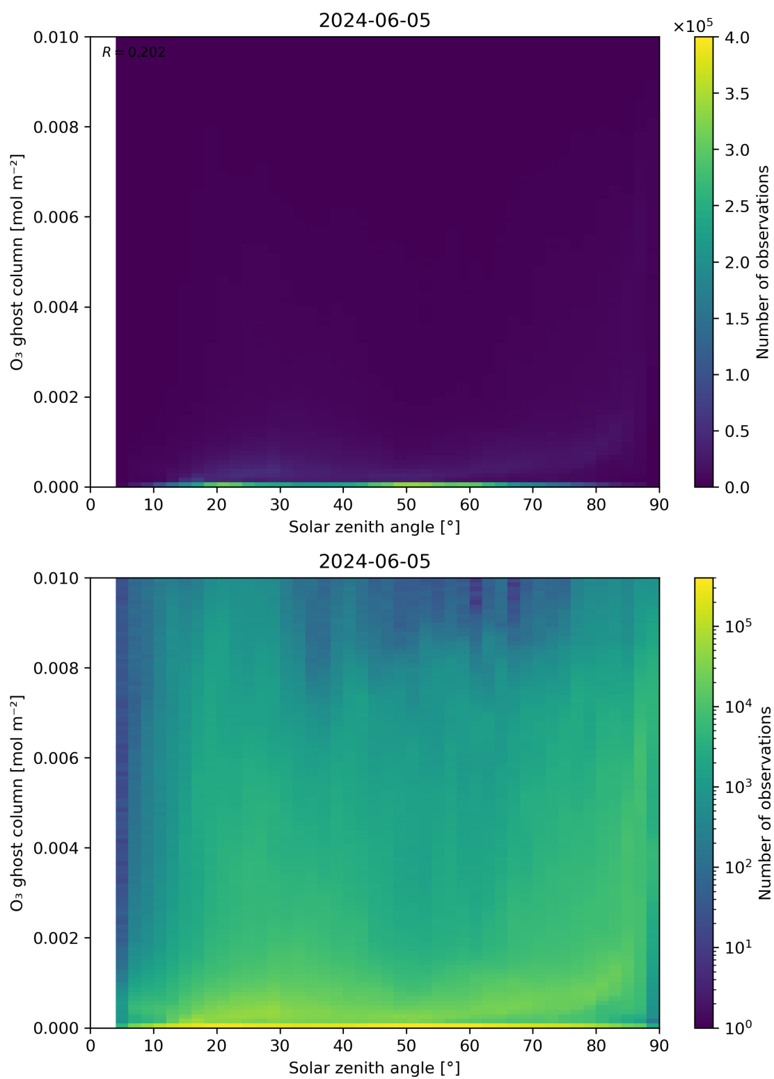
Figure 46: Scatter density plot of “Solar zenith angle” against “O 3 ghost column” for 2024-06-04 to 2024-06-06.
