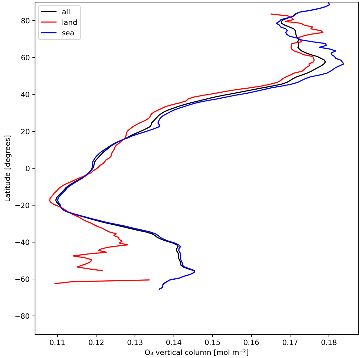
Figure 14: Zonal average of “O 3 vertical column” for 2024-06-04 to 2024-06-06.
