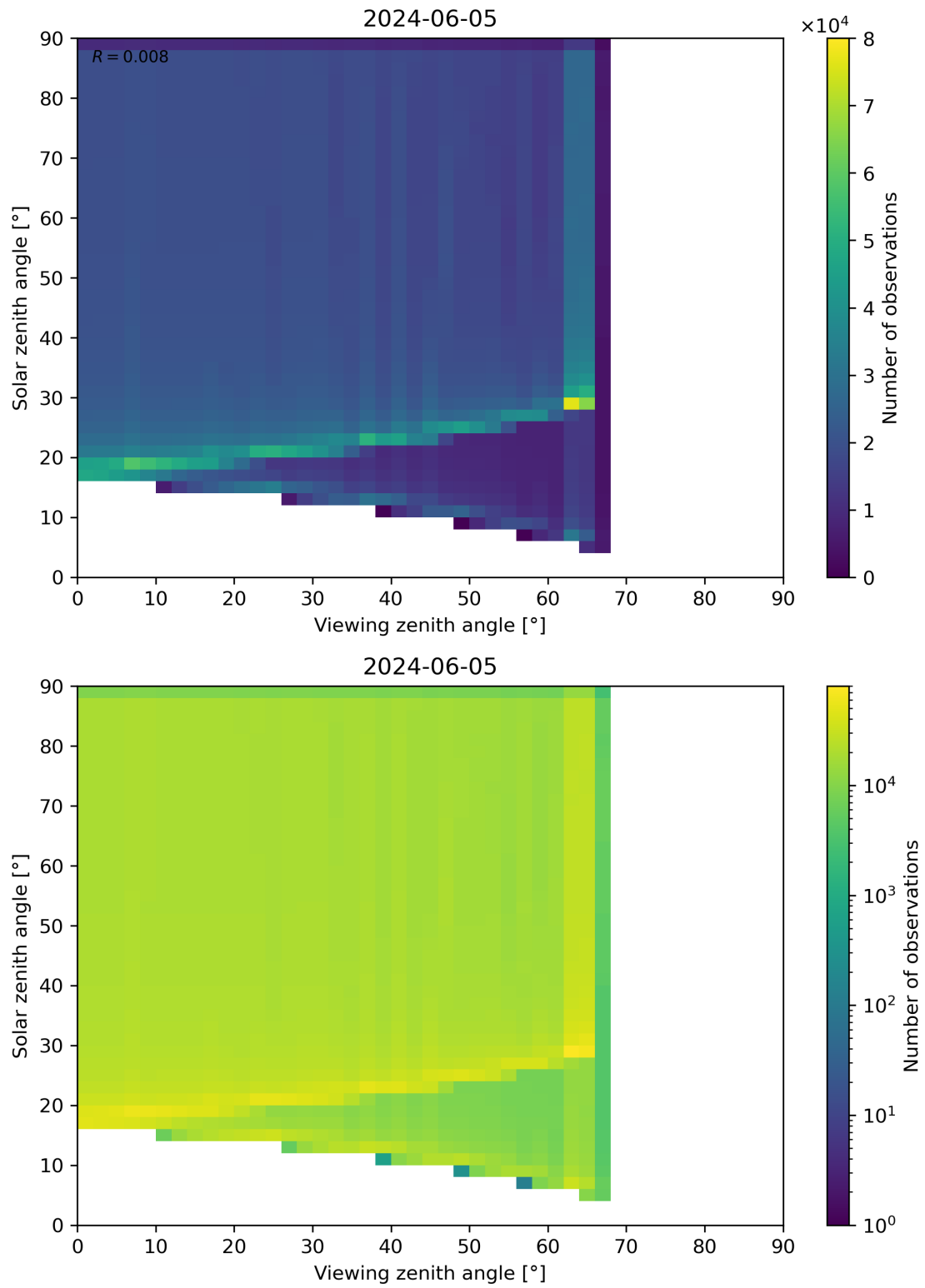
Figure 54: Scatter density plot of “Viewing zenith angle” against “Solar zenith angle” for 2024-06-04 to 2024-06-06.
