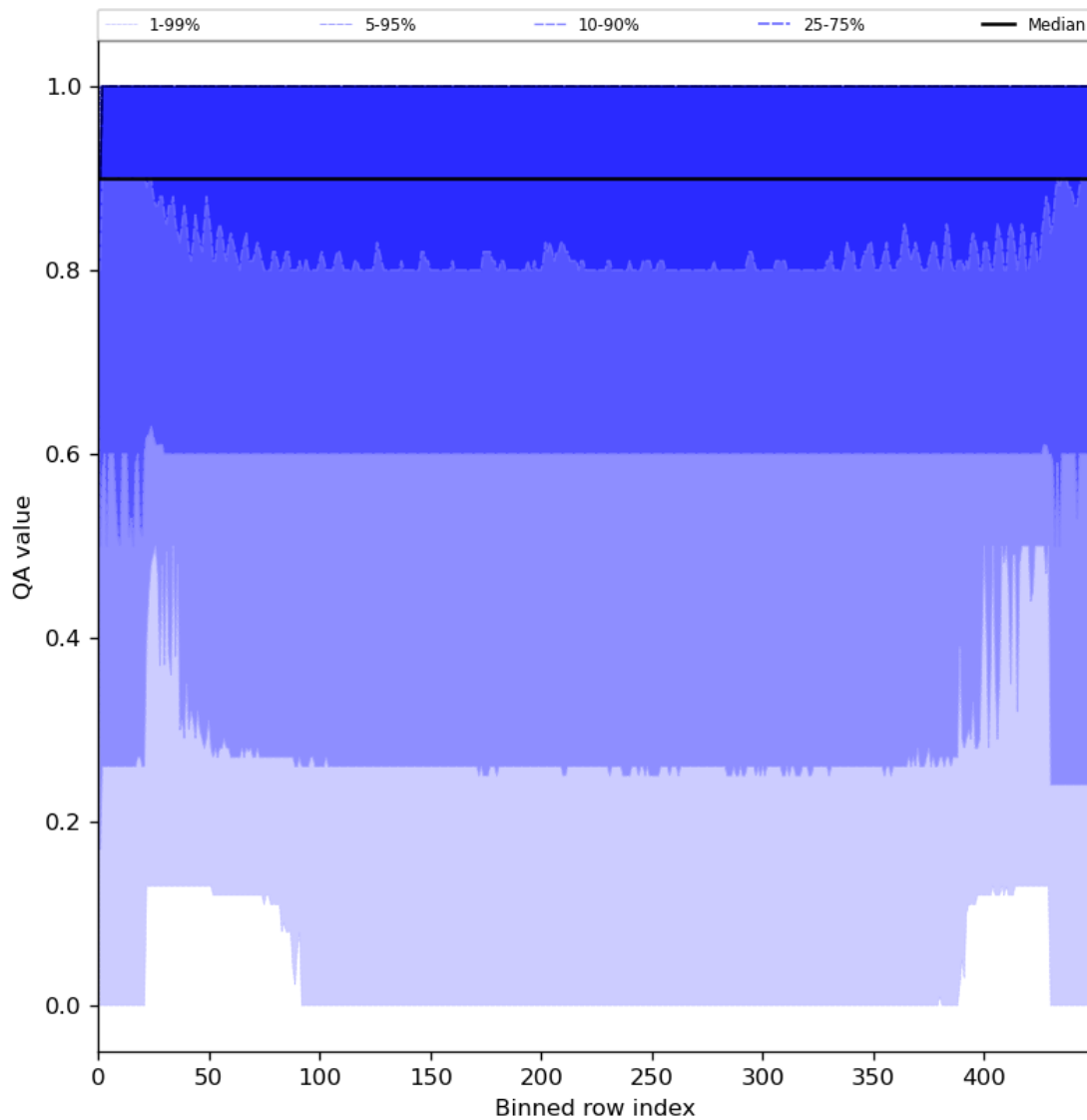
Figure 27: Along track statistics of “QA value” for 2024-06-04 to 2024-06-06
