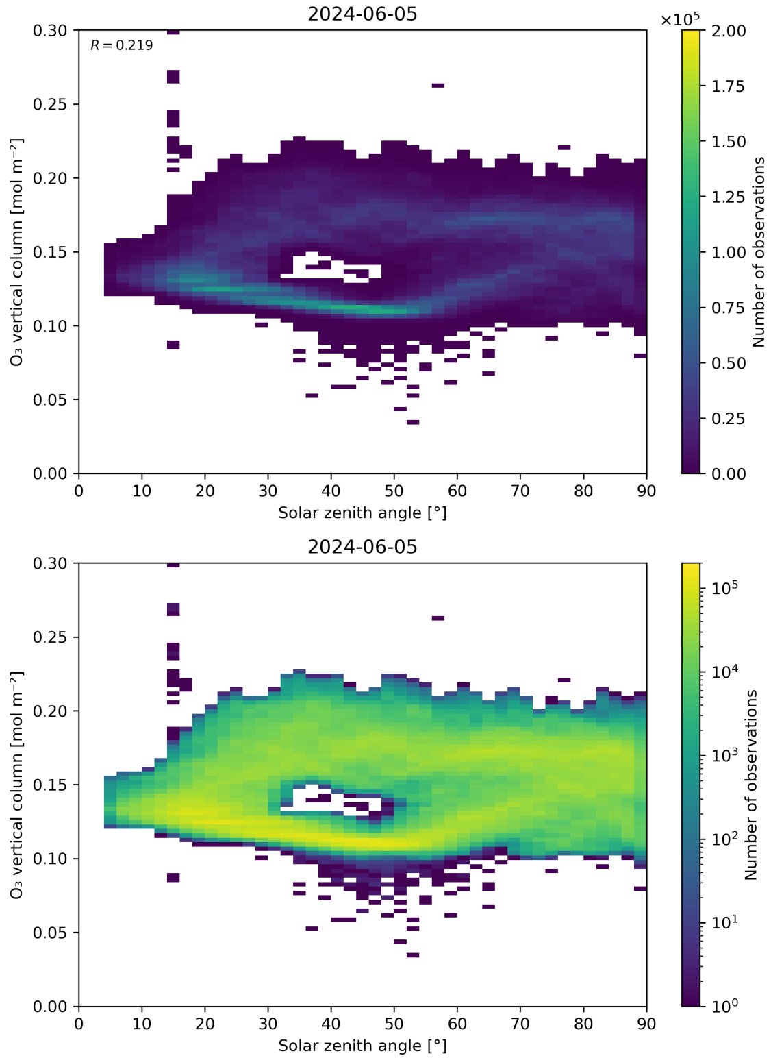
Figure 47: Scatter density plot of “Solar zenith angle” against “O 3 vertical column” for 2024-06-04 to 2024-06-06.
