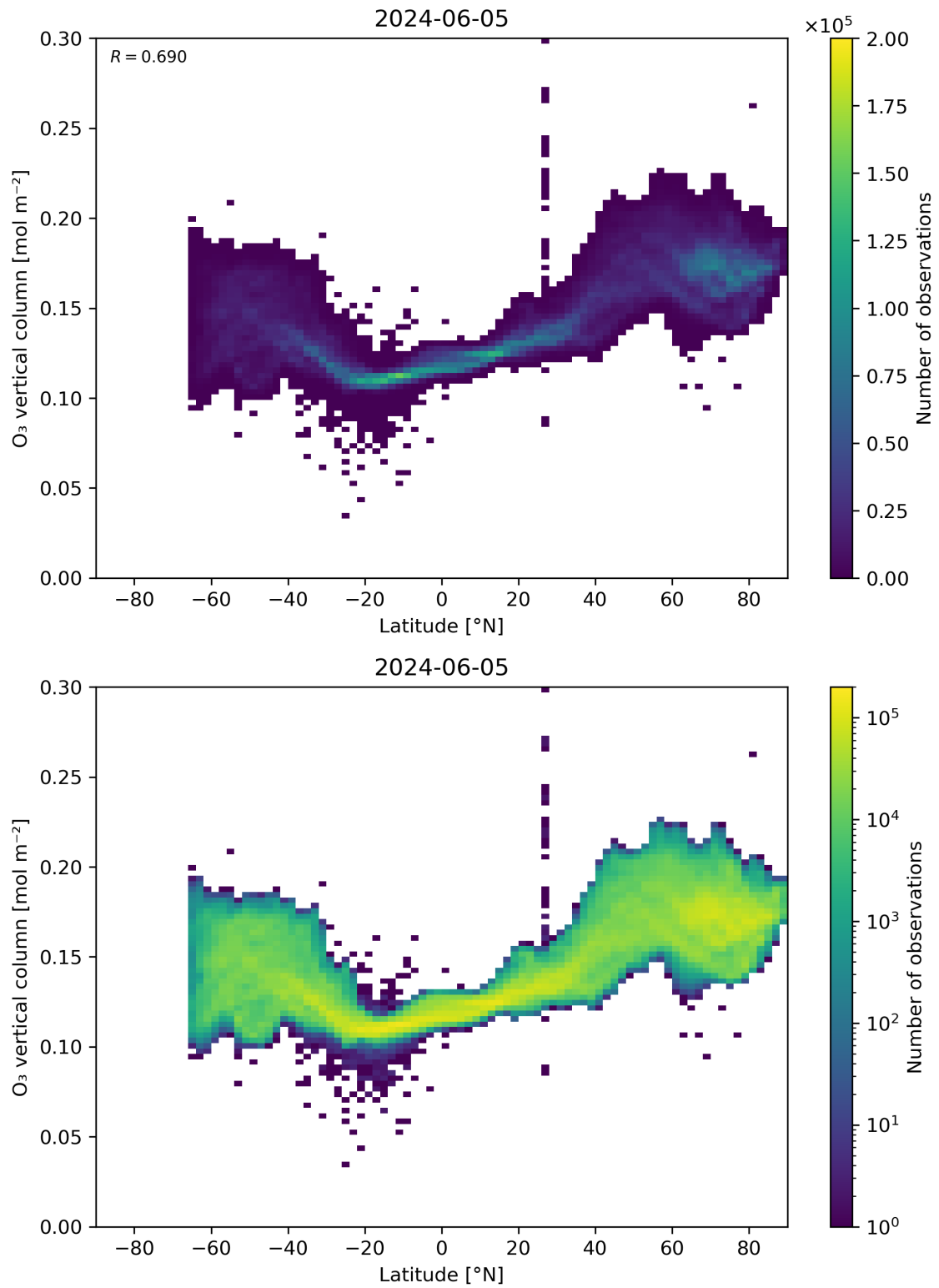
Figure 36: Scatter density plot of “Latitude” against “O 3 vertical column” for 2024-06-04 to 2024-06-06.
