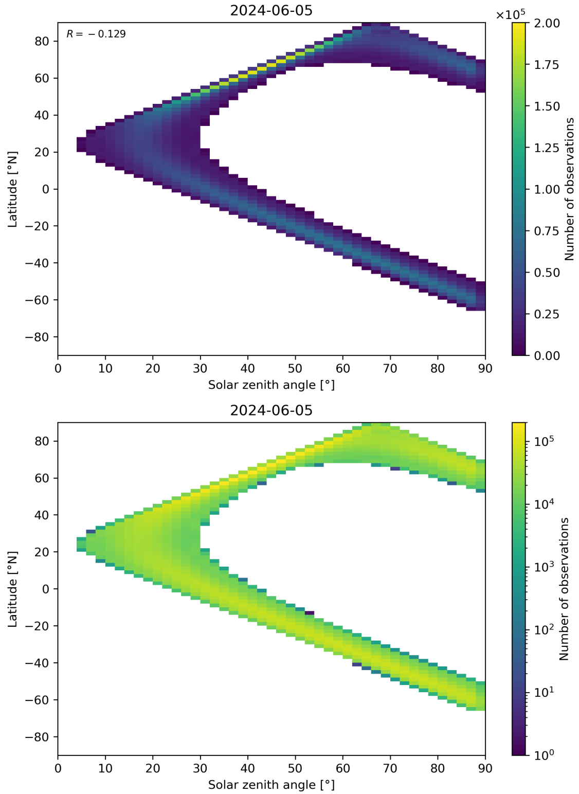
Figure 44: Scatter density plot of “Solar zenith angle” against “Latitude” for 2024-06-04 to 2024-06-06.
