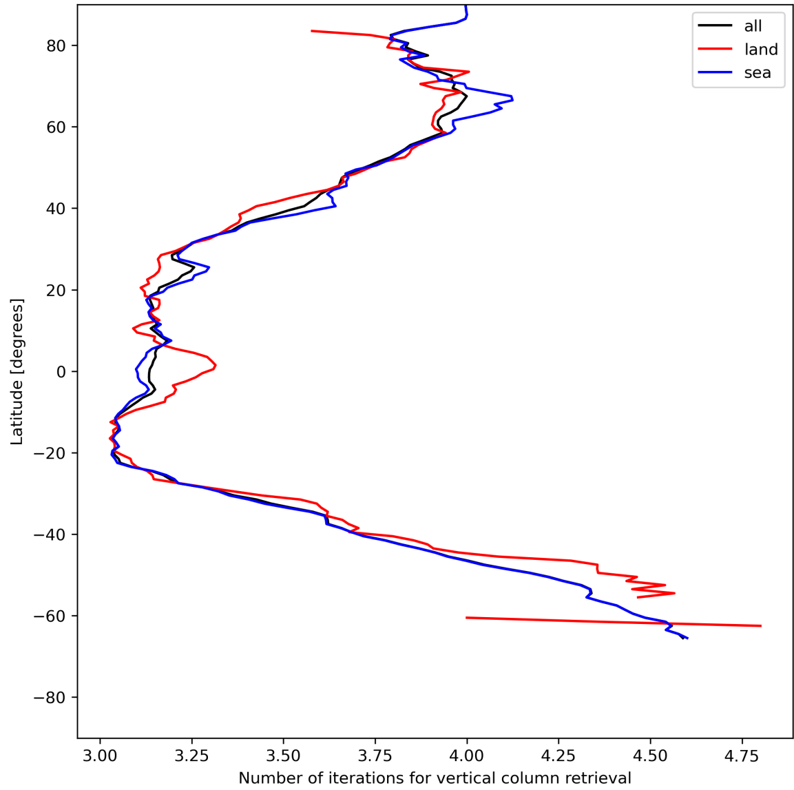
Figure 19: Zonal average of “Number of iterations for vertical column retrieval” for 2024-06-04 to 2024-06-06.
