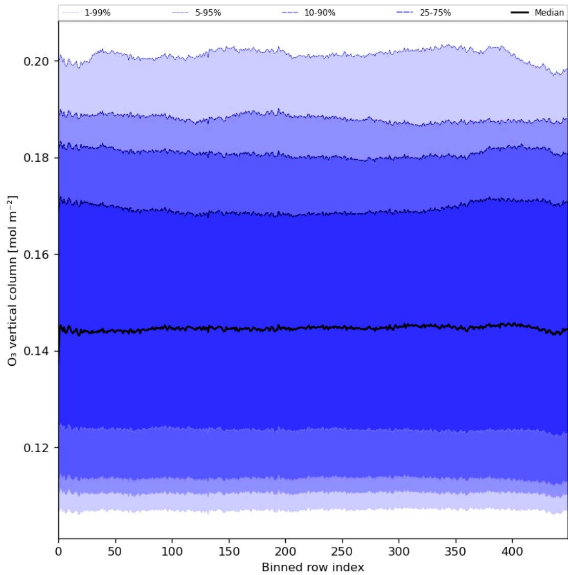
Figure 28: Along track statistics of “O 3 vertical column” for 2024-06-04 to 2024-06-06
