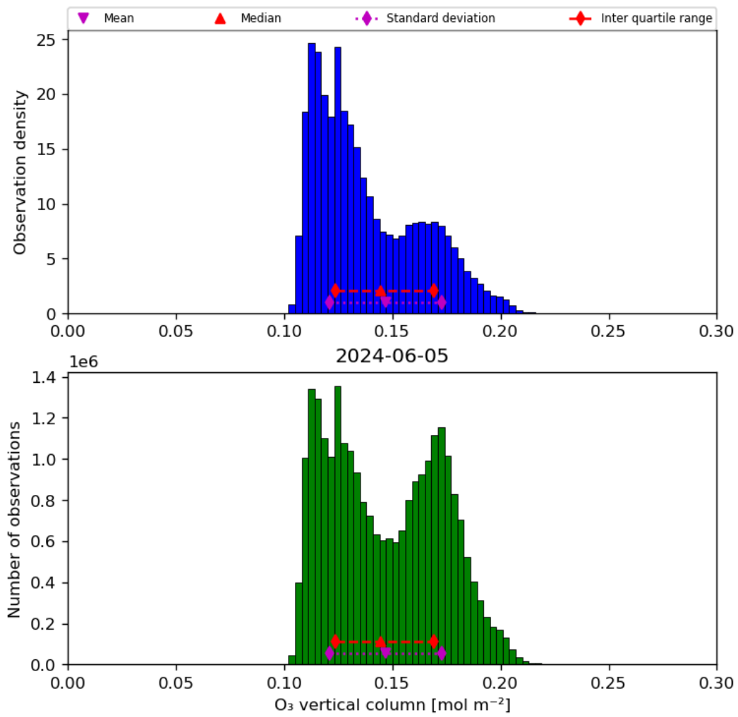
Figure 21: Histogram of “O 3 vertical column” for 2024-06-04 to 2024-06-06
