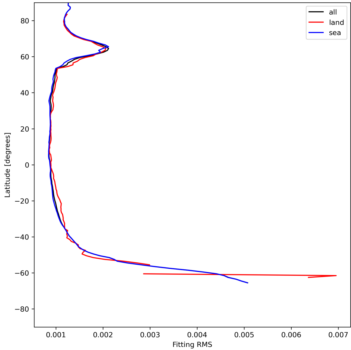
Figure 16: Zonal average of “Fitting RMS” for 2024-06-04 to 2024-06-06.
