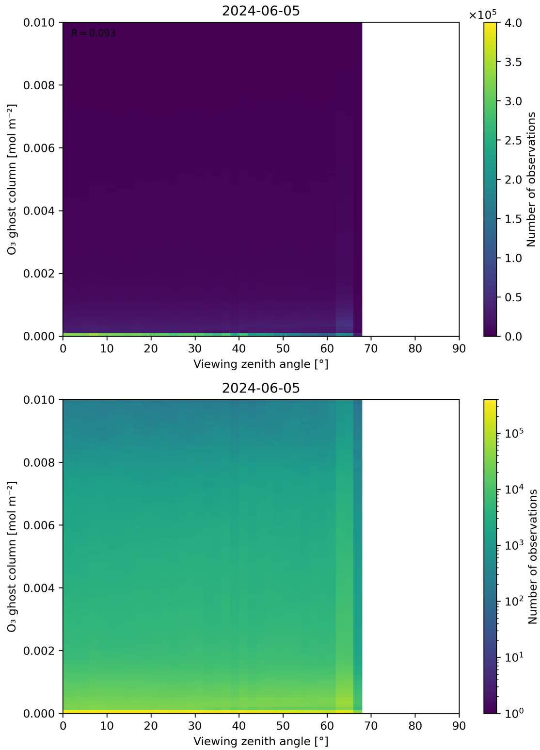
Figure 51: Scatter density plot of “Viewing zenith angle” against “O 3 ghost column” for 2024-06-04 to 2024-06-06.
