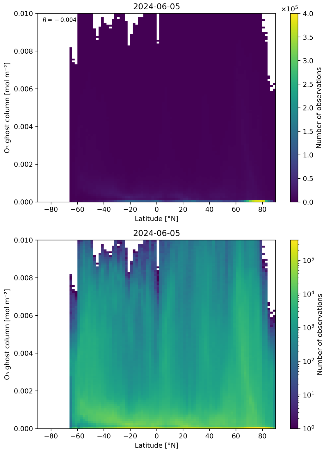
Figure 35: Scatter density plot of “Latitude” against “O 3 ghost column” for 2024-06-04 to 2024-06-06.
