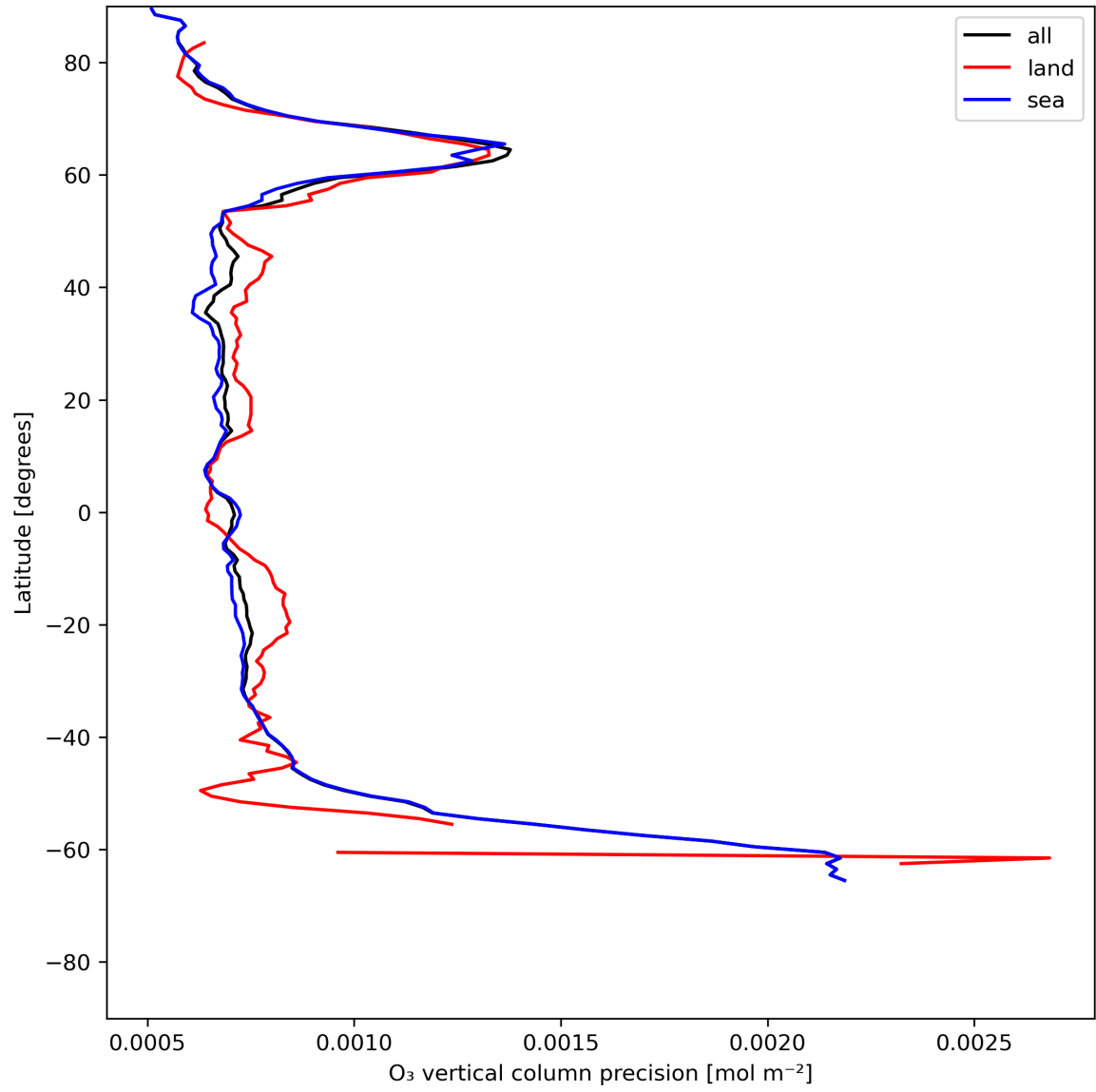
Figure 15: Zonal average of “O 3 vertical column precision” for 2024-06-04 to 2024-06-06.
