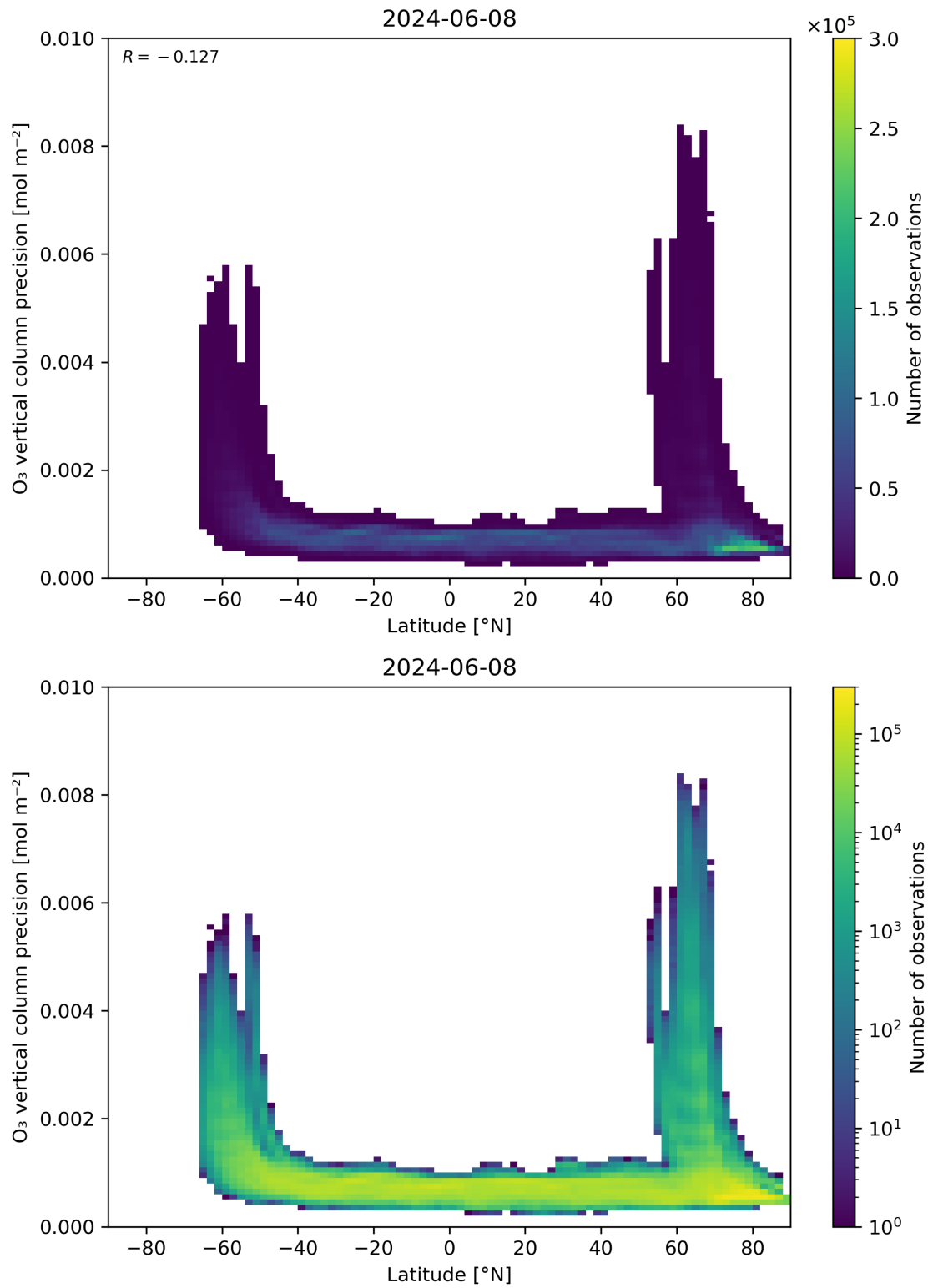
Figure 37: Scatter density plot of “Latitude” against “O 3 vertical column precision” for 2024-06-08 to 2024-06-09.
