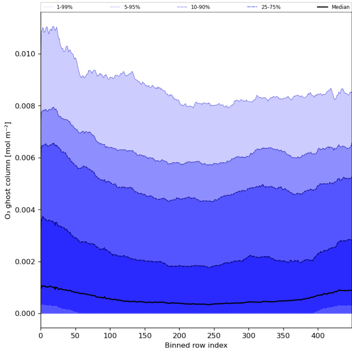
Figure 32: Along track statistics of “O 3 ghost column” for 2024-06-08 to 2024-06-09
