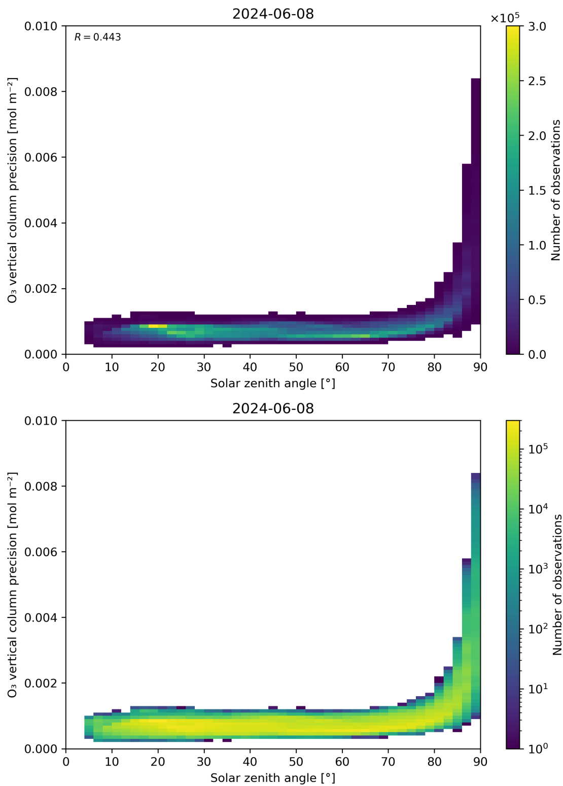
Figure 48: Scatter density plot of “Solar zenith angle” against “O 3 vertical column precision” for 2024-06-08 to 2024-06-09.
