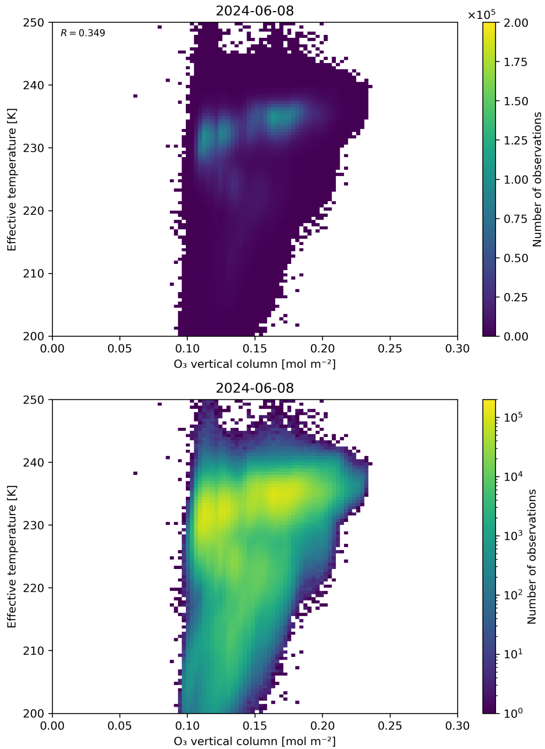
Figure 39: Scatter density plot of “O 3 vertical column” against “Effective temperature” for 2024-06-08 to 2024-06-09.
