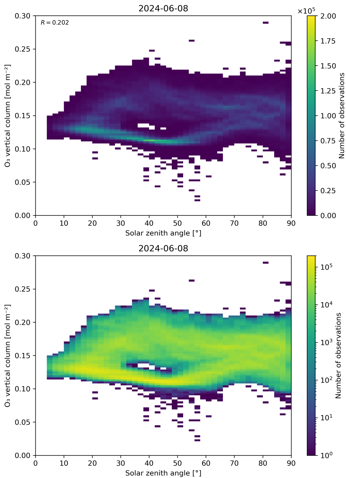
Figure 47: Scatter density plot of “Solar zenith angle” against “O 3 vertical column” for 2024-06-08 to 2024-06-09.
