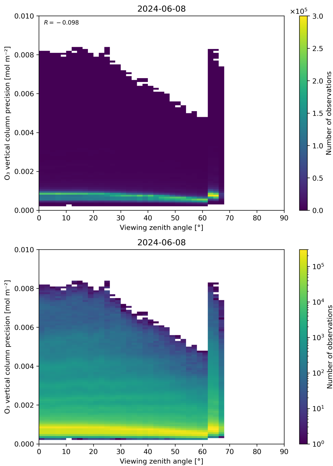
Figure 53: Scatter density plot of “Viewing zenith angle” against “O 3 vertical column precision” for 2024-06-08 to 2024-06-09.
