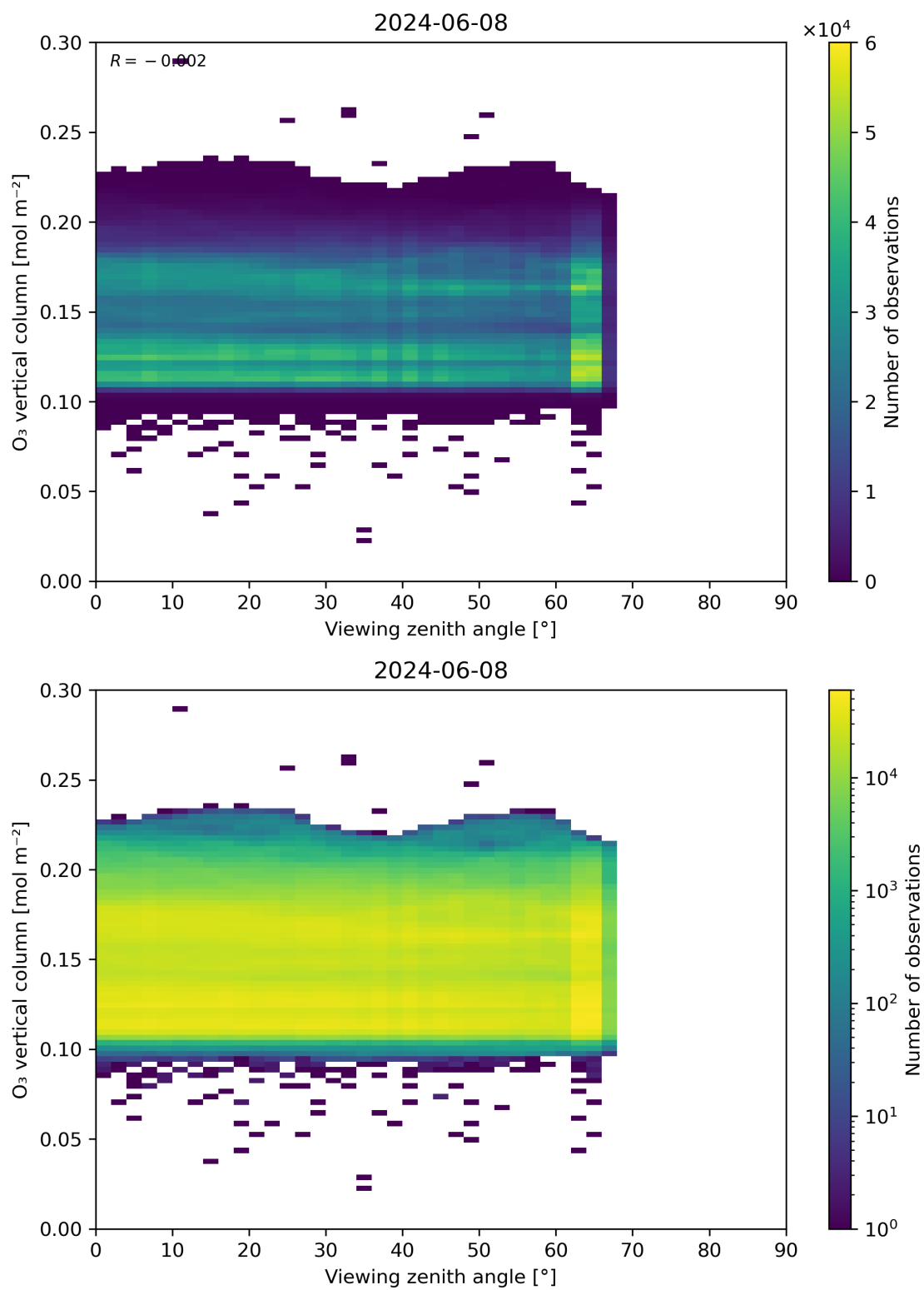
Figure 52: Scatter density plot of “Viewing zenith angle” against “O 3 vertical column” for 2024-06-08 to 2024-06-09.
