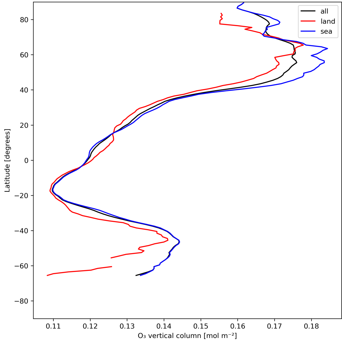
Figure 14: Zonal average of “O 3 vertical column” for 2024-06-08 to 2024-06-09.
