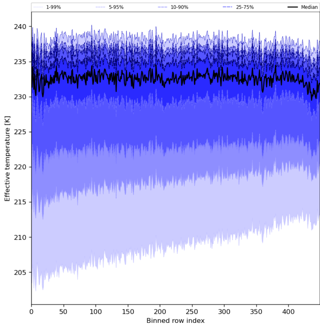
Figure 31: Along track statistics of “Effective temperature” for 2024-06-08 to 2024-06-09
