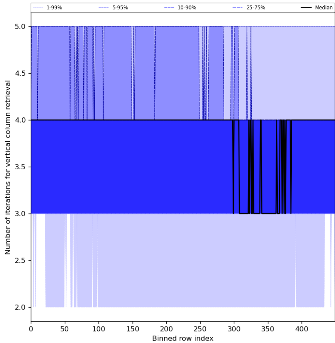
Figure 33: Along track statistics of “Number of iterations for vertical column retrieval” for 2024-06-08 to 2024-06-09
