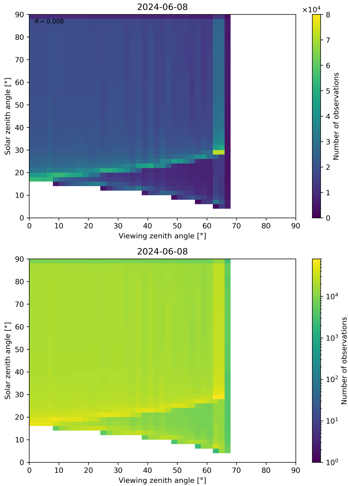
Figure 54: Scatter density plot of “Viewing zenith angle” against “Solar zenith angle” for 2024-06-08 to 2024-06-09.
