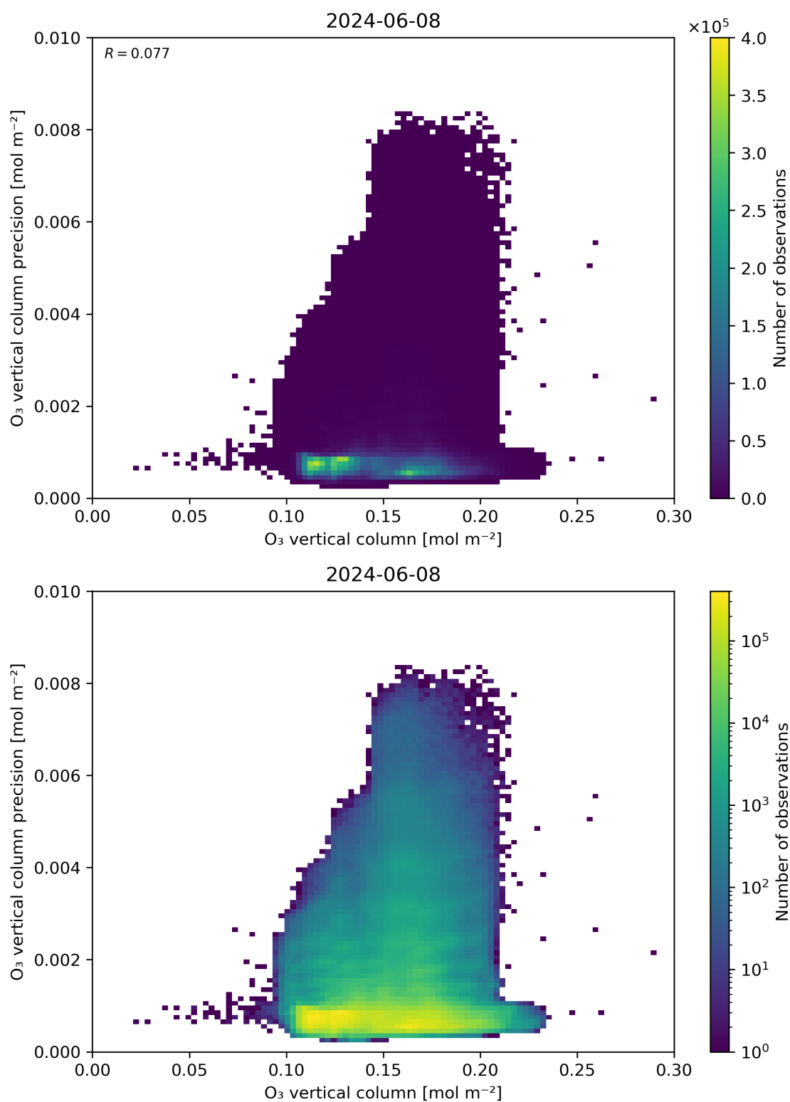
Figure 41: Scatter density plot of “O 3 vertical column” against “O 3 vertical column precision” for 2024-06-08 to 2024-06-09.
