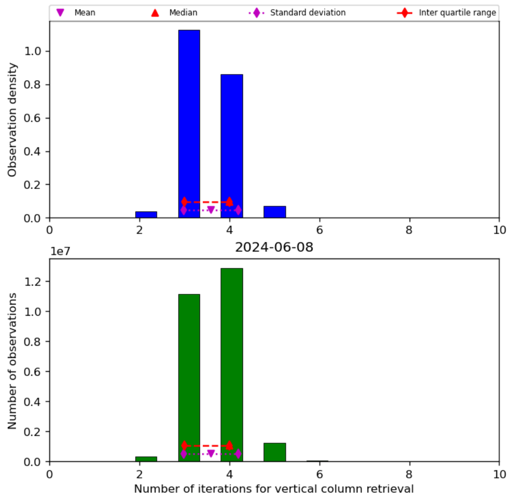
Figure 26: Histogram of “Number of iterations for vertical column retrieval” for 2024-06-08 to 2024-06-09
