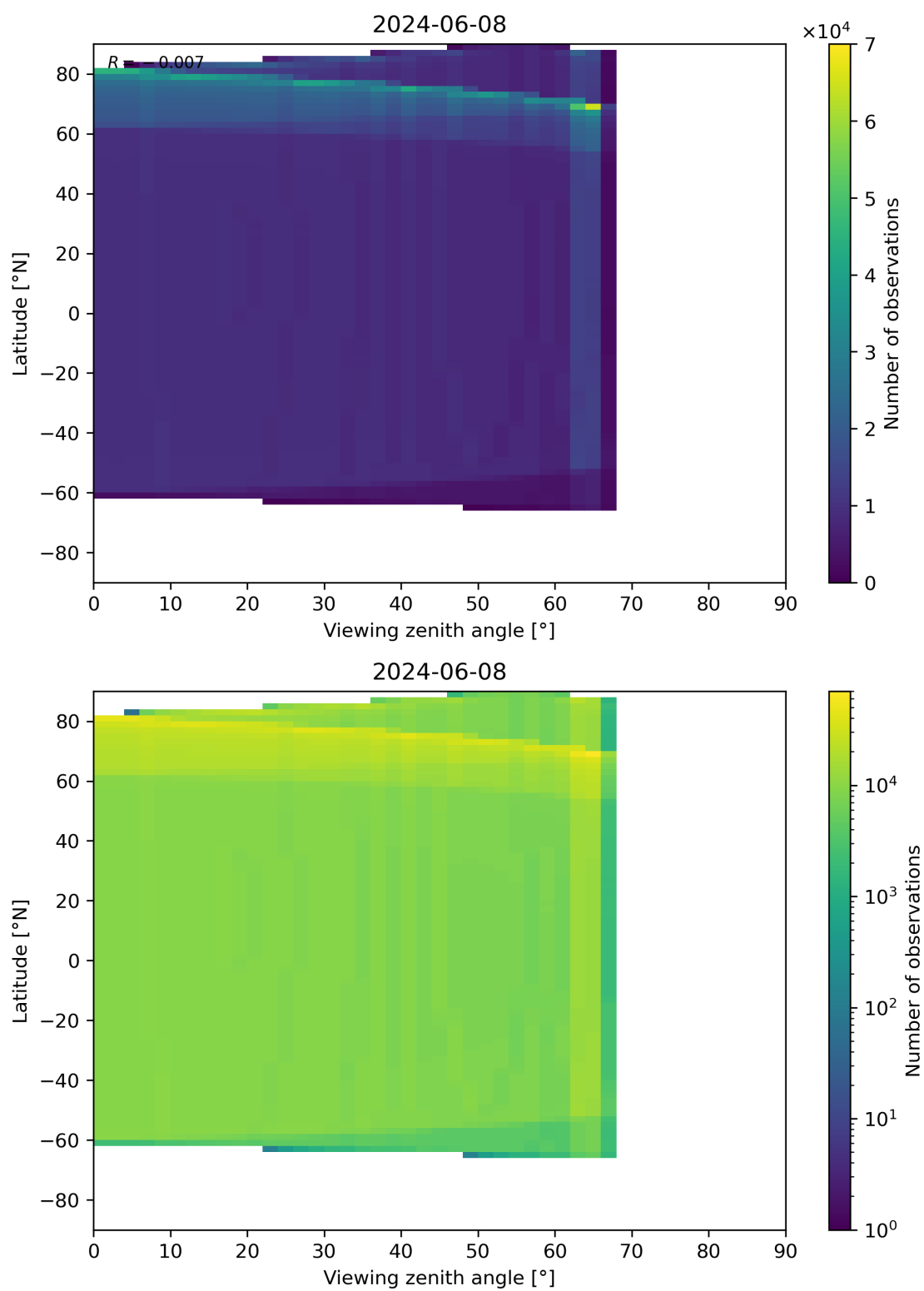
Figure 49: Scatter density plot of “Viewing zenith angle” against “Latitude” for 2024-06-08 to 2024-06-09.
