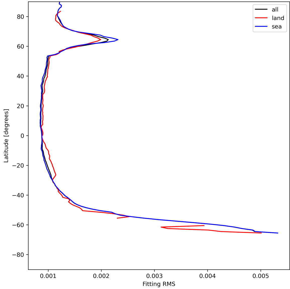
Figure 16: Zonal average of “Fitting RMS” for 2024-06-08 to 2024-06-09.
