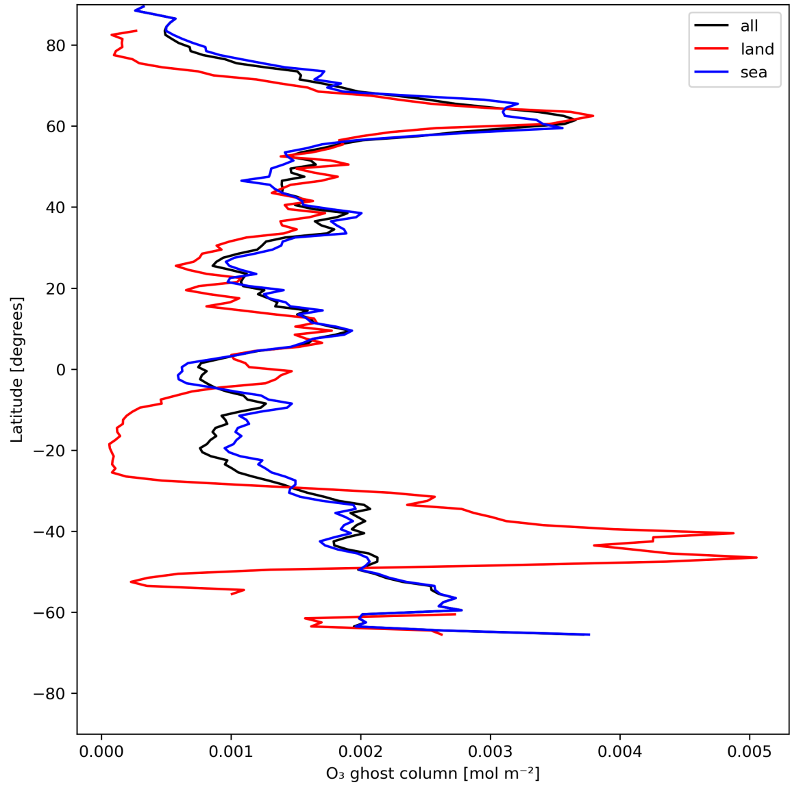
Figure 18: Zonal average of “O 3 ghost column” for 2024-06-08 to 2024-06-09.
