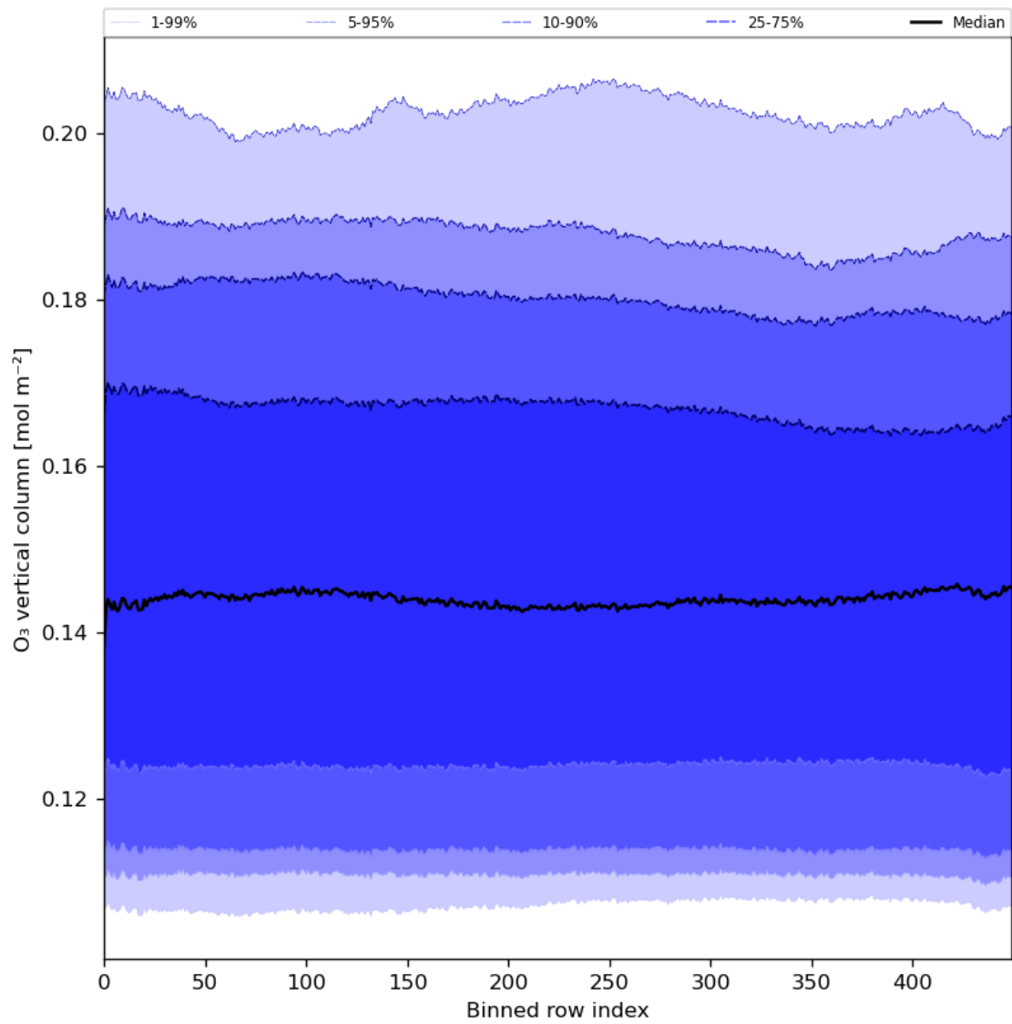
Figure 28: Along track statistics of “O 3 vertical column” for 2024-06-08 to 2024-06-09
