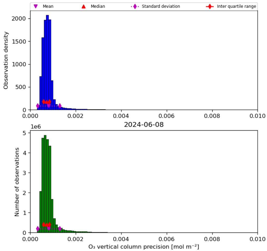
Figure 22: Histogram of “O 3 vertical column precision” for 2024-06-08 to 2024-06-09
