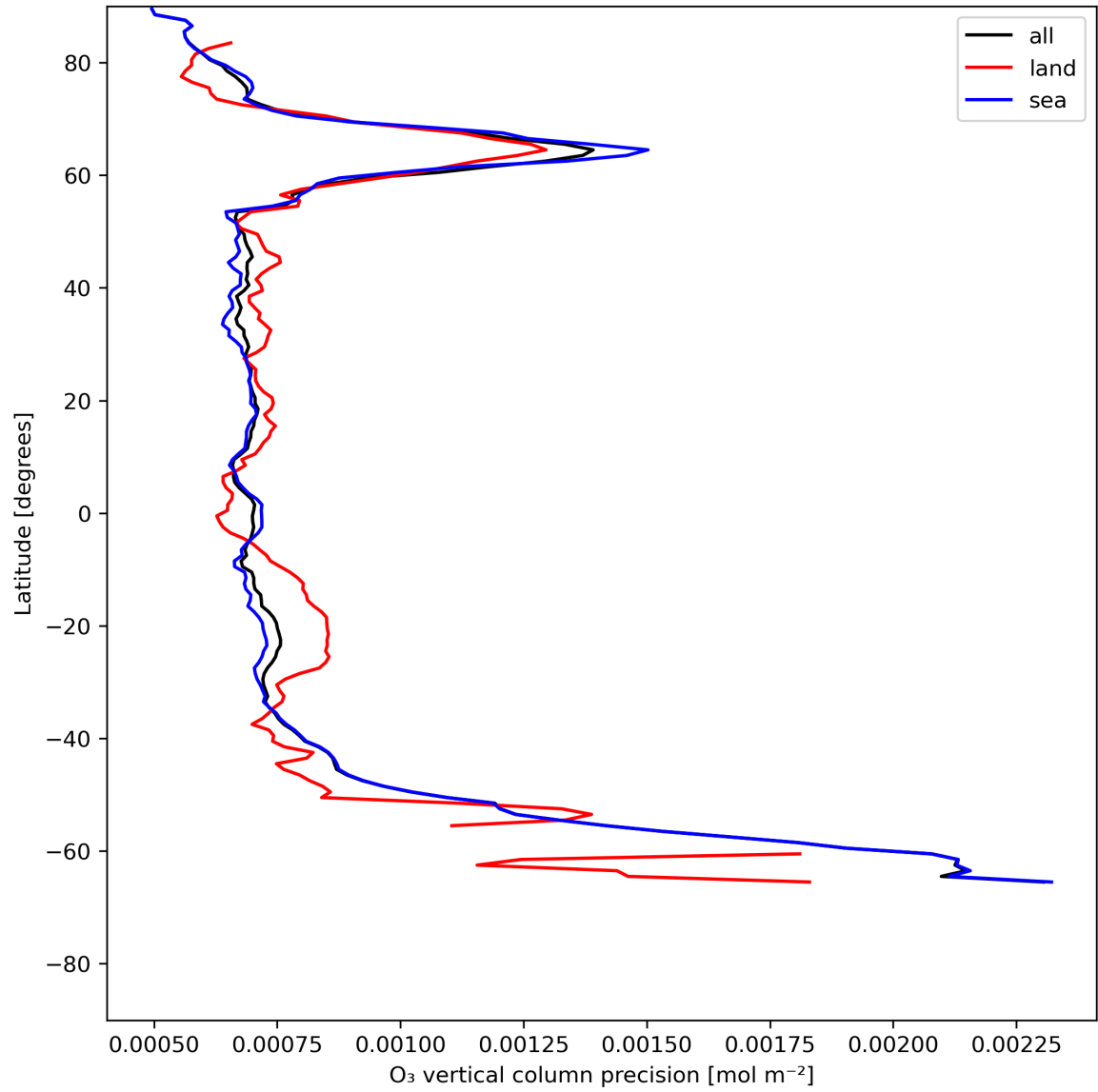
Figure 15: Zonal average of “O 3 vertical column precision” for 2024-06-08 to 2024-06-09.
