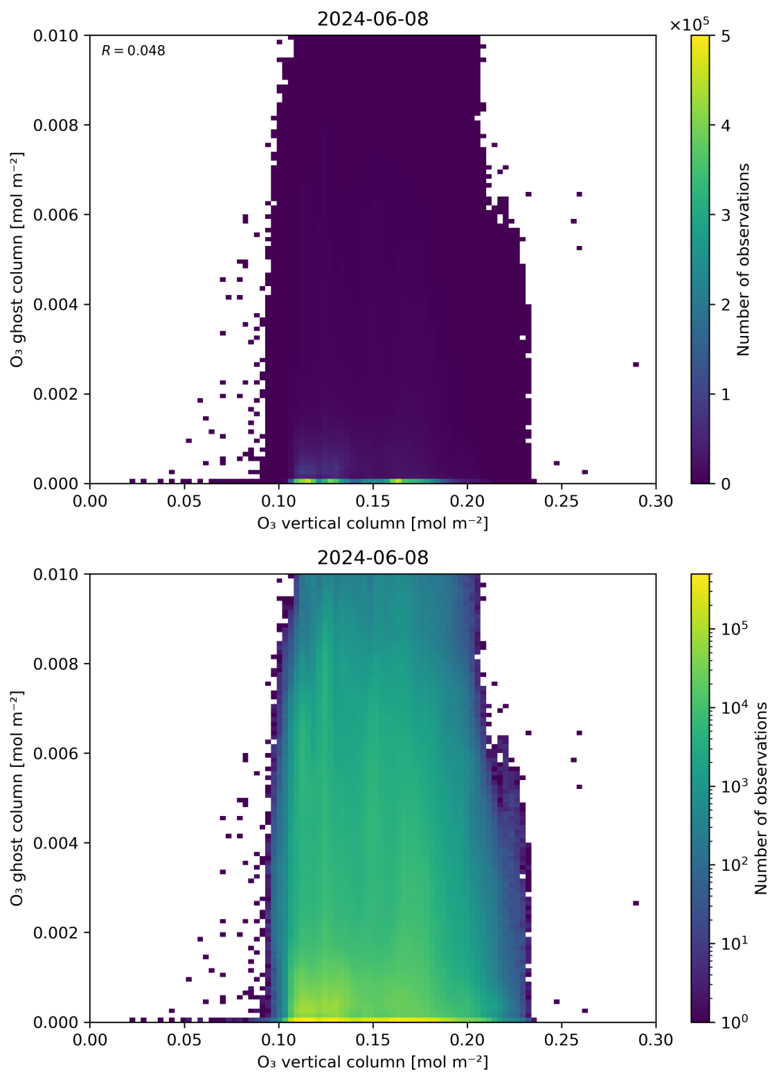
Figure 40: Scatter density plot of “O 3 vertical column” against “O 3 ghost column” for 2024-06-08 to 2024-06-09.
