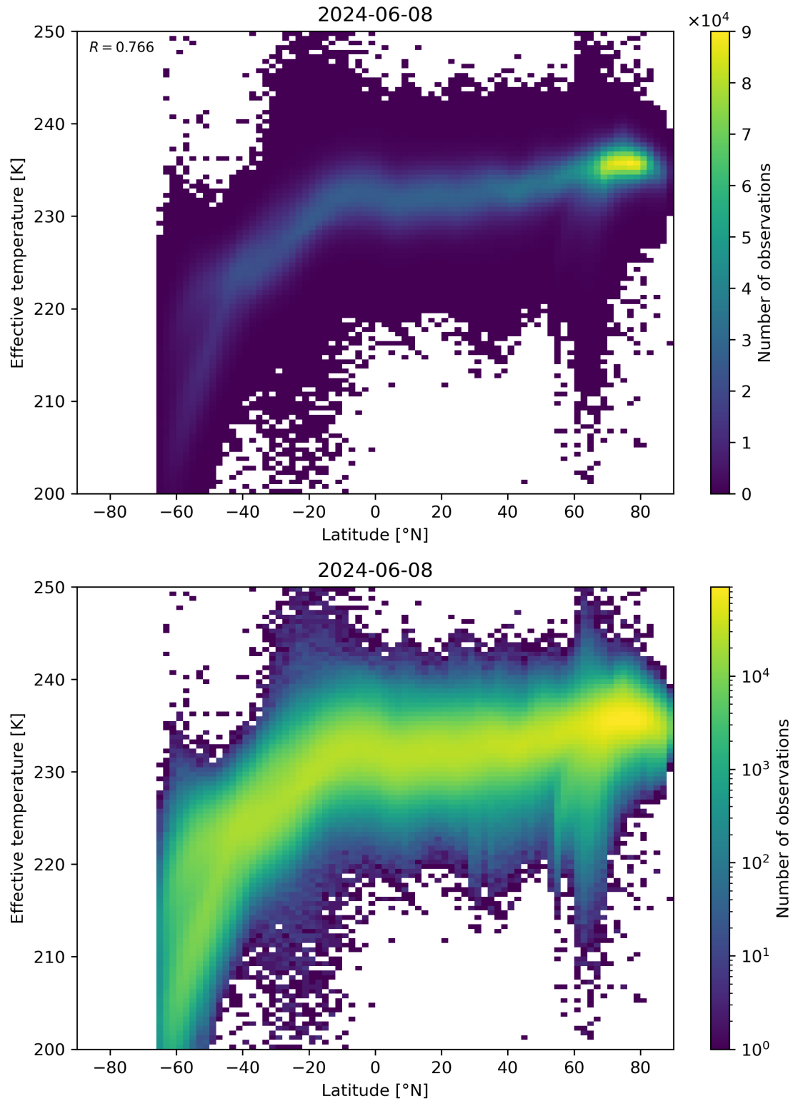
Figure 34: Scatter density plot of “Latitude” against “Effective temperature” for 2024-06-08 to 2024-06-09.
