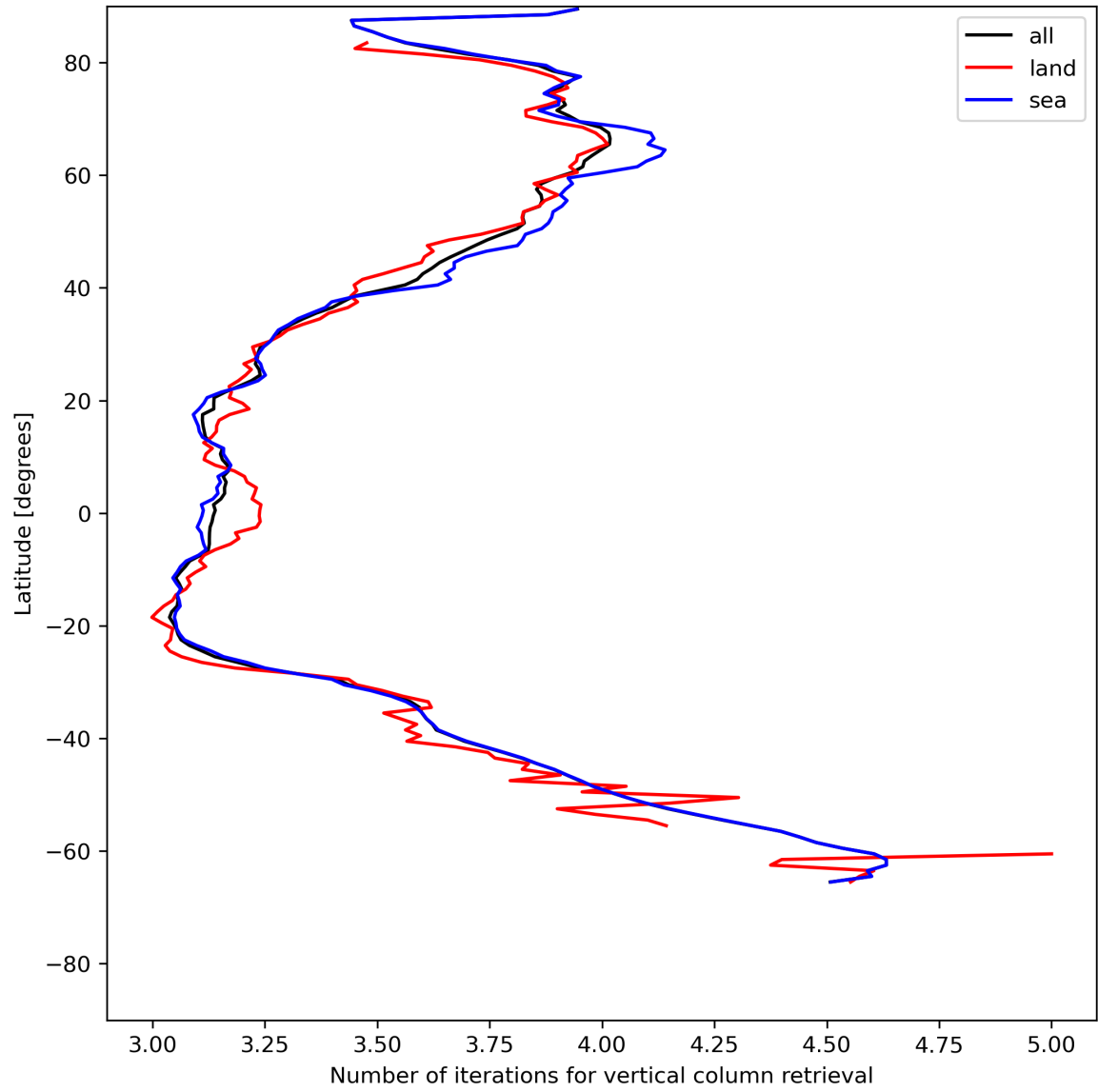
Figure 19: Zonal average of “Number of iterations for vertical column retrieval” for 2024-06-08 to 2024-06-09.
