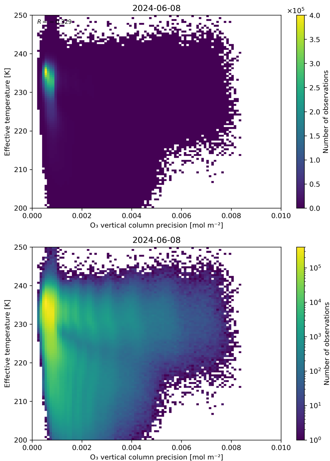
Figure 42: Scatter density plot of “O 3 vertical column precision” against “Effective temperature” for 2024-06-08 to 2024-06-09.
