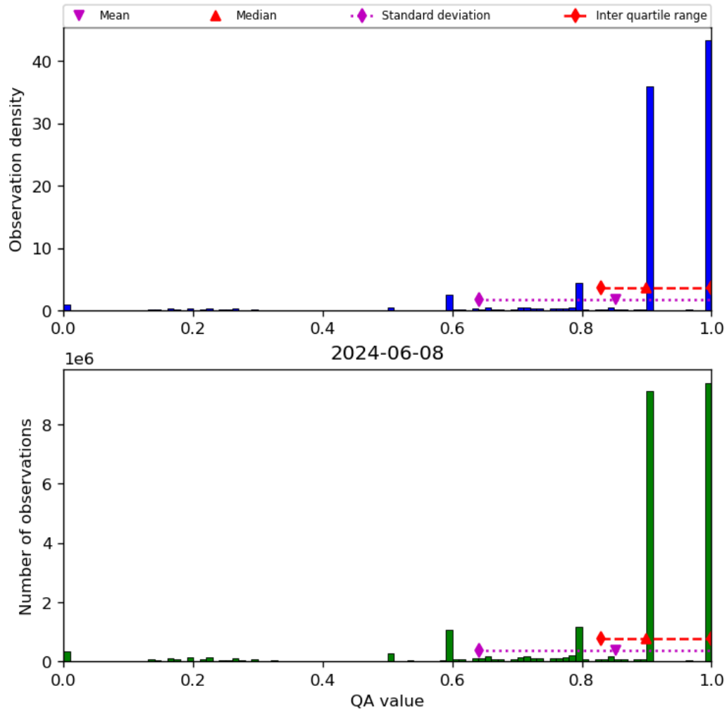
Figure 20: Histogram of “QA value” for 2024-06-08 to 2024-06-09
