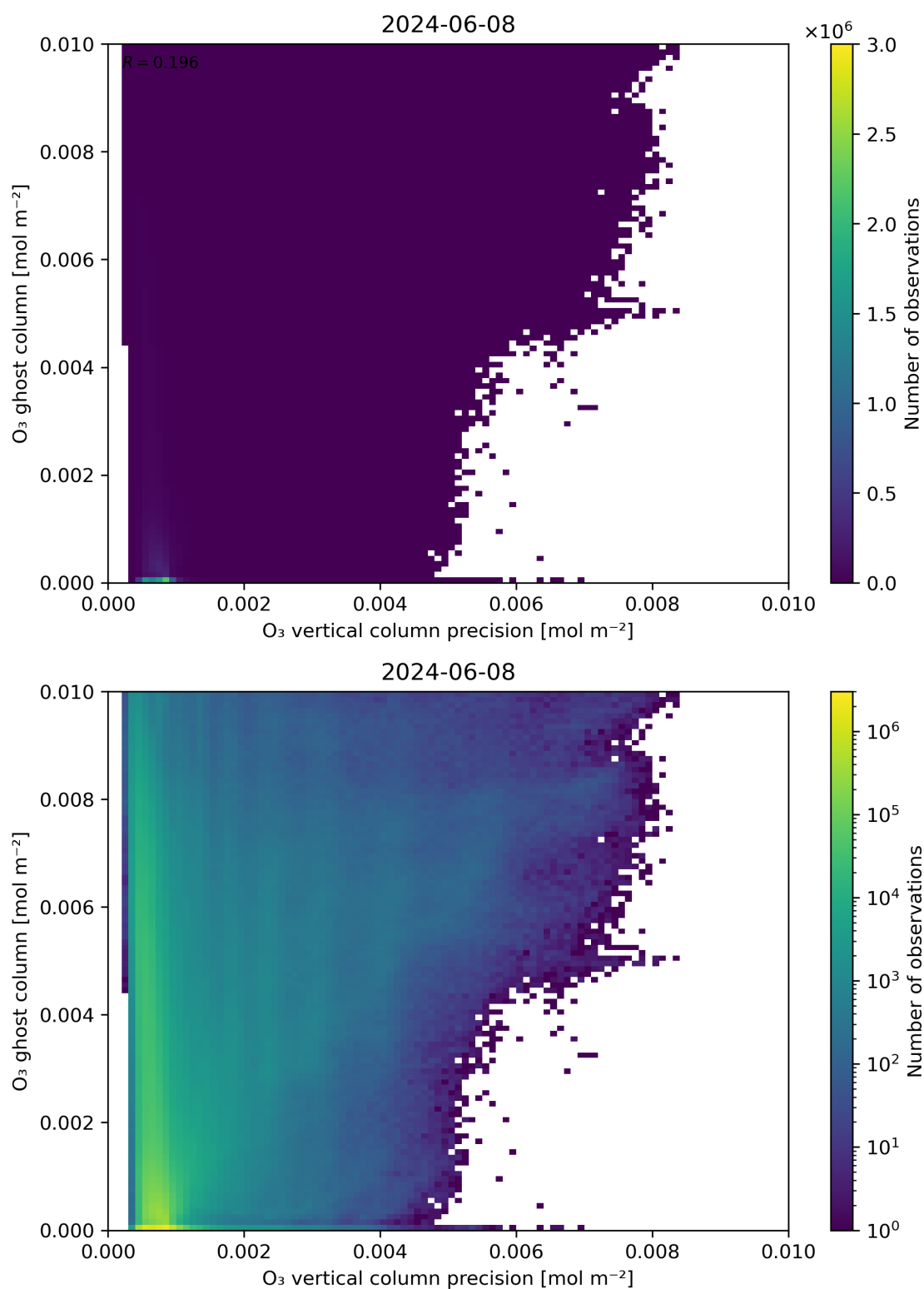
Figure 43: Scatter density plot of “O 3 vertical column precision” against “O 3 ghost column” for 2024-06-08 to 2024-06-09.
