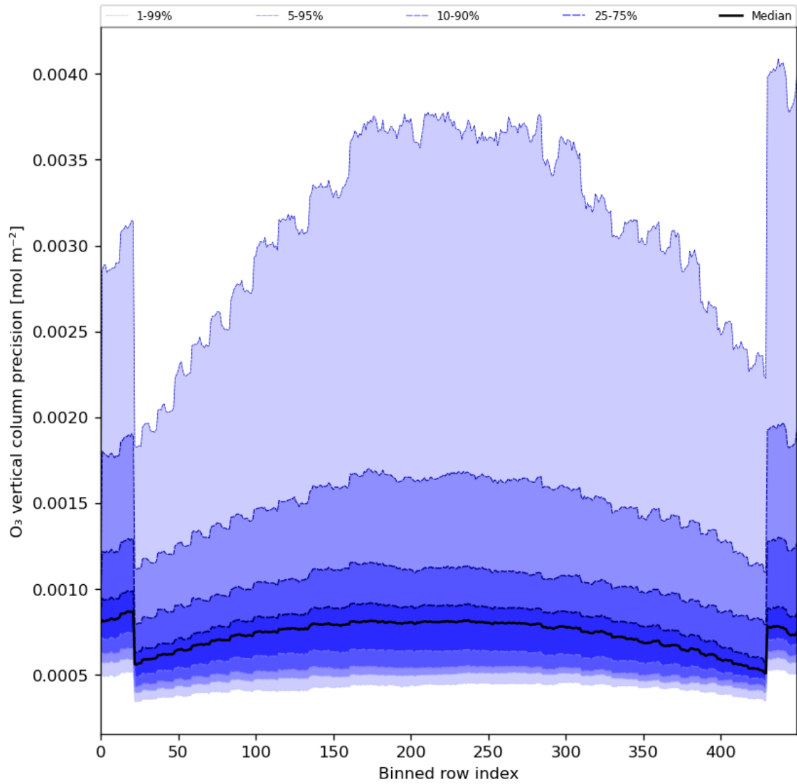
Figure 29: Along track statistics of “O 3 vertical column precision” for 2024-06-08 to 2024-06-09
