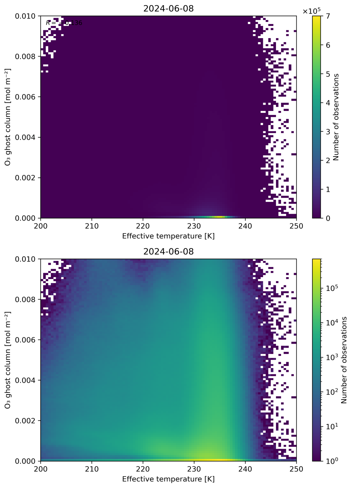
Figure 38: Scatter density plot of “Effective temperature” against “O 3 ghost column” for 2024-06-08 to 2024-06-09.
