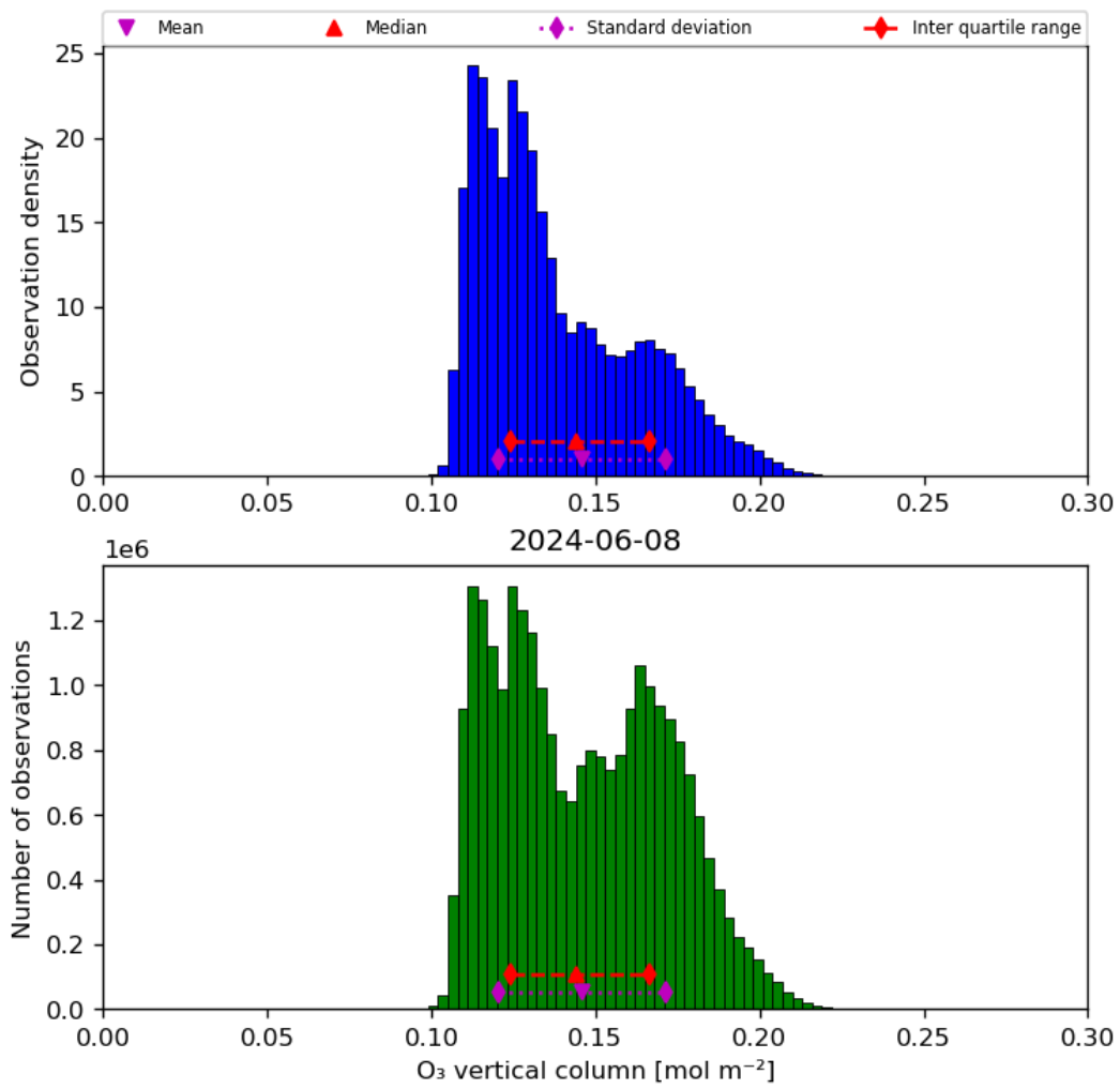
Figure 21: Histogram of “O 3 vertical column” for 2024-06-08 to 2024-06-09
