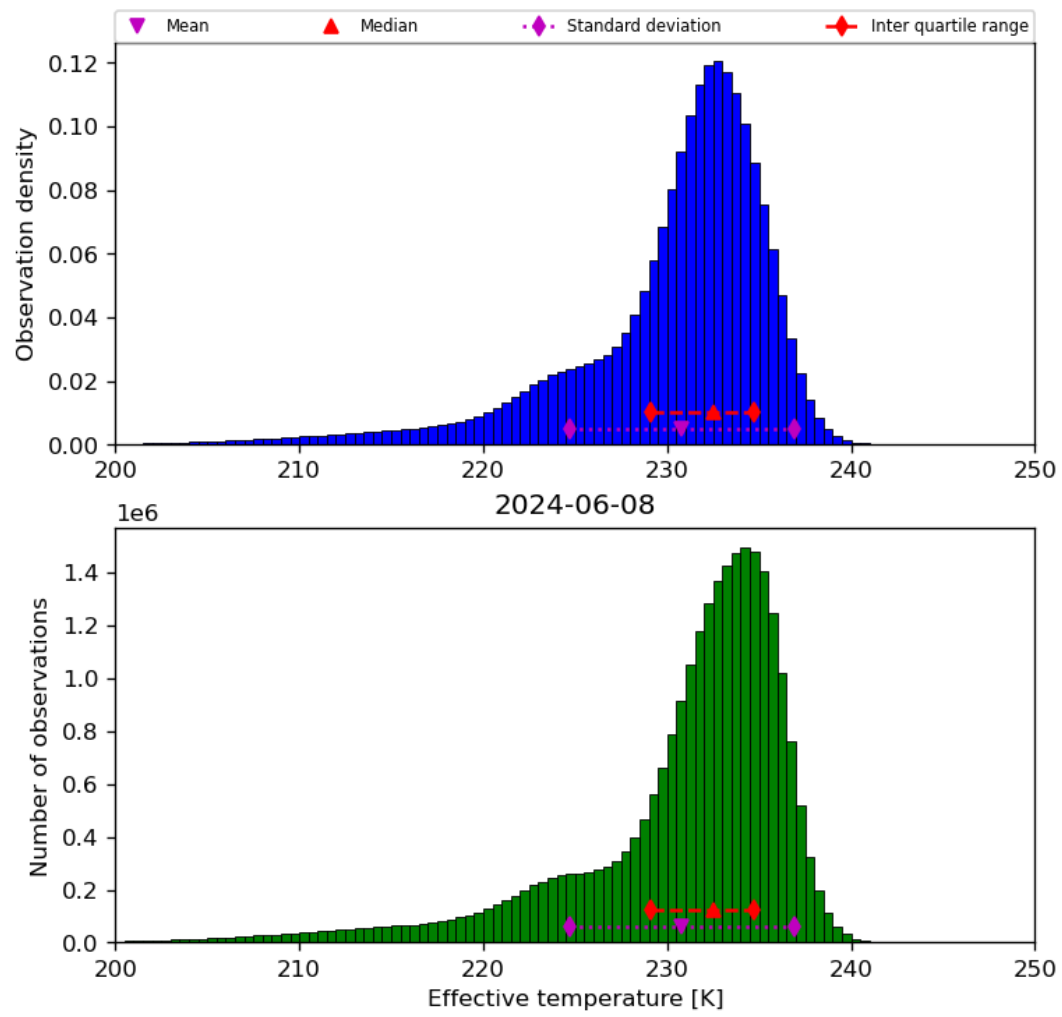
Figure 24: Histogram of “Effective temperature” for 2024-06-08 to 2024-06-09
