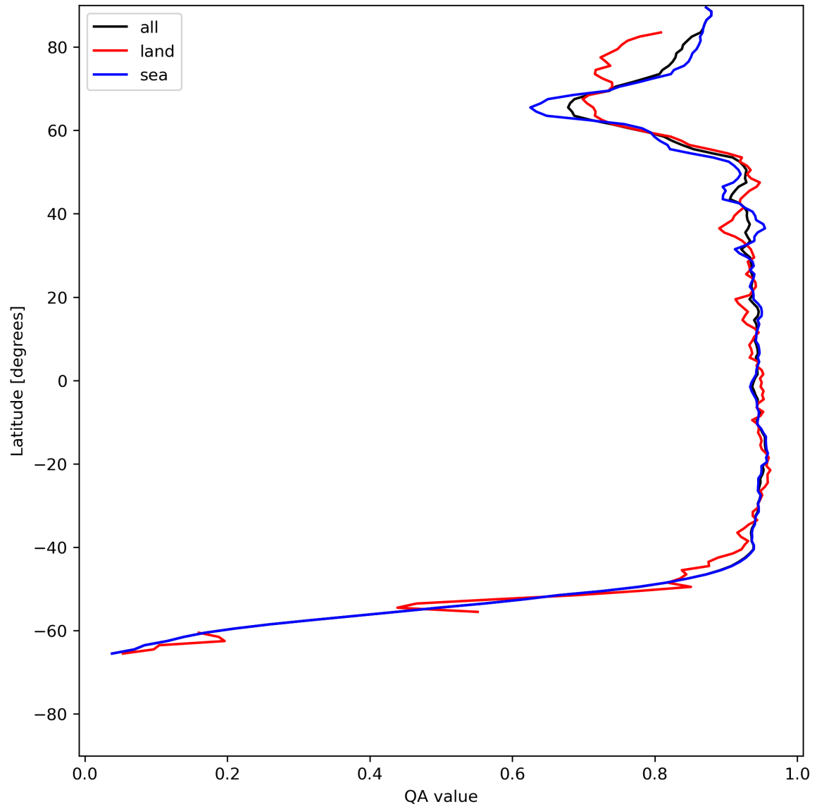
Figure 13: Zonal average of “QA value” for 2024-06-08 to 2024-06-09.
