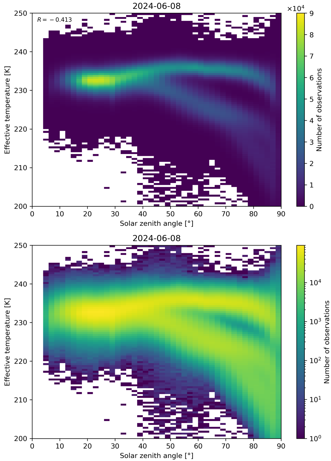
Figure 45: Scatter density plot of “Solar zenith angle” against “Effective temperature” for 2024-06-08 to 2024-06-09.
