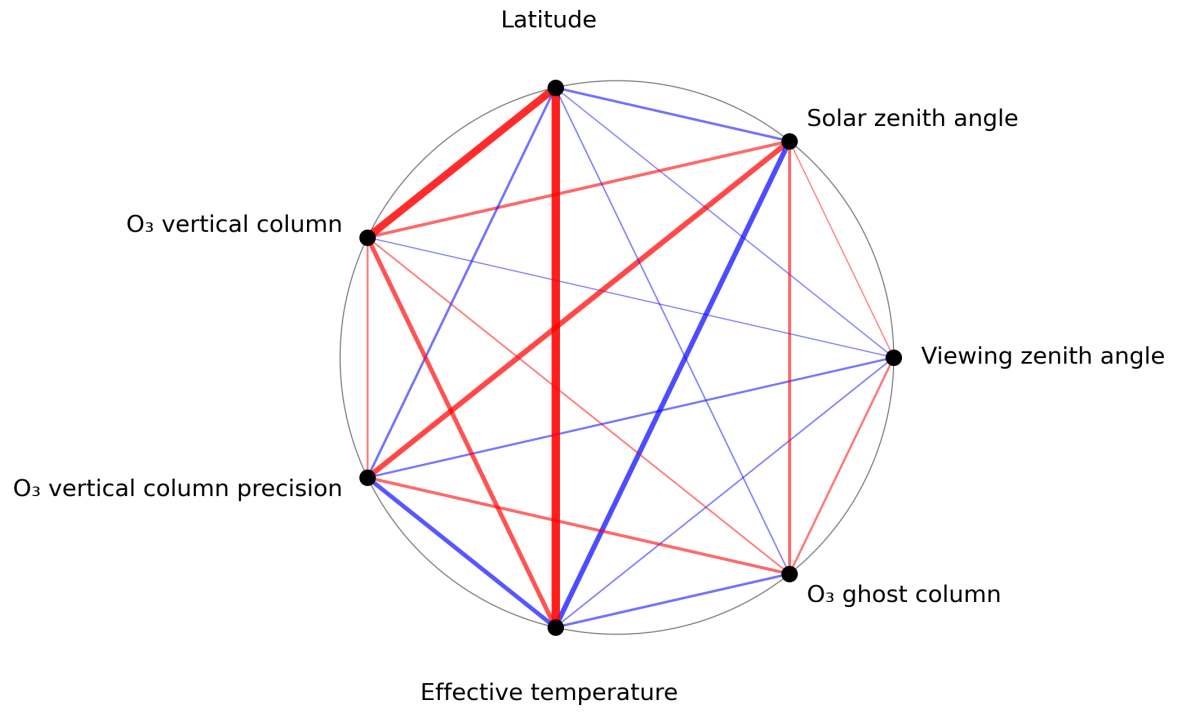
Figure 1: Map of correlation graph for 2024-06-08 to 2024-06-09.
