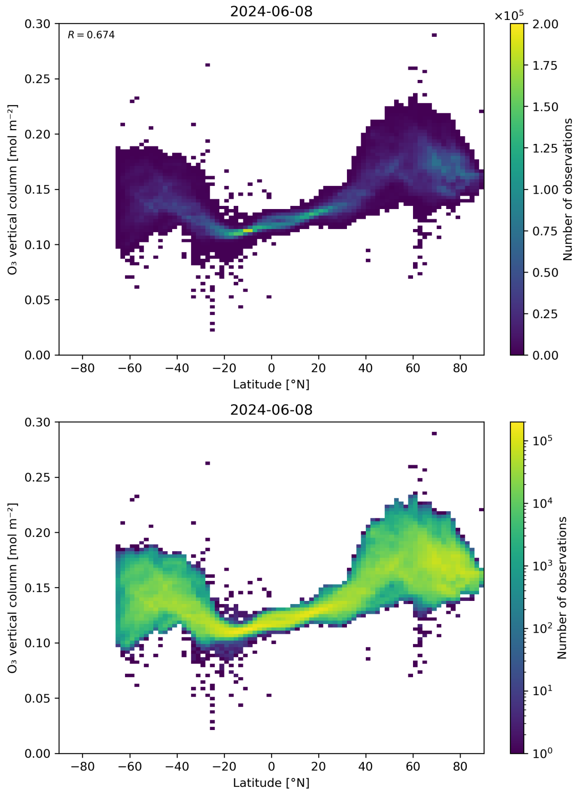
Figure 36: Scatter density plot of “Latitude” against “O 3 vertical column” for 2024-06-08 to 2024-06-09.
