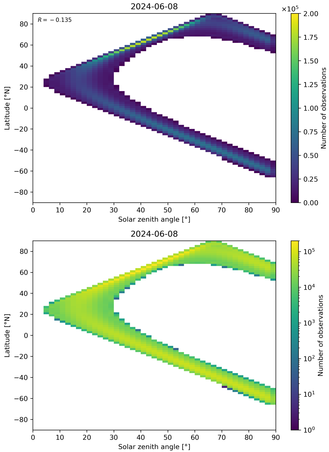
Figure 44: Scatter density plot of “Solar zenith angle” against “Latitude” for 2024-06-08 to 2024-06-09.
