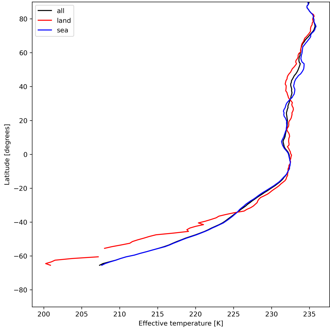
Figure 17: Zonal average of "Effective temperature" for 2024-06-08 to 2024-06-09.
