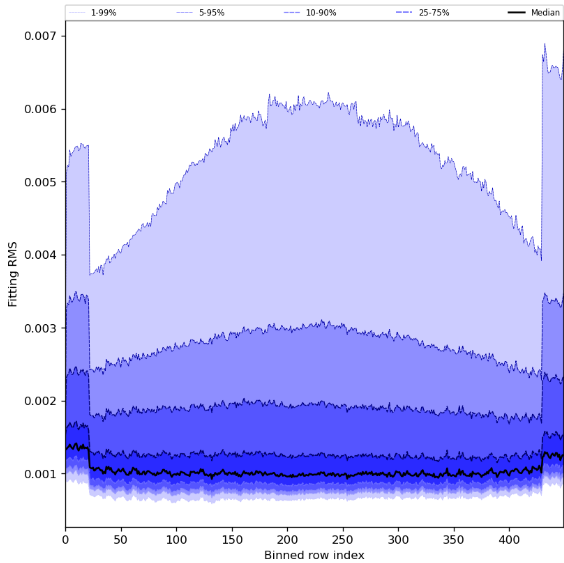
Figure 30: Along track statistics of “Fitting RMS” for 2024-06-08 to 2024-06-09
