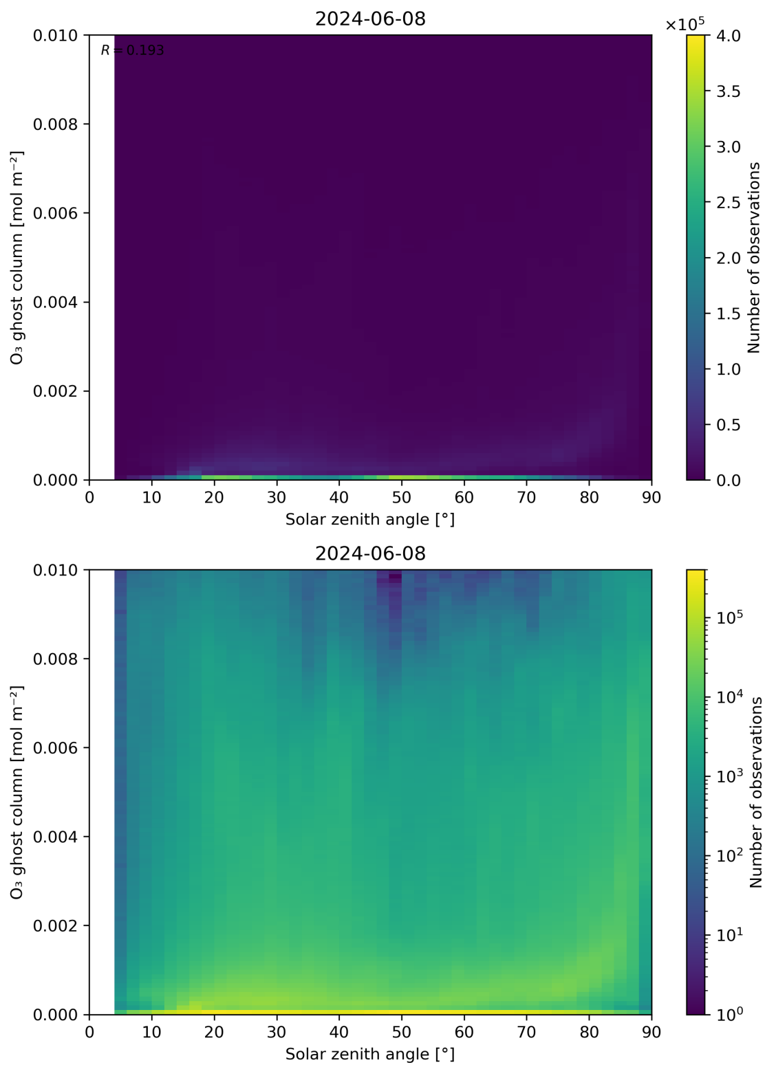
Figure 46: Scatter density plot of “Solar zenith angle” against “O 3 ghost column” for 2024-06-08 to 2024-06-09.
