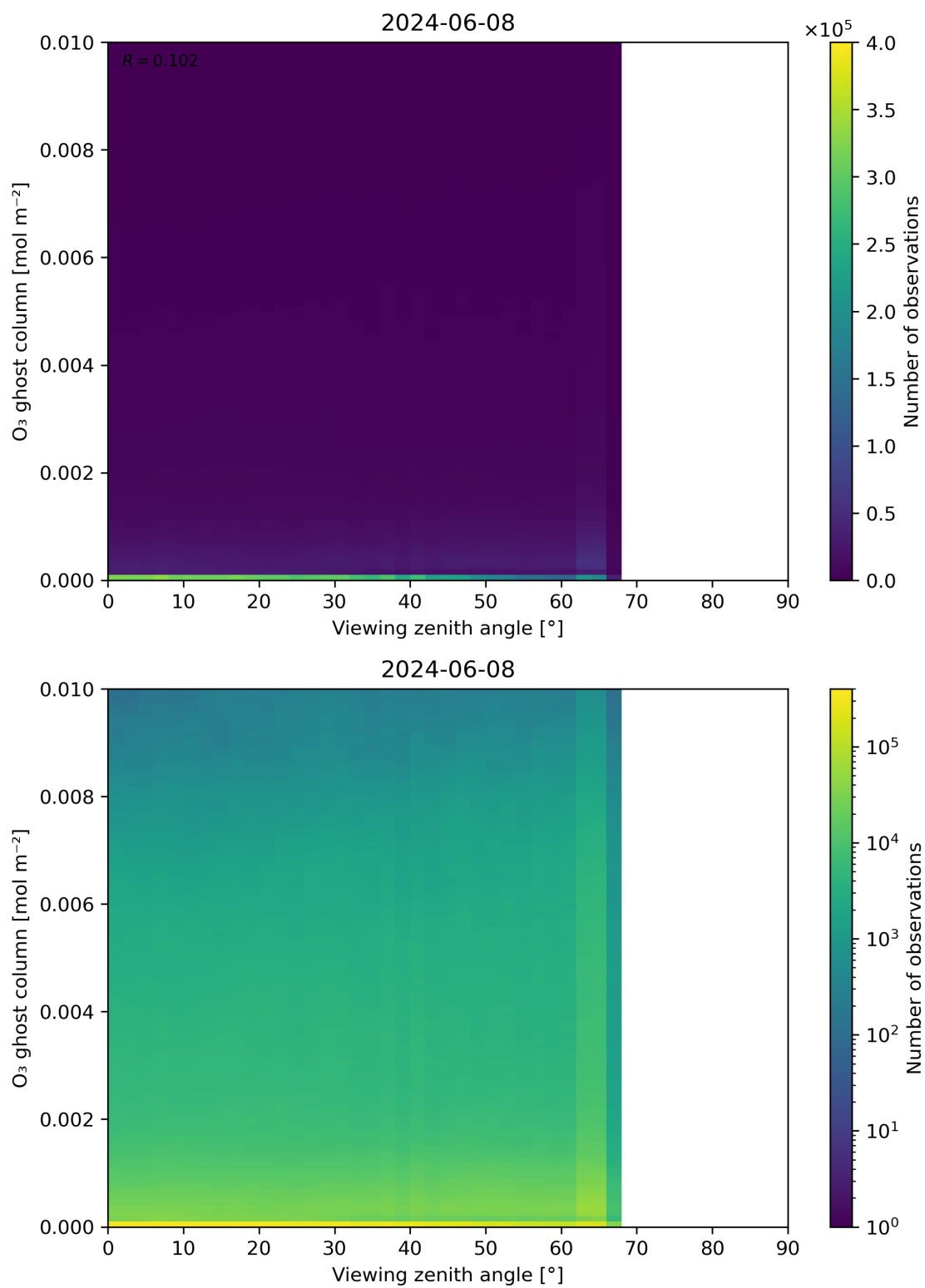
Figure 51: Scatter density plot of “Viewing zenith angle” against “O 3 ghost column” for 2024-06-08 to 2024-06-09.
