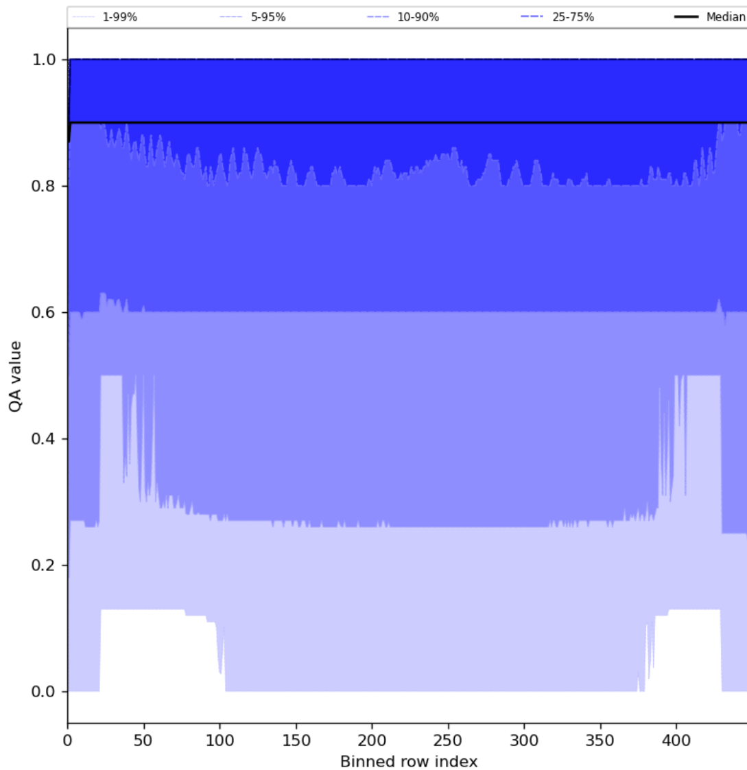
Figure 27: Along track statistics of “QA value” for 2024-06-08 to 2024-06-09
