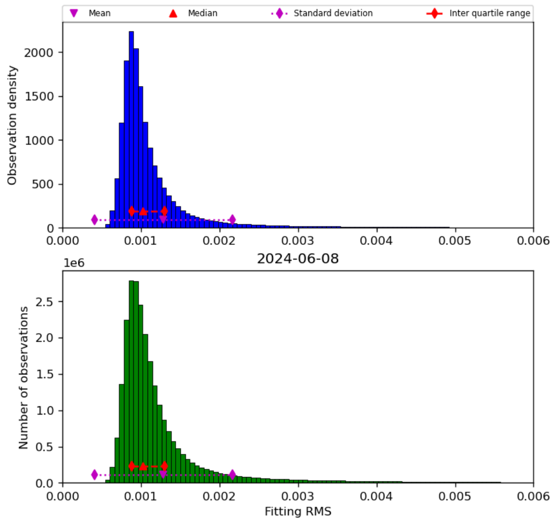
Figure 23: Histogram of “Fitting RMS” for 2024-06-08 to 2024-06-09
