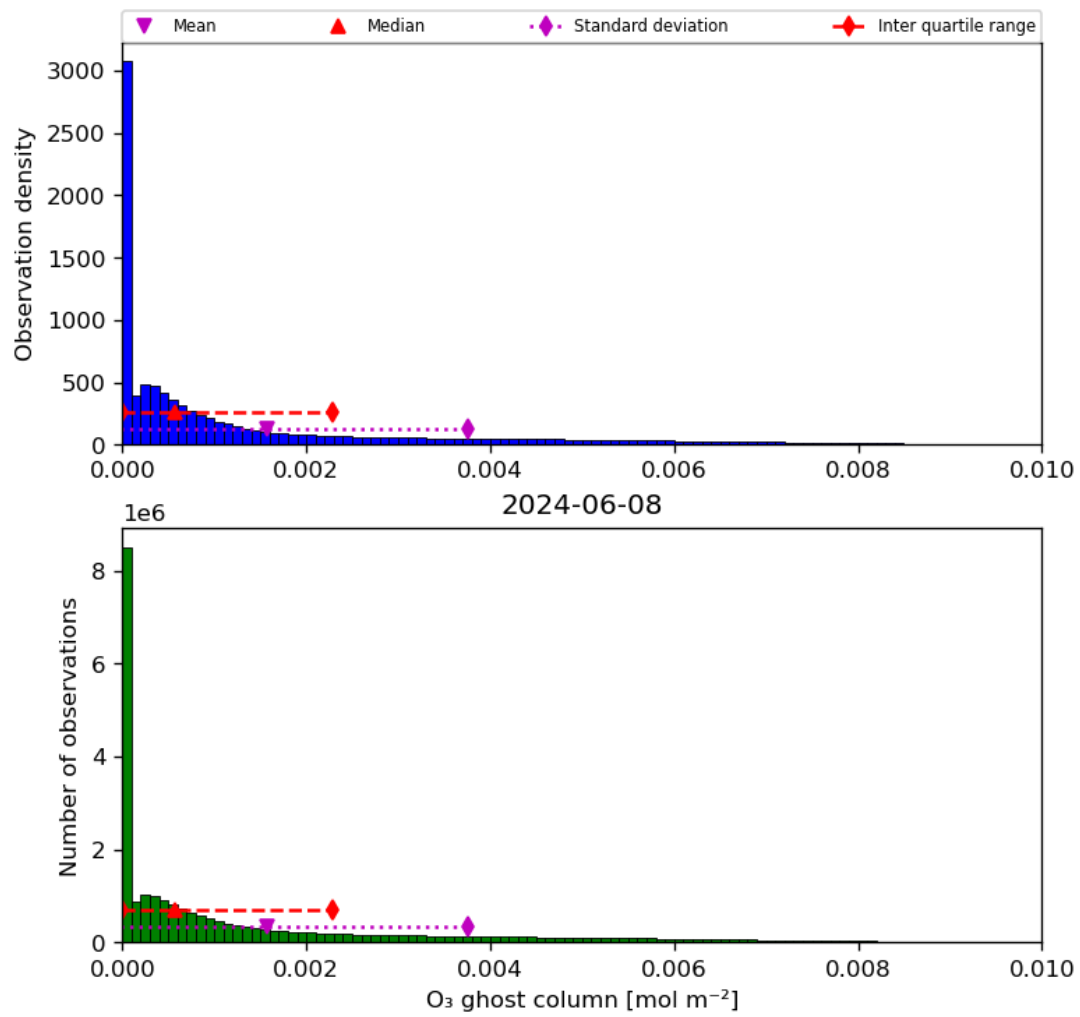
Figure 25: Histogram of “O 3 ghost column” for 2024-06-08 to 2024-06-09
