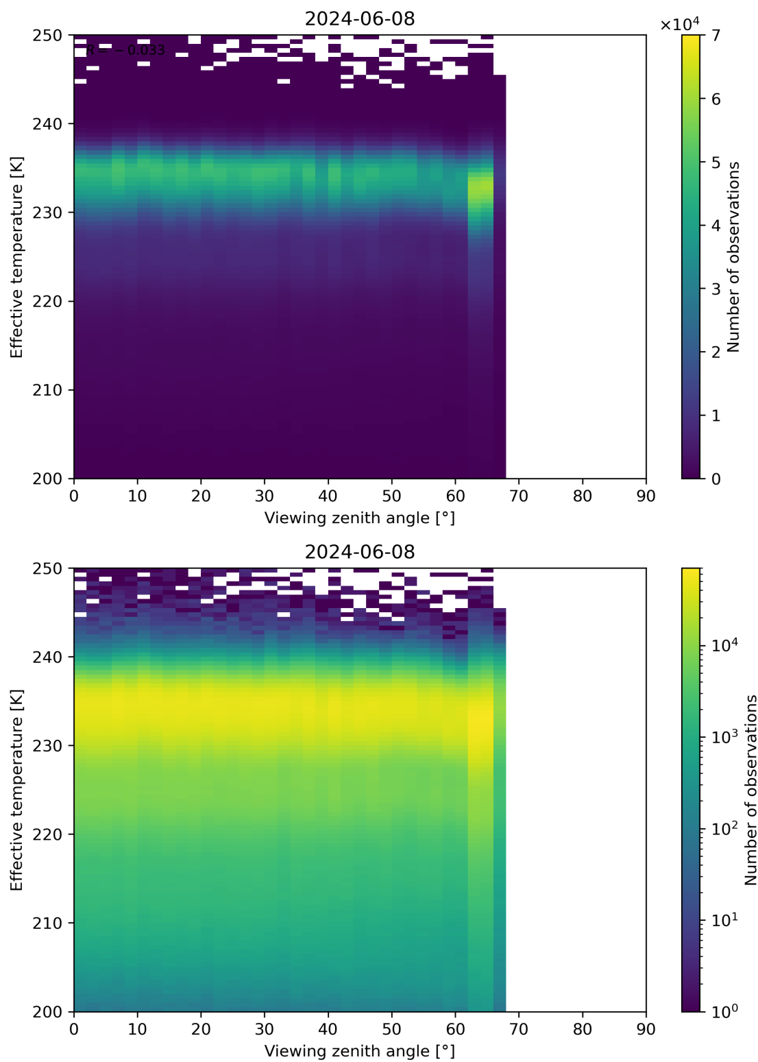
Figure 50: Scatter density plot of “Viewing zenith angle” against “Effective temperature” for 2024-06-08 to 2024-06-09.
