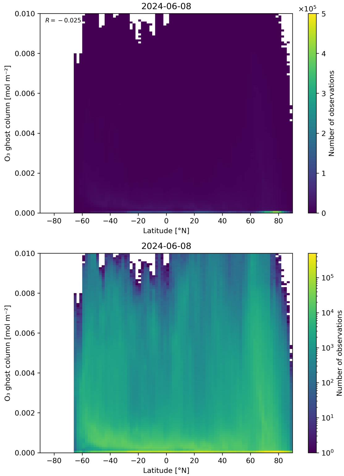
Figure 35: Scatter density plot of “Latitude” against “O 3 ghost column” for 2024-06-08 to 2024-06-09.
