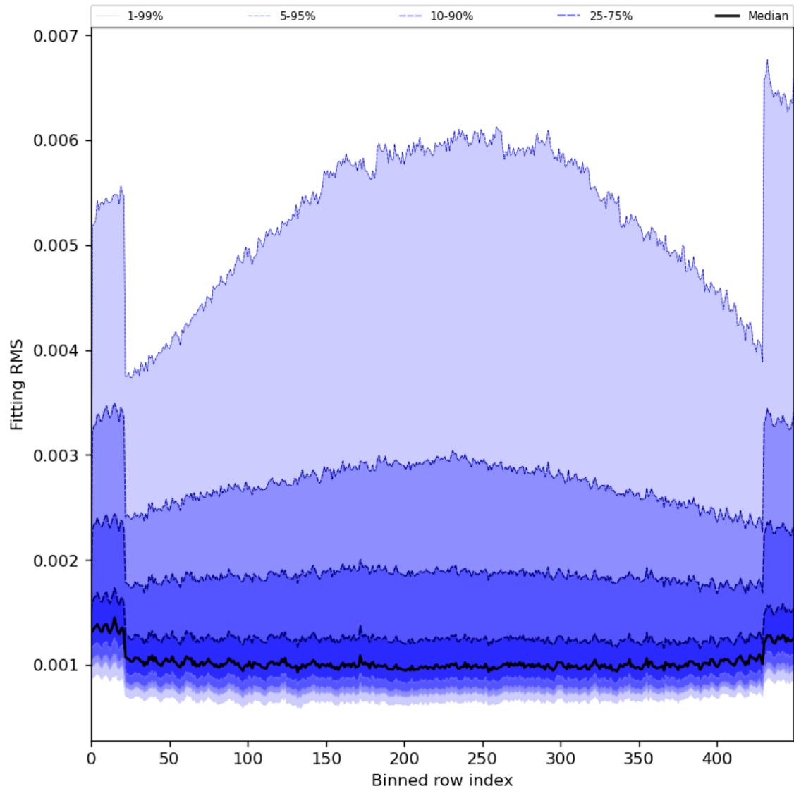
Figure 30: Along track statistics of “Fitting RMS” for 2024-06-08 to 2024-06-10
