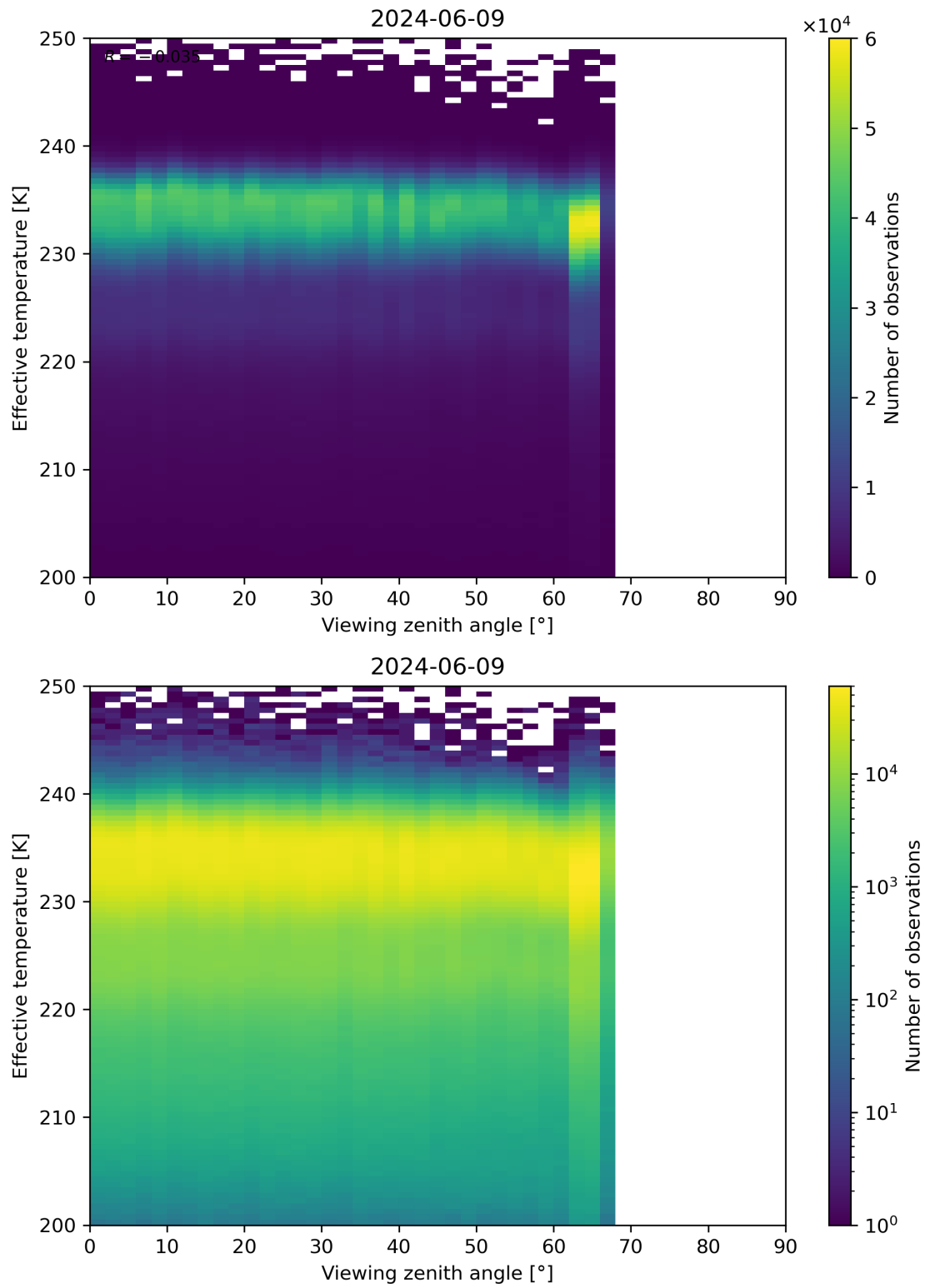
Figure 50: Scatter density plot of “Viewing zenith angle” against “Effective temperature” for 2024-06-08 to 2024-06-10.
