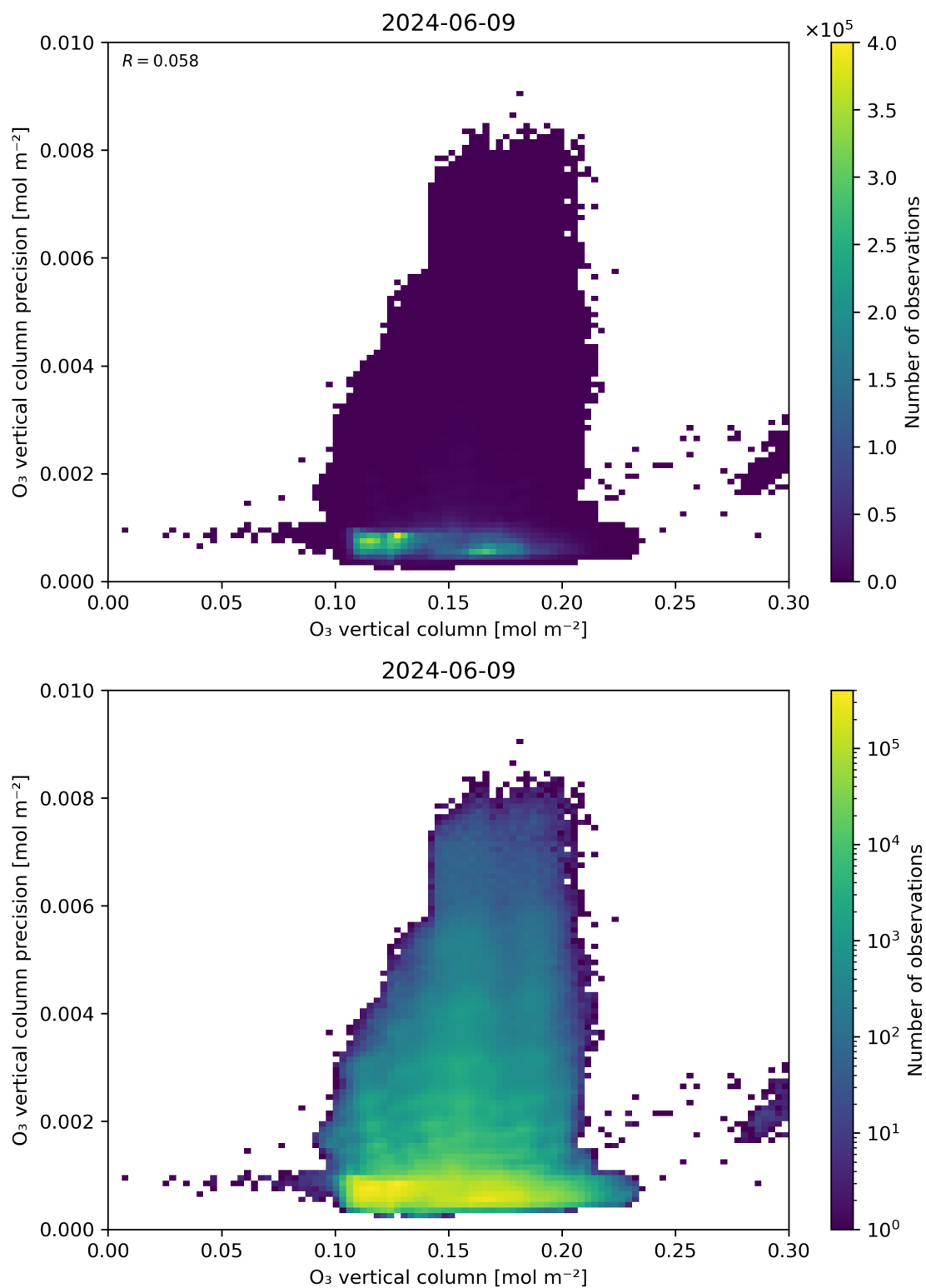
Figure 41: Scatter density plot of “O 3 vertical column” against “O 3 vertical column precision” for 2024-06-08 to 2024-06-10.
