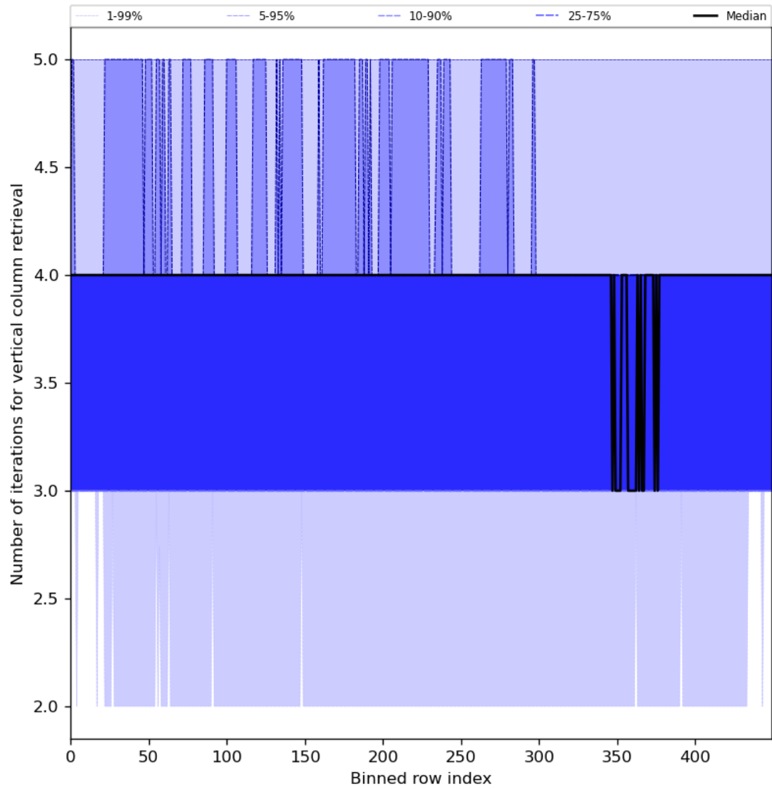
Figure 33: Along track statistics of “Number of iterations for vertical column retrieval” for 2024-06-08 to 2024-06-10
