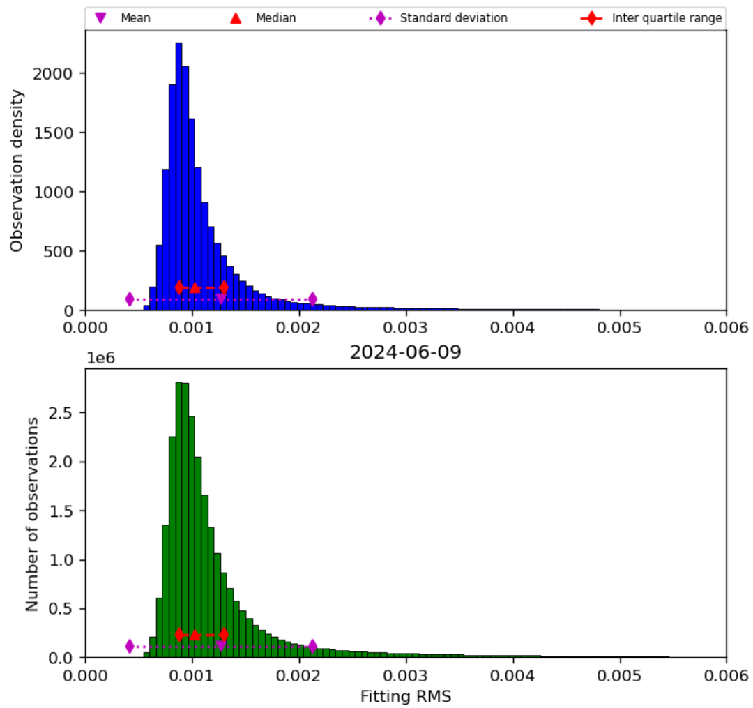
Figure 23: Histogram of “Fitting RMS” for 2024-06-08 to 2024-06-10
