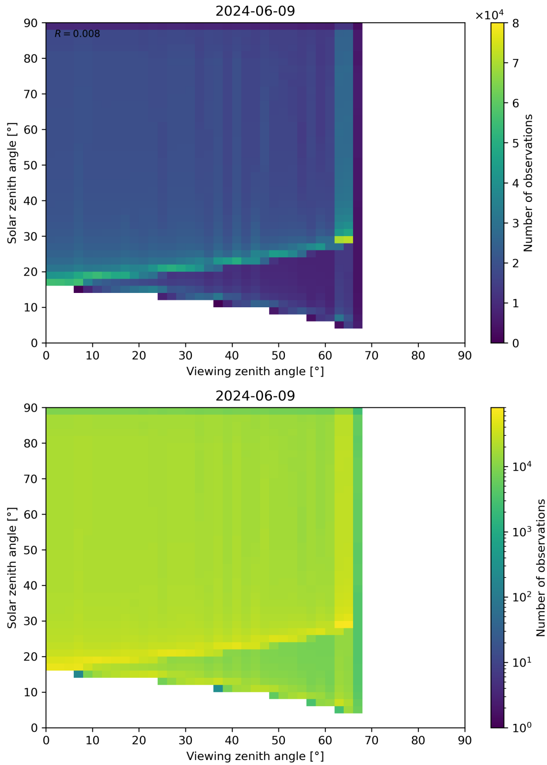
Figure 54: Scatter density plot of “Viewing zenith angle” against “Solar zenith angle” for 2024-06-08 to 2024-06-10.
