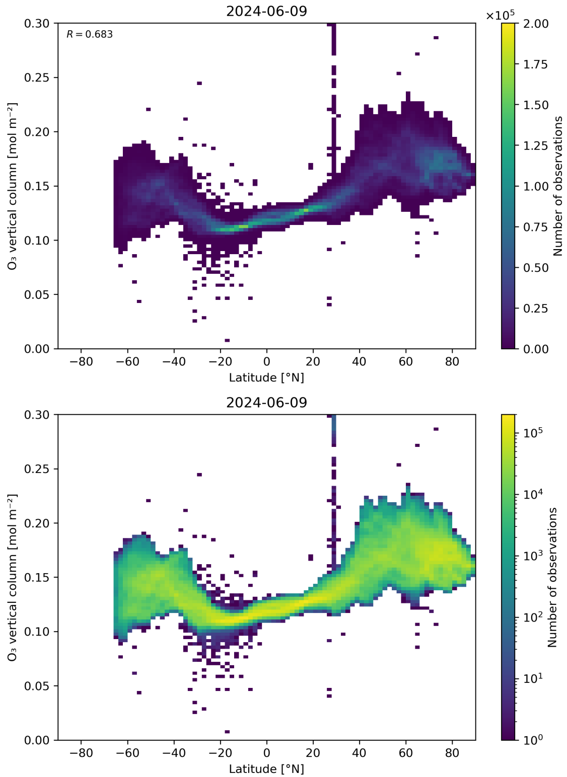
Figure 36: Scatter density plot of “Latitude” against “O 3 vertical column” for 2024-06-08 to 2024-06-10.
