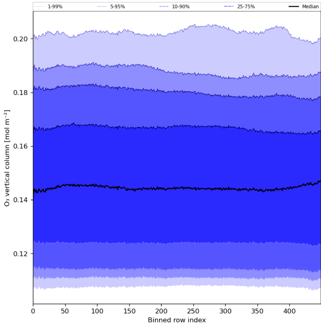
Figure 28: Along track statistics of "O 3 vertical column" for 2024-06-08 to 2024-06-10
