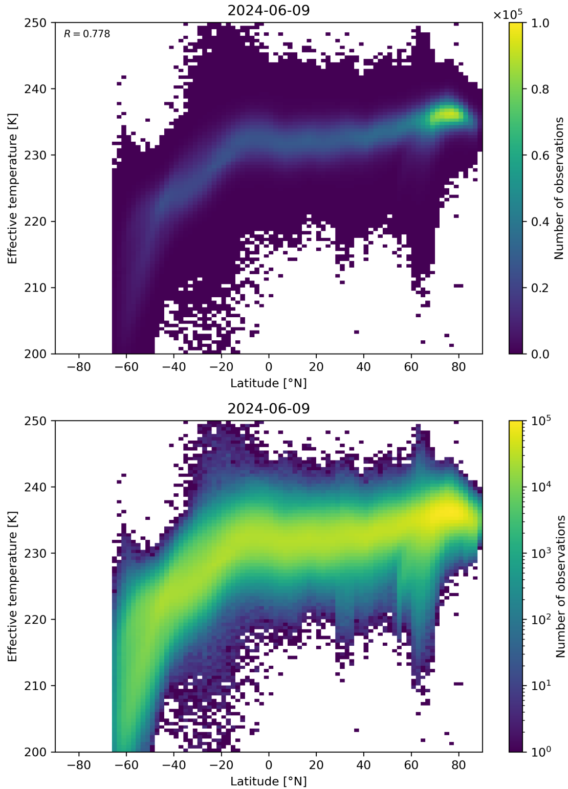
Figure 34: Scatter density plot of “Latitude” against “Effective temperature” for 2024-06-08 to 2024-06-10.
