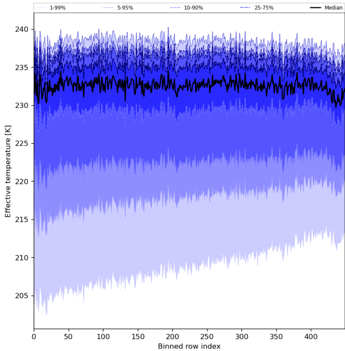
Figure 31: Along track statistics of “Effective temperature” for 2024-06-08 to 2024-06-10
