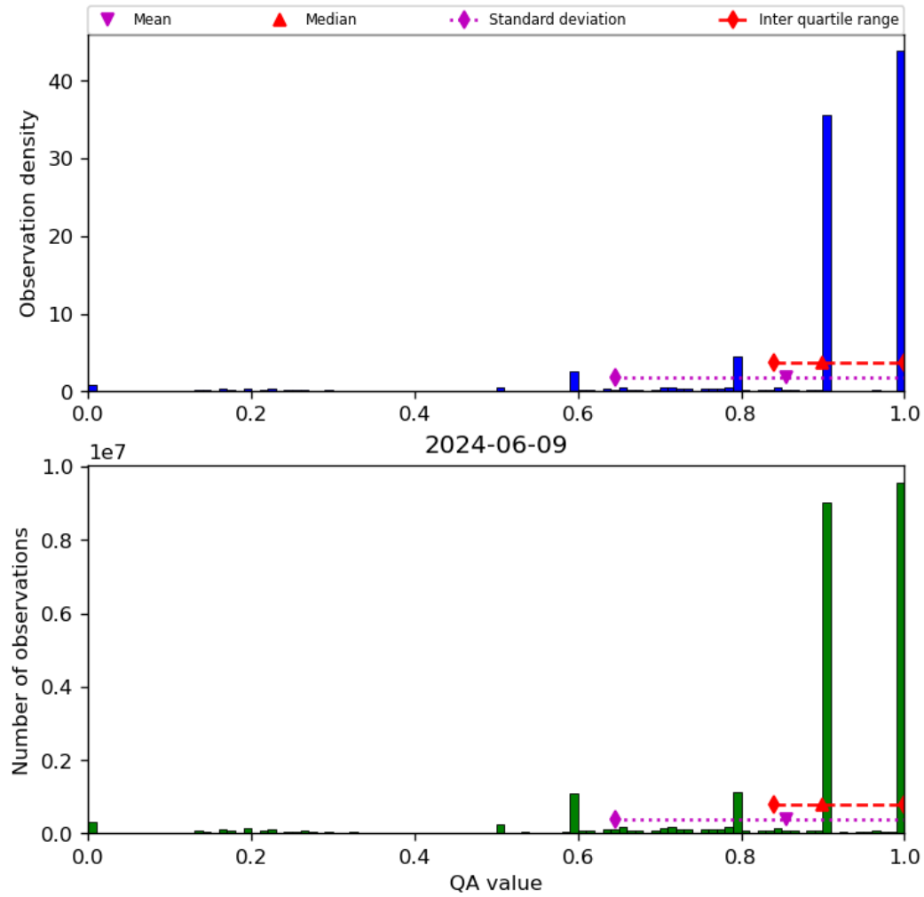
Figure 20: Histogram of “QA value” for 2024-06-08 to 2024-06-10
