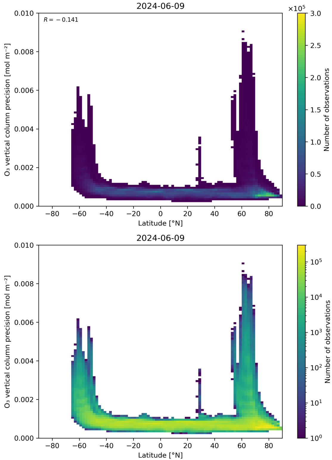
Figure 37: Scatter density plot of “Latitude” against “O 3 vertical column precision” for 2024-06-08 to 2024-06-10.
