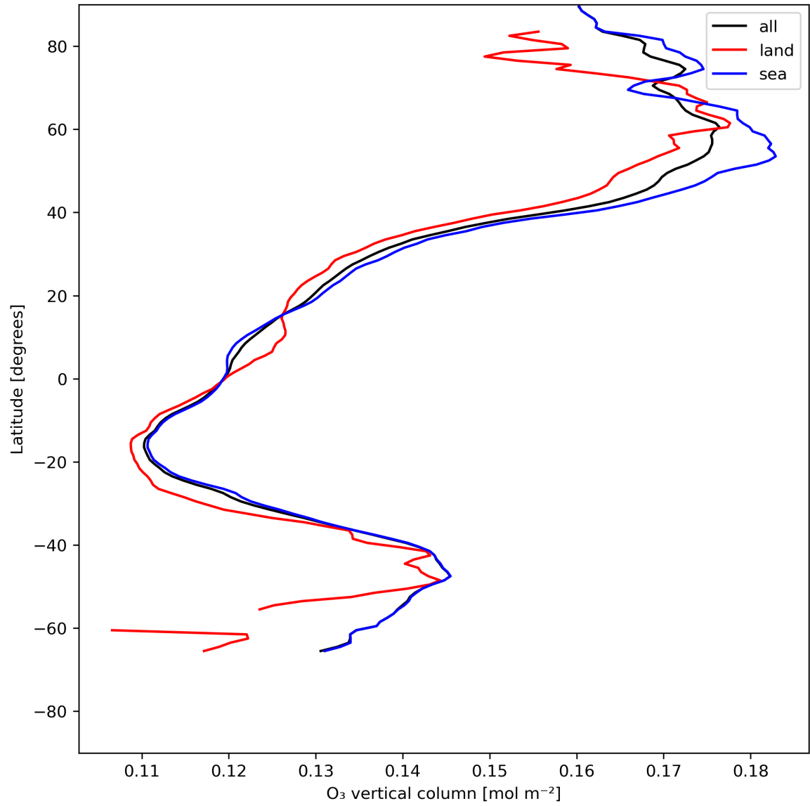
Figure 14: Zonal average of “O 3 vertical column” for 2024-06-08 to 2024-06-10.
