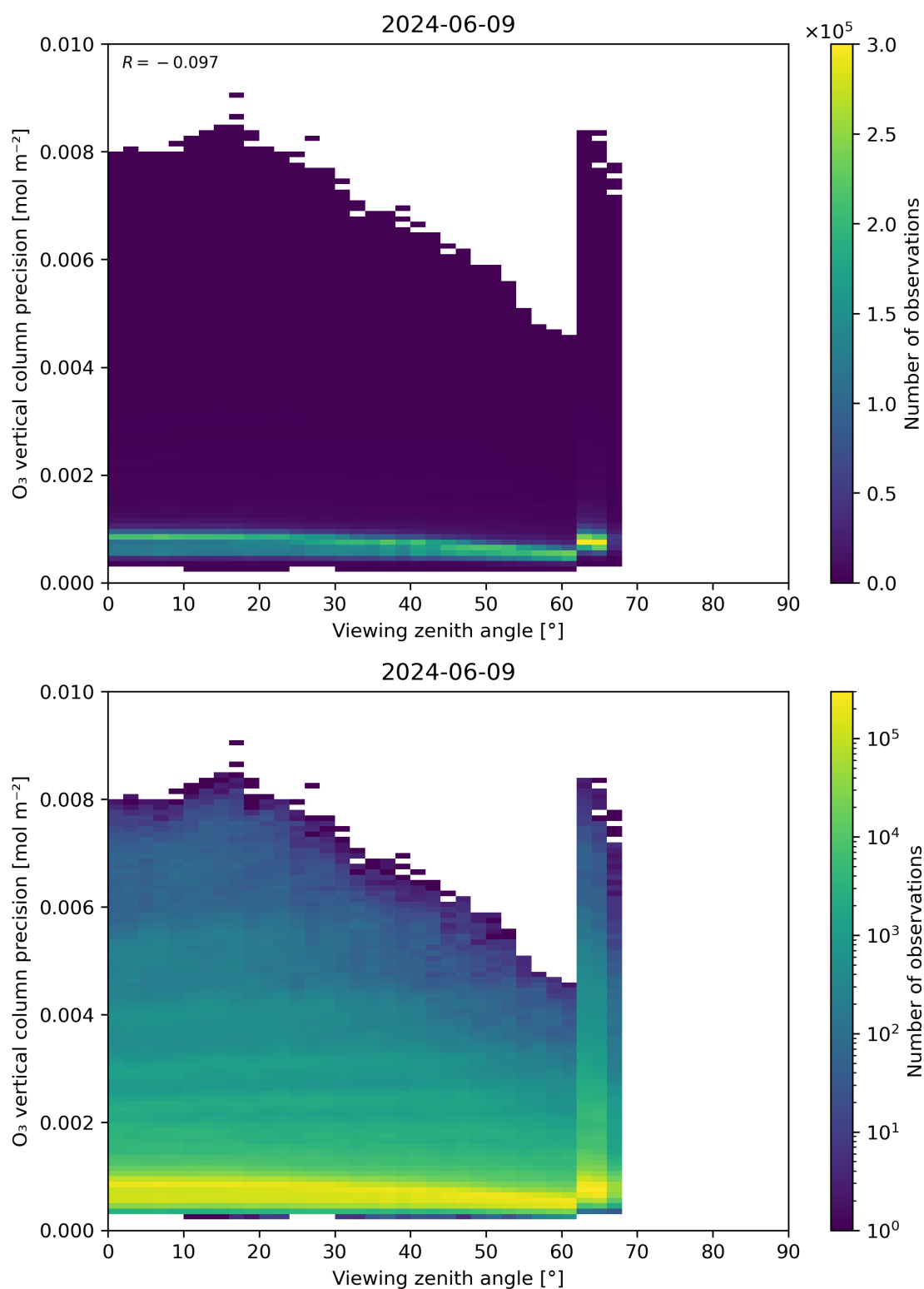
Figure 53: Scatter density plot of “Viewing zenith angle” against “O 3 vertical column precision” for 2024-06-08 to 2024-06-10.
