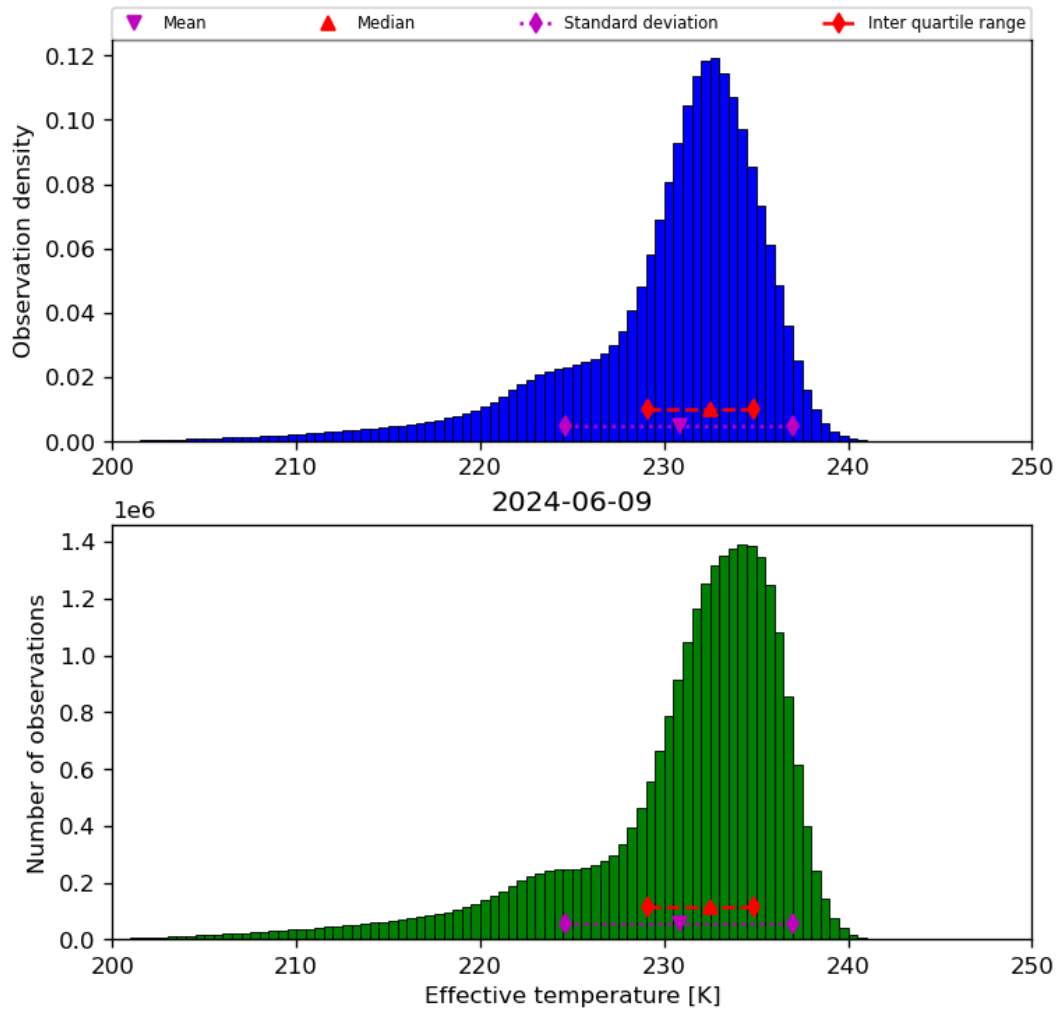
Figure 24: Histogram of “Effective temperature” for 2024-06-08 to 2024-06-10
