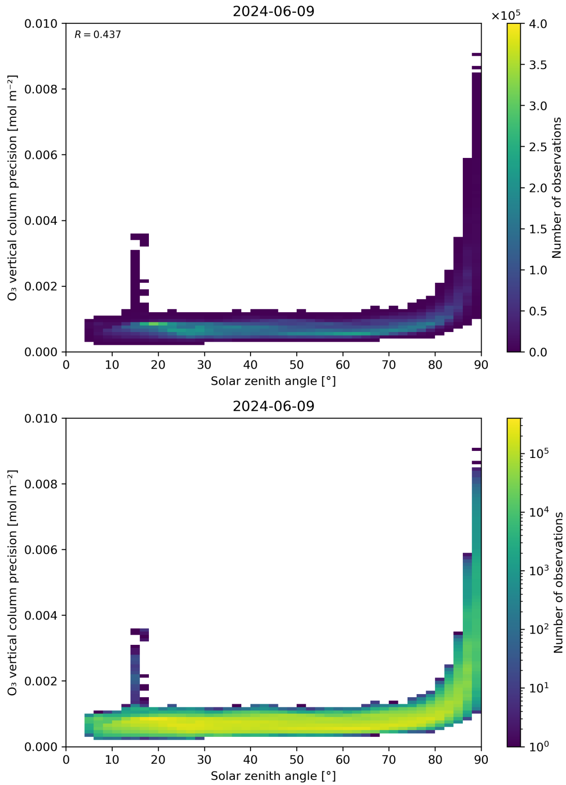
Figure 48: Scatter density plot of “Solar zenith angle” against “O 3 vertical column precision” for 2024-06-08 to 2024-06-10.
