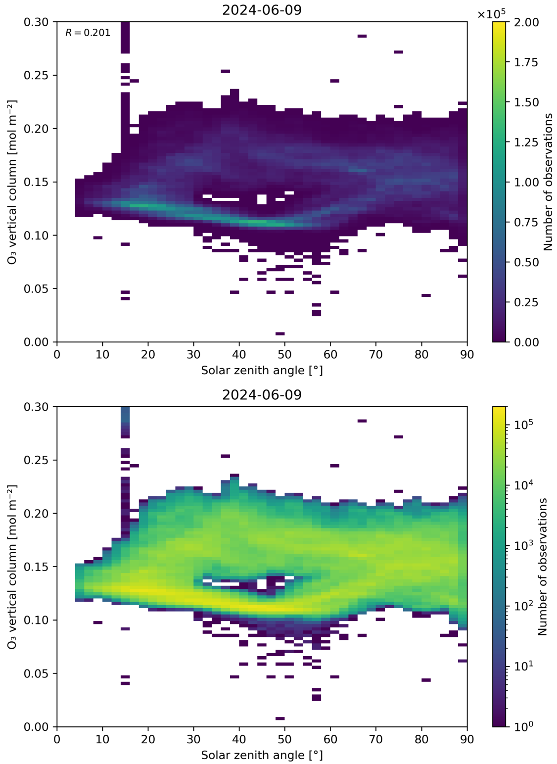
Figure 47: Scatter density plot of “Solar zenith angle” against “O 3 vertical column” for 2024-06-08 to 2024-06-10.
