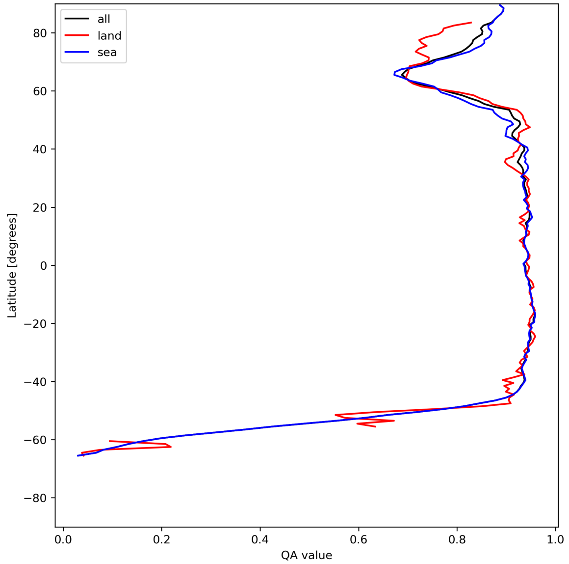
Figure 13: Zonal average of “QA value” for 2024-06-08 to 2024-06-10.
