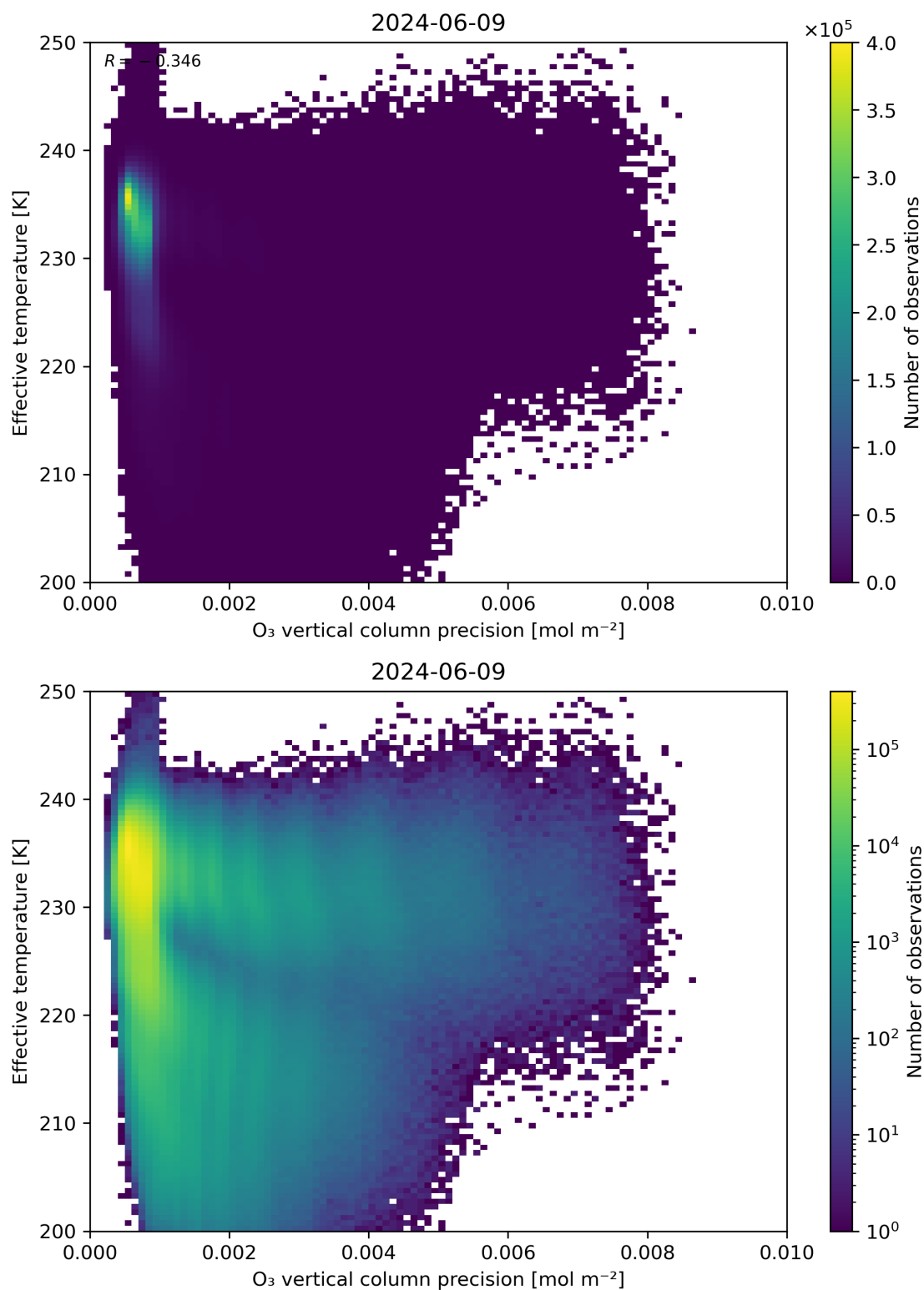
Figure 42: Scatter density plot of “O 3 vertical column precision” against “Effective temperature” for 2024-06-08 to 2024-06-10.
