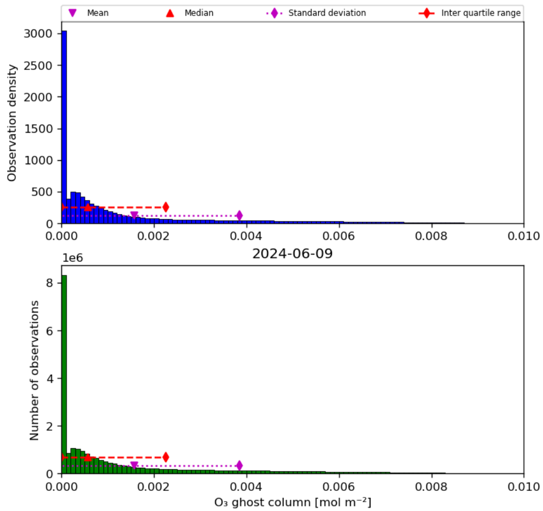
Figure 25: Histogram of “O 3 ghost column” for 2024-06-08 to 2024-06-10
