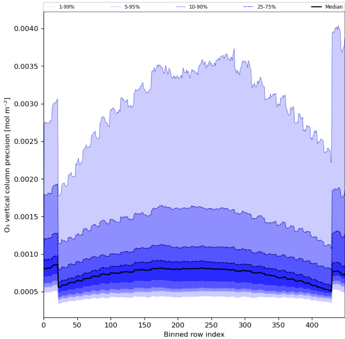
Figure 29: Along track statistics of “O 3 vertical column precision” for 2024-06-08 to 2024-06-10
