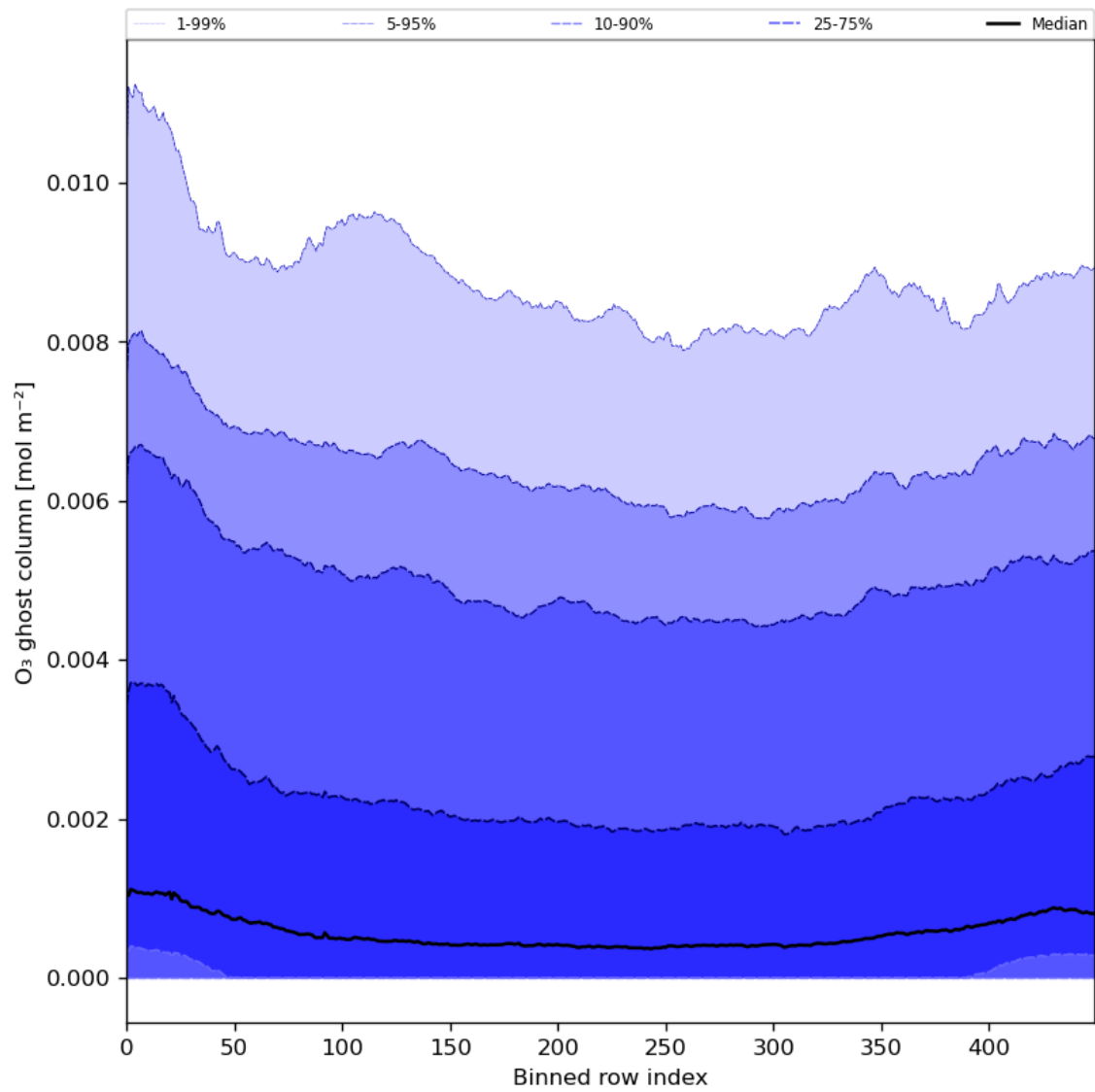
Figure 32: Along track statistics of “O 3 ghost column” for 2024-06-08 to 2024-06-10
