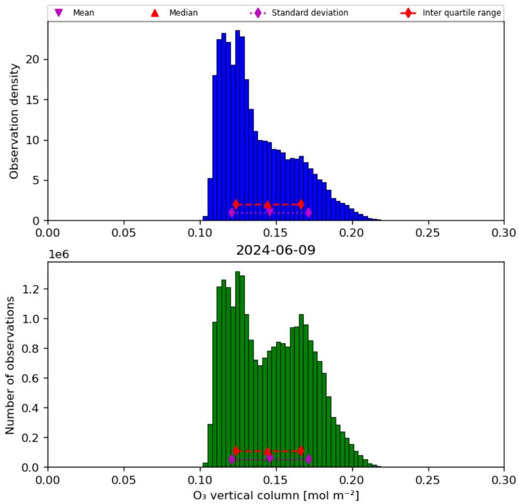
Figure 21: Histogram of “O 3 vertical column” for 2024-06-08 to 2024-06-10
