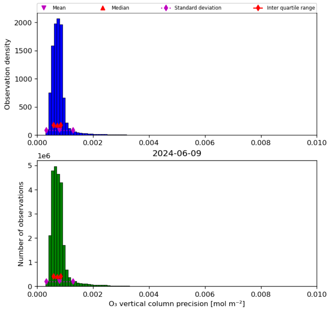
Figure 22: Histogram of “O 3 vertical column precision” for 2024-06-08 to 2024-06-10
