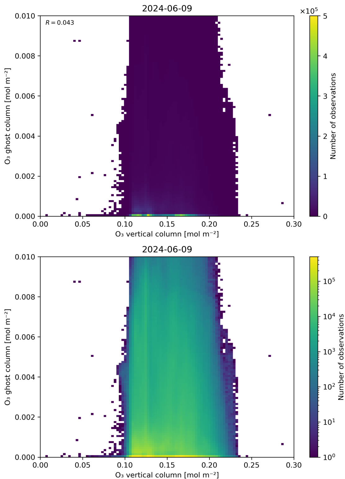
Figure 40: Scatter density plot of “O 3 vertical column” against “O 3 ghost column” for 2024-06-08 to 2024-06-10.
