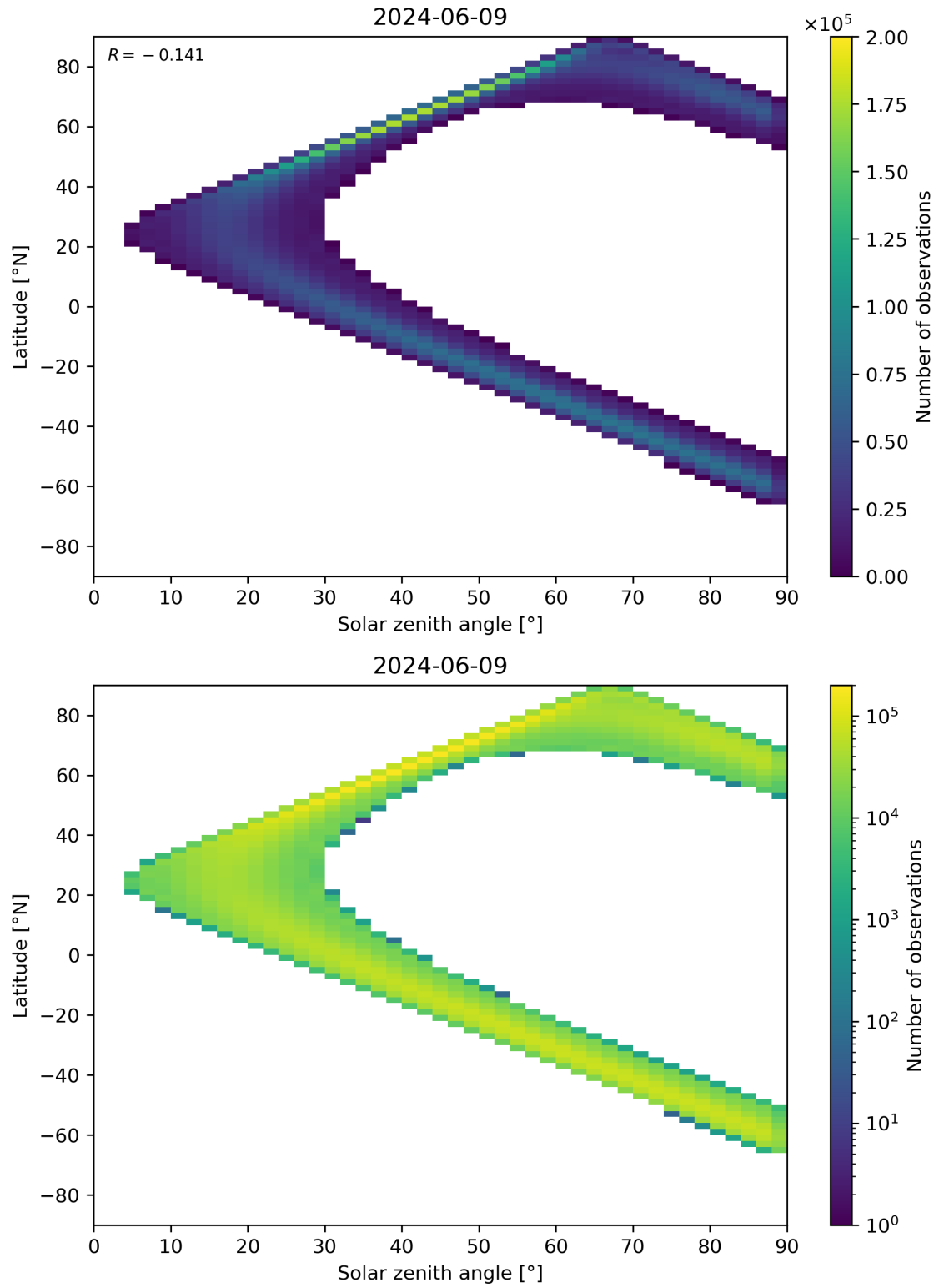
Figure 44: Scatter density plot of “Solar zenith angle” against “Latitude” for 2024-06-08 to 2024-06-10.
