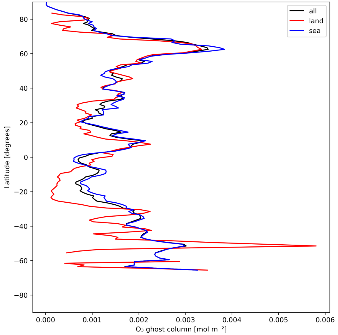
Figure 18: Zonal average of "O 3 ghost column" for 2024-06-08 to 2024-06-10.
