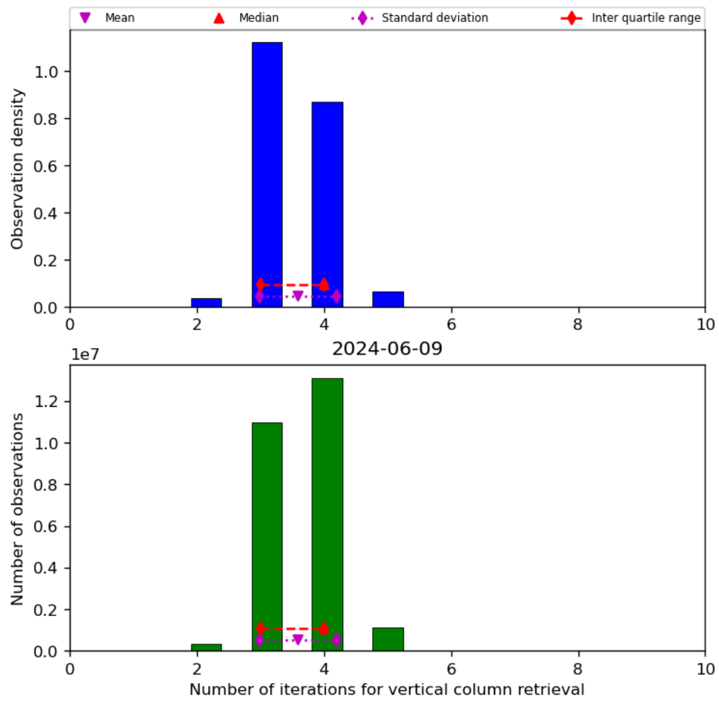
Figure 26: Histogram of “Number of iterations for vertical column retrieval” for 2024-06-08 to 2024-06-10
