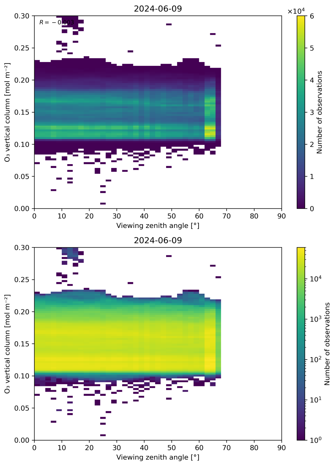
Figure 52: Scatter density plot of “Viewing zenith angle” against “O 3 vertical column” for 2024-06-08 to 2024-06-10.
