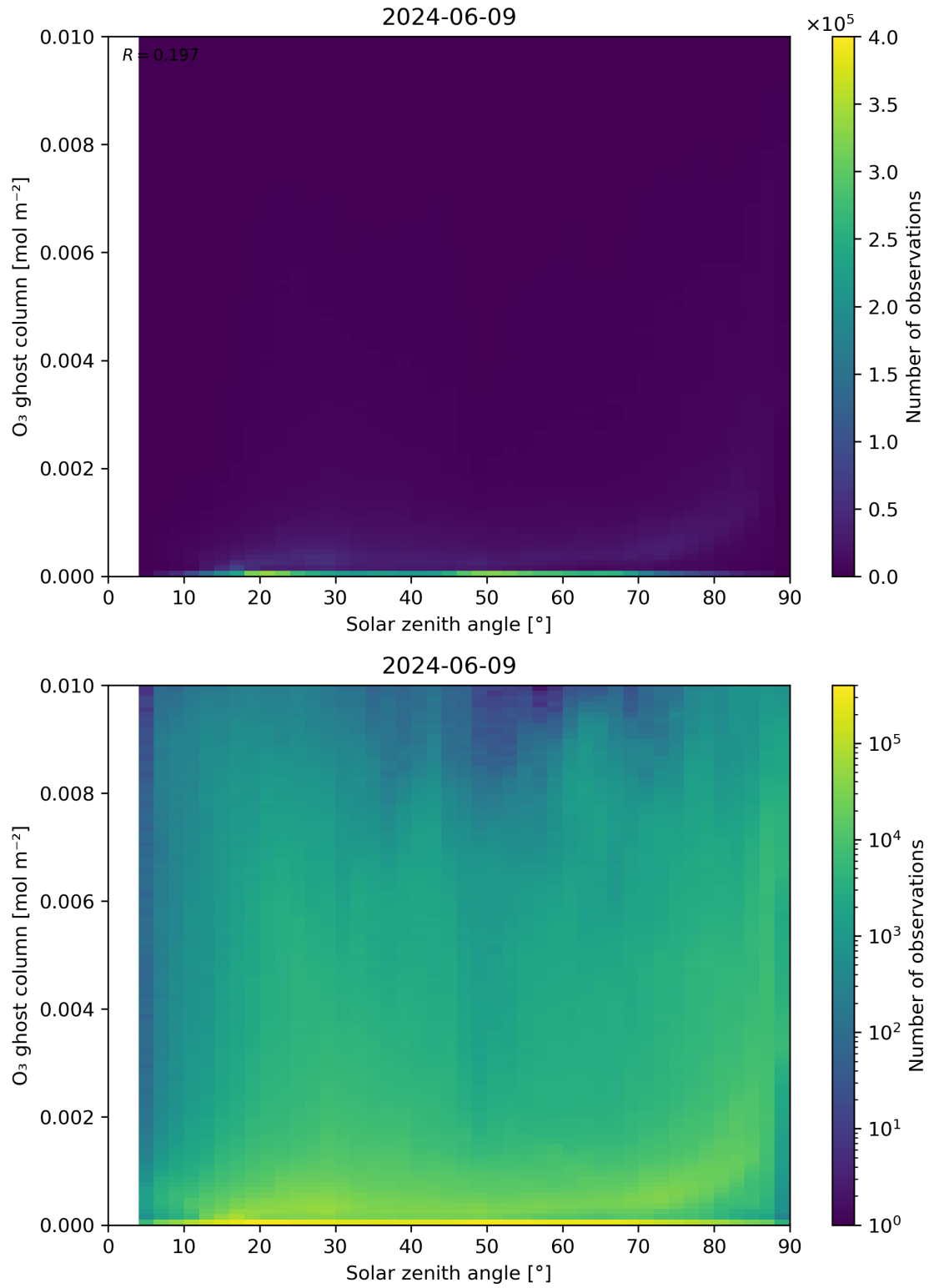
Figure 46: Scatter density plot of “Solar zenith angle” against “O 3 ghost column” for 2024-06-08 to 2024-06-10.
