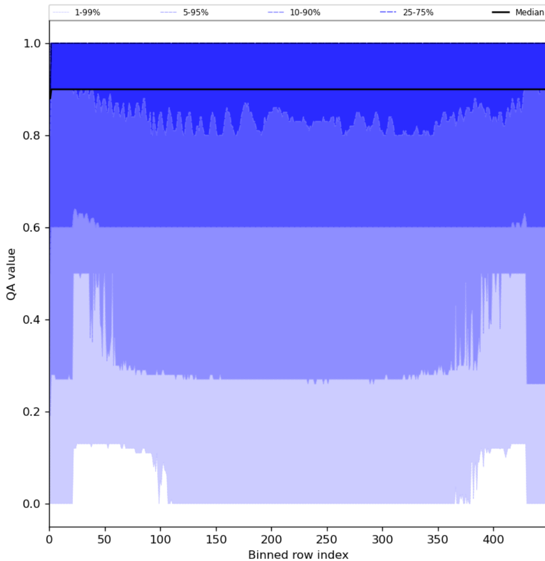
Figure 27: Along track statistics of “QA value” for 2024-06-08 to 2024-06-10
