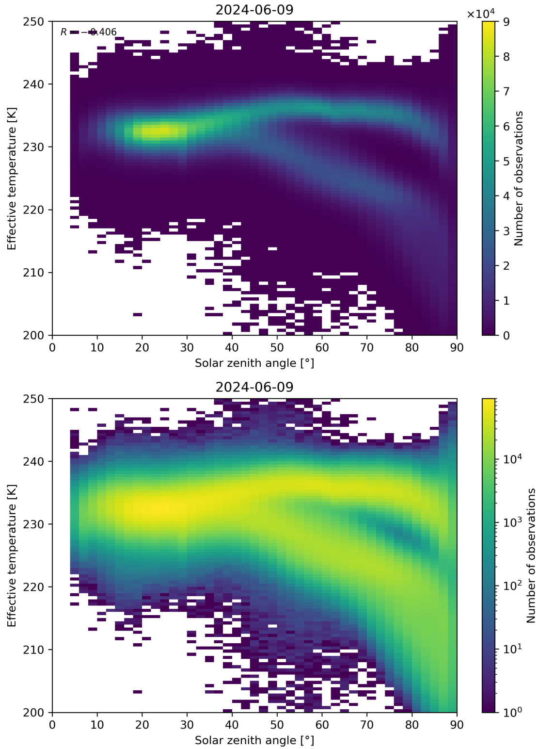
Figure 45: Scatter density plot of “Solar zenith angle” against “Effective temperature” for 2024-06-08 to 2024-06-10.
