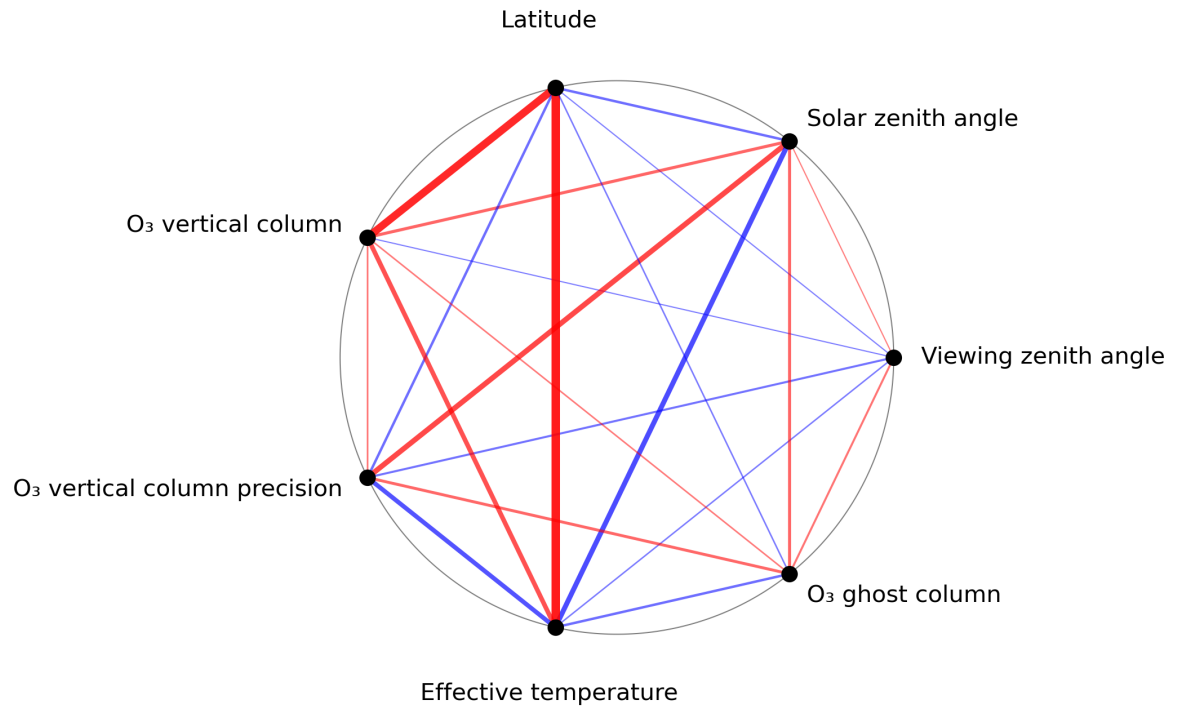
Figure 1: Map of correlation graph for 2024-06-08 to 2024-06-10.
