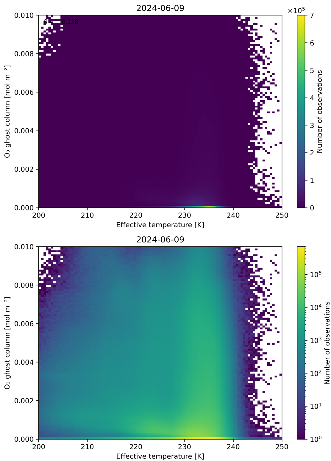
Figure 38: Scatter density plot of “Effective temperature” against “O 3 ghost column” for 2024-06-08 to 2024-06-10.
