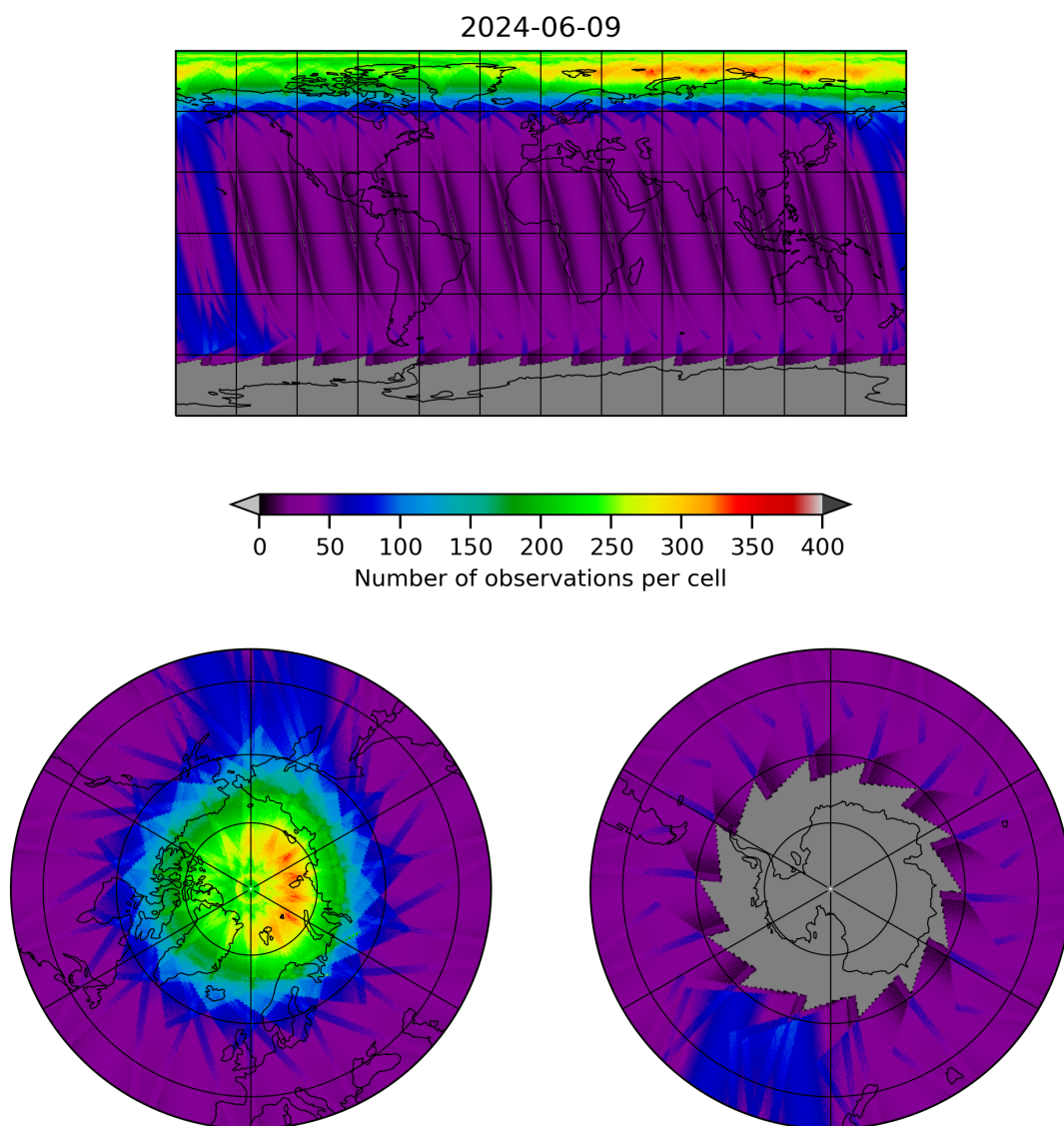
Figure 12: Map of the number of observations for 2024-06-08 to 2024-06-10
