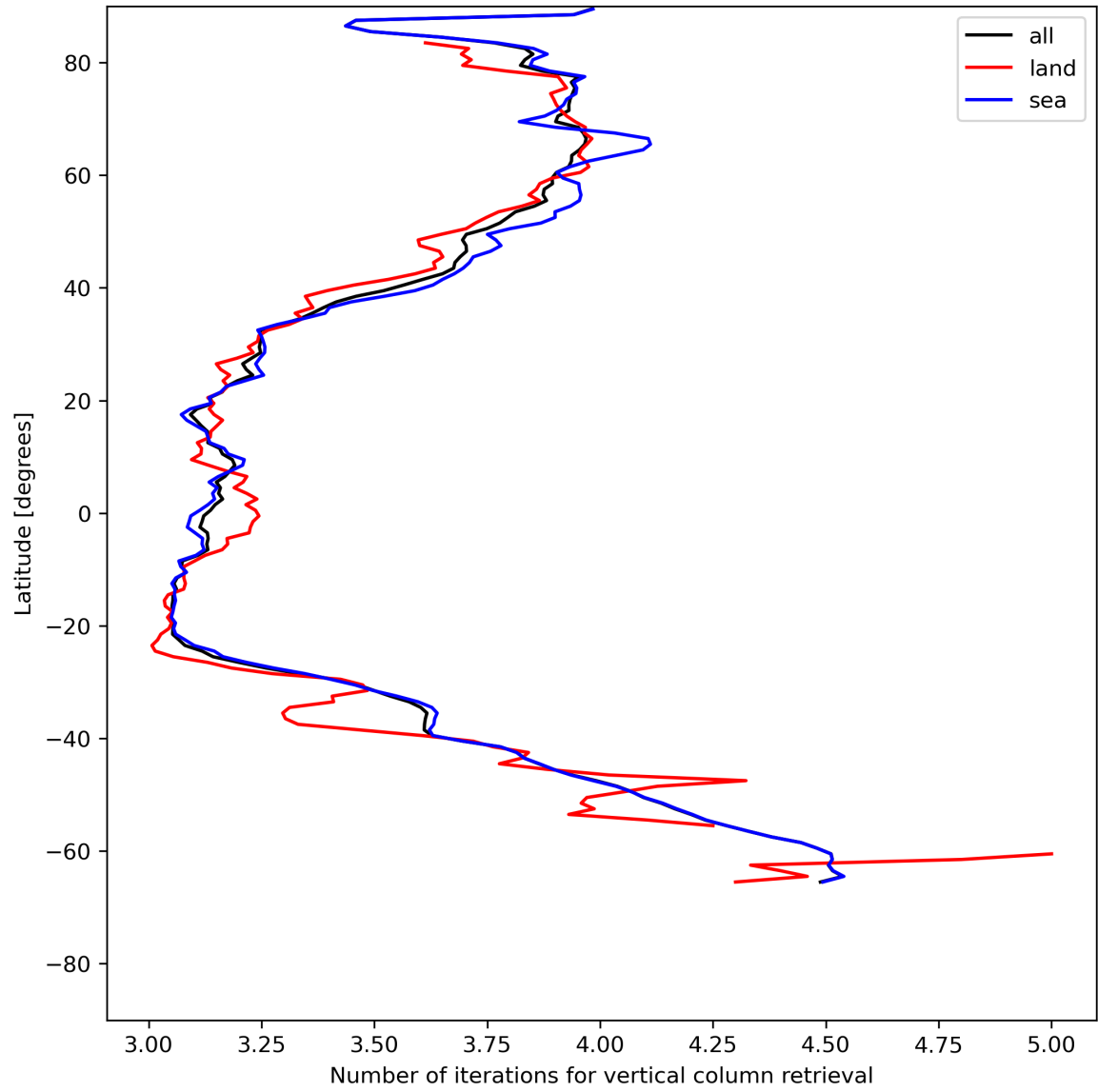
Figure 19: Zonal average of “Number of iterations for vertical column retrieval” for 2024-06-08 to 2024-06-10.
