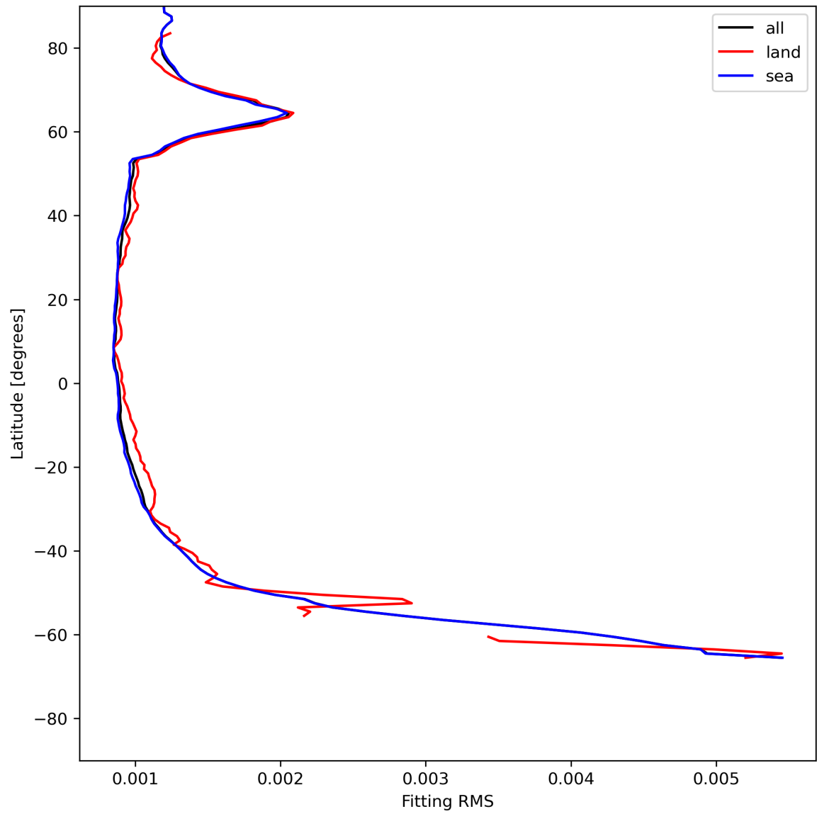
Figure 16: Zonal average of “Fitting RMS” for 2024-06-08 to 2024-06-10.
