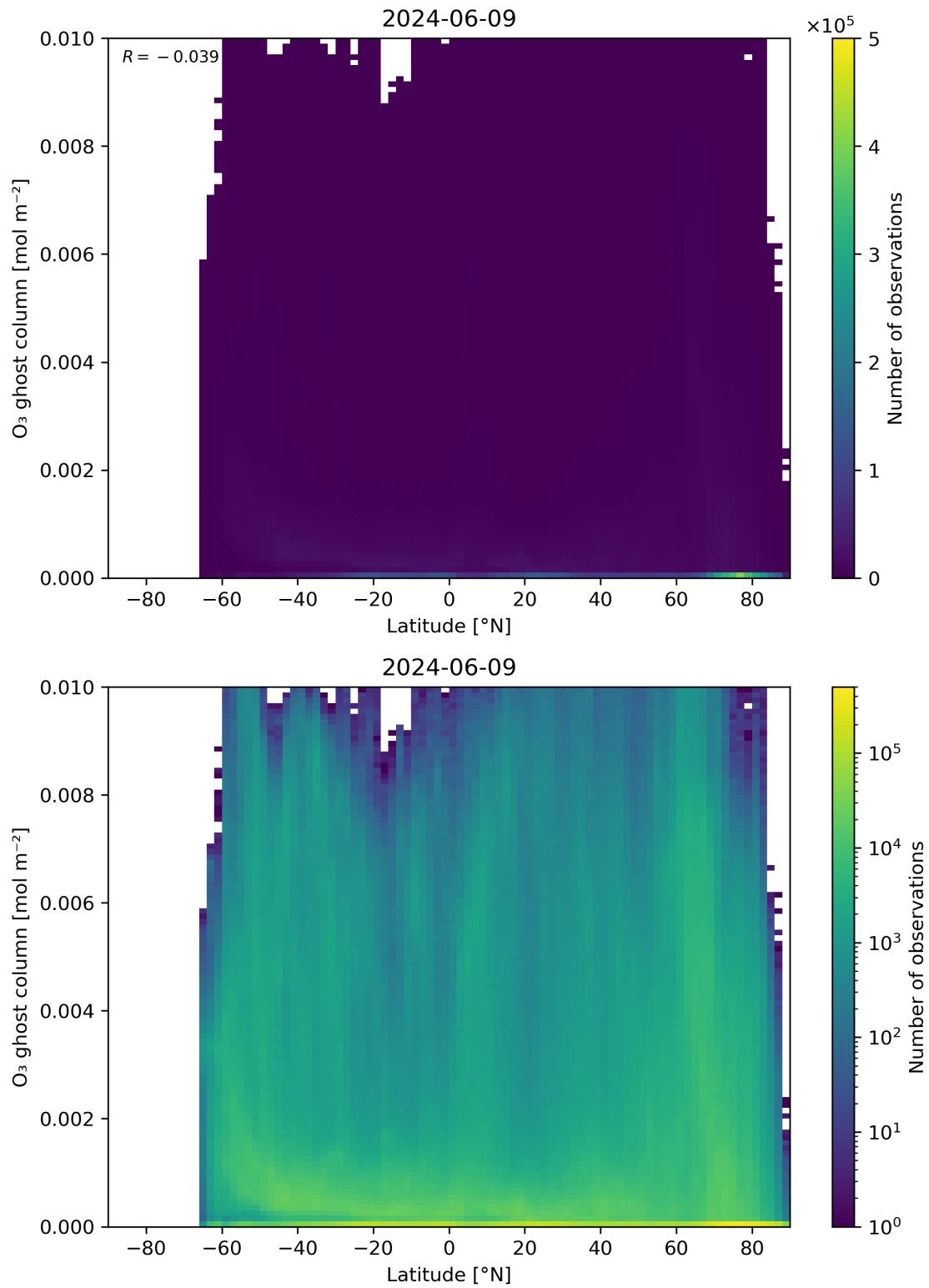
Figure 35: Scatter density plot of “Latitude” against “O 3 ghost column” for 2024-06-08 to 2024-06-10.
