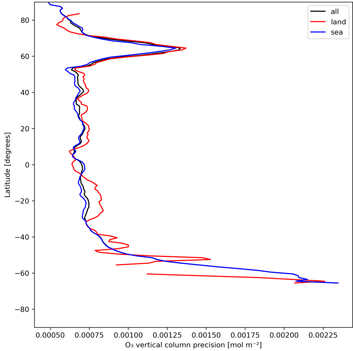
Figure 15: Zonal average of “O 3 vertical column precision” for 2024-06-08 to 2024-06-10.
