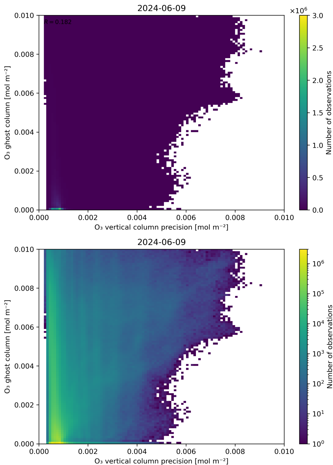
Figure 43: Scatter density plot of “ \text{O}_3 vertical column precision” against “ \text{O}_3 ghost column” for 2024-06-08 to 2024-06-10.
