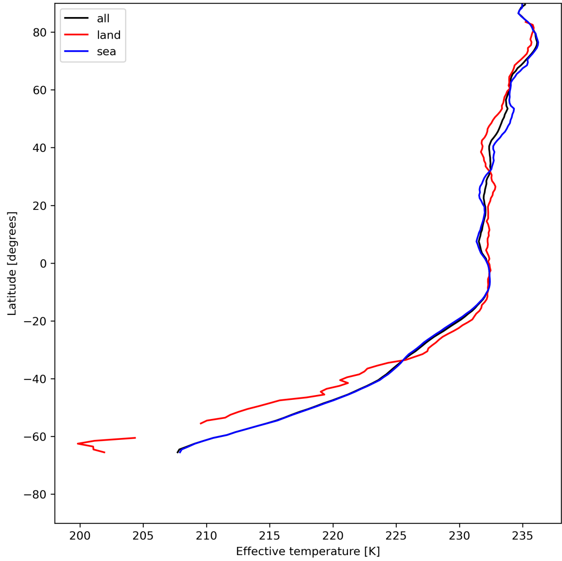
Figure 17: Zonal average of "Effective temperature" for 2024-06-08 to 2024-06-10.
