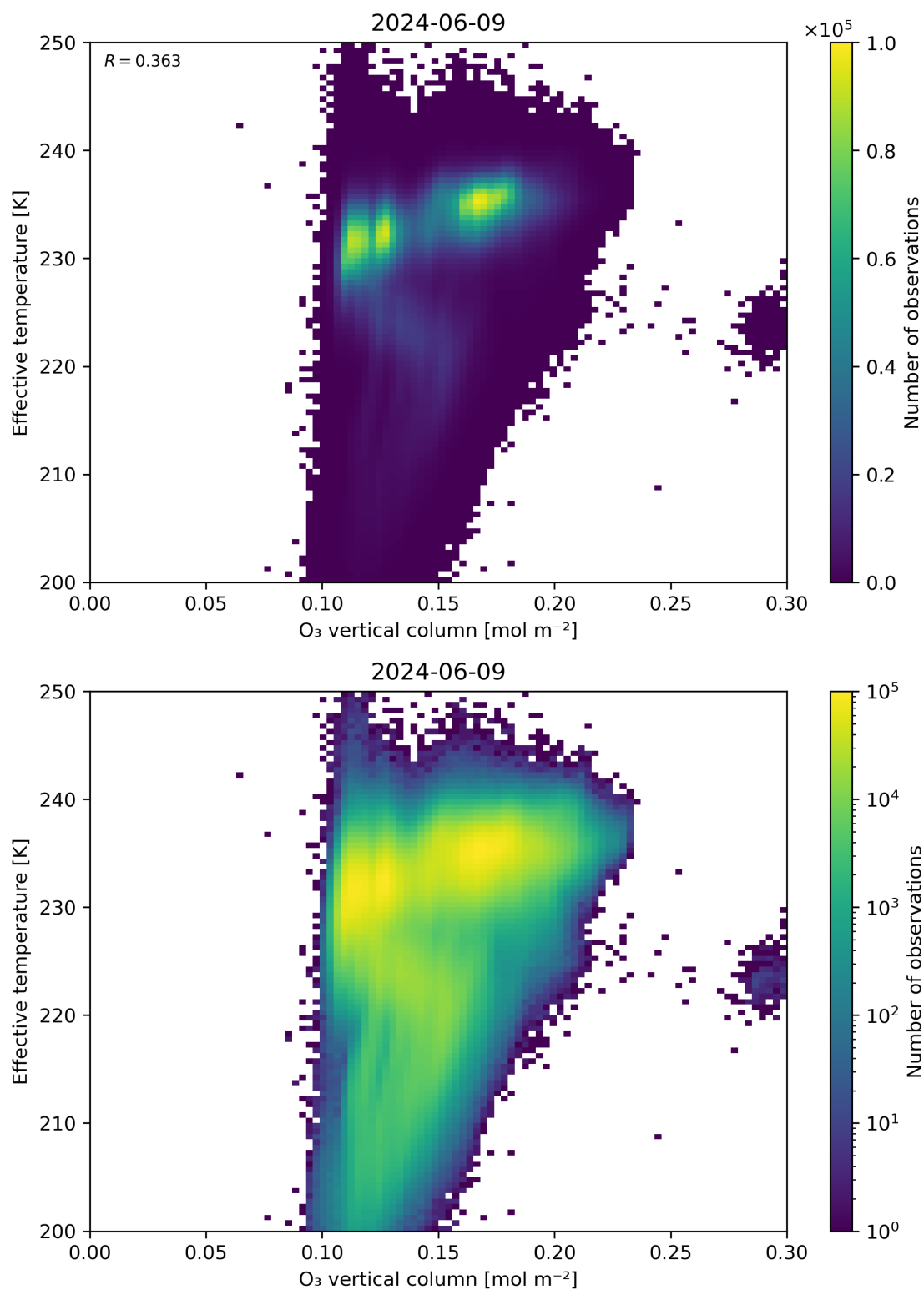
Figure 39: Scatter density plot of “O 3 vertical column” against “Effective temperature” for 2024-06-08 to 2024-06-10.
