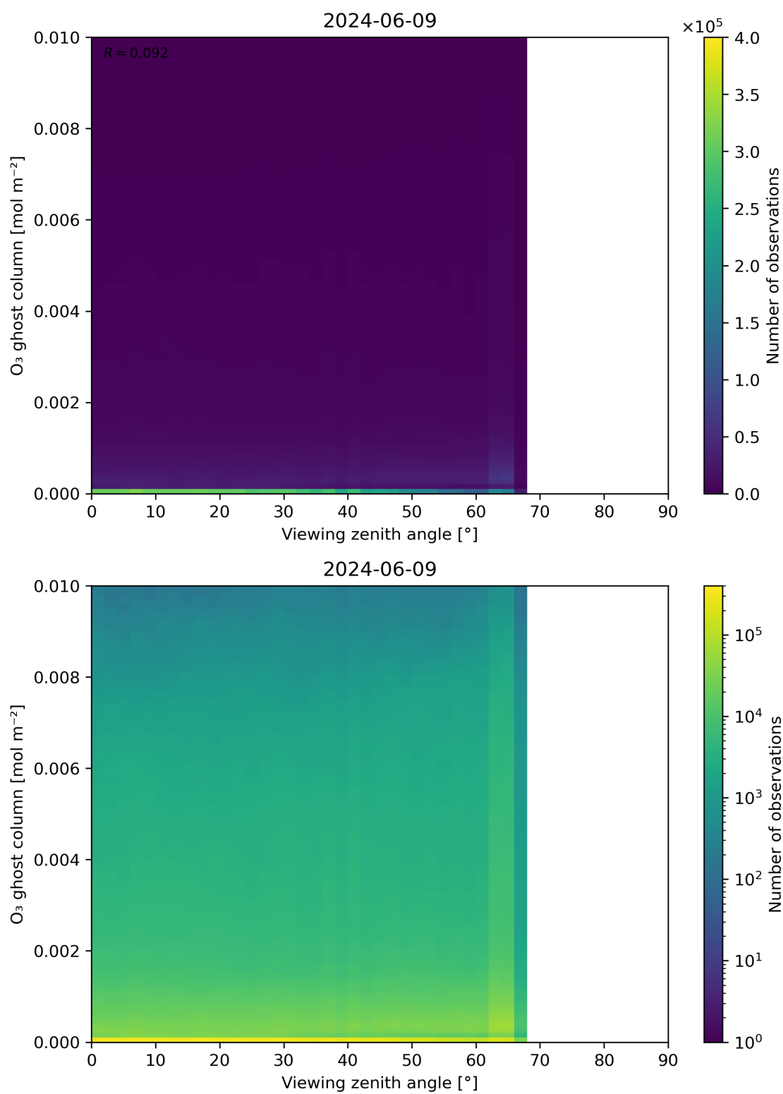
Figure 51: Scatter density plot of “Viewing zenith angle” against “O 3 ghost column” for 2024-06-08 to 2024-06-10.
