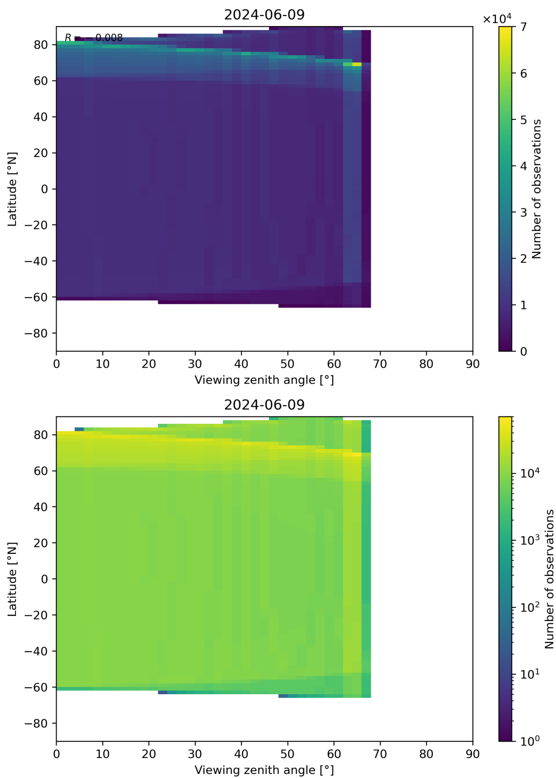
Figure 49: Scatter density plot of “Viewing zenith angle” against “Latitude” for 2024-06-08 to 2024-06-10.
