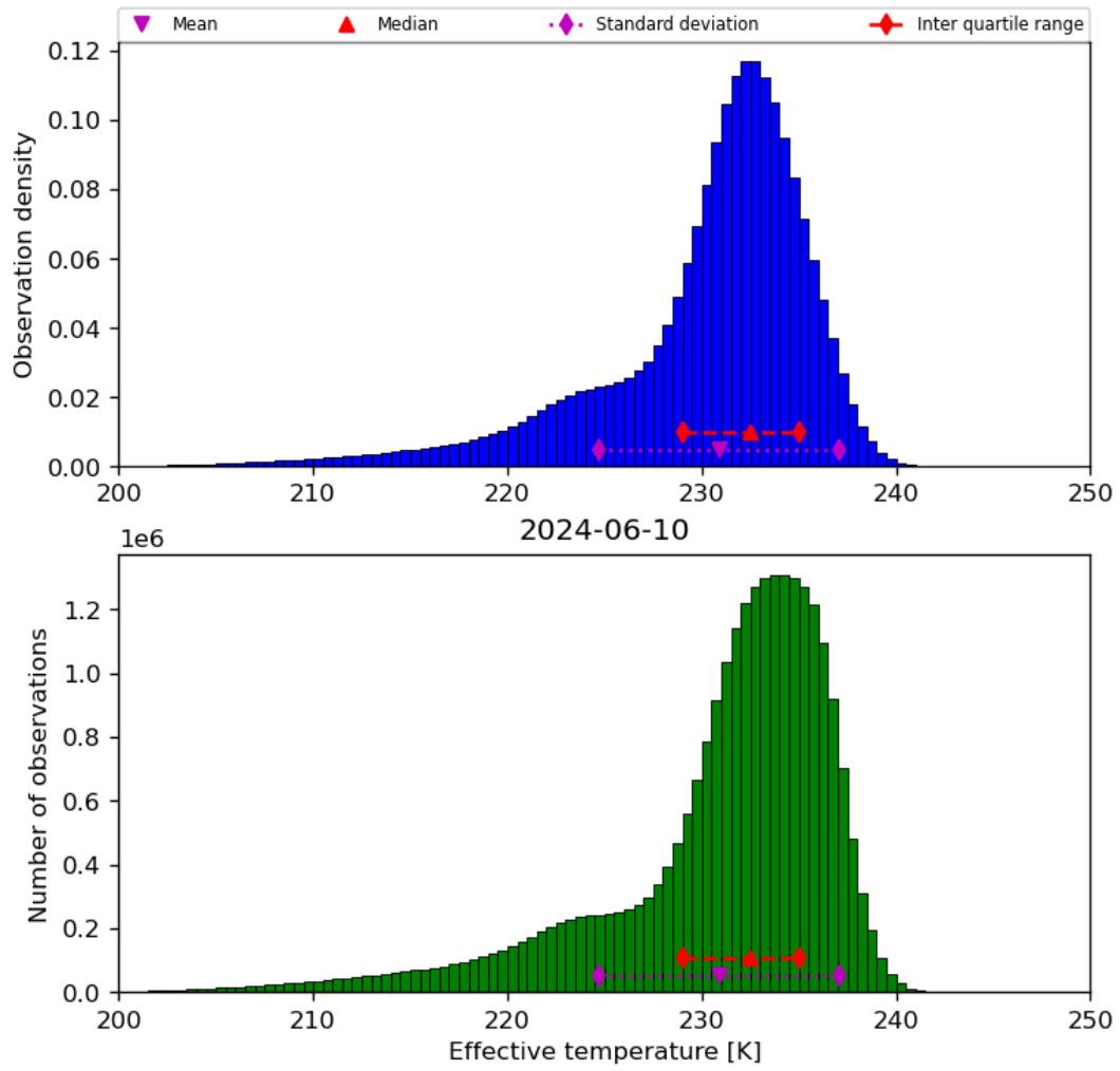
Figure 24: Histogram of “Effective temperature” for 2024-06-09 to 2024-06-11
