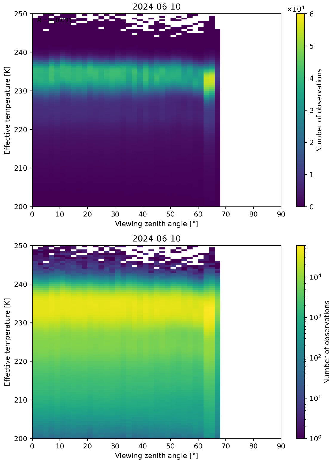
Figure 50: Scatter density plot of “Viewing zenith angle” against “Effective temperature” for 2024-06-09 to 2024-06-11.
