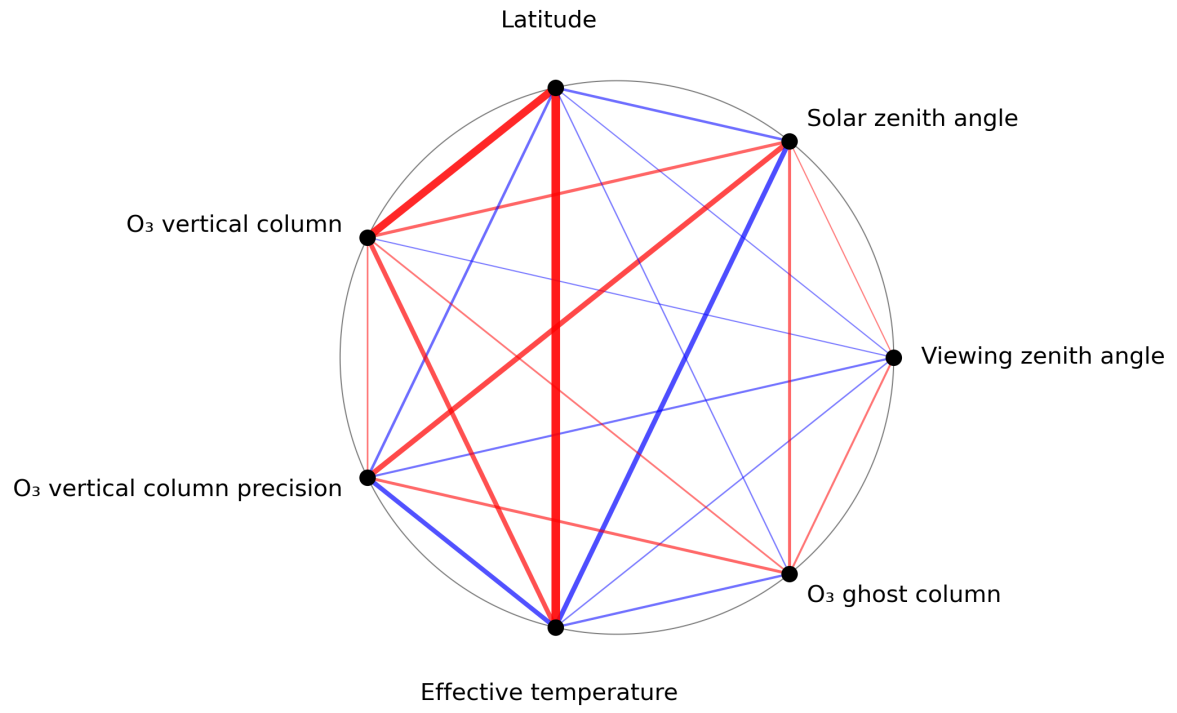
Figure 1: Map of correlation graph for 2024-06-09 to 2024-06-11.
