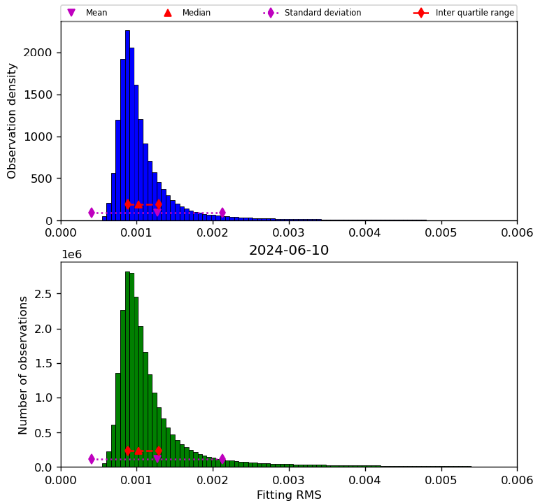
Figure 23: Histogram of “Fitting RMS” for 2024-06-09 to 2024-06-11
