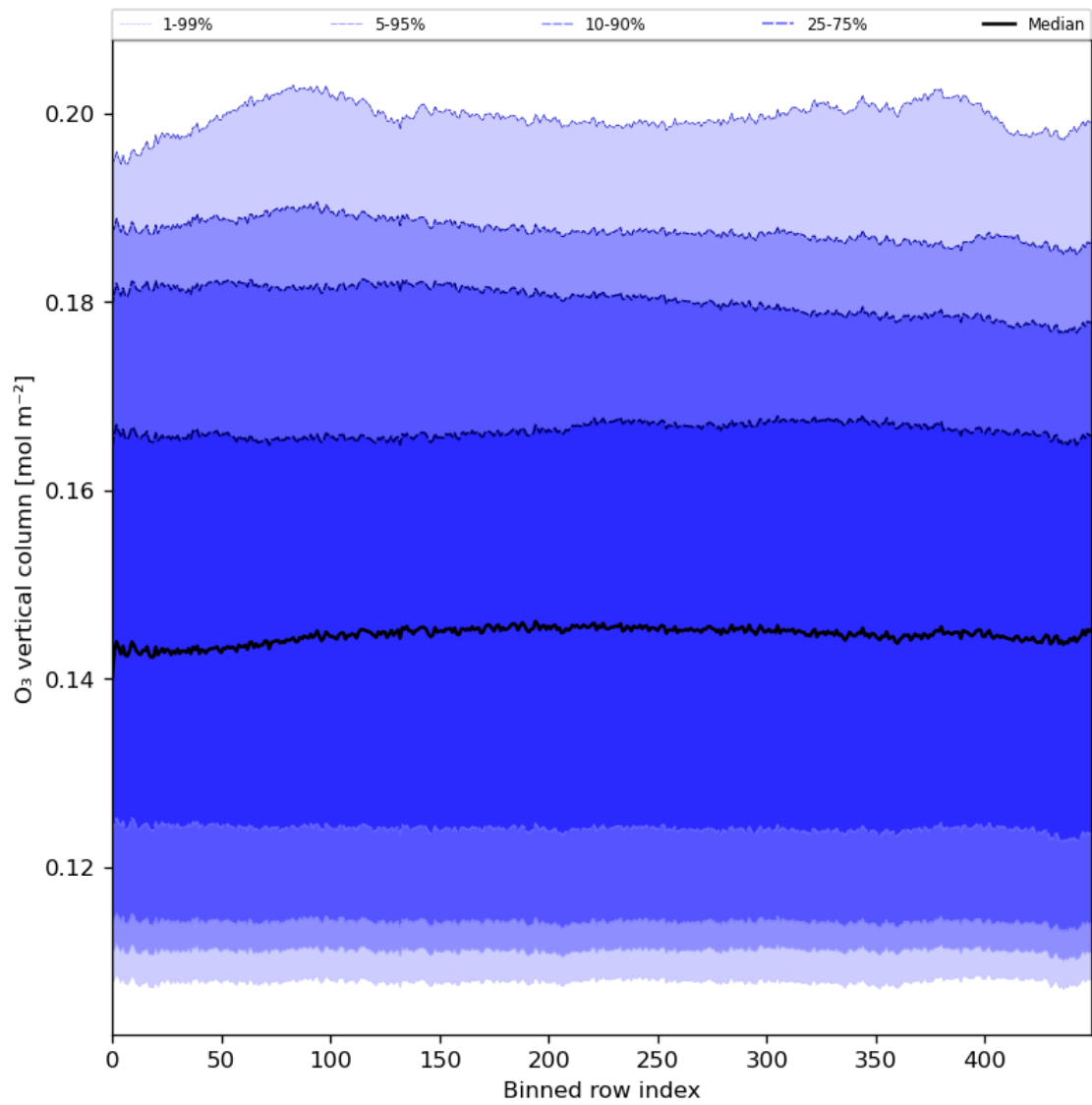
Figure 28: Along track statistics of “O 3 vertical column” for 2024-06-09 to 2024-06-11
