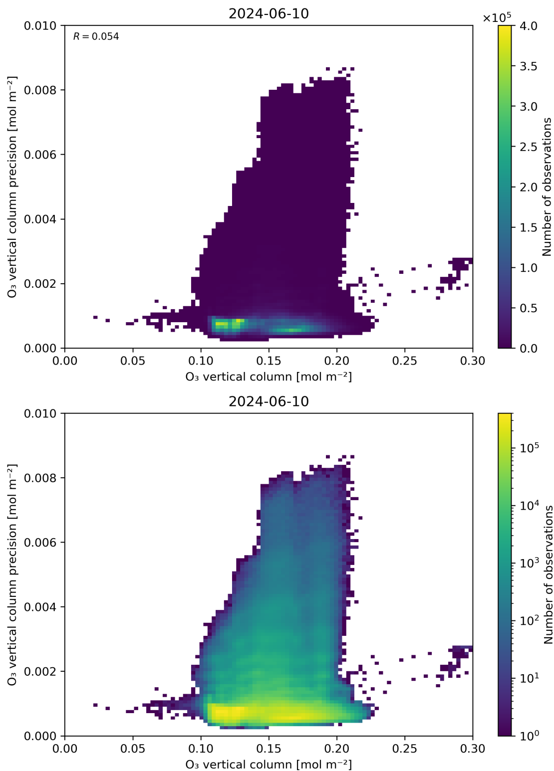
Figure 41: Scatter density plot of “O 3 vertical column” against “O 3 vertical column precision” for 2024-06-09 to 2024-06-11.
