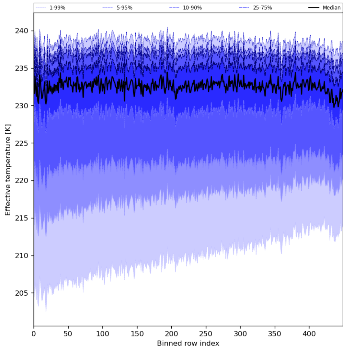
Figure 31: Along track statistics of “Effective temperature” for 2024-06-09 to 2024-06-11
