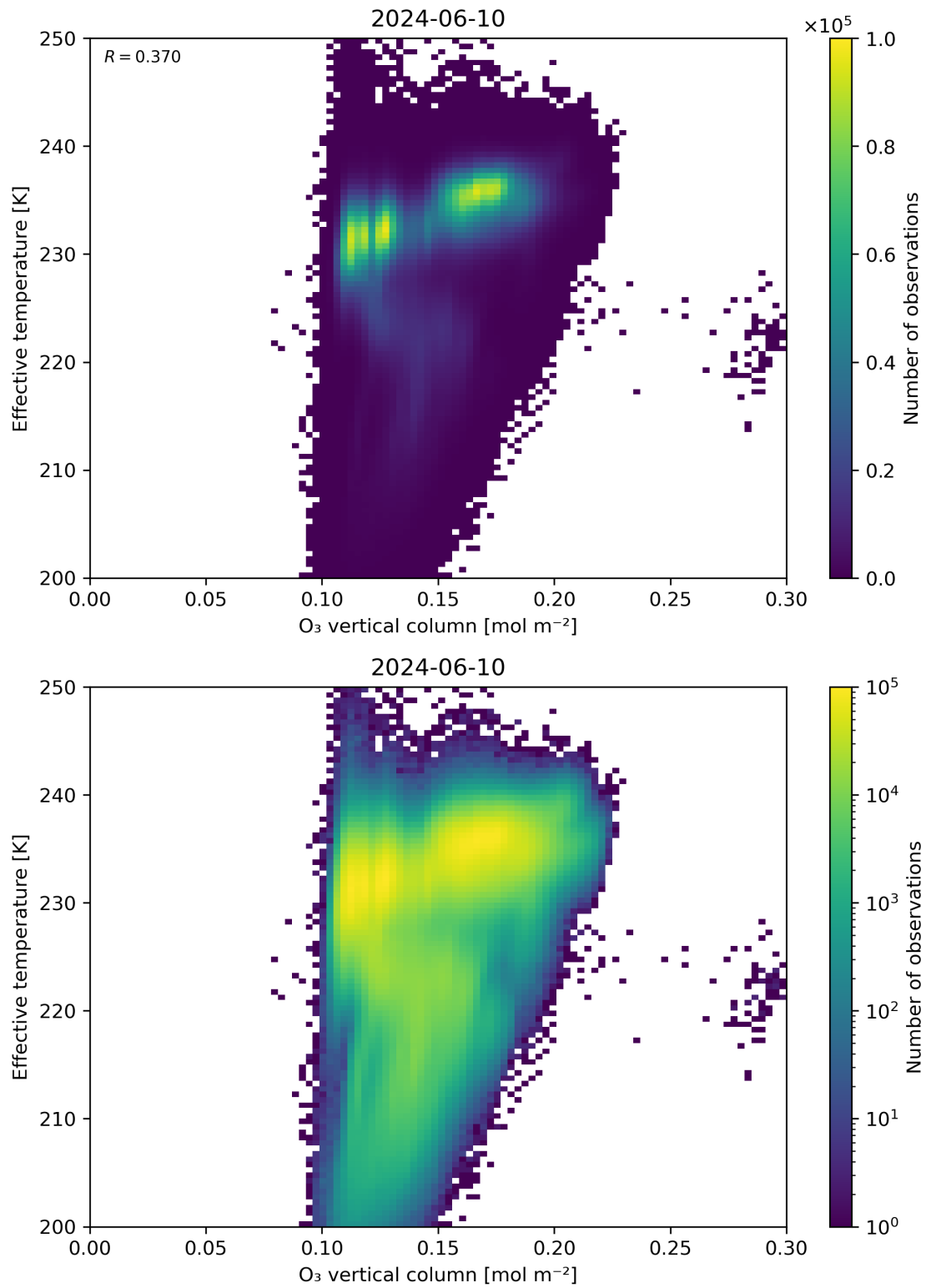
Figure 39: Scatter density plot of “O 3 vertical column” against “Effective temperature” for 2024-06-09 to 2024-06-11.
