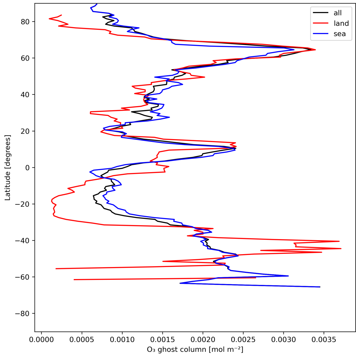
Figure 18: Zonal average of “O 3 ghost column” for 2024-06-09 to 2024-06-11.
