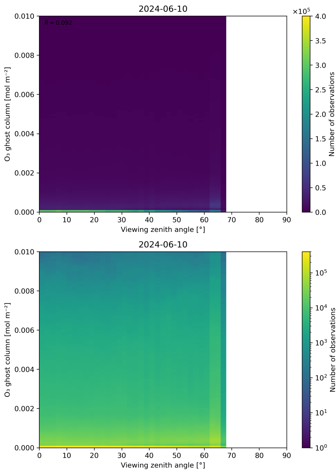
Figure 51: Scatter density plot of “Viewing zenith angle” against “O 3 ghost column” for 2024-06-09 to 2024-06-11.
