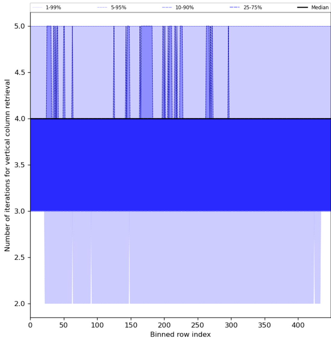
Figure 33: Along track statistics of “Number of iterations for vertical column retrieval” for 2024-06-09 to 2024-06-11
