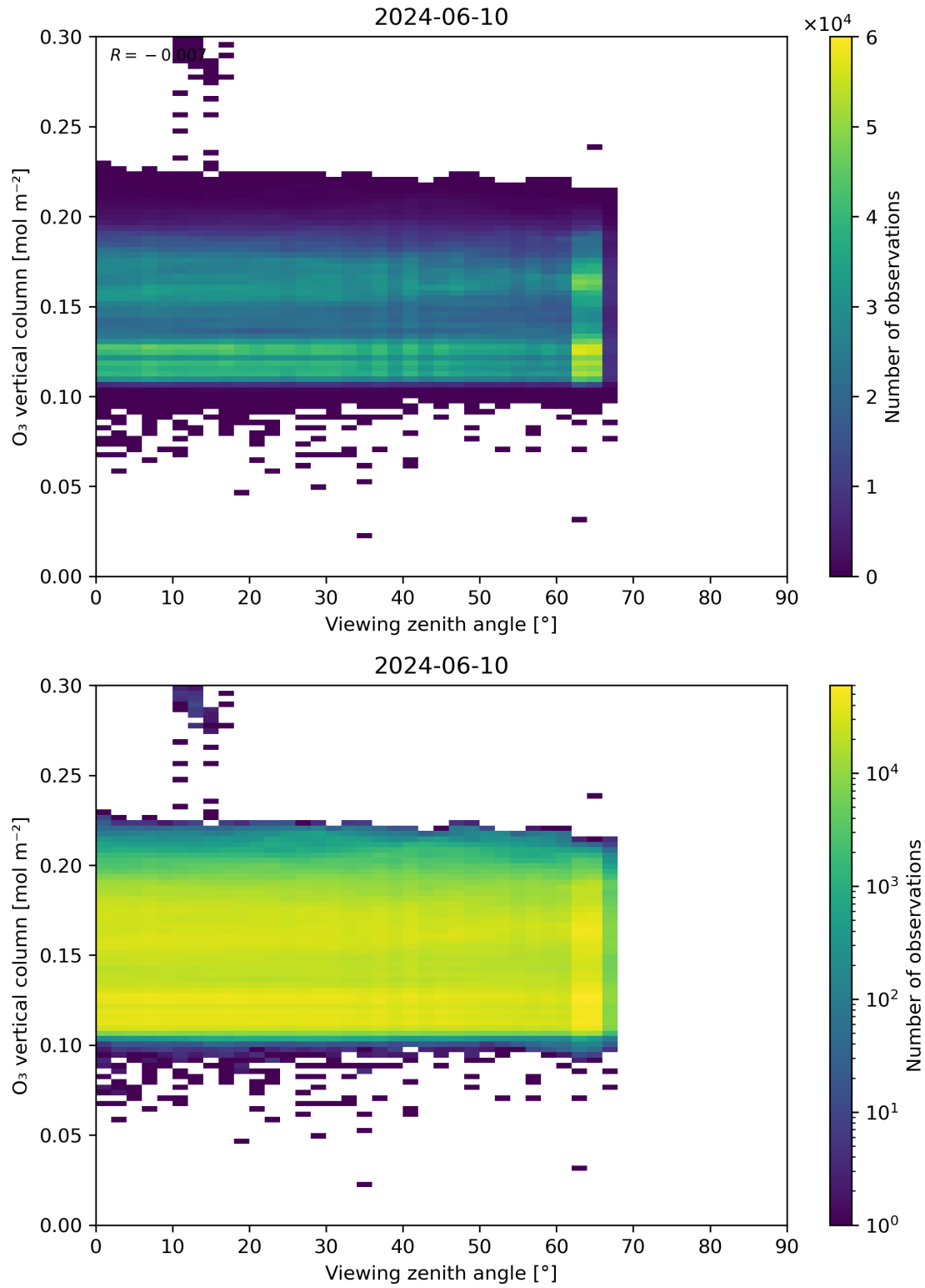
Figure 52: Scatter density plot of “Viewing zenith angle” against “O 3 vertical column” for 2024-06-09 to 2024-06-11.
