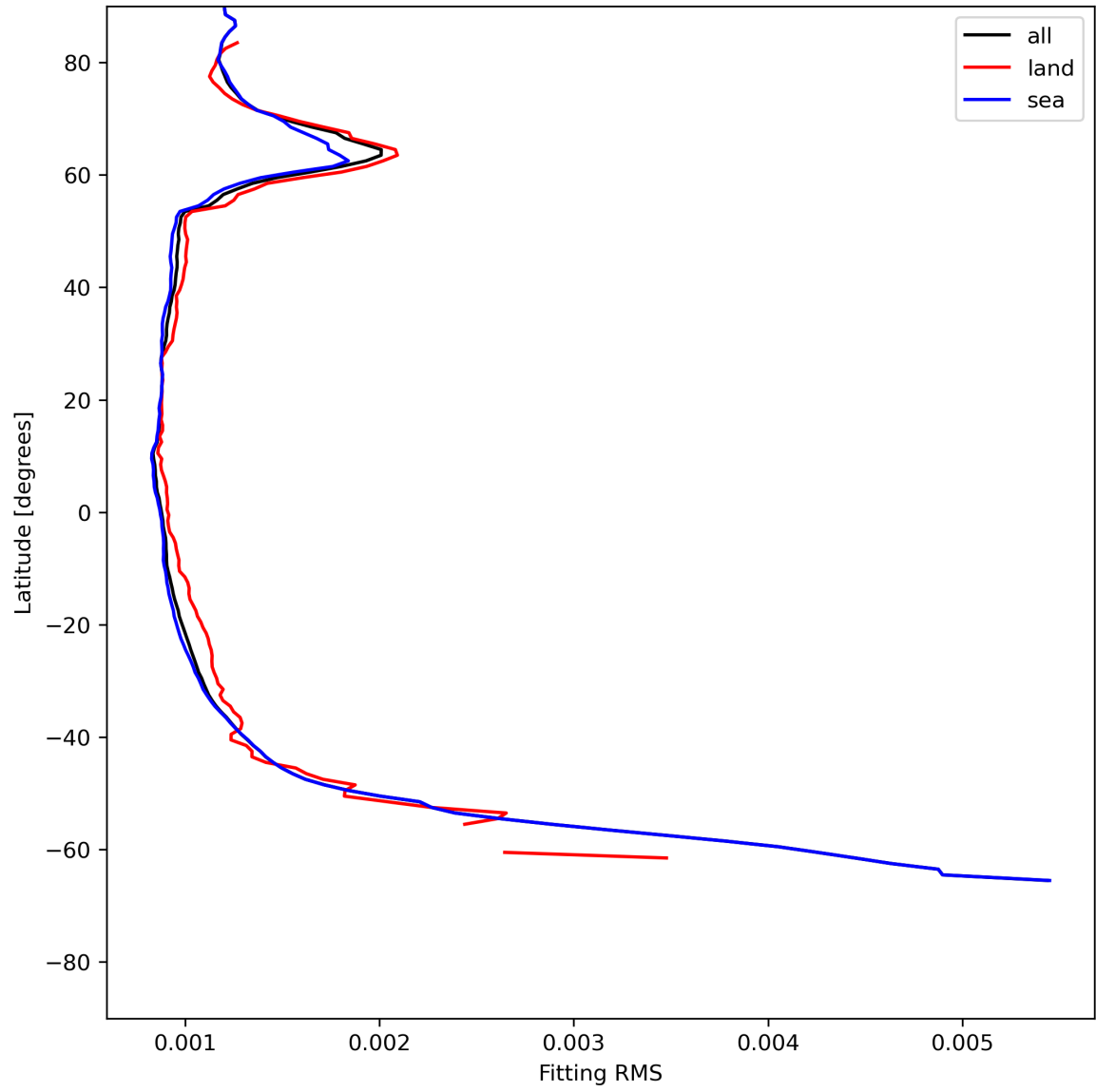
Figure 16: Zonal average of “Fitting RMS” for 2024-06-09 to 2024-06-11.
