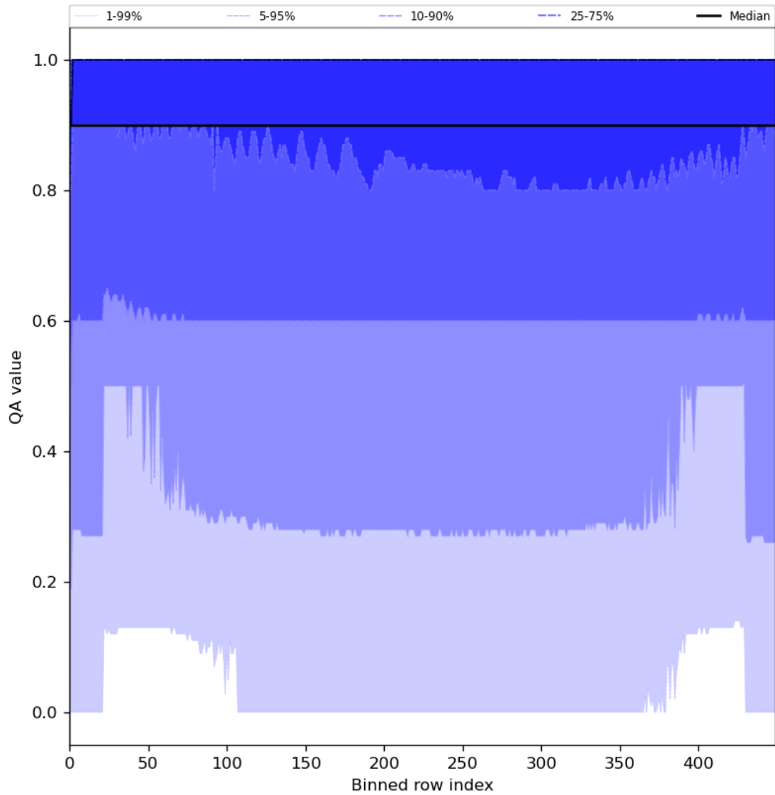
Figure 27: Along track statistics of “QA value” for 2024-06-09 to 2024-06-11
