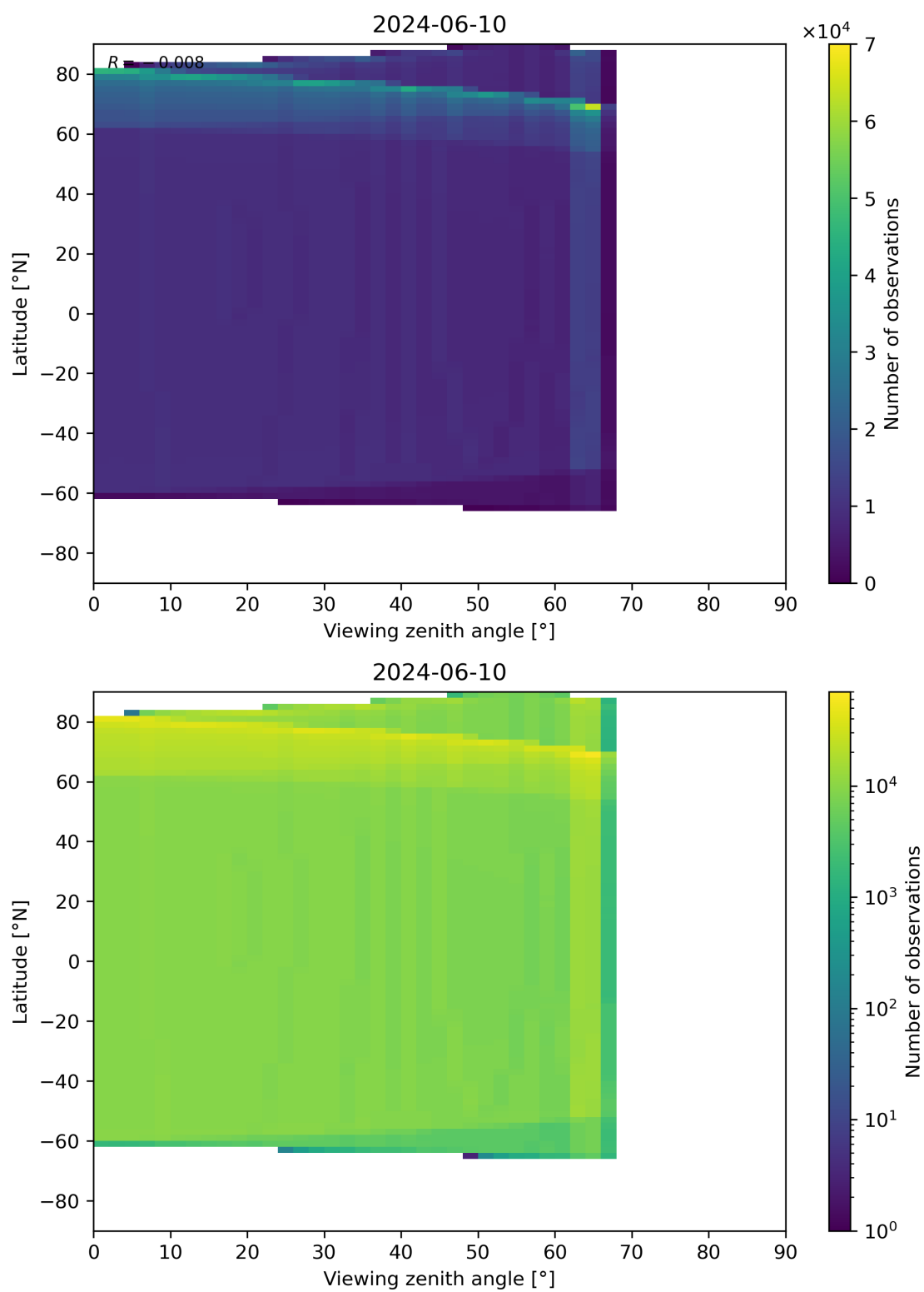
Figure 49: Scatter density plot of “Viewing zenith angle” against “Latitude” for 2024-06-09 to 2024-06-11.
