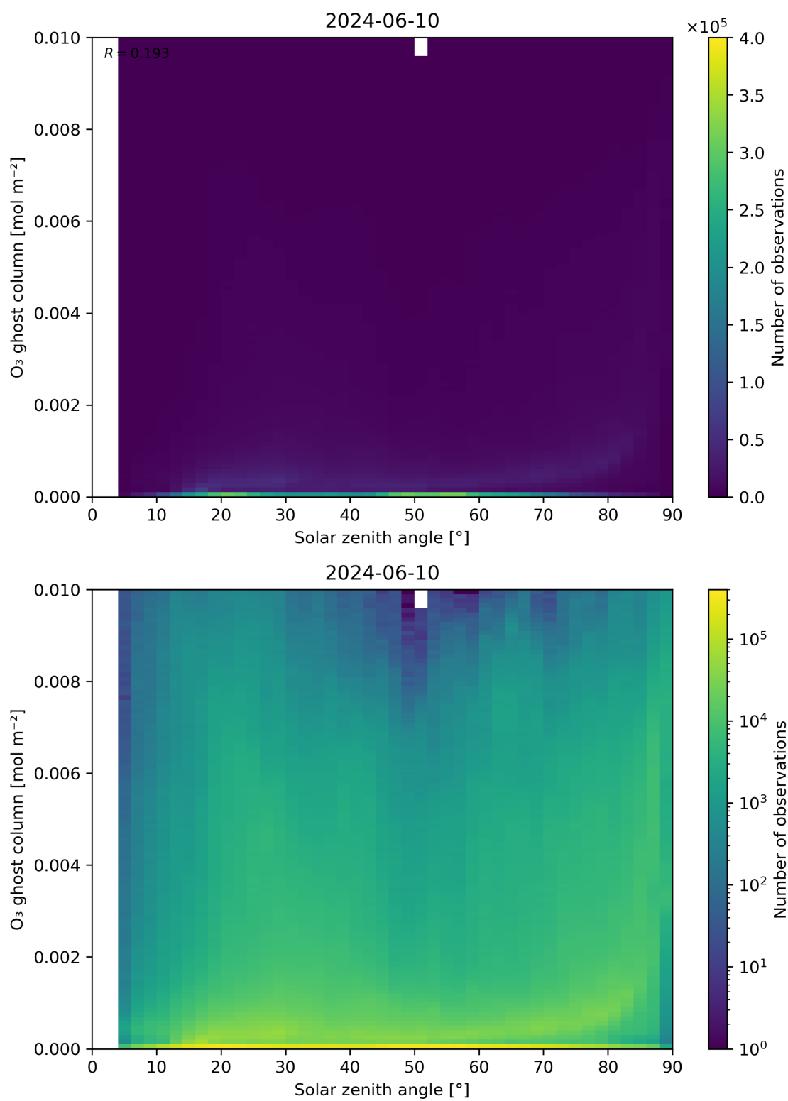
Figure 46: Scatter density plot of “Solar zenith angle” against “O 3 ghost column” for 2024-06-09 to 2024-06-11.
