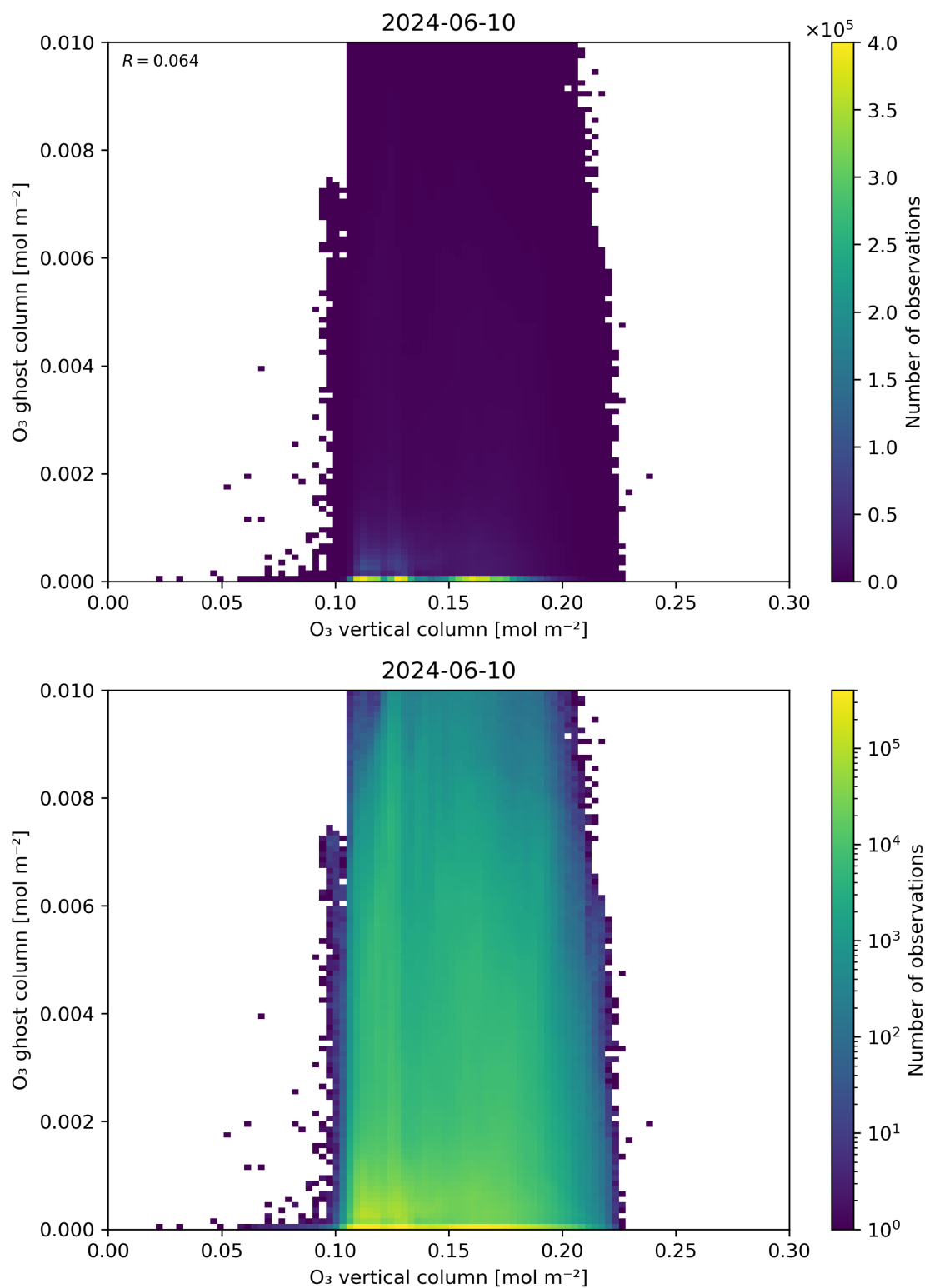
Figure 40: Scatter density plot of “O 3 vertical column” against “O 3 ghost column” for 2024-06-09 to 2024-06-11.
