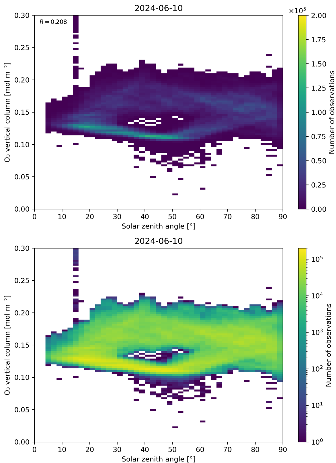
Figure 47: Scatter density plot of “Solar zenith angle” against “O 3 vertical column” for 2024-06-09 to 2024-06-11.
