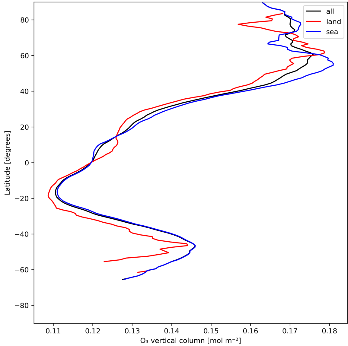
Figure 14: Zonal average of “O 3 vertical column” for 2024-06-09 to 2024-06-11.
