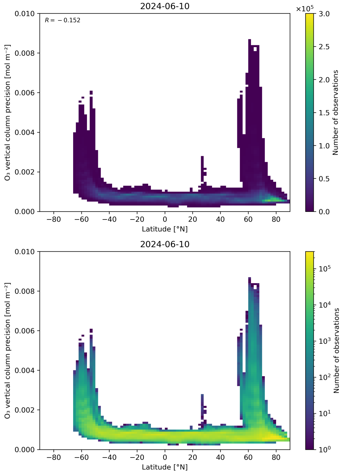
Figure 37: Scatter density plot of “Latitude” against “O 3 vertical column precision” for 2024-06-09 to 2024-06-11.
