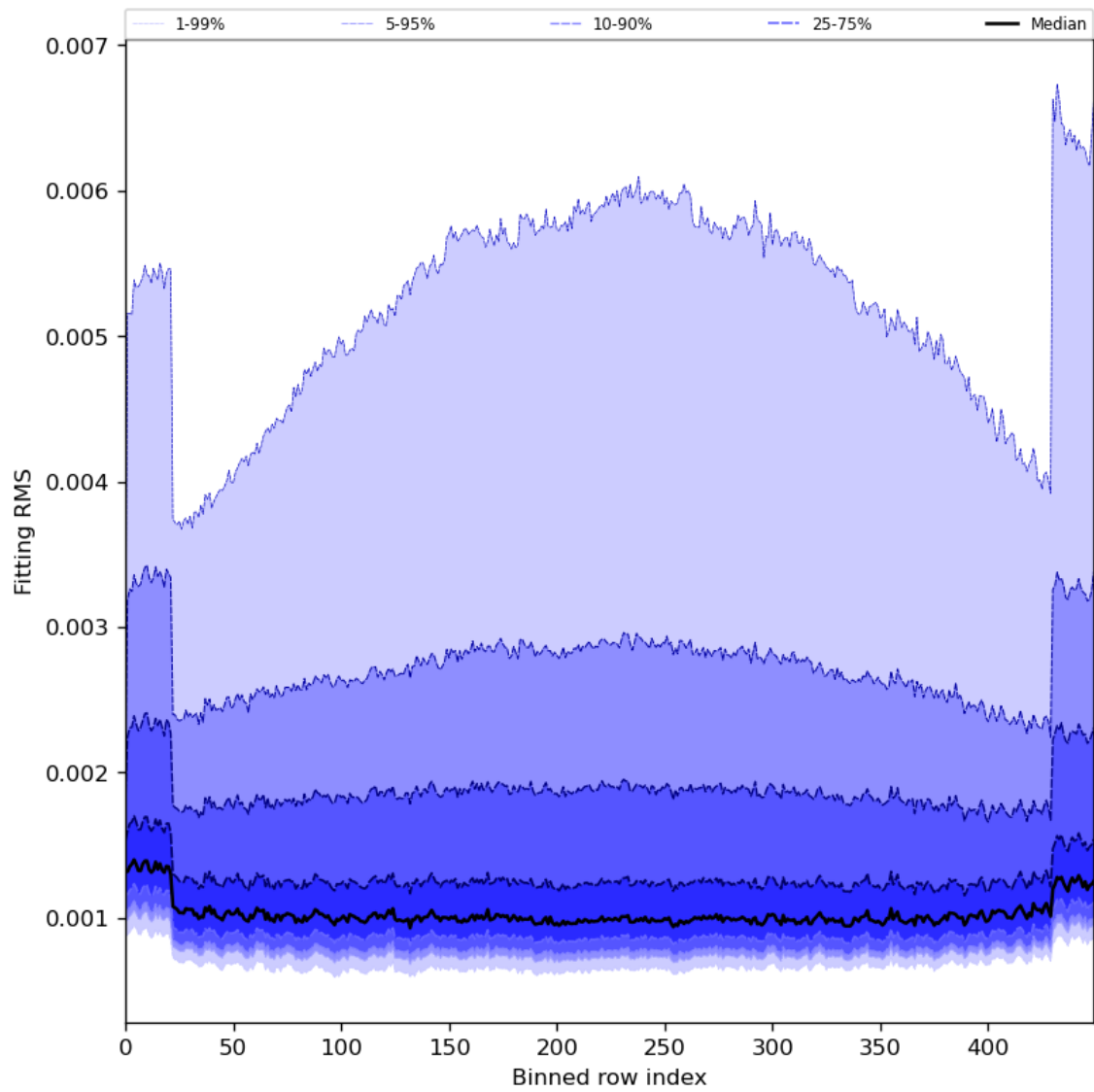
Figure 30: Along track statistics of “Fitting RMS” for 2024-06-09 to 2024-06-11
