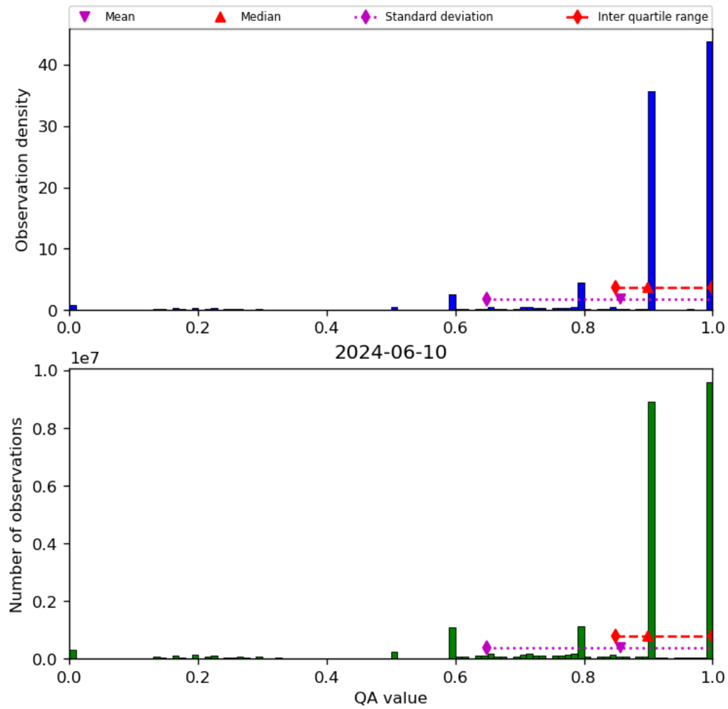
Figure 20: Histogram of “QA value” for 2024-06-09 to 2024-06-11
