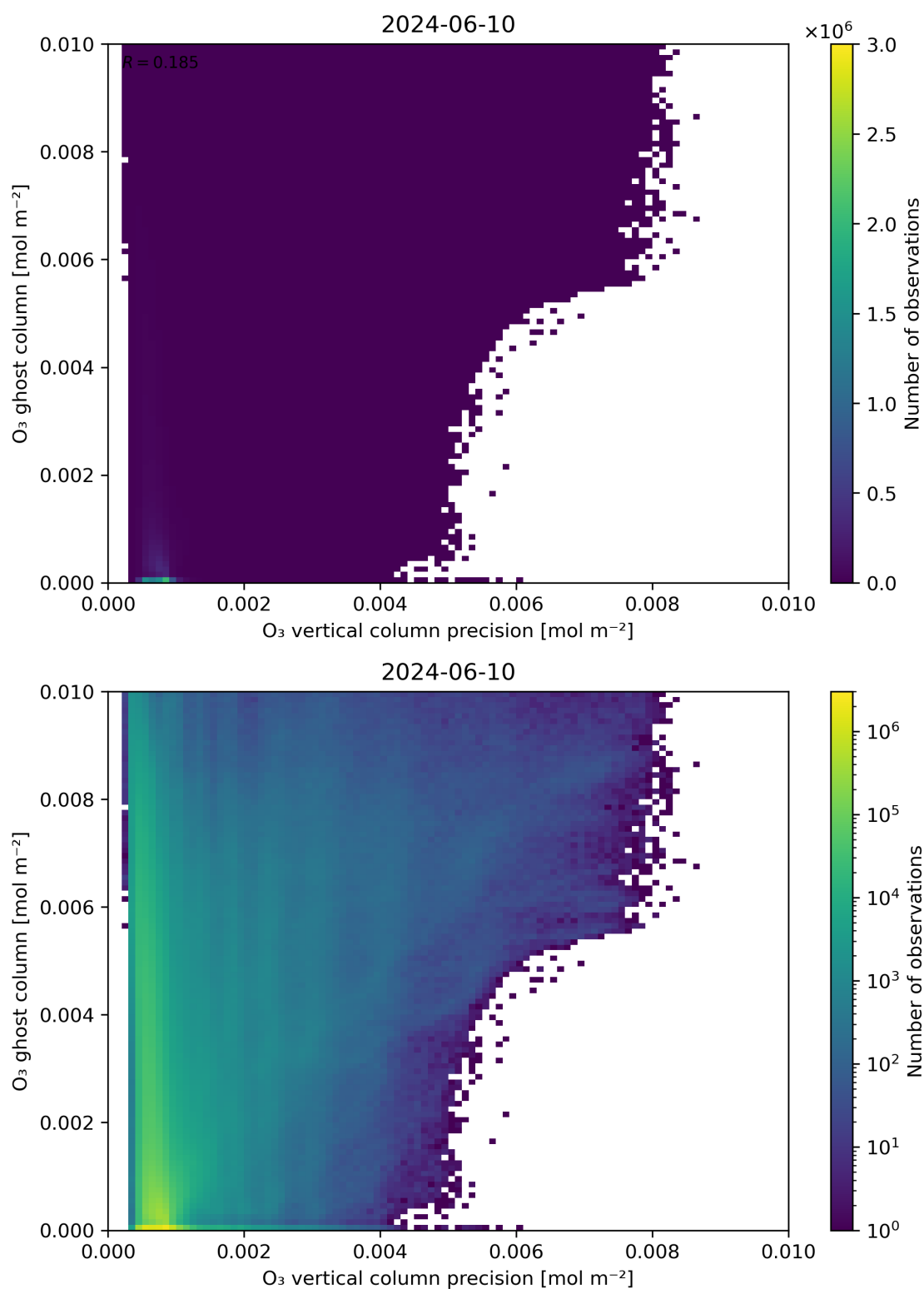
Figure 43: Scatter density plot of “ O_3 vertical column precision” against “ O_3 ghost column” for 2024-06-09 to 2024-06-11.
