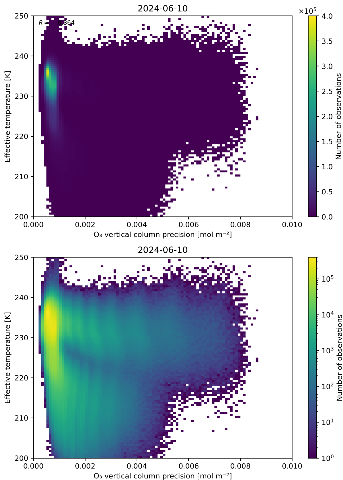
Figure 42: Scatter density plot of “O 3 vertical column precision” against “Effective temperature” for 2024-06-09 to 2024-06-11.
