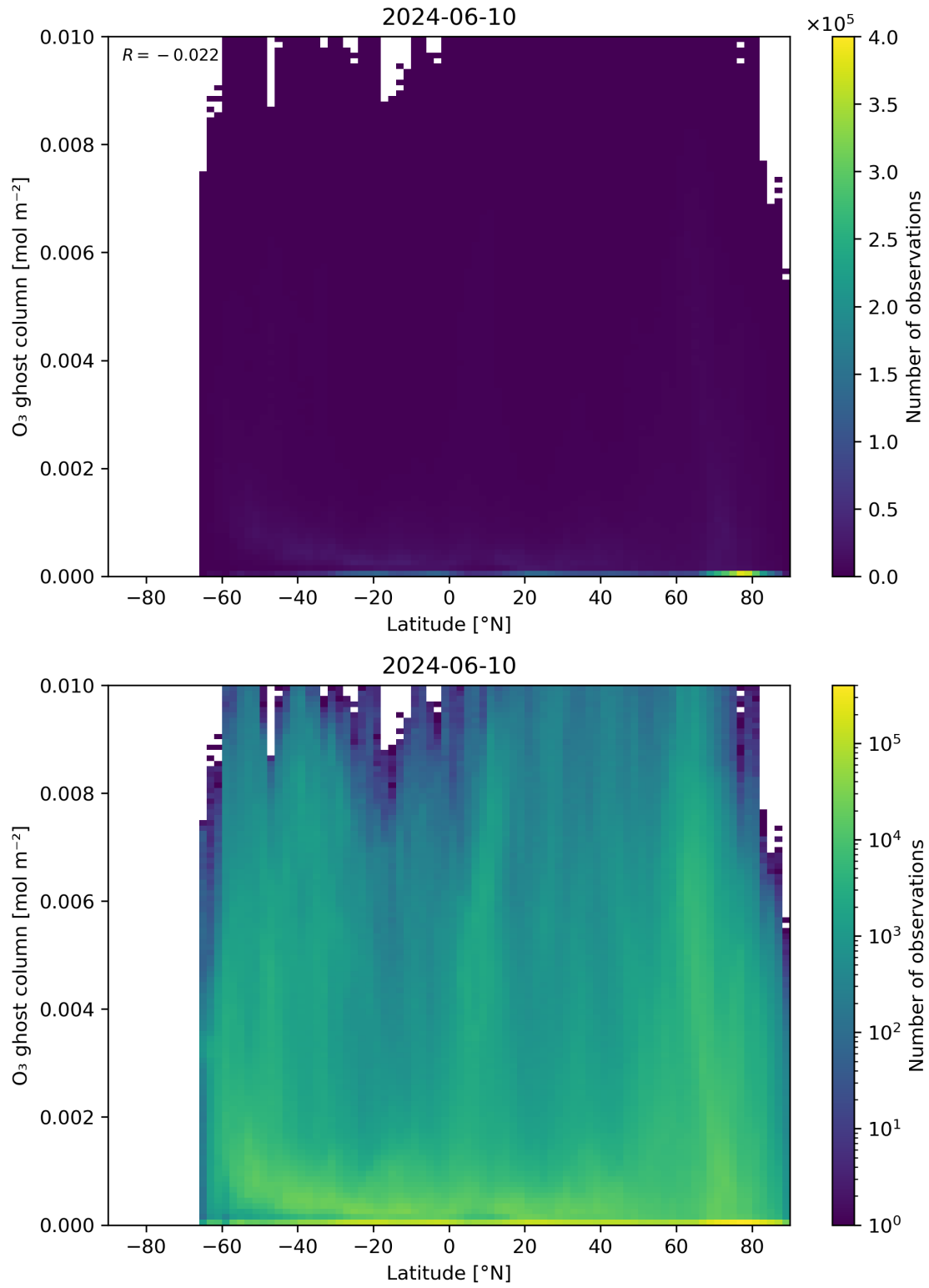
Figure 35: Scatter density plot of “Latitude” against “O 3 ghost column” for 2024-06-09 to 2024-06-11.
