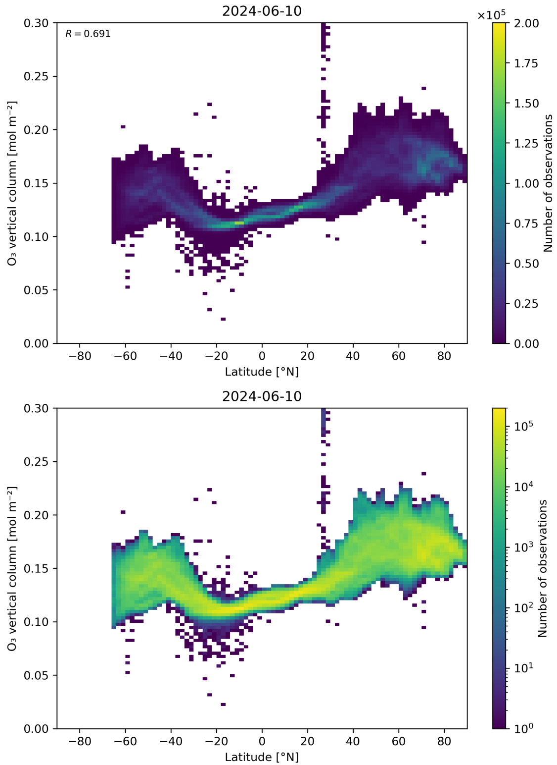
Figure 36: Scatter density plot of “Latitude” against “O 3 vertical column” for 2024-06-09 to 2024-06-11.
