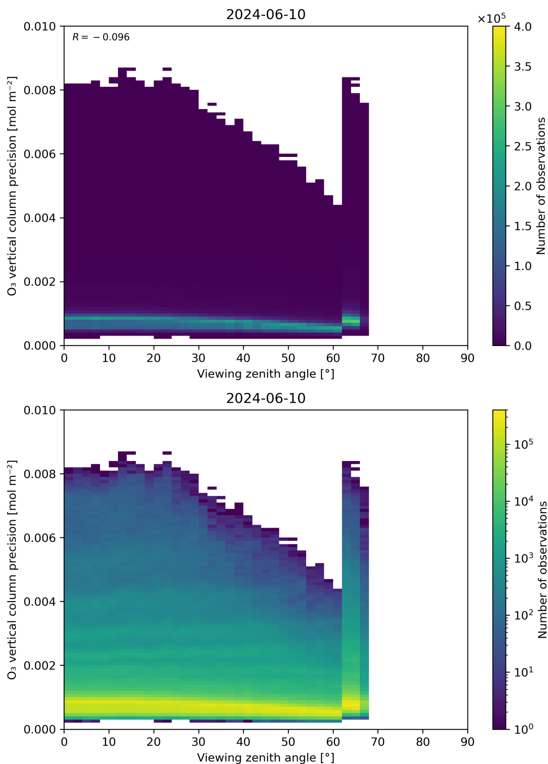
Figure 53: Scatter density plot of “Viewing zenith angle” against “O 3 vertical column precision” for 2024-06-09 to 2024-06-11.
