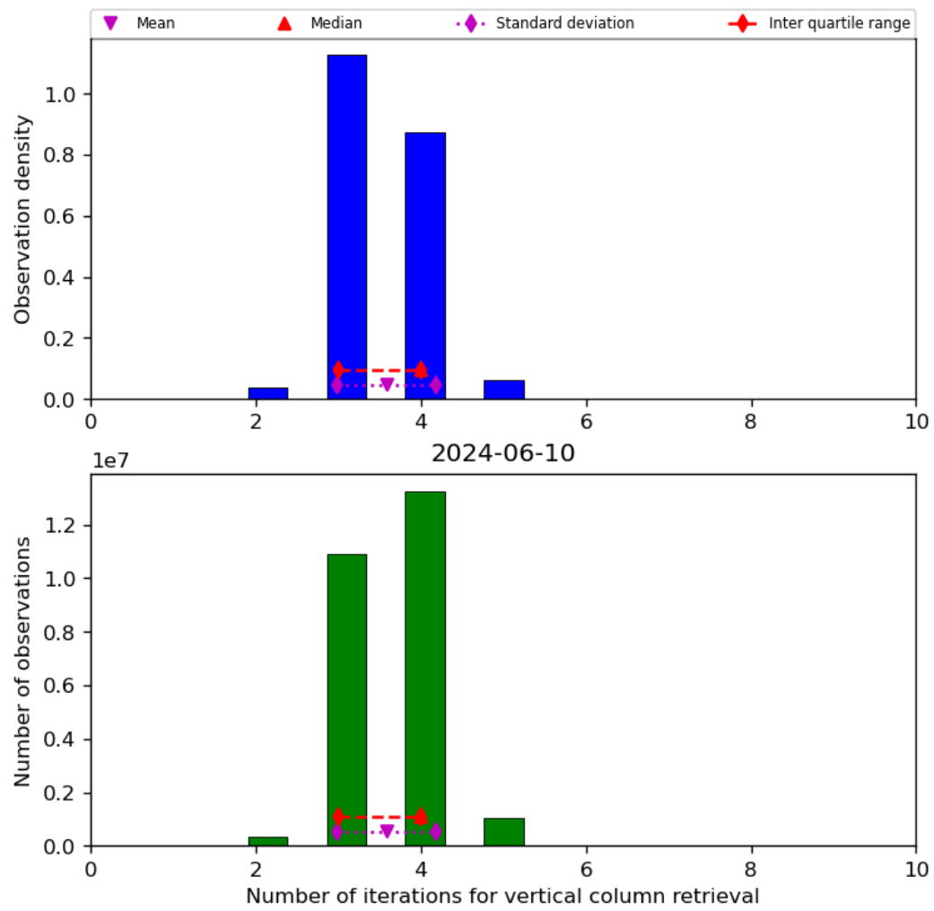
Figure 26: Histogram of “Number of iterations for vertical column retrieval” for 2024-06-09 to 2024-06-11
