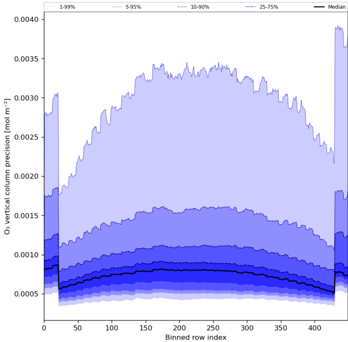
Figure 29: Along track statistics of “O 3 vertical column precision” for 2024-06-09 to 2024-06-11
