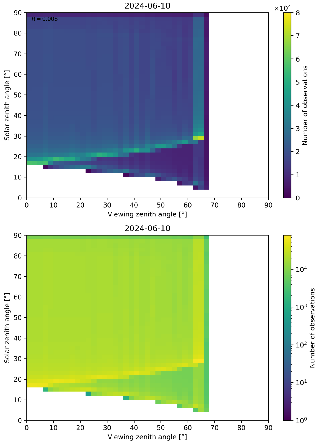
Figure 54: Scatter density plot of “Viewing zenith angle” against “Solar zenith angle” for 2024-06-09 to 2024-06-11.
