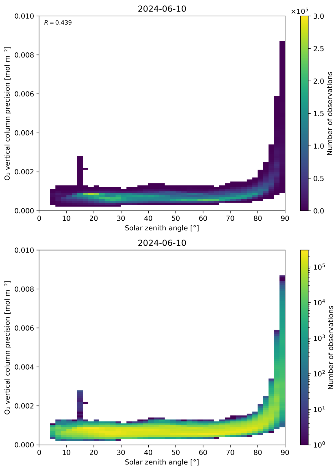
Figure 48: Scatter density plot of “Solar zenith angle” against “O 3 vertical column precision” for 2024-06-09 to 2024-06-11.
