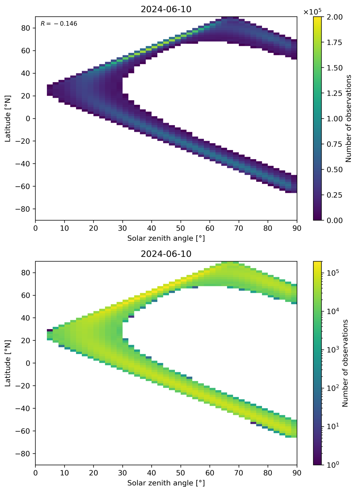
Figure 44: Scatter density plot of “Solar zenith angle” against “Latitude” for 2024-06-09 to 2024-06-11.
