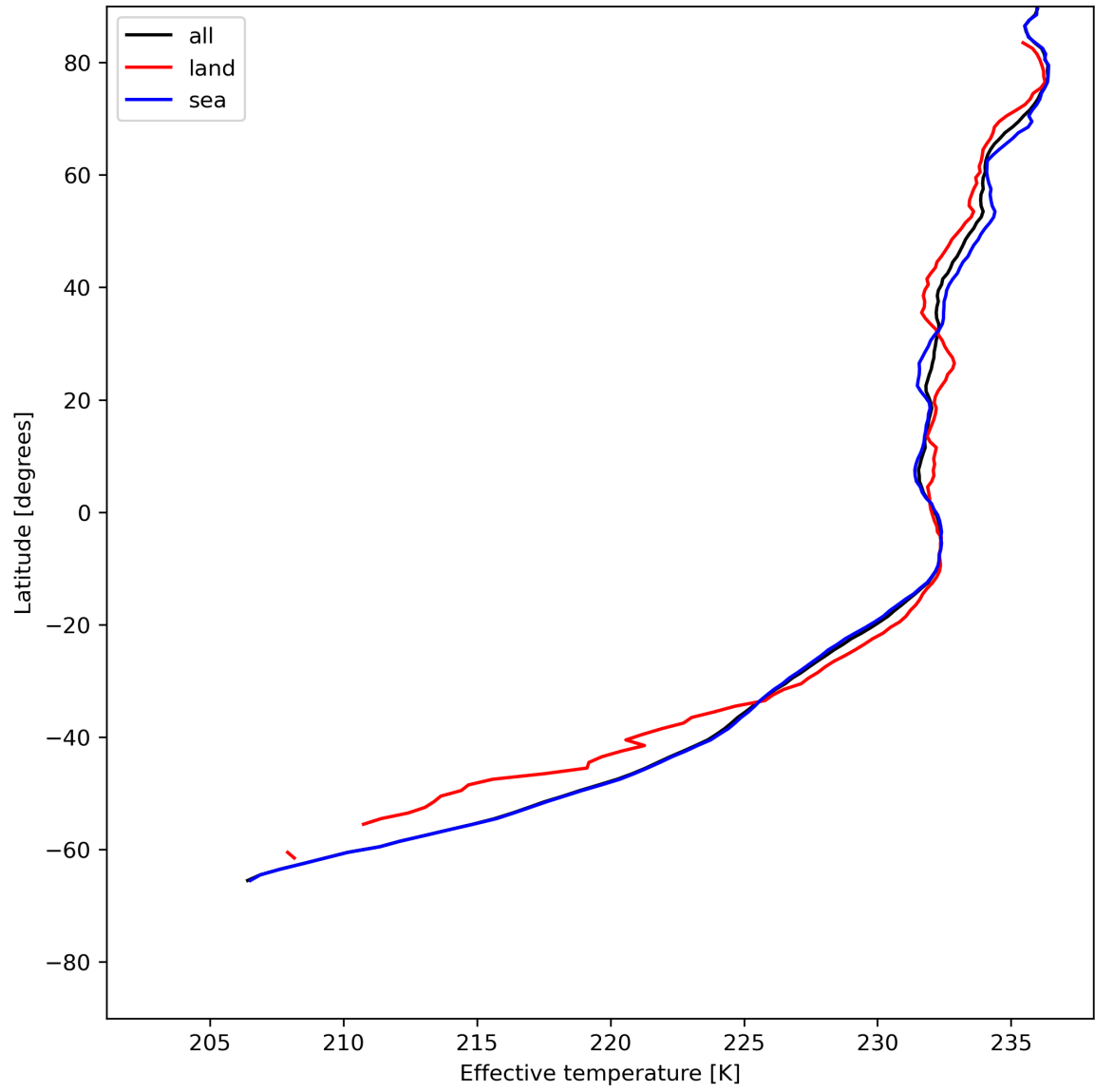
Figure 17: Zonal average of “Effective temperature” for 2024-06-09 to 2024-06-11.
