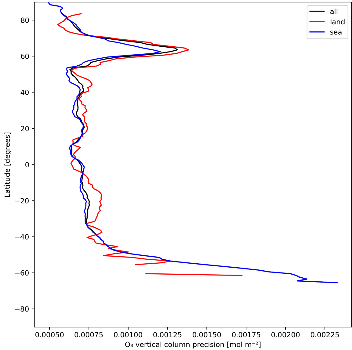
Figure 15: Zonal average of “O 3 vertical column precision” for 2024-06-09 to 2024-06-11.
