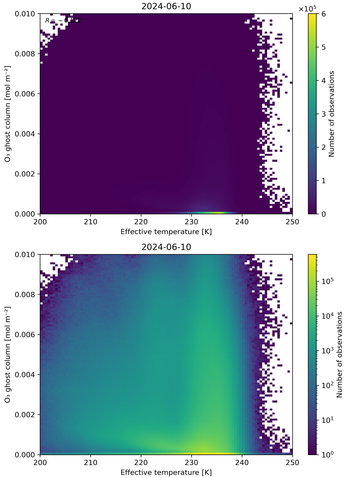
Figure 38: Scatter density plot of “Effective temperature” against “O 3 ghost column” for 2024-06-09 to 2024-06-11.
