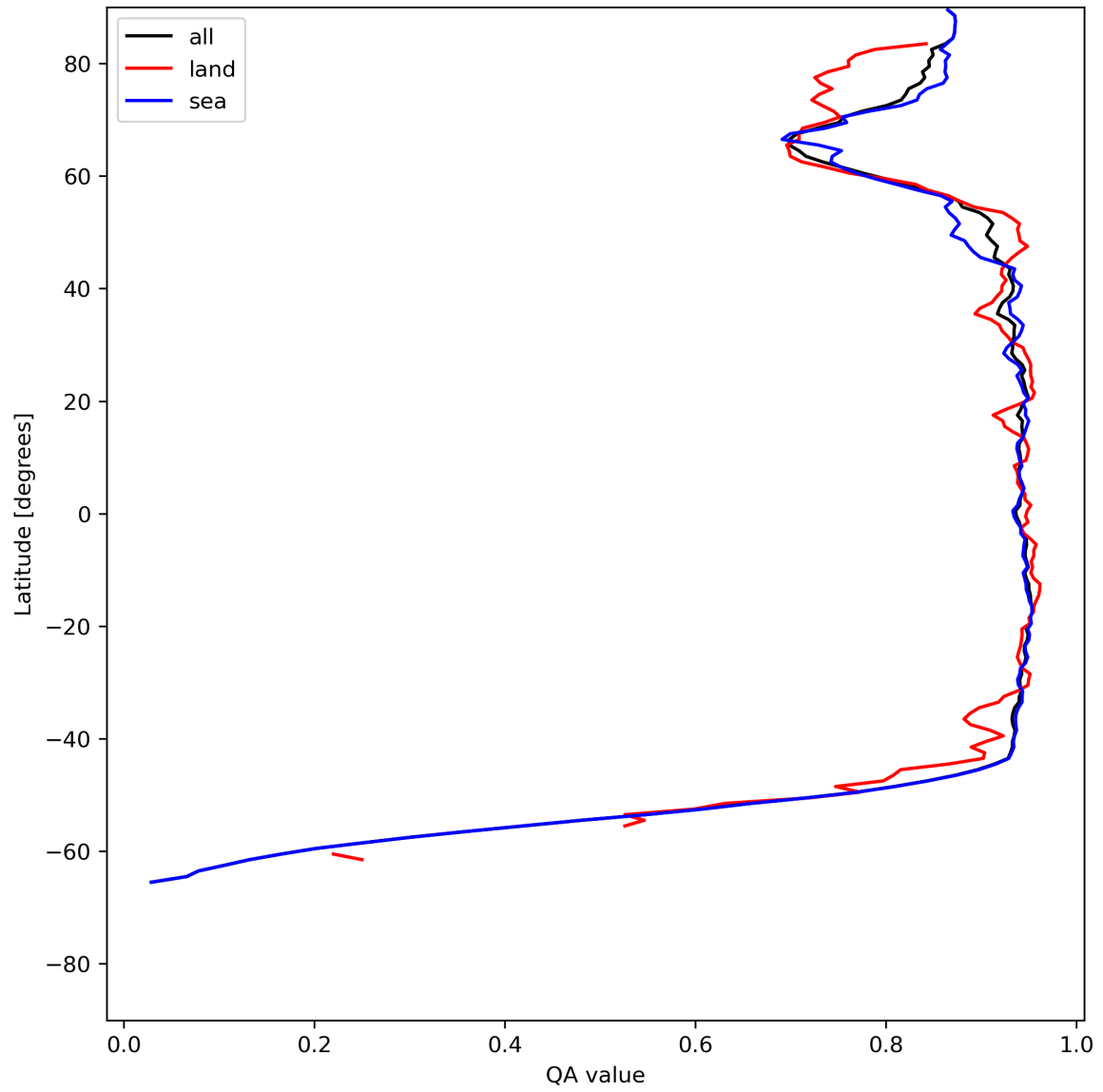
Figure 13: Zonal average of “QA value” for 2024-06-09 to 2024-06-11.
