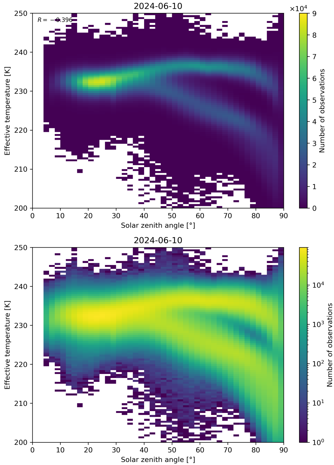
Figure 45: Scatter density plot of “Solar zenith angle” against “Effective temperature” for 2024-06-09 to 2024-06-11.
