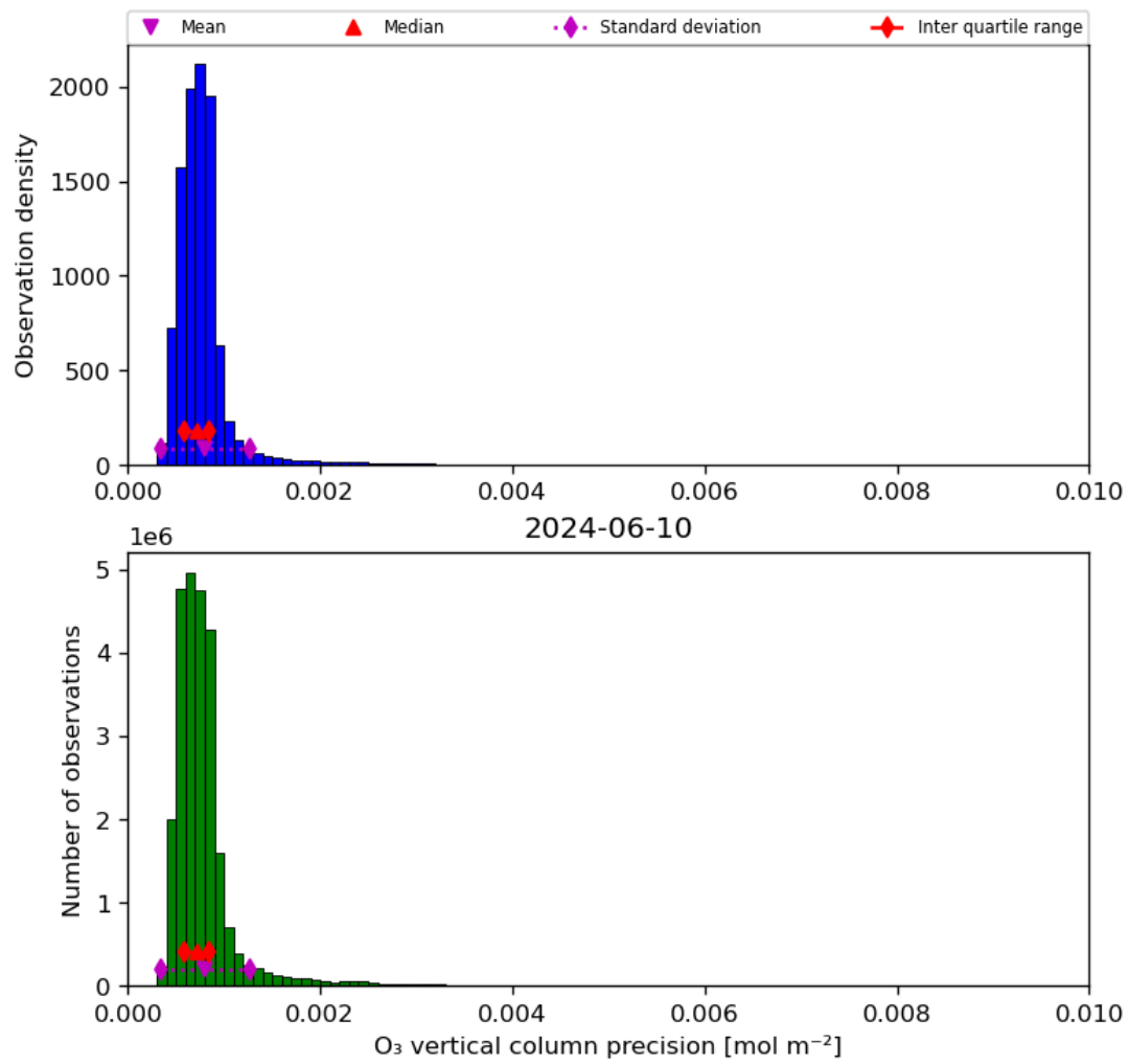
Figure 22: Histogram of “O 3 vertical column precision” for 2024-06-09 to 2024-06-11
