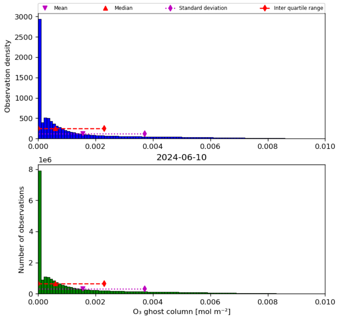
Figure 25: Histogram of “O 3 ghost column” for 2024-06-09 to 2024-06-11
