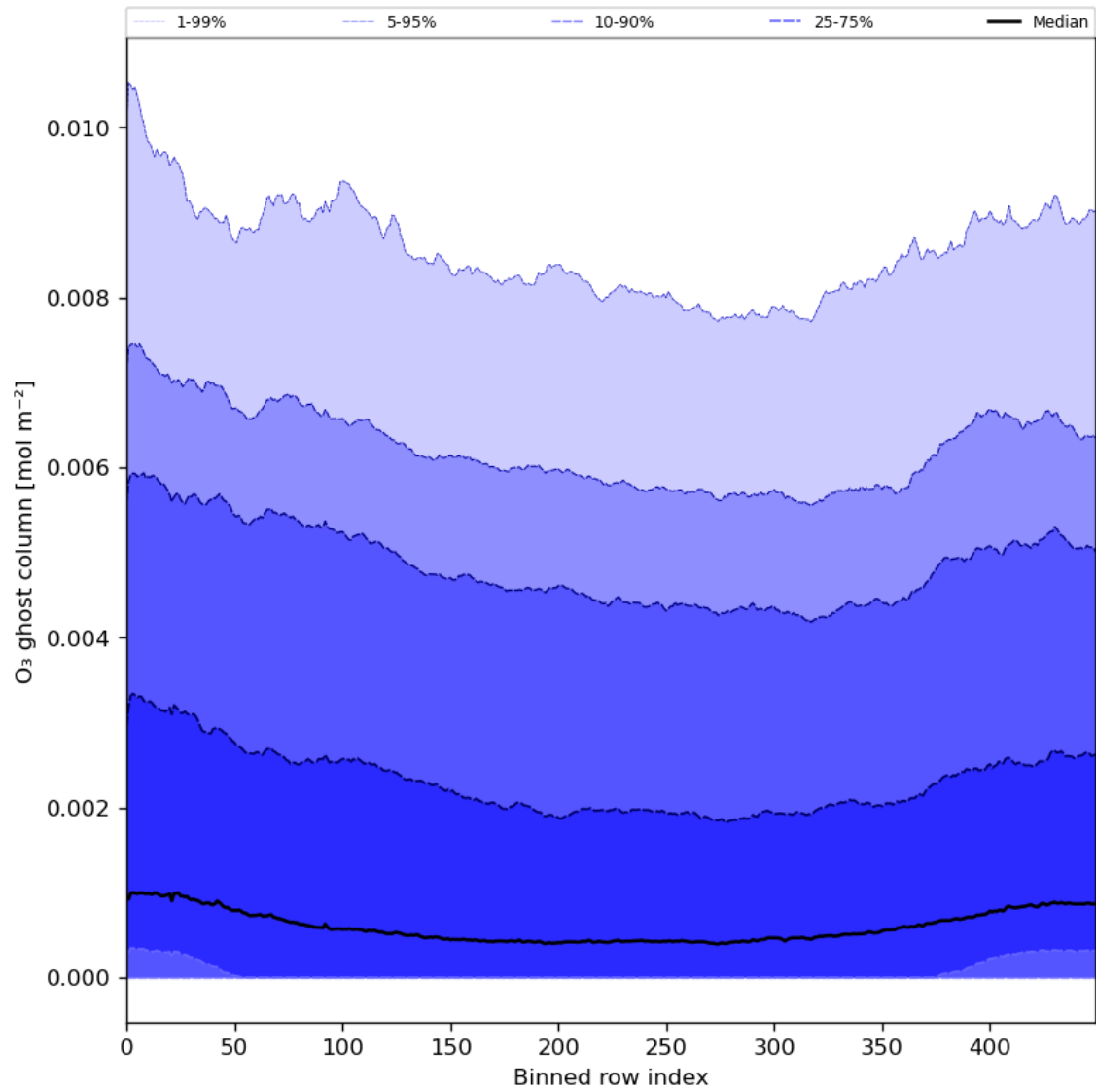
Figure 32: Along track statistics of “O 3 ghost column” for 2024-06-09 to 2024-06-11
