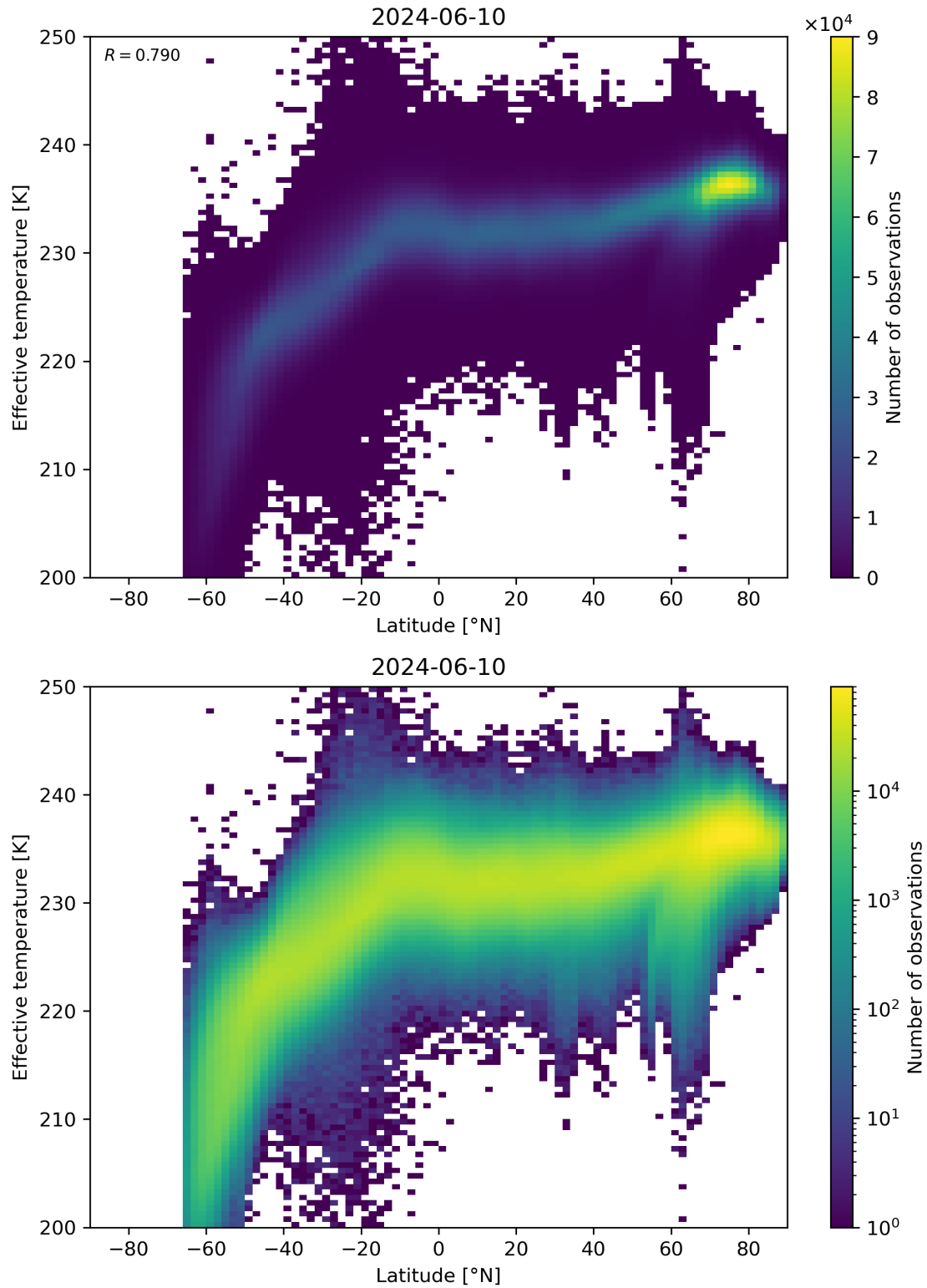
Figure 34: Scatter density plot of “Latitude” against “Effective temperature” for 2024-06-09 to 2024-06-11.
