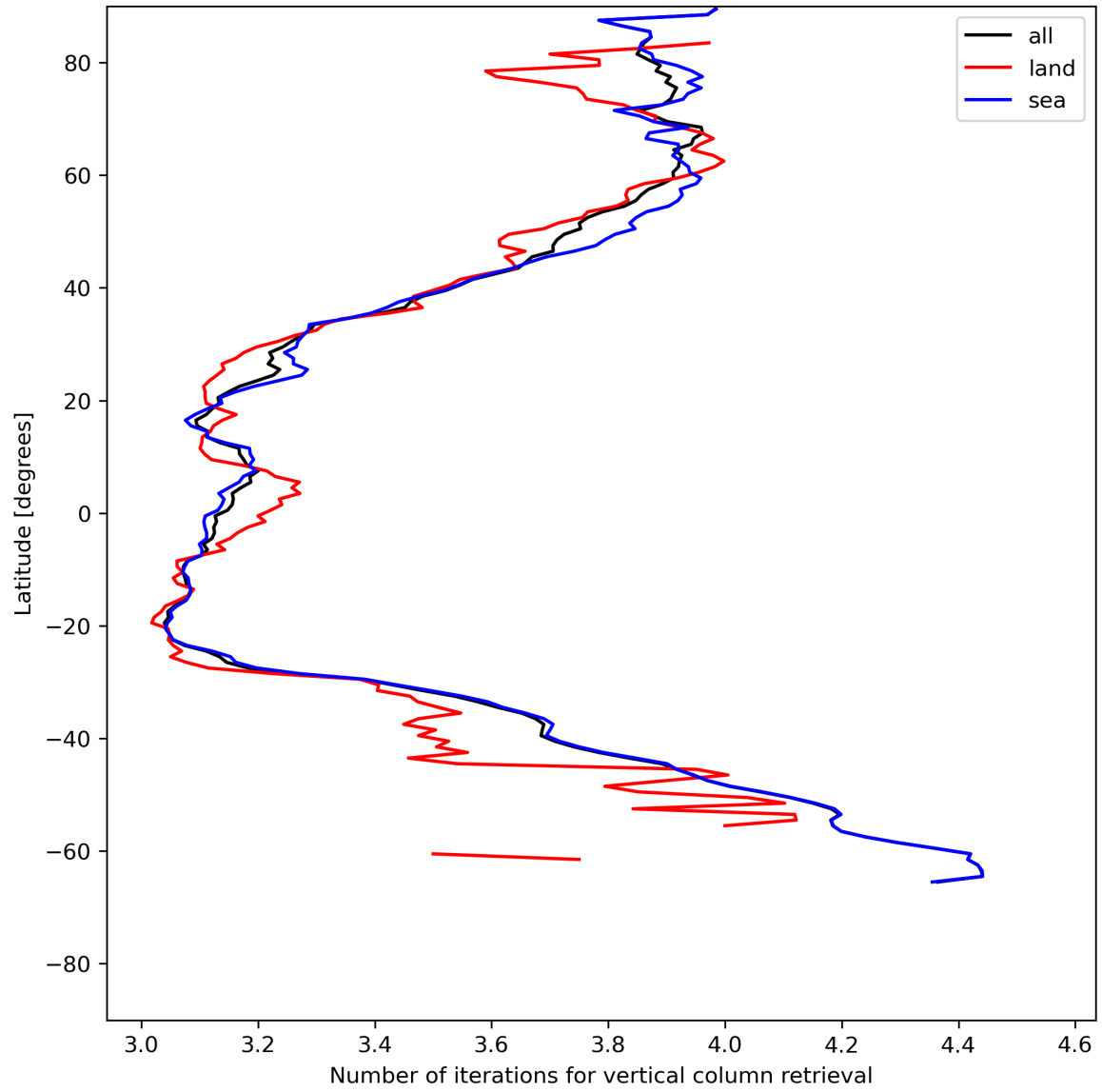
Figure 19: Zonal average of “Number of iterations for vertical column retrieval” for 2024-06-09 to 2024-06-11.
