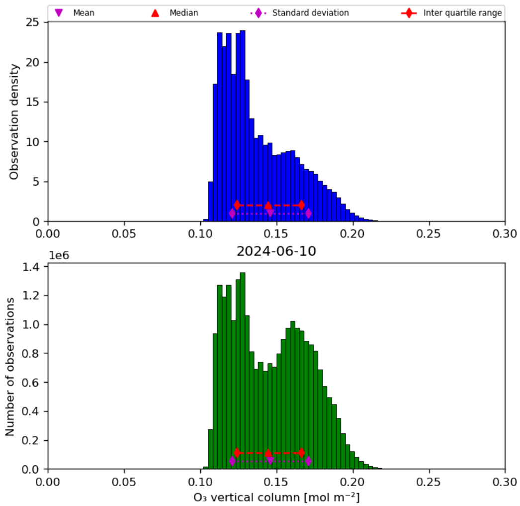
Figure 21: Histogram of “O 3 vertical column” for 2024-06-09 to 2024-06-11
