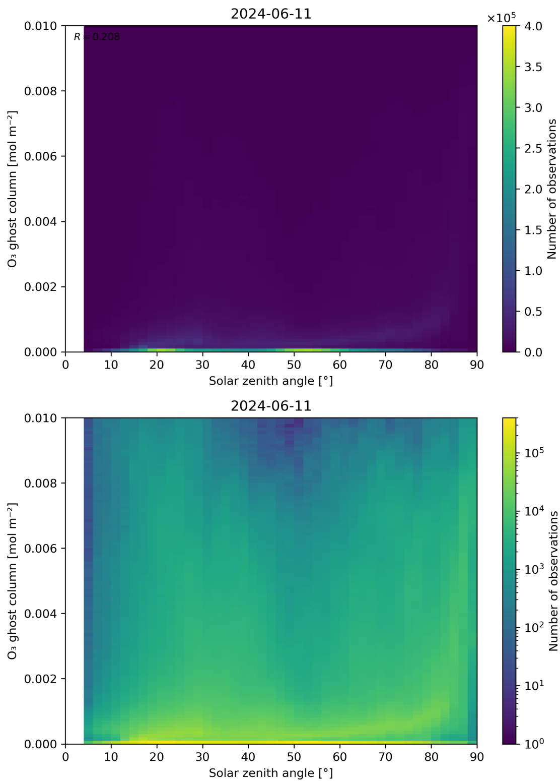
Figure 46: Scatter density plot of “Solar zenith angle” against “O 3 ghost column” for 2024-06-10 to 2024-06-12.
