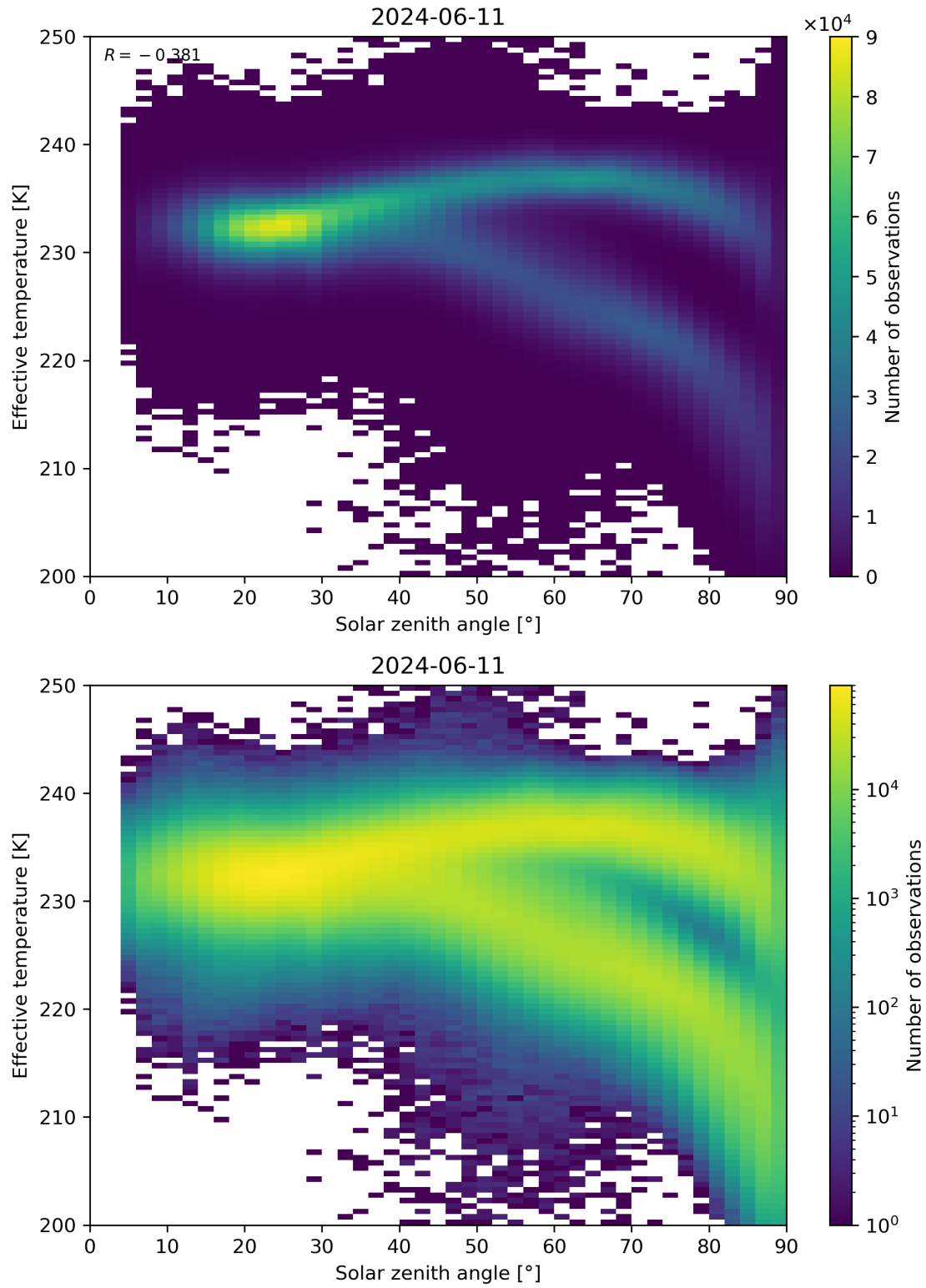
Figure 45: Scatter density plot of “Solar zenith angle” against “Effective temperature” for 2024-06-10 to 2024-06-12.
