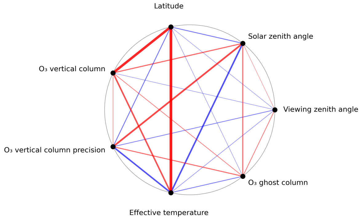
Figure 1: Map of correlation graph for 2024-06-10 to 2024-06-12.
