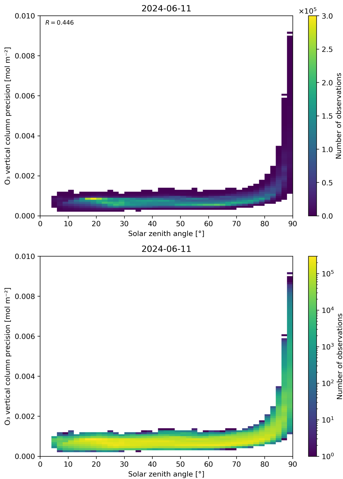
Figure 48: Scatter density plot of “Solar zenith angle” against “O 3 vertical column precision” for 2024-06-10 to 2024-06-12.
