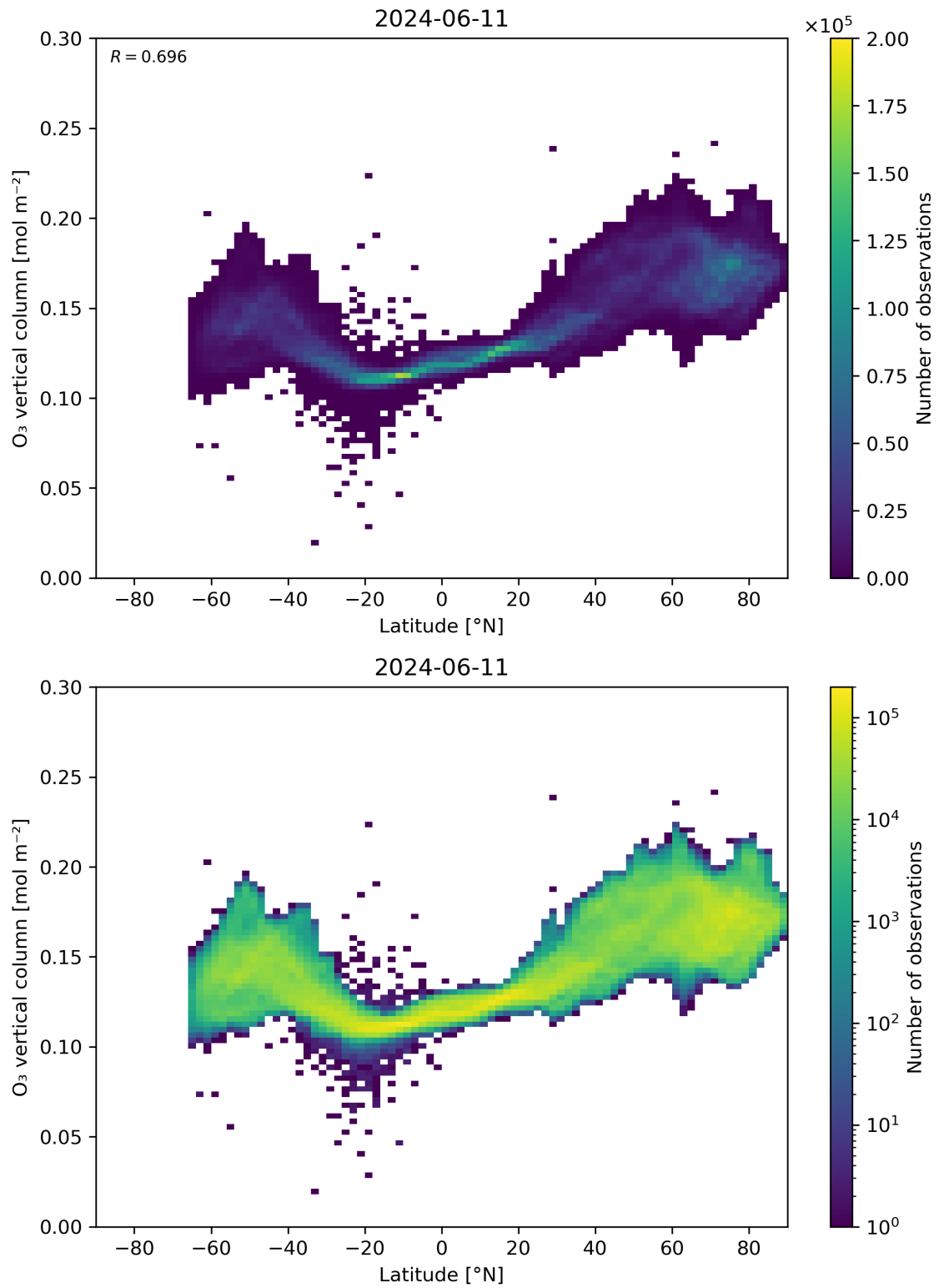
Figure 36: Scatter density plot of “Latitude” against “O 3 vertical column” for 2024-06-10 to 2024-06-12.
