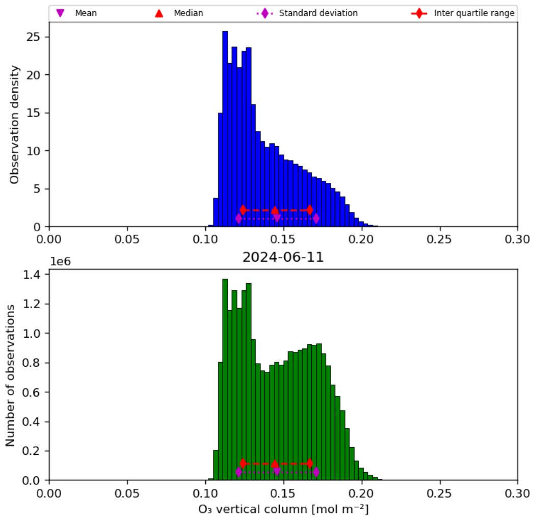
Figure 21: Histogram of “O 3 vertical column” for 2024-06-10 to 2024-06-12
