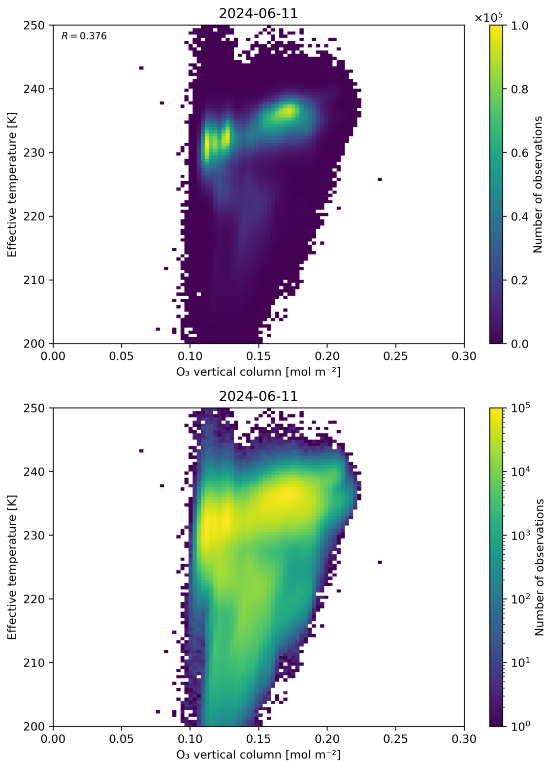
Figure 39: Scatter density plot of “O 3 vertical column” against “Effective temperature” for 2024-06-10 to 2024-06-12.
