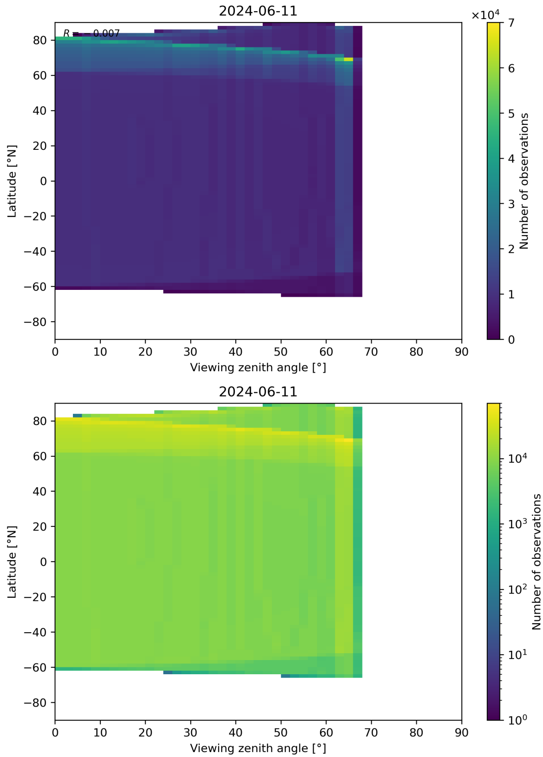
Figure 49: Scatter density plot of “Viewing zenith angle” against “Latitude” for 2024-06-10 to 2024-06-12.
