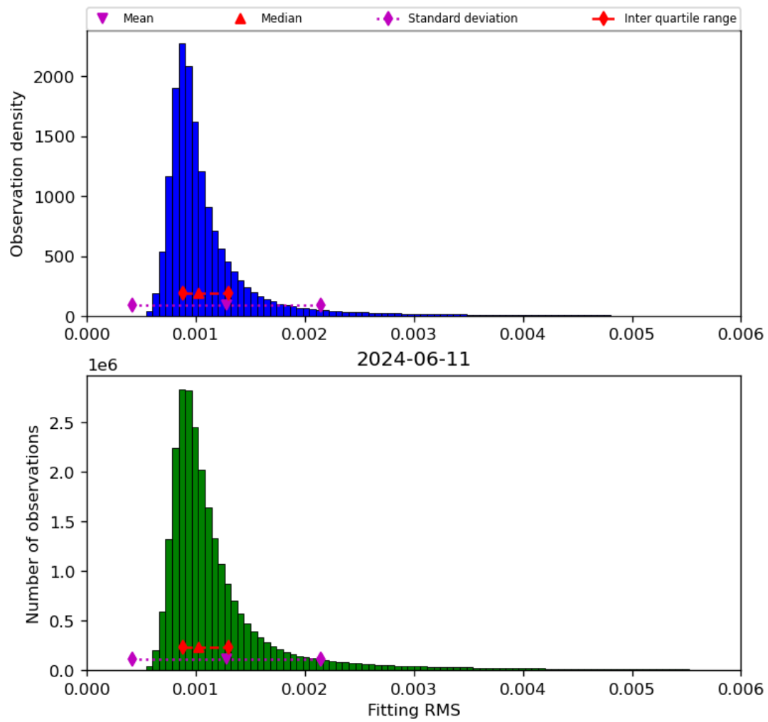
Figure 23: Histogram of “Fitting RMS” for 2024-06-10 to 2024-06-12
