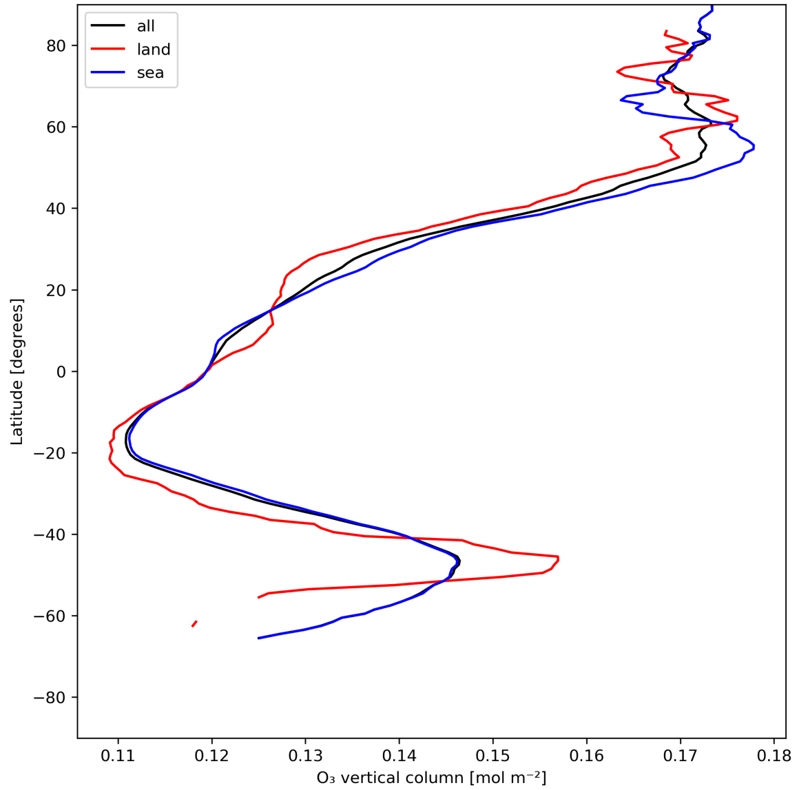
Figure 14: Zonal average of “O 3 vertical column” for 2024-06-10 to 2024-06-12.
