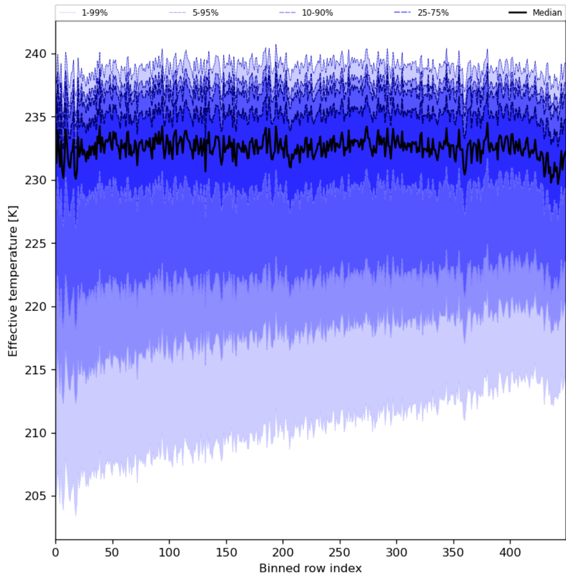
Figure 31: Along track statistics of “Effective temperature” for 2024-06-10 to 2024-06-12
