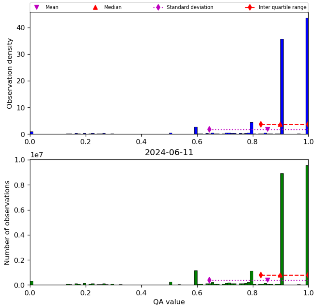
Figure 20: Histogram of “QA value” for 2024-06-10 to 2024-06-12
