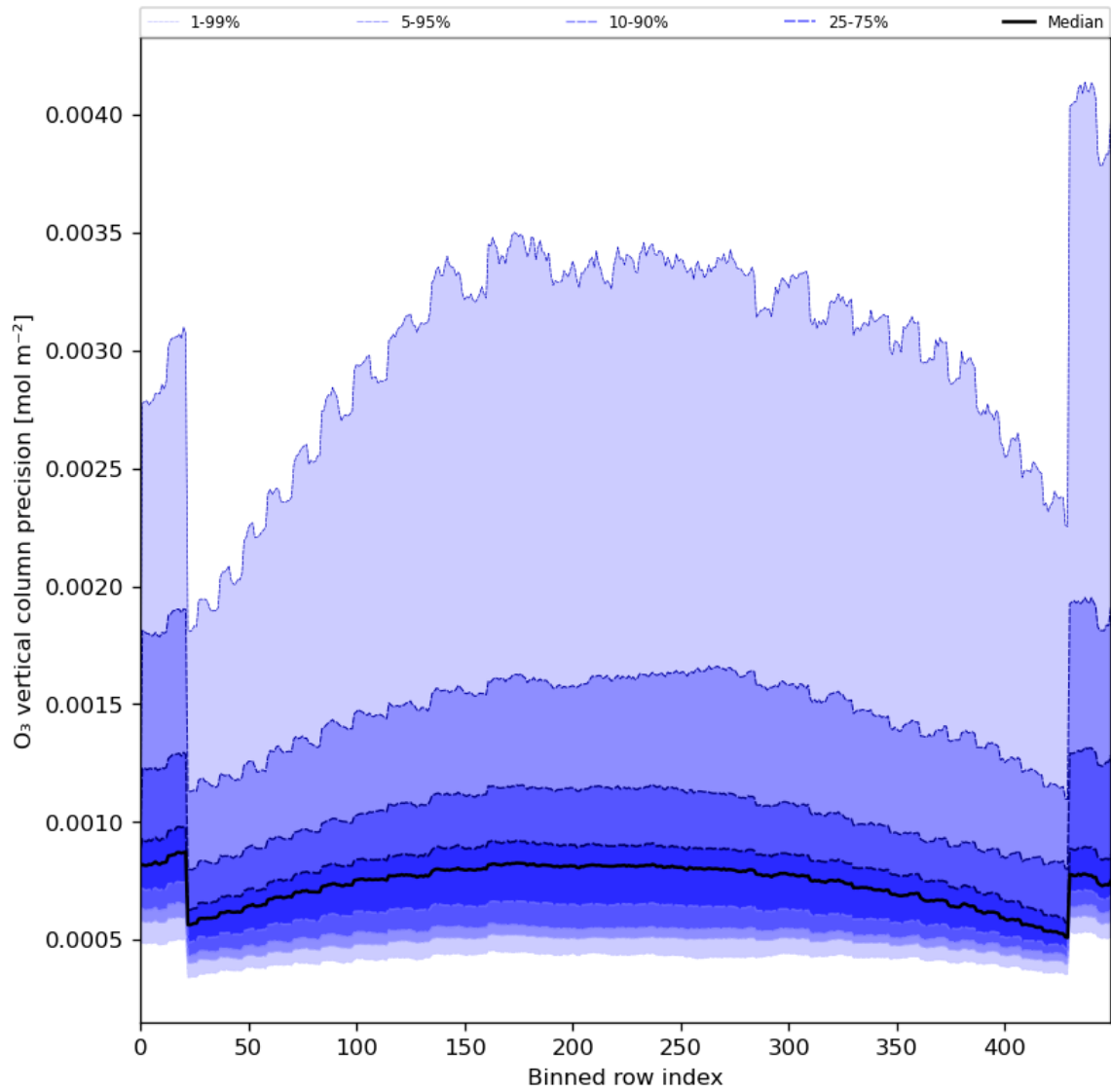
Figure 29: Along track statistics of “O 3 vertical column precision” for 2024-06-10 to 2024-06-12
