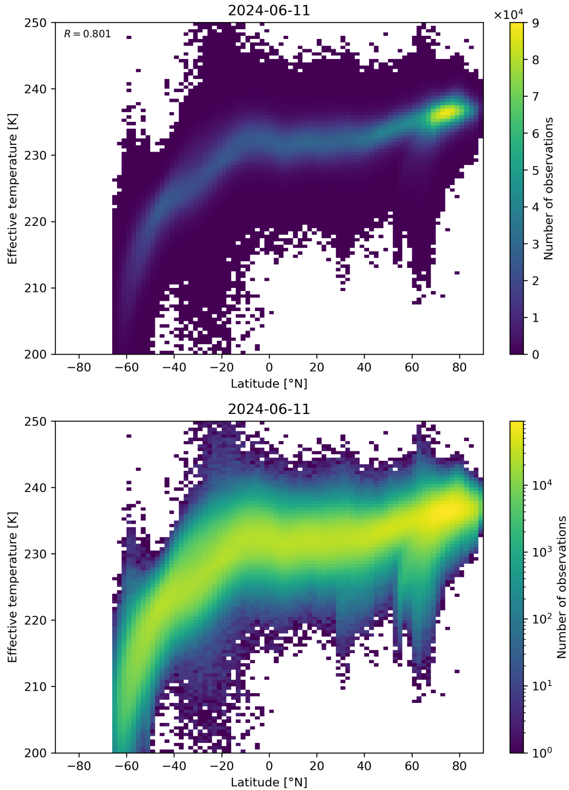
Figure 34: Scatter density plot of “Latitude” against “Effective temperature” for 2024-06-10 to 2024-06-12.
