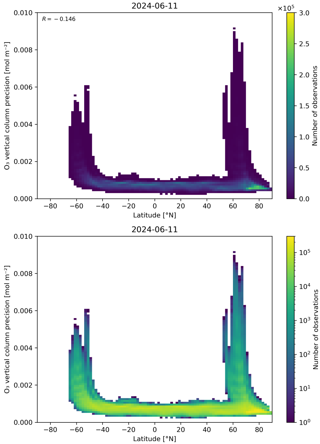
Figure 37: Scatter density plot of “Latitude” against “O 3 vertical column precision” for 2024-06-10 to 2024-06-12.
