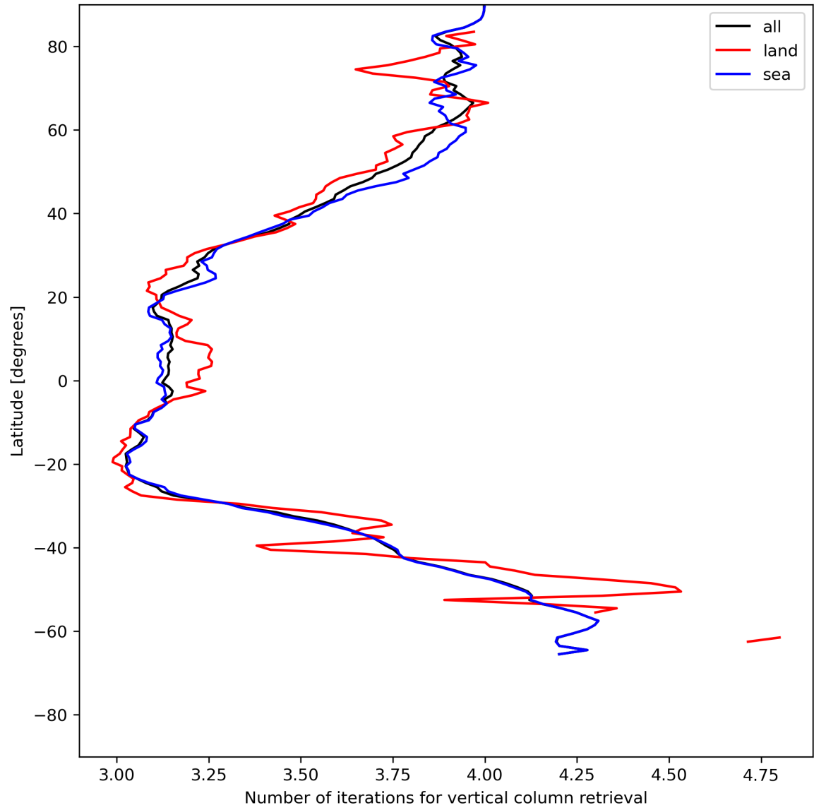
Figure 19: Zonal average of “Number of iterations for vertical column retrieval” for 2024-06-10 to 2024-06-12.
