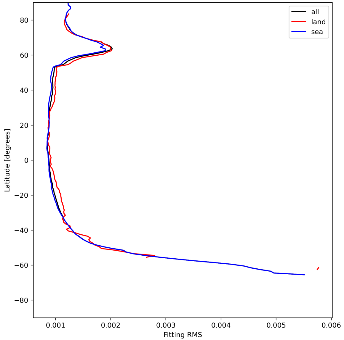
Figure 16: Zonal average of “Fitting RMS” for 2024-06-10 to 2024-06-12.
