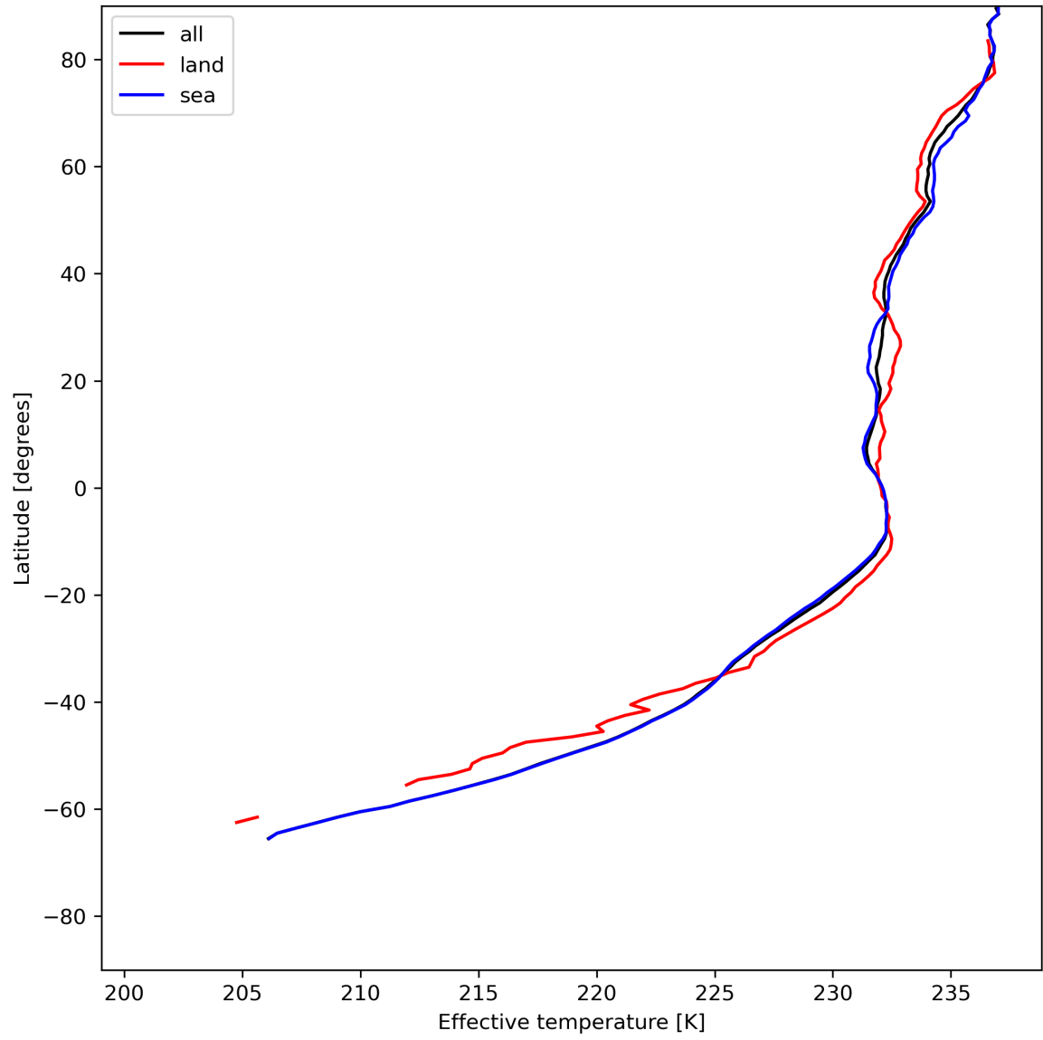
Figure 17: Zonal average of "Effective temperature" for 2024-06-10 to 2024-06-12.
