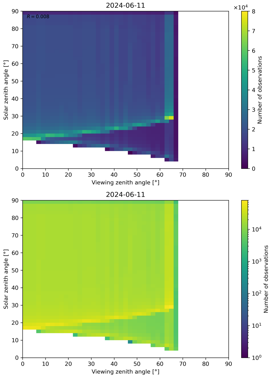
Figure 54: Scatter density plot of “Viewing zenith angle” against “Solar zenith angle” for 2024-06-10 to 2024-06-12.
