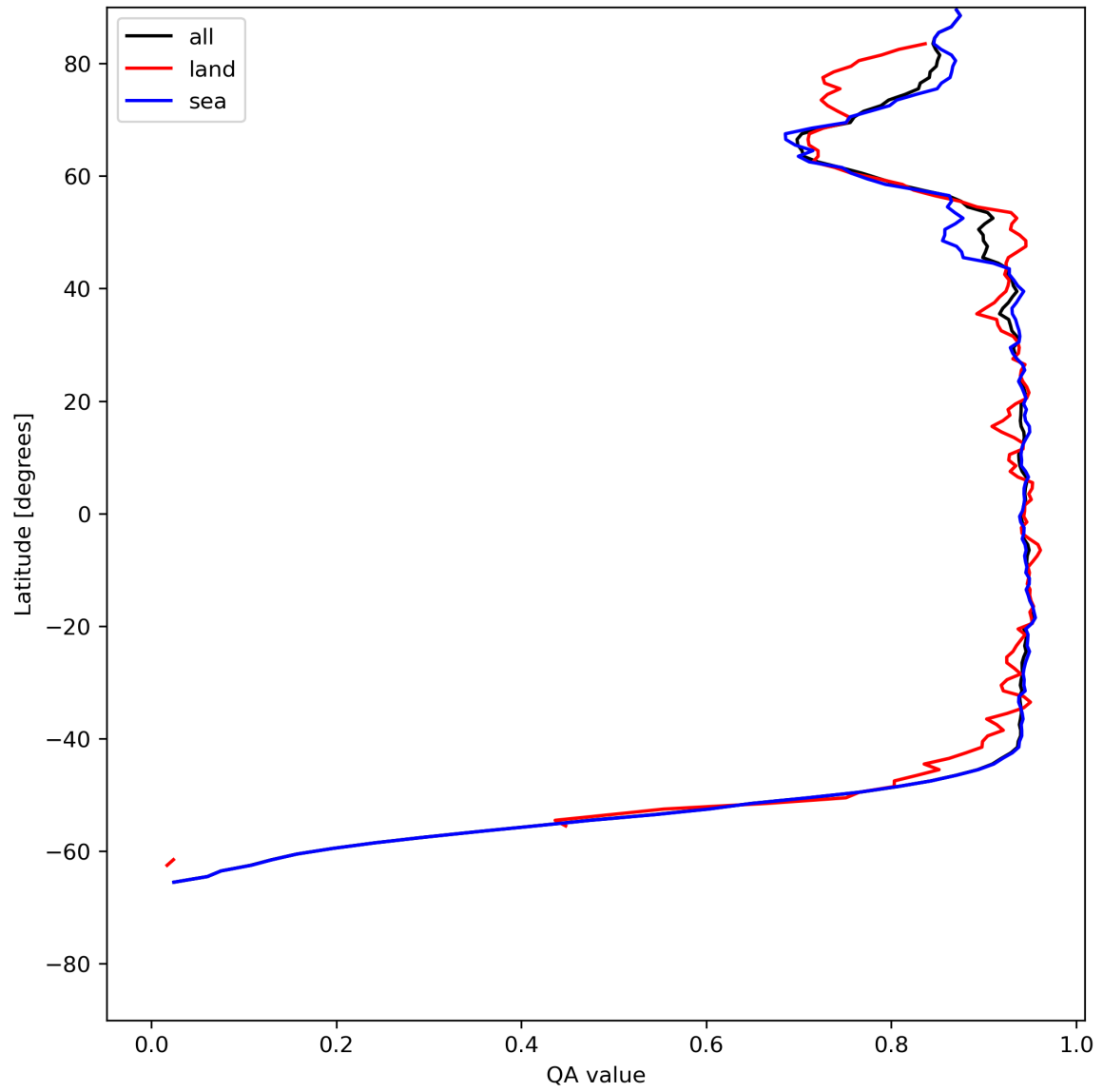
Figure 13: Zonal average of “QA value” for 2024-06-10 to 2024-06-12.
