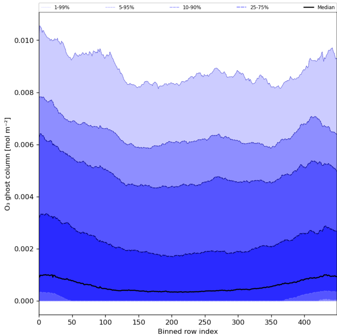
Figure 32: Along track statistics of “O 3 ghost column” for 2024-06-10 to 2024-06-12
