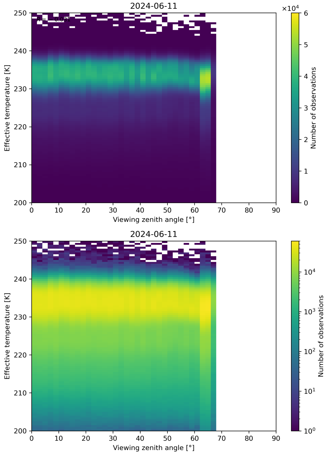
Figure 50: Scatter density plot of “Viewing zenith angle” against “Effective temperature” for 2024-06-10 to 2024-06-12.
