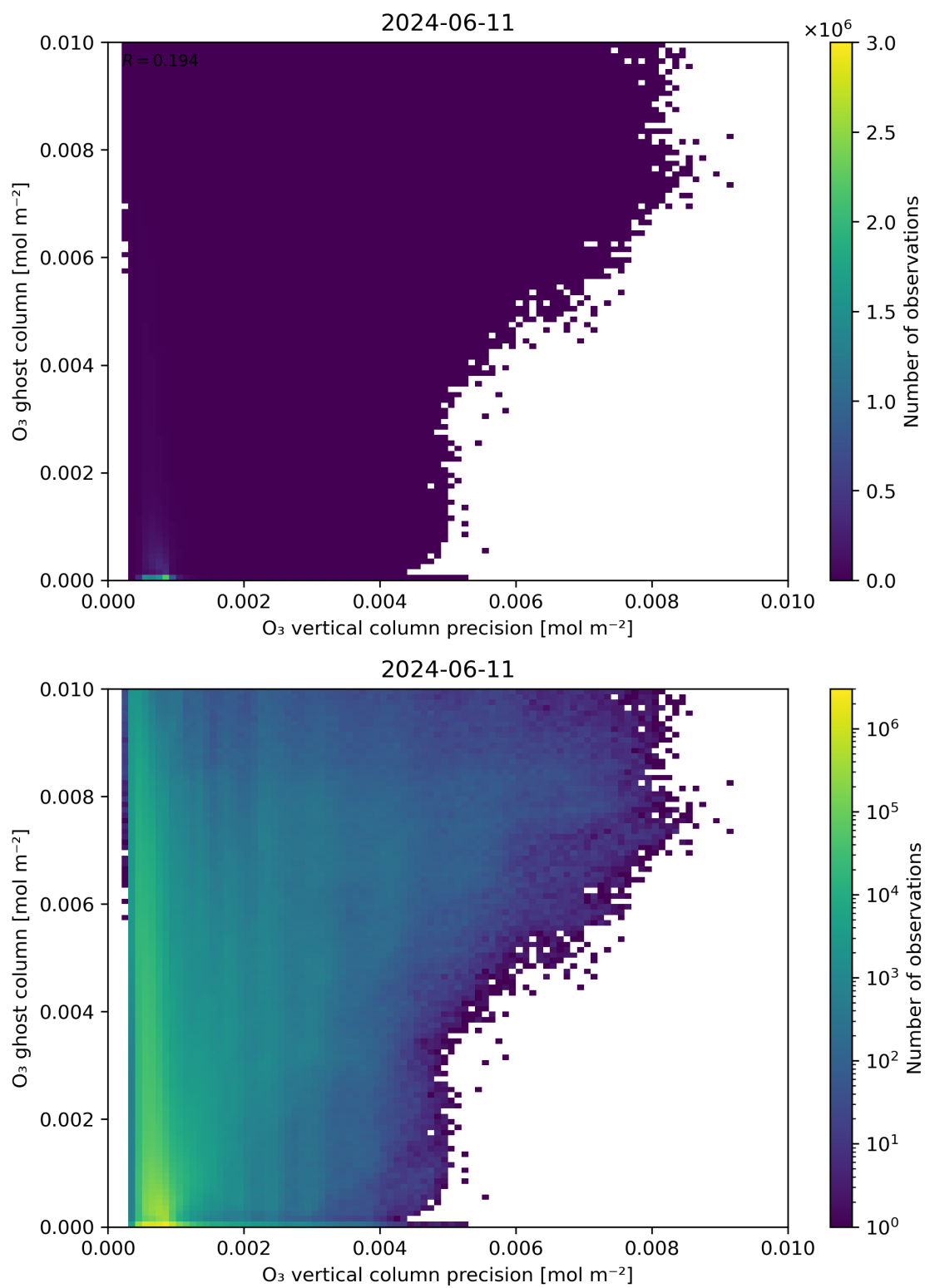
Figure 43: Scatter density plot of “ \text{O}_3 vertical column precision” against “ \text{O}_3 ghost column” for 2024-06-10 to 2024-06-12.
