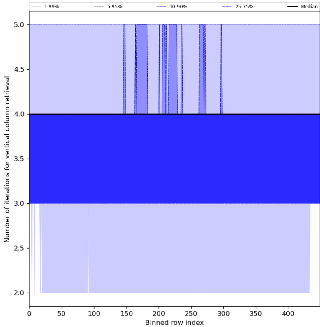
Figure 33: Along track statistics of “Number of iterations for vertical column retrieval” for 2024-06-10 to 2024-06-12
