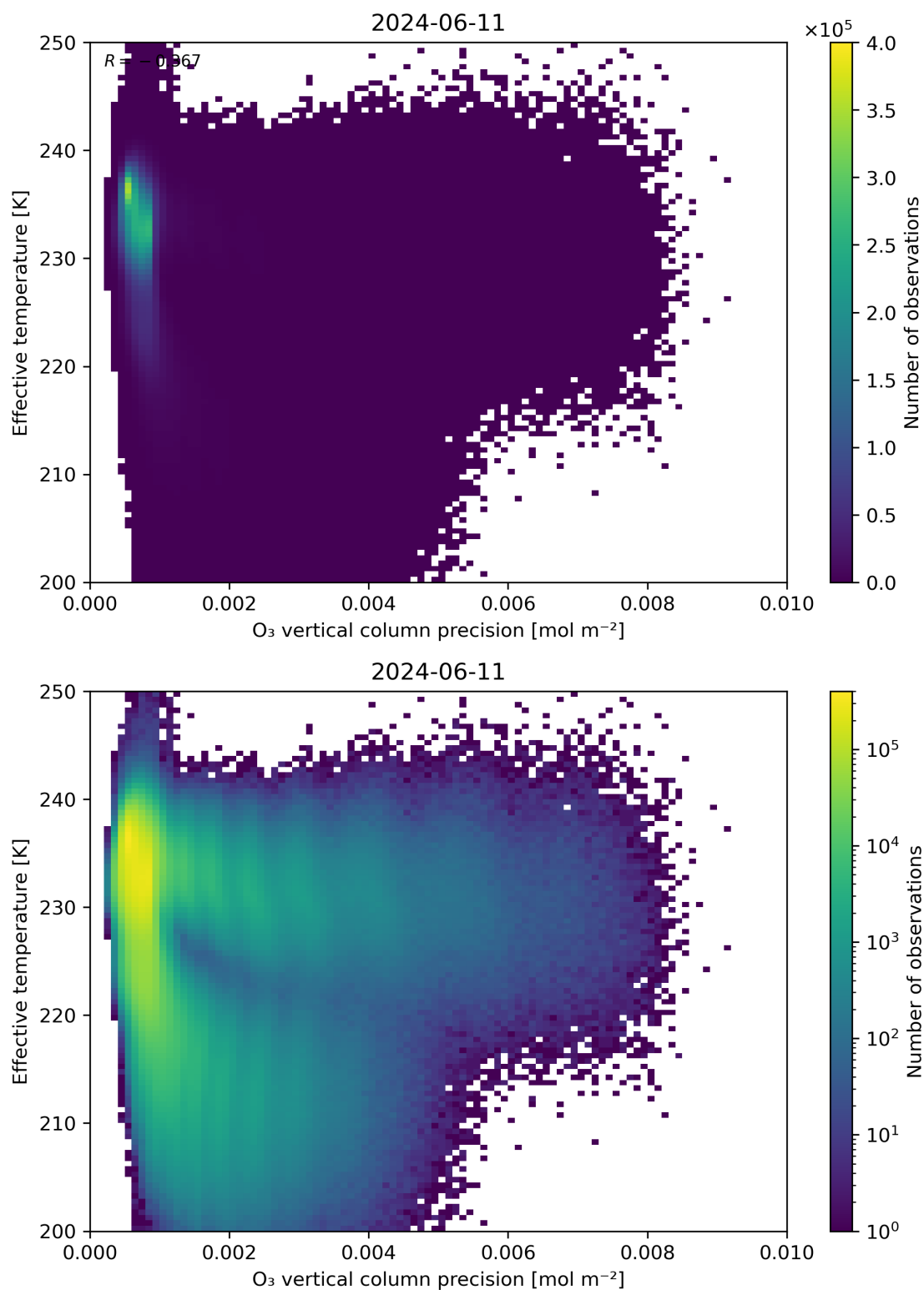
Figure 42: Scatter density plot of “O 3 vertical column precision” against “Effective temperature” for 2024-06-10 to 2024-06-12.
