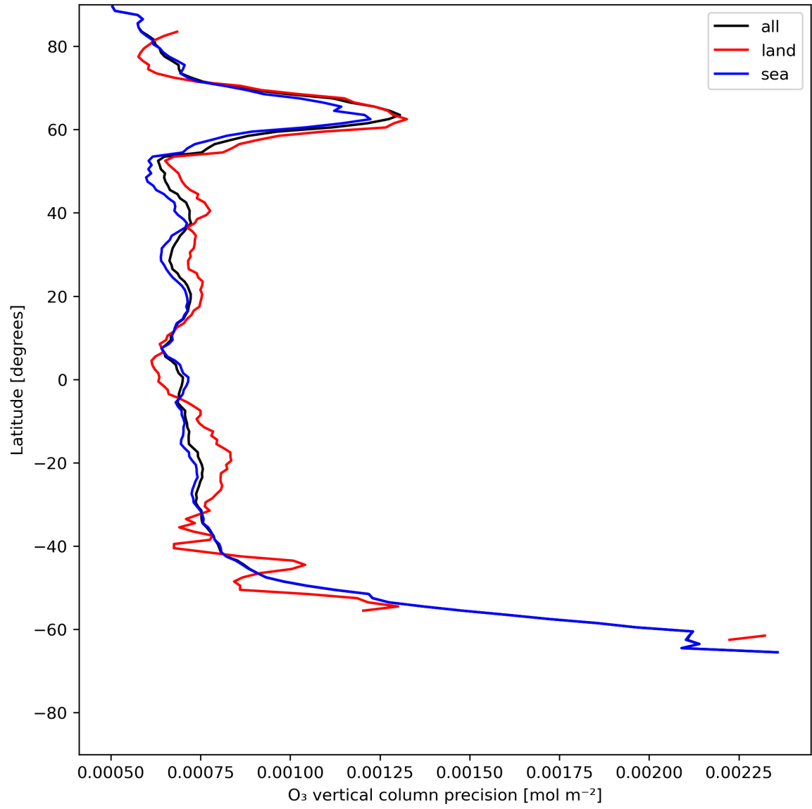
Figure 15: Zonal average of “O 3 vertical column precision” for 2024-06-10 to 2024-06-12.
