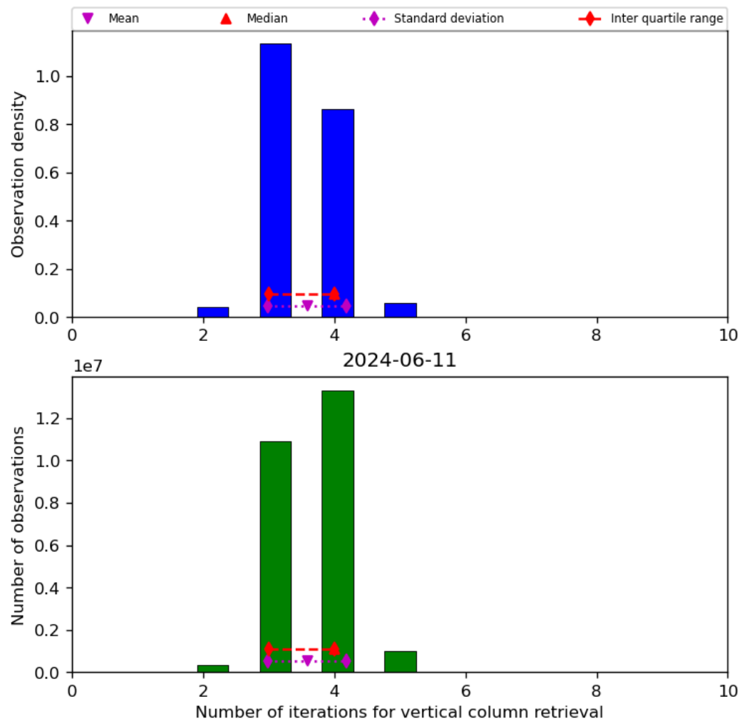
Figure 26: Histogram of “Number of iterations for vertical column retrieval” for 2024-06-10 to 2024-06-12
