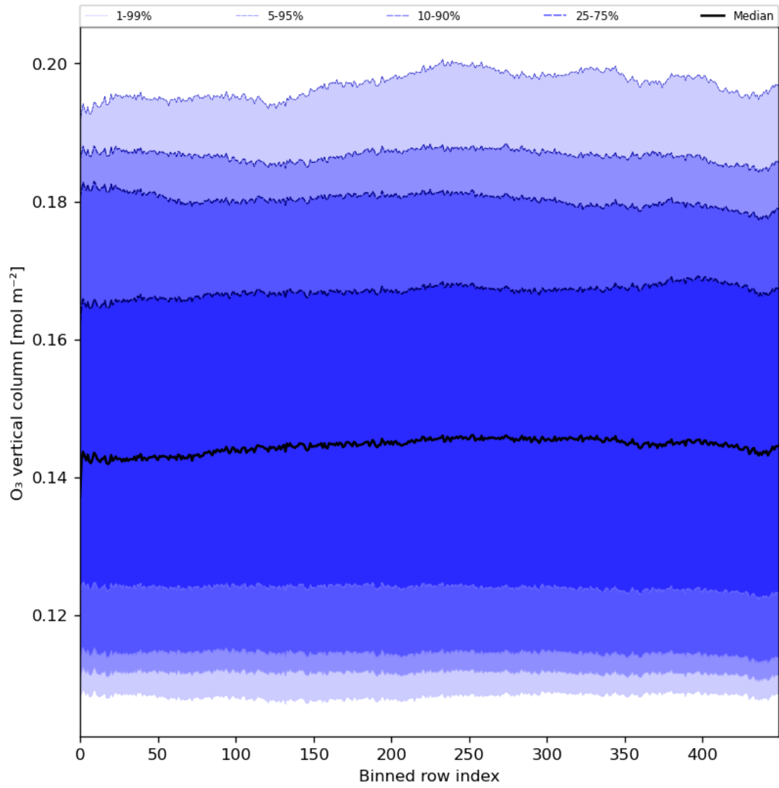
Figure 28: Along track statistics of “O 3 vertical column” for 2024-06-10 to 2024-06-12
