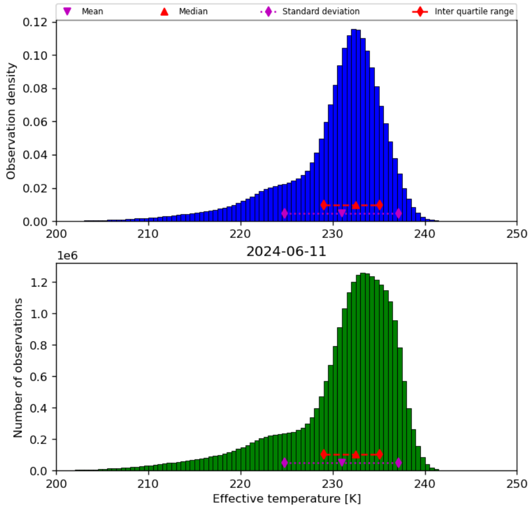
Figure 24: Histogram of “Effective temperature” for 2024-06-10 to 2024-06-12
