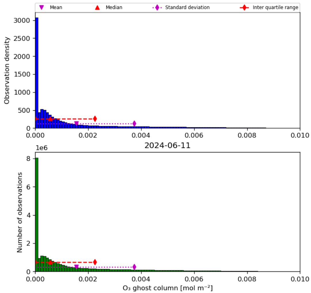
Figure 25: Histogram of “O 3 ghost column” for 2024-06-10 to 2024-06-12
