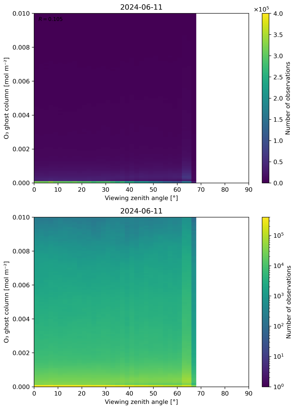
Figure 51: Scatter density plot of “Viewing zenith angle” against “O 3 ghost column” for 2024-06-10 to 2024-06-12.
