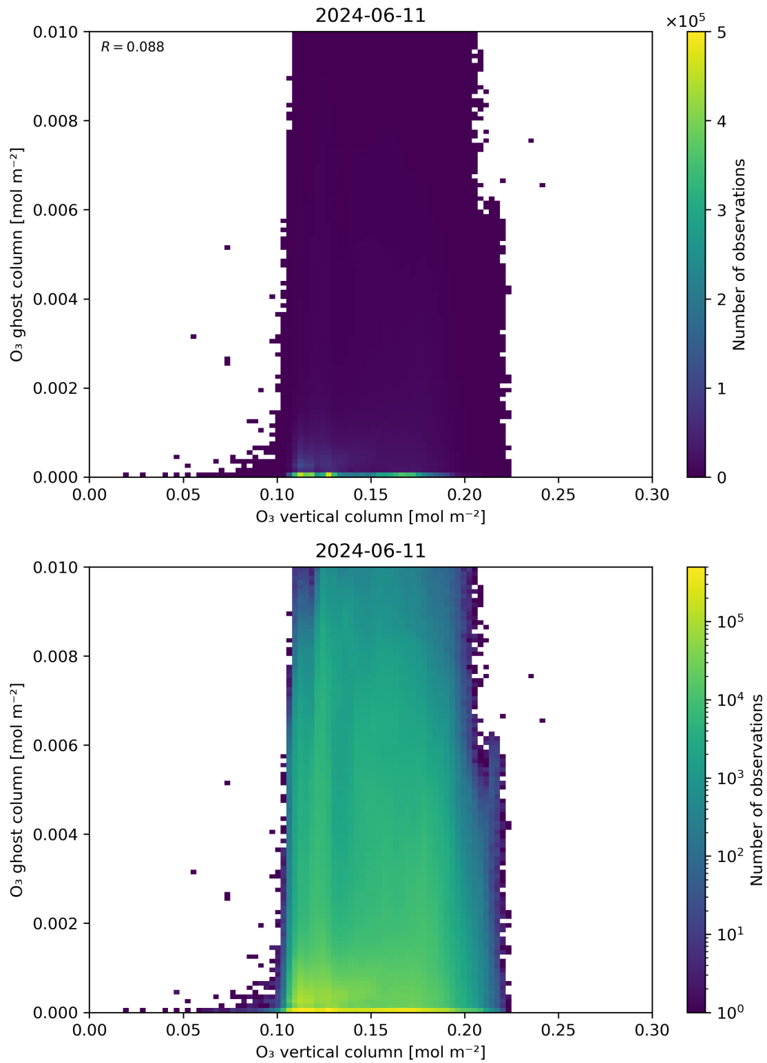
Figure 40: Scatter density plot of “O 3 vertical column” against “O 3 ghost column” for 2024-06-10 to 2024-06-12.
