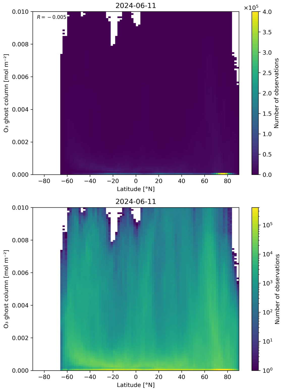
Figure 35: Scatter density plot of “Latitude” against “O 3 ghost column” for 2024-06-10 to 2024-06-12.
