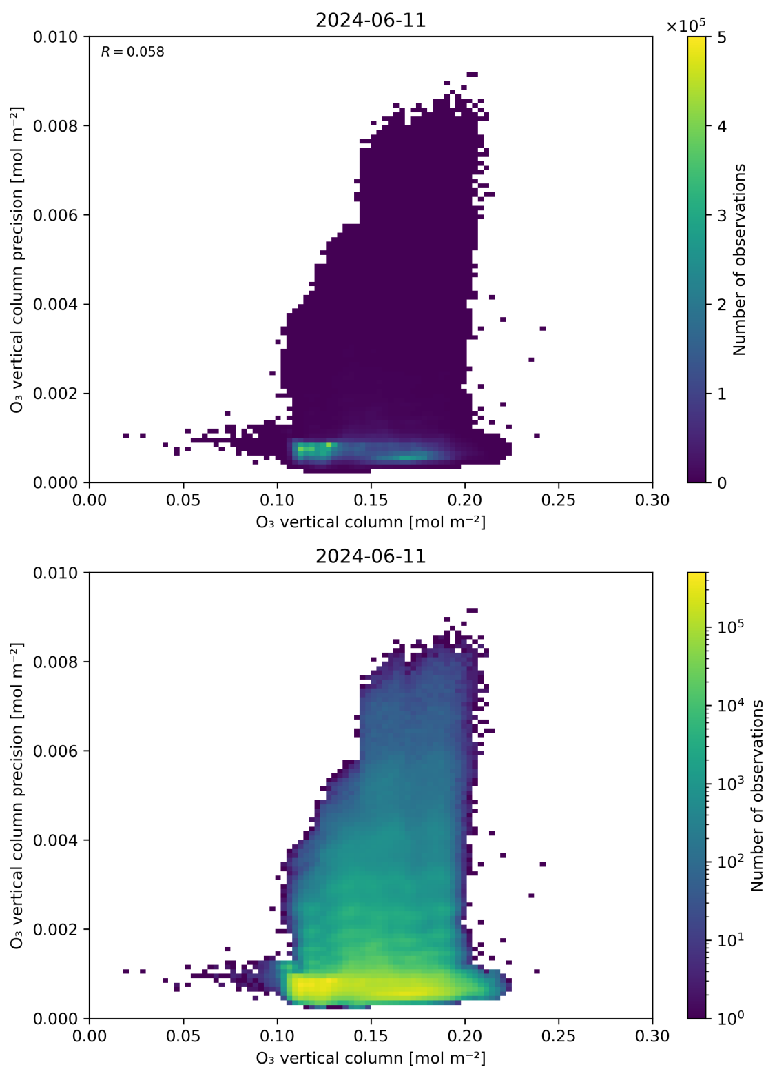
Figure 41: Scatter density plot of “O 3 vertical column” against “O 3 vertical column precision” for 2024-06-10 to 2024-06-12.
