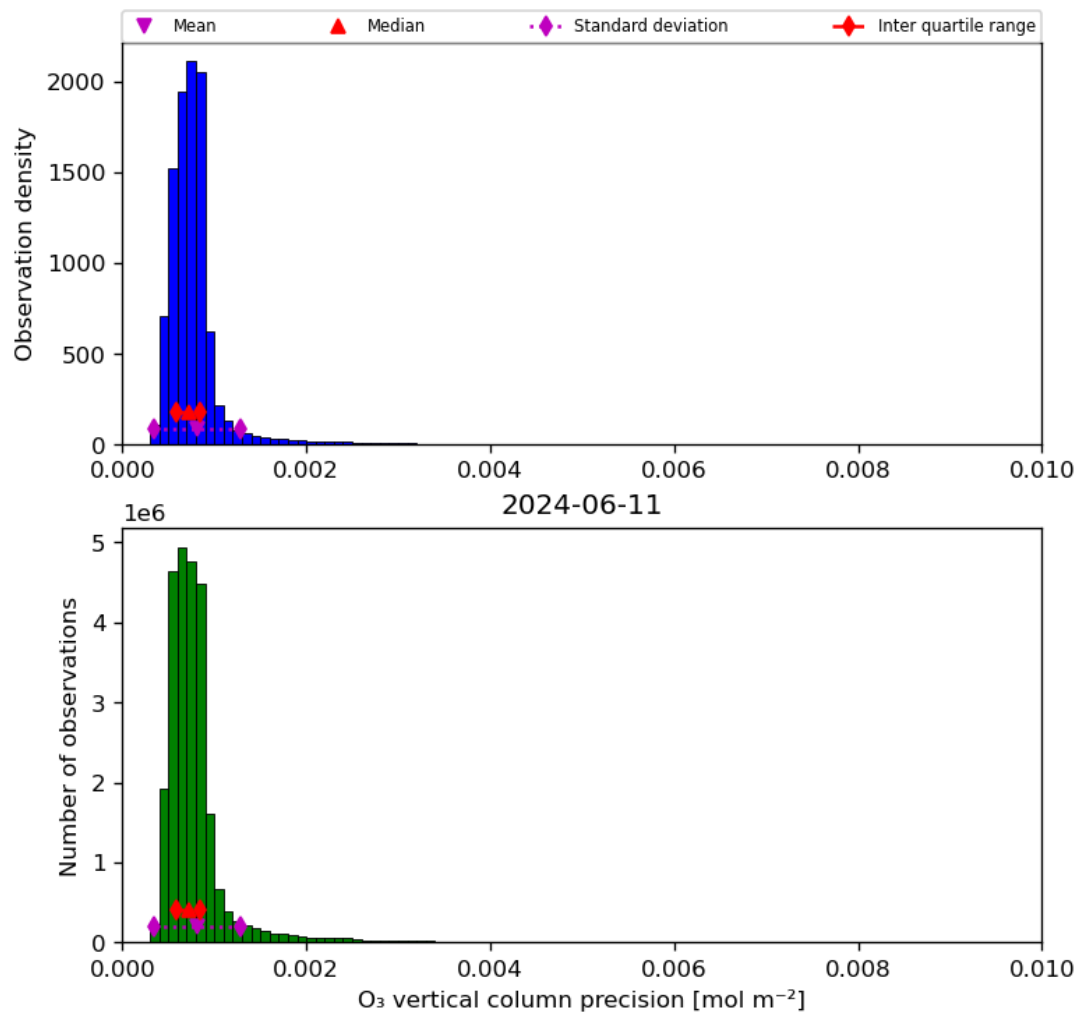
Figure 22: Histogram of “O 3 vertical column precision” for 2024-06-10 to 2024-06-12
