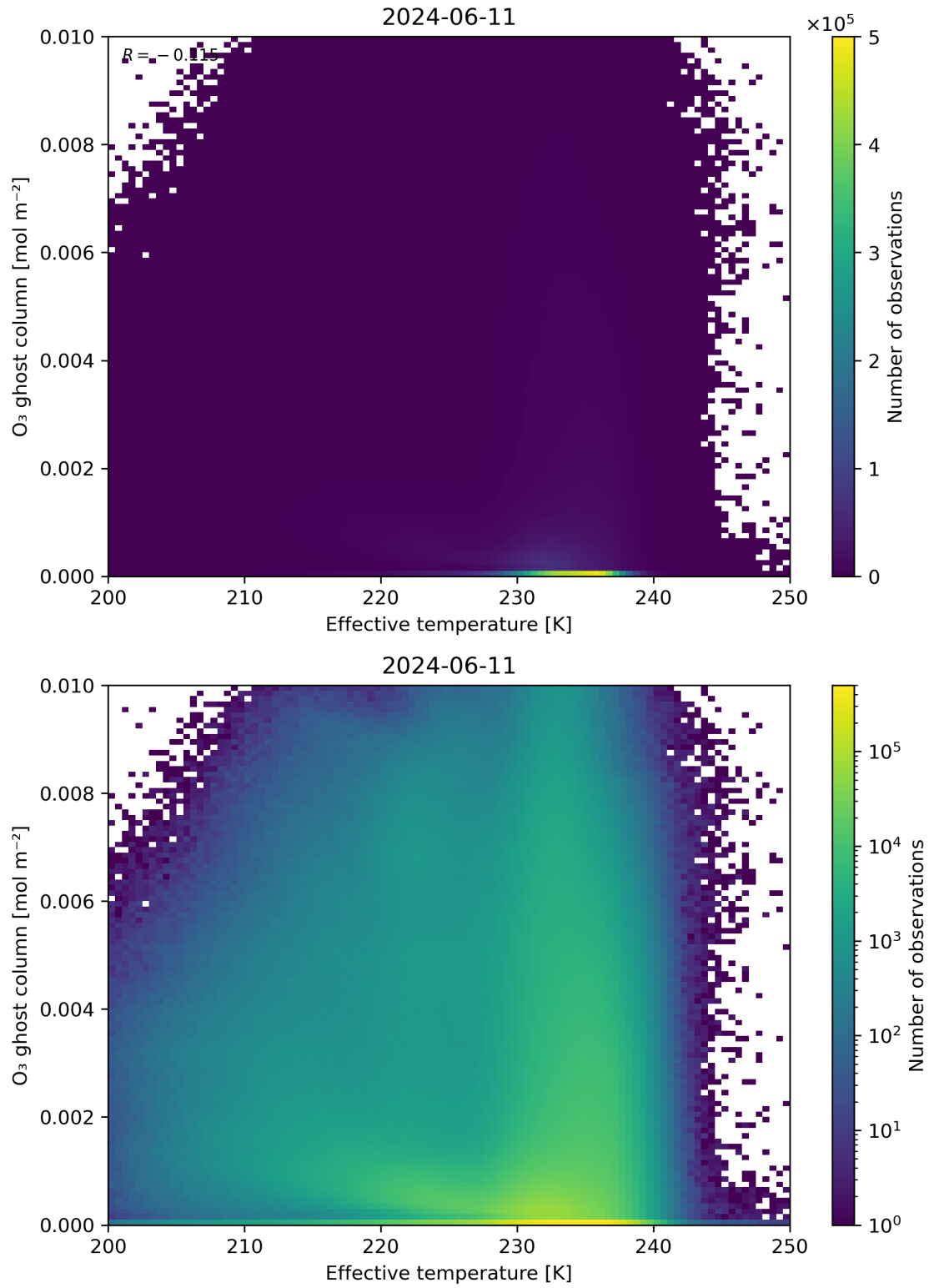
Figure 38: Scatter density plot of “Effective temperature” against “O 3 ghost column” for 2024-06-10 to 2024-06-12.
