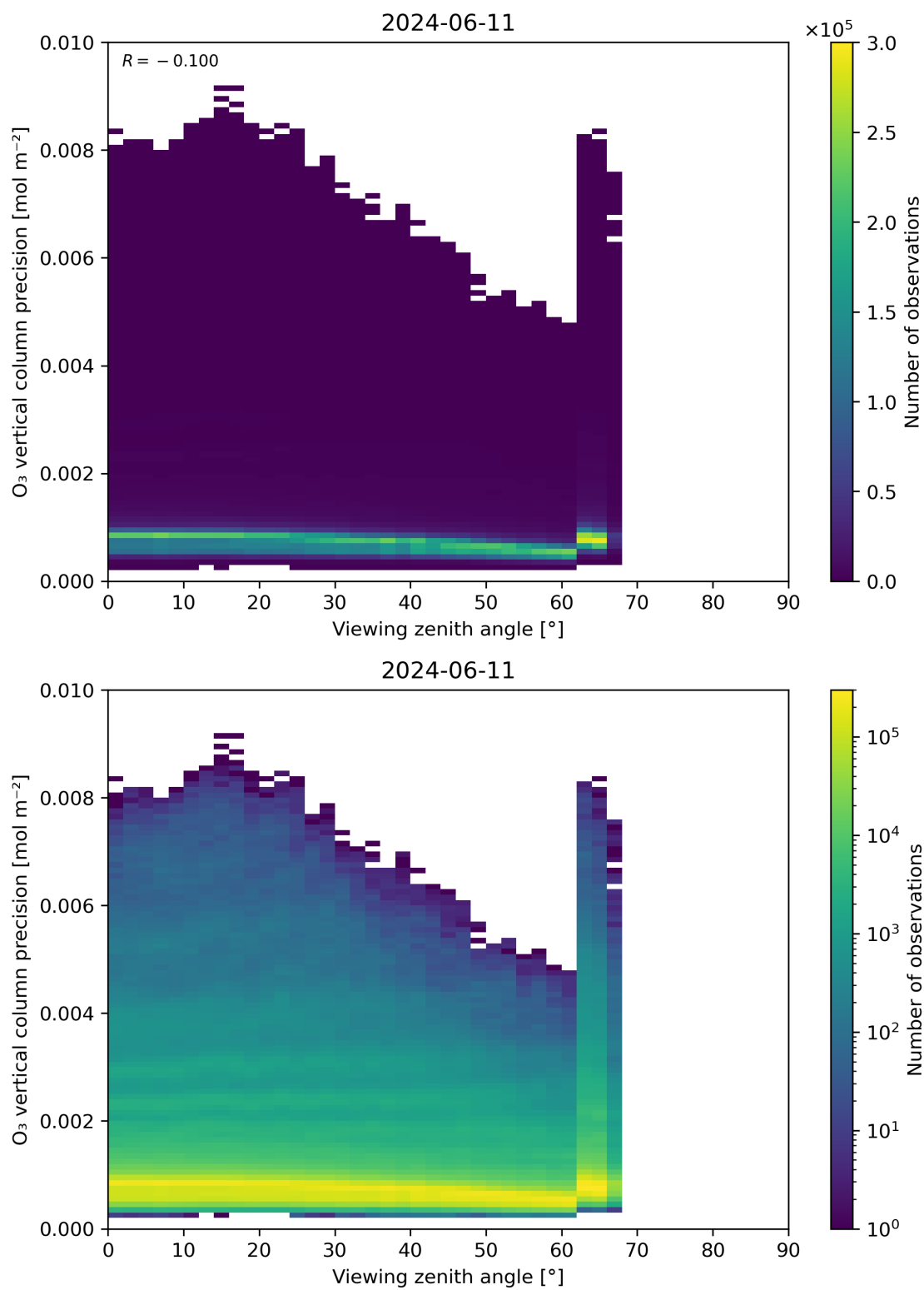
Figure 53: Scatter density plot of “Viewing zenith angle” against “O 3 vertical column precision” for 2024-06-10 to 2024-06-12.
