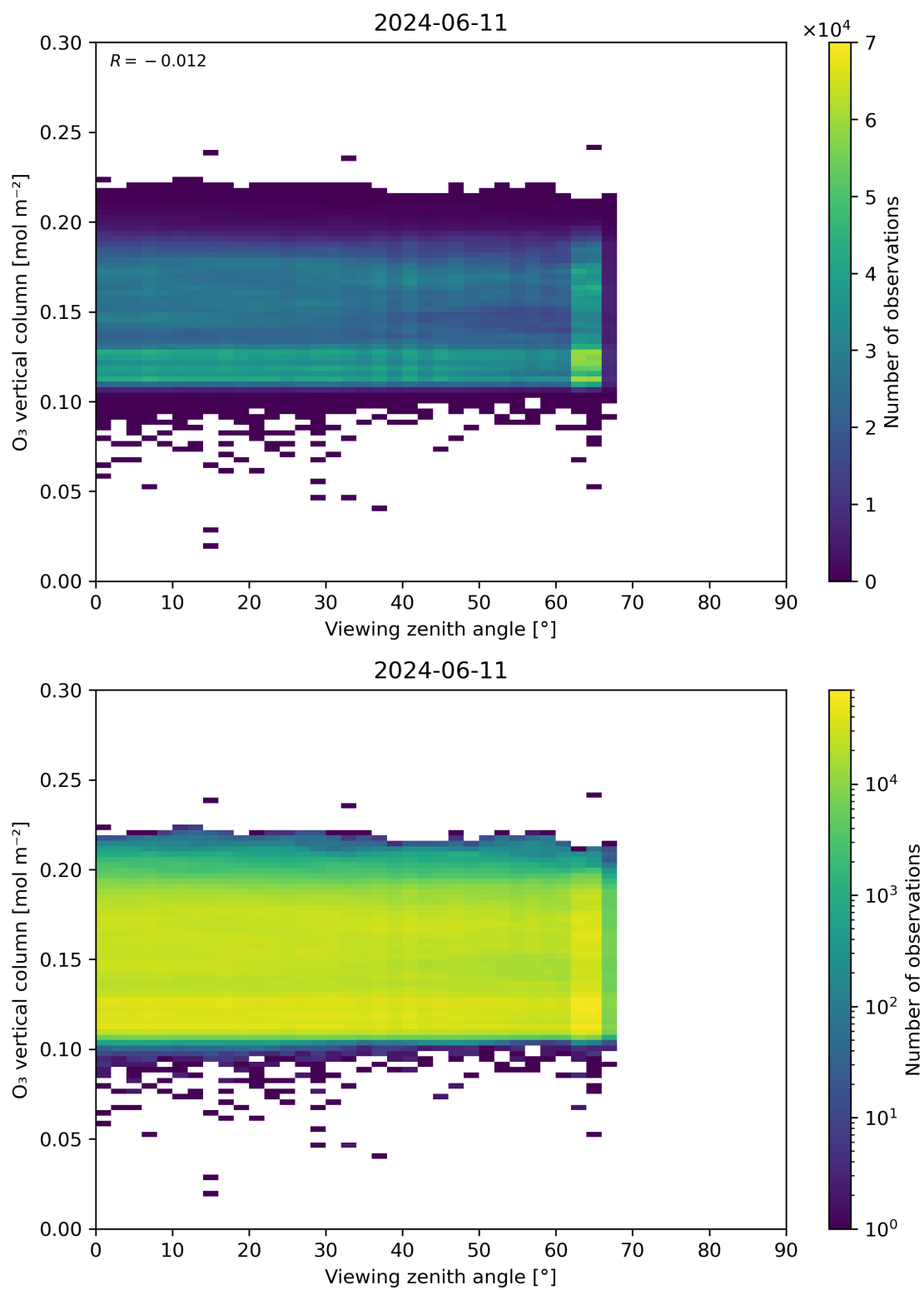
Figure 52: Scatter density plot of “Viewing zenith angle” against “O 3 vertical column” for 2024-06-10 to 2024-06-12.
