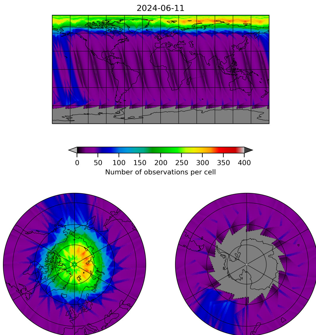
Figure 12: Map of the number of observations for 2024-06-10 to 2024-06-12
