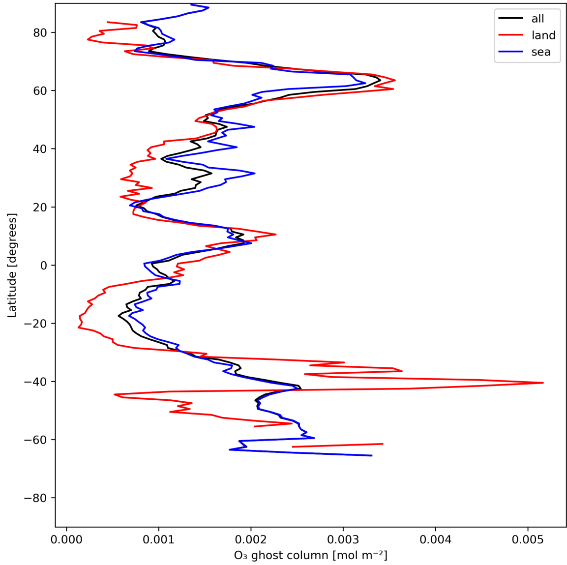
Figure 18: Zonal average of "O 3 ghost column" for 2024-06-10 to 2024-06-12.
