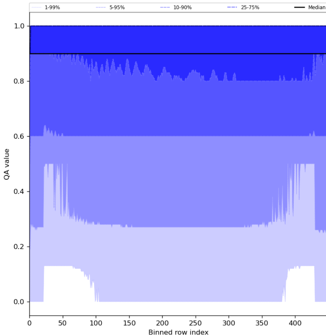
Figure 27: Along track statistics of “QA value” for 2024-06-10 to 2024-06-12
