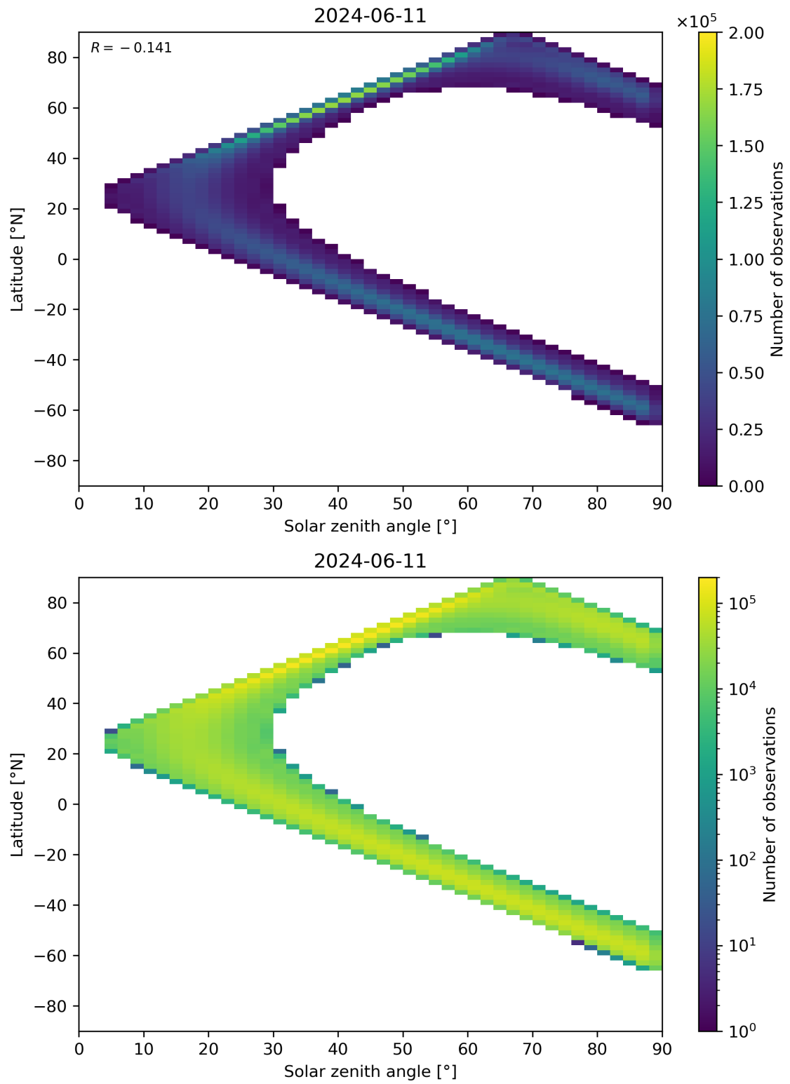
Figure 44: Scatter density plot of “Solar zenith angle” against “Latitude” for 2024-06-10 to 2024-06-12.
