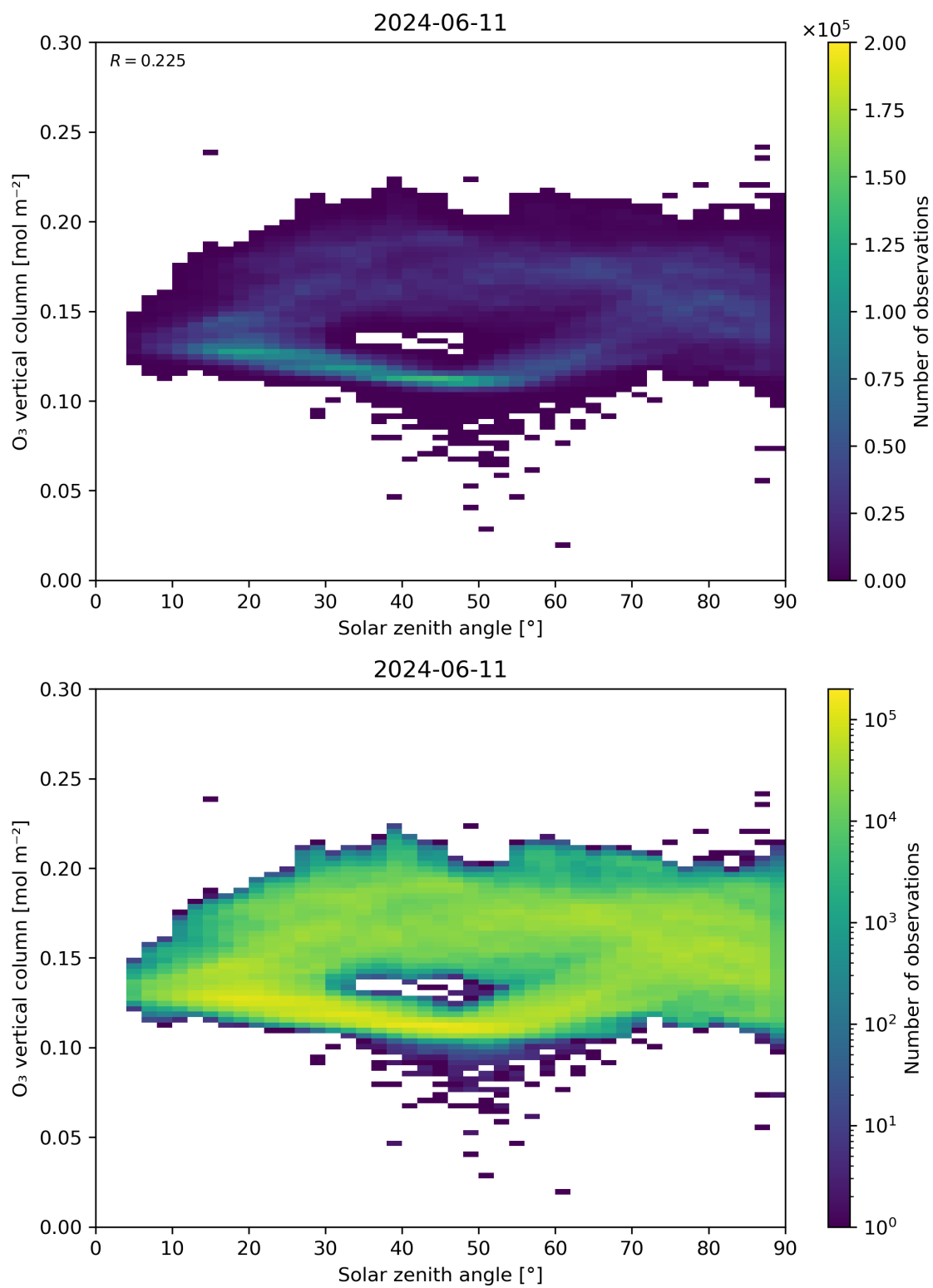
Figure 47: Scatter density plot of “Solar zenith angle” against “O 3 vertical column” for 2024-06-10 to 2024-06-12.
