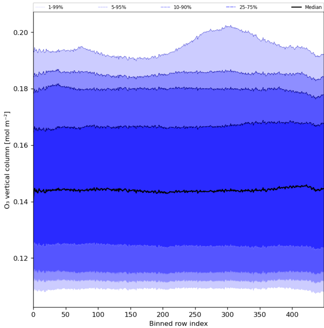
Figure 28: Along track statistics of “O 3 vertical column” for 2024-06-13 to 2024-06-14
