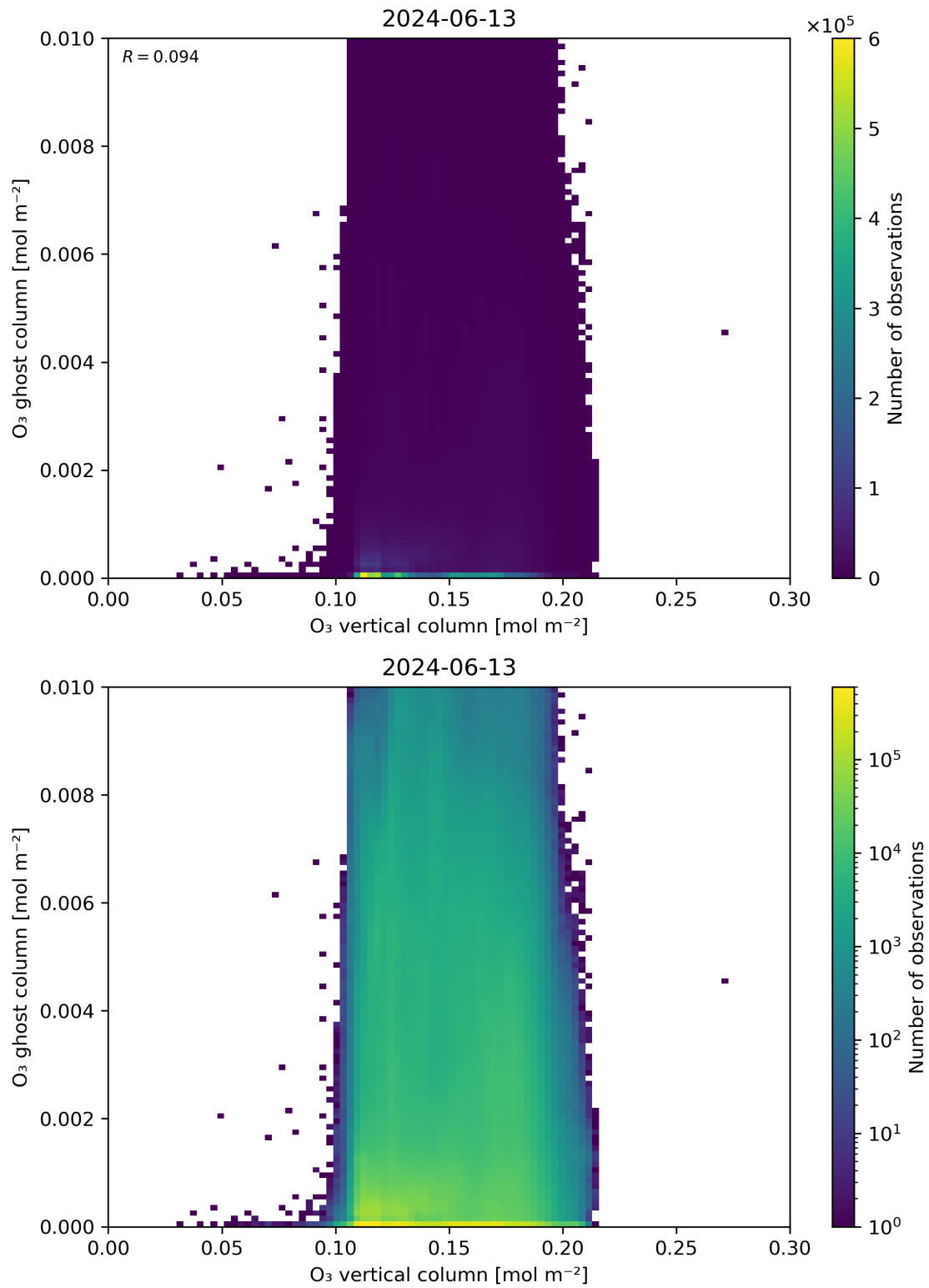
Figure 40: Scatter density plot of “O 3 vertical column” against “O 3 ghost column” for 2024-06-13 to 2024-06-14.
