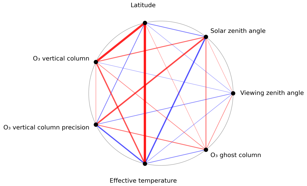
Figure 1: Map of correlation graph for 2024-06-13 to 2024-06-14.
