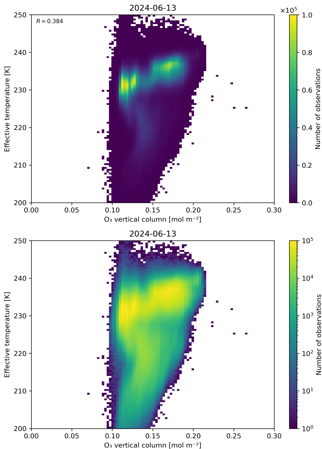
Figure 39: Scatter density plot of “O 3 vertical column” against “Effective temperature” for 2024-06-13 to 2024-06-14.
