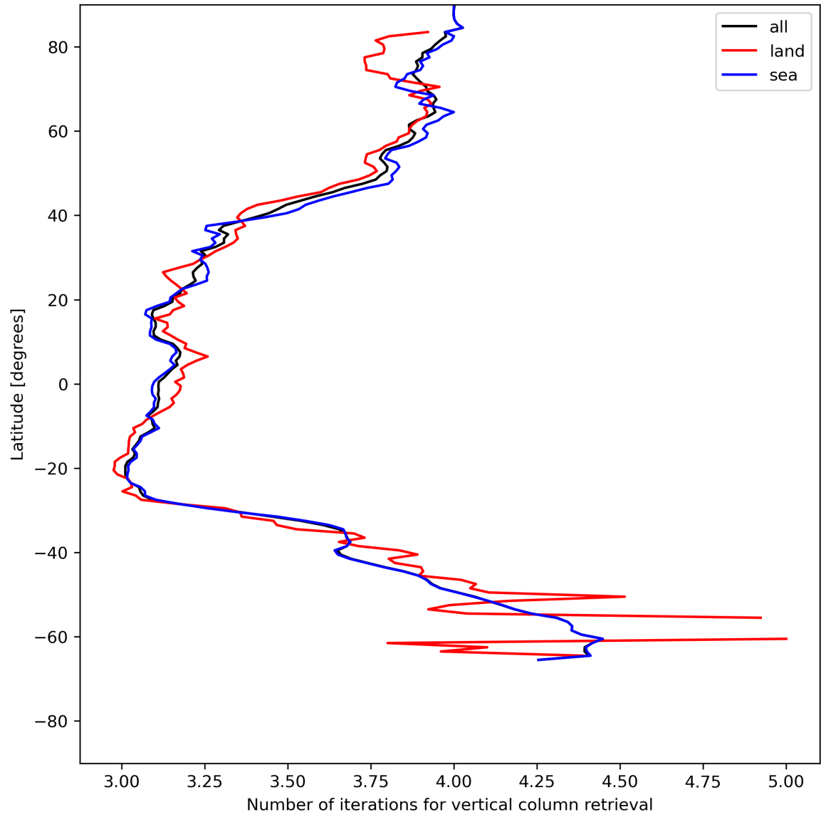
Figure 19: Zonal average of “Number of iterations for vertical column retrieval” for 2024-06-13 to 2024-06-14.
