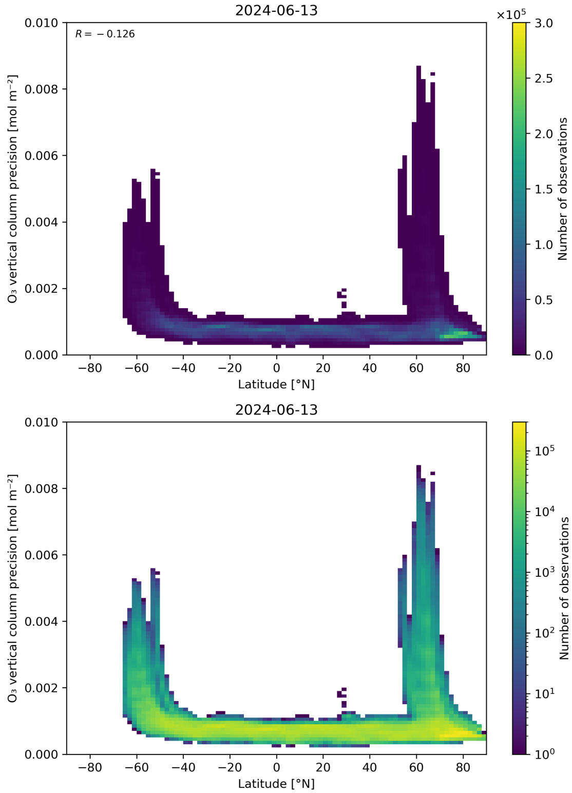
Figure 37: Scatter density plot of “Latitude” against “O 3 vertical column precision” for 2024-06-13 to 2024-06-14.
