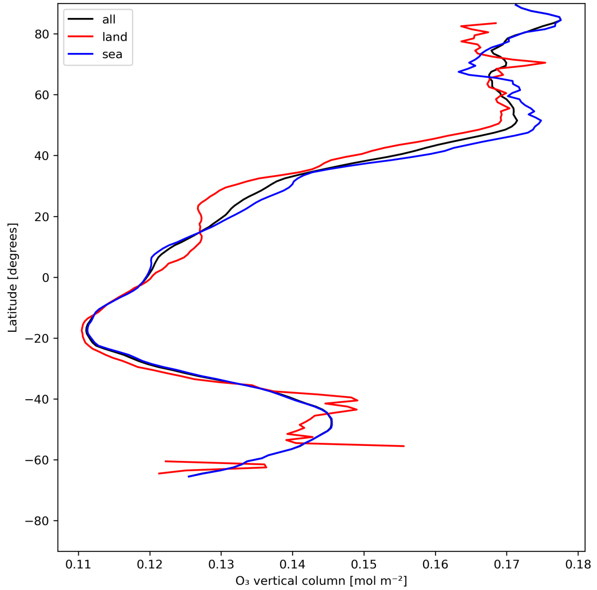
Figure 14: Zonal average of “O 3 vertical column” for 2024-06-13 to 2024-06-14.
