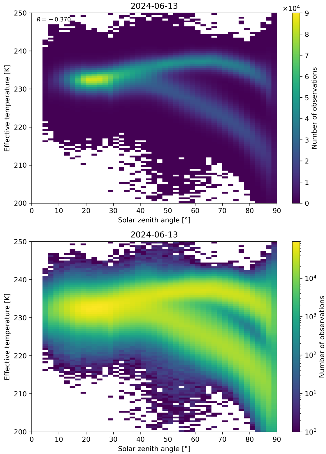
Figure 45: Scatter density plot of “Solar zenith angle” against “Effective temperature” for 2024-06-13 to 2024-06-14.
