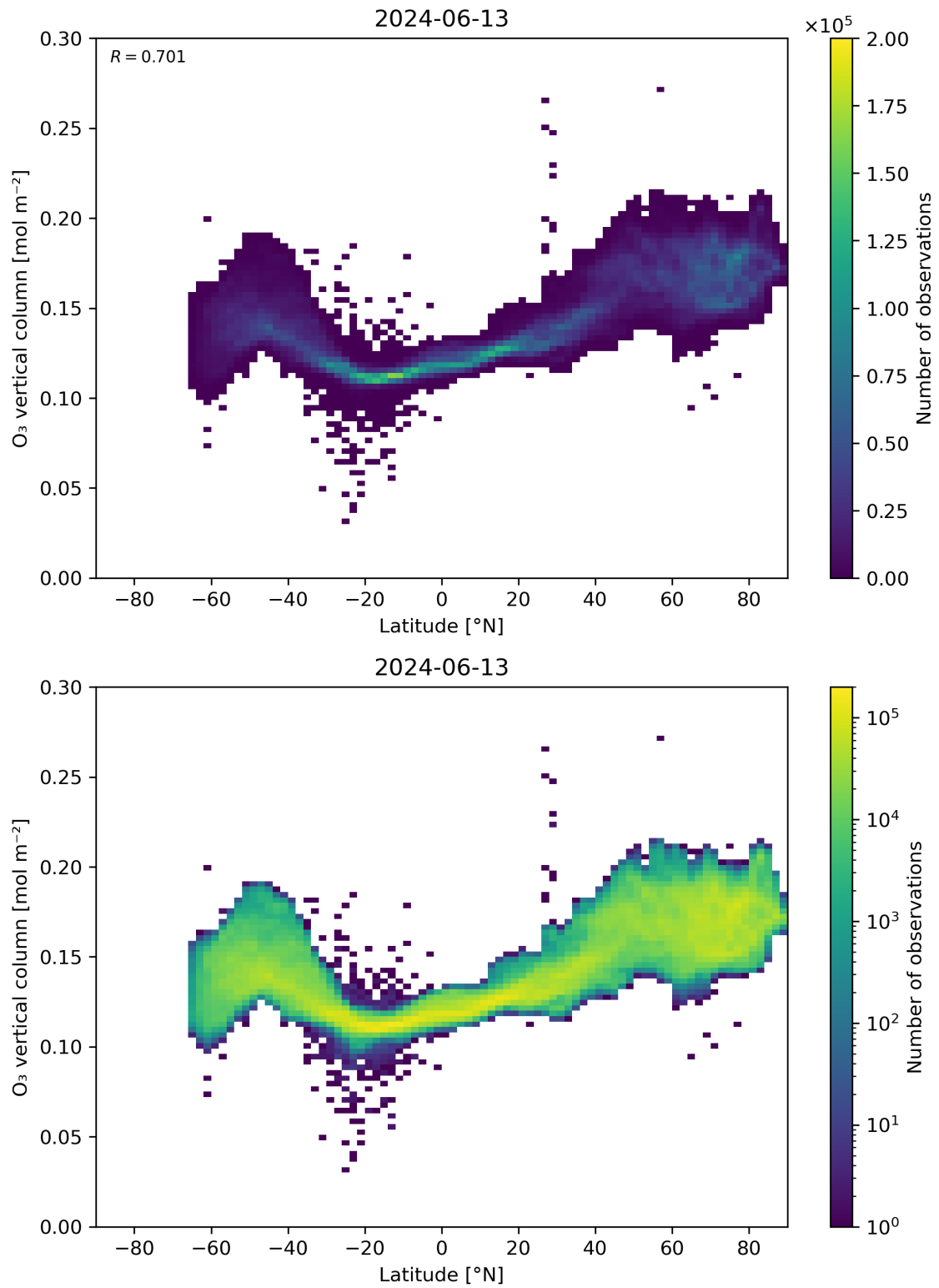
Figure 36: Scatter density plot of “Latitude” against “O 3 vertical column” for 2024-06-13 to 2024-06-14.
