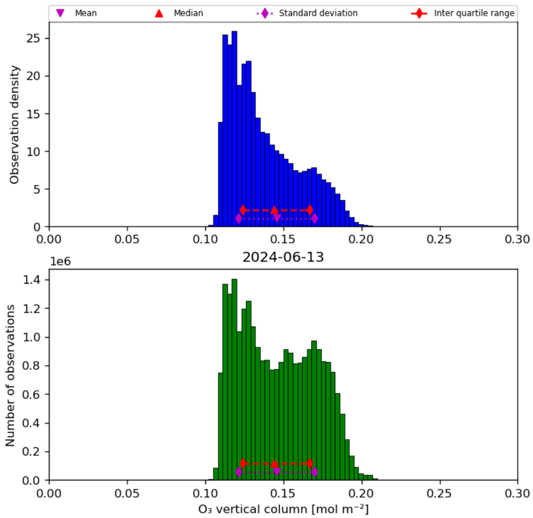
Figure 21: Histogram of “O 3 vertical column” for 2024-06-13 to 2024-06-14
