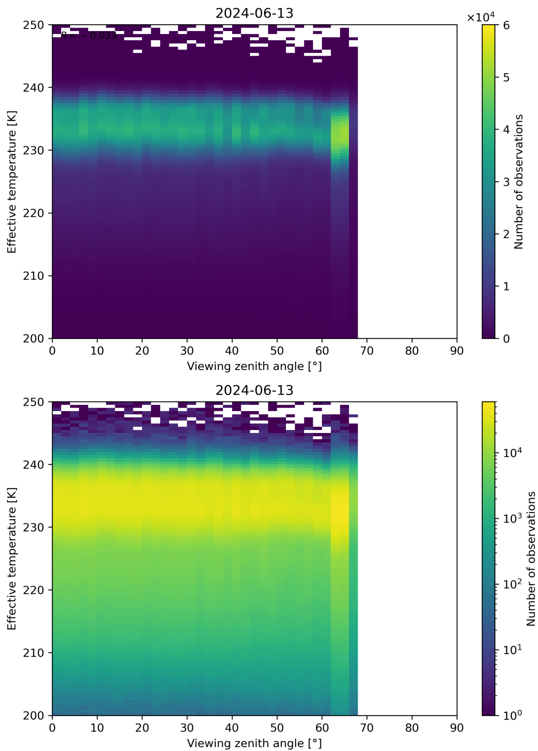
Figure 50: Scatter density plot of “Viewing zenith angle” against “Effective temperature” for 2024-06-13 to 2024-06-14.
