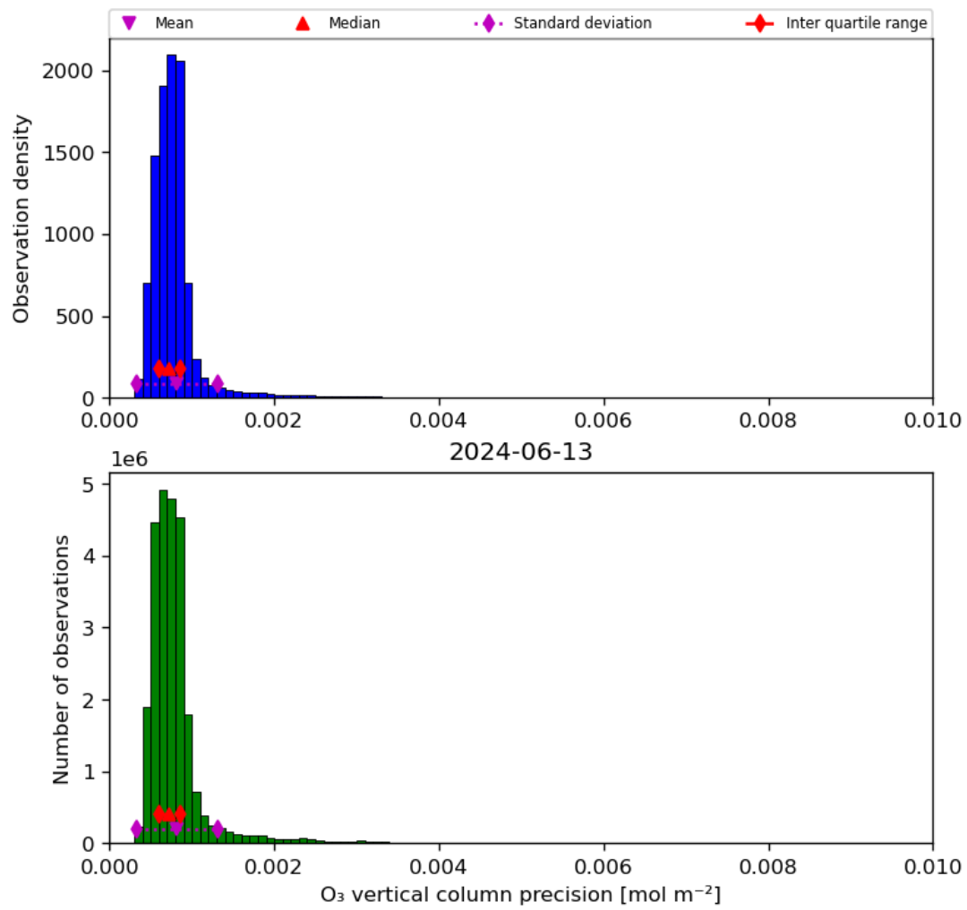
Figure 22: Histogram of “O 3 vertical column precision” for 2024-06-13 to 2024-06-14
