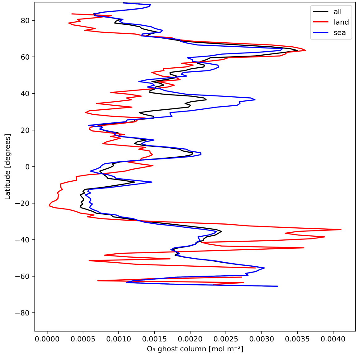
Figure 18: Zonal average of "O 3 ghost column" for 2024-06-13 to 2024-06-14.
