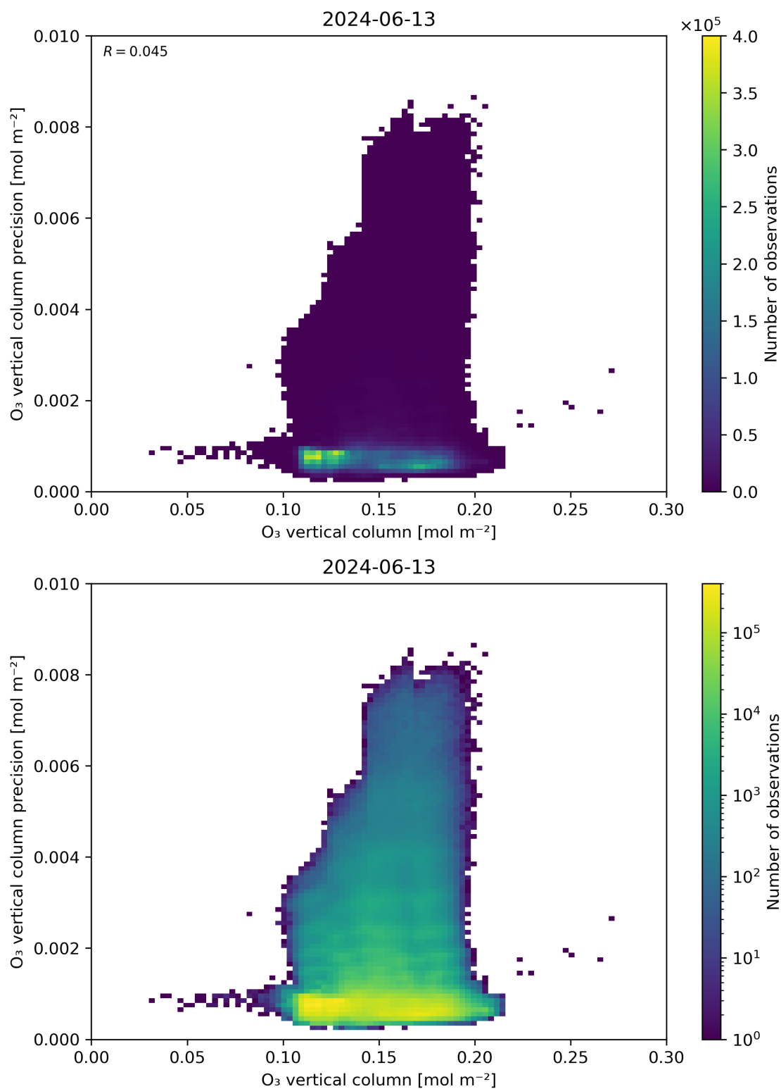
Figure 41: Scatter density plot of “O 3 vertical column” against “O 3 vertical column precision” for 2024-06-13 to 2024-06-14.
