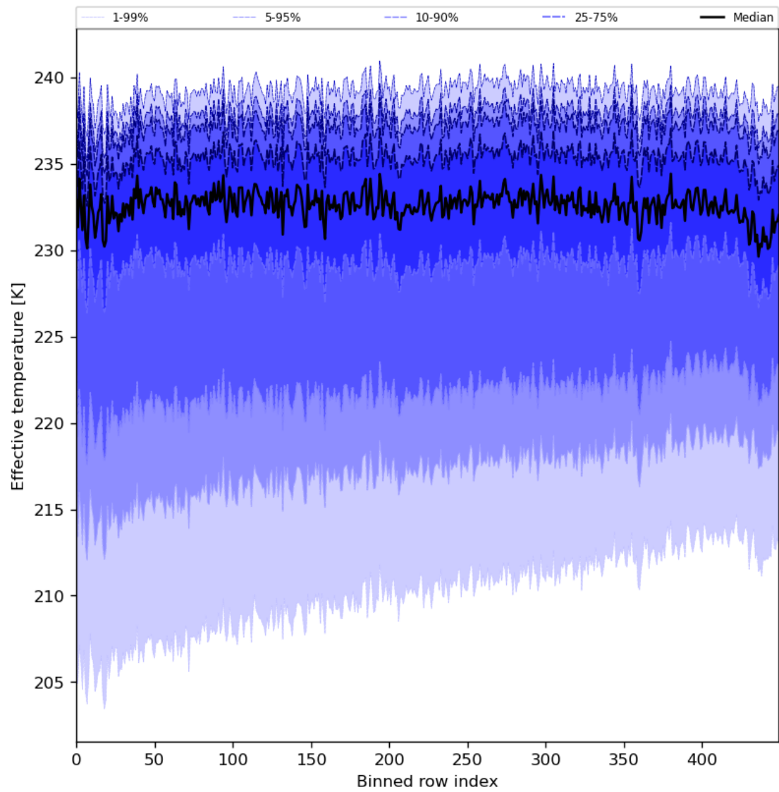
Figure 31: Along track statistics of “Effective temperature” for 2024-06-13 to 2024-06-14
