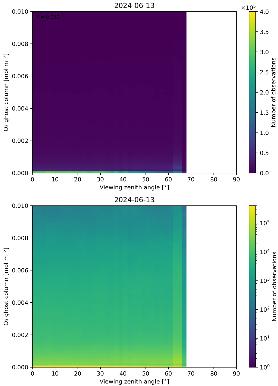
Figure 51: Scatter density plot of “Viewing zenith angle” against “O 3 ghost column” for 2024-06-13 to 2024-06-14.
