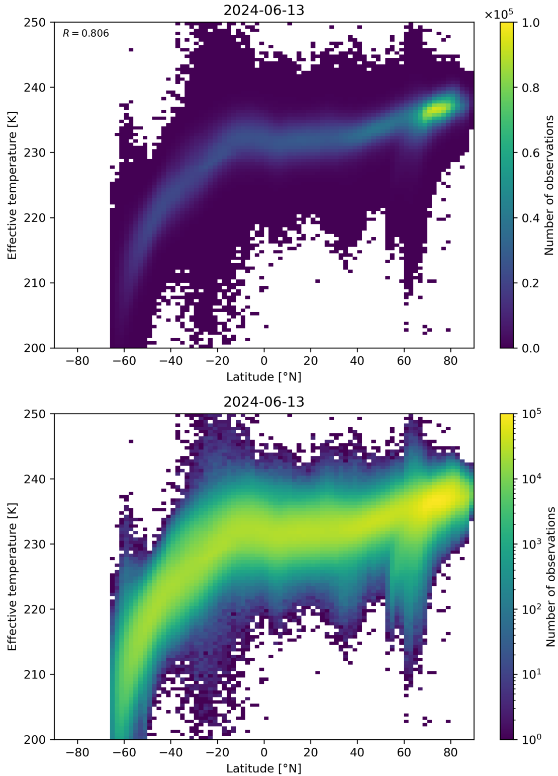
Figure 34: Scatter density plot of “Latitude” against “Effective temperature” for 2024-06-13 to 2024-06-14.
