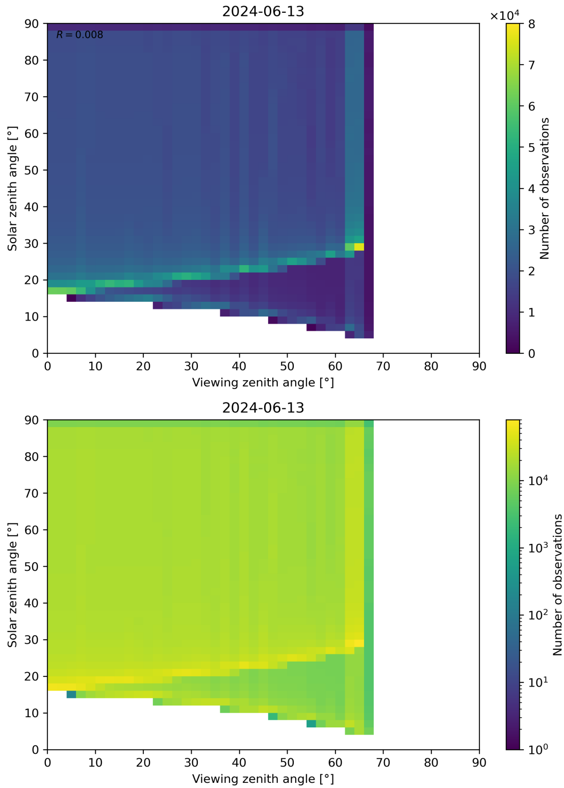
Figure 54: Scatter density plot of “Viewing zenith angle” against “Solar zenith angle” for 2024-06-13 to 2024-06-14.
