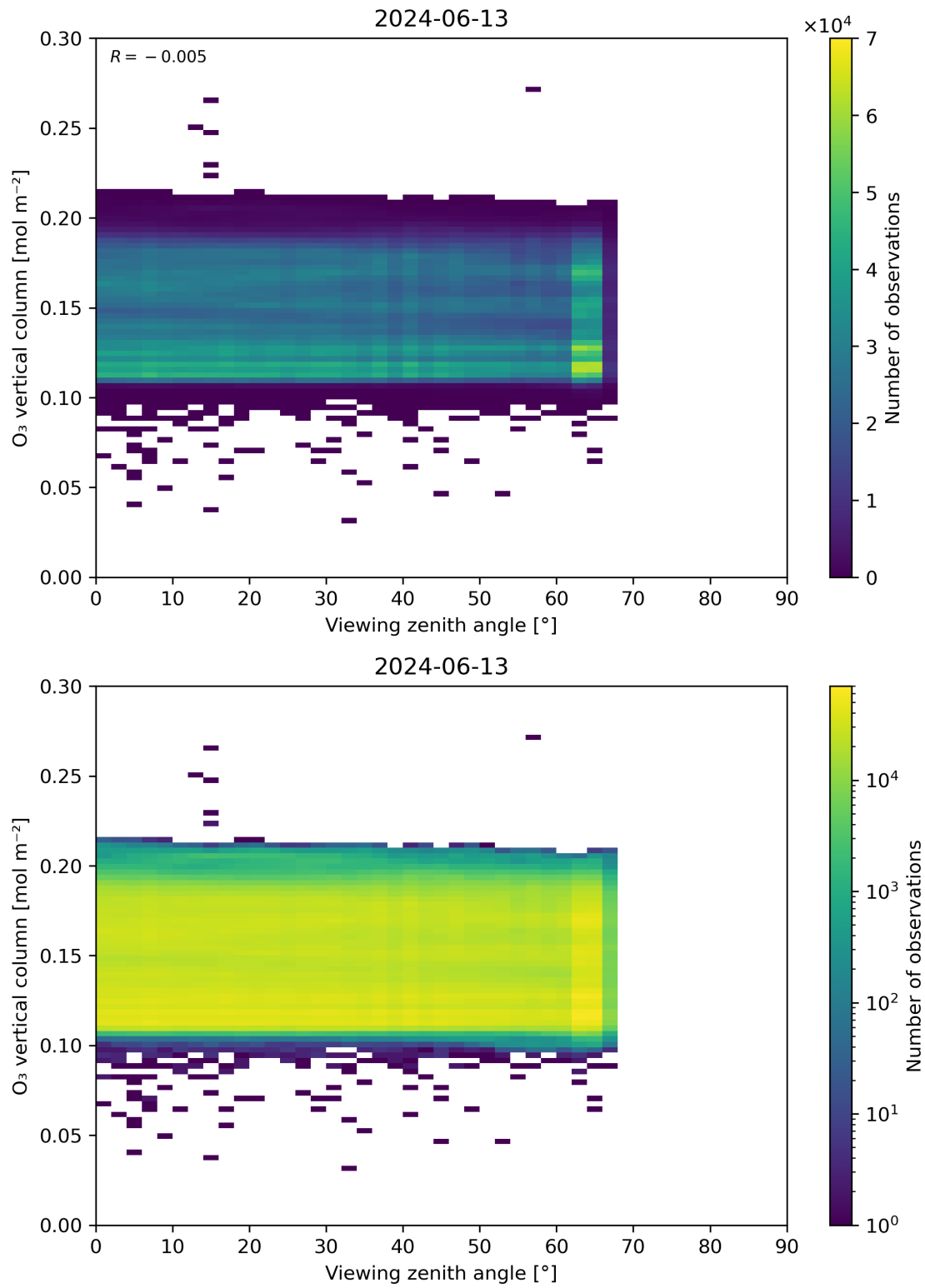
Figure 52: Scatter density plot of “Viewing zenith angle” against “O 3 vertical column” for 2024-06-13 to 2024-06-14.
