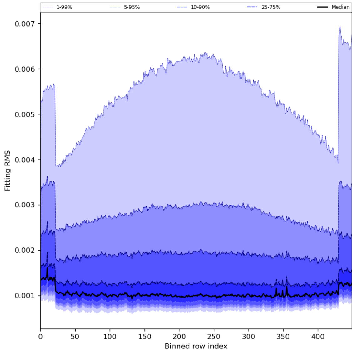
Figure 30: Along track statistics of “Fitting RMS” for 2024-06-13 to 2024-06-14
