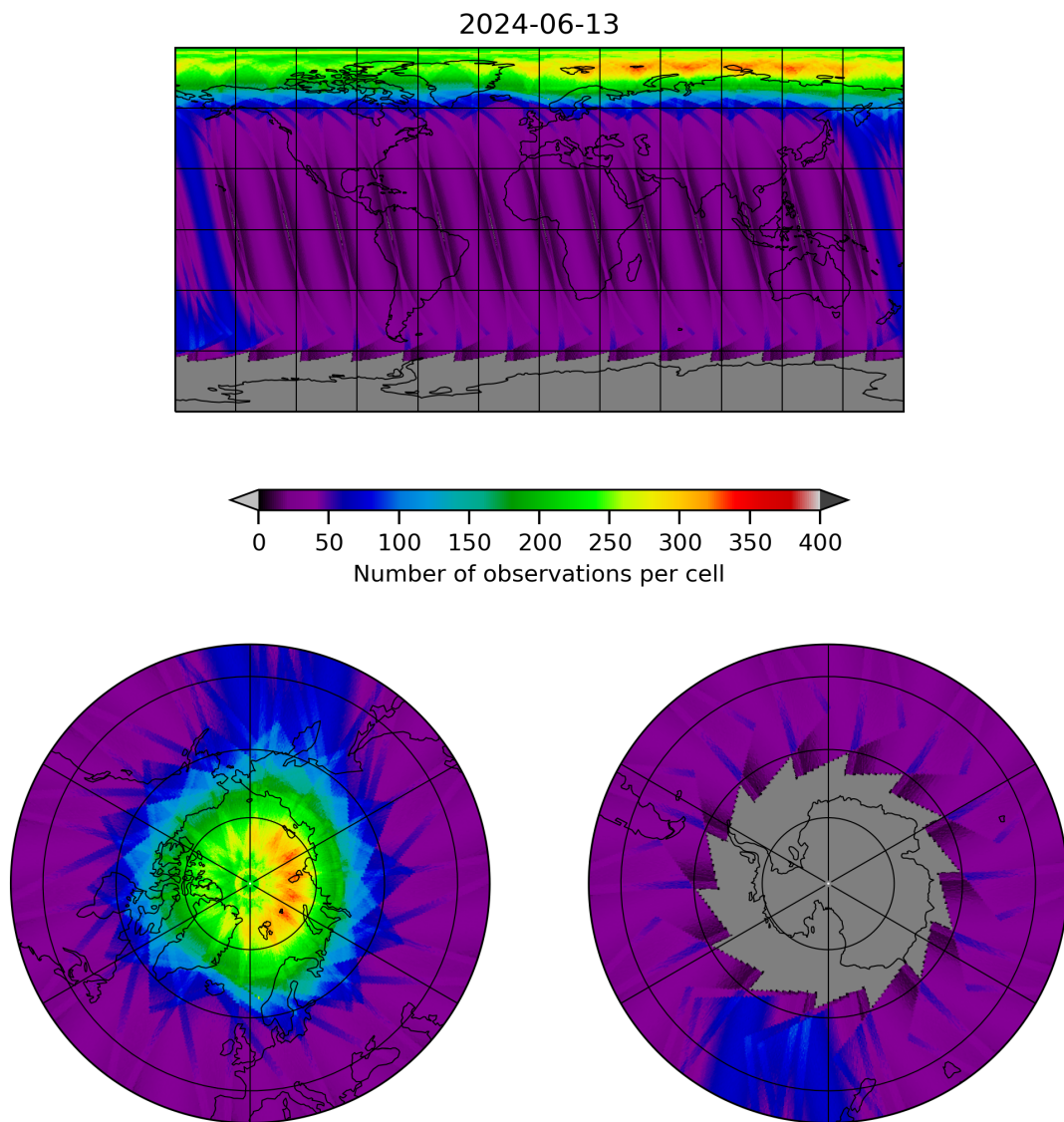
Figure 12: Map of the number of observations for 2024-06-13 to 2024-06-14
