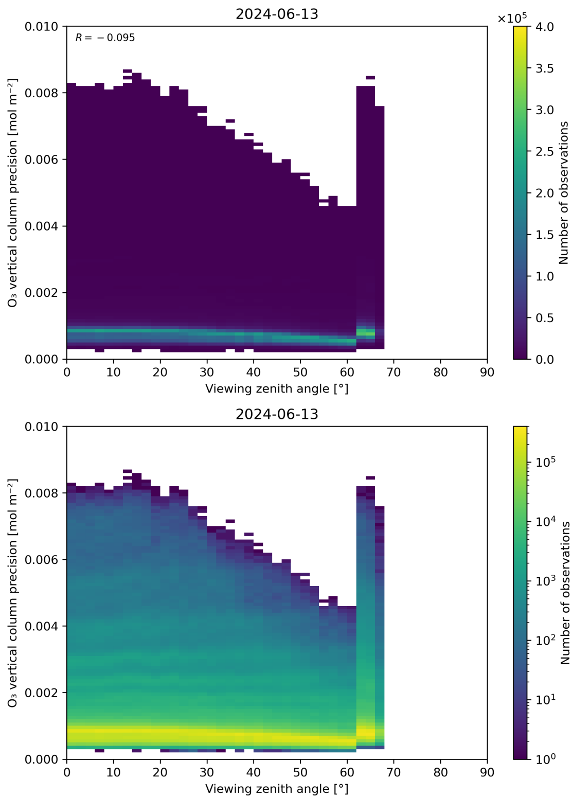
Figure 53: Scatter density plot of “Viewing zenith angle” against “O 3 vertical column precision” for 2024-06-13 to 2024-06-14.
