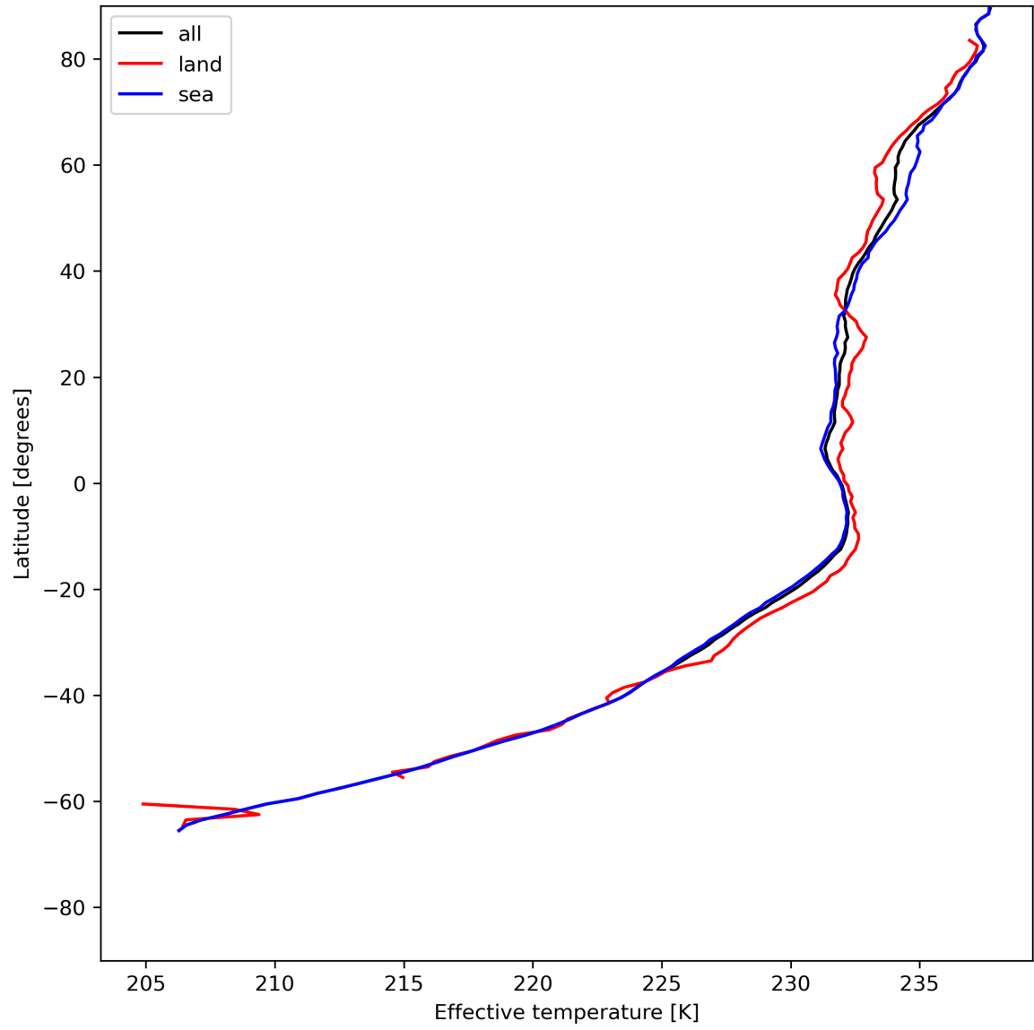
Figure 17: Zonal average of “Effective temperature” for 2024-06-13 to 2024-06-14.
