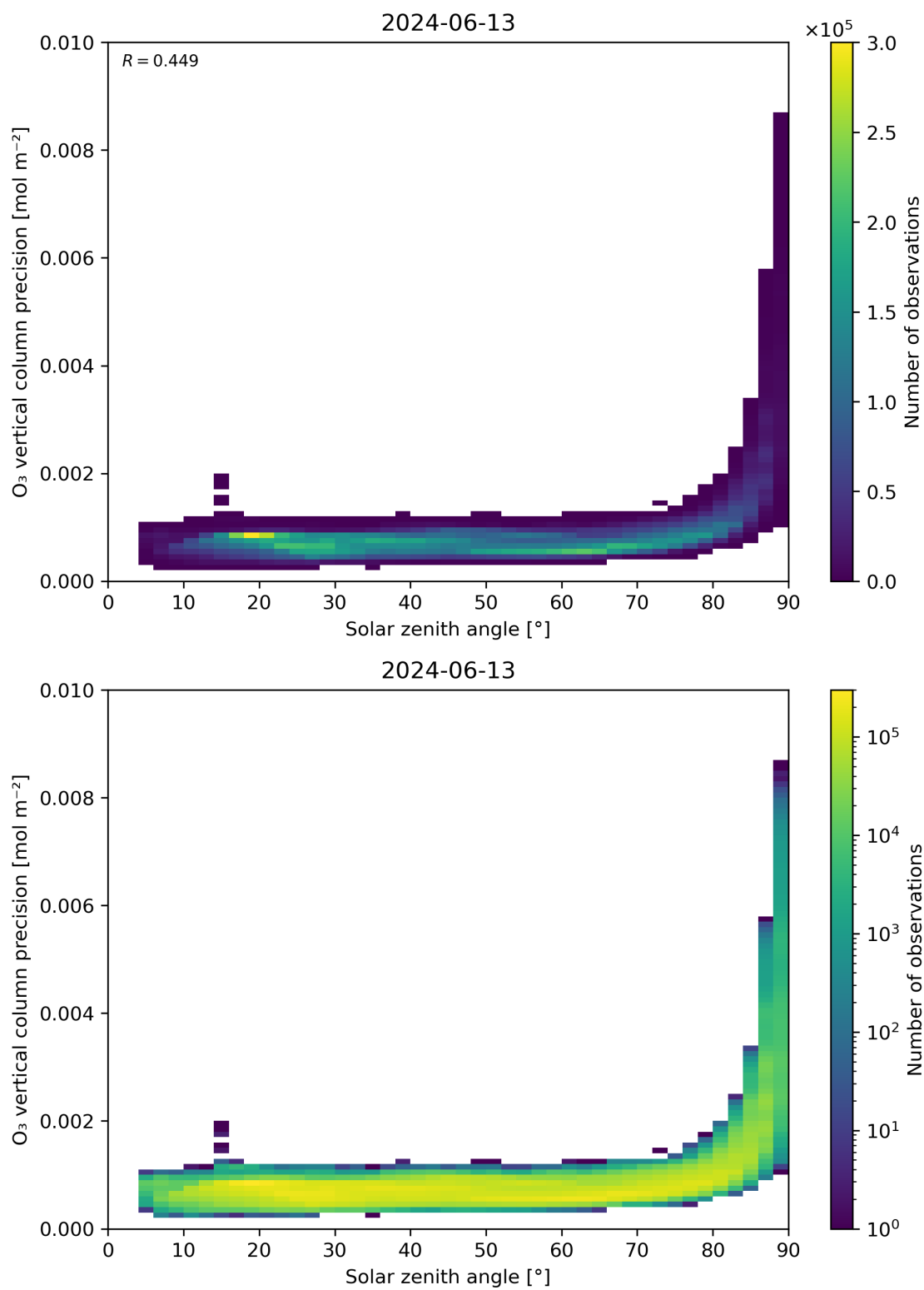
Figure 48: Scatter density plot of “Solar zenith angle” against “O 3 vertical column precision” for 2024-06-13 to 2024-06-14.
