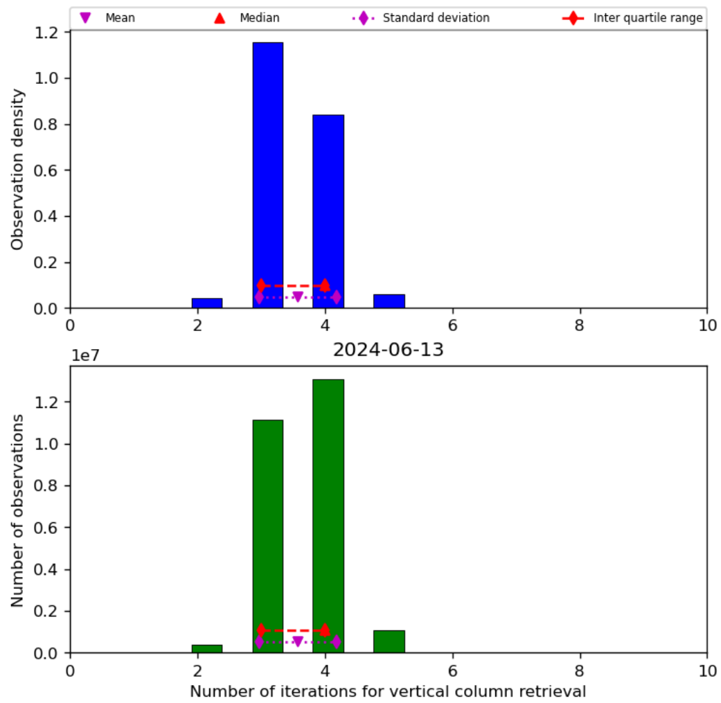
Figure 26: Histogram of “Number of iterations for vertical column retrieval” for 2024-06-13 to 2024-06-14
