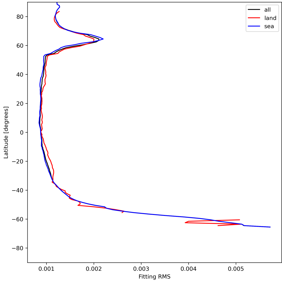
Figure 16: Zonal average of “Fitting RMS” for 2024-06-13 to 2024-06-14.
