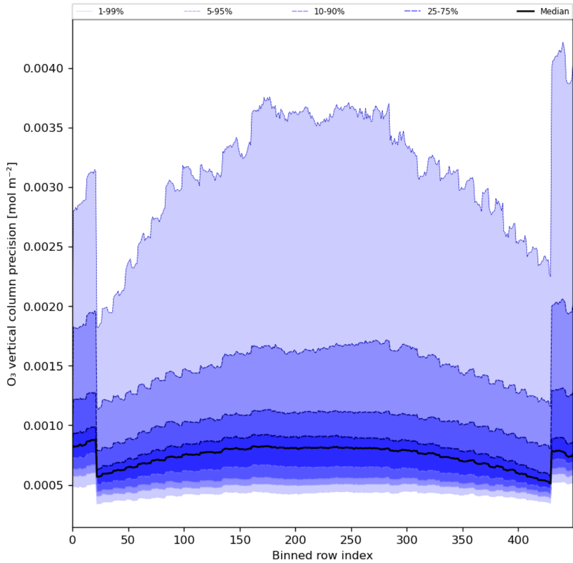
Figure 29: Along track statistics of “O 3 vertical column precision” for 2024-06-13 to 2024-06-14
