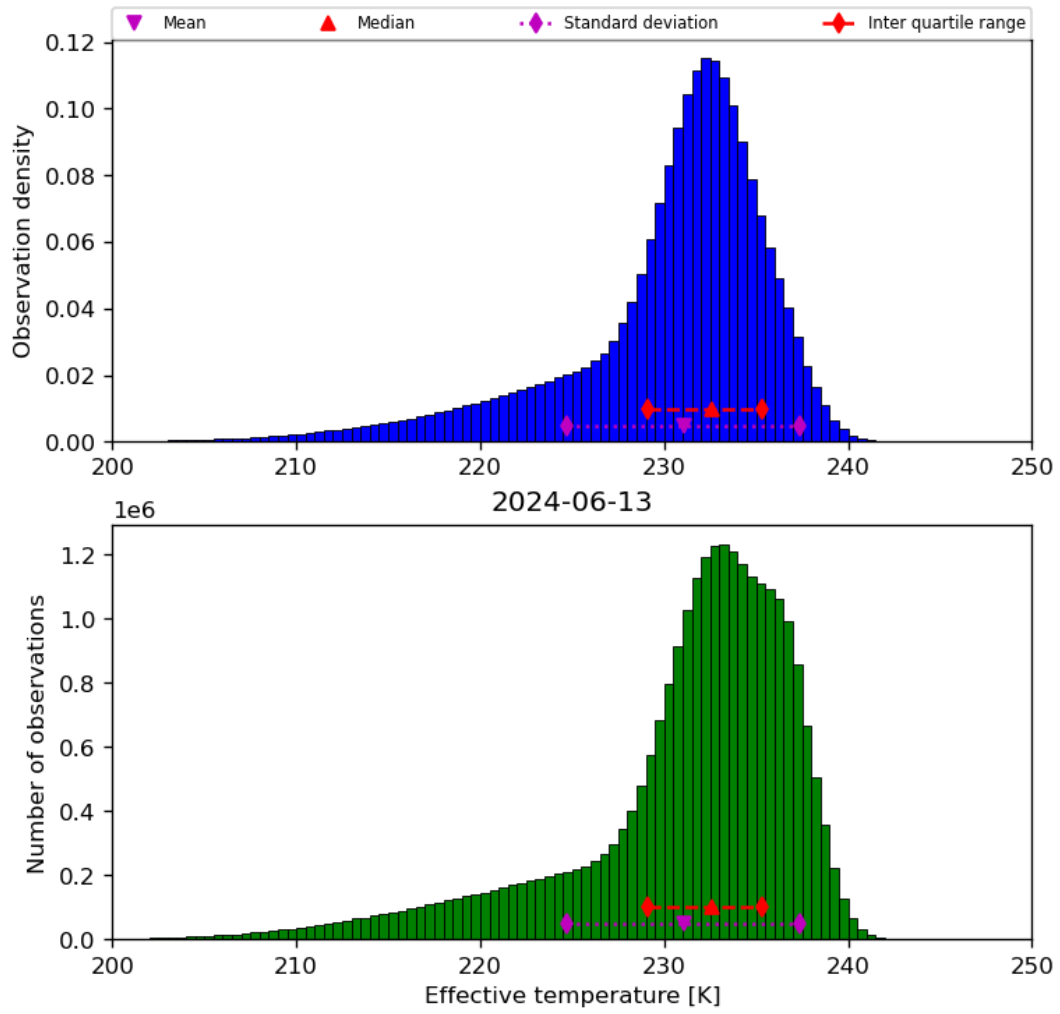
Figure 24: Histogram of “Effective temperature” for 2024-06-13 to 2024-06-14
