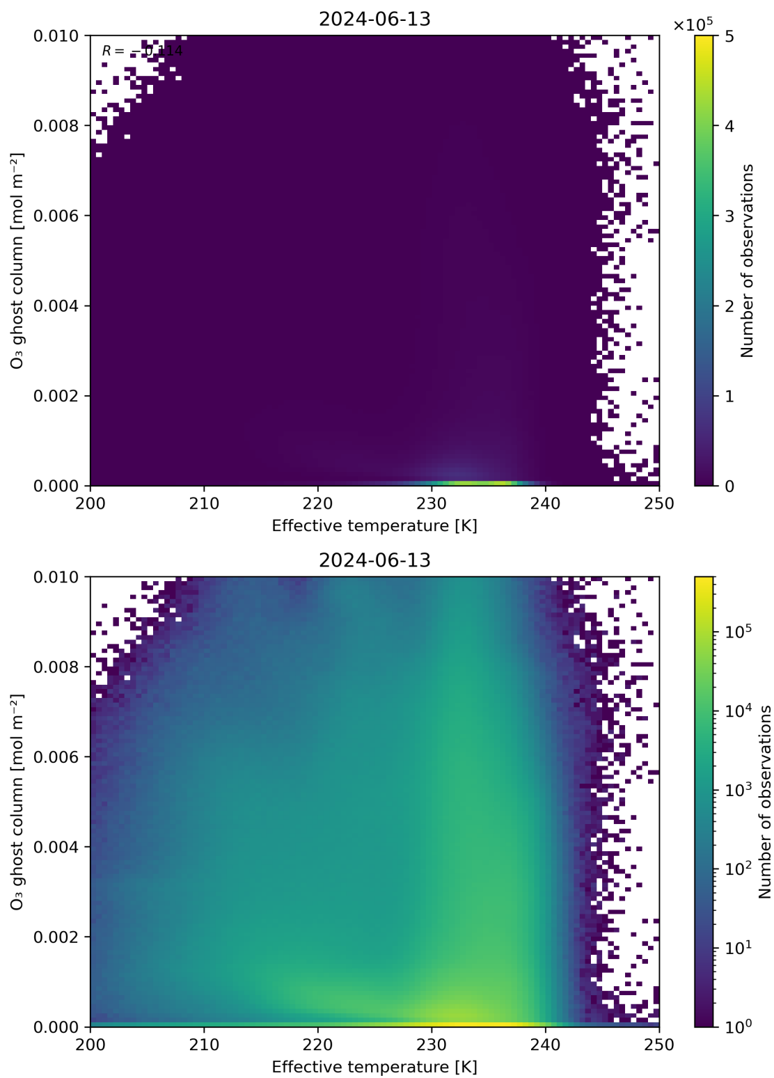
Figure 38: Scatter density plot of “Effective temperature” against “O 3 ghost column” for 2024-06-13 to 2024-06-14.
