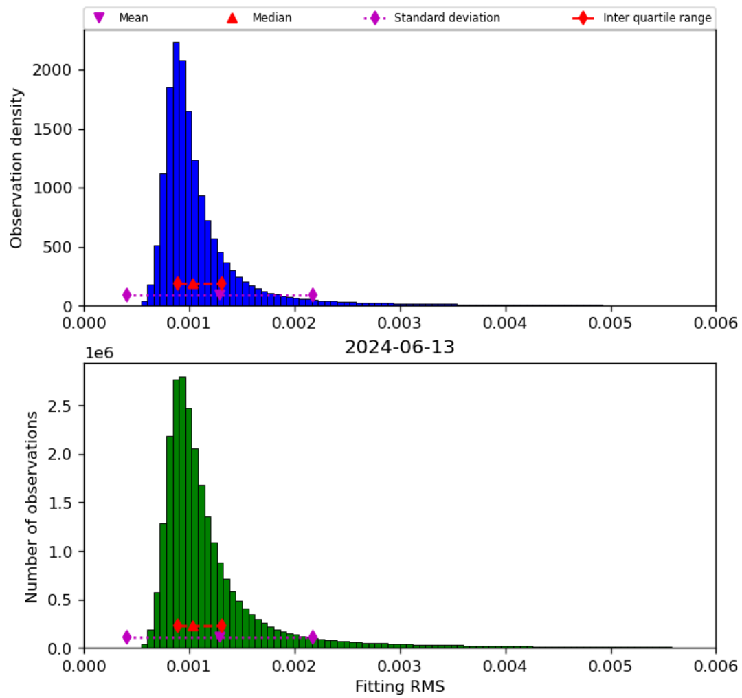
Figure 23: Histogram of "Fitting RMS" for 2024-06-13 to 2024-06-14
