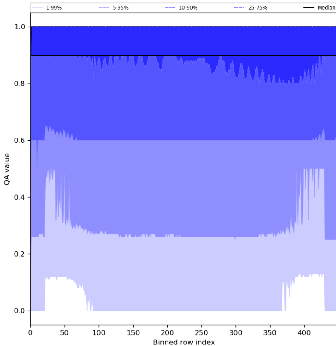
Figure 27: Along track statistics of “QA value” for 2024-06-13 to 2024-06-14
