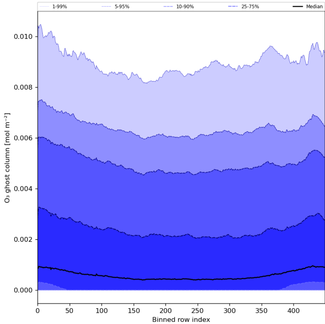
Figure 32: Along track statistics of "O 3 ghost column" for 2024-06-13 to 2024-06-14
