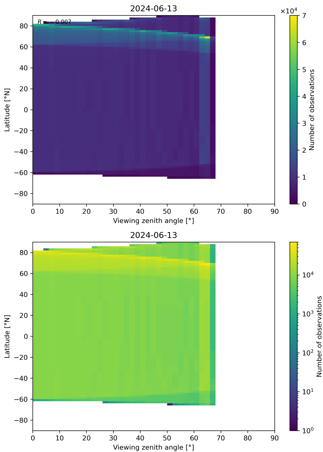
Figure 49: Scatter density plot of “Viewing zenith angle” against “Latitude” for 2024-06-13 to 2024-06-14.
