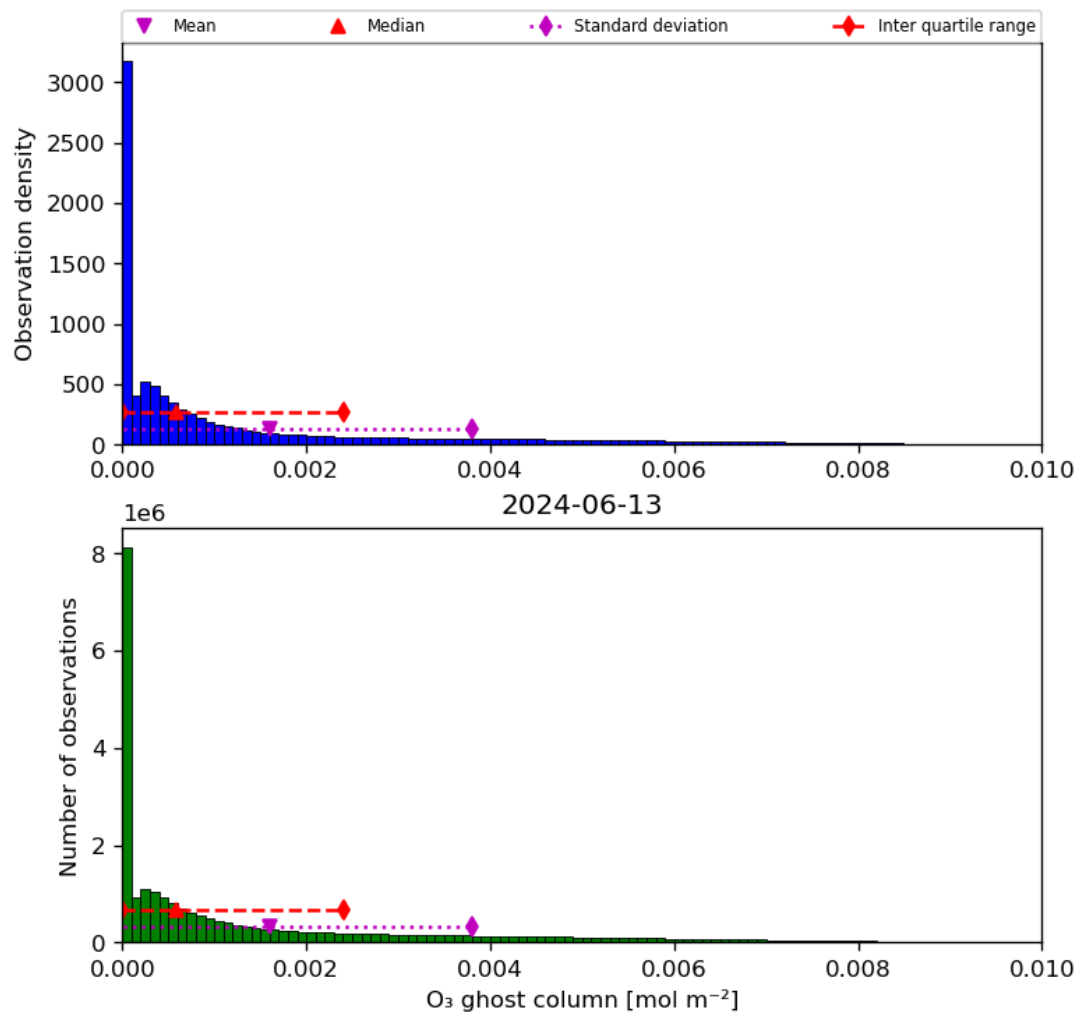
Figure 25: Histogram of “O 3 ghost column” for 2024-06-13 to 2024-06-14
