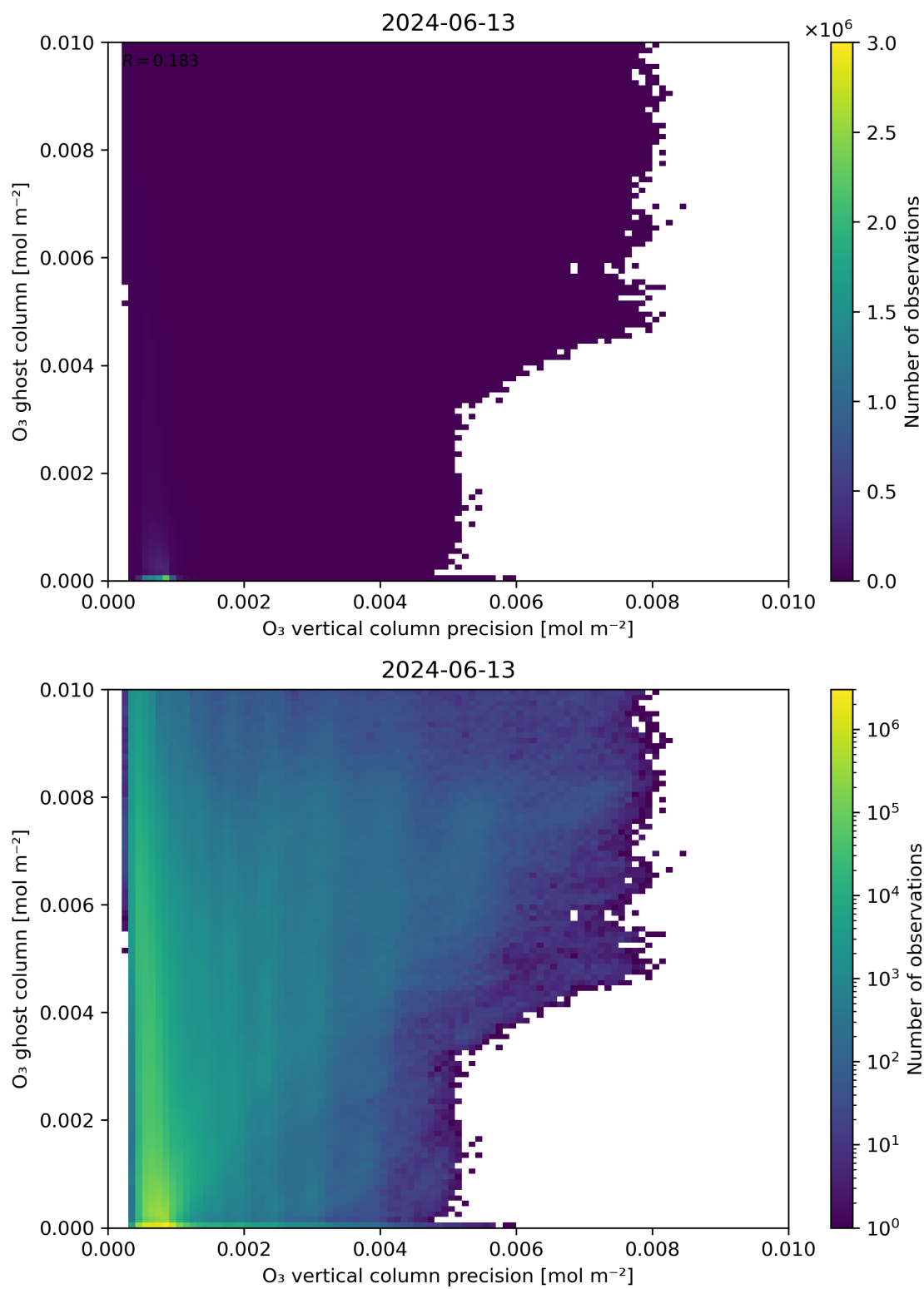
Figure 43: Scatter density plot of “ O_3 vertical column precision” against “ O_3 ghost column” for 2024-06-13 to 2024-06-14.
