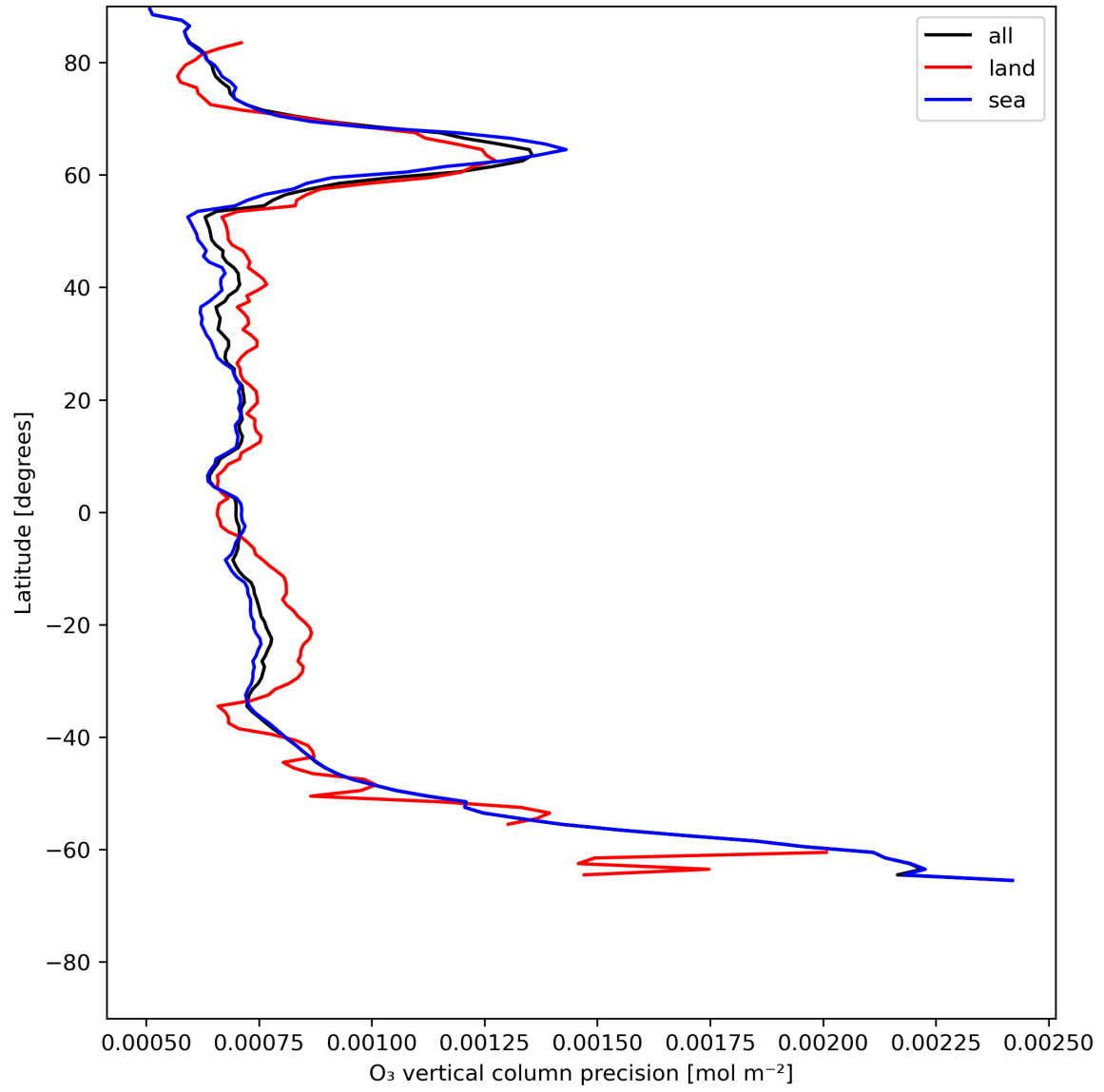
Figure 15: Zonal average of “O 3 vertical column precision” for 2024-06-13 to 2024-06-14.
