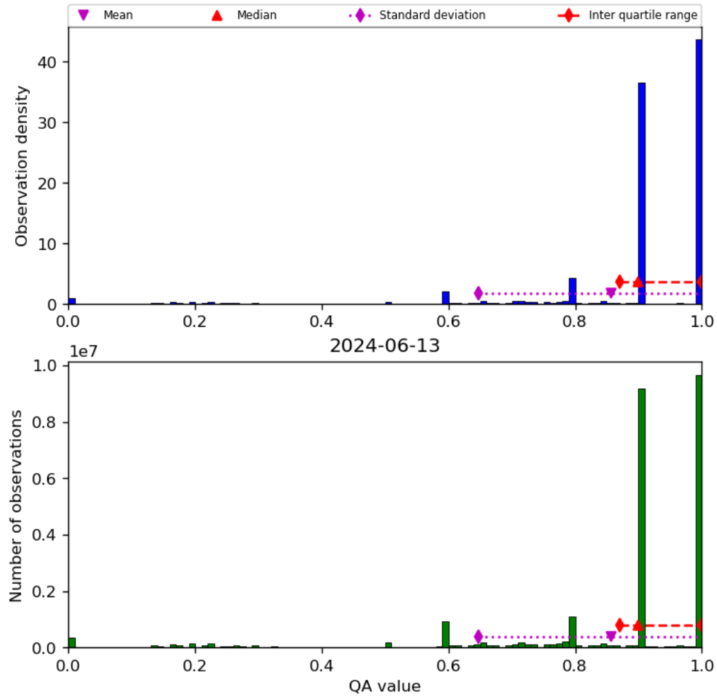
Figure 20: Histogram of “QA value” for 2024-06-13 to 2024-06-14
