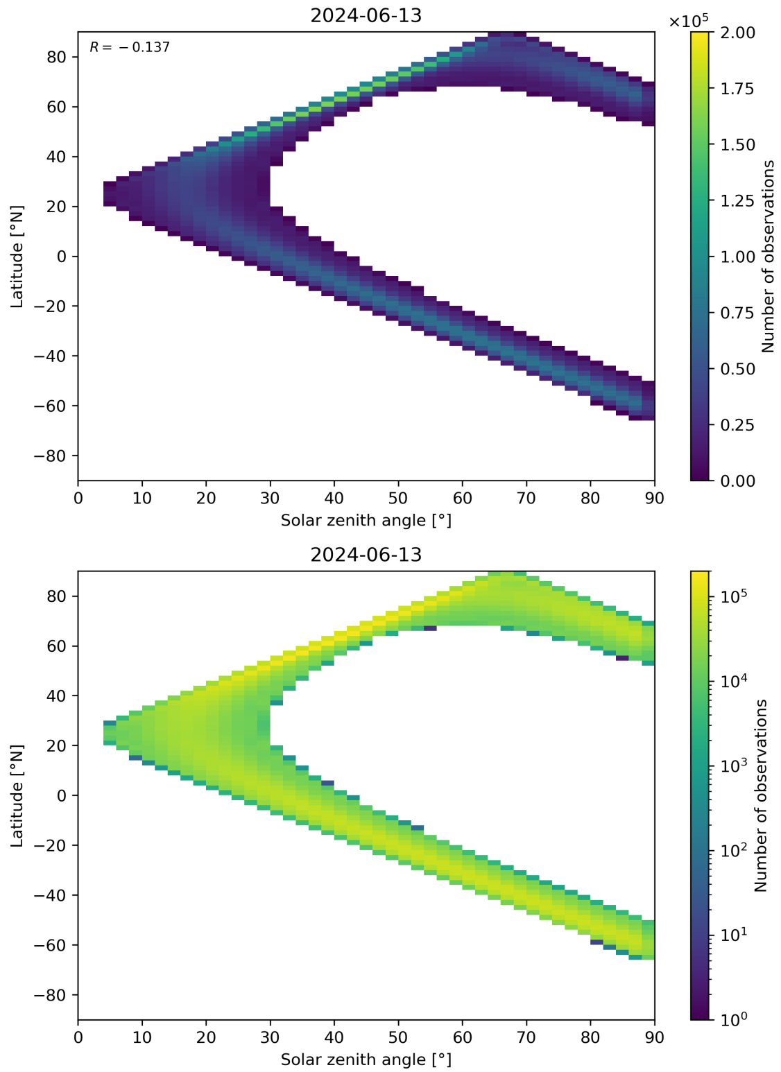
Figure 44: Scatter density plot of “Solar zenith angle” against “Latitude” for 2024-06-13 to 2024-06-14.
