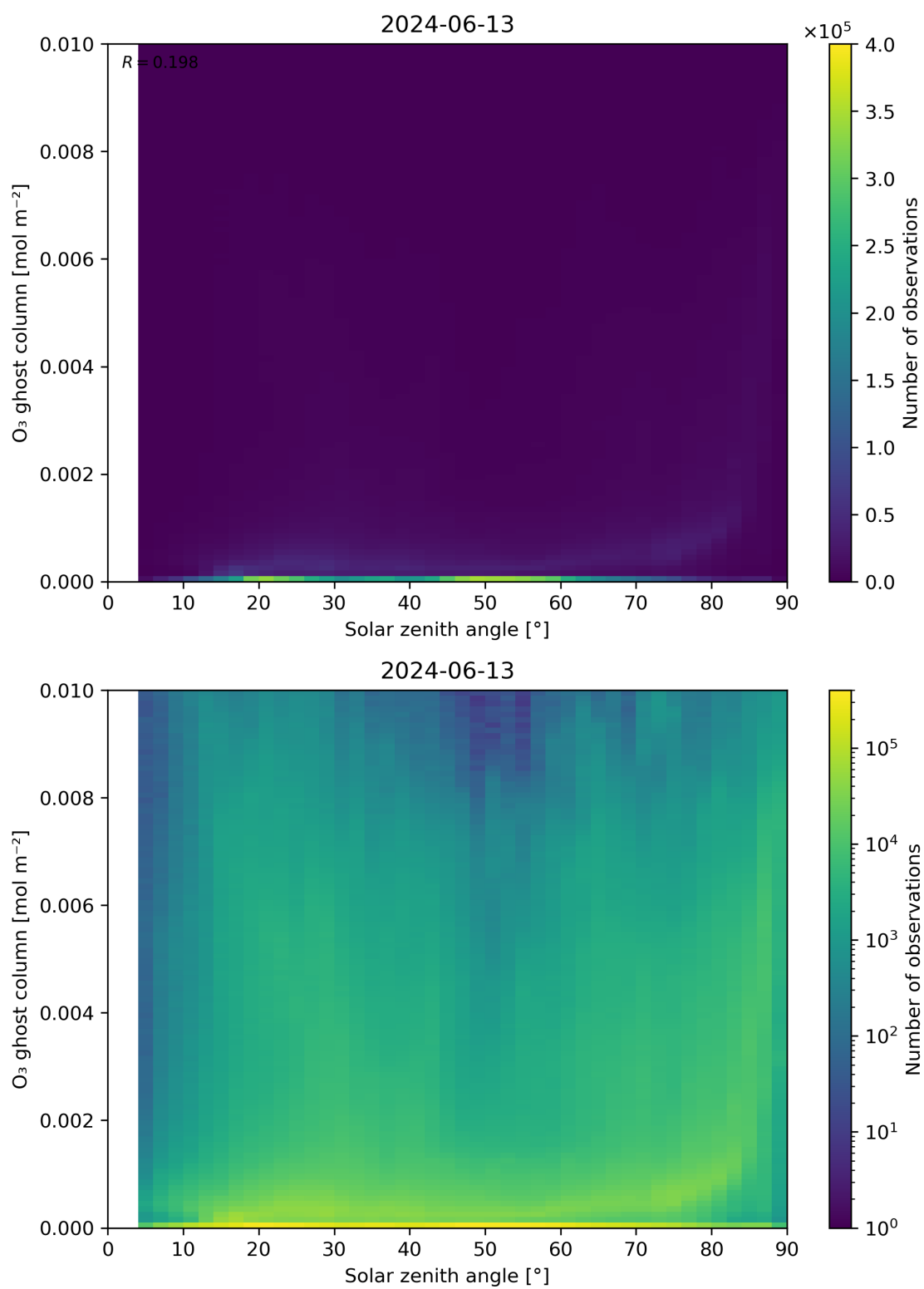
Figure 46: Scatter density plot of “Solar zenith angle” against “O 3 ghost column” for 2024-06-13 to 2024-06-14.
