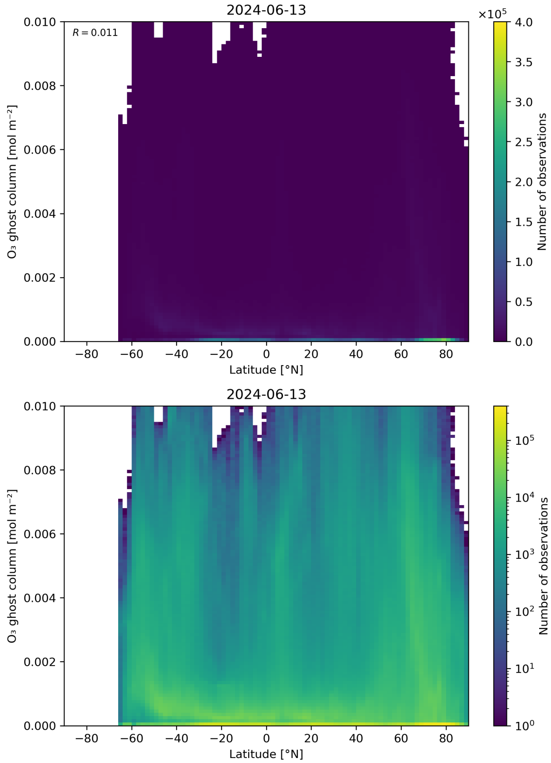
Figure 35: Scatter density plot of “Latitude” against “O 3 ghost column” for 2024-06-13 to 2024-06-14.
