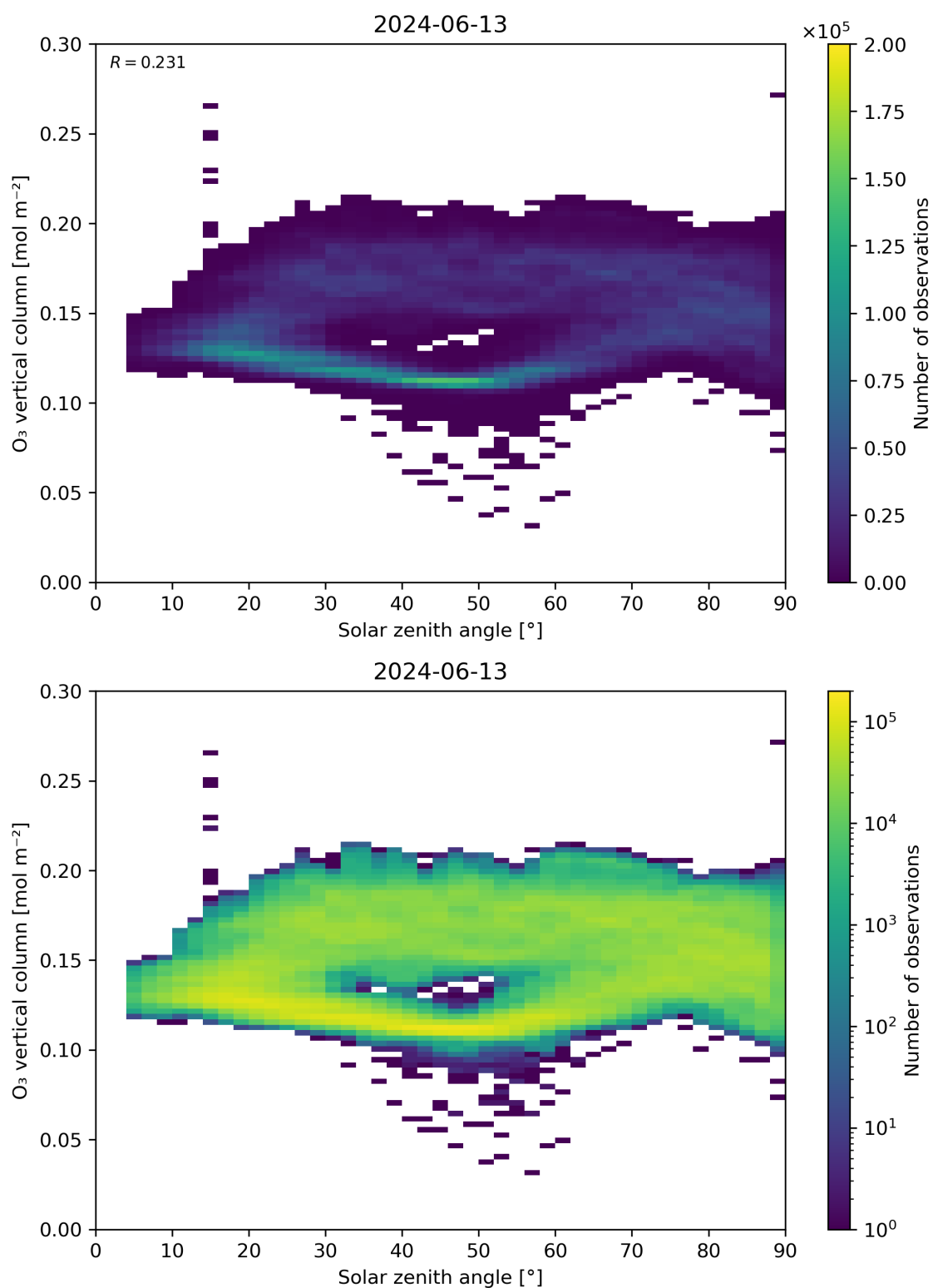
Figure 47: Scatter density plot of “Solar zenith angle” against “O 3 vertical column” for 2024-06-13 to 2024-06-14.
