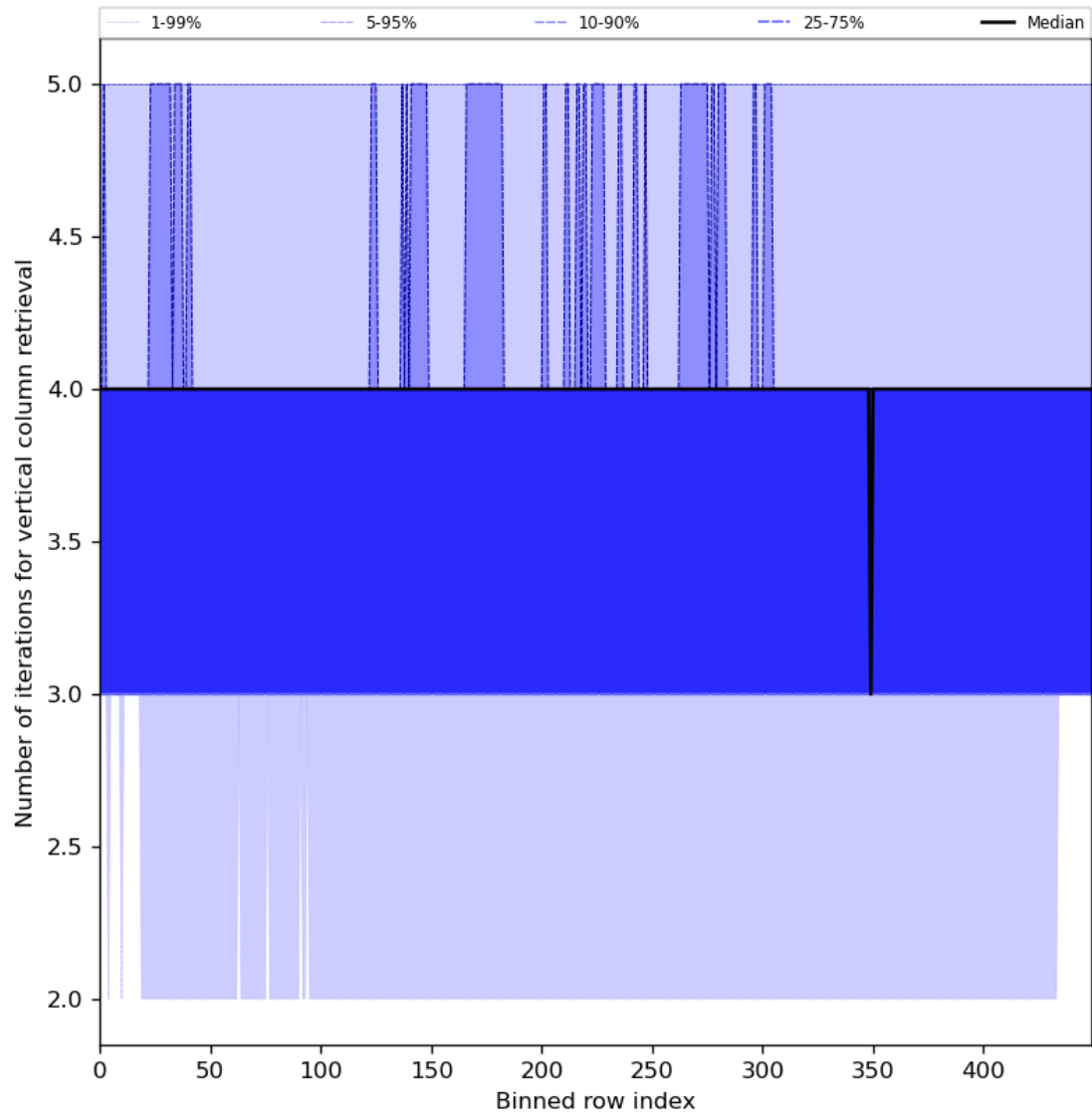
Figure 33: Along track statistics of “Number of iterations for vertical column retrieval” for 2024-06-13 to 2024-06-14
