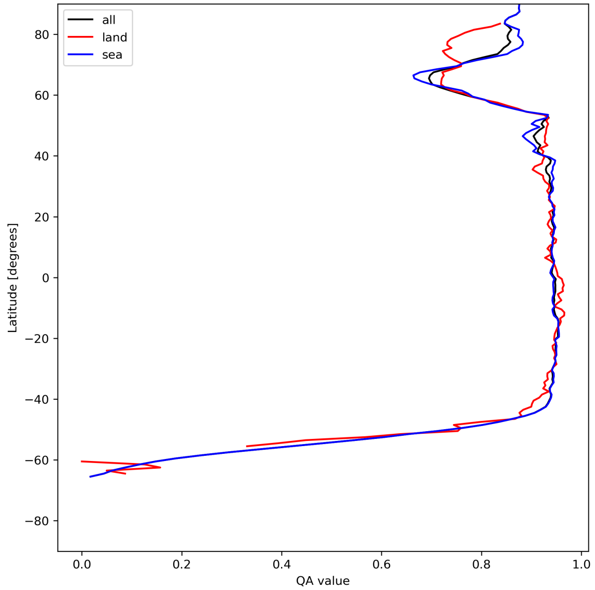
Figure 13: Zonal average of “QA value” for 2024-06-13 to 2024-06-14.
