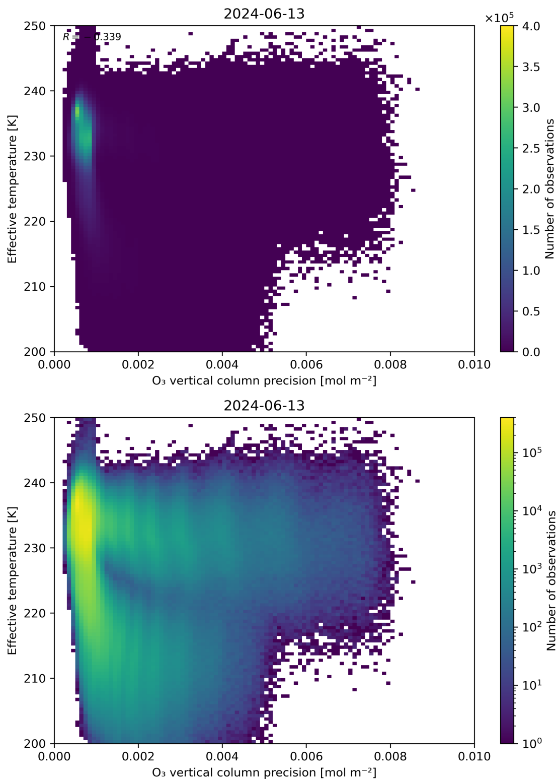
Figure 42: Scatter density plot of “O 3 vertical column precision” against “Effective temperature” for 2024-06-13 to 2024-06-14.
