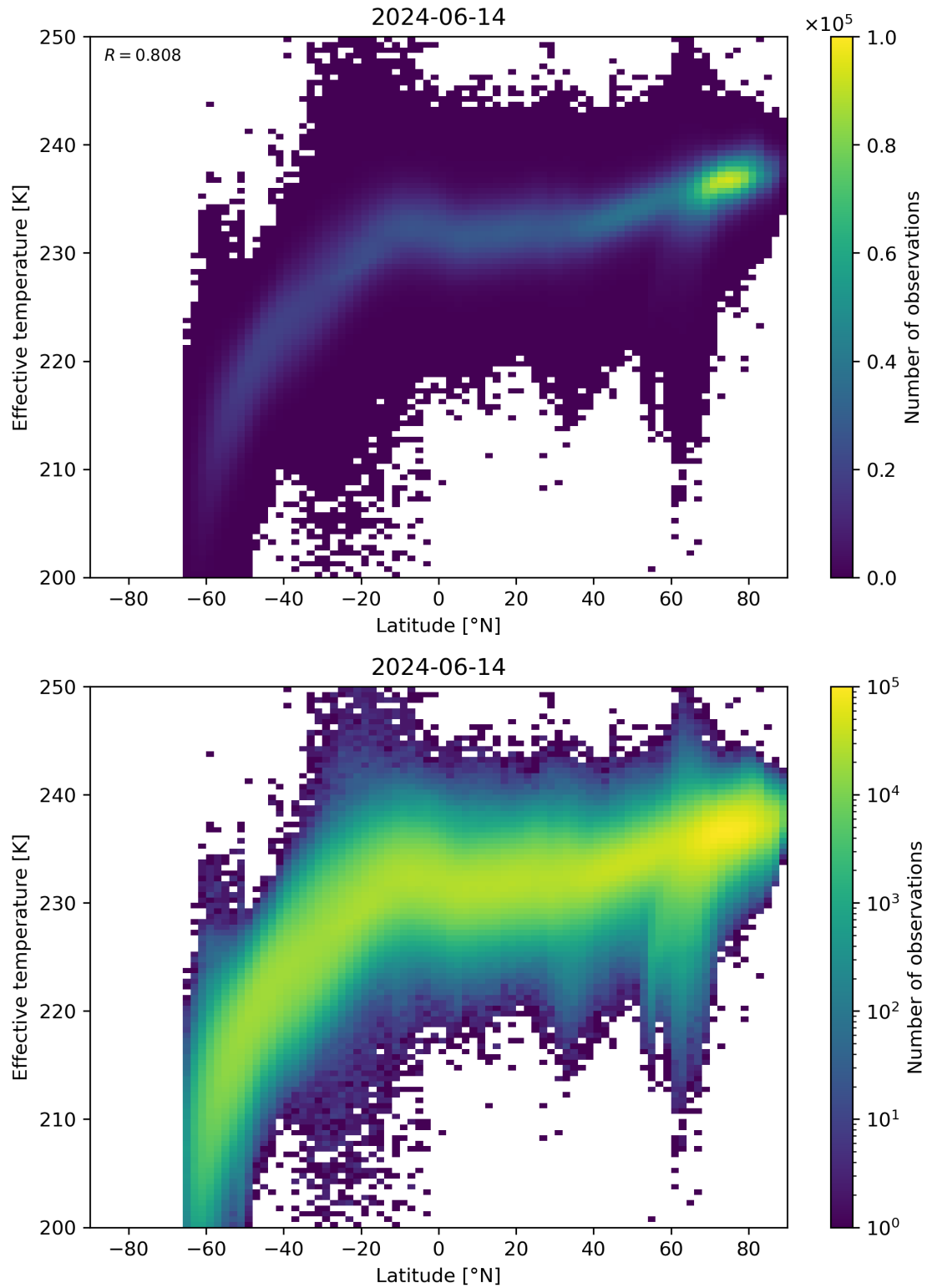
Figure 34: Scatter density plot of “Latitude” against “Effective temperature” for 2024-06-13 to 2024-06-15.
