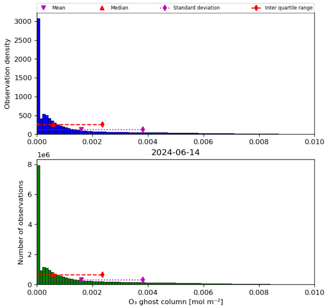
Figure 25: Histogram of “O 3 ghost column” for 2024-06-13 to 2024-06-15
