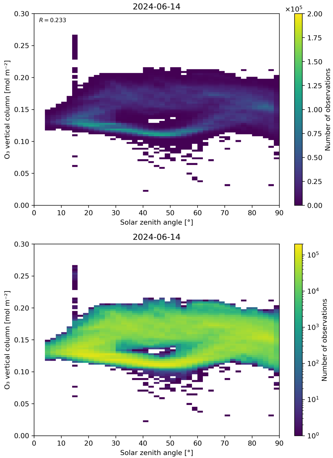
Figure 47: Scatter density plot of “Solar zenith angle” against “O 3 vertical column” for 2024-06-13 to 2024-06-15.
