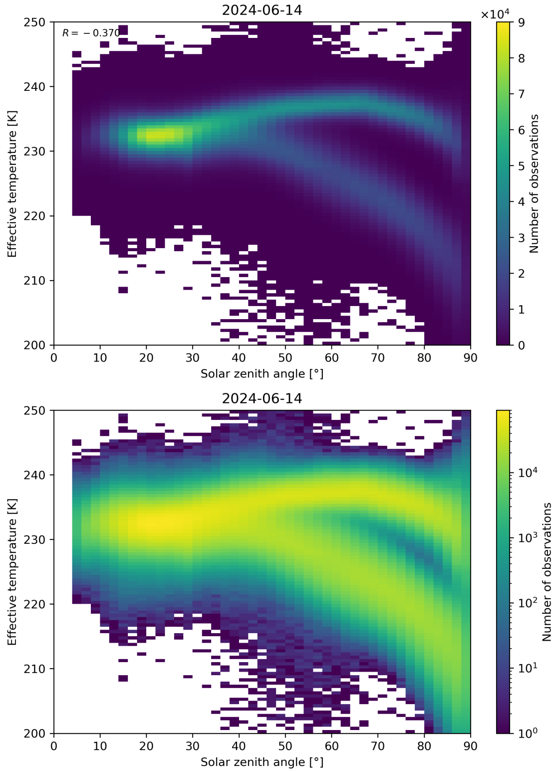
Figure 45: Scatter density plot of “Solar zenith angle” against “Effective temperature” for 2024-06-13 to 2024-06-15.
