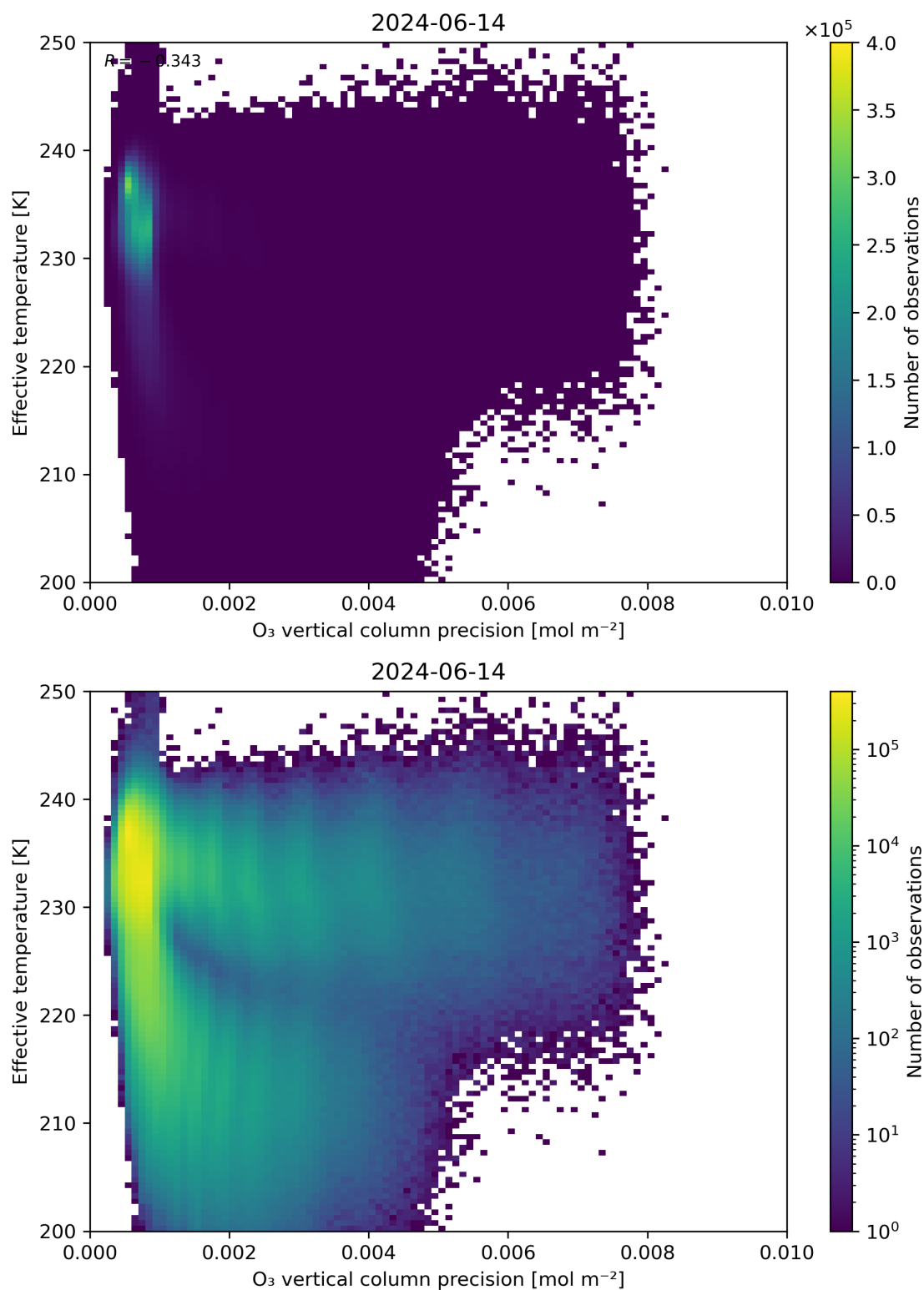
Figure 42: Scatter density plot of “O 3 vertical column precision” against “Effective temperature” for 2024-06-13 to 2024-06-15.
