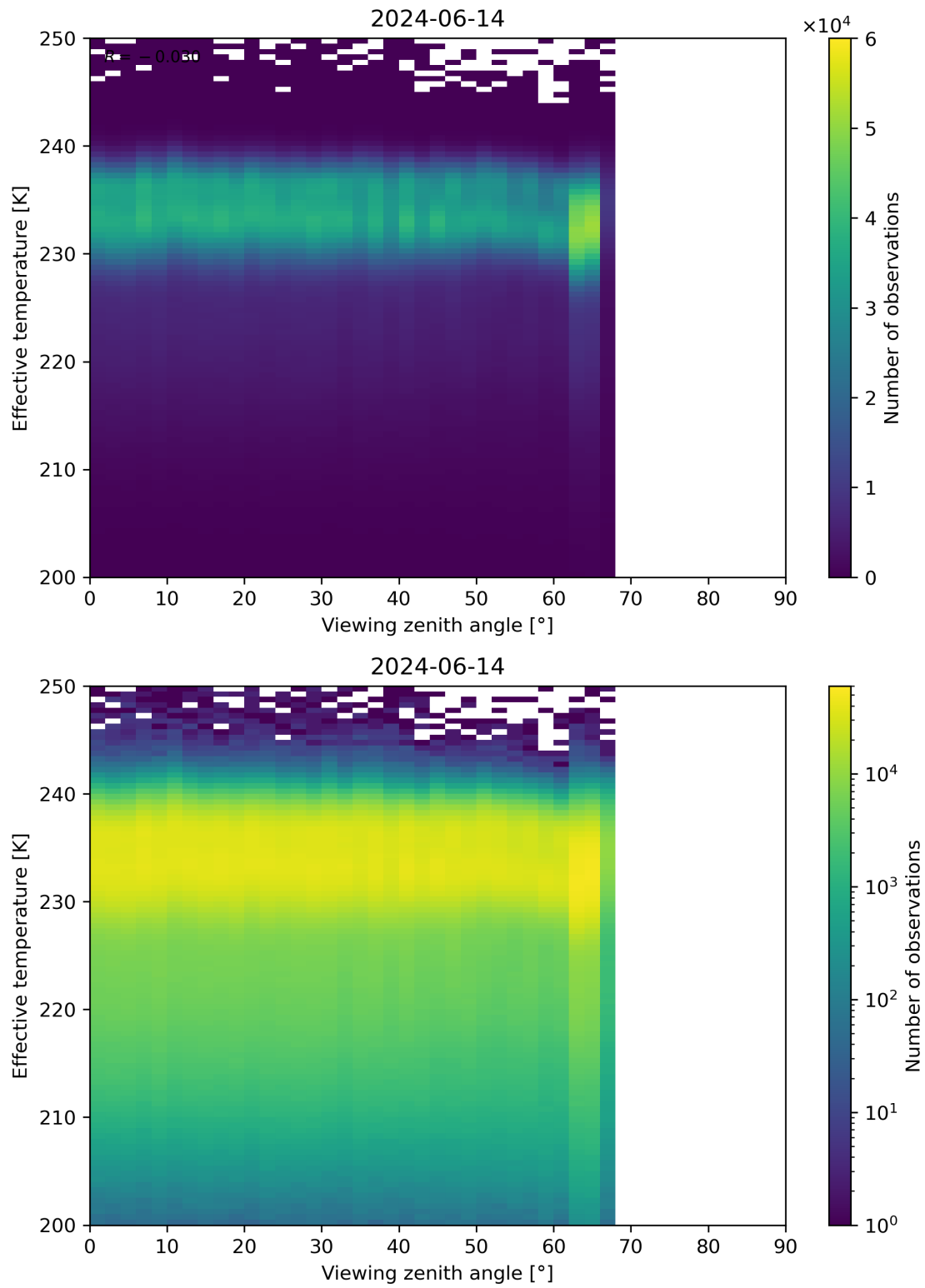
Figure 50: Scatter density plot of “Viewing zenith angle” against “Effective temperature” for 2024-06-13 to 2024-06-15.
