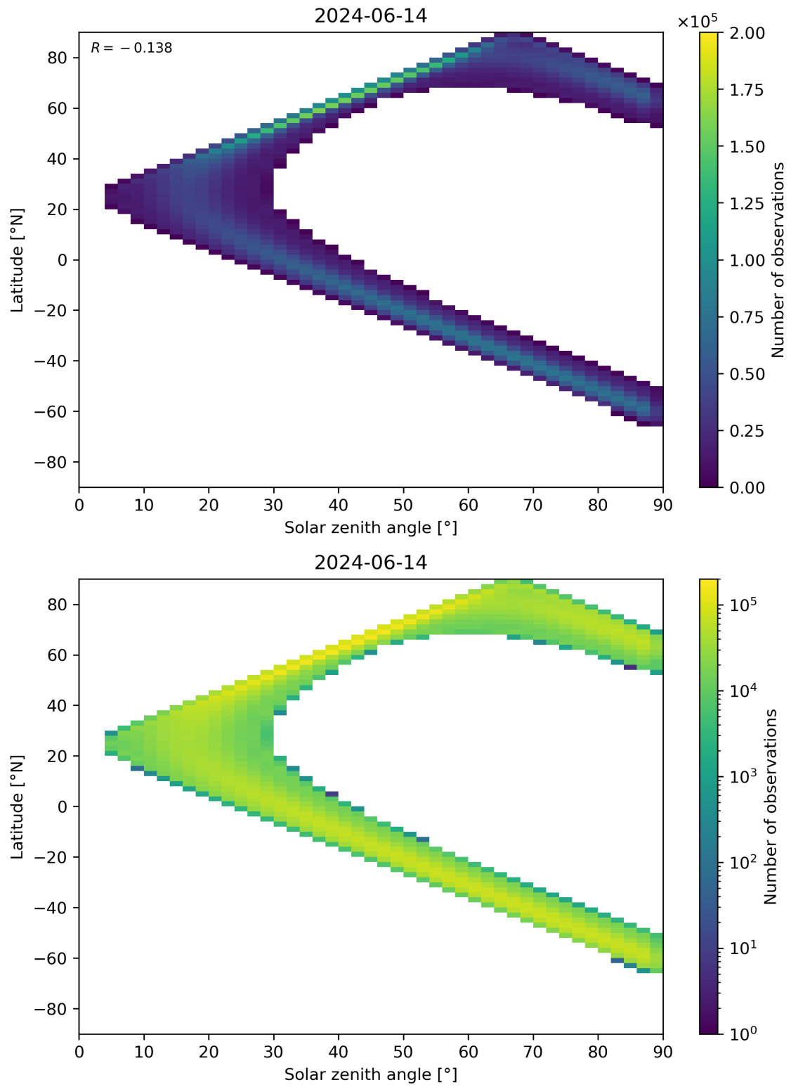
Figure 44: Scatter density plot of “Solar zenith angle” against “Latitude” for 2024-06-13 to 2024-06-15.
