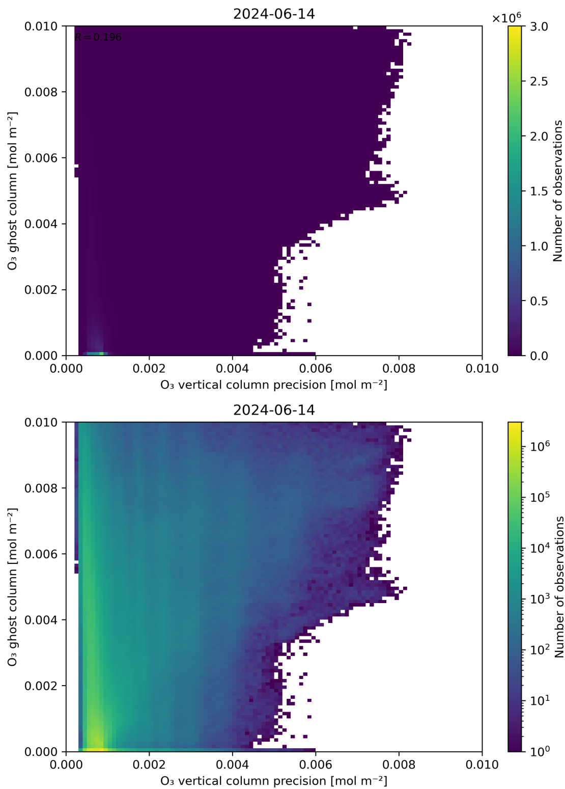
Figure 43: Scatter density plot of “ \text{O}_3 vertical column precision” against “ \text{O}_3 ghost column” for 2024-06-13 to 2024-06-15.
