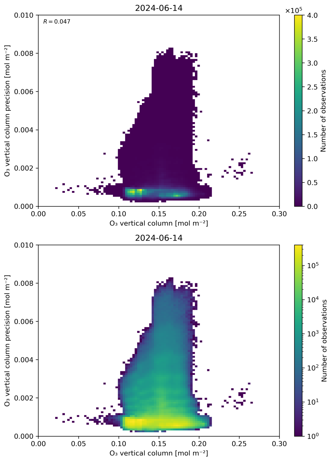
Figure 41: Scatter density plot of “O 3 vertical column” against “O 3 vertical column precision” for 2024-06-13 to 2024-06-15.
