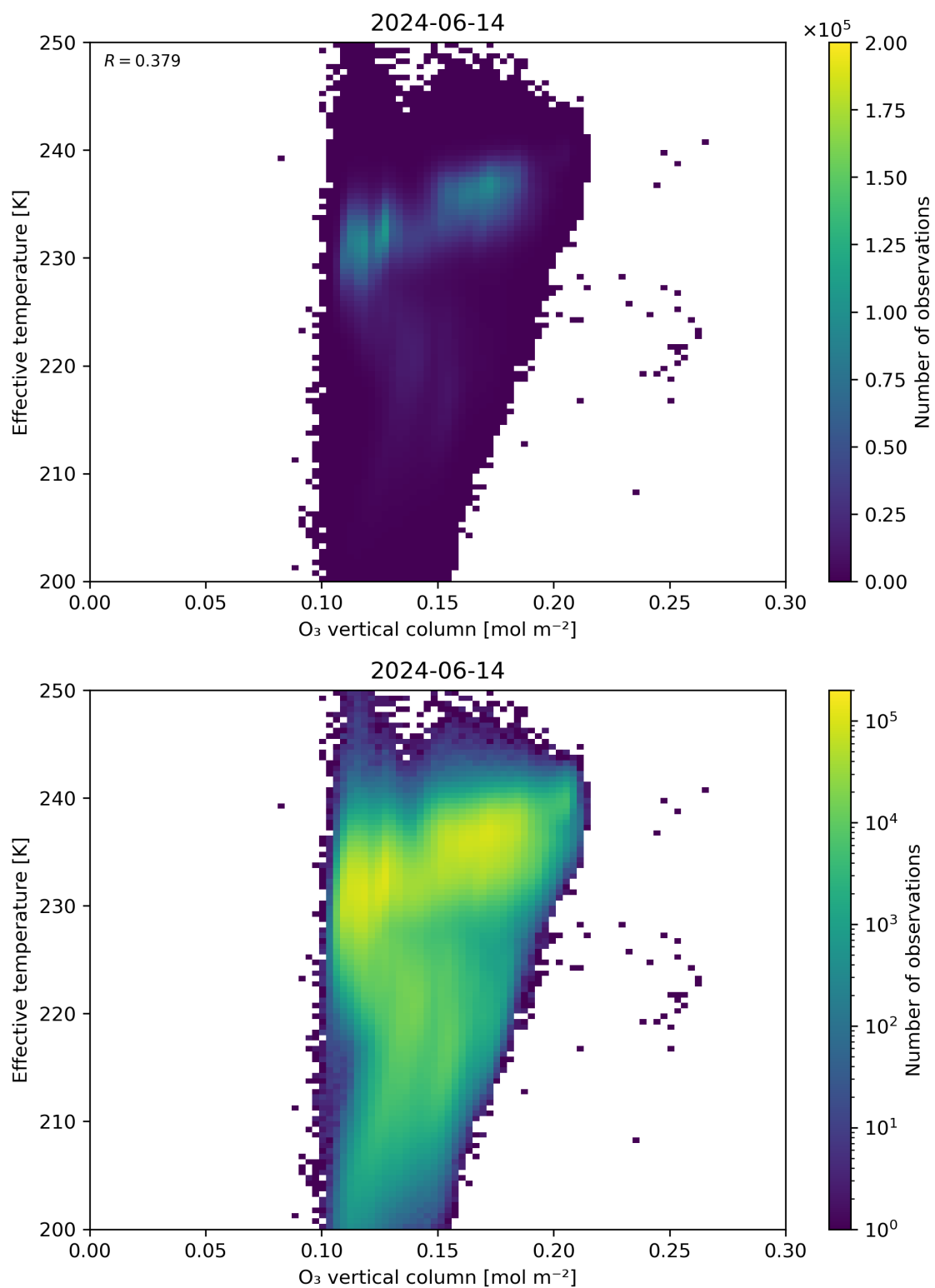
Figure 39: Scatter density plot of “O 3 vertical column” against “Effective temperature” for 2024-06-13 to 2024-06-15.
