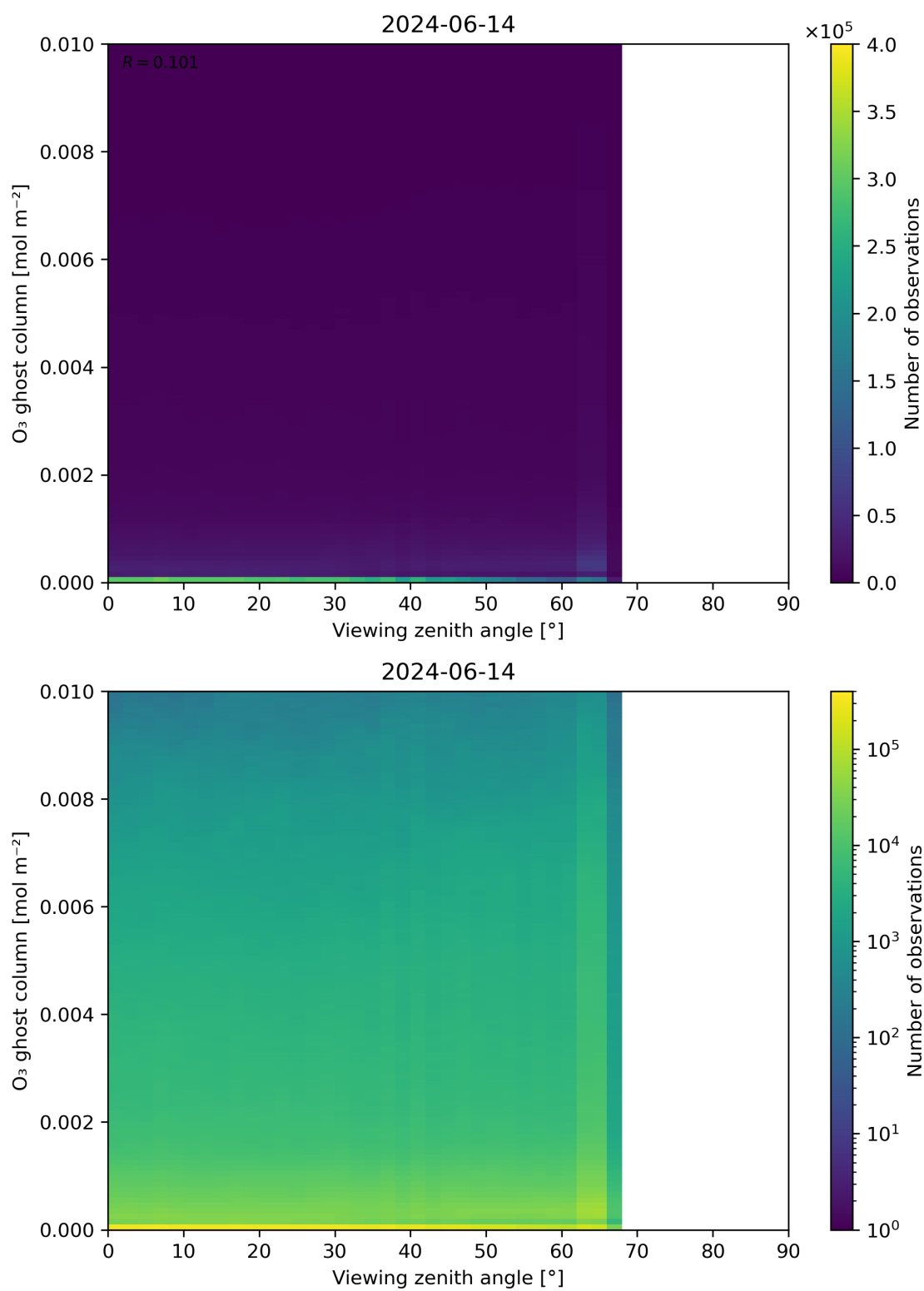
Figure 51: Scatter density plot of “Viewing zenith angle” against “O 3 ghost column” for 2024-06-13 to 2024-06-15.
