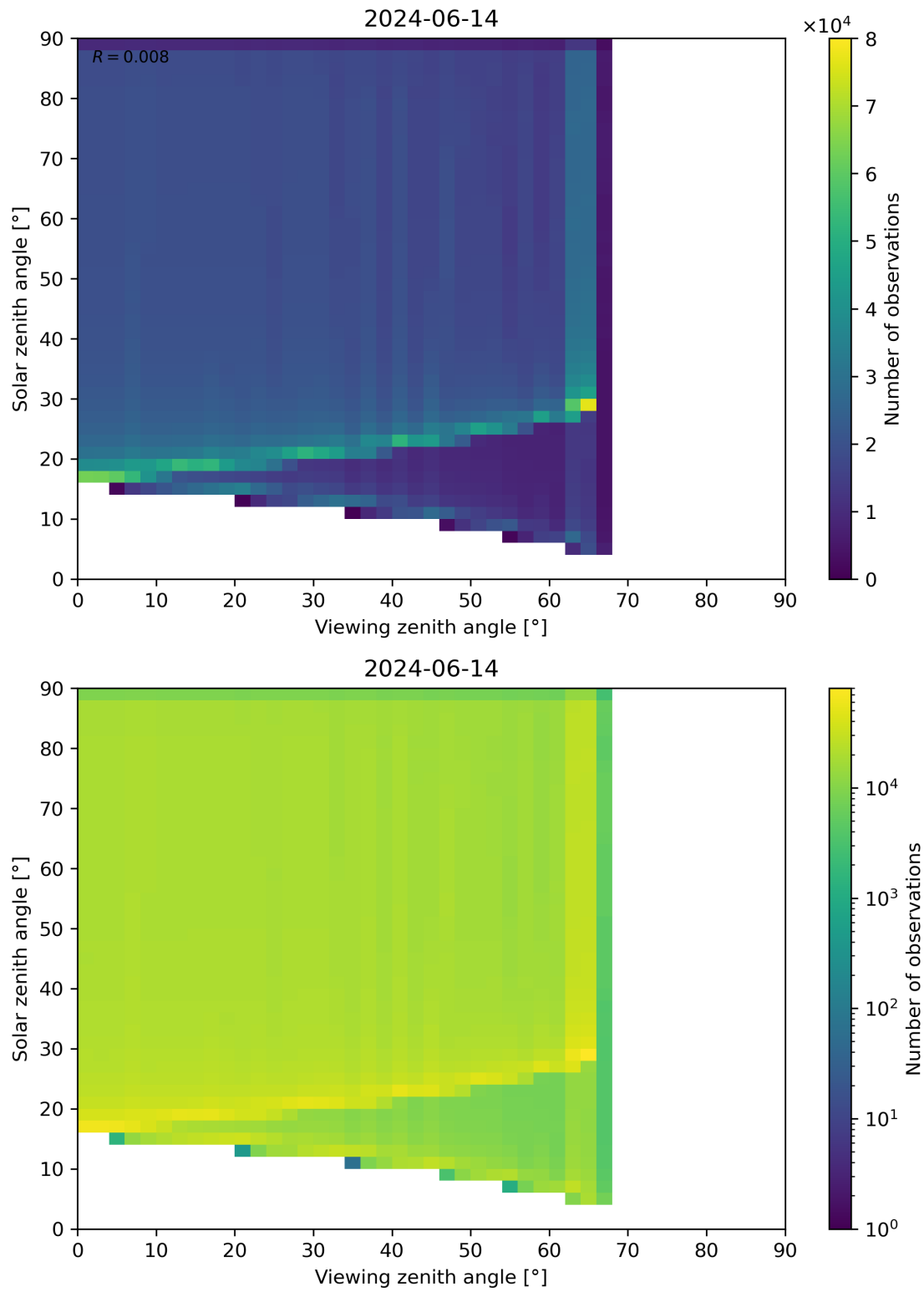
Figure 54: Scatter density plot of “Viewing zenith angle” against “Solar zenith angle” for 2024-06-13 to 2024-06-15.
