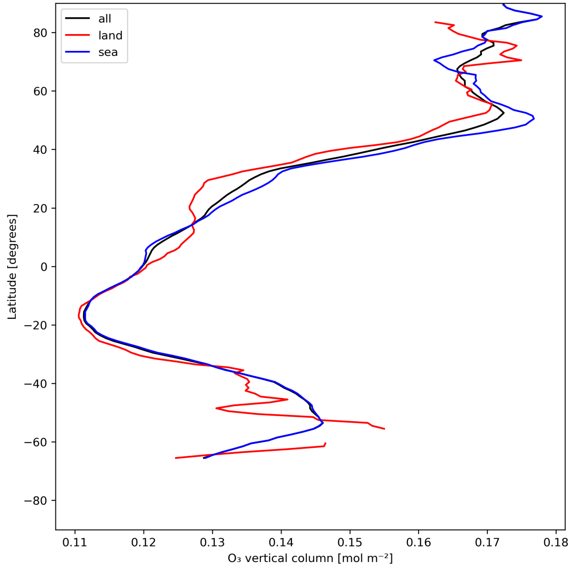
Figure 14: Zonal average of “O 3 vertical column” for 2024-06-13 to 2024-06-15.
