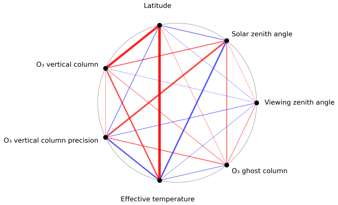
Figure 1: Map of correlation graph for 2024-06-13 to 2024-06-15.
