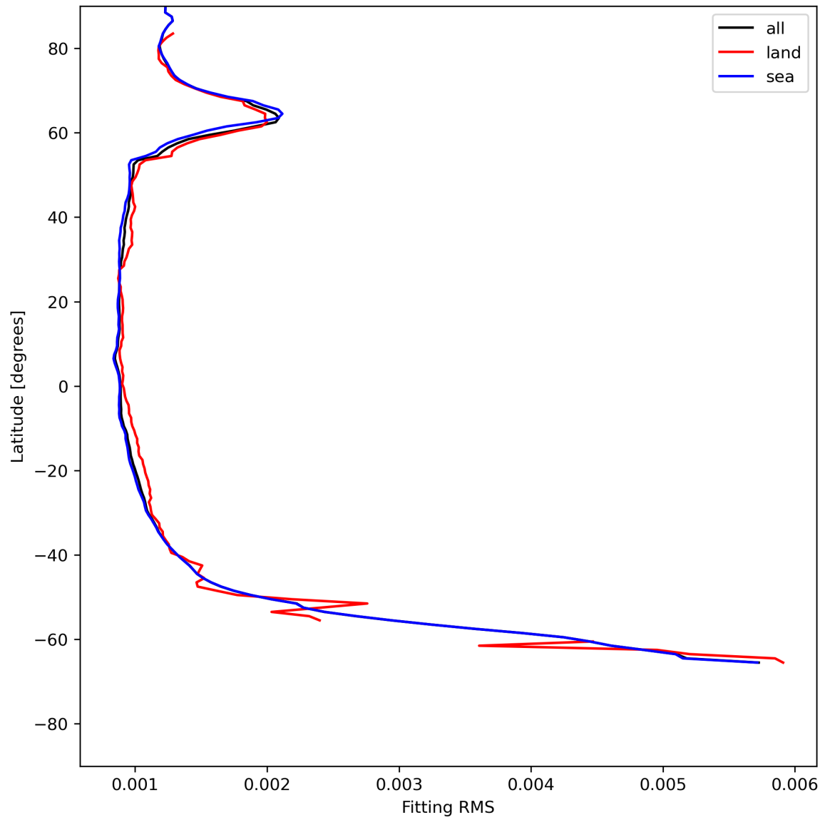
Figure 16: Zonal average of “Fitting RMS” for 2024-06-13 to 2024-06-15.
