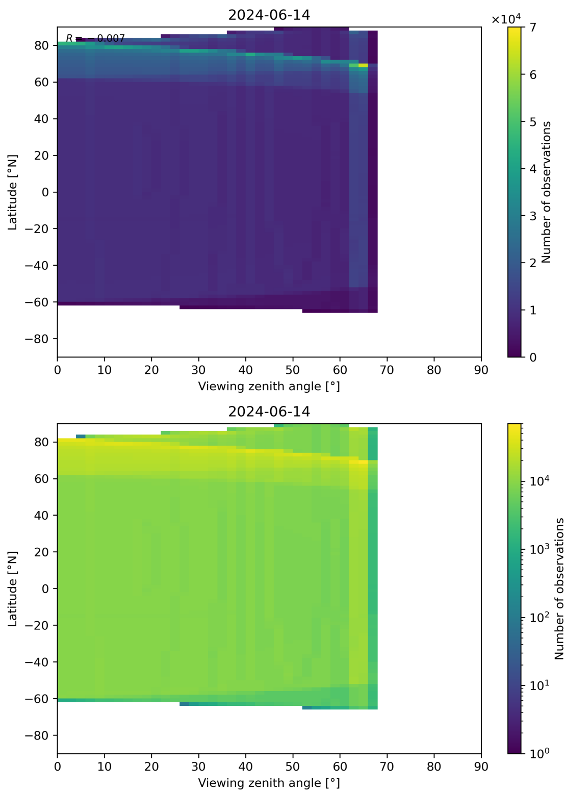
Figure 49: Scatter density plot of “Viewing zenith angle” against “Latitude” for 2024-06-13 to 2024-06-15.
