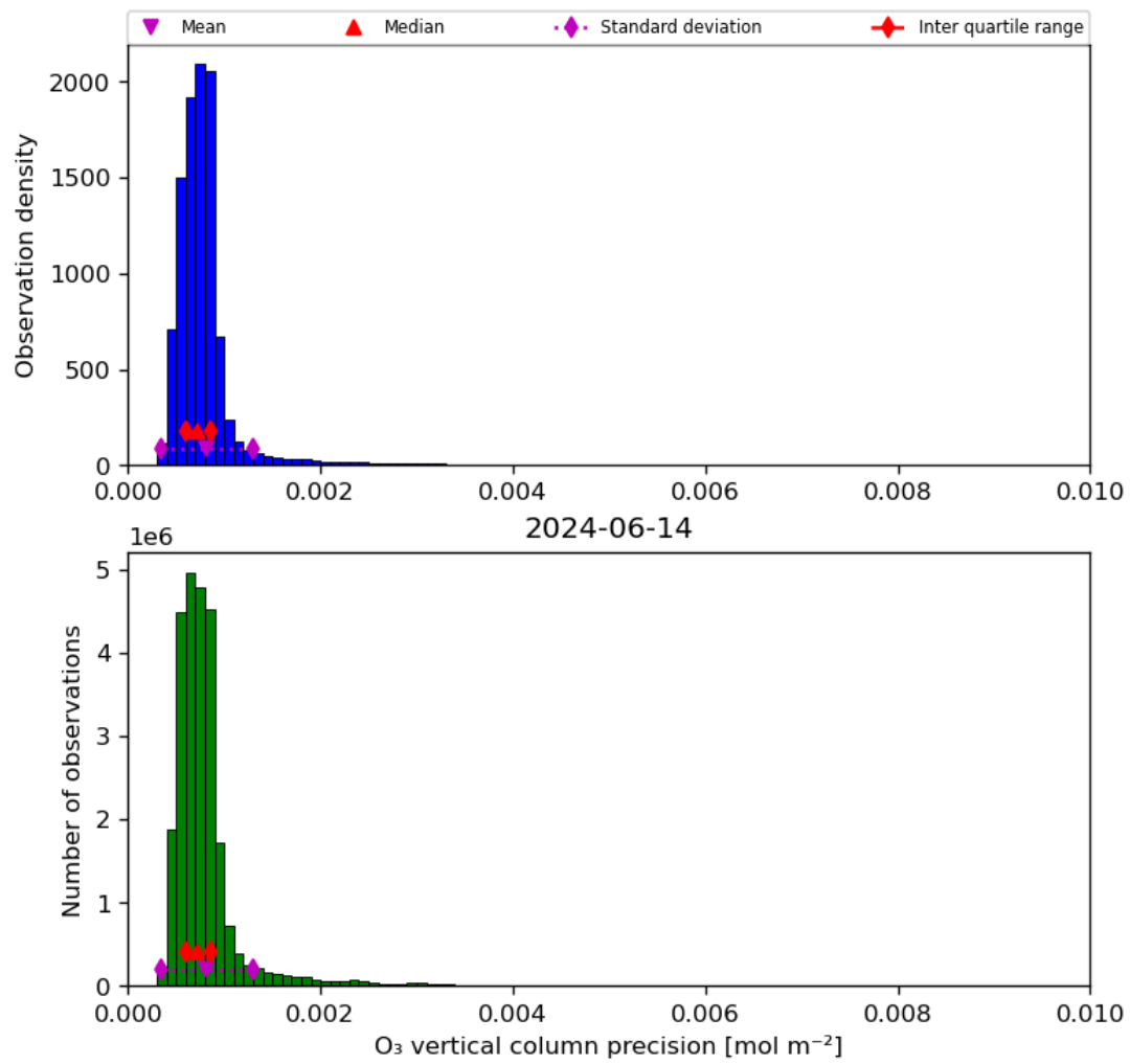
Figure 22: Histogram of “O 3 vertical column precision” for 2024-06-13 to 2024-06-15
