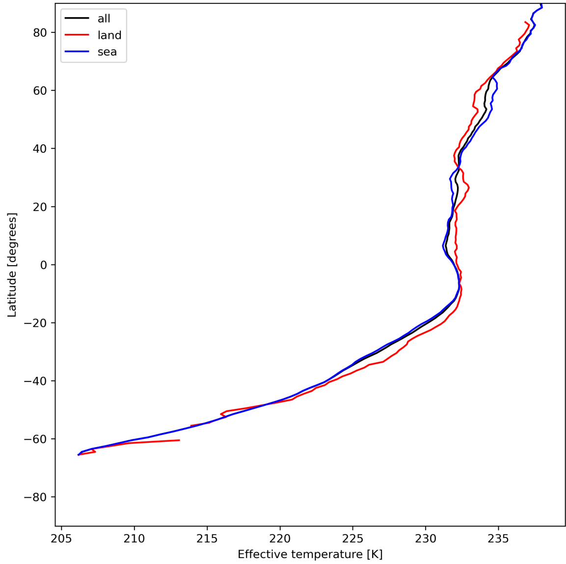
Figure 17: Zonal average of "Effective temperature" for 2024-06-13 to 2024-06-15.
