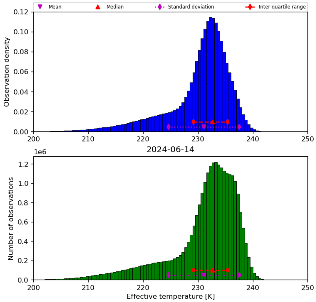
Figure 24: Histogram of “Effective temperature” for 2024-06-13 to 2024-06-15
