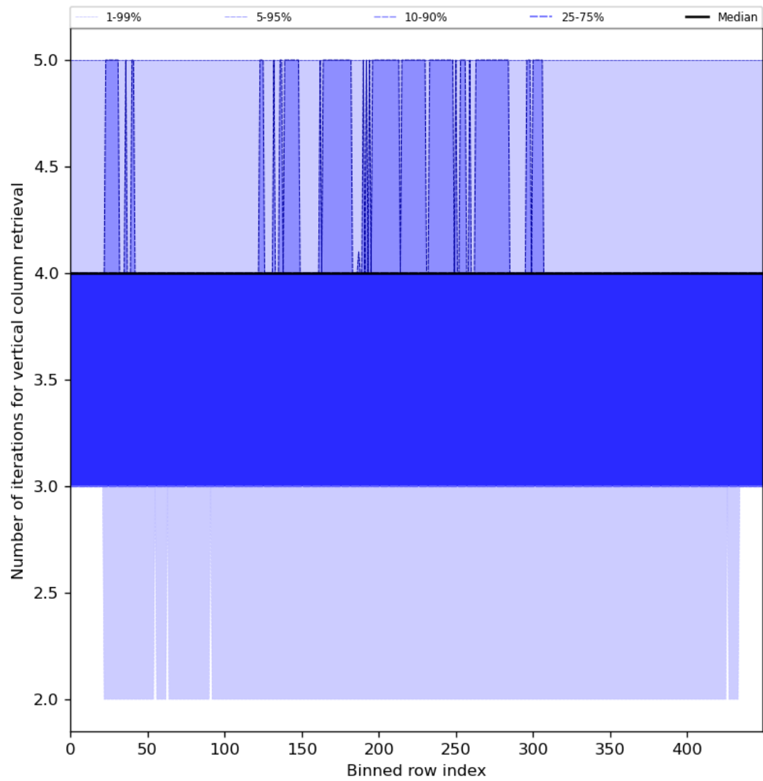
Figure 33: Along track statistics of “Number of iterations for vertical column retrieval” for 2024-06-13 to 2024-06-15
