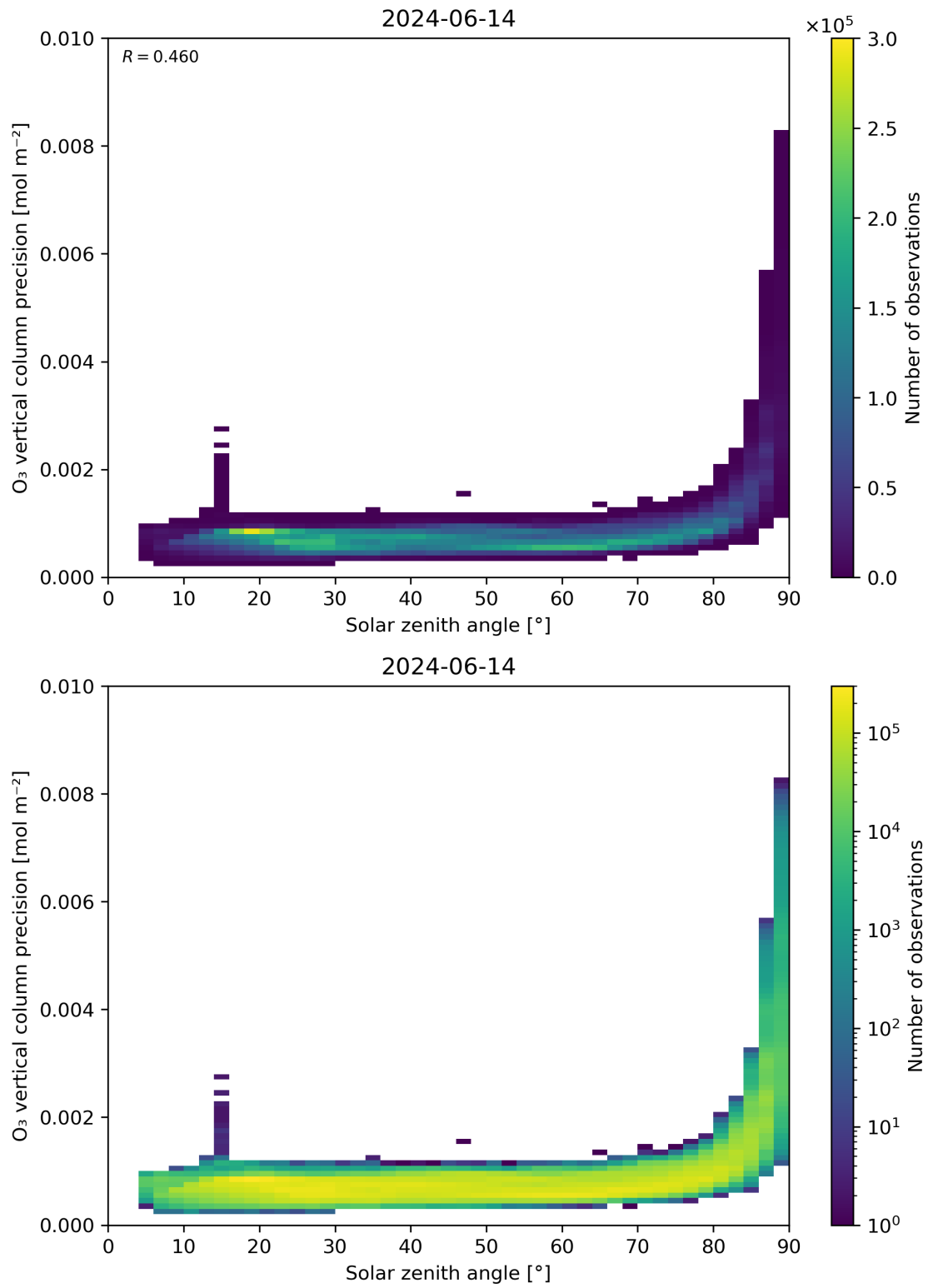
Figure 48: Scatter density plot of “Solar zenith angle” against “O 3 vertical column precision” for 2024-06-13 to 2024-06-15.
