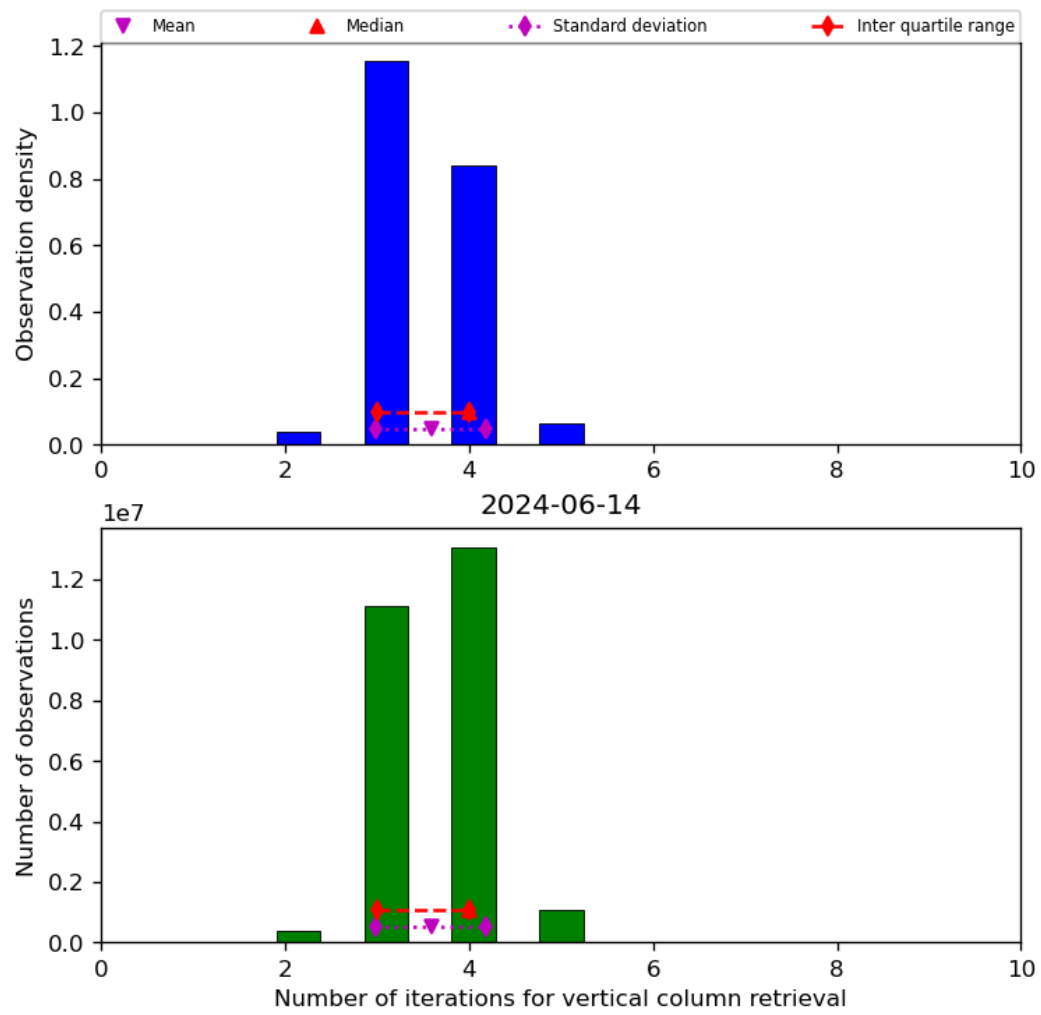
Figure 26: Histogram of “Number of iterations for vertical column retrieval” for 2024-06-13 to 2024-06-15
