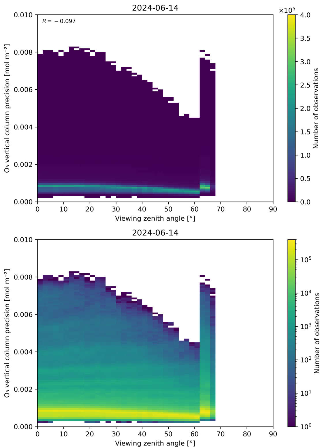
Figure 53: Scatter density plot of “Viewing zenith angle” against “O 3 vertical column precision” for 2024-06-13 to 2024-06-15.
