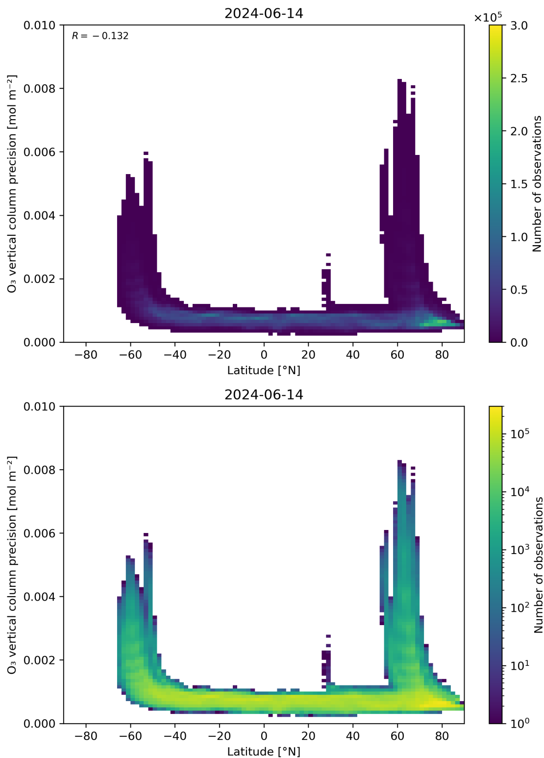
Figure 37: Scatter density plot of “Latitude” against “O 3 vertical column precision” for 2024-06-13 to 2024-06-15.
