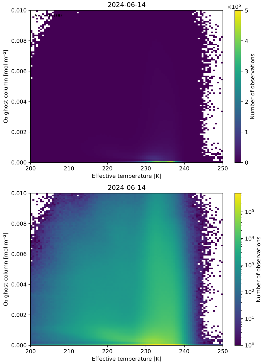
Figure 38: Scatter density plot of “Effective temperature” against “O 3 ghost column” for 2024-06-13 to 2024-06-15.
