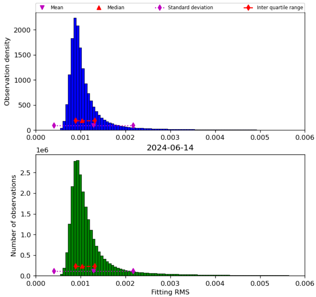
Figure 23: Histogram of “Fitting RMS” for 2024-06-13 to 2024-06-15
