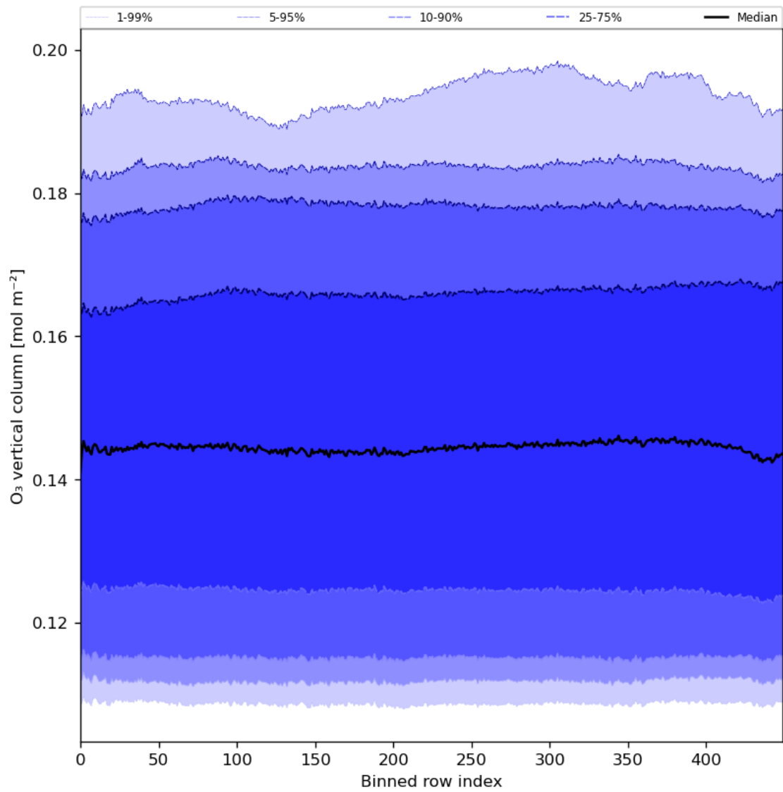
Figure 28: Along track statistics of “O 3 vertical column” for 2024-06-13 to 2024-06-15
