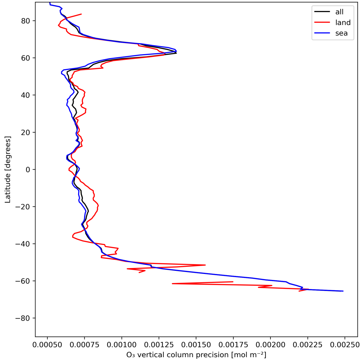
Figure 15: Zonal average of “O 3 vertical column precision” for 2024-06-13 to 2024-06-15.
