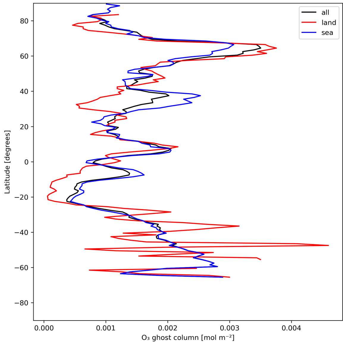
Figure 18: Zonal average of "O 3 ghost column" for 2024-06-13 to 2024-06-15.
