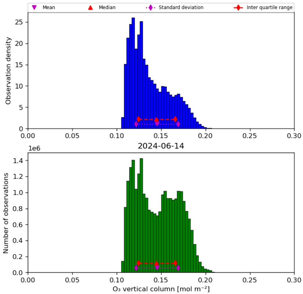
Figure 21: Histogram of “O 3 vertical column” for 2024-06-13 to 2024-06-15
