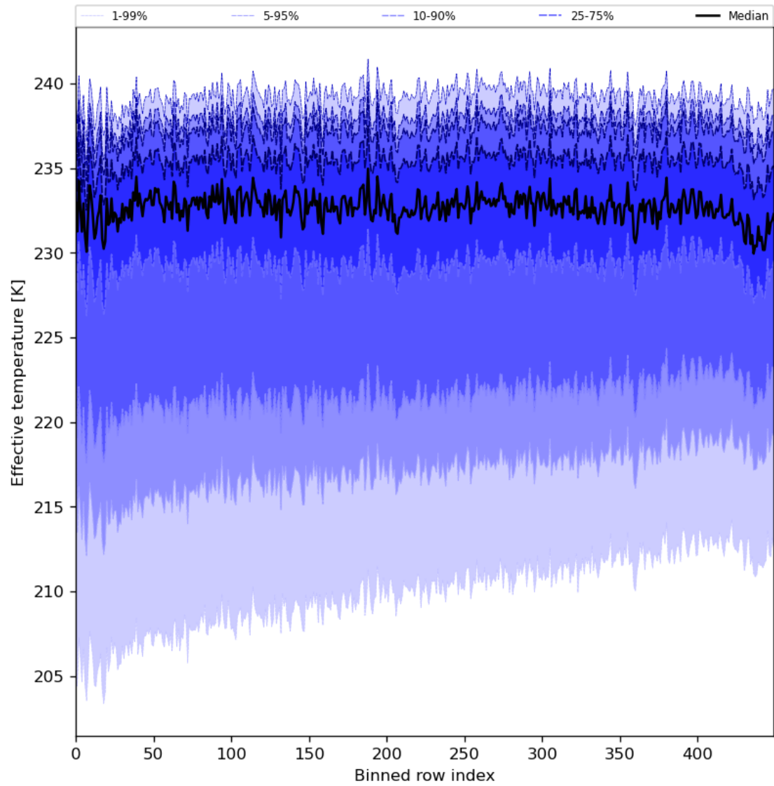
Figure 31: Along track statistics of "Effective temperature" for 2024-06-13 to 2024-06-15
