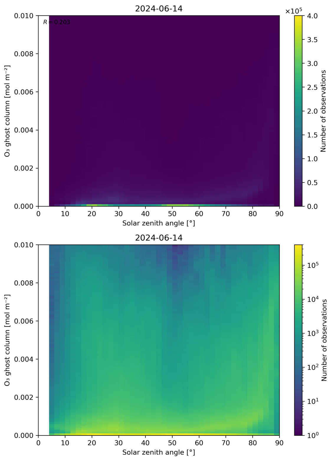
Figure 46: Scatter density plot of “Solar zenith angle” against “O 3 ghost column” for 2024-06-13 to 2024-06-15.
