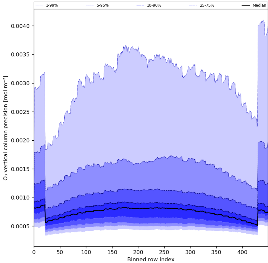
Figure 29: Along track statistics of “O 3 vertical column precision” for 2024-06-13 to 2024-06-15
