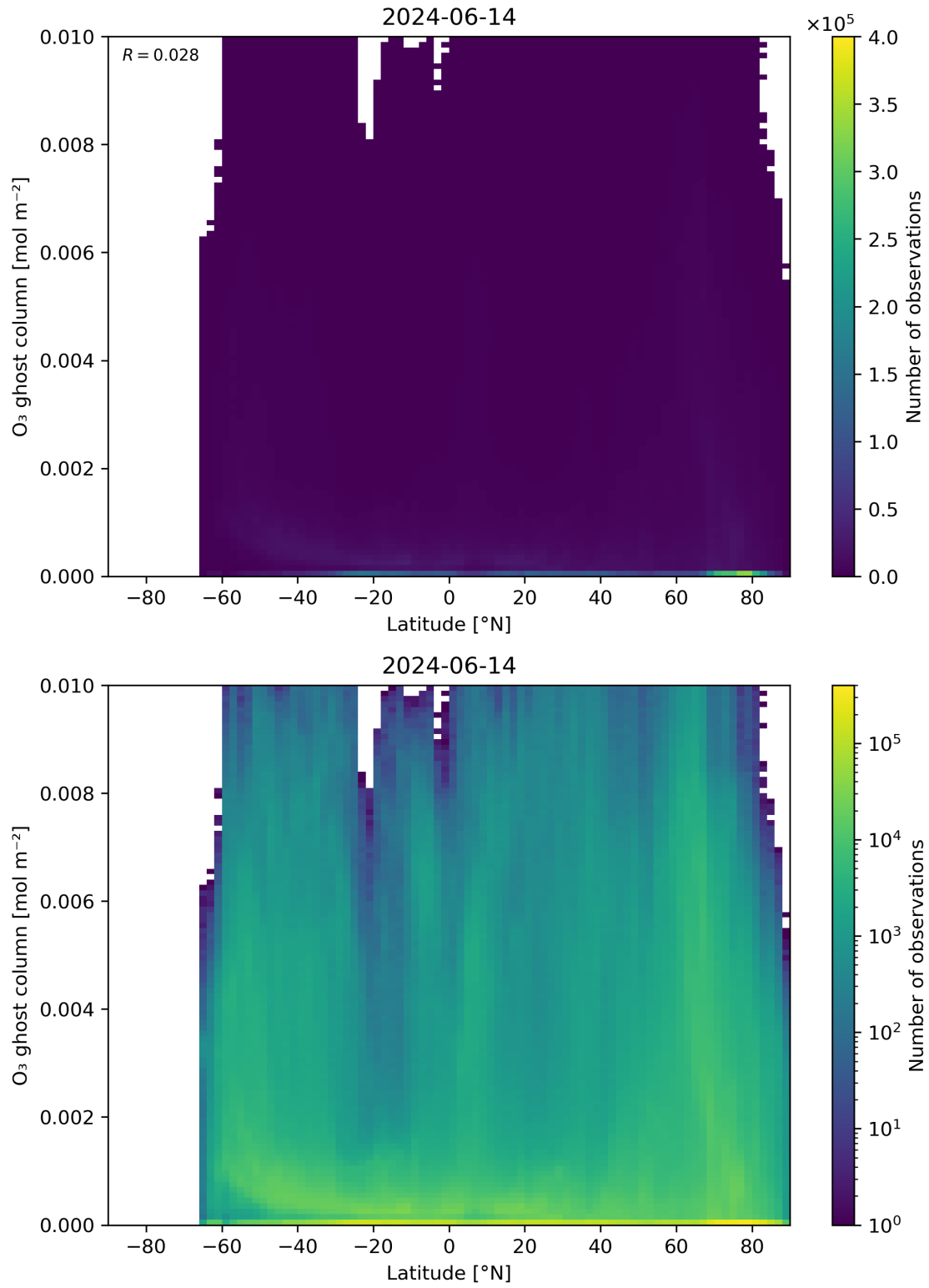
Figure 35: Scatter density plot of “Latitude” against “O 3 ghost column” for 2024-06-13 to 2024-06-15.
