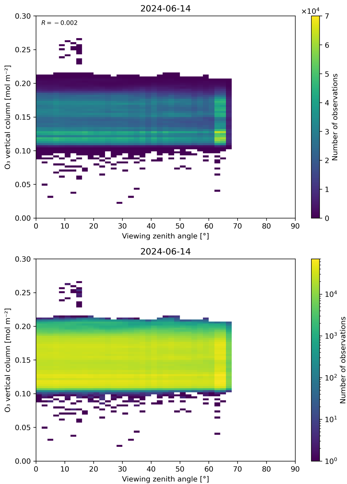
Figure 52: Scatter density plot of “Viewing zenith angle” against “O 3 vertical column” for 2024-06-13 to 2024-06-15.
