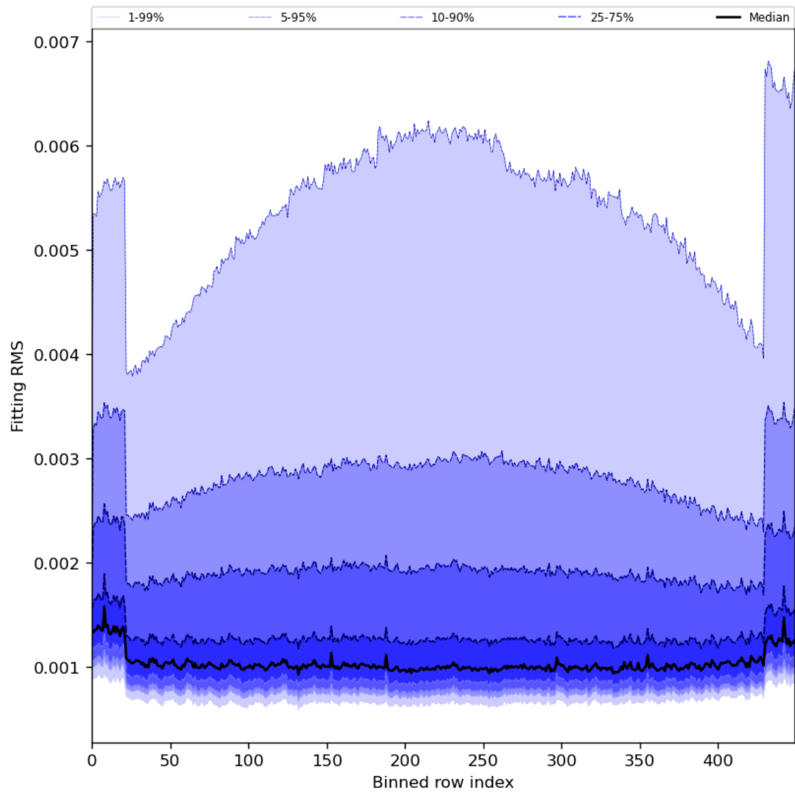
Figure 30: Along track statistics of “Fitting RMS” for 2024-06-13 to 2024-06-15
