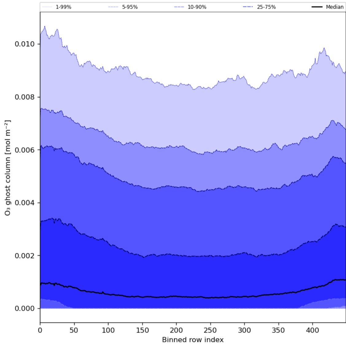
Figure 32: Along track statistics of “O 3 ghost column” for 2024-06-13 to 2024-06-15
