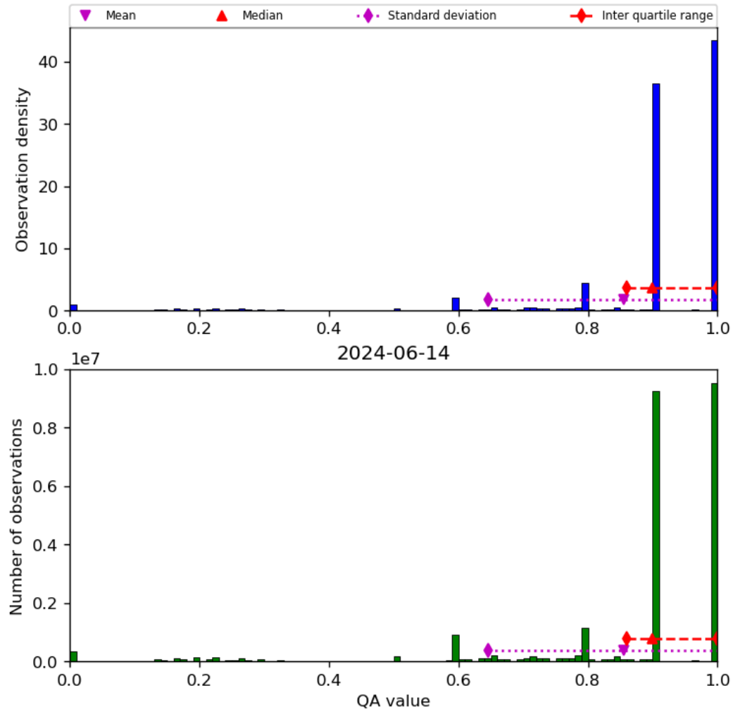
Figure 20: Histogram of “QA value” for 2024-06-13 to 2024-06-15
