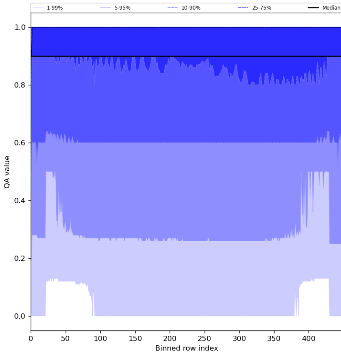
Figure 27: Along track statistics of “QA value” for 2024-06-13 to 2024-06-15
