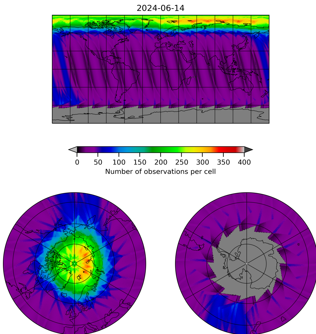
Figure 12: Map of the number of observations for 2024-06-13 to 2024-06-15
