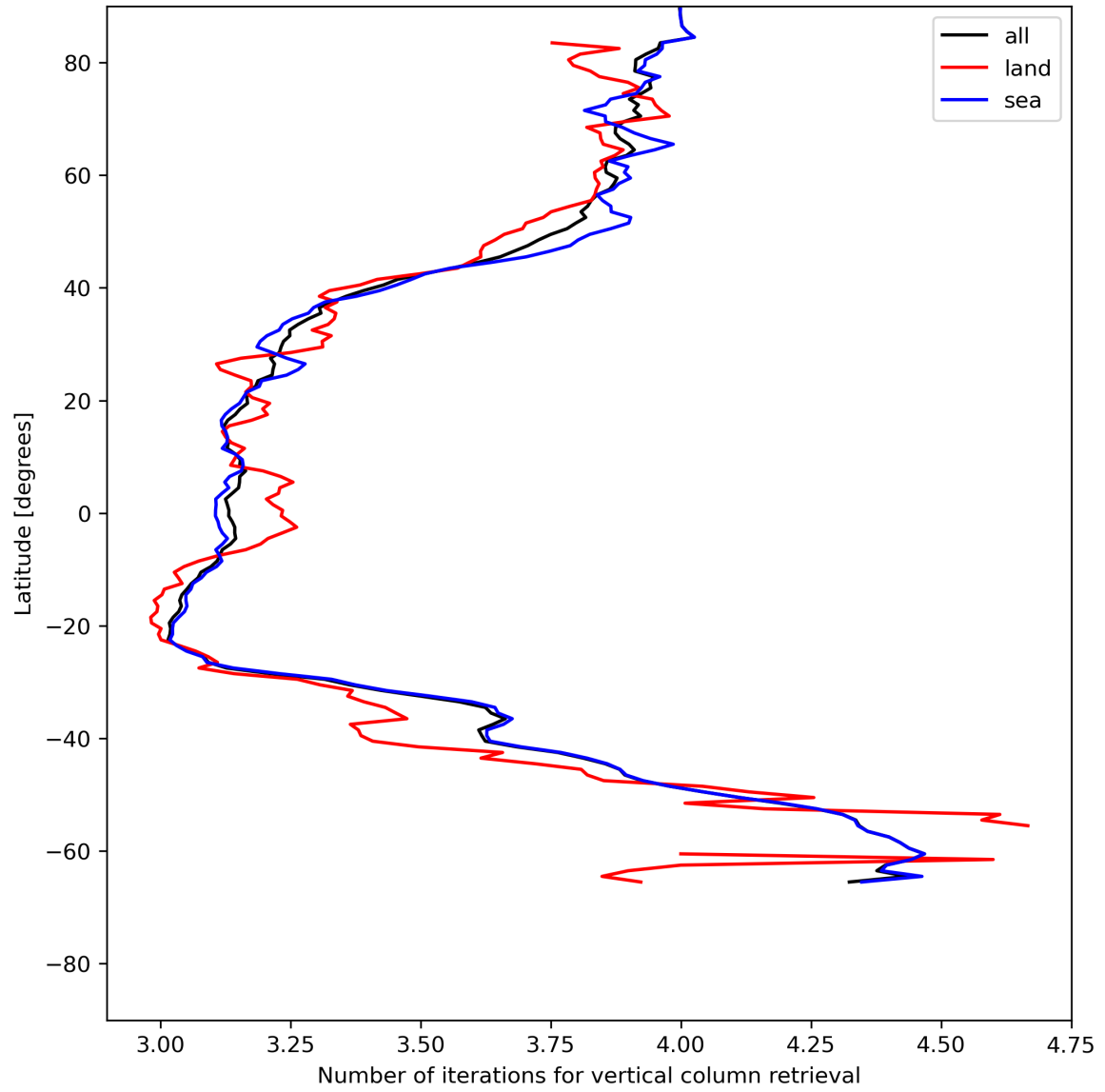
Figure 19: Zonal average of “Number of iterations for vertical column retrieval” for 2024-06-13 to 2024-06-15.
