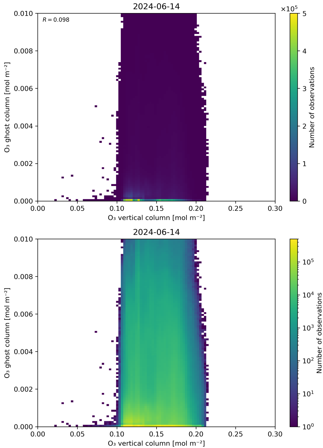
Figure 40: Scatter density plot of “O 3 vertical column” against “O 3 ghost column” for 2024-06-13 to 2024-06-15.
