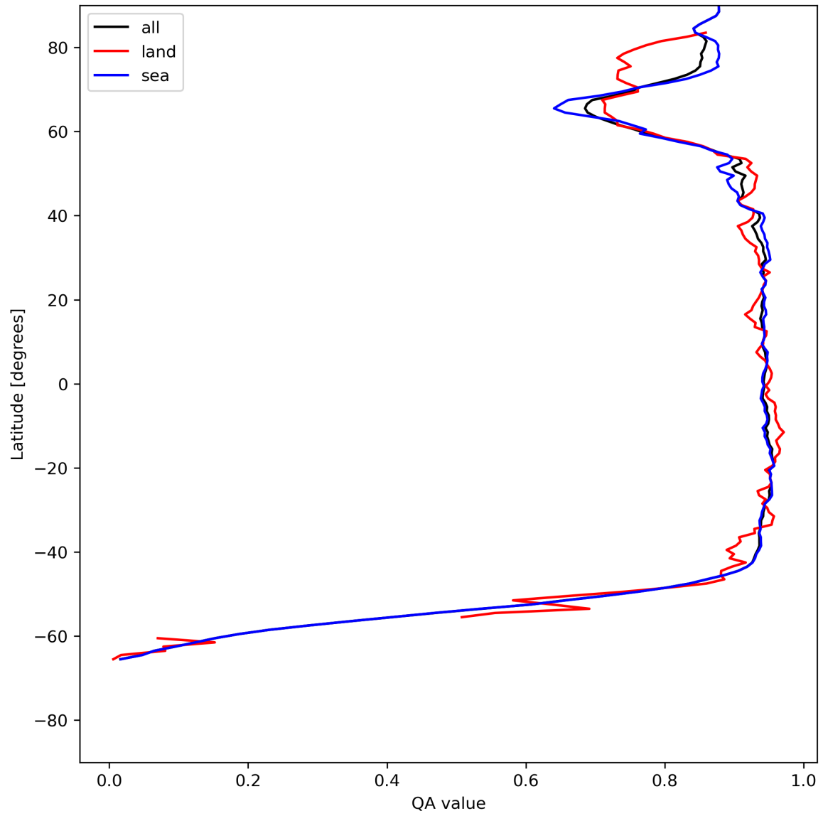
Figure 13: Zonal average of “QA value” for 2024-06-13 to 2024-06-15.
