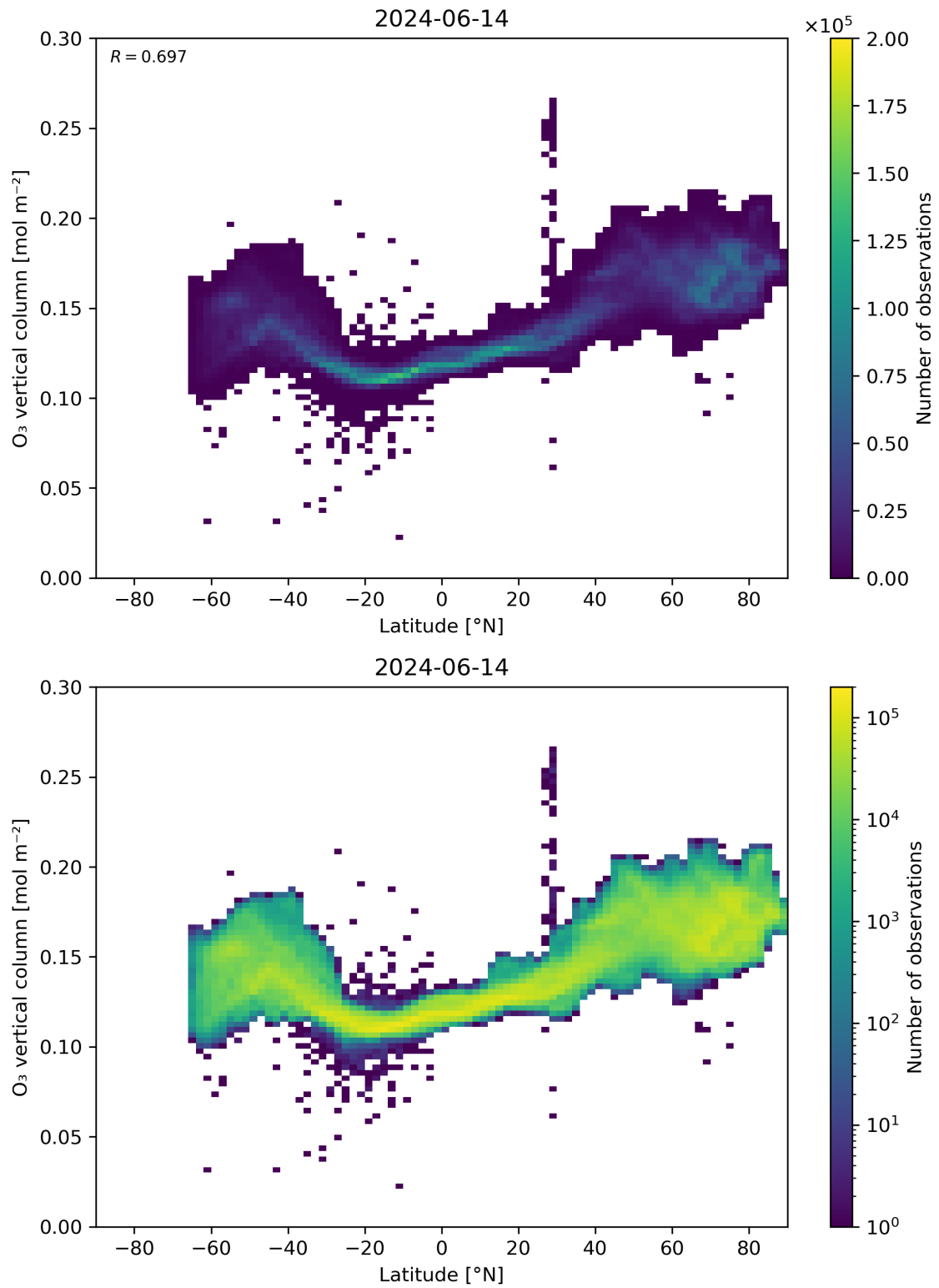
Figure 36: Scatter density plot of “Latitude” against “O 3 vertical column” for 2024-06-13 to 2024-06-15.
