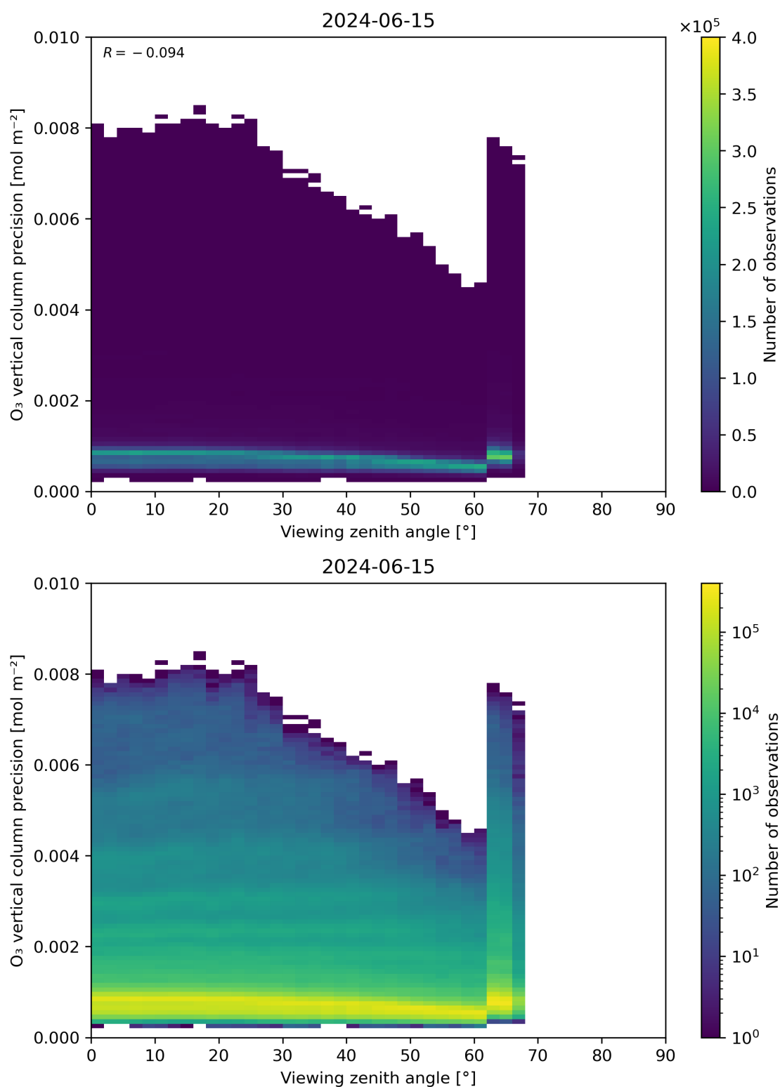
Figure 53: Scatter density plot of “Viewing zenith angle” against “O 3 vertical column precision” for 2024-06-14 to 2024-06-16.
