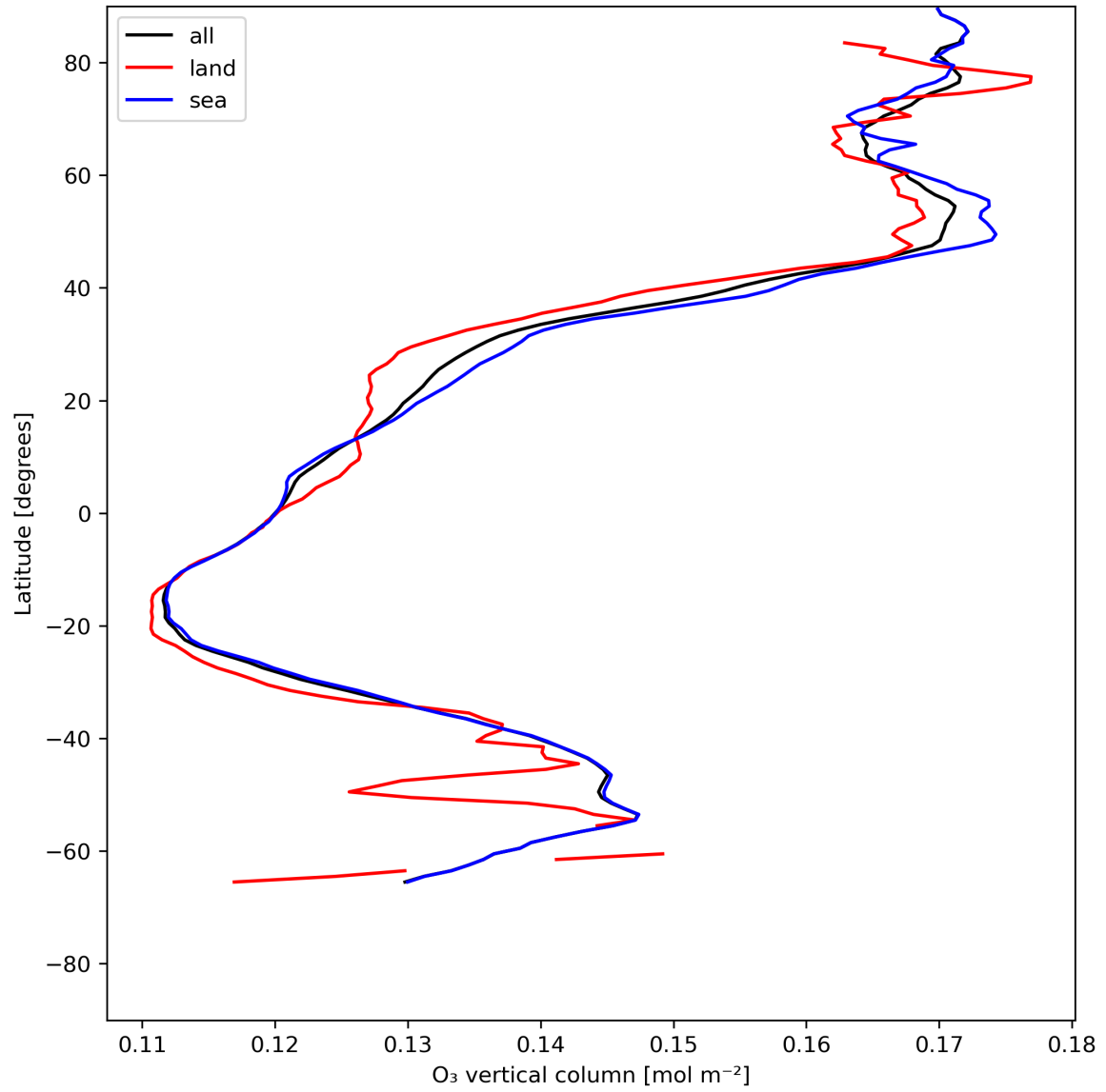
Figure 14: Zonal average of “O 3 vertical column” for 2024-06-14 to 2024-06-16.
