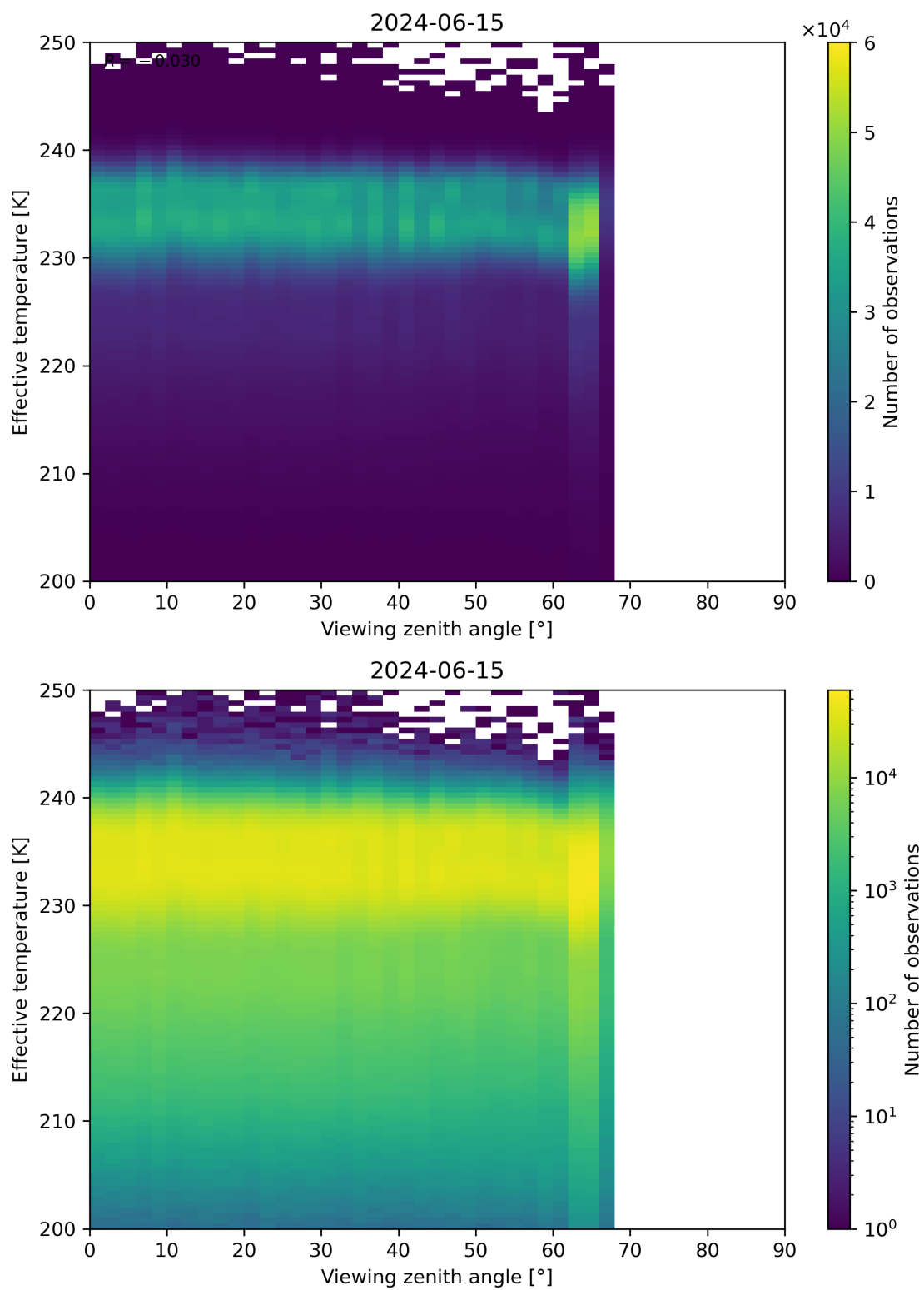
Figure 50: Scatter density plot of “Viewing zenith angle” against “Effective temperature” for 2024-06-14 to 2024-06-16.
