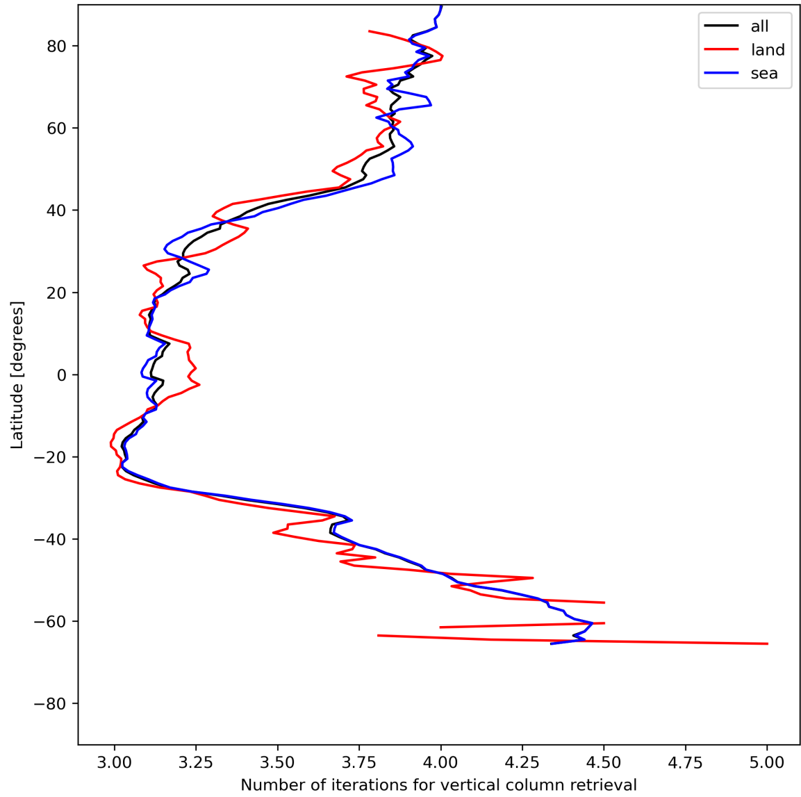
Figure 19: Zonal average of “Number of iterations for vertical column retrieval” for 2024-06-14 to 2024-06-16.
