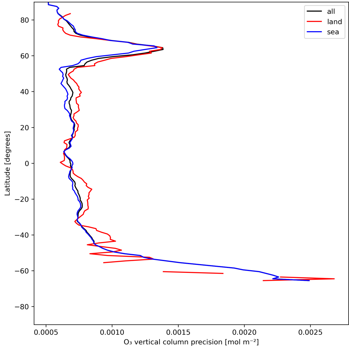
Figure 15: Zonal average of “O 3 vertical column precision” for 2024-06-14 to 2024-06-16.
