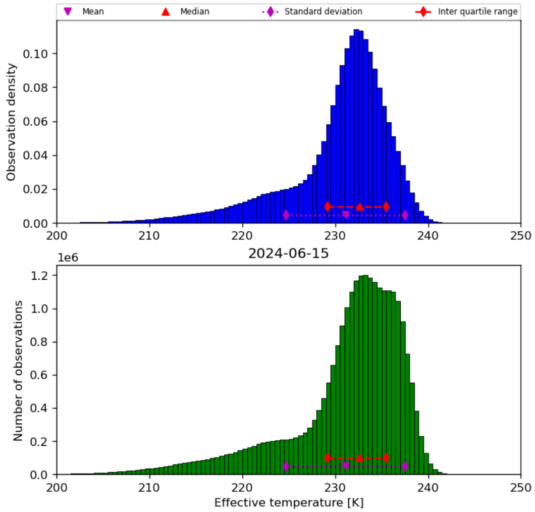
Figure 24: Histogram of “Effective temperature” for 2024-06-14 to 2024-06-16
