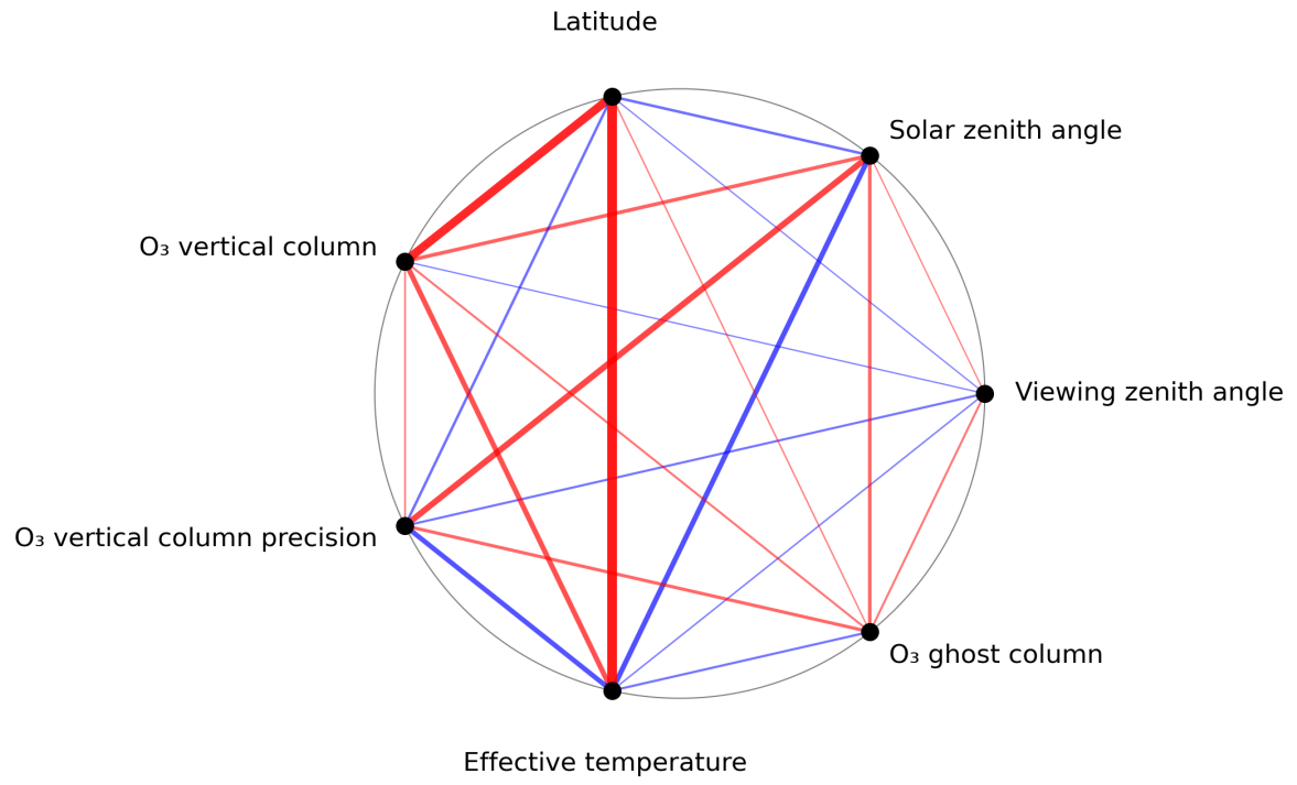
Figure 1: Map of correlation graph for 2024-06-14 to 2024-06-16.
