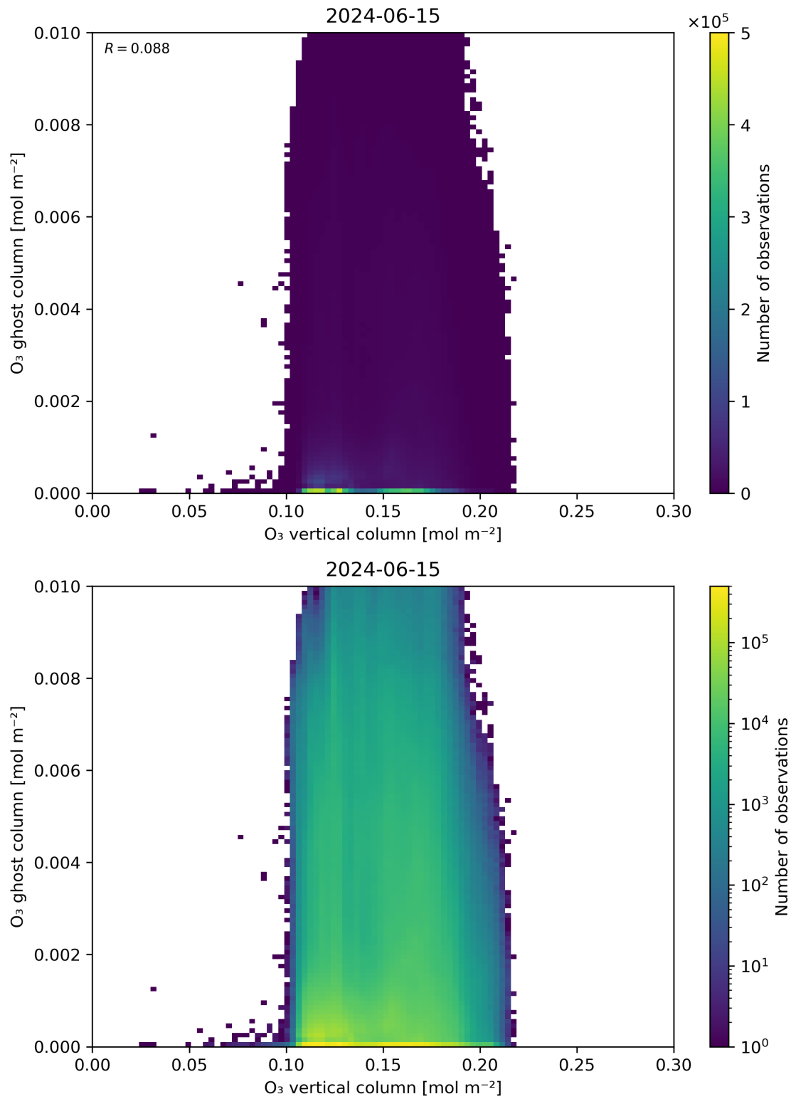
Figure 40: Scatter density plot of “O 3 vertical column” against “O 3 ghost column” for 2024-06-14 to 2024-06-16.
