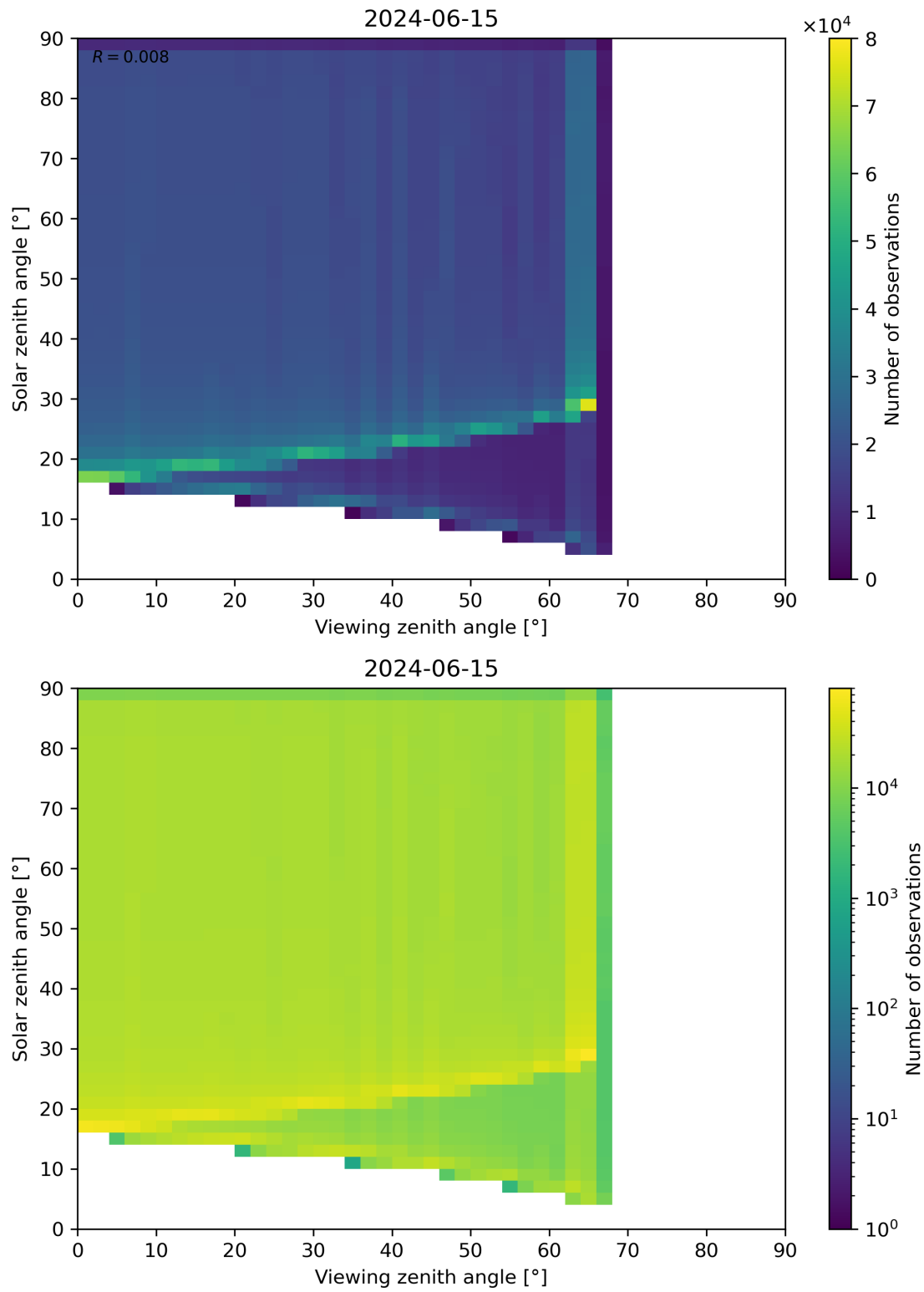
Figure 54: Scatter density plot of “Viewing zenith angle” against “Solar zenith angle” for 2024-06-14 to 2024-06-16.
