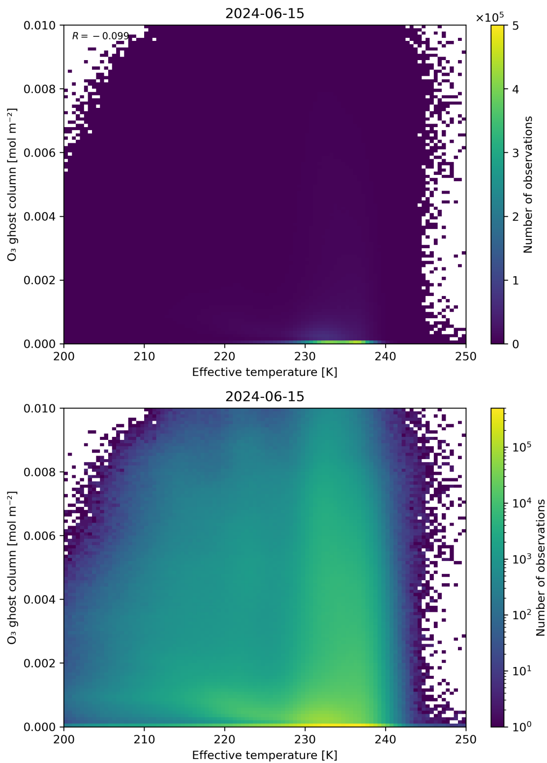
Figure 38: Scatter density plot of “Effective temperature” against “O 3 ghost column” for 2024-06-14 to 2024-06-16.
