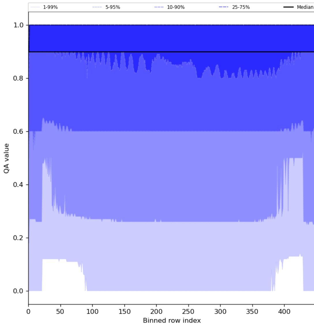
Figure 27: Along track statistics of “QA value” for 2024-06-14 to 2024-06-16
