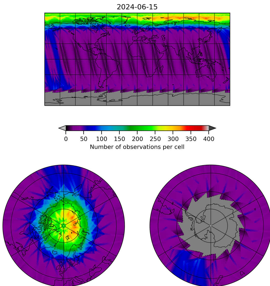
Figure 12: Map of the number of observations for 2024-06-14 to 2024-06-16
