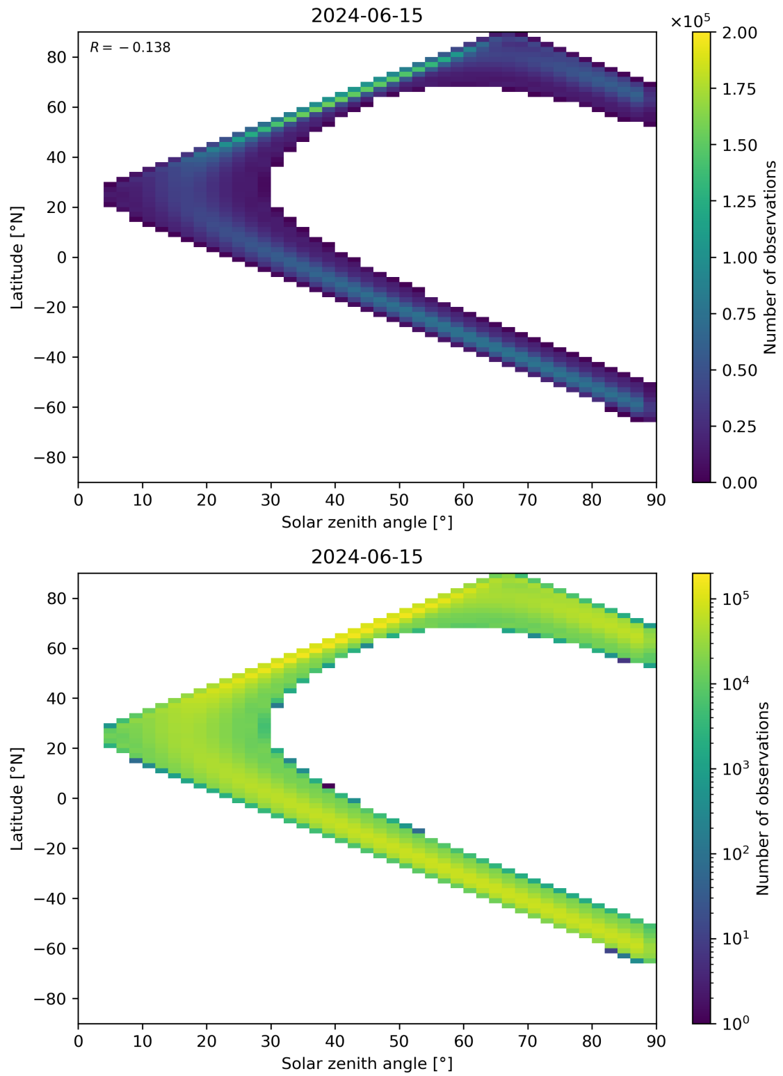
Figure 44: Scatter density plot of “Solar zenith angle” against “Latitude” for 2024-06-14 to 2024-06-16.
