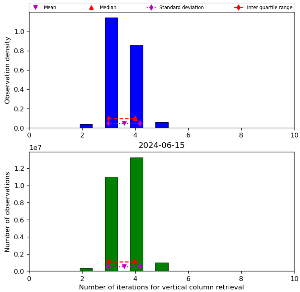
Figure 26: Histogram of “Number of iterations for vertical column retrieval” for 2024-06-14 to 2024-06-16
