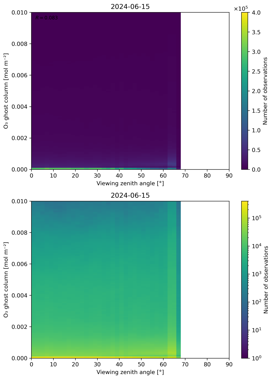
Figure 51: Scatter density plot of “Viewing zenith angle” against “O 3 ghost column” for 2024-06-14 to 2024-06-16.
