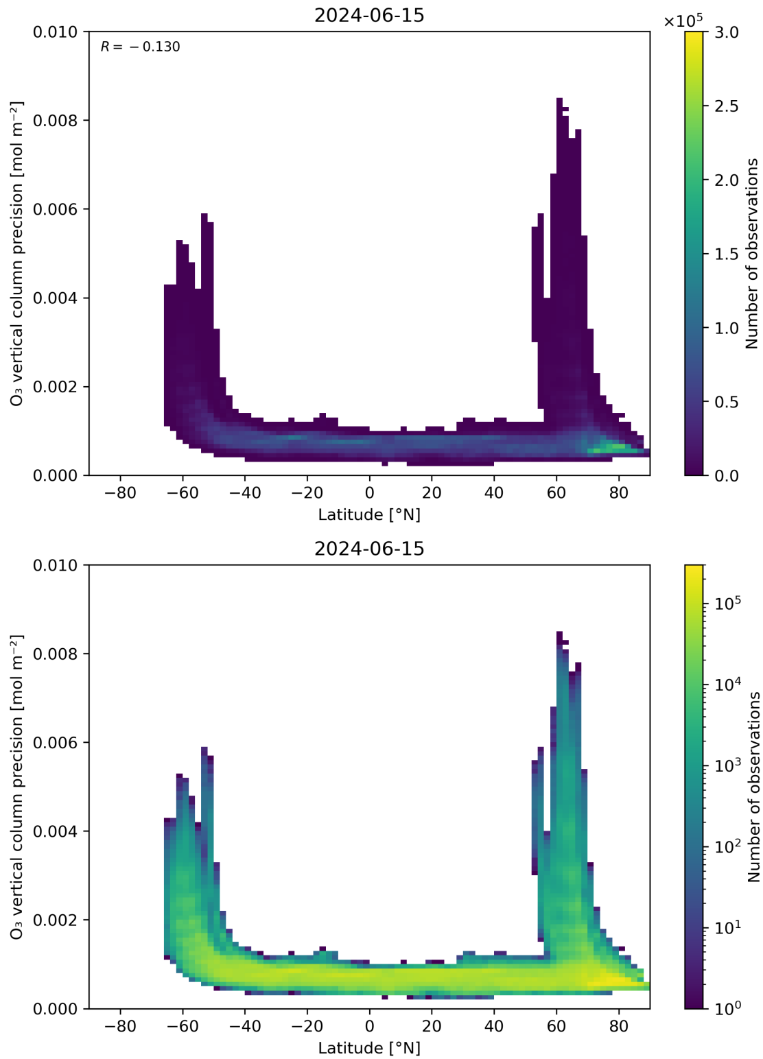
Figure 37: Scatter density plot of “Latitude” against “O 3 vertical column precision” for 2024-06-14 to 2024-06-16.
