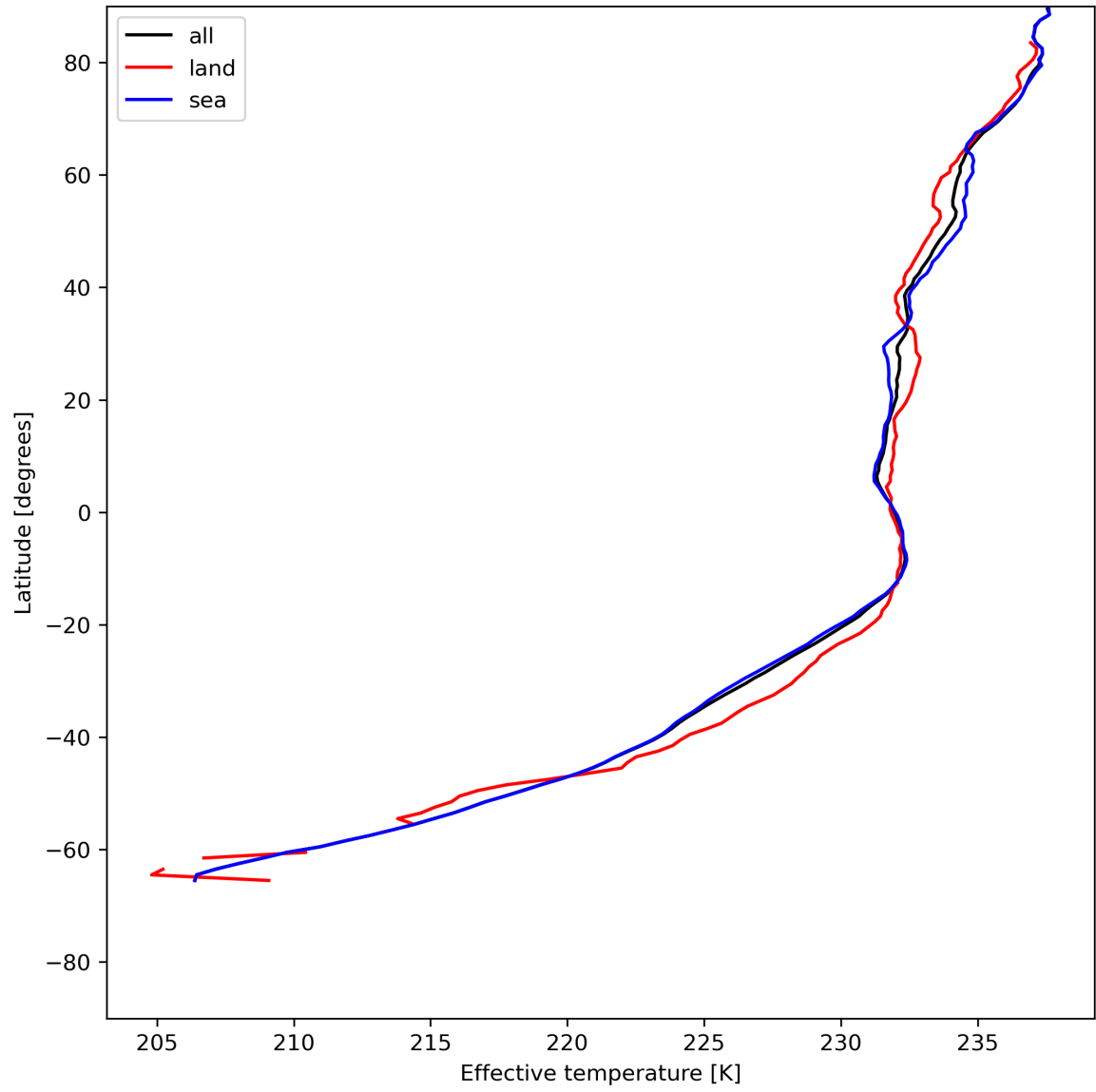
Figure 17: Zonal average of "Effective temperature" for 2024-06-14 to 2024-06-16.
