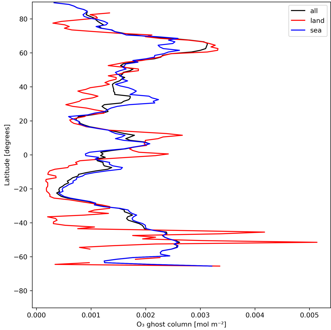
Figure 18: Zonal average of "O 3 ghost column" for 2024-06-14 to 2024-06-16.
