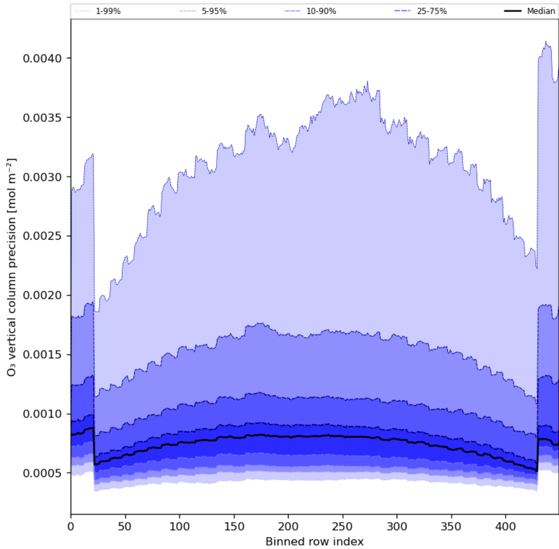
Figure 29: Along track statistics of “O 3 vertical column precision” for 2024-06-14 to 2024-06-16
