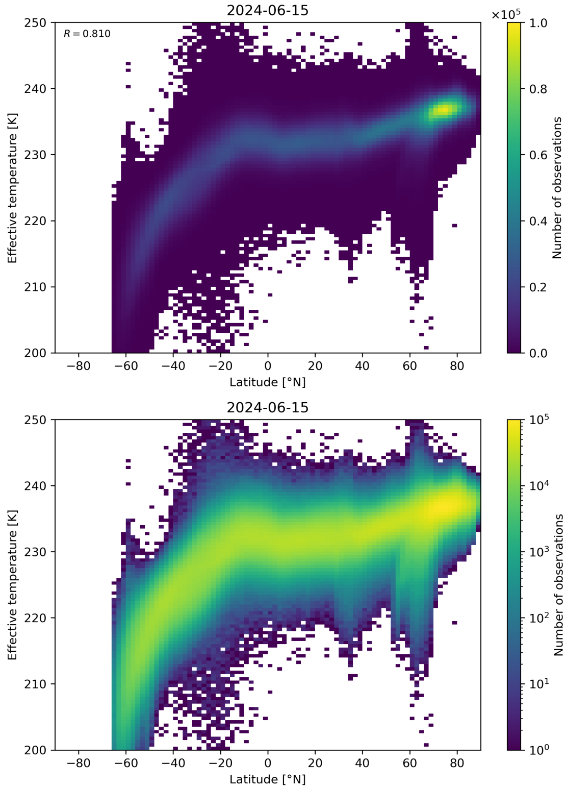
Figure 34: Scatter density plot of “Latitude” against “Effective temperature” for 2024-06-14 to 2024-06-16.
