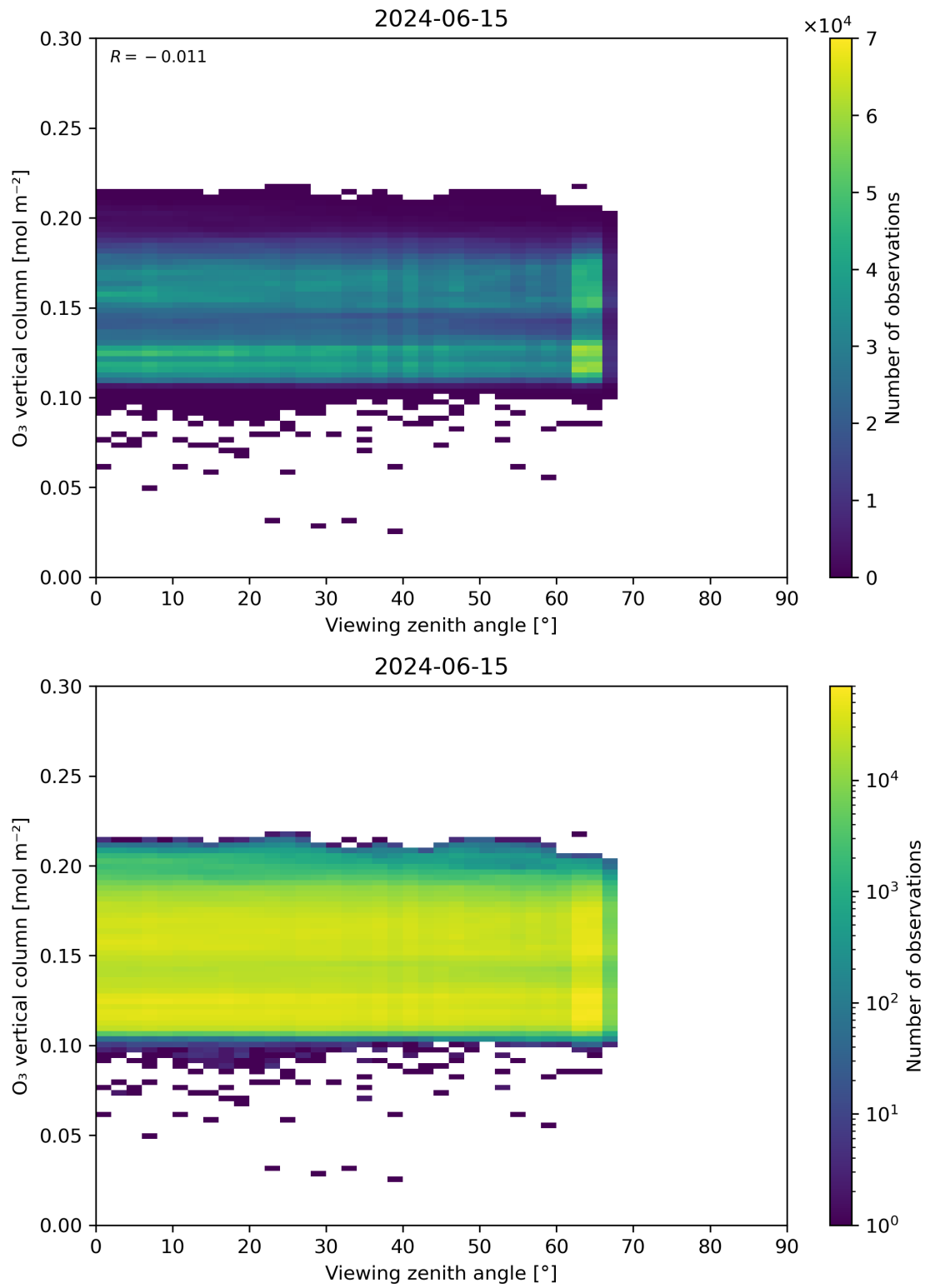
Figure 52: Scatter density plot of “Viewing zenith angle” against “O 3 vertical column” for 2024-06-14 to 2024-06-16.
