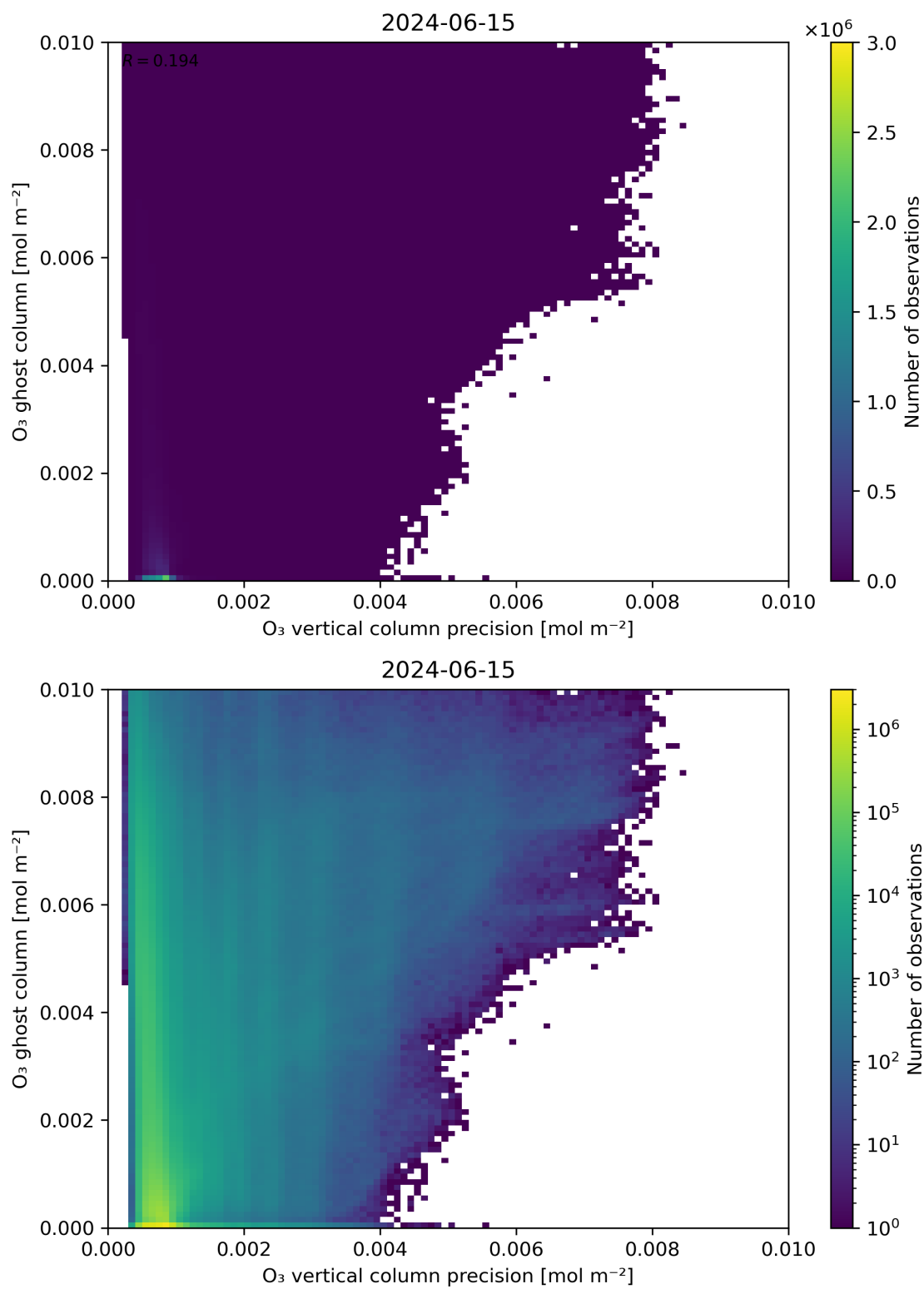
Figure 43: Scatter density plot of “ \text{O}_3 vertical column precision” against “ \text{O}_3 ghost column” for 2024-06-14 to 2024-06-16.
