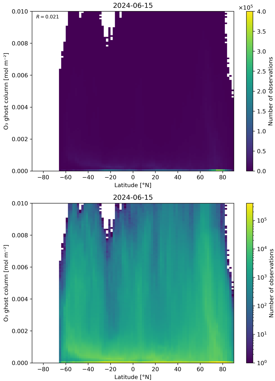
Figure 35: Scatter density plot of “Latitude” against “O 3 ghost column” for 2024-06-14 to 2024-06-16.
