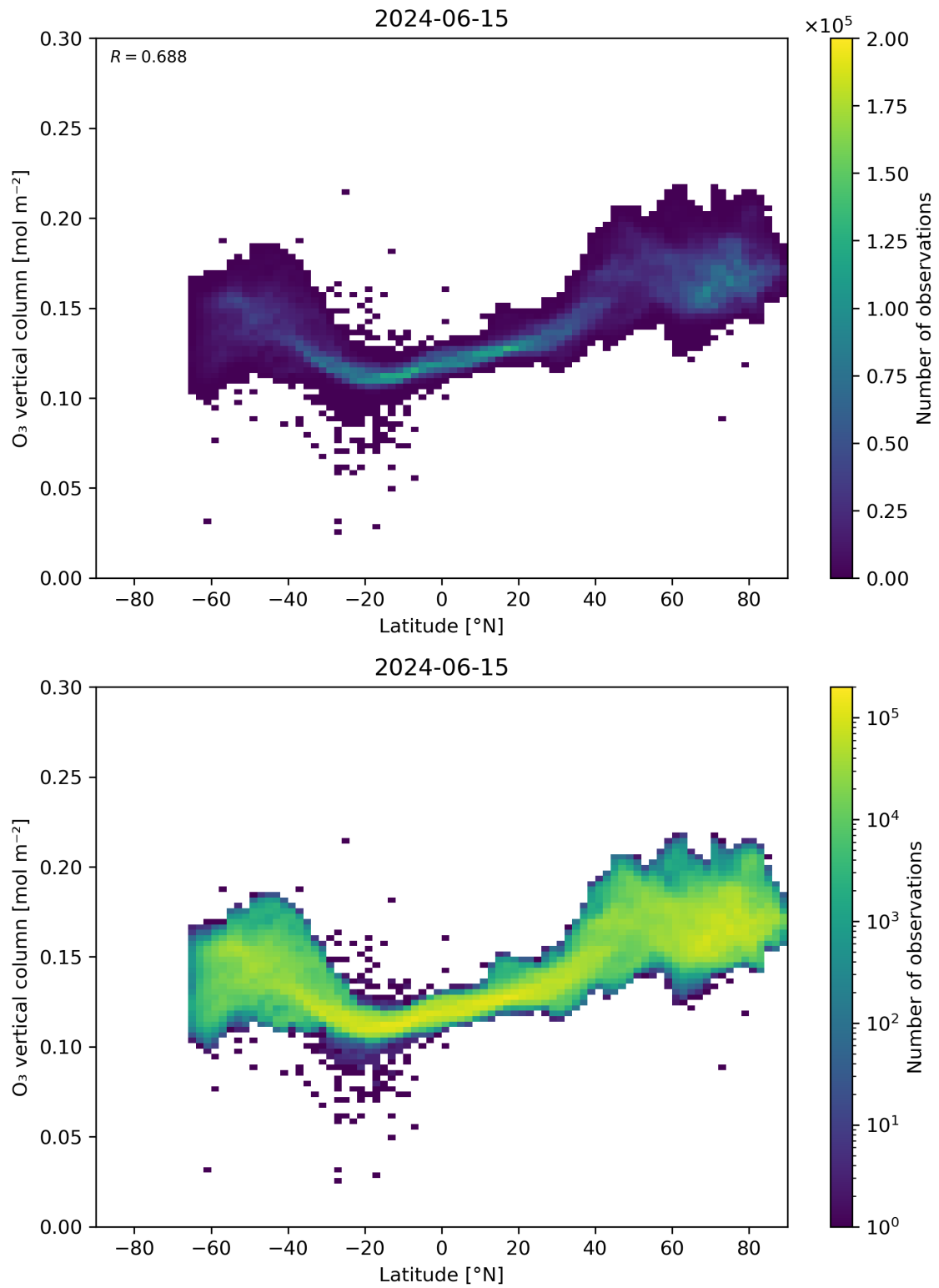
Figure 36: Scatter density plot of “Latitude” against “O 3 vertical column” for 2024-06-14 to 2024-06-16.
