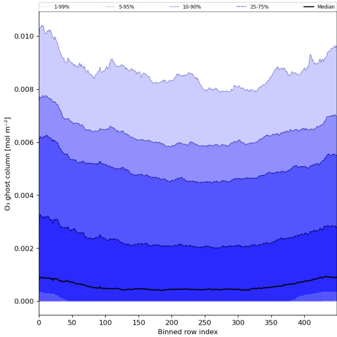
Figure 32: Along track statistics of “O 3 ghost column” for 2024-06-14 to 2024-06-16
