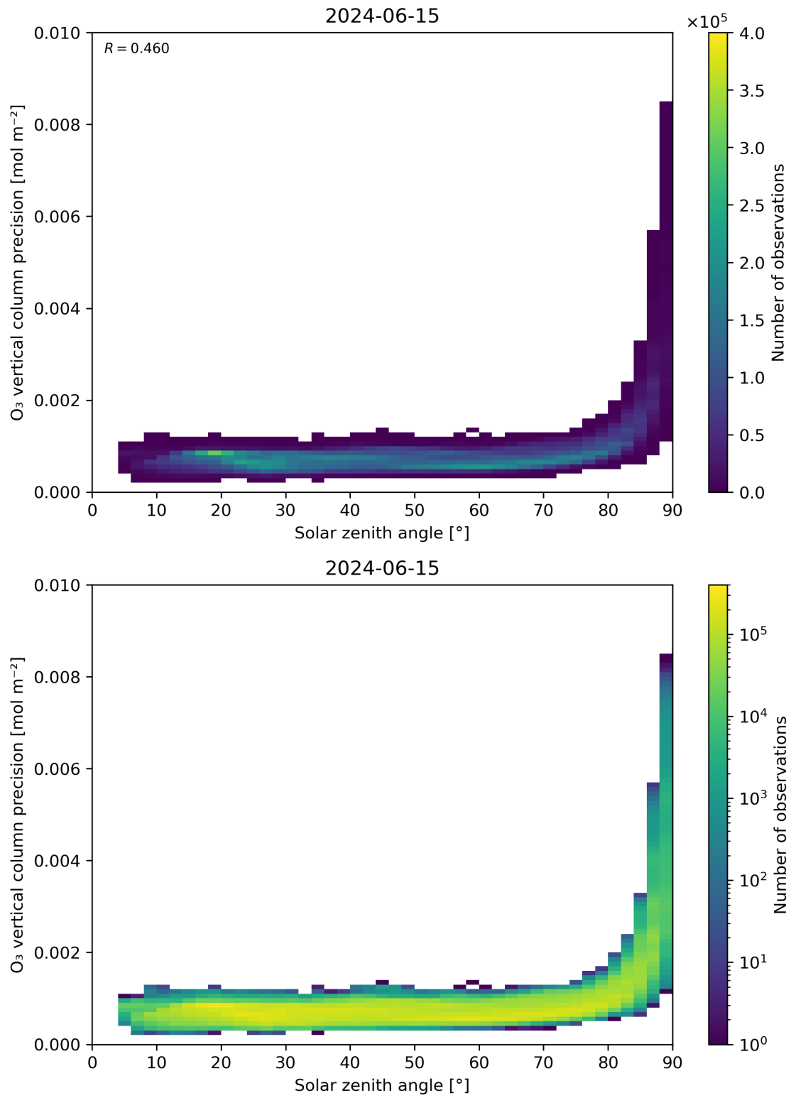
Figure 48: Scatter density plot of “Solar zenith angle” against “O 3 vertical column precision” for 2024-06-14 to 2024-06-16.
