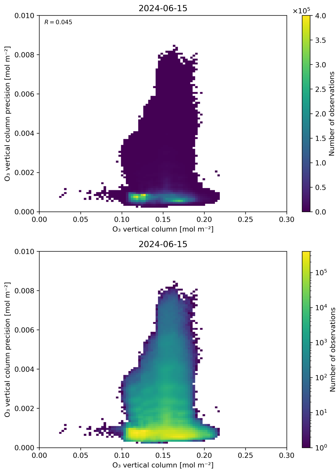
Figure 41: Scatter density plot of “O 3 vertical column” against “O 3 vertical column precision” for 2024-06-14 to 2024-06-16.
