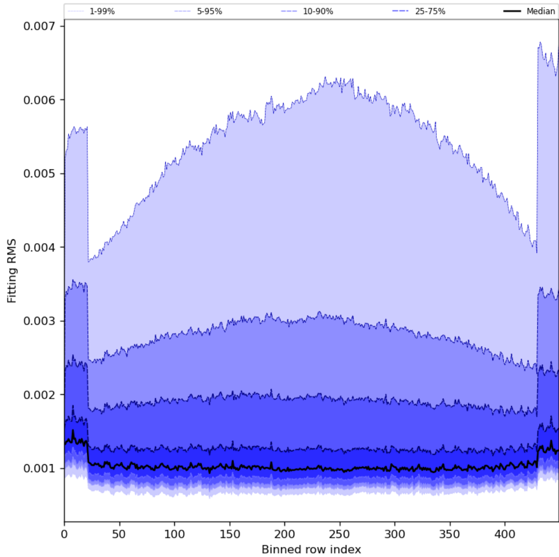
Figure 30: Along track statistics of “Fitting RMS” for 2024-06-14 to 2024-06-16
