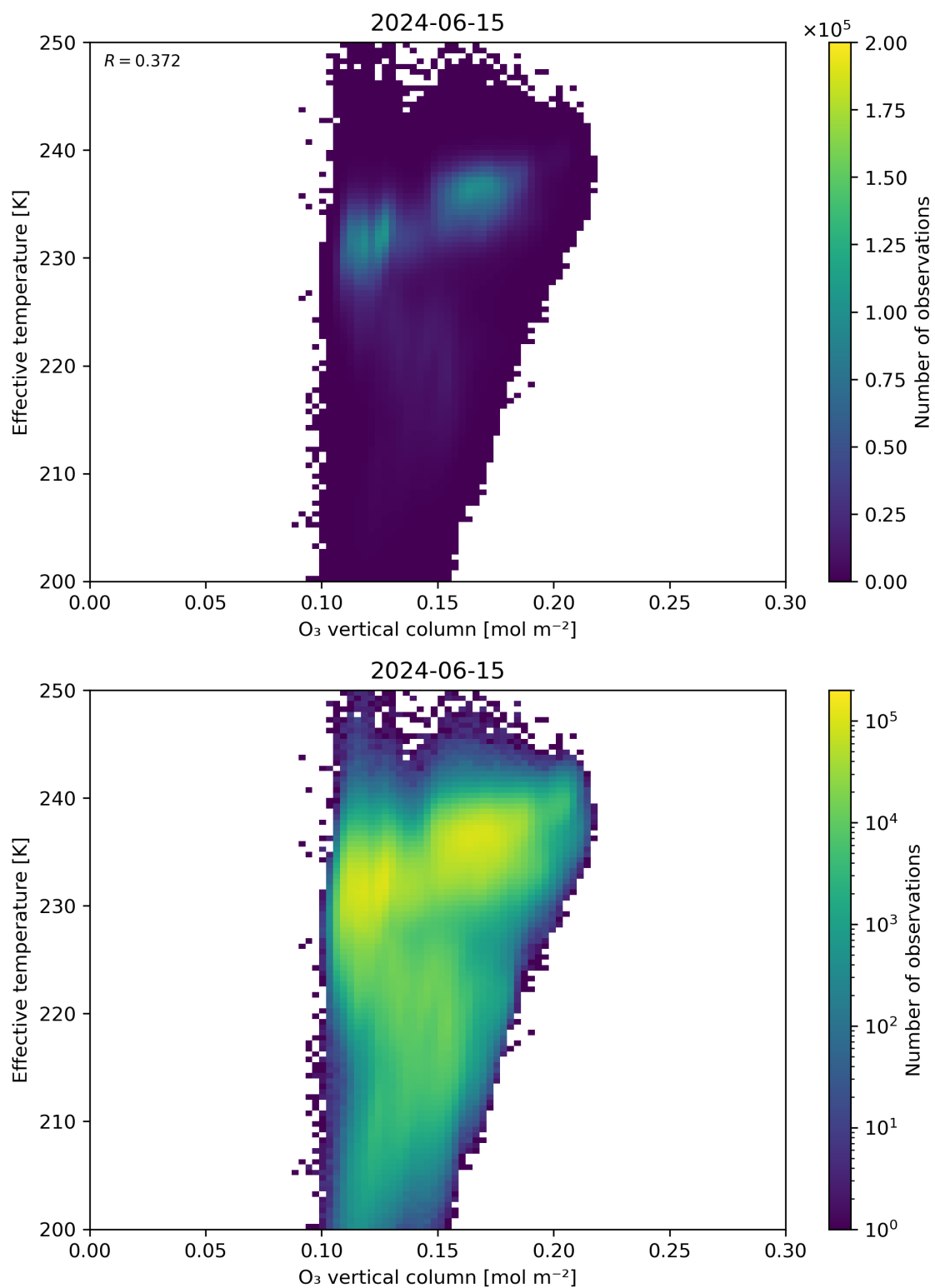
Figure 39: Scatter density plot of “O 3 vertical column” against “Effective temperature” for 2024-06-14 to 2024-06-16.
