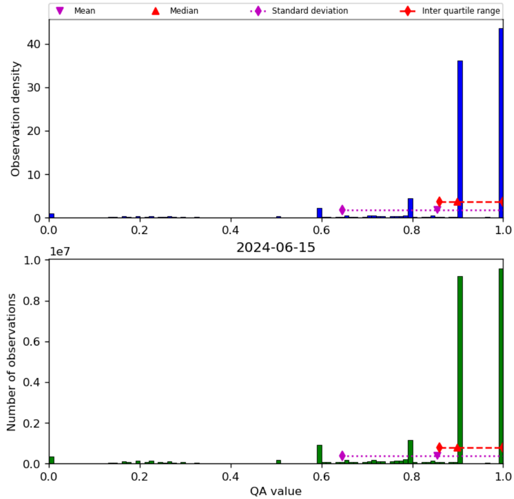
Figure 20: Histogram of “QA value” for 2024-06-14 to 2024-06-16
