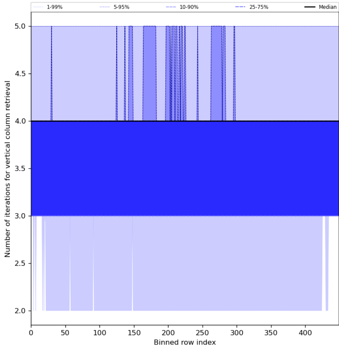
Figure 33: Along track statistics of “Number of iterations for vertical column retrieval” for 2024-06-14 to 2024-06-16
