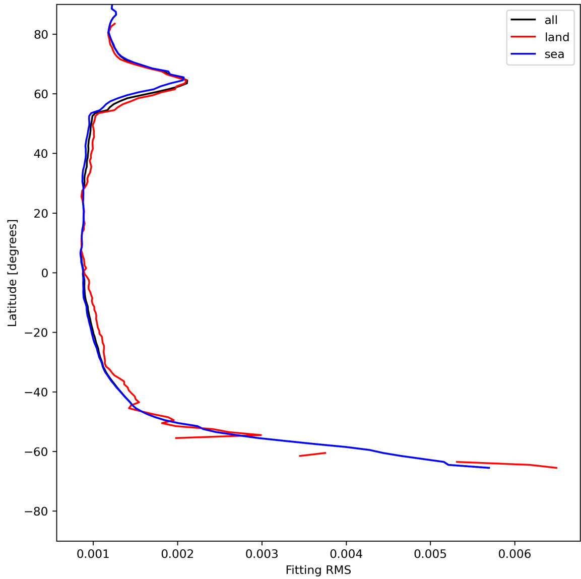
Figure 16: Zonal average of “Fitting RMS” for 2024-06-14 to 2024-06-16.
