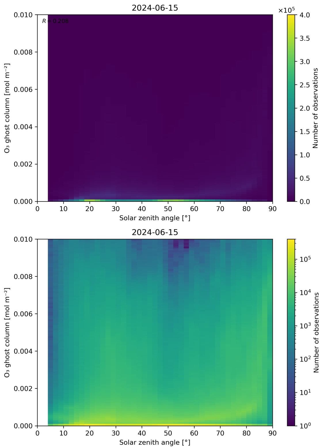
Figure 46: Scatter density plot of “Solar zenith angle” against “O 3 ghost column” for 2024-06-14 to 2024-06-16.
