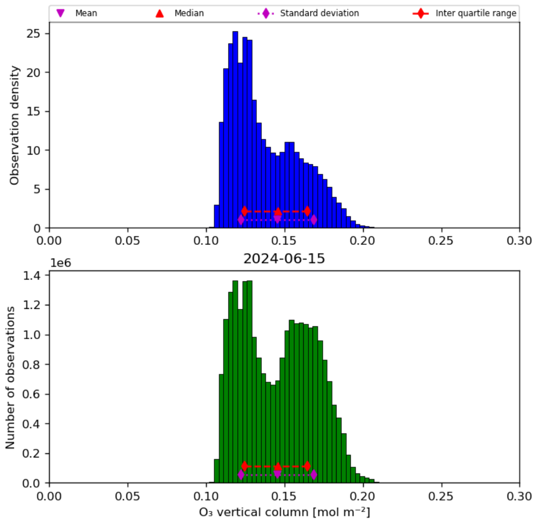
Figure 21: Histogram of “O 3 vertical column” for 2024-06-14 to 2024-06-16
