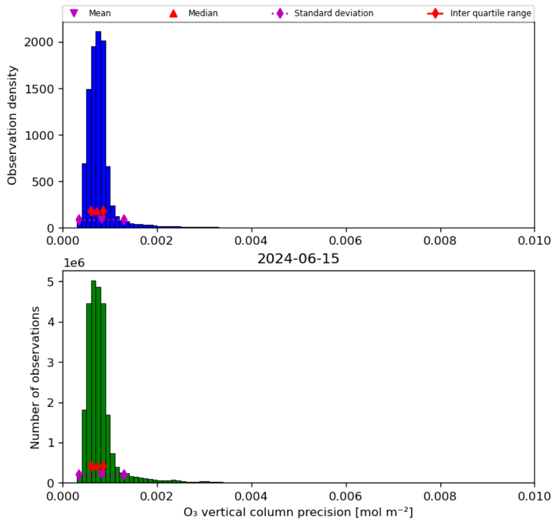
Figure 22: Histogram of “O 3 vertical column precision” for 2024-06-14 to 2024-06-16
