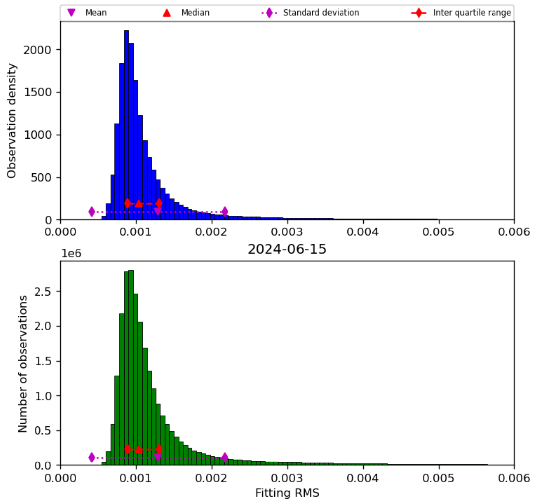
Figure 23: Histogram of “Fitting RMS” for 2024-06-14 to 2024-06-16
