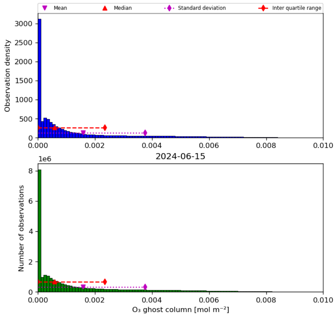
Figure 25: Histogram of “O 3 ghost column” for 2024-06-14 to 2024-06-16
