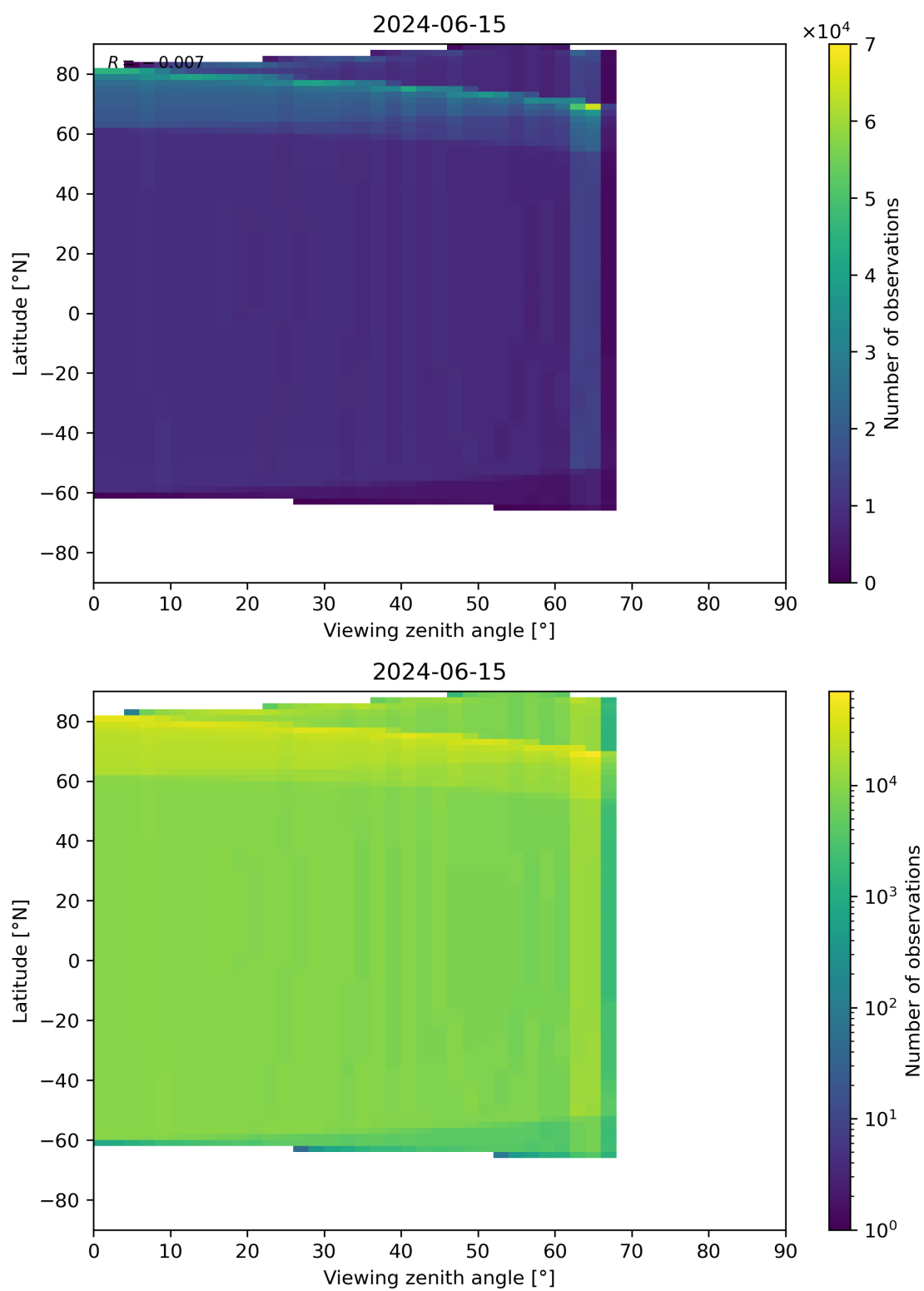
Figure 49: Scatter density plot of “Viewing zenith angle” against “Latitude” for 2024-06-14 to 2024-06-16.
