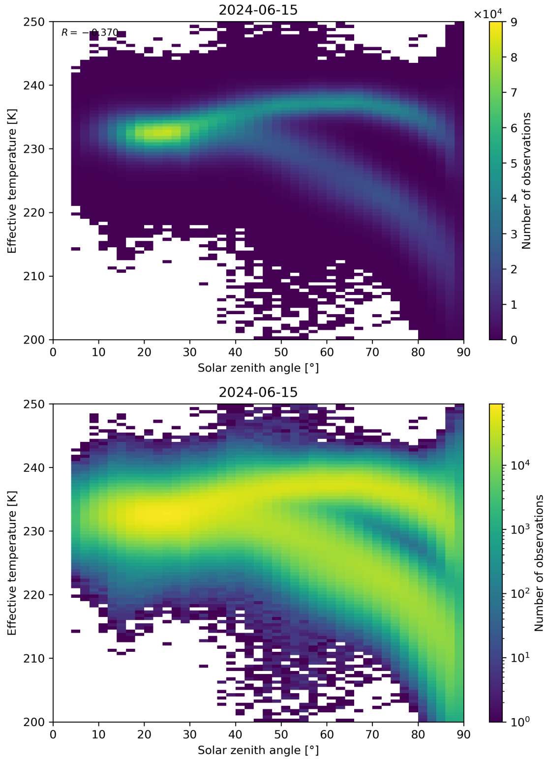
Figure 45: Scatter density plot of “Solar zenith angle” against “Effective temperature” for 2024-06-14 to 2024-06-16.
