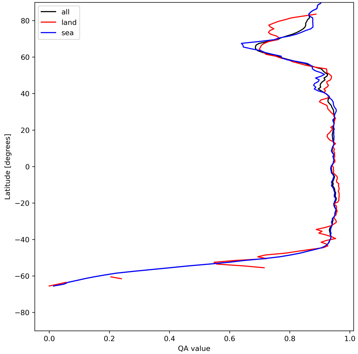
Figure 13: Zonal average of “QA value” for 2024-06-14 to 2024-06-16.
