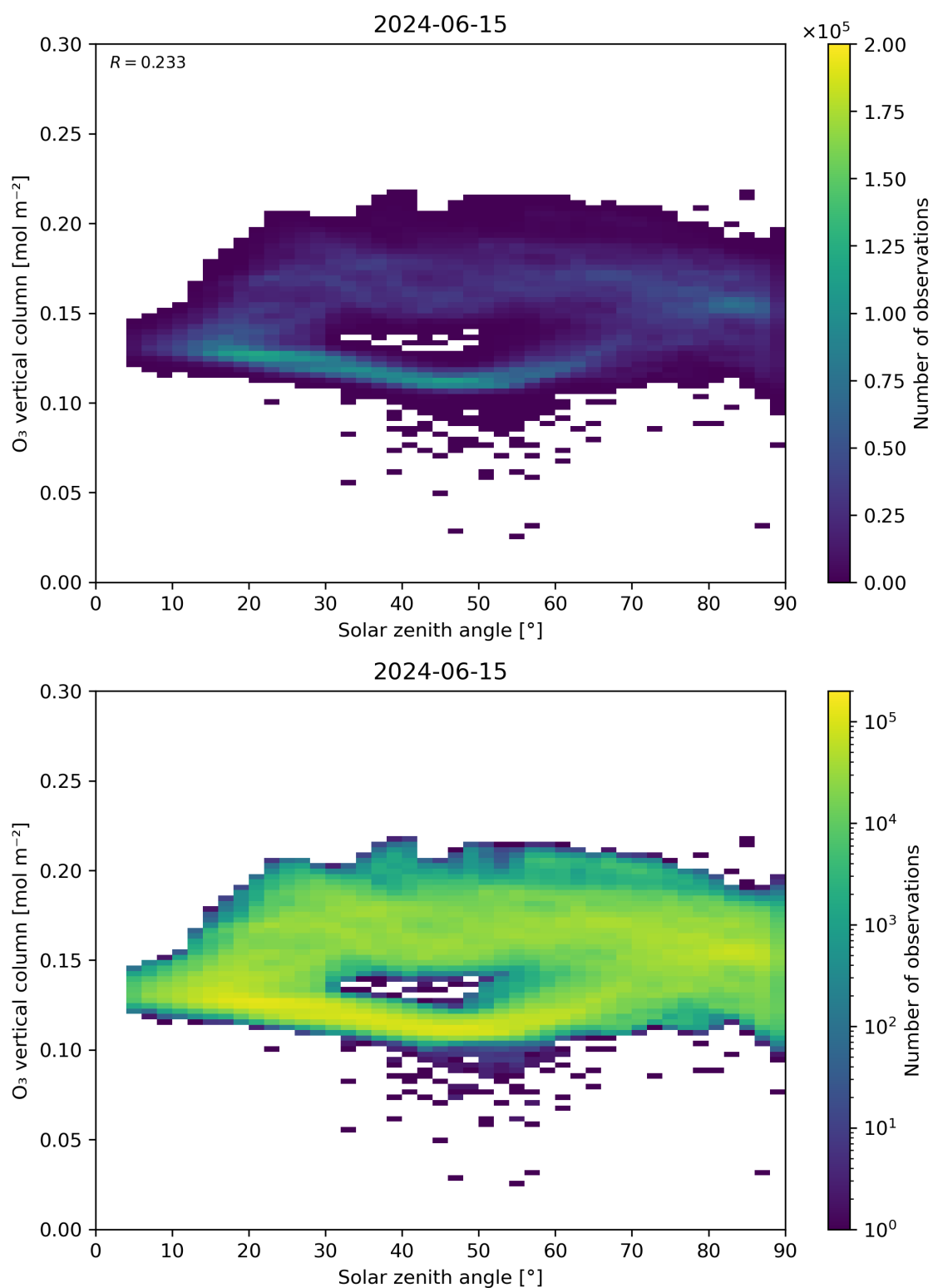
Figure 47: Scatter density plot of “Solar zenith angle” against “O 3 vertical column” for 2024-06-14 to 2024-06-16.
