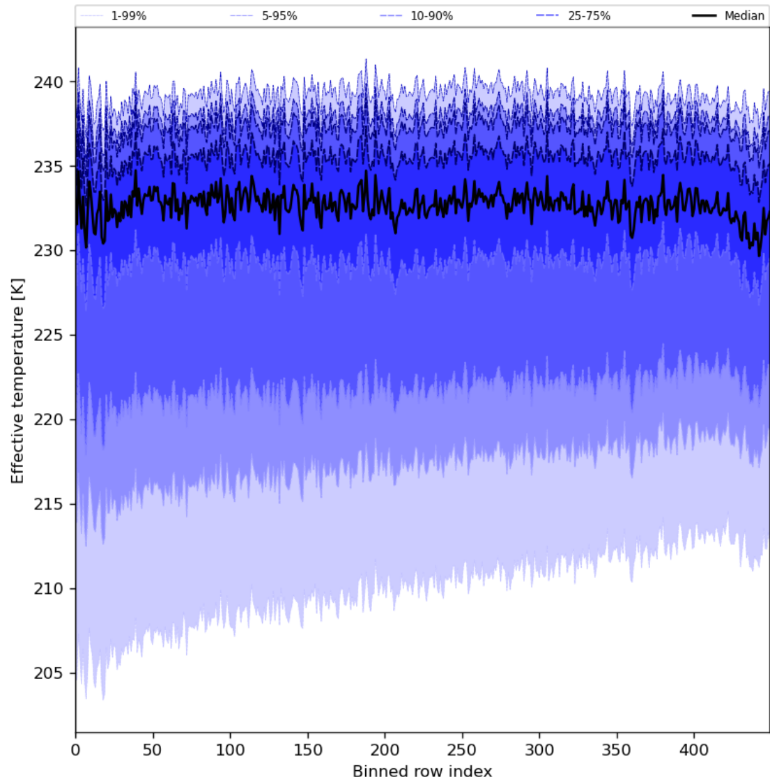
Figure 31: Along track statistics of “Effective temperature” for 2024-06-14 to 2024-06-16
