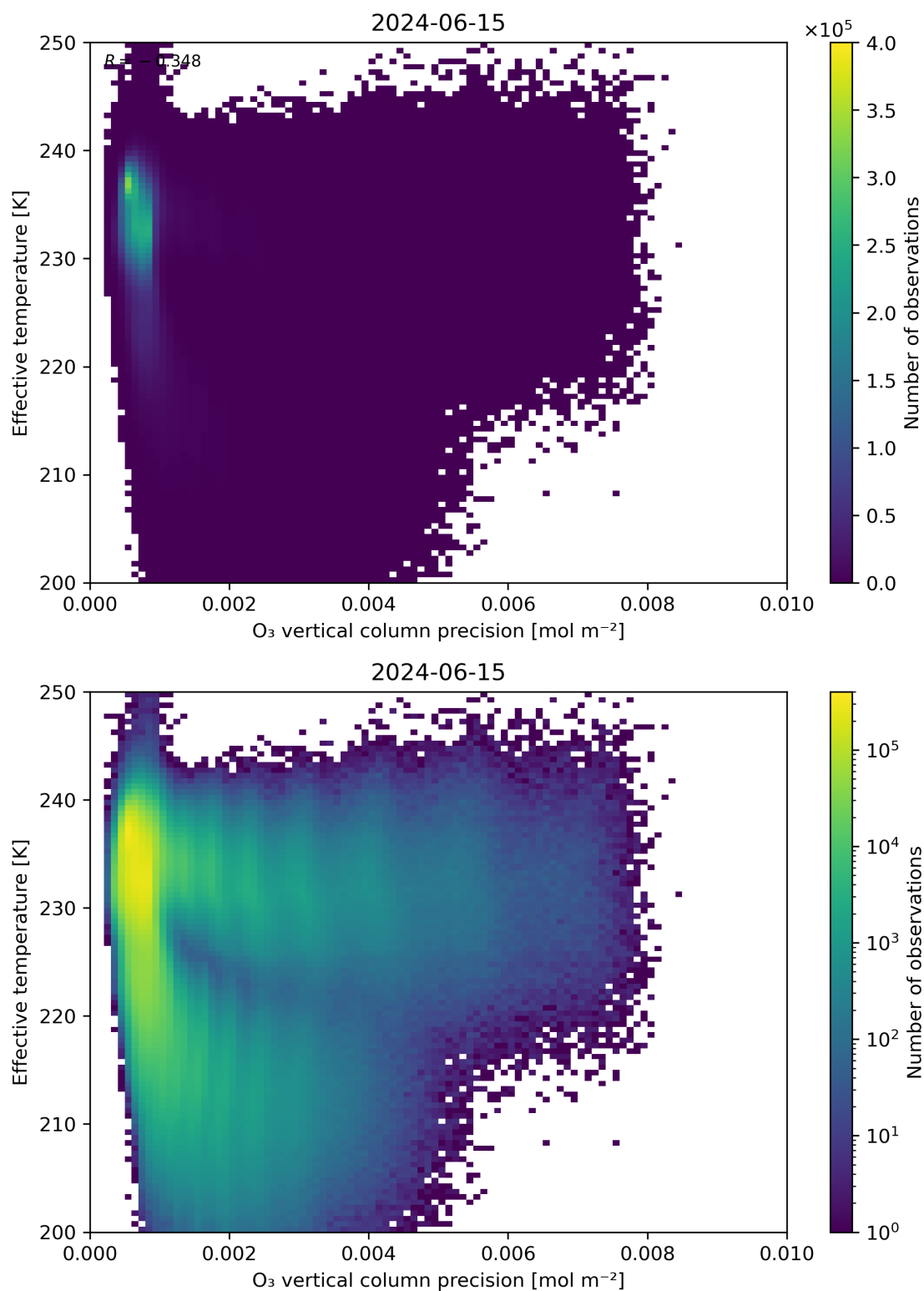
Figure 42: Scatter density plot of “O 3 vertical column precision” against “Effective temperature” for 2024-06-14 to 2024-06-16.
