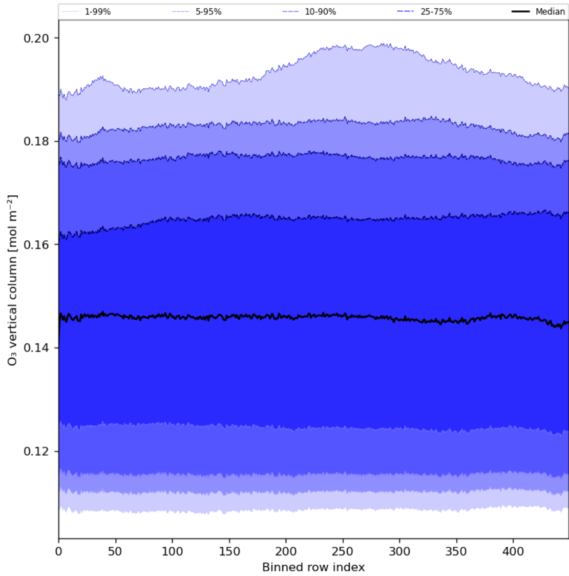
Figure 28: Along track statistics of “ \text{O}_3 vertical column” for 2024-06-14 to 2024-06-16
