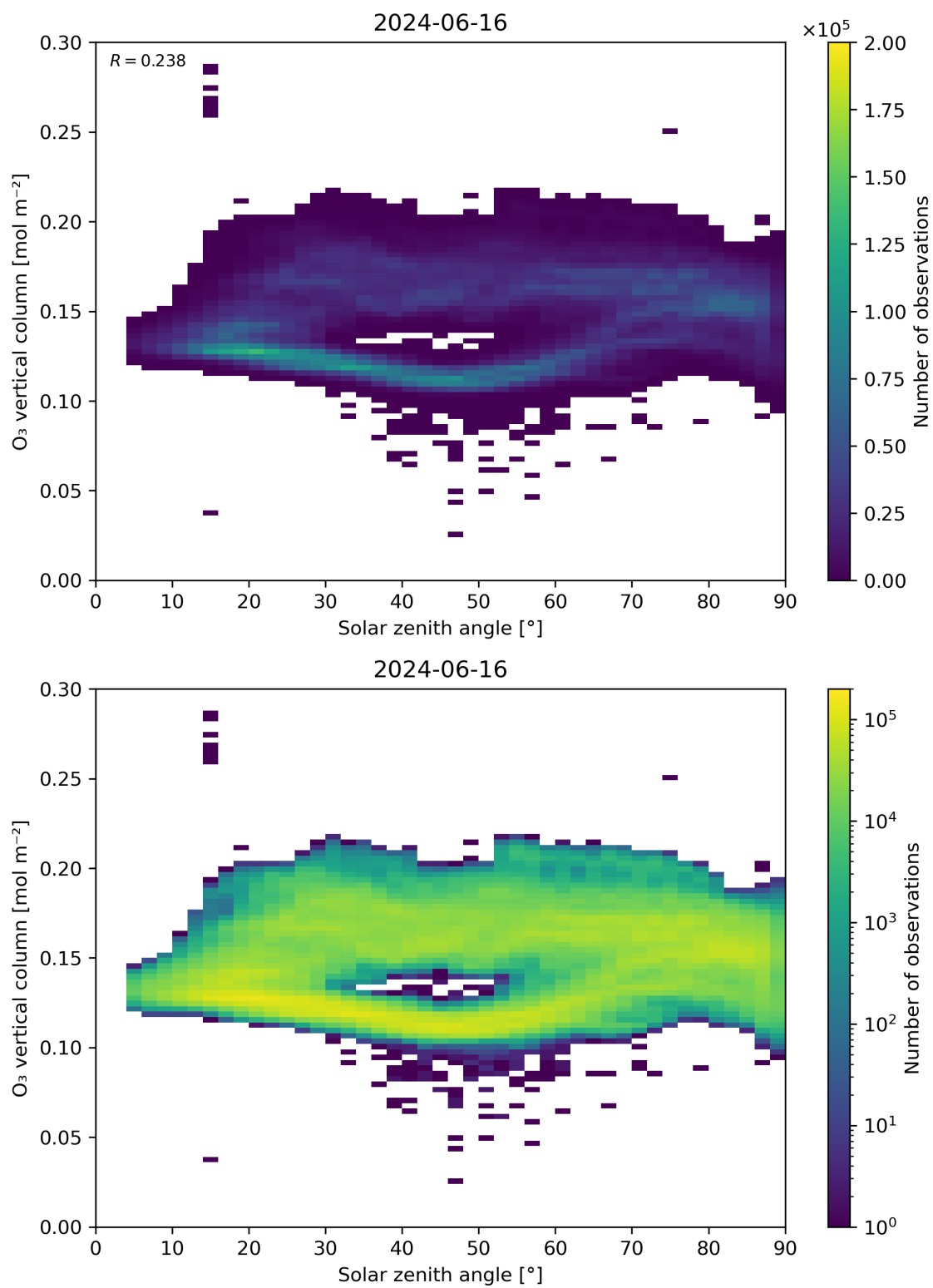
Figure 47: Scatter density plot of “Solar zenith angle” against “O 3 vertical column” for 2024-06-15 to 2024-06-17.
