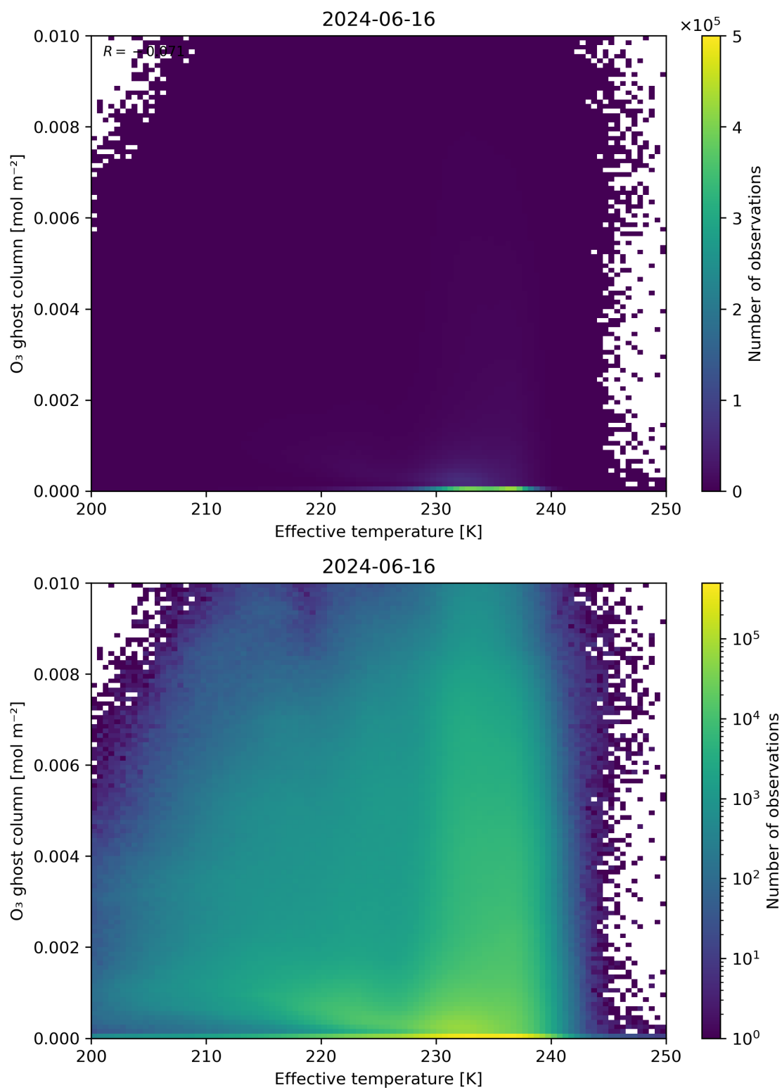
Figure 38: Scatter density plot of “Effective temperature” against “O 3 ghost column” for 2024-06-15 to 2024-06-17.
