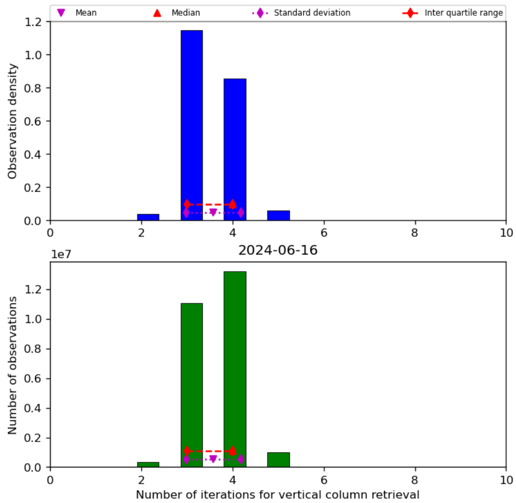
Figure 26: Histogram of “Number of iterations for vertical column retrieval” for 2024-06-15 to 2024-06-17
