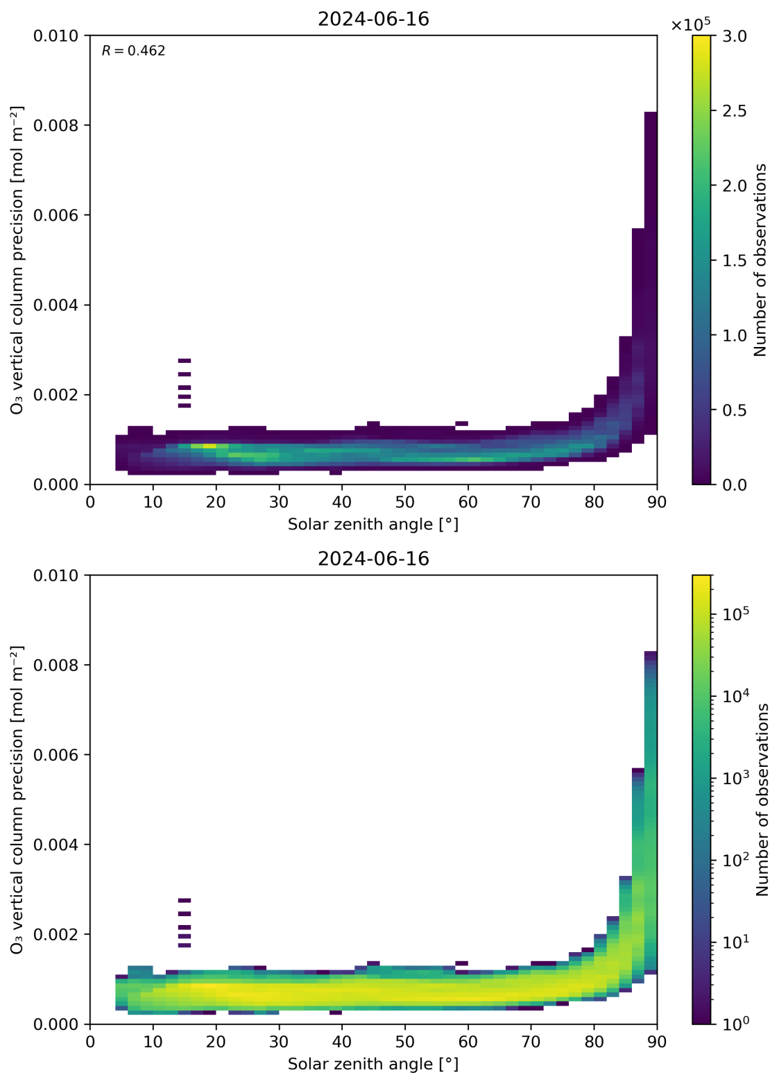
Figure 48: Scatter density plot of “Solar zenith angle” against “O 3 vertical column precision” for 2024-06-15 to 2024-06-17.
