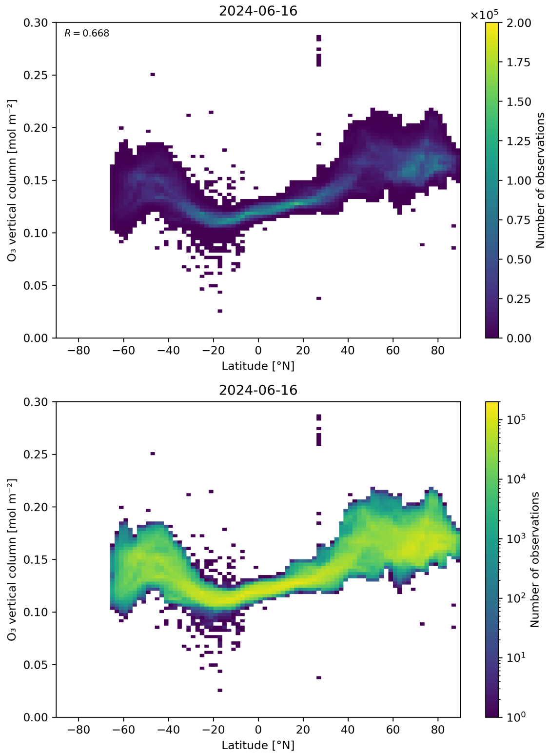
Figure 36: Scatter density plot of “Latitude” against “O 3 vertical column” for 2024-06-15 to 2024-06-17.
