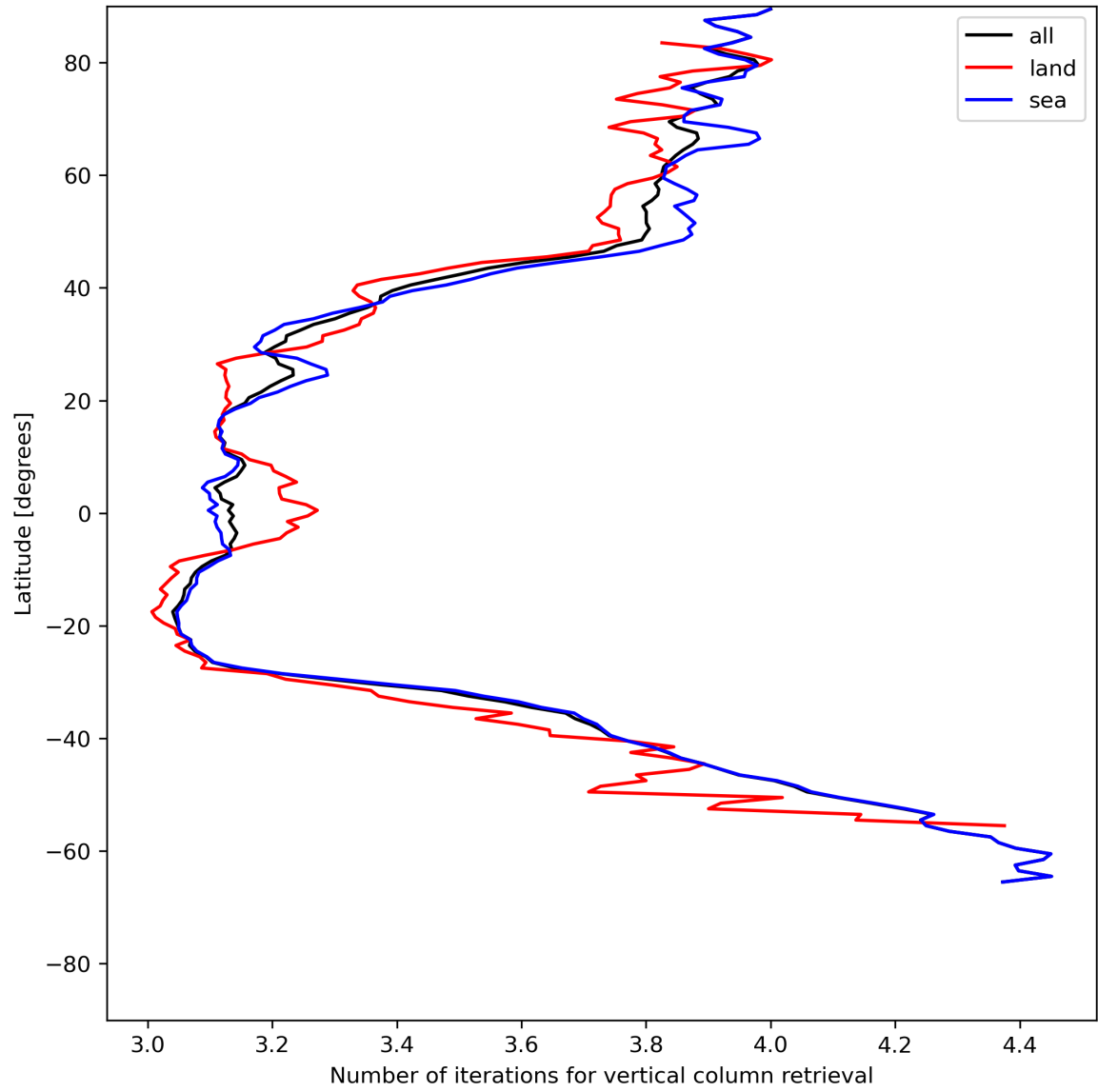
Figure 19: Zonal average of “Number of iterations for vertical column retrieval” for 2024-06-15 to 2024-06-17.
