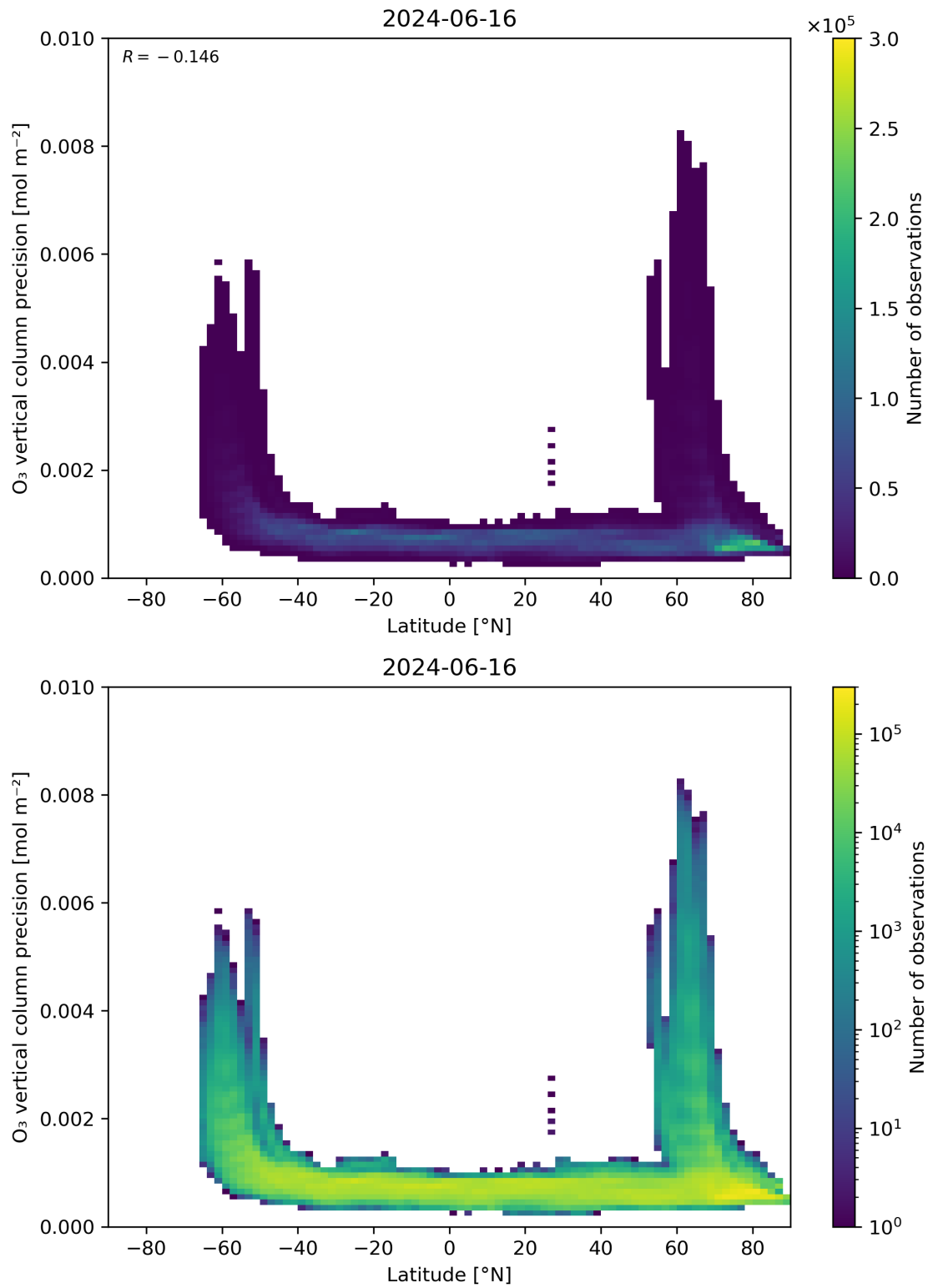
Figure 37: Scatter density plot of “Latitude” against “O 3 vertical column precision” for 2024-06-15 to 2024-06-17.
