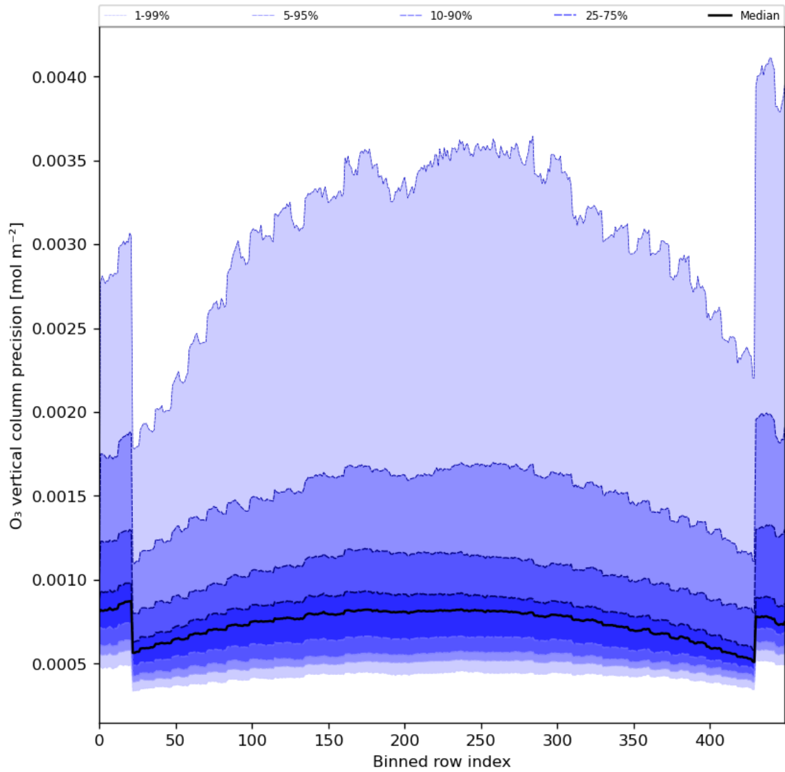
Figure 29: Along track statistics of “O 3 vertical column precision” for 2024-06-15 to 2024-06-17
