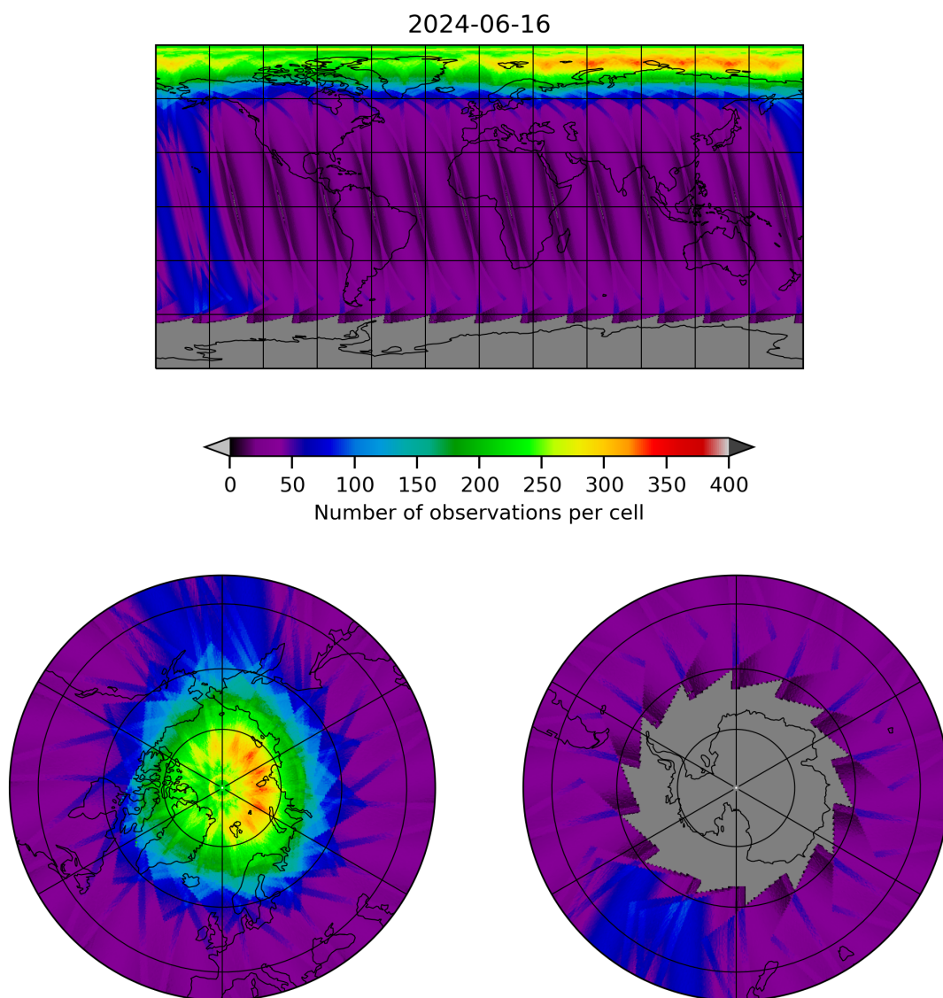
Figure 12: Map of the number of observations for 2024-06-15 to 2024-06-17
