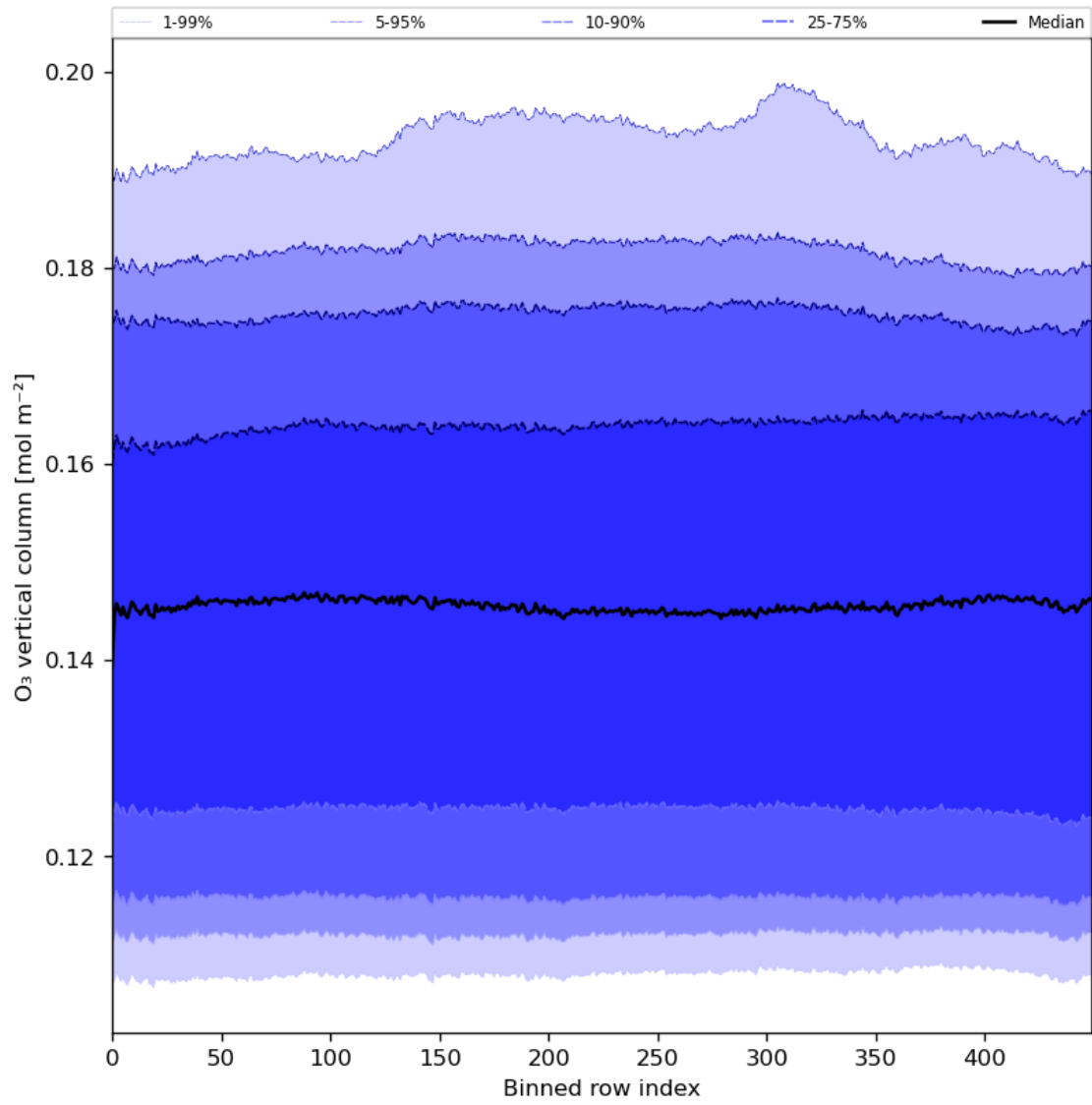
Figure 28: Along track statistics of “O 3 vertical column” for 2024-06-15 to 2024-06-17
