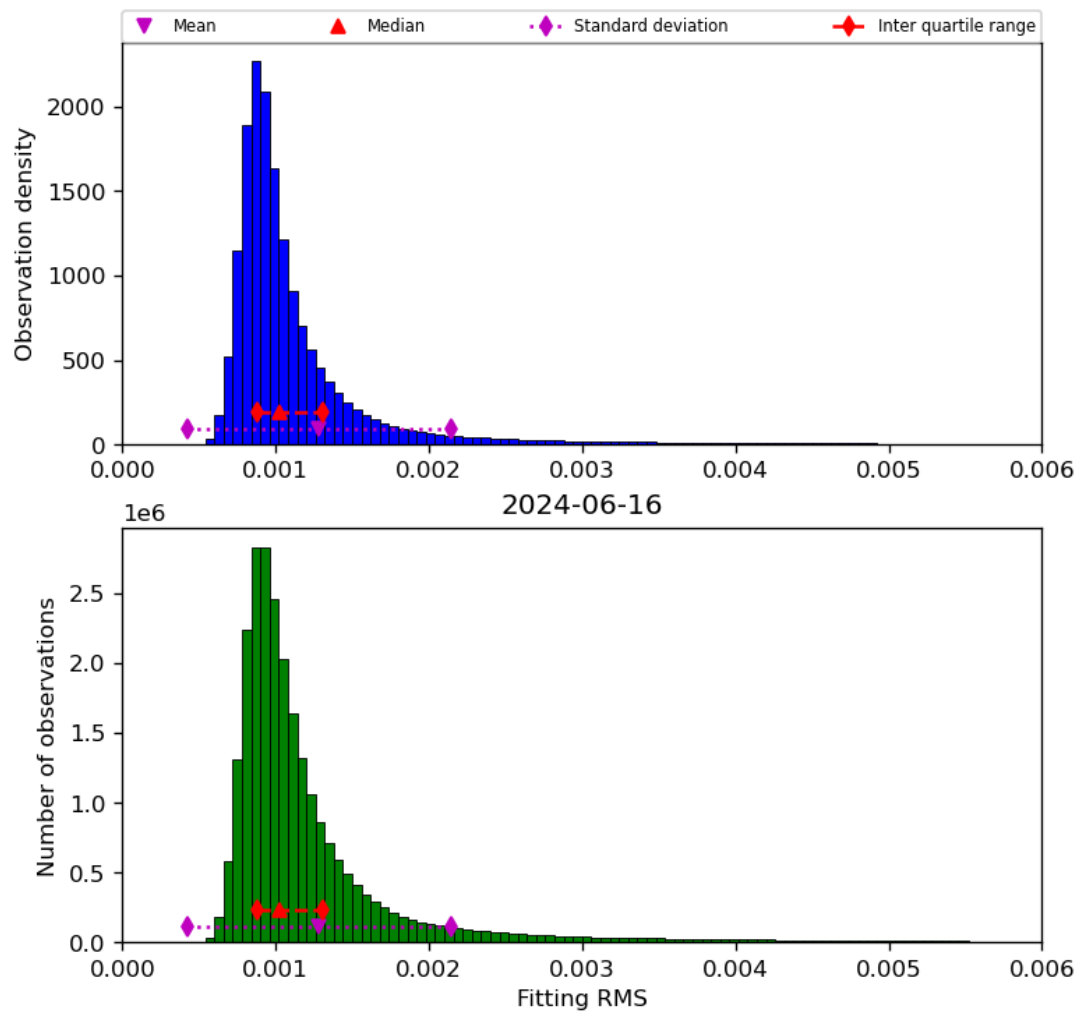
Figure 23: Histogram of “Fitting RMS” for 2024-06-15 to 2024-06-17
