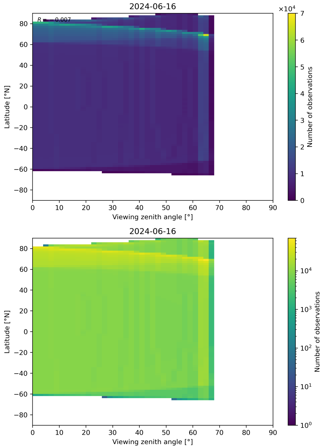
Figure 49: Scatter density plot of “Viewing zenith angle” against “Latitude” for 2024-06-15 to 2024-06-17.
