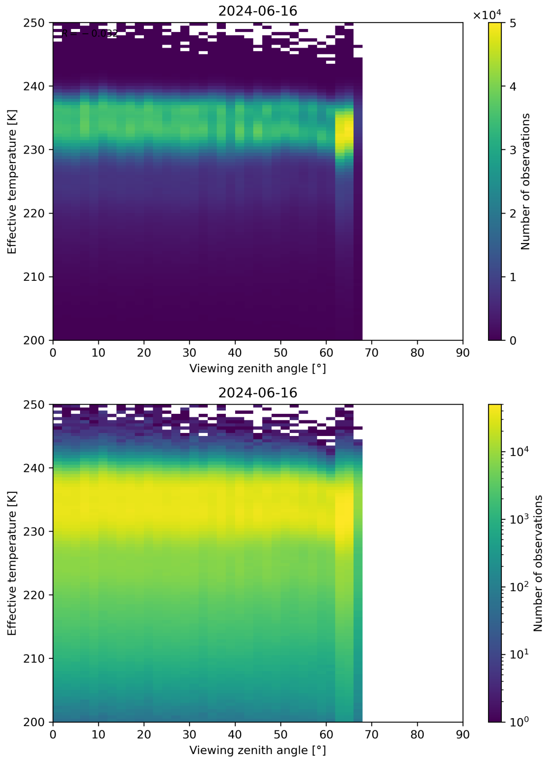
Figure 50: Scatter density plot of “Viewing zenith angle” against “Effective temperature” for 2024-06-15 to 2024-06-17.
