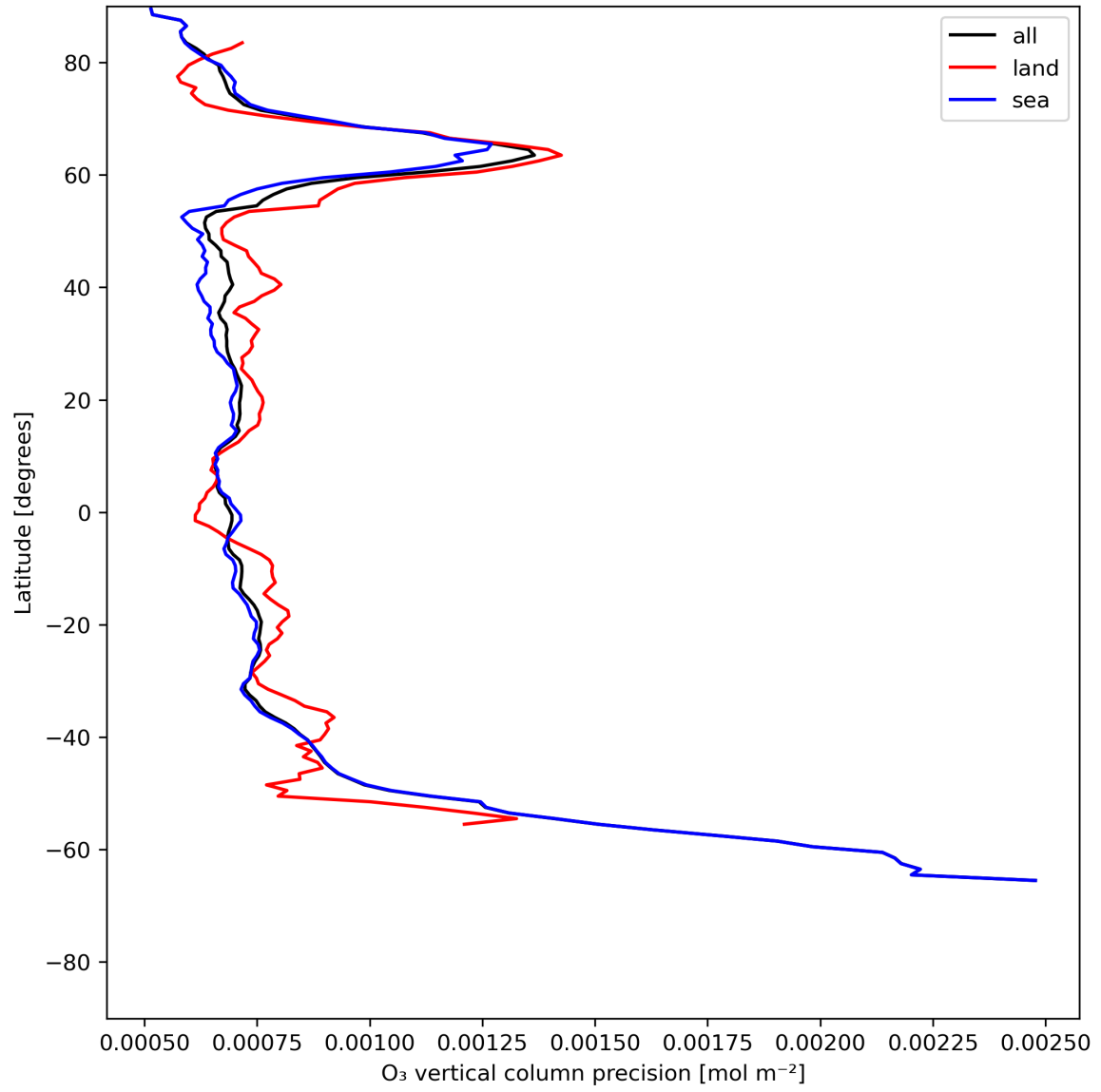
Figure 15: Zonal average of "O 3 vertical column precision" for 2024-06-15 to 2024-06-17.
