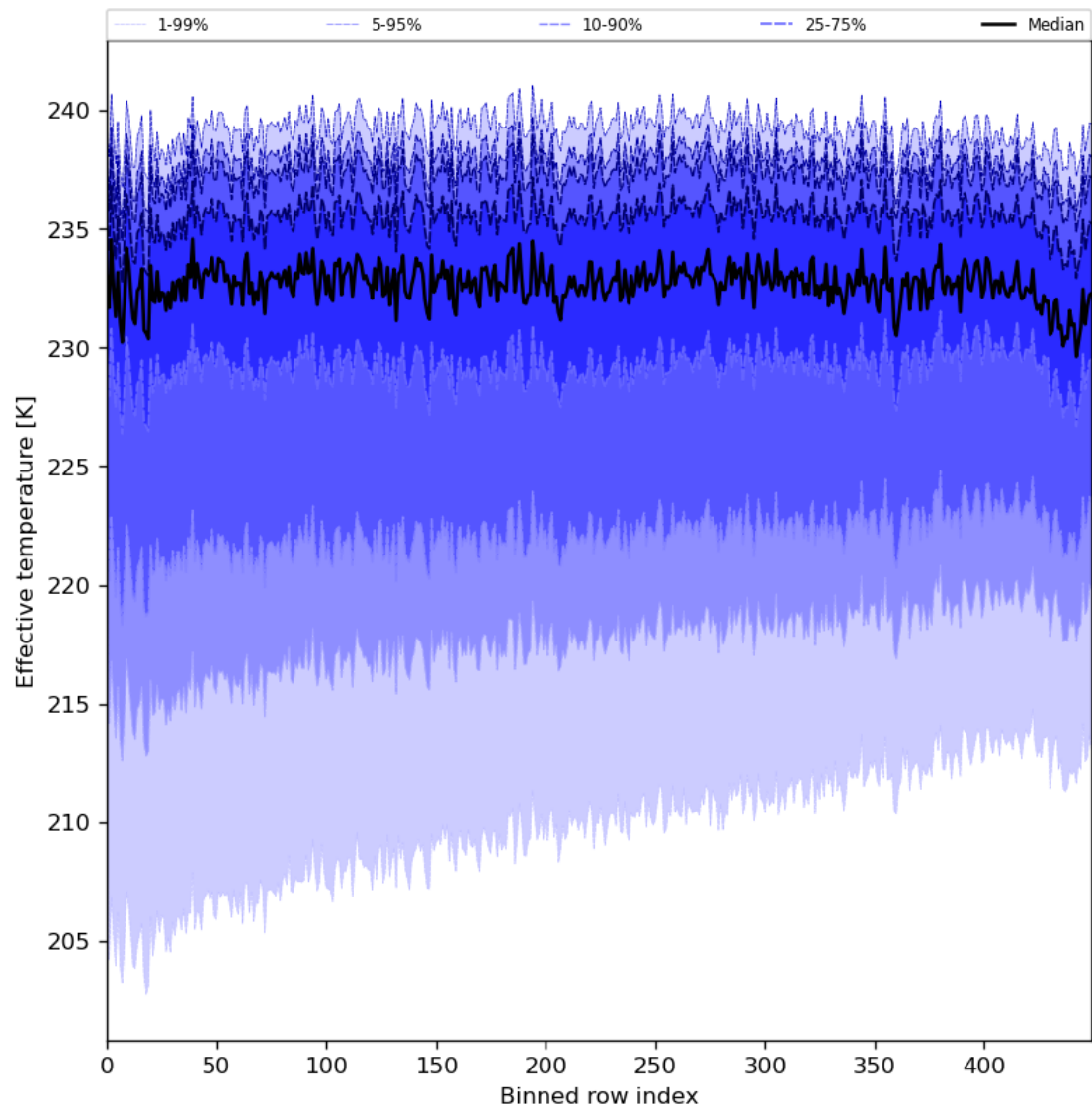
Figure 31: Along track statistics of “Effective temperature” for 2024-06-15 to 2024-06-17
