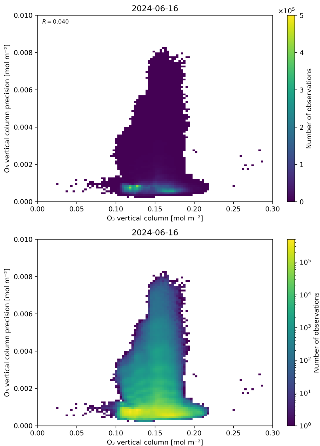
Figure 41: Scatter density plot of “O 3 vertical column” against “O 3 vertical column precision” for 2024-06-15 to 2024-06-17.
