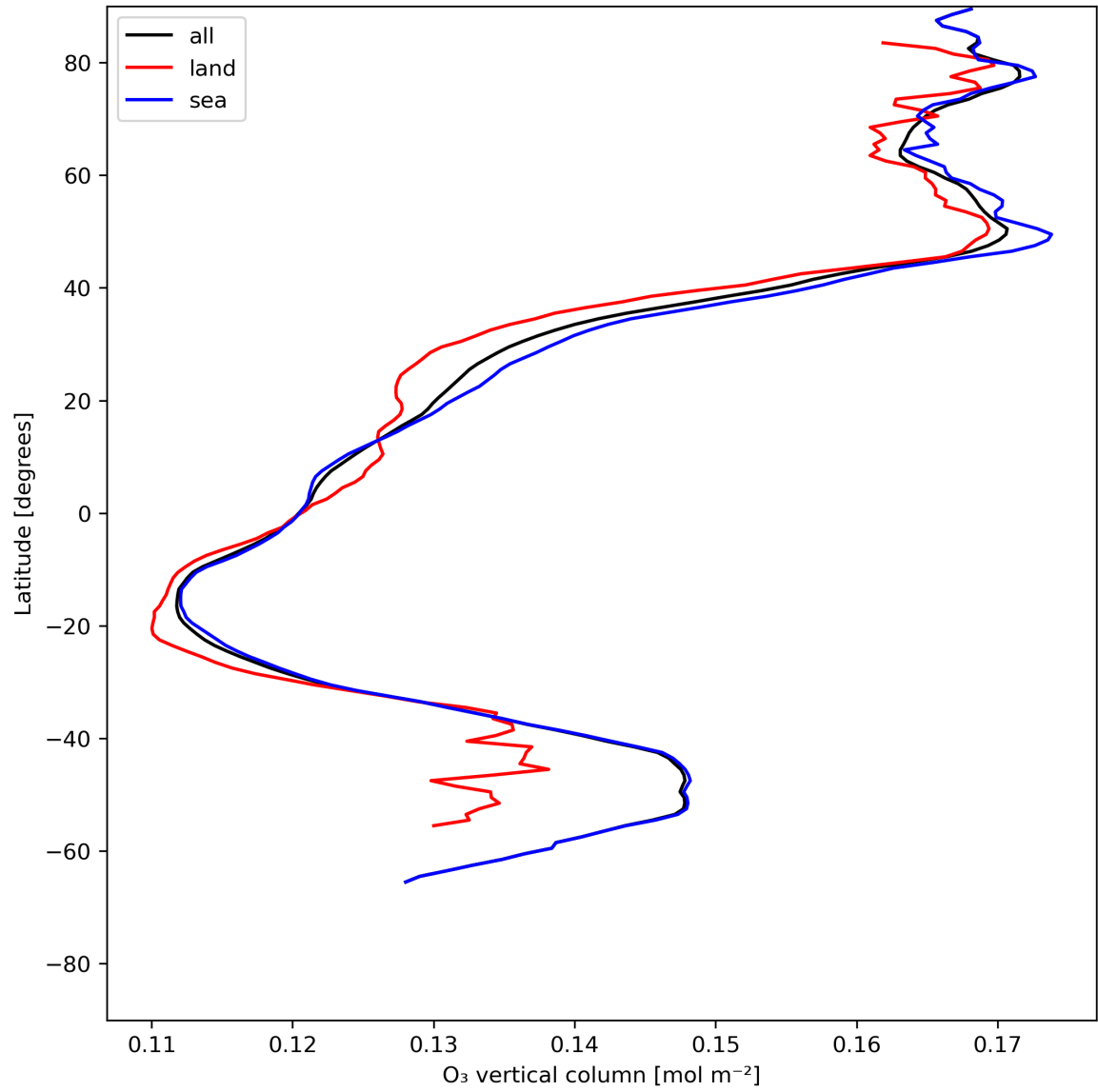
Figure 14: Zonal average of “O 3 vertical column” for 2024-06-15 to 2024-06-17.
