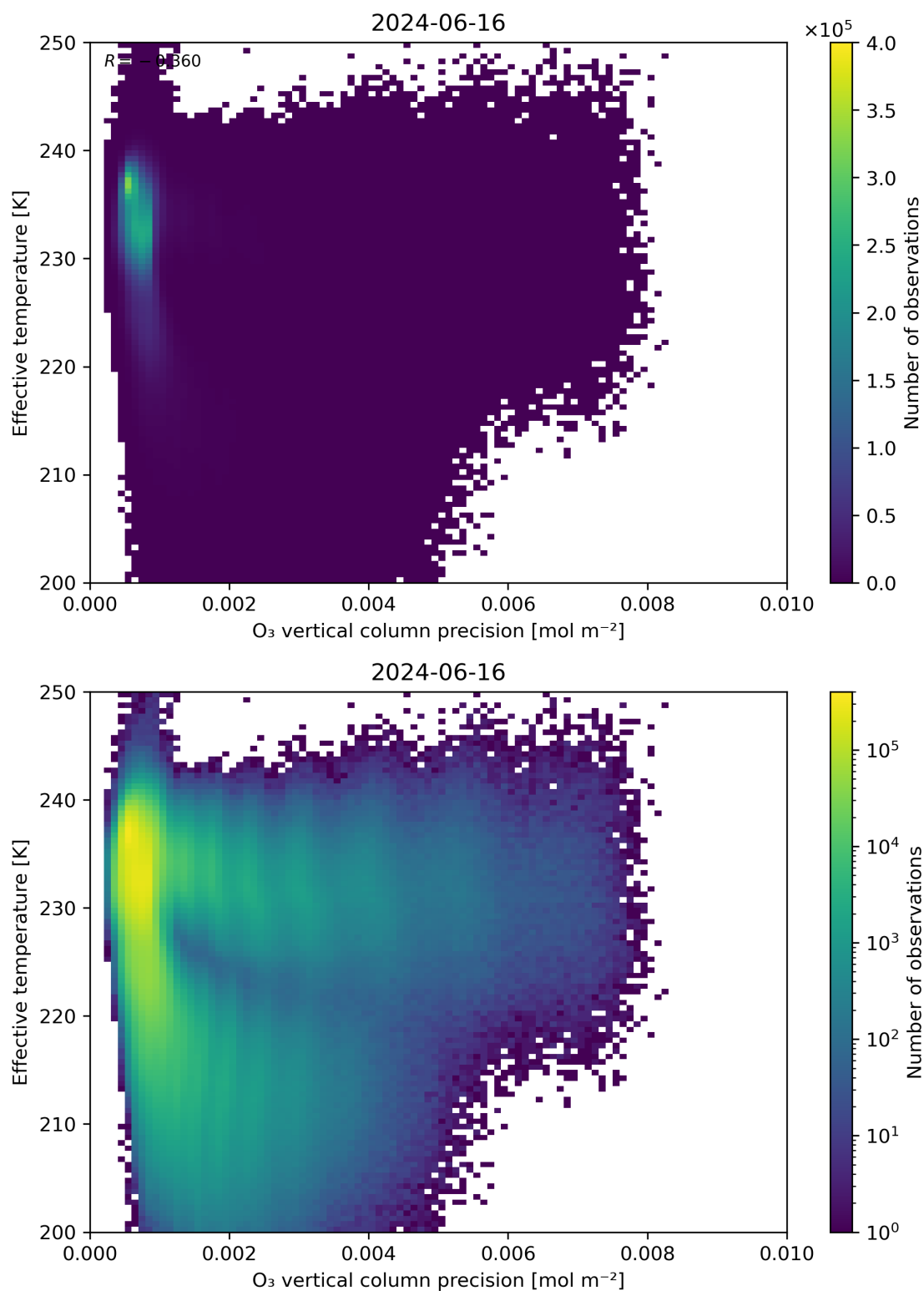
Figure 42: Scatter density plot of “O 3 vertical column precision” against “Effective temperature” for 2024-06-15 to 2024-06-17.
