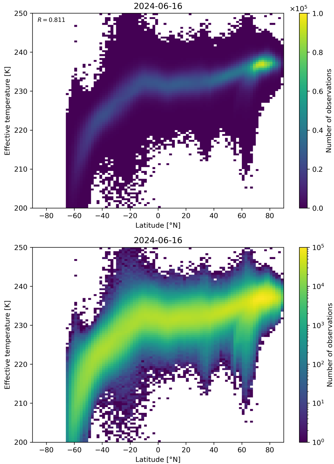
Figure 34: Scatter density plot of “Latitude” against “Effective temperature” for 2024-06-15 to 2024-06-17.
