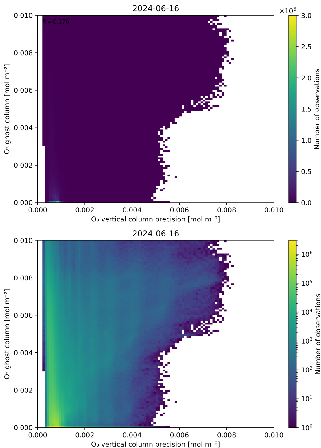
Figure 43: Scatter density plot of “ \text{O}_3 vertical column precision” against “ \text{O}_3 ghost column” for 2024-06-15 to 2024-06-17.
