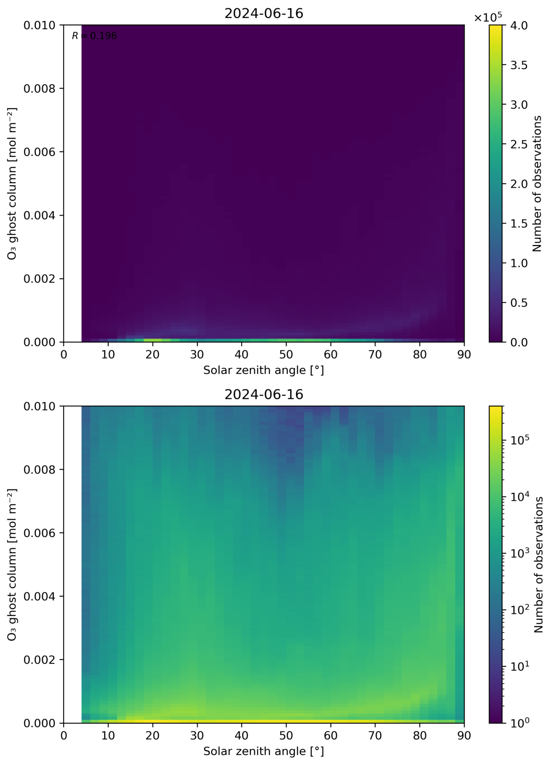
Figure 46: Scatter density plot of “Solar zenith angle” against “O 3 ghost column” for 2024-06-15 to 2024-06-17.
