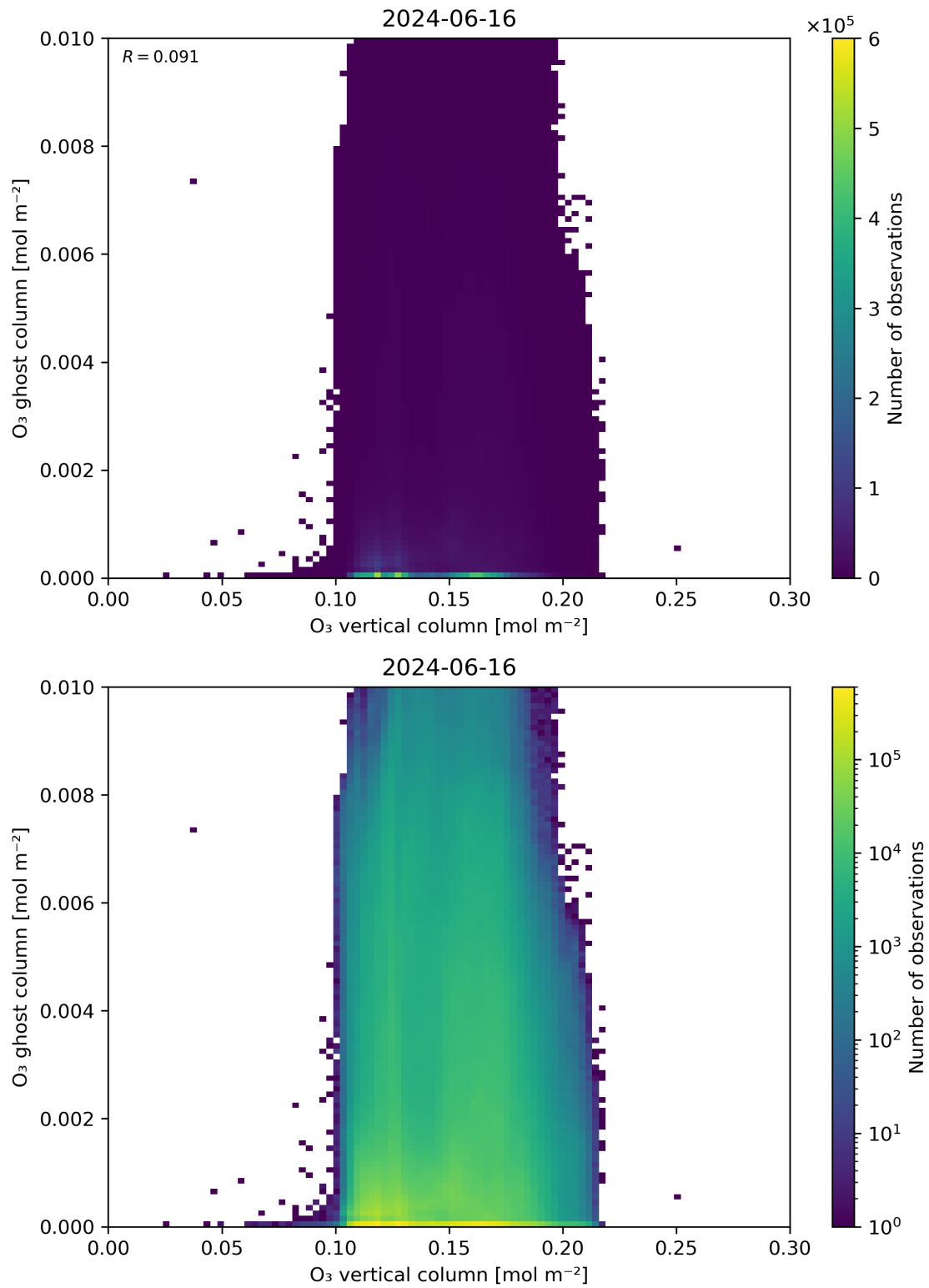
Figure 40: Scatter density plot of “O 3 vertical column” against “O 3 ghost column” for 2024-06-15 to 2024-06-17.
