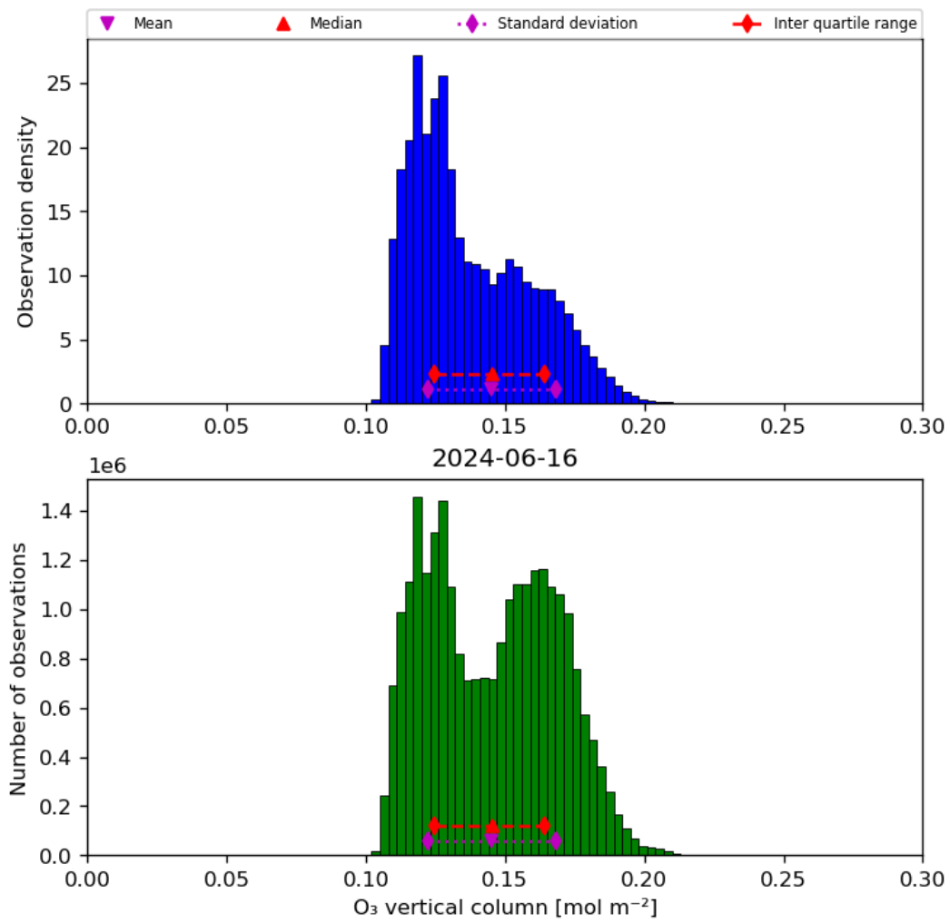
Figure 21: Histogram of “O 3 vertical column” for 2024-06-15 to 2024-06-17
