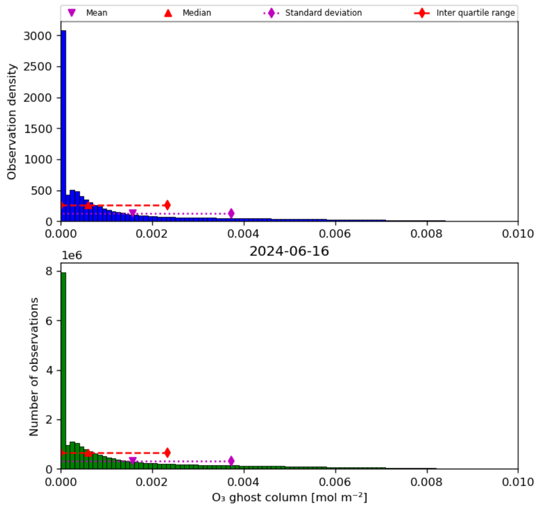
Figure 25: Histogram of “O 3 ghost column” for 2024-06-15 to 2024-06-17
