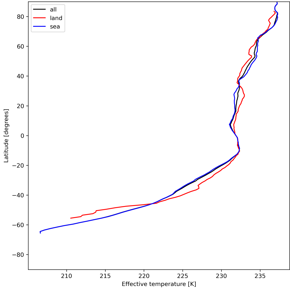
Figure 17: Zonal average of “Effective temperature” for 2024-06-15 to 2024-06-17.
