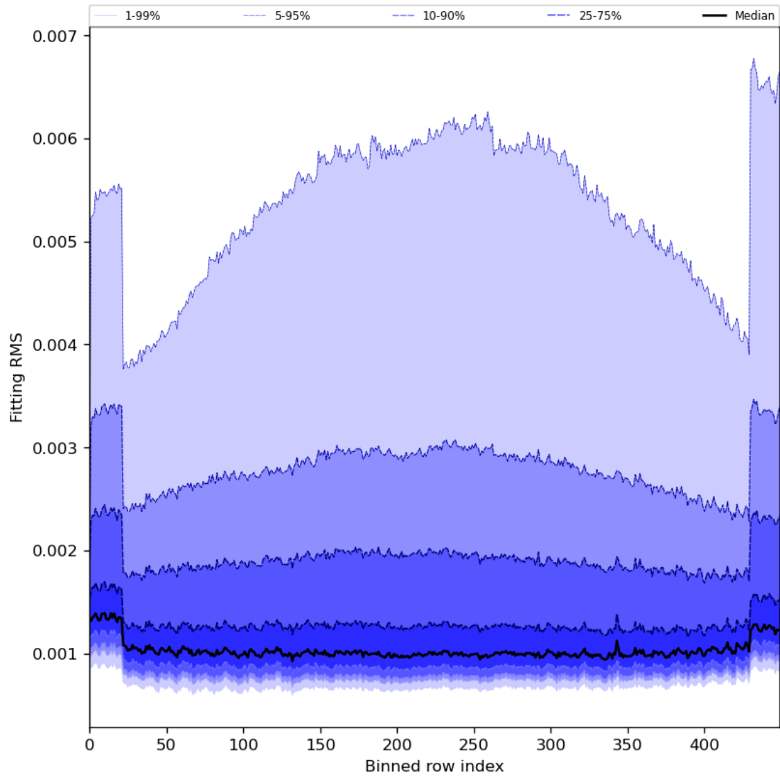
Figure 30: Along track statistics of “Fitting RMS” for 2024-06-15 to 2024-06-17
