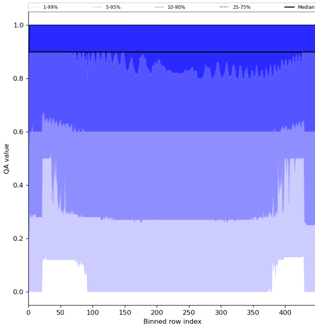
Figure 27: Along track statistics of “QA value” for 2024-06-15 to 2024-06-17
