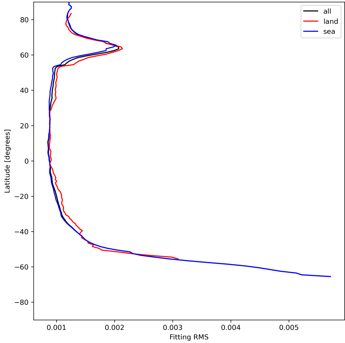
Figure 16: Zonal average of “Fitting RMS” for 2024-06-15 to 2024-06-17.
