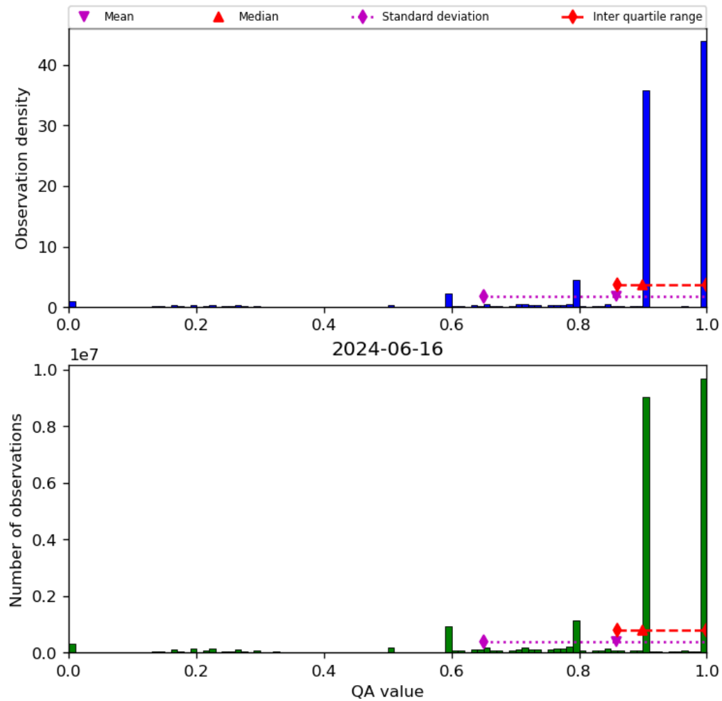
Figure 20: Histogram of “QA value” for 2024-06-15 to 2024-06-17
