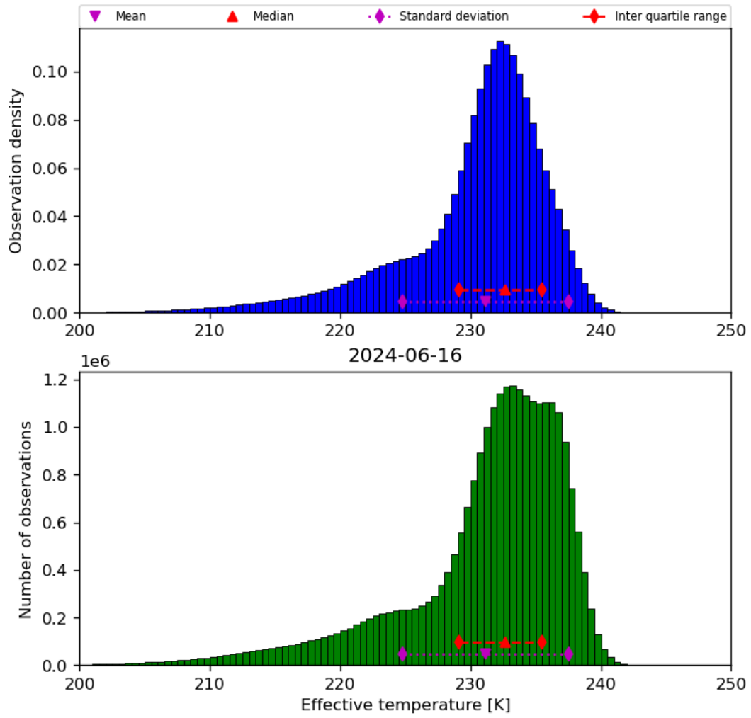
Figure 24: Histogram of “Effective temperature” for 2024-06-15 to 2024-06-17
