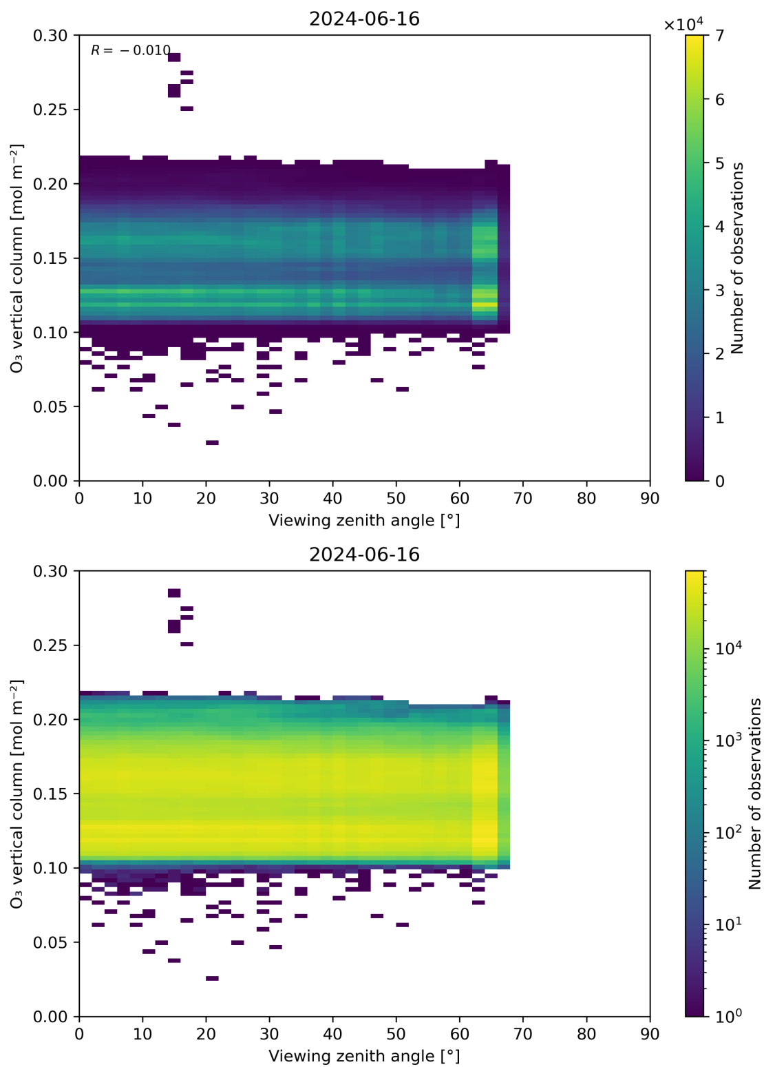
Figure 52: Scatter density plot of “Viewing zenith angle” against “O 3 vertical column” for 2024-06-15 to 2024-06-17.
