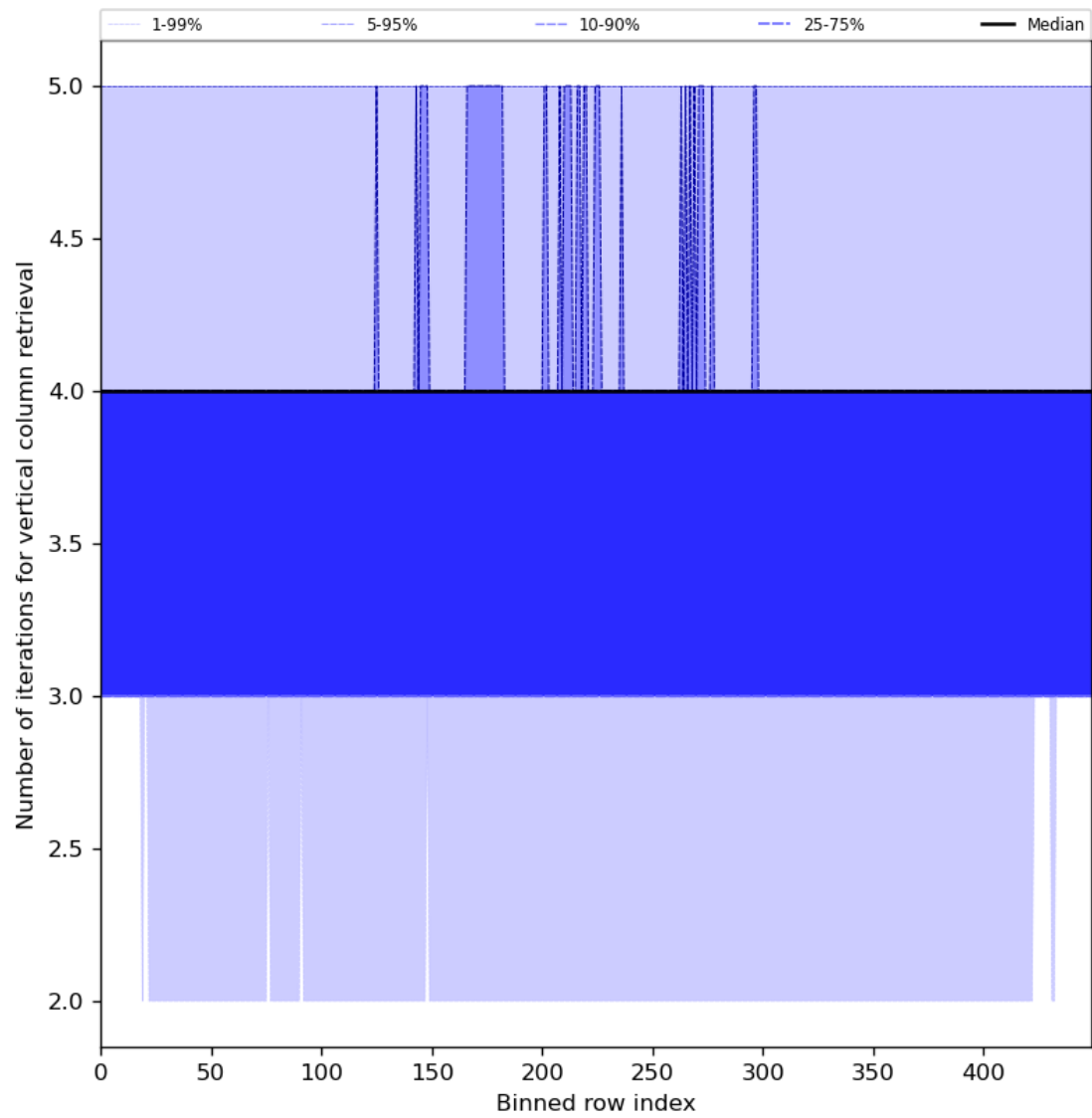
Figure 33: Along track statistics of “Number of iterations for vertical column retrieval” for 2024-06-15 to 2024-06-17
