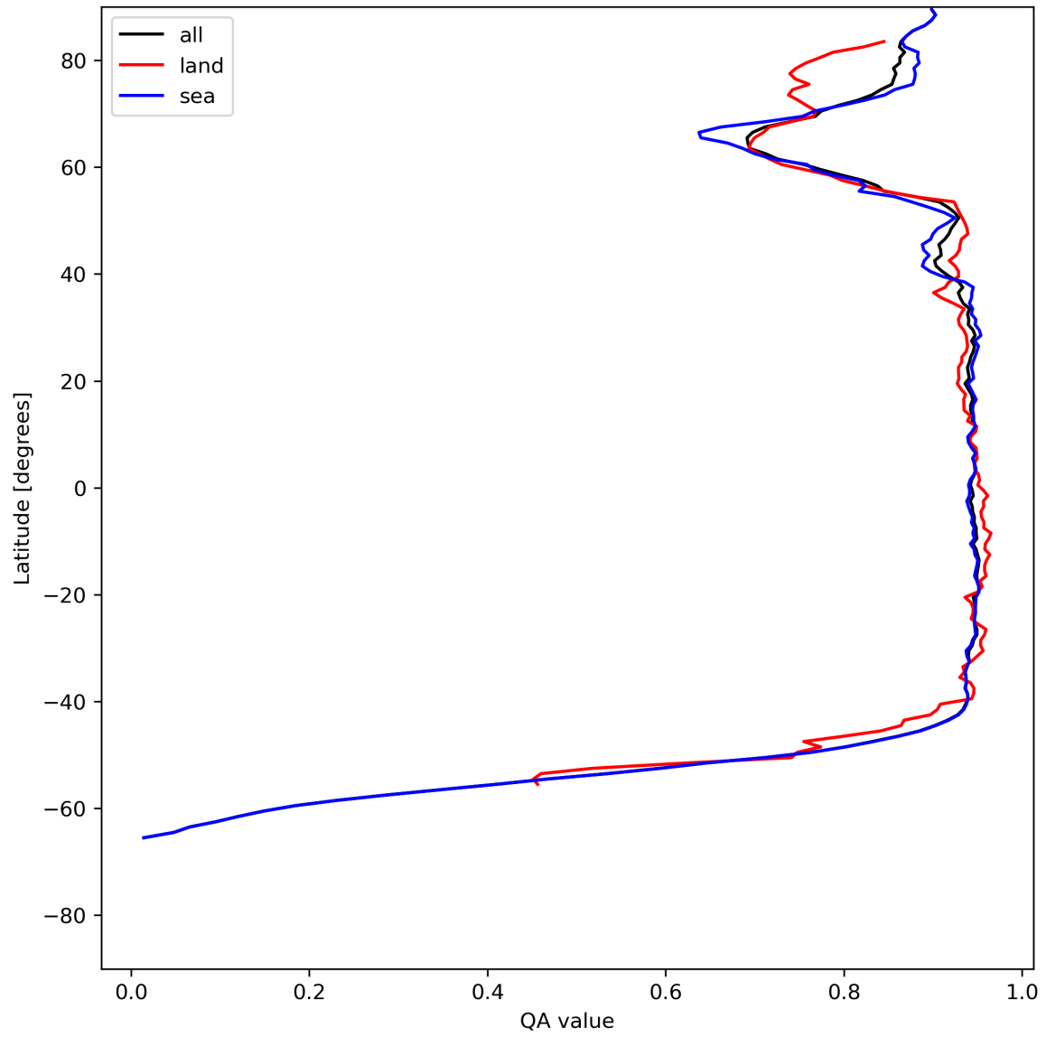
Figure 13: Zonal average of “QA value” for 2024-06-15 to 2024-06-17.
