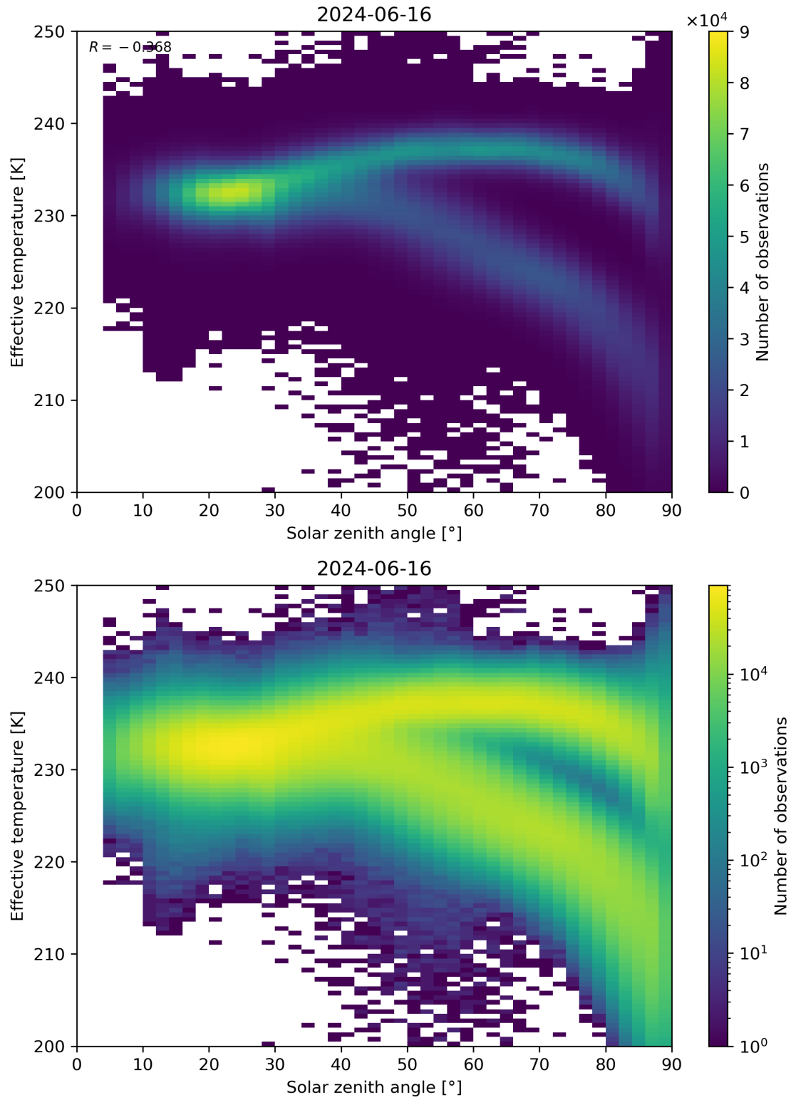
Figure 45: Scatter density plot of “Solar zenith angle” against “Effective temperature” for 2024-06-15 to 2024-06-17.
