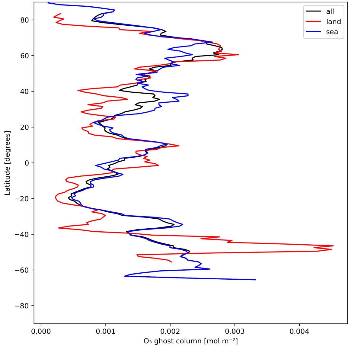
Figure 18: Zonal average of "O 3 ghost column" for 2024-06-15 to 2024-06-17.
