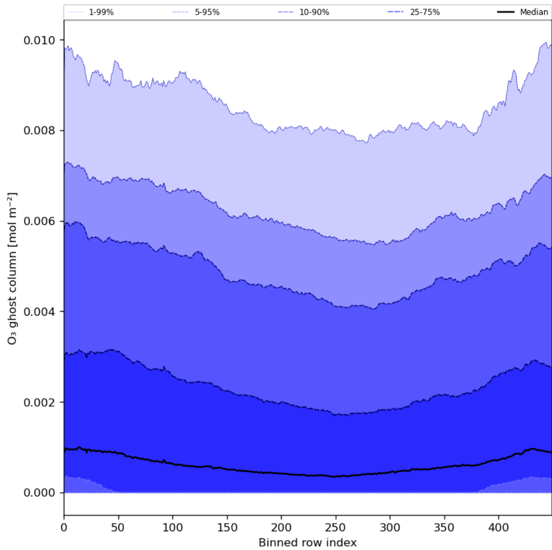
Figure 32: Along track statistics of “O 3 ghost column” for 2024-06-15 to 2024-06-17
