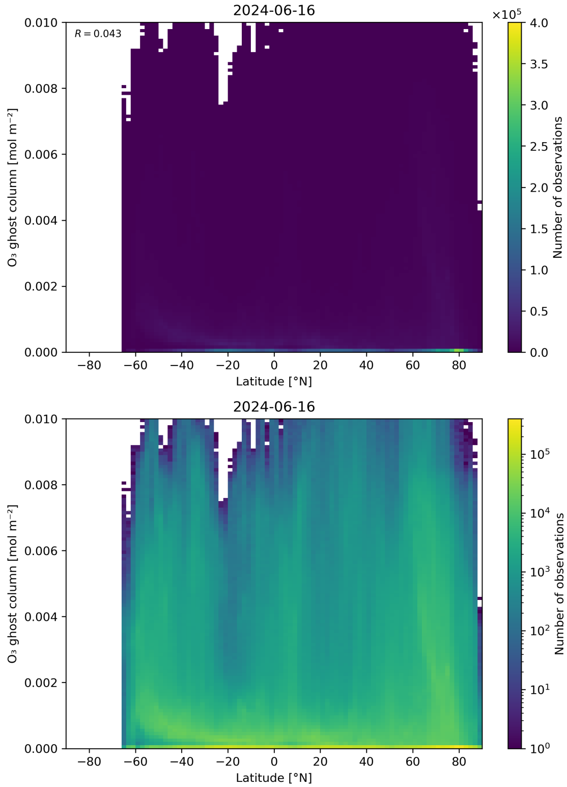
Figure 35: Scatter density plot of “Latitude” against “O 3 ghost column” for 2024-06-15 to 2024-06-17.
