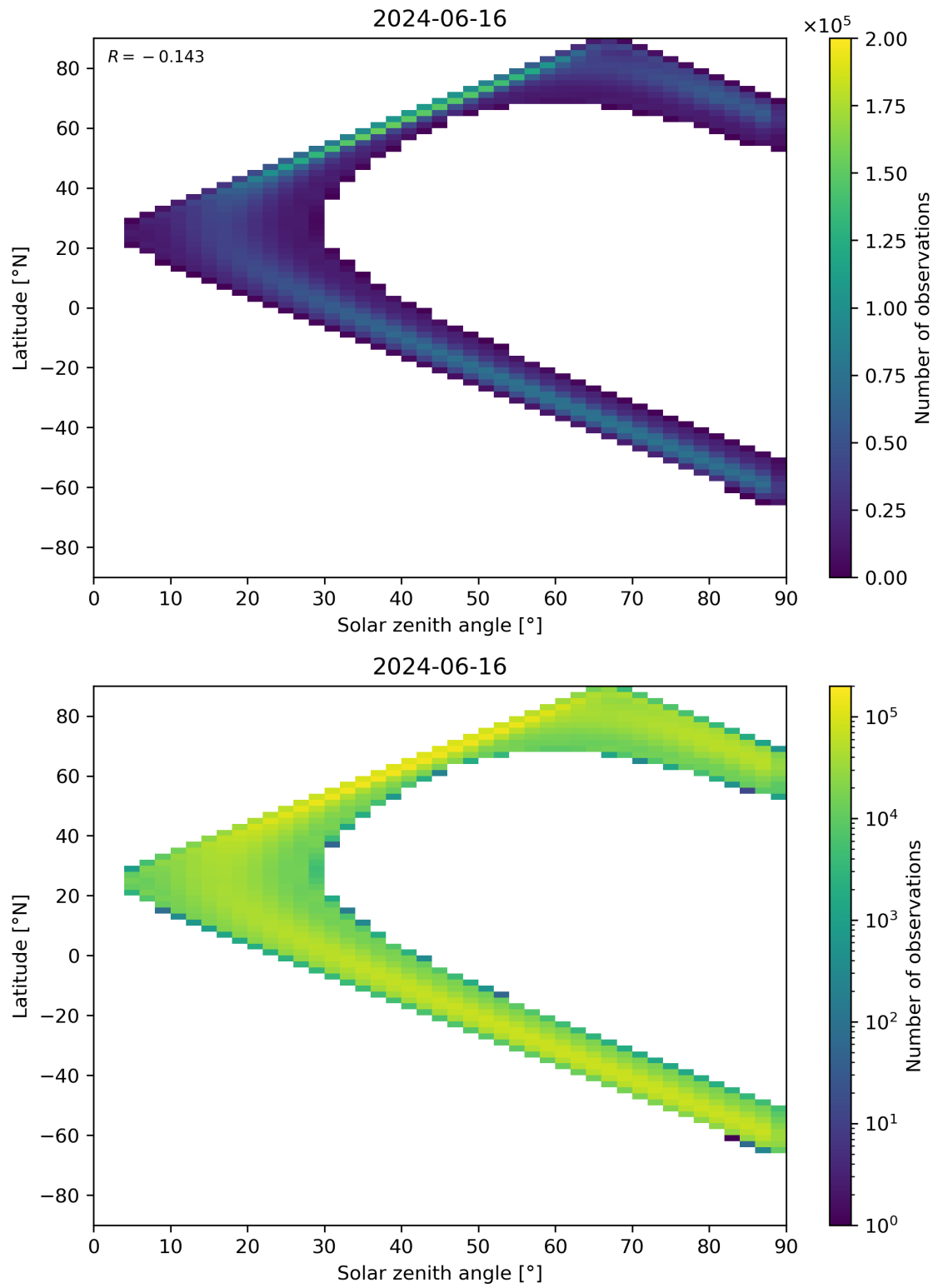
Figure 44: Scatter density plot of “Solar zenith angle” against “Latitude” for 2024-06-15 to 2024-06-17.
