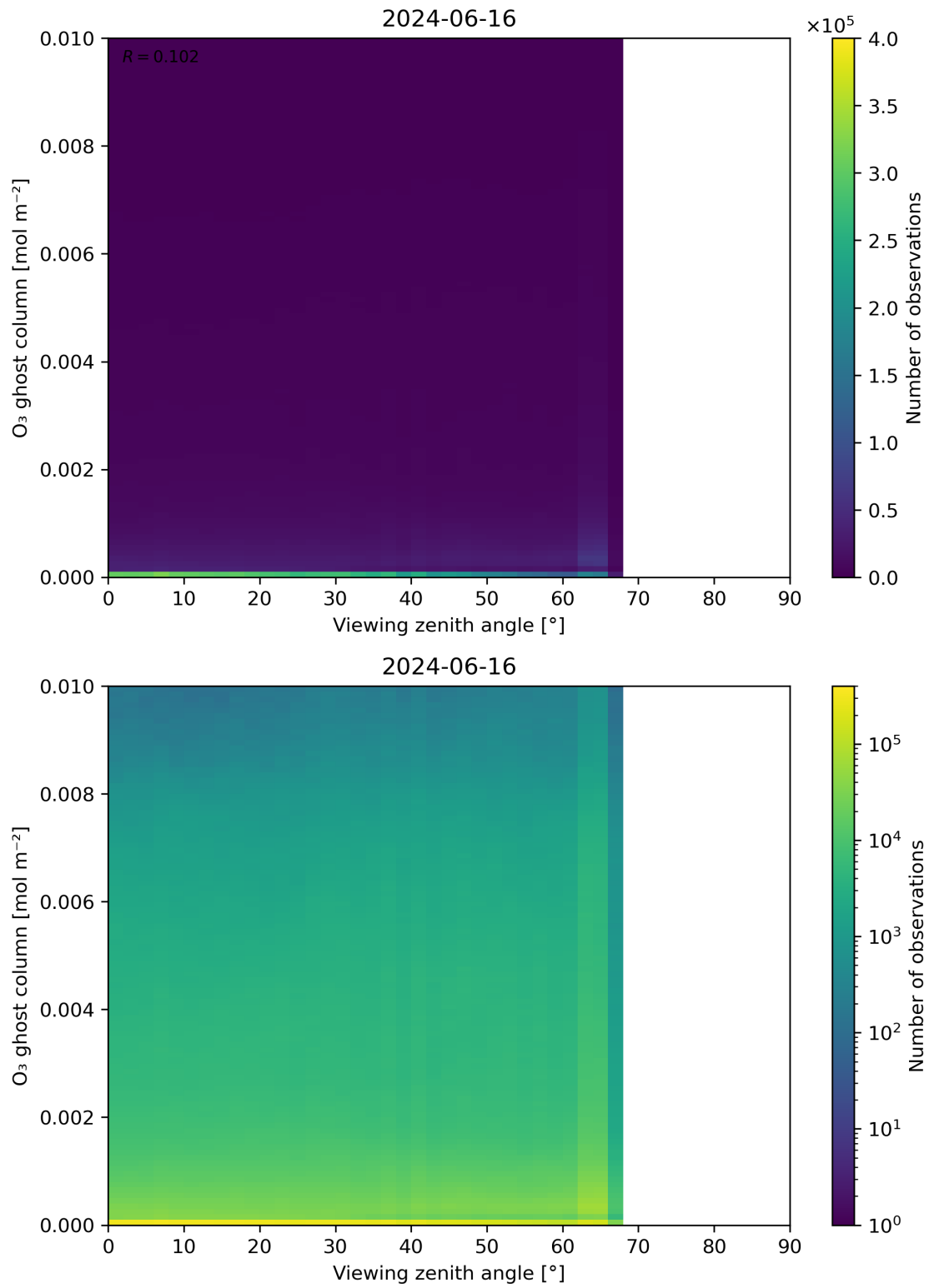
Figure 51: Scatter density plot of “Viewing zenith angle” against “O 3 ghost column” for 2024-06-15 to 2024-06-17.
