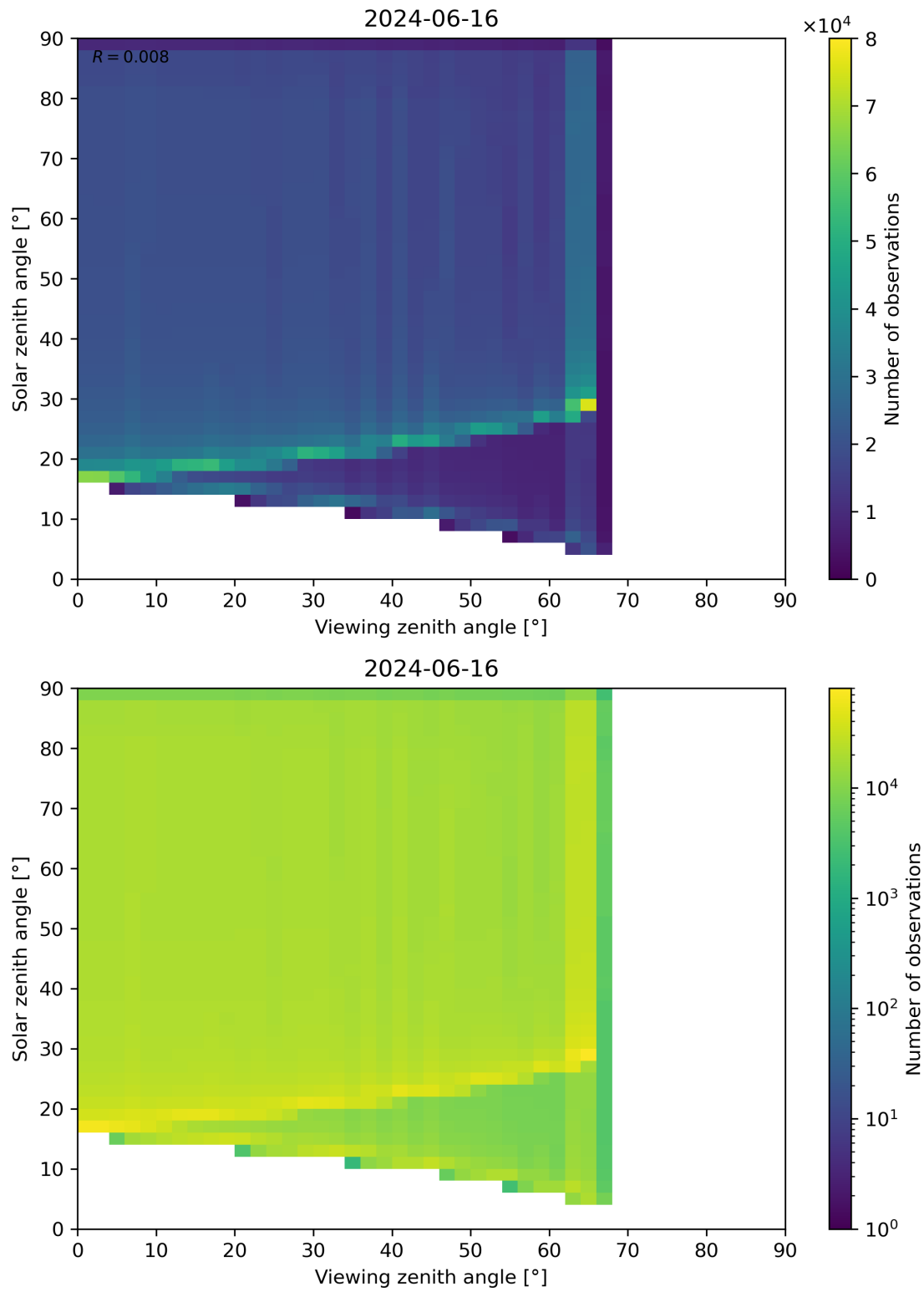
Figure 54: Scatter density plot of “Viewing zenith angle” against “Solar zenith angle” for 2024-06-15 to 2024-06-17.
