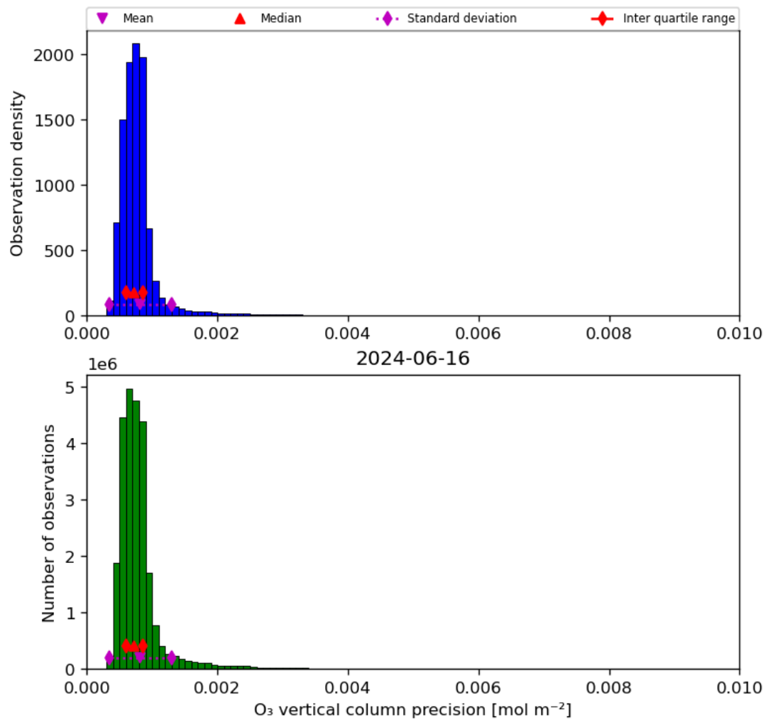
Figure 22: Histogram of “O 3 vertical column precision” for 2024-06-15 to 2024-06-17
