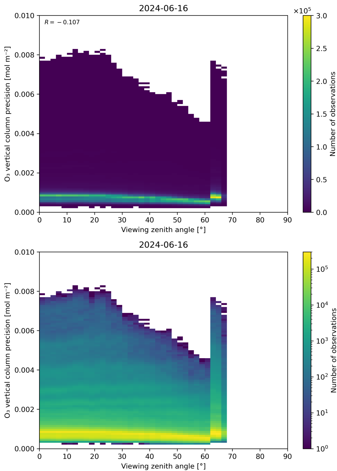
Figure 53: Scatter density plot of “Viewing zenith angle” against “O 3 vertical column precision” for 2024-06-15 to 2024-06-17.
