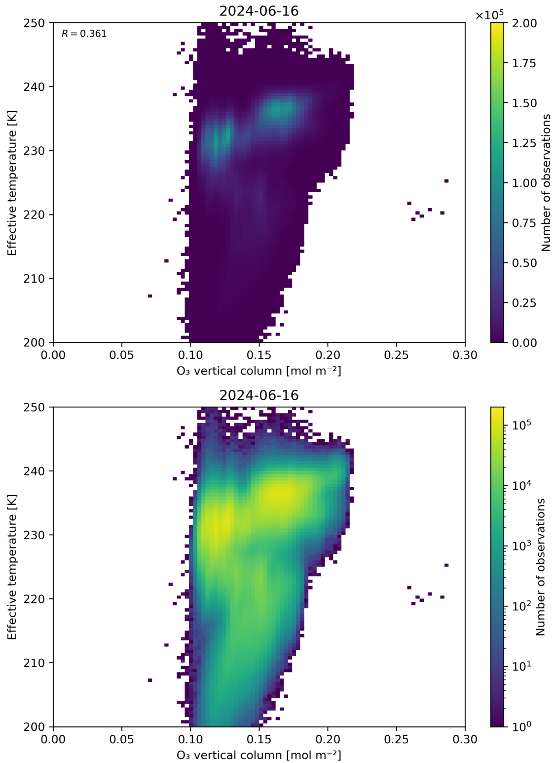
Figure 39: Scatter density plot of “O 3 vertical column” against “Effective temperature” for 2024-06-15 to 2024-06-17.
