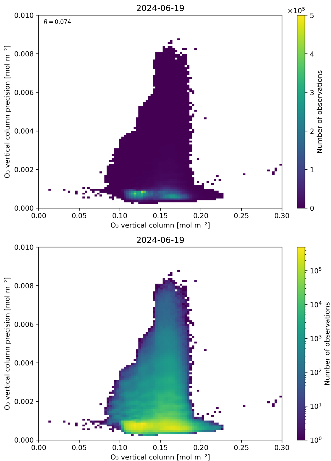
Figure 41: Scatter density plot of “O 3 vertical column” against “O 3 vertical column precision” for 2024-06-19 to 2024-06-20.
