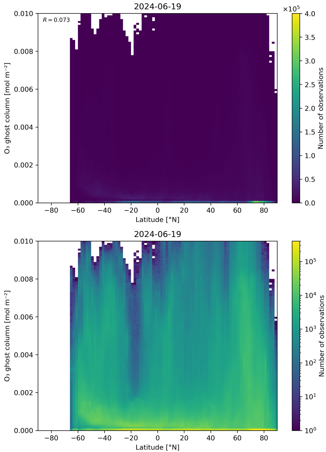
Figure 35: Scatter density plot of “Latitude” against “O 3 ghost column” for 2024-06-19 to 2024-06-20.
