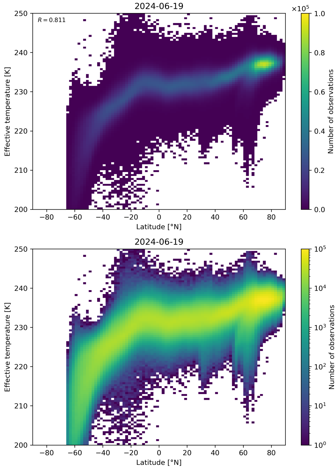
Figure 34: Scatter density plot of “Latitude” against “Effective temperature” for 2024-06-19 to 2024-06-20.
