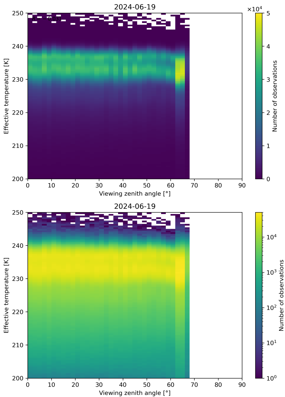
Figure 50: Scatter density plot of “Viewing zenith angle” against “Effective temperature” for 2024-06-19 to 2024-06-20.
