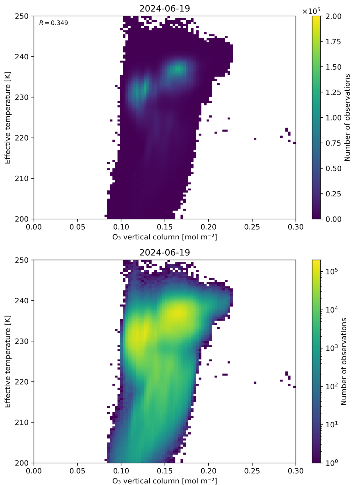
Figure 39: Scatter density plot of “O 3 vertical column” against “Effective temperature” for 2024-06-19 to 2024-06-20.
