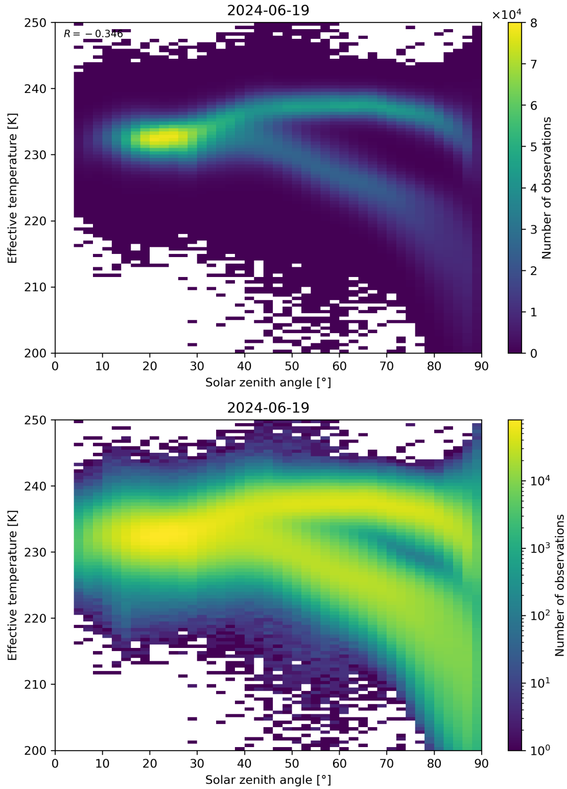
Figure 45: Scatter density plot of “Solar zenith angle” against “Effective temperature” for 2024-06-19 to 2024-06-20.
