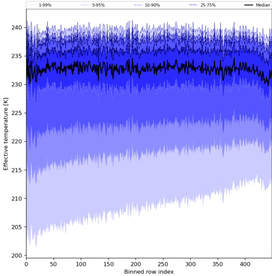
Figure 31: Along track statistics of “Effective temperature” for 2024-06-19 to 2024-06-20
