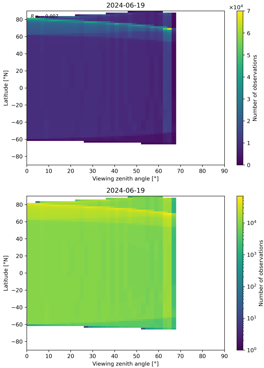
Figure 49: Scatter density plot of “Viewing zenith angle” against “Latitude” for 2024-06-19 to 2024-06-20.
