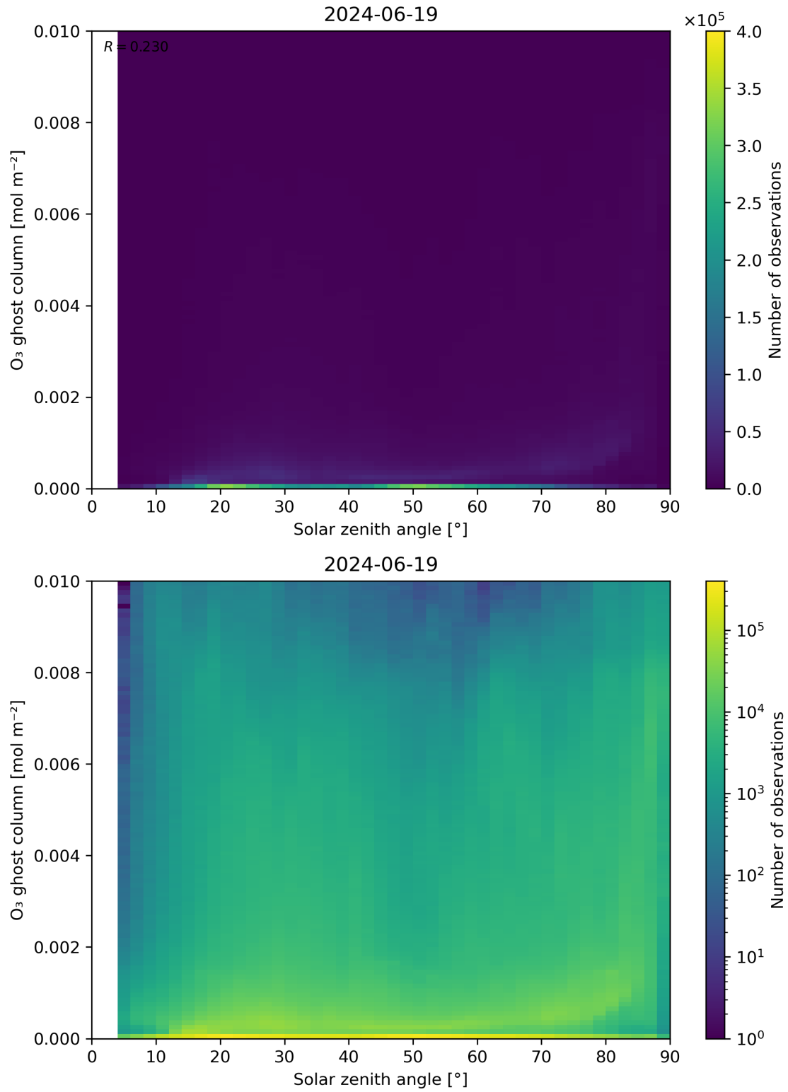
Figure 46: Scatter density plot of “Solar zenith angle” against “O 3 ghost column” for 2024-06-19 to 2024-06-20.
