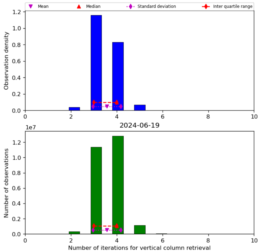
Figure 26: Histogram of “Number of iterations for vertical column retrieval” for 2024-06-19 to 2024-06-20
