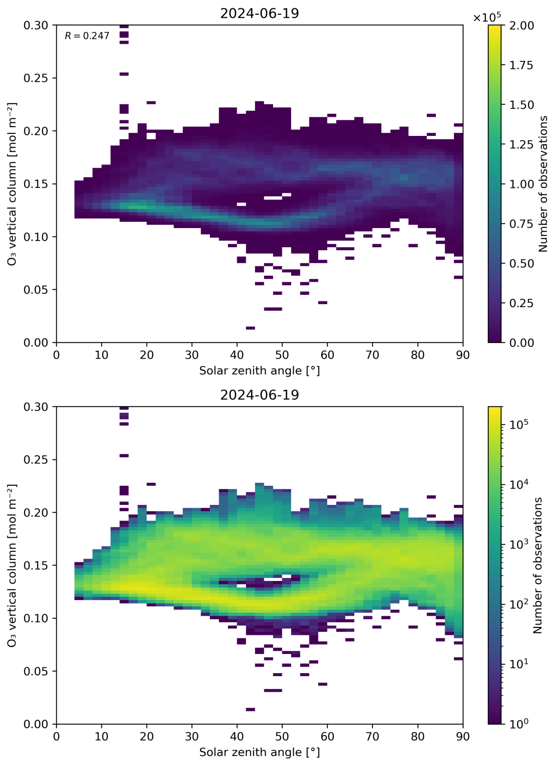
Figure 47: Scatter density plot of “Solar zenith angle” against “O 3 vertical column” for 2024-06-19 to 2024-06-20.
