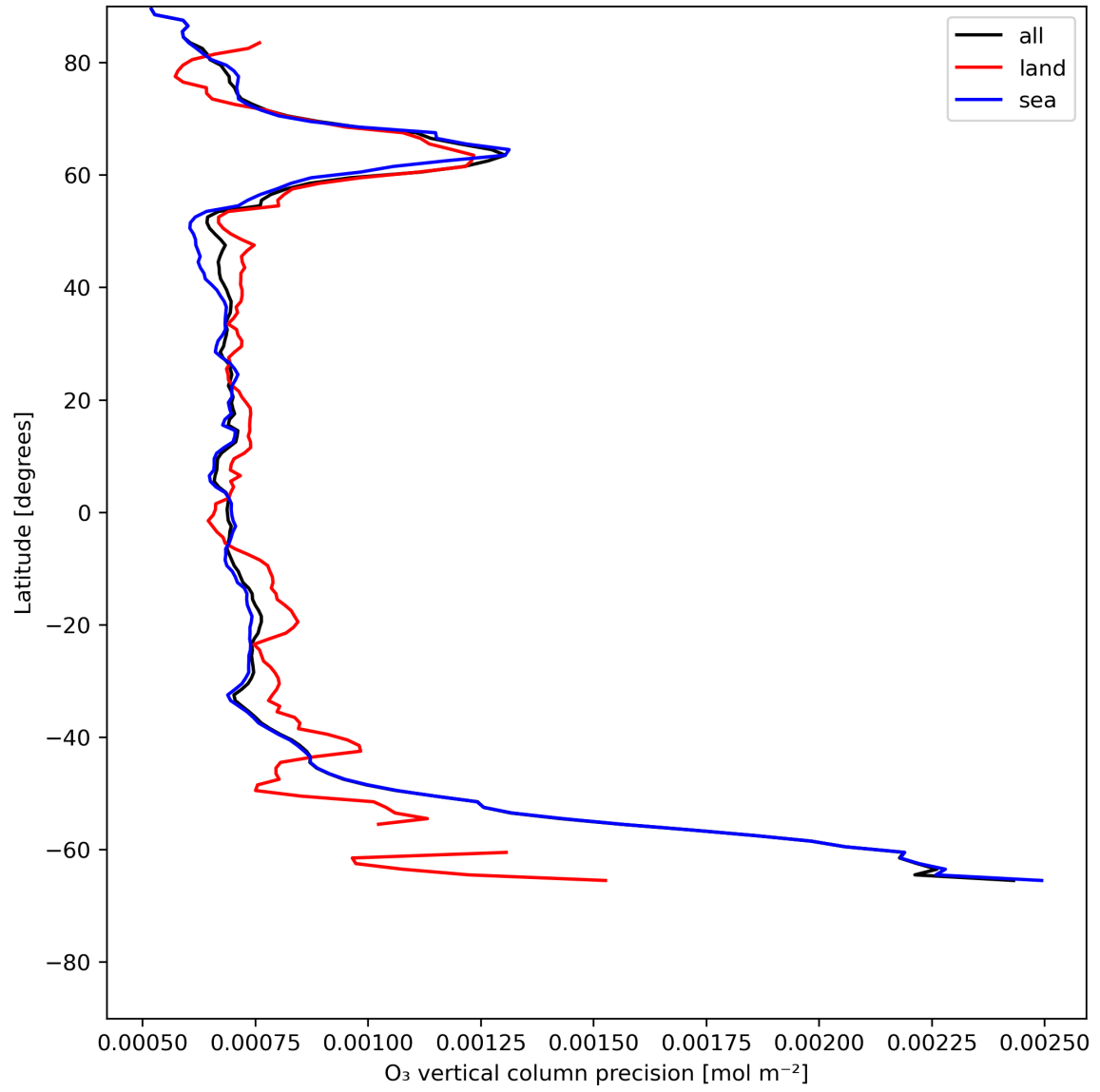
Figure 15: Zonal average of “O 3 vertical column precision” for 2024-06-19 to 2024-06-20.
