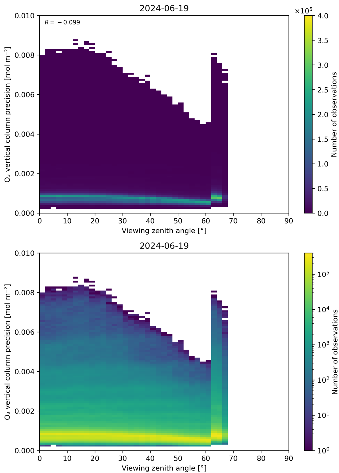
Figure 53: Scatter density plot of “Viewing zenith angle” against “O 3 vertical column precision” for 2024-06-19 to 2024-06-20.
