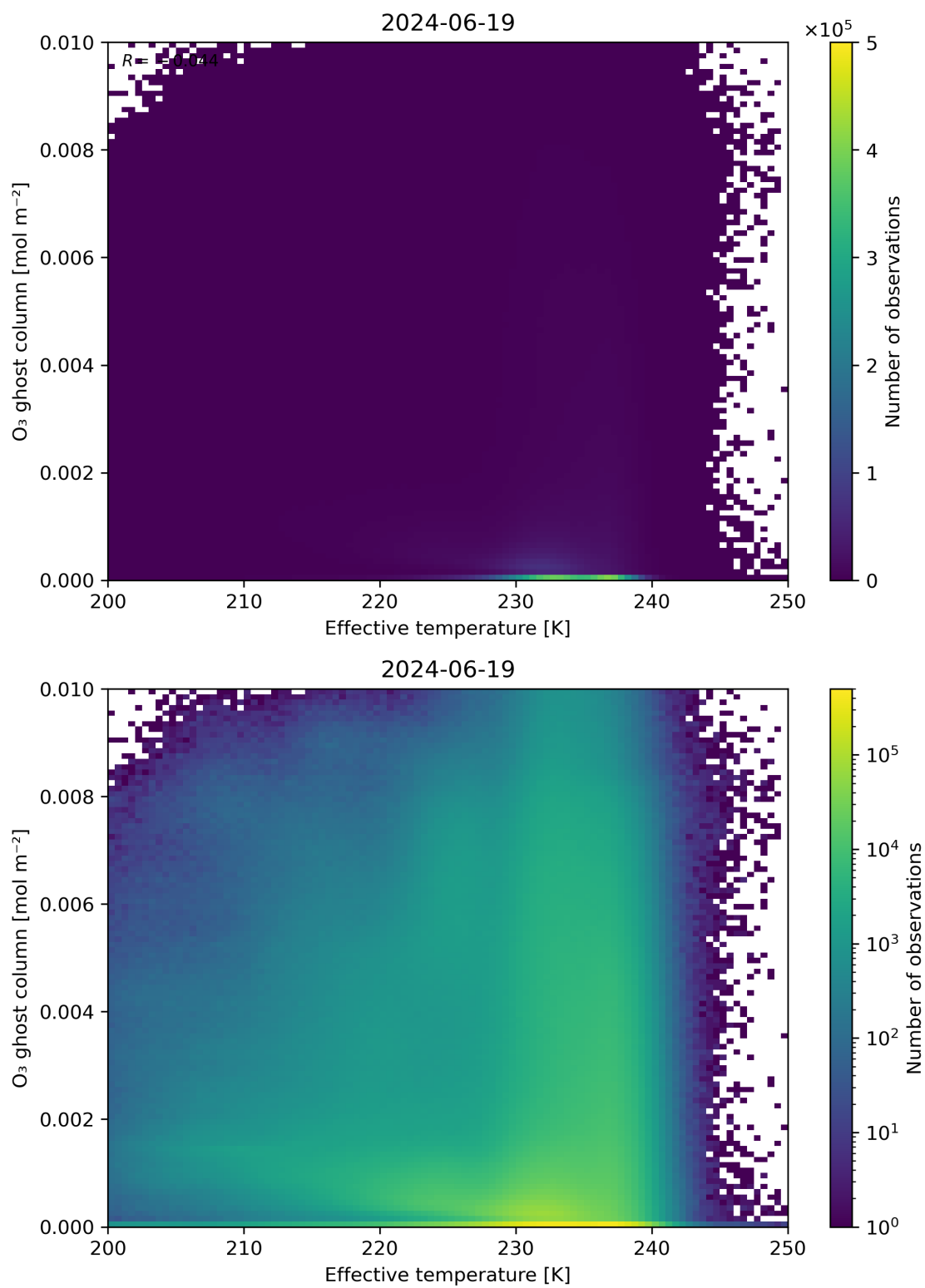
Figure 38: Scatter density plot of “Effective temperature” against “O 3 ghost column” for 2024-06-19 to 2024-06-20.
