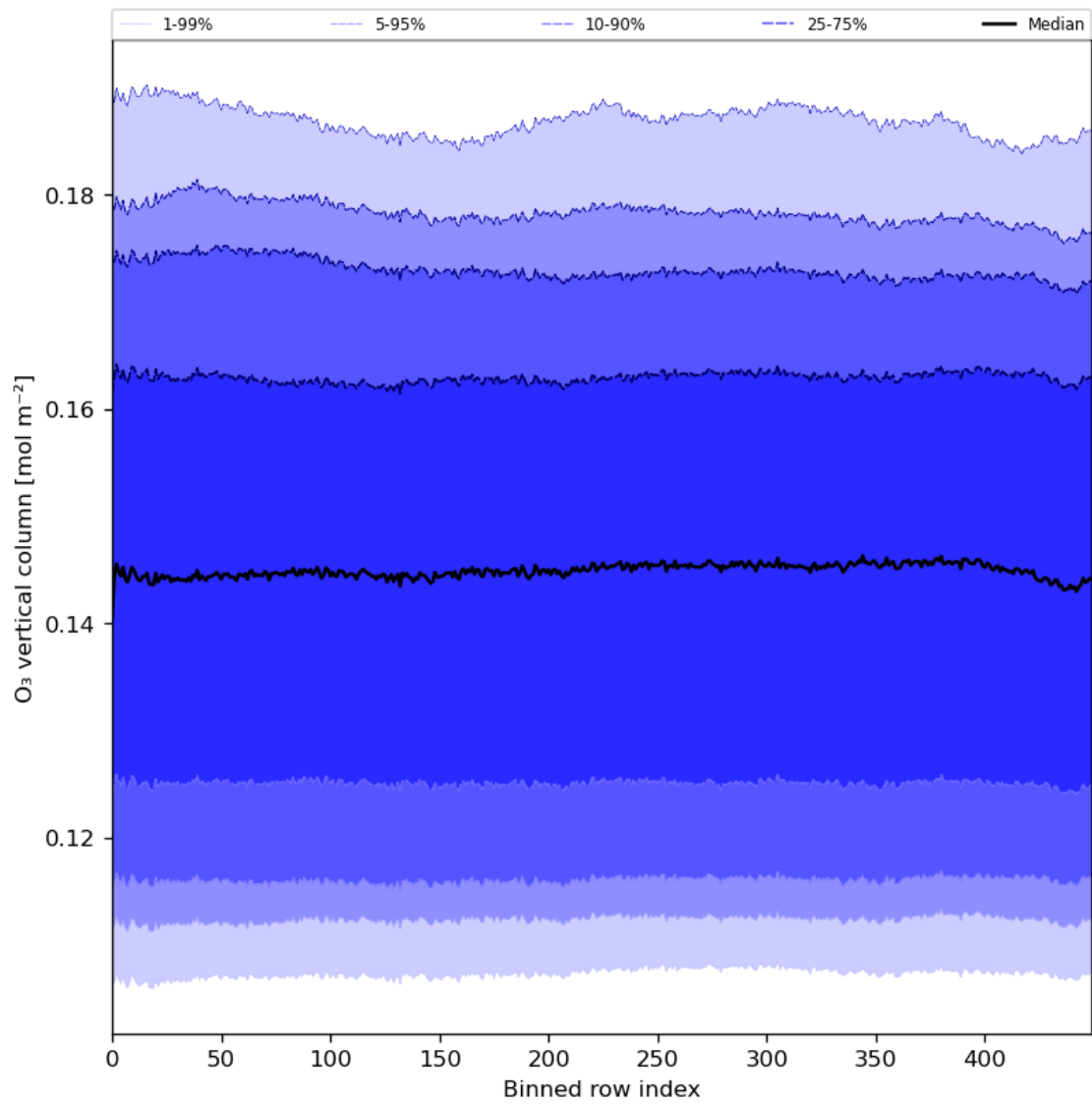
Figure 28: Along track statistics of “O 3 vertical column” for 2024-06-19 to 2024-06-20
