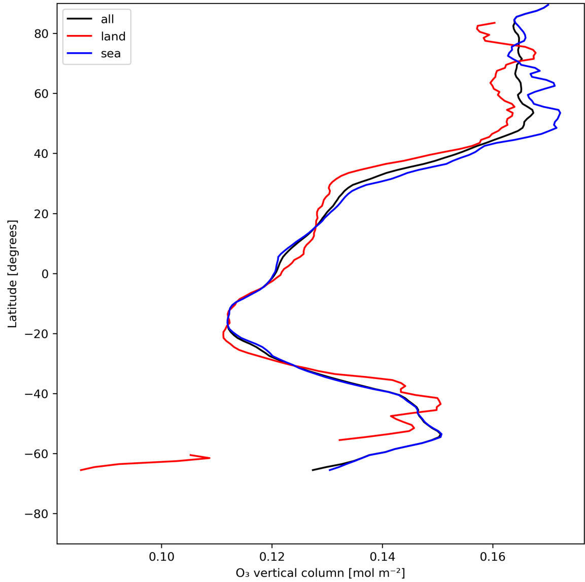
Figure 14: Zonal average of “O 3 vertical column” for 2024-06-19 to 2024-06-20.
