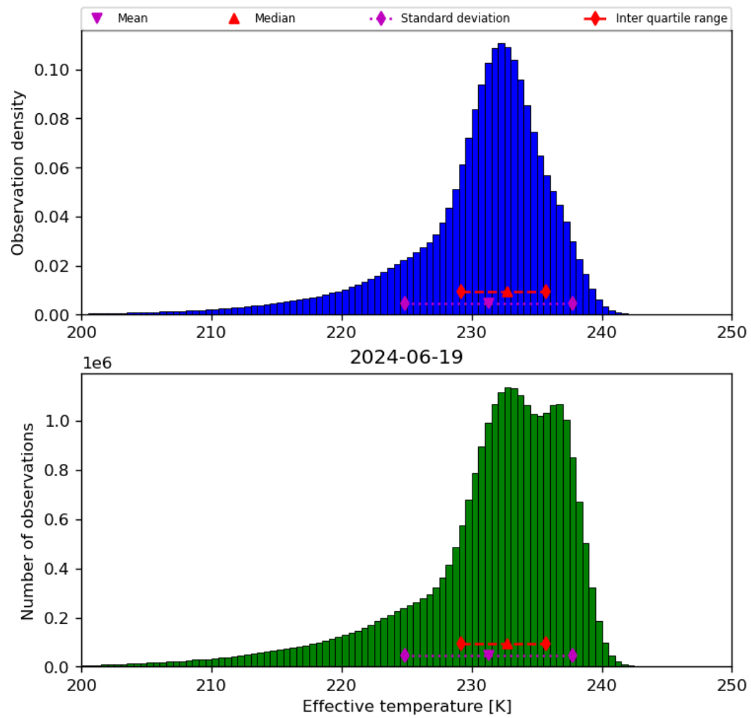
Figure 24: Histogram of “Effective temperature” for 2024-06-19 to 2024-06-20
