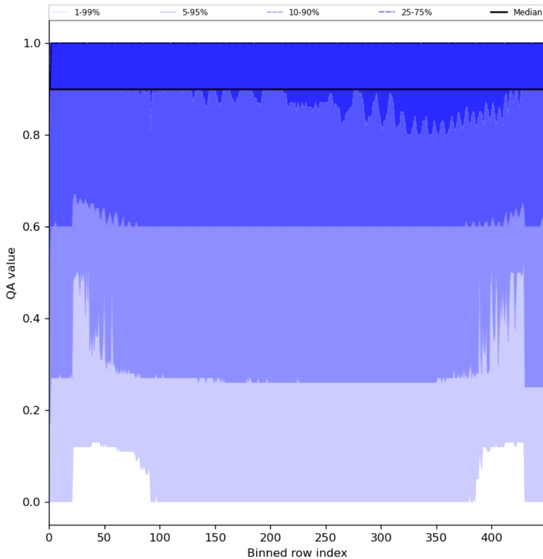
Figure 27: Along track statistics of “QA value” for 2024-06-19 to 2024-06-20
