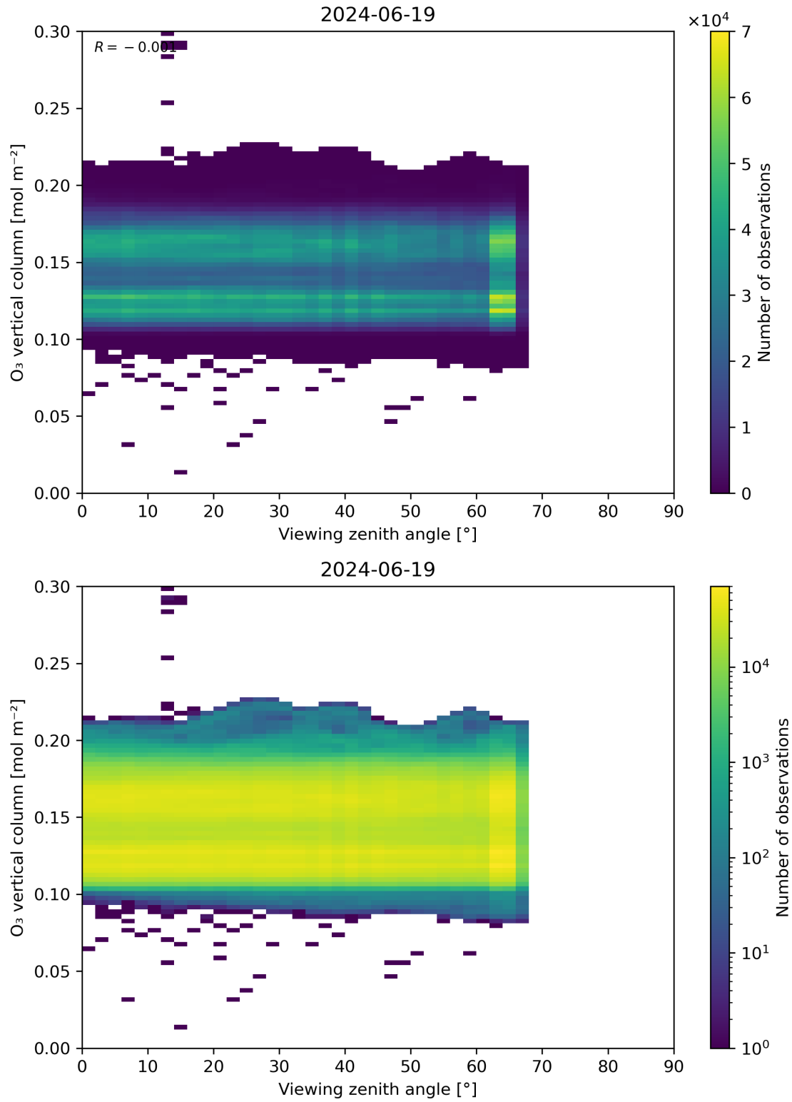
Figure 52: Scatter density plot of “Viewing zenith angle” against “O 3 vertical column” for 2024-06-19 to 2024-06-20.
