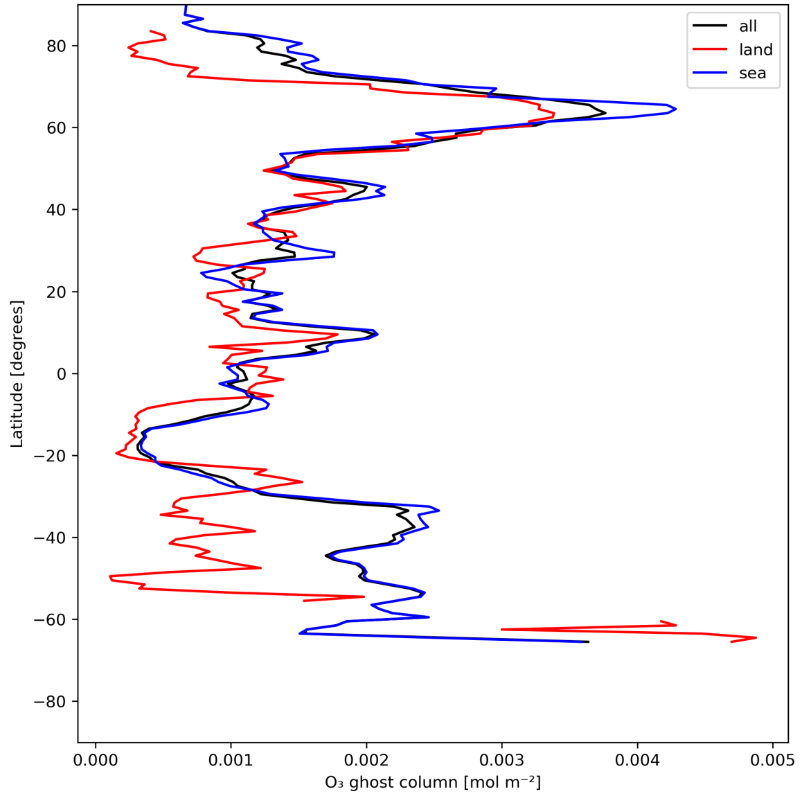
Figure 18: Zonal average of “O 3 ghost column” for 2024-06-19 to 2024-06-20.
