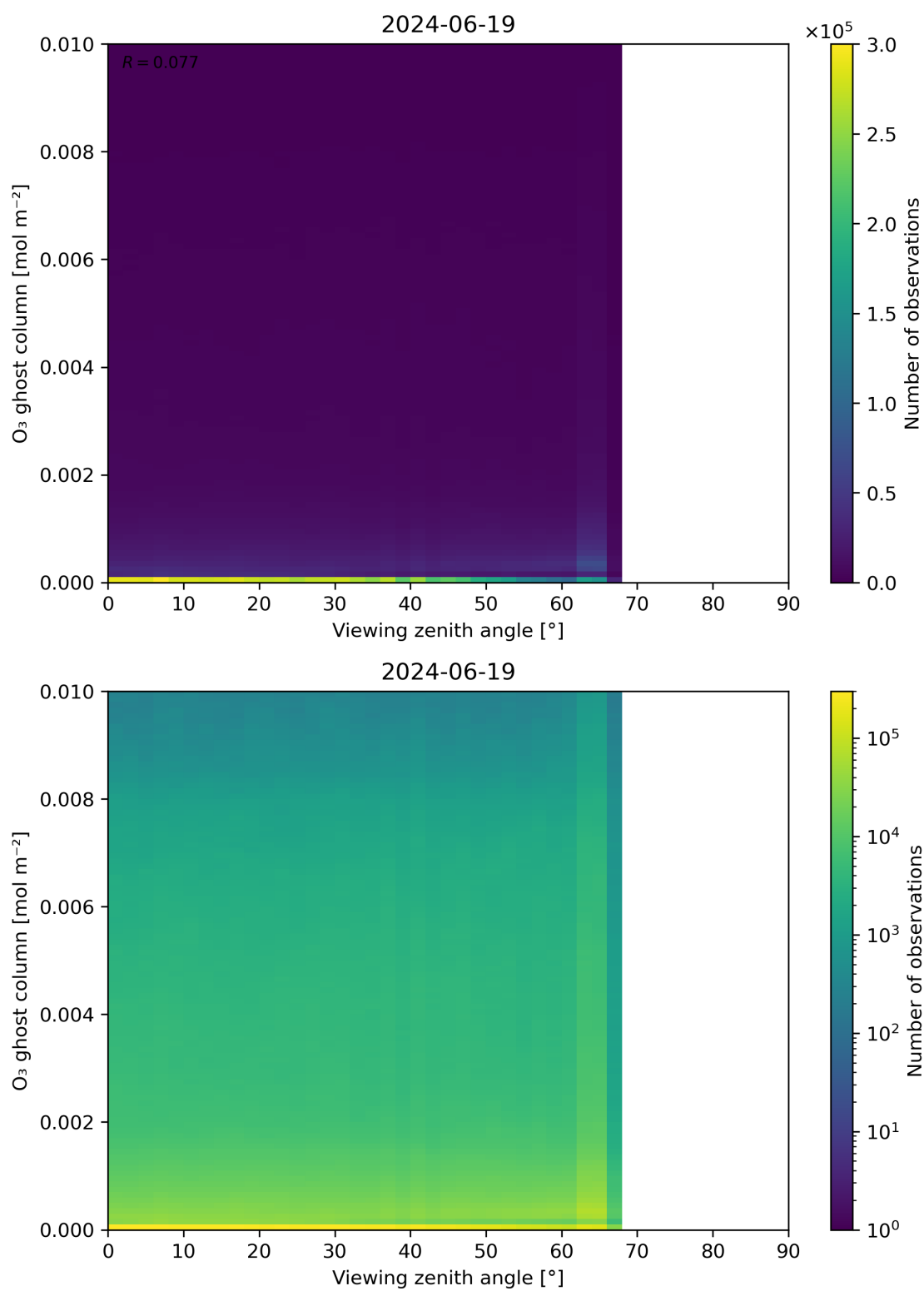
Figure 51: Scatter density plot of “Viewing zenith angle” against “O 3 ghost column” for 2024-06-19 to 2024-06-20.
