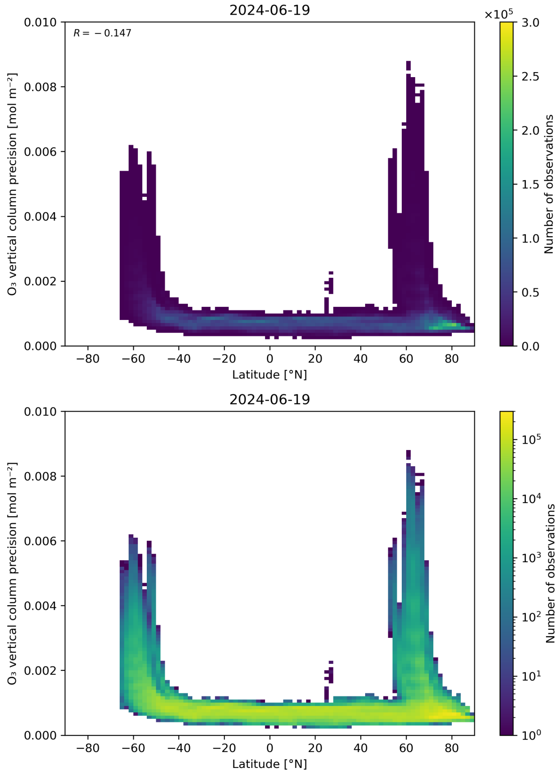
Figure 37: Scatter density plot of “Latitude” against “O 3 vertical column precision” for 2024-06-19 to 2024-06-20.
