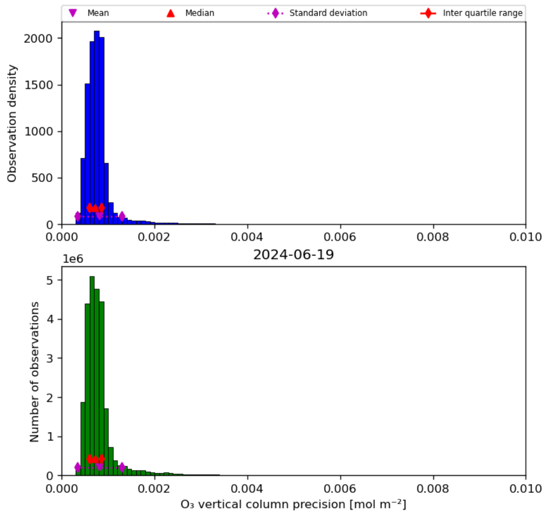
Figure 22: Histogram of “O 3 vertical column precision” for 2024-06-19 to 2024-06-20
