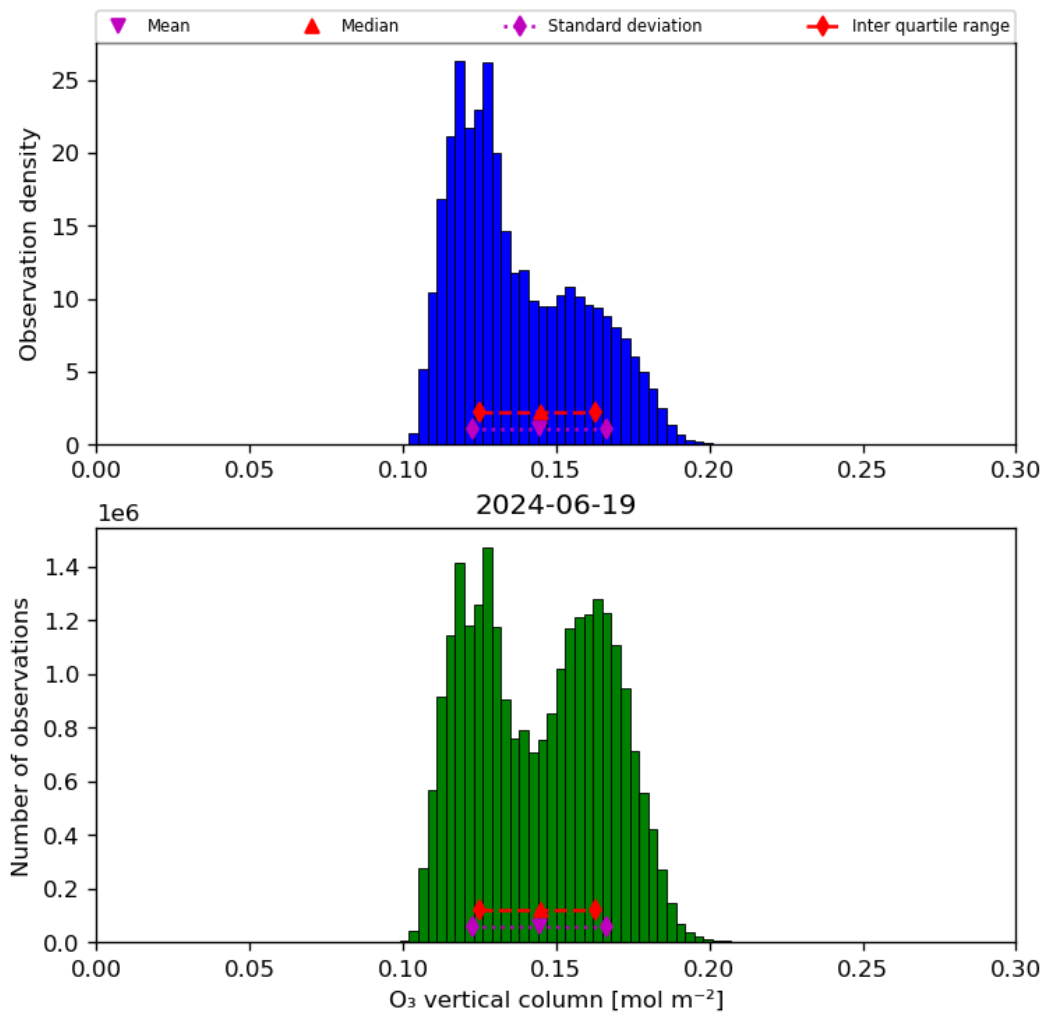
Figure 21: Histogram of “O 3 vertical column” for 2024-06-19 to 2024-06-20
