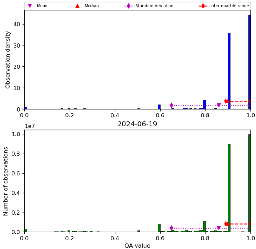
Figure 20: Histogram of “QA value” for 2024-06-19 to 2024-06-20
