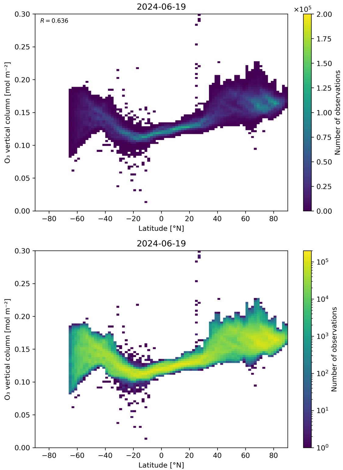
Figure 36: Scatter density plot of “Latitude” against “O 3 vertical column” for 2024-06-19 to 2024-06-20.
