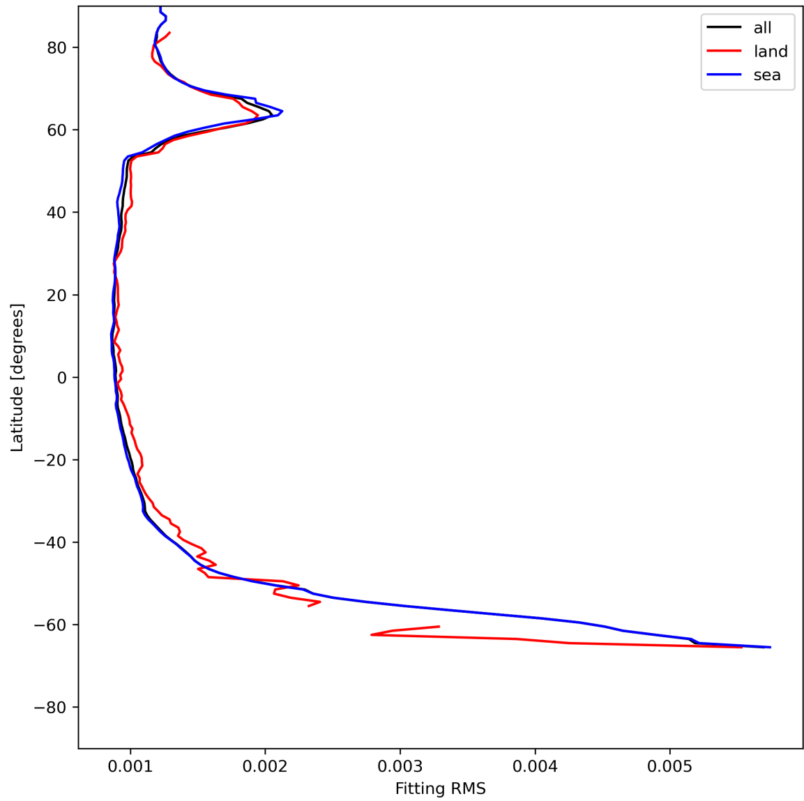
Figure 16: Zonal average of “Fitting RMS” for 2024-06-19 to 2024-06-20.
