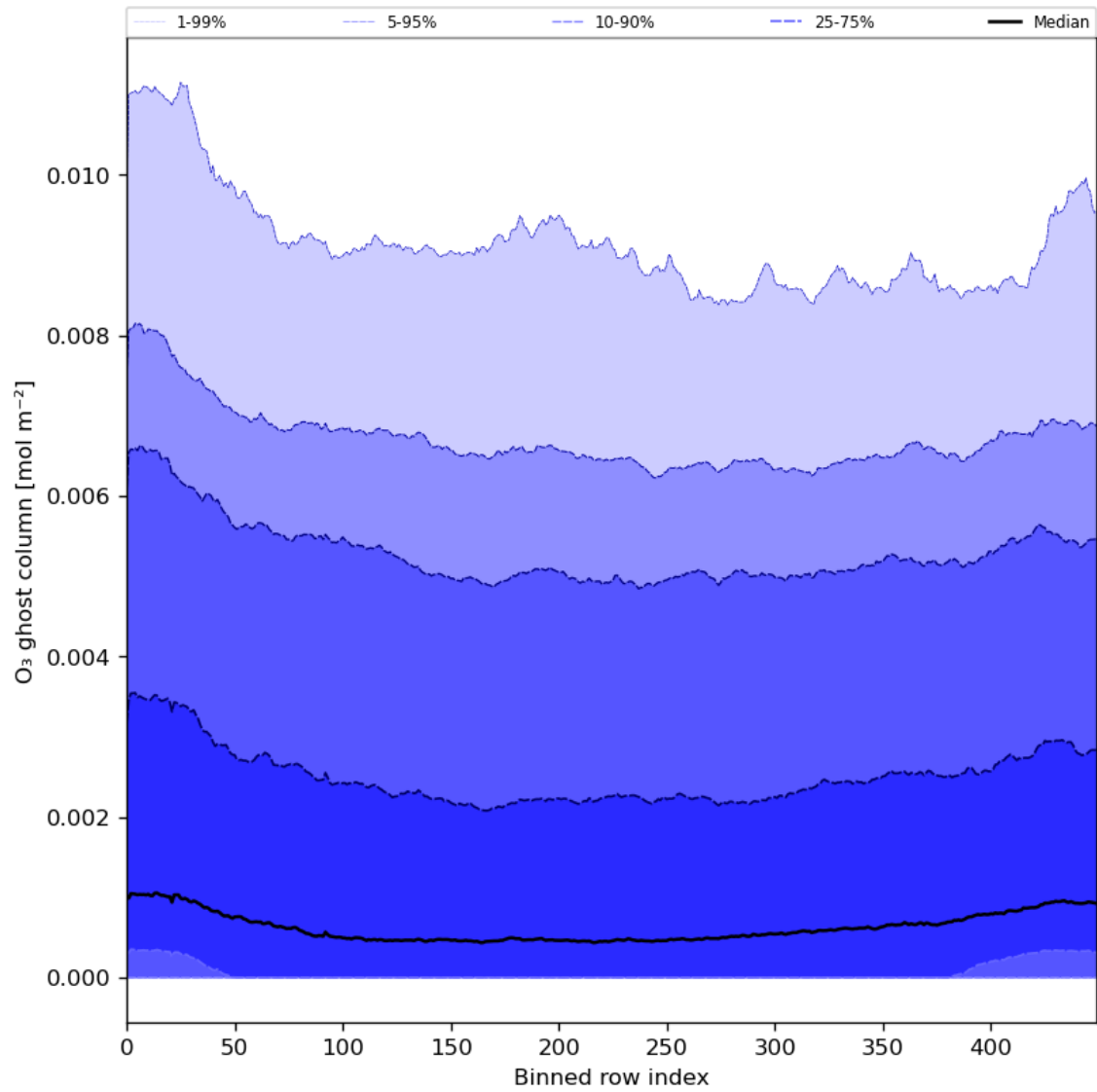
Figure 32: Along track statistics of "O 3 ghost column" for 2024-06-19 to 2024-06-20
