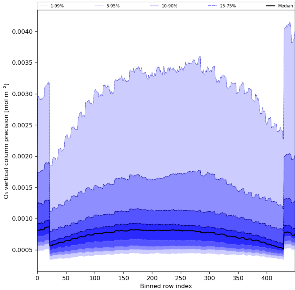
Figure 29: Along track statistics of "O 3 vertical column precision" for 2024-06-19 to 2024-06-20
