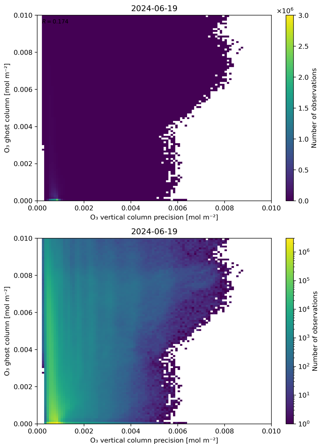
Figure 43: Scatter density plot of “ \text{O}_3 vertical column precision” against “ \text{O}_3 ghost column” for 2024-06-19 to 2024-06-20.
