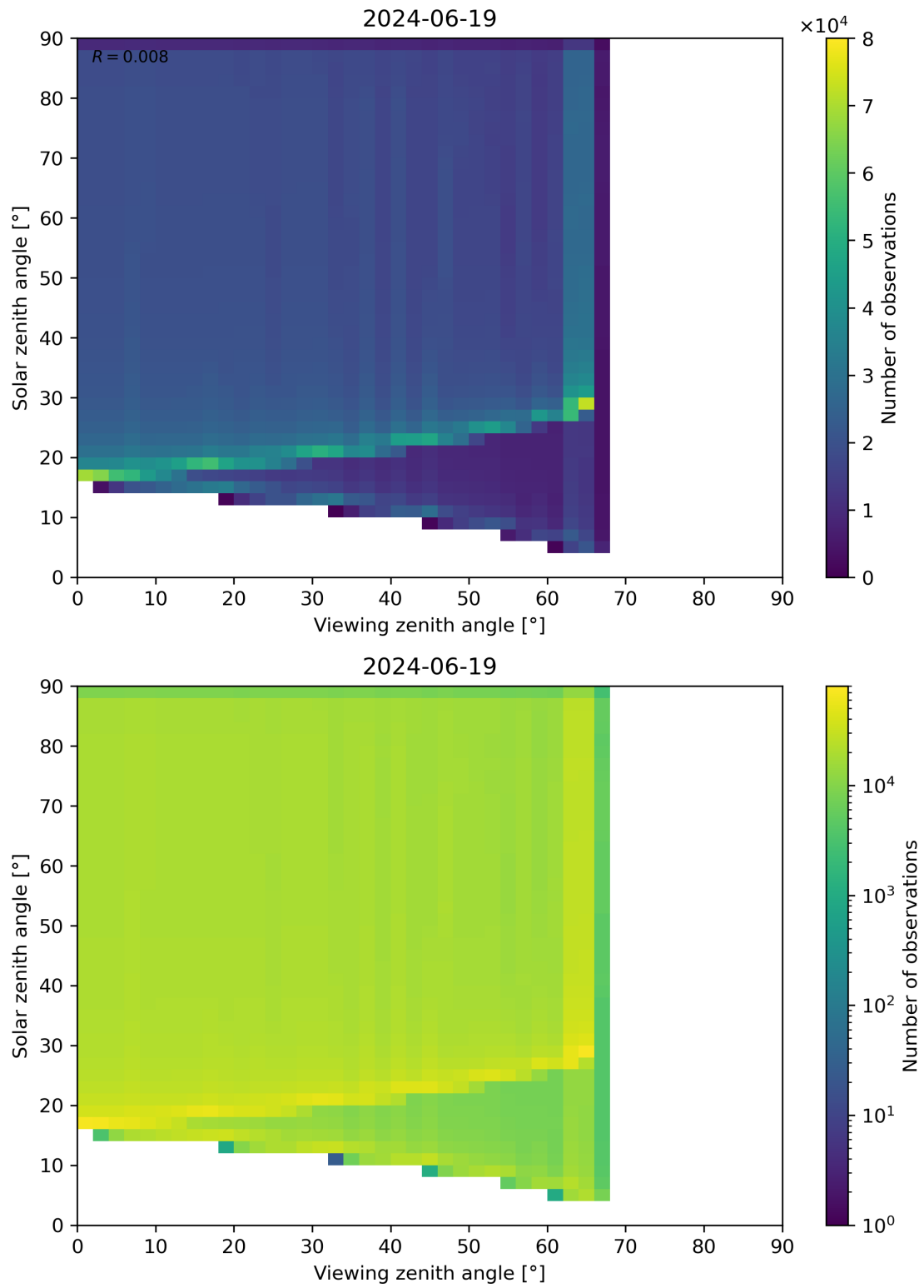
Figure 54: Scatter density plot of “Viewing zenith angle” against “Solar zenith angle” for 2024-06-19 to 2024-06-20.
