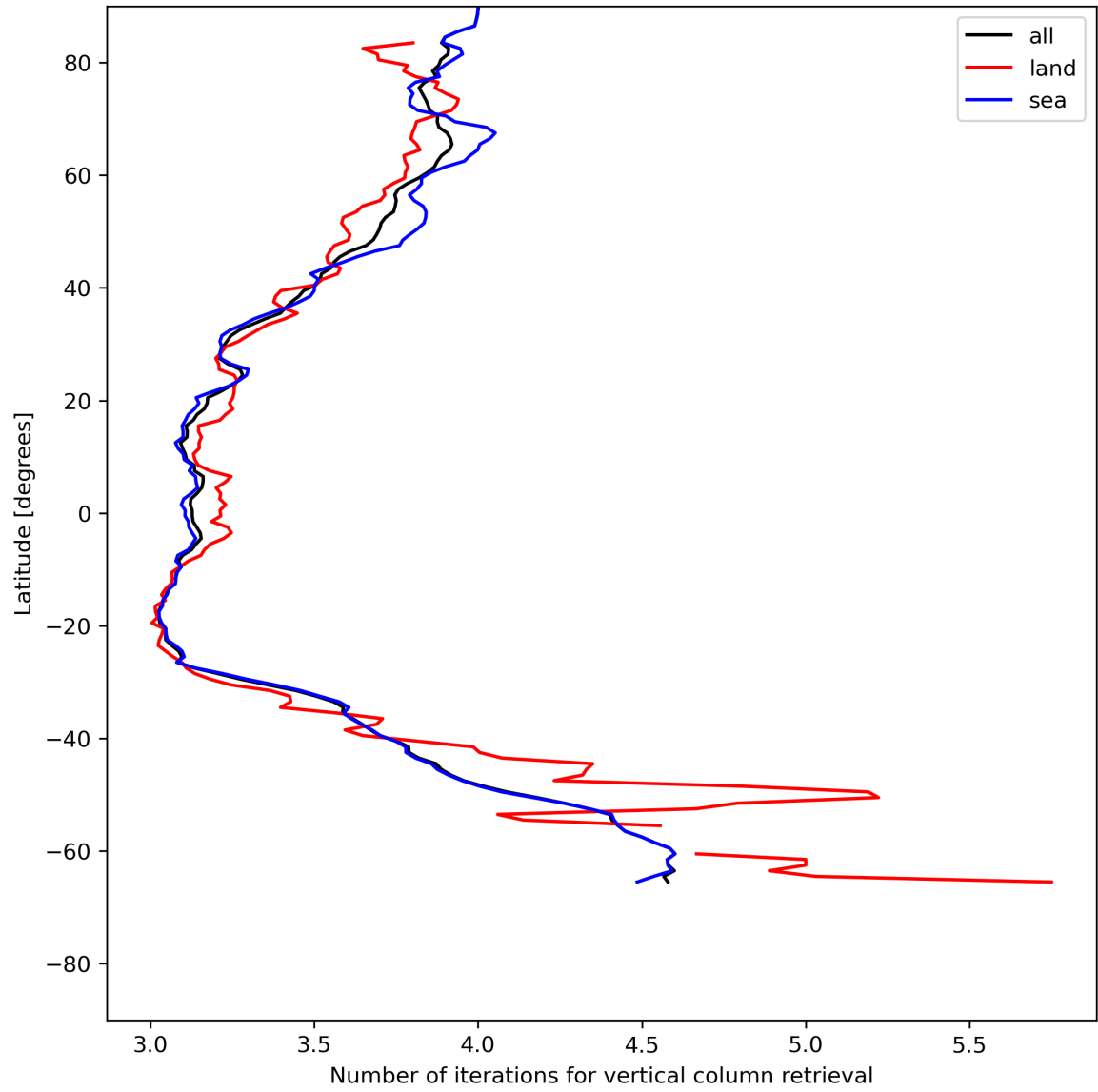
Figure 19: Zonal average of “Number of iterations for vertical column retrieval” for 2024-06-19 to 2024-06-20.
