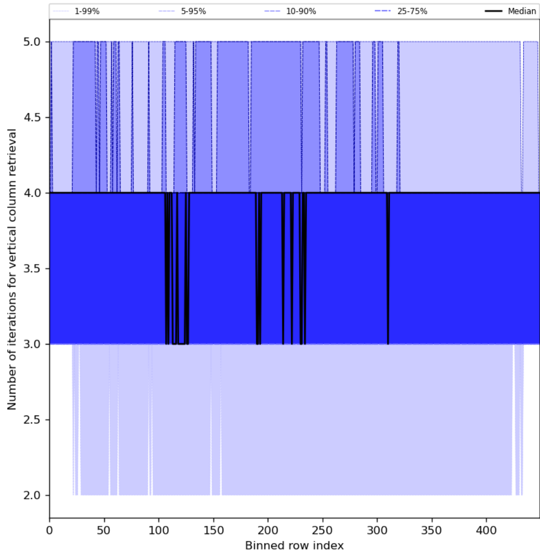
Figure 33: Along track statistics of “Number of iterations for vertical column retrieval” for 2024-06-19 to 2024-06-20
