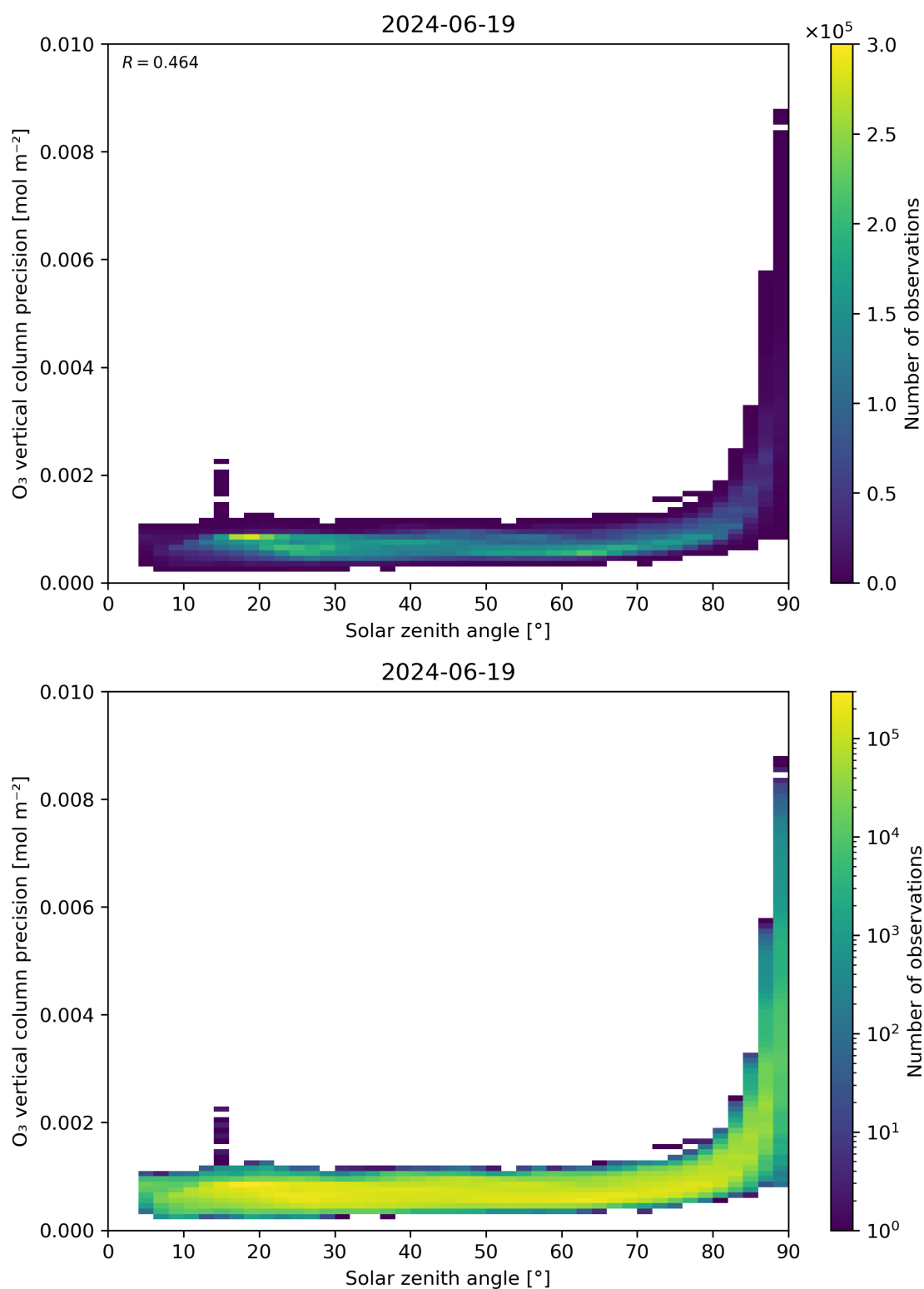
Figure 48: Scatter density plot of “Solar zenith angle” against “O 3 vertical column precision” for 2024-06-19 to 2024-06-20.
