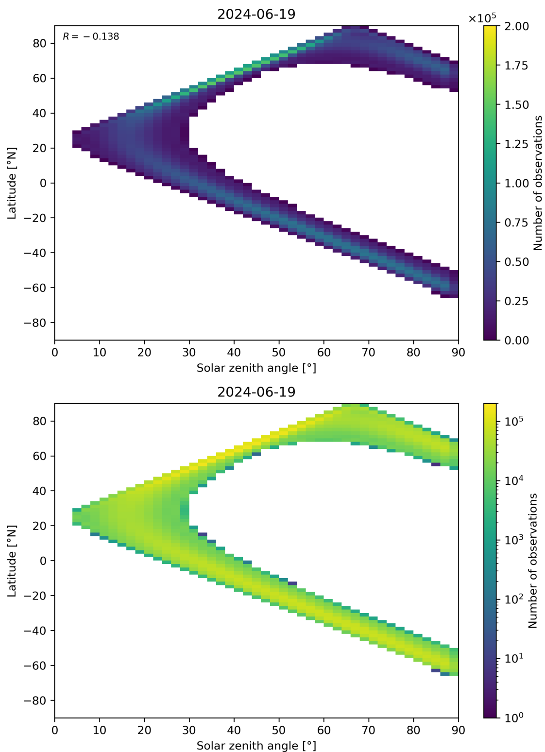
Figure 44: Scatter density plot of “Solar zenith angle” against “Latitude” for 2024-06-19 to 2024-06-20.
