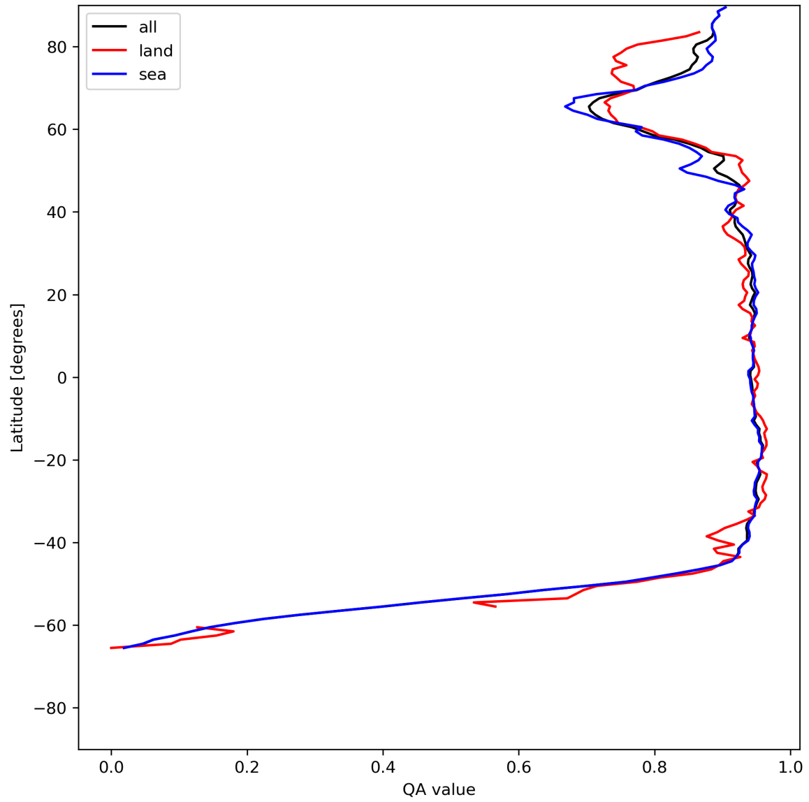
Figure 13: Zonal average of “QA value” for 2024-06-19 to 2024-06-20.
