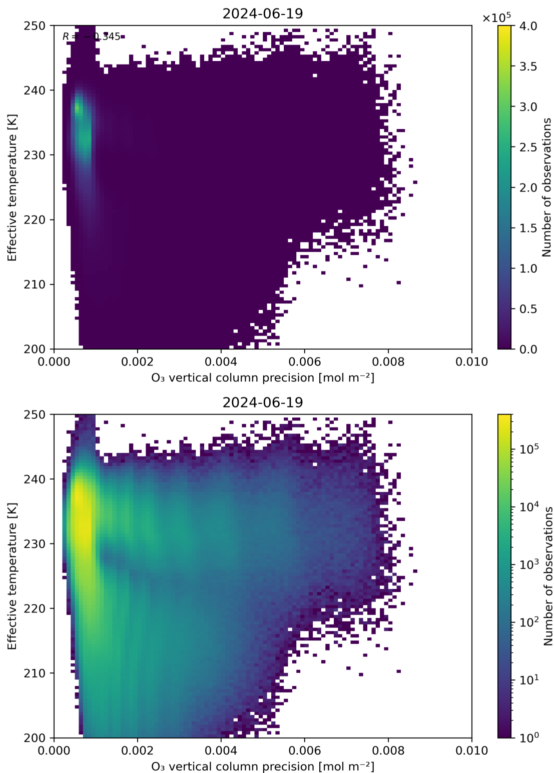
Figure 42: Scatter density plot of “O 3 vertical column precision” against “Effective temperature” for 2024-06-19 to 2024-06-20.
