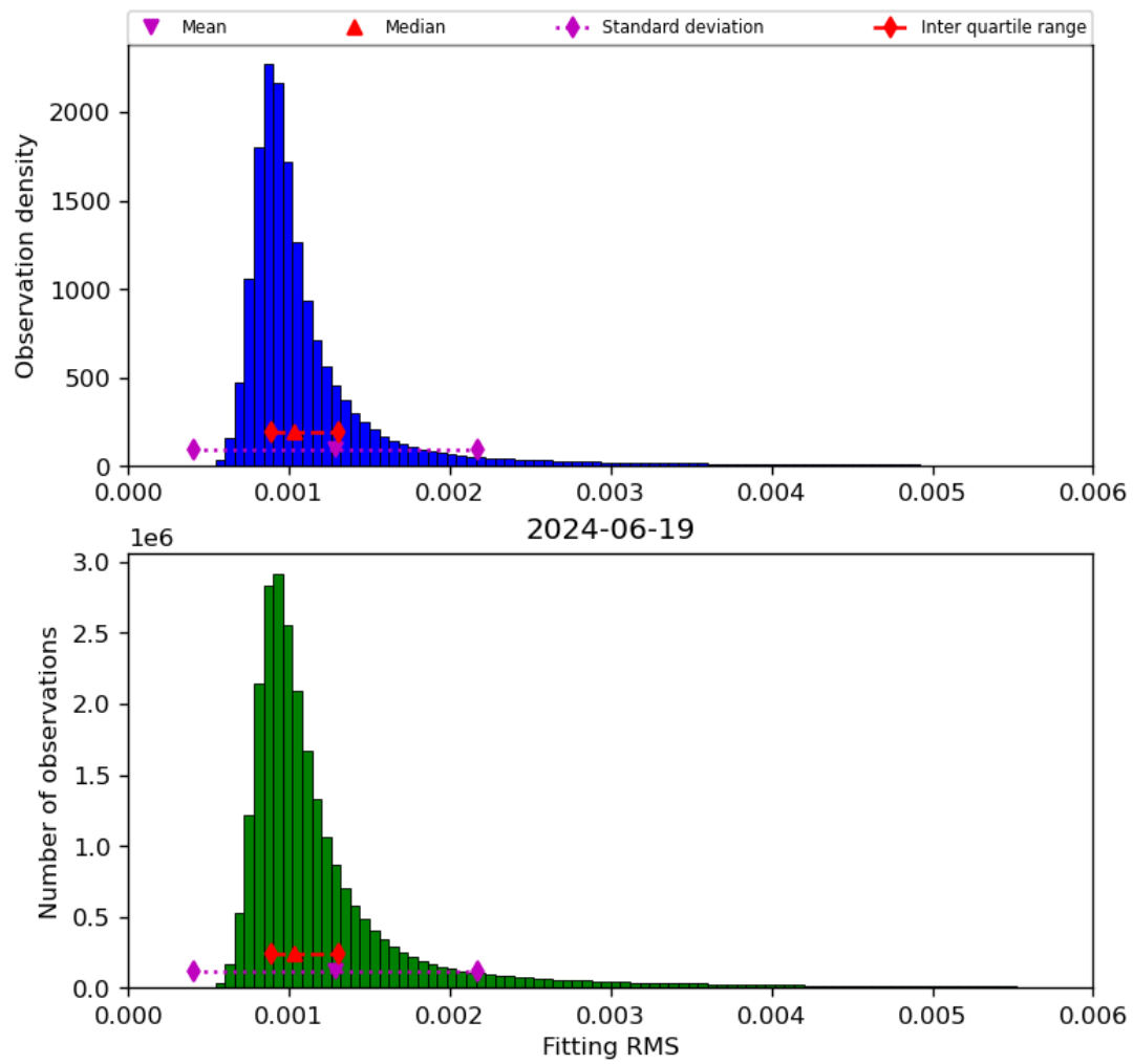
Figure 23: Histogram of “Fitting RMS” for 2024-06-19 to 2024-06-20
