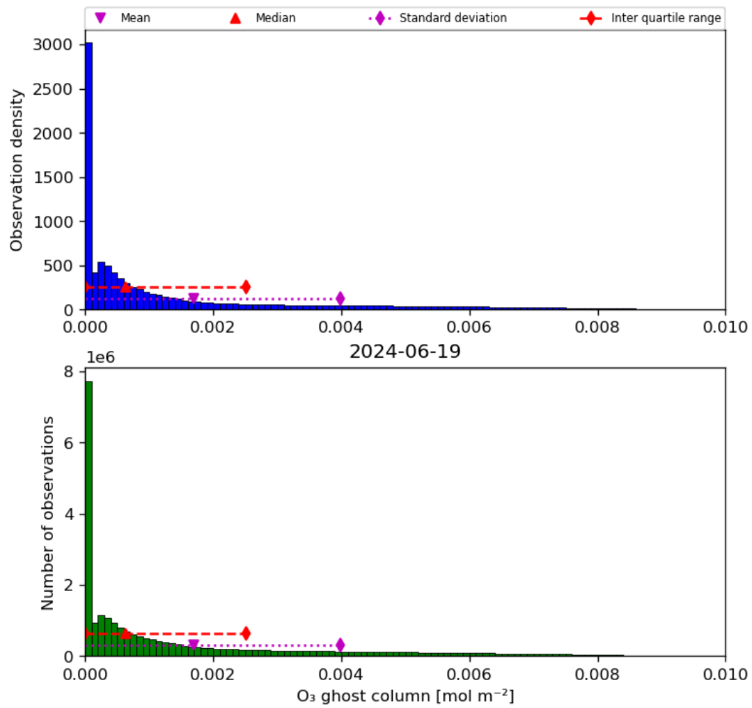
Figure 25: Histogram of “O 3 ghost column” for 2024-06-19 to 2024-06-20
