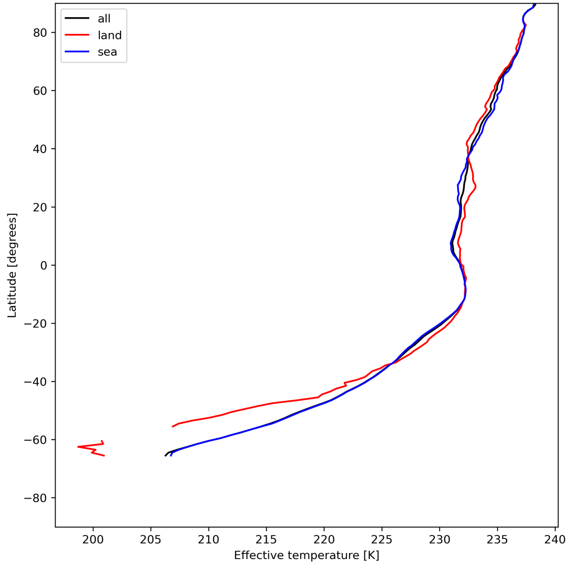
Figure 17: Zonal average of "Effective temperature" for 2024-06-19 to 2024-06-20.
