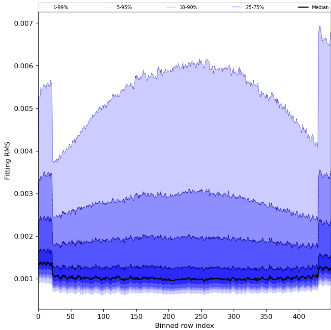
Figure 30: Along track statistics of “Fitting RMS” for 2024-06-19 to 2024-06-20
