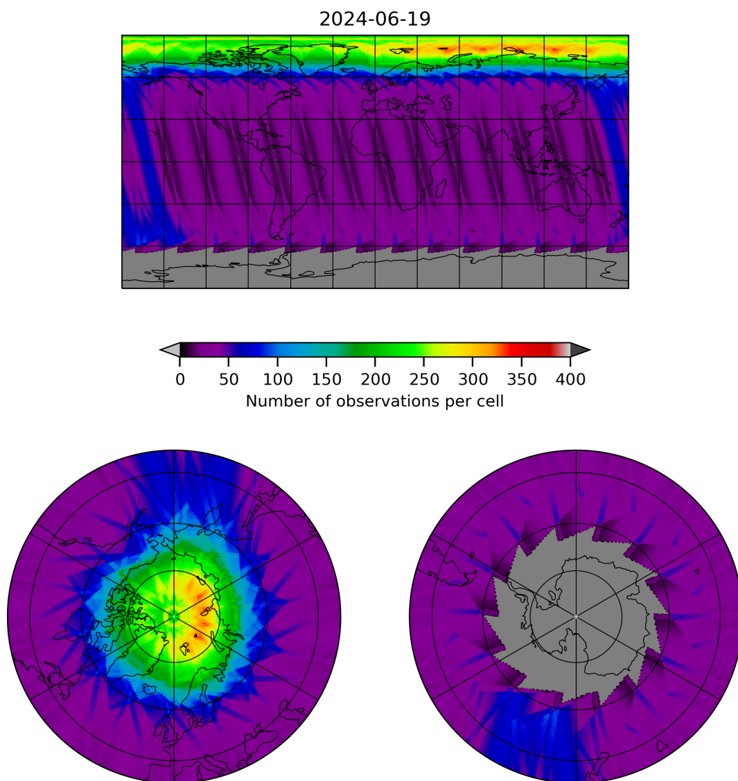
Figure 12: Map of the number of observations for 2024-06-19 to 2024-06-20
