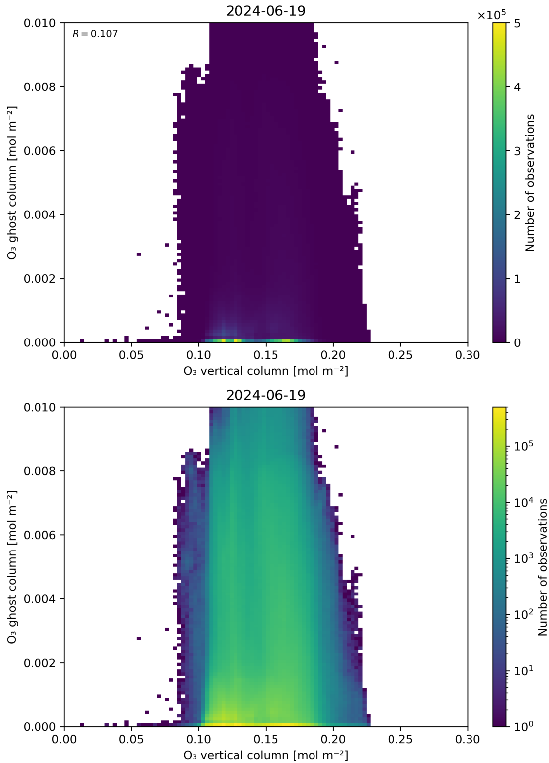
Figure 40: Scatter density plot of “O 3 vertical column” against “O 3 ghost column” for 2024-06-19 to 2024-06-20.
