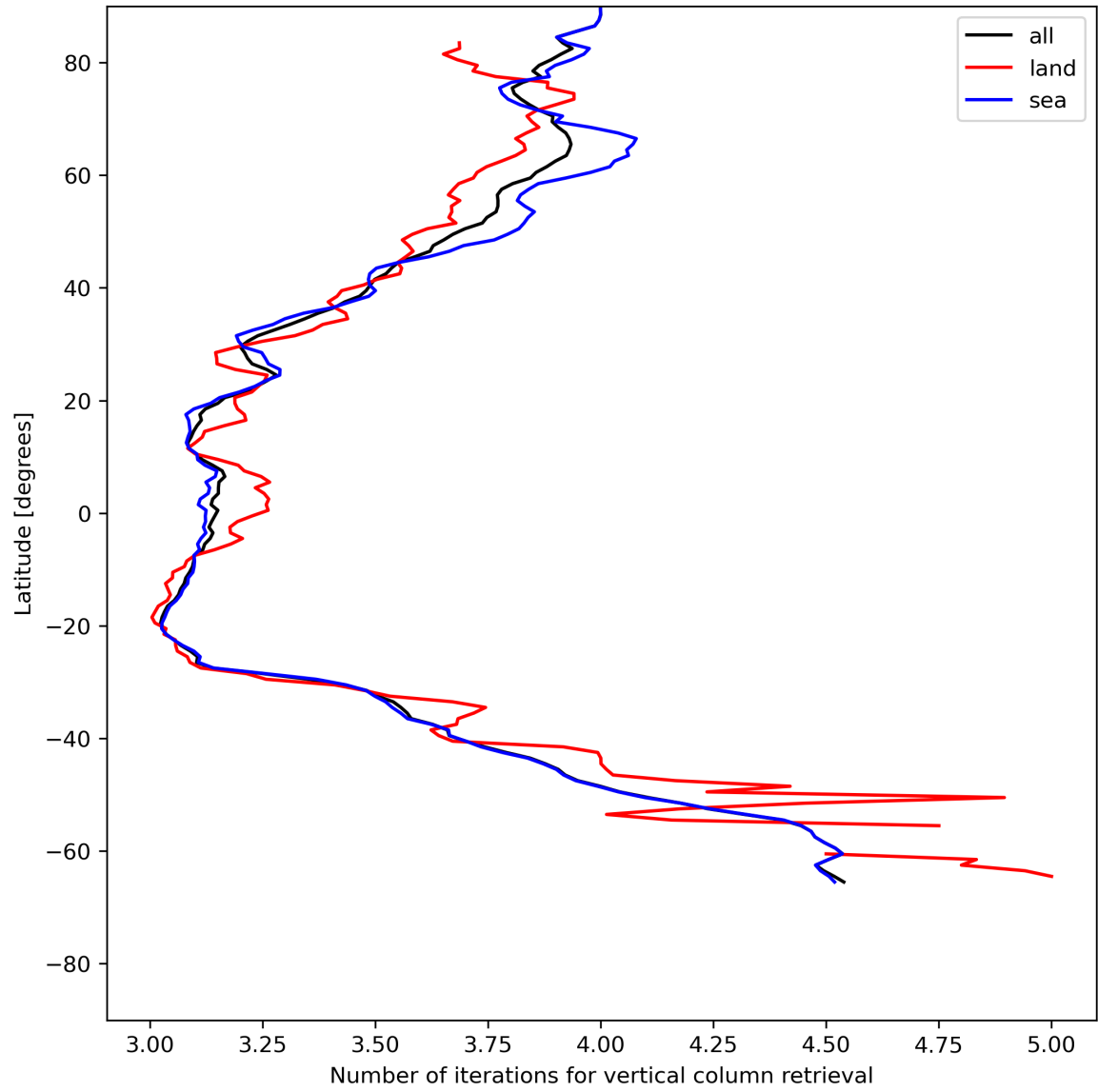
Figure 19: Zonal average of “Number of iterations for vertical column retrieval” for 2024-06-19 to 2024-06-21.
