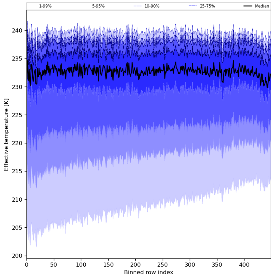
Figure 31: Along track statistics of “Effective temperature” for 2024-06-19 to 2024-06-21
