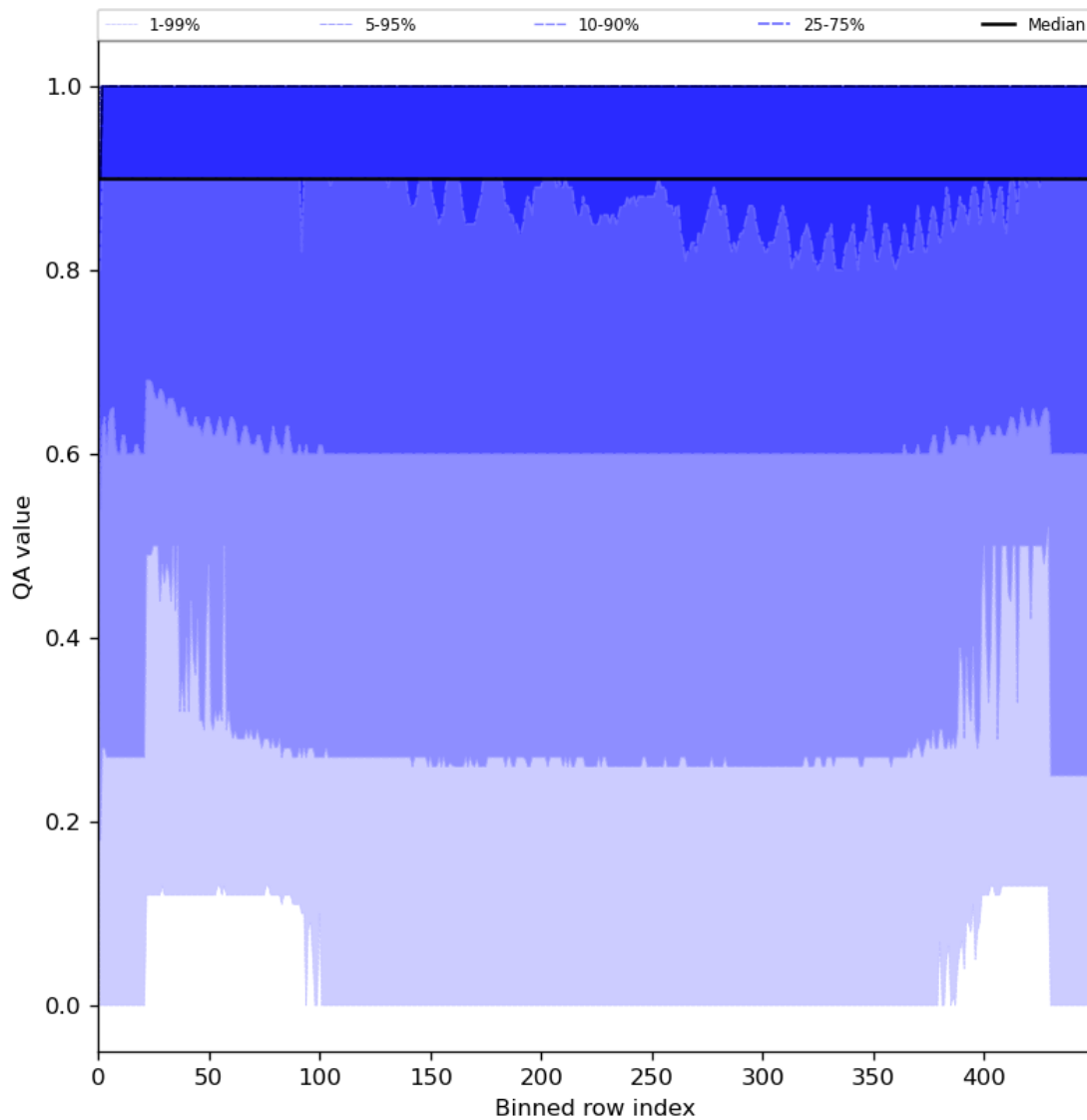
Figure 27: Along track statistics of “QA value” for 2024-06-19 to 2024-06-21
