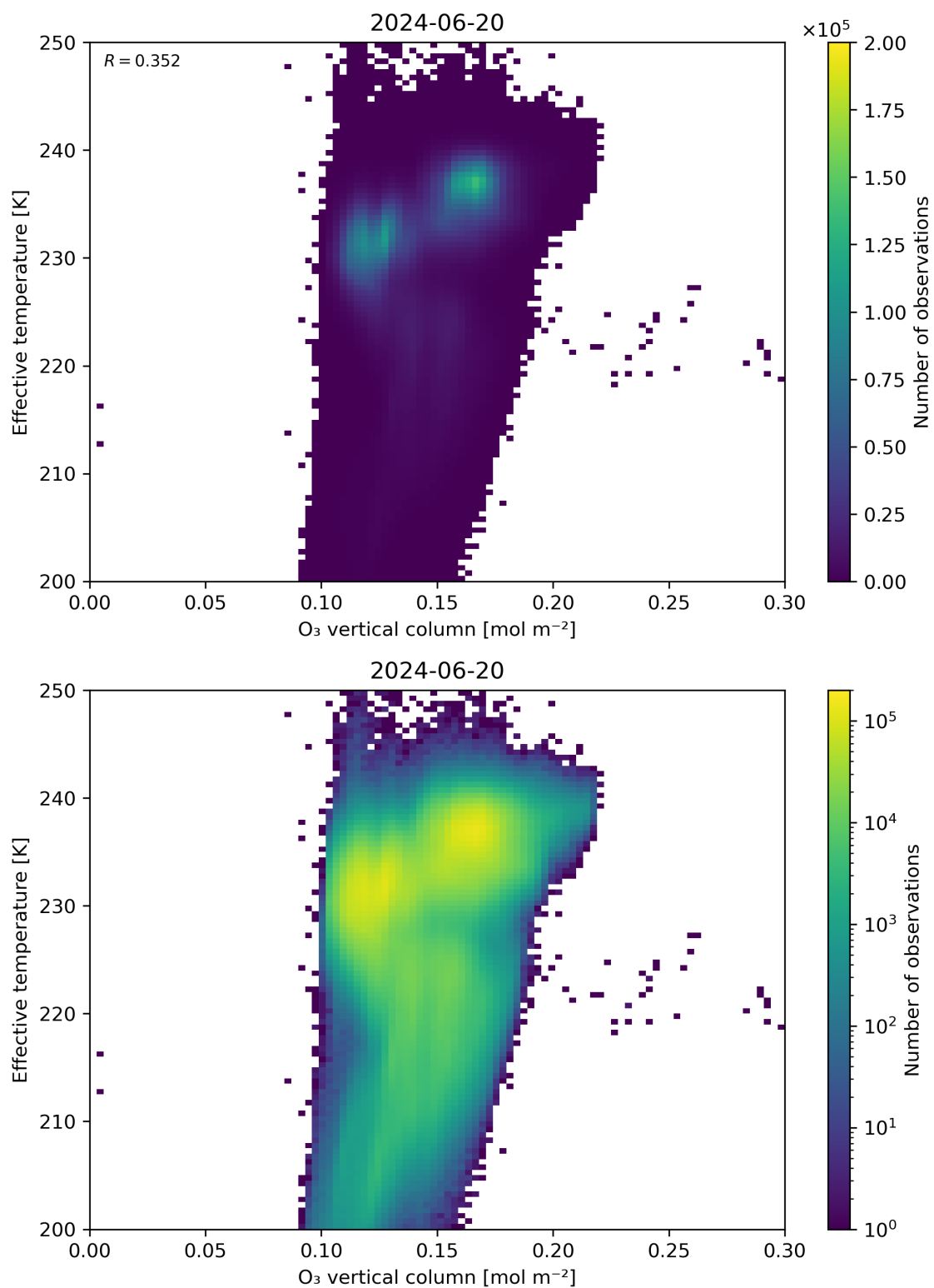
Figure 39: Scatter density plot of “O 3 vertical column” against “Effective temperature” for 2024-06-19 to 2024-06-21.
