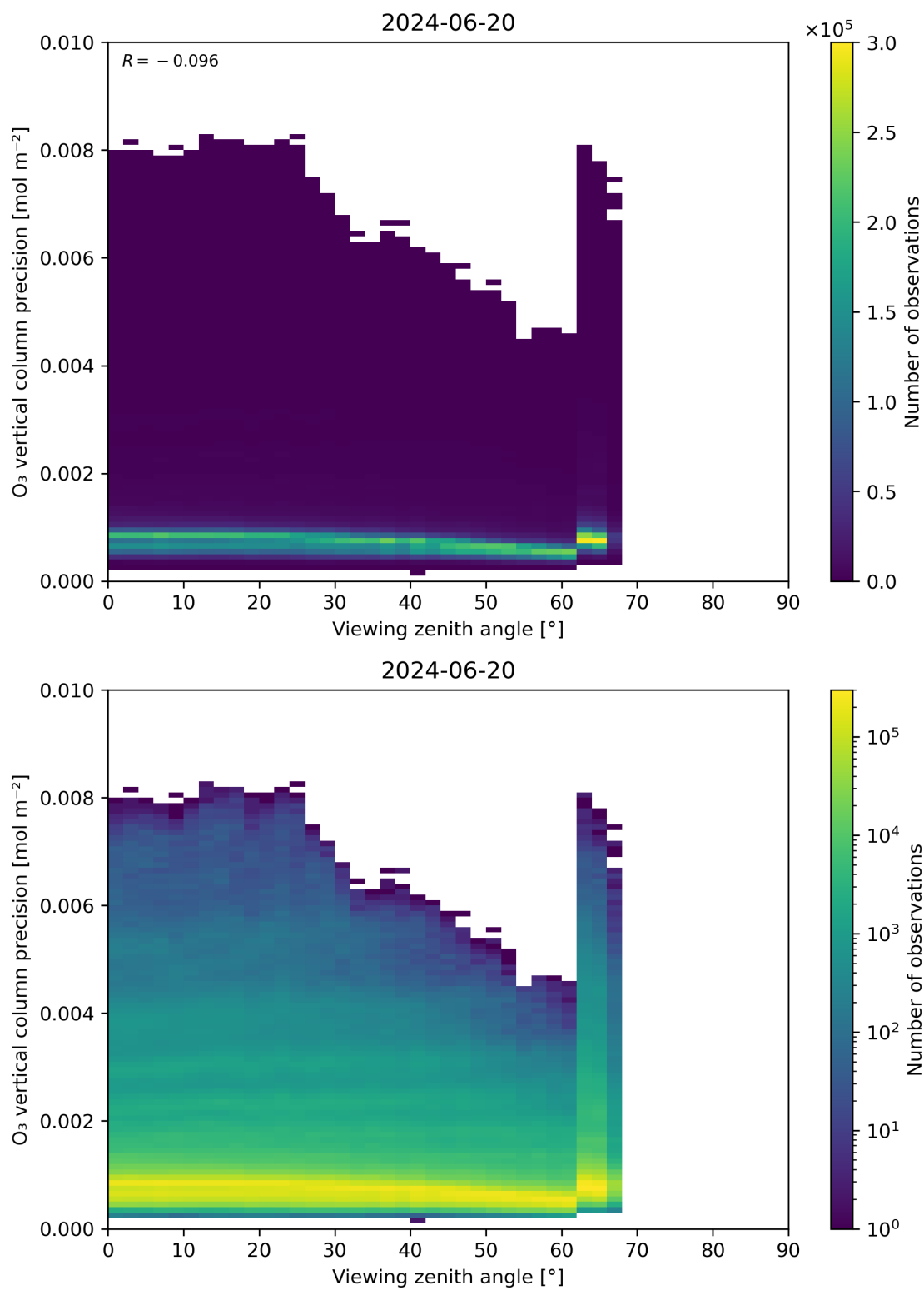
Figure 53: Scatter density plot of “Viewing zenith angle” against “O 3 vertical column precision” for 2024-06-19 to 2024-06-21.
