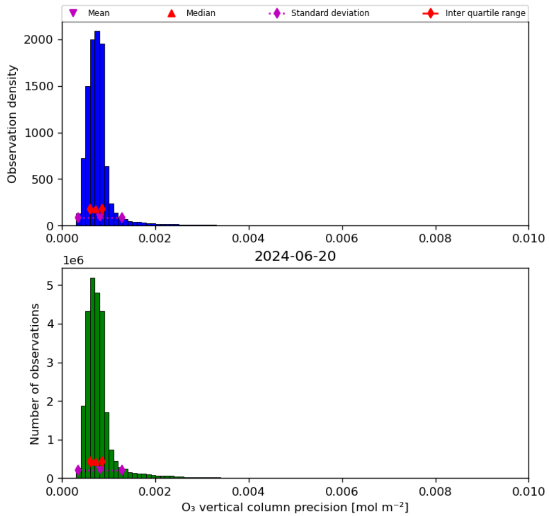
Figure 22: Histogram of “O 3 vertical column precision” for 2024-06-19 to 2024-06-21
