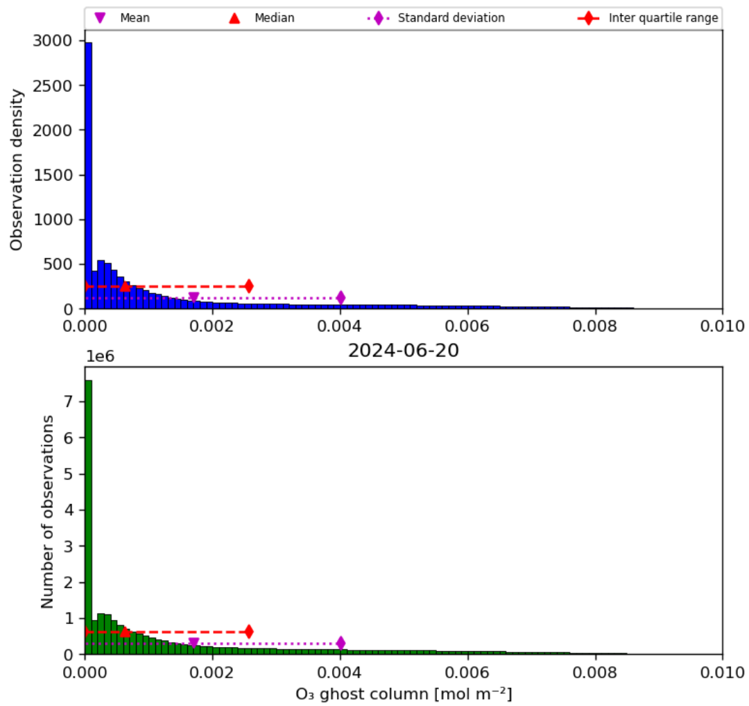
Figure 25: Histogram of “O 3 ghost column” for 2024-06-19 to 2024-06-21
