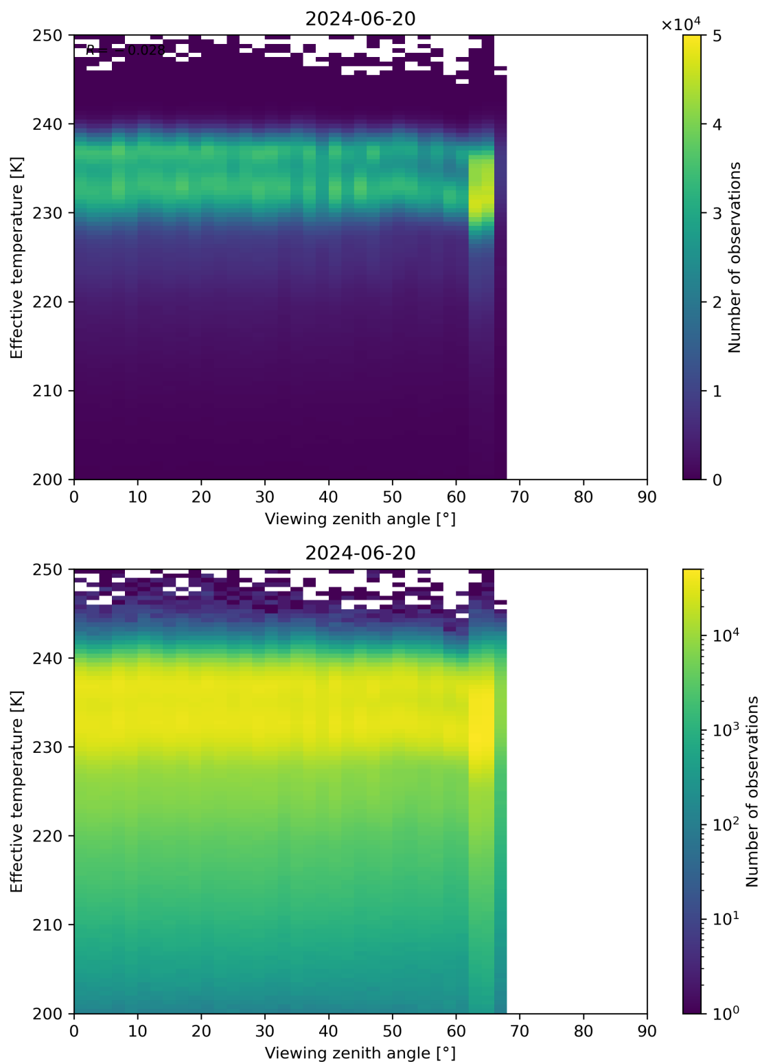
Figure 50: Scatter density plot of “Viewing zenith angle” against “Effective temperature” for 2024-06-19 to 2024-06-21.
