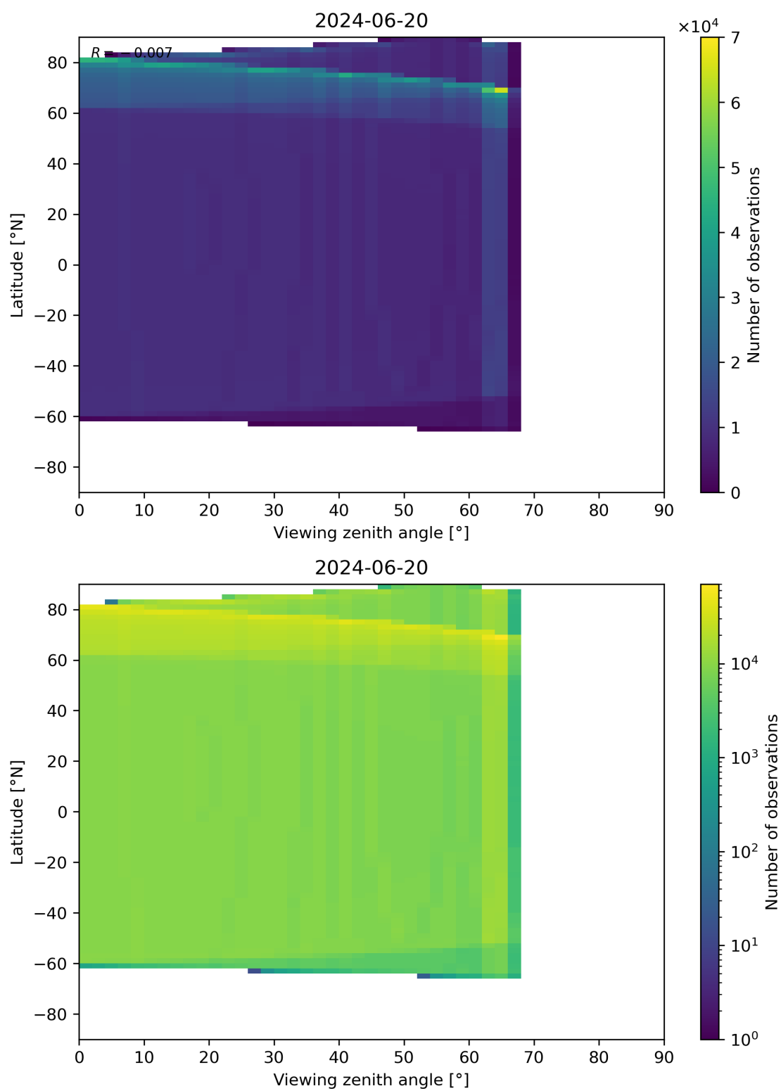
Figure 49: Scatter density plot of “Viewing zenith angle” against “Latitude” for 2024-06-19 to 2024-06-21.
