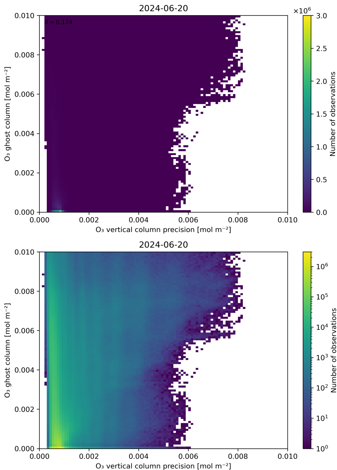
Figure 43: Scatter density plot of “ \text{O}_3 vertical column precision” against “ \text{O}_3 ghost column” for 2024-06-19 to 2024-06-21.
