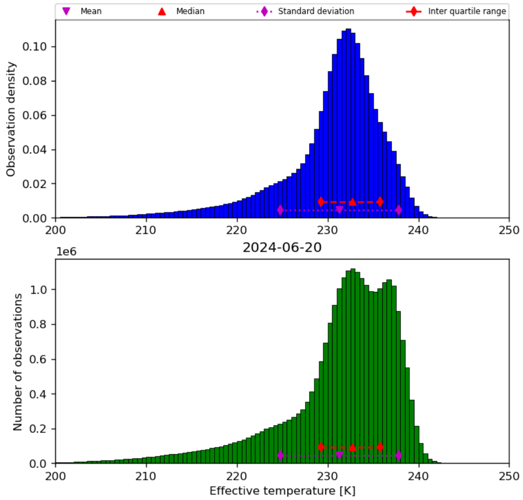
Figure 24: Histogram of “Effective temperature” for 2024-06-19 to 2024-06-21
