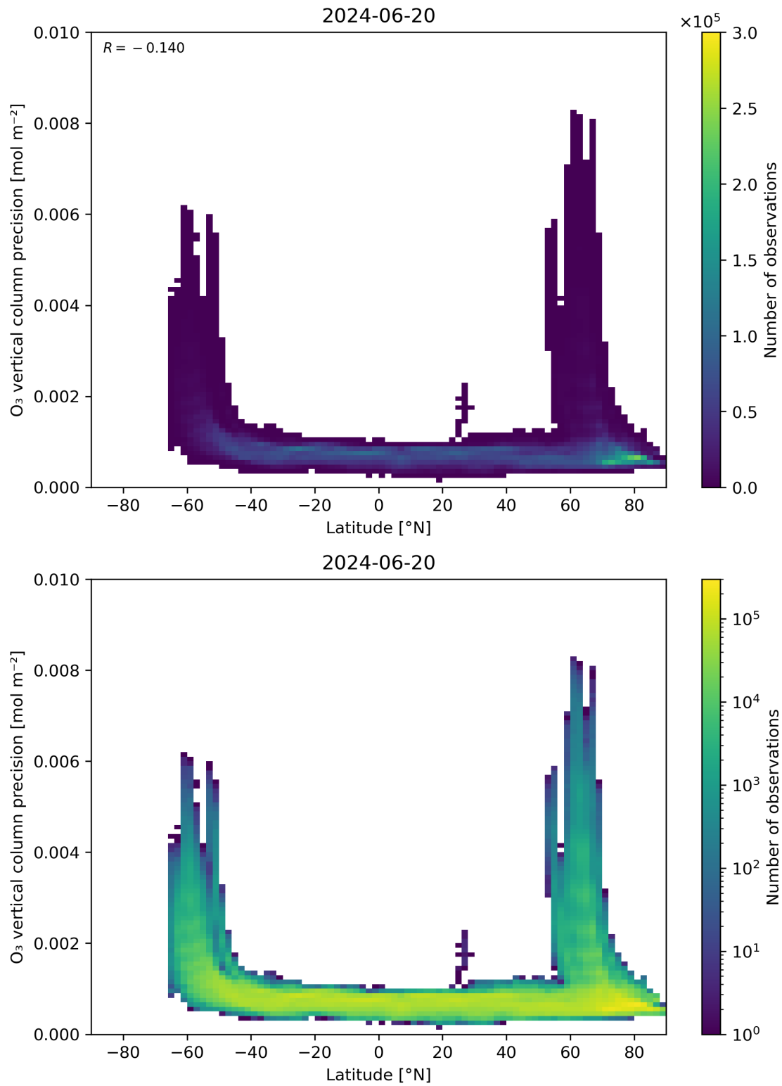
Figure 37: Scatter density plot of “Latitude” against “O 3 vertical column precision” for 2024-06-19 to 2024-06-21.
