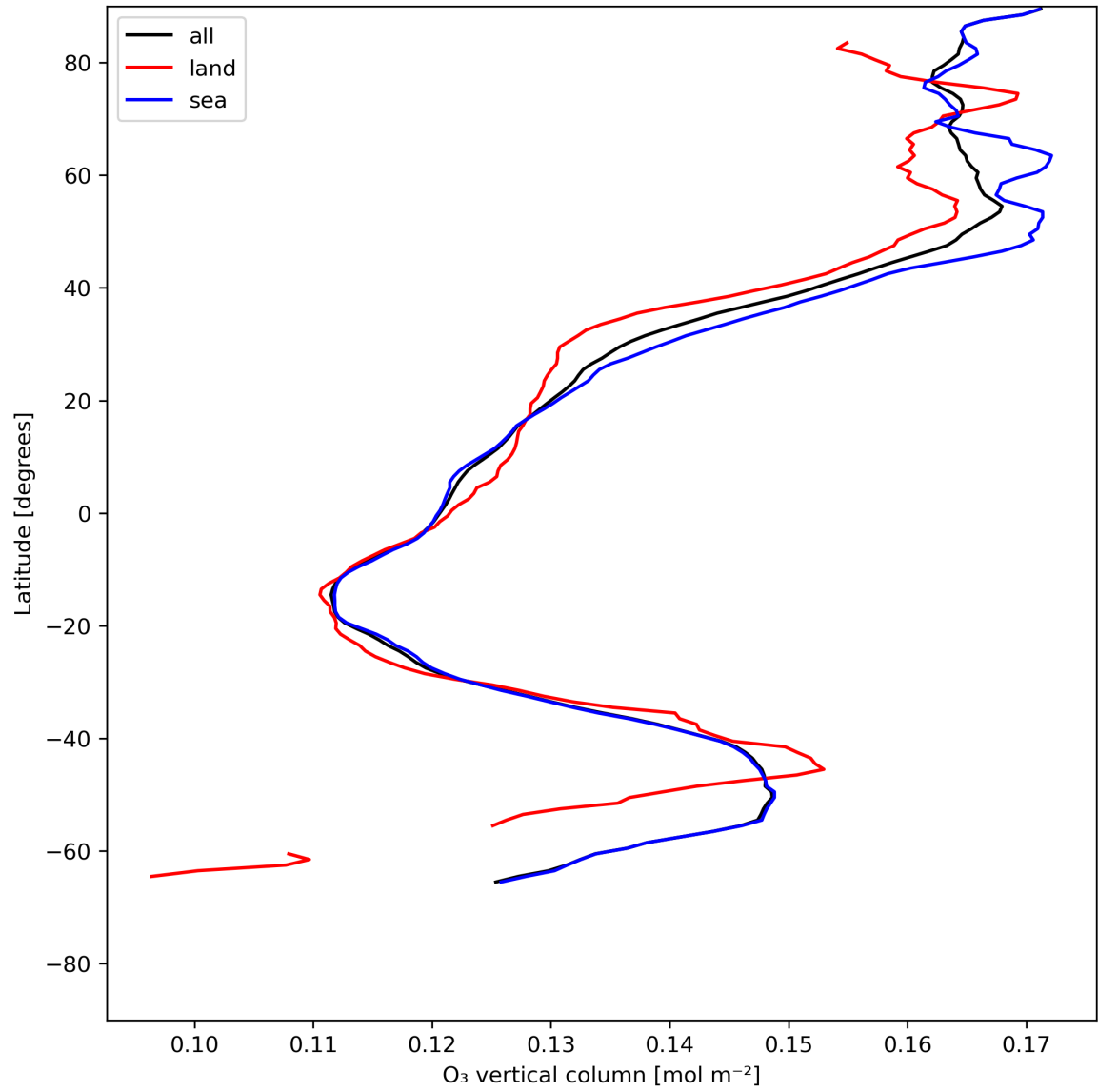
Figure 14: Zonal average of “O 3 vertical column” for 2024-06-19 to 2024-06-21.
