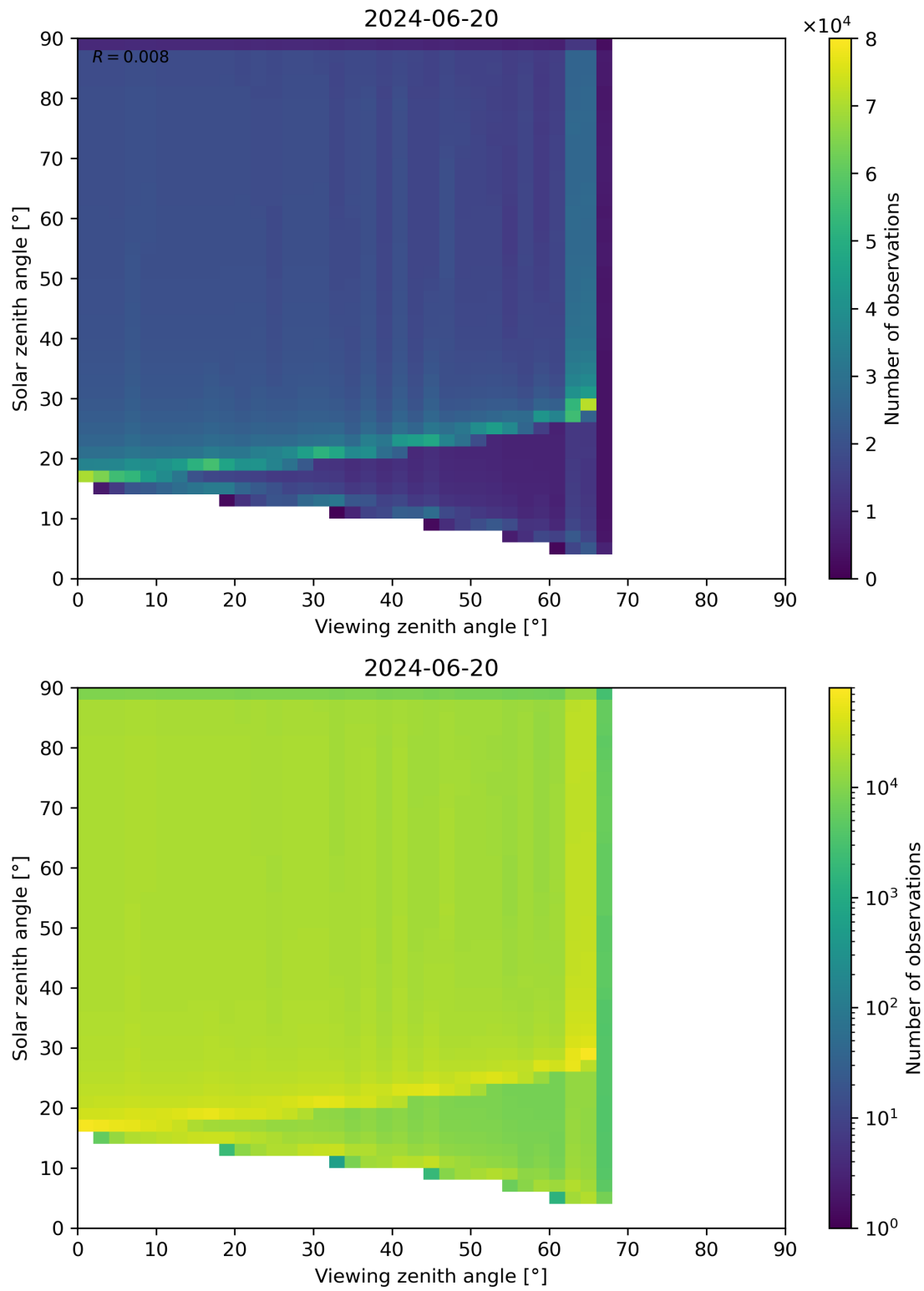
Figure 54: Scatter density plot of “Viewing zenith angle” against “Solar zenith angle” for 2024-06-19 to 2024-06-21.
