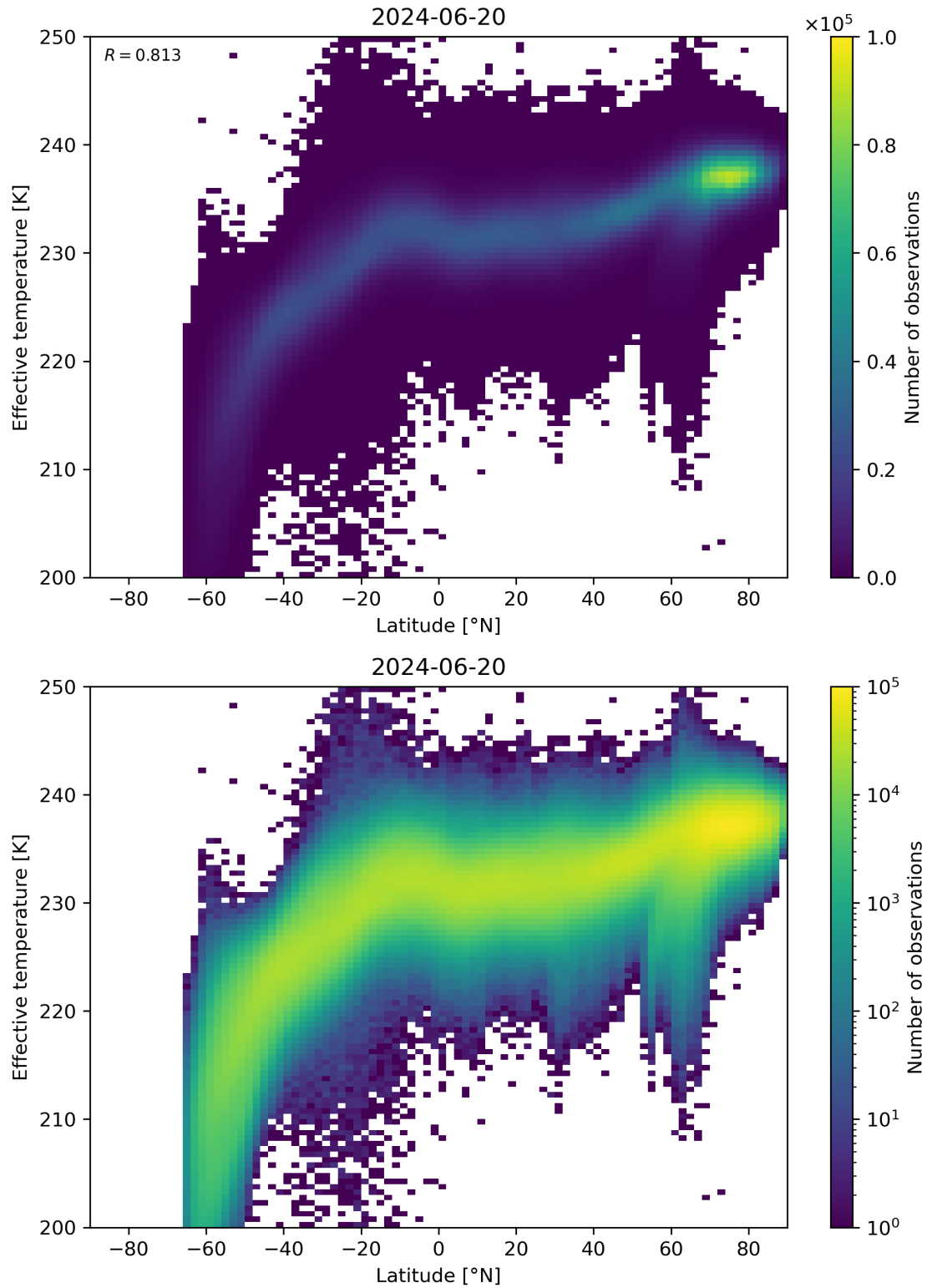
Figure 34: Scatter density plot of “Latitude” against “Effective temperature” for 2024-06-19 to 2024-06-21.
