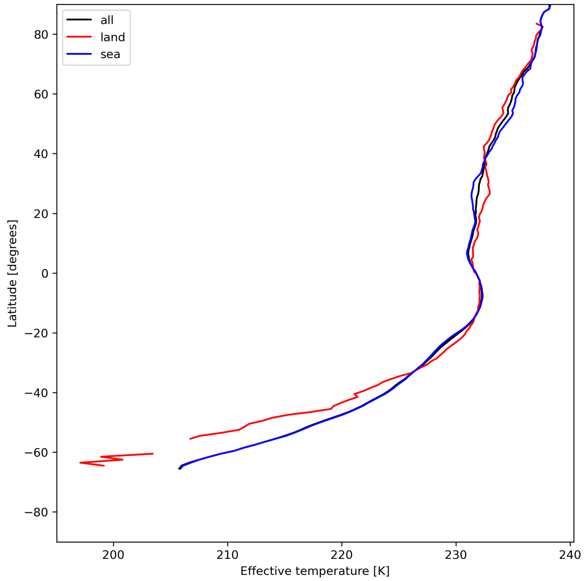
Figure 17: Zonal average of "Effective temperature" for 2024-06-19 to 2024-06-21.
