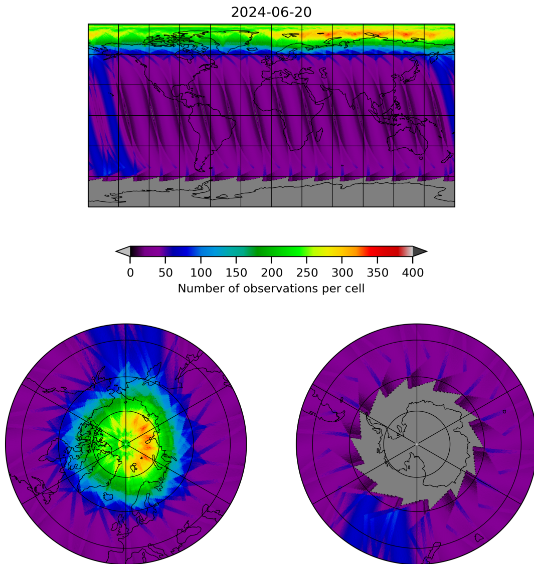
Figure 12: Map of the number of observations for 2024-06-19 to 2024-06-21
