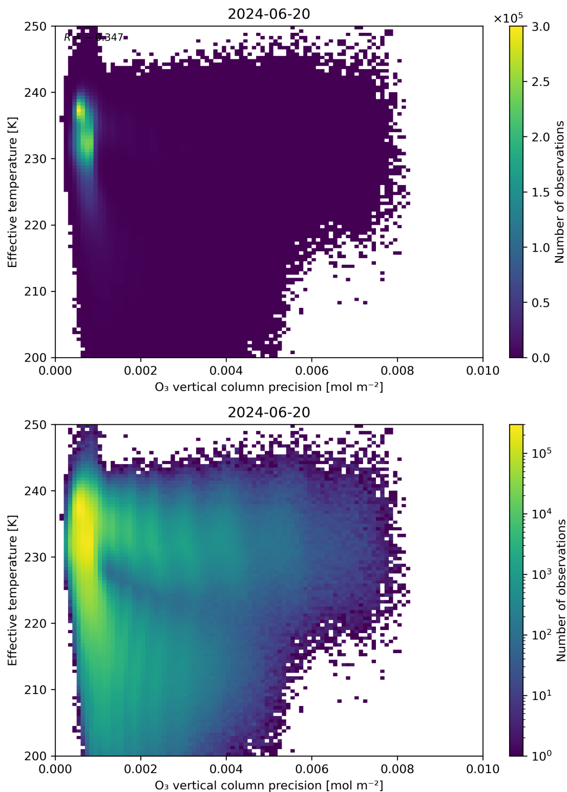
Figure 42: Scatter density plot of “O 3 vertical column precision” against “Effective temperature” for 2024-06-19 to 2024-06-21.
