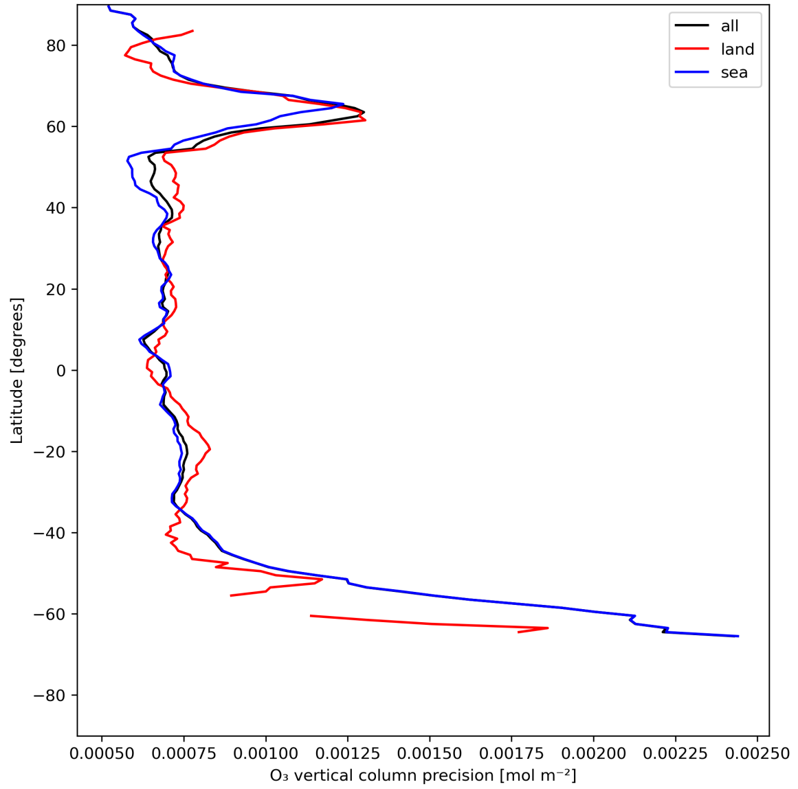
Figure 15: Zonal average of “O 3 vertical column precision” for 2024-06-19 to 2024-06-21.
