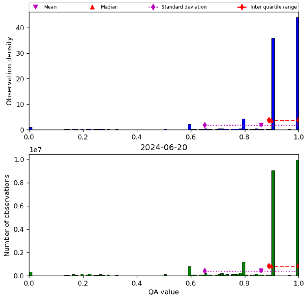
Figure 20: Histogram of “QA value” for 2024-06-19 to 2024-06-21
