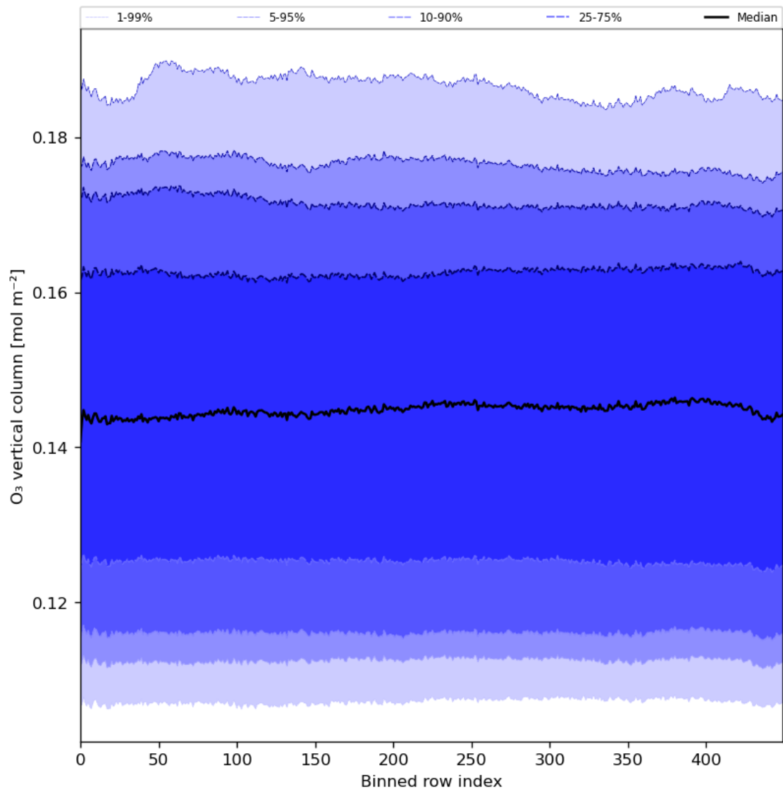
Figure 28: Along track statistics of “O 3 vertical column” for 2024-06-19 to 2024-06-21
