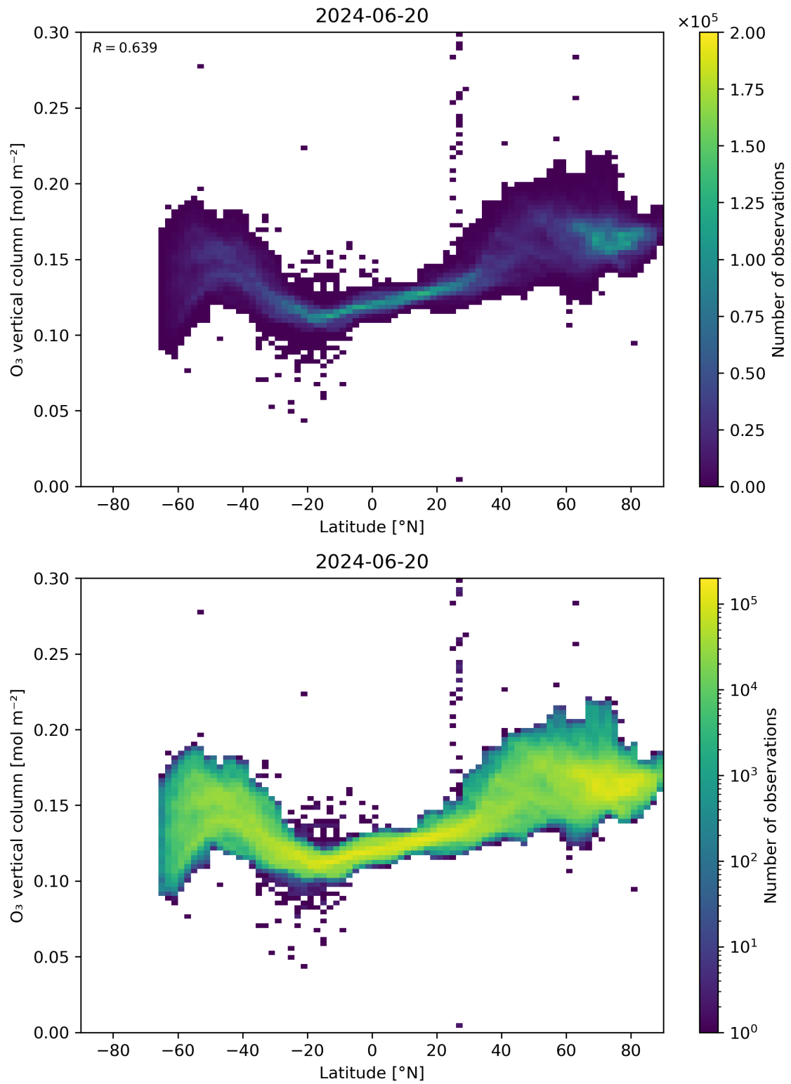
Figure 36: Scatter density plot of “Latitude” against “O 3 vertical column” for 2024-06-19 to 2024-06-21.
