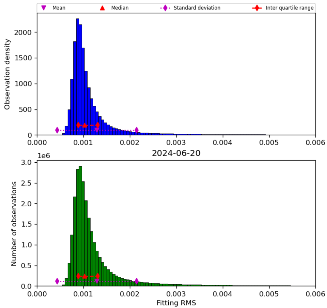
Figure 23: Histogram of “Fitting RMS” for 2024-06-19 to 2024-06-21
