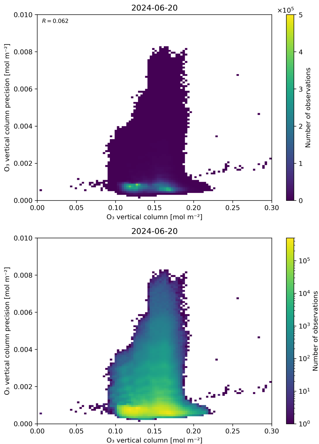
Figure 41: Scatter density plot of “O 3 vertical column” against “O 3 vertical column precision” for 2024-06-19 to 2024-06-21.
