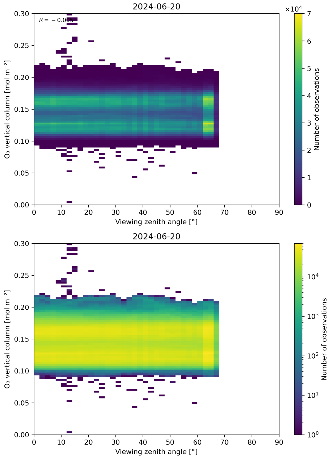
Figure 52: Scatter density plot of “Viewing zenith angle” against “O 3 vertical column” for 2024-06-19 to 2024-06-21.
