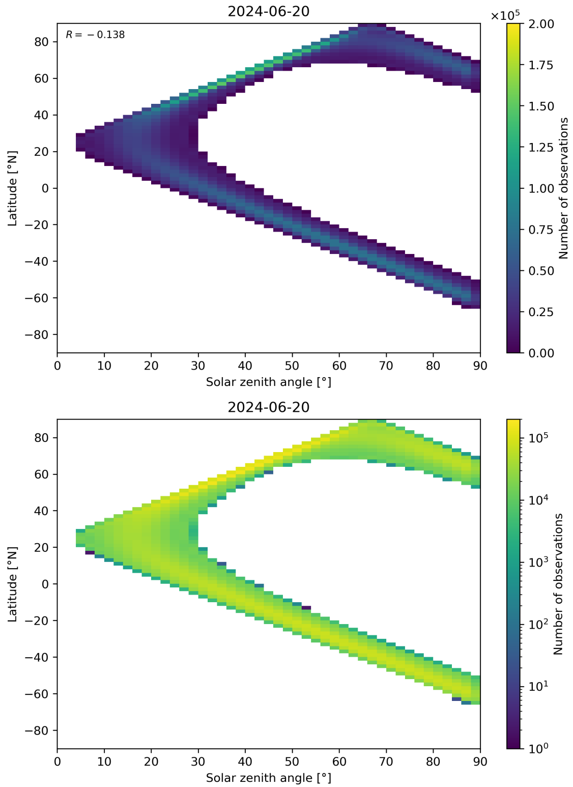
Figure 44: Scatter density plot of “Solar zenith angle” against “Latitude” for 2024-06-19 to 2024-06-21.
