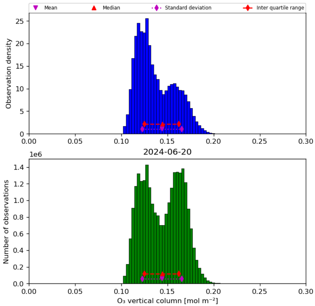
Figure 21: Histogram of “O 3 vertical column” for 2024-06-19 to 2024-06-21
