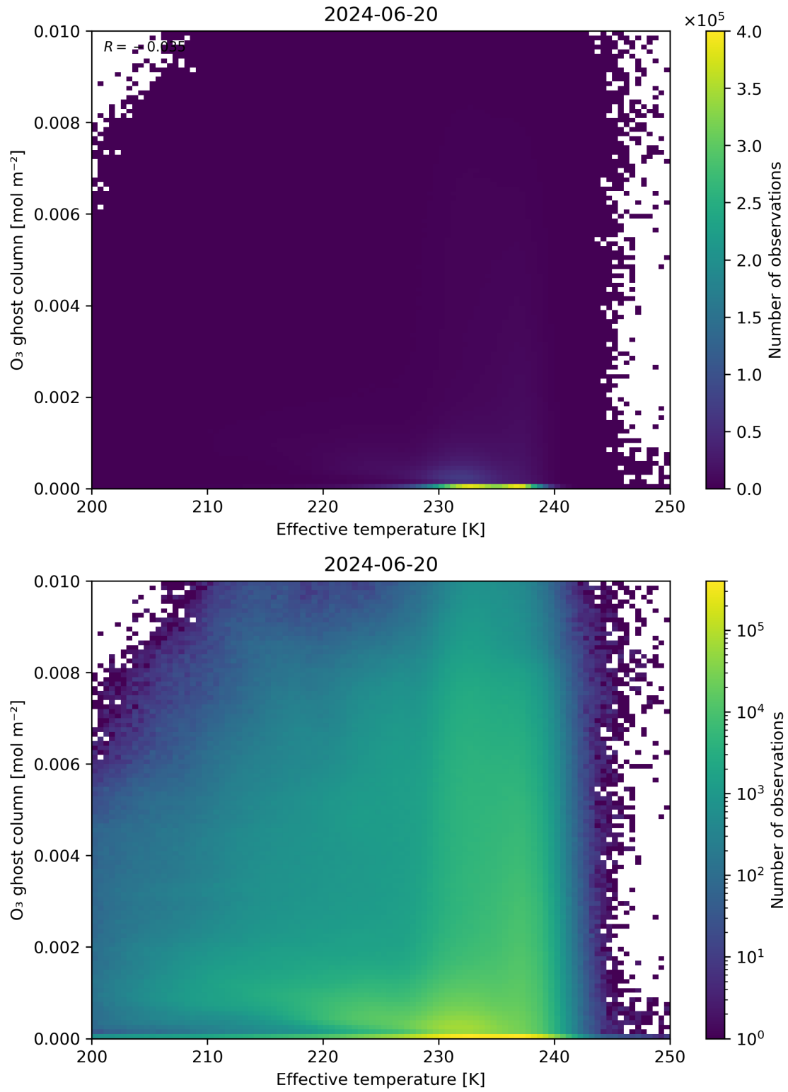
Figure 38: Scatter density plot of “Effective temperature” against “O 3 ghost column” for 2024-06-19 to 2024-06-21.
