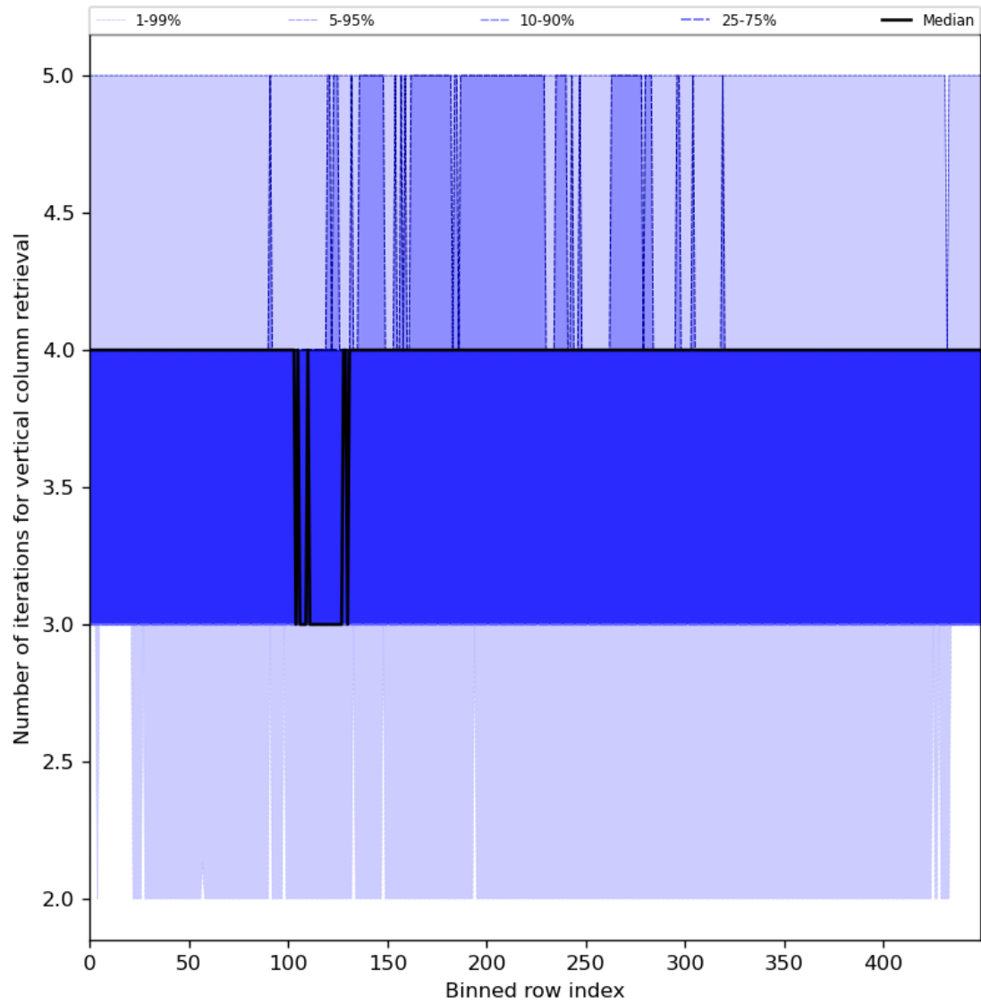
Figure 33: Along track statistics of “Number of iterations for vertical column retrieval” for 2024-06-19 to 2024-06-21
