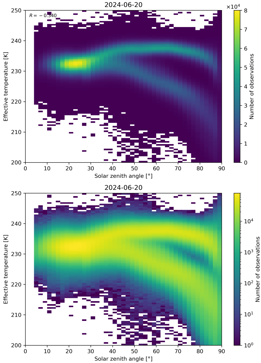
Figure 45: Scatter density plot of “Solar zenith angle” against “Effective temperature” for 2024-06-19 to 2024-06-21.
