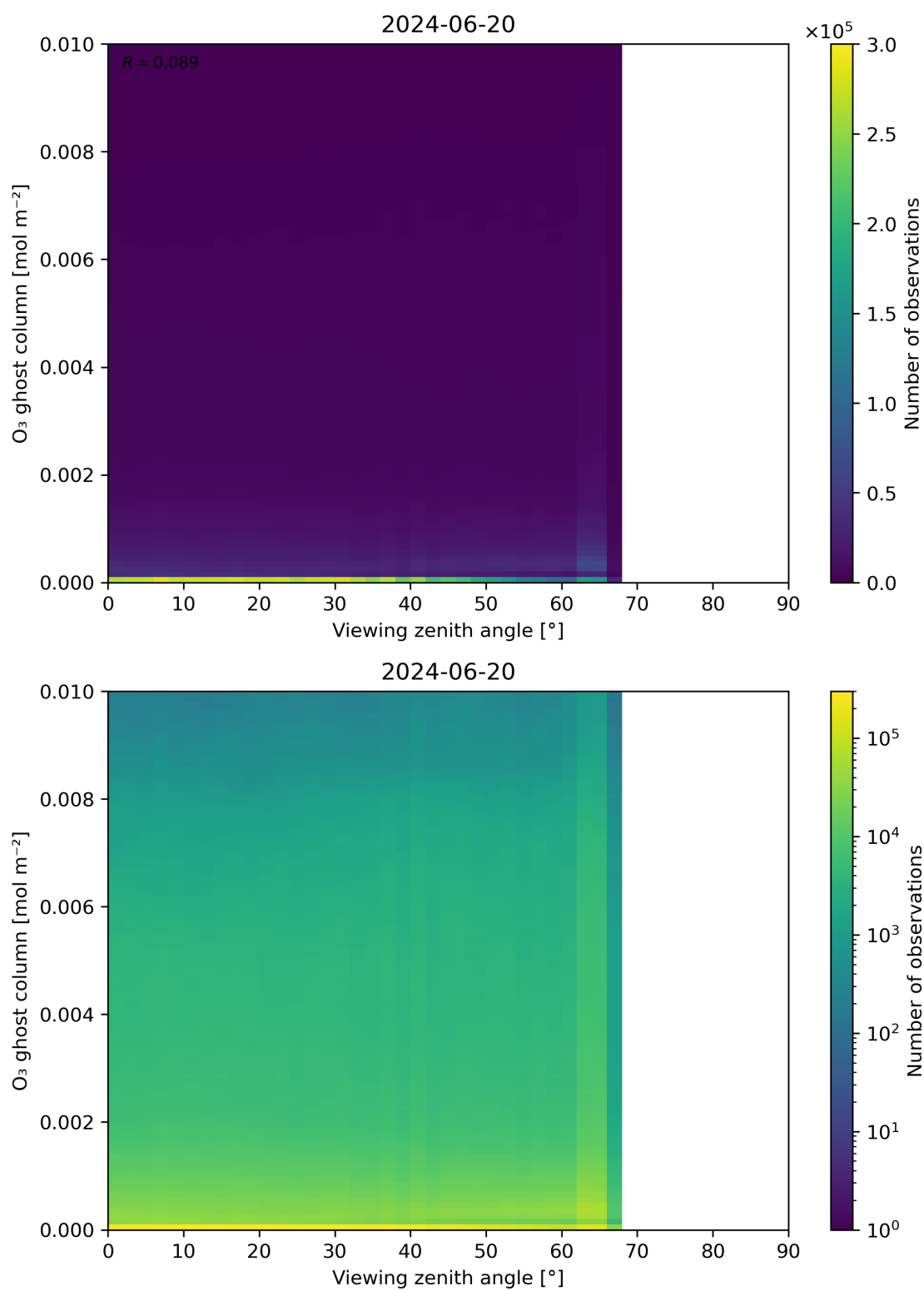
Figure 51: Scatter density plot of “Viewing zenith angle” against “O 3 ghost column” for 2024-06-19 to 2024-06-21.
