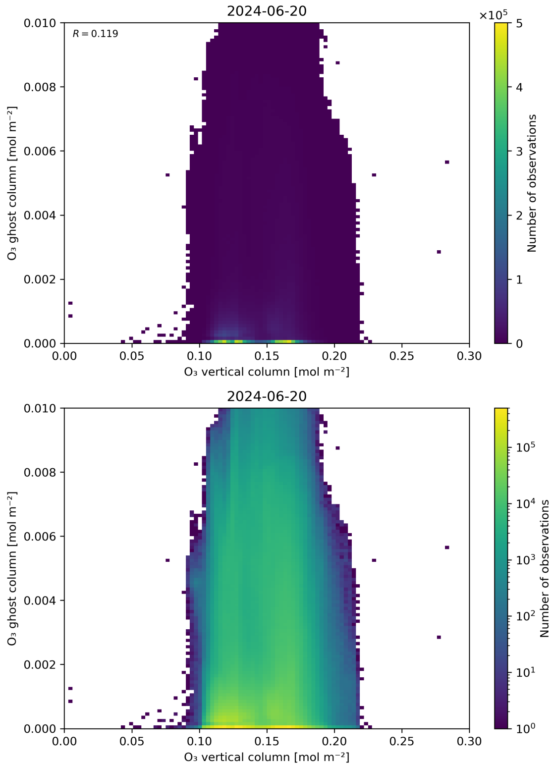
Figure 40: Scatter density plot of “O 3 vertical column” against “O 3 ghost column” for 2024-06-19 to 2024-06-21.
