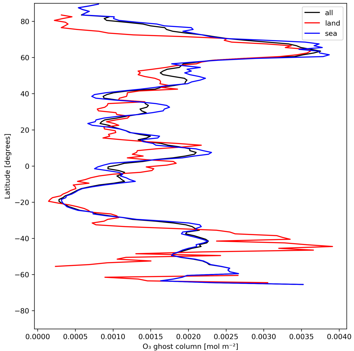
Figure 18: Zonal average of "O 3 ghost column" for 2024-06-19 to 2024-06-21.
