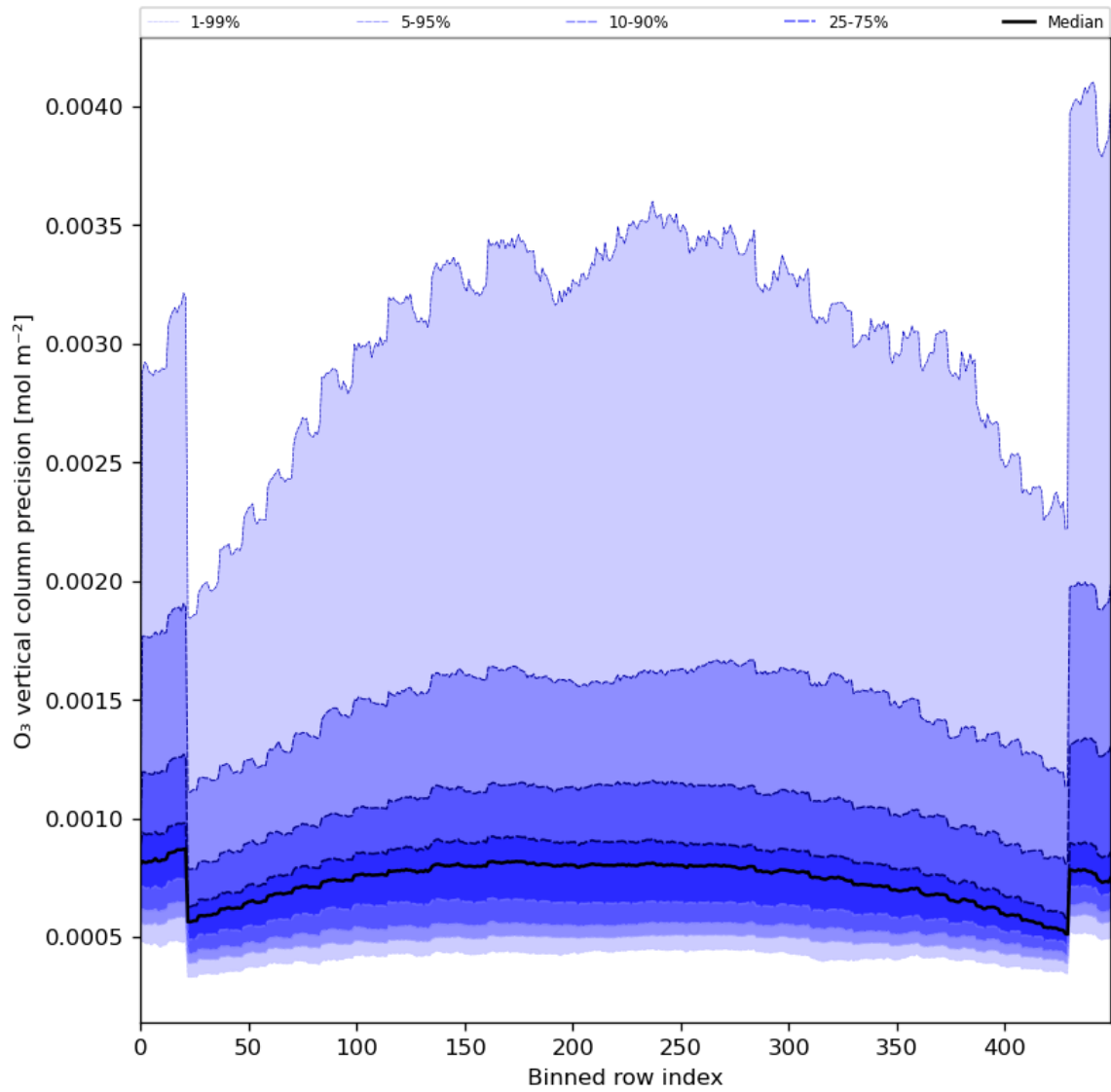
Figure 29: Along track statistics of “O 3 vertical column precision” for 2024-06-19 to 2024-06-21
