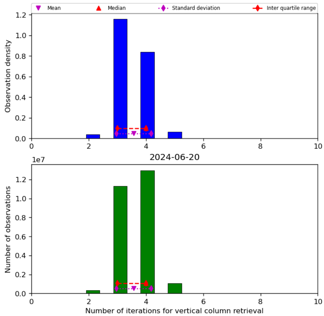
Figure 26: Histogram of “Number of iterations for vertical column retrieval” for 2024-06-19 to 2024-06-21
