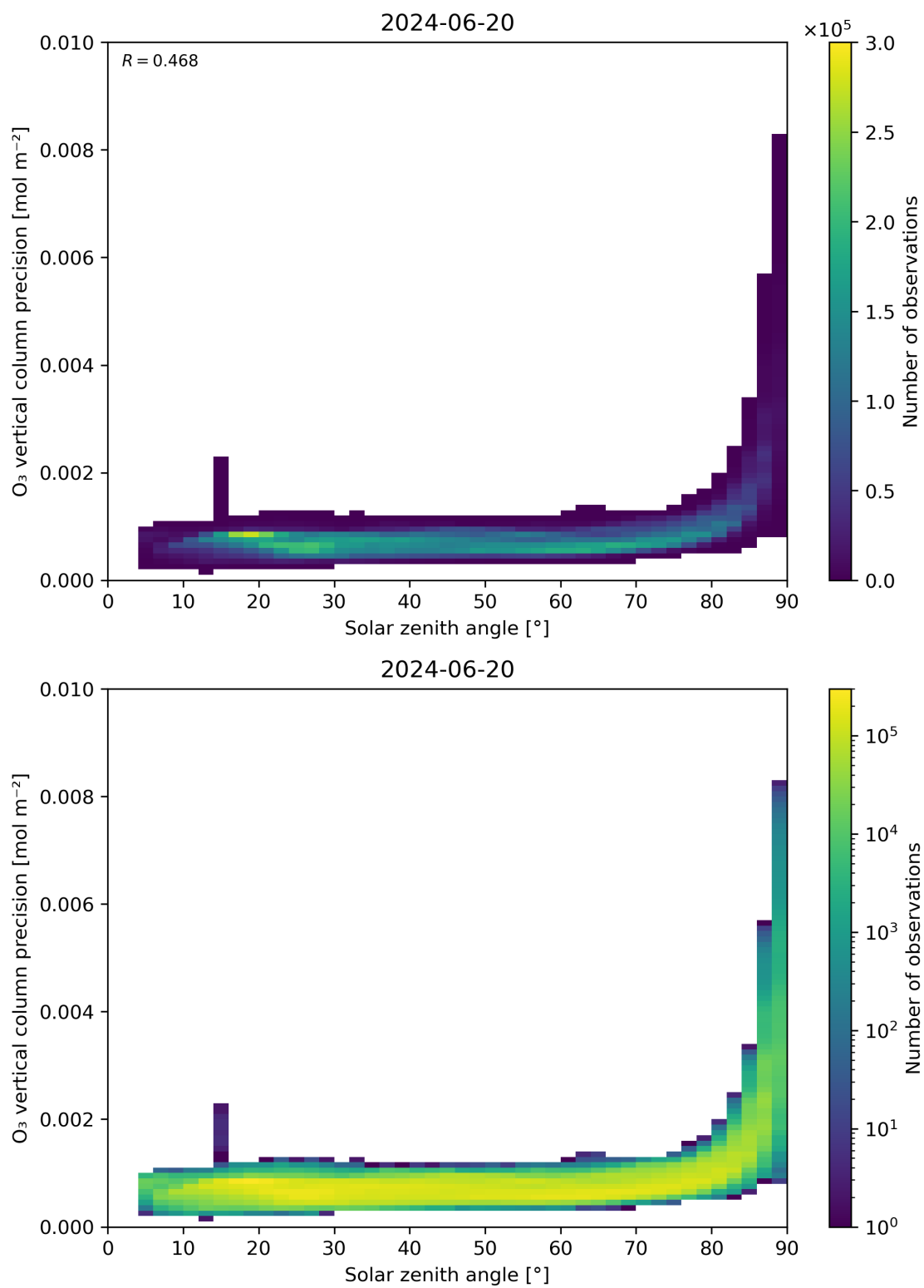
Figure 48: Scatter density plot of “Solar zenith angle” against “O 3 vertical column precision” for 2024-06-19 to 2024-06-21.
