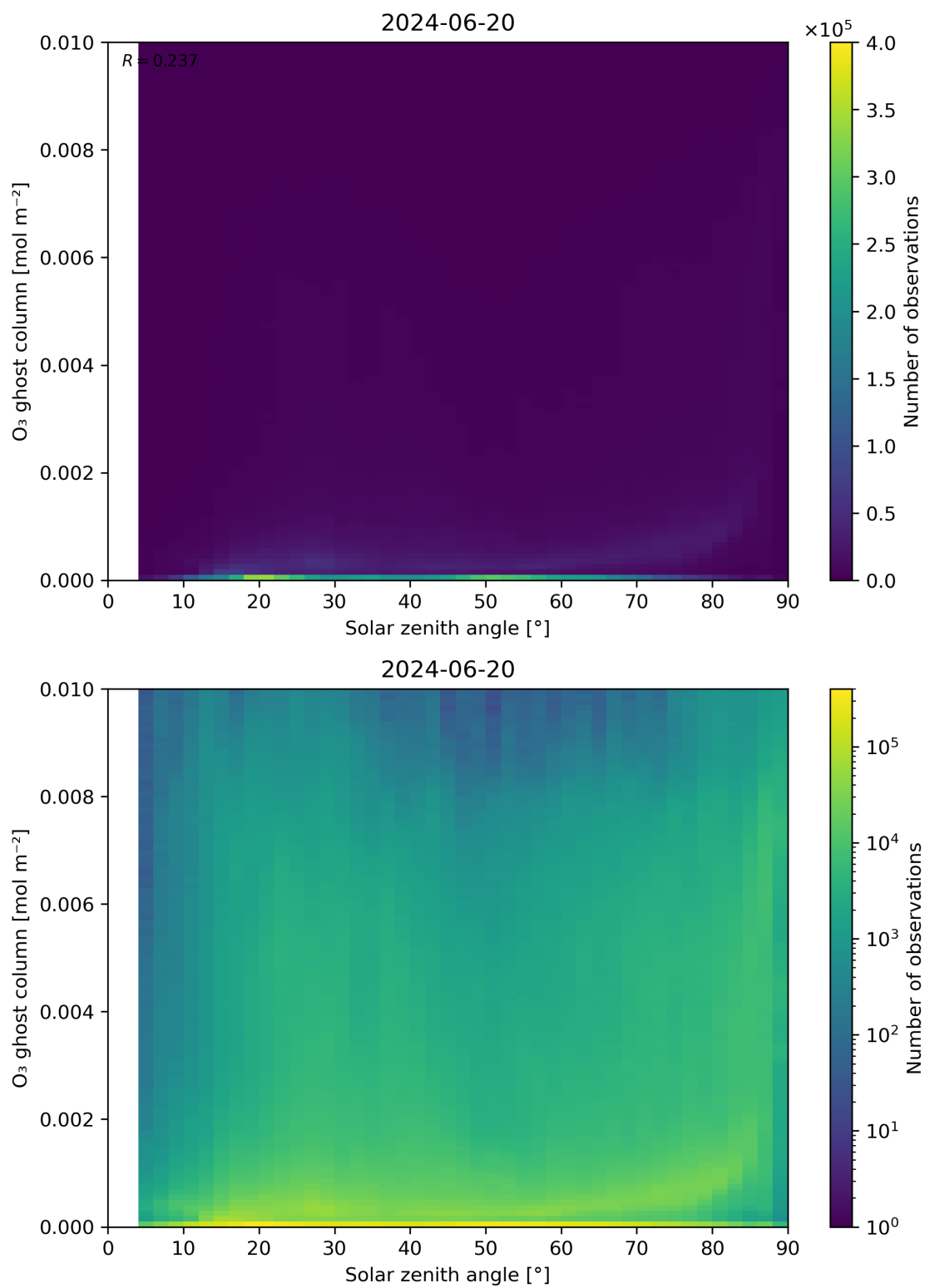
Figure 46: Scatter density plot of “Solar zenith angle” against “O 3 ghost column” for 2024-06-19 to 2024-06-21.
