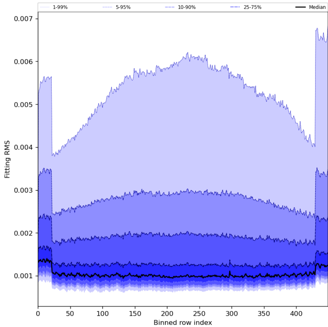
Figure 30: Along track statistics of “Fitting RMS” for 2024-06-19 to 2024-06-21
