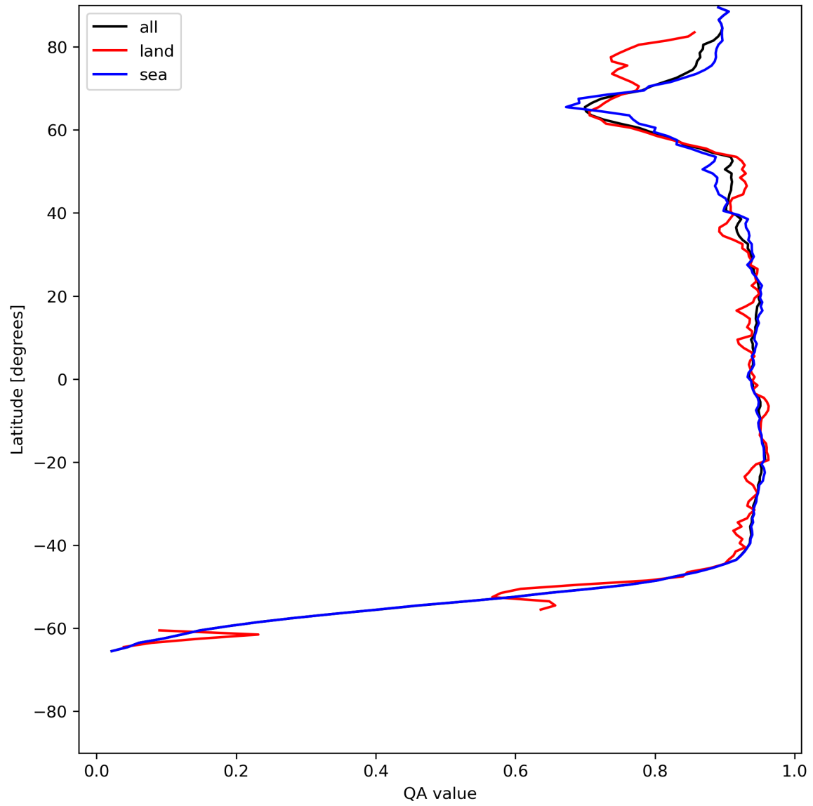
Figure 13: Zonal average of “QA value” for 2024-06-19 to 2024-06-21.
