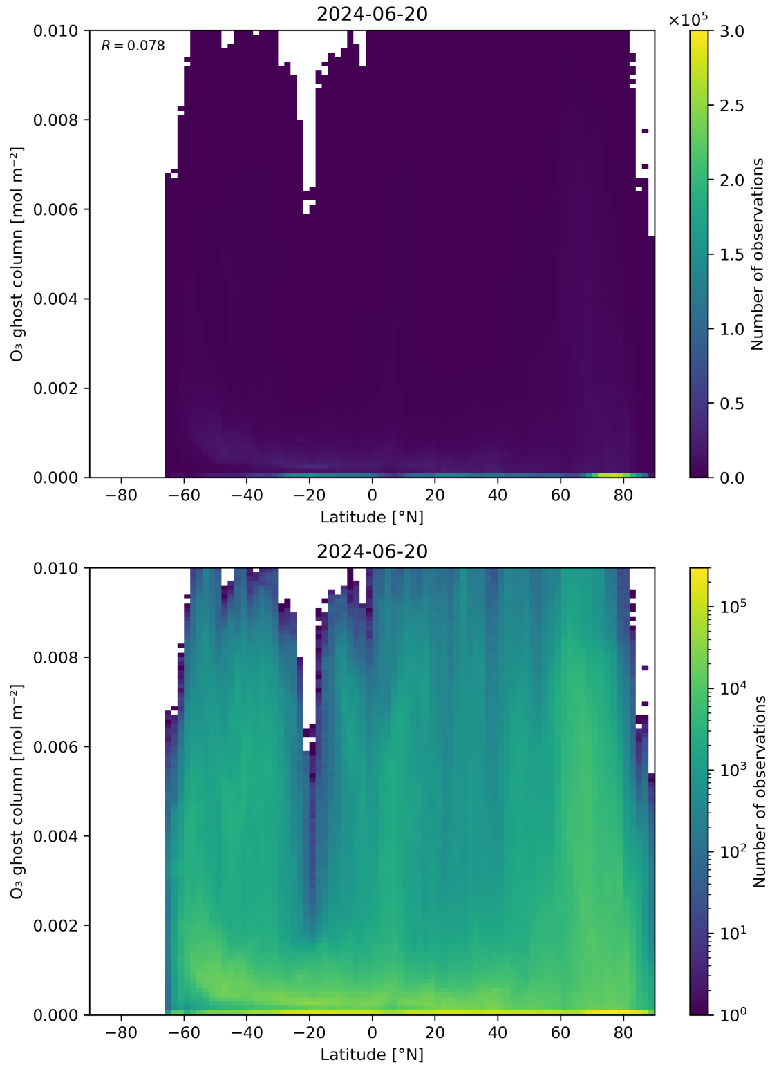
Figure 35: Scatter density plot of “Latitude” against “O 3 ghost column” for 2024-06-19 to 2024-06-21.
