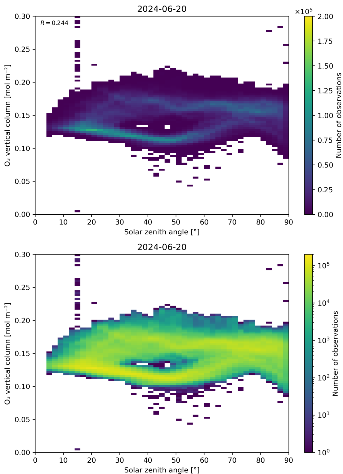
Figure 47: Scatter density plot of “Solar zenith angle” against “O 3 vertical column” for 2024-06-19 to 2024-06-21.
