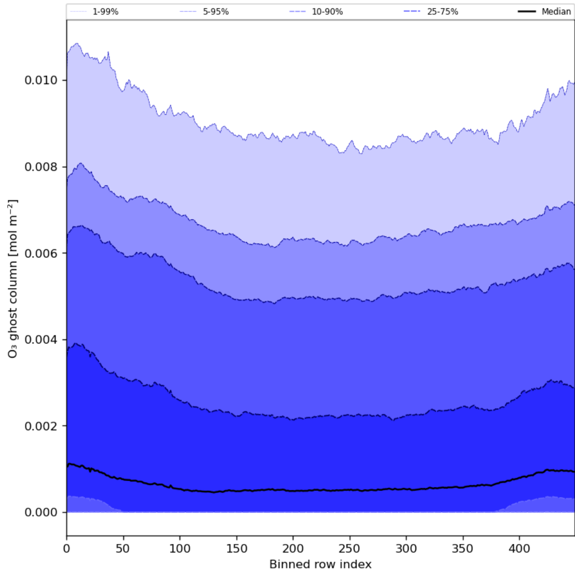
Figure 32: Along track statistics of “O 3 ghost column” for 2024-06-19 to 2024-06-21
