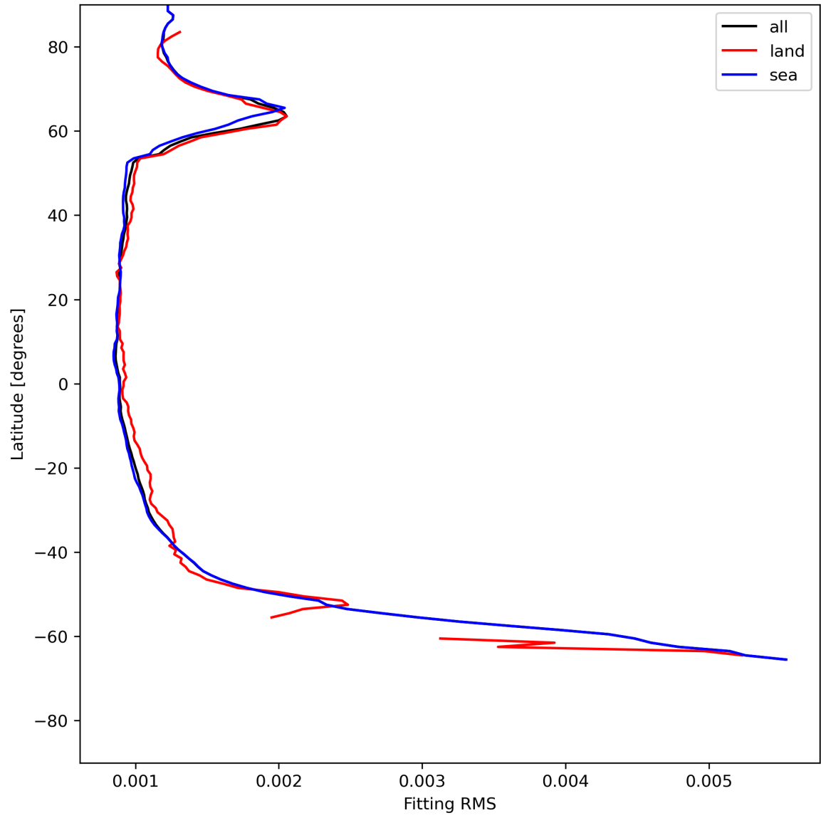
Figure 16: Zonal average of “Fitting RMS” for 2024-06-19 to 2024-06-21.
