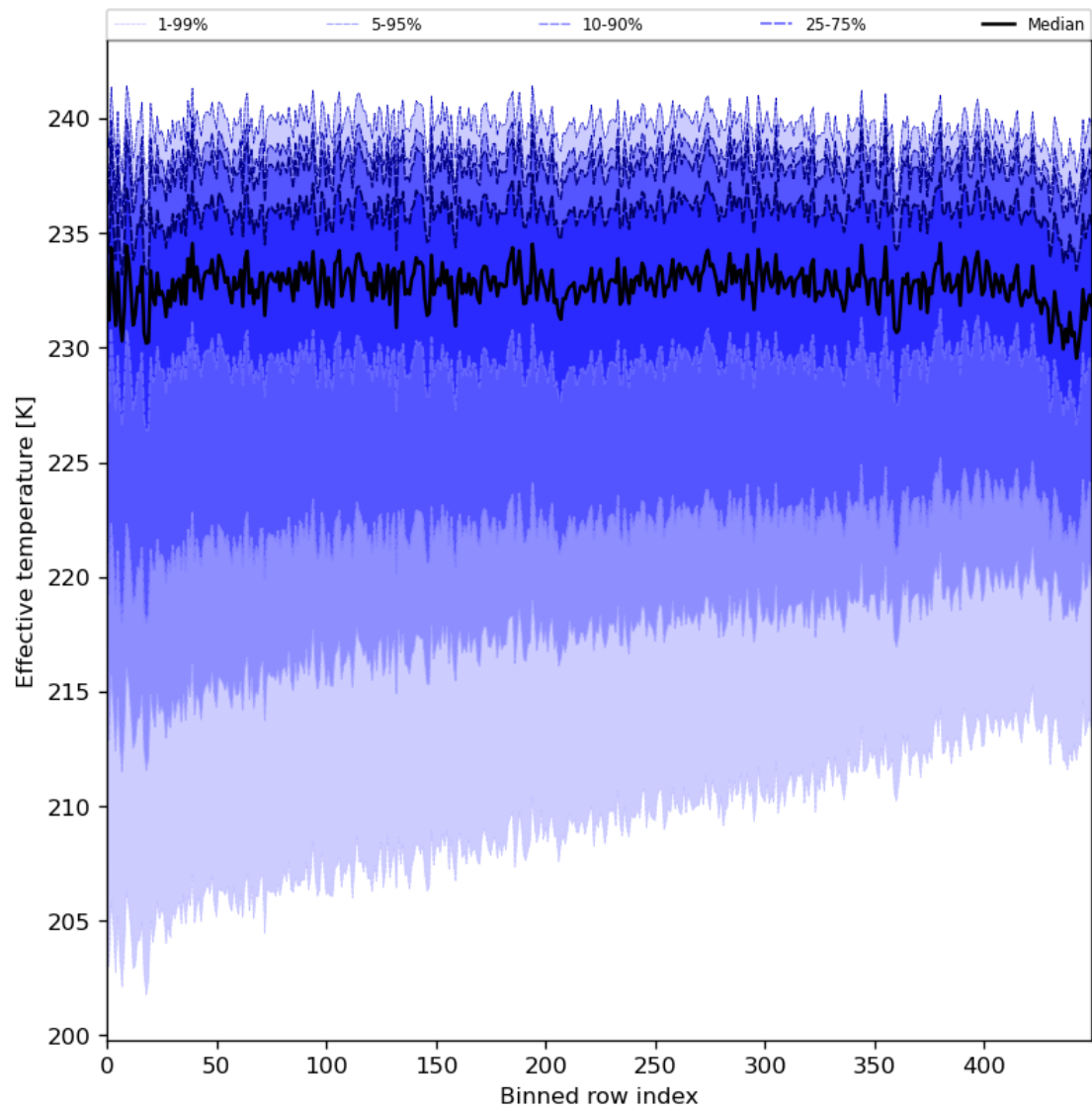
Figure 31: Along track statistics of “Effective temperature” for 2024-06-20 to 2024-06-22
