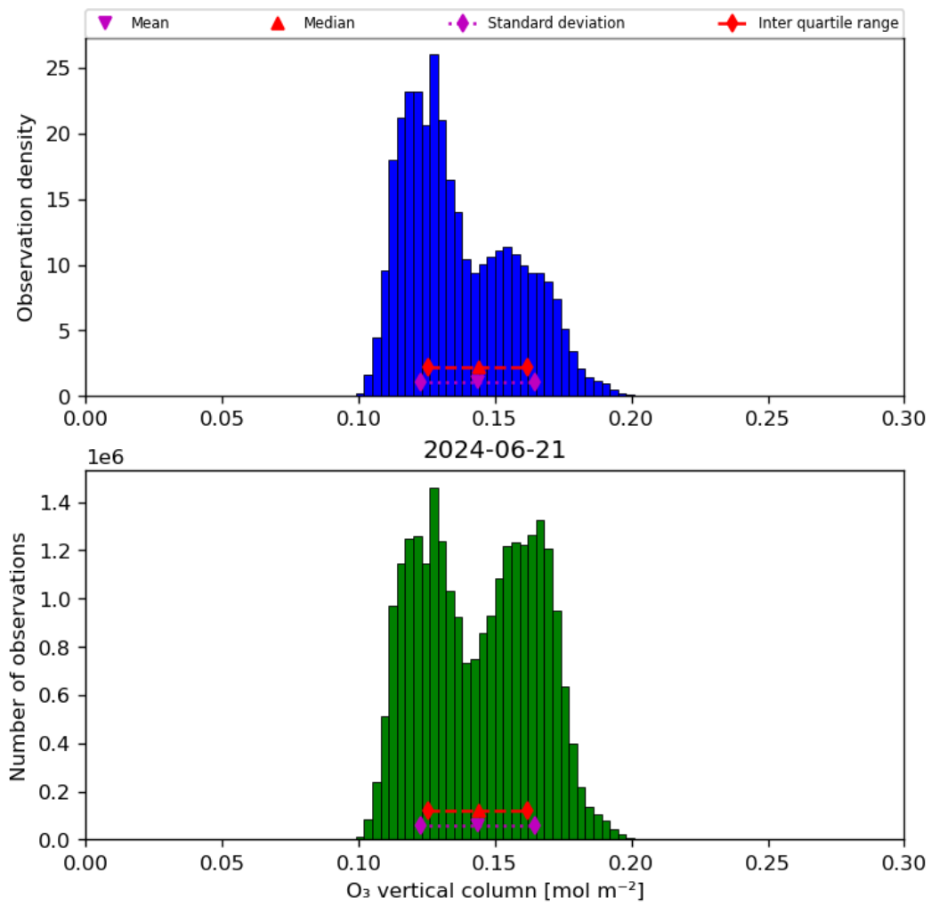
Figure 21: Histogram of “O 3 vertical column” for 2024-06-20 to 2024-06-22
