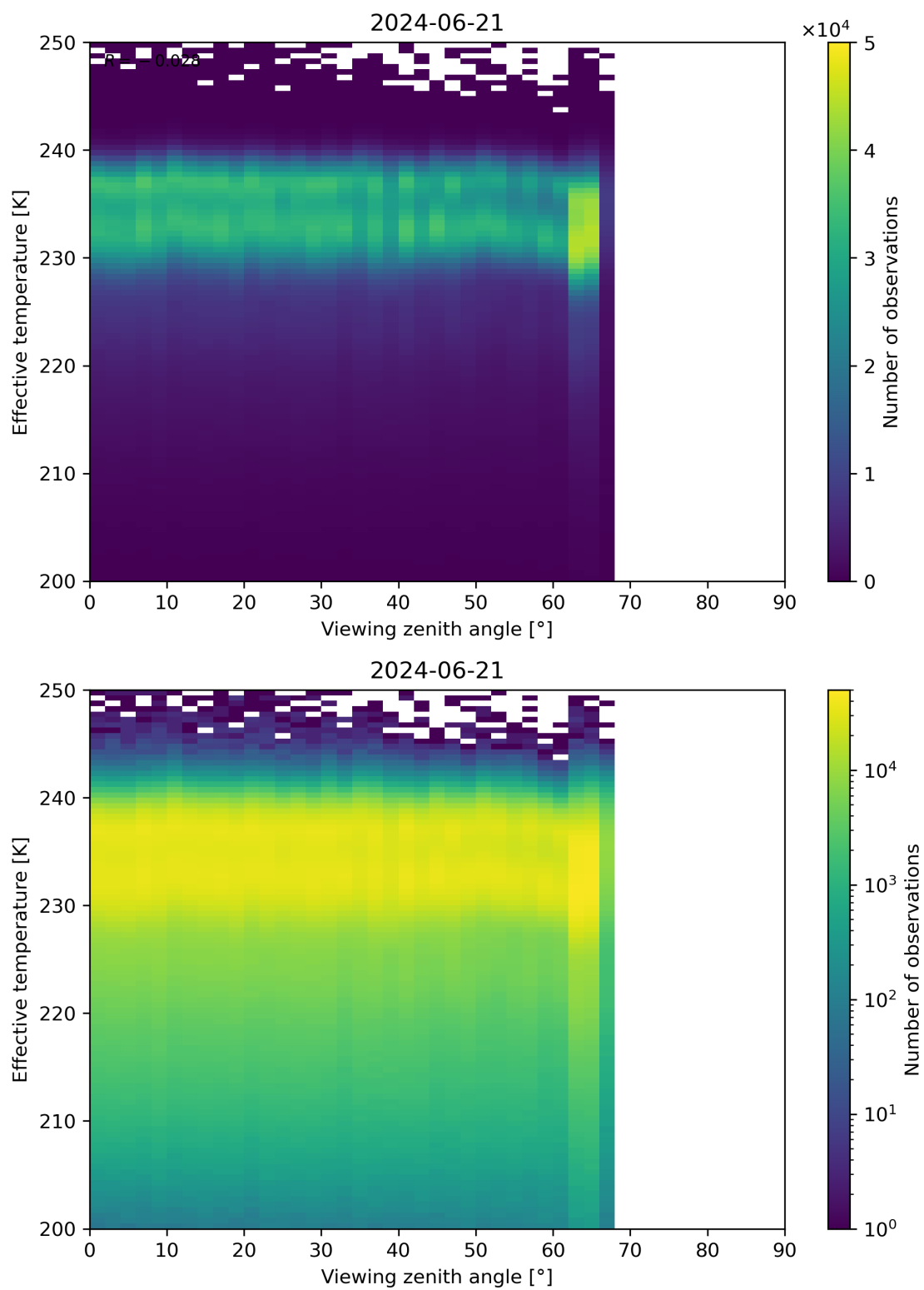
Figure 50: Scatter density plot of “Viewing zenith angle” against “Effective temperature” for 2024-06-20 to 2024-06-22.
