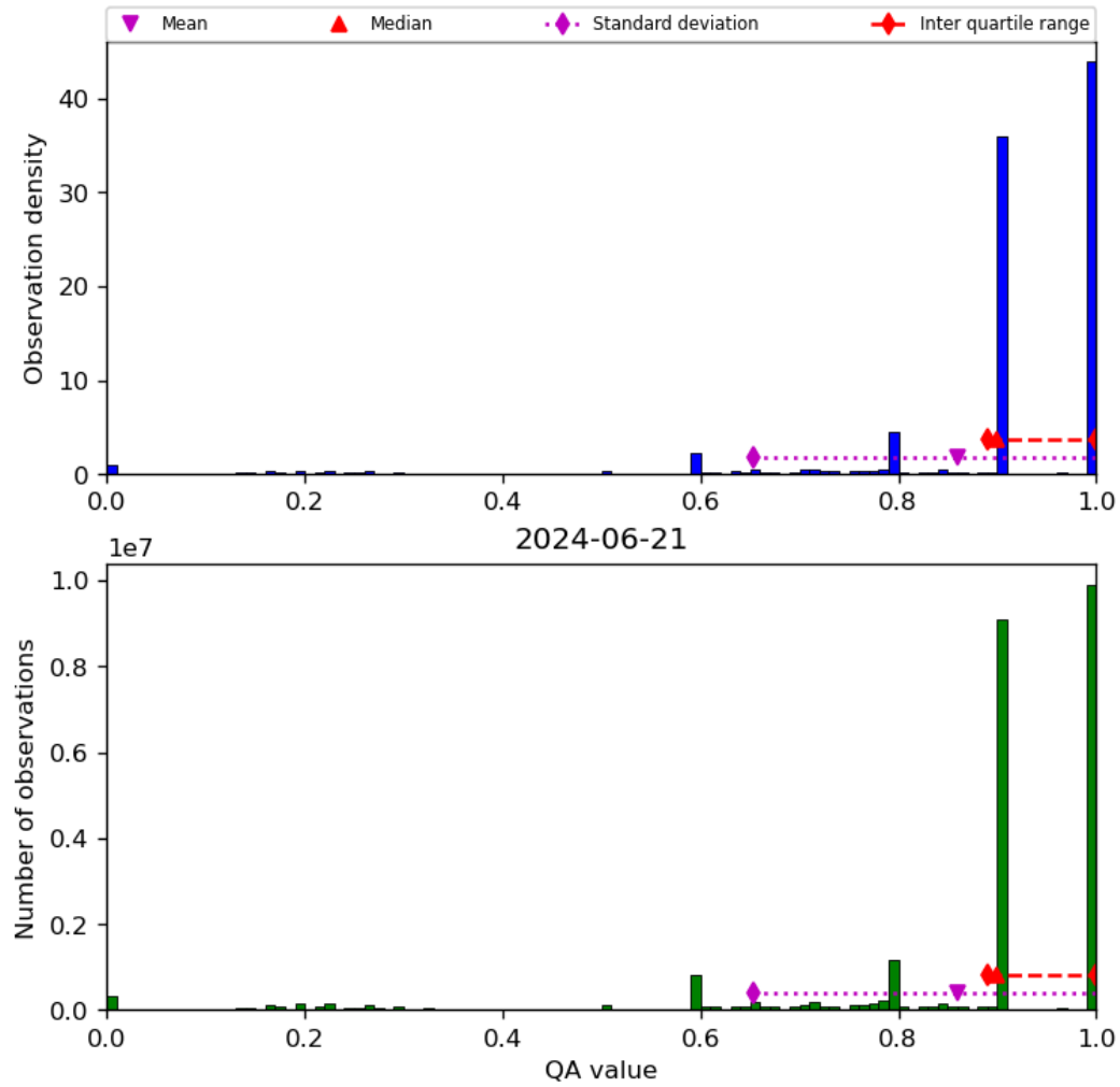
Figure 20: Histogram of “QA value” for 2024-06-20 to 2024-06-22
