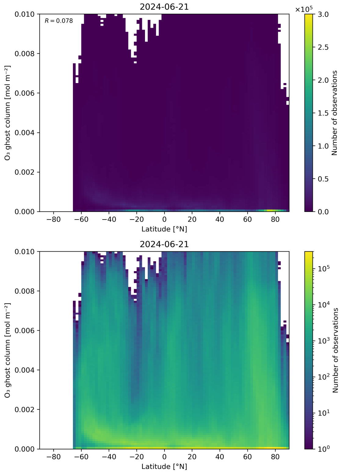
Figure 35: Scatter density plot of “Latitude” against “O 3 ghost column” for 2024-06-20 to 2024-06-22.
