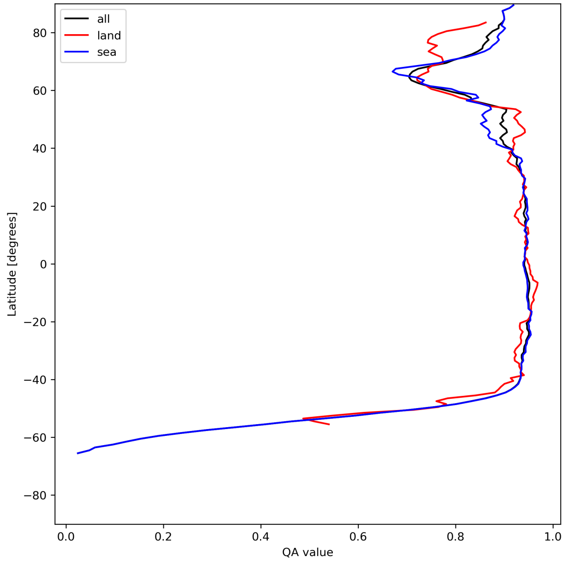
Figure 13: Zonal average of “QA value” for 2024-06-20 to 2024-06-22.
