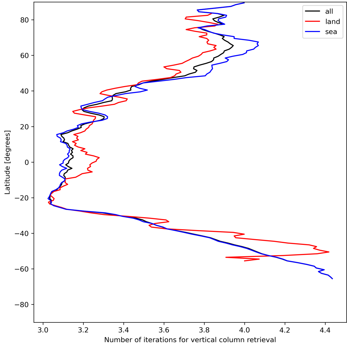
Figure 19: Zonal average of “Number of iterations for vertical column retrieval” for 2024-06-20 to 2024-06-22.
