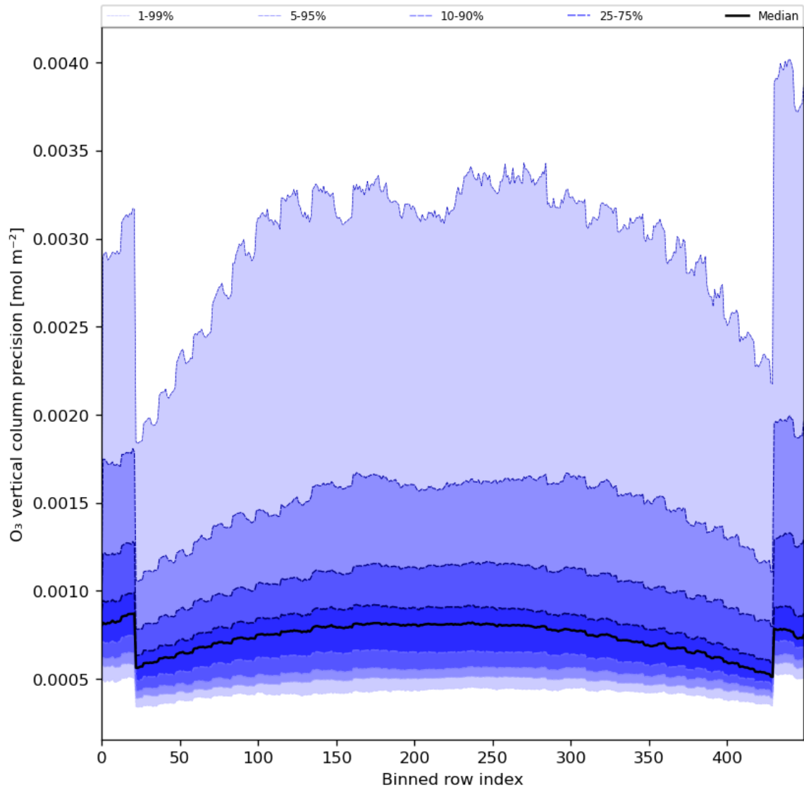
Figure 29: Along track statistics of “O 3 vertical column precision” for 2024-06-20 to 2024-06-22
