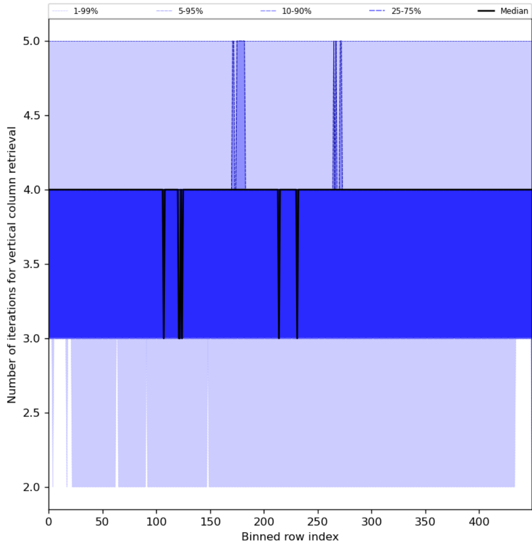
Figure 33: Along track statistics of “Number of iterations for vertical column retrieval” for 2024-06-20 to 2024-06-22
