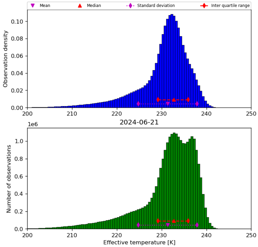
Figure 24: Histogram of “Effective temperature” for 2024-06-20 to 2024-06-22
