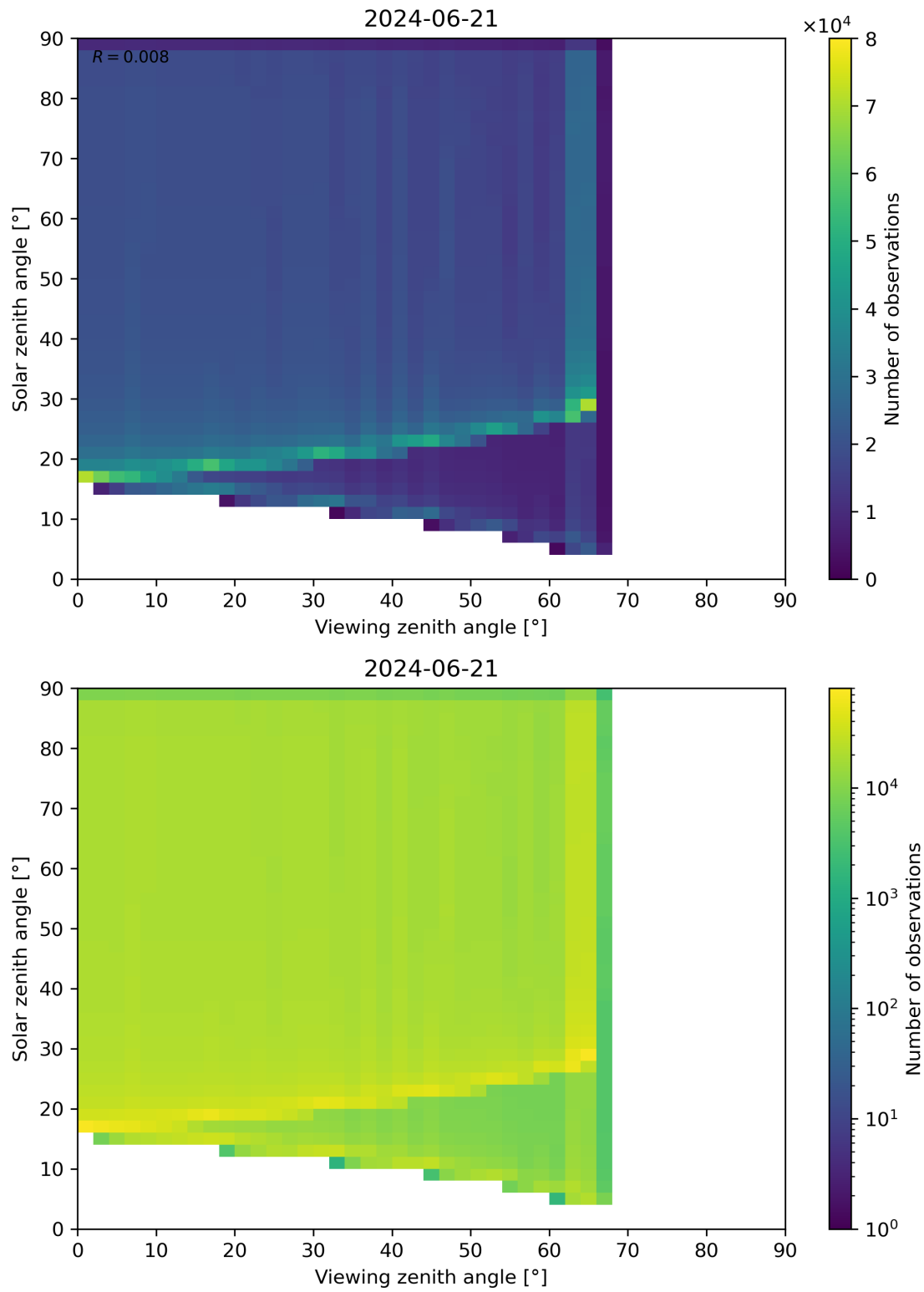
Figure 54: Scatter density plot of “Viewing zenith angle” against “Solar zenith angle” for 2024-06-20 to 2024-06-22.
