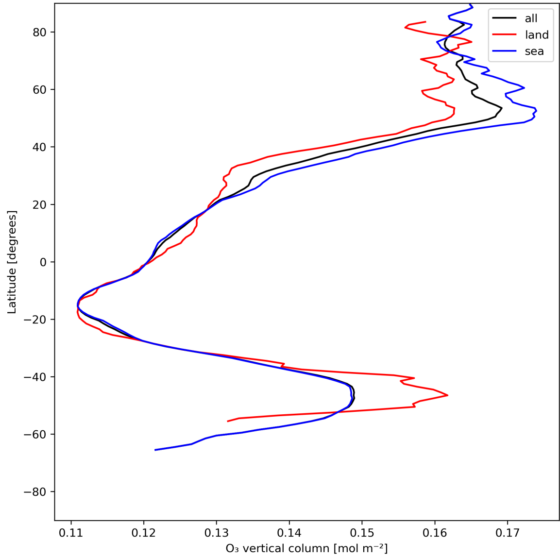
Figure 14: Zonal average of “O 3 vertical column” for 2024-06-20 to 2024-06-22.
