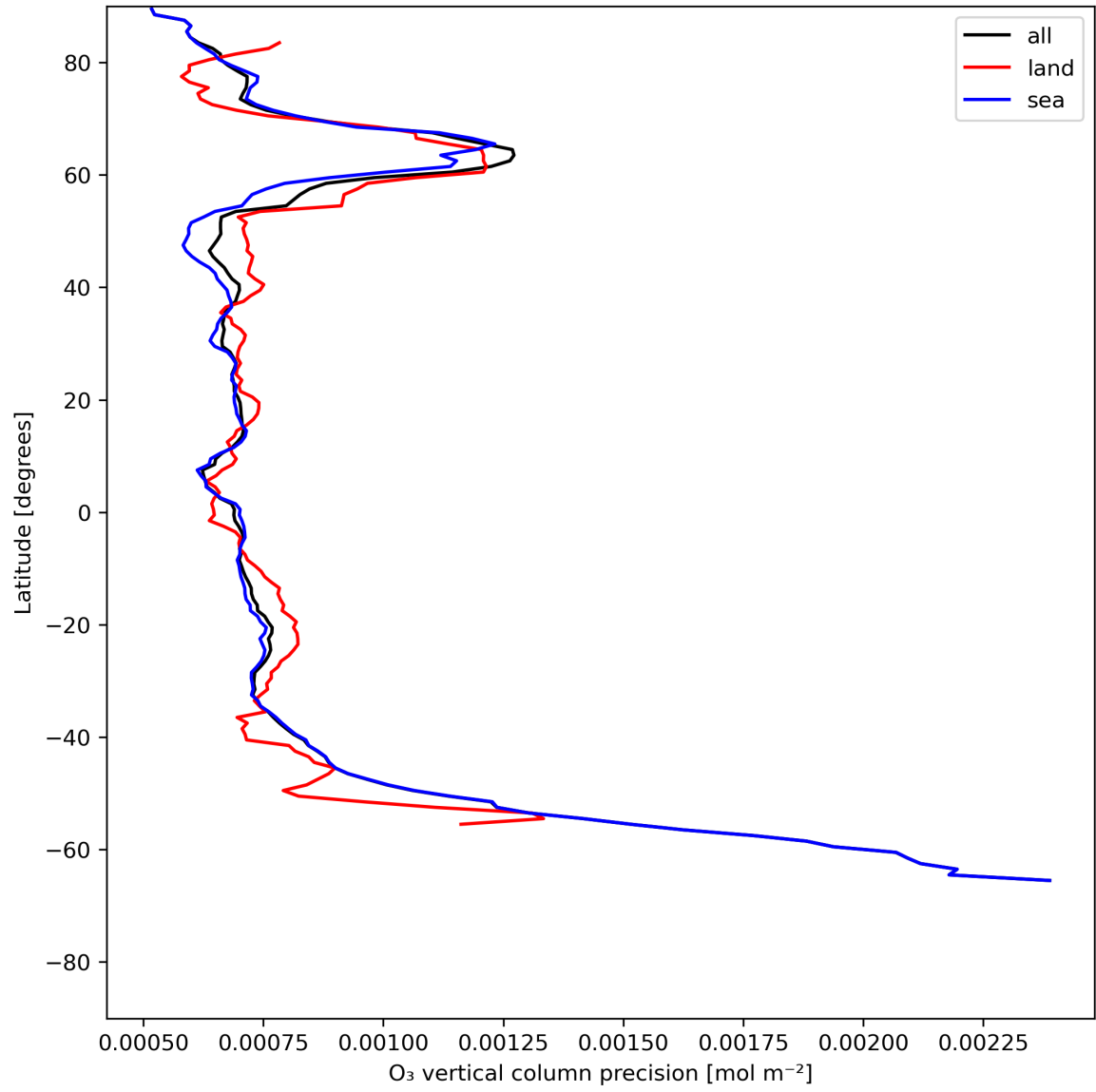
Figure 15: Zonal average of “O 3 vertical column precision” for 2024-06-20 to 2024-06-22.
