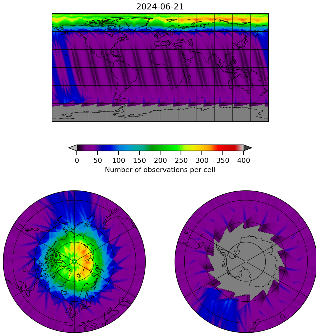
Figure 12: Map of the number of observations for 2024-06-20 to 2024-06-22
