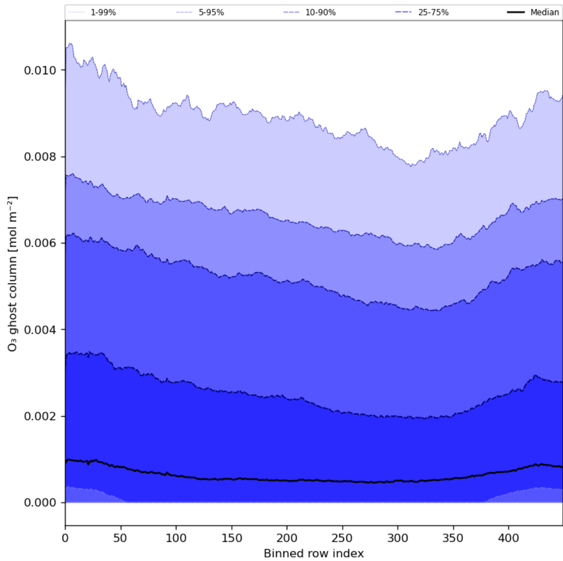
Figure 32: Along track statistics of “O 3 ghost column” for 2024-06-20 to 2024-06-22
