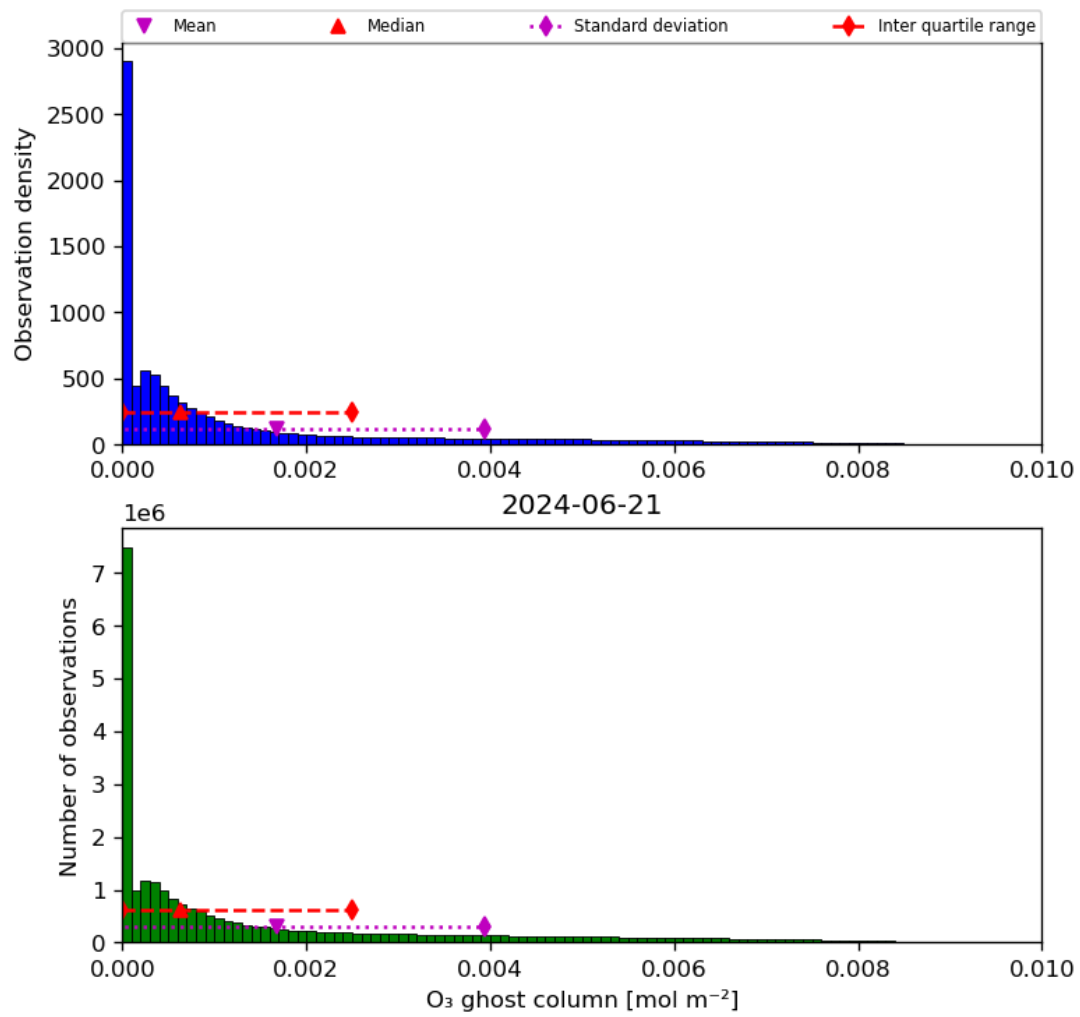
Figure 25: Histogram of “O 3 ghost column” for 2024-06-20 to 2024-06-22
