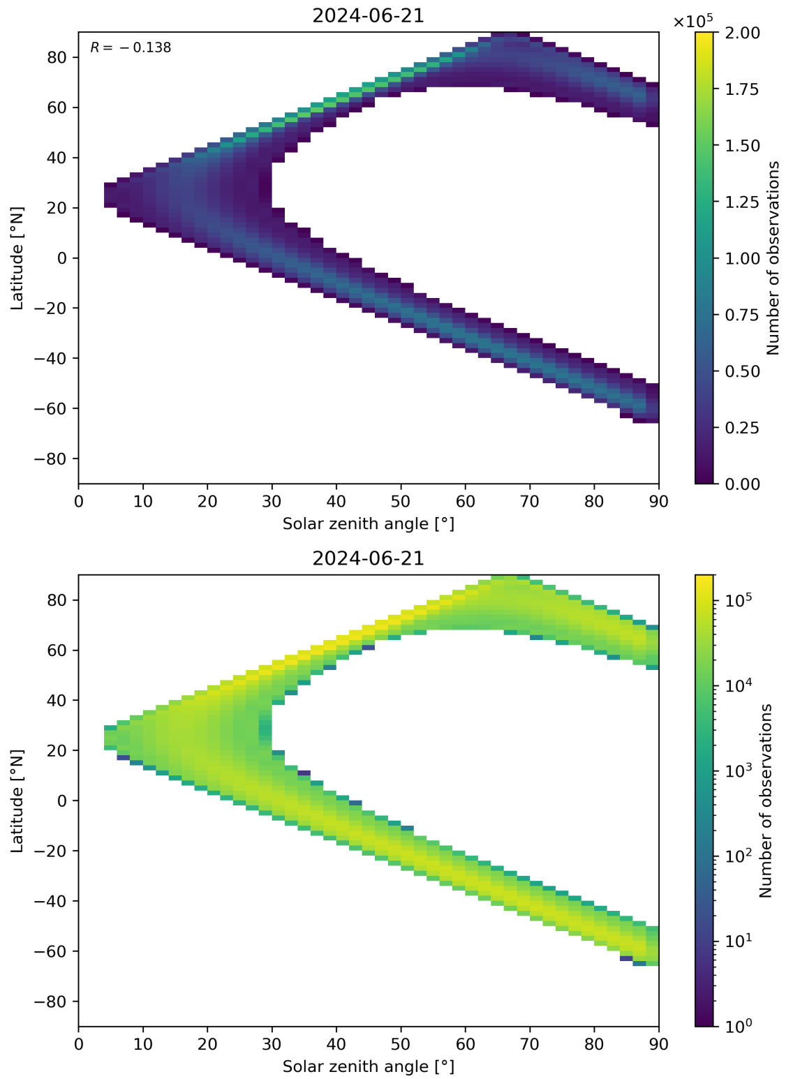
Figure 44: Scatter density plot of “Solar zenith angle” against “Latitude” for 2024-06-20 to 2024-06-22.
