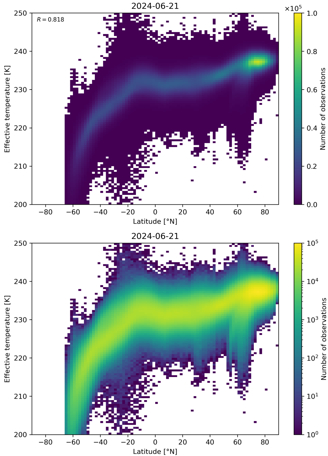
Figure 34: Scatter density plot of “Latitude” against “Effective temperature” for 2024-06-20 to 2024-06-22.
