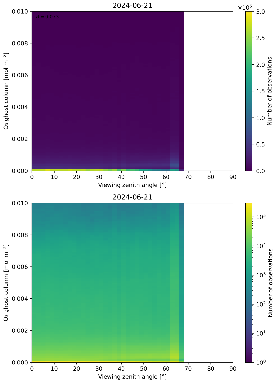
Figure 51: Scatter density plot of “Viewing zenith angle” against “O 3 ghost column” for 2024-06-20 to 2024-06-22.
