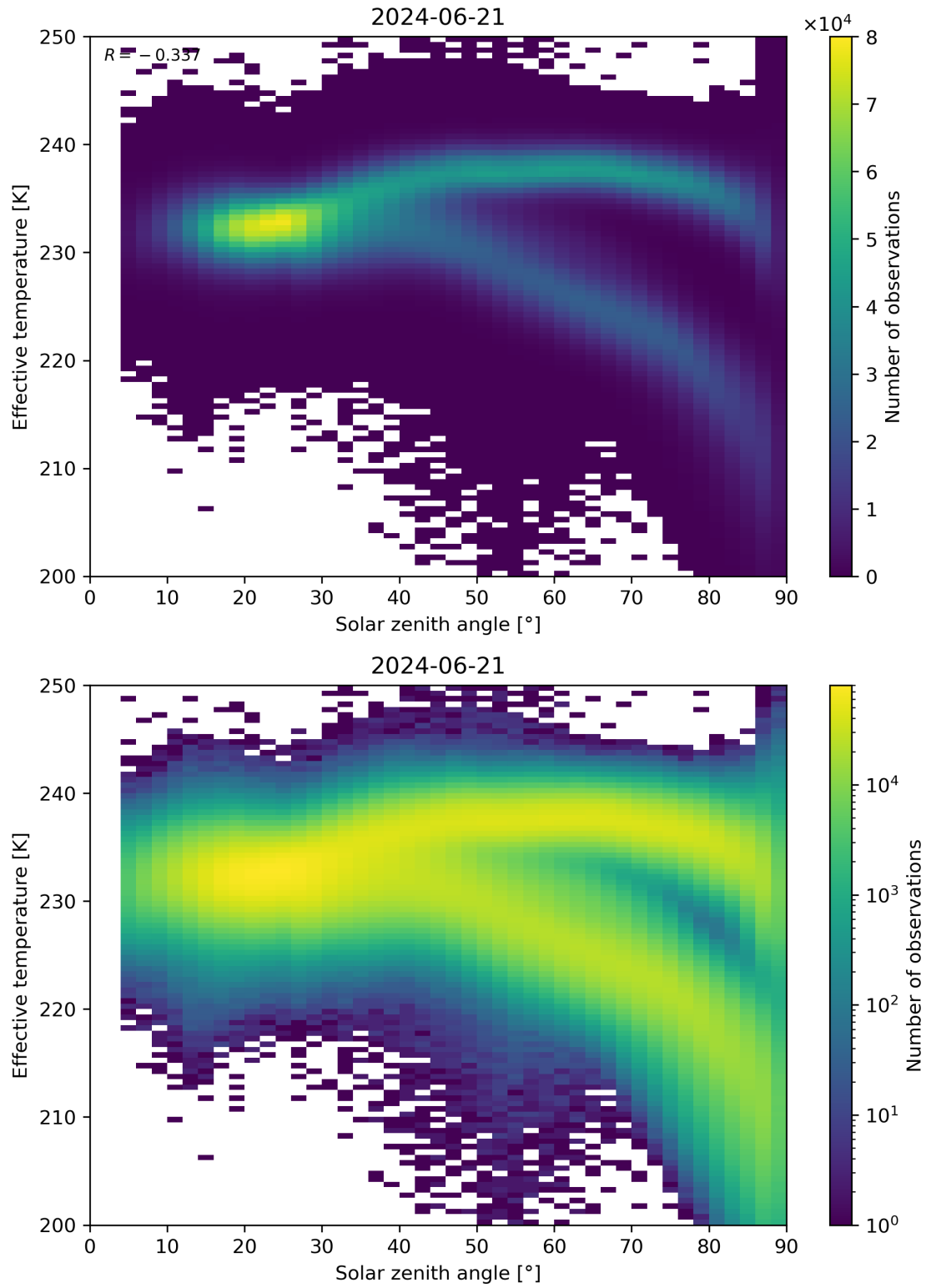
Figure 45: Scatter density plot of “Solar zenith angle” against “Effective temperature” for 2024-06-20 to 2024-06-22.
