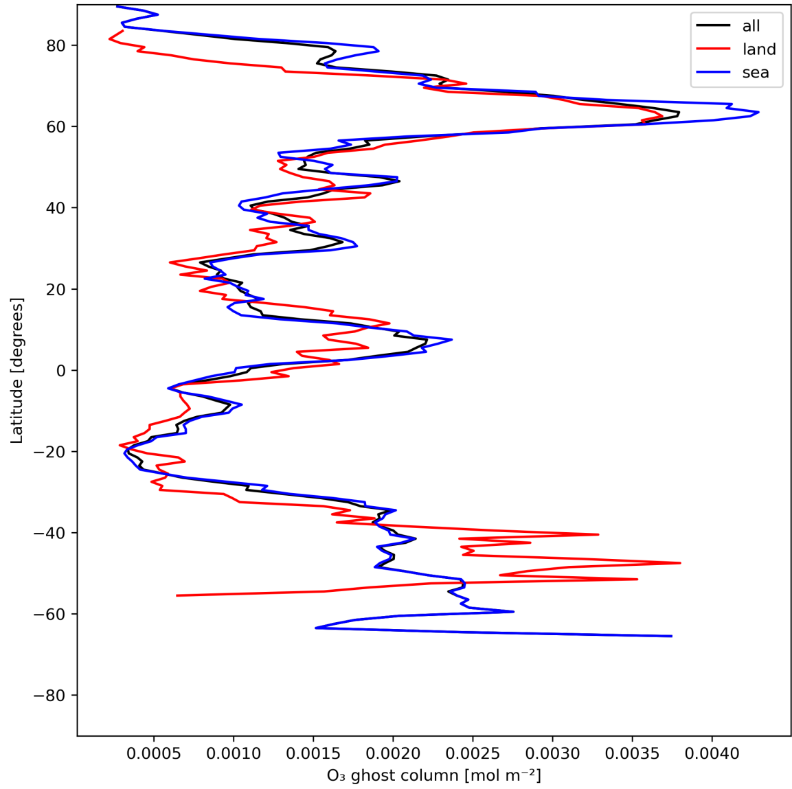
Figure 18: Zonal average of "O 3 ghost column" for 2024-06-20 to 2024-06-22.
