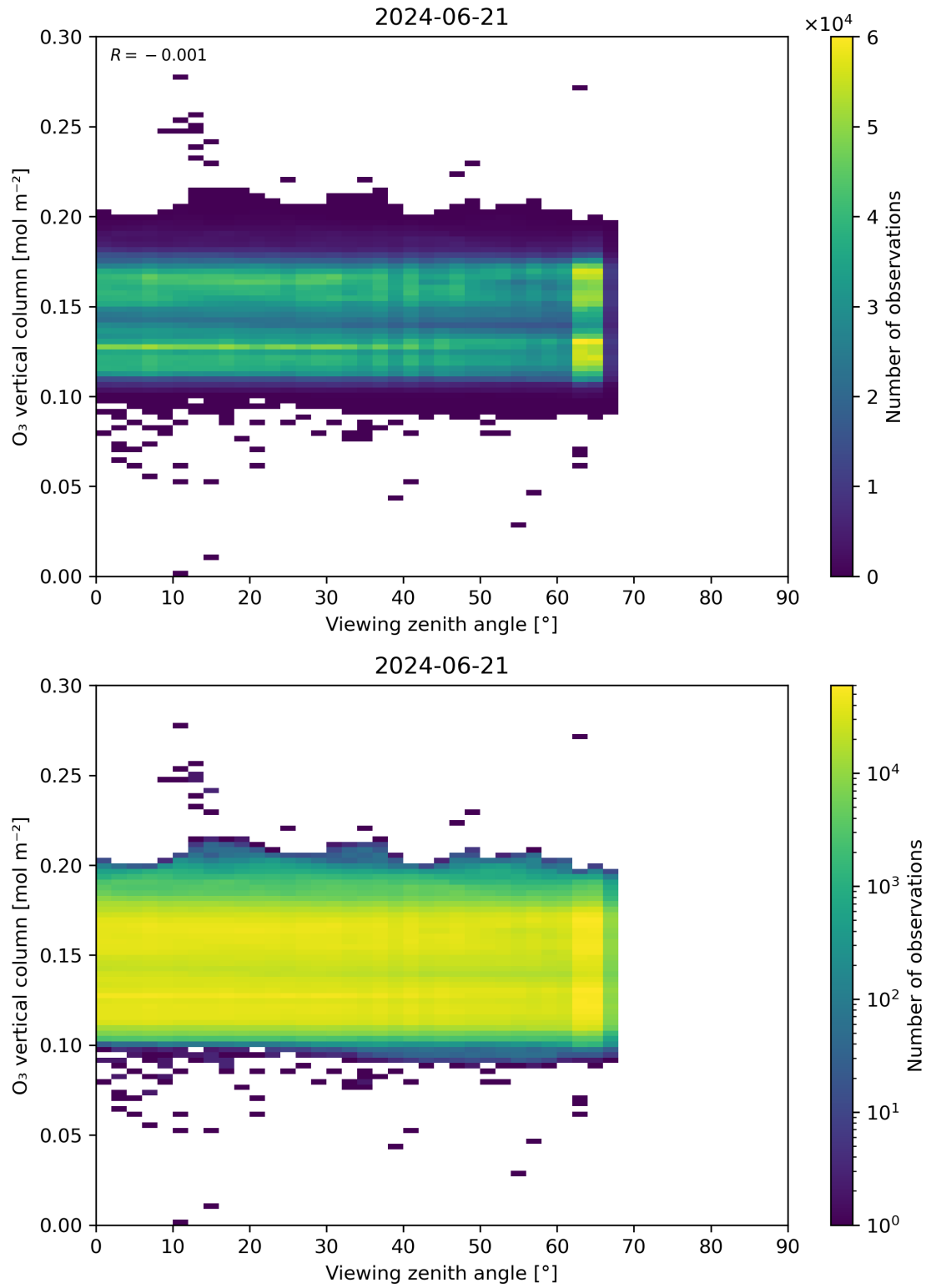
Figure 52: Scatter density plot of “Viewing zenith angle” against “O 3 vertical column” for 2024-06-20 to 2024-06-22.
