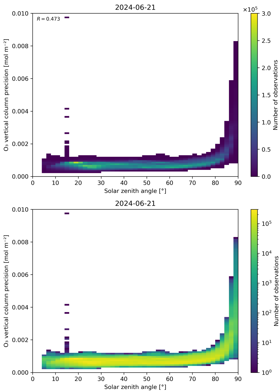
Figure 48: Scatter density plot of “Solar zenith angle” against “O 3 vertical column precision” for 2024-06-20 to 2024-06-22.
