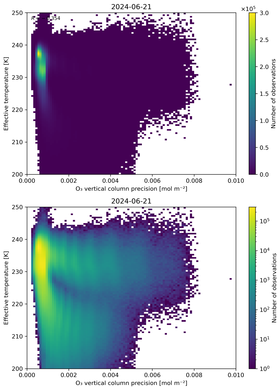
Figure 42: Scatter density plot of “O 3 vertical column precision” against “Effective temperature” for 2024-06-20 to 2024-06-22.
