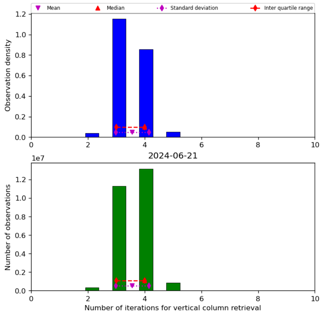
Figure 26: Histogram of “Number of iterations for vertical column retrieval” for 2024-06-20 to 2024-06-22
