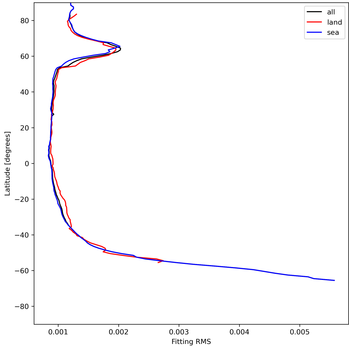
Figure 16: Zonal average of “Fitting RMS” for 2024-06-20 to 2024-06-22.
