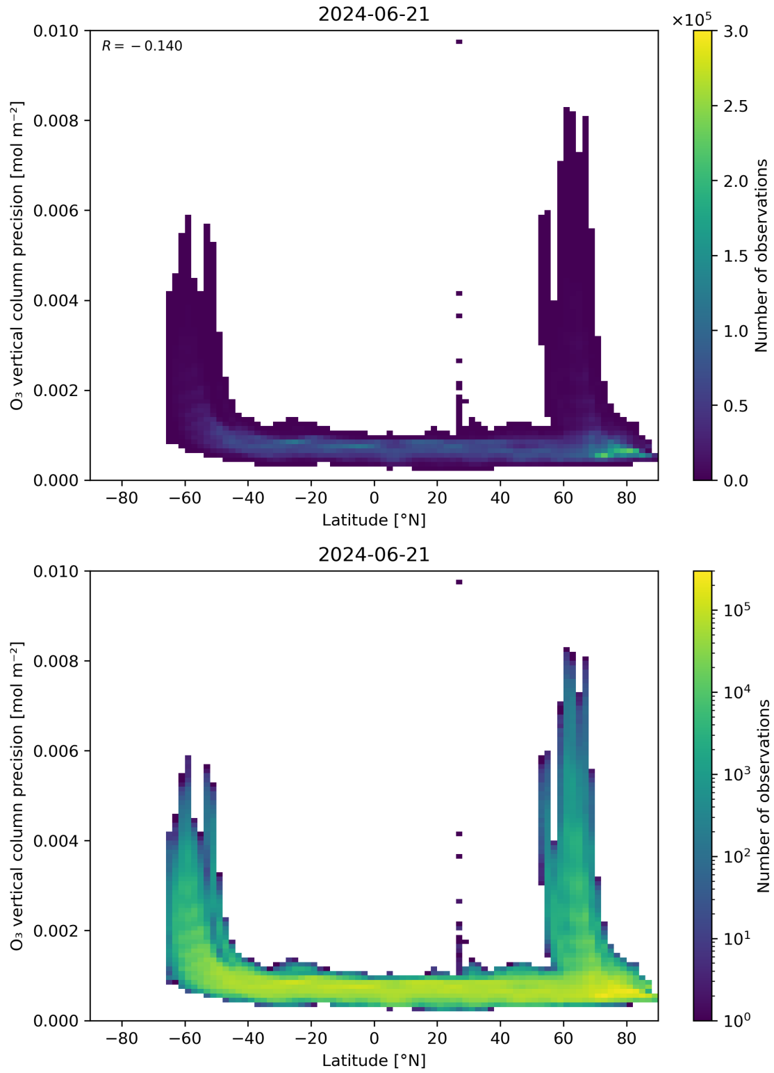
Figure 37: Scatter density plot of “Latitude” against “O 3 vertical column precision” for 2024-06-20 to 2024-06-22.
