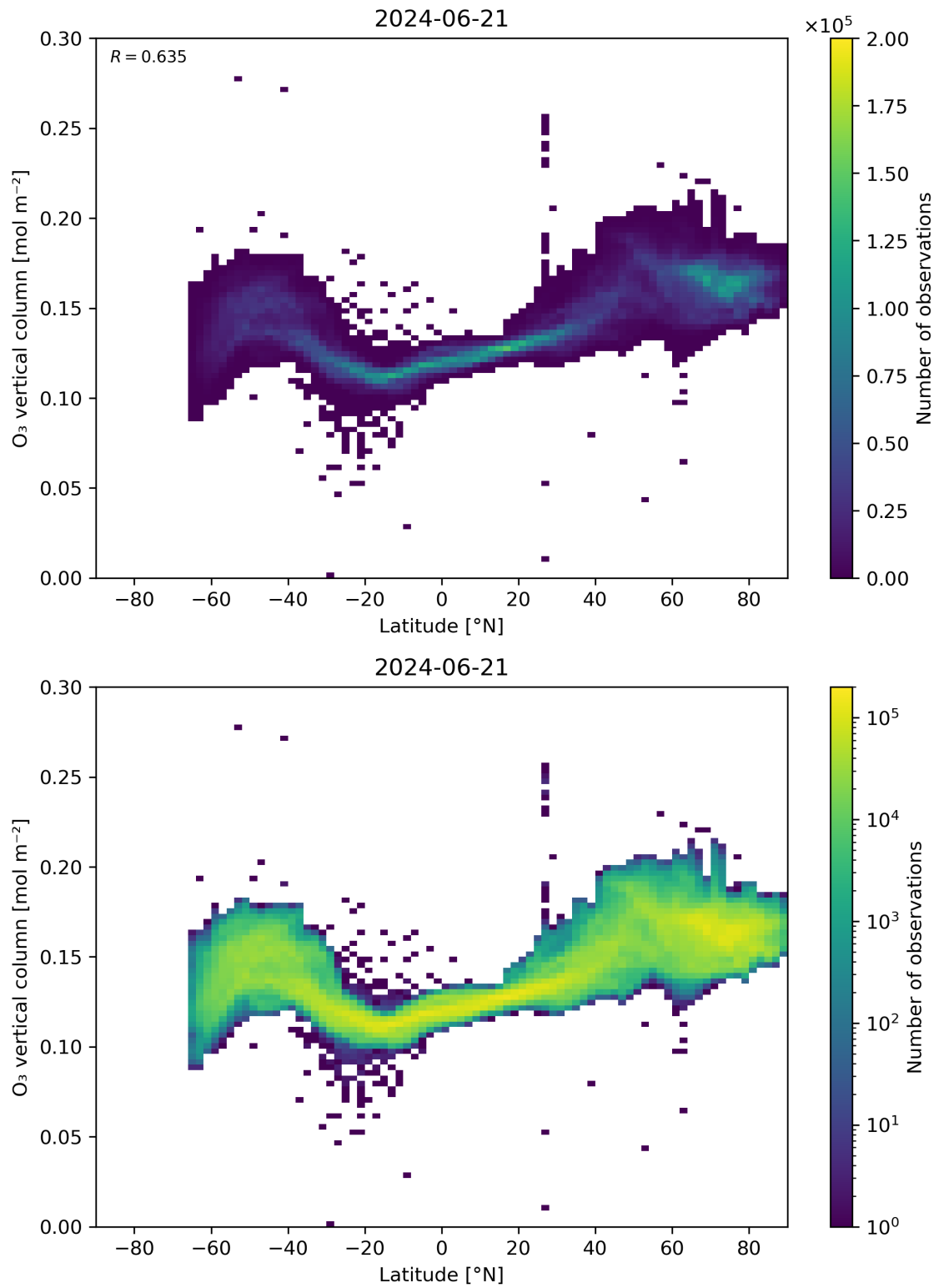
Figure 36: Scatter density plot of “Latitude” against “O 3 vertical column” for 2024-06-20 to 2024-06-22.
