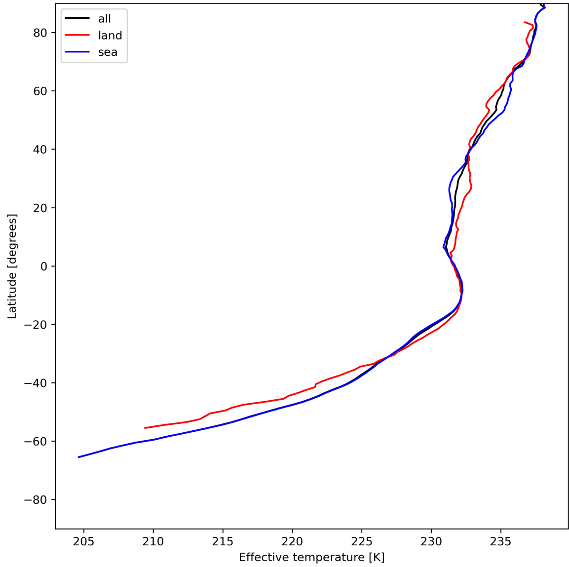
Figure 17: Zonal average of "Effective temperature" for 2024-06-20 to 2024-06-22.
