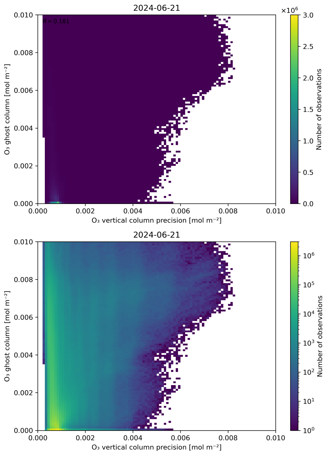
Figure 43: Scatter density plot of “ O_3 vertical column precision” against “ O_3 ghost column” for 2024-06-20 to 2024-06-22.
