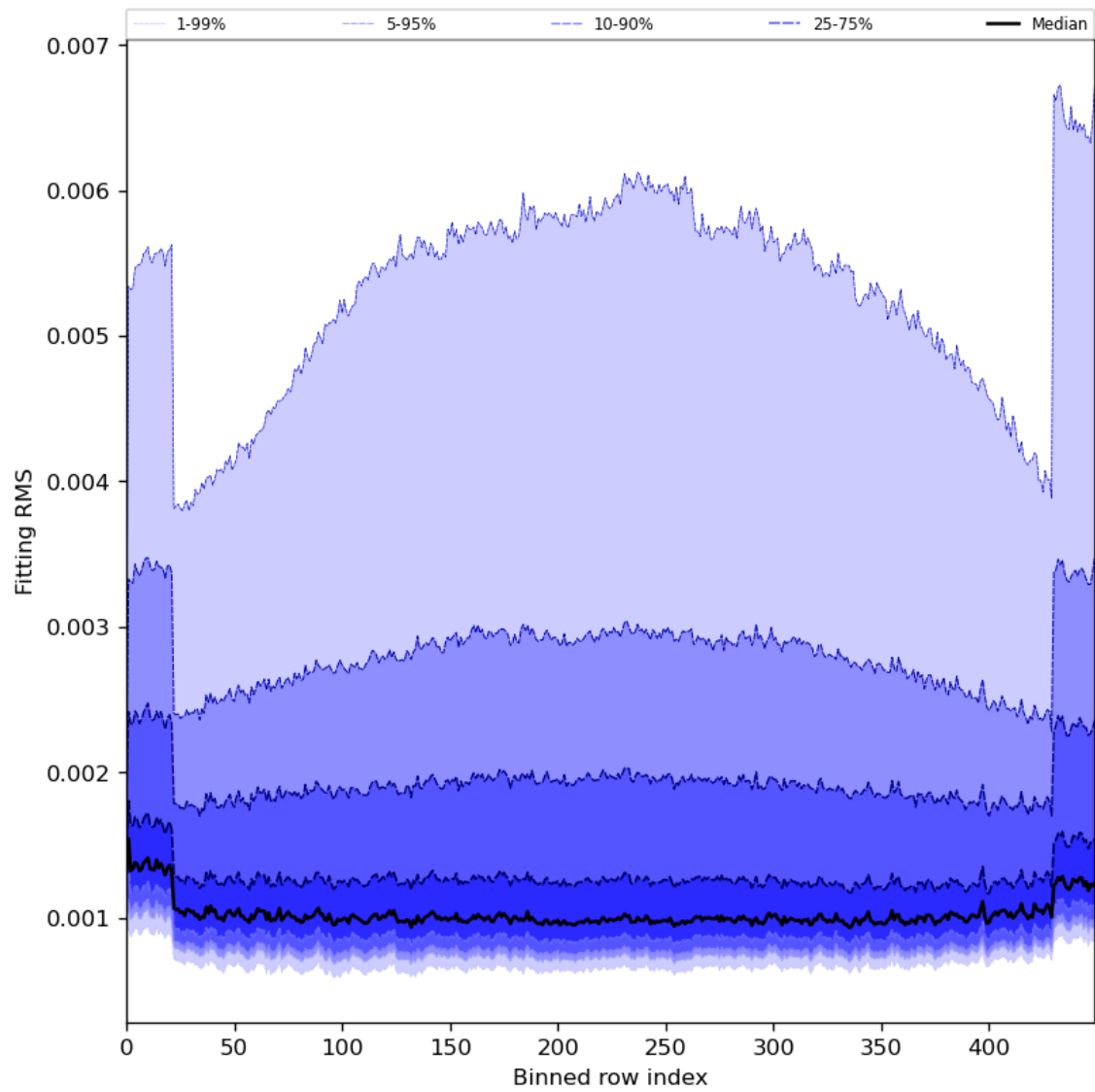
Figure 30: Along track statistics of “Fitting RMS” for 2024-06-20 to 2024-06-22
