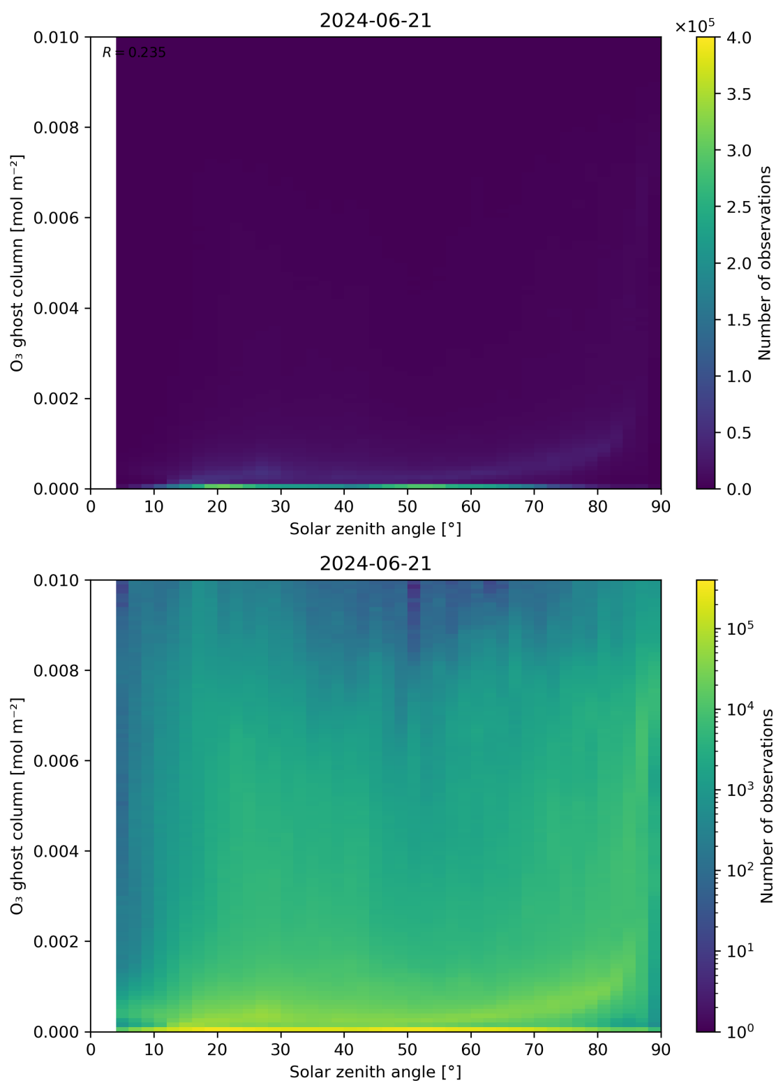
Figure 46: Scatter density plot of “Solar zenith angle” against “O 3 ghost column” for 2024-06-20 to 2024-06-22.
