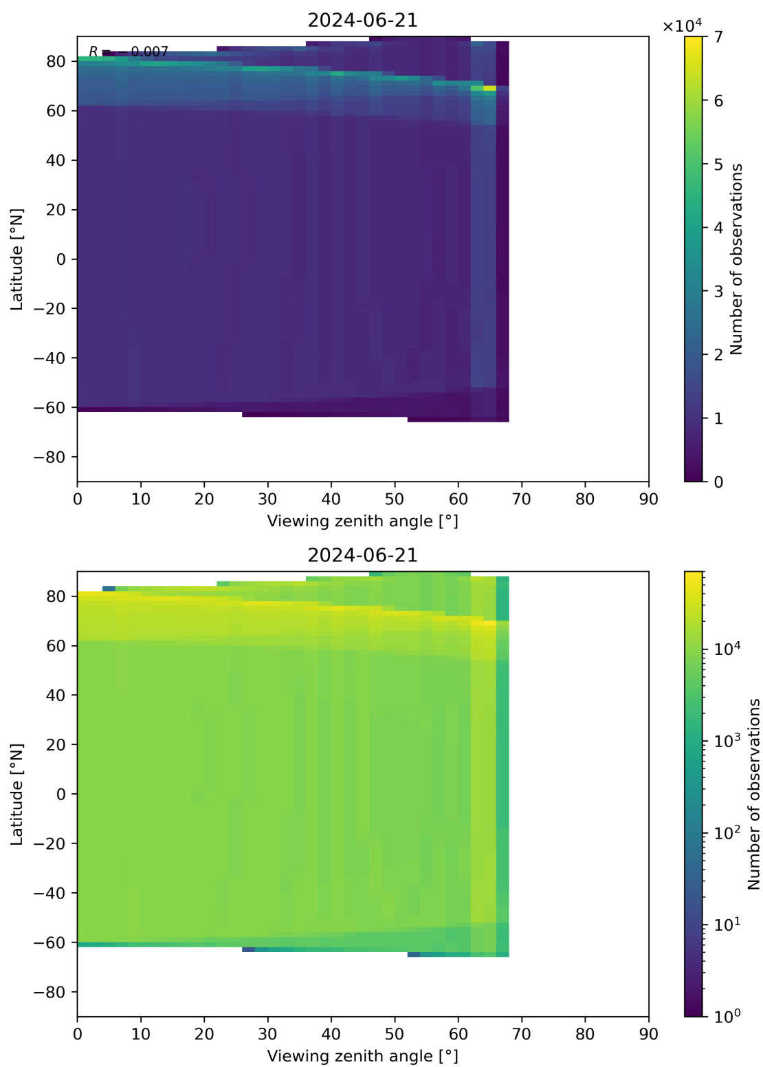
Figure 49: Scatter density plot of “Viewing zenith angle” against “Latitude” for 2024-06-20 to 2024-06-22.
