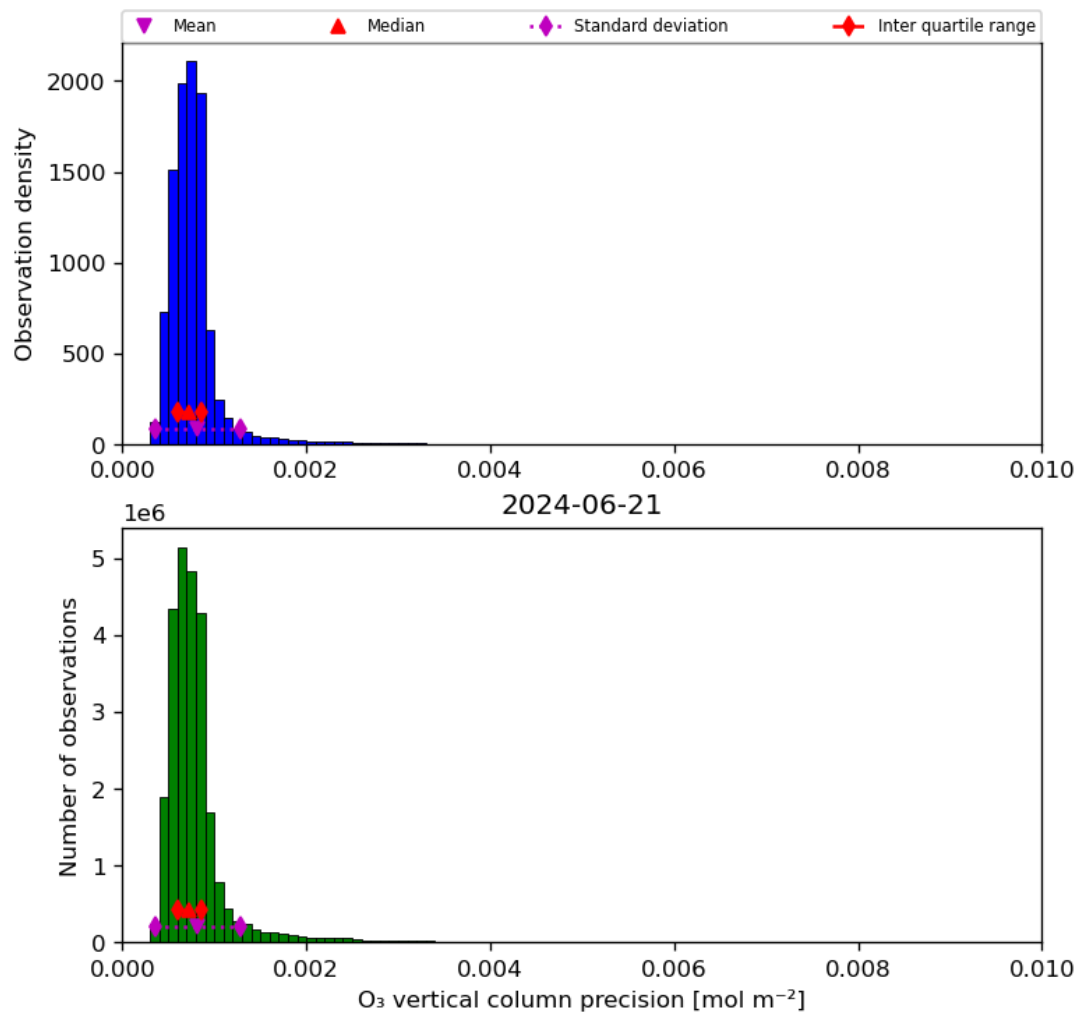
Figure 22: Histogram of “O 3 vertical column precision” for 2024-06-20 to 2024-06-22
