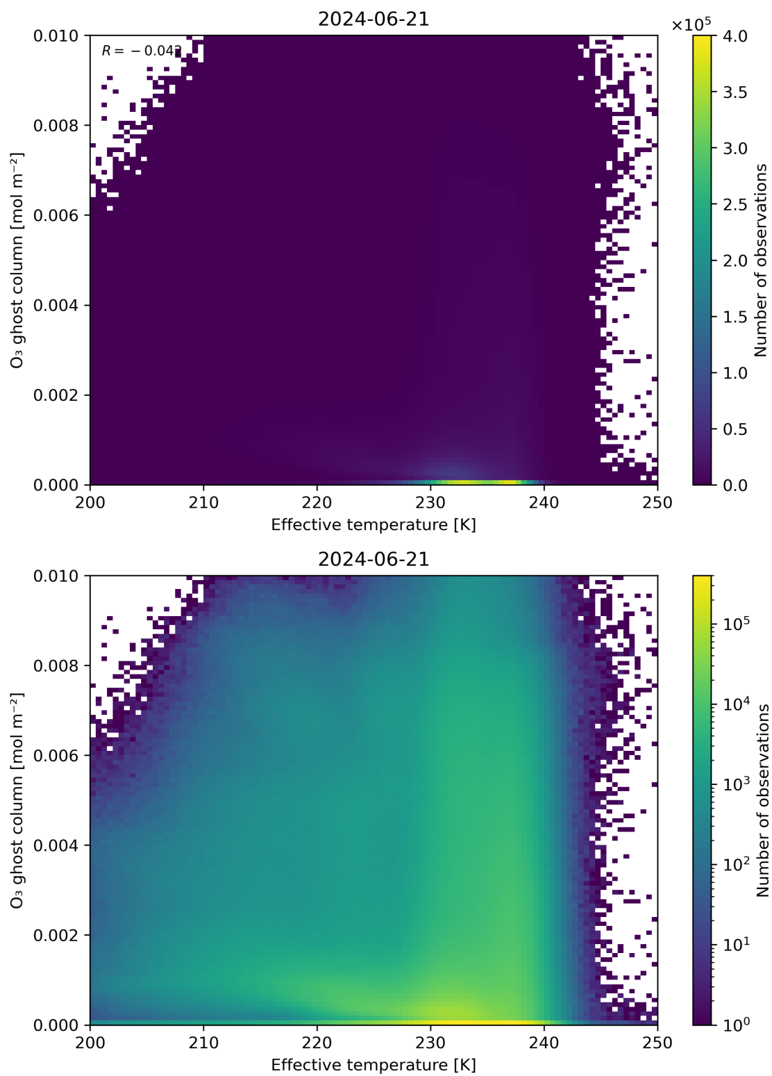
Figure 38: Scatter density plot of “Effective temperature” against “O 3 ghost column” for 2024-06-20 to 2024-06-22.
