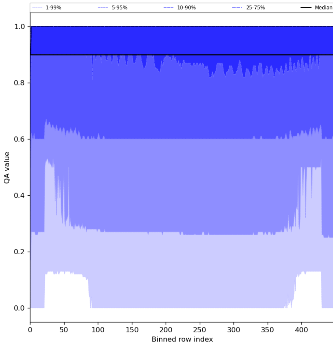
Figure 27: Along track statistics of “QA value” for 2024-06-20 to 2024-06-22
