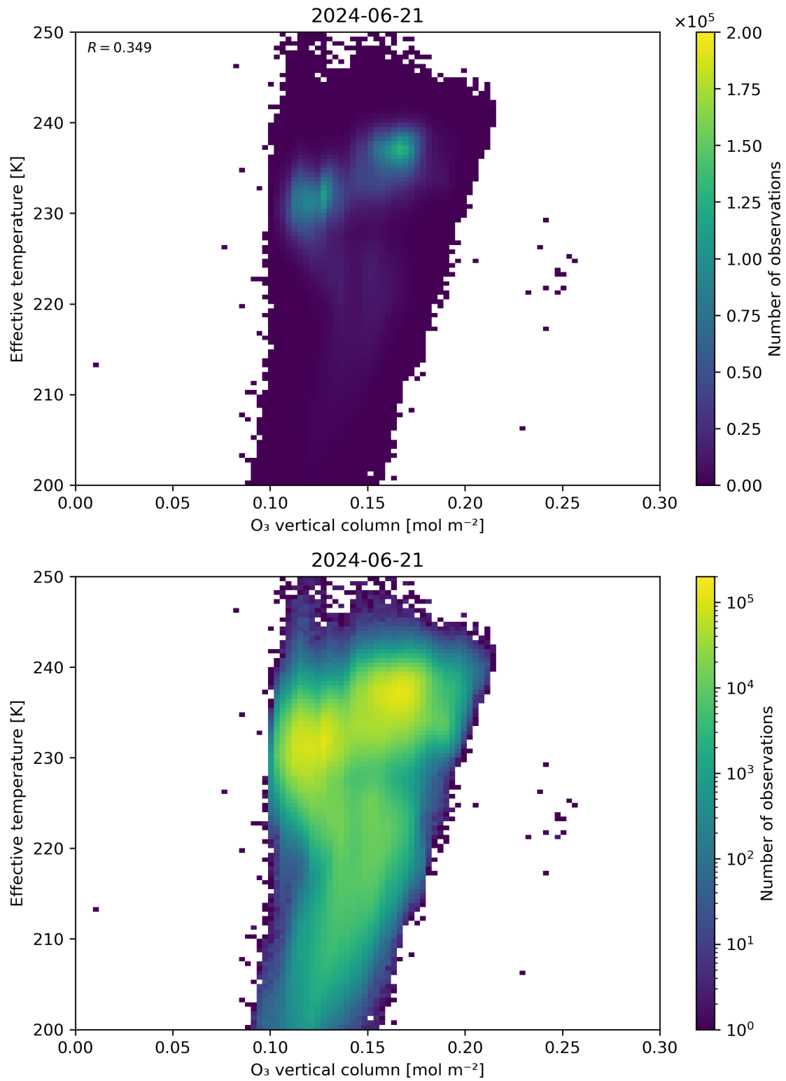
Figure 39: Scatter density plot of “O 3 vertical column” against “Effective temperature” for 2024-06-20 to 2024-06-22.
