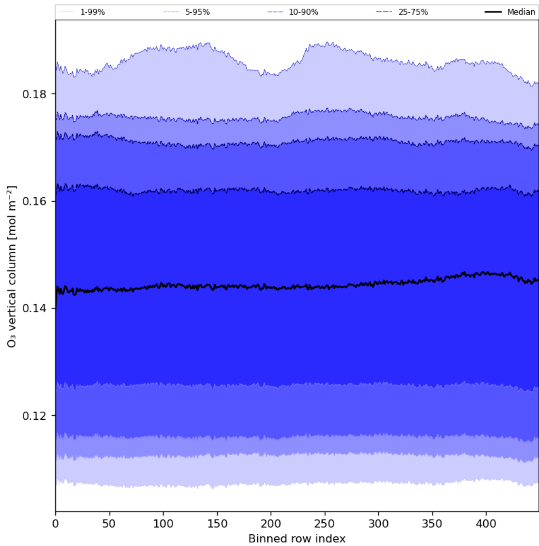
Figure 28: Along track statistics of “O 3 vertical column” for 2024-06-20 to 2024-06-22
