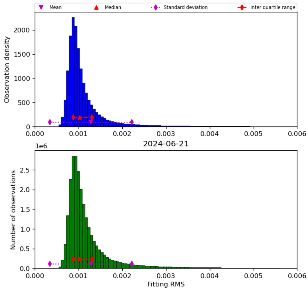
Figure 23: Histogram of “Fitting RMS” for 2024-06-20 to 2024-06-22
