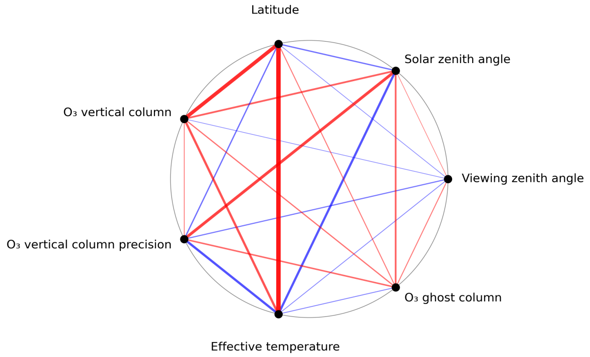
Figure 1: Map of correlation graph for 2024-06-20 to 2024-06-22.
