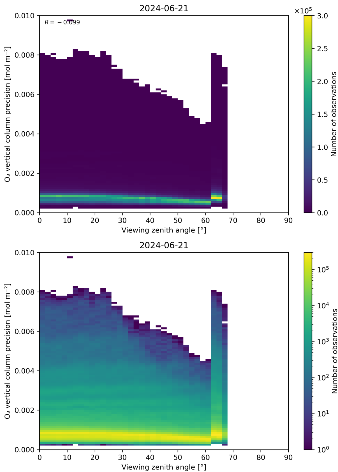
Figure 53: Scatter density plot of “Viewing zenith angle” against “O 3 vertical column precision” for 2024-06-20 to 2024-06-22.
