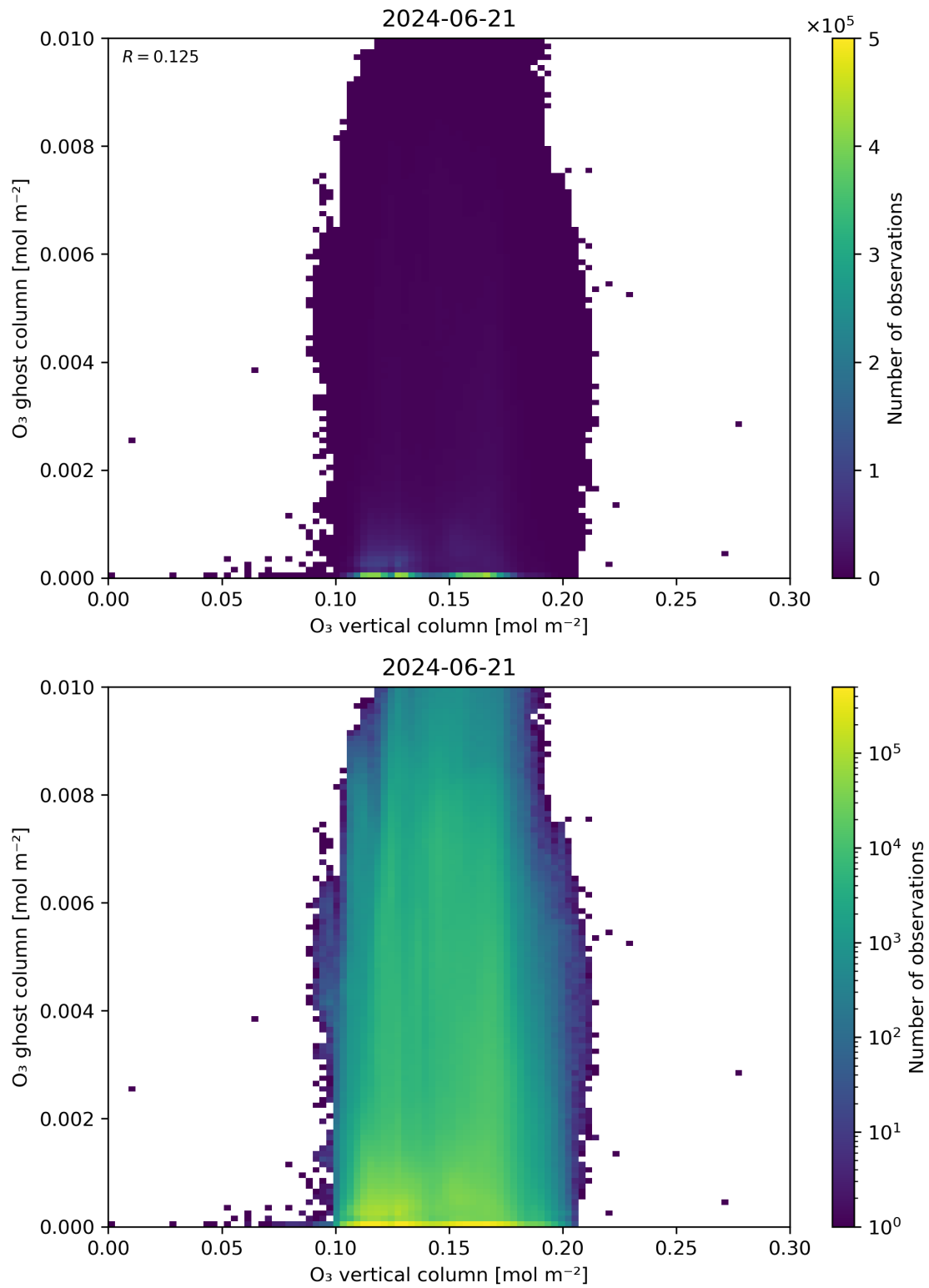
Figure 40: Scatter density plot of “O 3 vertical column” against “O 3 ghost column” for 2024-06-20 to 2024-06-22.
