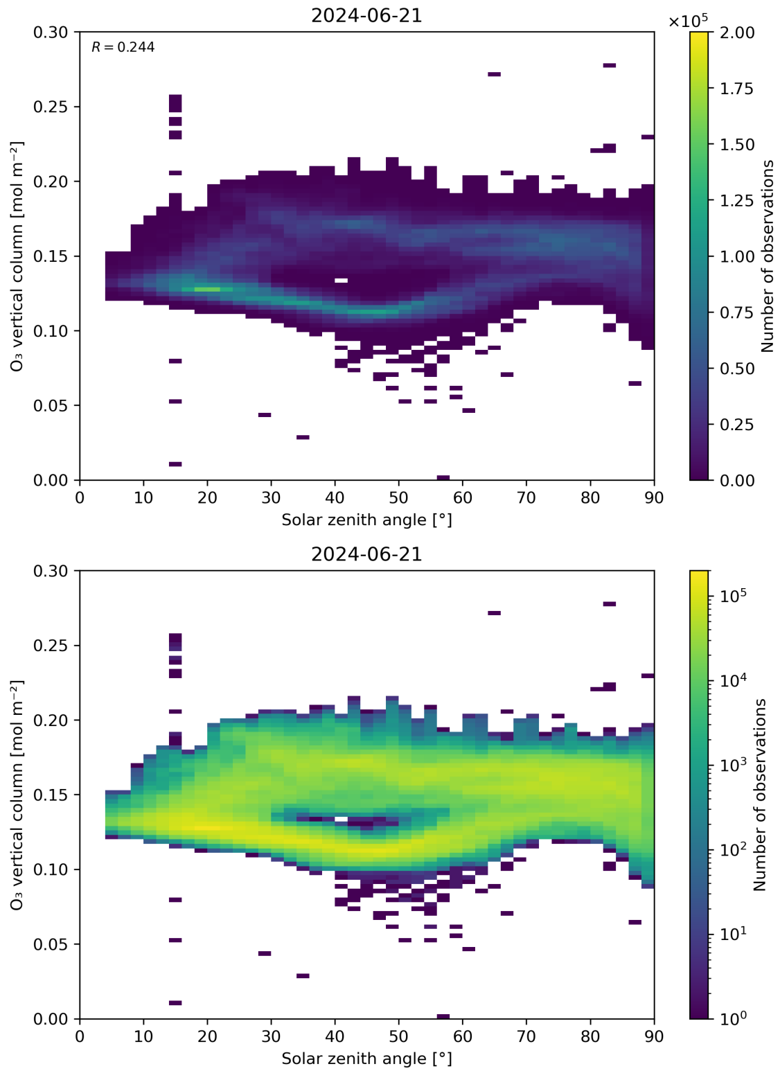
Figure 47: Scatter density plot of “Solar zenith angle” against “O 3 vertical column” for 2024-06-20 to 2024-06-22.
