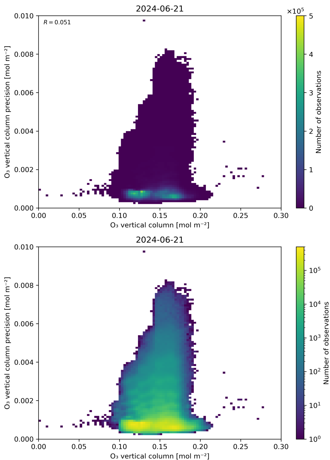
Figure 41: Scatter density plot of “O 3 vertical column” against “O 3 vertical column precision” for 2024-06-20 to 2024-06-22.
