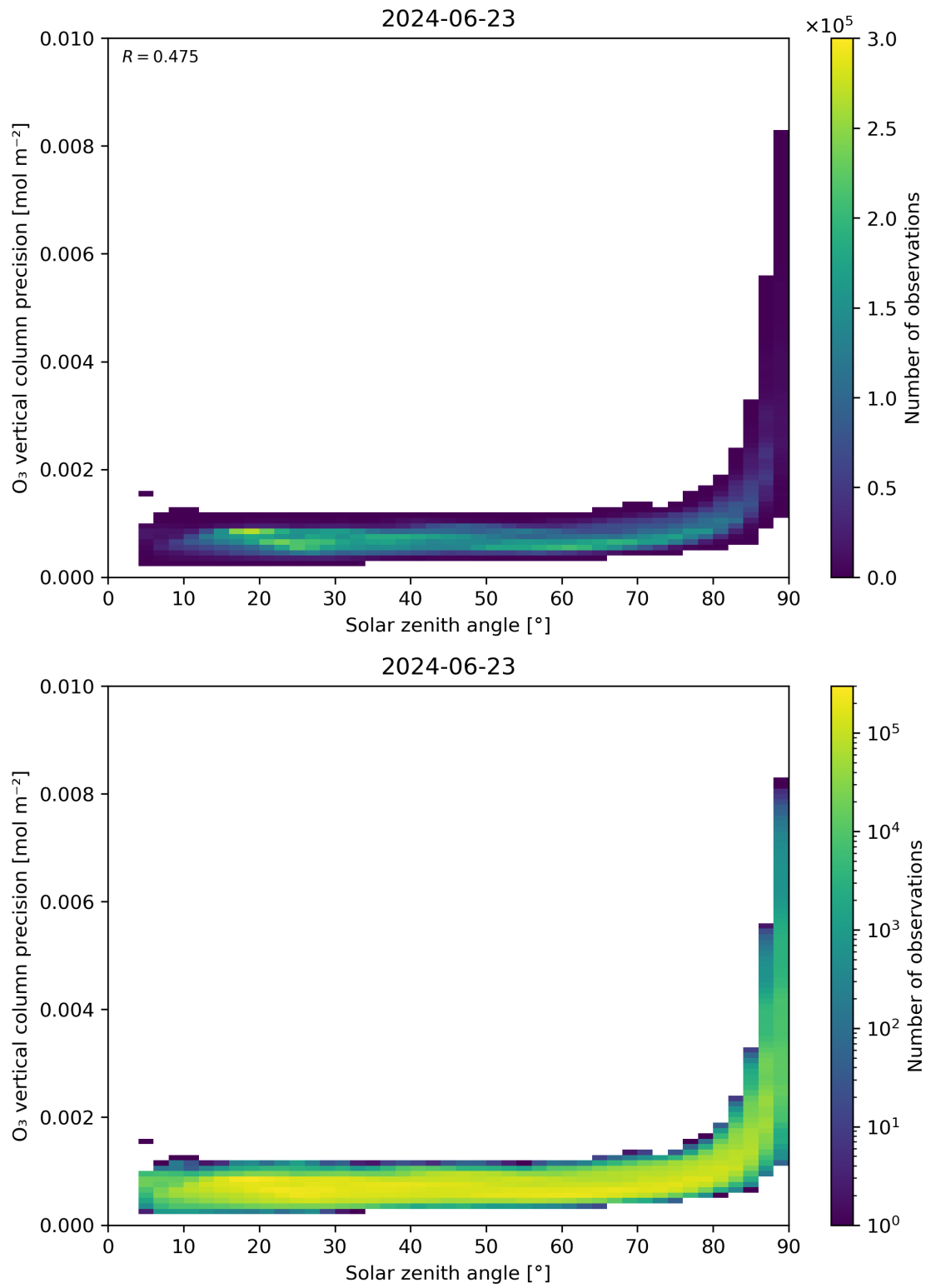
Figure 48: Scatter density plot of “Solar zenith angle” against “O 3 vertical column precision” for 2024-06-22 to 2024-06-24.
