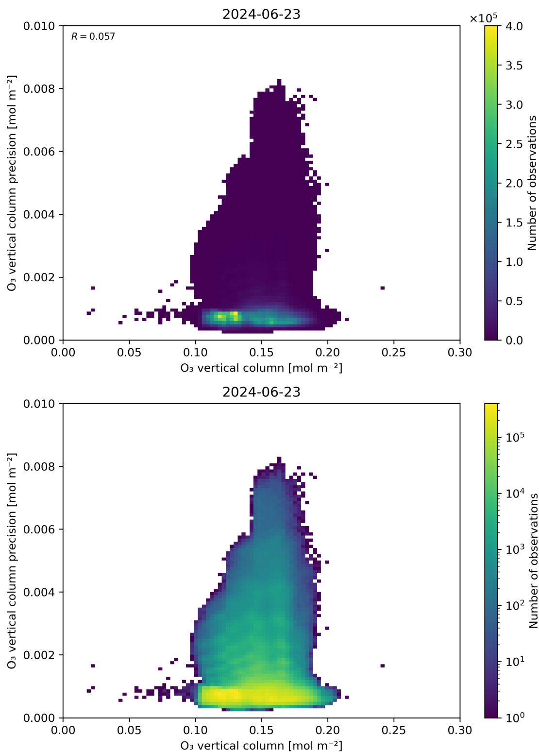
Figure 41: Scatter density plot of “O 3 vertical column” against “O 3 vertical column precision” for 2024-06-22 to 2024-06-24.
