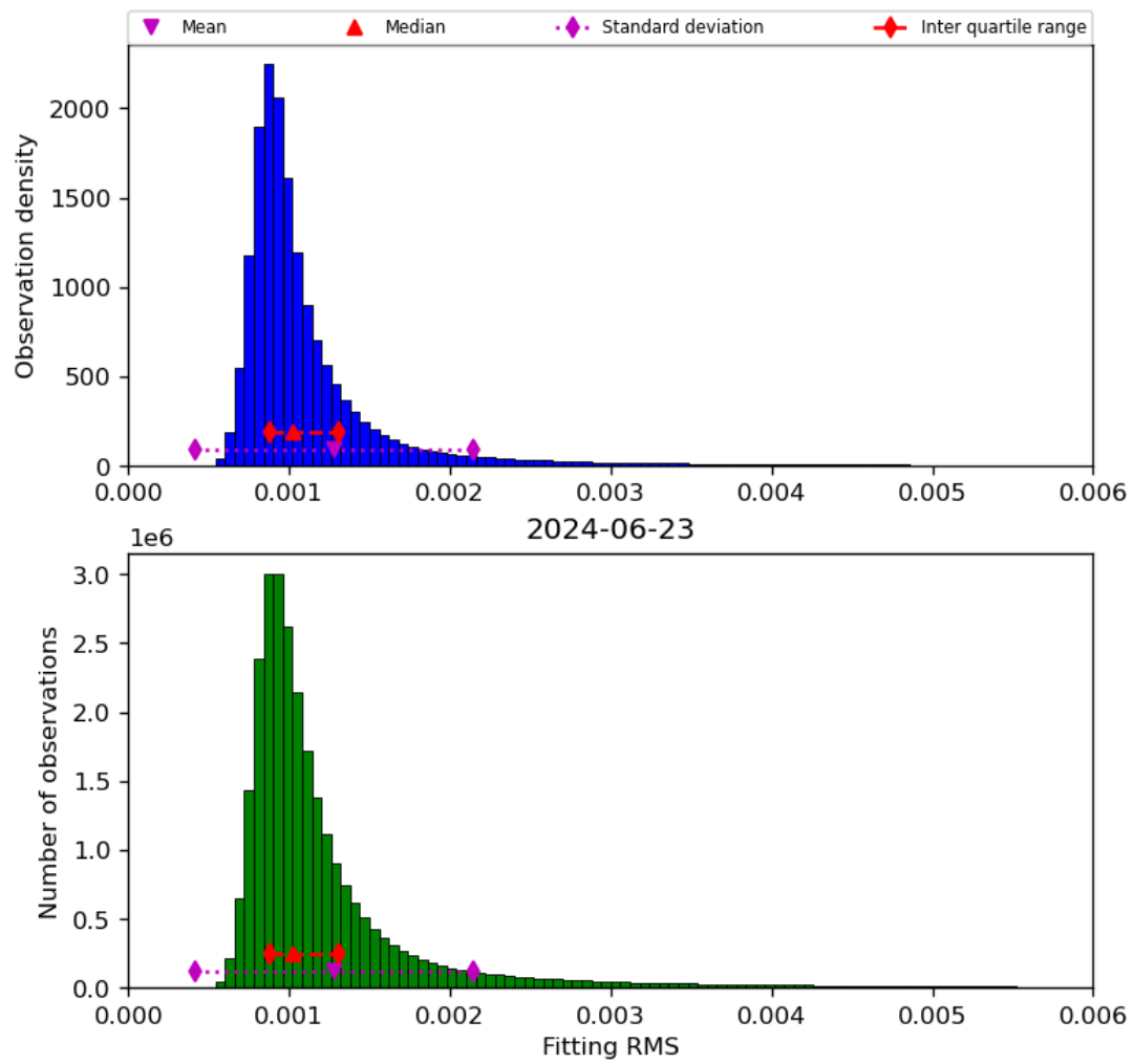
Figure 23: Histogram of “Fitting RMS” for 2024-06-22 to 2024-06-24
