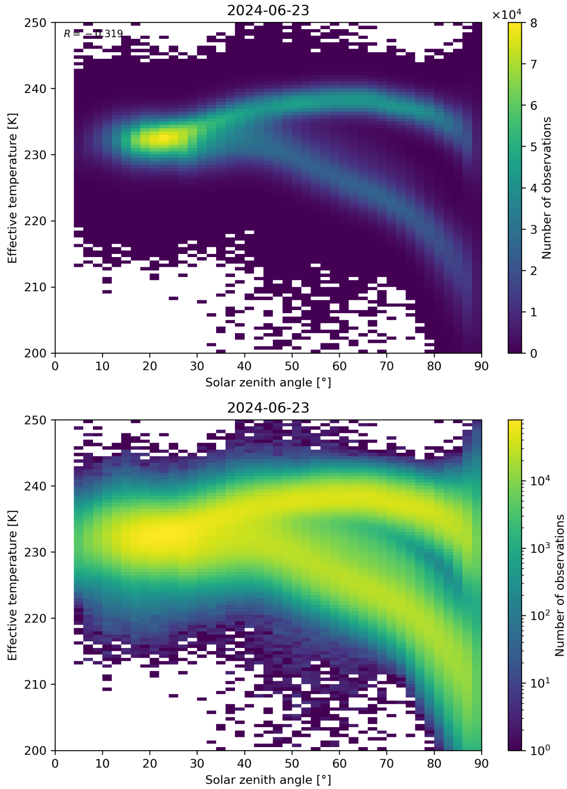
Figure 45: Scatter density plot of “Solar zenith angle” against “Effective temperature” for 2024-06-22 to 2024-06-24.
