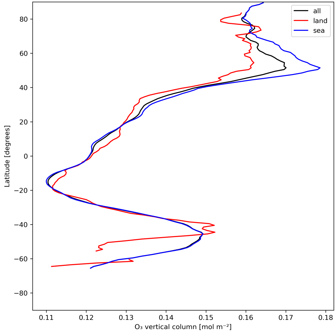
Figure 14: Zonal average of “O 3 vertical column” for 2024-06-22 to 2024-06-24.
