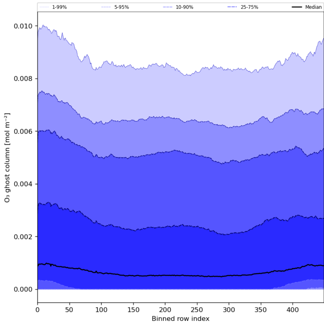
Figure 32: Along track statistics of “O 3 ghost column” for 2024-06-22 to 2024-06-24
