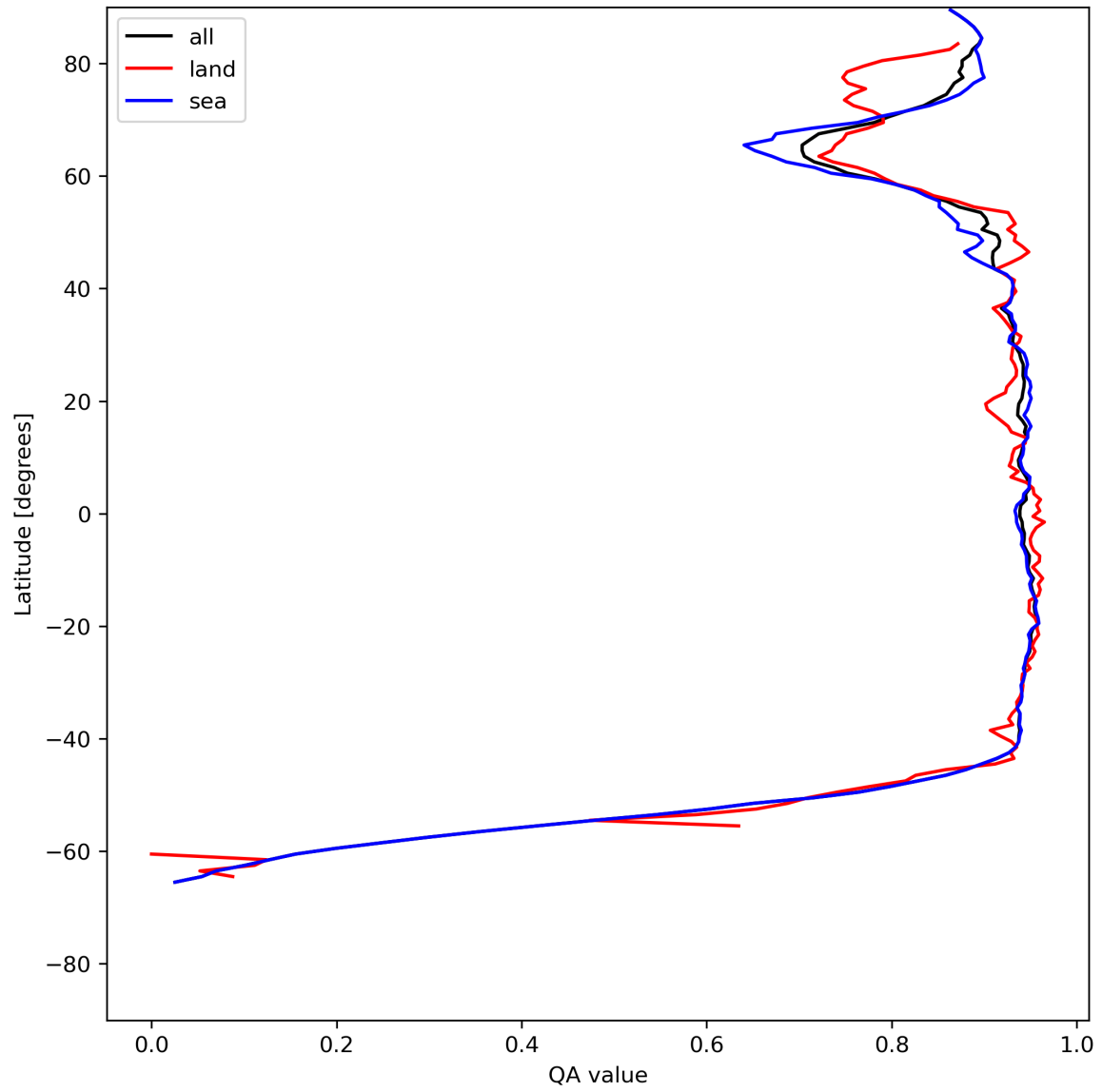
Figure 13: Zonal average of “QA value” for 2024-06-22 to 2024-06-24.
