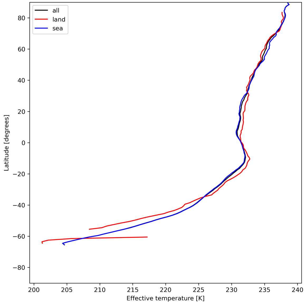
Figure 17: Zonal average of “Effective temperature” for 2024-06-22 to 2024-06-24.
