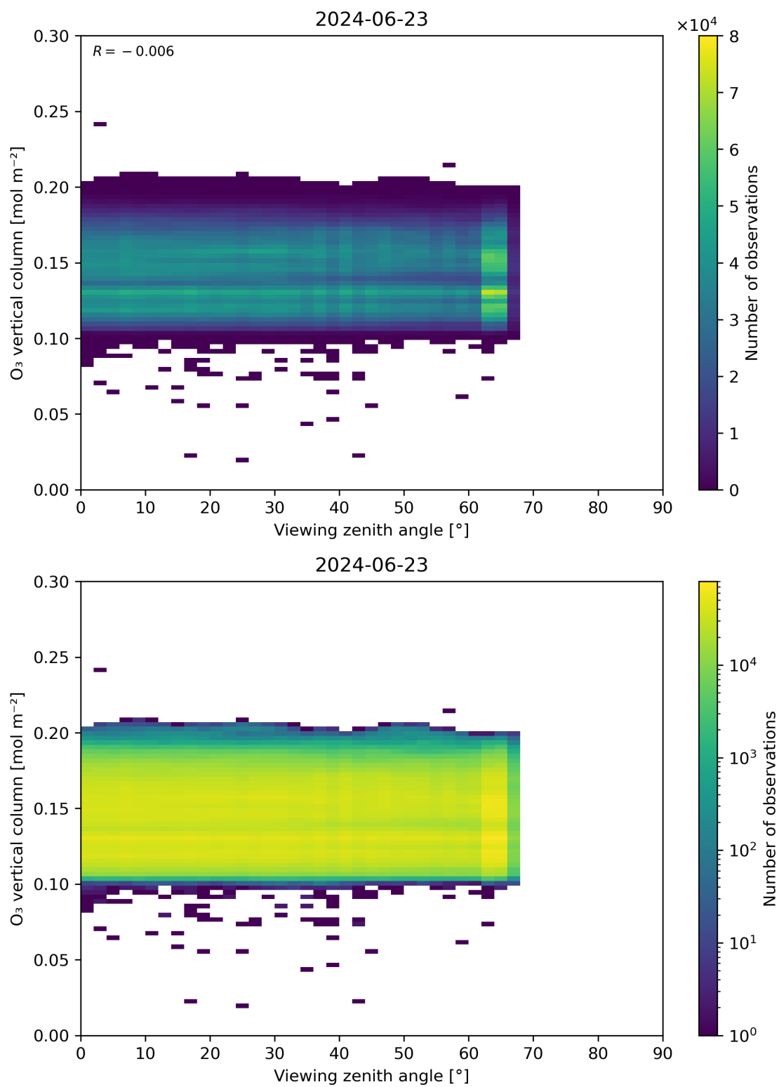
Figure 52: Scatter density plot of “Viewing zenith angle” against “O 3 vertical column” for 2024-06-22 to 2024-06-24.
