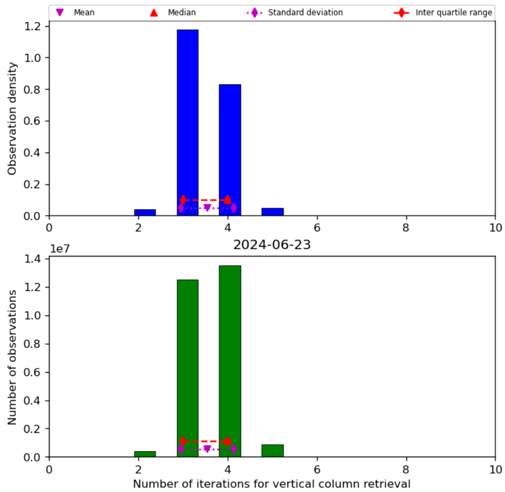
Figure 26: Histogram of “Number of iterations for vertical column retrieval” for 2024-06-22 to 2024-06-24
