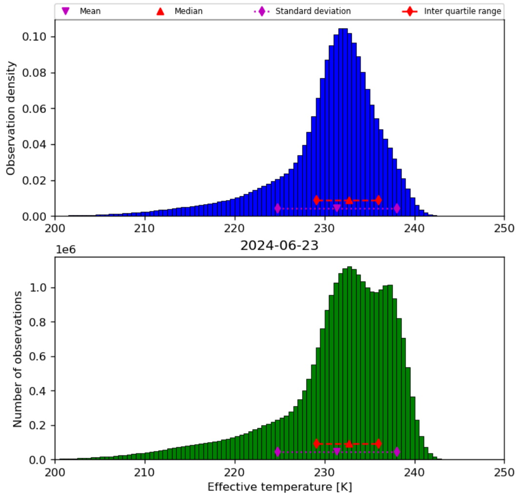
Figure 24: Histogram of “Effective temperature” for 2024-06-22 to 2024-06-24
