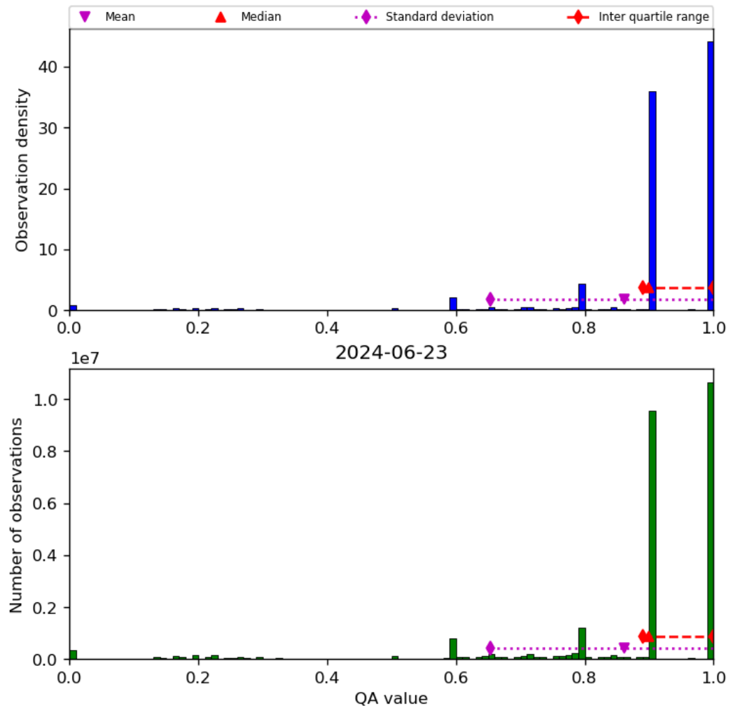
Figure 20: Histogram of “QA value” for 2024-06-22 to 2024-06-24
