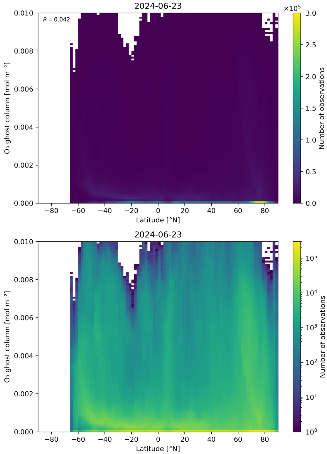
Figure 35: Scatter density plot of “Latitude” against “O 3 ghost column” for 2024-06-22 to 2024-06-24.
