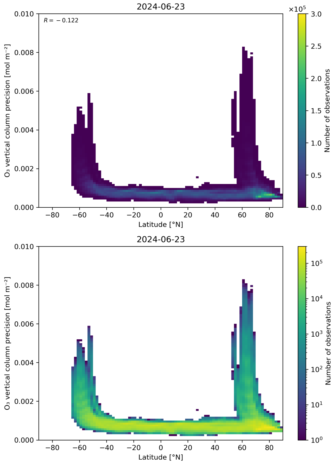
Figure 37: Scatter density plot of “Latitude” against “O 3 vertical column precision” for 2024-06-22 to 2024-06-24.
