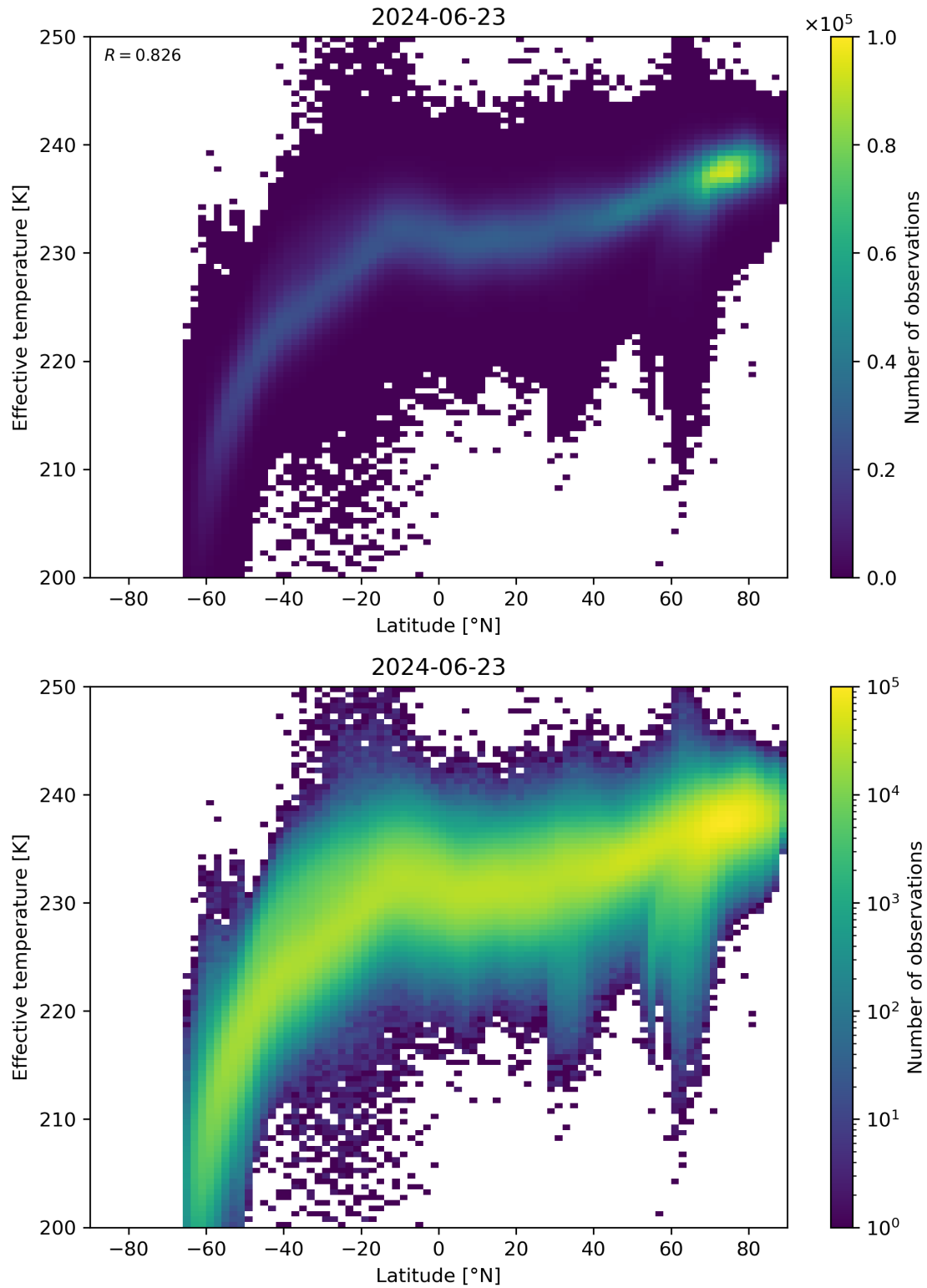
Figure 34: Scatter density plot of “Latitude” against “Effective temperature” for 2024-06-22 to 2024-06-24.
