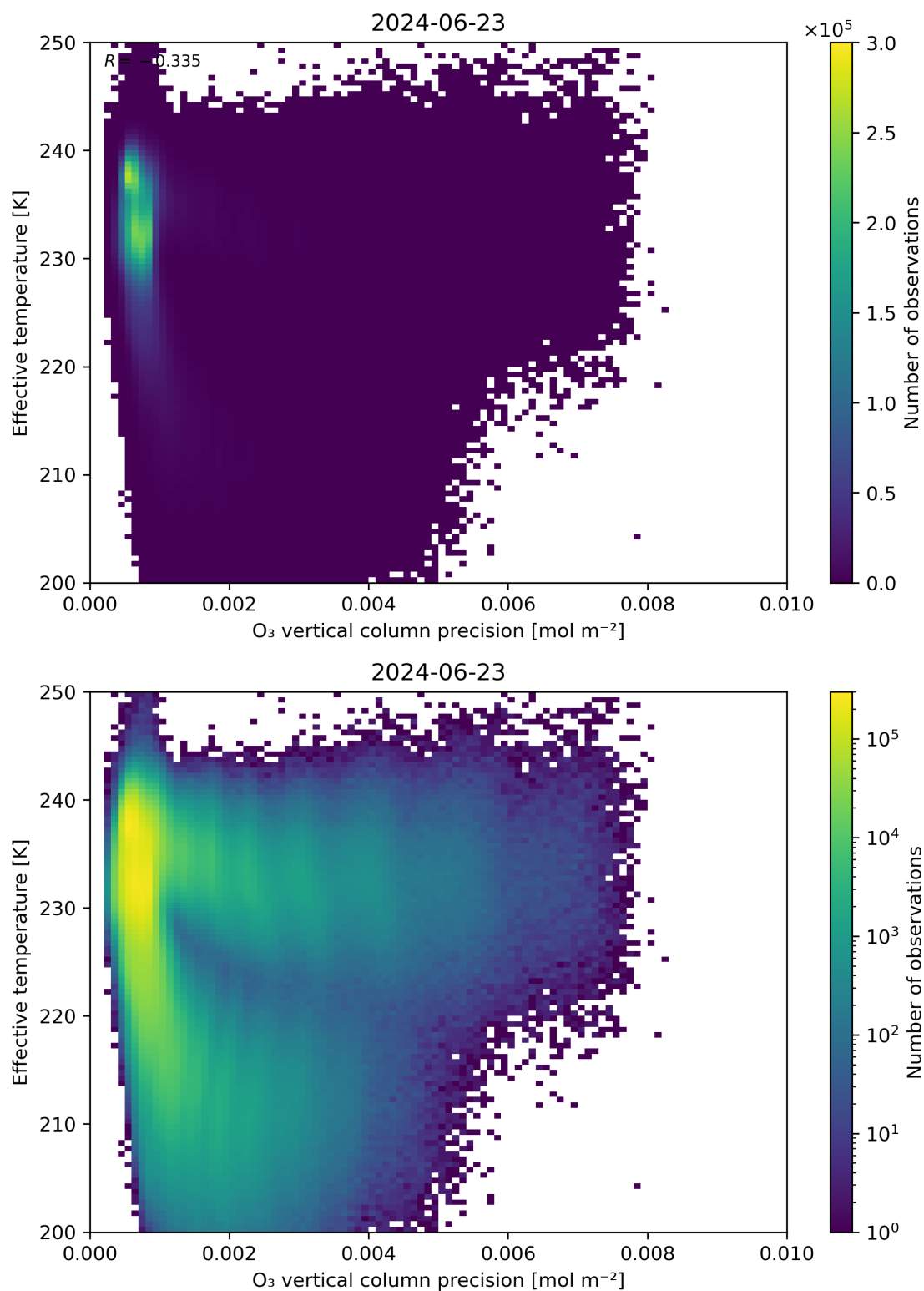
Figure 42: Scatter density plot of “O 3 vertical column precision” against “Effective temperature” for 2024-06-22 to 2024-06-24.
