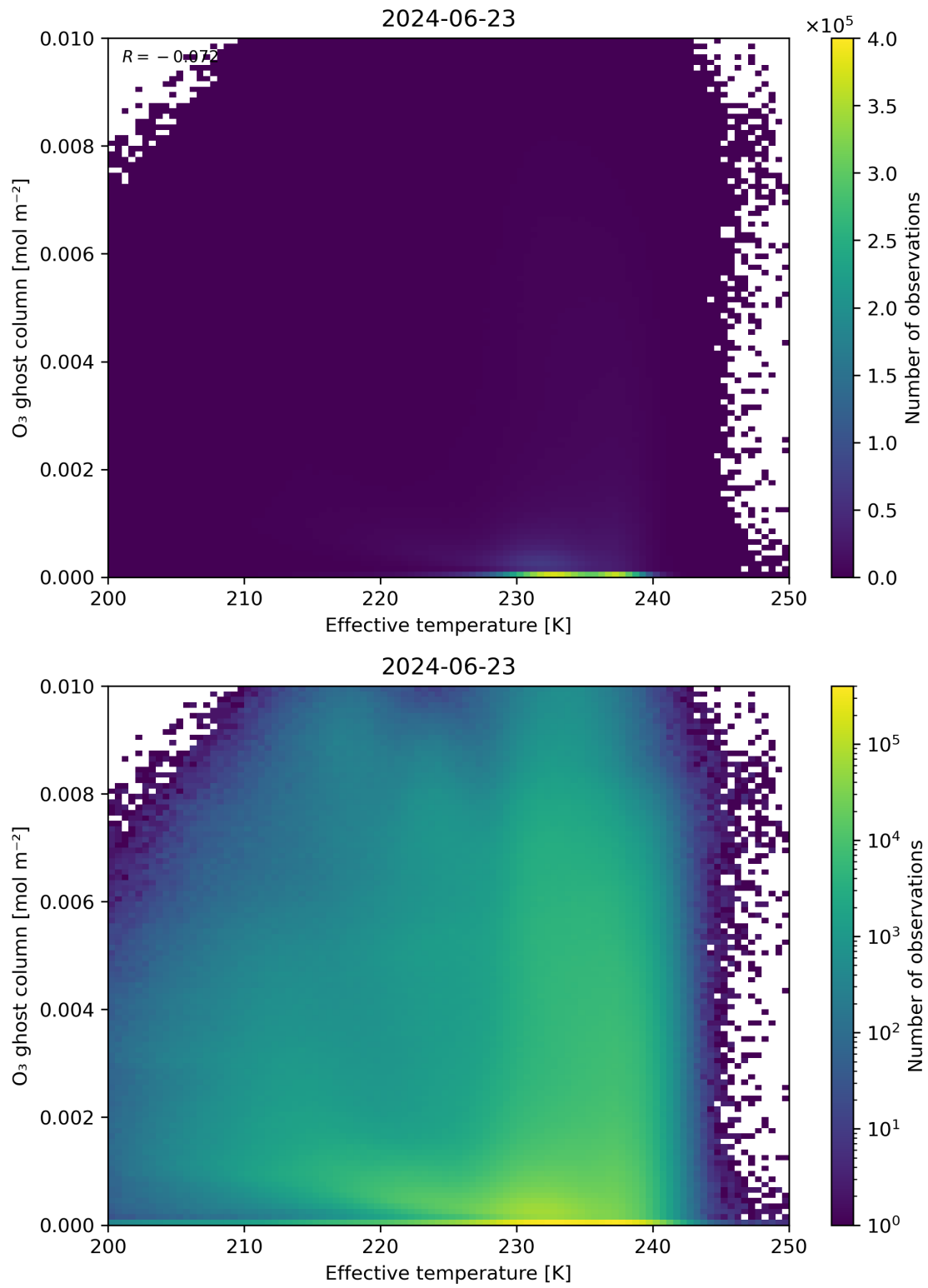
Figure 38: Scatter density plot of “Effective temperature” against “O 3 ghost column” for 2024-06-22 to 2024-06-24.
