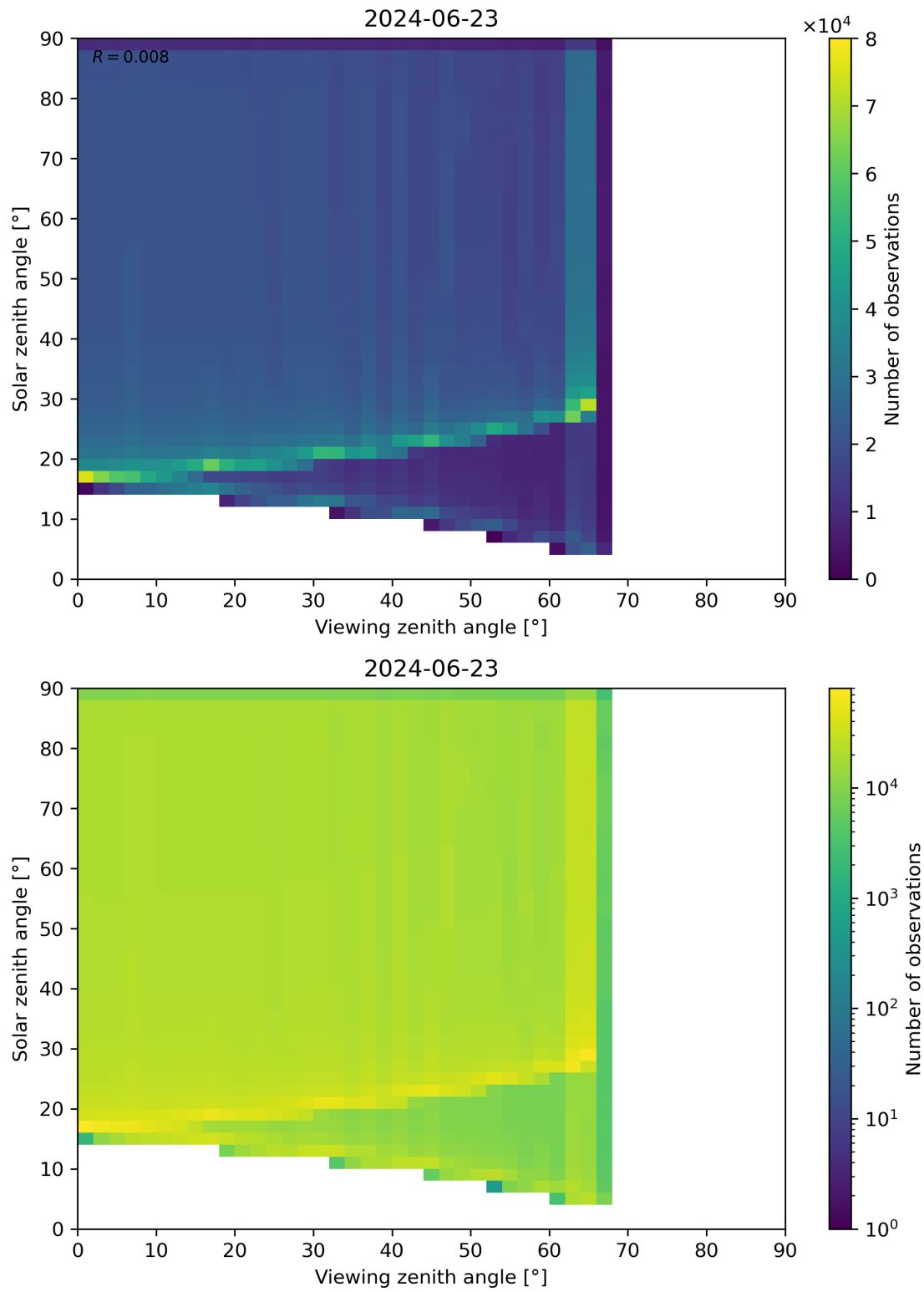
Figure 54: Scatter density plot of “Viewing zenith angle” against “Solar zenith angle” for 2024-06-22 to 2024-06-24.
