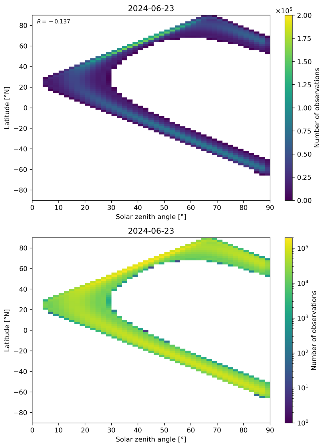
Figure 44: Scatter density plot of “Solar zenith angle” against “Latitude” for 2024-06-22 to 2024-06-24.
