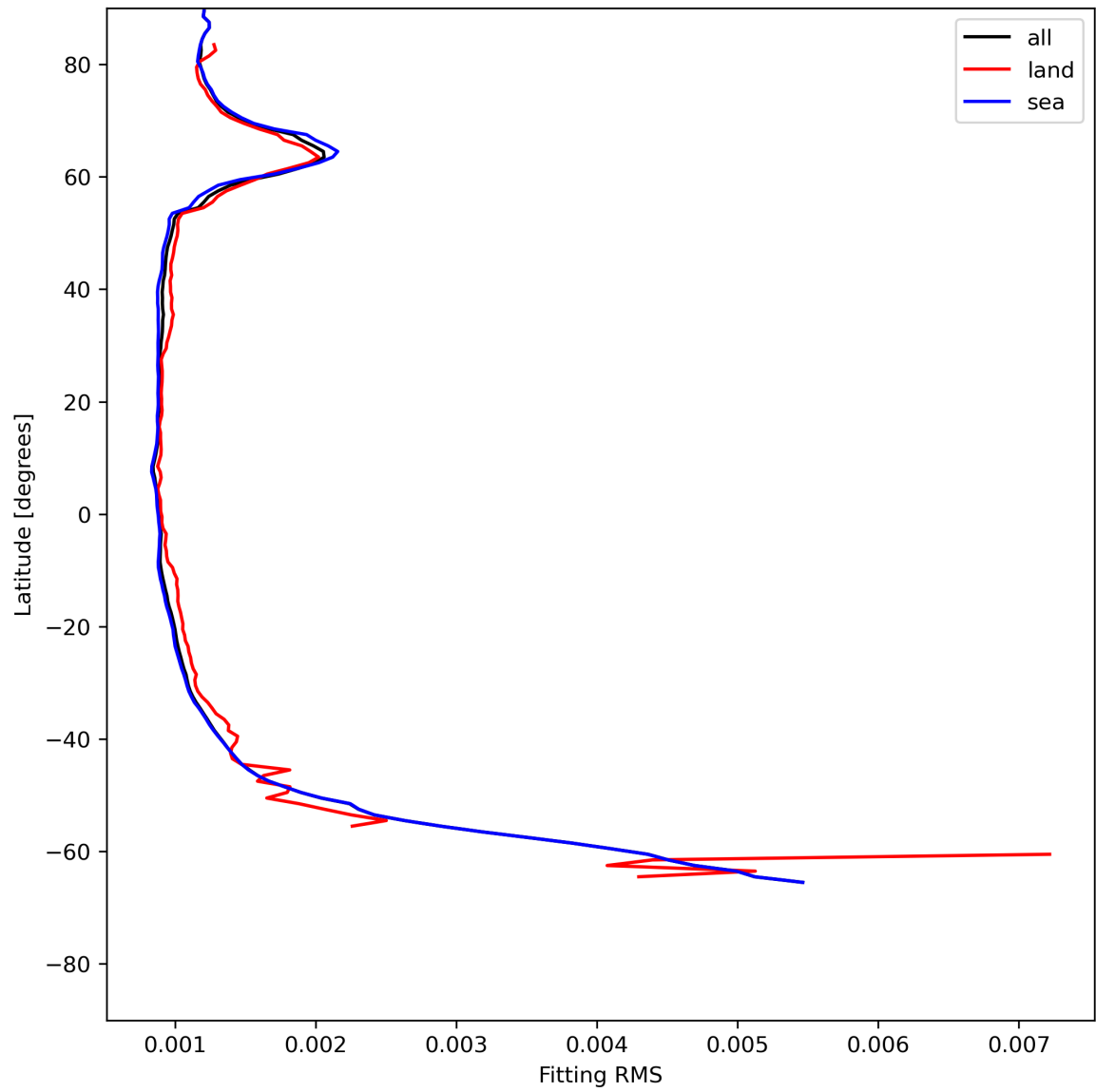
Figure 16: Zonal average of “Fitting RMS” for 2024-06-22 to 2024-06-24.
