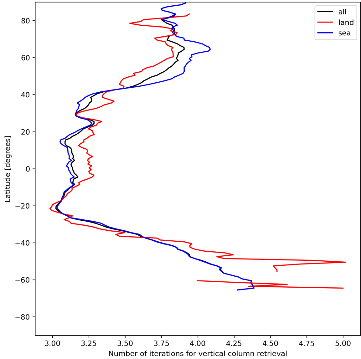
Figure 19: Zonal average of “Number of iterations for vertical column retrieval” for 2024-06-22 to 2024-06-24.
