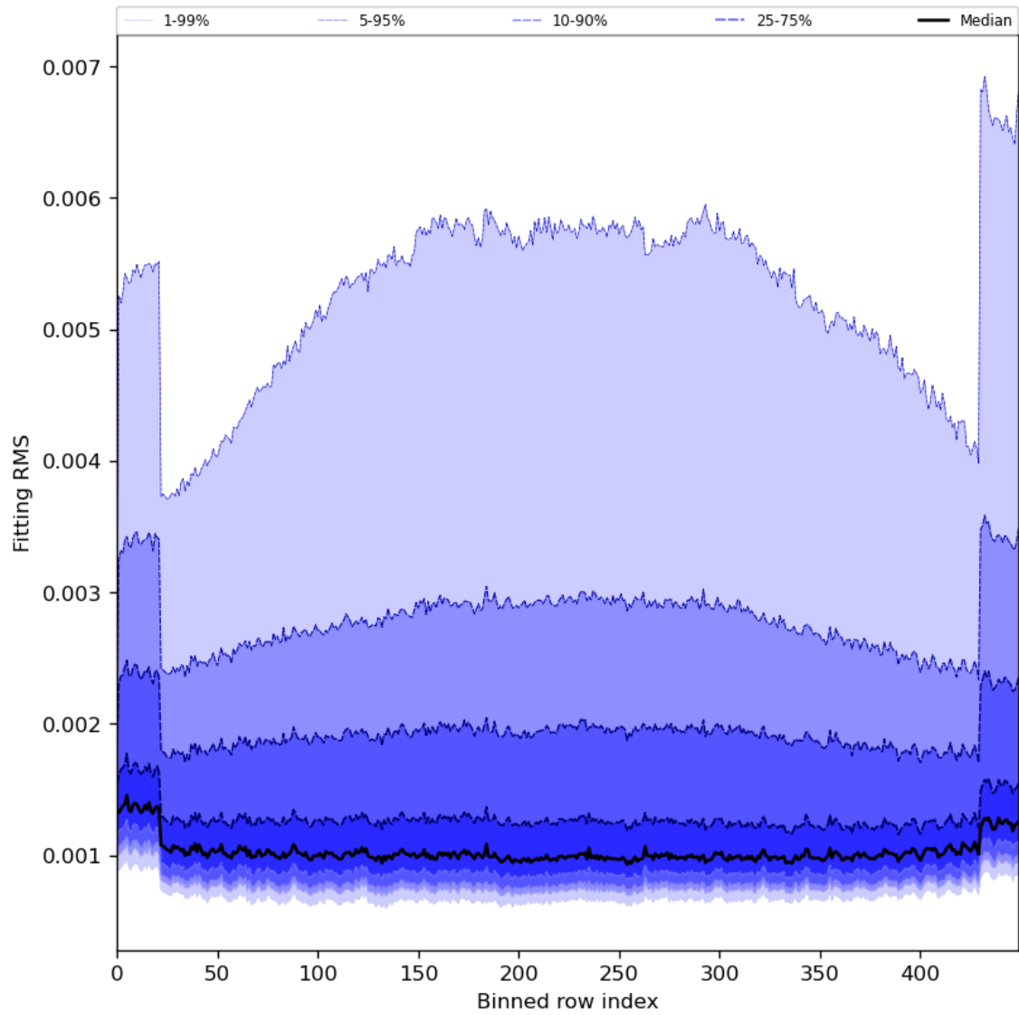
Figure 30: Along track statistics of “Fitting RMS” for 2024-06-22 to 2024-06-24
