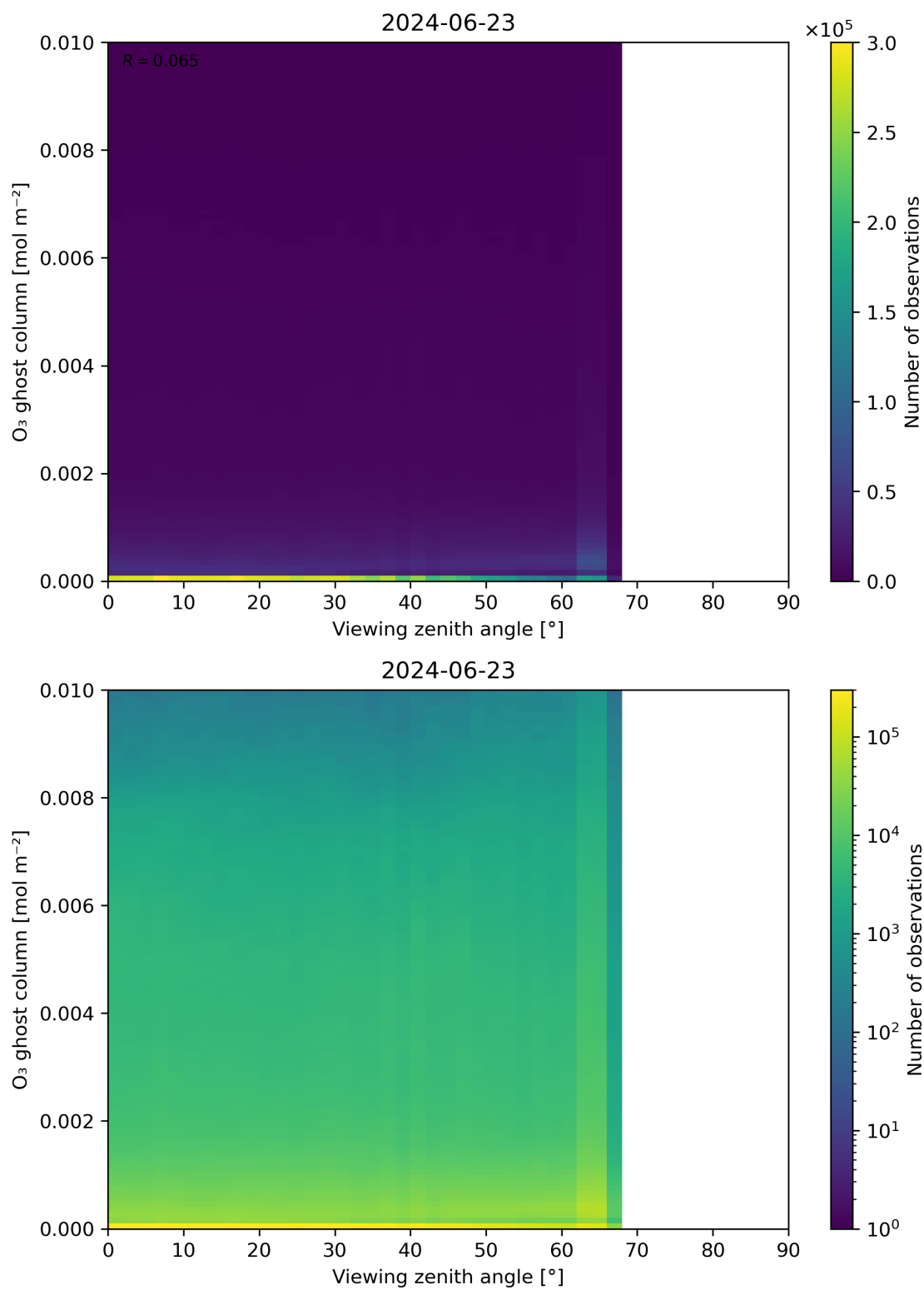
Figure 51: Scatter density plot of “Viewing zenith angle” against “O 3 ghost column” for 2024-06-22 to 2024-06-24.
