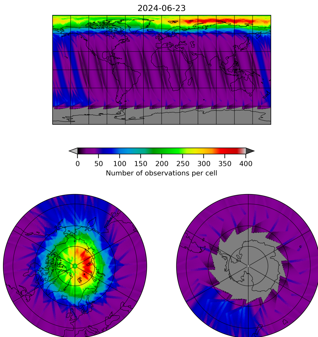
Figure 12: Map of the number of observations for 2024-06-22 to 2024-06-24
