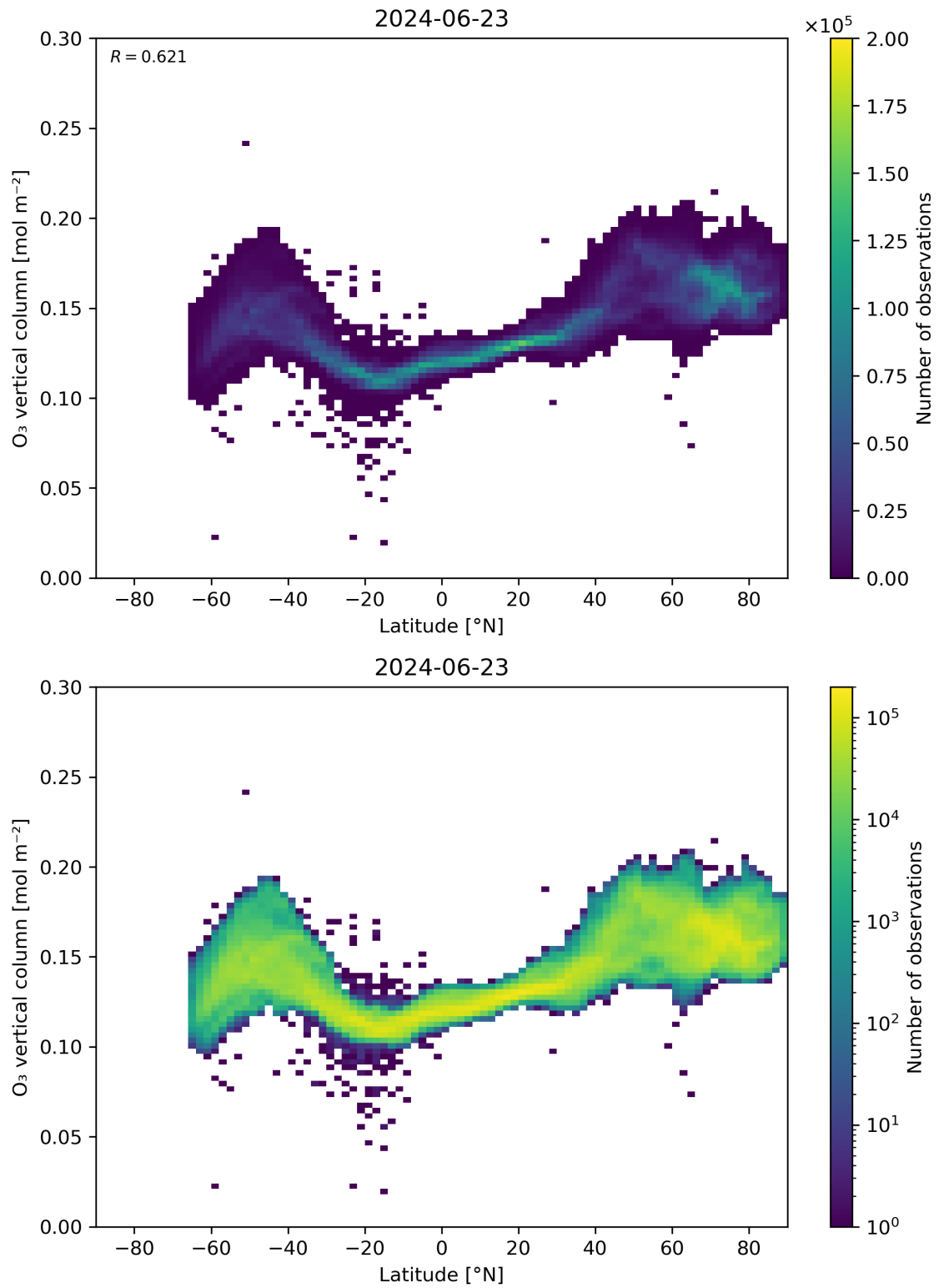
Figure 36: Scatter density plot of “Latitude” against “O 3 vertical column” for 2024-06-22 to 2024-06-24.
