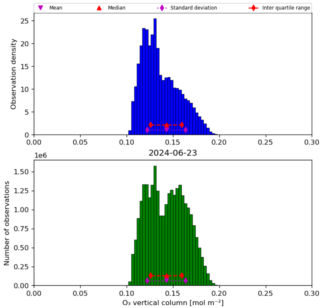
Figure 21: Histogram of “O 3 vertical column” for 2024-06-22 to 2024-06-24
