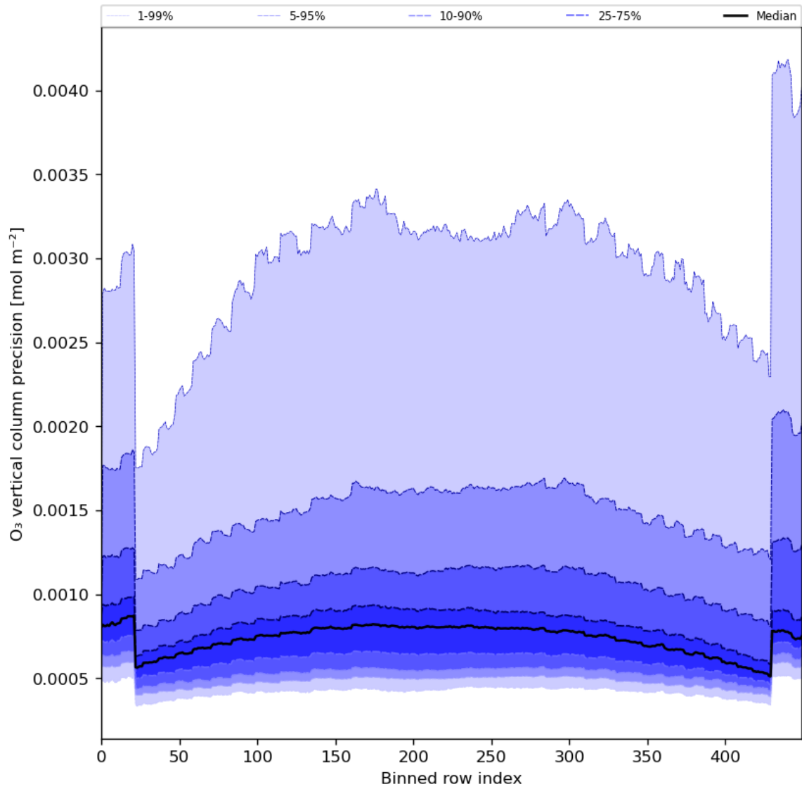
Figure 29: Along track statistics of “O 3 vertical column precision” for 2024-06-22 to 2024-06-24
