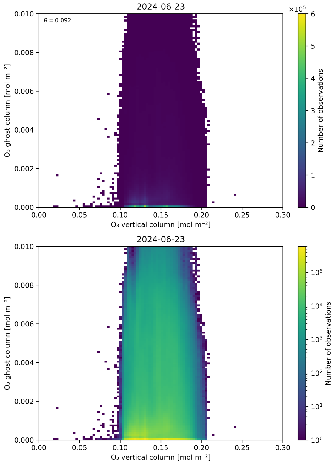
Figure 40: Scatter density plot of “O 3 vertical column” against “O 3 ghost column” for 2024-06-22 to 2024-06-24.
