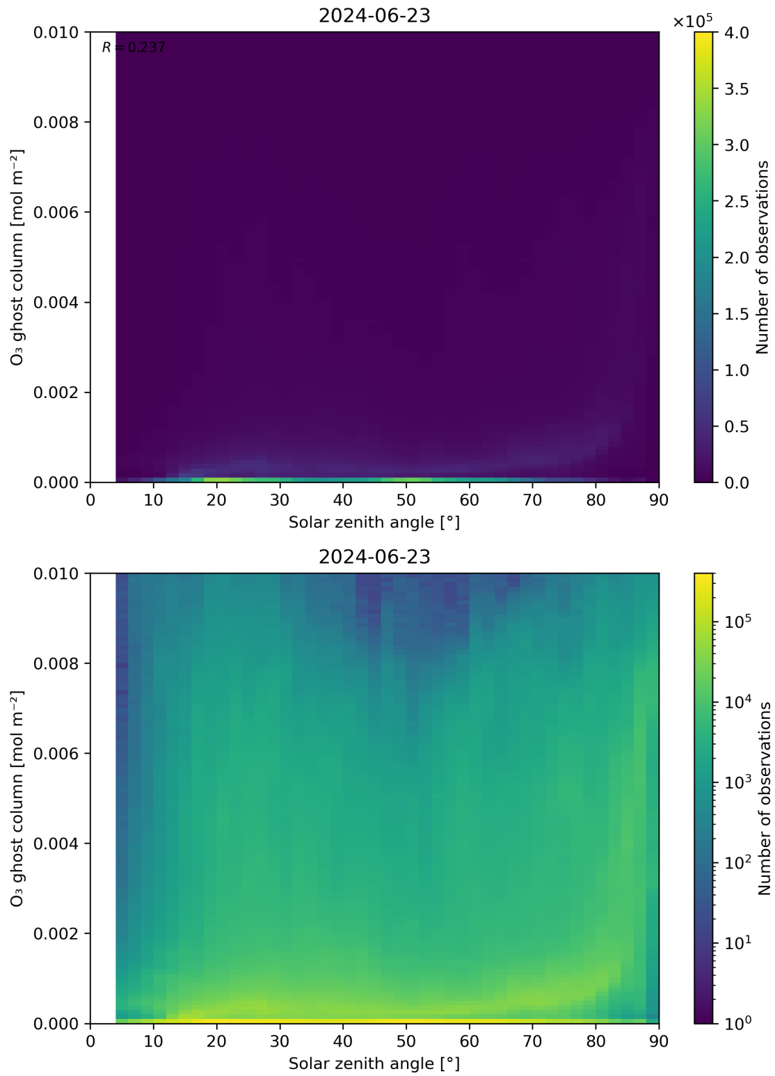
Figure 46: Scatter density plot of “Solar zenith angle” against “O 3 ghost column” for 2024-06-22 to 2024-06-24.
