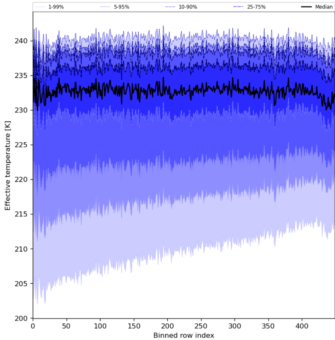
Figure 31: Along track statistics of “Effective temperature” for 2024-06-22 to 2024-06-24
