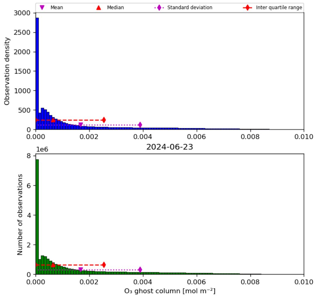
Figure 25: Histogram of “O 3 ghost column” for 2024-06-22 to 2024-06-24
