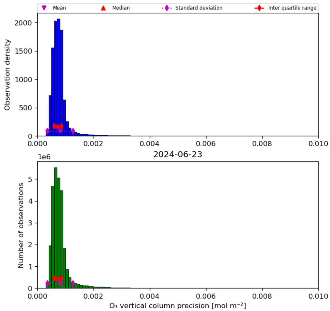
Figure 22: Histogram of “O 3 vertical column precision” for 2024-06-22 to 2024-06-24
