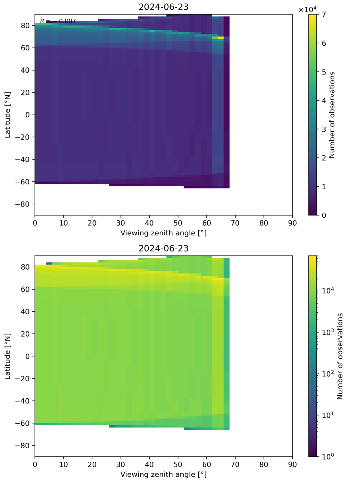
Figure 49: Scatter density plot of “Viewing zenith angle” against “Latitude” for 2024-06-22 to 2024-06-24.
