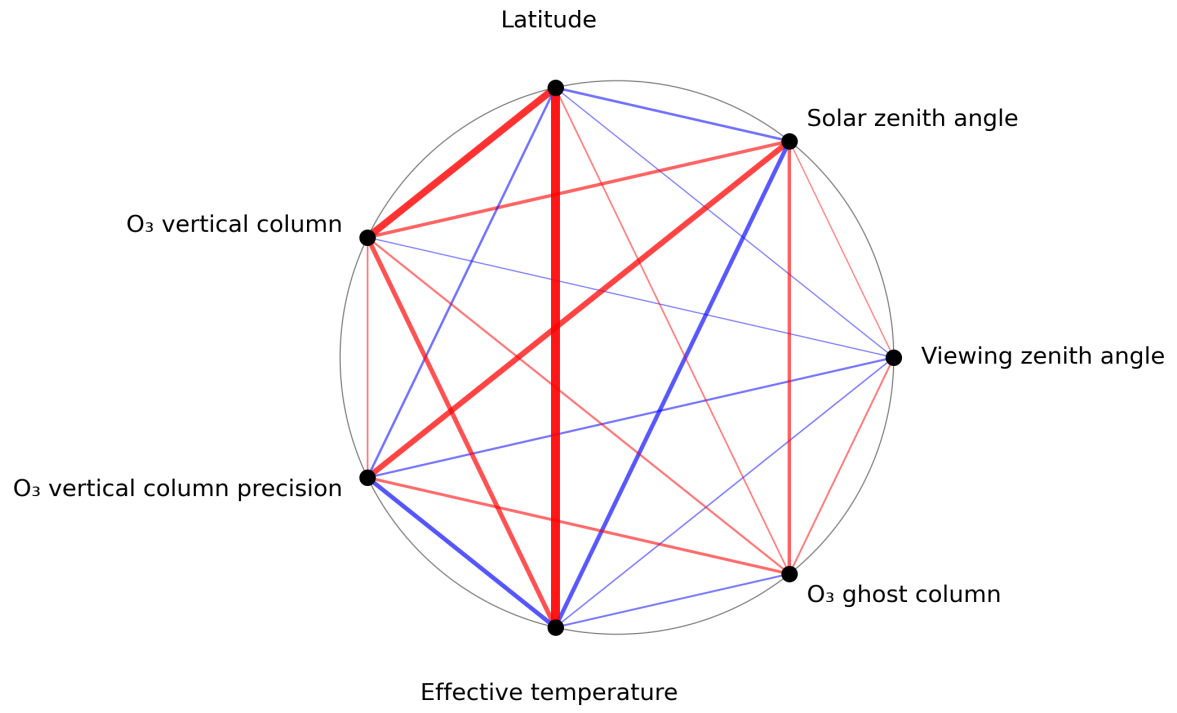
Figure 1: Map of correlation graph for 2024-06-22 to 2024-06-24.
