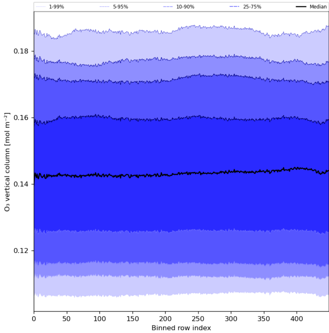
Figure 28: Along track statistics of “O 3 vertical column” for 2024-06-22 to 2024-06-24
