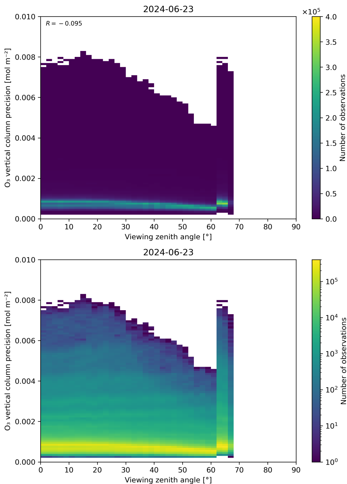
Figure 53: Scatter density plot of “Viewing zenith angle” against “O 3 vertical column precision” for 2024-06-22 to 2024-06-24.
