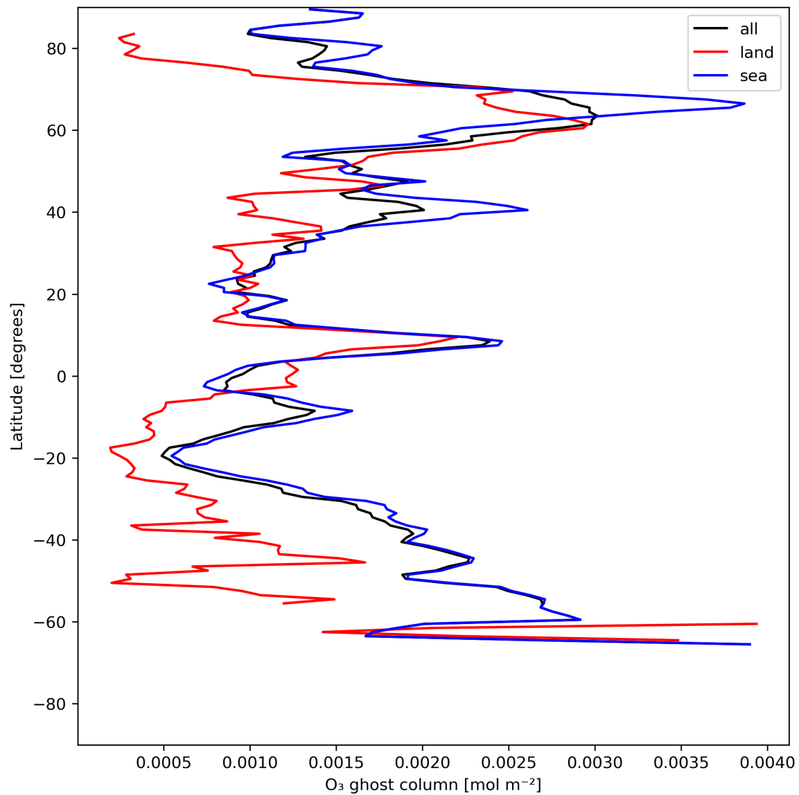
Figure 18: Zonal average of "O 3 ghost column" for 2024-06-22 to 2024-06-24.
