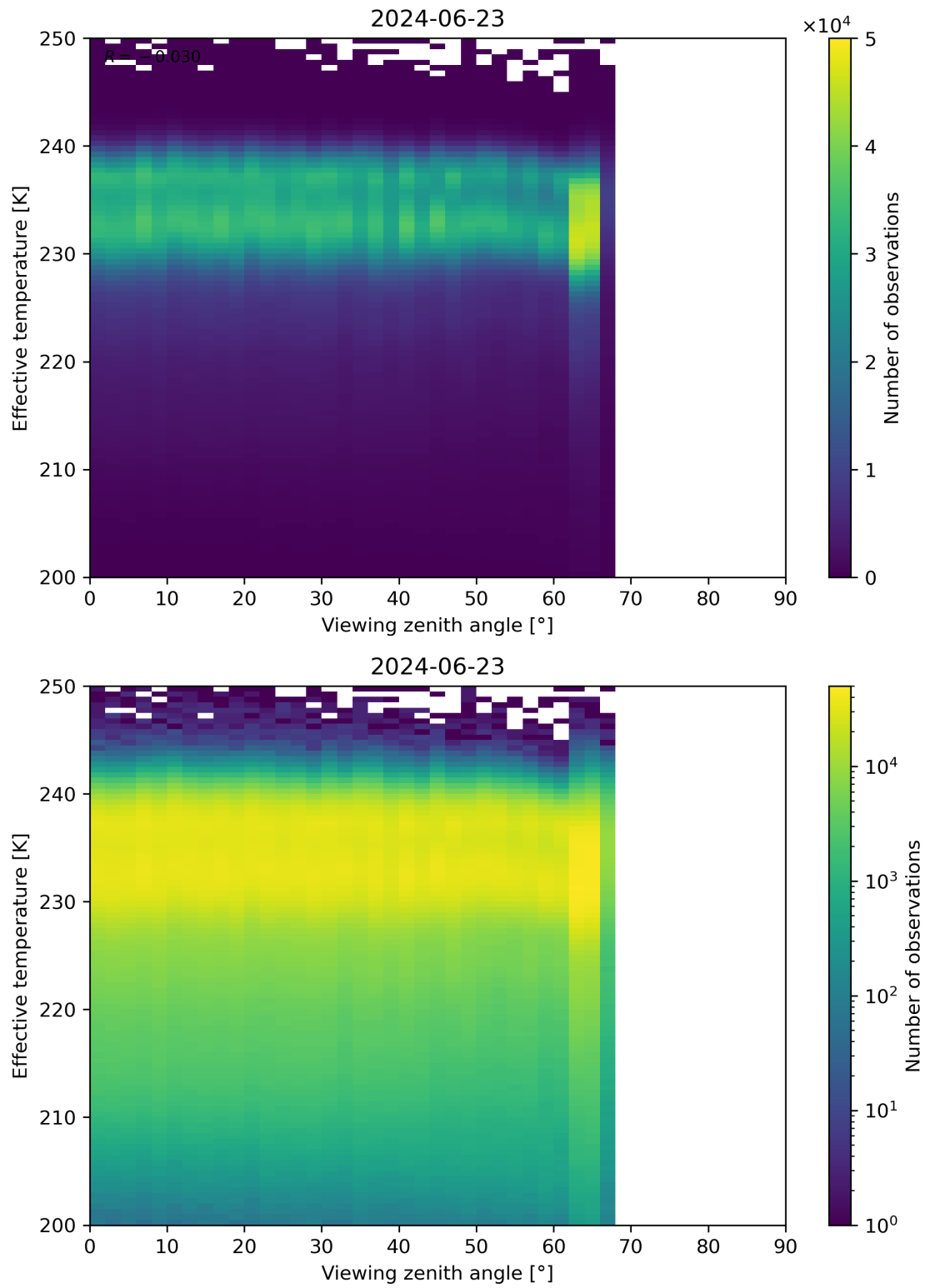
Figure 50: Scatter density plot of “Viewing zenith angle” against “Effective temperature” for 2024-06-22 to 2024-06-24.
