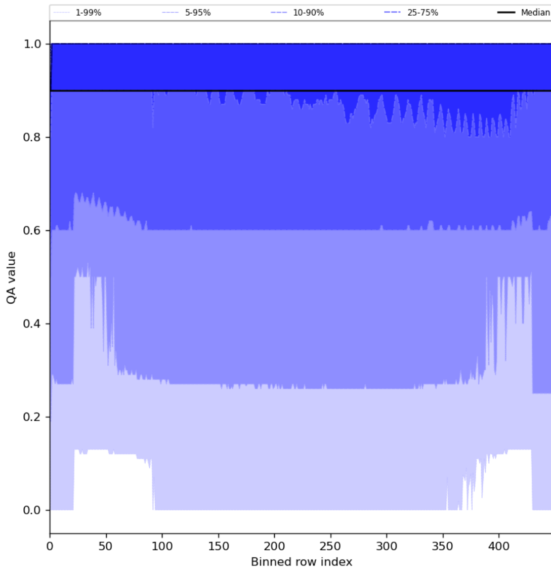
Figure 27: Along track statistics of “QA value” for 2024-06-22 to 2024-06-24
