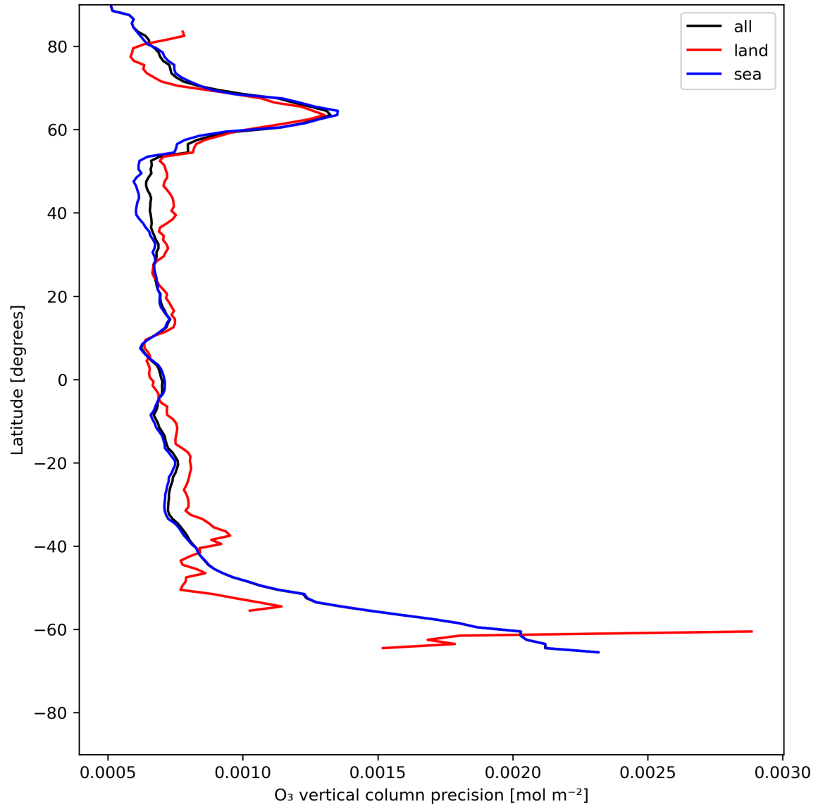
Figure 15: Zonal average of “O 3 vertical column precision” for 2024-06-22 to 2024-06-24.
