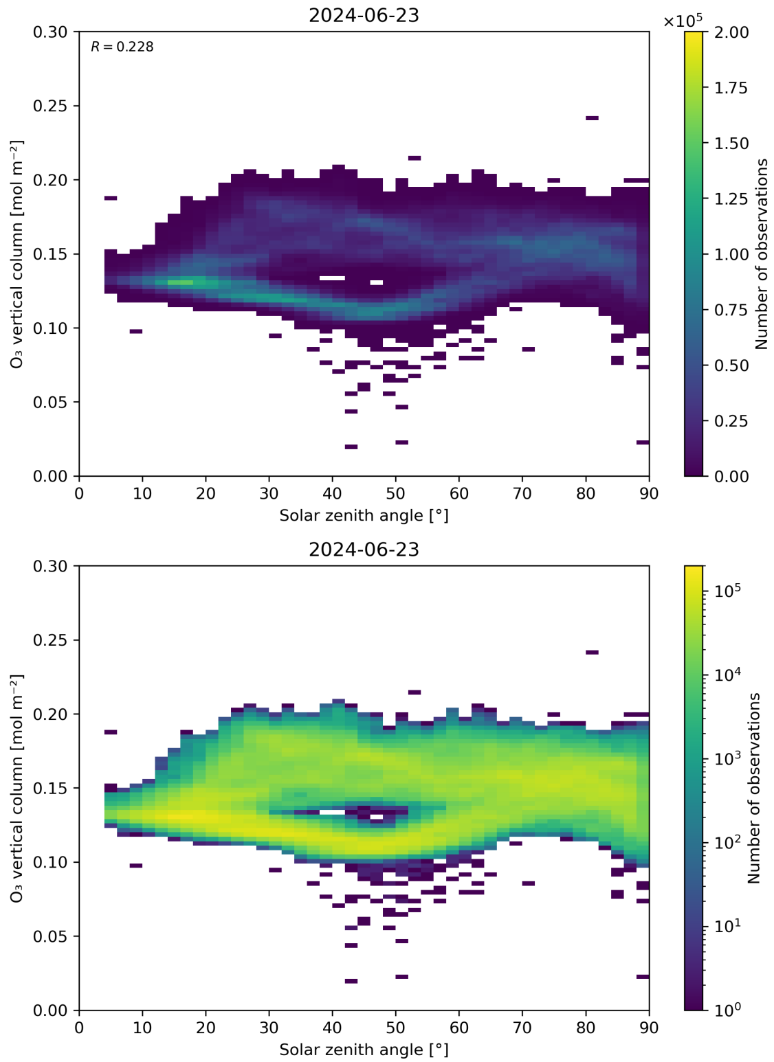
Figure 47: Scatter density plot of “Solar zenith angle” against “O 3 vertical column” for 2024-06-22 to 2024-06-24.
