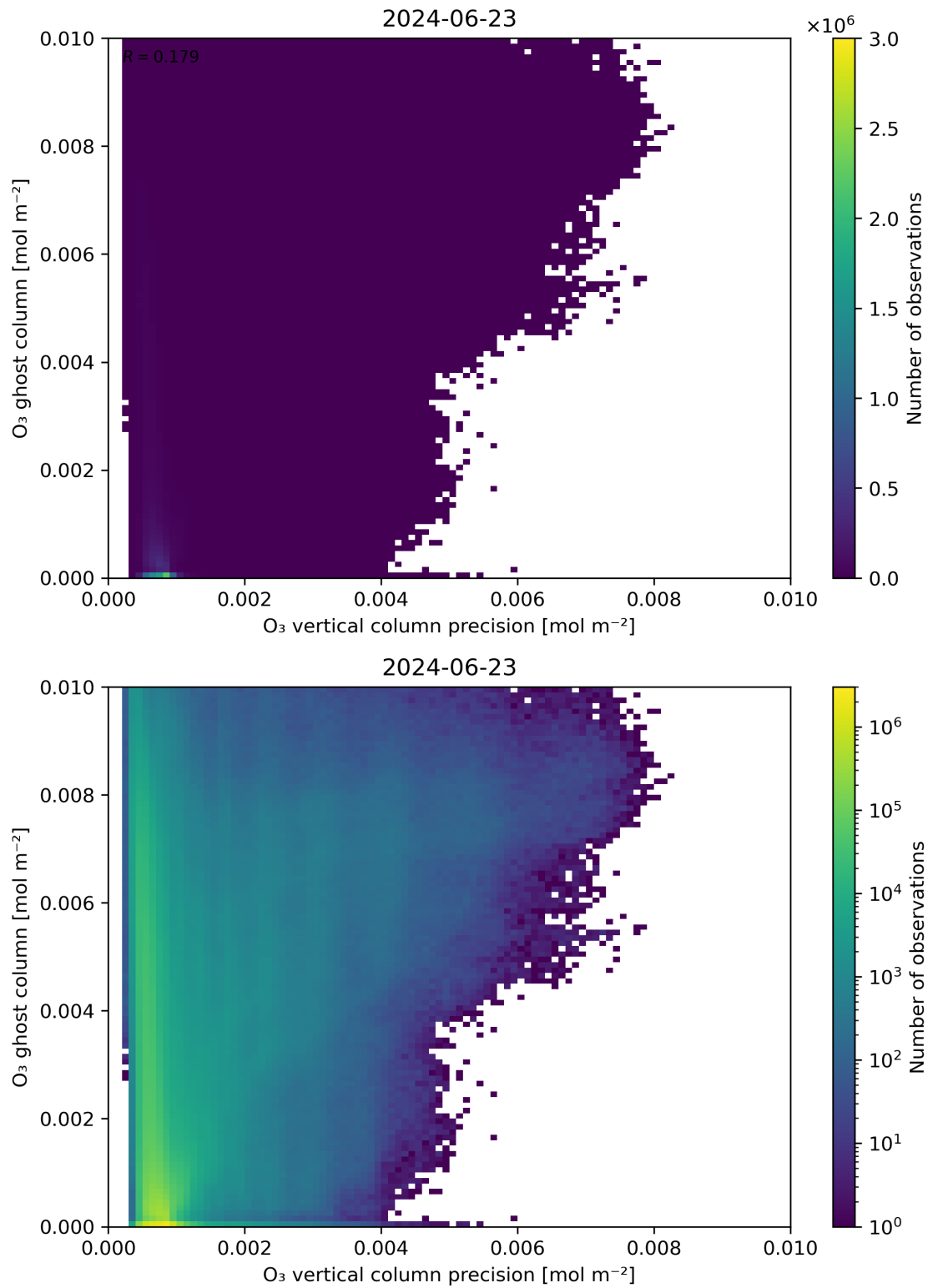
Figure 43: Scatter density plot of “ \text{O}_3 vertical column precision” against “ \text{O}_3 ghost column” for 2024-06-22 to 2024-06-24.
