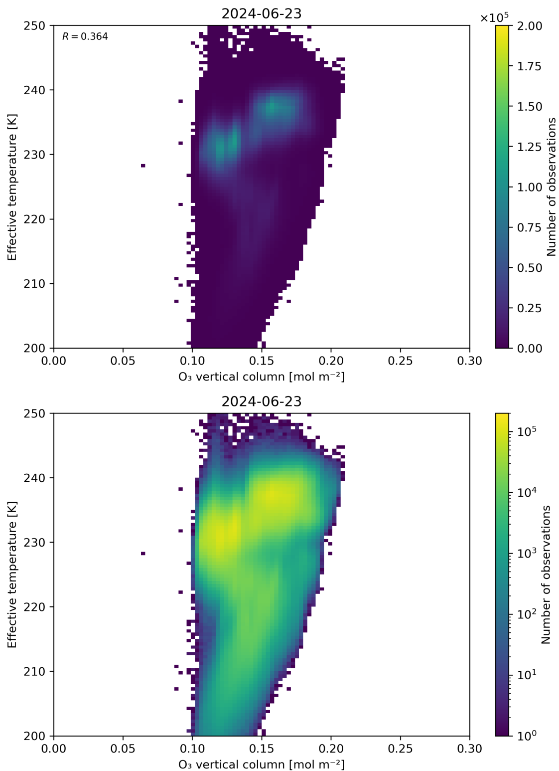
Figure 39: Scatter density plot of “O 3 vertical column” against “Effective temperature” for 2024-06-22 to 2024-06-24.
