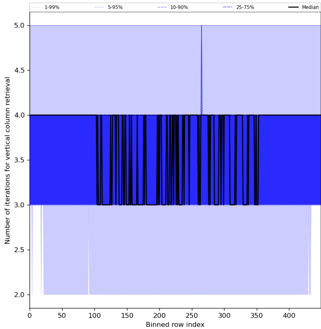
Figure 33: Along track statistics of “Number of iterations for vertical column retrieval” for 2024-06-22 to 2024-06-24
